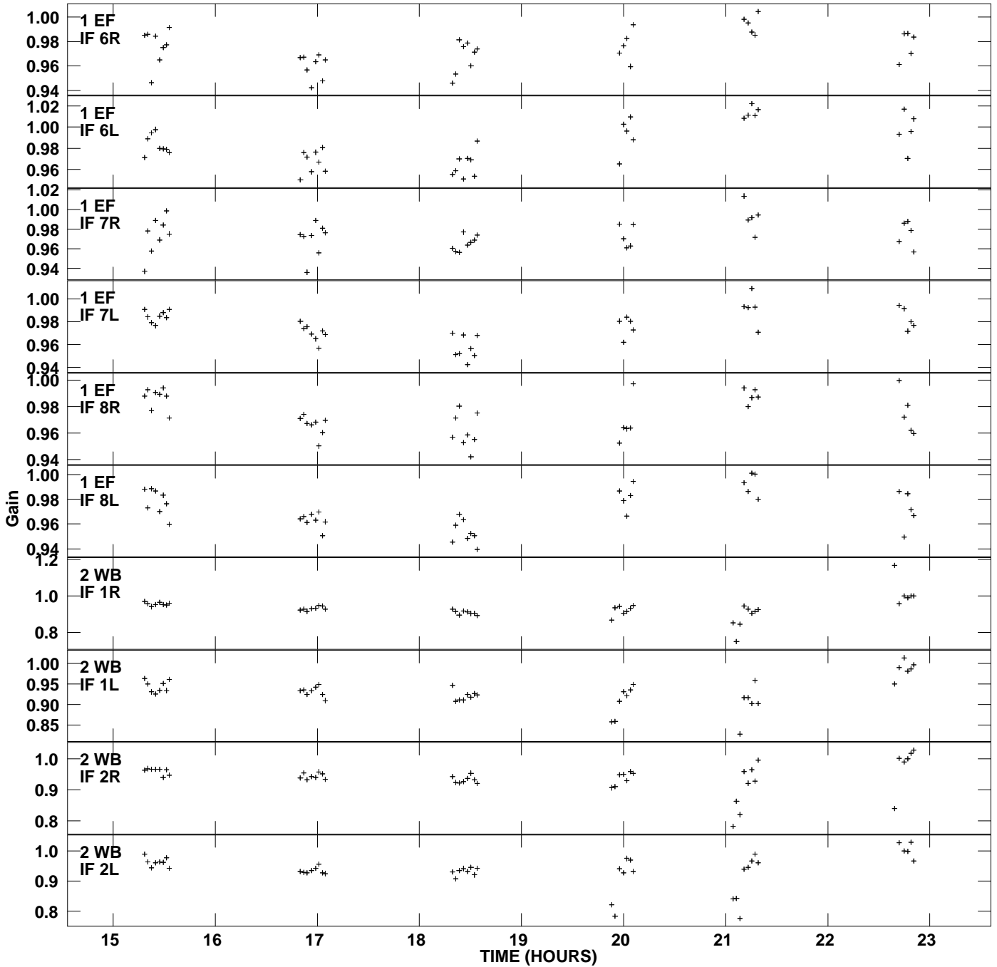
Plot file version 2 created 22-MAR-2012 00:08:23 Gain amp vs UTC time for J0038+2303.MULTI.1 SN 2 Rpol & Lpol IF 1 - 8
