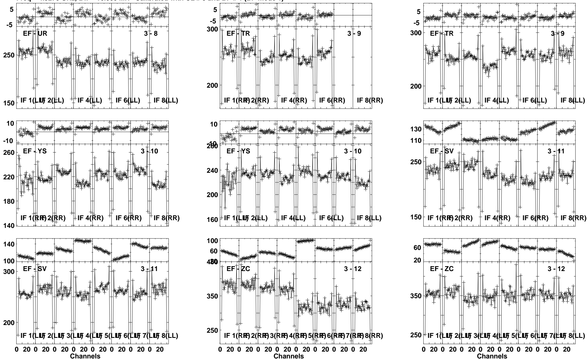
Lower frame: Milli Ampl Jy Top frame: Phas deg Vector averaged cross-power spectrum Several baselines displayed Timerange: 00/10:54:31 to 00/10:59:29
