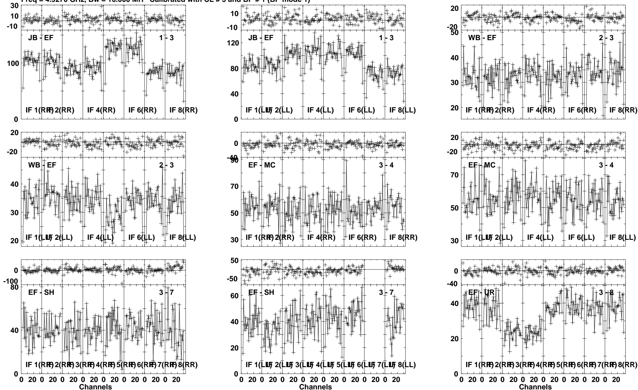
Lower frame: Milli Ampl Jy Top frame: Phas deg Vector averaged cross-power spectrum Several baselines displayed Timerange: 00/10:48:01 to 00/10:53:29
