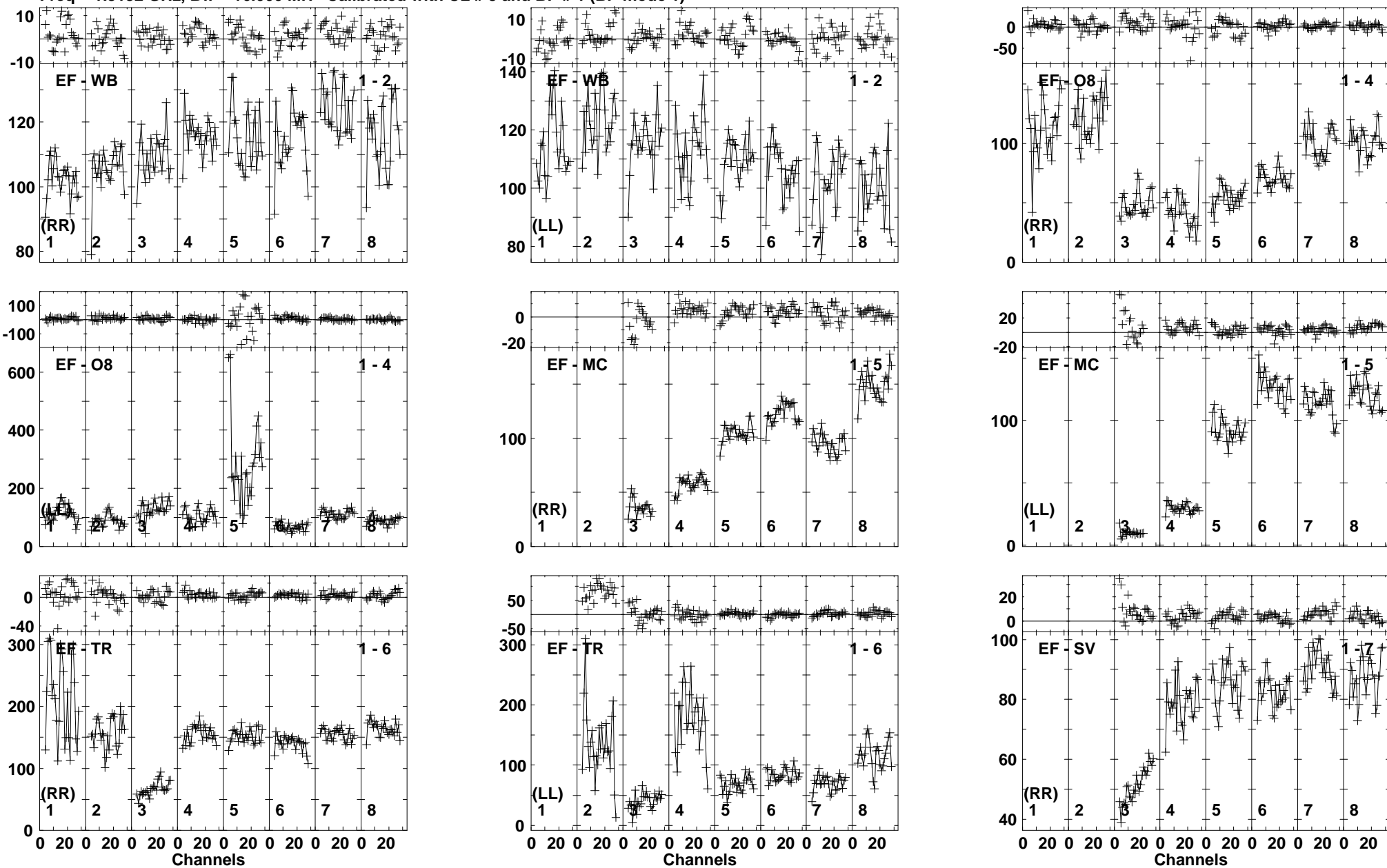
Lower frame: Milli Ampl Jy Top frame: Phas deg Vector averaged cross-power spectrum Baseline: EF (01) - WB (02) Timerange: 00/18:19:33 to 00/18:22:29
