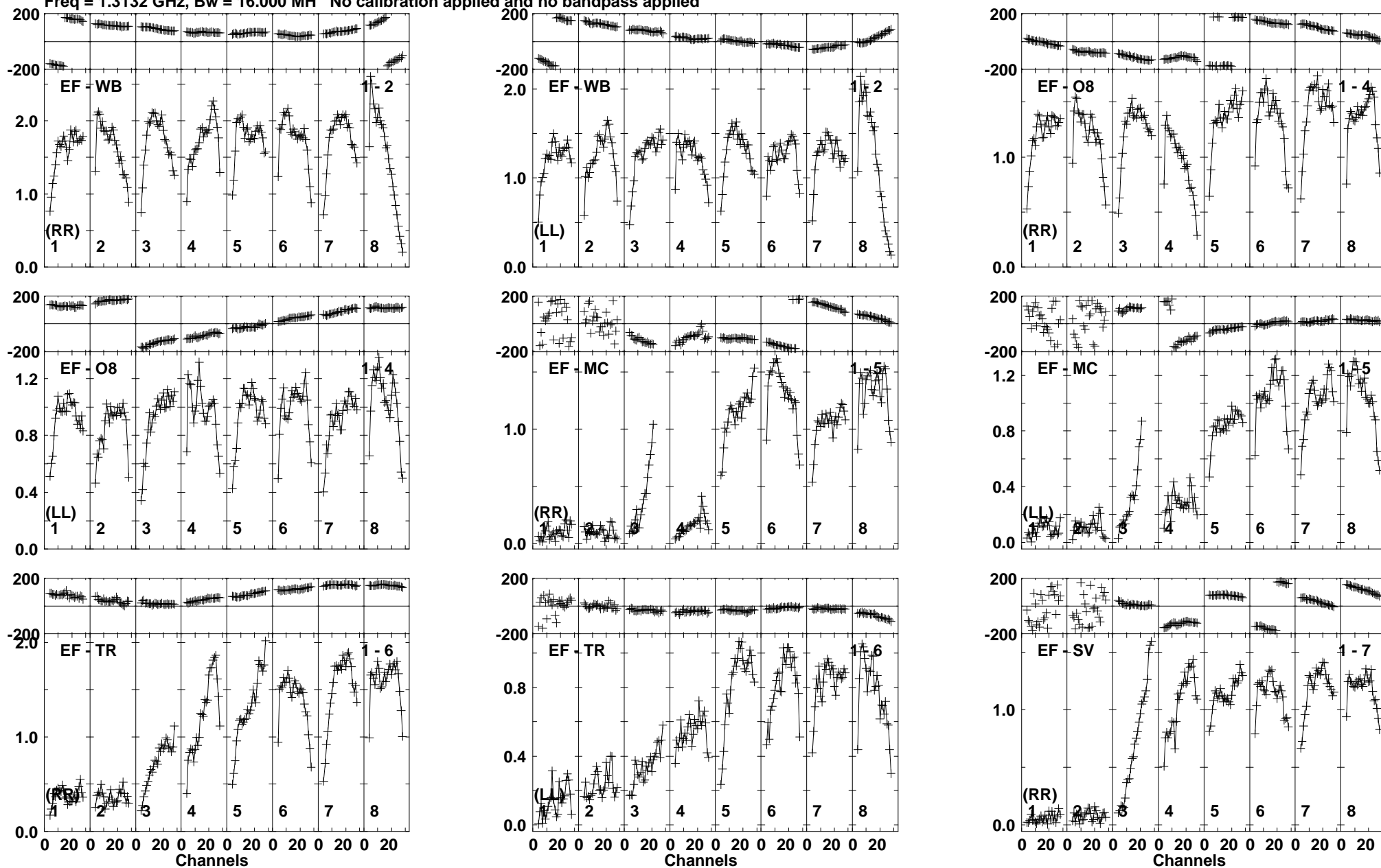
Lower frame: Milli Ampl Jy Top frame: Phas deg Vector averaged cross-power spectrum Baseline: EF (01) - WB (02) Timerange: 00/21:47:33 to 00/21:50:29
