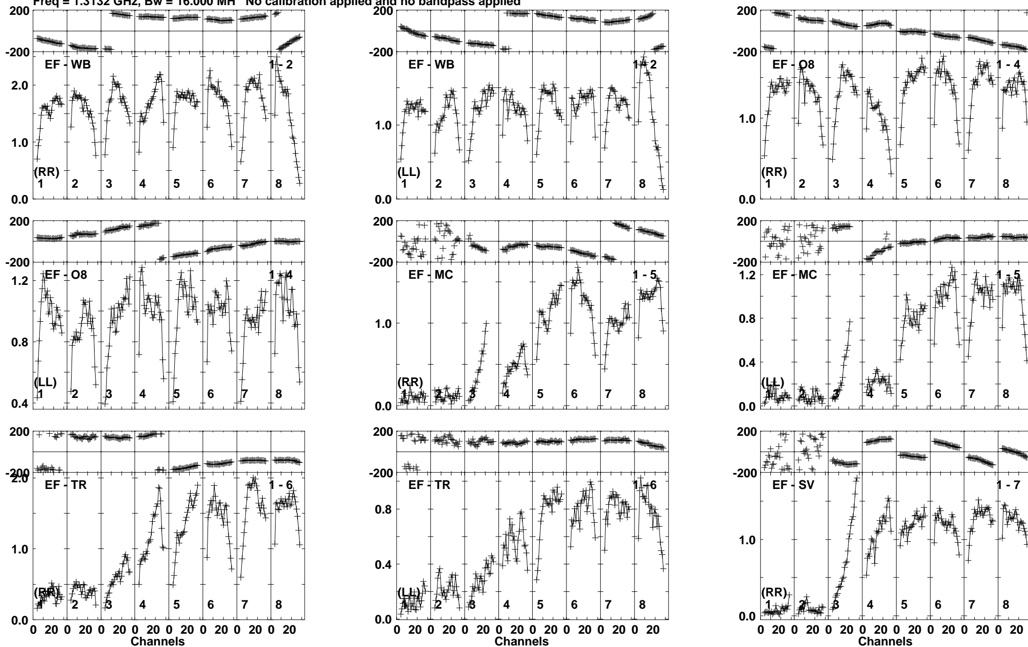
Lower frame: Milli Ampl Jy Top frame: Phas deg Vector averaged cross-power spectrum Baseline: EF (01) - WB (02) Timerange: 01/00:35:33 to 01/00:38:29
