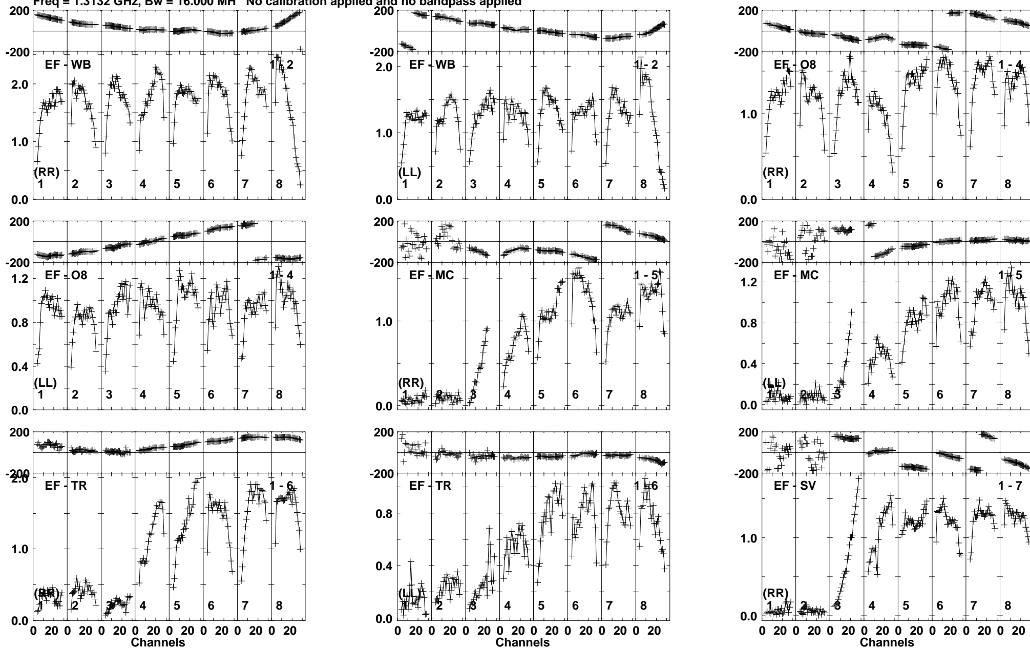
Lower frame: Milli Ampl Jy Top frame: Phas deg Vector averaged cross-power spectrum Baseline: EF (01) - WB (02) Timerange: 00/23:22:03 to 00/23:24:59
