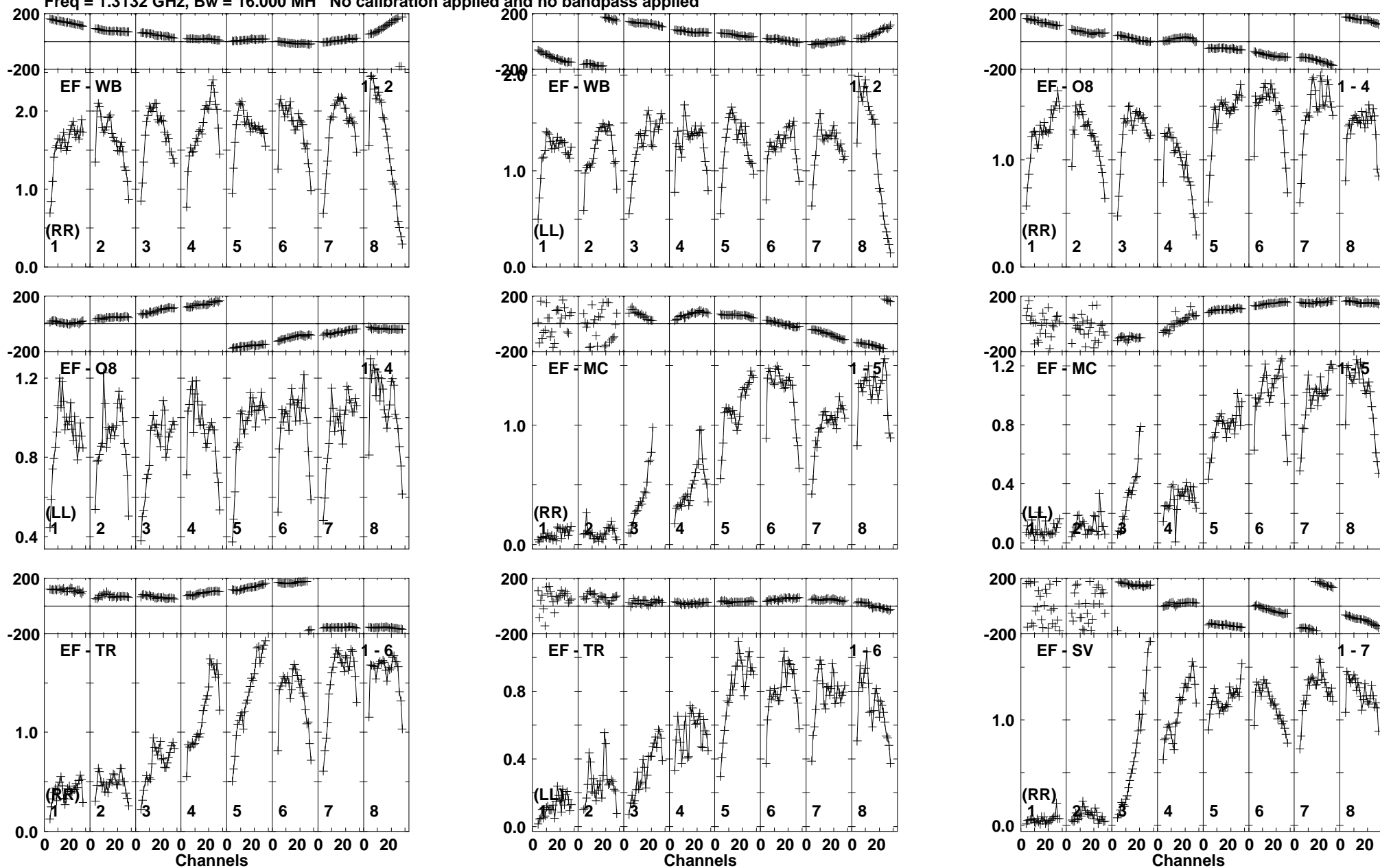
Lower frame: Milli Ampl Jy Top frame: Phas deg Vector averaged cross-power spectrum Baseline: EF (01) - WB (02) Timerange: 01/01:14:13 to 01/01:17:09
