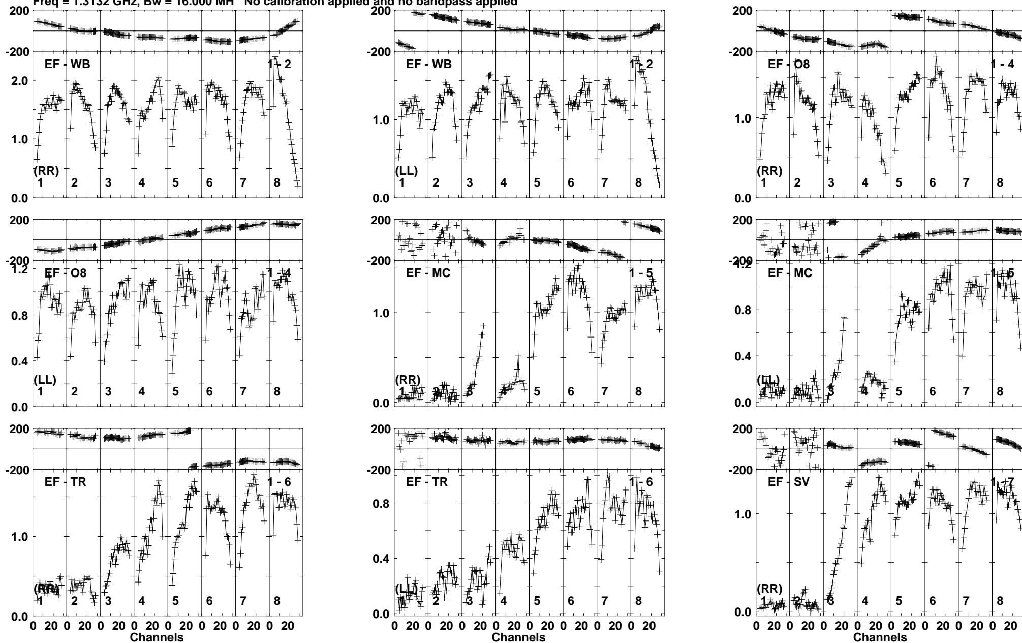
Lower frame: Milli Ampl Jy Top frame: Phas deg Vector averaged cross-power spectrum Baseline: EF (01) - WB (02) Timerange: 01/02:48:43 to 01/02:51:39
