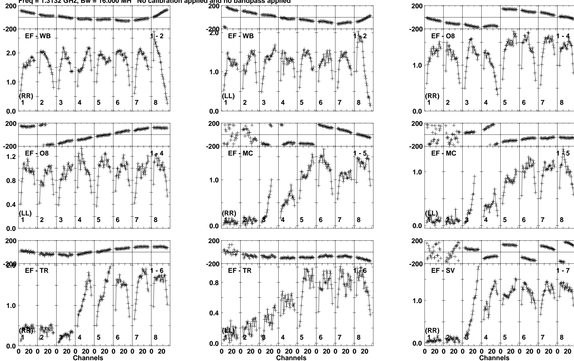
Lower frame: Milli Ampl Jy Top frame: Phas deg Vector averaged cross-power spectrum Baseline: EF (01) - WB (02) Timerange: 00/23:32:33 to 00/23:35:29
