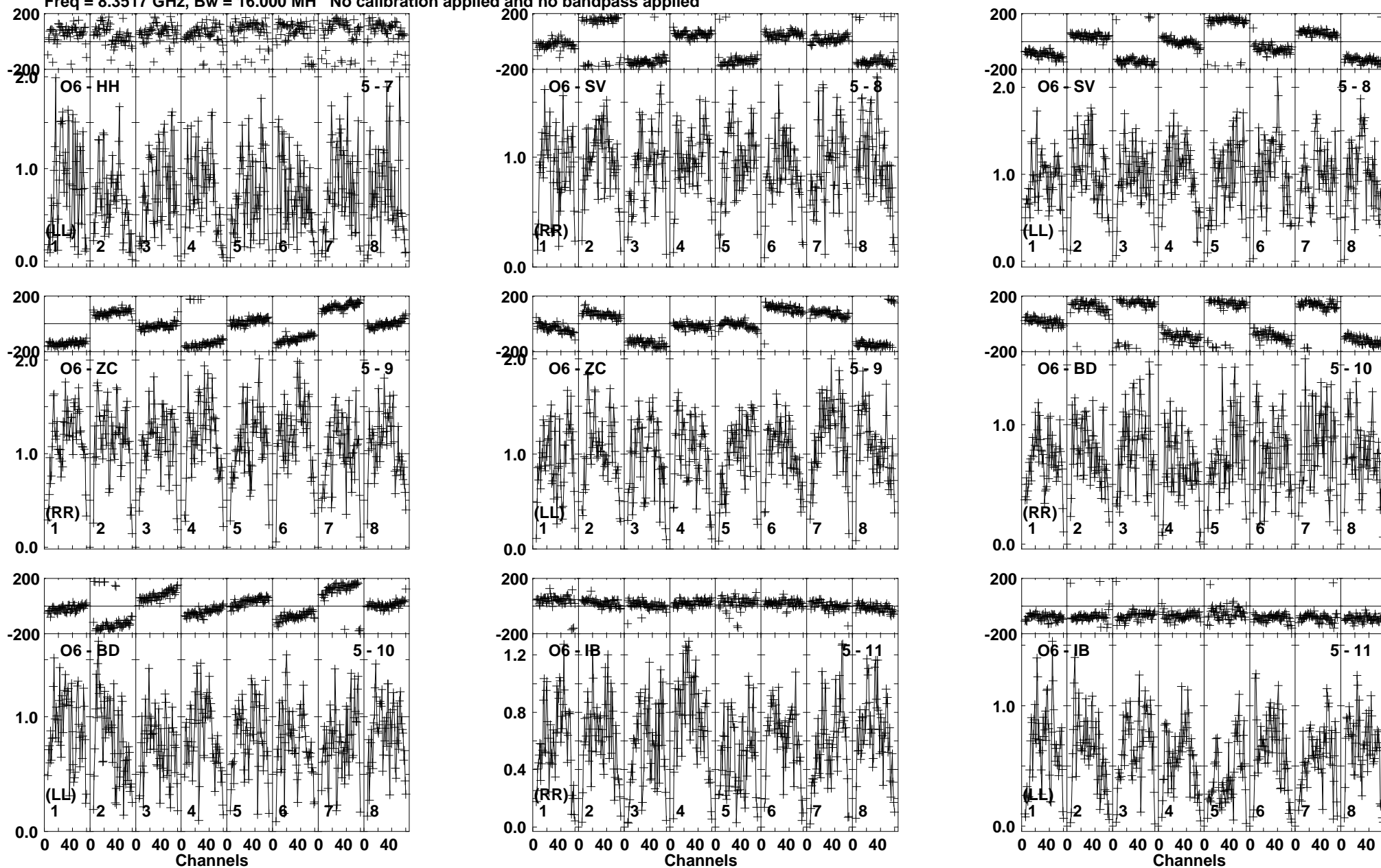
Lower frame: Milli Ampl Jy Top frame: Phas deg Vector averaged cross-power spectrum Baseline: O6 (05) - HH (07) Timerange: 00/02:11:46 to 00/02:12:29
