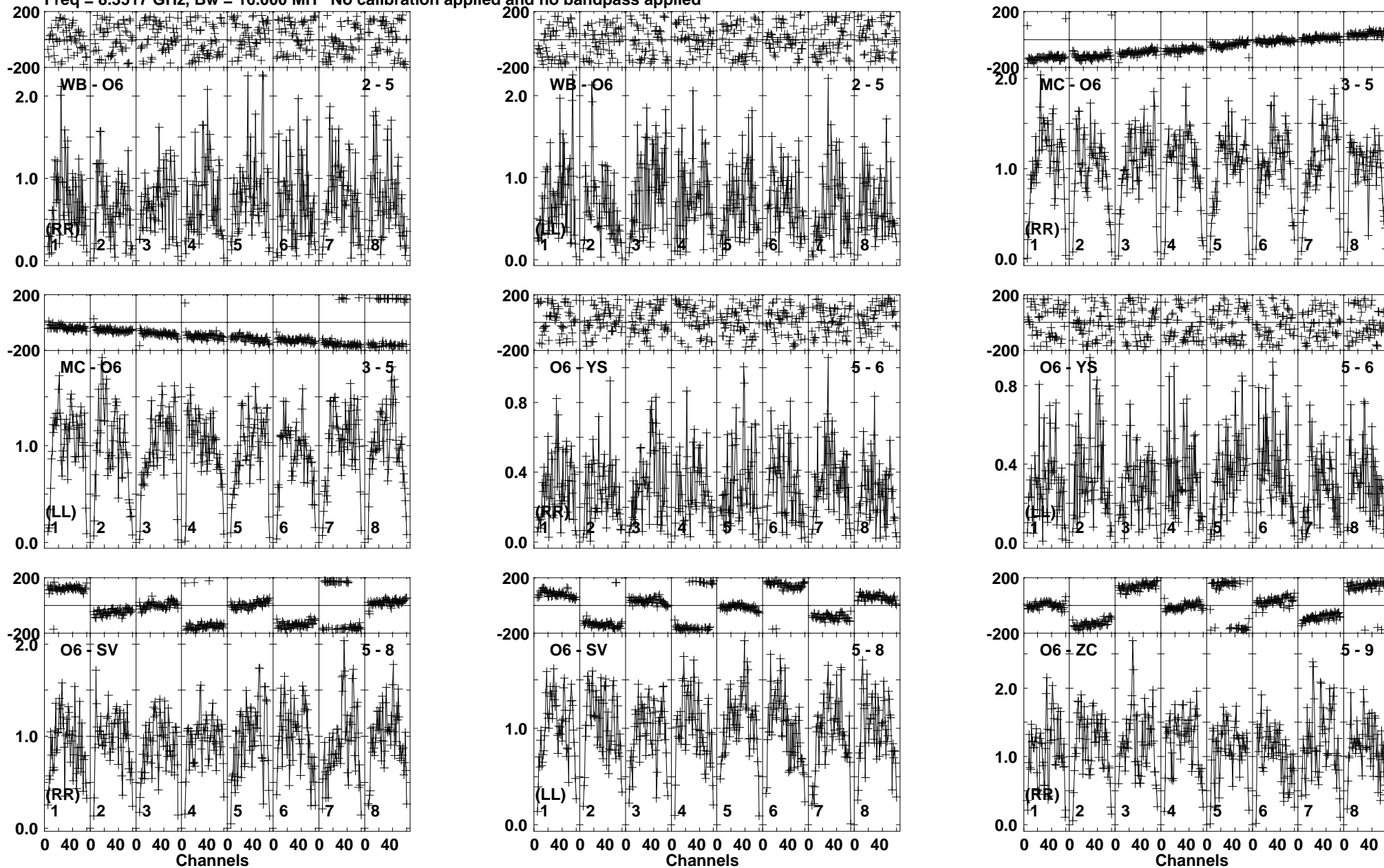
Lower frame: Milli Ampl Jy Top frame: Phas deg Vector averaged cross-power spectrum Baseline: WB (02) - O6 (05) Timerange: 00/05:45:20 to 00/05:46:05
