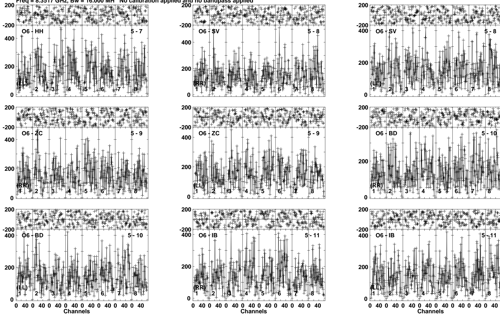
Lower frame: Micro Ampl Jy Top frame: Phas deg Vector averaged cross-power spectrum Baseline: O6 (05) - HH (07) Timerange: 00/03:52:56 to 00/03:55:09
