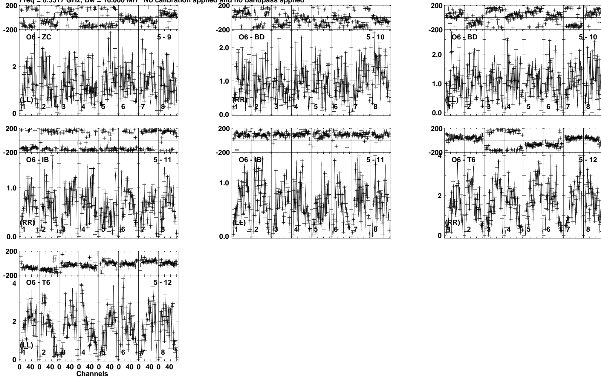
Lower frame: Milli Ampl Jy Top frame: Phas deg Vector averaged cross-power spectrum Baseline: O6 (05) - ZC (09) Timerange: 00:02:29:07 to 00:02:29:34
