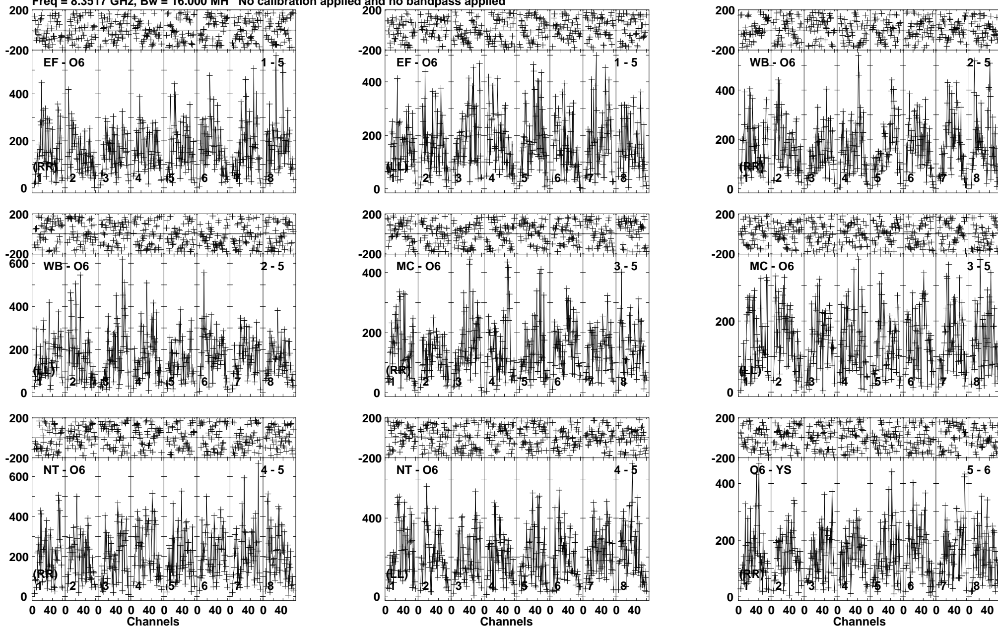
Lower frame: Micro Ampl Jy Top frame: Phas deg Vector averaged cross-power spectrum Baseline: EF (01) - O6 (05) Timerange: 00/06:20:16 to 00/06:22:30
