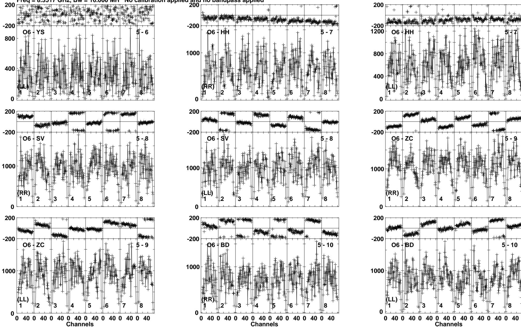
Lower frame: Micro Ampl Jy Top frame: Phas deg Vector averaged cross-power spectrum Baseline: O6 (05) - YS (06) Timerange: 00/03:15:41 to 00/03:16:09
