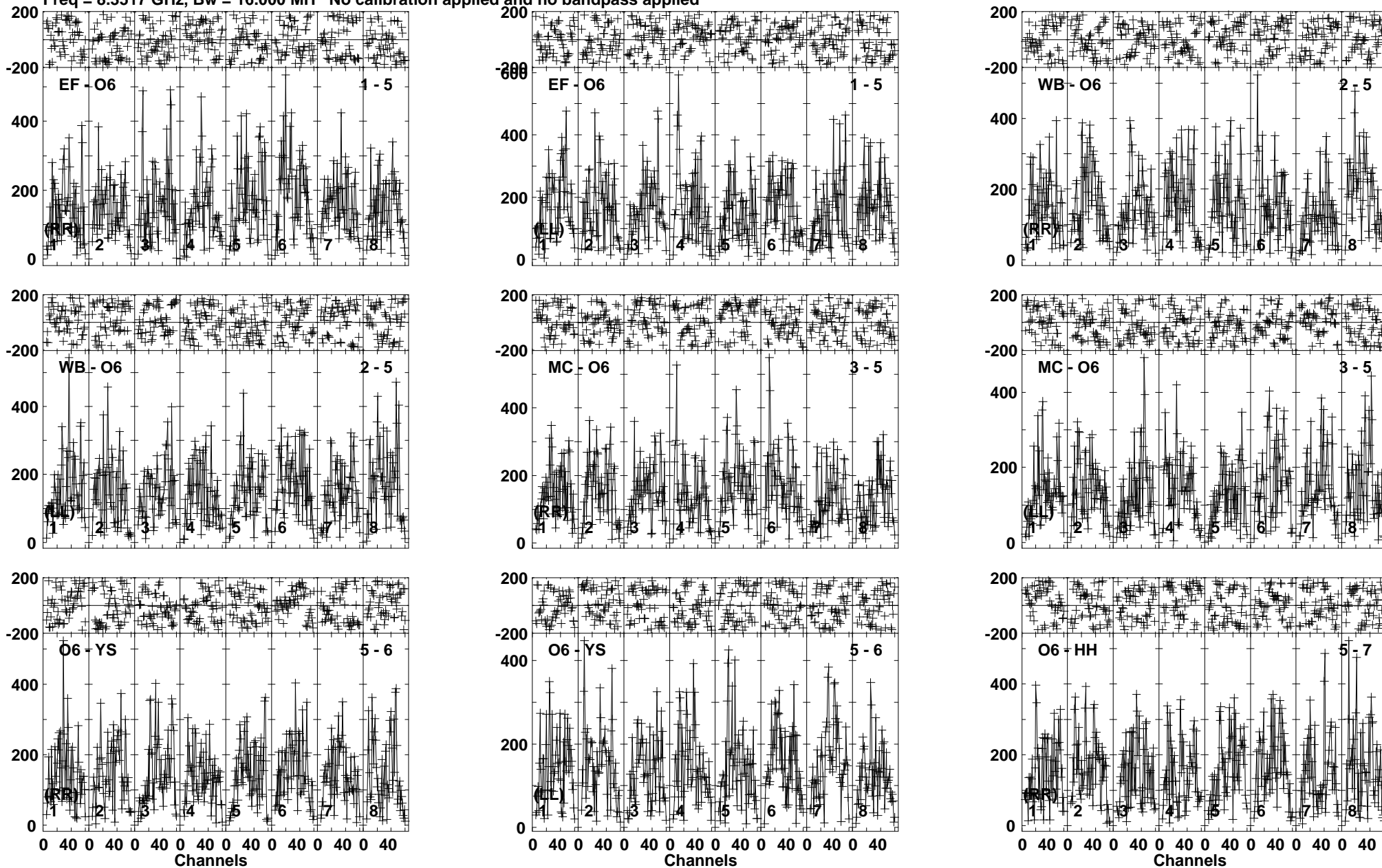
Lower frame: Micro Ampl Jy Top frame: Phas deg Vector averaged cross-power spectrum Baseline: EF (01) - O6 (05) Timerange: 00/08:51:46 to 00/08:54:00
