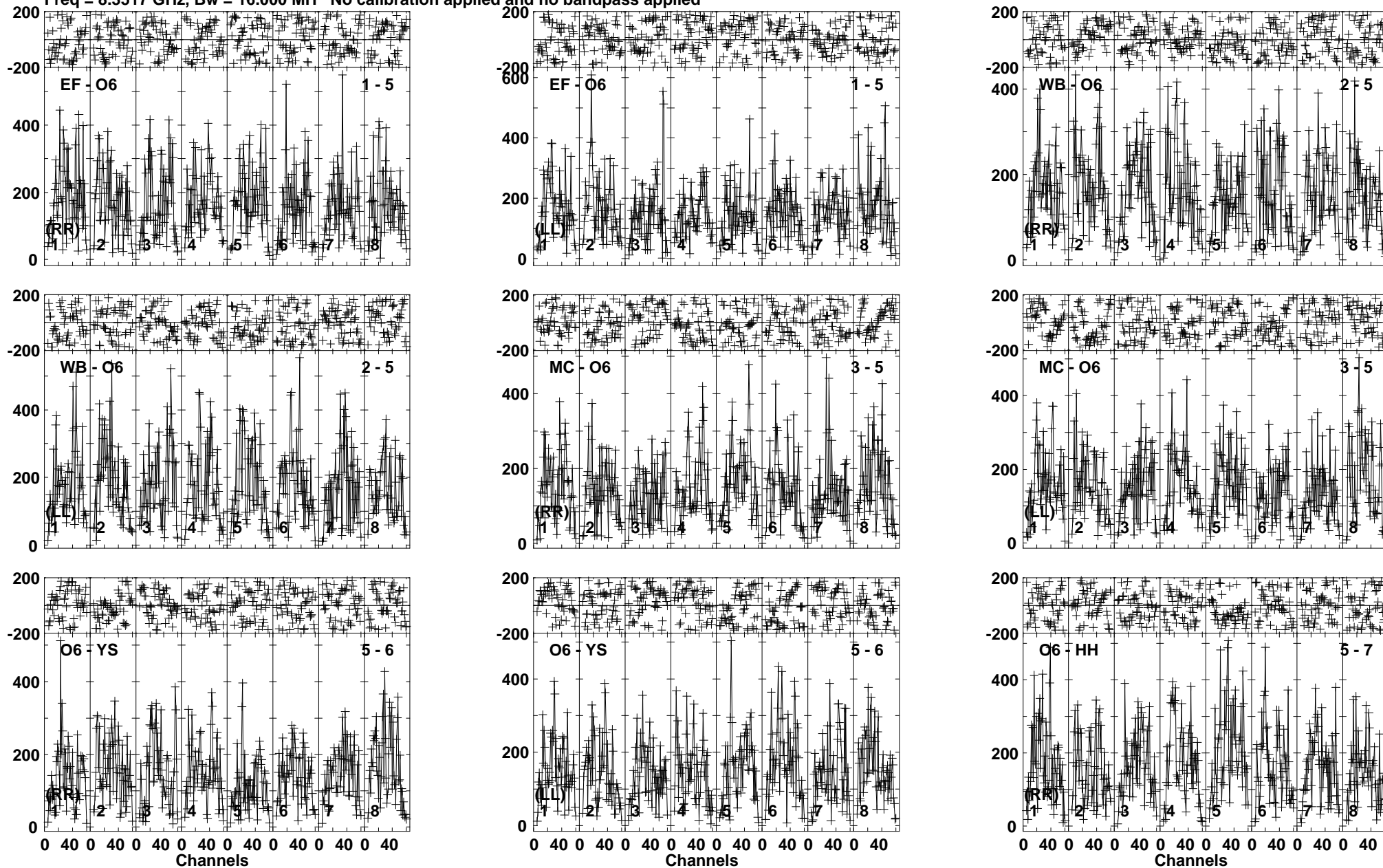
Lower frame: Micro Ampl Jy Top frame: Phas deg Vector averaged cross-power spectrum Baseline: EF (01) - O6 (05) Timerange: 00/06:51:16 to 00/06:53:29
