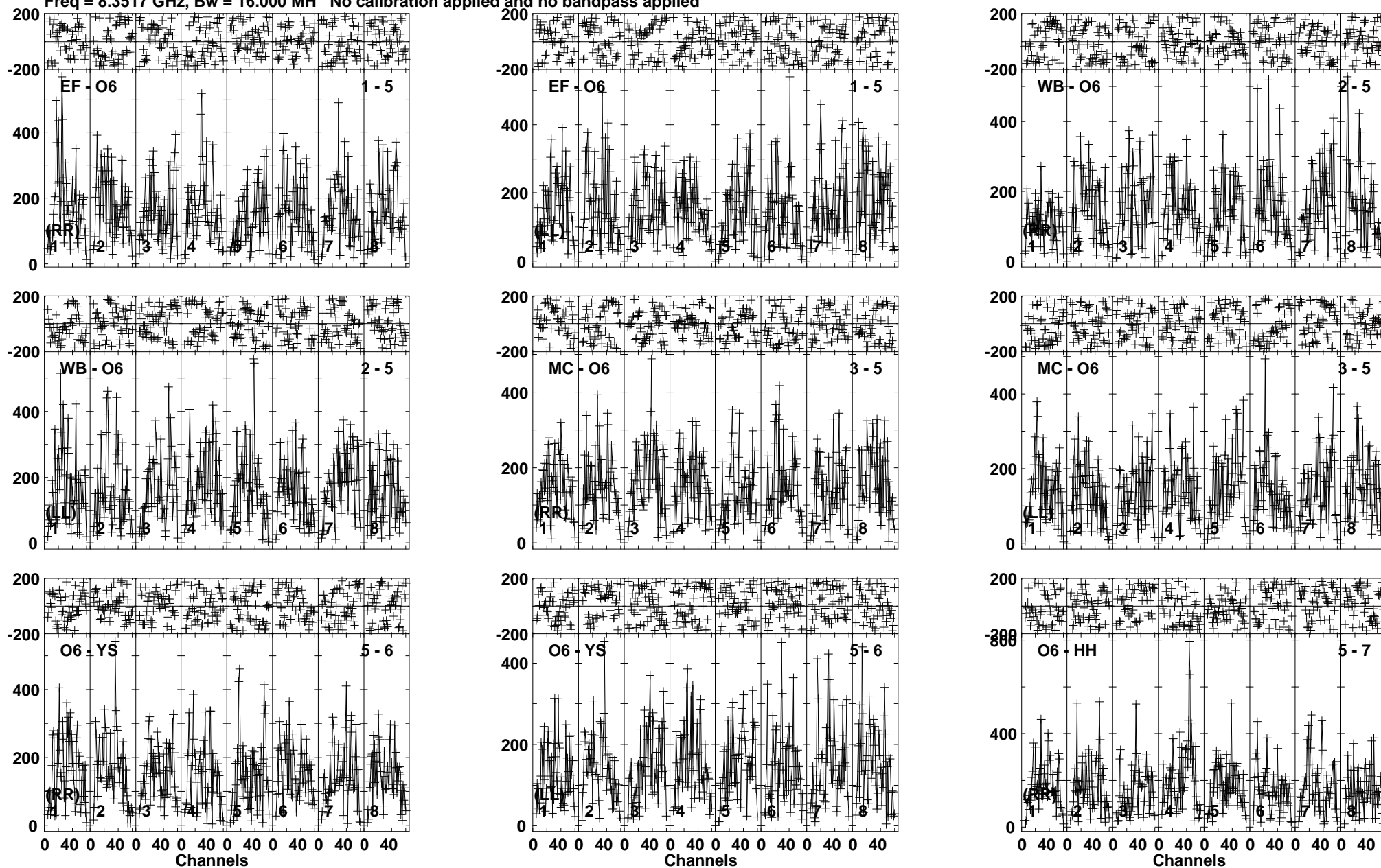
Lower frame: Micro Ampl Jy Top frame: Phas deg Vector averaged cross-power spectrum Baseline: EF (01) - O6 (05) Timerange: 00/07:20:30 to 00/07:22:44
