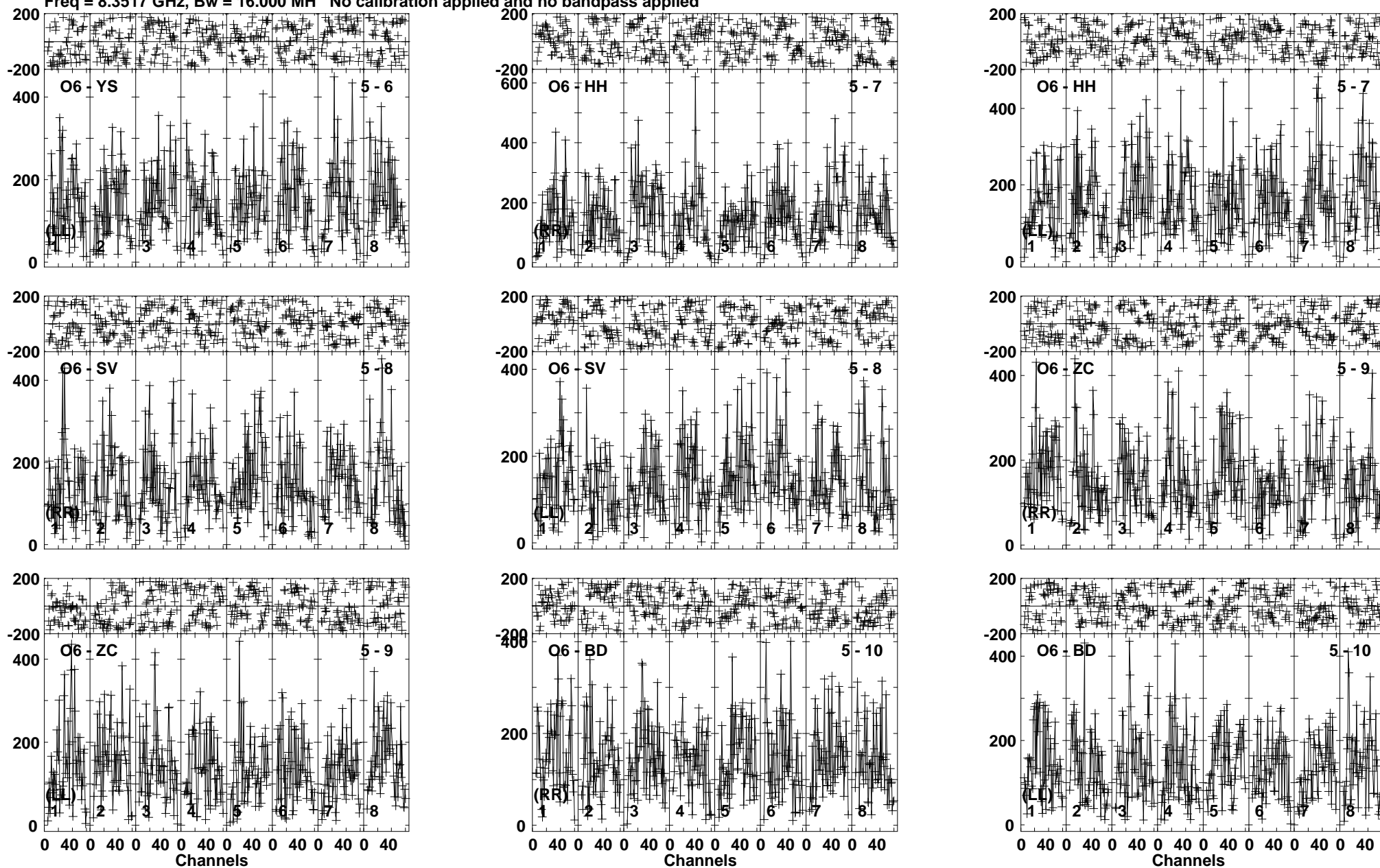
Lower frame: Micro Ampl Jy Top frame: Phas deg Vector averaged cross-power spectrum Baseline: O6 (05) - YS (06) Timerange: 00/03:16:11 to 00/03:18:24
