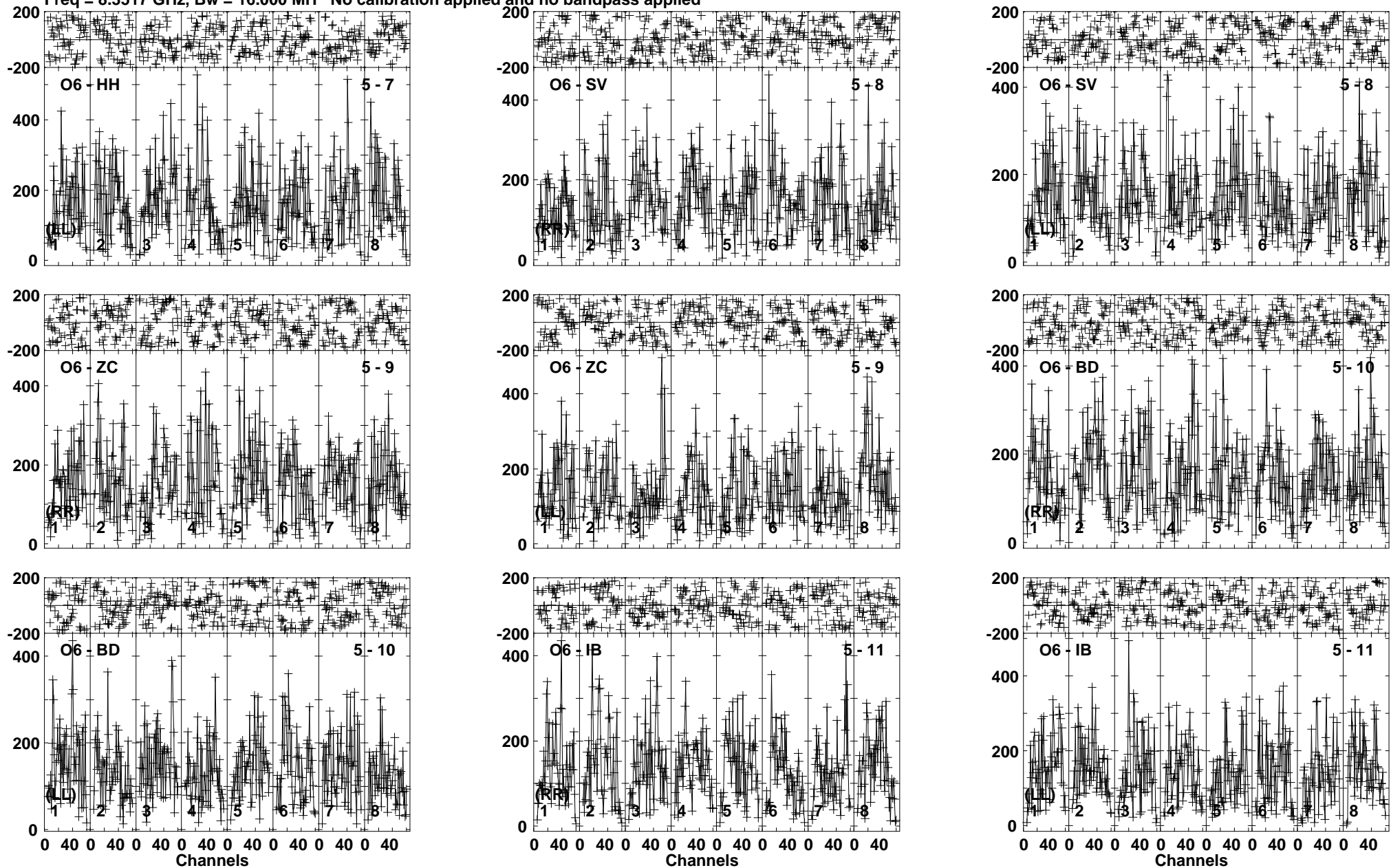
Lower frame: Micro Ampl Jy Top frame: Phas deg Vector averaged cross-power spectrum Baseline: O6 (05) - HH (07) Timerange: 00/04:16:21 to 00/04:18:34
