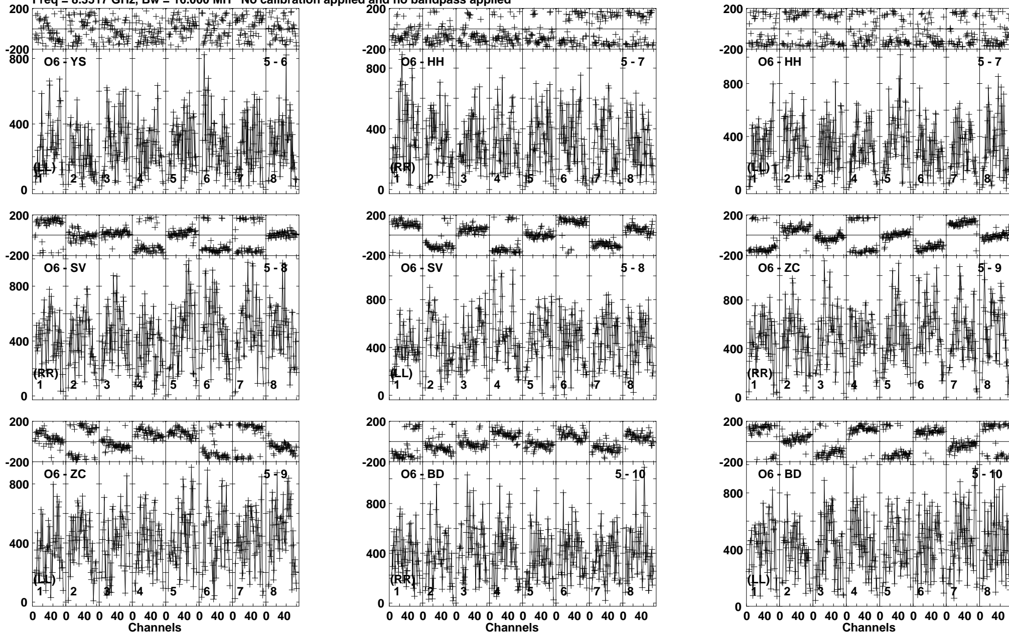
Lower frame: Micro Ampl Jy Top frame: Phas deg Vector averaged cross-power spectrum Baseline: O6 (05) - YS (06) Timerange: 00/01:42:25 to 00/01:43:10
