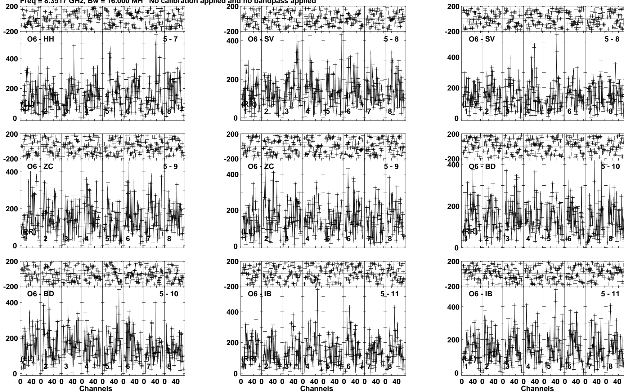
Lower frame: Micro Ampl Jy Top frame: Phas deg Vector averaged cross-power spectrum Baseline: O6 (05) - HH (07) Timerange: 00/03:36:16 to 00/03:38:30
