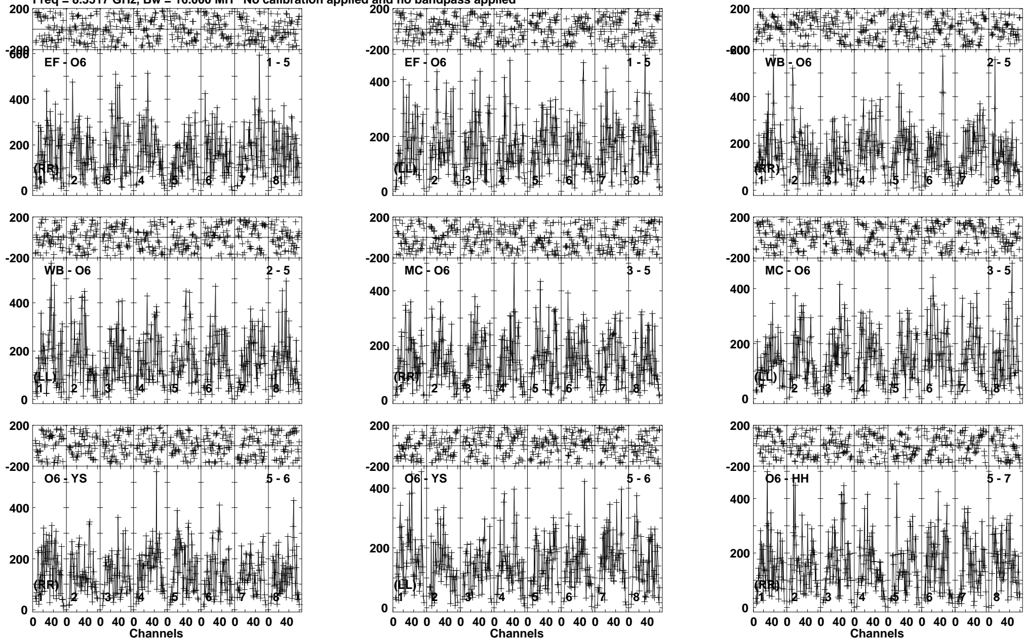
Lower frame: Micro Ampl Jy Top frame: Phas deg Vector averaged cross-power spectrum Baseline: EF (01) - O6 (05) Timerange: 00/09:31:56 to 00/09:34:09
