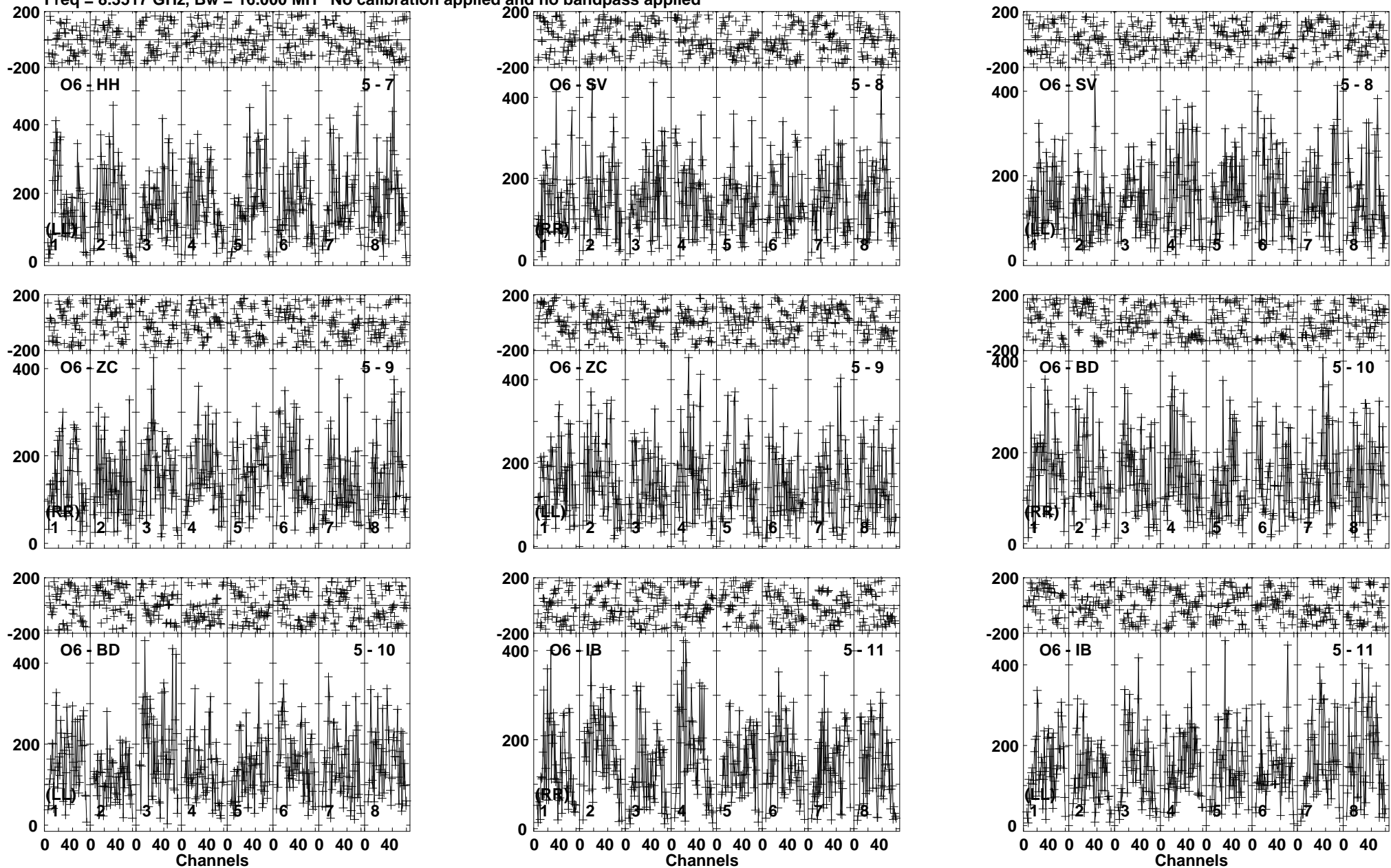
Lower frame: Micro Ampl Jy Top frame: Phas deg Vector averaged cross-power spectrum Baseline: O6 (05) - HH (07) Timerange: 00/04:22:46 to 00/04:24:59
