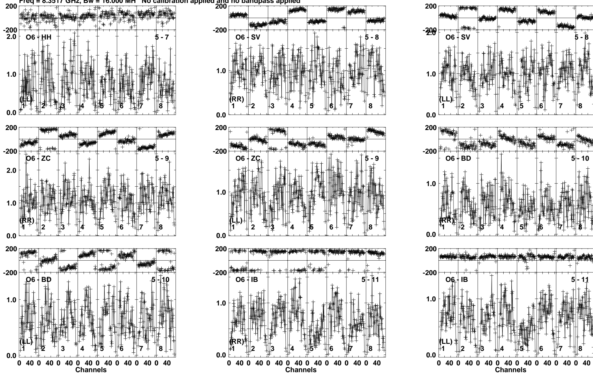
Lower frame: Milli Ampl Jy Top frame: Phas deg Vector averaged cross-power spectrum Baseline: O6 (05) - HH (07) Timerange: 00/05:10:05 to 00/05:10:49
