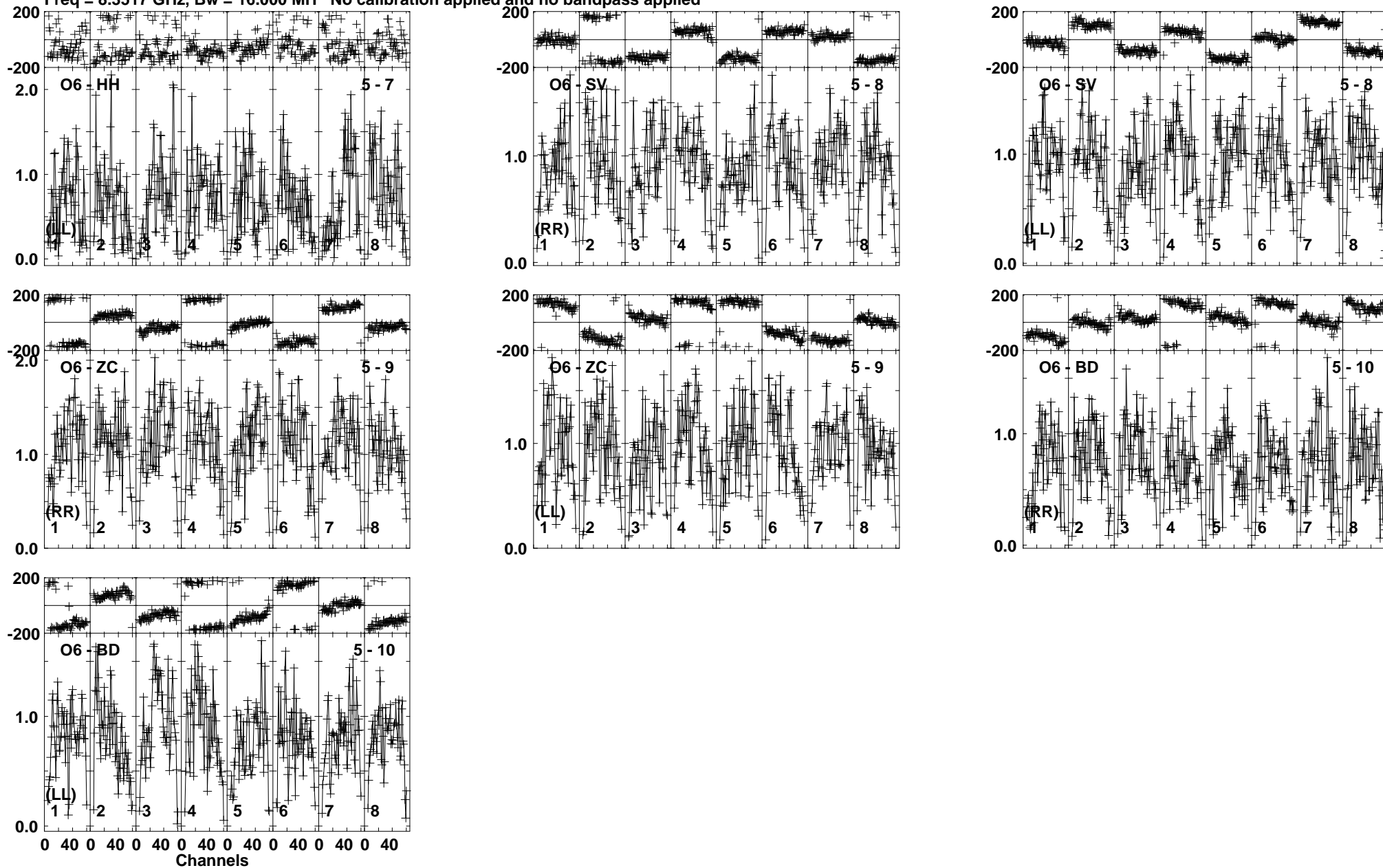
Lower frame: Milli Ampl Jy Top frame: Phas deg Vector averaged cross-power spectrum Baseline: O6 (05) - HH (07) Timerange: 00/01:11:30 to 00/01:12:15
