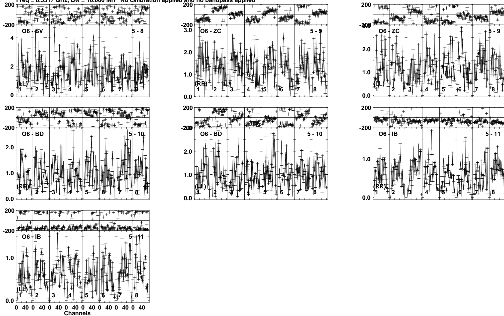
Lower frame: Milli Ampl Jy Top frame: Phas deg Vector averaged cross-power spectrum Baseline: O6 (05) - SV (08) Timerange: 00/01:23:06 to 00/01:23:35
