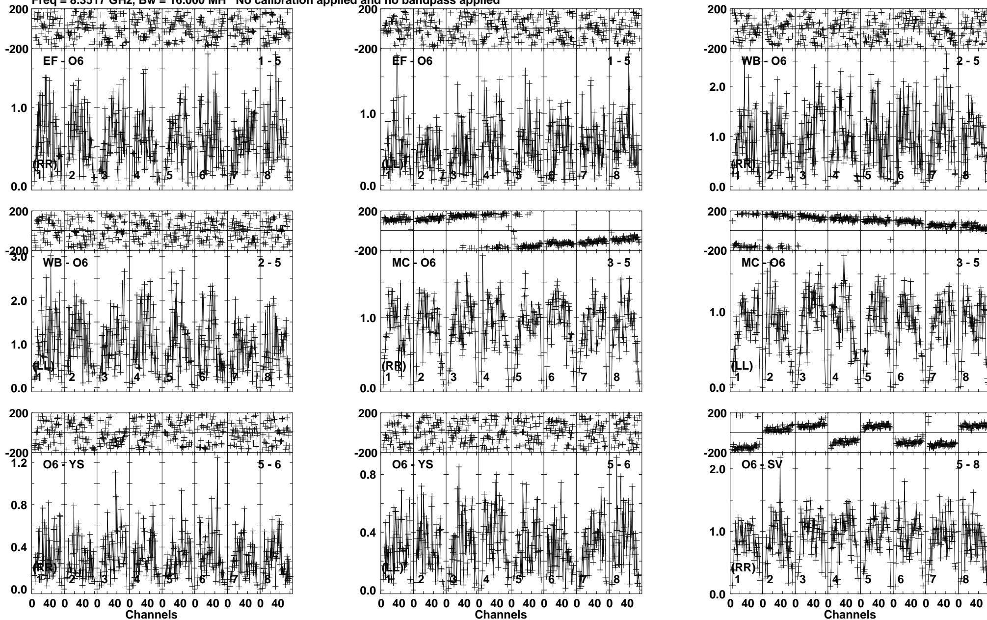
Lower frame: Milli Ampl Jy Top frame: Phas deg Vector averaged cross-power spectrum Baseline: EF (01) - O6 (05) Timerange: 00/02:01:05 to 00/02:01:50
