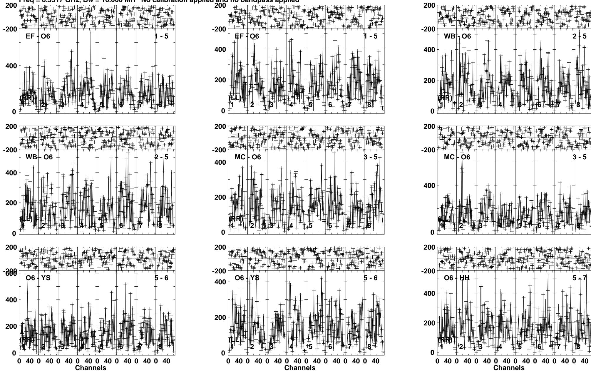
Lower frame: Micro Ampl Jy Top frame: Phas deg Vector averaged cross-power spectrum Baseline: EF (01) - O6 (05) Timerange: 00/04:22:46 to 00/04:24:59
