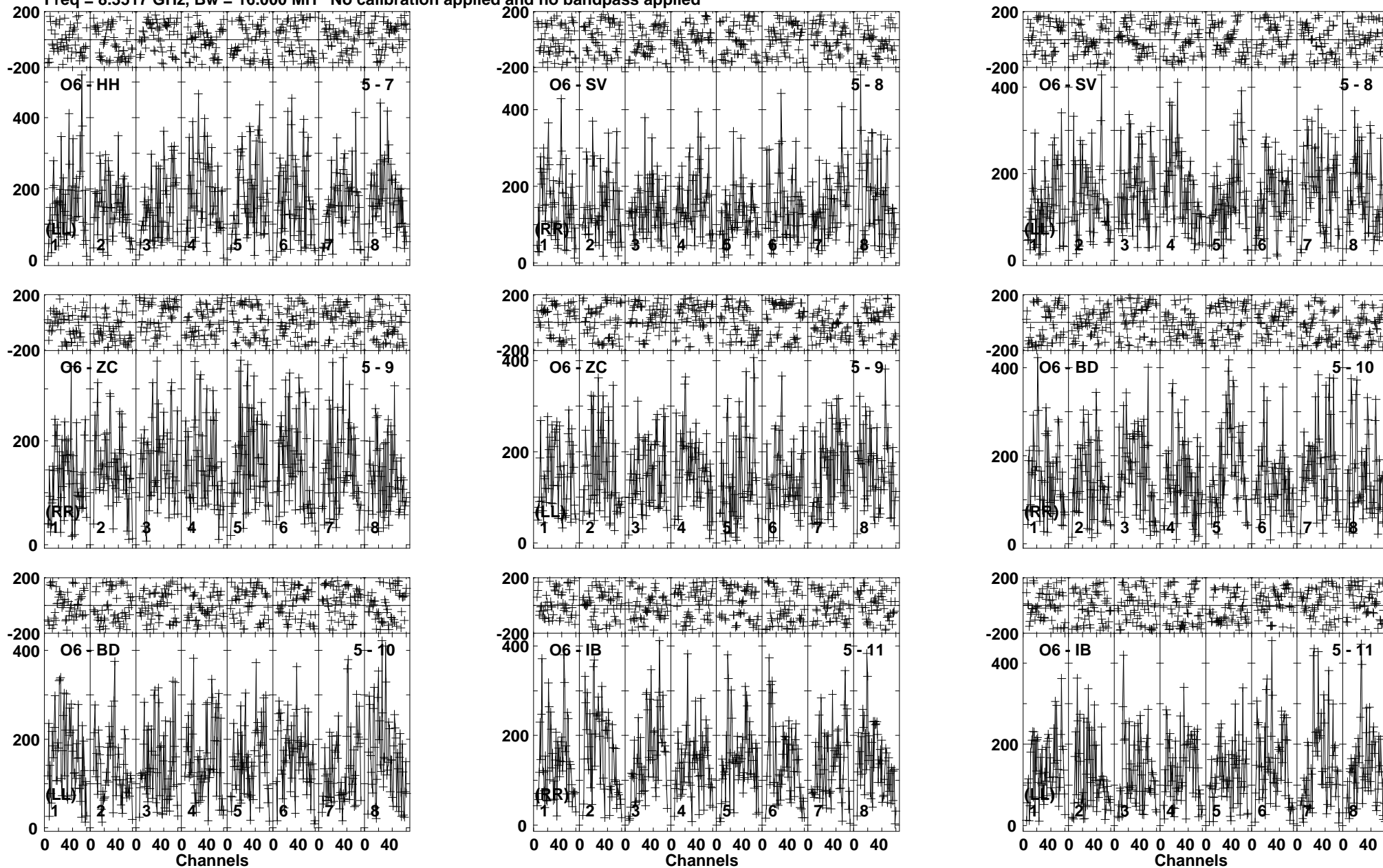
Lower frame: Micro Ampl Jy Top frame: Phas deg Vector averaged cross-power spectrum Baseline: O6 (05) - HH (07) Timerange: 00/04:47:45 to 00/04:49:59
