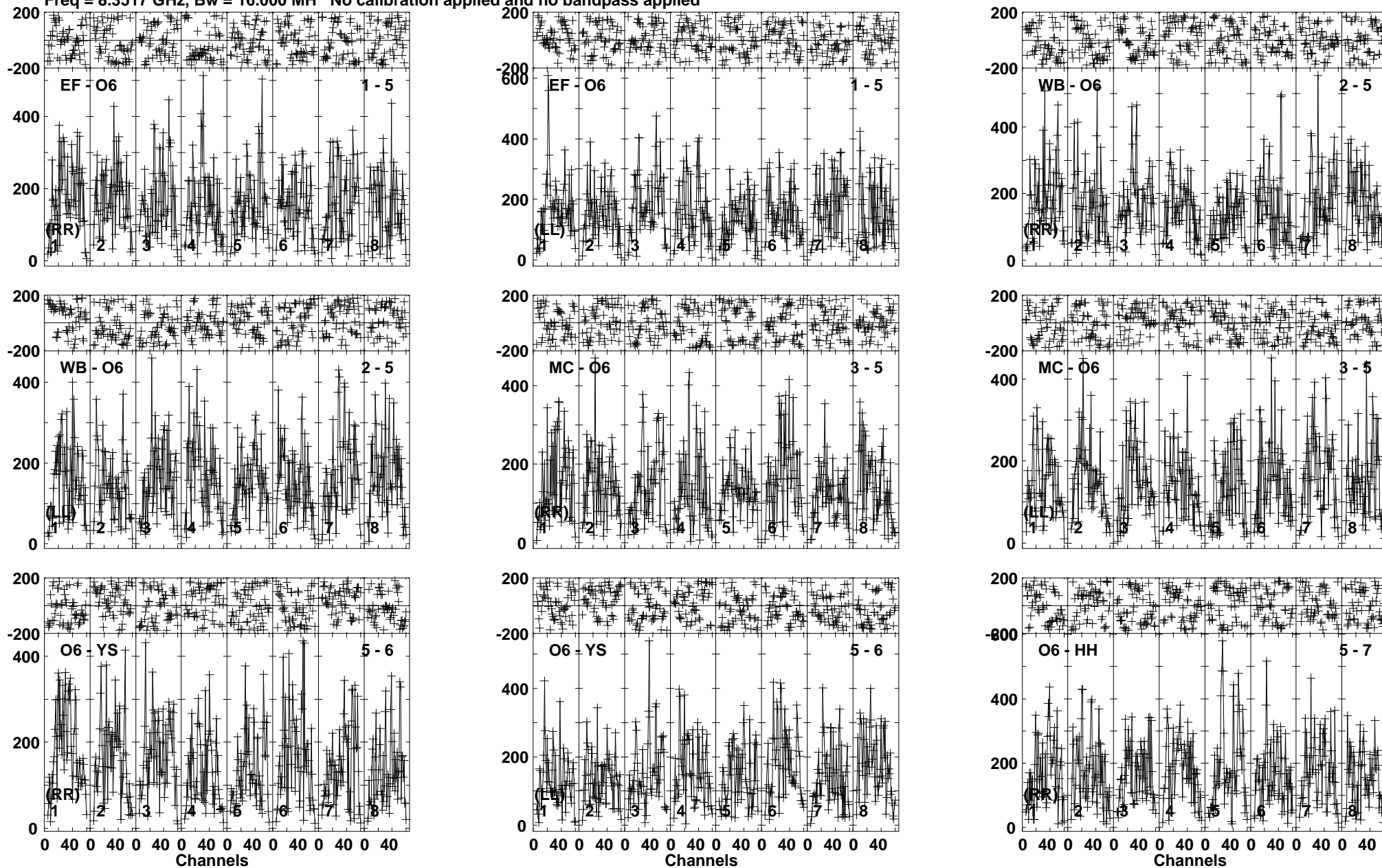
Lower frame: Micro Ampl Jy Top frame: Phas deg Vector averaged cross-power spectrum Baseline: EF (01) - O6 (05) Timerange: 00/08:11:35 to 00/08:13:49
