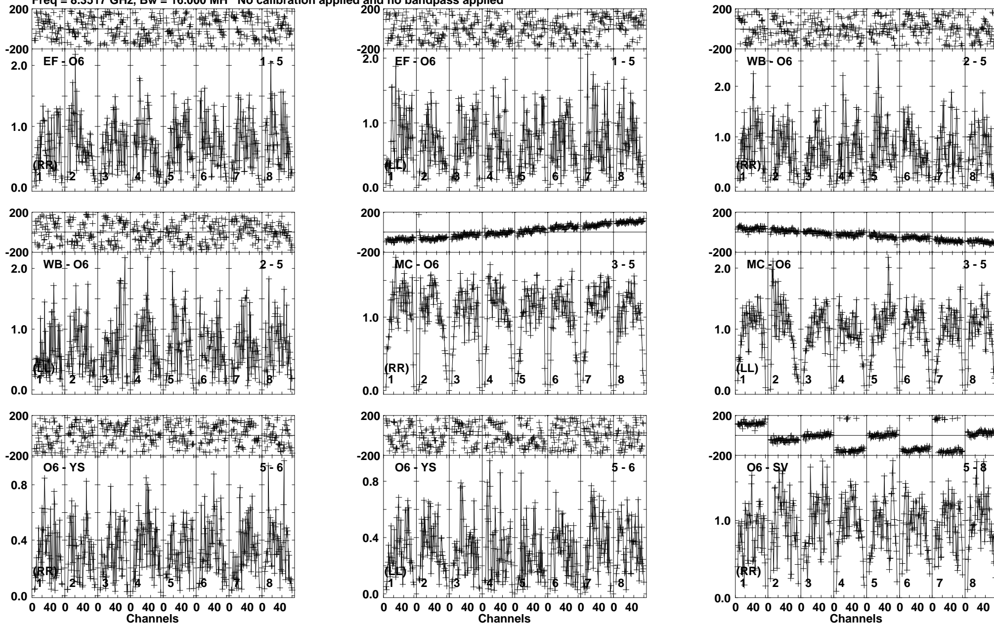
Lower frame: Milli Ampl Jy Top frame: Phas deg Vector averaged cross-power spectrum Baseline: EF (01) - O6 (05) Timerange: 00/06:45:35 to 00/06:46:19
