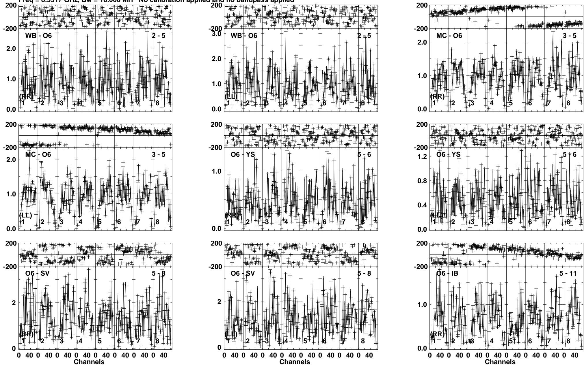
Lower frame: Milli Ampl Jy Top frame: Phas deg Vector averaged cross-power spectrum Baseline: WB (02) - O6 (05) Timerange: 00/08:48:15 to 00/08:48:44
