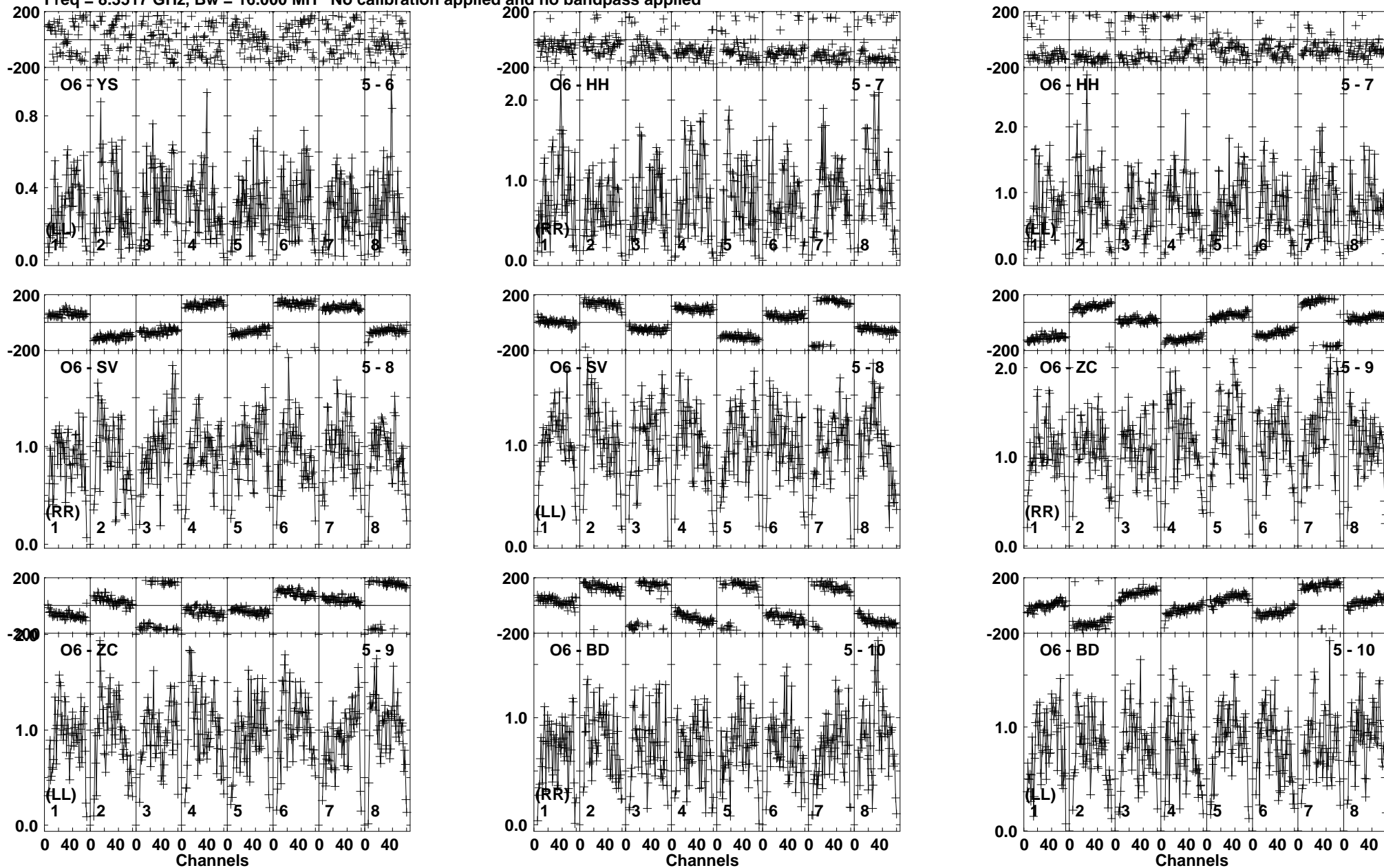
Lower frame: Milli Ampl Jy Top frame: Phas deg Vector averaged cross-power spectrum Baseline: O6 (05) - YS (06) Timerange: 00/03:18:25 to 00/03:19:09
