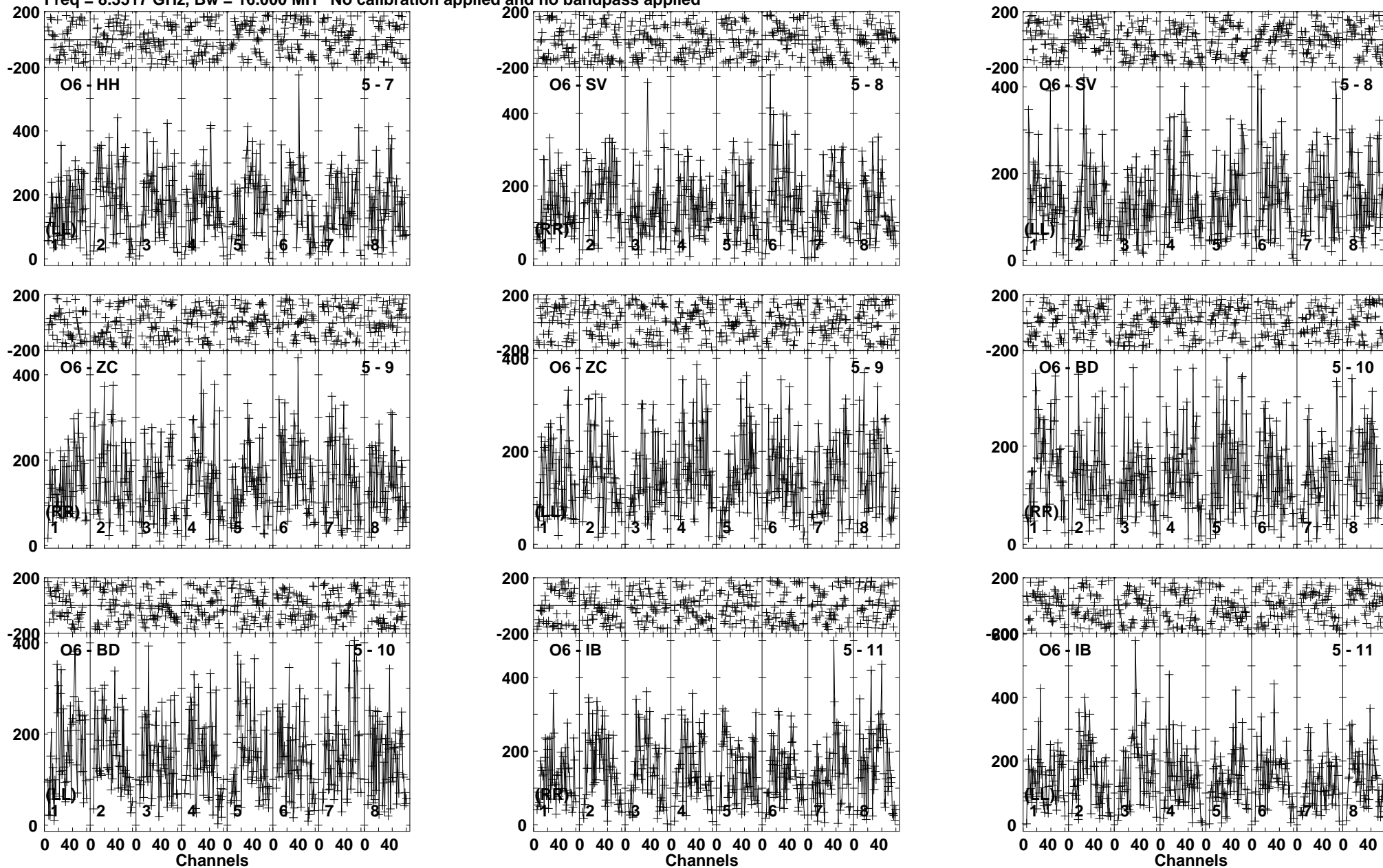
Lower frame: Micro Ampl Jy Top frame: Phas deg Vector averaged cross-power spectrum Baseline: O6 (05) - HH (07) Timerange: 00/03:09:46 to 00/03:11:59
