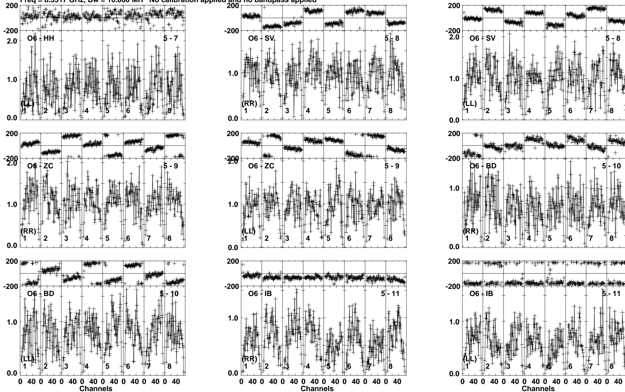
Lower frame: Milli Ampl Jy Top frame: Phas deg Vector averaged cross-power spectrum Baseline: O6 (05) - HH (07) Timerange: 00/03:41:30 to 00/03:42:14
