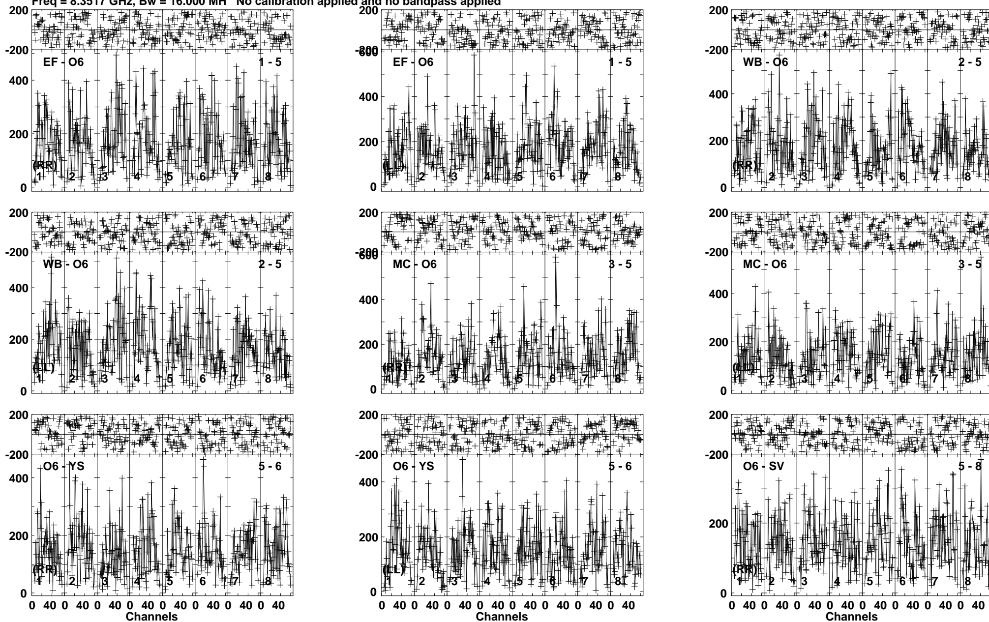
Lower frame: Micro Ampl Jy Top frame: Phas deg Vector averaged cross-power spectrum Baseline: EF (01) - O6 (05) Timerange: 00/10:01:11 to 00/10:03:25
