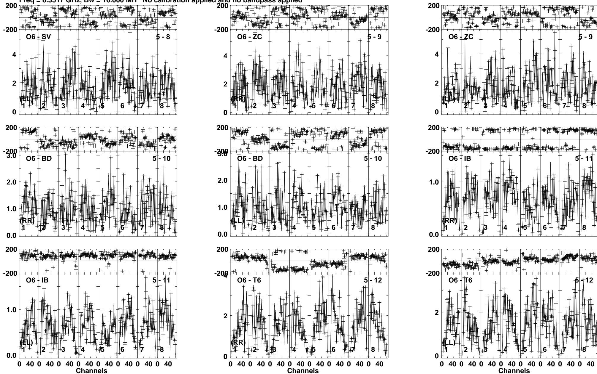
Lower frame: Milli Ampl Jy Top frame: Phas deg Vector averaged cross-power spectrum Baseline: O6 (05) - SV (08) Timerange: 00/03:23:36 to 00/03:24:04
