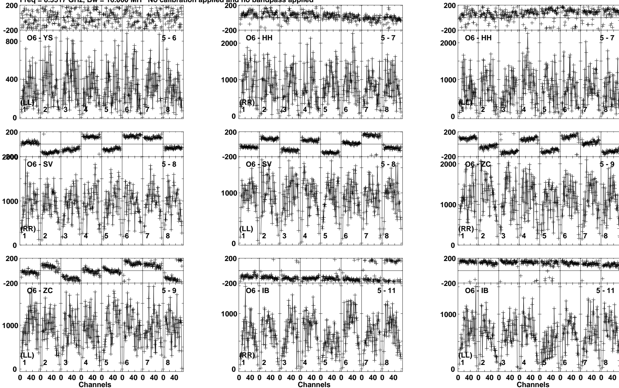
Lower frame: Micro Ampl Jy Top frame: Phas deg Vector averaged cross-power spectrum Baseline: O6 (05) - YS (06) Timerange: 00/06:36:11 to 00/06:36:55
