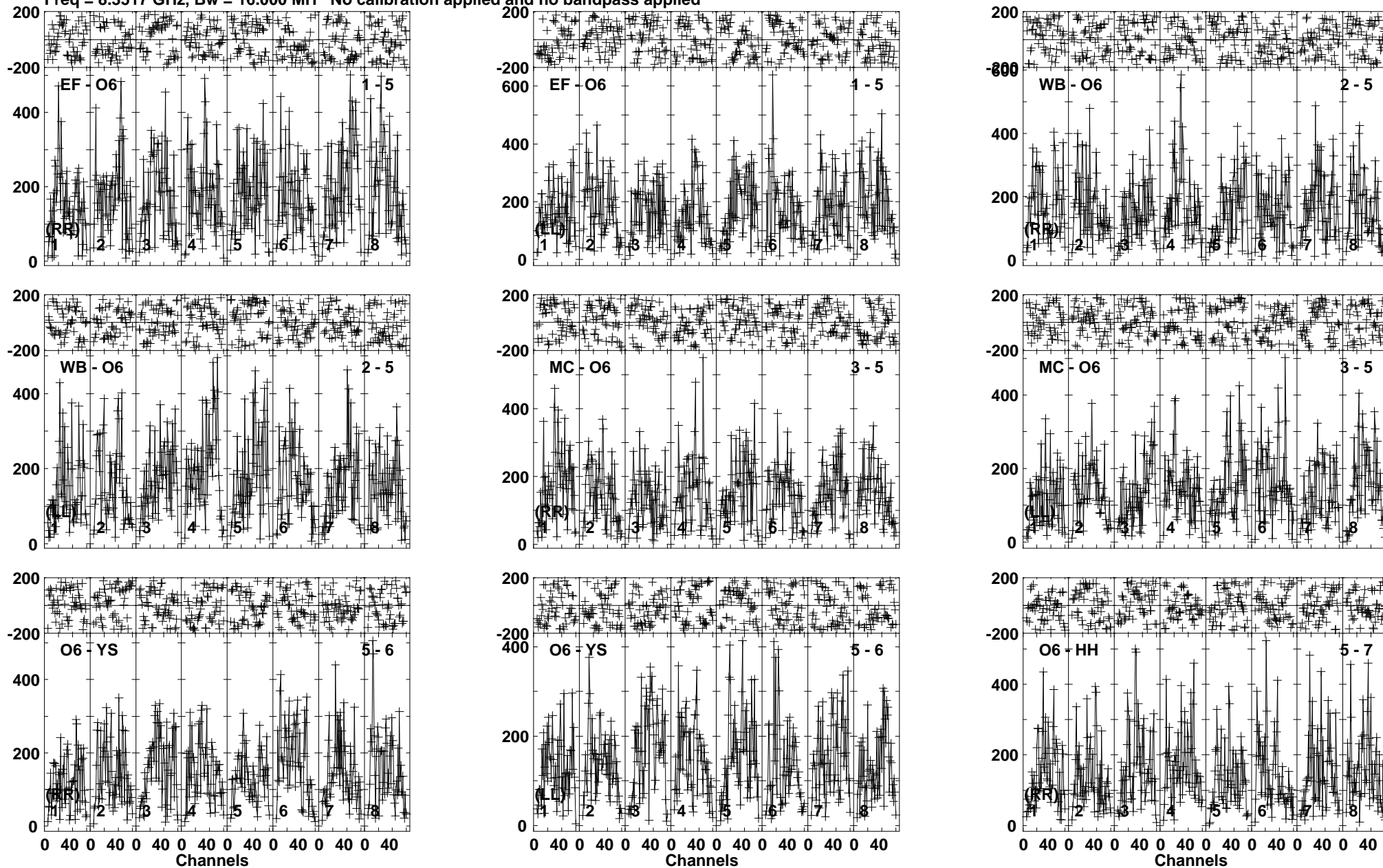
Lower frame: Micro Ampl Jy Top frame: Phas deg Vector averaged cross-power spectrum Baseline: EF (01) - O6 (05) Timerange: 00/08:37:25 to 00/08:39:39
