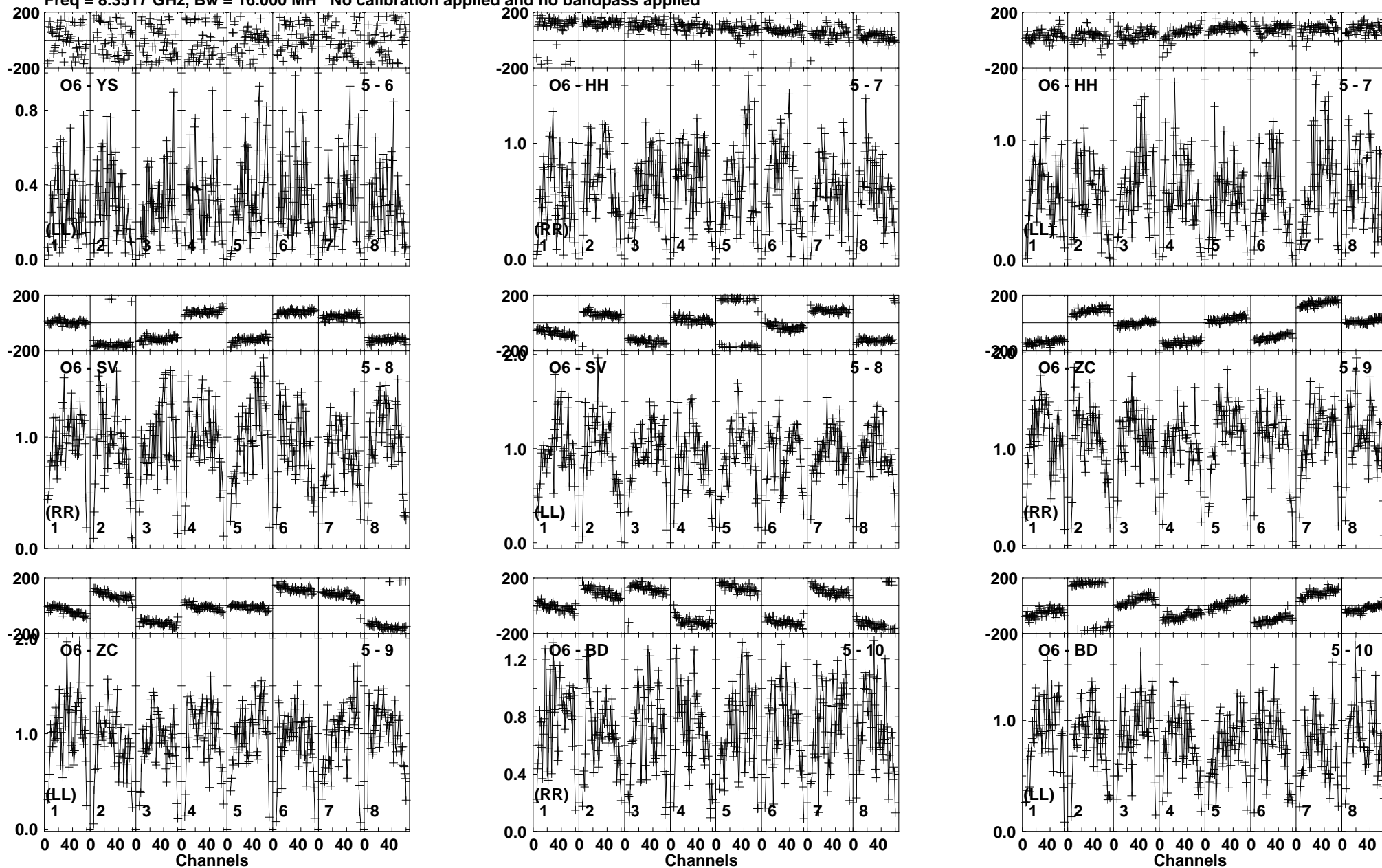
Lower frame: Milli Ampl Jy Top frame: Phas deg Vector averaged cross-power spectrum Baseline: O6 (05) - YS (06) Timerange: 00/02:15:26 to 00/02:15:54
