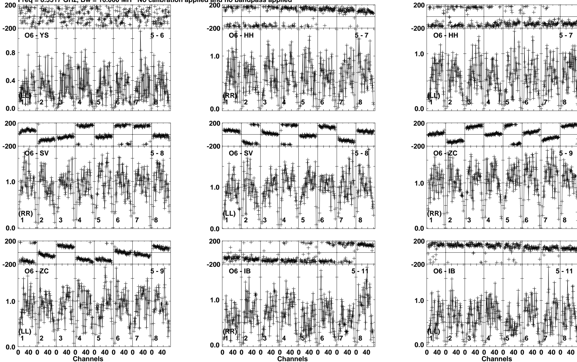
Lower frame: Milli Ampl Jy Top frame: Phas deg Vector averaged cross-power spectrum Baseline: O6 (05) - YS (06) Timerange: 00/07:20:00 to 00/07:20:30
