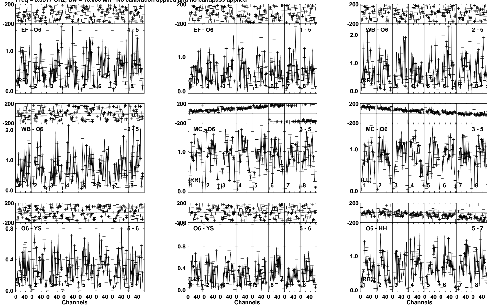
Lower frame: Milli Ampl Jy Top frame: Phas deg Vector averaged cross-power spectrum Baseline: EF (01) - O6 (05) Timerange: 00/01:38:01 to 00/01:38:44
