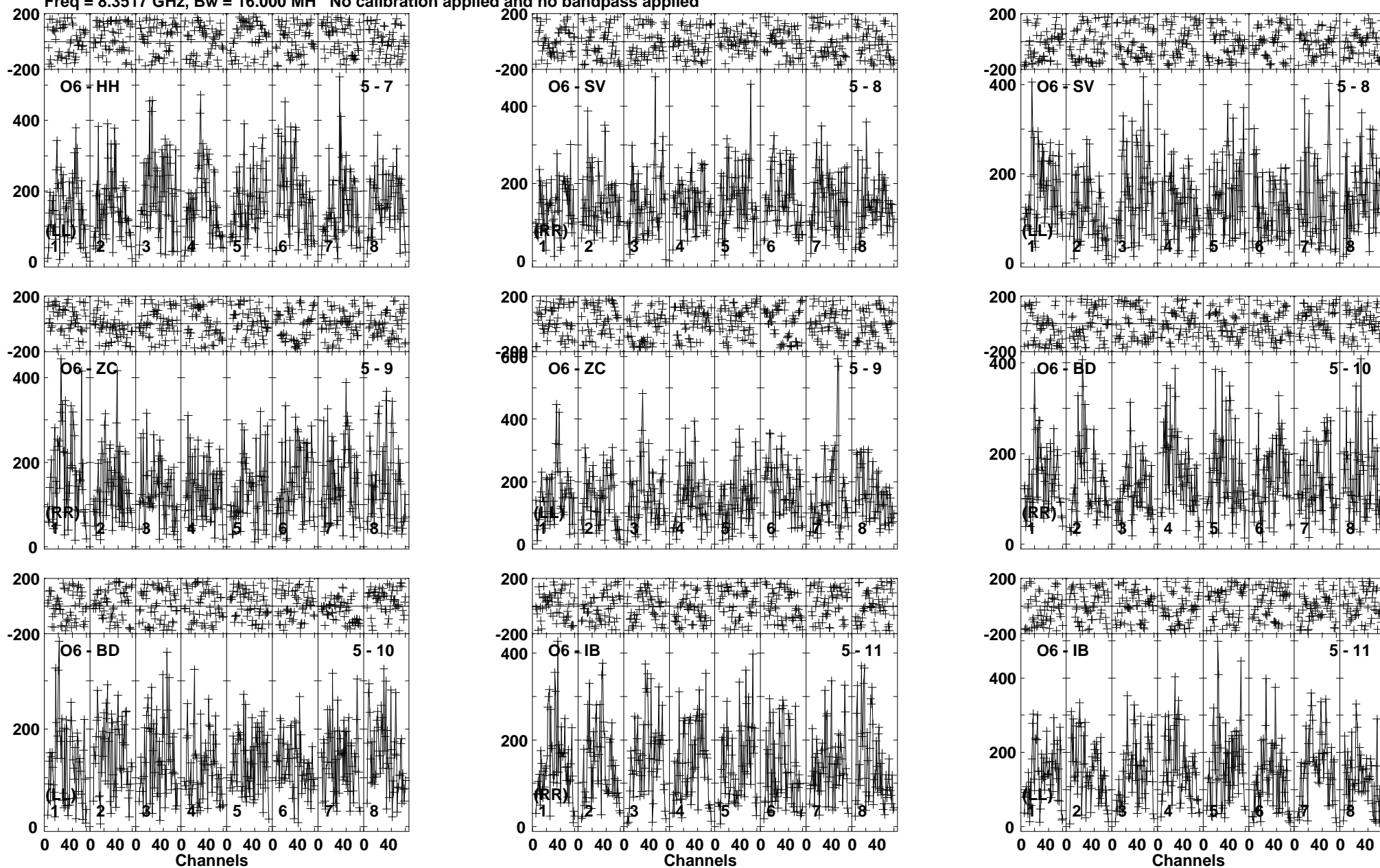
Lower frame: Micro Ampl Jy Top frame: Phas deg Vector averaged cross-power spectrum Baseline: O6 (05) - HH (07) Timerange: 00/03:49:56 to 00/03:52:09
