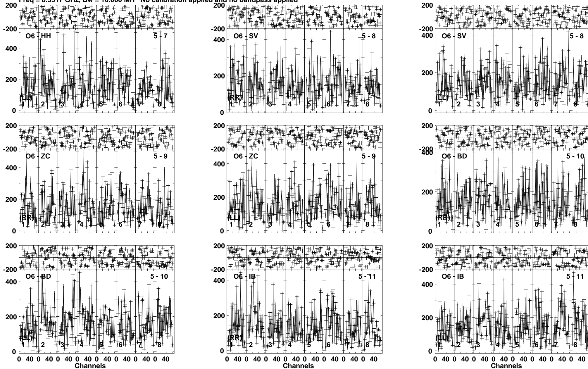
Lower frame: Micro Ampl Jy Top frame: Phas deg Vector averaged cross-power spectrum Baseline: O6 (05) - HH (07) Timerange: 00/05:07:51 to 00/05:10:04
