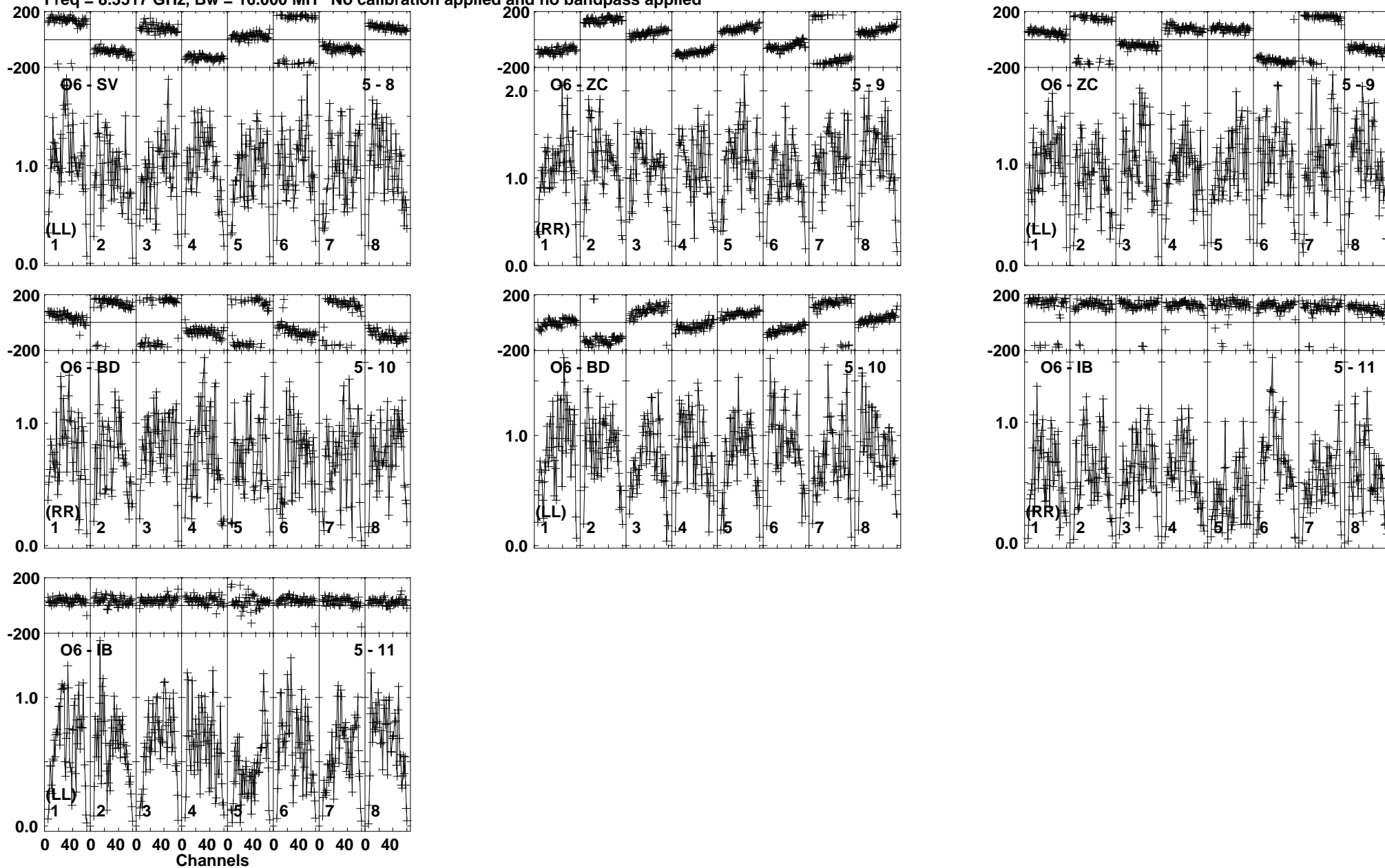
Lower frame: Milli Ampl Jy Top frame: Phas deg Vector averaged cross-power spectrum Baseline: O6 (05) - SV (08) Timerange: 00/02:01:05 to 00/02:01:50
