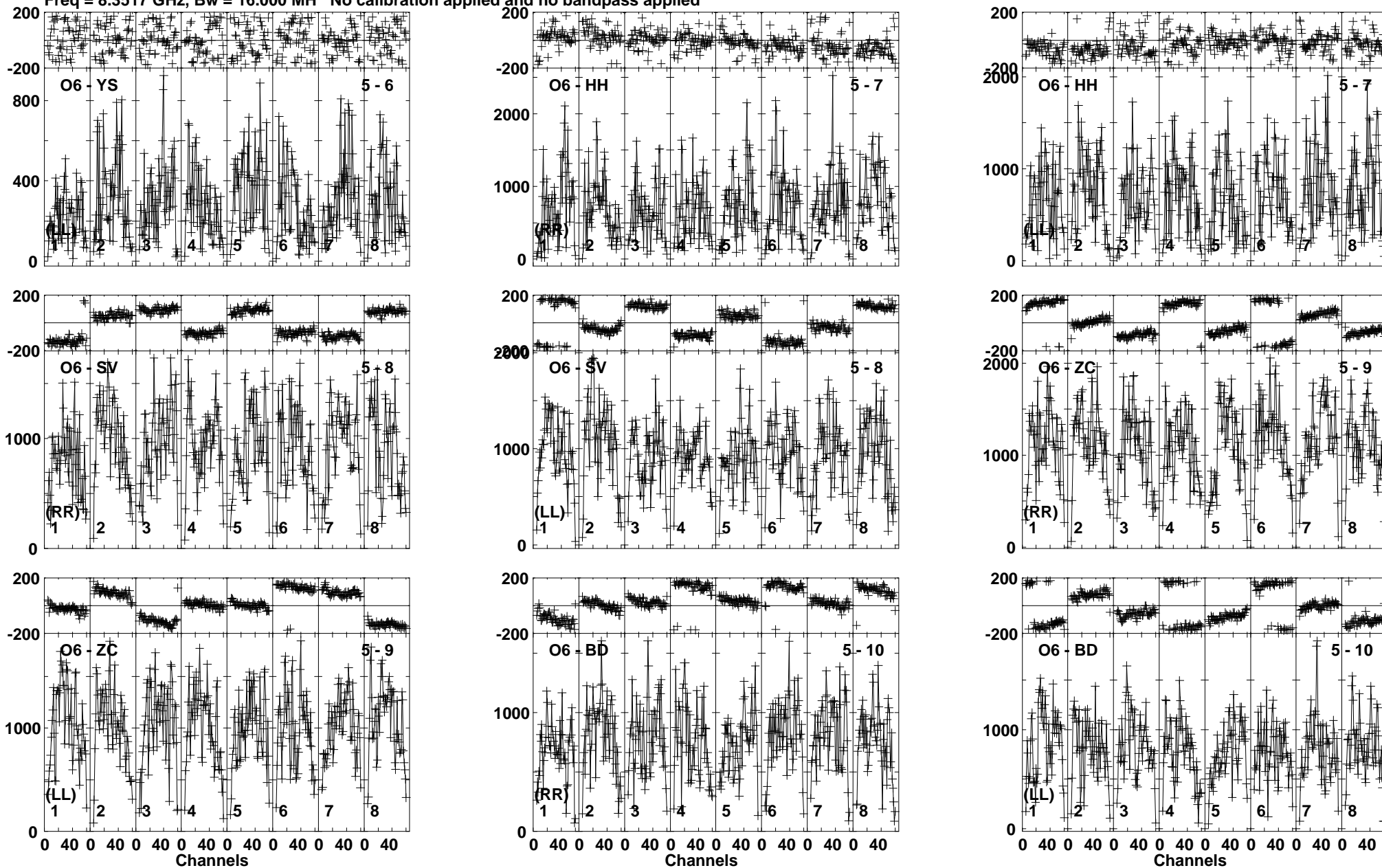
Lower frame: Micro Ampl Jy Top frame: Phas deg Vector averaged cross-power spectrum Baseline: O6 (05) - YS (06) Timerange: 00/01:45:56 to 00/01:46:40
