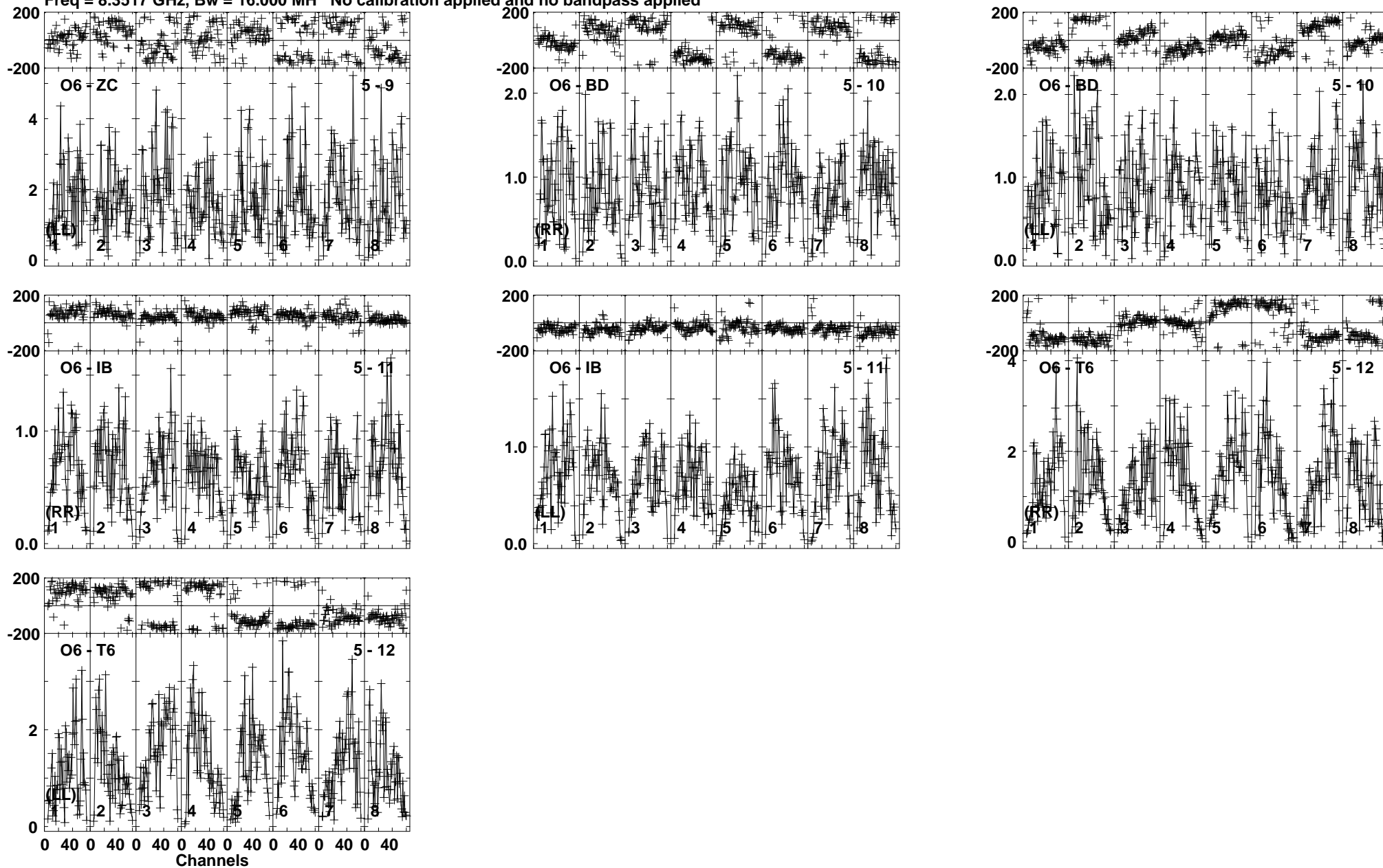
Lower frame: Milli Ampl Jy Top frame: Phas deg Vector averaged cross-power spectrum Baseline: O6 (05) - ZC (09) Timerange: 00/03:49:27 to 00/03:49:55
