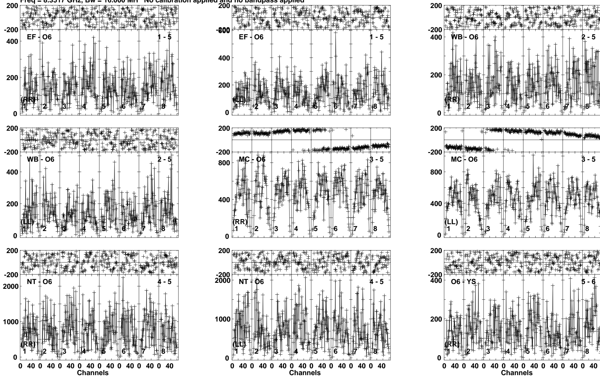
Lower frame: Micro Ampl Jy Top frame: Phas deg Vector averaged cross-power spectrum Baseline: EF (01) - O6 (05) Timerange: 00/10:57:56 to 00/10:59:59
