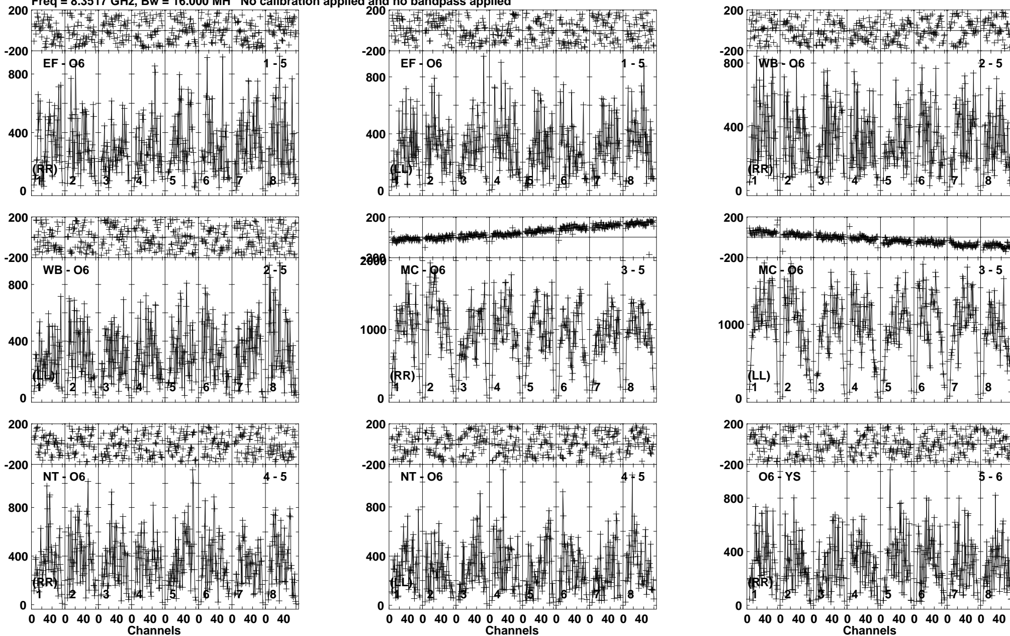
Lower frame: Micro Ampl Jy Top frame: Phas deg Vector averaged cross-power spectrum Baseline: EF (01) - O6 (05) Timerange: 00/03:35:46 to 00/03:36:14
