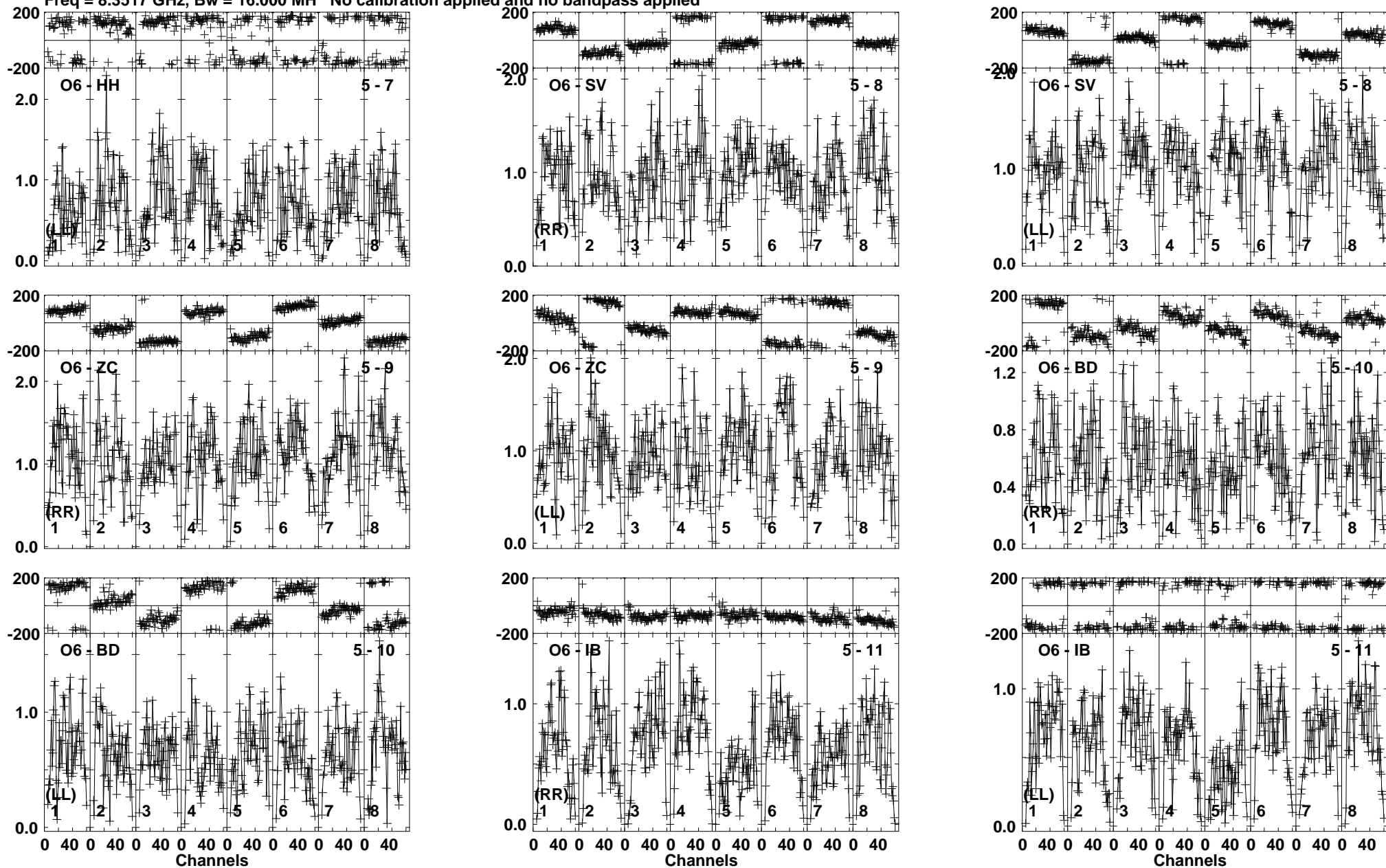
Lower frame: Milli Ampl Jy Top frame: Phas deg Vector averaged cross-power spectrum Baseline: O6 (05) - HH (07) Timerange: 00/05:02:11 to 00/05:02:55
