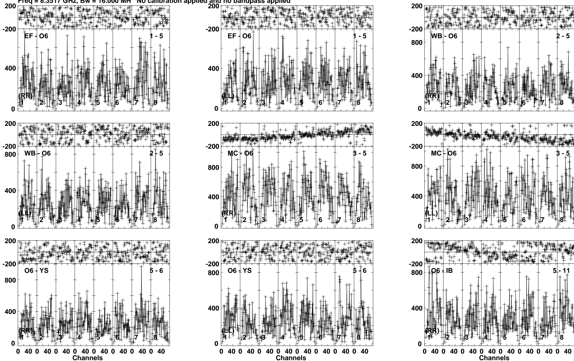
Lower frame: Micro Ampl Jy Top frame: Phas deg Vector averaged cross-power spectrum Baseline: EF (01) - O6 (05) Timerange: 00/10:27:56 to 00/10:28:40
