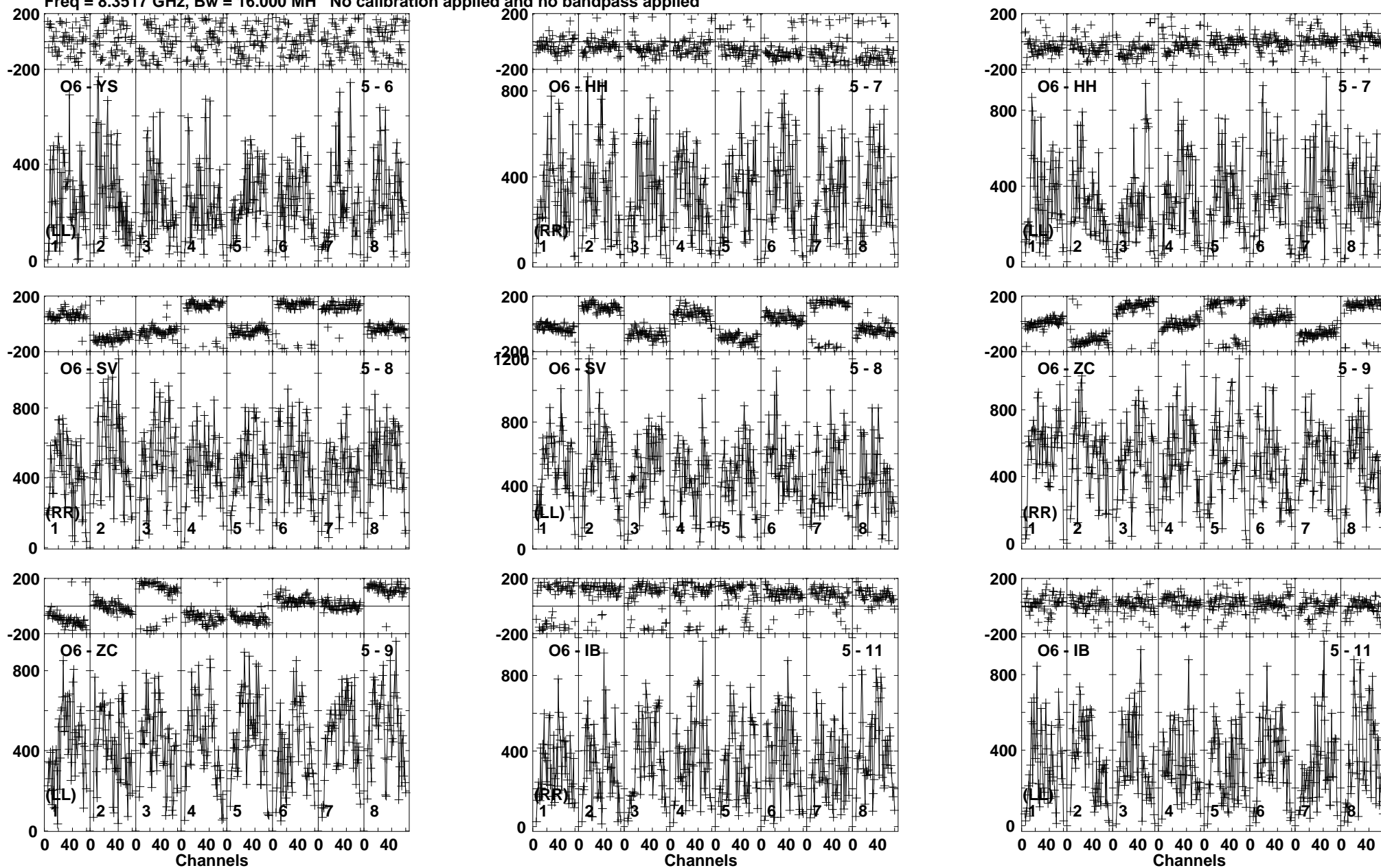
Lower frame: Micro Ampl Jy Top frame: Phas deg Vector averaged cross-power spectrum Baseline: O6 (05) - YS (06) Timerange: 00/06:26:56 to 00/06:27:40
