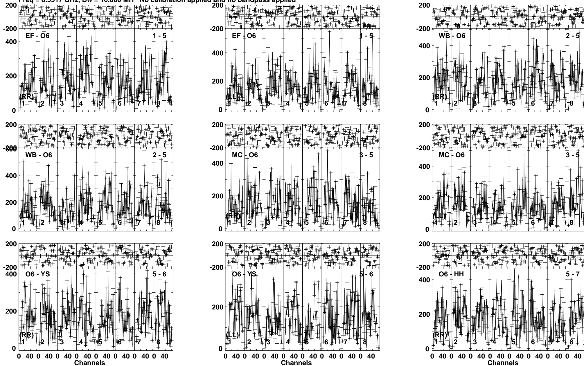
Lower frame: Micro Ampl Jy Top frame: Phas deg Vector averaged cross-power spectrum Baseline: EF (01) - O6 (05) Timerange: 00/05:07:51 to 00/05:10:04
