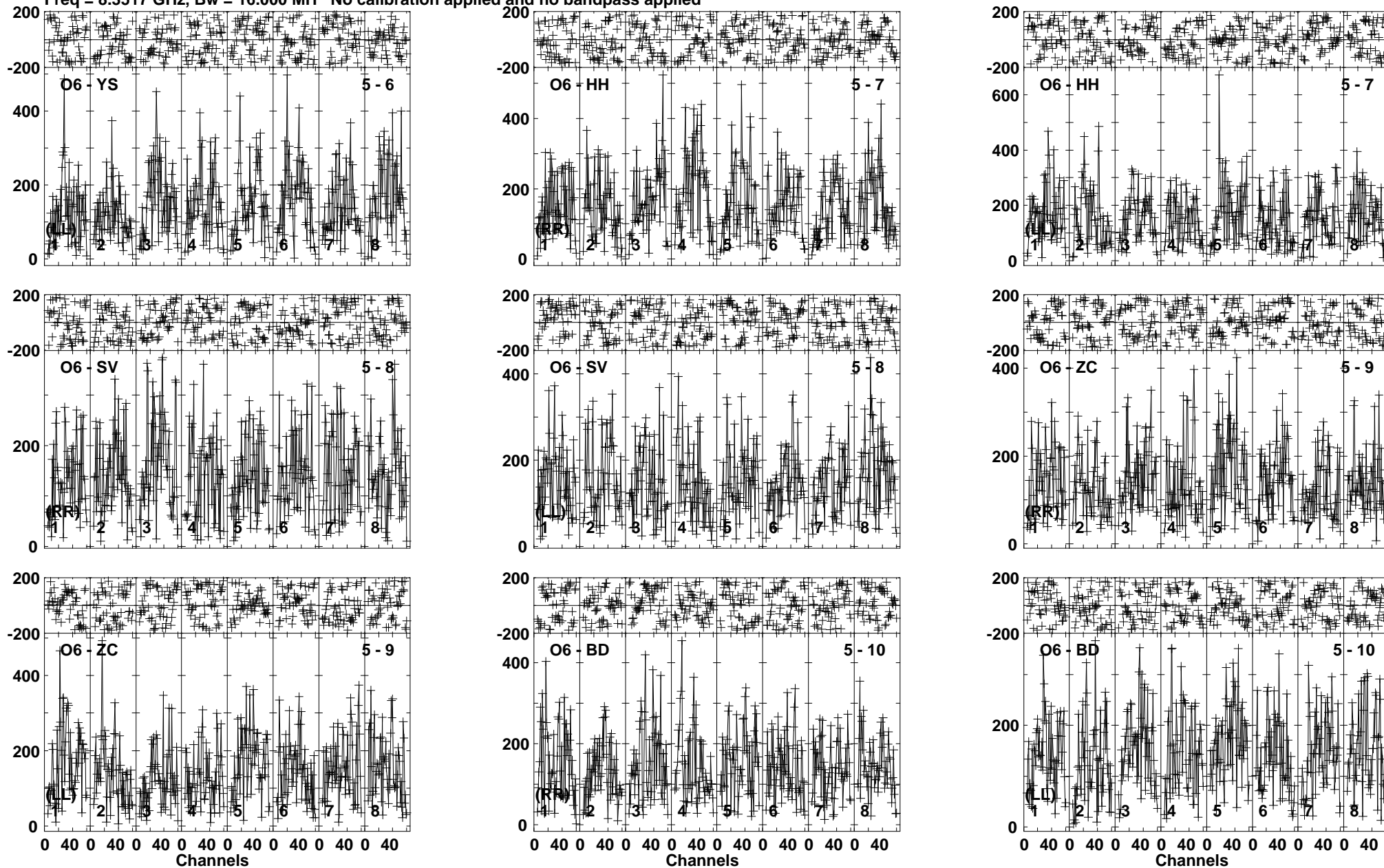
Lower frame: Micro Ampl Jy Top frame: Phas deg Vector averaged cross-power spectrum Baseline: O6 (05) - YS (06) Timerange: 00/02:15:55 to 00/02:18:10
