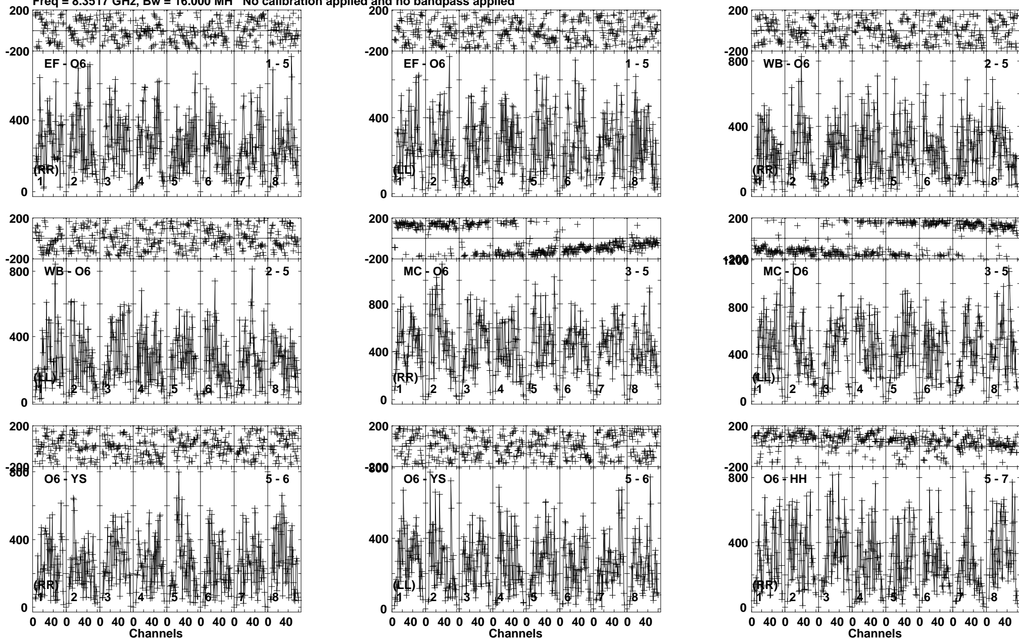
Lower frame: Micro Ampl Jy Top frame: Phas deg Vector averaged cross-power spectrum Baseline: EF (01) - O6 (05) Timerange: 00/08:27:25 to 00/08:28:09
