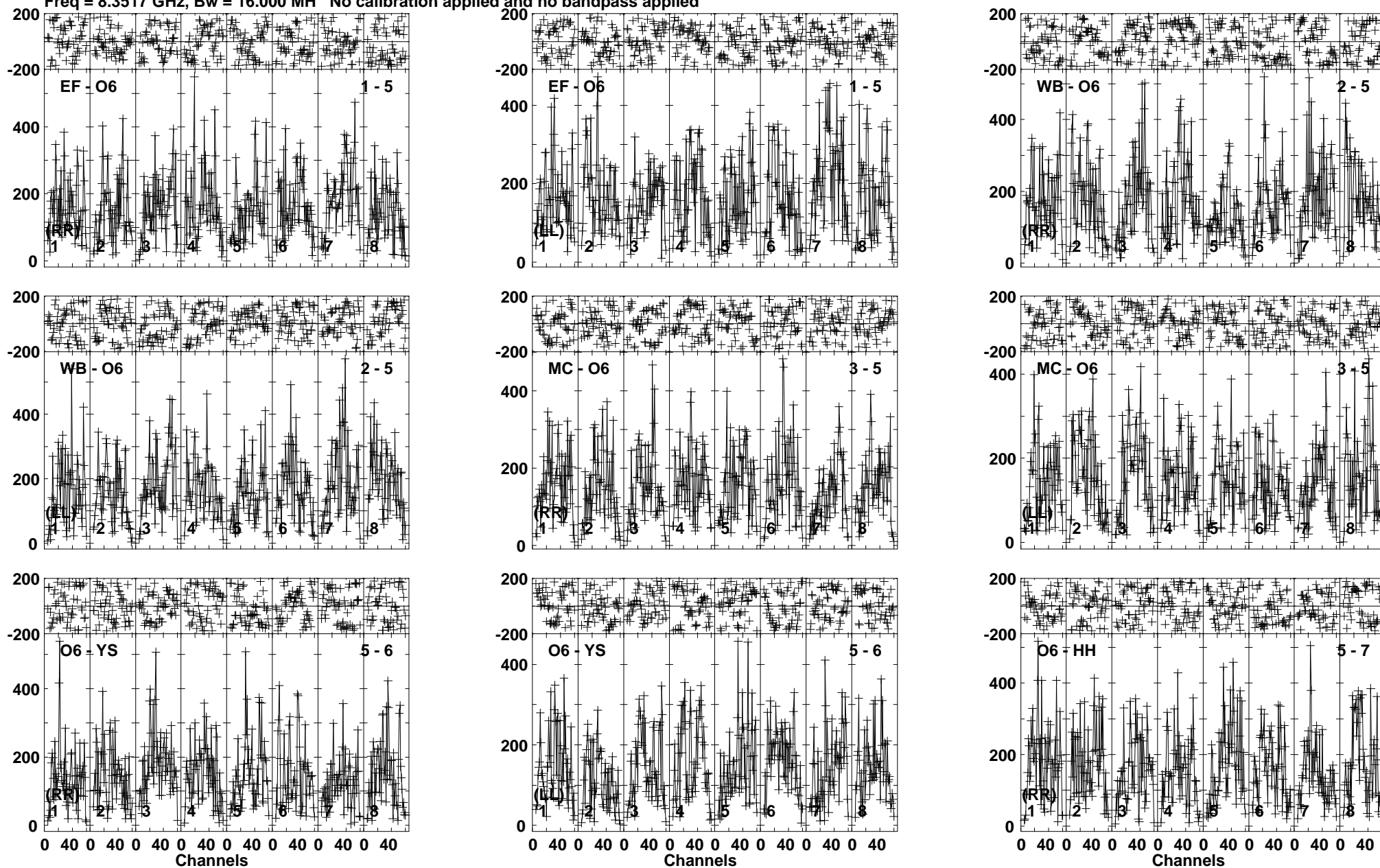
Lower frame: Micro Ampl Jy Top frame: Phas deg Vector averaged cross-power spectrum Baseline: EF (01) - O6 (05) Timerange: 00/09:41:06 to 00/09:43:20
