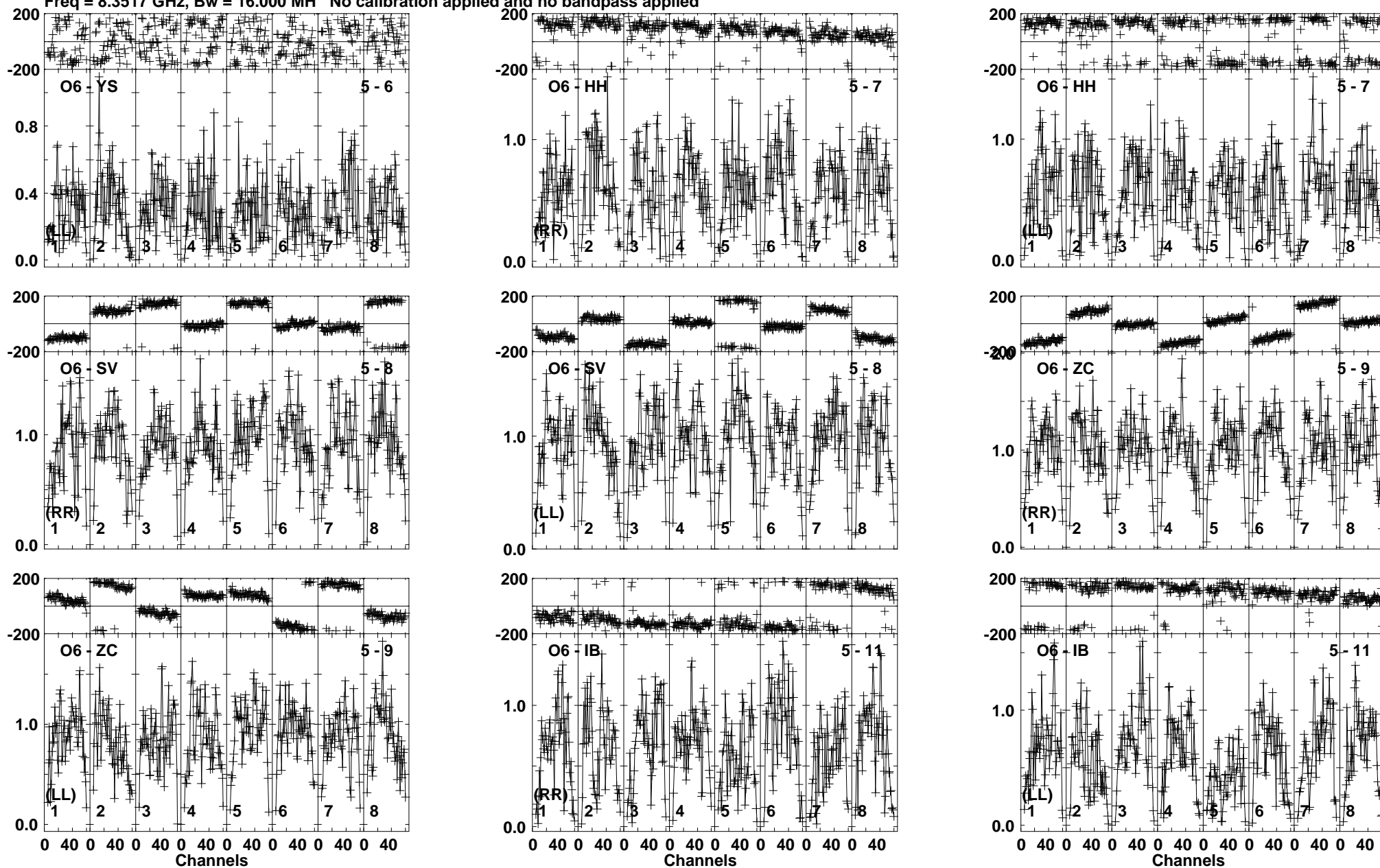
Lower frame: Milli Ampl Jy Top frame: Phas deg Vector averaged cross-power spectrum Baseline: O6 (05) - YS (06) Timerange: 00/07:40:06 to 00/07:40:34
