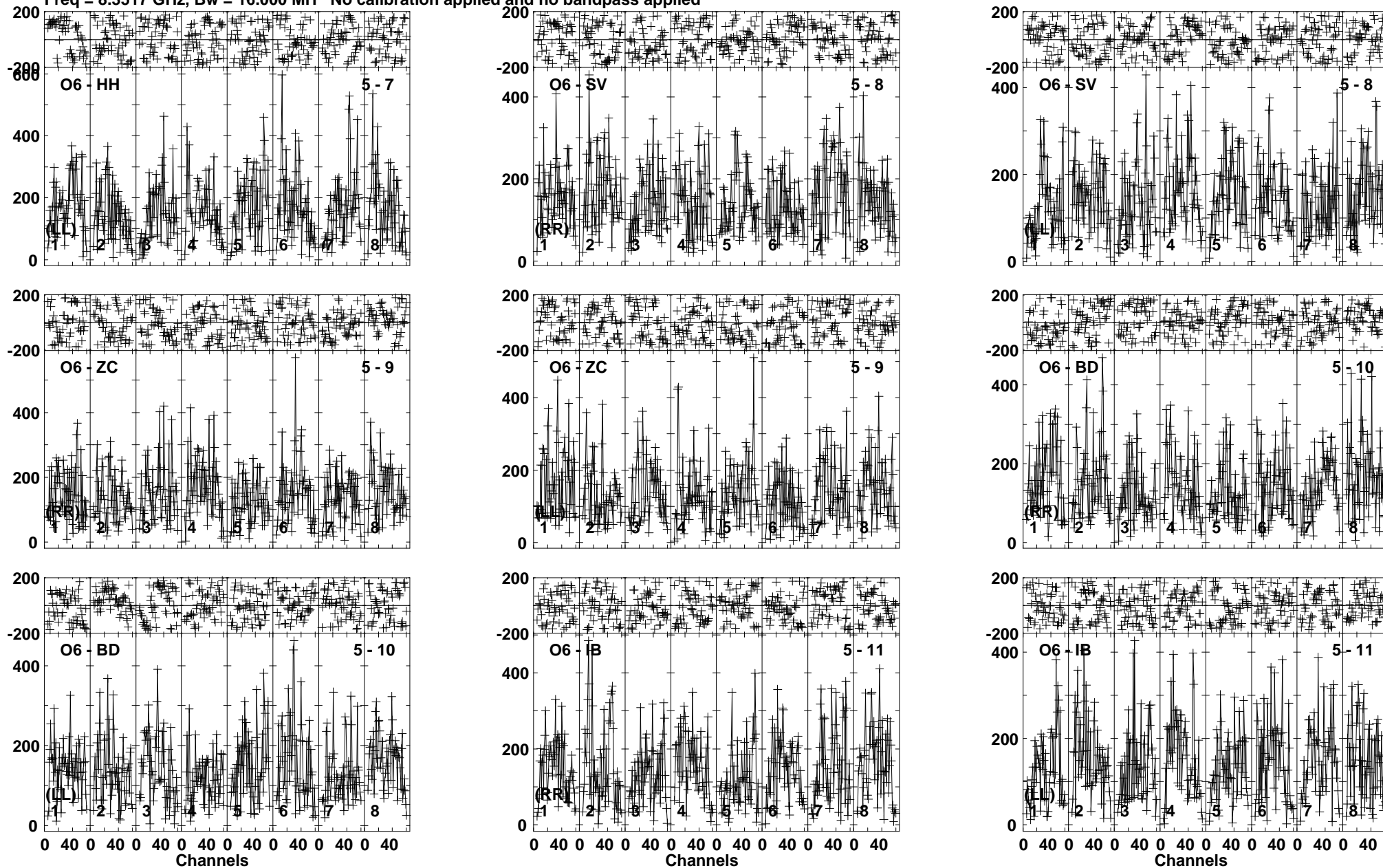
Lower frame: Micro Ampl Jy Top frame: Phas deg Vector averaged cross-power spectrum Baseline: O6 (05) - HH (07) Timerange: 00/01:18:40 to 00/01:20:54
