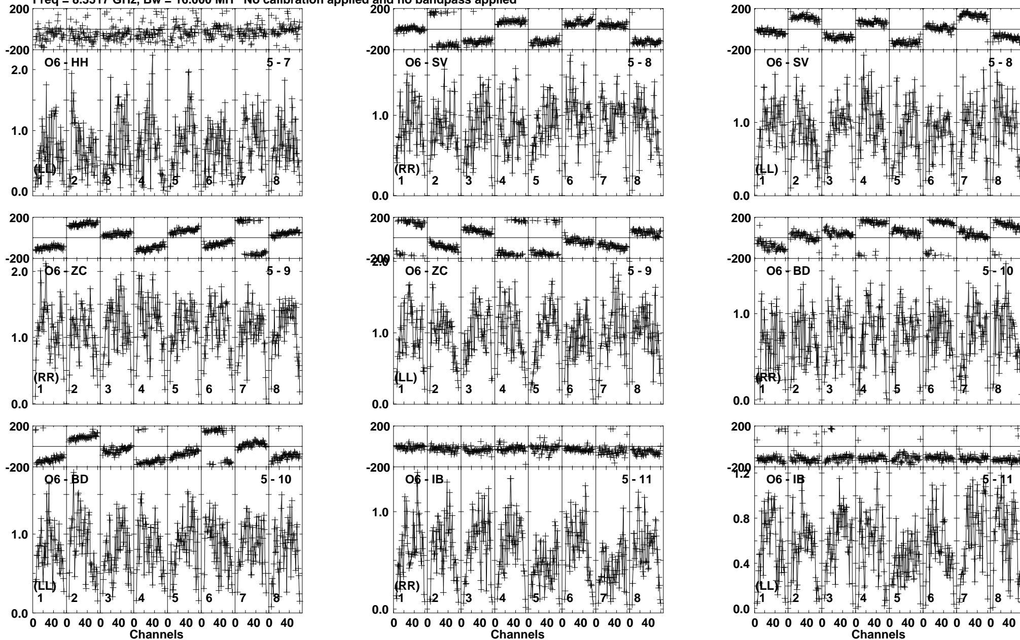
Lower frame: Milli Ampl Jy Top frame: Phas deg Vector averaged cross-power spectrum Baseline: O6 (05) - HH (07) Timerange: 00/01:31:35 to 00/01:32:20
