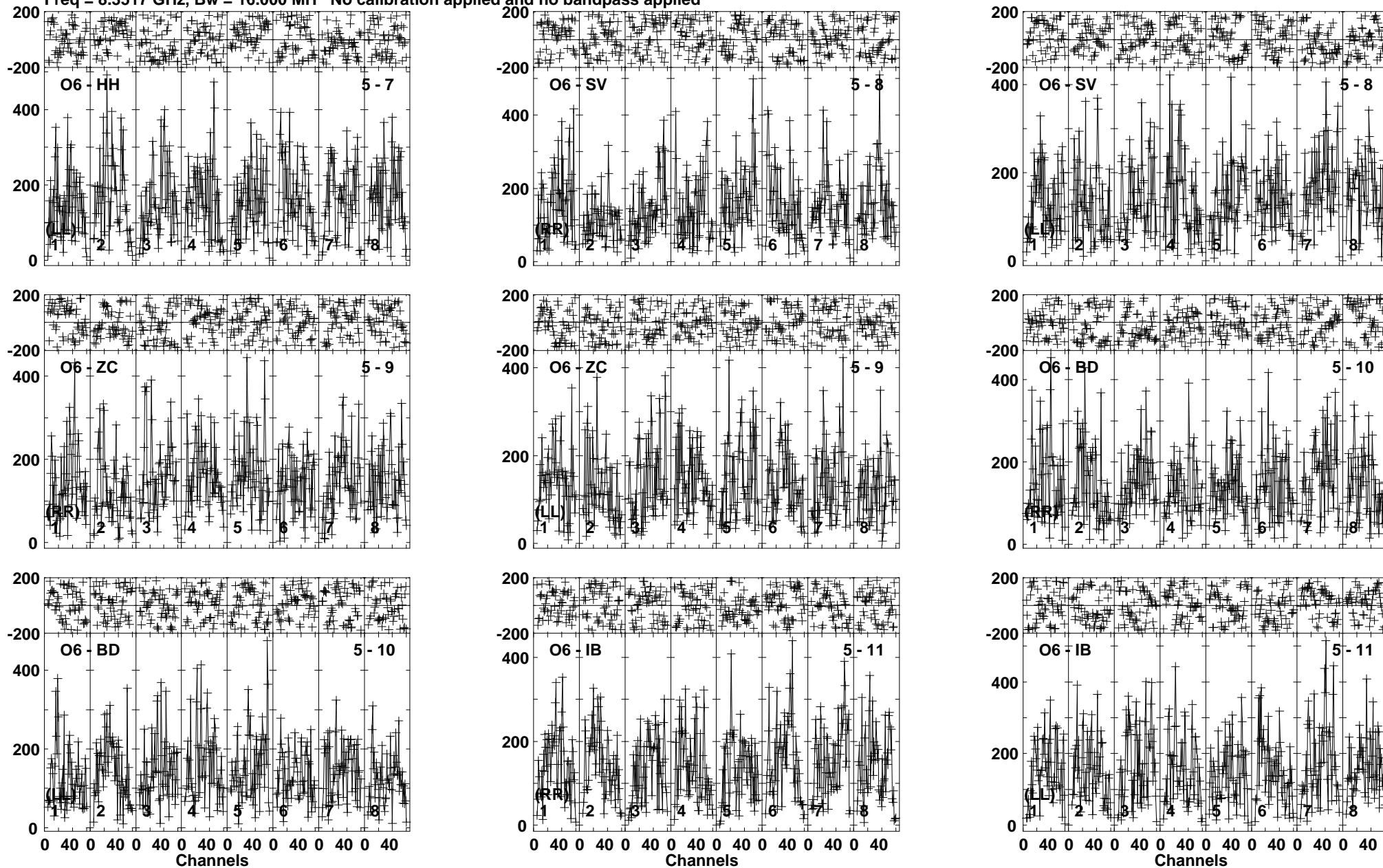
Lower frame: Micro Ampl Jy Top frame: Phas deg Vector averaged cross-power spectrum Baseline: O6 (05) - HH (07) Timerange: 00/04:36:26 to 00/04:38:40
