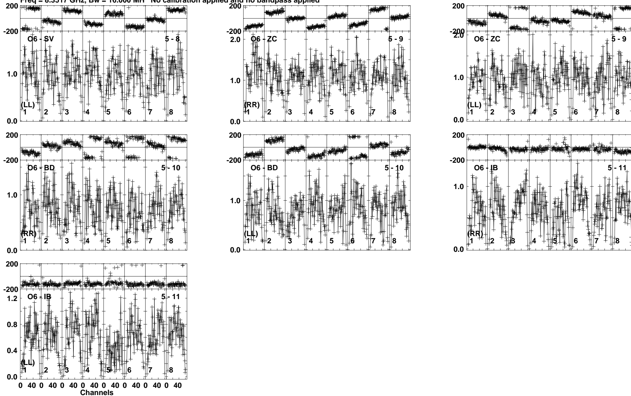
Lower frame: Milli Ampl Jy Top frame: Phas deg Vector averaged cross-power spectrum Baseline: O6 (05) - SV (08) Timerange: 00/03:06:15 to 00/03:06:59
