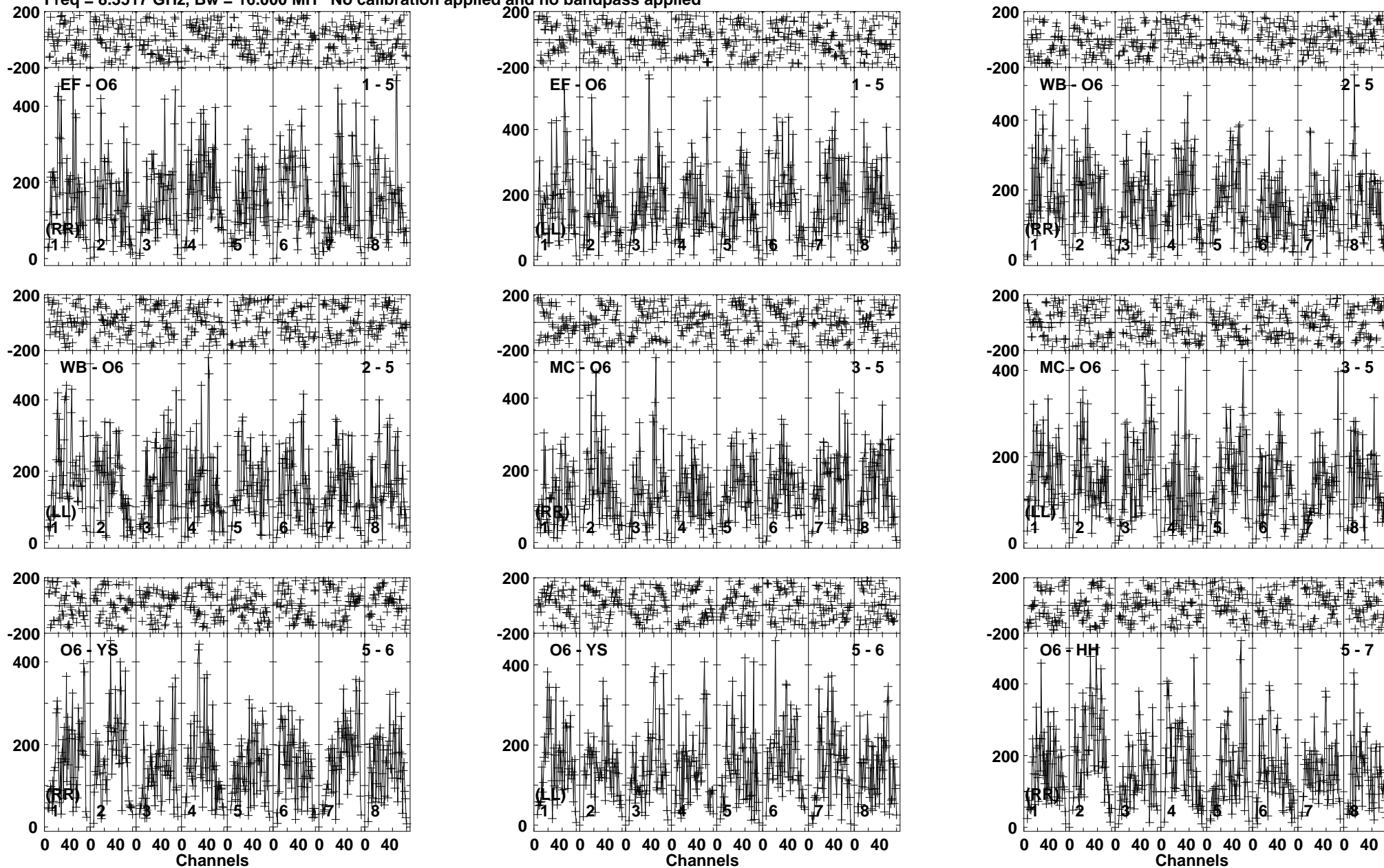
Lower frame: Micro Ampl Jy Top frame: Phas deg Vector averaged cross-power spectrum Baseline: EF (01) - O6 (05) Timerange: 00/06:08:07 to 00/06:10:20
