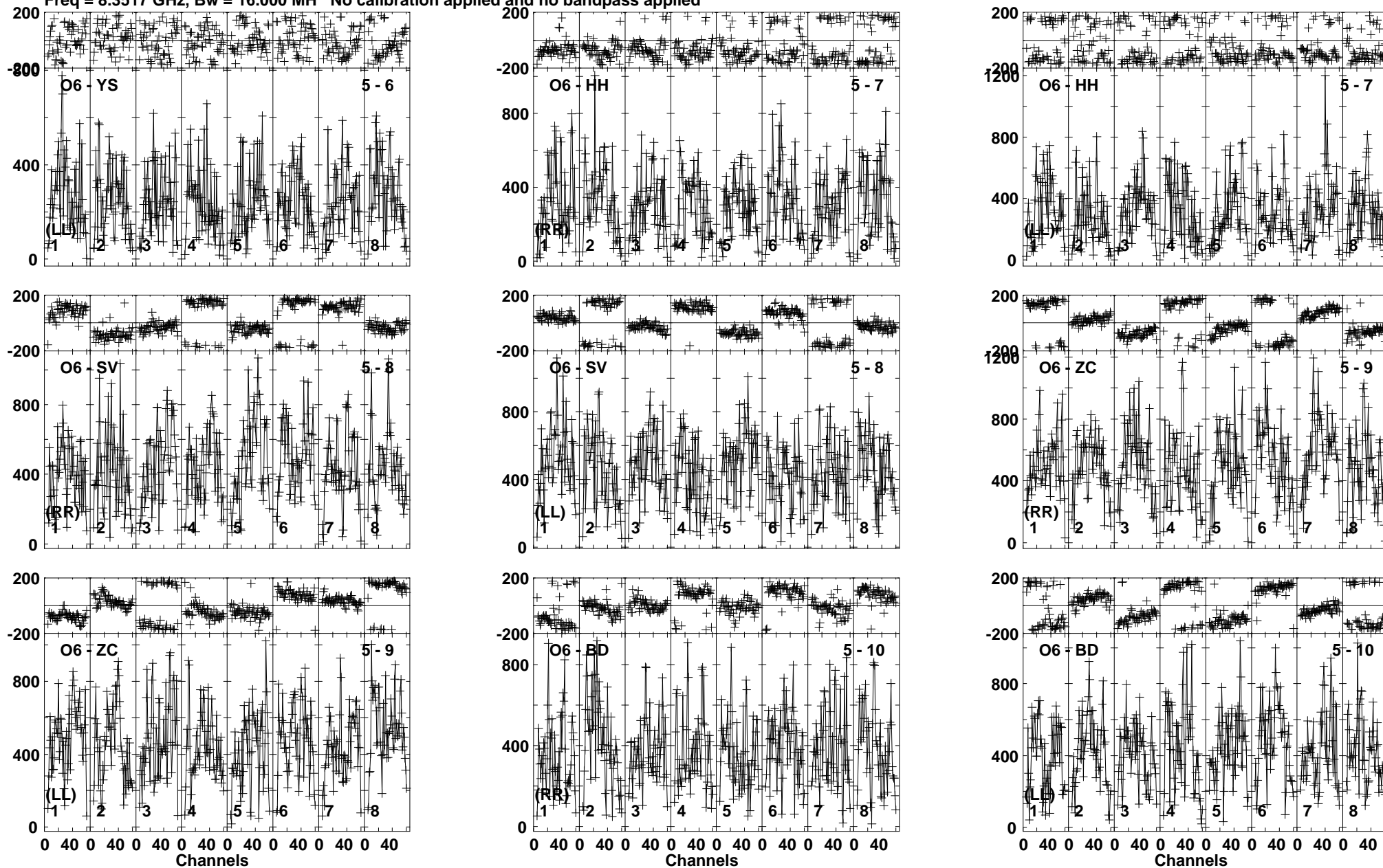
Lower frame: Micro Ampl Jy Top frame: Phas deg Vector averaged cross-power spectrum Baseline: O6 (05) - YS (06) Timerange: 00/02:02:30 to 00/02:03:15
