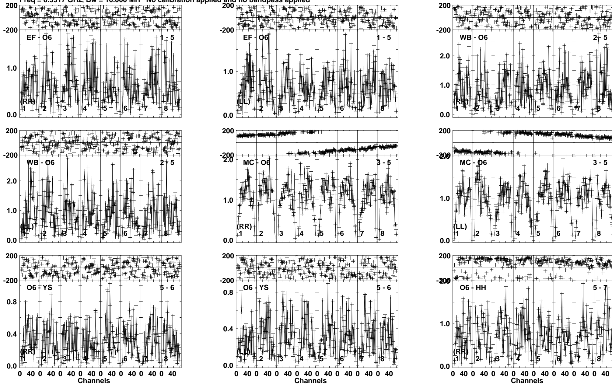
Lower frame: Milli Ampl Jy Top frame: Phas deg Vector averaged cross-power spectrum Baseline: EF (01) - O6 (05) Timerange: 00/06:16:05 to 00/06:16:49
