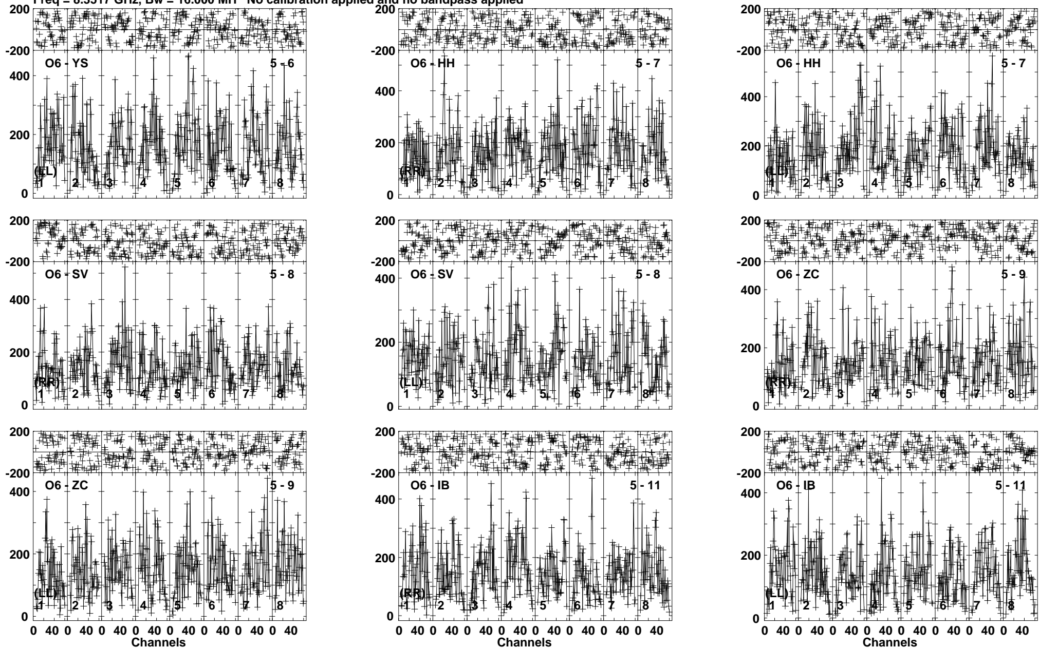
Lower frame: Micro Ampl Jy Top frame: Phas deg Vector averaged cross-power spectrum Baseline: O6 (05) - YS (06) Timerange: 00/06:23:15 to 00/06:25:29
