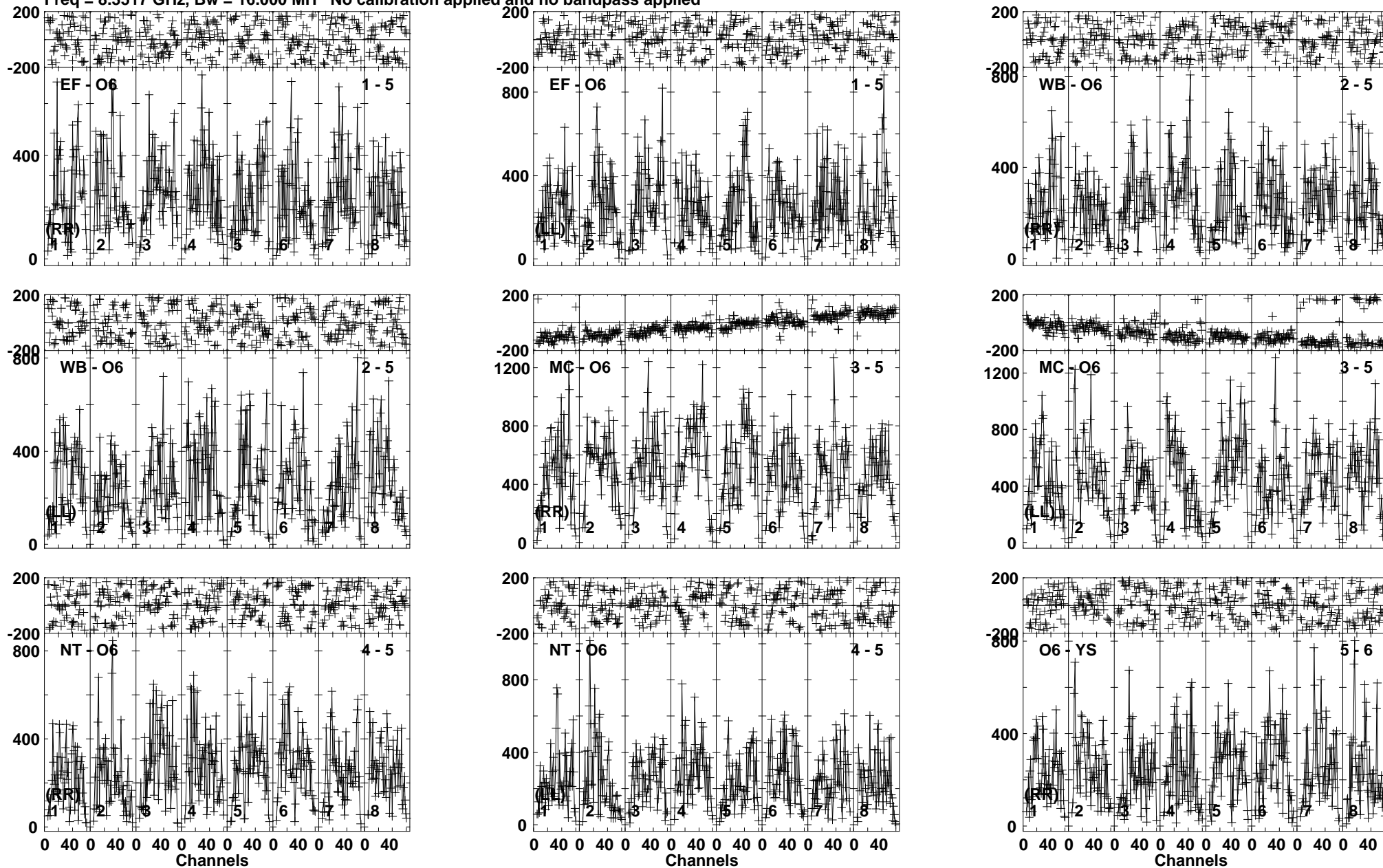
Lower frame: Micro Ampl Jy Top frame: Phas deg Vector averaged cross-power spectrum Baseline: EF (01) - O6 (05) Timerange: 00/03:42:55 to 00/03:43:40
