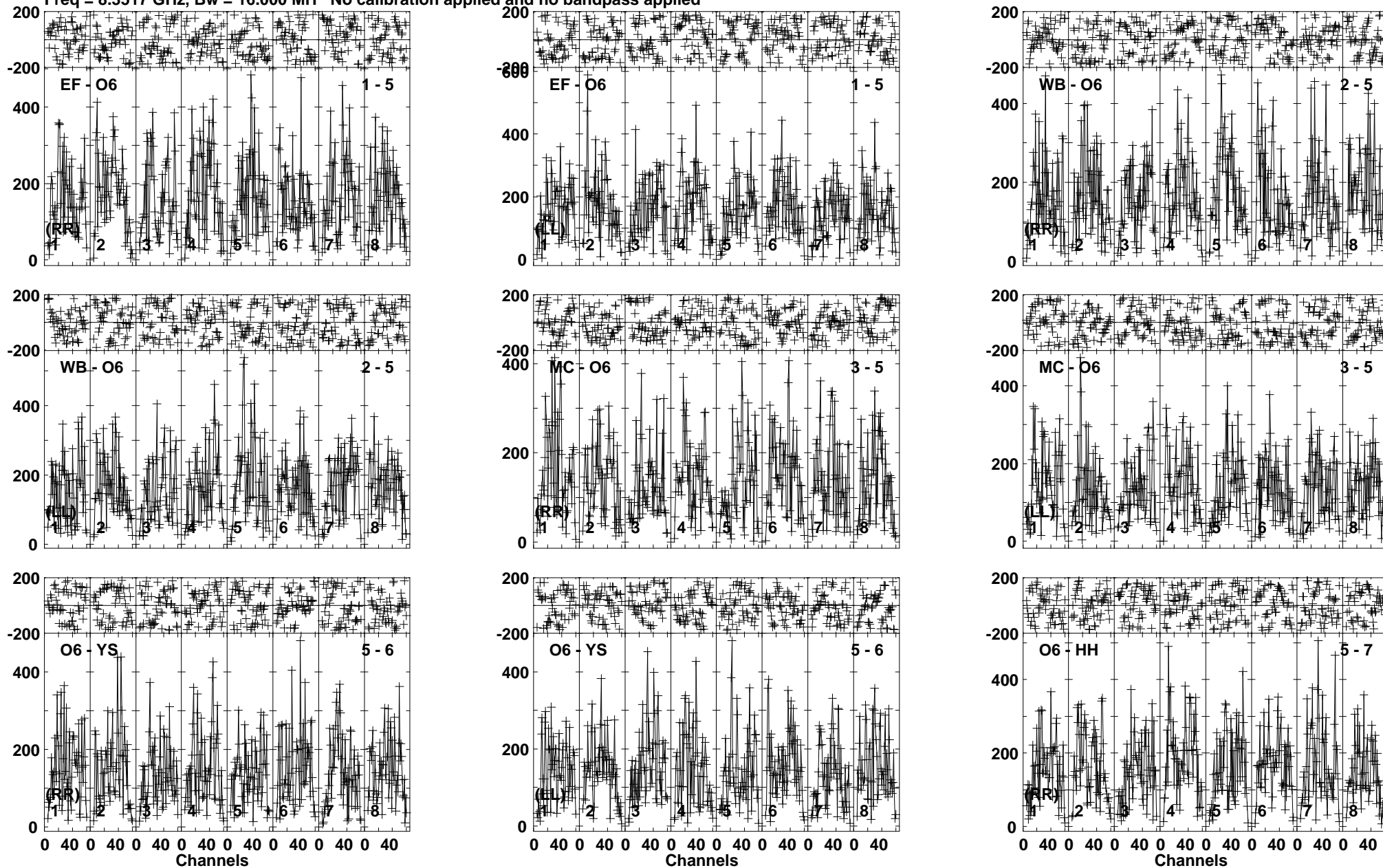
Lower frame: Micro Ampl Jy Top frame: Phas deg Vector averaged cross-power spectrum Baseline: EF (01) - O6 (05) Timerange: 00/02:52:41 to 00/02:54:54
