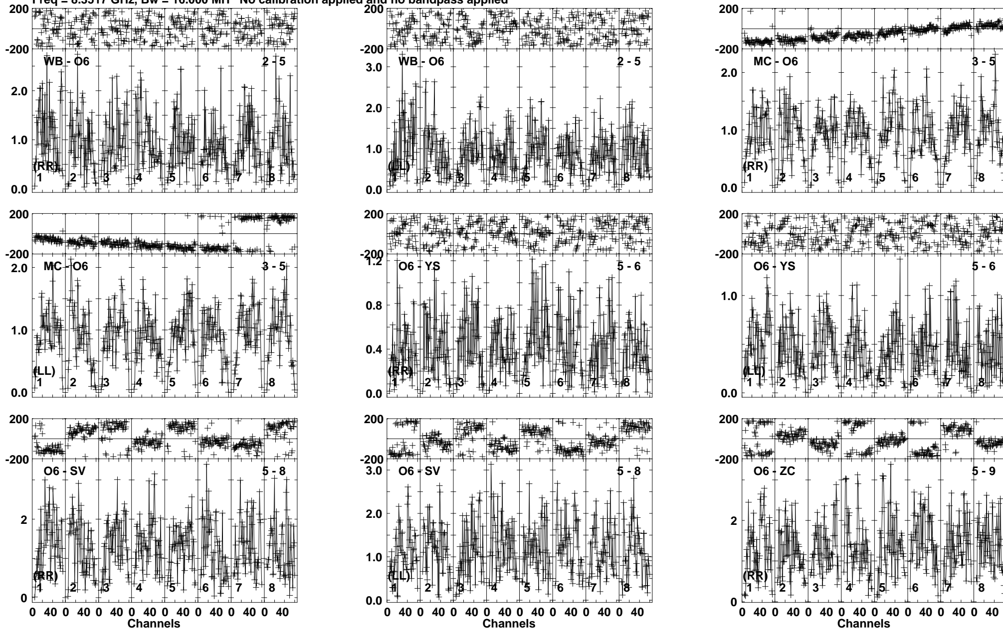
Lower frame: Milli Ampl Jy Top frame: Phas deg Vector averaged cross-power spectrum Baseline: WB (02) - O6 (05) Timerange: 00/02:09:02 to 00/02:09:30
