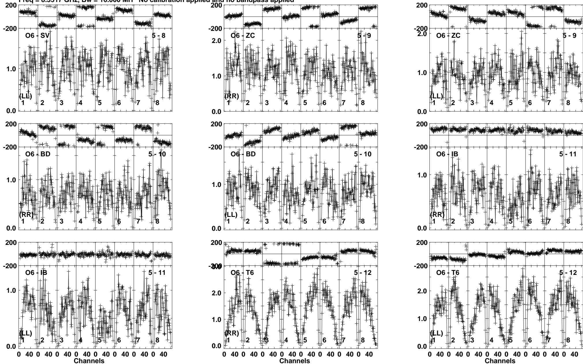
Lower frame: Milli Ampl Jy Top frame: Phas deg Vector averaged cross-power spectrum Baseline: O6 (05) - SV (08) Timerange: 00/03:26:20 to 00/03:27:04
