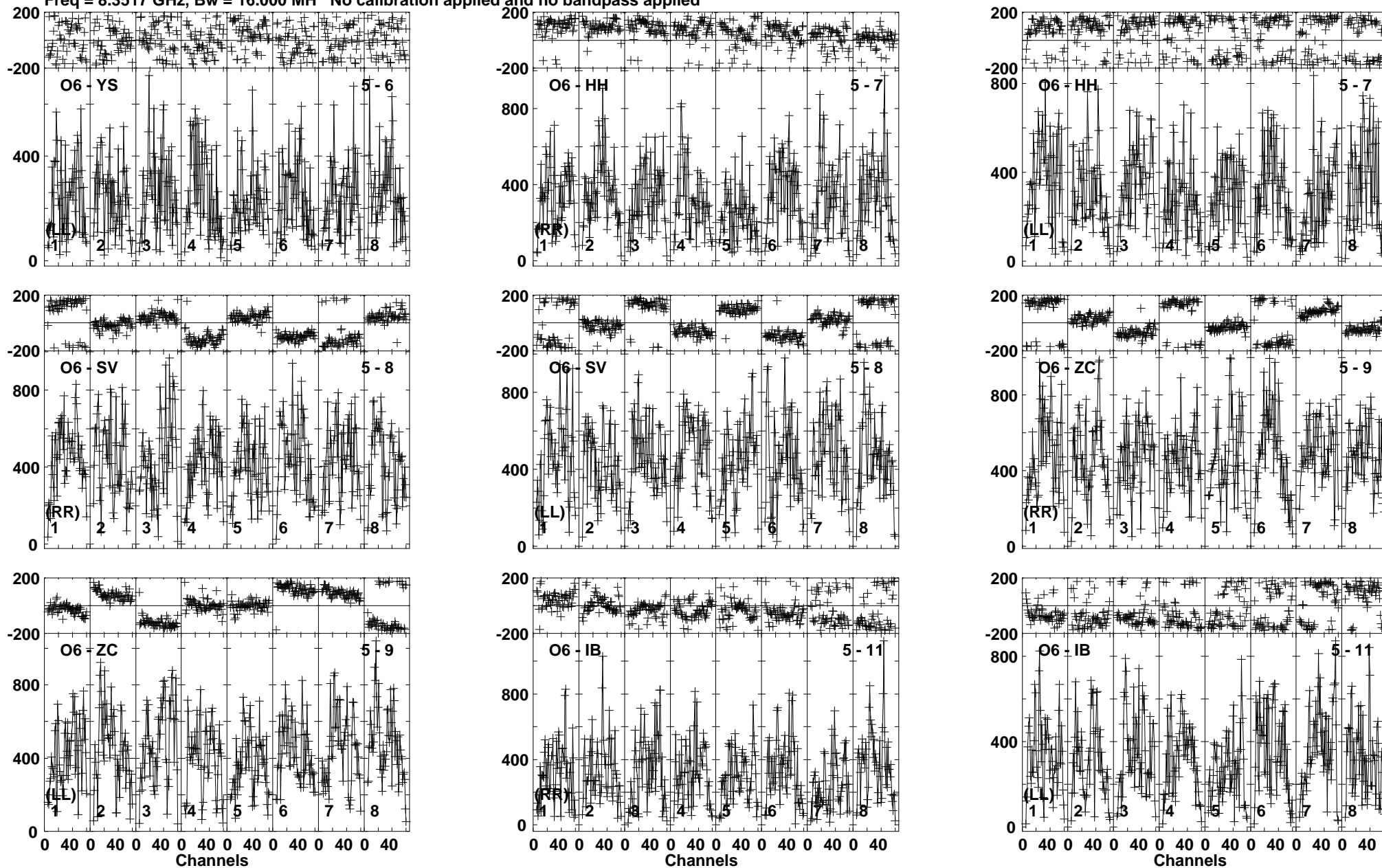
Lower frame: Micro Ampl Jy Top frame: Phas deg Vector averaged cross-power spectrum Baseline: O6 (05) - YS (06) Timerange: 00/08:07:21 to 00/08:08:05
