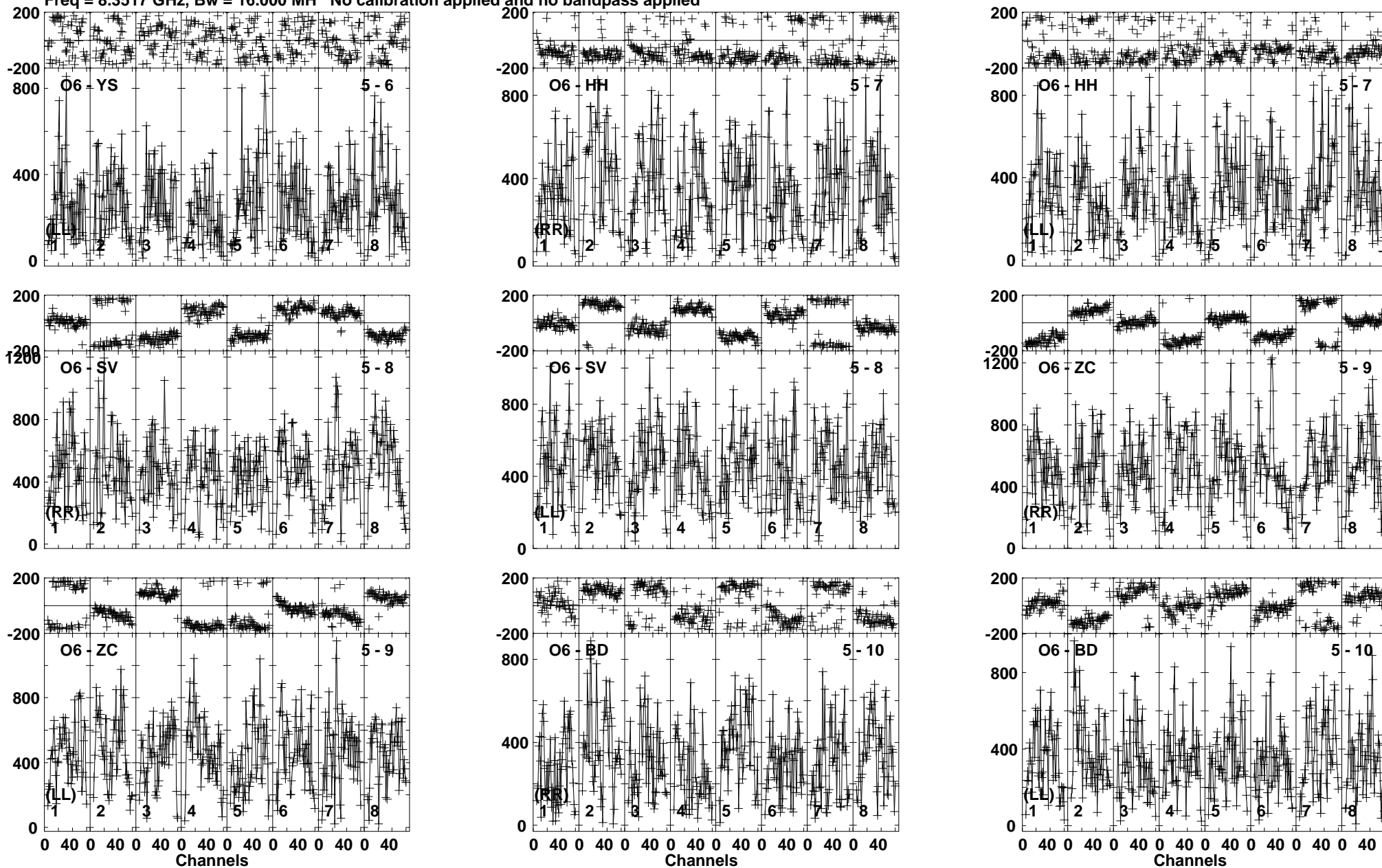
Lower frame: Micro Ampl Jy Top frame: Phas deg Vector averaged cross-power spectrum Baseline: O6 (05) - YS (06) Timerange: 00/05:06:35 to 00/05:07:19
