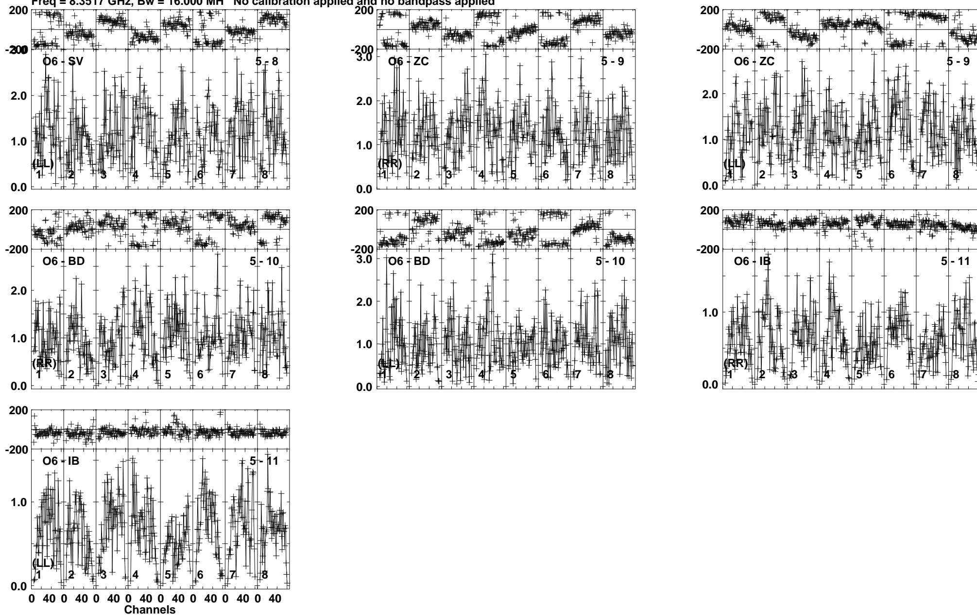
Lower frame: Milli Ampl Jy Top frame: Phas deg Vector averaged cross-power spectrum Baseline: O6 (05) - SV (08) Timerange: 00/01:43:10 to 00/01:43:40
