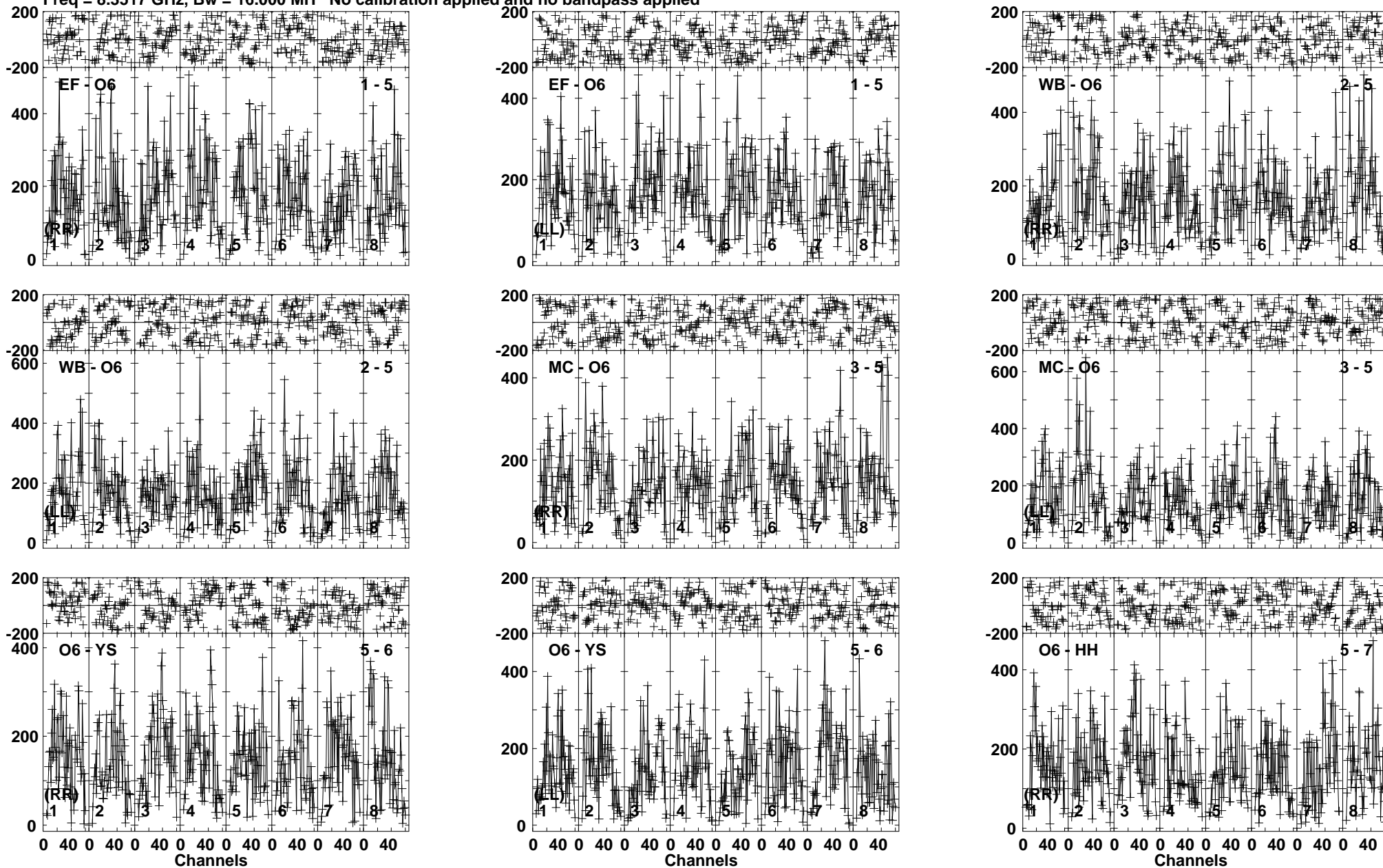
Lower frame: Micro Ampl Jy Top frame: Phas deg Vector averaged cross-power spectrum Baseline: EF (01) - O6 (05) Timerange: 00/07:31:26 to 00/07:33:39
