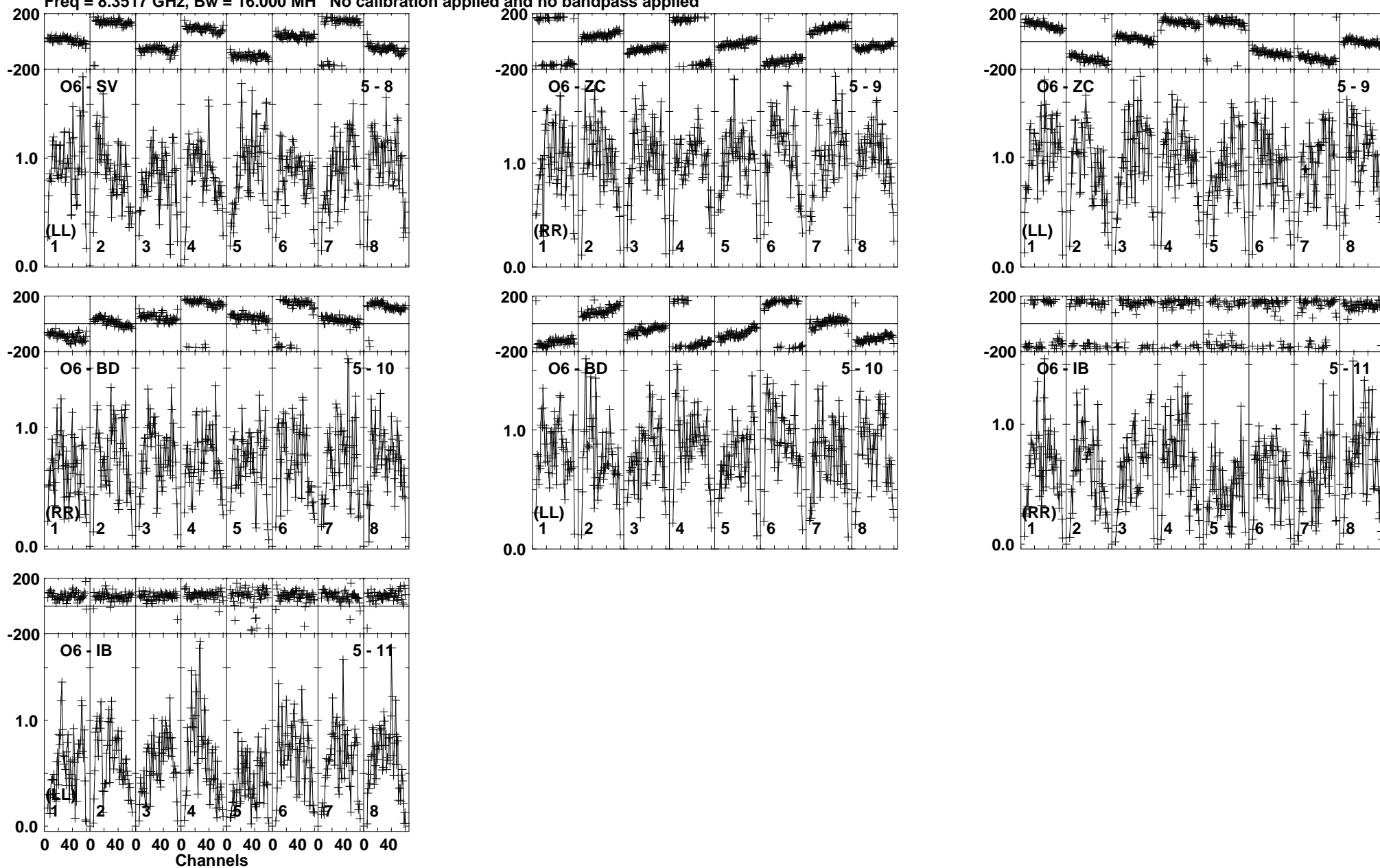
Lower frame: Milli Ampl Jy Top frame: Phas deg Vector averaged cross-power spectrum Baseline: O6 (05) - SV (08) Timerange: 00/01:15:11 to 00/01:15:40
