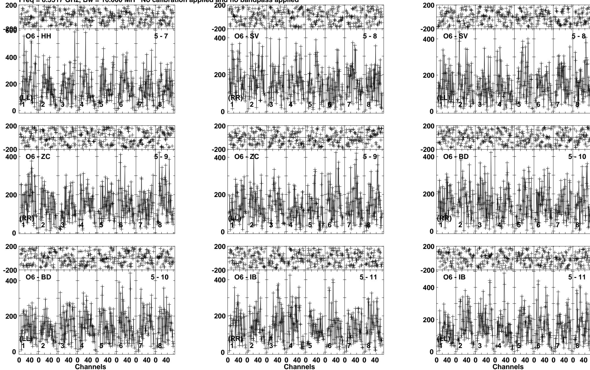
Lower frame: Micro Ampl Jy Top frame: Phas deg Vector averaged cross-power spectrum Baseline: O6 (05) - HH (07) Timerange: 00/05:13:37 to 00/05:15:50
