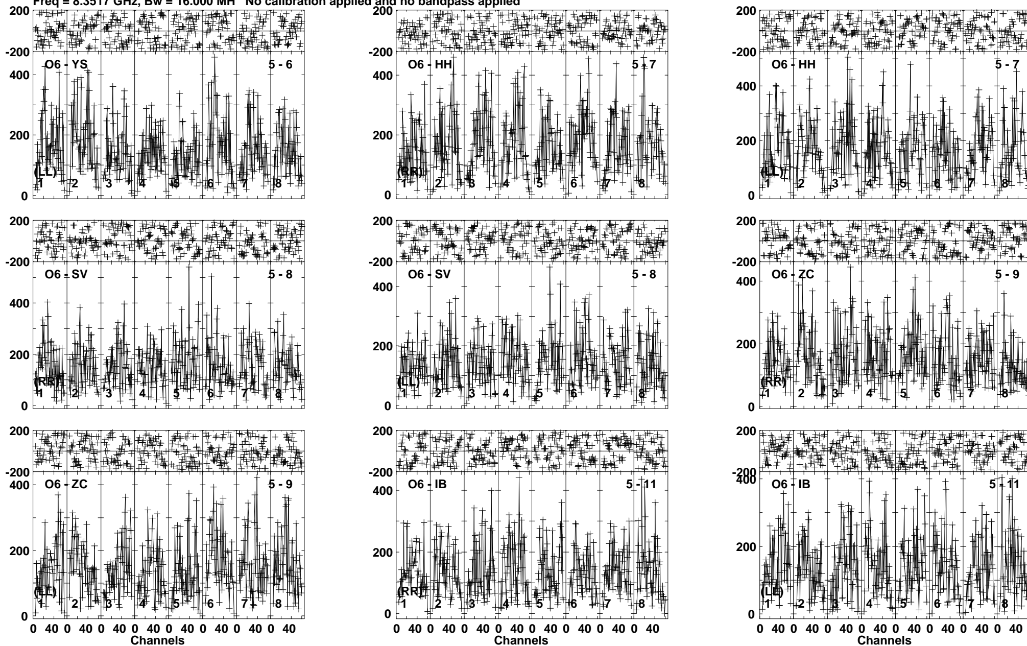
Lower frame: Micro Ampl Jy Top frame: Phas deg Vector averaged cross-power spectrum Baseline: O6 (05) - YS (06) Timerange: 00/06:40:21 to 00/06:42:34
