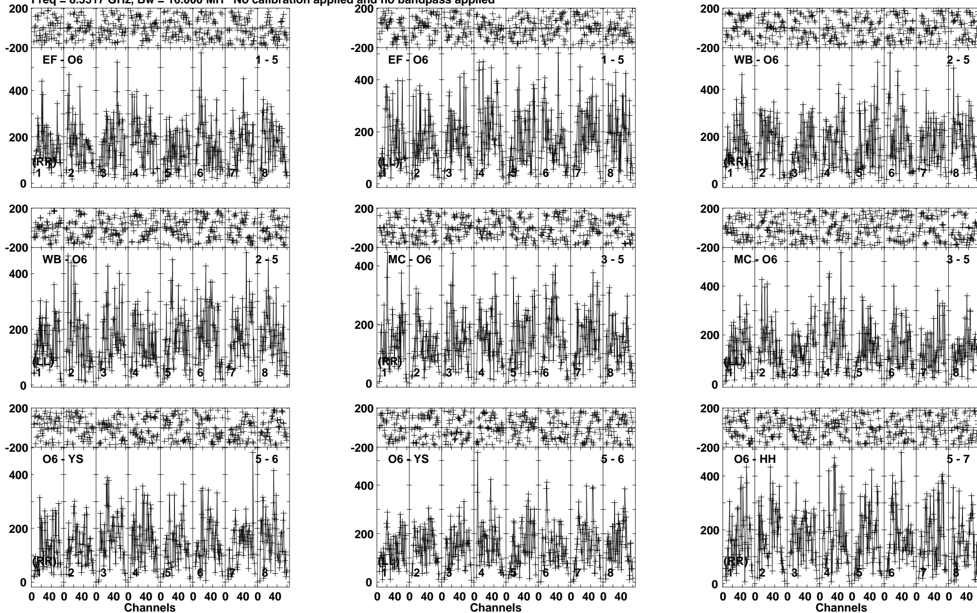
Lower frame: Micro Ampl Jy Top frame: Phas deg Vector averaged cross-power spectrum Baseline: EF (01) - O6 (05) Timerange: 00/06:31:10 to 00/06:33:24
