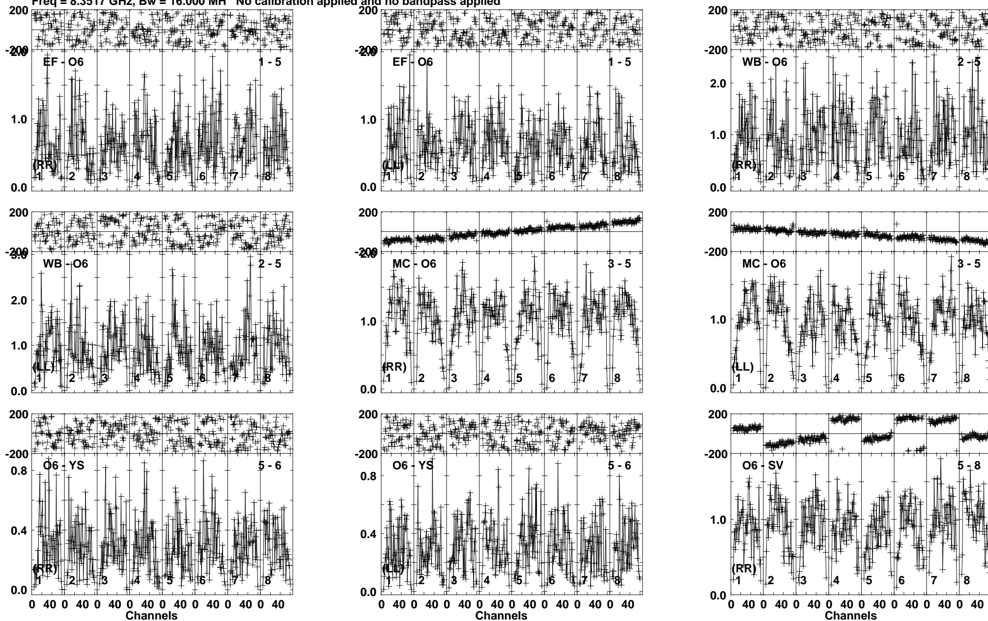
Lower frame: Milli Ampl Jy Top frame: Phas deg Vector averaged cross-power spectrum Baseline: EF (01) - O6 (05) Timerange: 00/08:02:56 to 00/08:03:39
