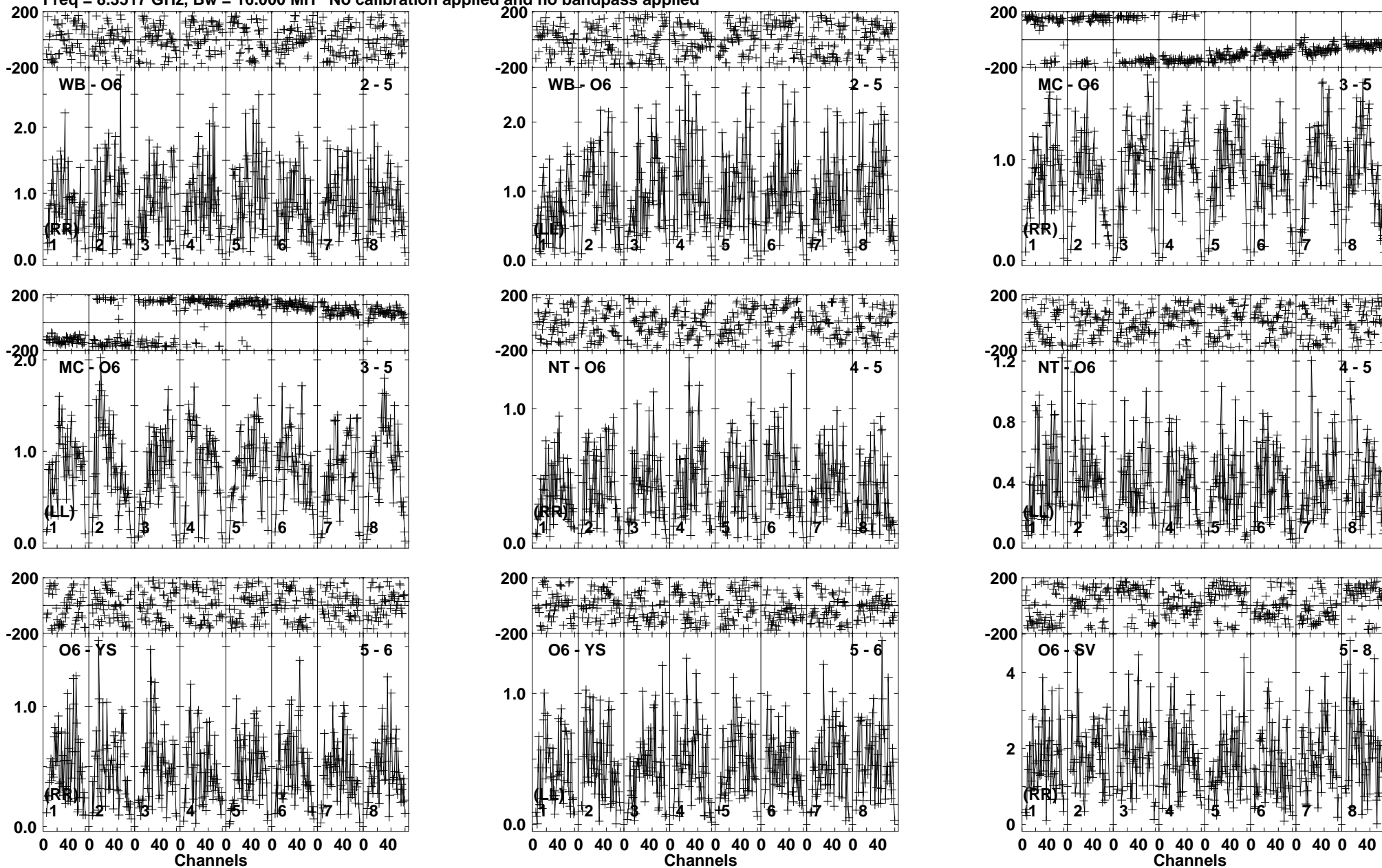
Lower frame: Milli Ampl Jy Top frame: Phas deg Vector averaged cross-power spectrum Baseline: WB (02) - O6 (05) Timerange: 00/01:23:06 to 00/01:23:35
