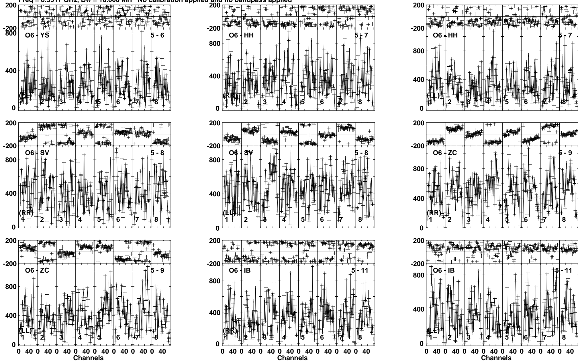
Lower frame: Micro Ampl Jy Top frame: Phas deg Vector averaged cross-power spectrum Baseline: O6 (05) - YS (06) Timerange: 00/07:07:06 to 00/07:07:50
