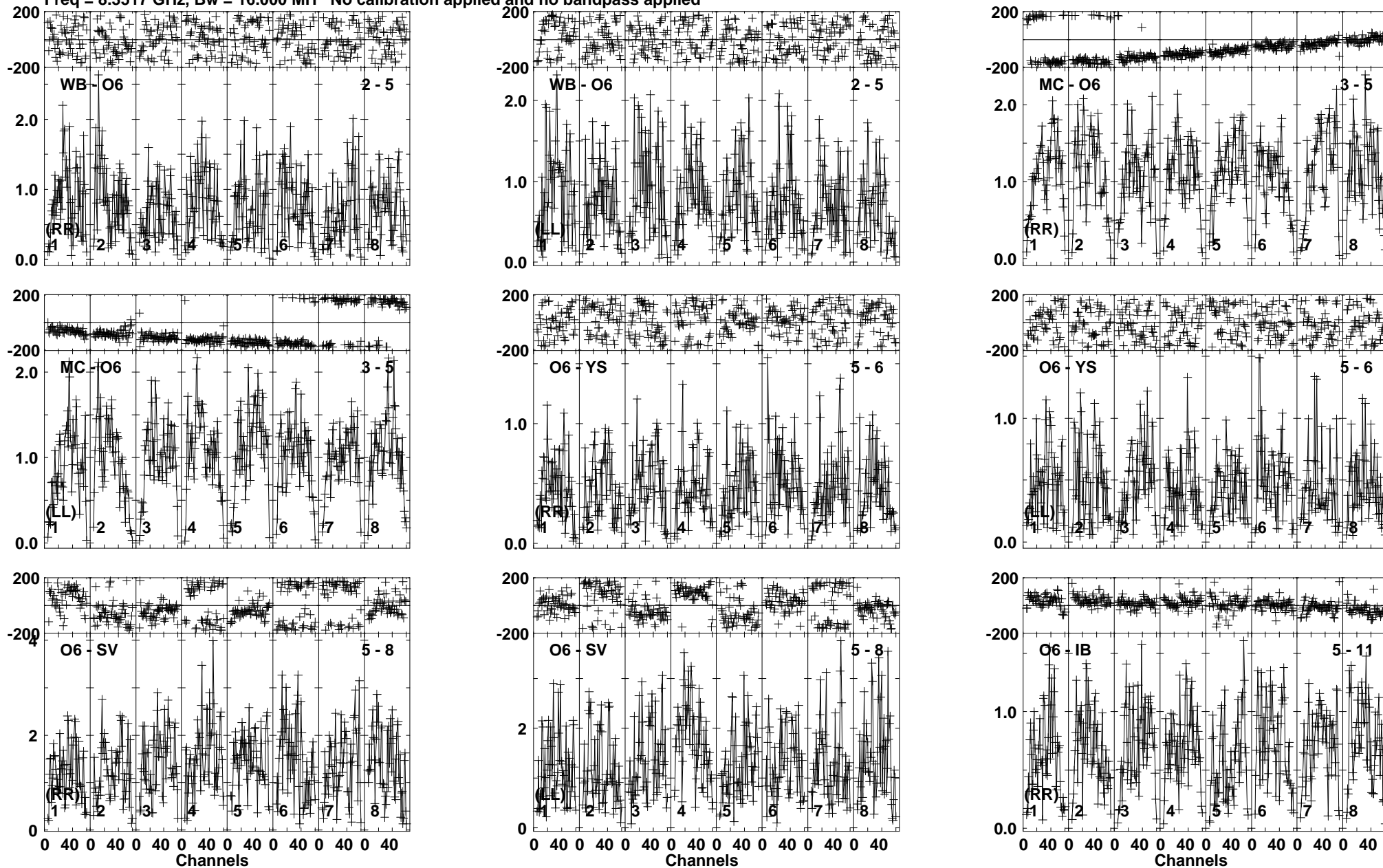
Lower frame: Milli Ampl Jy Top frame: Phas deg Vector averaged cross-power spectrum Baseline: WB (02) - O6 (05) Timerange: 00/06:27:40 to 00/06:28:10
