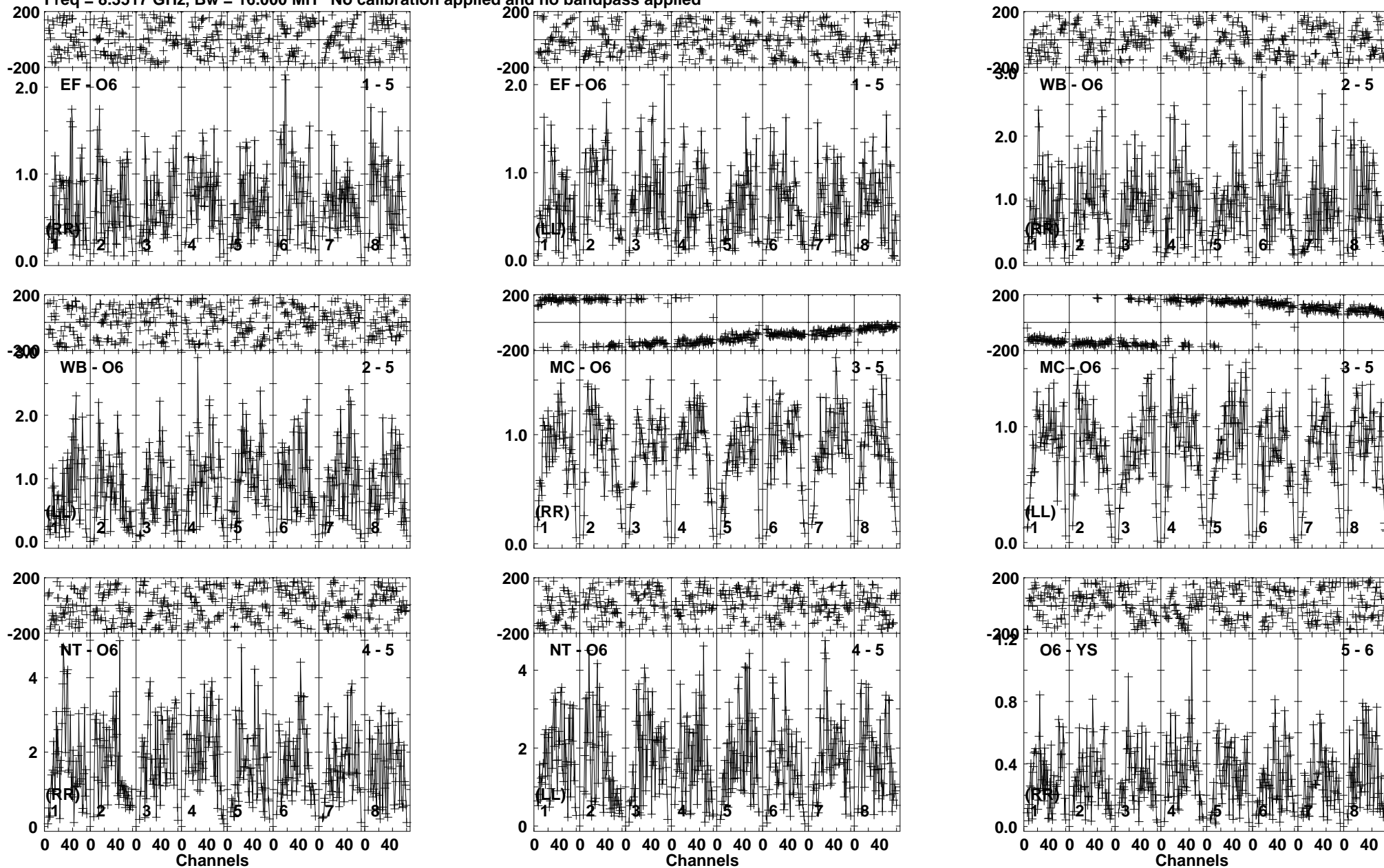
Lower frame: Milli Ampl Jy Top frame: Phas deg Vector averaged cross-power spectrum Baseline: EF (01) - O6 (05) Timerange: 00/01:45:56 to 00/01:46:40
