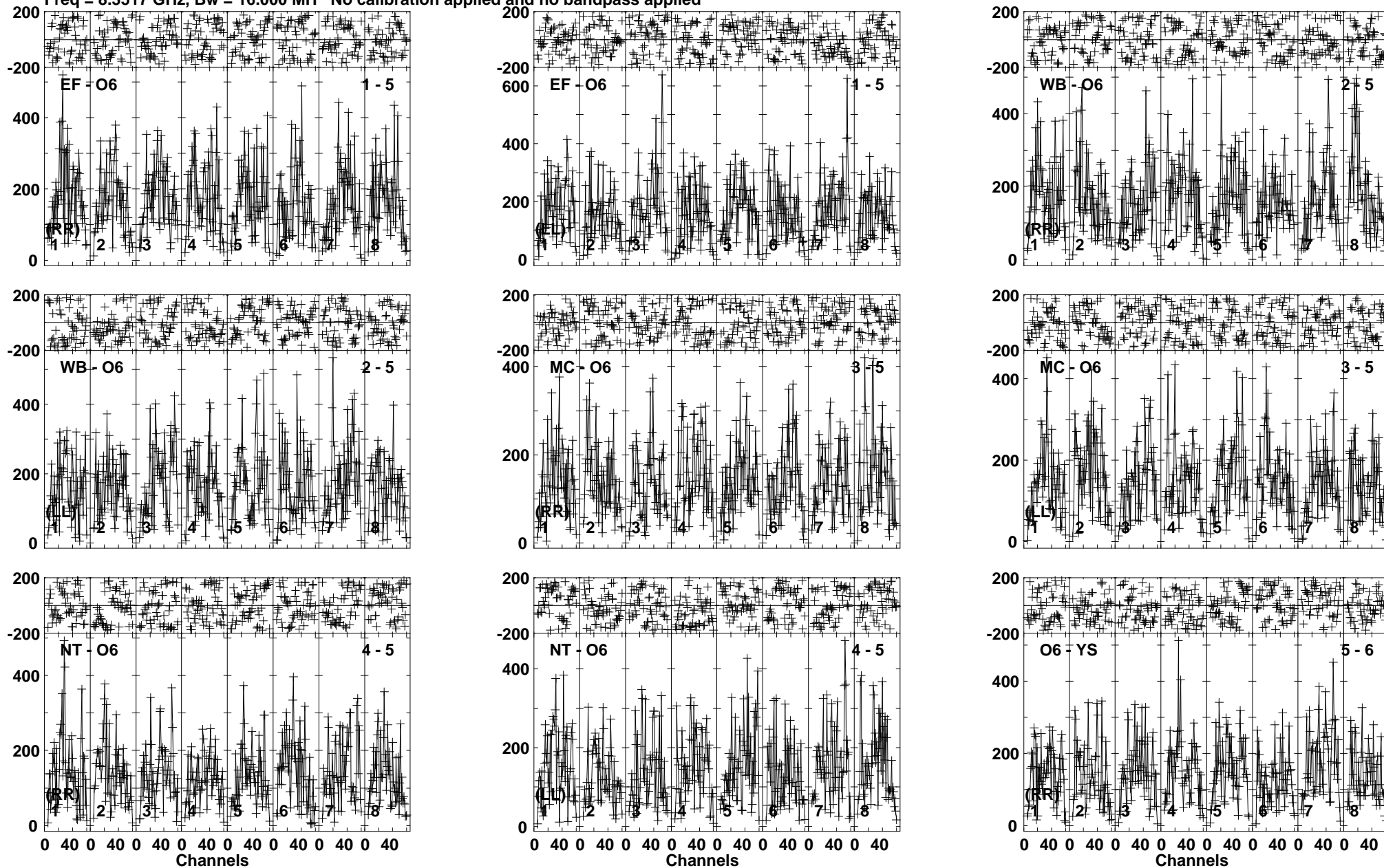
Lower frame: Micro Ampl Jy Top frame: Phas deg Vector averaged cross-power spectrum Baseline: EF (01) - O6 (05) Timerange: 00/01:43:42 to 00/01:45:54
