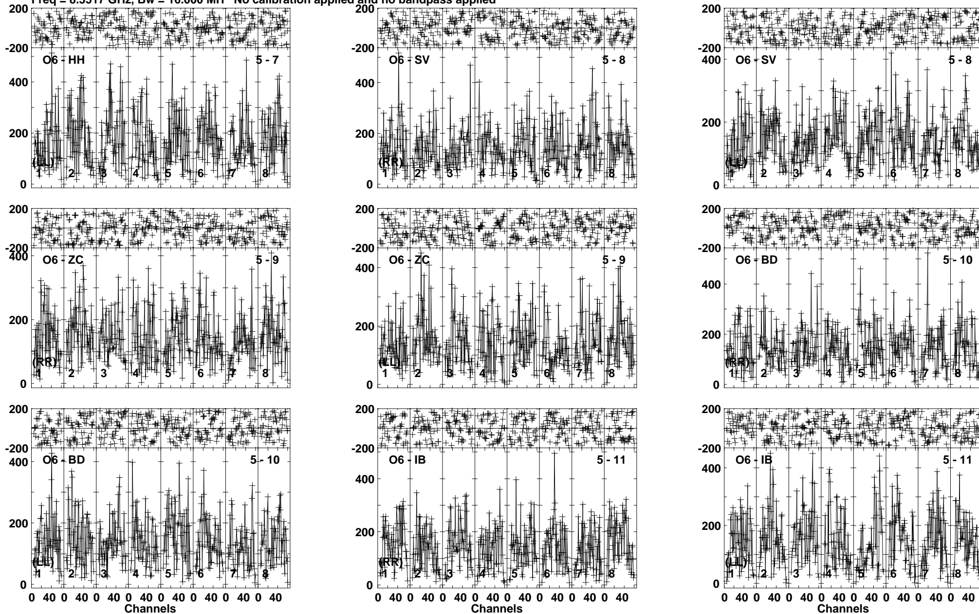
Lower frame: Micro Ampl Jy Top frame: Phas deg Vector averaged cross-power spectrum Baseline: O6 (05) - HH (07) Timerange: 00/01:49:26 to 00/01:51:39
