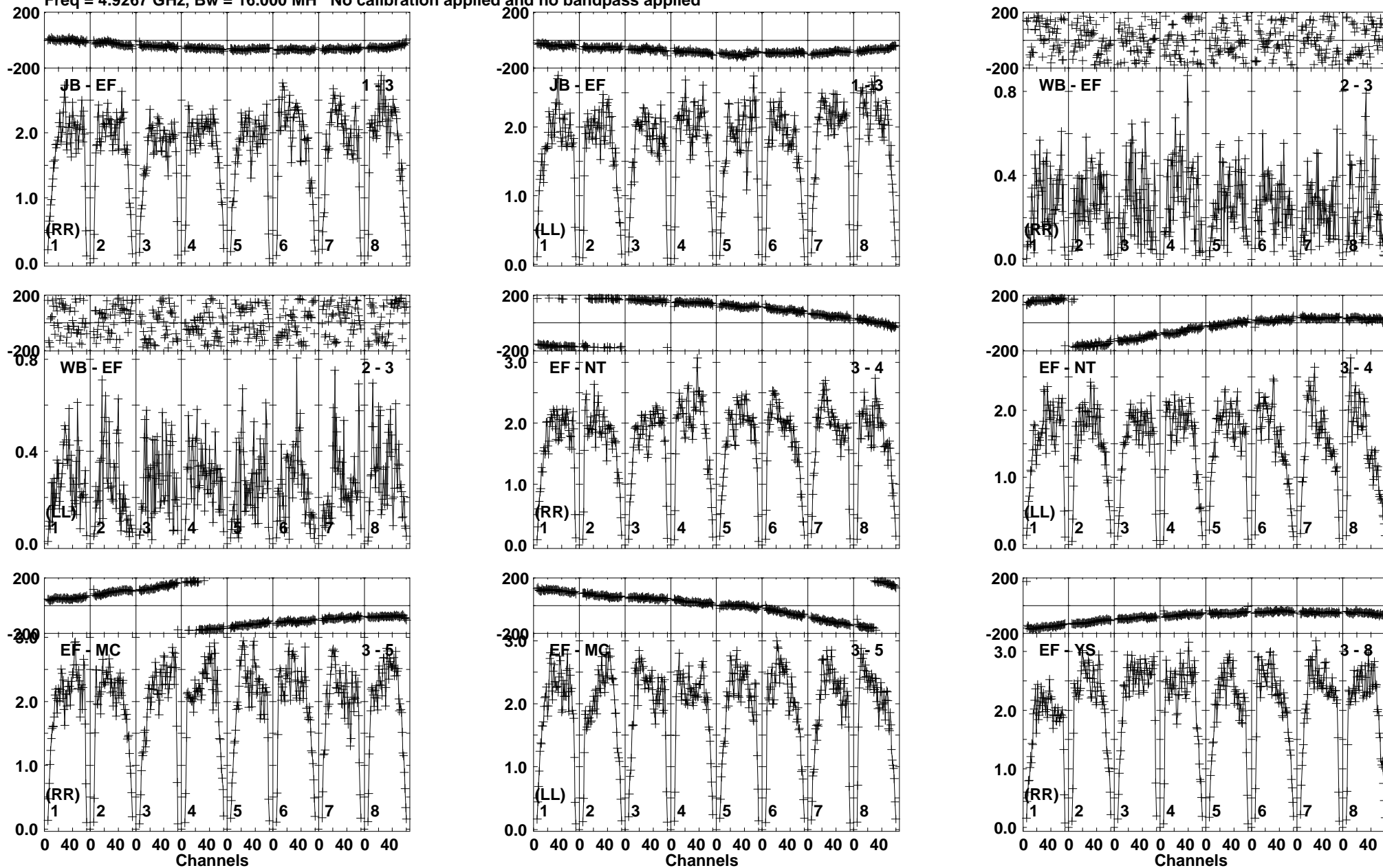
Lower frame: Milli Ampl Jy Top frame: Phas deg Vector averaged cross-power spectrum Baseline: JB (01) - EF (03) Timerange: 00:16:10:40 to 00:16:12:10
