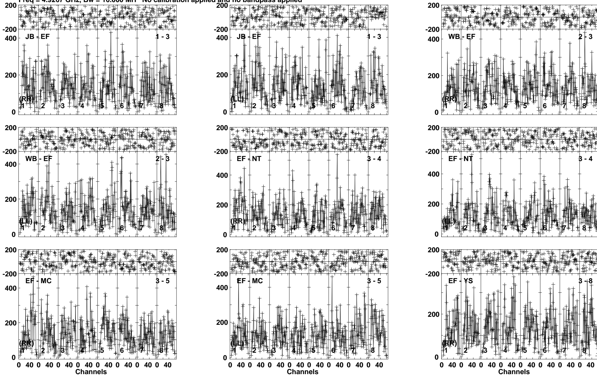
Lower frame: Micro Ampl Jy Top frame: Phas deg Vector averaged cross-power spectrum Baseline: JB (01) - EF (03) Timerange: 00/14:06:40 to 00/14:09:40
