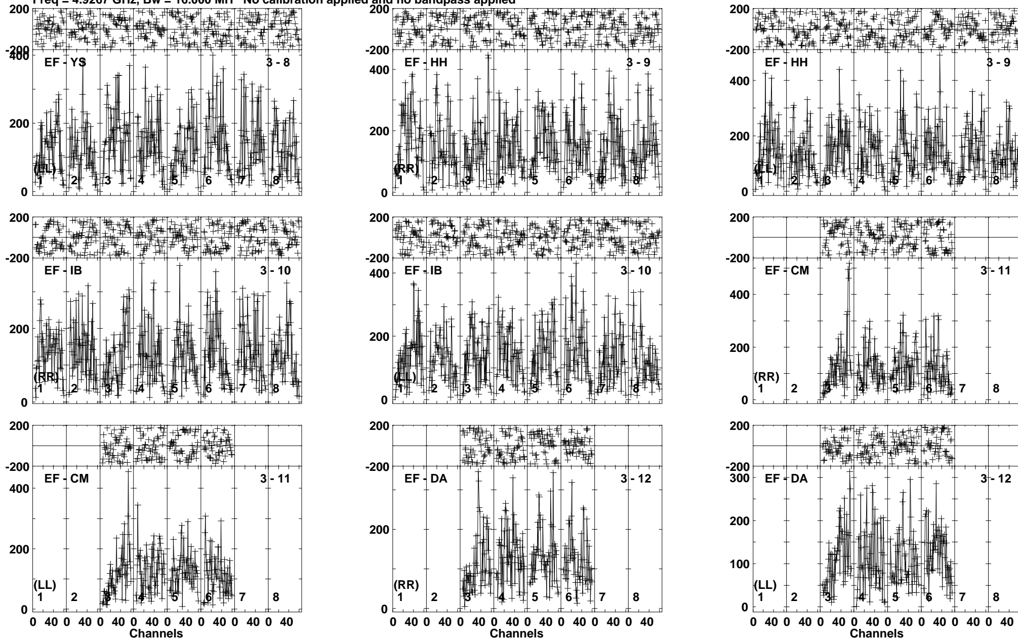
Lower frame: Micro Ampl Jy Top frame: Phas deg Vector averaged cross-power spectrum Baseline: EF (03) - YS (08) Timerange: 00/14:06:40 to 00/14:09:40
