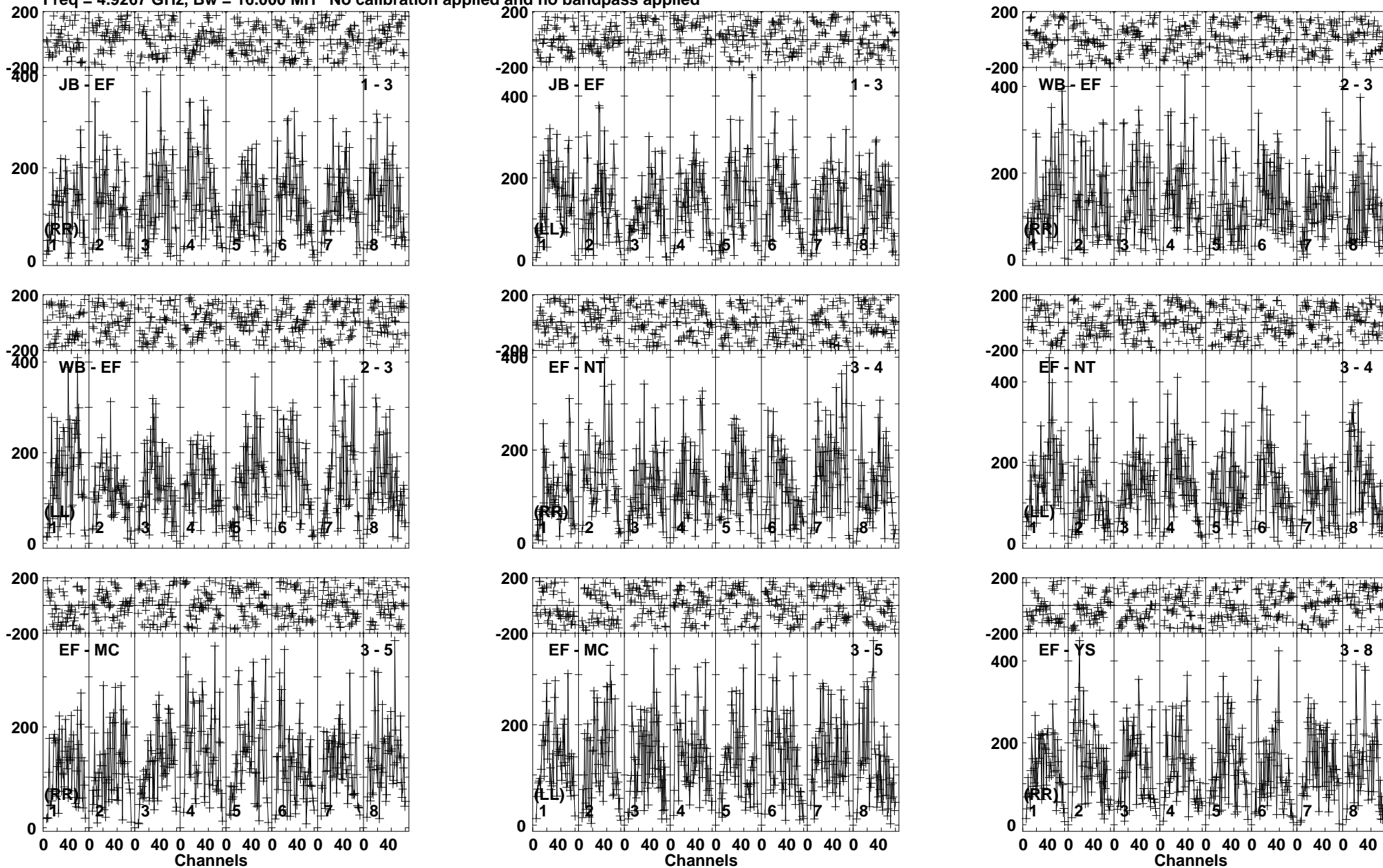
Lower frame: Micro Ampl Jy Top frame: Phas deg Vector averaged cross-power spectrum Baseline: JB (01) - EF (03) Timerange: 00/14:44:51 to 00/14:47:49
