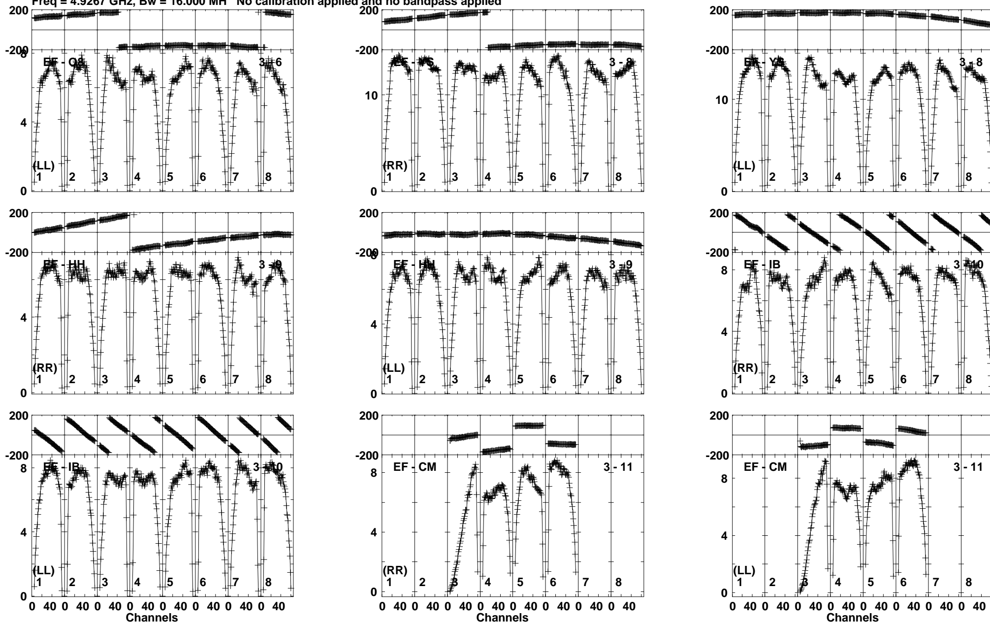
Lower frame: Milli Ampl Jy Top frame: Phas deg Vector averaged cross-power spectrum Baseline: EF (03) - O8 (06) Timerange: 01/09:29:41 to 01/09:30:40
