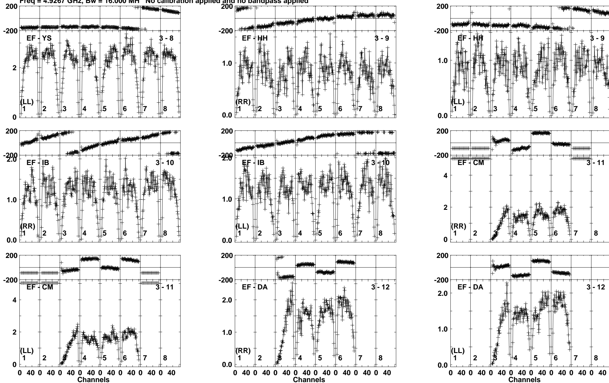
Lower frame: Milli Ampl Jy Top frame: Phas deg Vector averaged cross-power spectrum Baseline: EF (03) - YS (08) Timerange: 00:16:16:50 to 00:16:18:19
