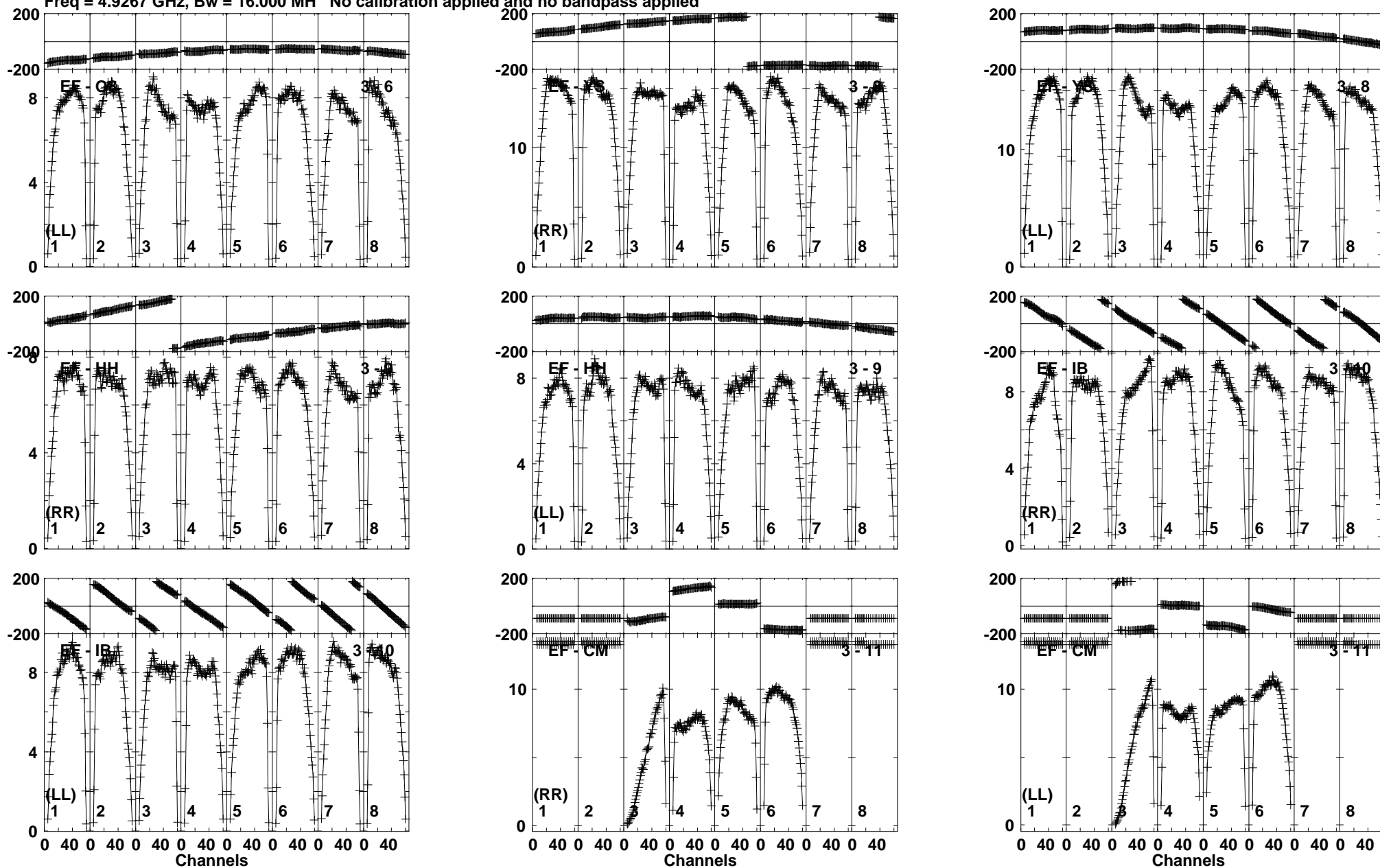
Lower frame: Milli Amply Jy Top frame: Phas deg Vector averaged cross-power spectrum Baseline: EF (03) - O8 (06) Timerange: 01/12:22:30 to 01/12:23:29
