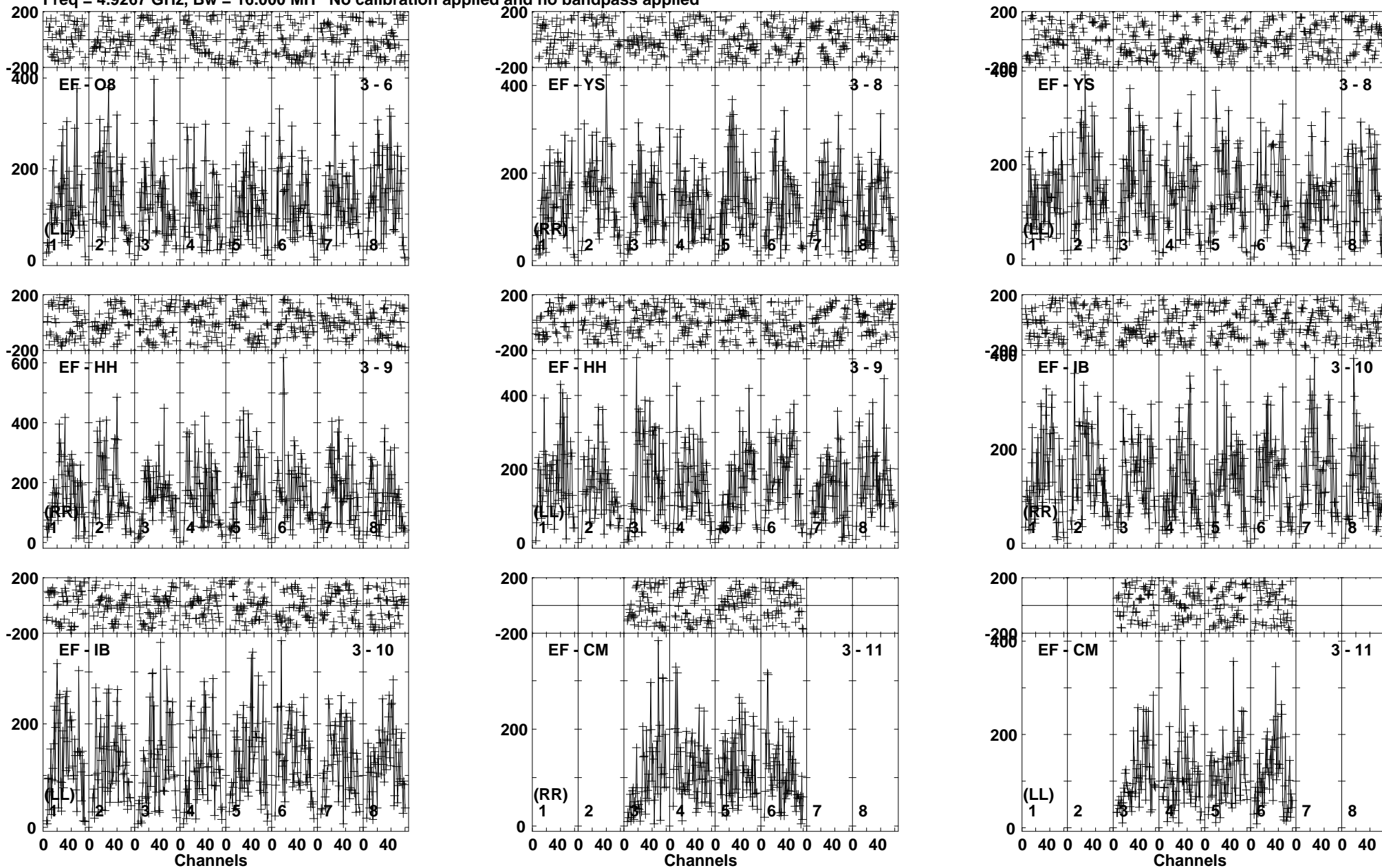
Lower frame: Micro Ampl Jy Top frame: Phas deg Vector averaged cross-power spectrum Baseline: EF (03) - O8 (06) Timerange: 01/12:18:50 to 01/12:21:50
