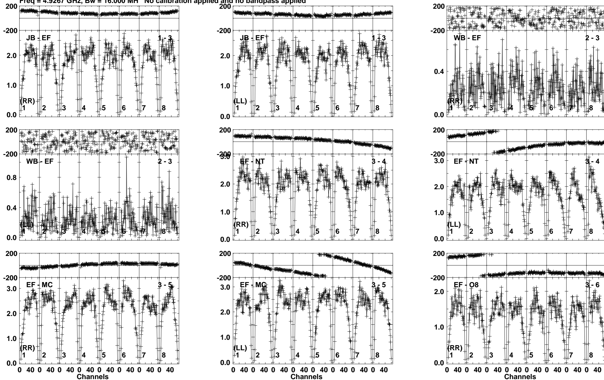
Lower frame: Milli Ampl Jy Top frame: Phas deg Vector averaged cross-power spectrum Baseline: JB (01) - EF (03) Timerange: 01/12:02:10 to 01/12:03:40
