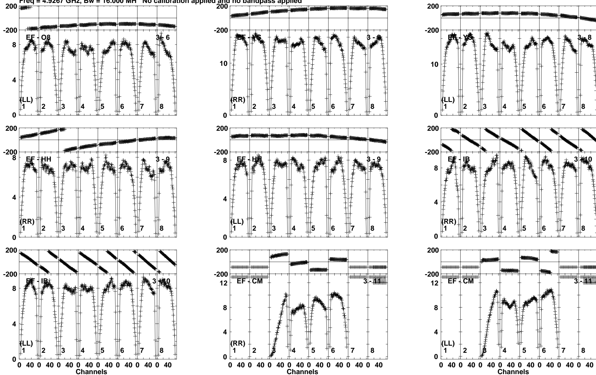
Lower frame: Milli Ampl Jy Top frame: Phas deg Vector averaged cross-power spectrum Baseline: EF (03) - O8 (06) Timerange: 01/12:01:11 to 01/12:02:09
