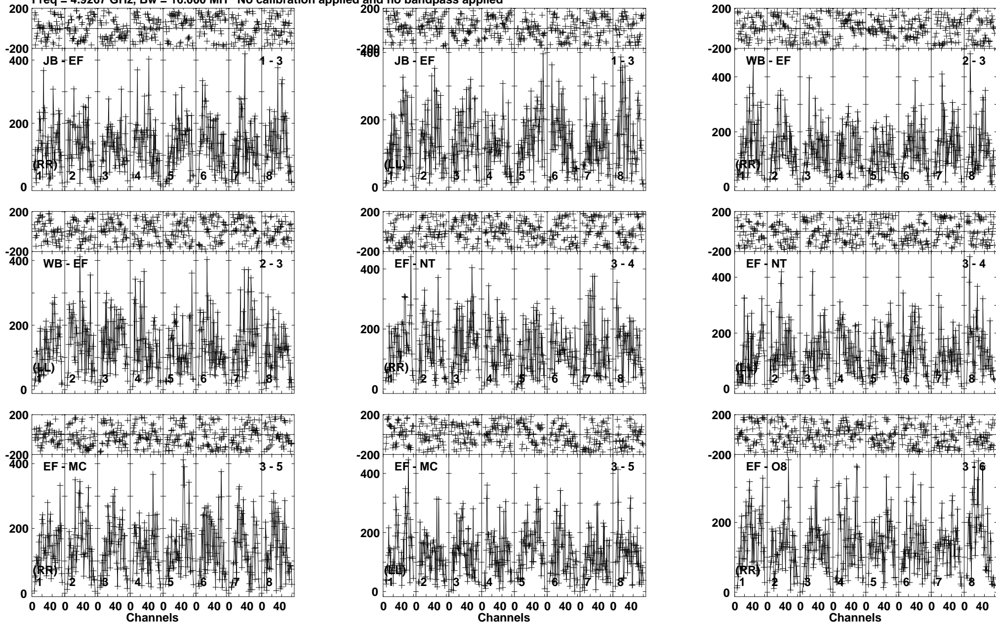
Lower frame: Micro Ampl Jy Top frame: Phas deg Vector averaged cross-power spectrum Baseline: JB (01) - EF (03) Timerange: 01/11:53:00 to 01/11:56:00
