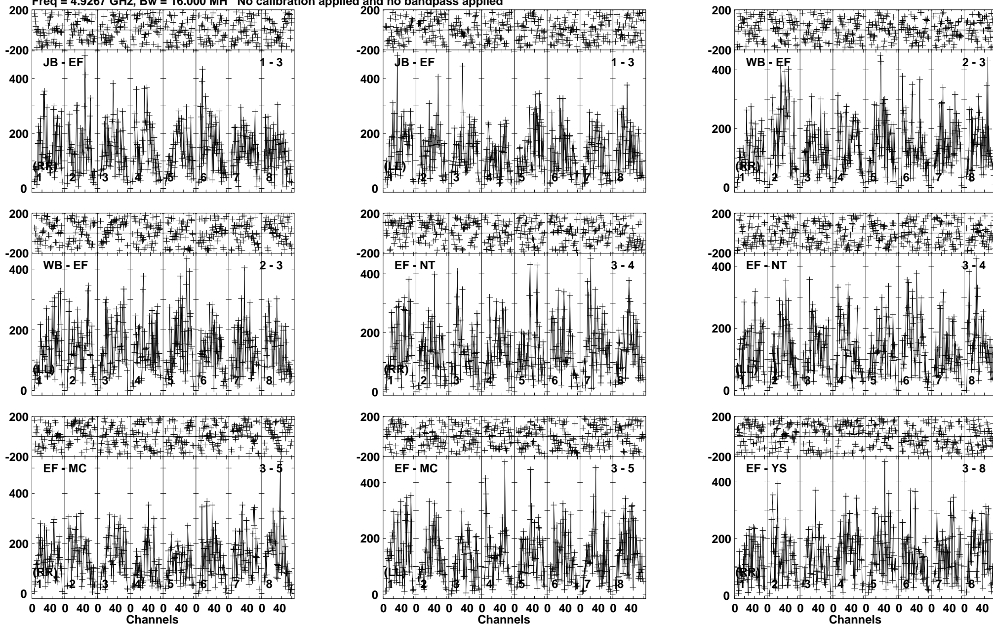
Lower frame: Micro Ampl Jy Top frame: Phas deg Vector averaged cross-power spectrum Baseline: JB (01) - EF (03) Timerange: 00/16:18:21 to 00/16:21:20
