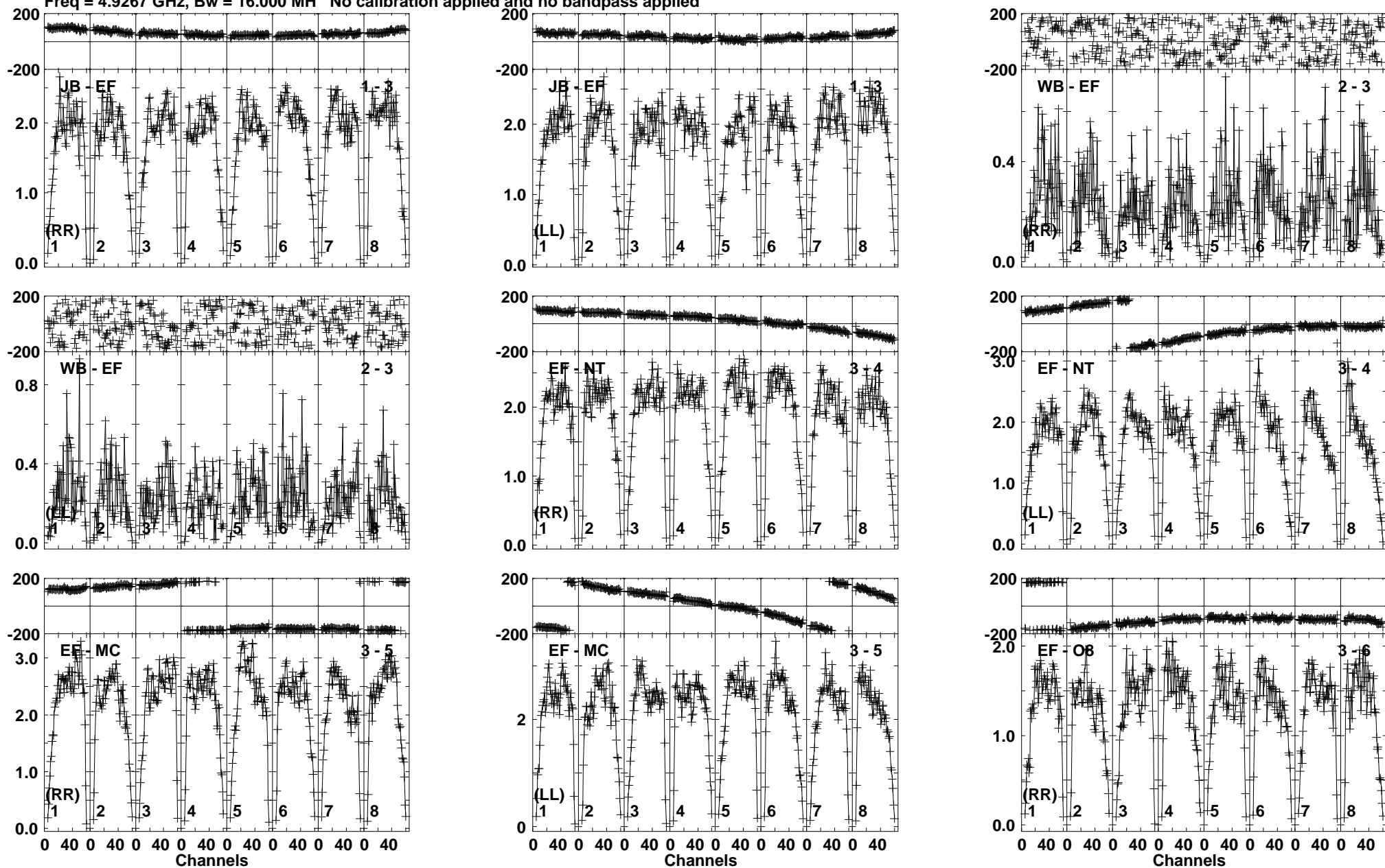
Lower frame: Milli Ampl Jy Top frame: Phas deg Vector averaged cross-power spectrum Baseline: JB (01) - EF (03) Timerange: 01/11:40:50 to 01/11:42:20
