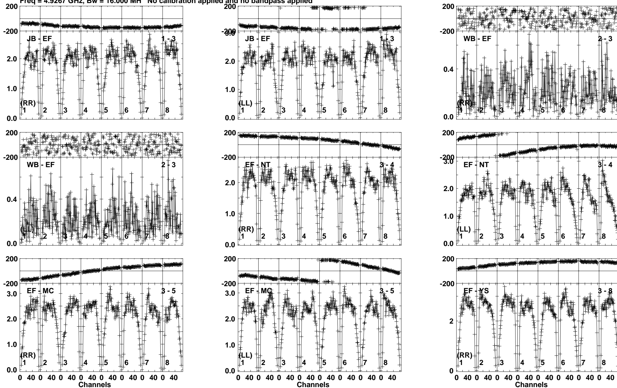
Lower frame: Milli Ampl Jy Top frame: Phas deg Vector averaged cross-power spectrum Baseline: JB (01) - EF (03) Timerange: 00/14:47:51 to 00/14:49:19
