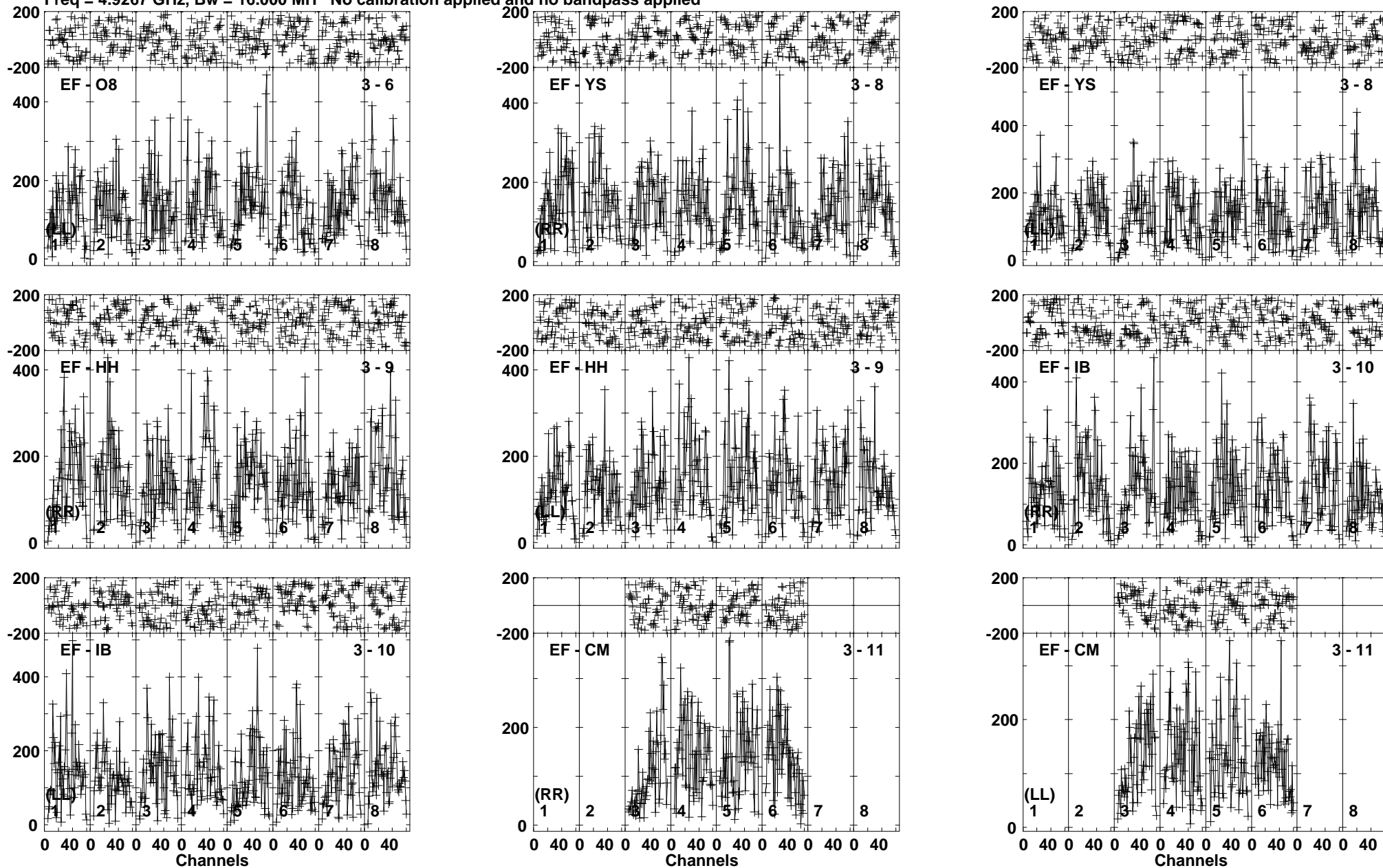
Lower frame: Micro Ampl Jy Top frame: Phas deg Vector averaged cross-power spectrum Baseline: EF (03) - O8 (06) Timerange: 01/12:03:40 to 01/12:06:40
