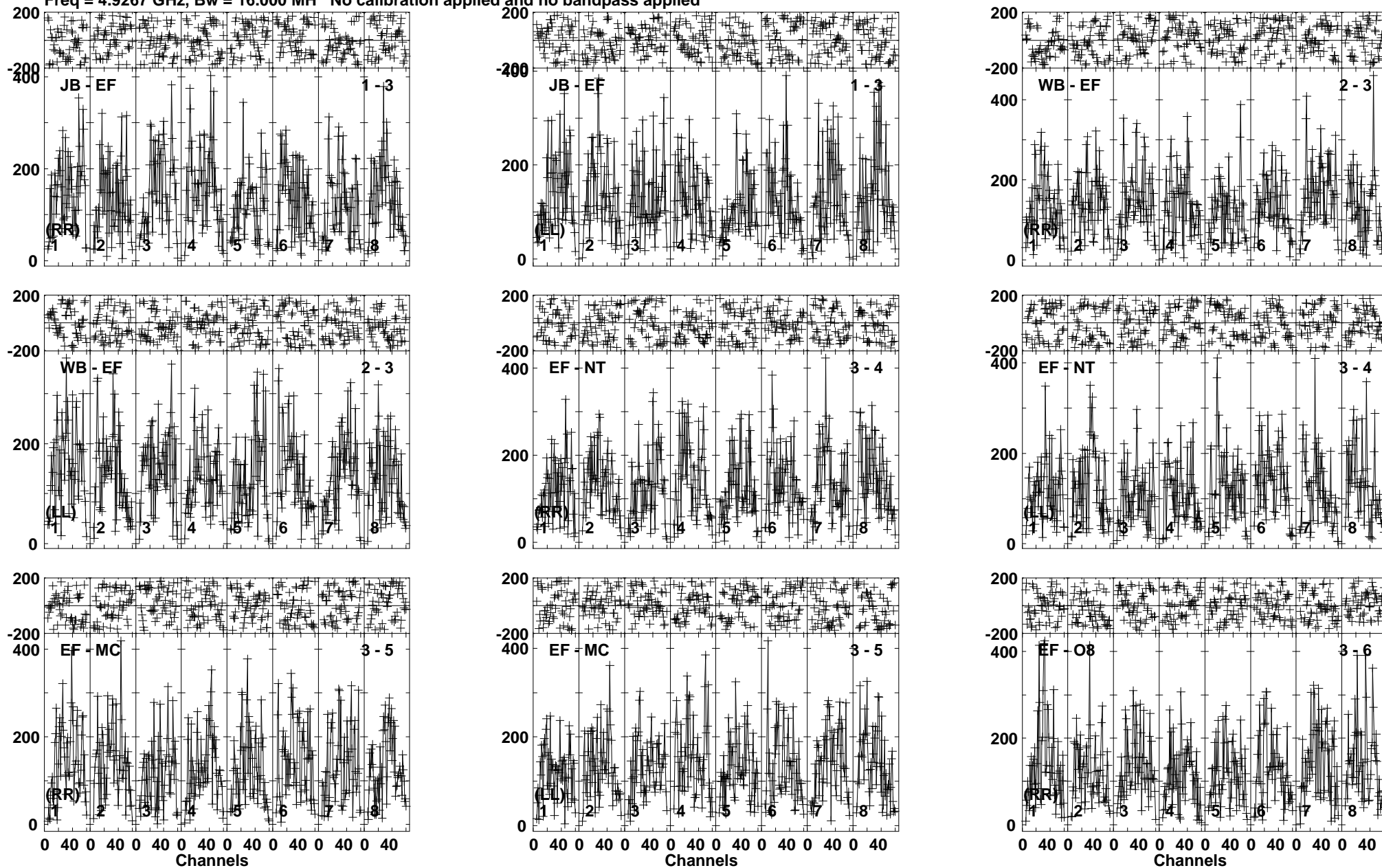
Lower frame: Micro Ampl Jy Top frame: Phas deg Vector averaged cross-power spectrum Baseline: JB (01) - EF (03) Timerange: 01/10:19:20 to 01/10:22:20
