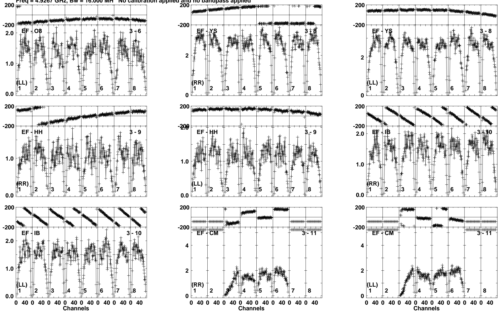
Lower frame: Milli Ampl Jy Top frame: Phas deg Vector averaged cross-power spectrum Baseline: EF (03) - O8 (06) Timerange: 01/12:23:31 to 01/12:24:59
