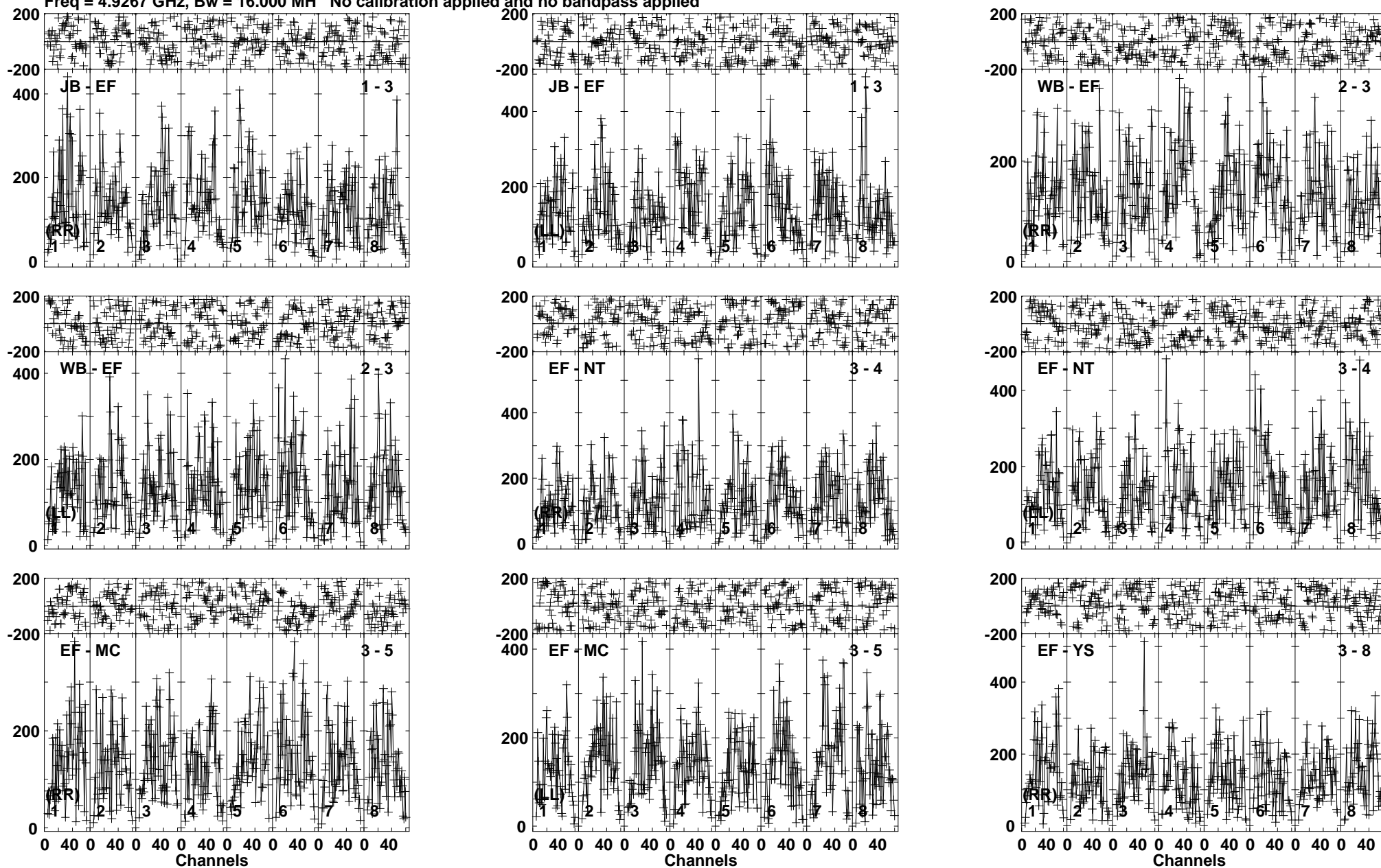
Lower frame: Micro Ampl Jy Top frame: Phas deg Vector averaged cross-power spectrum Baseline: JB (01) - EF (03) Timerange: 00/15:50:50 to 00/15:53:50
