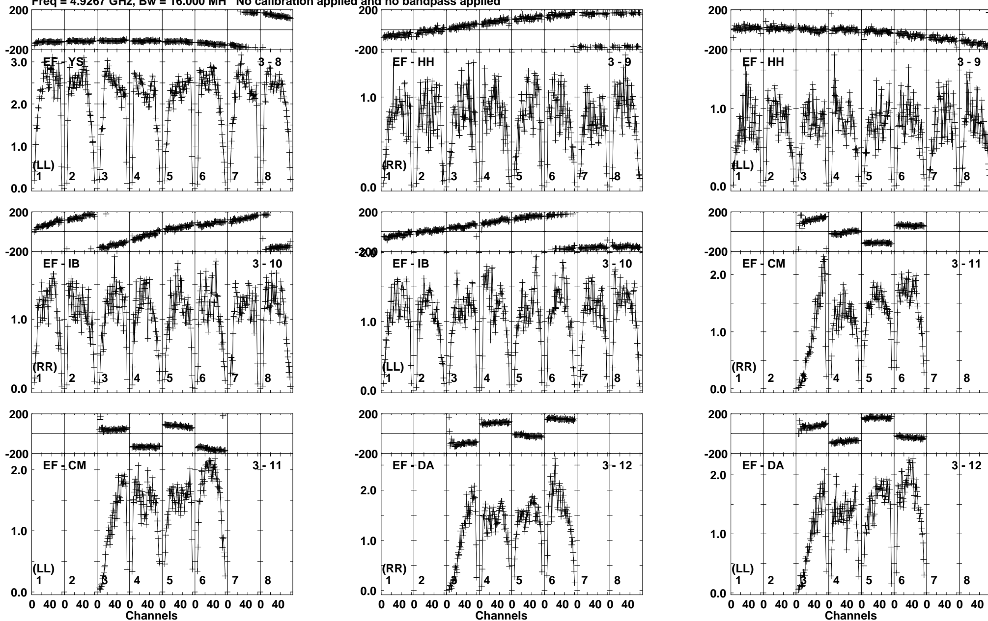
Lower frame: Milli Ampl Jy Top frame: Phas deg Vector averaged cross-power spectrum Baseline: EF (03) - YS (08) Timerange: 00/16:38:10 to 00/16:39:40
