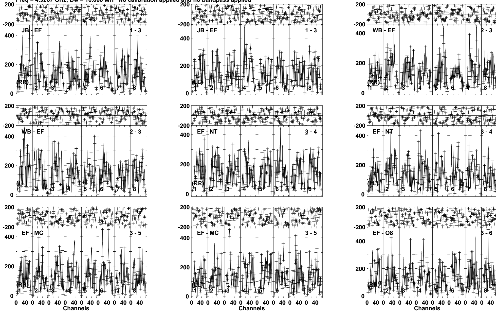
Lower frame: Micro Ampl Jy Top frame: Phas deg Vector averaged cross-power spectrum Baseline: JB (01) - EF (03) Timerange: 01/09:53:30 to 01/09:56:30
