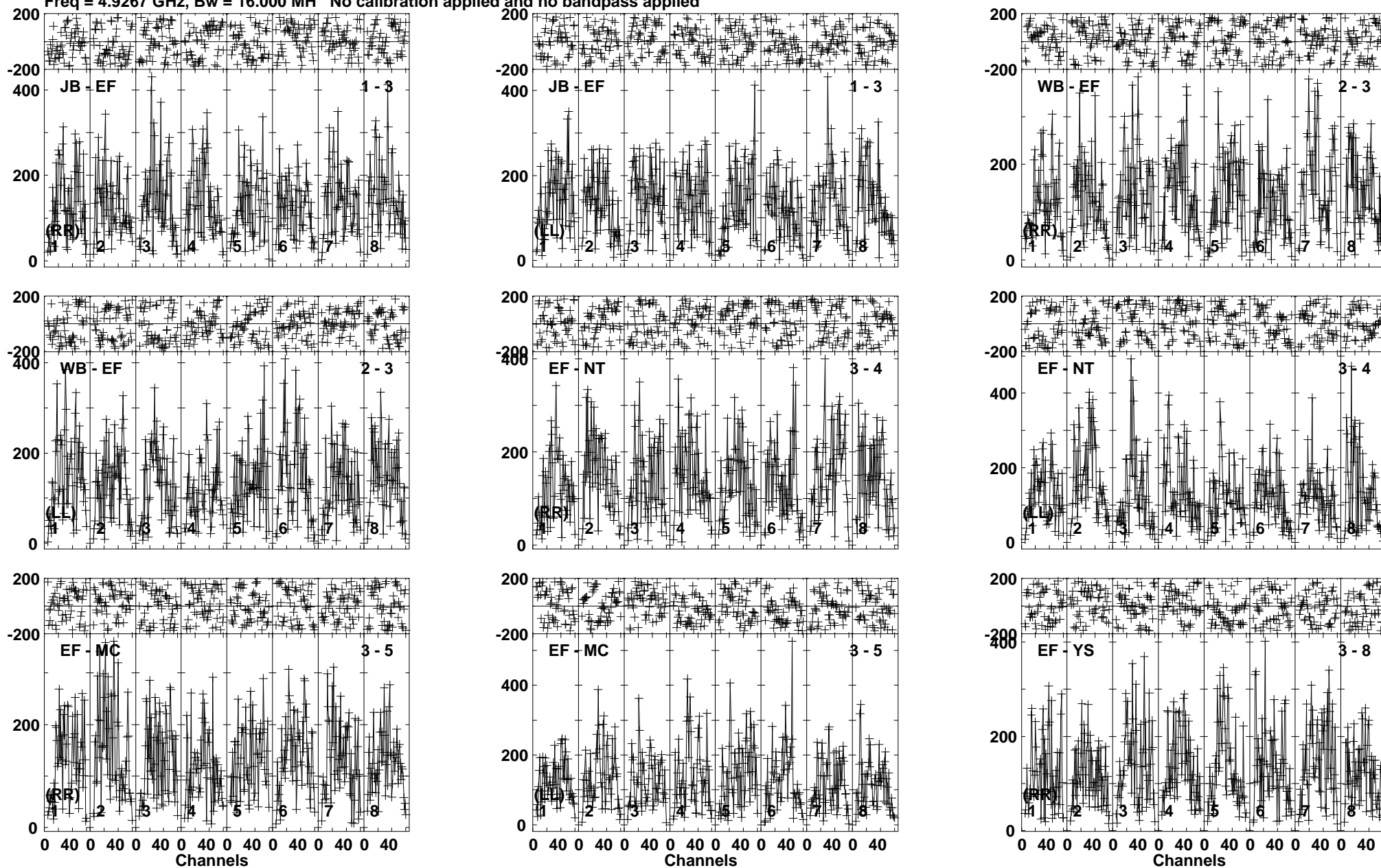
Lower frame: Micro Ampl Jy Top frame: Phas deg Vector averaged cross-power spectrum Baseline: JB (01) - EF (03) Timerange: 00/13:13:20 to 00/13:16:20
