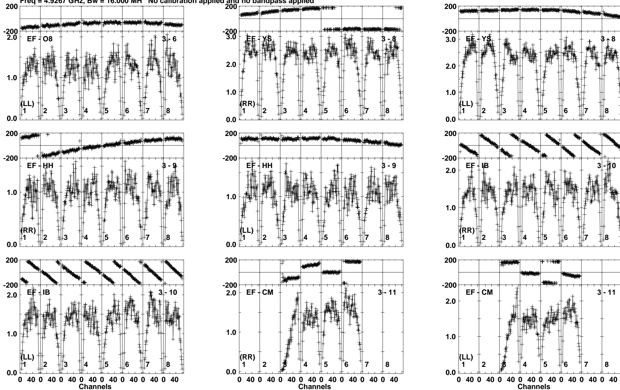
Lower frame: Milli Ampl Jy Top frame: Phas deg Vector averaged cross-power spectrum Baseline: EF (03) - O8 (06) Timerange: 01/10:07:11 to 01/10:08:40
