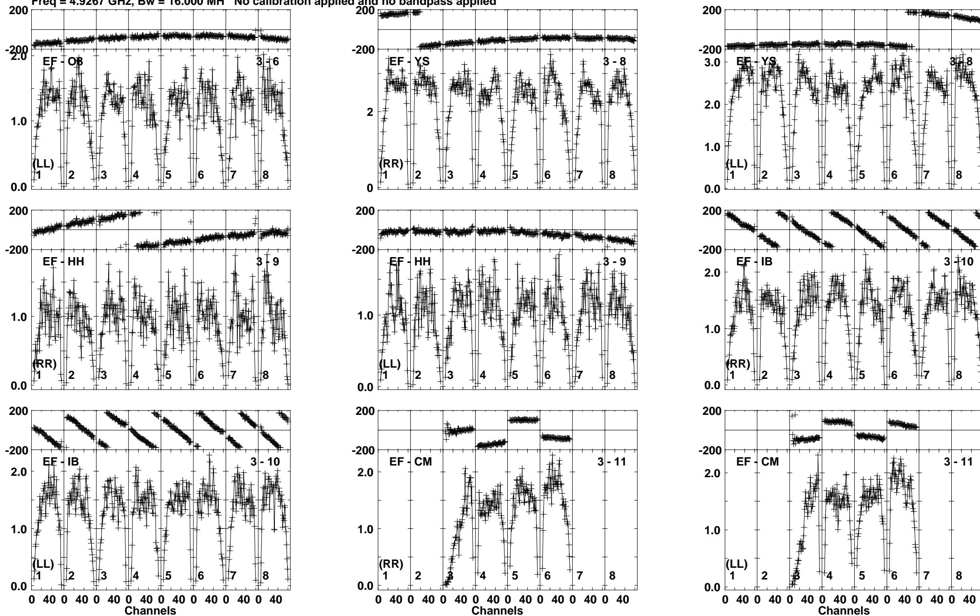
Lower frame: Milli Ampl Jy Top frame: Phas deg Vector averaged cross-power spectrum Baseline: EF (03) - O8 (06) Timerange: 01/10:45:21 to 01/10:46:49
