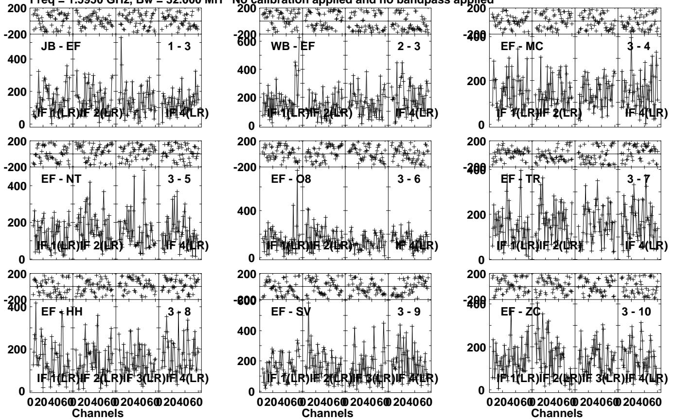
Lower frame: Micro Ampl Jy Top frame: Phas deg Vector averaged cross-power spectrum Several baselines displayed Timerange: 01/10:18:11 to 01/10:19:09
