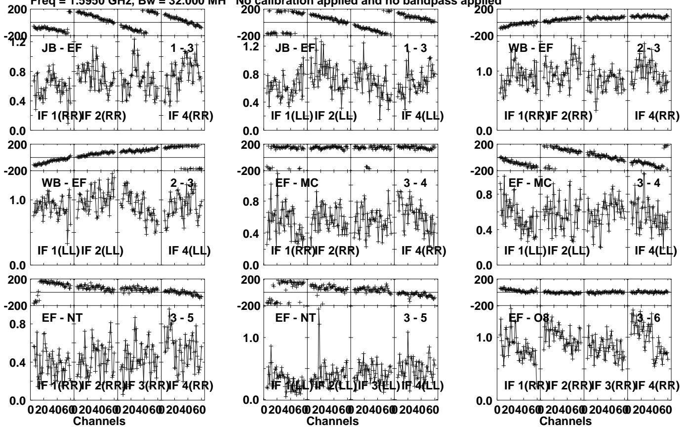
Lower frame: Milli Ampl Jy Top frame: Phas deg Vector averaged cross-power spectrum Several baselines displayed Timerange: 01/11:43:41 to 01/11:44:39
