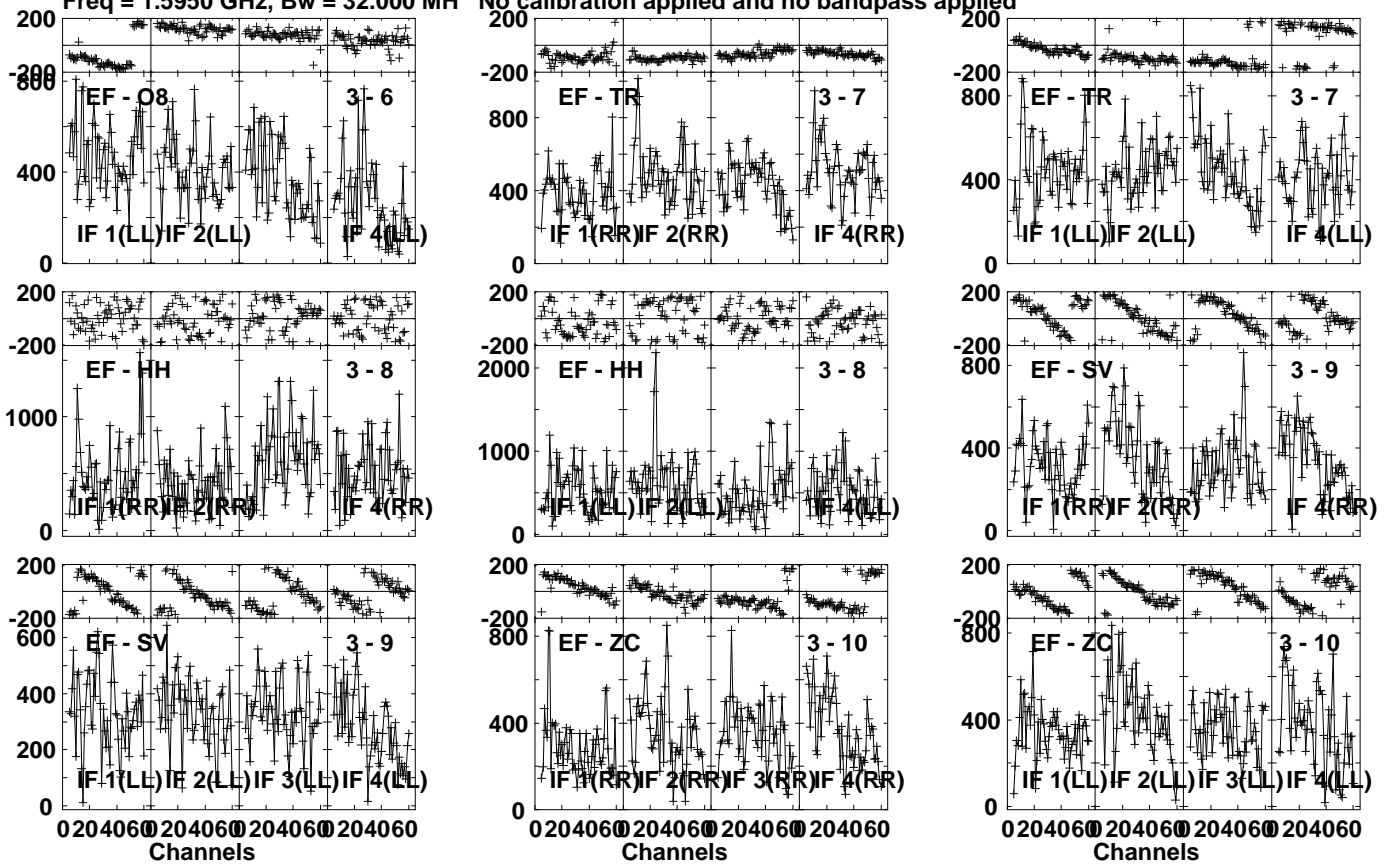
Lower frame: Micro Ampl Jy Top frame: Phas deg Vector averaged cross-power spectrum Several baselines displayed Timerange: 01/00:50:21 to 01/00:51:49
