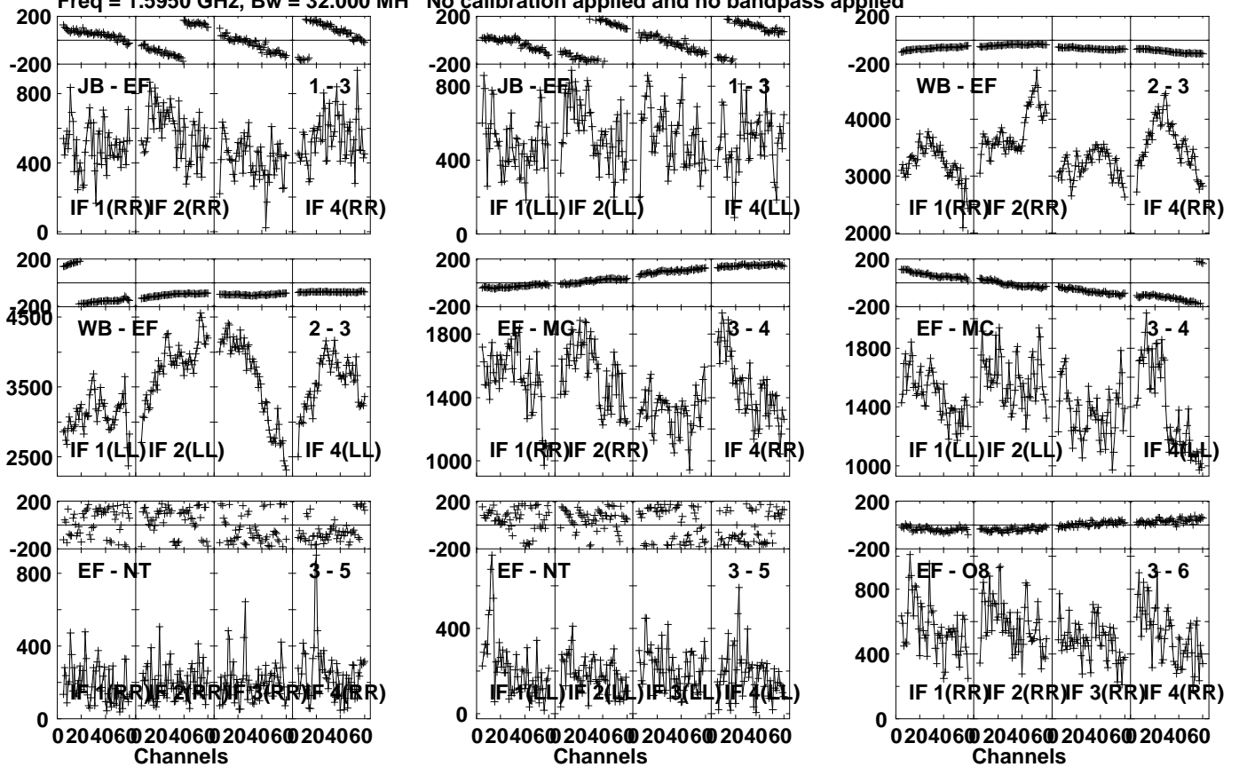
Lower frame: Micro Ampl Jy Top frame: Phas deg Vector averaged cross-power spectrum Several baselines displayed Timerange: 00/14:08:51 to 00/14:09:49
