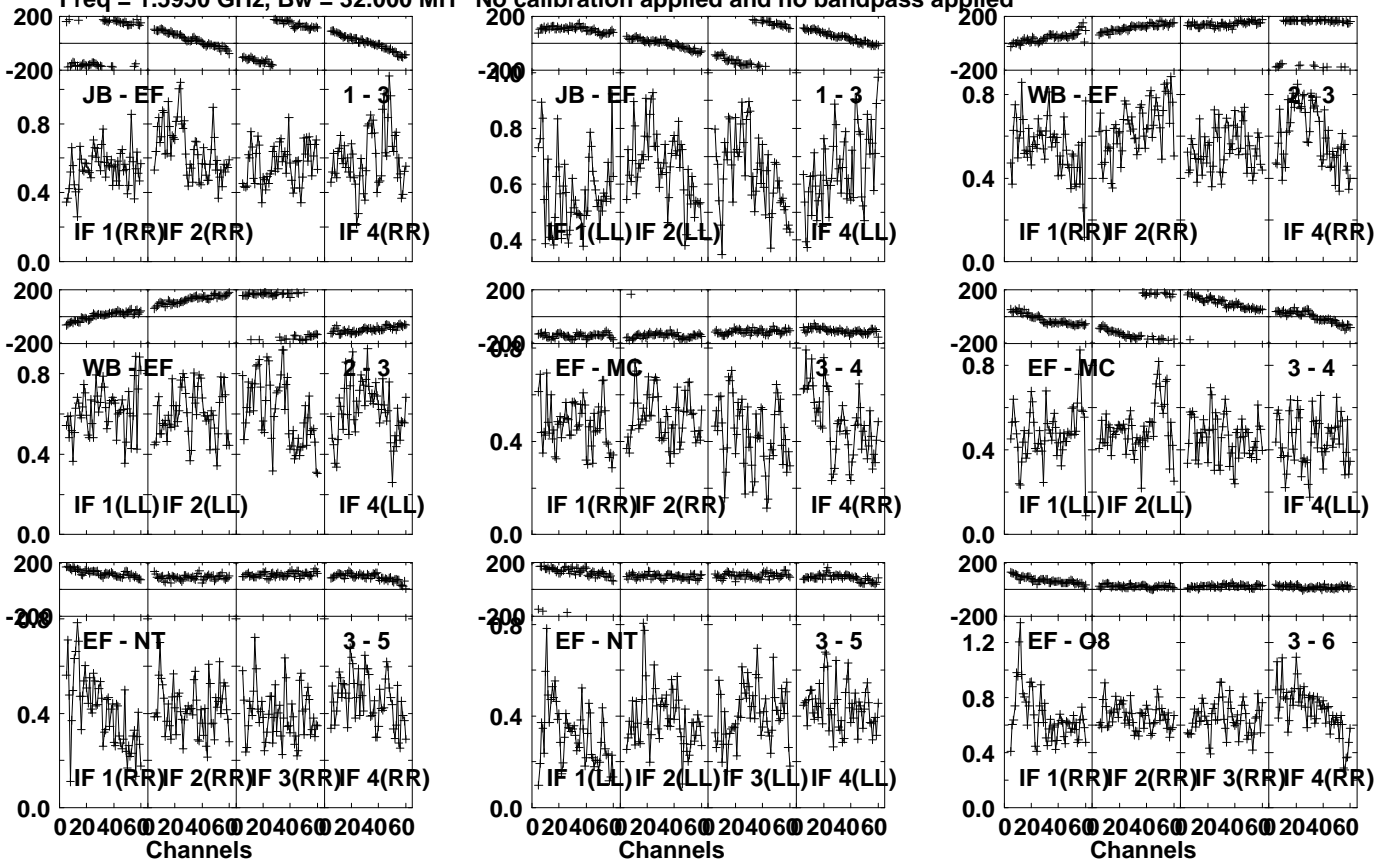
Lower frame: Milli Ampl Jy Top frame: Phas deg Vector averaged cross-power spectrum Several baselines displayed Timerange: 01/12:05:21 to 01/12:06:29
