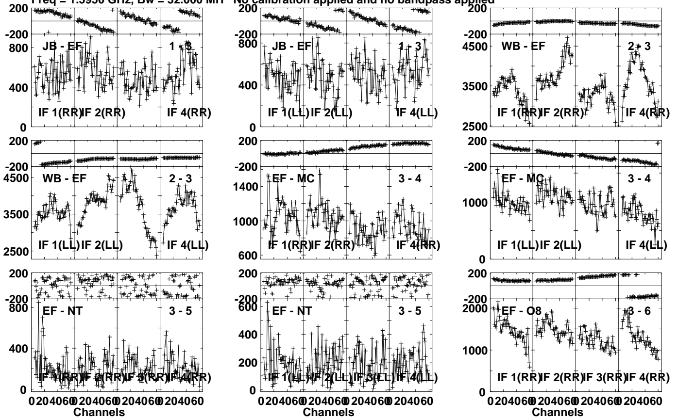
Lower frame: Micro Ampl Jy Top frame: Phas deg Vector averaged cross-power spectrum Several baselines displayed Timerange: 00/15:01:11 to 00/15:02:09
