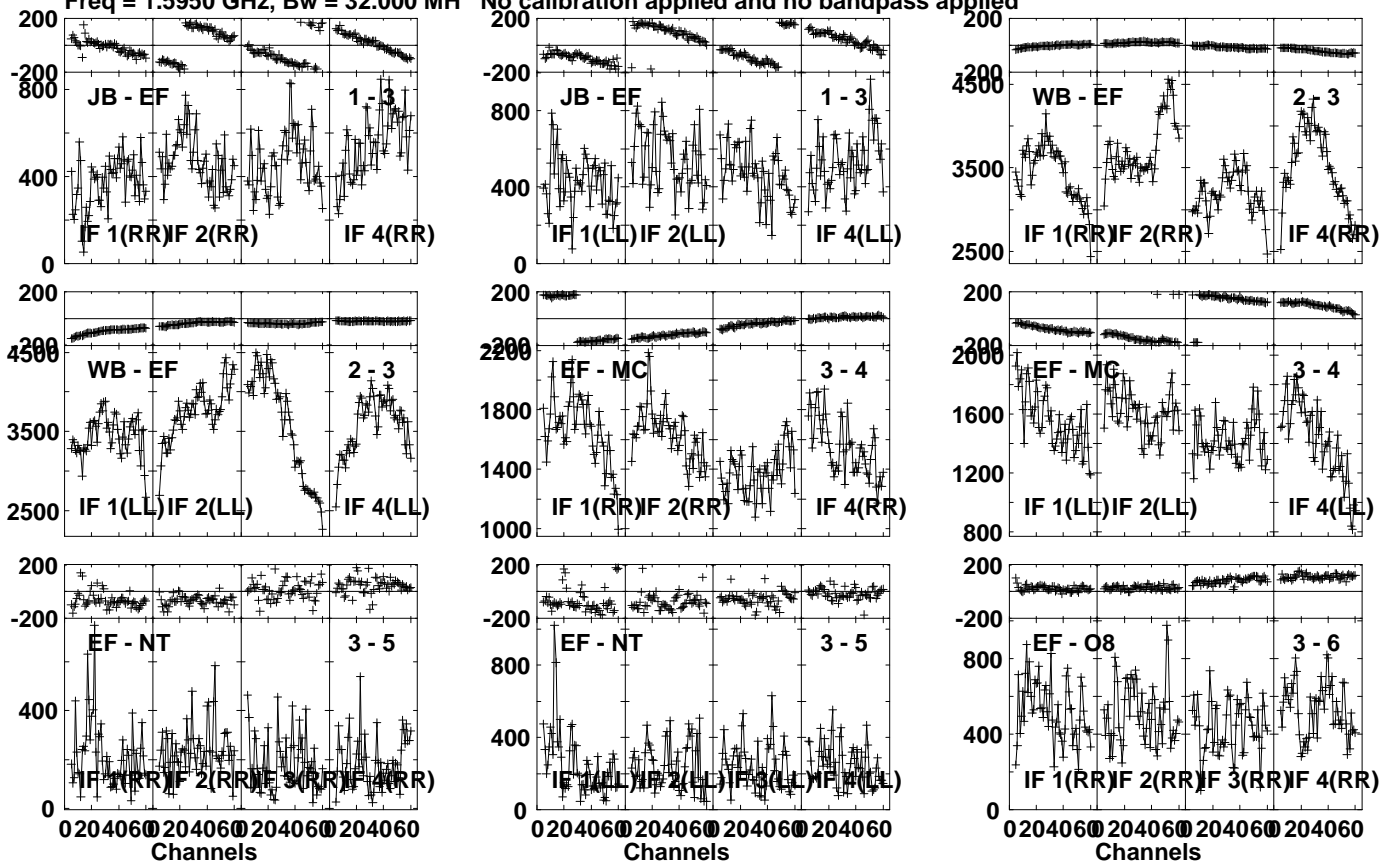
Lower frame: Micro Ampl Jy Top frame: Phas deg Vector averaged cross-power spectrum Several baselines displayed Timerange: 00/13:53:21 to 00/13:54:49
