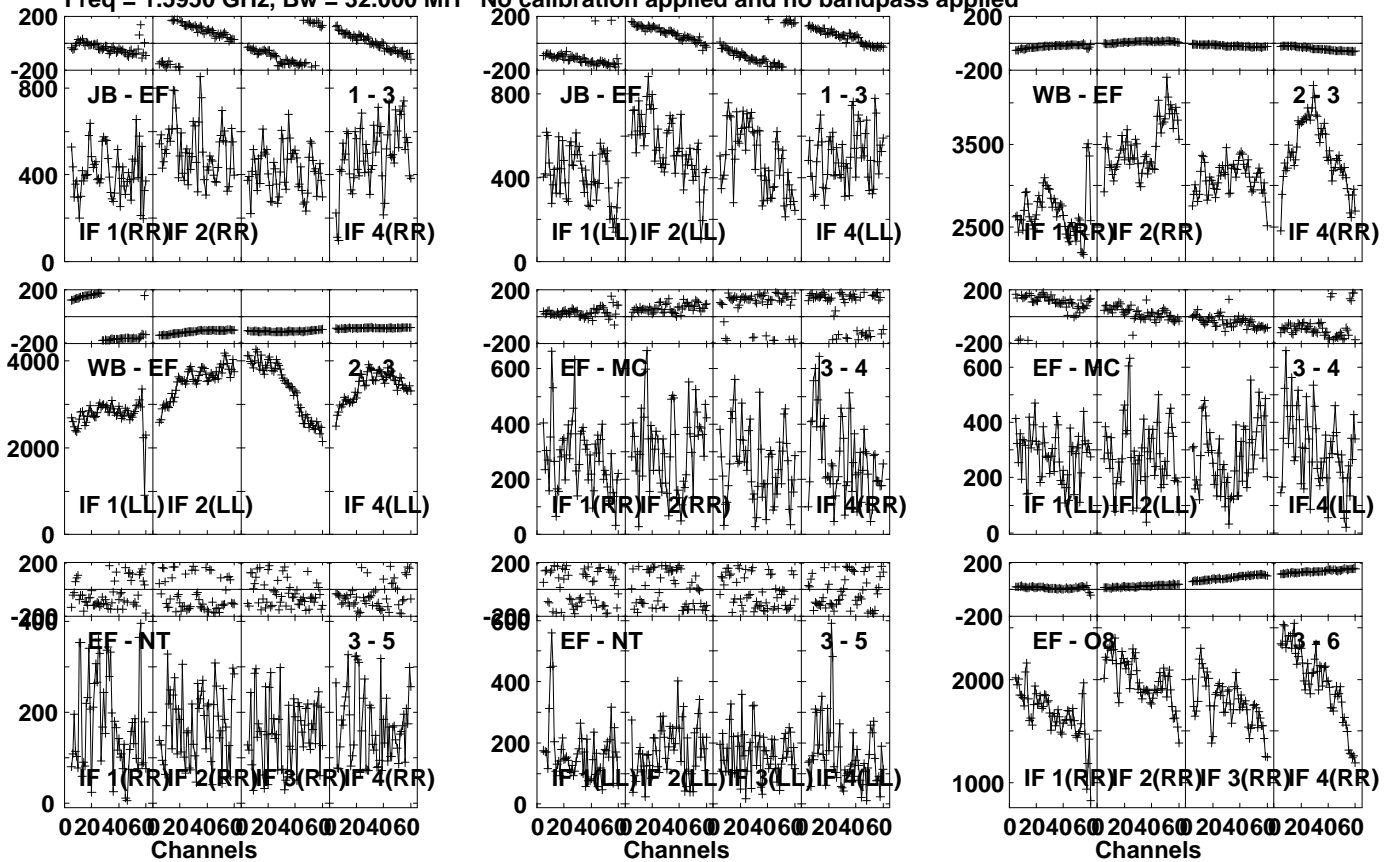
Lower frame: Micro Ampl Jy Top frame: Phas deg Vector averaged cross-power spectrum Several baselines displayed Timerange: 00/16:55:51 to 00/16:56:49
