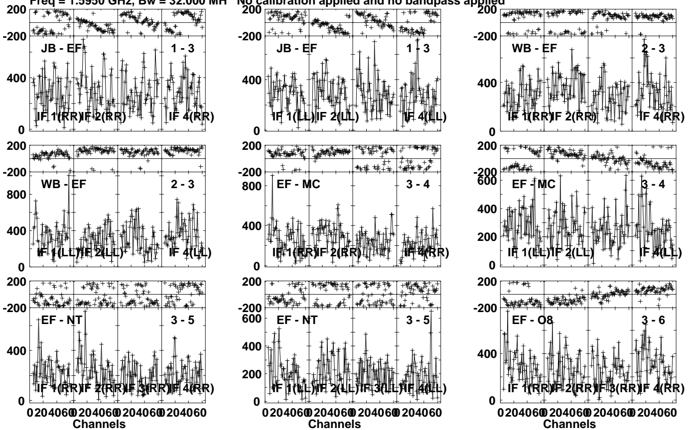
Lower frame: Micro Ampl Jy Top frame: Phas deg Vector averaged cross-power spectrum Several baselines displayed Timerange: 00/13:22:11 to 00/13:23:39
