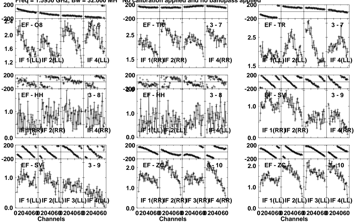
Lower frame: Milli Ampl Jy Top frame: Phas deg Vector averaged cross-power spectrum Several baselines displayed Timerange: 01/03:15:11 to 01/03:16:39
