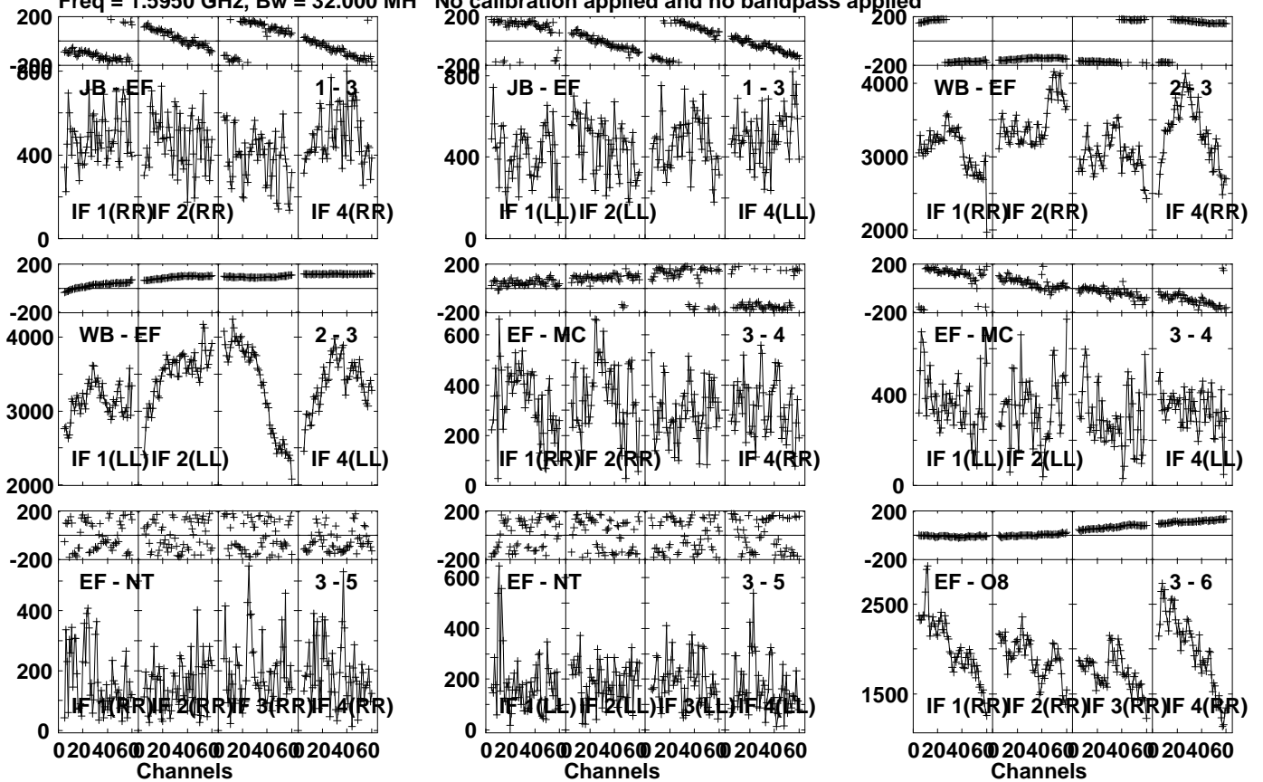
Lower frame: Micro Ampl Jy Top frame: Phas deg Vector averaged cross-power spectrum Several baselines displayed Timerange: 00/16:40:21 to 00/16:41:49
