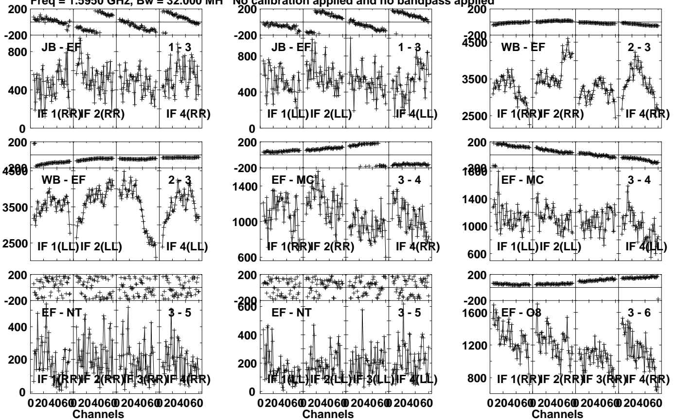
Lower frame: Micro Ampl Jy Top frame: Phas deg Vector averaged cross-power spectrum Several baselines displayed Timerange: 00/14:51:11 to 00/14:52:09
