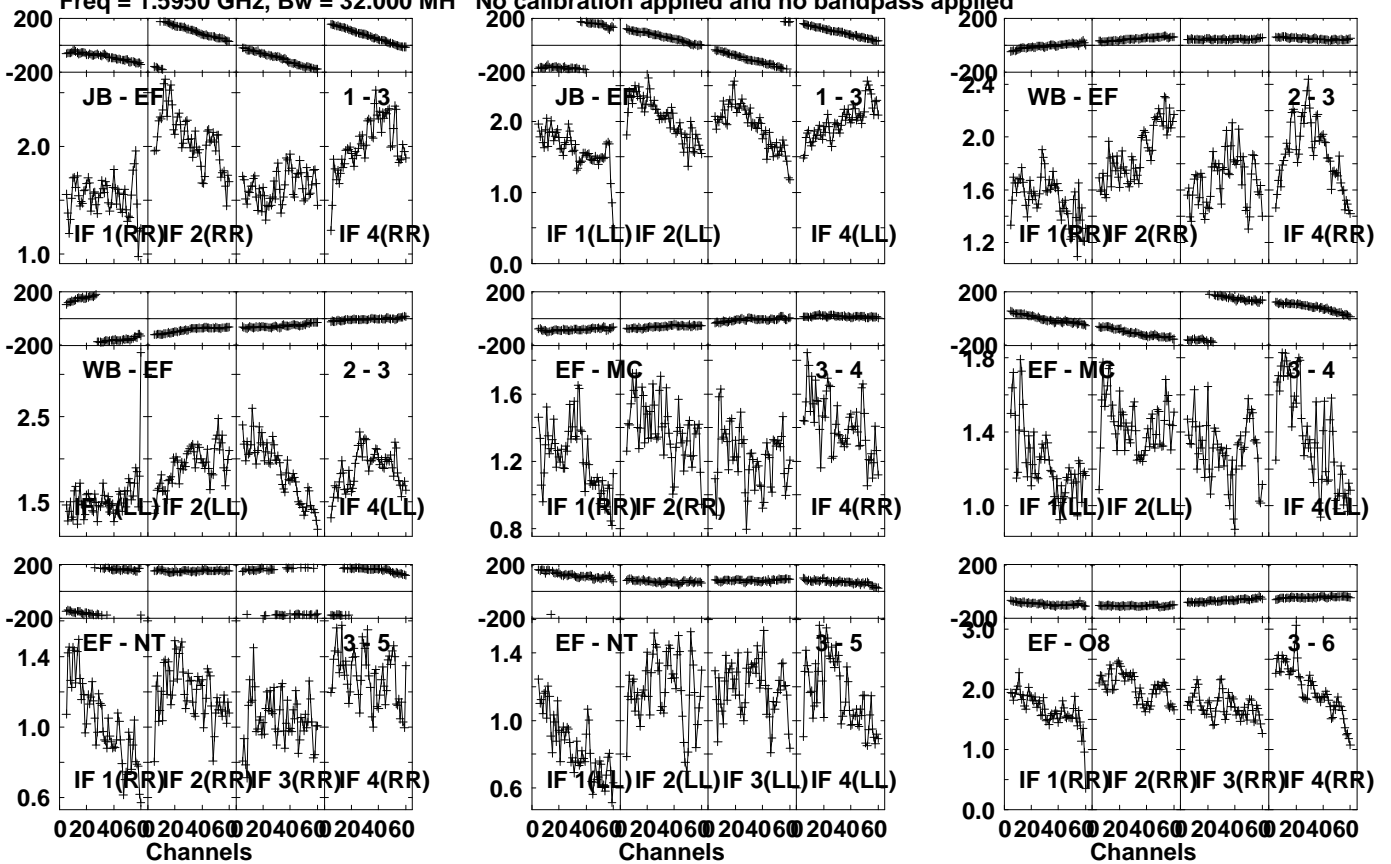
Lower frame: Milli Ampl Jy Top frame: Phas deg Vector averaged cross-power spectrum Several baselines displayed Timerange: 01/03:40:41 to 01/03:41:39
