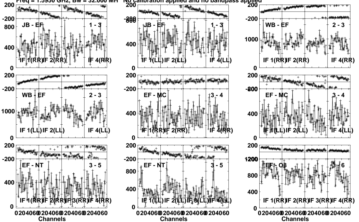
Lower frame: Micro Ampl Jy Top frame: Phas deg Vector averaged cross-power spectrum Several baselines displayed Timerange: 01/10:34:31 to 01/10:35:59
