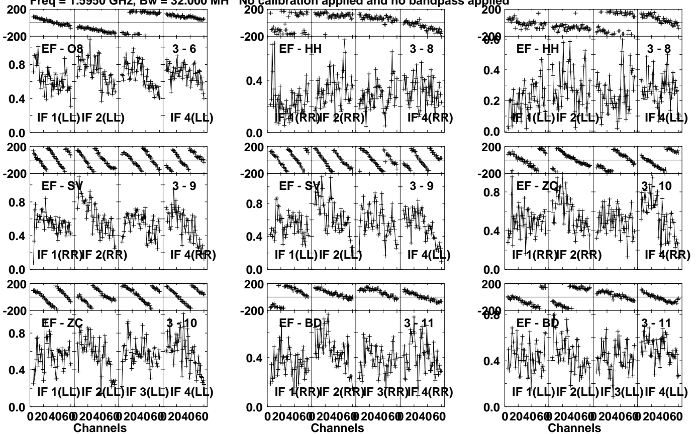
Lower frame: Milli Amp Jy Top frame: Phas deg Vector averaged cross-power spectrum Several baselines displayed Timerange: 01/12:05:21 to 01/12:06:29
