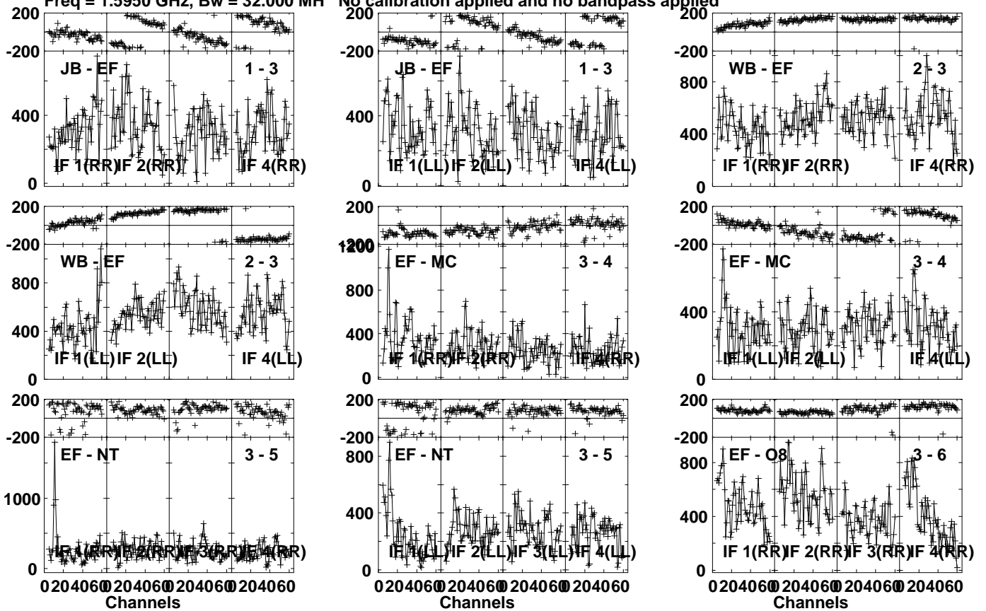
Lower frame: Micro Ampl Jy Top frame: Phas deg Vector averaged cross-power spectrum Several baselines displayed Timerange: 00/23:53:31 to 00/23:54:59
