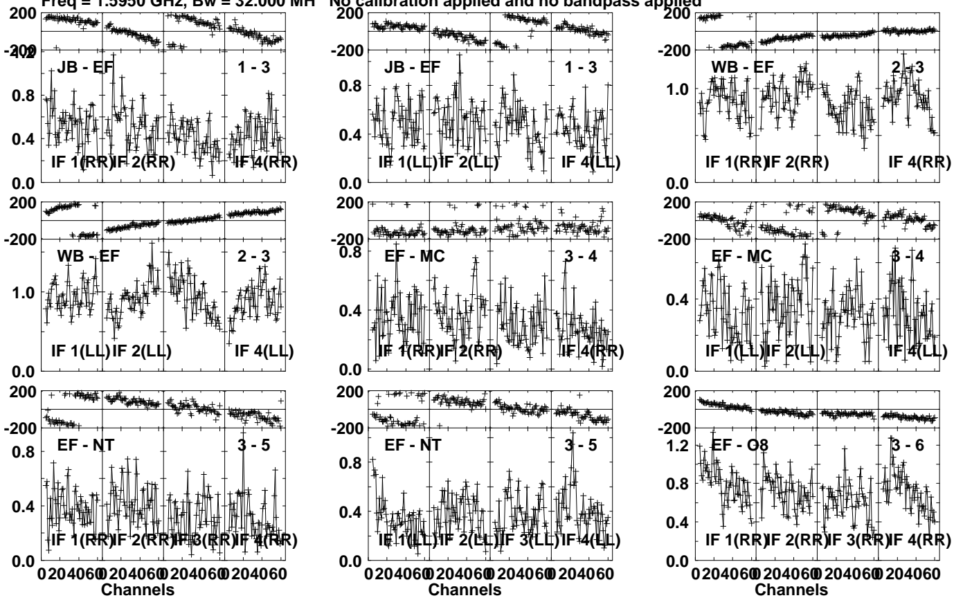
Lower frame: Milli Ampl Jy Top frame: Phas deg Vector averaged cross-power spectrum Several baselines displayed Timerange: 01/09:46:21 to 01/09:47:19
