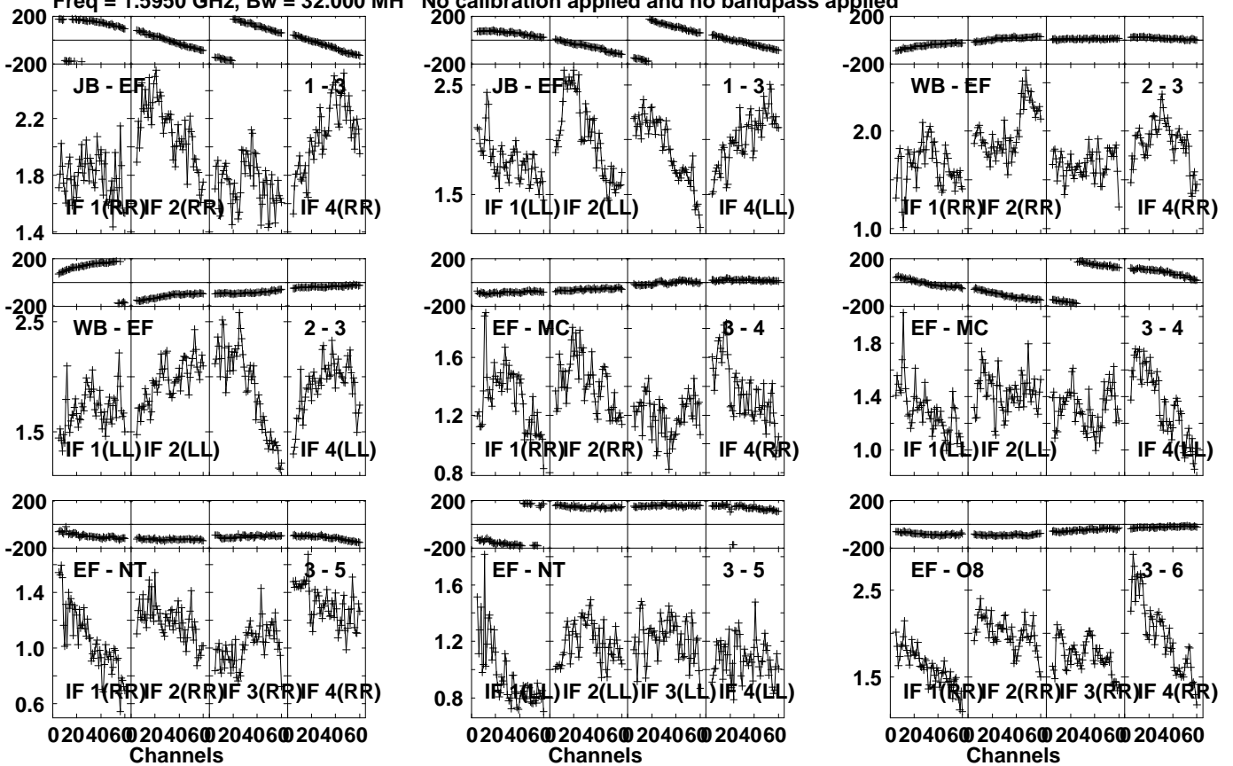
Lower frame: Milli Ampl Jy Top frame: Phas deg Vector averaged cross-power spectrum Several baselines displayed Timerange: 01/03:20:41 to 01/03:21:39
