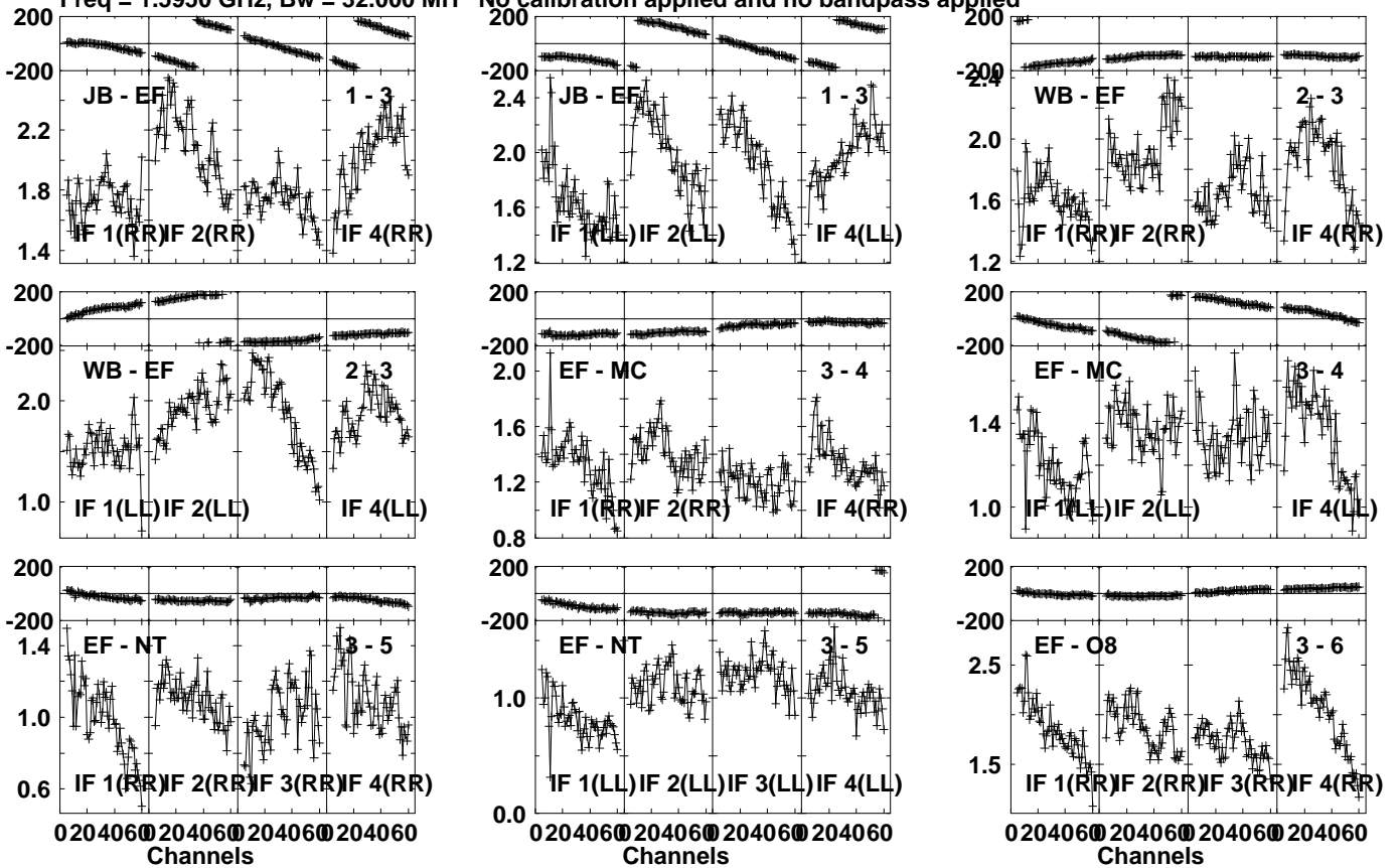
Lower frame: Milli Ampl Jy Top frame: Phas deg Vector averaged cross-power spectrum Several baselines displayed Timerange: 01/02:30:41 to 01/02:31:39
