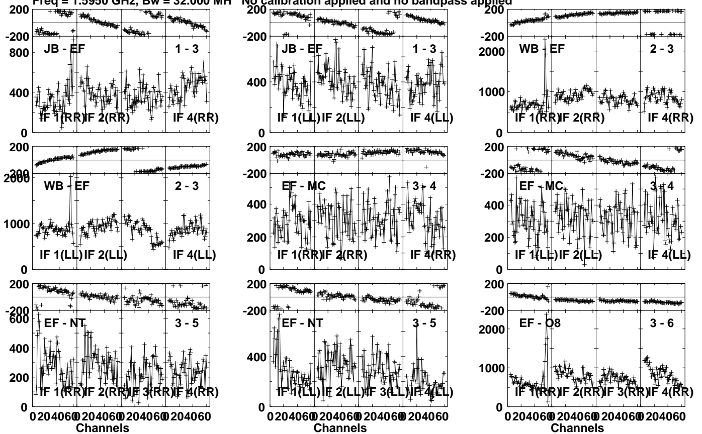
Lower frame: Micro Ampl Jy Top frame: Phas deg Vector averaged cross-power spectrum Several baselines displayed Timerange: 01/10:29:51 to 01/10:30:59
