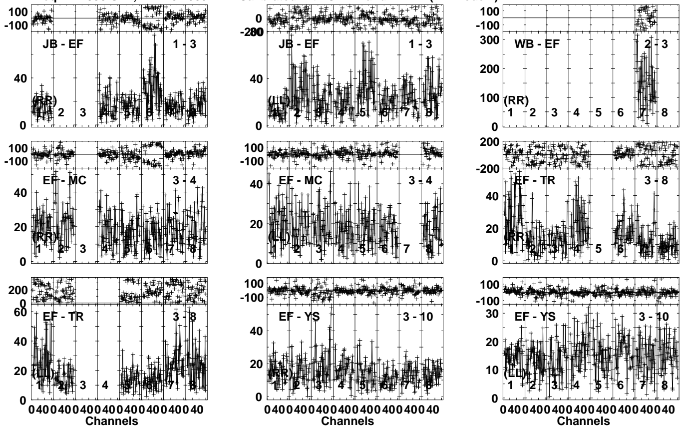
Lower frame: Milli Ampl Jy Top frame: Phas deg Vector averaged cross-power spectrum Several baselines displayed Timerange: 01/00:15:31 to 01/00:16:49
