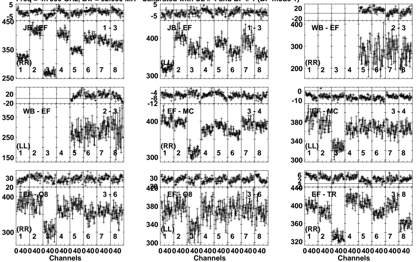
Lower frame: Milli Ampl Jy Top frame: Phas deg Vector averaged cross-power spectrum Several baselines displayed Timerange: 00/13:33:52 to 00/13:35:28
