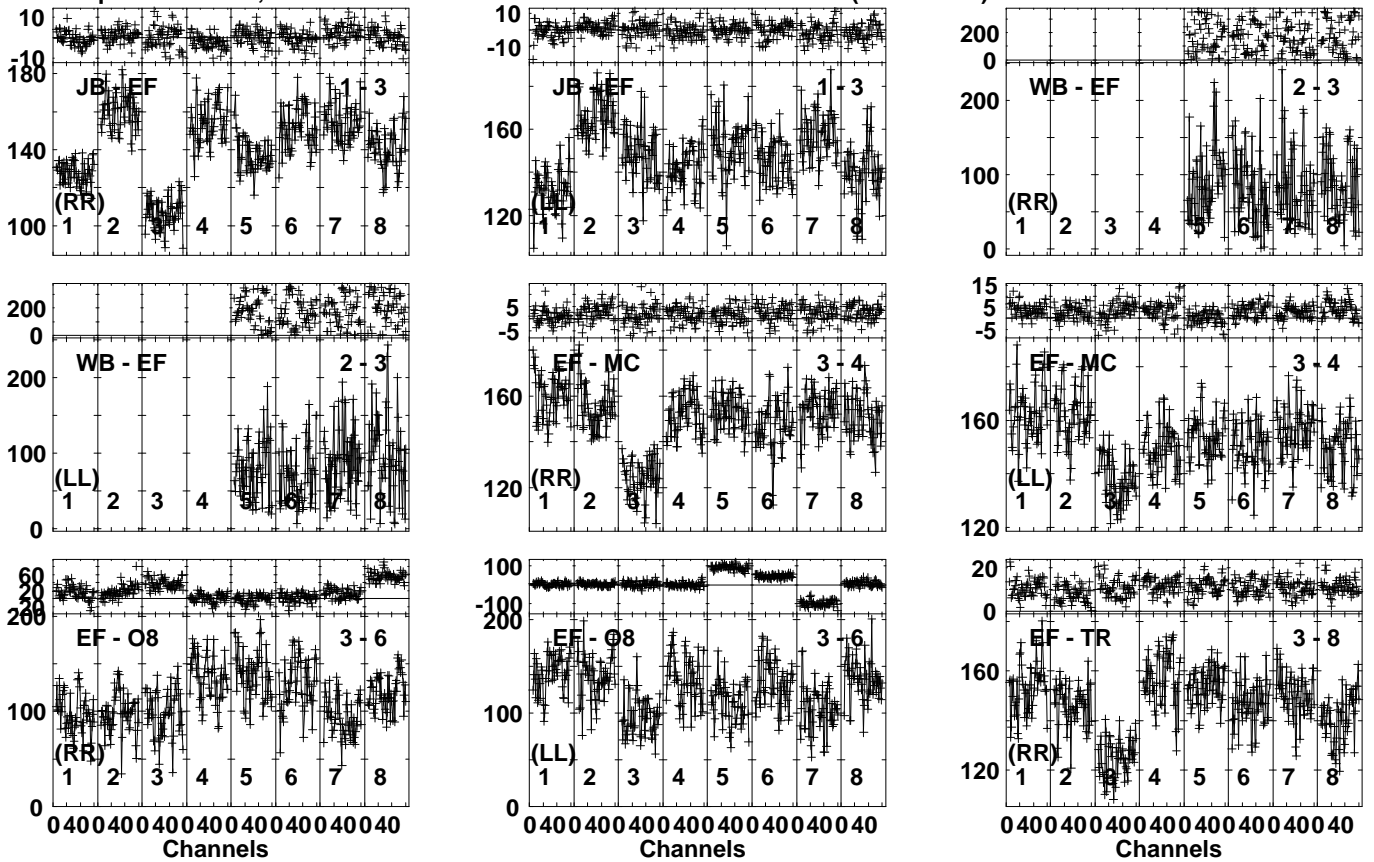
Lower frame: Milli Ampl Jy Top frame: Phas deg Vector averaged cross-power spectrum Several baselines displayed Timerange: 00/19:42:01 to 00/19:43:09
