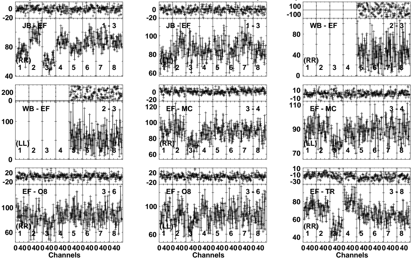
Lower frame: Milli Ampl Jy Top frame: Phas deg Vector averaged cross-power spectrum Several baselines displayed Timerange: 00/13:44:42 to 00/13:45:58
