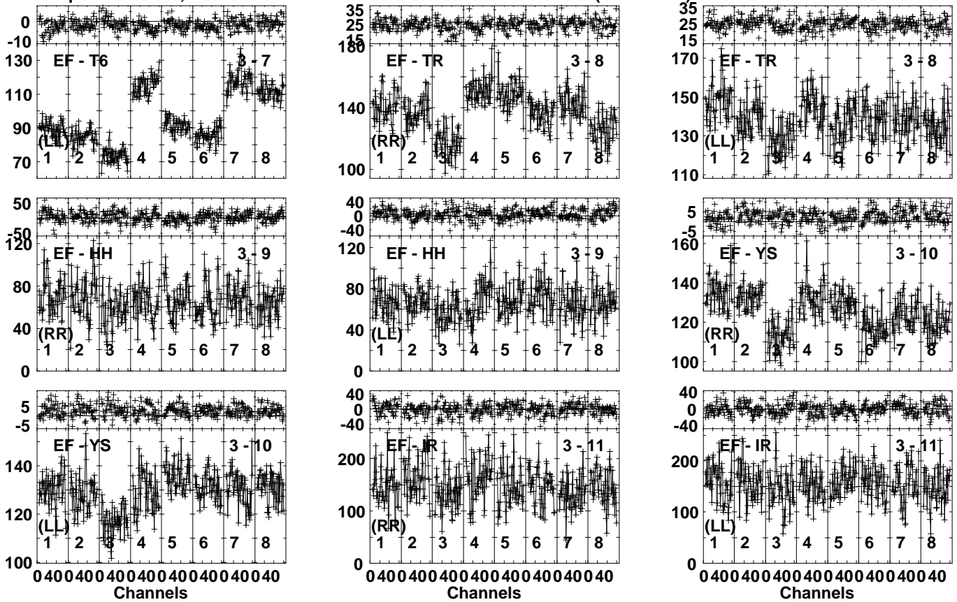
Lower frame: Milli Ampl Jy Top frame: Phas deg Vector averaged cross-power spectrum Several baselines displayed Timerange: 00/18:22:31 to 00/18:23:39
