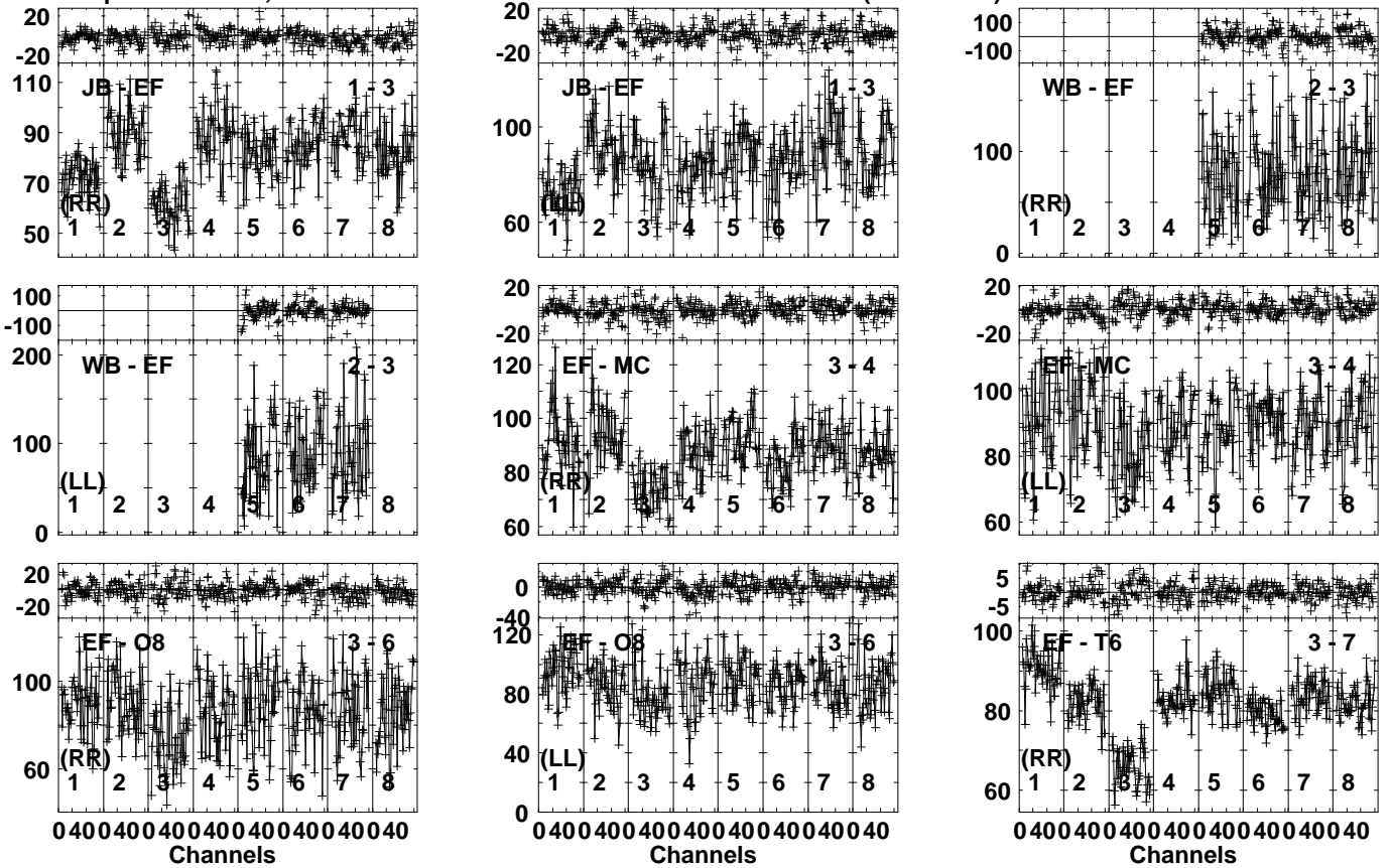
Lower frame: Milli Ampl Jy Top frame: Phas deg Vector averaged cross-power spectrum Several baselines displayed Timerange: 00/16:41:31 to 00/16:42:39
