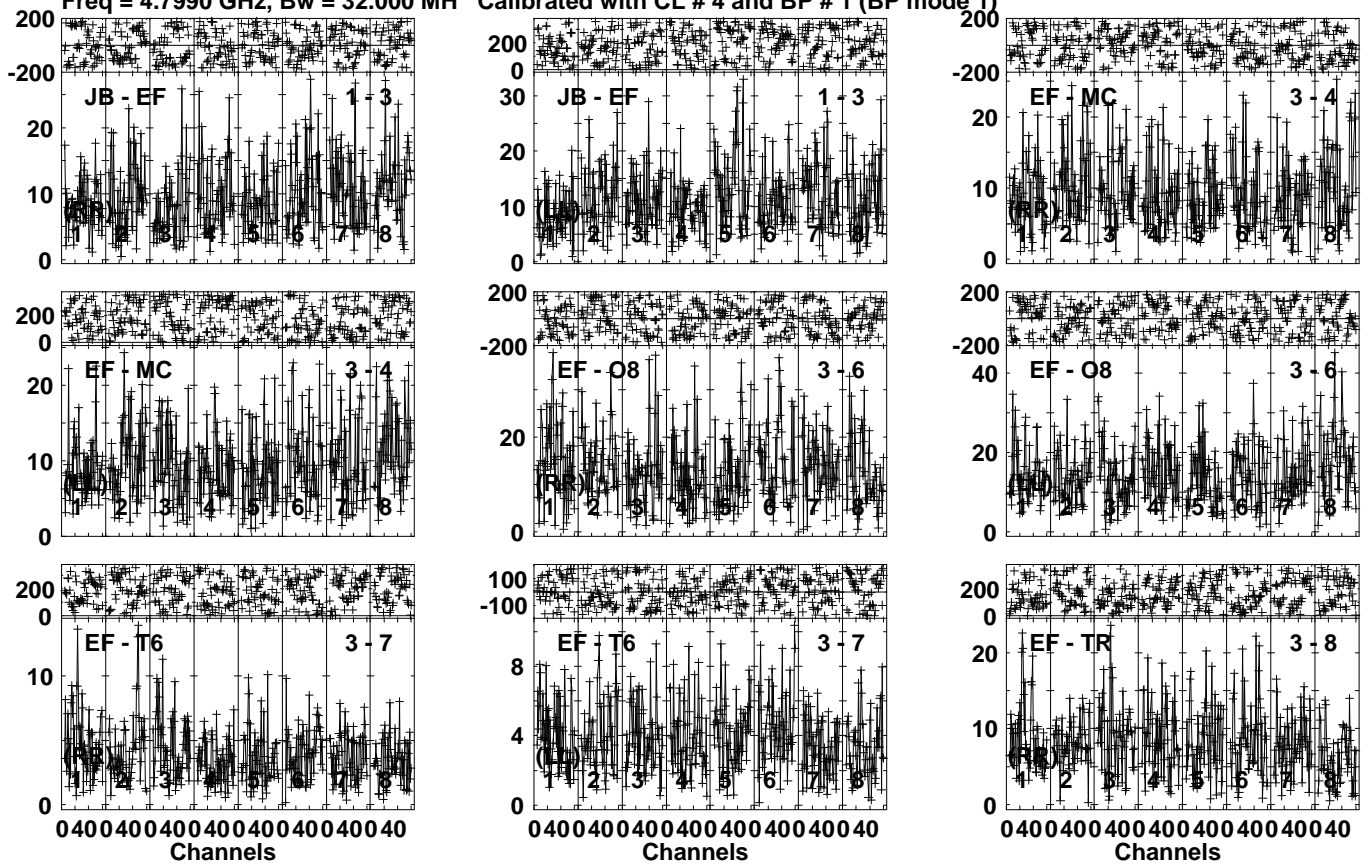
Lower frame: Milli Ampl Jy Top frame: Phas deg Vector averaged cross-power spectrum Several baselines displayed Timerange: 00/15:03:11 to 00/15:05:49
