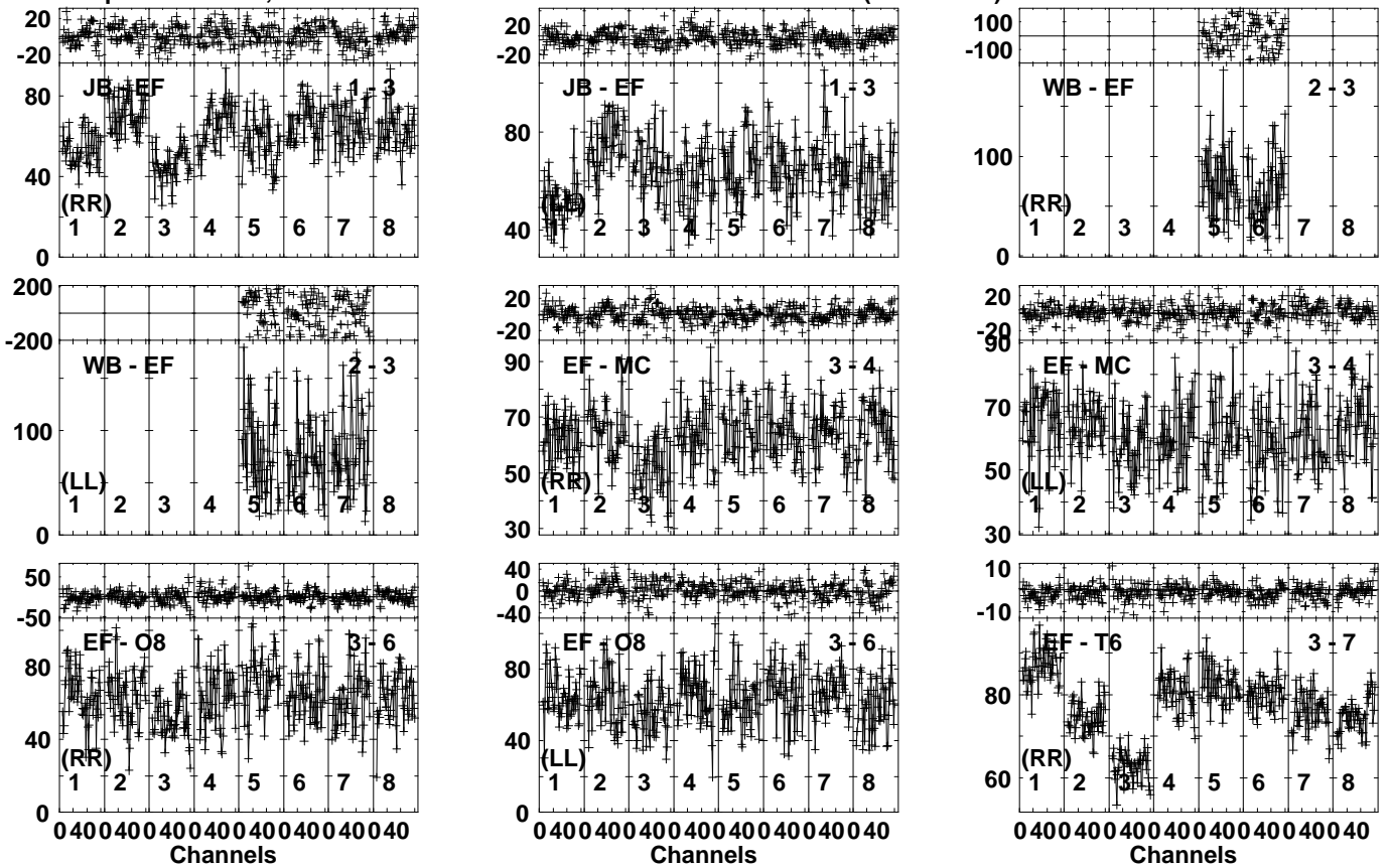
Lower frame: Milli Ampl Jy Top frame: Phas deg Vector averaged cross-power spectrum Several baselines displayed Timerange: 00/15:45:11 to 00/15:46:19
