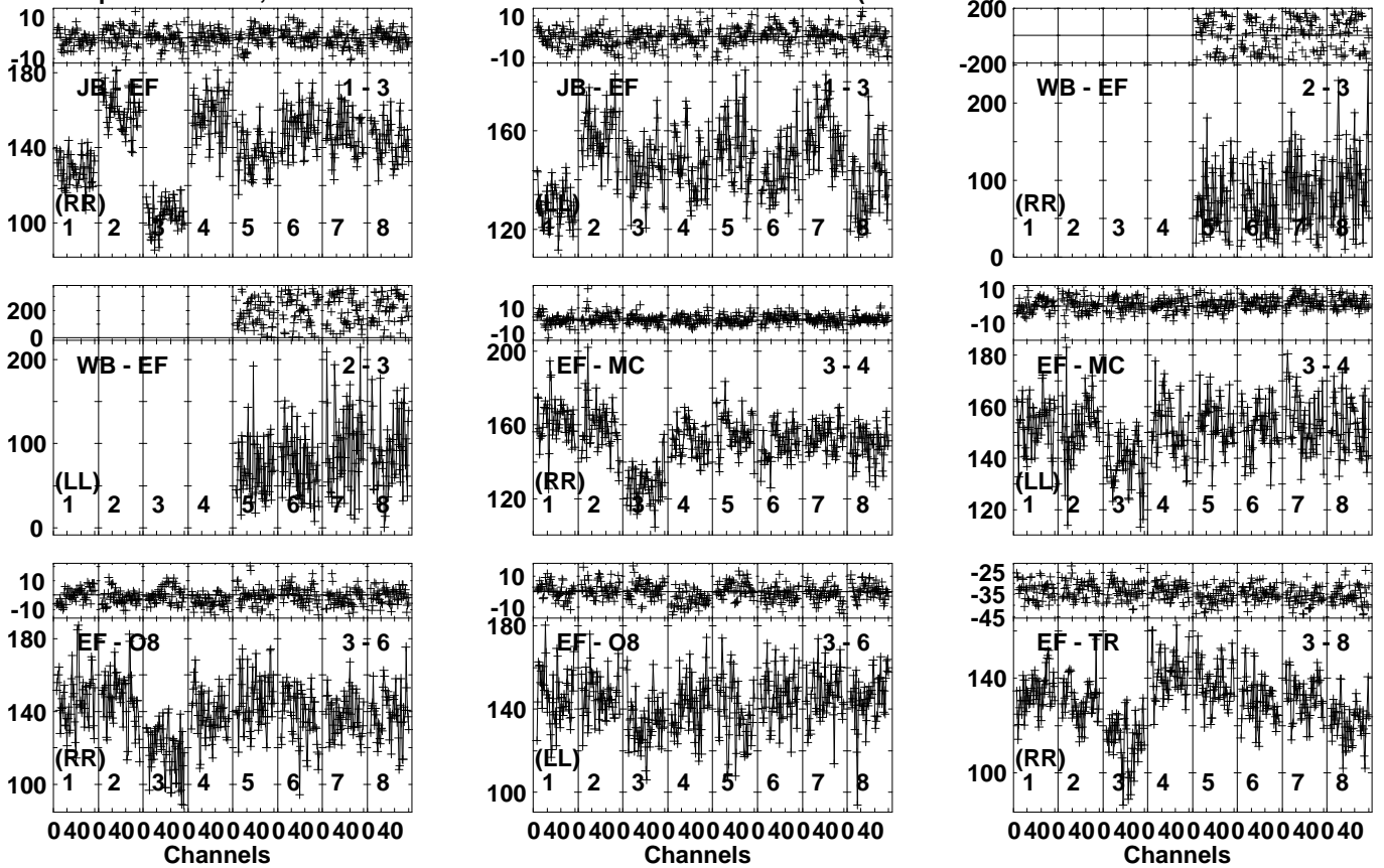
Lower frame: Milli Ampl Jy Top frame: Phas deg Vector averaged cross-power spectrum Several baselines displayed Timerange: 00/18:25:21 to 00/18:26:29
