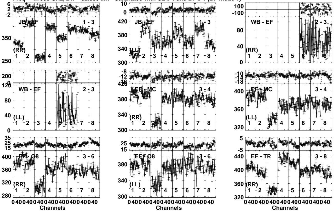
Lower frame: Milli Ampl Jy Top frame: Phas deg Vector averaged cross-power spectrum Several baselines displayed Timerange: 00/13:09:32 to 00/13:11:08
