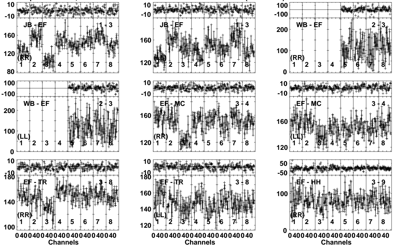
Lower frame: Milli Ampl Jy Top frame: Phas deg Vector averaged cross-power spectrum Several baselines displayed Timerange: 00/20:29:41 to 00/20:30:49
