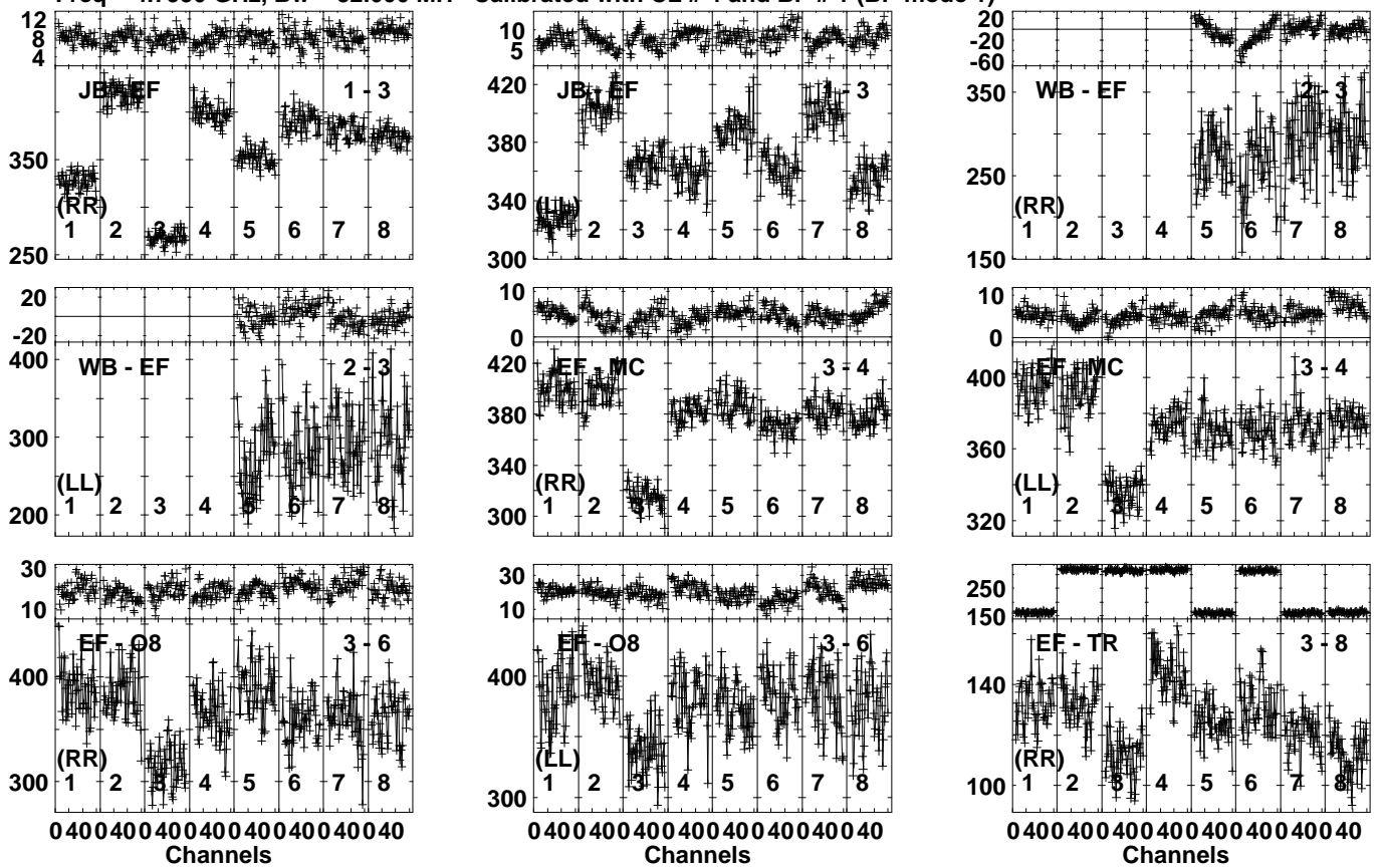
Lower frame: Milli Ampl Jy Top frame: Phas deg Vector averaged cross-power spectrum Several baselines displayed Timerange: 00/12:45:12 to 00/12:46:48
