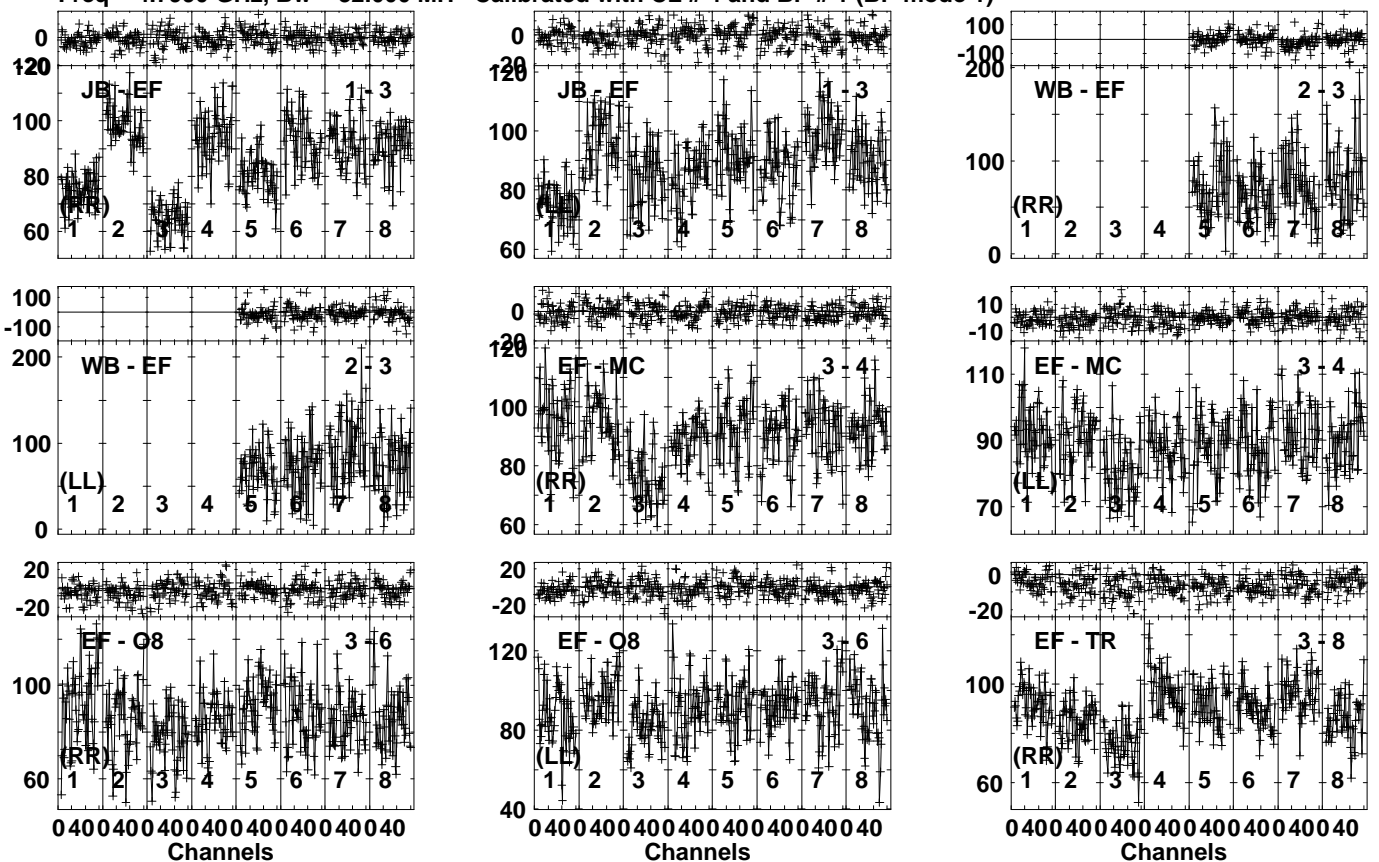
Lower frame: Milli Ampl Jy Top frame: Phas deg Vector averaged cross-power spectrum Several baselines displayed Timerange: 00/13:23:52 to 00/13:25:08
