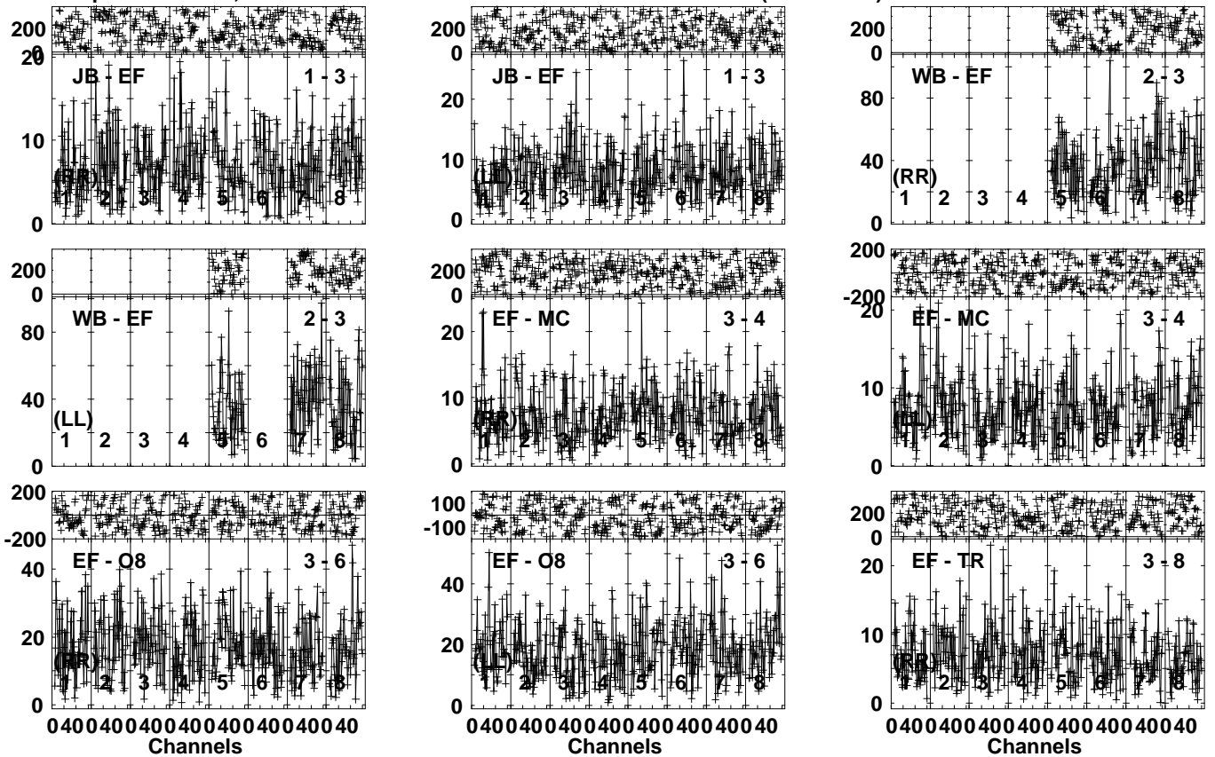
Lower frame: Milli Ampl Jy Top frame: Phas deg Vector averaged cross-power spectrum Several baselines displayed Timerange: 00/12:52:52 to 00/12:55:28
