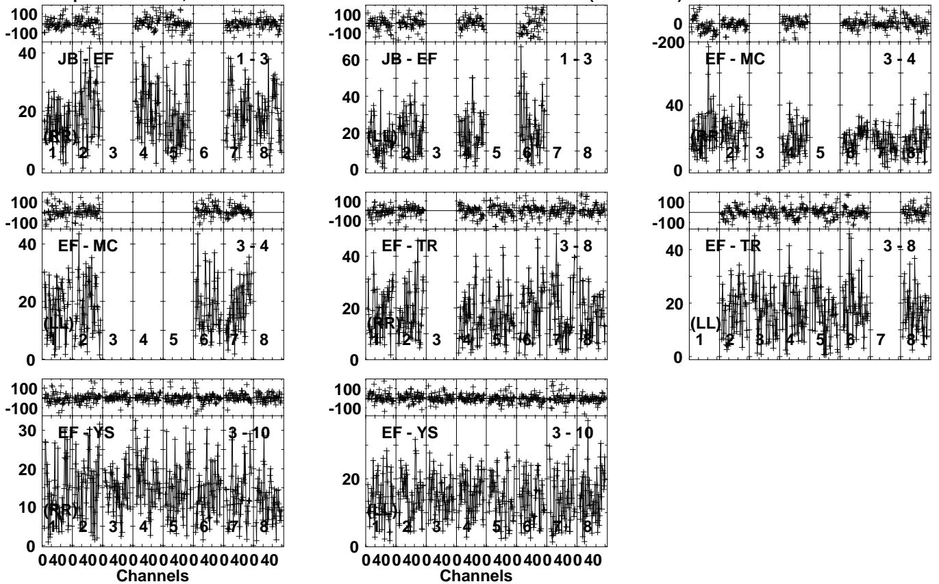
Lower frame: Milli Ampl Jy Top frame: Phas deg Vector averaged cross-power spectrum Several baselines displayed Timerange: 01/01:03:21 to 01/01:04:39
