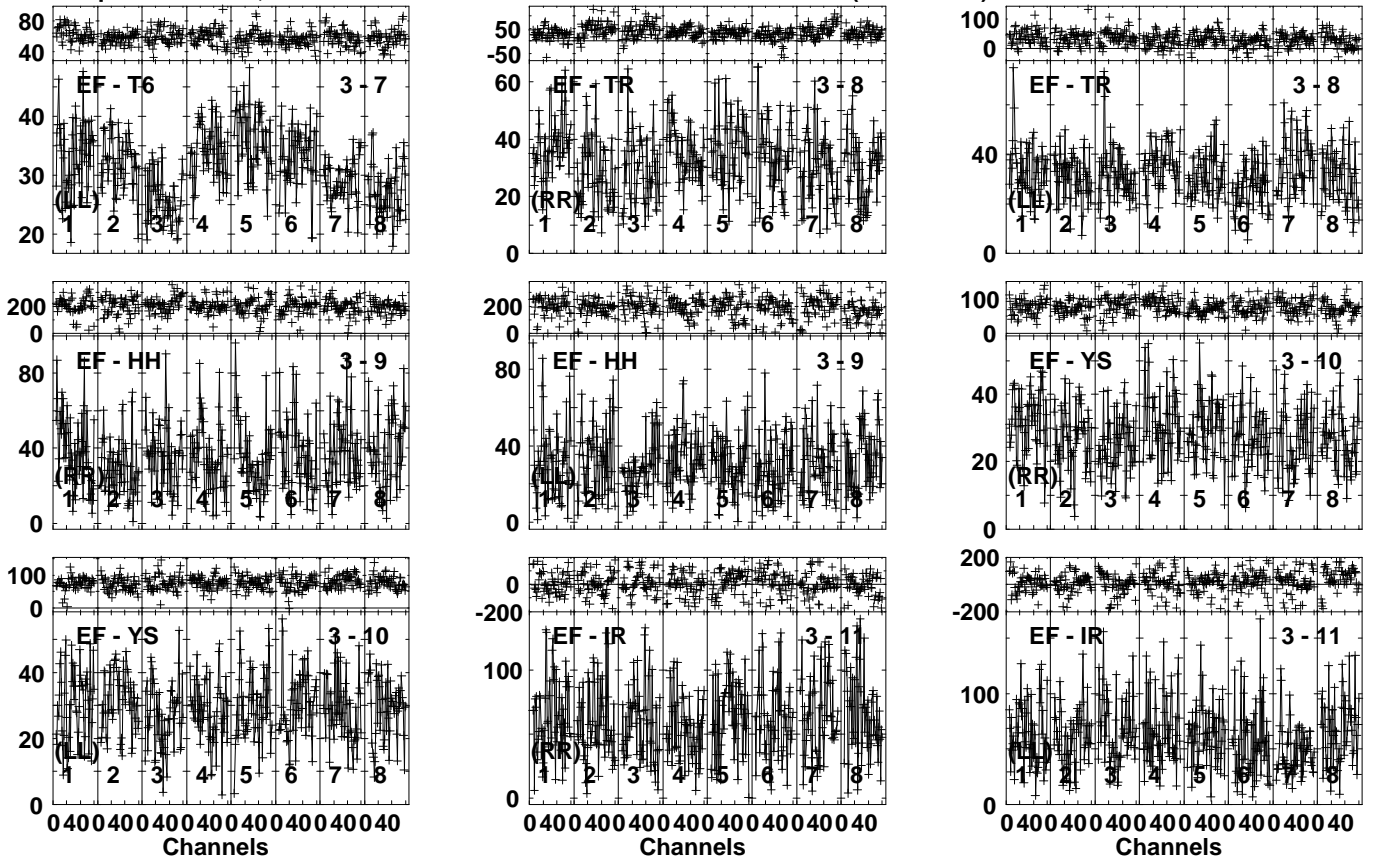
Lower frame: Milli Ampl Jy Top frame: Phas deg Vector averaged cross-power spectrum Several baselines displayed Timerange: 00/14:55:41 to 00/14:57:19
