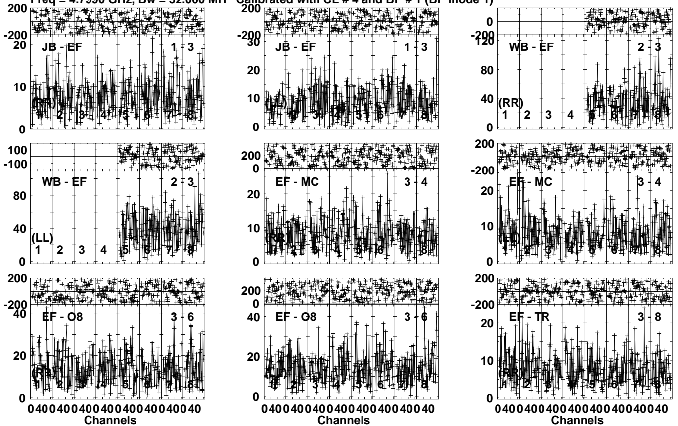
Lower frame: Milli Ampl Jy Top frame: Phas deg Vector averaged cross-power spectrum Several baselines displayed Timerange: 00/13:49:32 to 00/13:52:08
