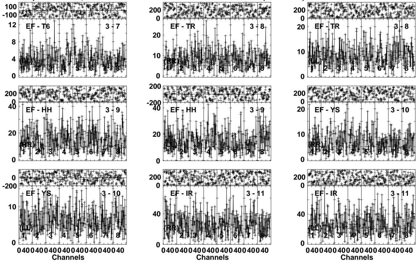
Lower frame: Milli Ampl Jy Top frame: Phas deg Vector averaged cross-power spectrum Several baselines displayed Timerange: 00/15:15:01 to 00/15:17:39
