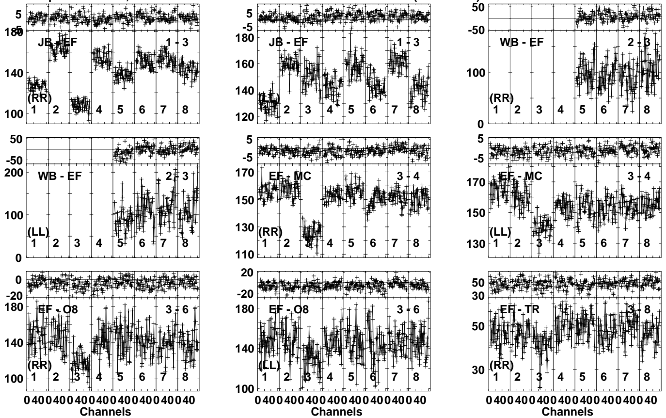
Lower frame: Milli Ampl Jy Top frame: Phas deg Vector averaged cross-power spectrum Several baselines displayed Timerange: 00/19:20:51 to 00/19:23:09
