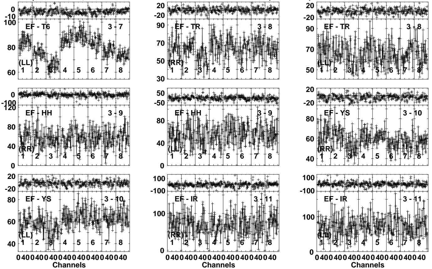
Lower frame: Milli Ampl Jy Top frame: Phas deg Vector averaged cross-power spectrum Several baselines displayed Timerange: 00/15:30:01 to 00/15:31:09
