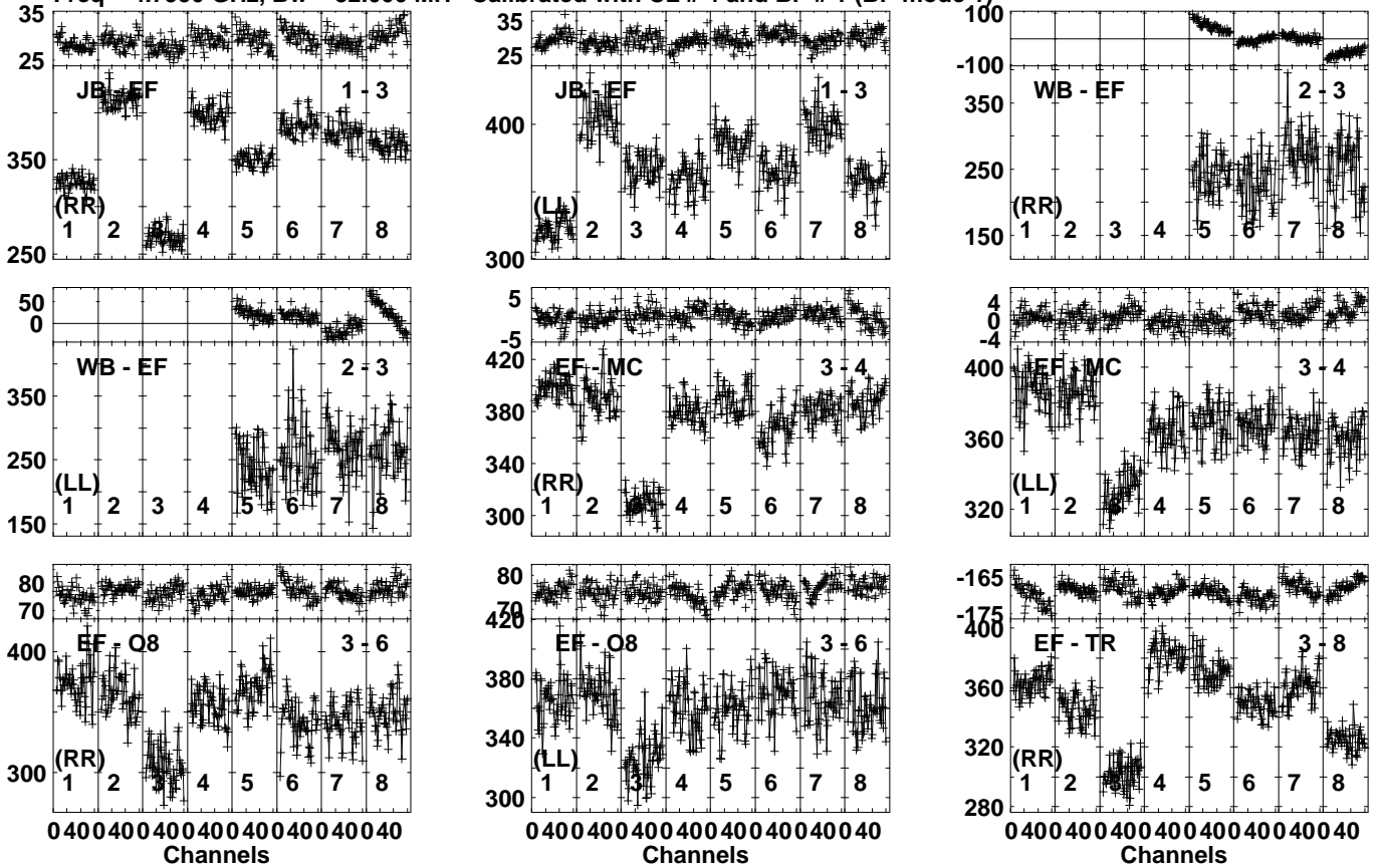
Lower frame: Milli Ampl Jy Top frame: Phas deg Vector averaged cross-power spectrum Several baselines displayed Timerange: 00/14:10:22 to 00/14:11:58
