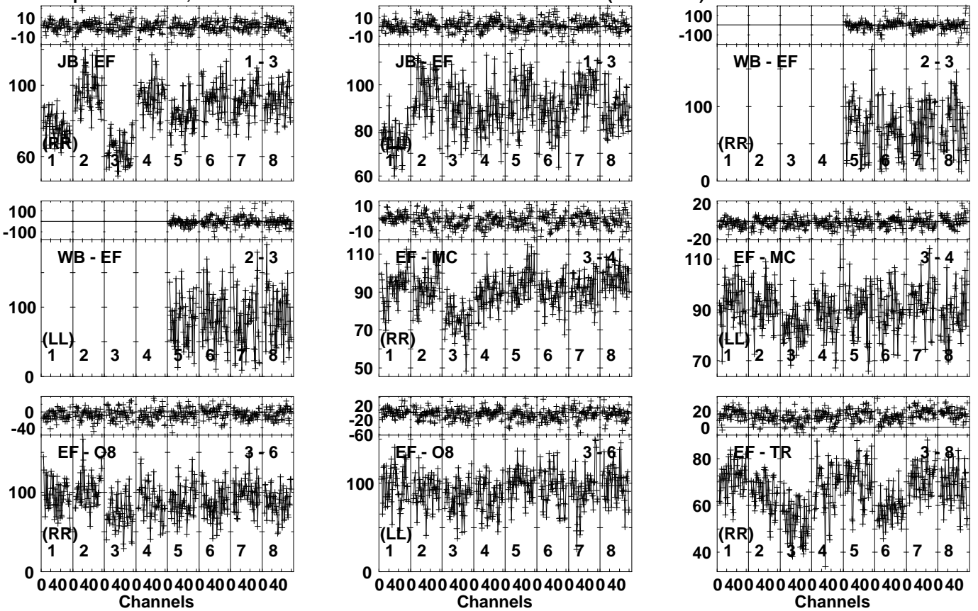
Lower frame: Milli Ampl Jy Top frame: Phas deg Vector averaged cross-power spectrum Several baselines displayed Timerange: 00/12:47:22 to 00/12:48:38
