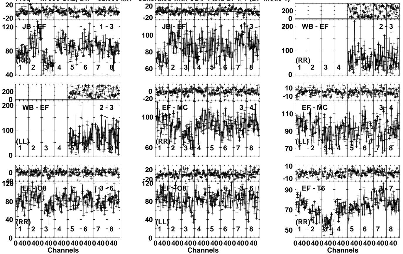
Lower frame: Milli Ampl Jy Top frame: Phas deg Vector averaged cross-power spectrum Several baselines displayed Timerange: 00:17:59:11 to 00:18:00:19
