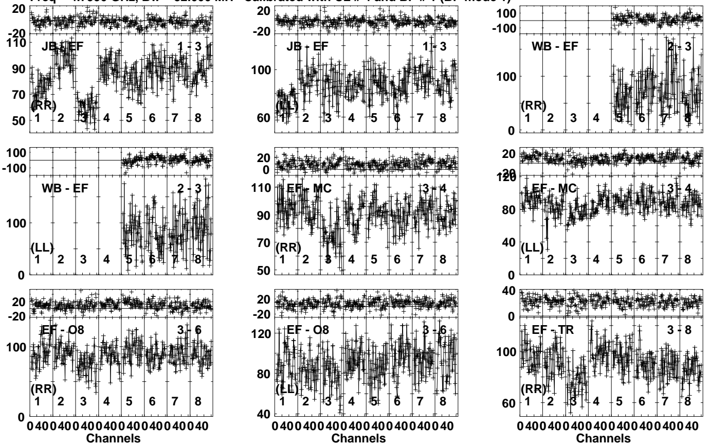
Lower frame: Milli Ampl Jy Top frame: Phas deg Vector averaged cross-power spectrum Several baselines displayed Timerange: 00/13:52:12 to 00/13:53:38
