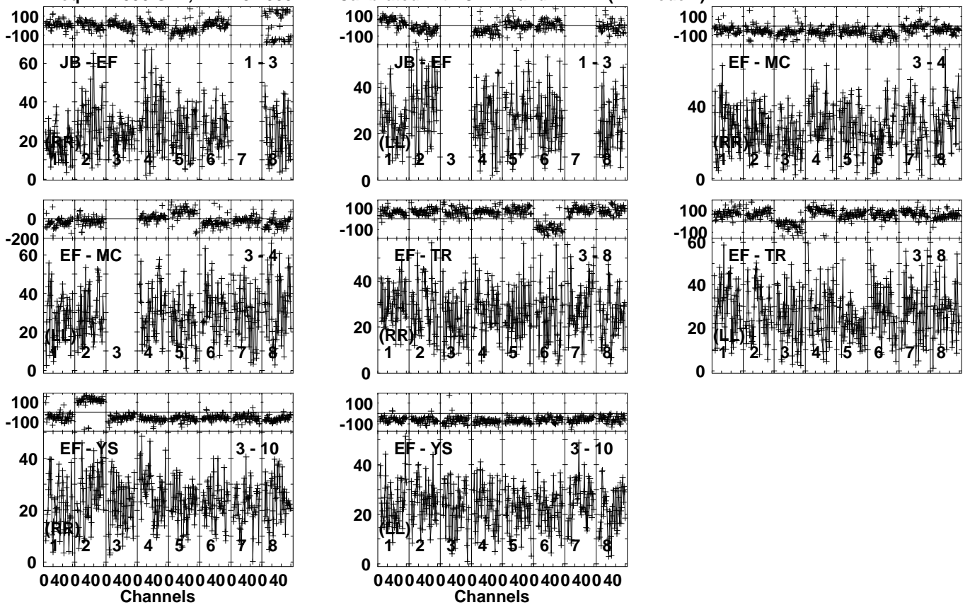
Lower frame: Milli Ampl Jy Top frame: Phas deg Vector averaged cross-power spectrum Several baselines displayed Timerange: 01/00:01:47 to 01/00:03:13
