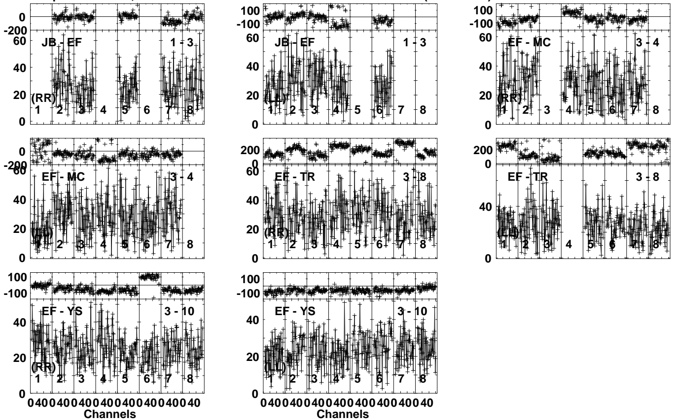
Lower frame: Milli Ampl Jy Top frame: Phas deg Vector averaged cross-power spectrum Several baselines displayed Timerange: 01/00:37:01 to 01/00:38:29
