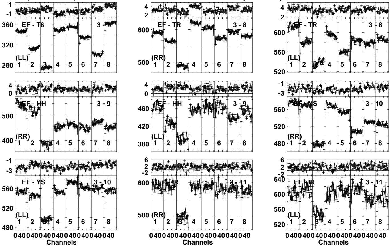
Lower frame: Milli Ampl Jy Top frame: Phas deg Vector averaged cross-power spectrum Several baselines displayed Timerange: 00/12:13:02 to 00/12:16:58
