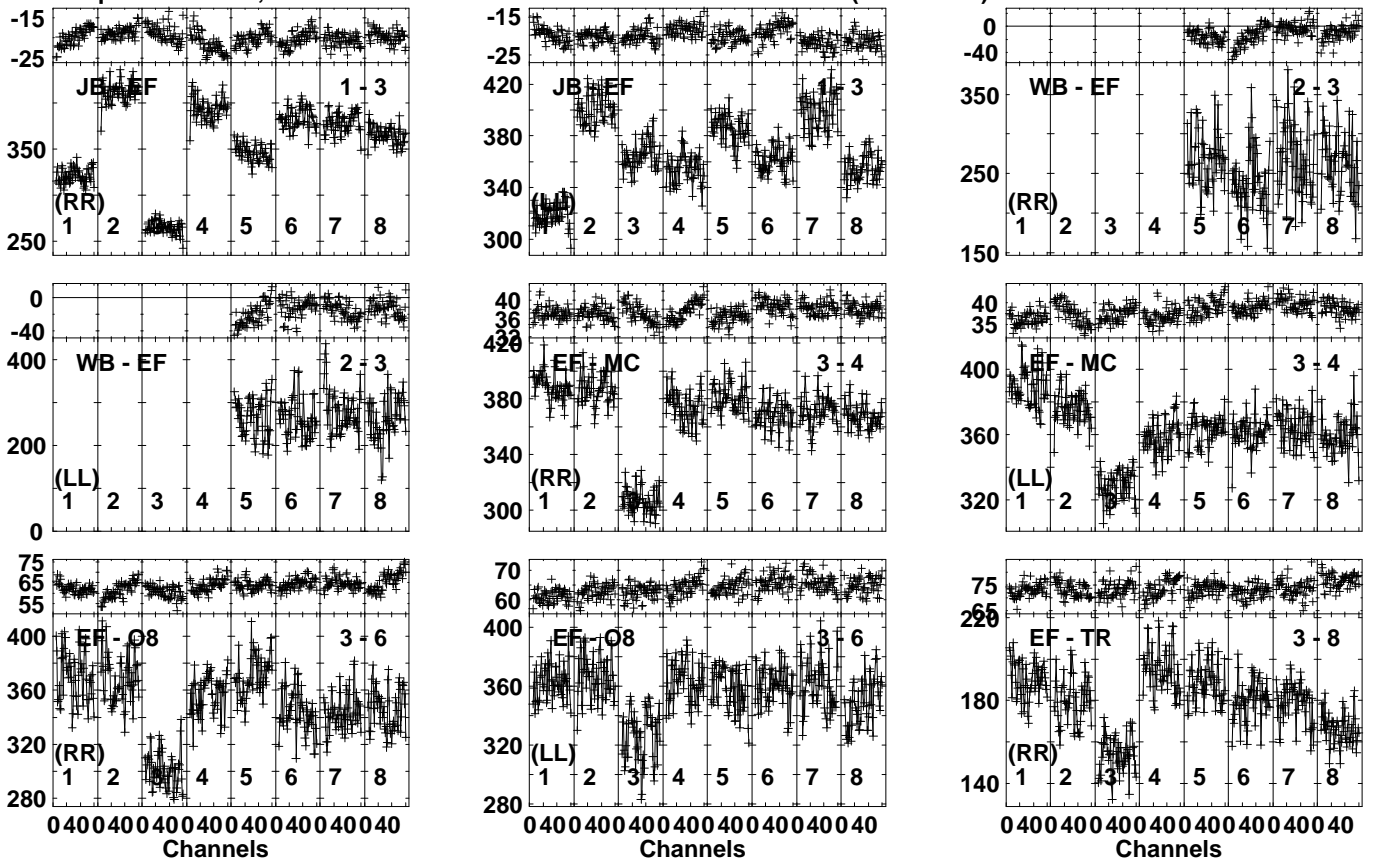
Lower frame: Milli Ampl Jy Top frame: Phas deg Vector averaged cross-power spectrum Several baselines displayed Timerange: 00/13:58:12 to 00/13:59:48
