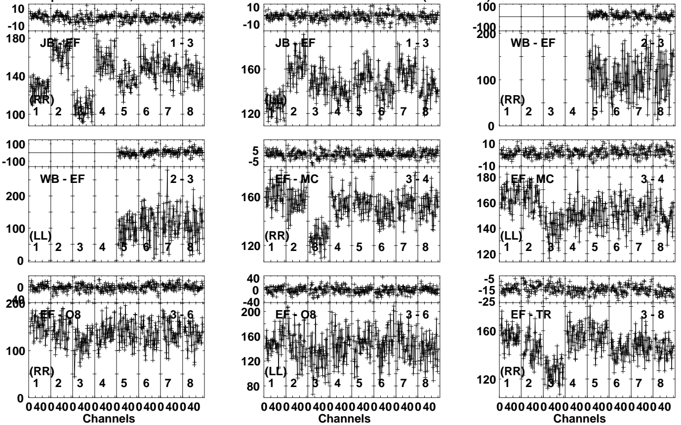
Lower frame: Milli Ampl Jy Top frame: Phas deg Vector averaged cross-power spectrum Several baselines displayed Timerange: 00/19:32:01 to 00/19:33:09
