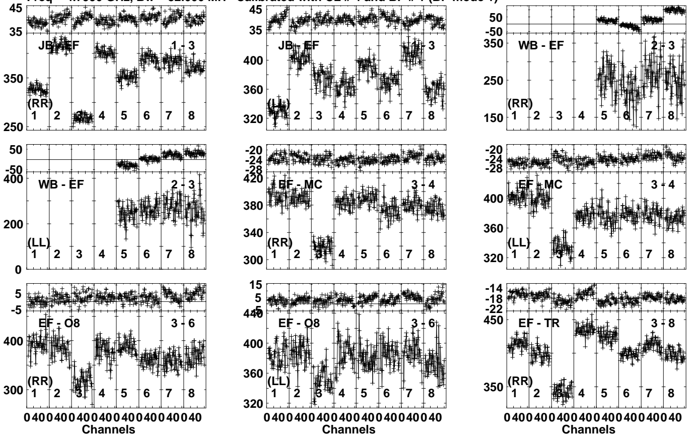
Lower frame: Milli Ampl Jy Top frame: Phas deg Vector averaged cross-power spectrum Several baselines displayed Timerange: 00/12:33:02 to 00/12:34:38
