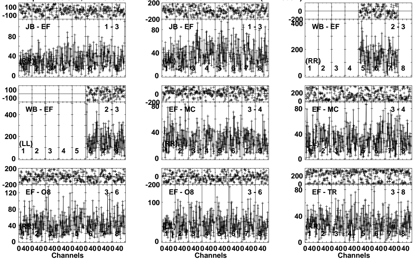
Lower frame: Milli Ampl Jy Top frame: Phas deg Vector averaged cross-power spectrum Several baselines displayed Timerange: 00/20:03:41 to 00/20:04:49
