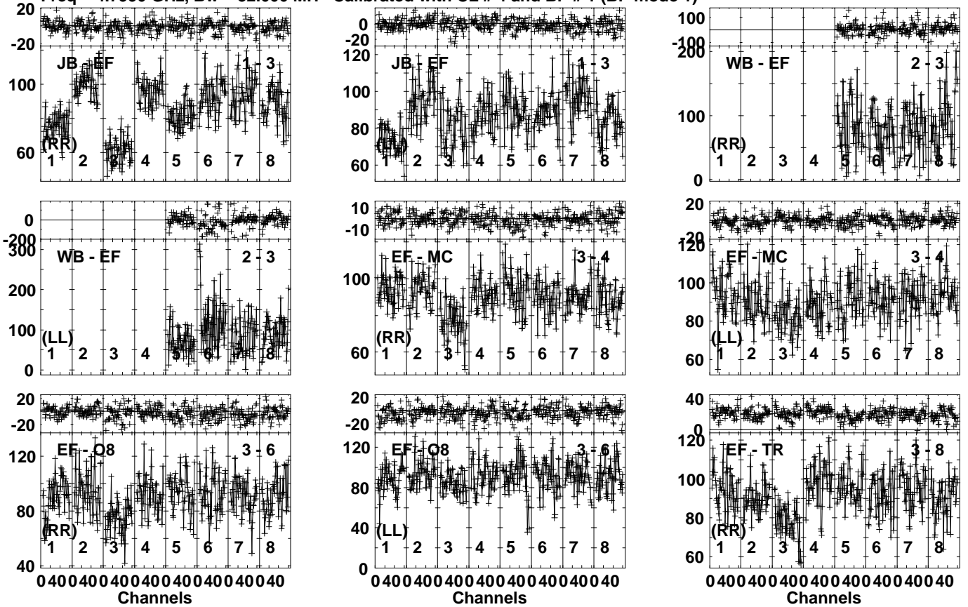
Lower frame: Milli Ampl Jy Top frame: Phas deg Vector averaged cross-power spectrum Several baselines displayed Timerange: 00/12:51:22 to 00/12:52:48
