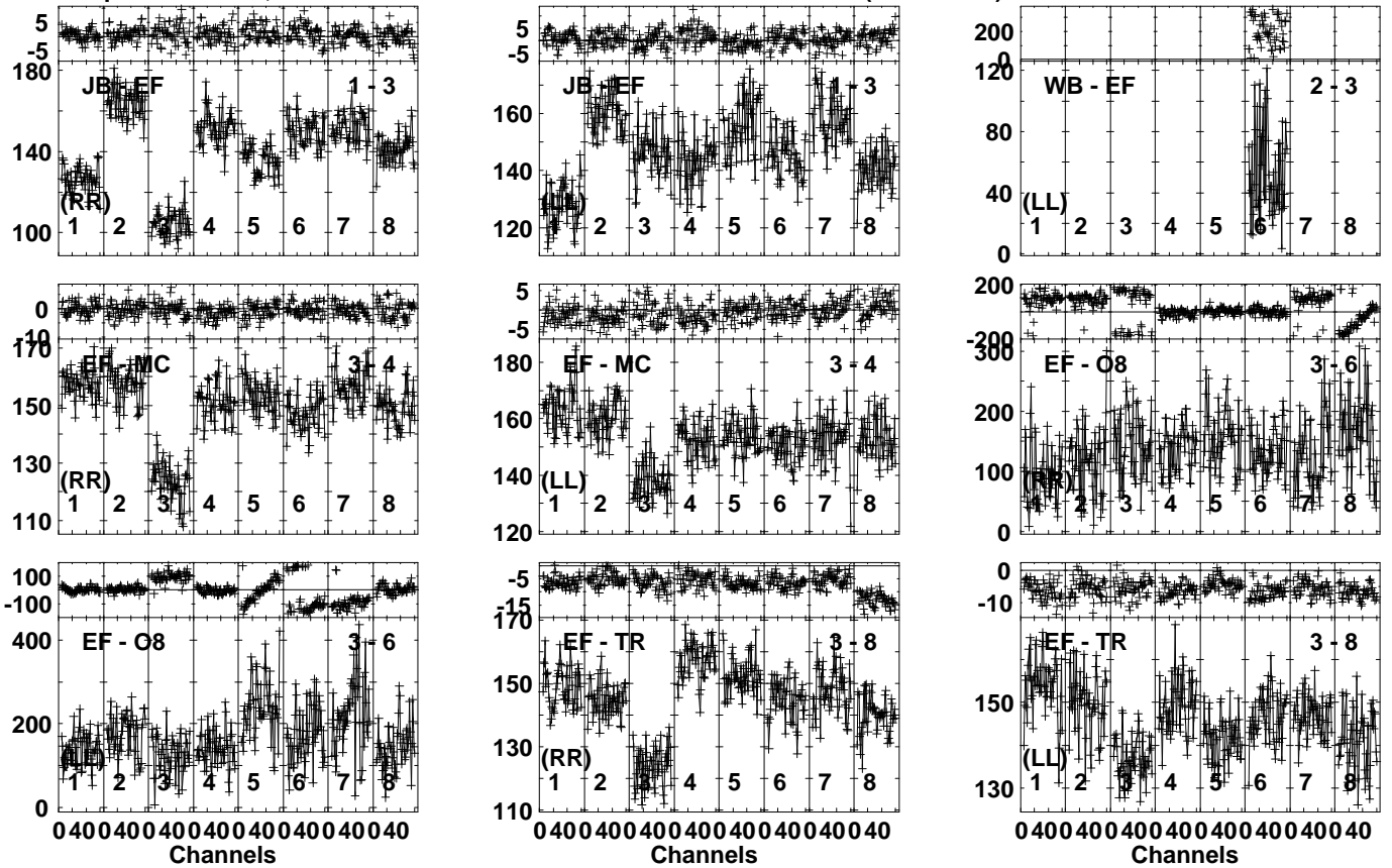
Lower frame: Milli Ampl Jy Top frame: Phas deg Vector averaged cross-power spectrum Several baselines displayed Timerange: 00/20:07:31 to 00/20:09:49
