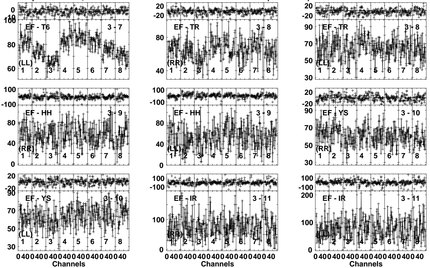
Lower frame: Milli Ampl Jy Top frame: Phas deg Vector averaged cross-power spectrum Several baselines displayed Timerange: 00/14:57:51 to 00/14:58:59
