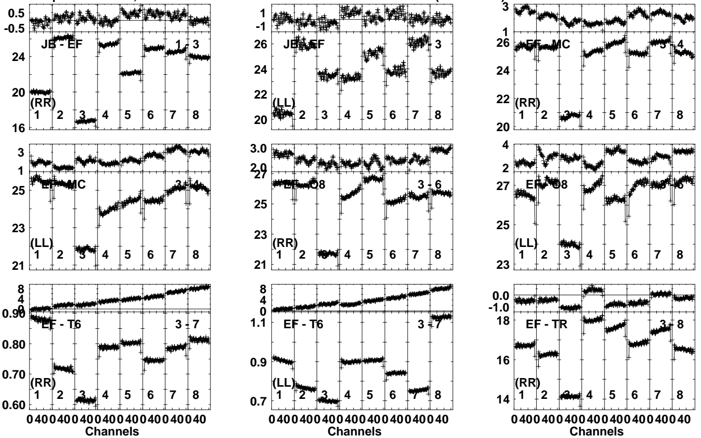
Lower frame: Ampl Jy Top frame: Phas deg Vector averaged cross-power spectrum Several baselines displayed Timerange: 00/11:52:46 to 00/12:02:58
