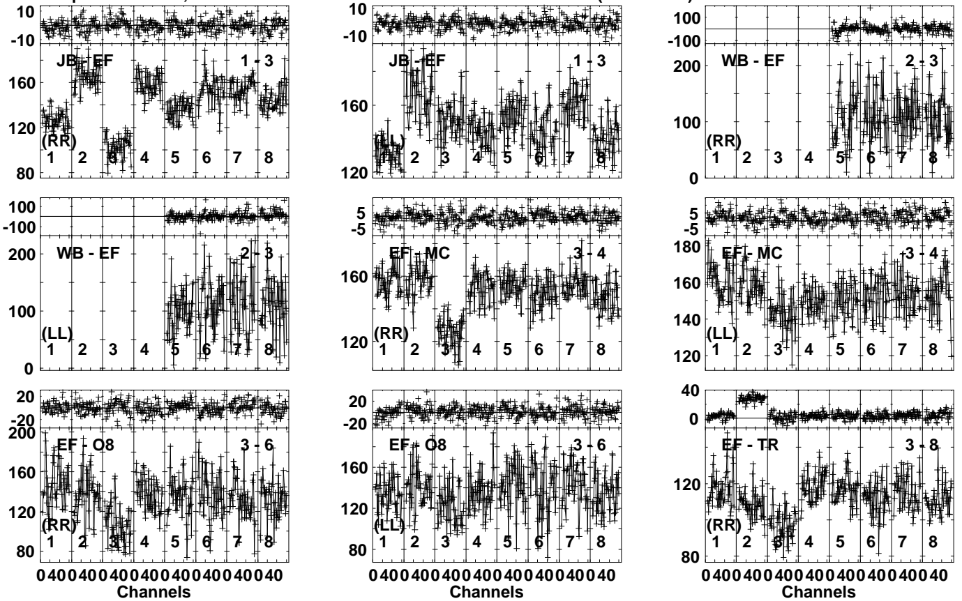
Lower frame: Milli Ampl Jy Top frame: Phas deg Vector averaged cross-power spectrum Several baselines displayed Timerange: 00:19:39:11 to 00:19:40:19
