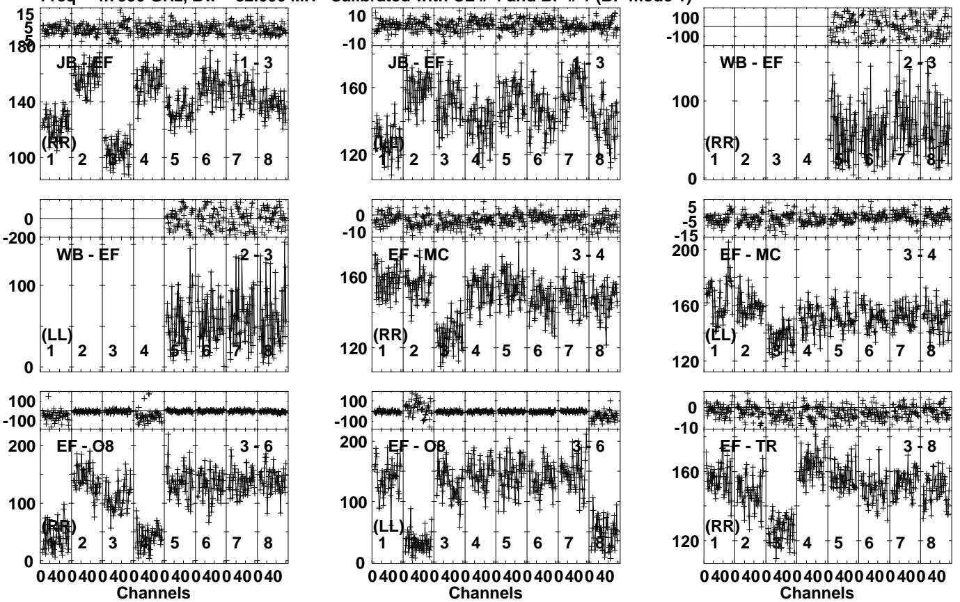
Lower frame: Milli Ampl Jy Top frame: Phas deg Vector averaged cross-power spectrum Several baselines displayed Timerange: 00/18:42:31 to 00/18:43:39
