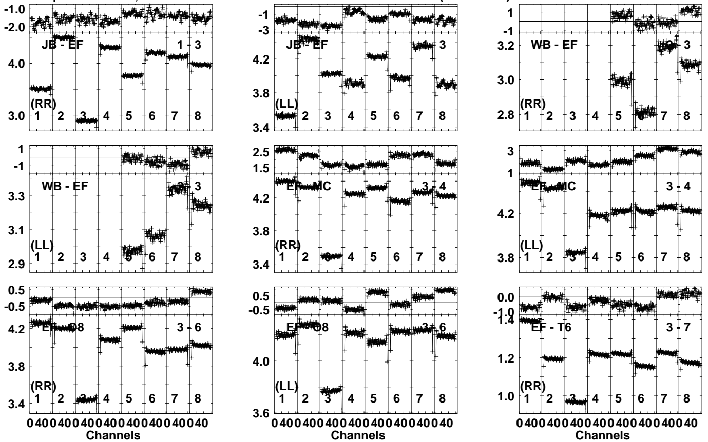
Lower frame: Ampl Jy Top frame: Phas deg Vector averaged cross-power spectrum Several baselines displayed Timerange: 00/16:56:31 to 00/17:00:29
