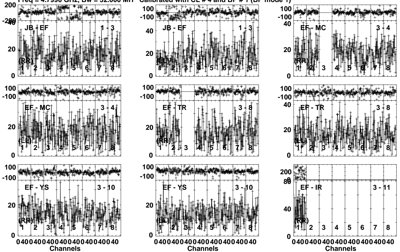
Lower frame: Milli Ampl Jy Top frame: Phas deg Vector averaged cross-power spectrum Several baselines displayed Timerange: 00/23:25:11 to 00/23:26:29
