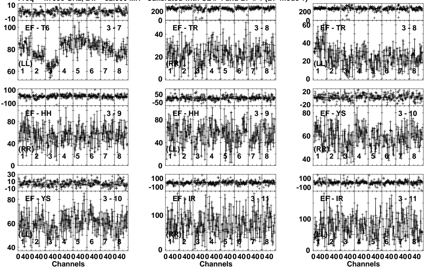
Lower frame: Milli Ampl Jy Top frame: Phas deg Vector averaged cross-power spectrum Several baselines displayed Timerange: 00/16:17:21 to 00/16:18:29
