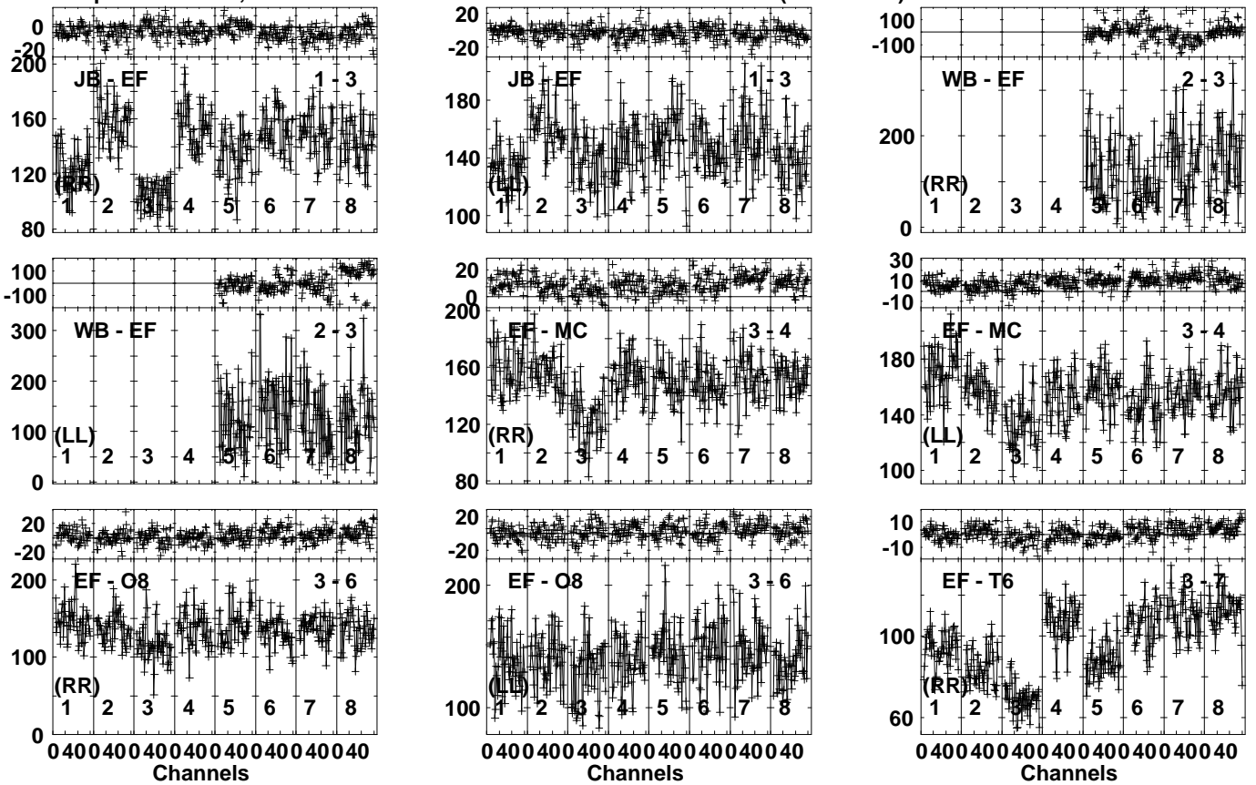
Lower frame: Milli Ampl Jy Top frame: Phas deg Vector averaged cross-power spectrum Several baselines displayed Timerange: 00/18:18:41 to 00/18:19:49
