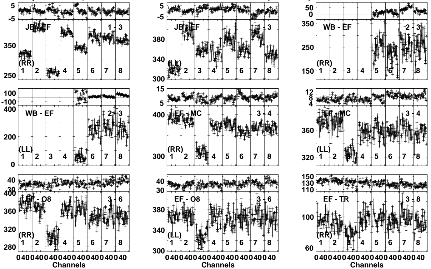
Lower frame: Milli Ampl Jy Top frame: Phas deg Vector averaged cross-power spectrum Several baselines displayed Timerange: 00/13:21:42 to 00/13:23:18
