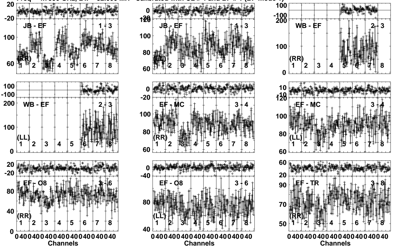
Lower frame: Milli Ampl Jy Top frame: Phas deg Vector averaged cross-power spectrum Several baselines displayed Timerange: 00/20:02:31 to 00/20:03:39
