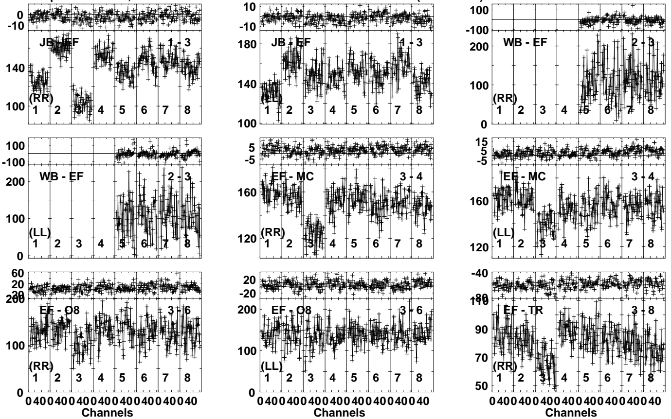
Lower frame: Milli Ampl Jy Top frame: Phas deg Vector averaged cross-power spectrum Several baselines displayed Timerange: 00/18:45:21 to 00/18:46:29
