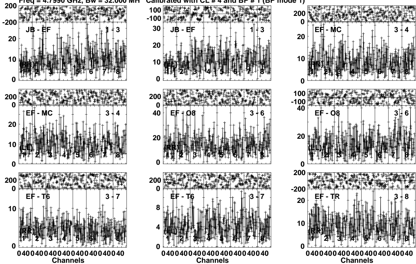
Lower frame: Milli Ampl Jy Top frame: Phas deg Vector averaged cross-power spectrum Several baselines displayed Timerange: 00/16:45:31 to 00/16:47:39
