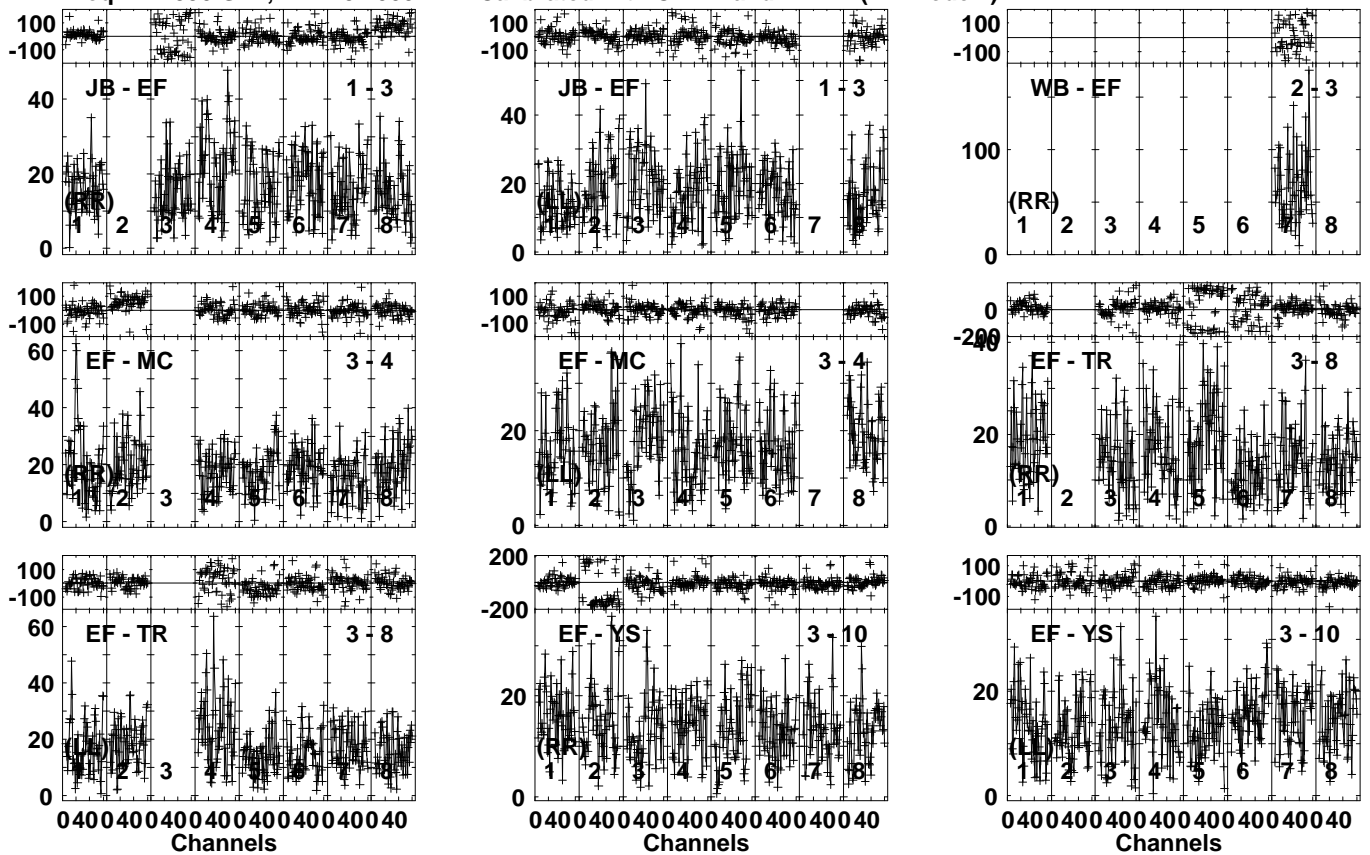
Lower frame: Milli Ampl Jy Top frame: Phas deg Vector averaged cross-power spectrum Several baselines displayed Timerange: 01/00:12:11 to 01/00:13:29
