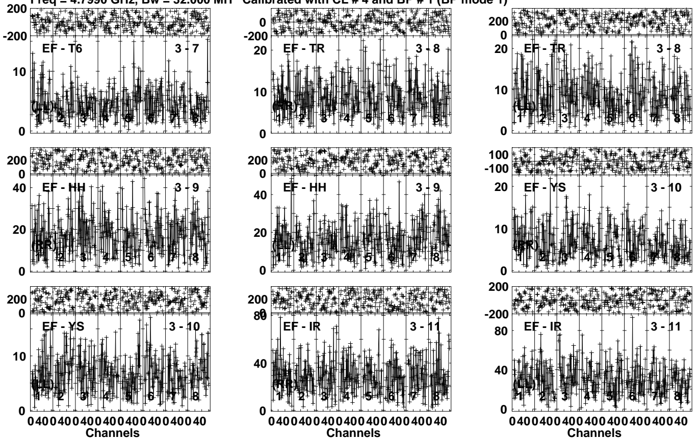
Lower frame: Milli Ampl Jy Top frame: Phas deg Vector averaged cross-power spectrum Several baselines displayed Timerange: 00/16:28:51 to 00/16:30:59
