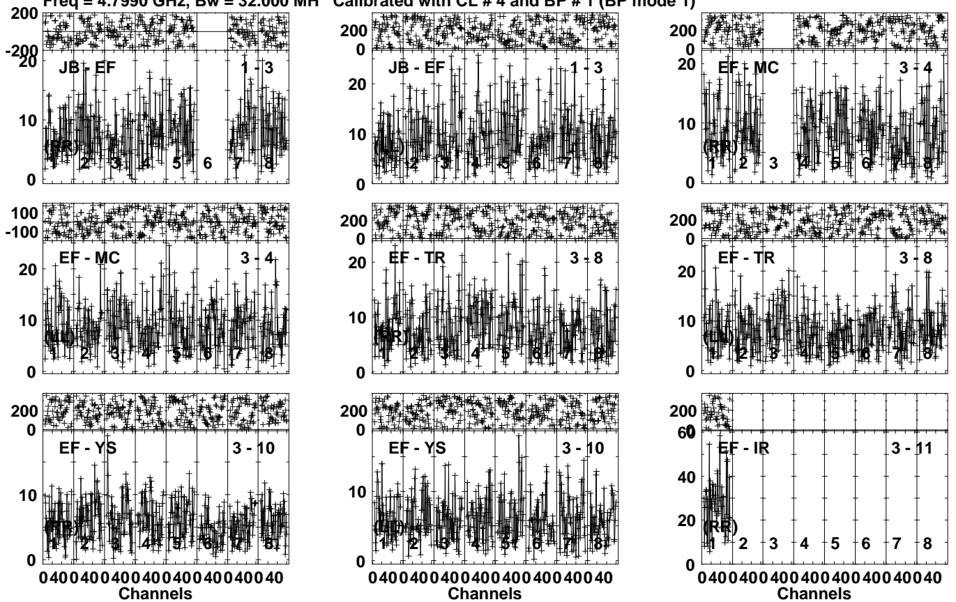
Lower frame: Milli Ampl Jy Top frame: Phas deg Vector averaged cross-power spectrum Several baselines displayed Timerange: 00/23:29:51 to 00/23:32:23
