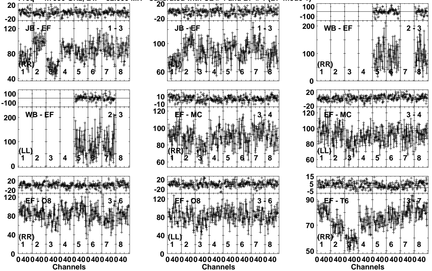
Lower frame: Milli Ampl Jy Top frame: Phas deg Vector averaged cross-power spectrum Several baselines displayed Timerange: 00/17:49:11 to 00/17:50:19
