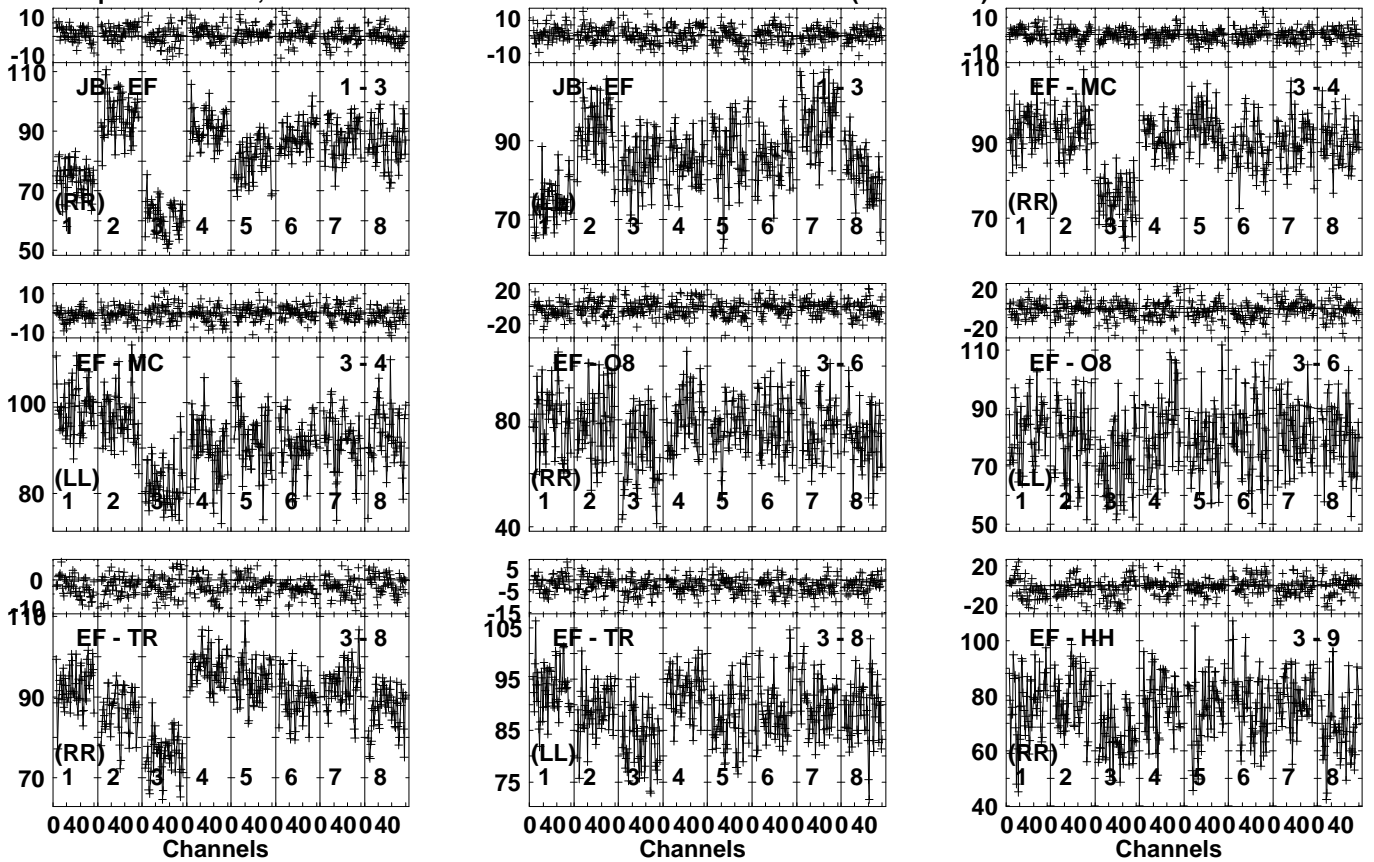
Lower frame: Milli Ampl Jy Top frame: Phas deg Vector averaged cross-power spectrum Several baselines displayed Timerange: 00/18:47:31 to 00/18:49:49
