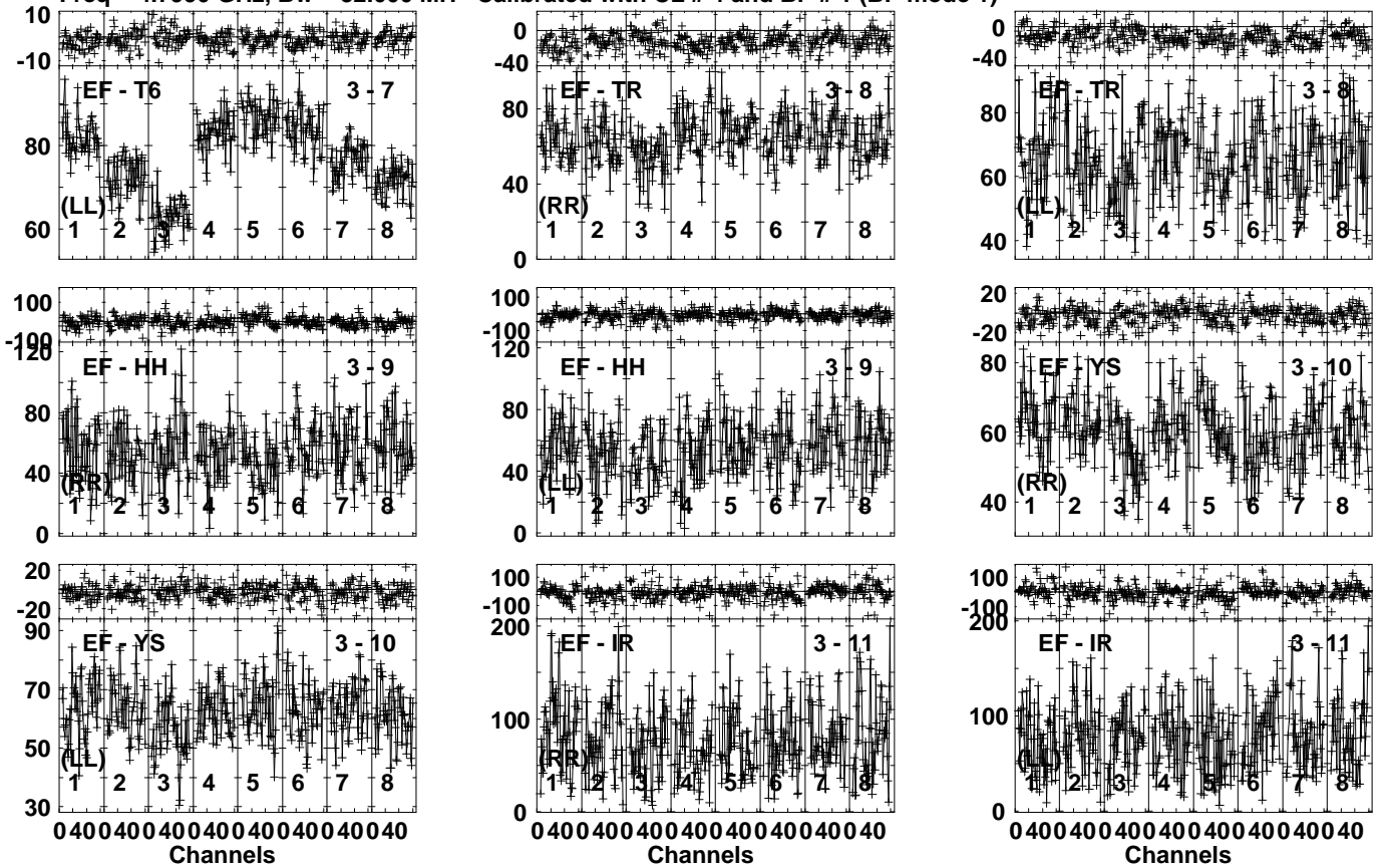
Lower frame: Milli Ampl Jy Top frame: Phas deg Vector averaged cross-power spectrum Several baselines displayed Timerange: 00/14:54:31 to 00/14:55:39
