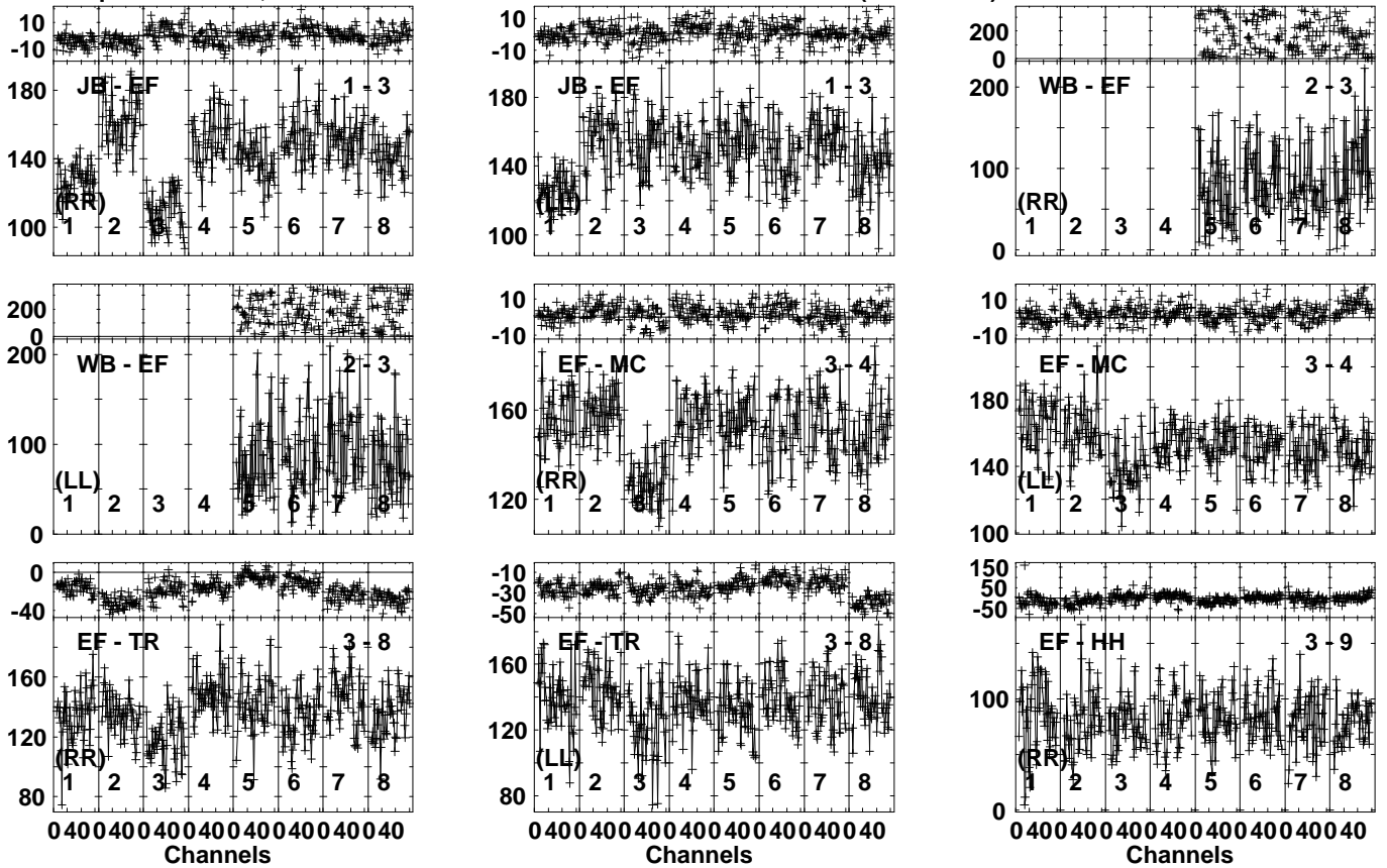
Lower frame: Milli Ampl Jy Top frame: Phas deg Vector averaged cross-power spectrum Several baselines displayed Timerange: 00/20:22:41 to 00/20:23:49
