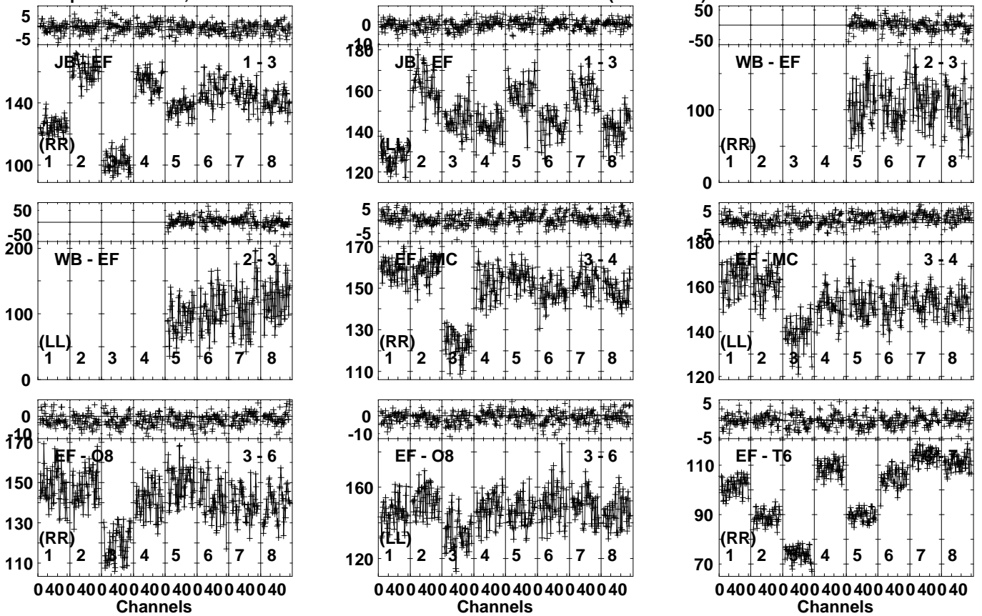
Lower frame: Milli Ampl Jy Top frame: Phas deg Vector averaged cross-power spectrum Several baselines displayed Timerange: 00/18:14:11 to 00/18:16:29
