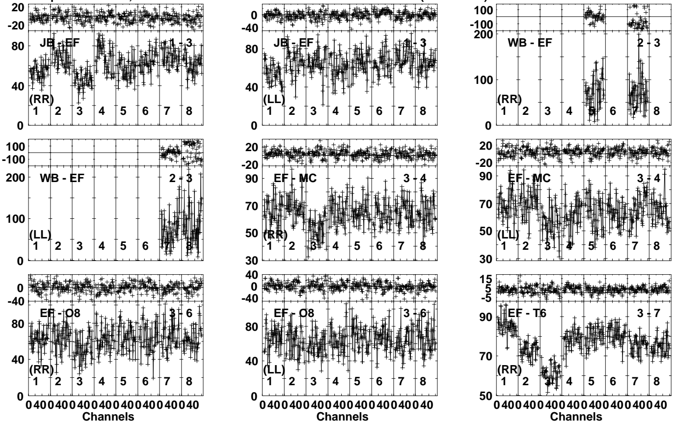
Lower frame: Milli Ampl Jy Top frame: Phas deg Vector averaged cross-power spectrum Several baselines displayed Timerange: 00/16:08:51 to 00/16:09:59
