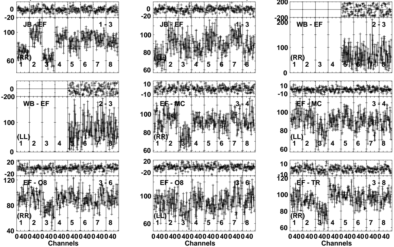
Lower frame: Milli Ampl Jy Top frame: Phas deg Vector averaged cross-power spectrum Several baselines displayed Timerange: 00/12:35:12 to 00/12:36:28
