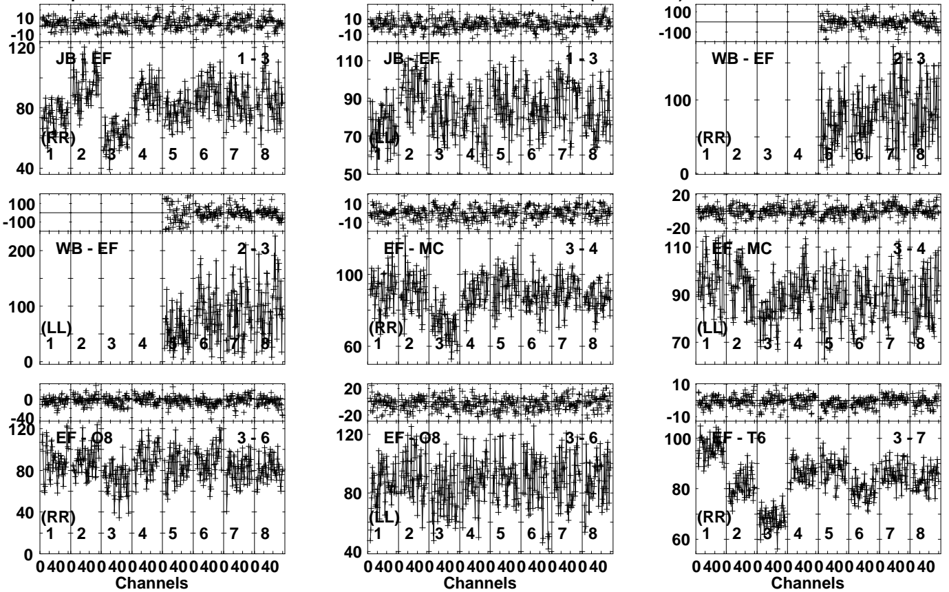
Lower frame: Milli Ampl Jy Top frame: Phas deg Vector averaged cross-power spectrum Several baselines displayed Timerange: 00:16:31:31 to 00:16:32:39
