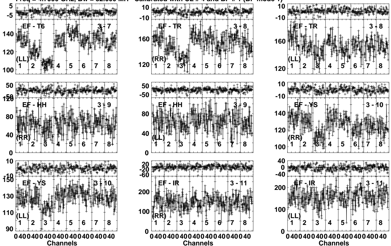
Lower frame: Milli Ampl Jy Top frame: Phas deg Vector averaged cross-power spectrum Several baselines displayed Timerange: 00/17:19:21 to 00/17:20:29
