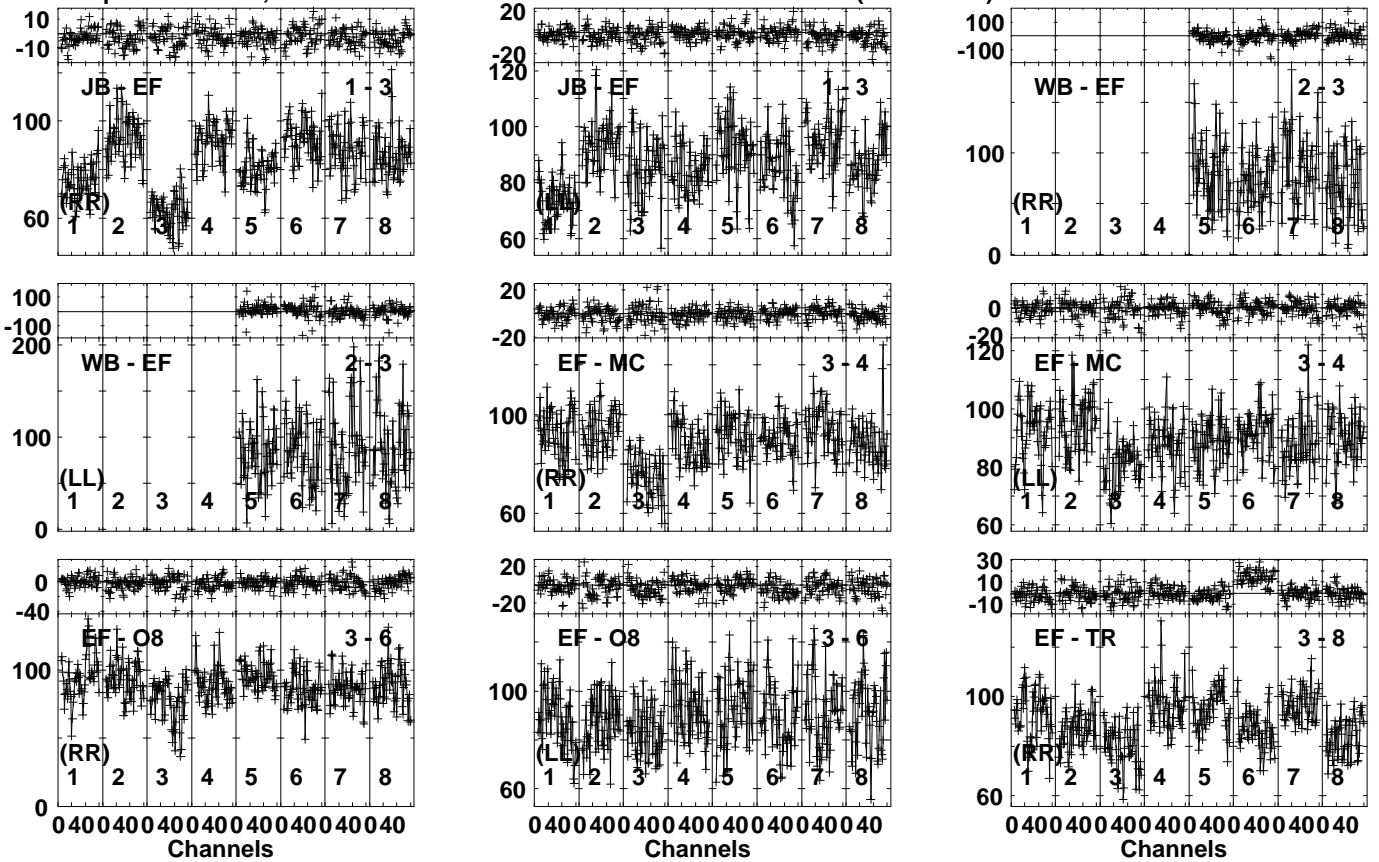
Lower frame: Milli Ampl Jy Top frame: Phas deg Vector averaged cross-power spectrum Several baselines displayed Timerange: 00/14:00:22 to 00/14:01:38
