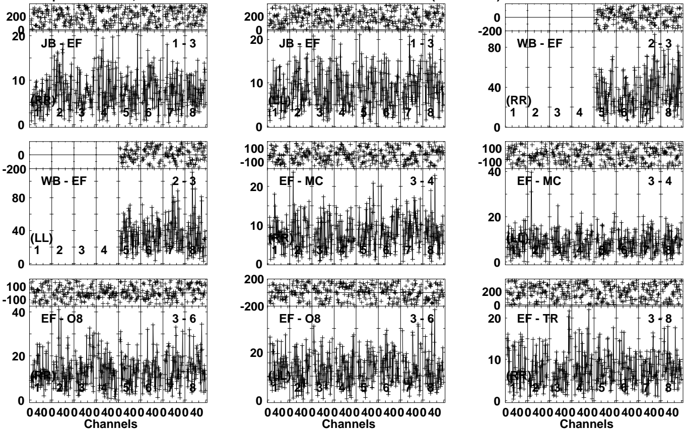
Lower frame: Milli Ampl Jy Top frame: Phas deg Vector averaged cross-power spectrum Several baselines displayed Timerange: 00/13:53:42 to 00/13:56:18
