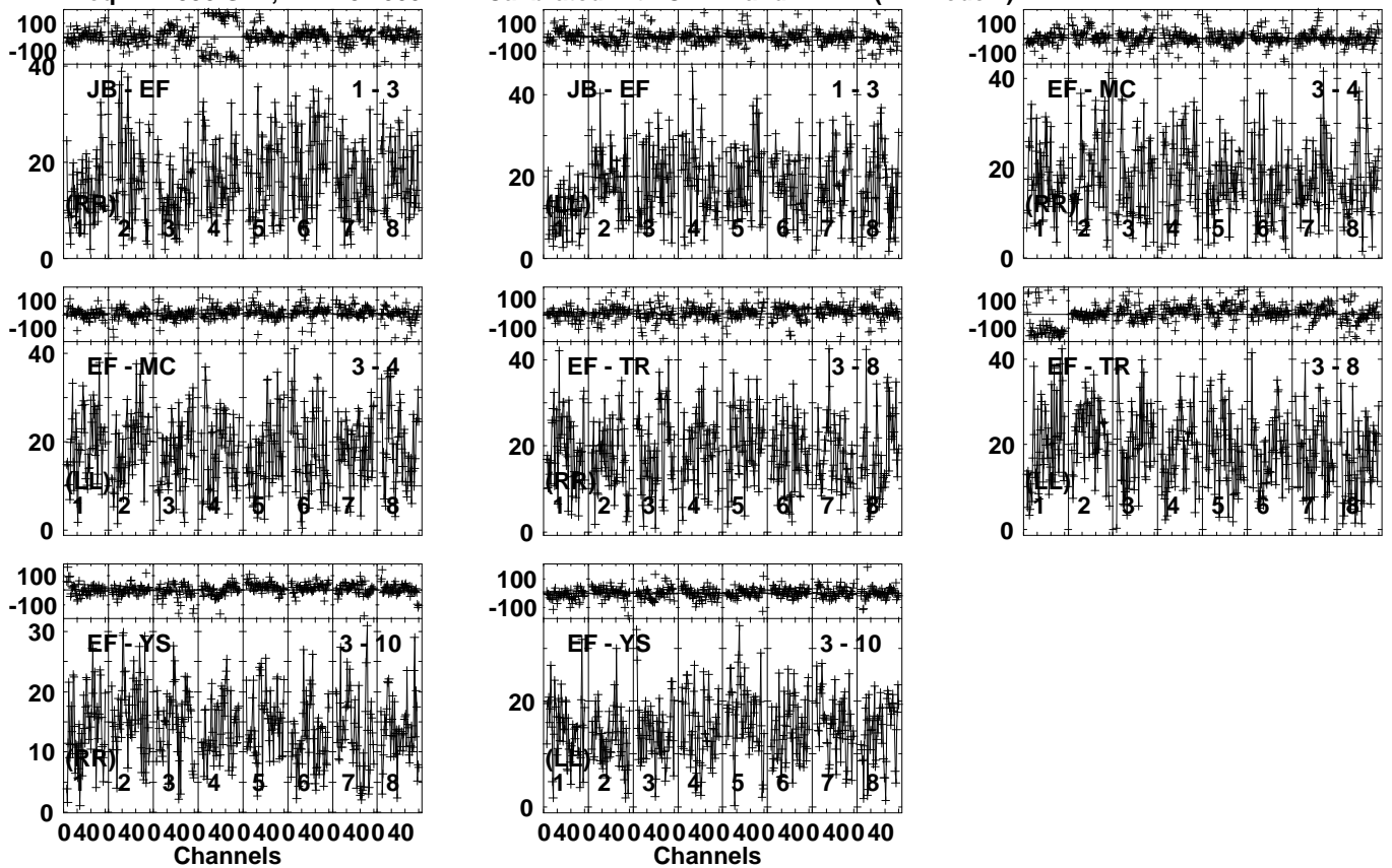
Lower frame: Milli Ampl Jy Top frame: Phas deg Vector averaged cross-power spectrum Several baselines displayed Timerange: 00/21:58:27 to 00/21:59:53
