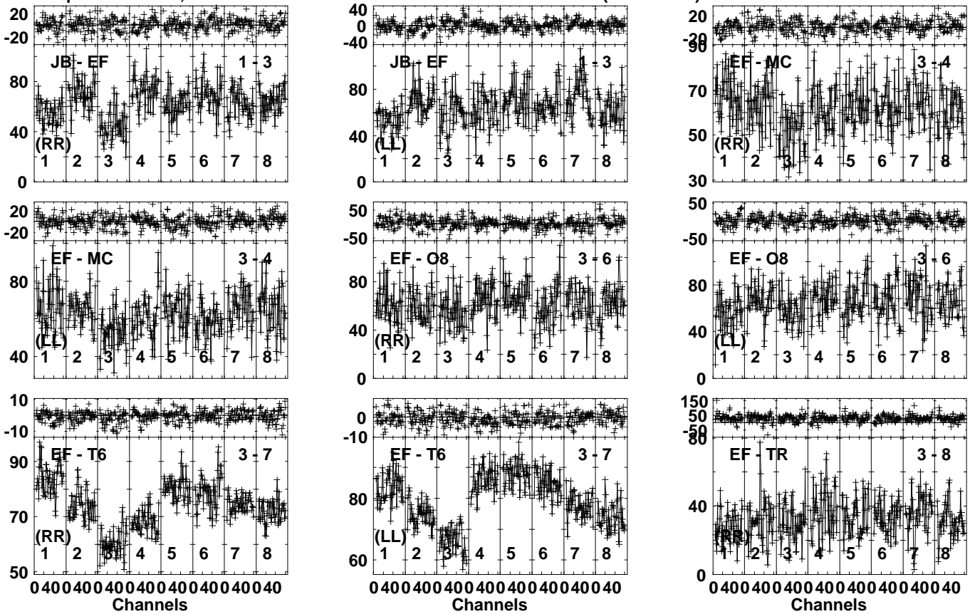
Lower frame: Milli Ampl Jy Top frame: Phas deg Vector averaged cross-power spectrum Several baselines displayed Timerange: 00/15:06:21 to 00/15:07:29
