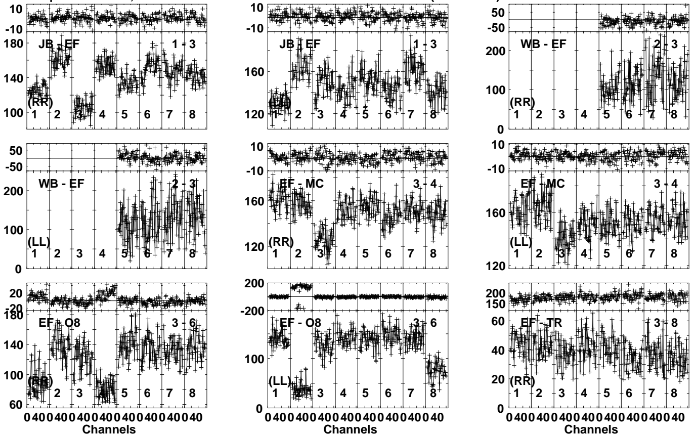
Lower frame: Milli Ampl Jy Top frame: Phas deg Vector averaged cross-power spectrum Several baselines displayed Timerange: 00:18:35:21 to 00:18:36:29
