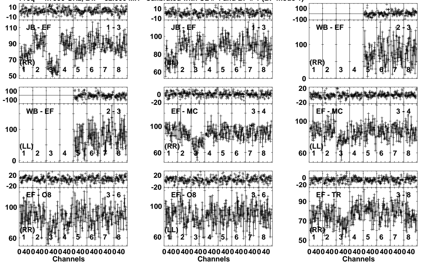
Lower frame: Milli Ampl Jy Top frame: Phas deg Vector averaged cross-power spectrum Several baselines displayed Timerange: 00/13:56:52 to 00/13:58:08
