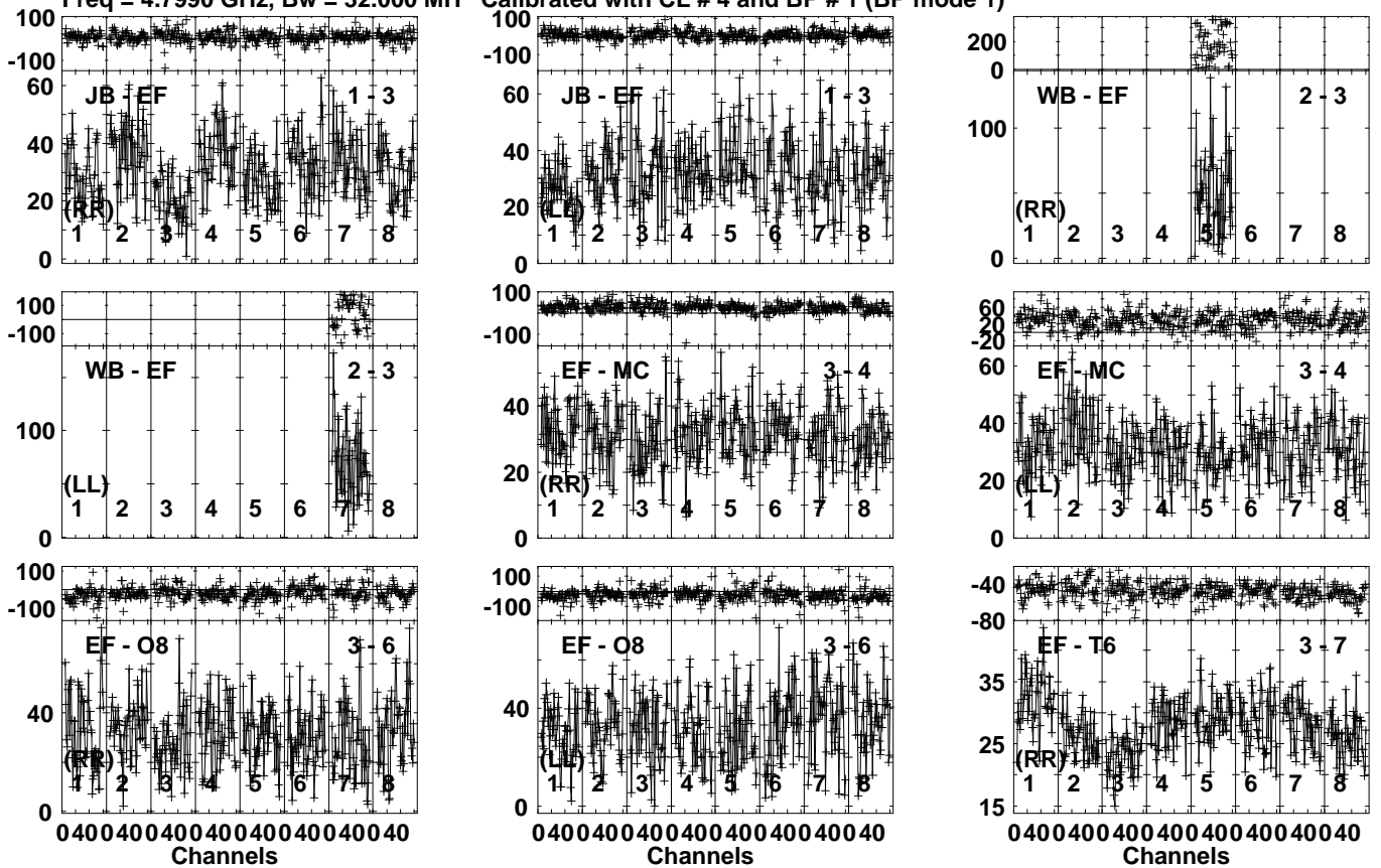
Lower frame: Milli Ampl Jy Top frame: Phas deg Vector averaged cross-power spectrum Several baselines displayed Timerange: 00/16:06:41 to 00/16:08:19
