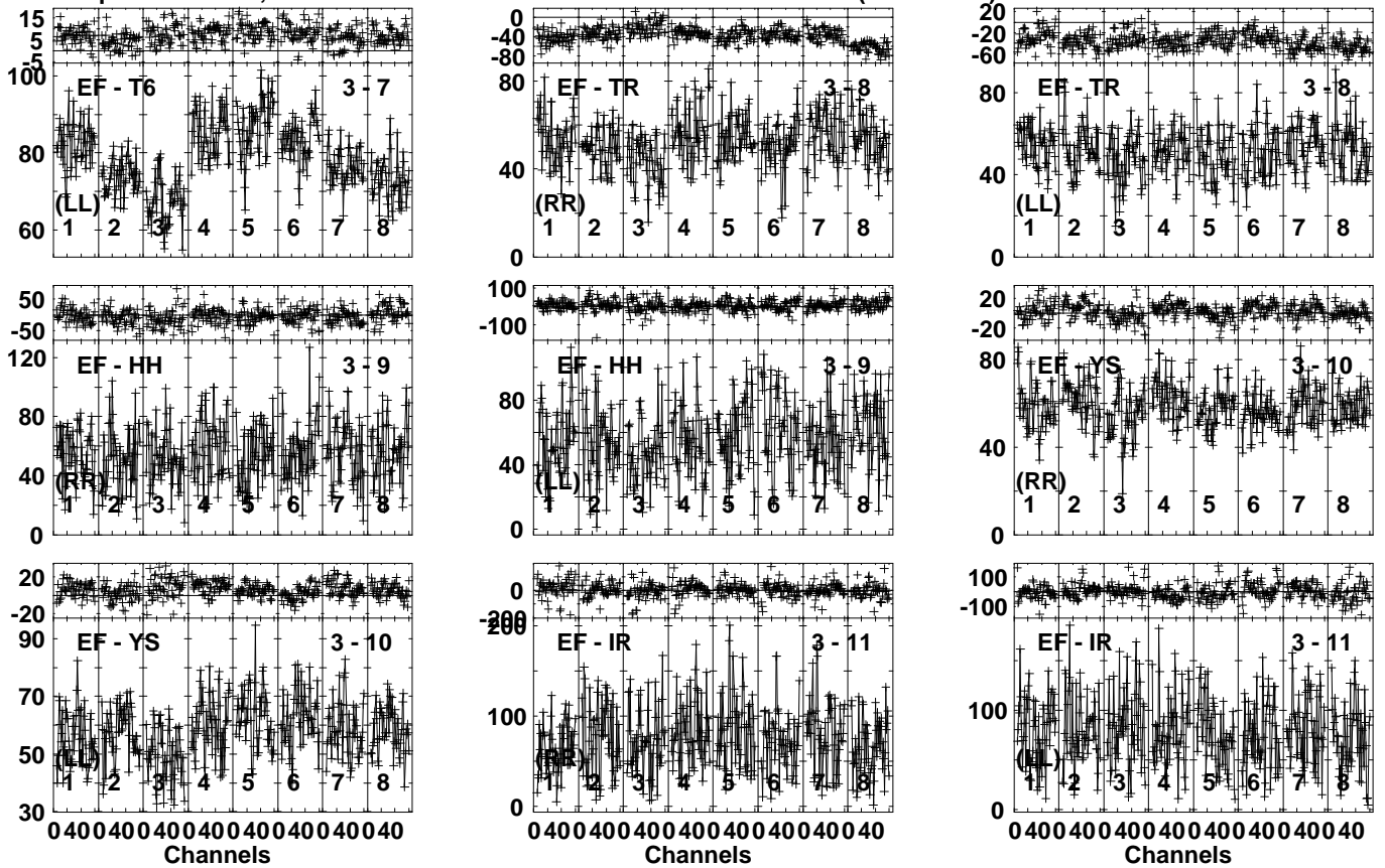
Lower frame: Milli Ampl Jy Top frame: Phas deg Vector averaged cross-power spectrum Several baselines displayed Timerange: 00/16:12:41 to 00/16:14:09
