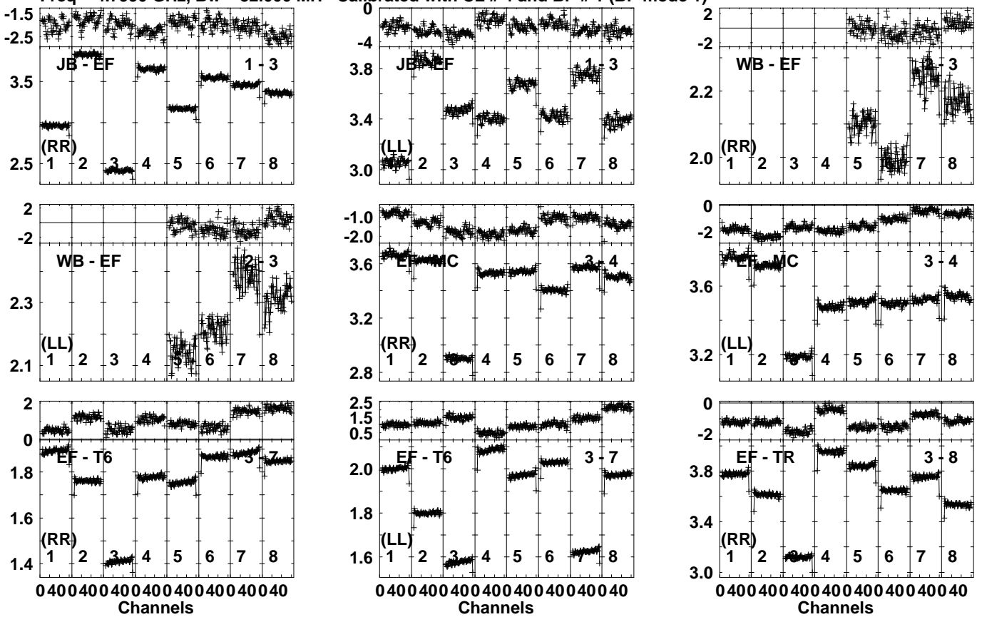
Lower frame: Ampl Jy Top frame: Phas deg Vector averaged cross-power spectrum Several baselines displayed Timerange: 01/01:14:49 to 01/01:16:39
