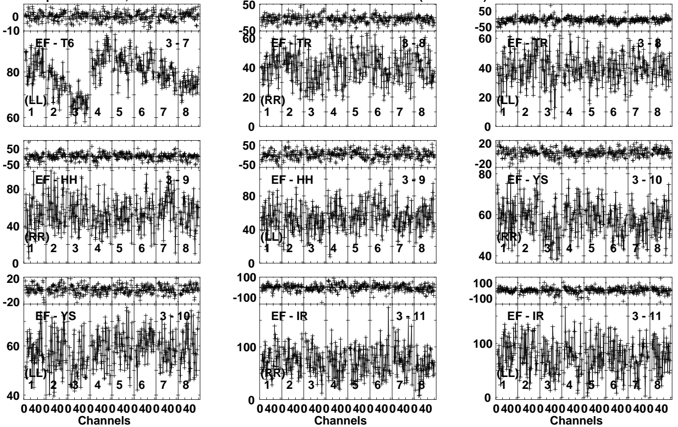
Lower frame: Milli Ampl Jy Top frame: Phas deg Vector averaged cross-power spectrum Several baselines displayed Timerange: 00/16:20:41 to 00/16:21:49
