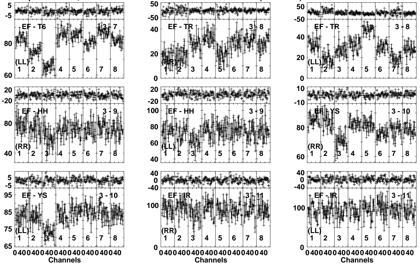
Lower frame: Milli Ampl Jy Top frame: Phas deg Vector averaged cross-power spectrum Several baselines displayed Timerange: 00/17:40:51 to 00/17:43:09
