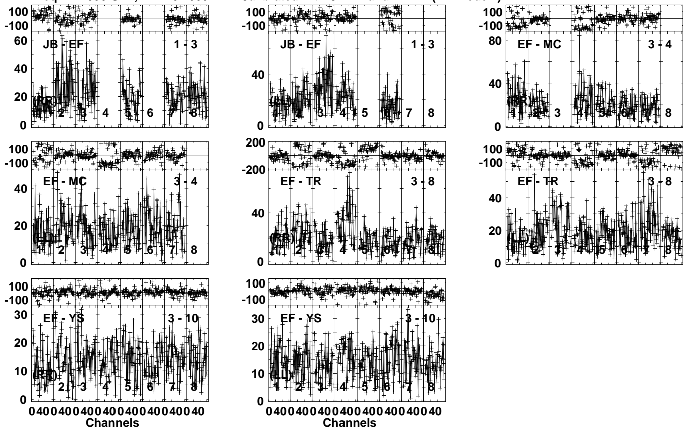
Lower frame: Milli Ampl Jy Top frame: Phas deg Vector averaged cross-power spectrum Several baselines displayed Timerange: 01/00:39:01 to 01/00:40:19
