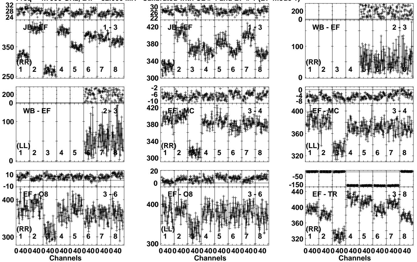
Lower frame: Milli Ampl Jy Top frame: Phas deg Vector averaged cross-power spectrum Several baselines displayed Timerange: 00/12:57:22 to 00/12:58:58
