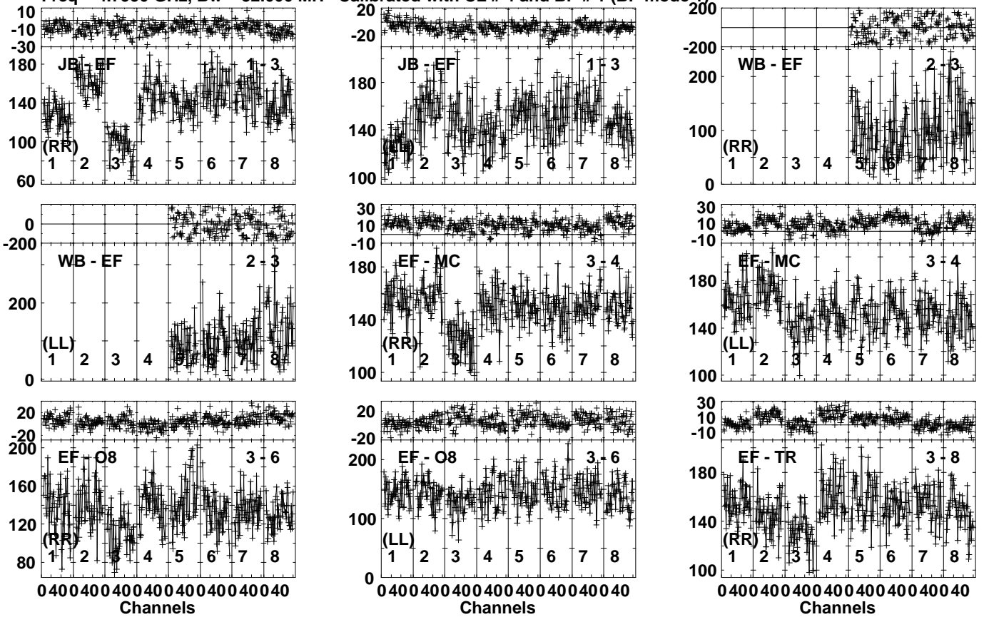
Lower frame: Milli Ampl Jy Top frame: Phas deg Vector averaged cross-power spectrum Several baselines displayed Timerange: 00/18:28:41 to 00/18:29:49
