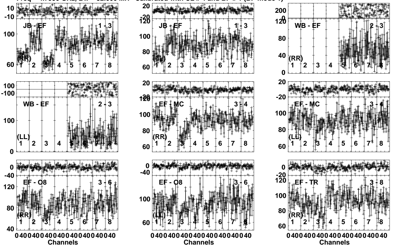
Lower frame: Milli Ampl Jy Top frame: Phas deg Vector averaged cross-power spectrum Several baselines displayed Timerange: 00/12:39:12 to 00/12:40:38
