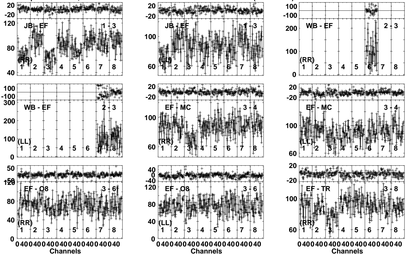
Lower frame: Milli Ampl Jy Top frame: Phas deg Vector averaged cross-power spectrum Several baselines displayed Timerange: 00/19:18:41 to 00/19:19:49
