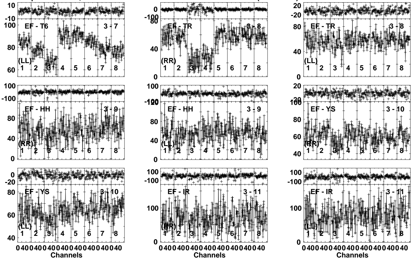
Lower frame: Milli Ampl Jy Top frame: Phas deg Vector averaged cross-power spectrum Several baselines displayed Timerange: 00/15:21:31 to 00/15:22:39
