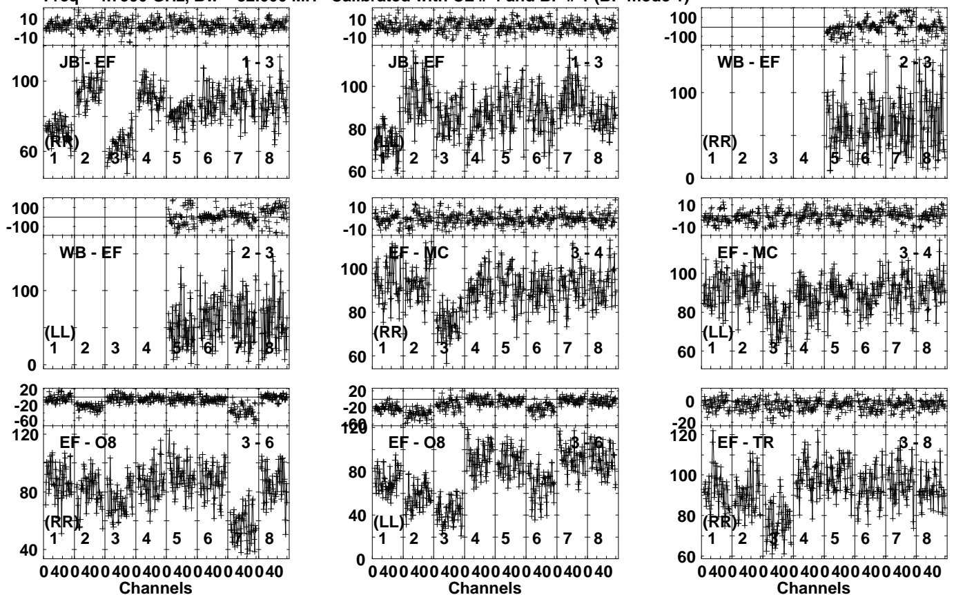
Lower frame: Milli Ampl Jy Top frame: Phas deg Vector averaged cross-power spectrum Several baselines displayed Timerange: 00/13:20:22 to 00/13:21:38
