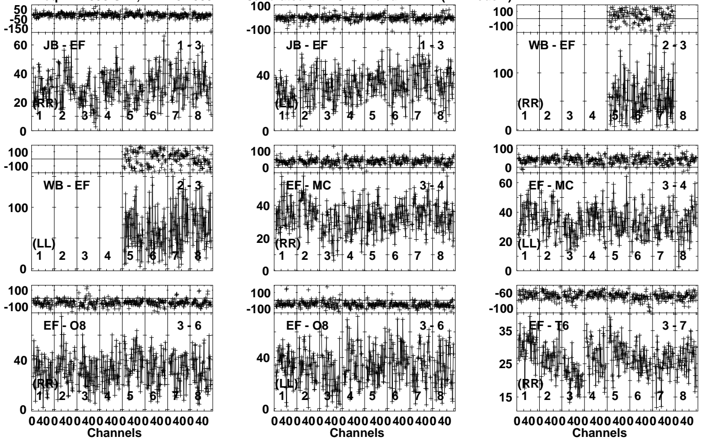
Lower frame: Milli Ampl Jy Top frame: Phas deg Vector averaged cross-power spectrum Several baselines displayed Timerange: 00/16:18:31 to 00/16:20:09
