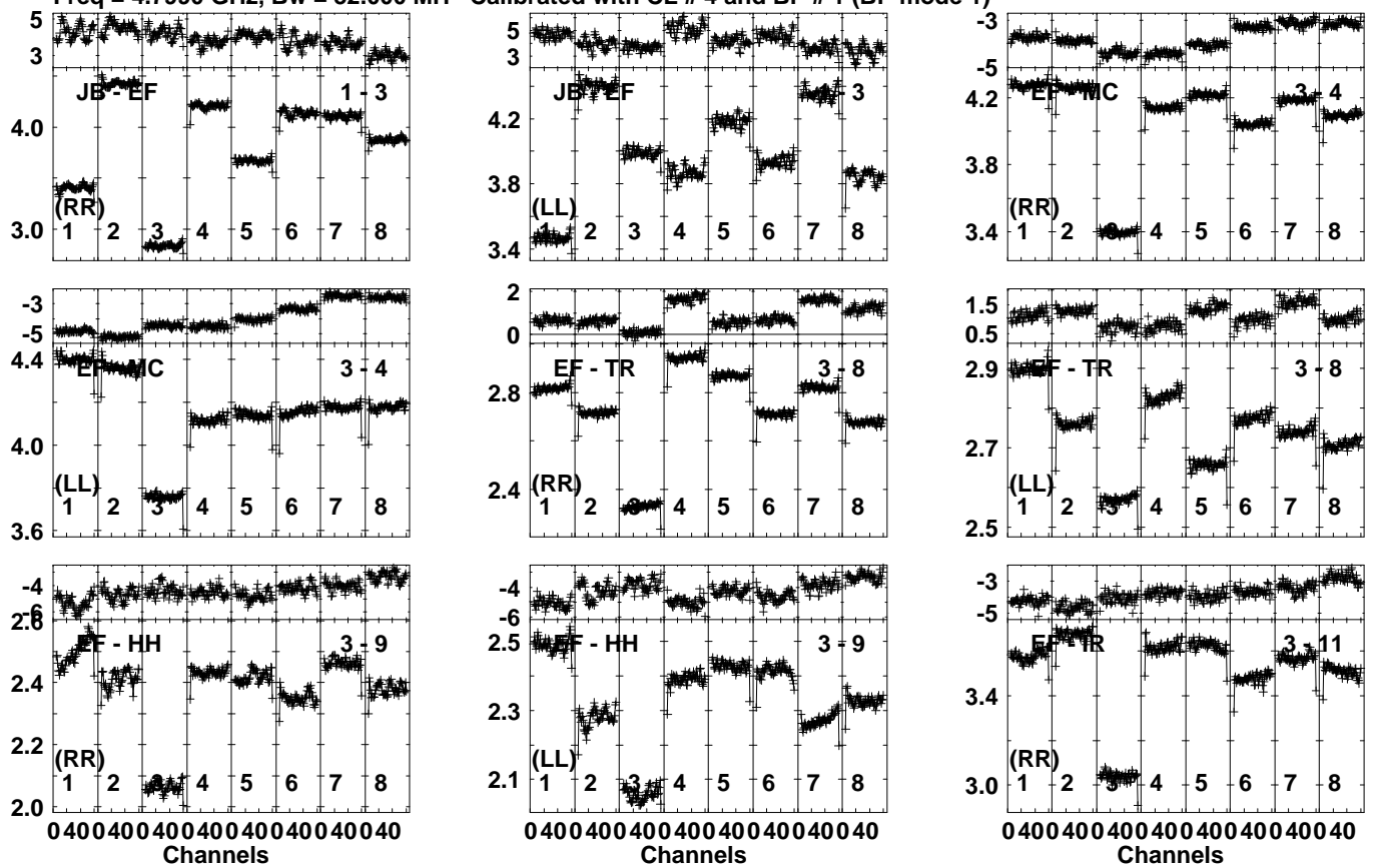
Lower frame: Ampl Jy Top frame: Phas deg Vector averaged cross-power spectrum Several baselines displayed Timerange: 00/20:31:51 to 00/20:35:49
