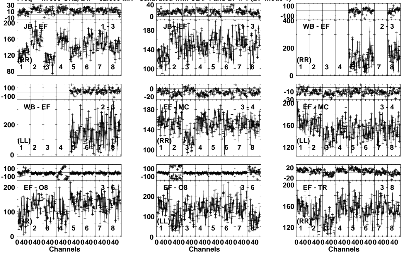
Lower frame: Milli Ampl Jy Top frame: Phas deg Vector averaged cross-power spectrum Several baselines displayed Timerange: 00/18:38:41 to 00/18:39:49
