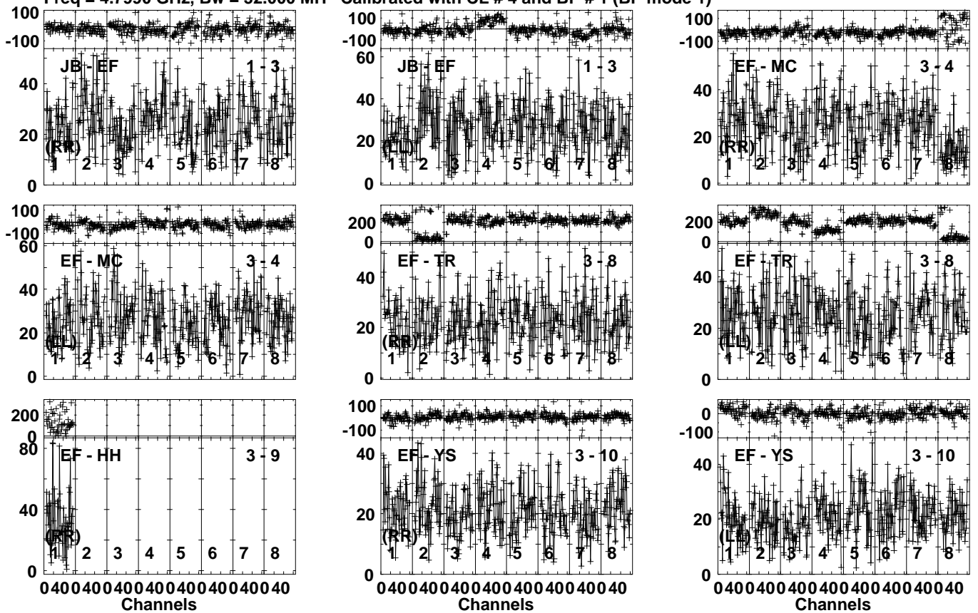
Lower frame: Milli Ampl Jy Top frame: Phas deg Vector averaged cross-power spectrum Several baselines displayed Timerange: 00/21:40:47 to 00/21:42:13
