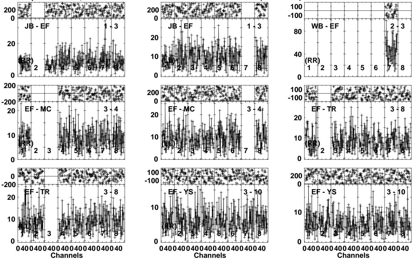
Lower frame: Milli Ampl Jy Top frame: Phas deg Vector averaged cross-power spectrum Several baselines displayed Timerange: 01/00:09:11 to 01/00:11:39
