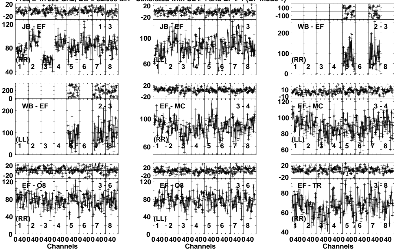
Lower frame: Milli Ampl Jy Top frame: Phas deg Vector averaged cross-power spectrum Several baselines displayed Timerange: 00/19:55:21 to 00/19:56:29
