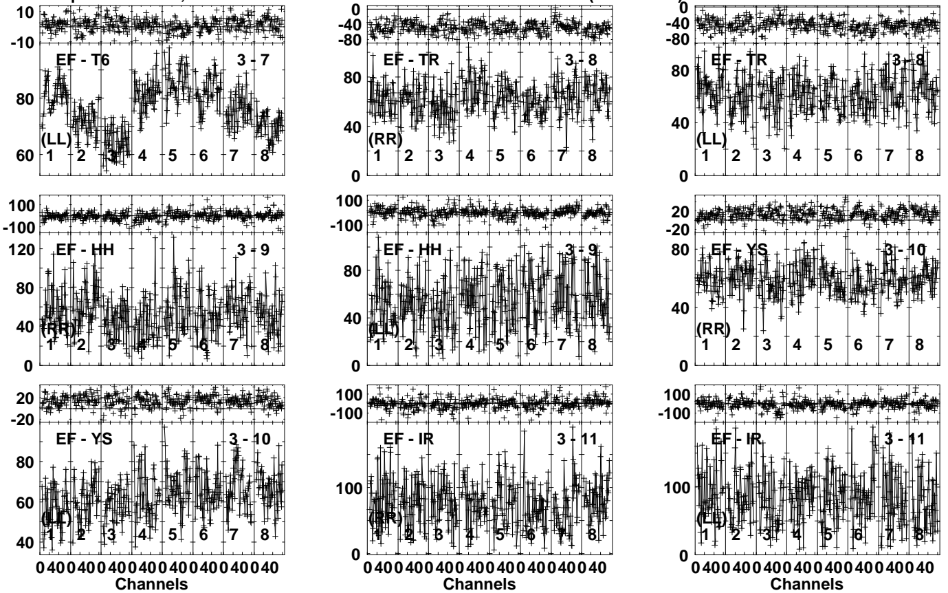
Lower frame: Milli Ampl Jy Top frame: Phas deg Vector averaged cross-power spectrum Several baselines displayed Timerange: 00/14:49:51 to 00/14:51:19
