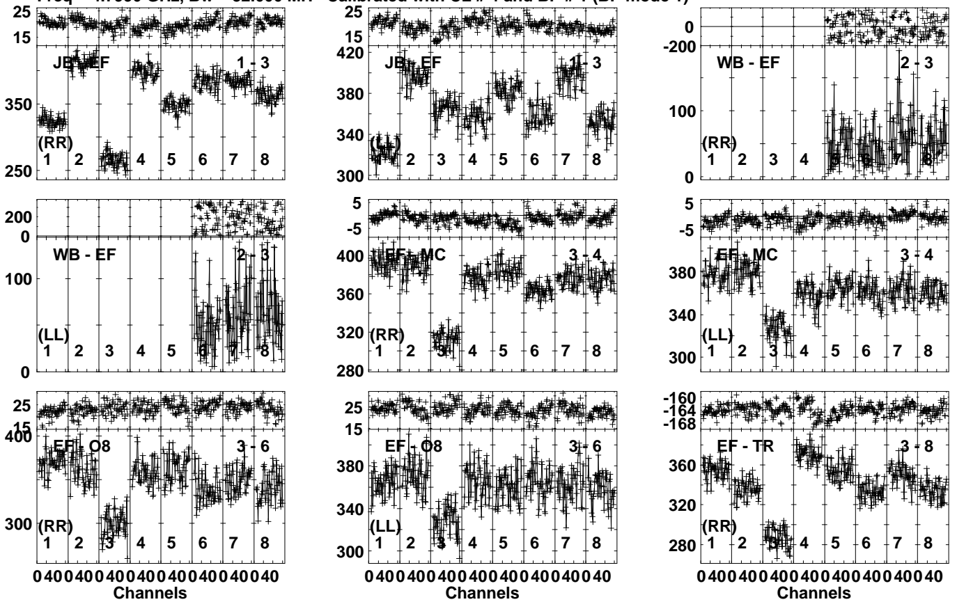
Lower frame: Milli Ampl Jy Top frame: Phas deg Vector averaged cross-power spectrum Several baselines displayed Timerange: 00/13:46:02 to 00/13:47:38
