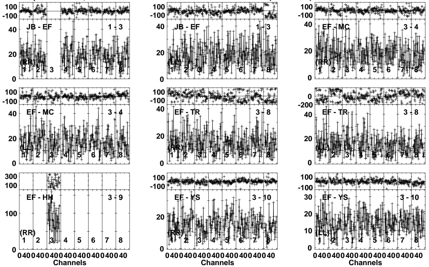
Lower frame: Milli Ampl Jy Top frame: Phas deg Vector averaged cross-power spectrum Several baselines displayed Timerange: 00/22:10:11 to 00/22:11:39
