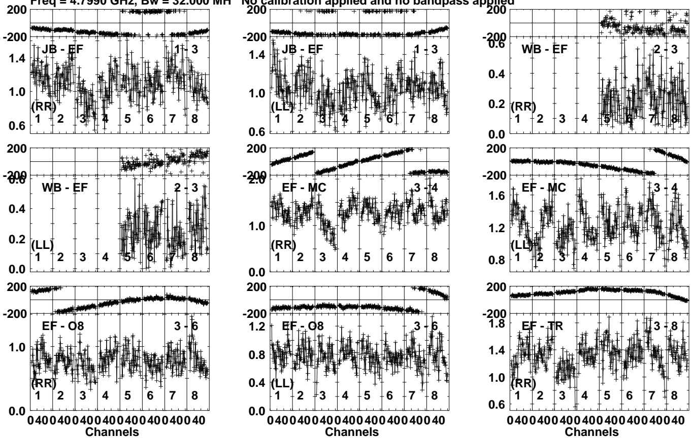
Lower frame: Milli Ampl Jy Top frame: Phas deg Vector averaged cross-power spectrum Several baselines displayed Timerange: 00/19:05:51 to 00/19:06:59
