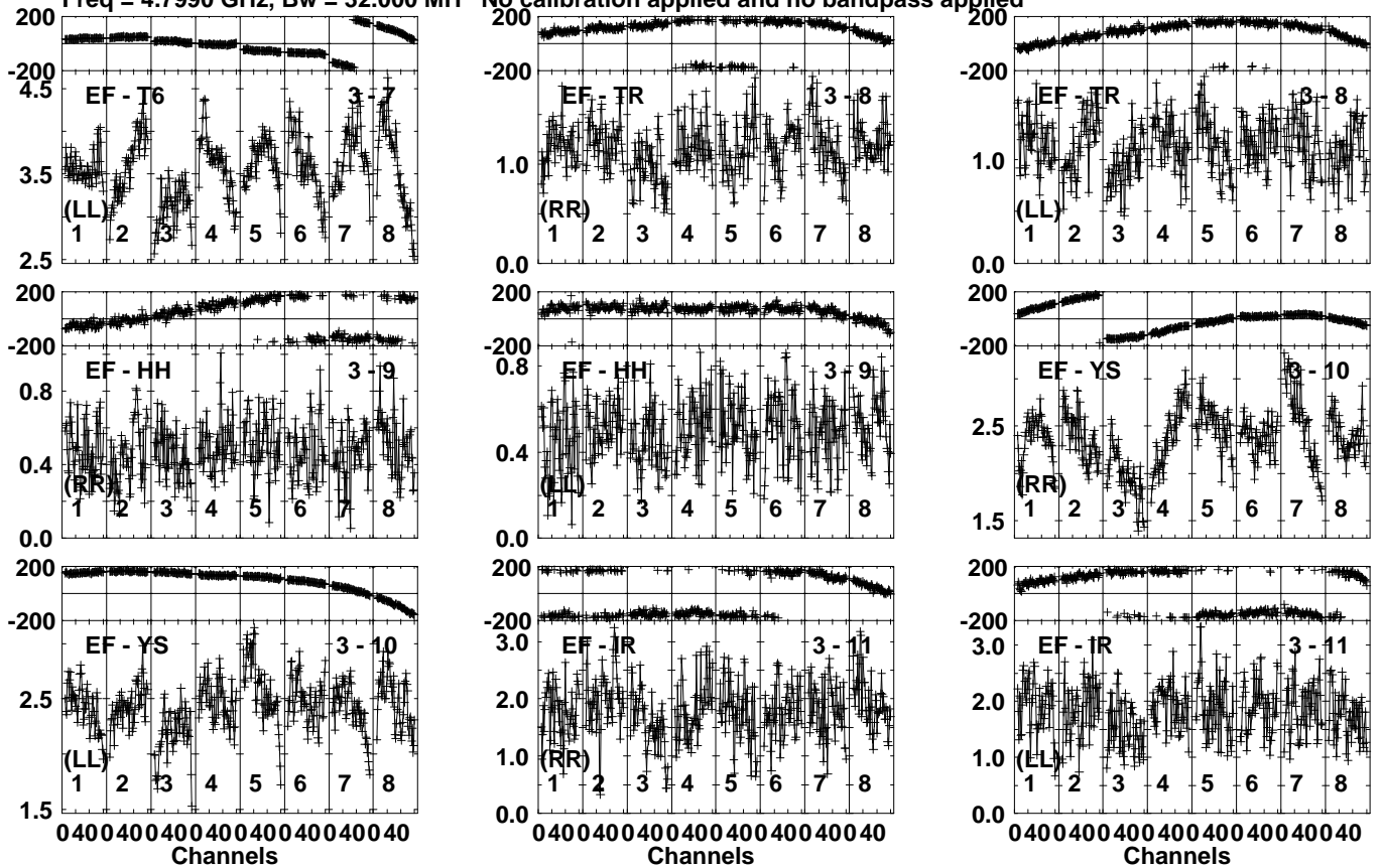
Lower frame: Milli Ampl Jy Top frame: Phas deg Vector averaged cross-power spectrum Several baselines displayed Timerange: 00/17:32:11 to 00/17:33:19
