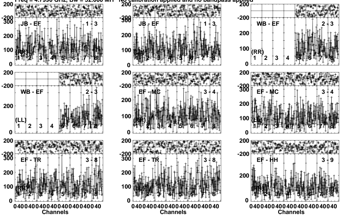
Lower frame: Micro Ampl Jy Top frame: Phas deg Vector averaged cross-power spectrum Several baselines displayed Timerange: 00/22:46:57 to 00/22:49:23
