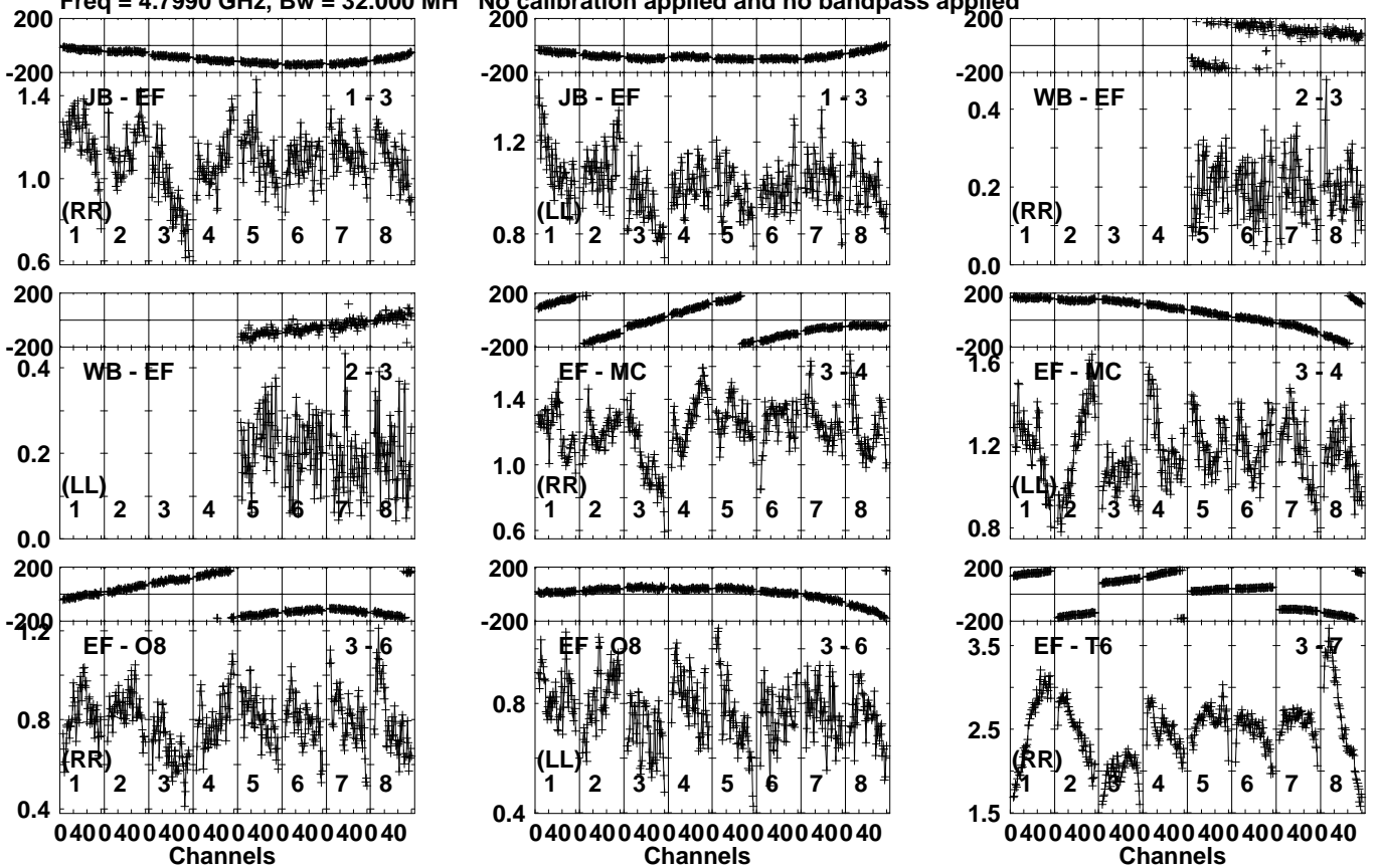
Lower frame: Milli Ampl Jy Top frame: Phas deg Vector averaged cross-power spectrum Several baselines displayed Timerange: 00/16:23:11 to 00/16:25:29
