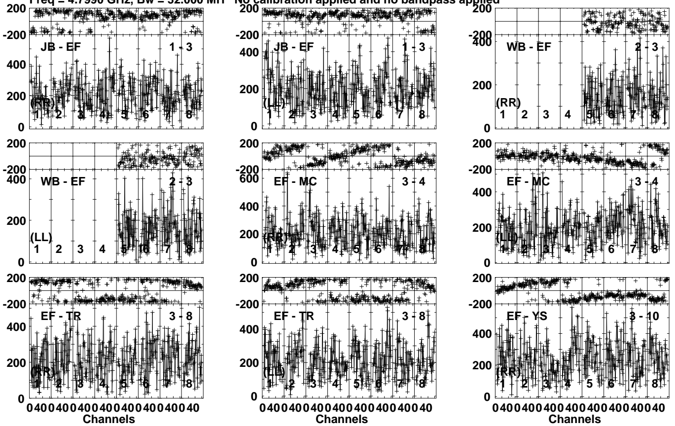
Lower frame: Micro Ampl Jy Top frame: Phas deg Vector averaged cross-power spectrum Several baselines displayed Timerange: 01/00:00:27 to 01/00:01:43
