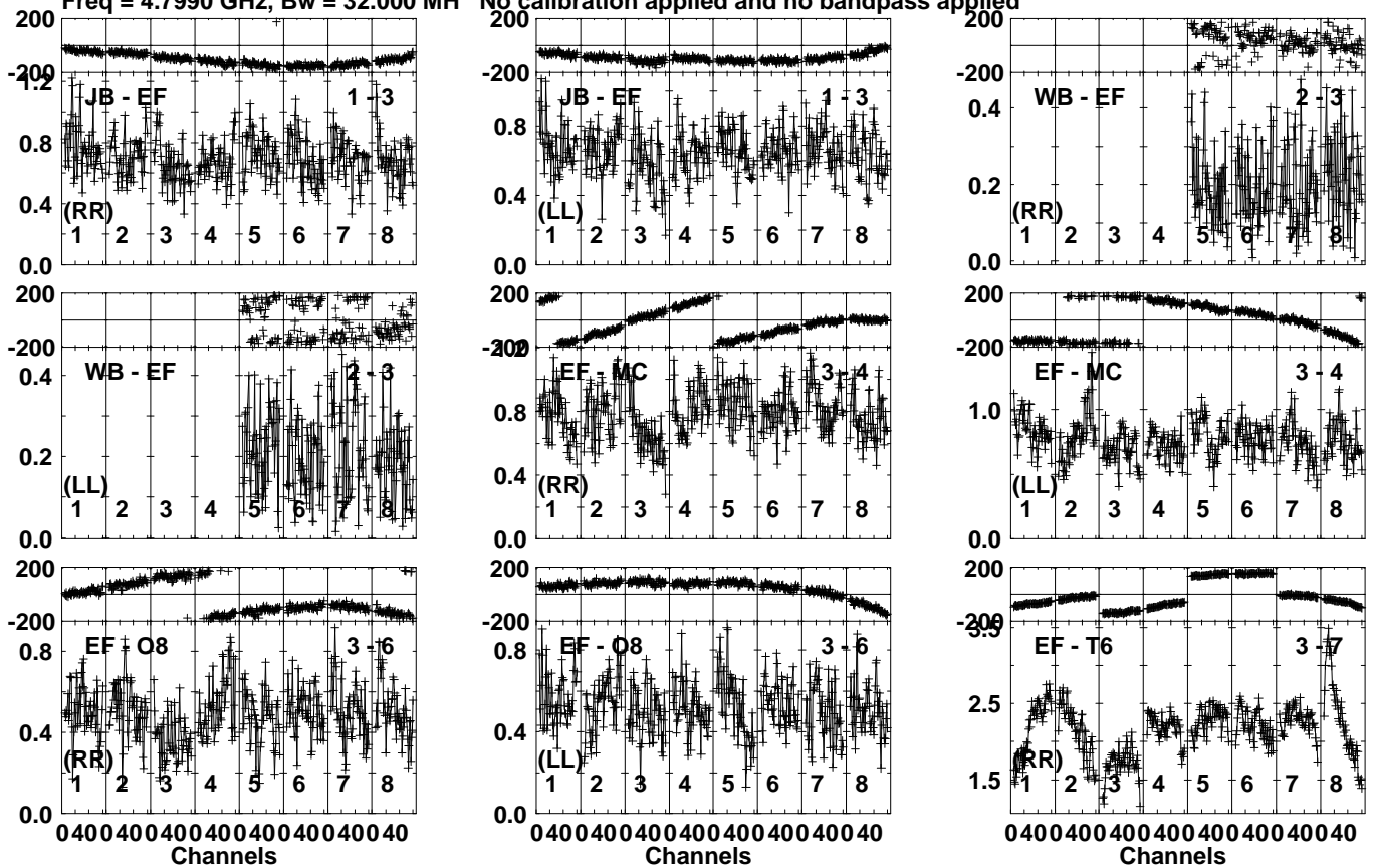
Lower frame: Milli Ampl Jy Top frame: Phas deg Vector averaged cross-power spectrum Several baselines displayed Timerange: 00/15:37:11 to 00/15:38:39
