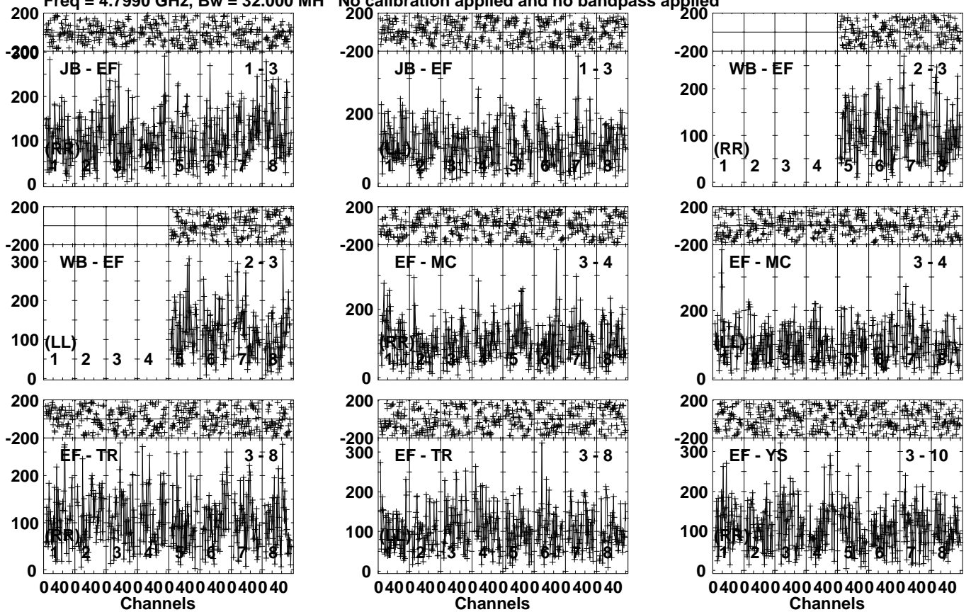
Lower frame: Micro Ampl Jy Top frame: Phas deg Vector averaged cross-power spectrum Several baselines displayed Timerange: 00/23:53:21 to 00/23:55:53
