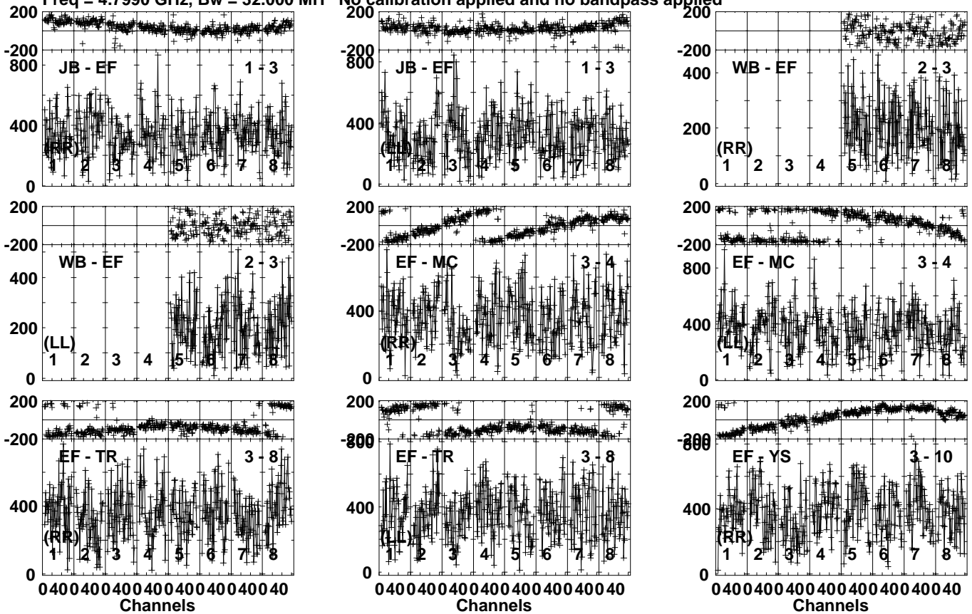
Lower frame: Micro Ampl Jy Top frame: Phas deg Vector averaged cross-power spectrum Several baselines displayed Timerange: 00/21:29:01 to 00/21:30:29
