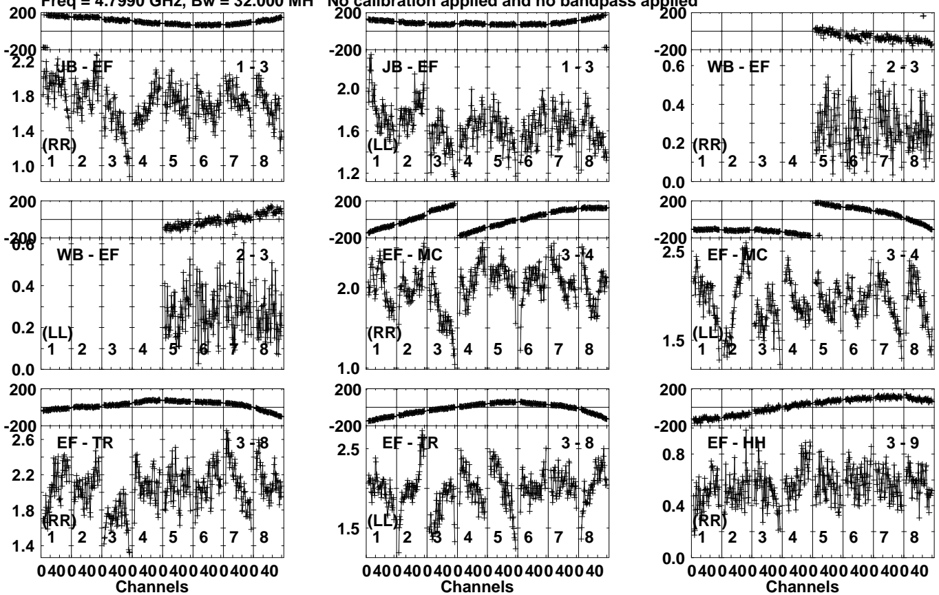
Lower frame: Milli Ampl Jy Top frame: Phas deg Vector averaged cross-power spectrum Several baselines displayed Timerange: 00/20:26:41 to 00/20:27:49
