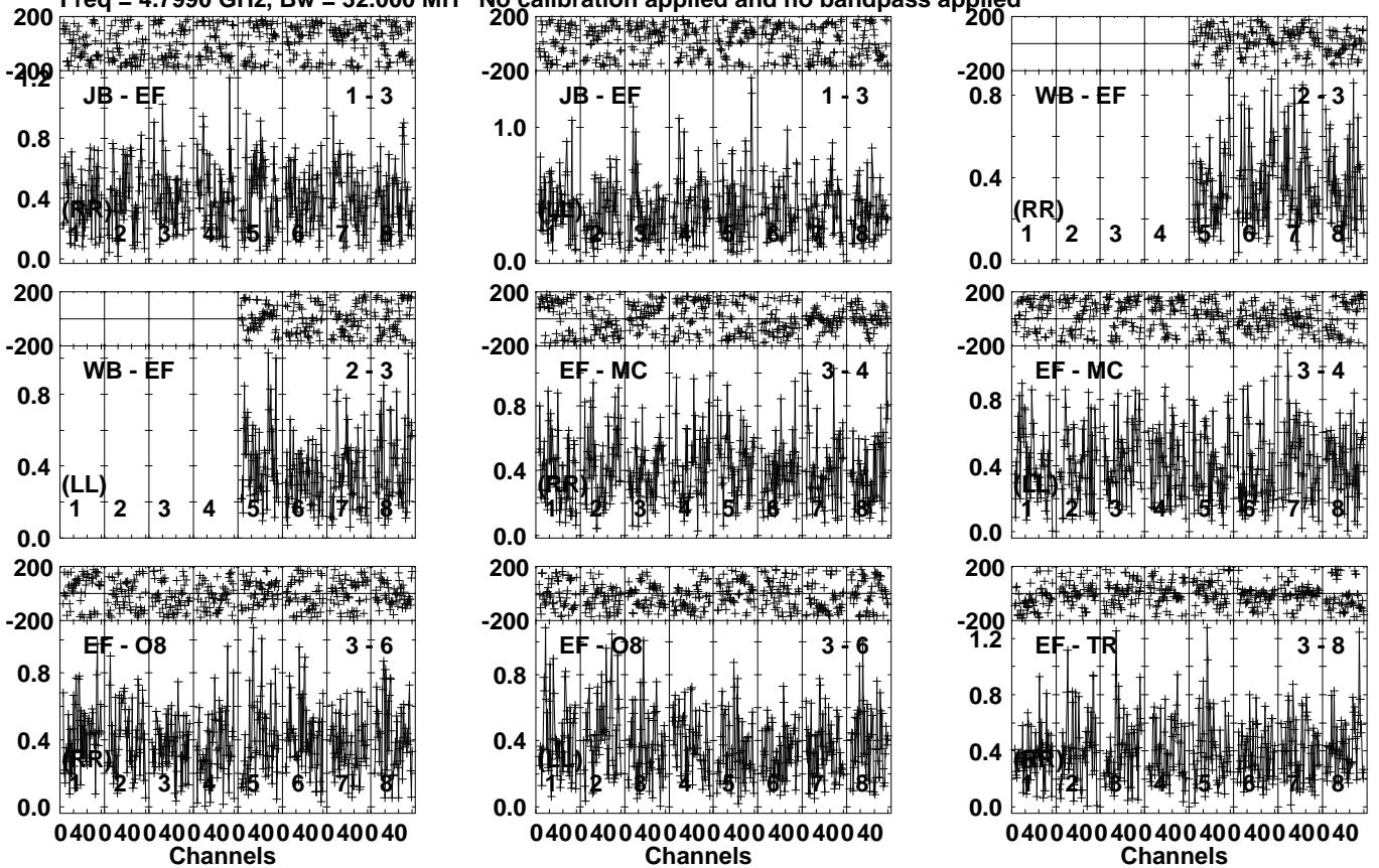
Lower frame: Milli Ampl Jy Top frame: Phas deg Vector averaged cross-power spectrum Several baselines displayed Timerange: 00/19:53:41 to 00/19:54:49
