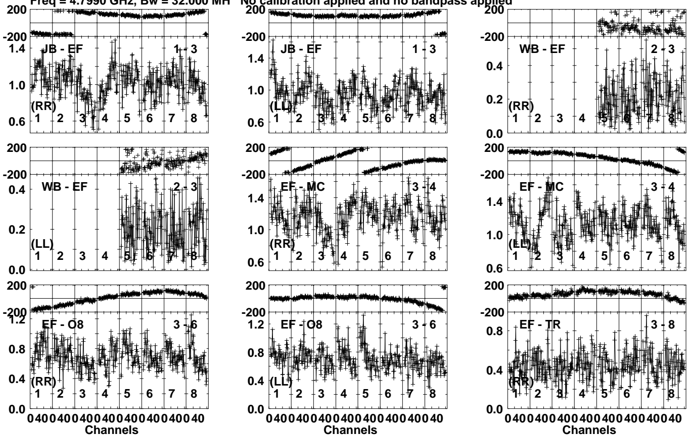
Lower frame: Milli Ampl Jy Top frame: Phas deg Vector averaged cross-power spectrum Several baselines displayed Timerange: 00/20:05:21 to 00/20:06:29
