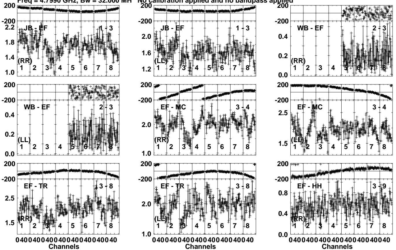
Lower frame: Milli Ampl Jy Top frame: Phas deg Vector averaged cross-power spectrum Several baselines displayed Timerange: 00/20:12:11 to 00/20:13:19
