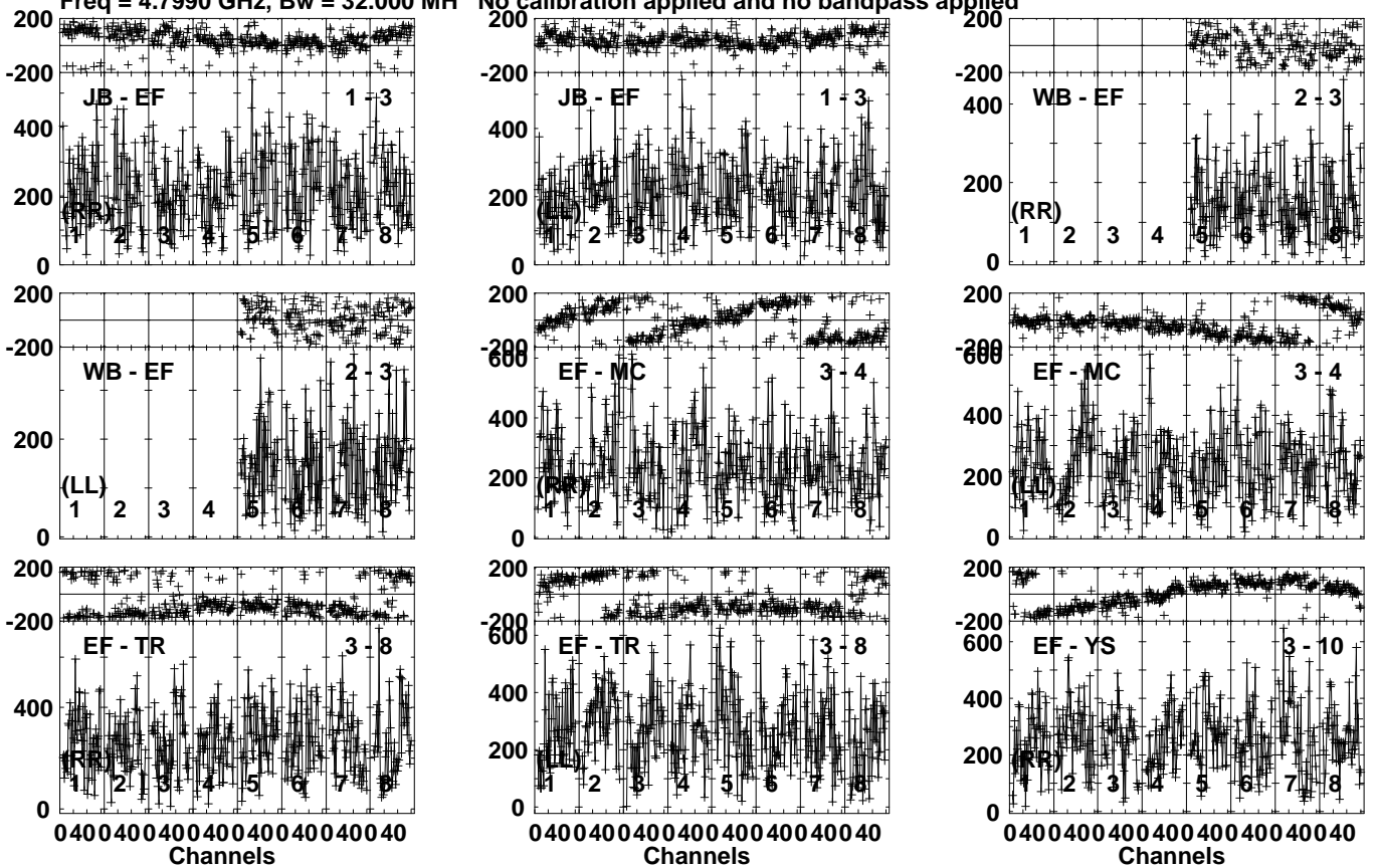
Lower frame: Micro Ampl Jy Top frame: Phas deg Vector averaged cross-power spectrum Several baselines displayed Timerange: 00/21:58:27 to 00/21:59:53
