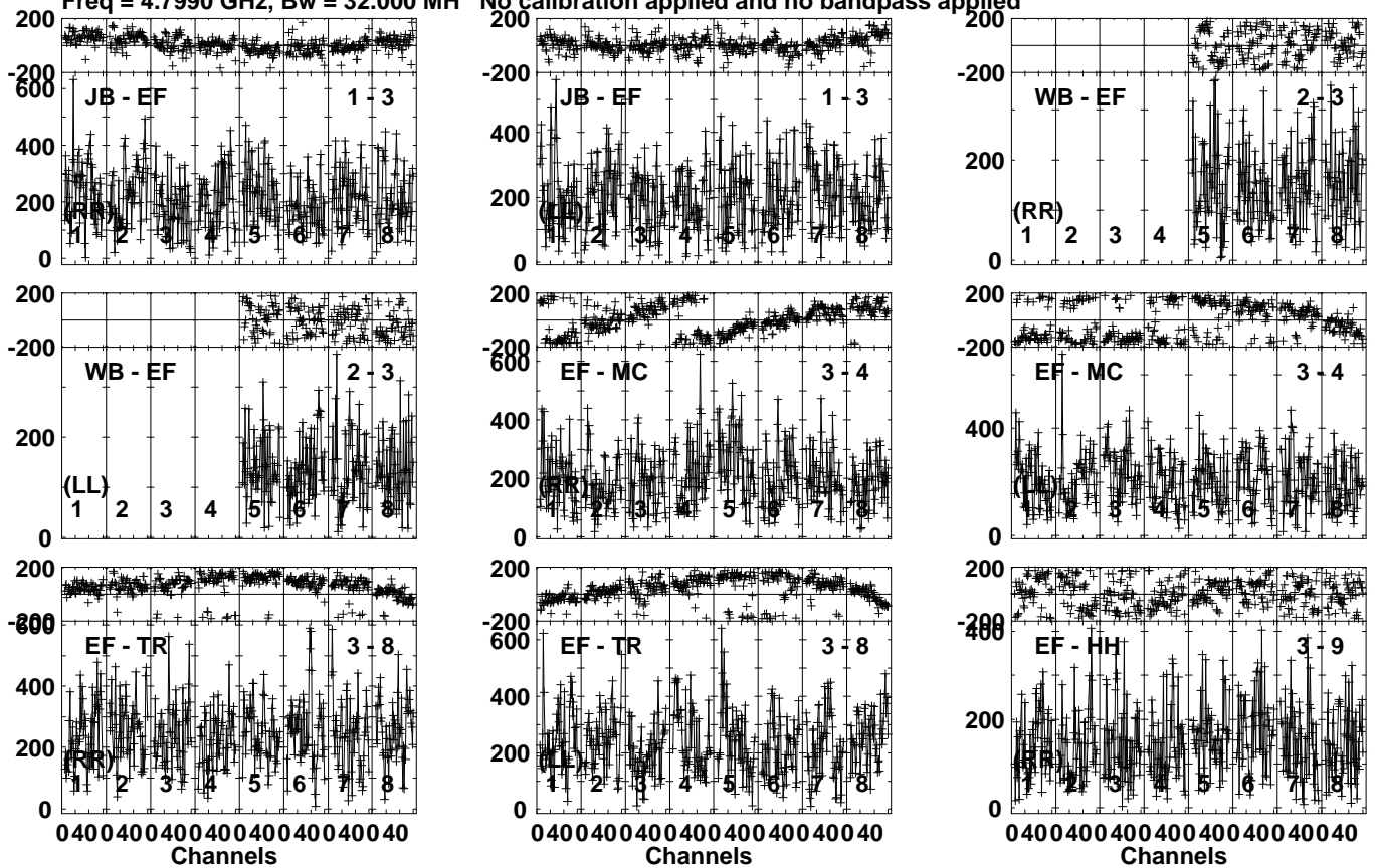
Lower frame: Micro Ampl Jy Top frame: Phas deg Vector averaged cross-power spectrum Several baselines displayed Timerange: 00/22:49:57 to 00/22:51:13
