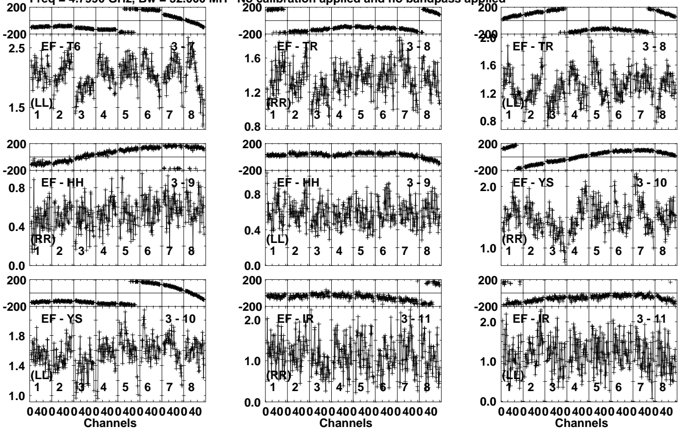
Lower frame: Milli Ampl Jy Top frame: Phas deg Vector averaged cross-power spectrum Several baselines displayed Timerange: 00/18:12:01 to 00/18:13:09
