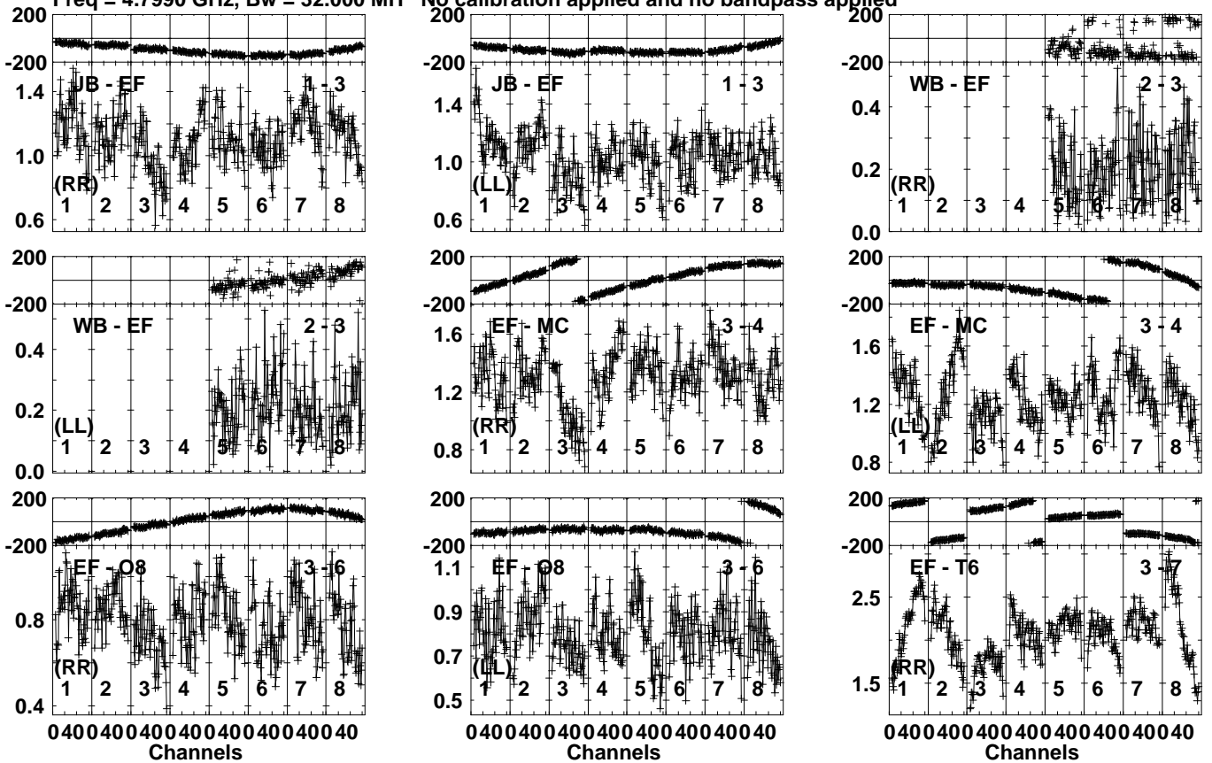
Lower frame: Milli Ampl Jy Top frame: Phas deg Vector averaged cross-power spectrum Several baselines displayed Timerange: 00/18:02:01 to 00/18:03:09
