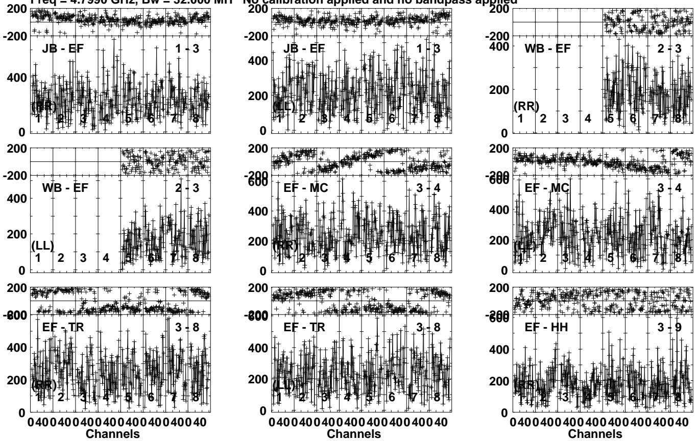
Lower frame: Micro Ampl Jy Top frame: Phas deg Vector averaged cross-power spectrum Several baselines displayed Timerange: 00/22:06:17 to 00/22:07:33
