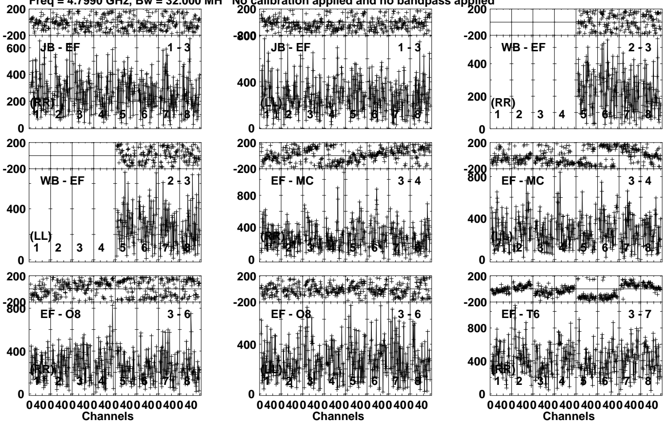
Lower frame: Micro Ampl Jy Top frame: Phas deg Vector averaged cross-power spectrum Several baselines displayed Timerange: 00/16:52:41 to 00/16:53:49
