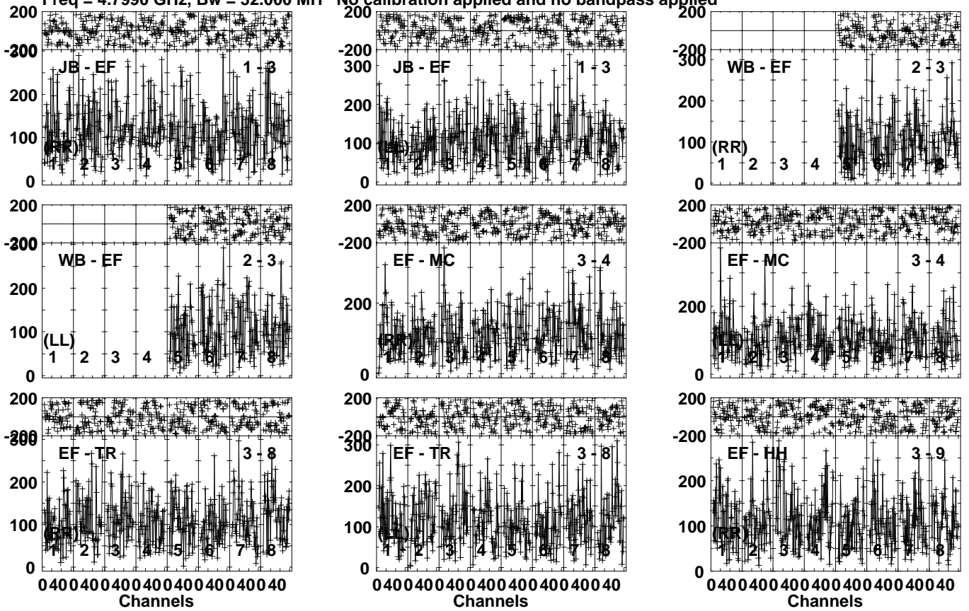
Lower frame: Micro Ampl Jy Top frame: Phas deg Vector averaged cross-power spectrum Several baselines displayed Timerange: 00/22:35:11 to 00/22:37:39
