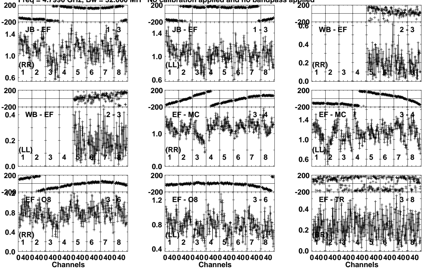
Lower frame: Milli Ampl Jy Top frame: Phas deg Vector averaged cross-power spectrum Several baselines displayed Timerange: 00/13:03:32 to 00/13:04:58
