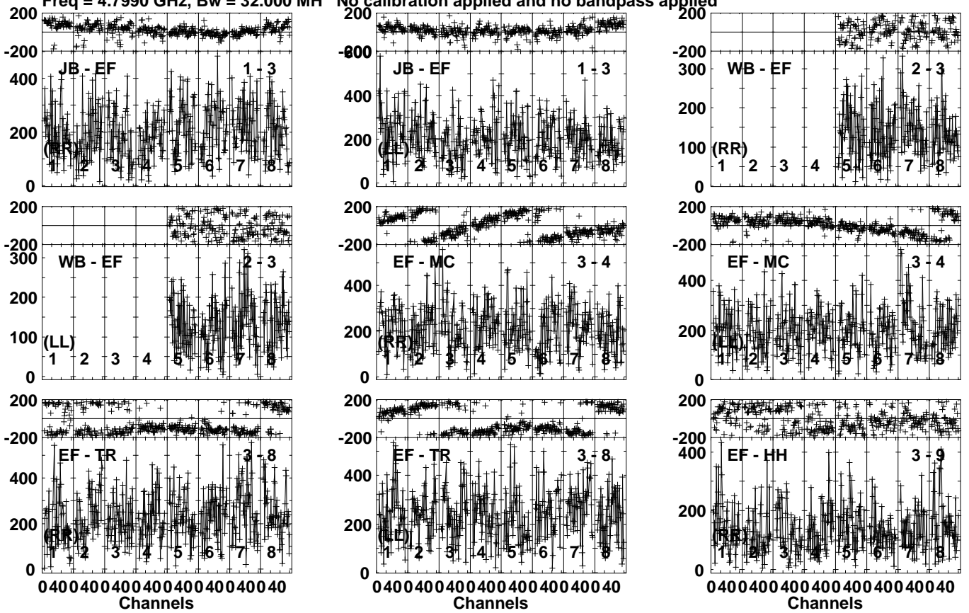
Lower frame: Micro Ampl Jy Top frame: Phas deg Vector averaged cross-power spectrum Several baselines displayed Timerange: 00/22:14:41 to 00/22:15:59
