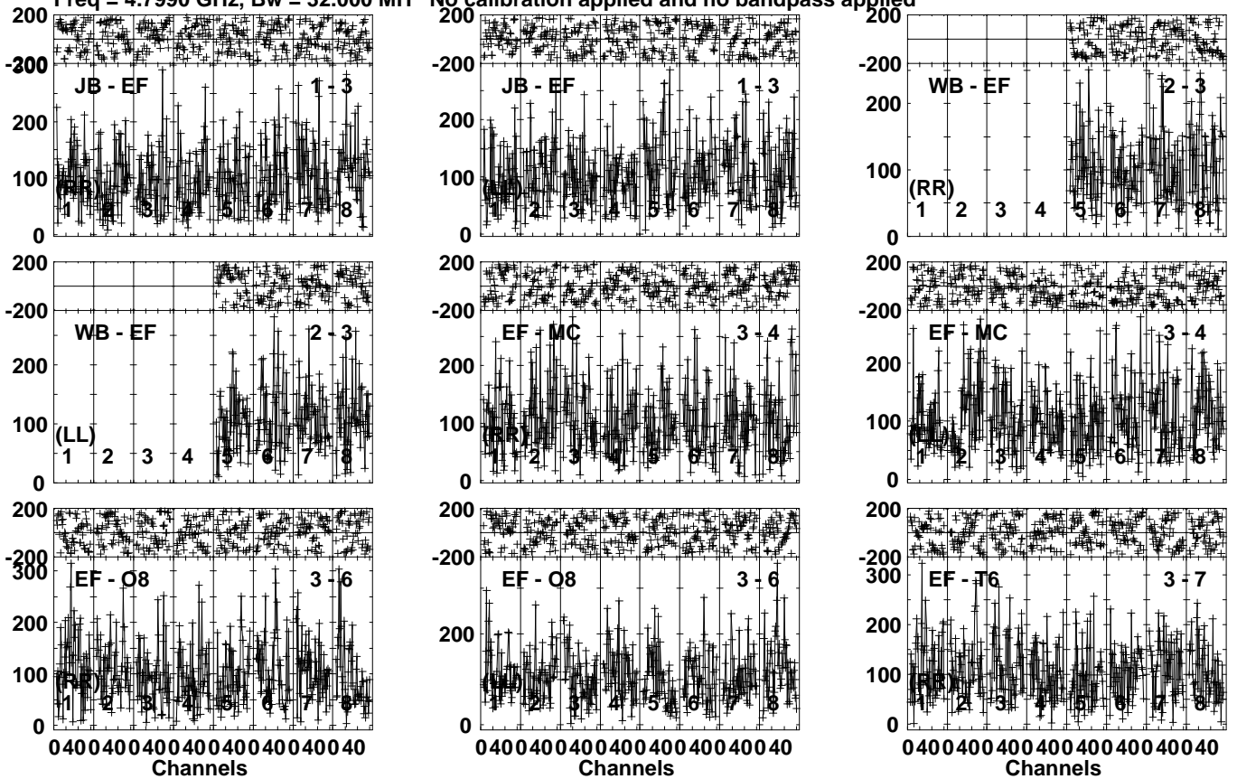
Lower frame: Micro Ampl Jy Top frame: Phas deg Vector averaged cross-power spectrum Several baselines displayed Timerange: 00/15:03:11 to 00/15:05:49
