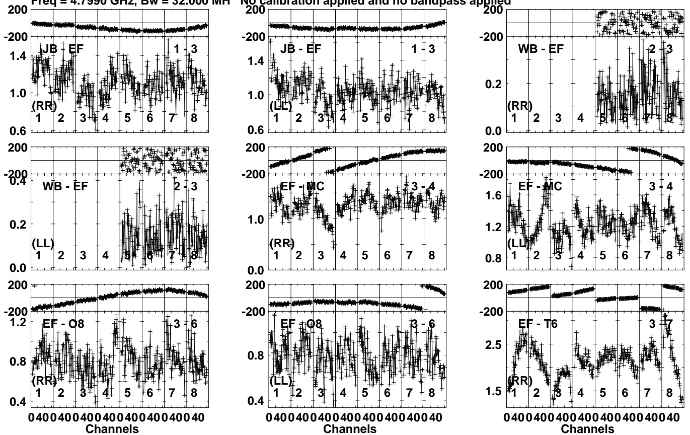
Lower frame: Milli Ampl Jy Top frame: Phas deg Vector averaged cross-power spectrum Several baselines displayed Timerange: 00/17:52:01 to 00/17:53:09
