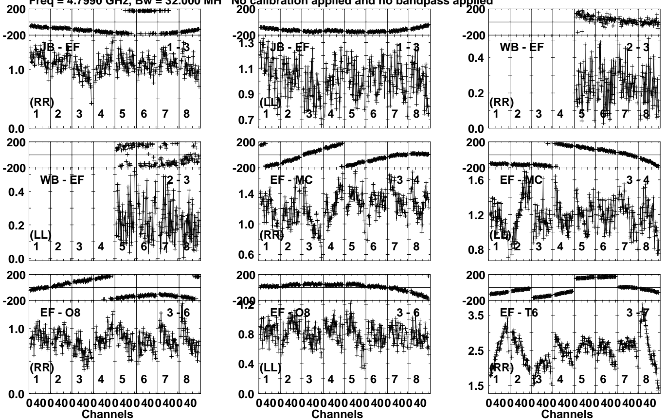
Lower frame: Milli Ampl Jy Top frame: Phas deg Vector averaged cross-power spectrum Several baselines displayed Timerange: 00/16:34:21 to 00/16:35:29
