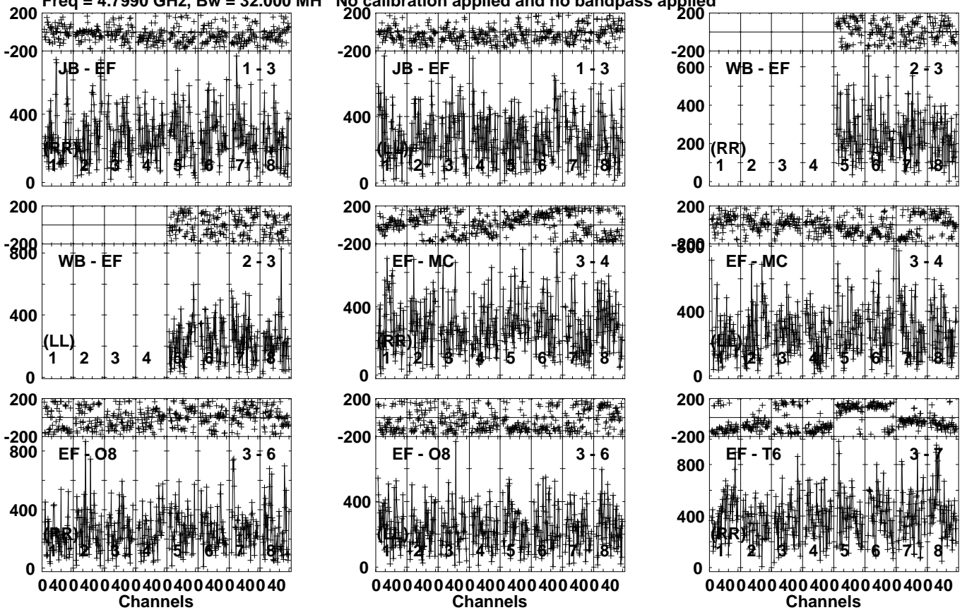
Lower frame: Micro Ampl Jy Top frame: Phas deg Vector averaged cross-power spectrum Several baselines displayed Timerange: 00/17:50:21 to 00/17:51:29
