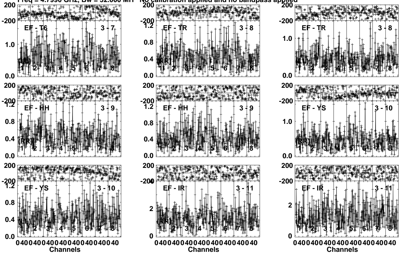
Lower frame: Milli Ampl Jy Top frame: Phas deg Vector averaged cross-power spectrum Several baselines displayed Timerange: 00/17:37:01 to 00/17:38:09
