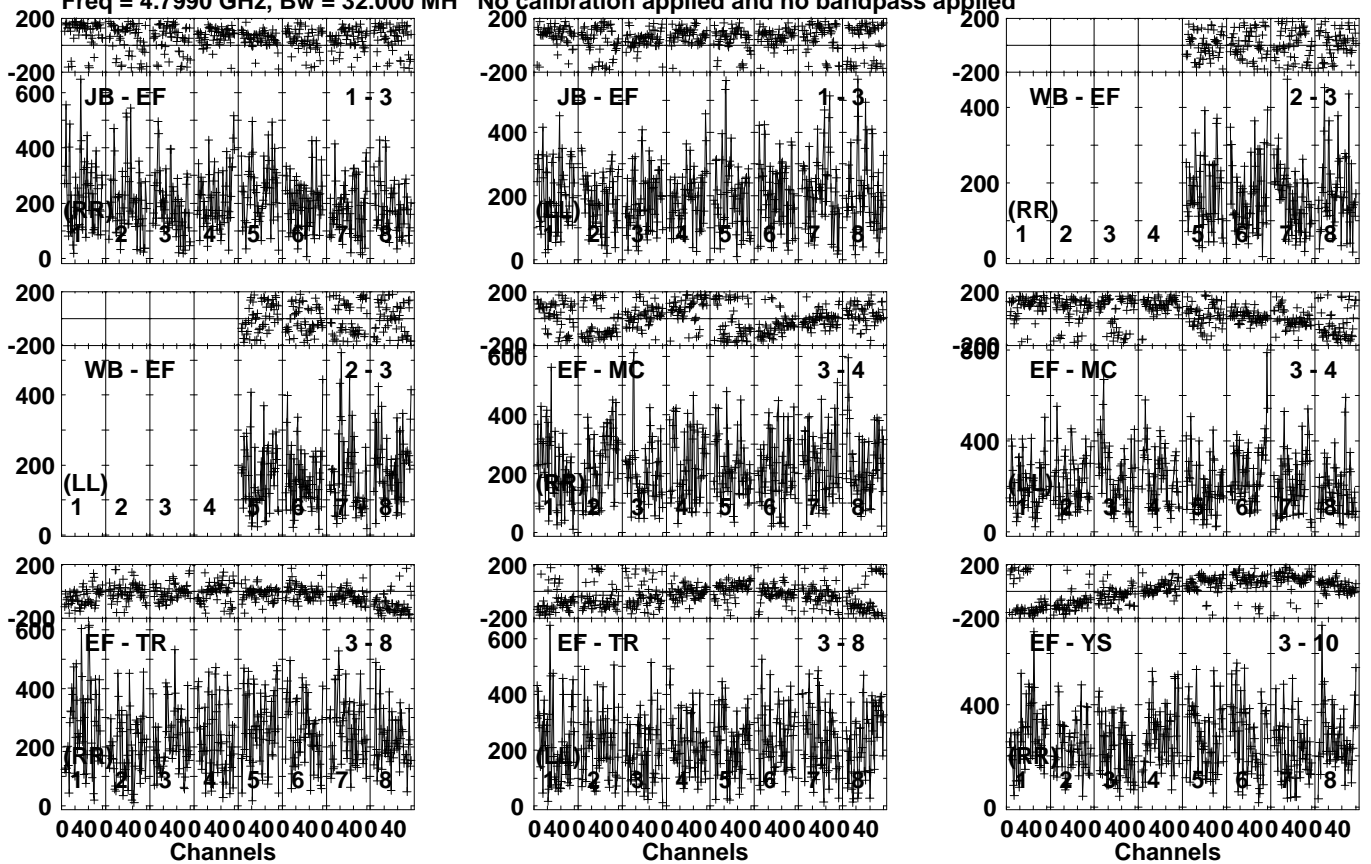
Lower frame: Micro Ampl Jy Top frame: Phas deg Vector averaged cross-power spectrum Several baselines displayed Timerange: 01/00:42:57 to 01/00:44:23
