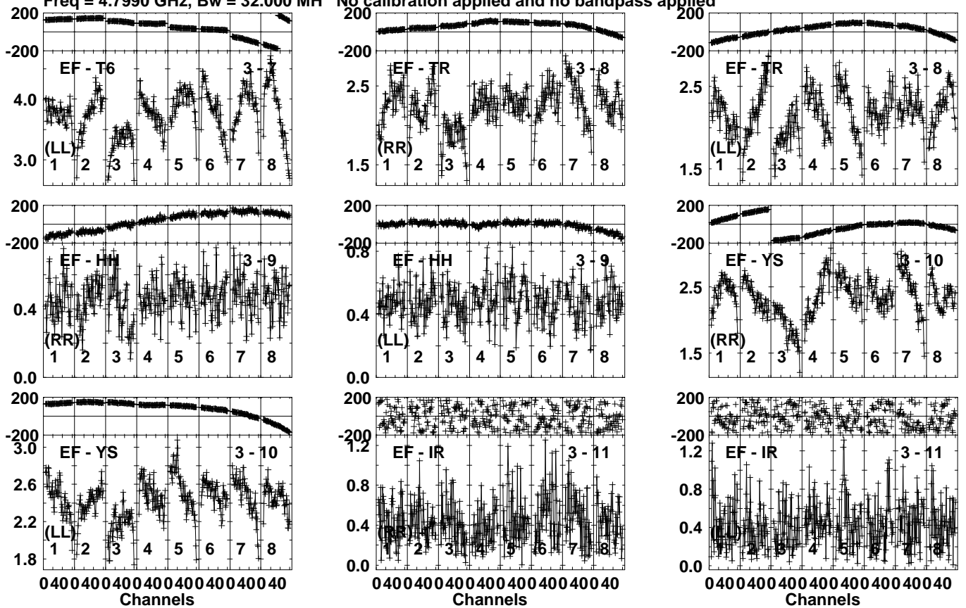
Lower frame: Milli Ampl Jy Top frame: Phas deg Vector averaged cross-power spectrum Several baselines displayed Timerange: 00/17:16:31 to 00/17:17:39
