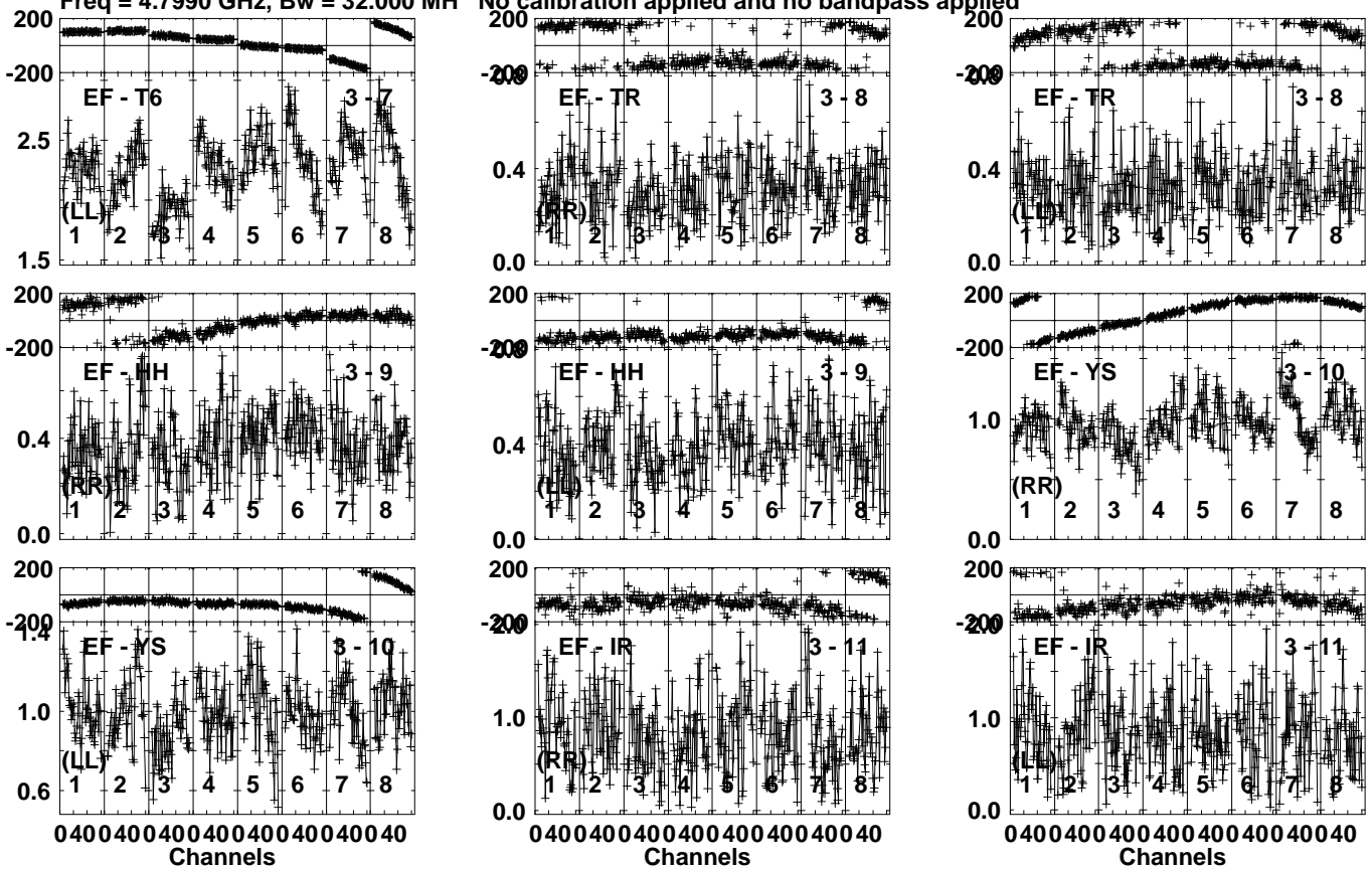
Lower frame: Milli Ampl Jy Top frame: Phas deg Vector averaged cross-power spectrum Several baselines displayed Timerange: 00/15:53:41 to 00/15:54:49
