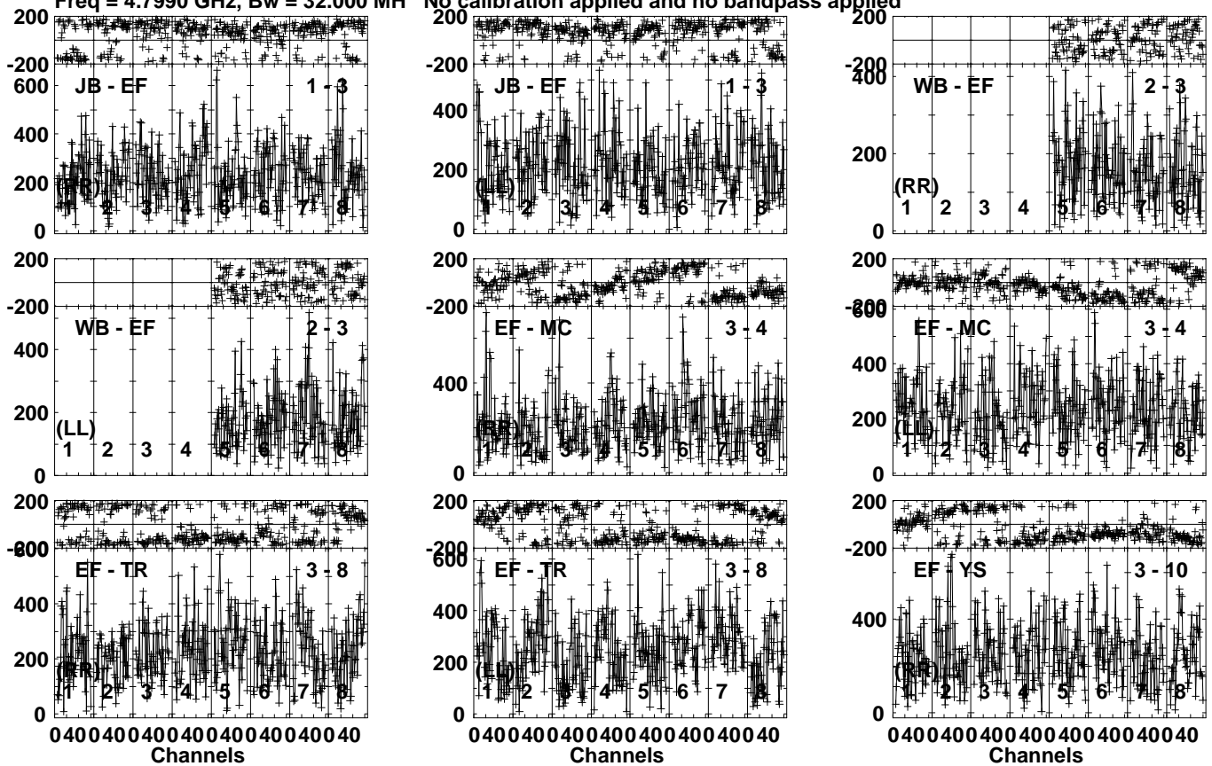
Lower frame: Micro Ampl Jy Top frame: Phas deg Vector averaged cross-power spectrum Several baselines displayed Timerange: 00/23:55:57 to 00/23:57:23
