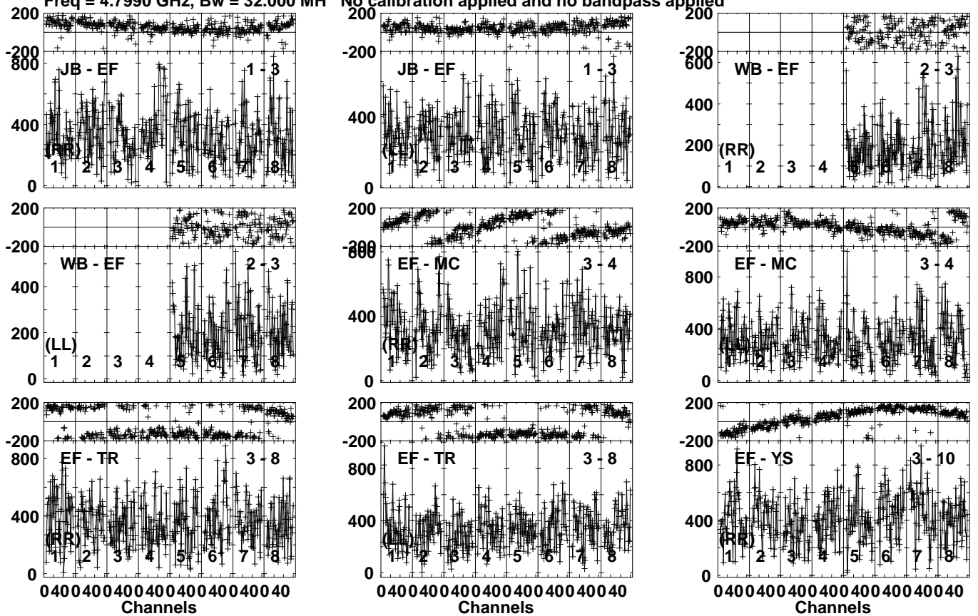
Lower frame: Micro Ampl Jy Top frame: Phas deg Vector averaged cross-power spectrum Several baselines displayed Timerange: 01/00:25:17 to 01/00:26:43
