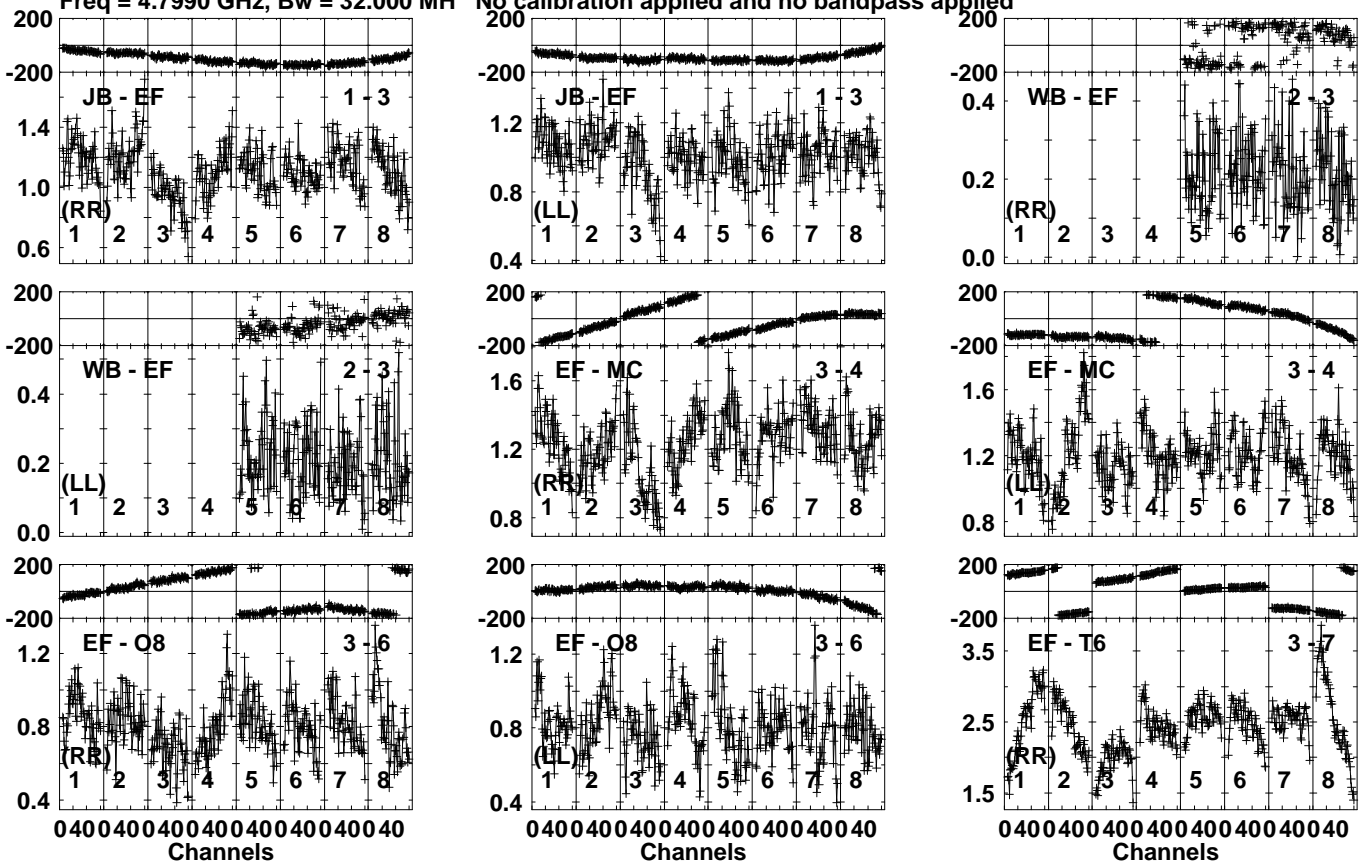
Lower frame: Milli Ampl Jy Top frame: Phas deg Vector averaged cross-power spectrum Several baselines displayed Timerange: 00/16:54:21 to 00/16:55:29
