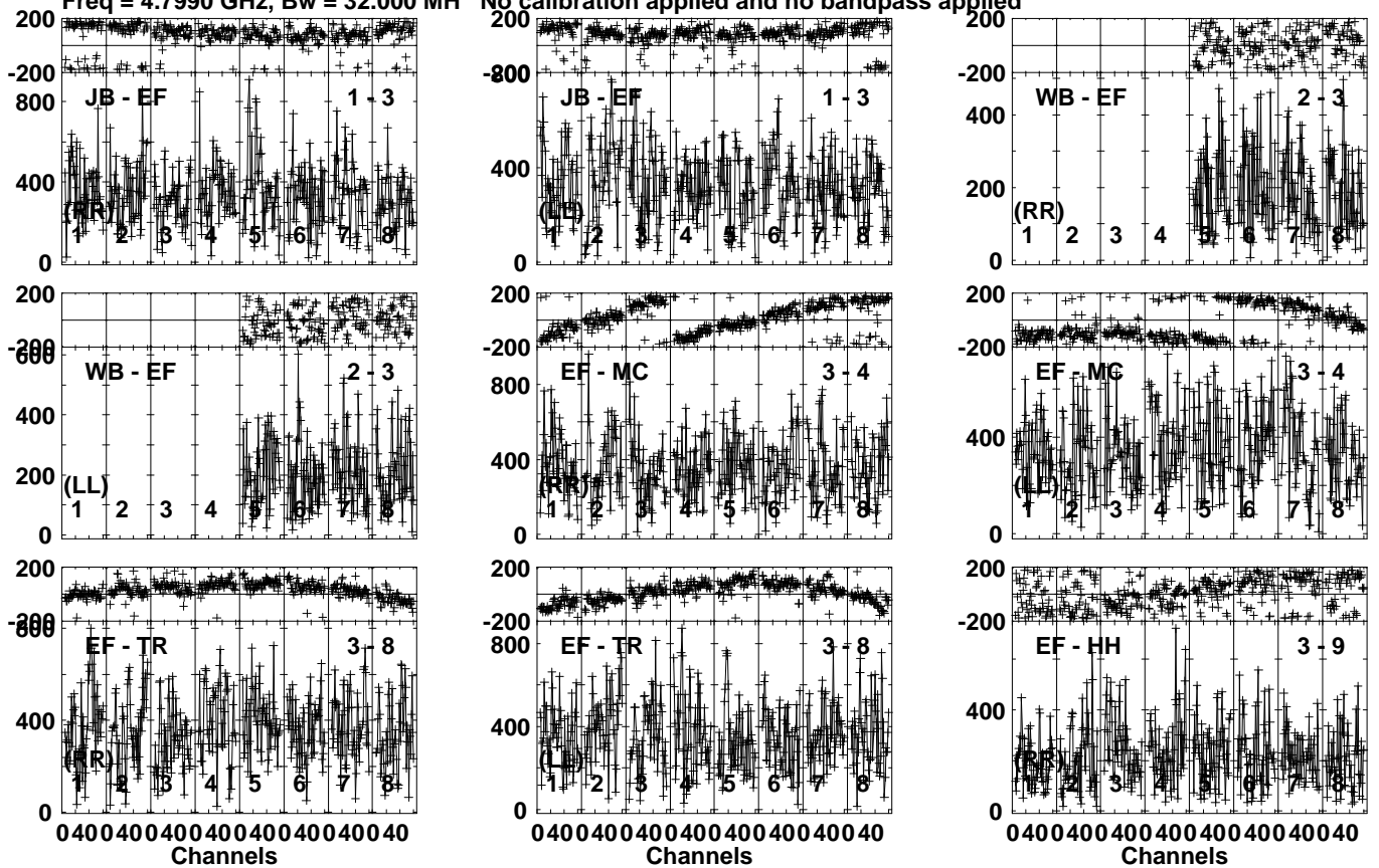
Lower frame: Micro Ampl Jy Top frame: Phas deg Vector averaged cross-power spectrum Several baselines displayed Timerange: 00/23:26:31 to 00/23:27:59
