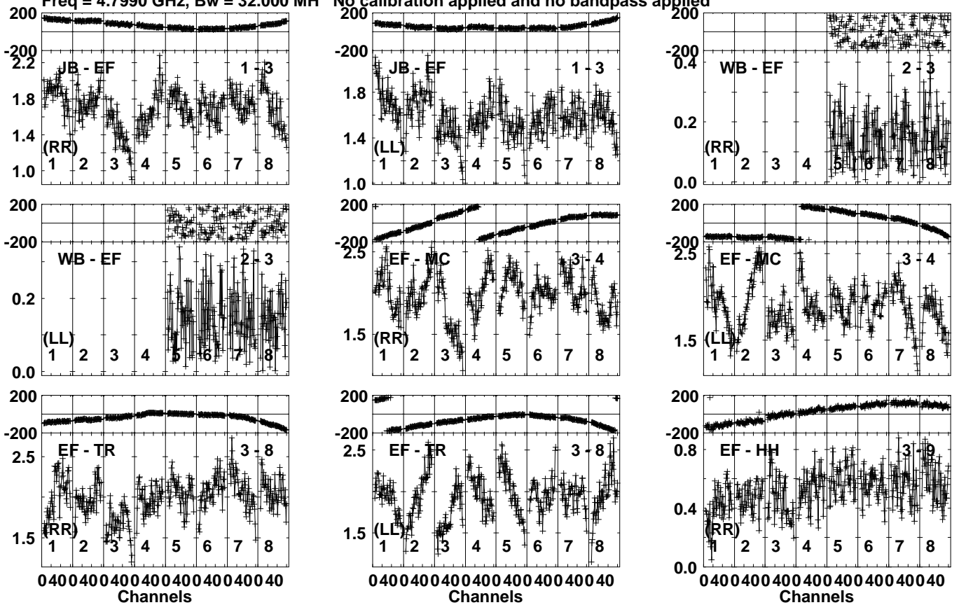
Lower frame: Milli Ampl Jy Top frame: Phas deg Vector averaged cross-power spectrum Several baselines displayed Timerange: 00/20:16:11 to 00/20:17:19
