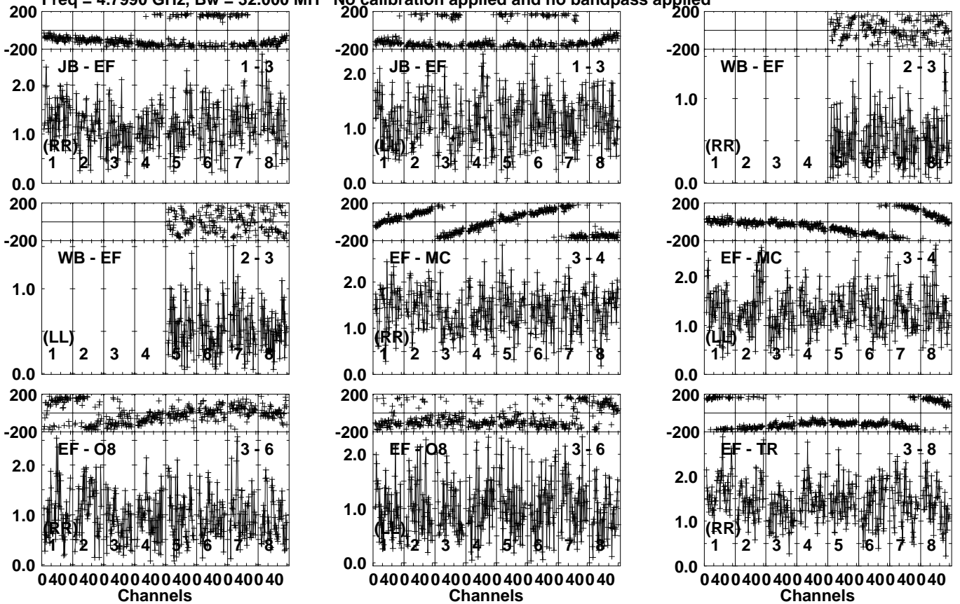
Lower frame: Milli Ampl Jy Top frame: Phas deg Vector averaged cross-power spectrum Several baselines displayed Timerange: 00/19:02:01 to 00/19:03:09
