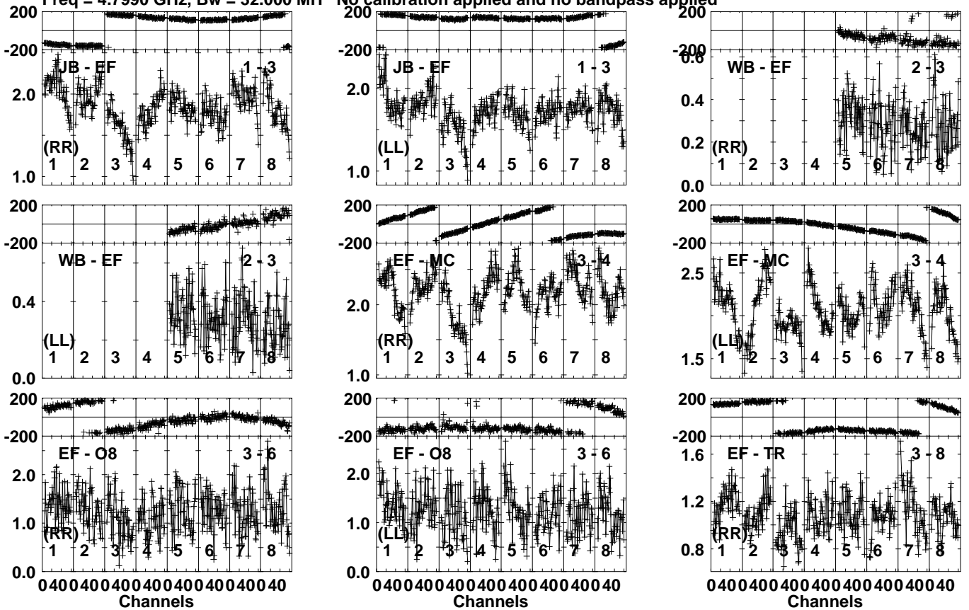
Lower frame: Milli Ampl Jy Top frame: Phas deg Vector averaged cross-power spectrum Several baselines displayed Timerange: 00/19:29:11 to 00/19:30:19
