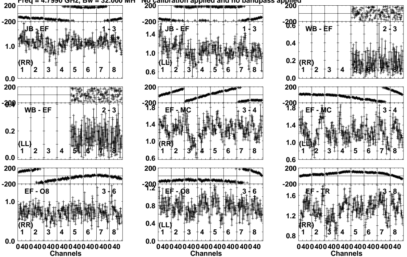
Lower frame: Milli Ampl Jy Top frame: Phas deg Vector averaged cross-power spectrum Several baselines displayed Timerange: 00/19:15:51 to 00/19:16:59
