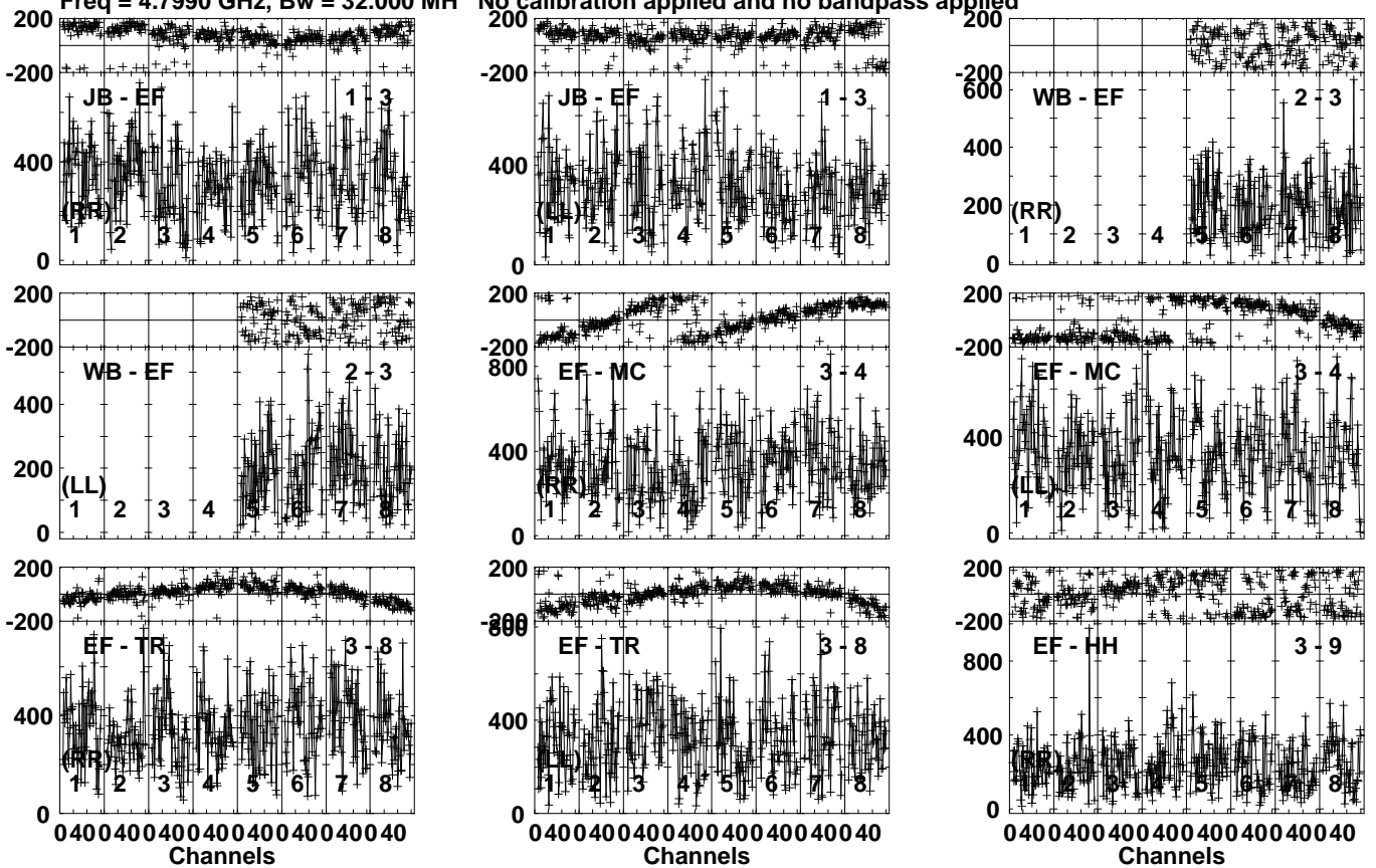
Lower frame: Micro Ampl Jy Top frame: Phas deg Vector averaged cross-power spectrum Several baselines displayed Timerange: 00/23:14:47 to 00/23:16:13
