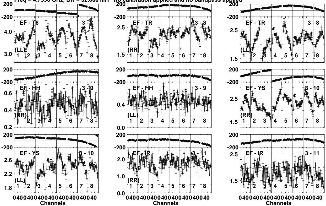
Lower frame: Milli Ampl Jy Top frame: Phas deg Vector averaged cross-power spectrum Several baselines displayed Timerange: 00/17:08:39 to 00/17:10:49
