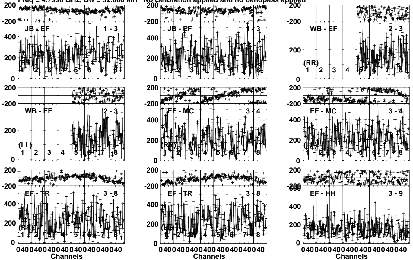
Lower frame: Micro Ampl Jy Top frame: Phas deg Vector averaged cross-power spectrum Several baselines displayed Timerange: 00/23:16:47 to 00/23:18:03
