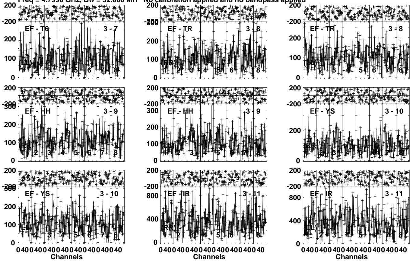
Lower frame: Micro Ampl Jy Top frame: Phas deg Vector averaged cross-power spectrum Several baselines displayed Timerange: 00/16:10:01 to 00/16:12:39
