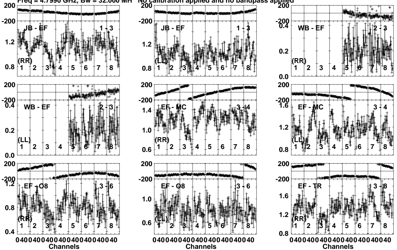
Lower frame: Milli Ampl Jy Top frame: Phas deg Vector averaged cross-power spectrum Several baselines displayed Timerange: 00/12:31:42 to 00/12:32:58
