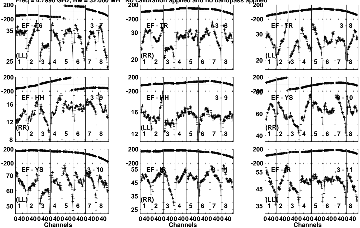
Lower frame: Milli Ampl Jy Top frame: Phas deg Vector averaged cross-power spectrum Several baselines displayed Timerange: 00/16:56:31 to 00/17:00:29
