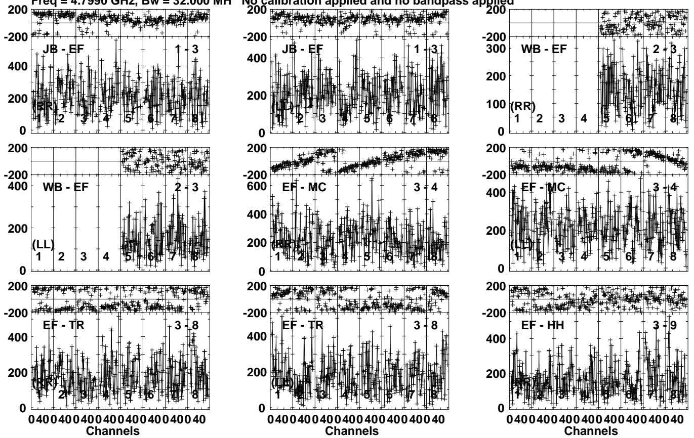
Lower frame: Micro Ampl Jy Top frame: Phas deg Vector averaged cross-power spectrum Several baselines displayed Timerange: 00/21:42:47 to 00/21:44:03
