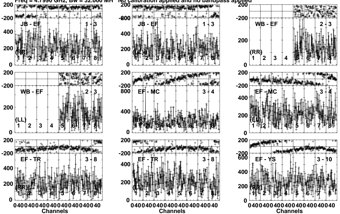
Lower frame: Micro Ampl Jy Top frame: Phas deg Vector averaged cross-power spectrum Several baselines displayed Timerange: 00/23:36:57 to 00/23:38:13
