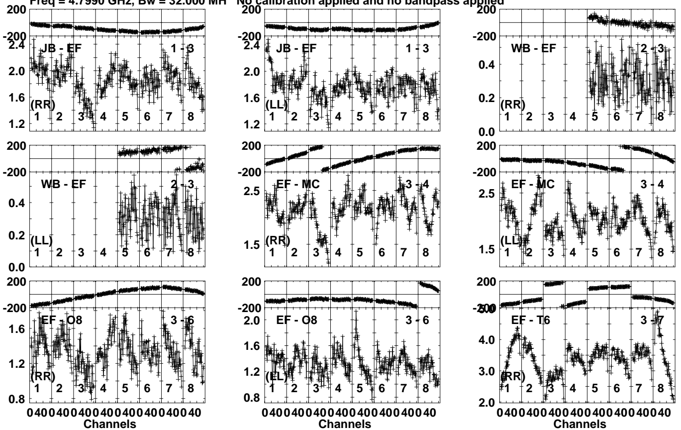
Lower frame: Milli Ampl Jy Top frame: Phas deg Vector averaged cross-power spectrum Several baselines displayed Timerange: 00/17:35:51 to 00/17:36:59
