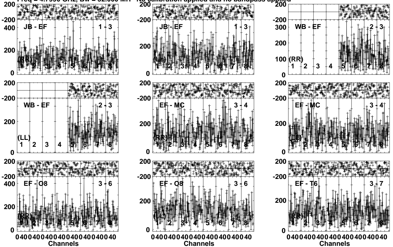
Lower frame: Micro Ampl Jy Top frame: Phas deg Vector averaged cross-power spectrum Several baselines displayed Timerange: 00/16:35:31 to 00/16:37:39
