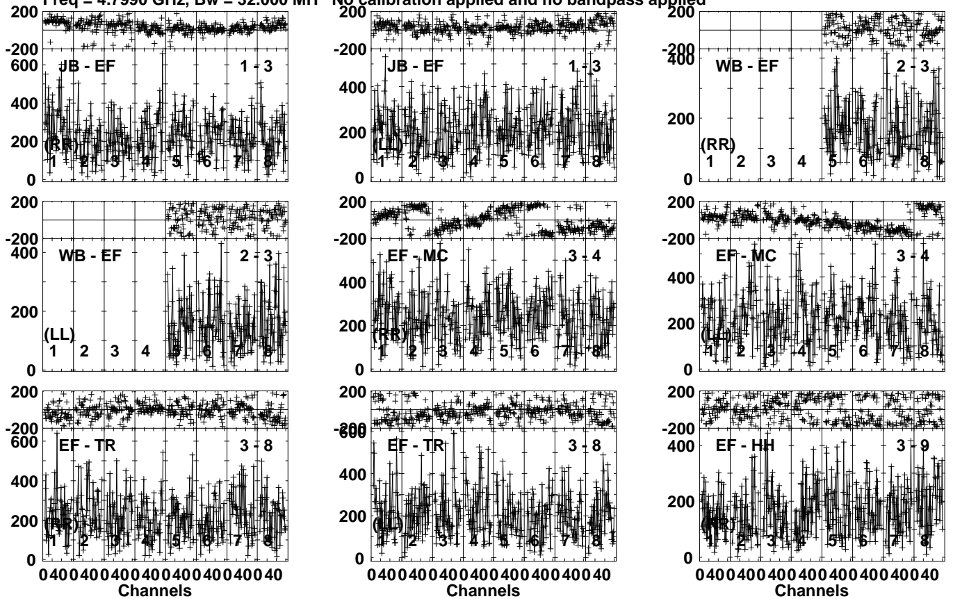
Lower frame: Micro Ampl Jy Top frame: Phas deg Vector averaged cross-power spectrum Several baselines displayed Timerange: 00/22:10:11 to 00/22:11:39
