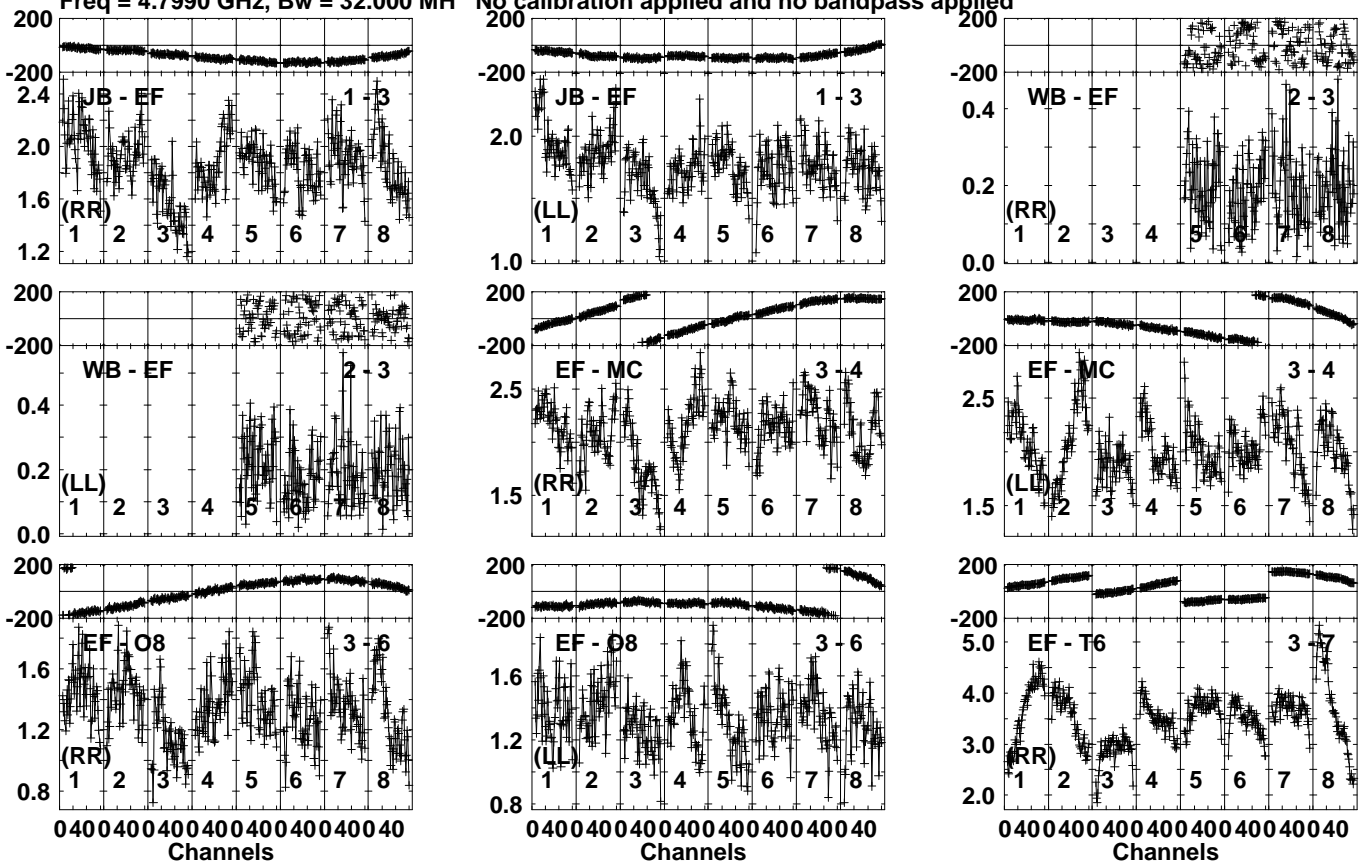
Lower frame: Milli Ampl Jy Top frame: Phas deg Vector averaged cross-power spectrum Several baselines displayed Timerange: 00/17:29:01 to 00/17:30:09
