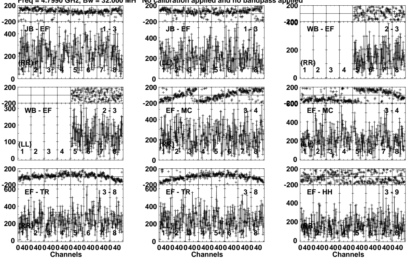
Lower frame: Micro Ampl Jy Top frame: Phas deg Vector averaged cross-power spectrum Several baselines displayed Timerange: 00/23:01:41 to 00/23:02:59
