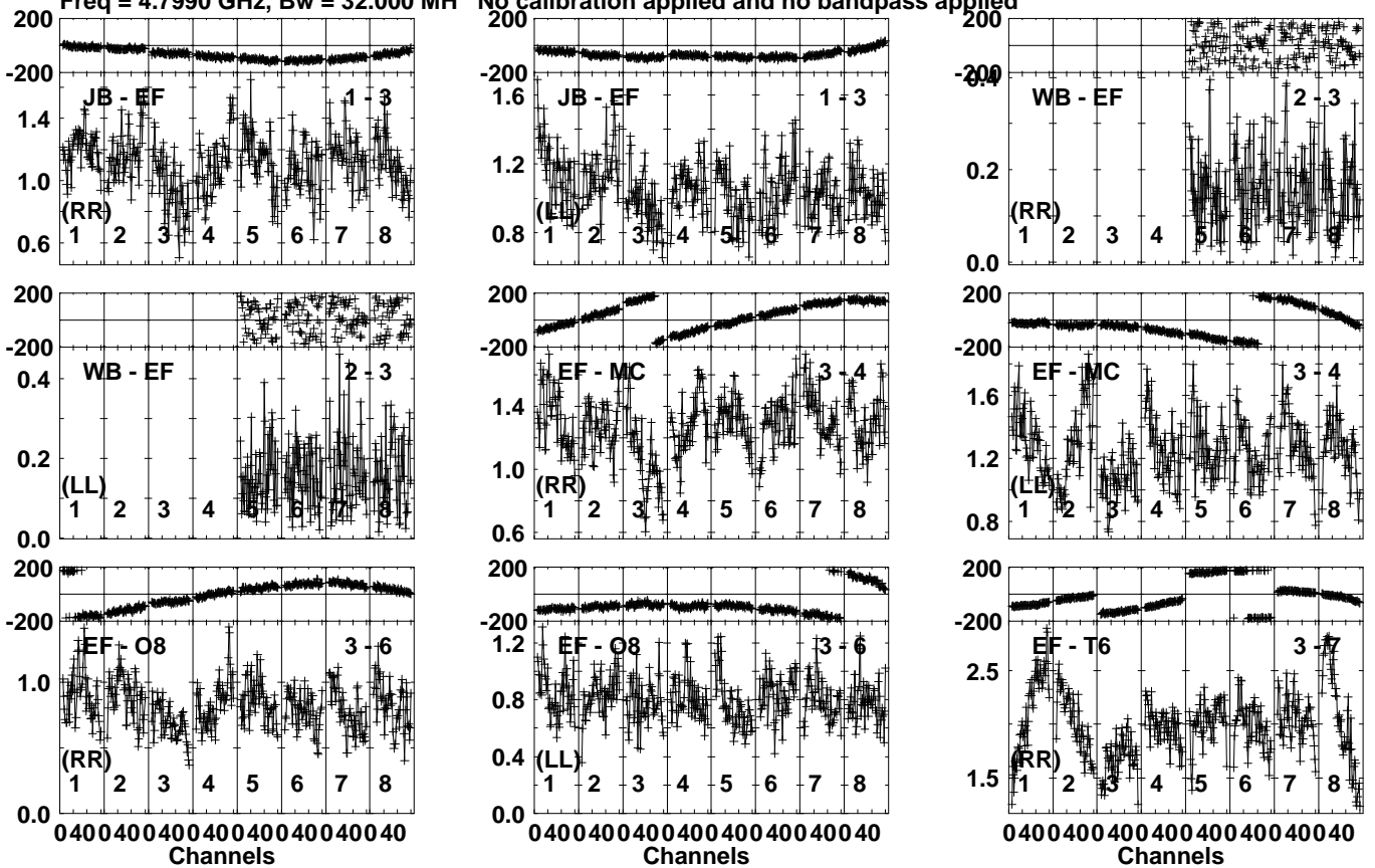
Lower frame: Milli Ampl Jy Top frame: Phas deg Vector averaged cross-power spectrum Several baselines displayed Timerange: 00/18:09:11 to 00/18:10:19
