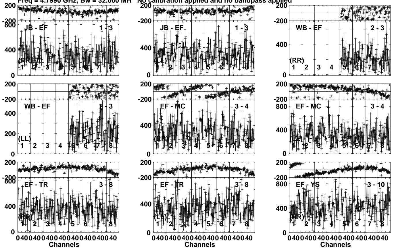
Lower frame: Micro Ampl Jy Top frame: Phas deg Vector averaged cross-power spectrum Several baselines displayed Timerange: 01/00:48:47 to 01/00:50:13
