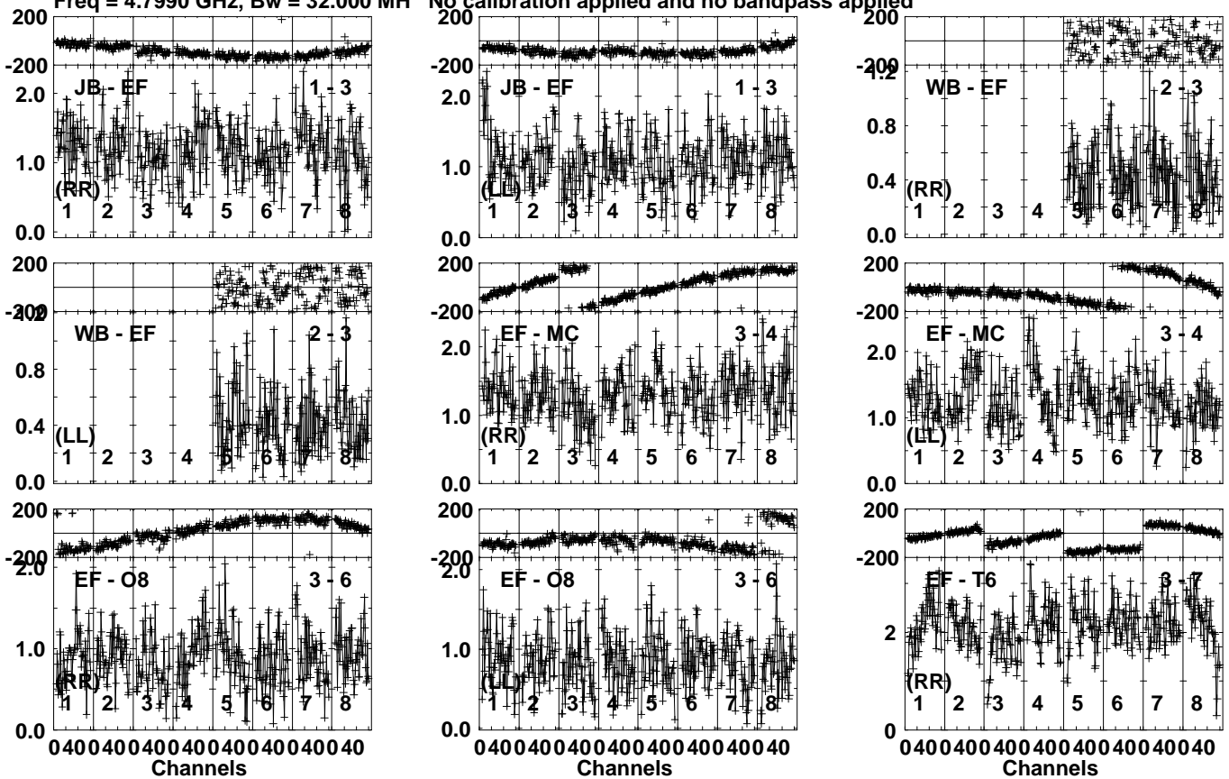
Lower frame: Milli Ampl Jy Top frame: Phas deg Vector averaged cross-power spectrum Several baselines displayed Timerange: 00/17:55:21 to 00/17:56:29
