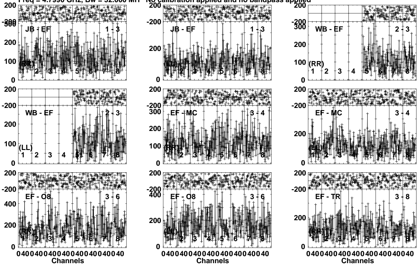
Lower frame: Micro Ampl Jy Top frame: Phas deg Vector averaged cross-power spectrum Several baselines displayed Timerange: 00/19:13:11 to 00/19:15:19
