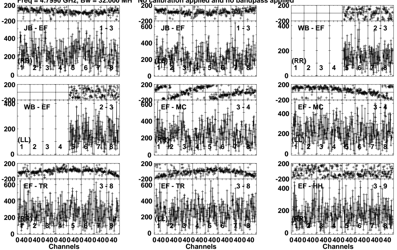
Lower frame: Micro Ampl Jy Top frame: Phas deg Vector averaged cross-power spectrum Several baselines displayed Timerange: 00/21:11:27 to 00/21:12:53
