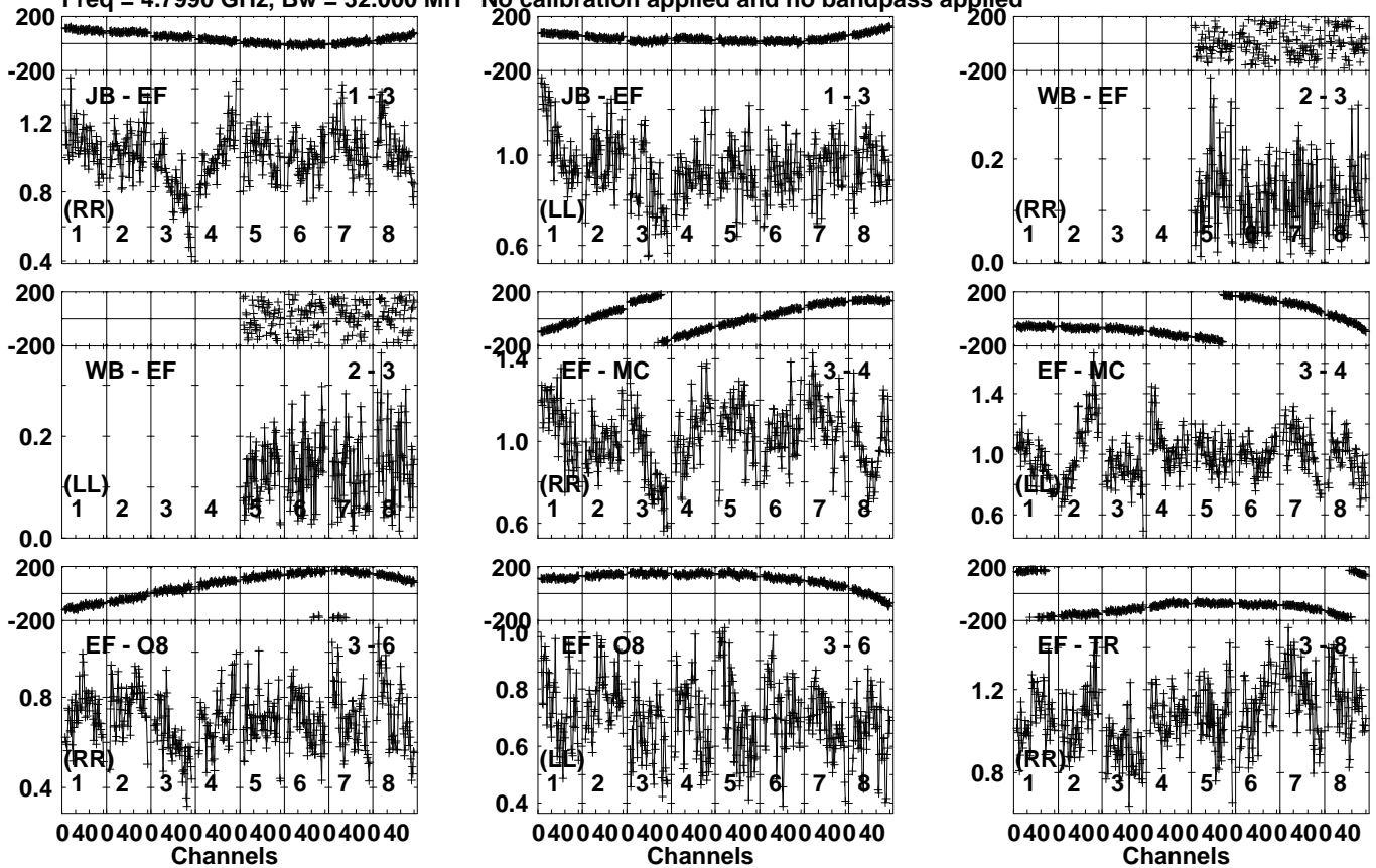
Lower frame: Milli Ampl Jy Top frame: Phas deg Vector averaged cross-power spectrum Several baselines displayed Timerange: 00/14:12:32 to 00/14:13:48
