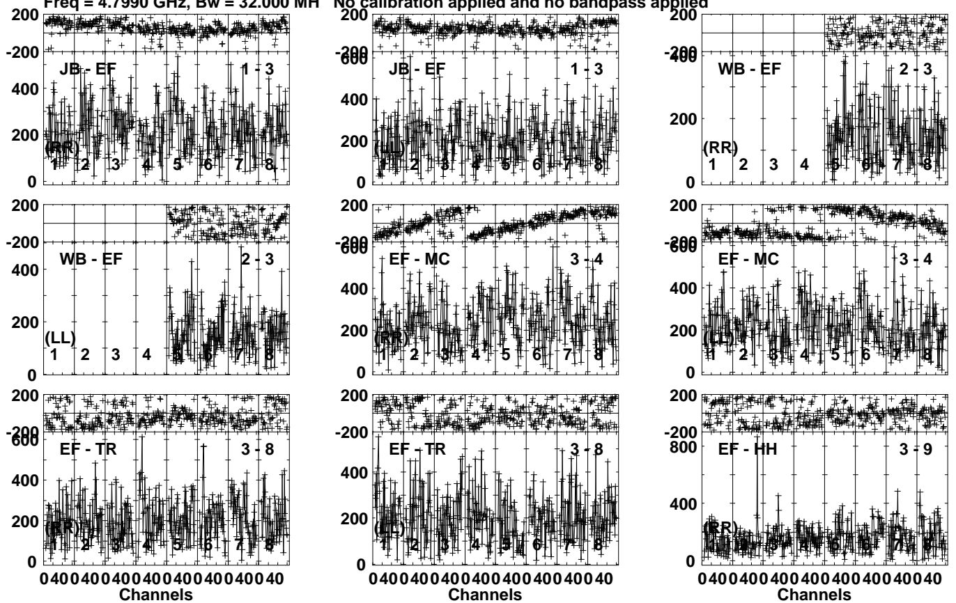
Lower frame: Micro Ampl Jy Top frame: Phas deg Vector averaged cross-power spectrum Several baselines displayed Timerange: 00/21:34:57 to 00/21:36:23
