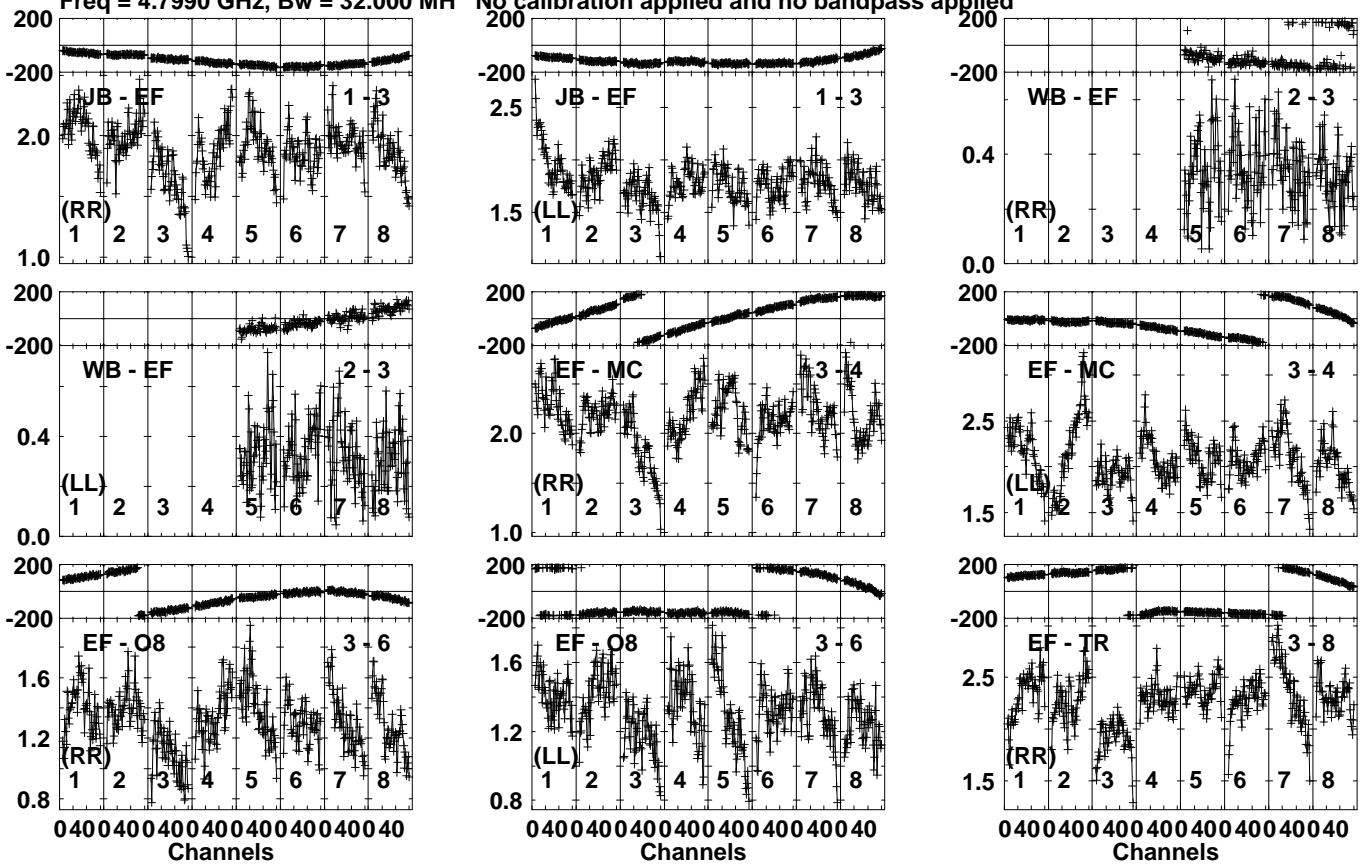
Lower frame: Milli Ampl Jy Top frame: Phas deg Vector averaged cross-power spectrum Several baselines displayed Timerange: 00/18:32:31 to 00/18:33:39
