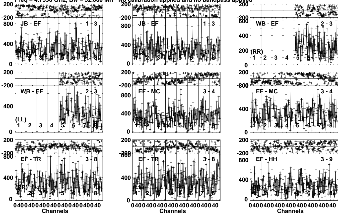
Lower frame: Micro Ampl Jy Top frame: Phas deg Vector averaged cross-power spectrum Several baselines displayed Timerange: 00/20:27:51 to 00/20:29:09
