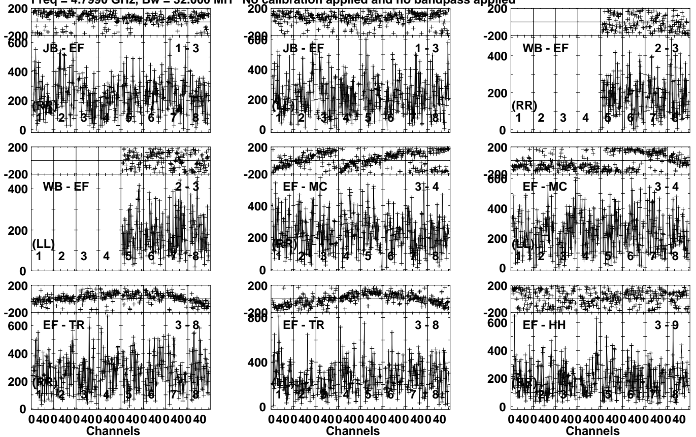
Lower frame: Micro Ampl Jy Top frame: Phas deg Vector averaged cross-power spectrum Several baselines displayed Timerange: 00/23:20:41 to 00/23:22:09
