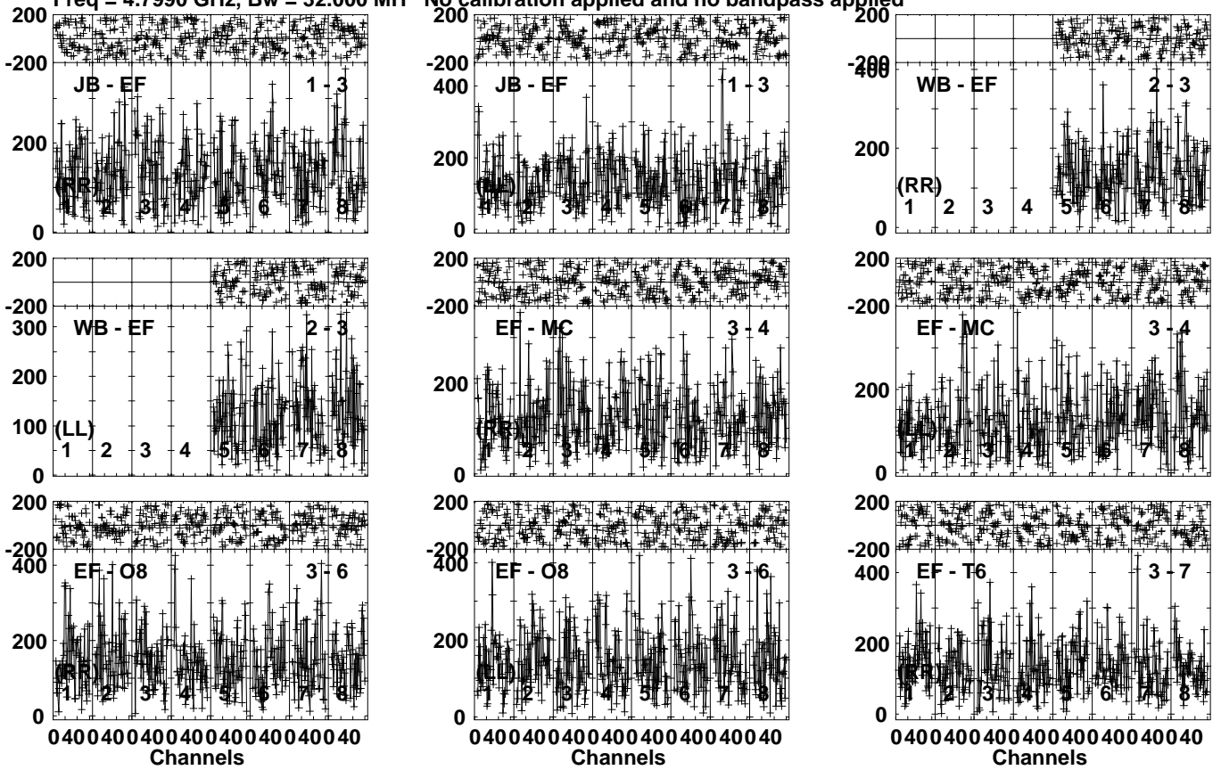
Lower frame: Micro Ampl Jy Top frame: Phas deg Vector averaged cross-power spectrum Several baselines displayed Timerange: 00/17:56:31 to 00/17:58:39
