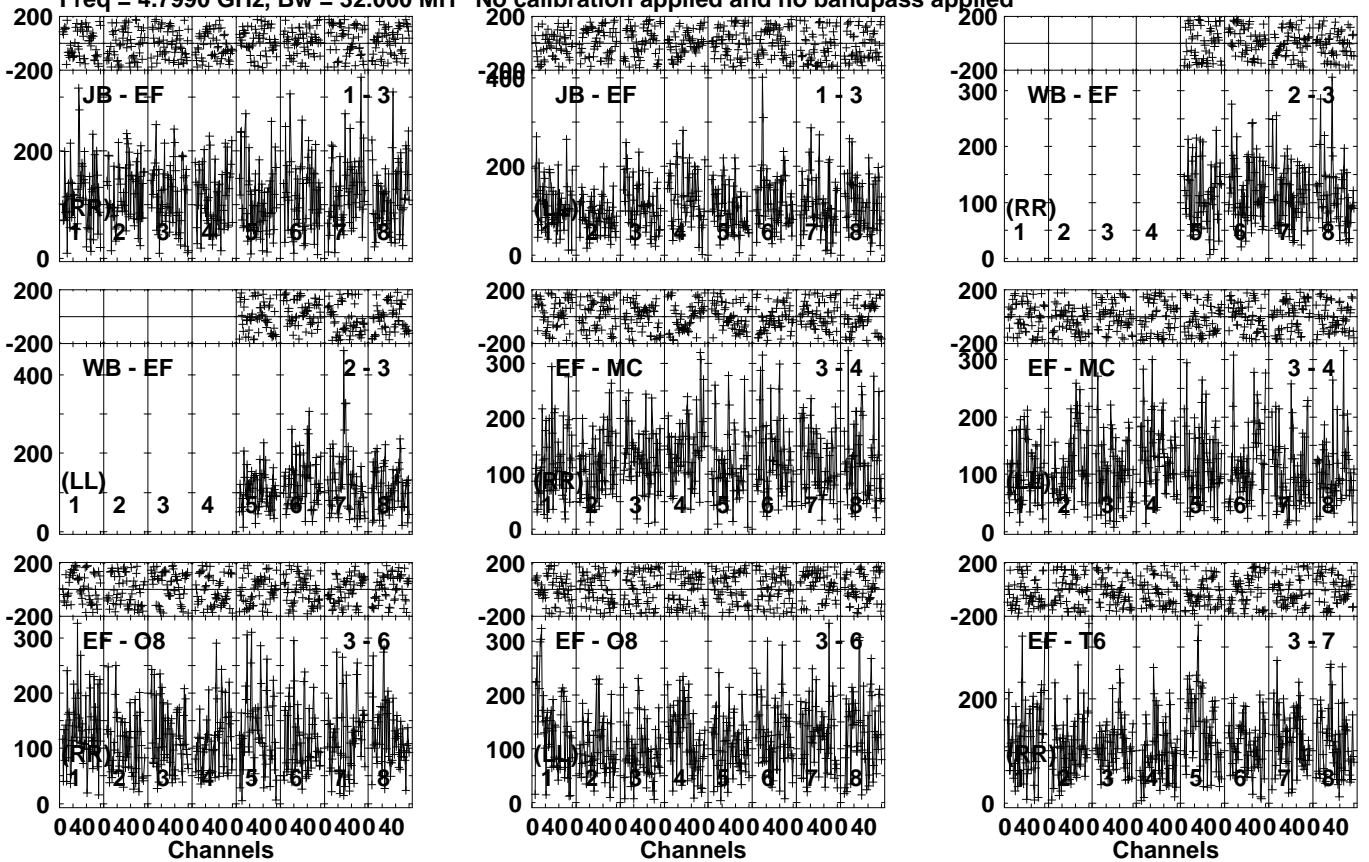
Lower frame: Micro Ampl Jy Top frame: Phas deg Vector averaged cross-power spectrum Several baselines displayed Timerange: 00/17:10:51 to 00/17:12:49
