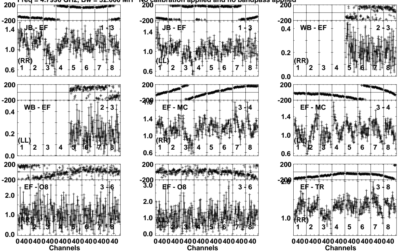
Lower frame: Milli Ampl Jy Top frame: Phas deg Vector averaged cross-power spectrum Several baselines displayed Timerange: 00/13:15:42 to 00/13:17:08
