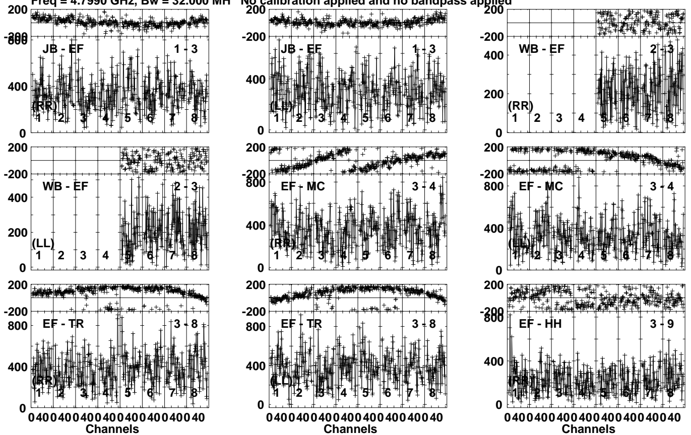
Lower frame: Micro Ampl Jy Top frame: Phas deg Vector averaged cross-power spectrum Several baselines displayed Timerange: 00/22:51:17 to 00/22:52:43
