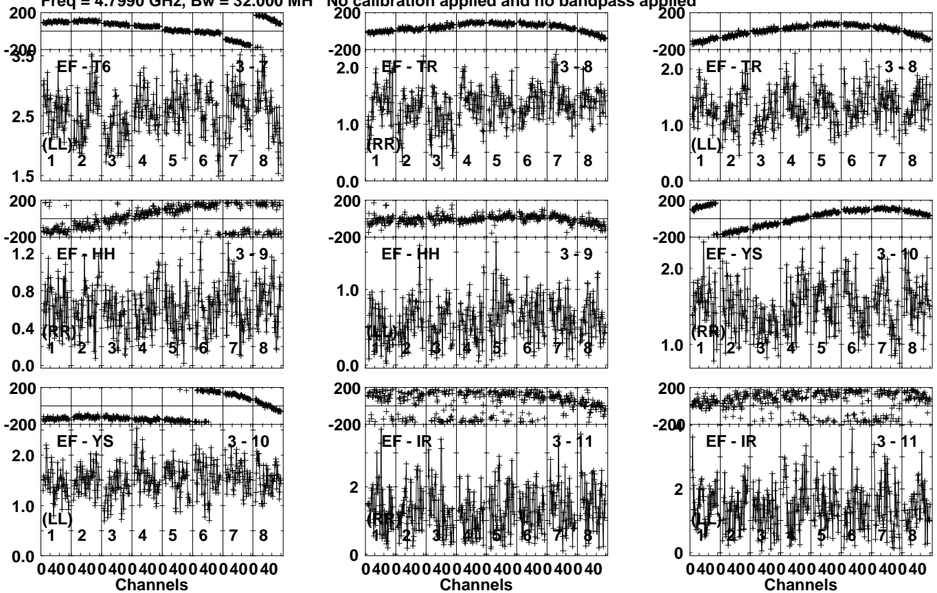
Lower frame: Milli Ampl Jy Top frame: Phas deg Vector averaged cross-power spectrum Several baselines displayed Timerange: 00/16:27:41 to 00/16:28:49
