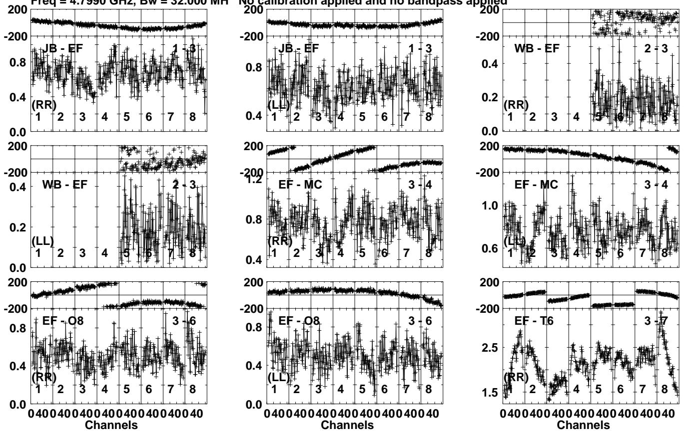
Lower frame: Milli Ampl Jy Top frame: Phas deg Vector averaged cross-power spectrum Several baselines displayed Timerange: 00/15:33:21 to 00/15:34:29
