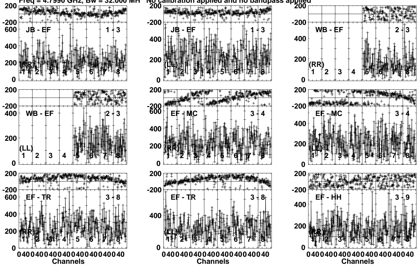
Lower frame: Micro Ampl Jy Top frame: Phas deg Vector averaged cross-power spectrum Several baselines displayed Timerange: 00/22:53:17 to 00/22:54:33
