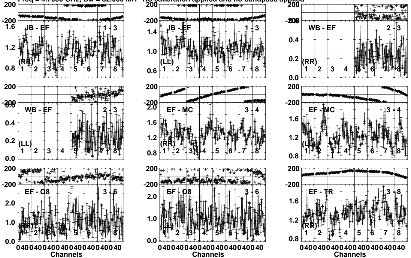
Lower frame: Milli Ampl Jy Top frame: Phas deg Vector averaged cross-power spectrum Several baselines displayed Timerange: 00/19:08:41 to 00/19:09:49
