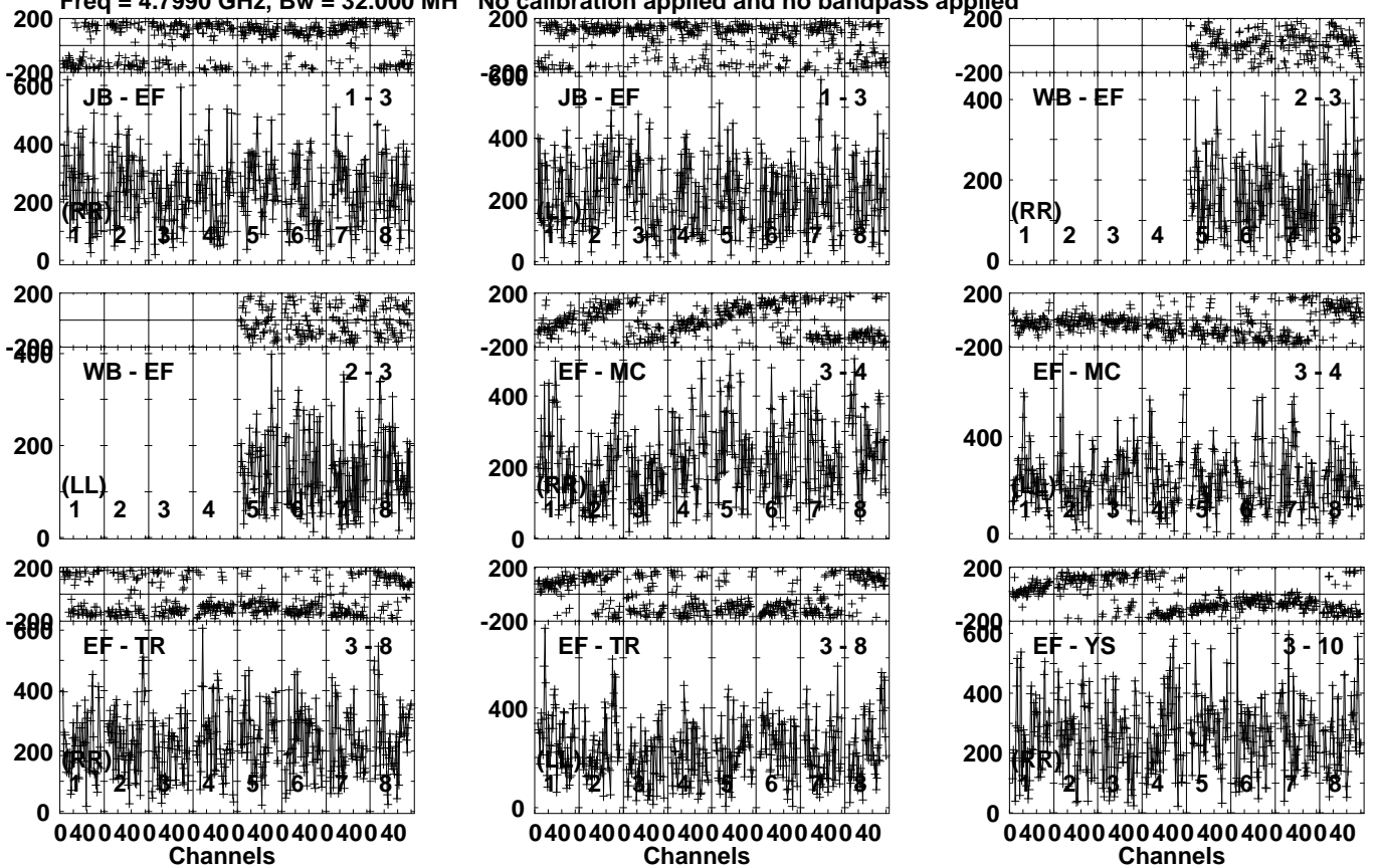
Lower frame: Micro Ampl Jy Top frame: Phas deg Vector averaged cross-power spectrum Several baselines displayed Timerange: 00/23:52:01 to 00/23:53:19
