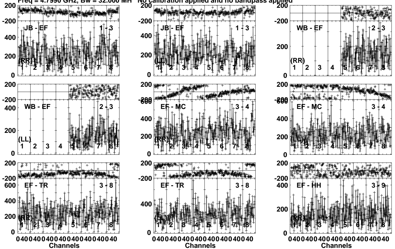
Lower frame: Micro Ampl Jy Top frame: Phas deg Vector averaged cross-power spectrum Several baselines displayed Timerange: 00/21:19:17 to 00/21:20:33
