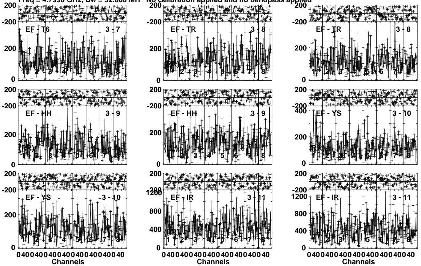
Lower frame: Micro Ampl Jy Top frame: Phas deg Vector averaged cross-power spectrum Several baselines displayed Timerange: 00/16:38:51 to 00/16:40:59
