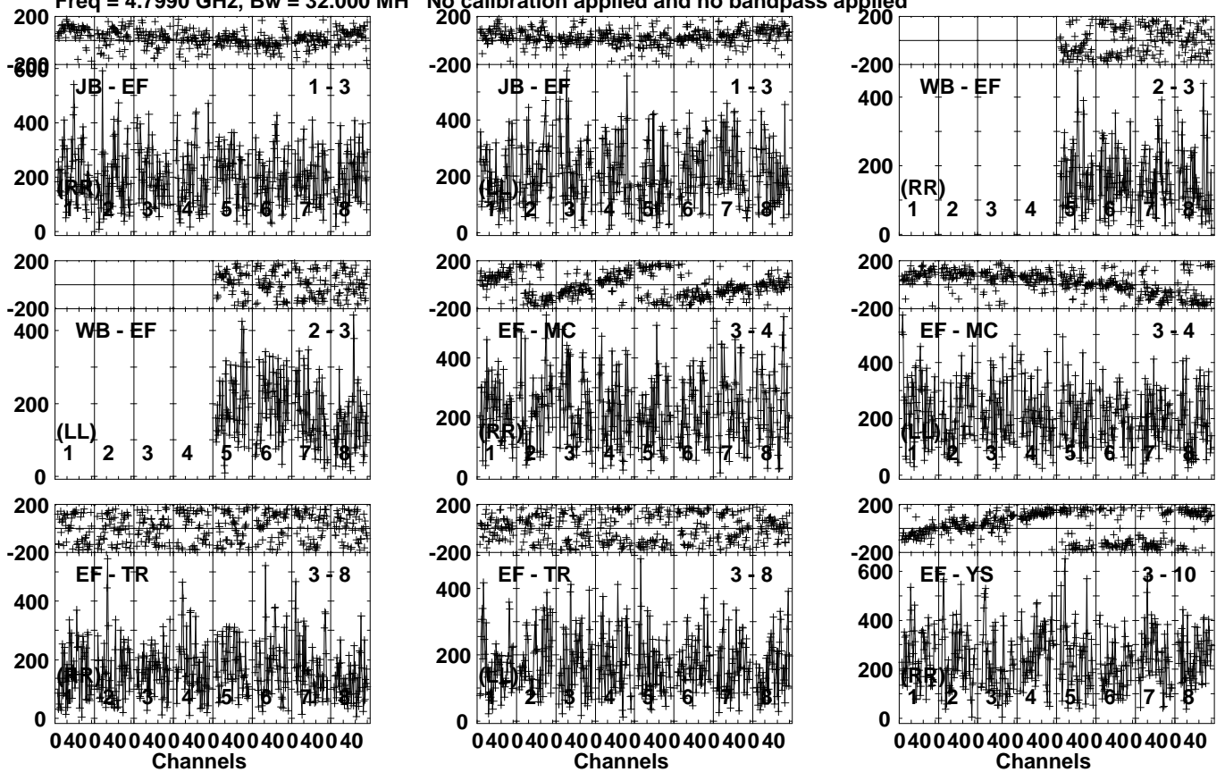
Lower frame: Micro Ampl Jy Top frame: Phas deg Vector averaged cross-power spectrum Several baselines displayed Timerange: 01/00:15:31 to 01/00:16:49
