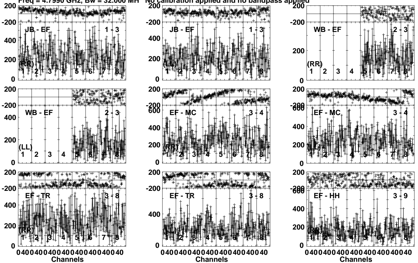
Lower frame: Micro Ampl Jy Top frame: Phas deg Vector averaged cross-power spectrum Several baselines displayed Timerange: 00/20:59:41 to 00/21:01:09
