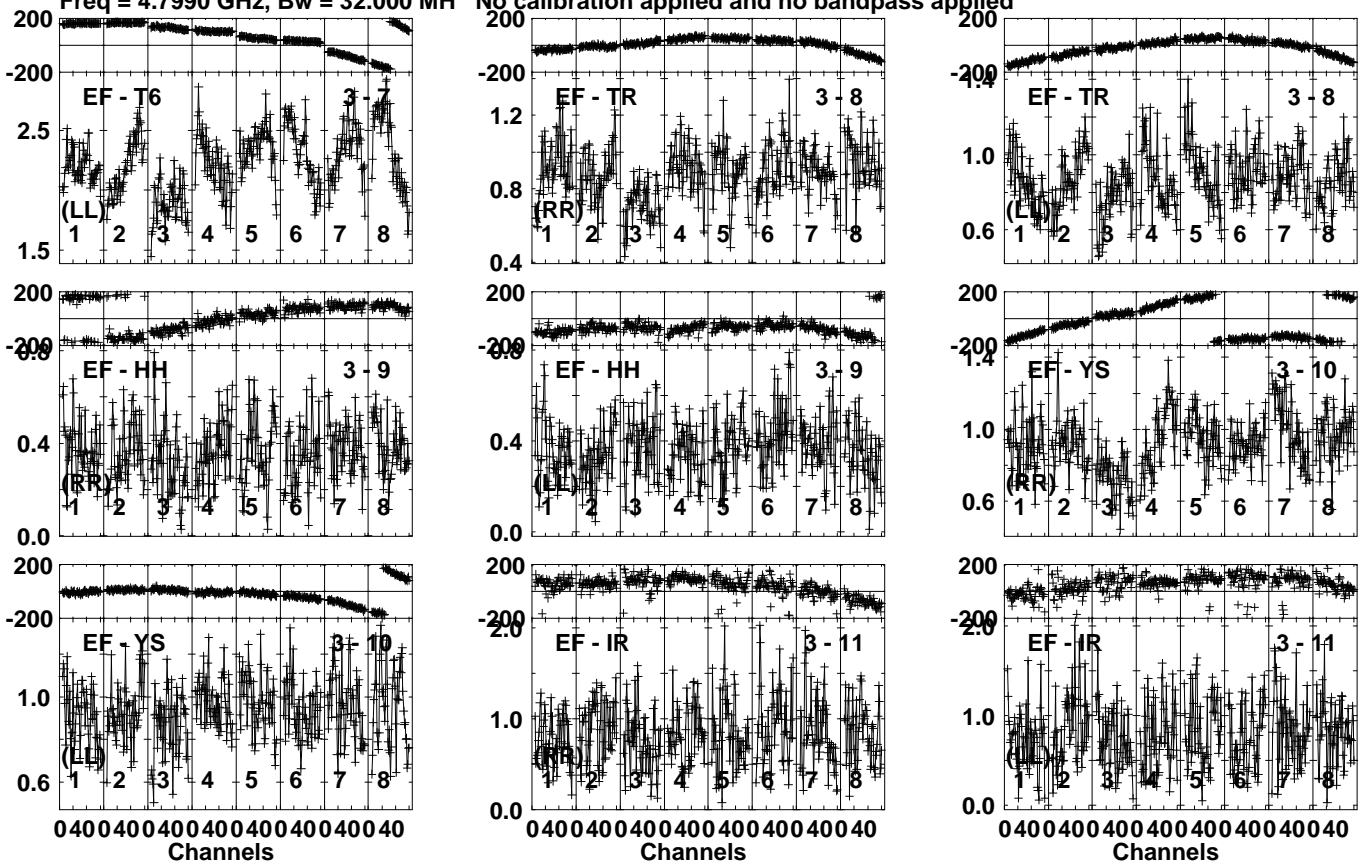
Lower frame: Milli Ampl Jy Top frame: Phas deg Vector averaged cross-power spectrum Several baselines displayed Timerange: 00/15:41:51 to 00/15:42:59
