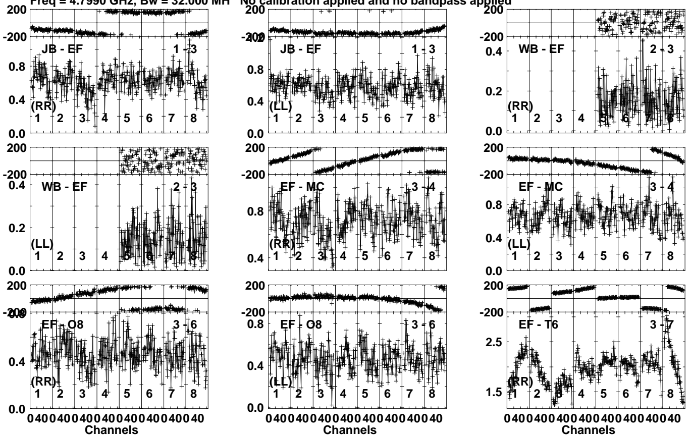
Lower frame: Milli Ampl Jy Top frame: Phas deg Vector averaged cross-power spectrum Several baselines displayed Timerange: 00/15:09:41 to 00/15:10:49
