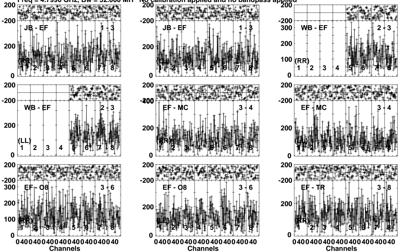
Lower frame: Micro Ampl Jy Top frame: Phas deg Vector averaged cross-power spectrum Several baselines displayed Timerange: 00/19:46:31 to 00/19:48:39
