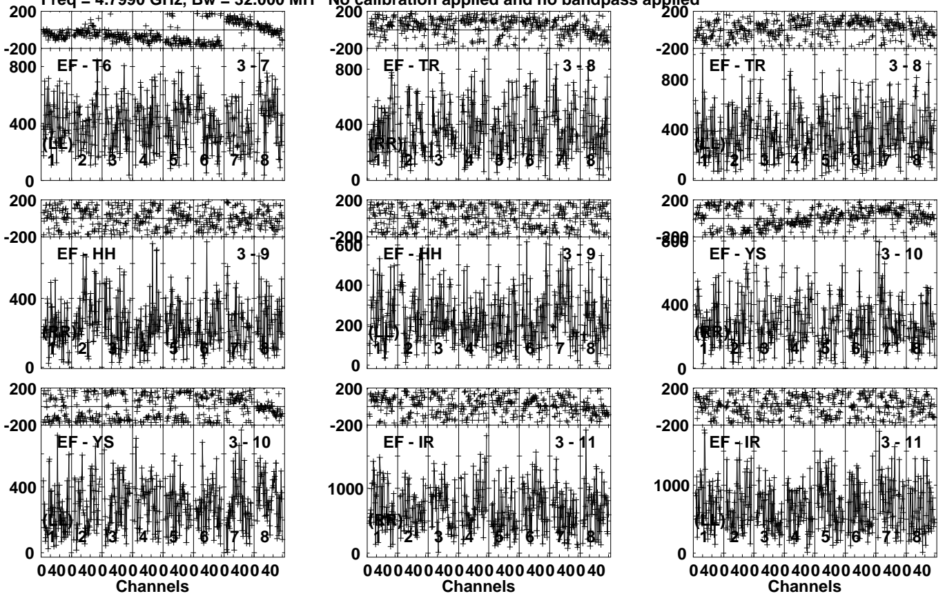
Lower frame: Micro Ampl Jy Top frame: Phas deg Vector averaged cross-power spectrum Several baselines displayed Timerange: 00/16:42:41 to 00/16:43:49
