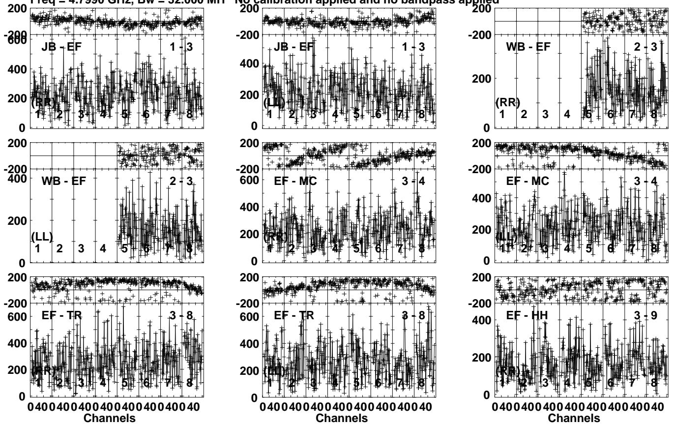
Lower frame: Micro Ampl Jy Top frame: Phas deg Vector averaged cross-power spectrum Several baselines displayed Timerange: 00/22:33:41 to 00/22:35:09
