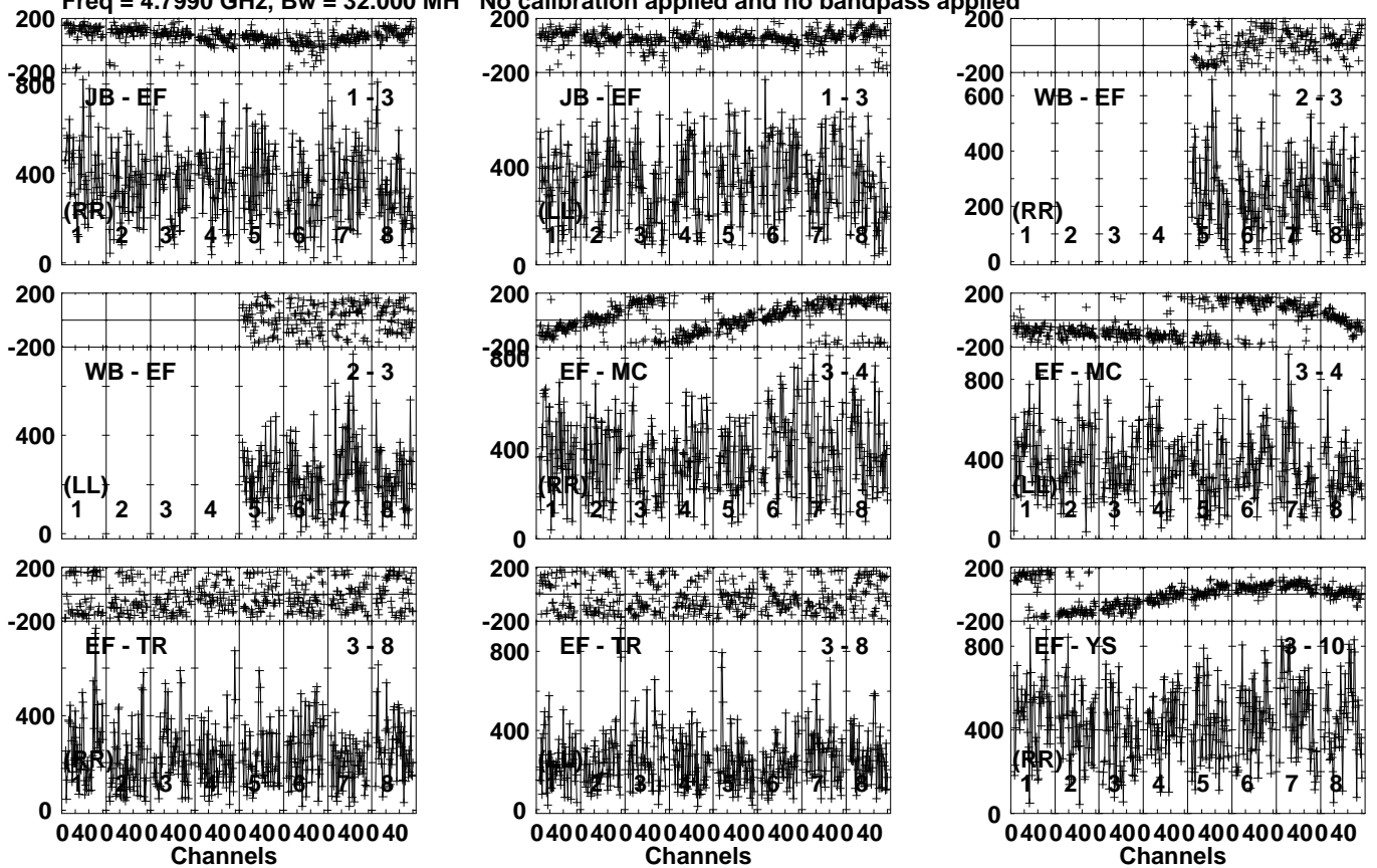
Lower frame: Micro Ampl Jy Top frame: Phas deg Vector averaged cross-power spectrum Several baselines displayed Timerange: 00/21:52:31 to 00/21:53:59
