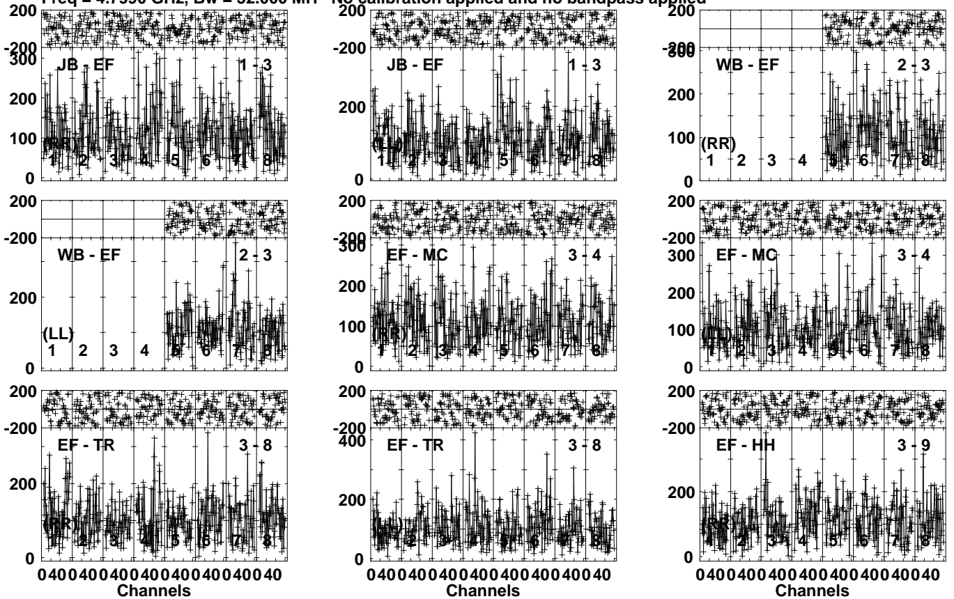
Lower frame: Micro Ampl Jy Top frame: Phas deg Vector averaged cross-power spectrum Several baselines displayed Timerange: 00/22:23:27 to 00/22:25:53
