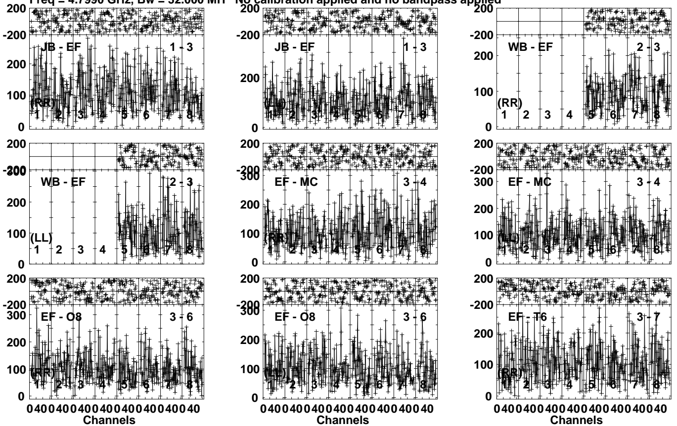
Lower frame: Micro Ampl Jy Top frame: Phas deg Vector averaged cross-power spectrum Several baselines displayed Timerange: 00/15:38:41 to 00/15:41:19
