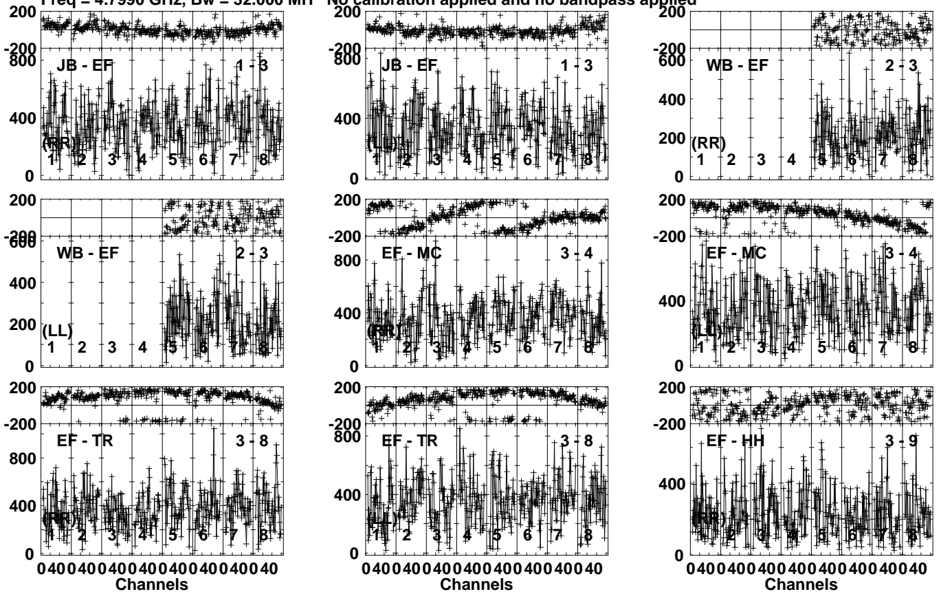
Lower frame: Micro Ampl Jy Top frame: Phas deg Vector averaged cross-power spectrum Several baselines displayed Timerange: 00/22:39:31 to 00/22:40:59
