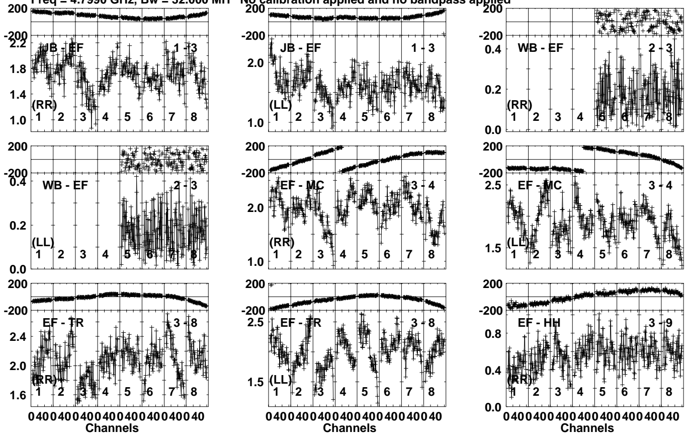
Lower frame: Milli Ampl Jy Top frame: Phas deg Vector averaged cross-power spectrum Several baselines displayed Timerange: 00/20:19:11 to 00/20:20:19
