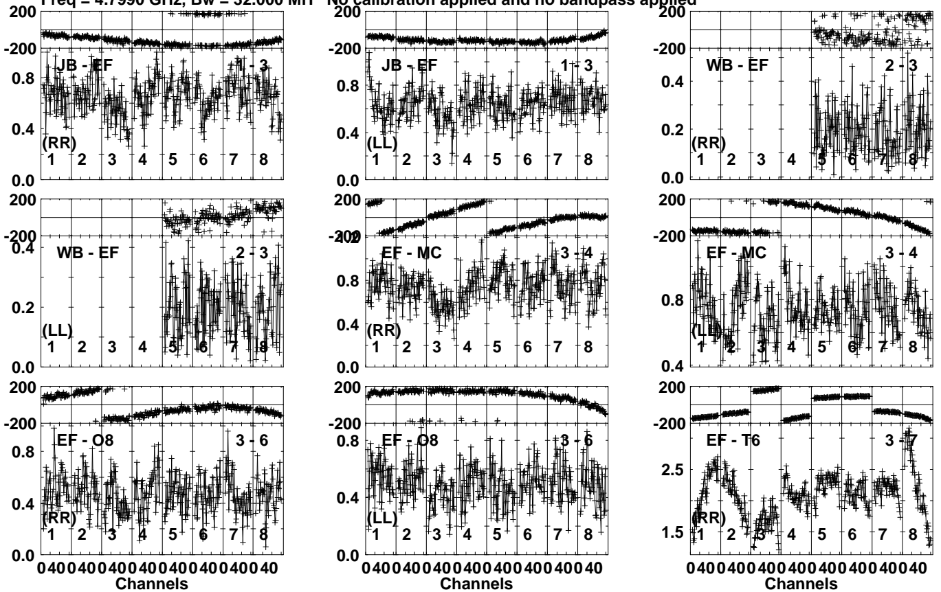
Lower frame: Milli Ampl Jy Top frame: Phas deg Vector averaged cross-power spectrum Several baselines displayed Timerange: 00/15:25:21 to 00/15:26:49
