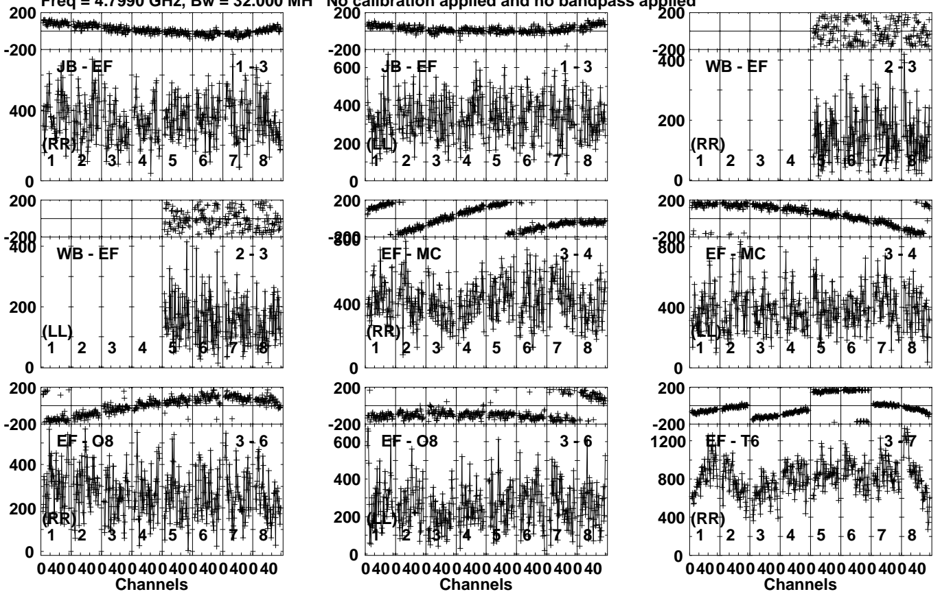
Lower frame: Micro Ampl Jy Top frame: Phas deg Vector averaged cross-power spectrum Several baselines displayed Timerange: 00/15:54:51 to 00/15:56:29
