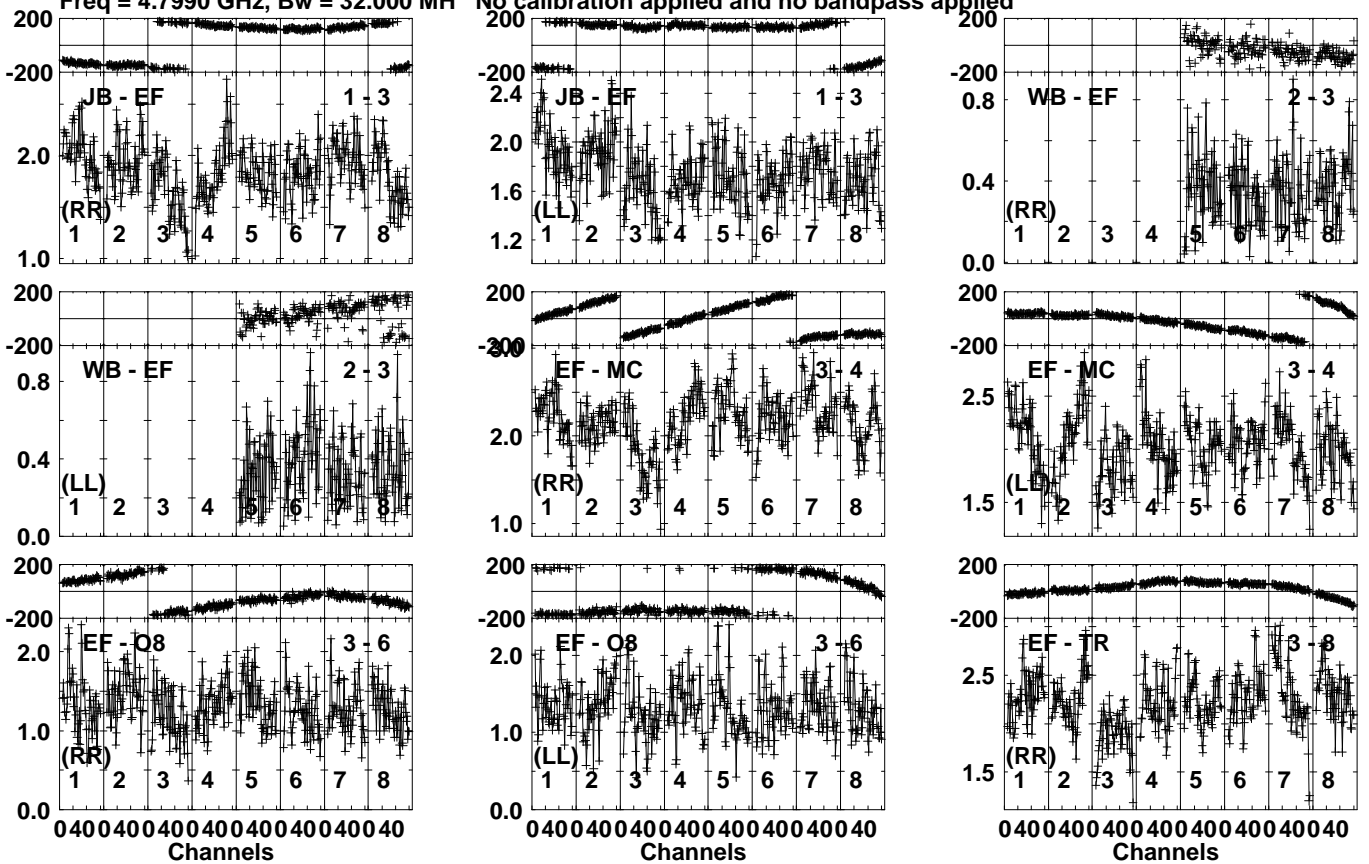
Lower frame: Milli Ampl Jy Top frame: Phas deg Vector averaged cross-power spectrum Several baselines displayed Timerange: 00/19:25:21 to 00/19:26:29
