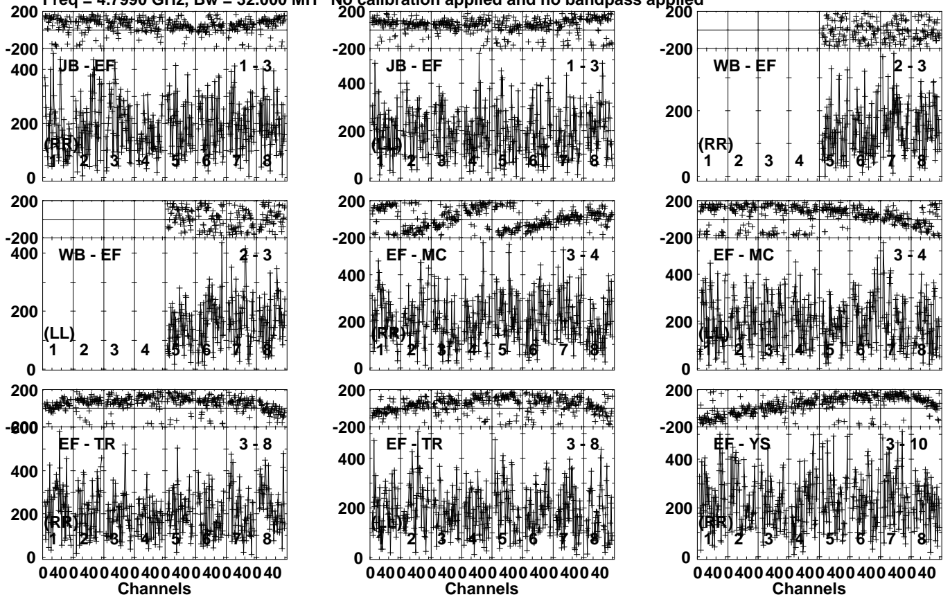
Lower frame: Micro Ampl Jy Top frame: Phas deg Vector averaged cross-power spectrum Several baselines displayed Timerange: 01/00:35:41 to 01/00:36:59
