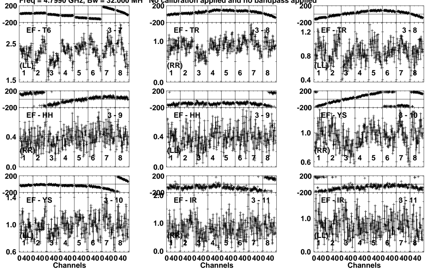
Lower frame: Milli Ampl Jy Top frame: Phas deg Vector averaged cross-power spectrum Several baselines displayed Timerange: 00/15:57:01 to 00/15:58:09
