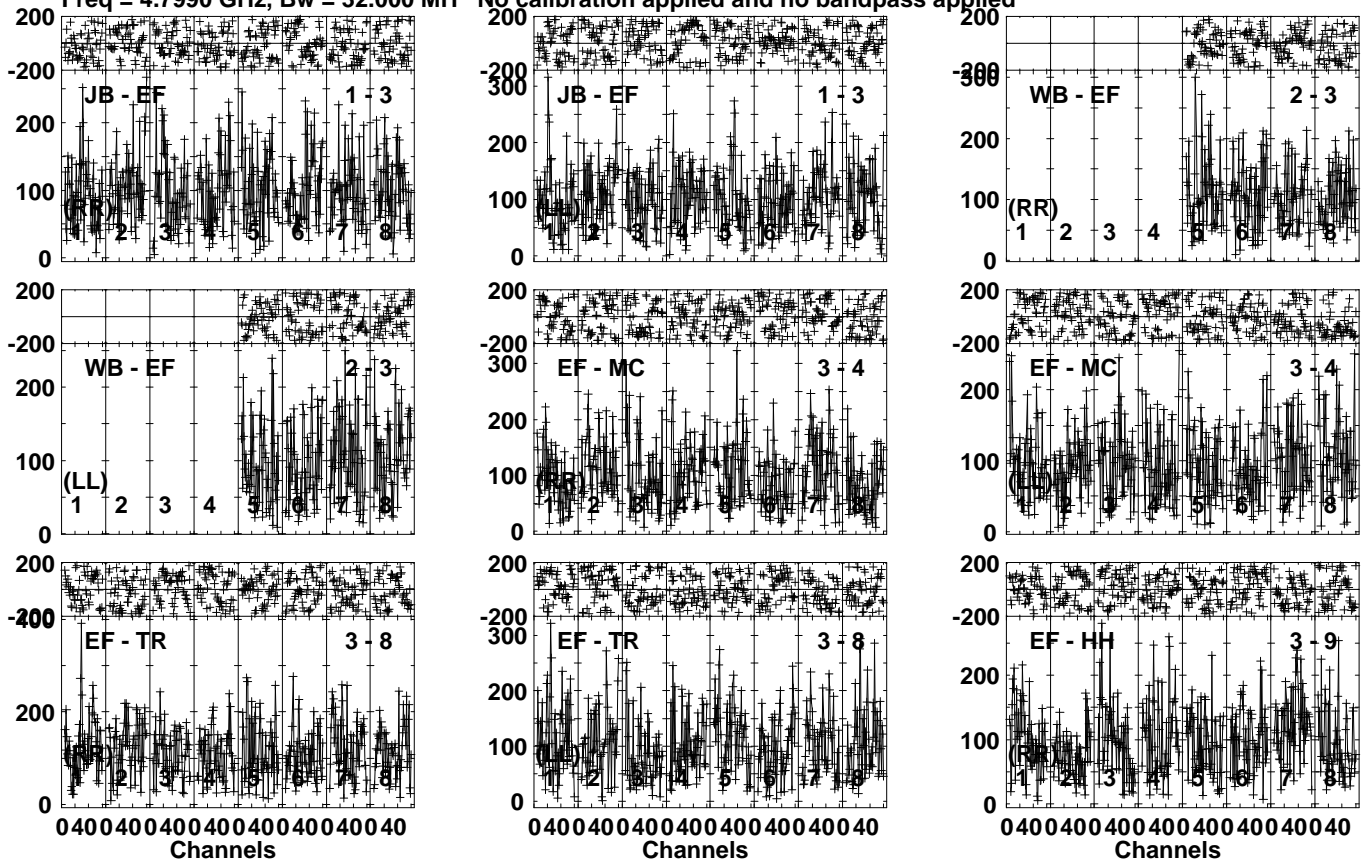
Lower frame: Micro Ampl Jy Top frame: Phas deg Vector averaged cross-power spectrum Several baselines displayed Timerange: 00/21:48:11 to 00/21:50:39
