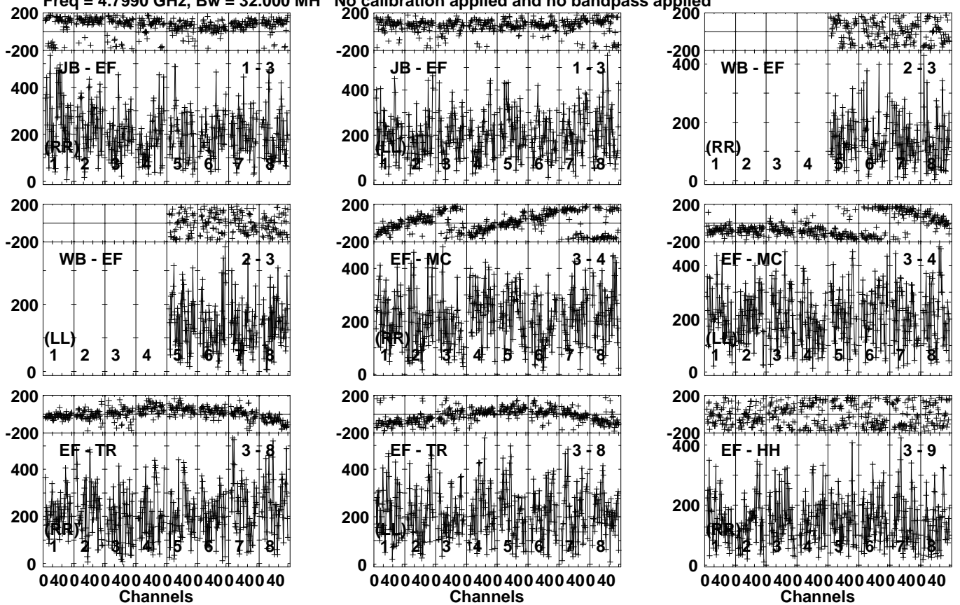
Lower frame: Micro Ampl Jy Top frame: Phas deg Vector averaged cross-power spectrum Several baselines displayed Timerange: 00/23:25:11 to 00/23:26:29
