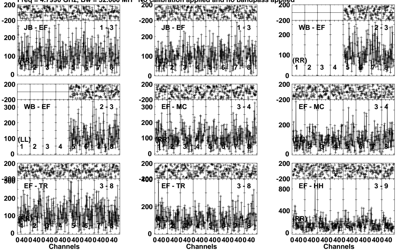
Lower frame: Micro Ampl Jy Top frame: Phas deg Vector averaged cross-power spectrum Several baselines displayed Timerange: 00/21:59:57 to 00/22:02:23
