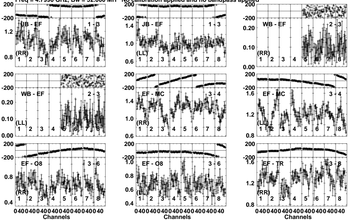
Lower frame: Milli Ampl Jy Top frame: Phas deg Vector averaged cross-power spectrum Several baselines displayed Timerange: 00/19:44:11 to 00/19:46:29
