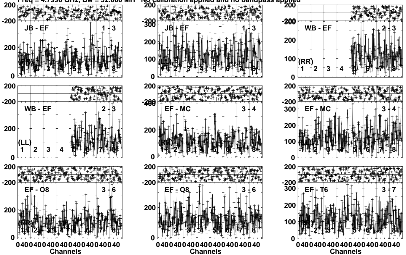
Lower frame: Micro Ampl Jy Top frame: Phas deg Vector averaged cross-power spectrum Several baselines displayed Timerange: 00/17:23:41 to 00/17:25:39
