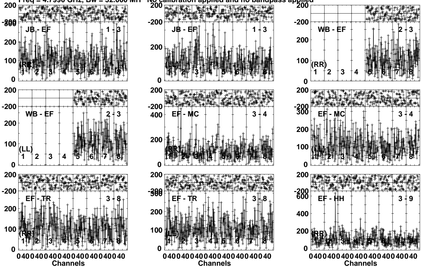
Lower frame: Micro Ampl Jy Top frame: Phas deg Vector averaged cross-power spectrum Several baselines displayed Timerange: 00/22:54:37 to 00/22:57:09
