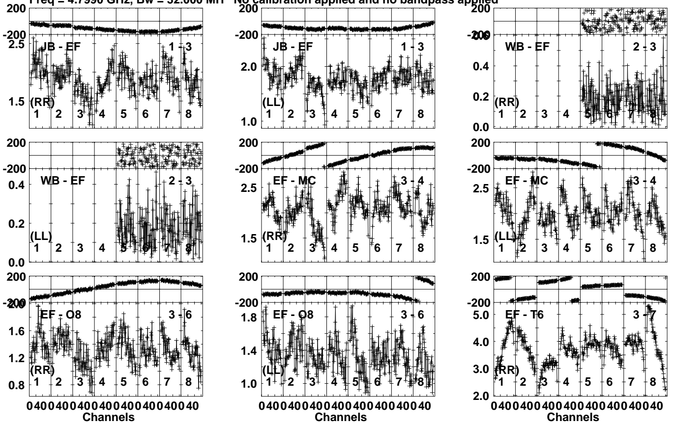
Lower frame: Milli Ampl Jy Top frame: Phas deg Vector averaged cross-power spectrum Several baselines displayed Timerange: 00/17:12:51 to 00/17:13:59
