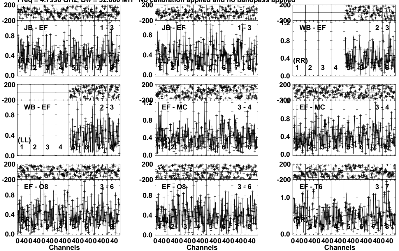
Lower frame: Milli Ampl Jy Top frame: Phas deg Vector averaged cross-power spectrum Several baselines displayed Timerange: 00/18:10:21 to 00/18:11:29
