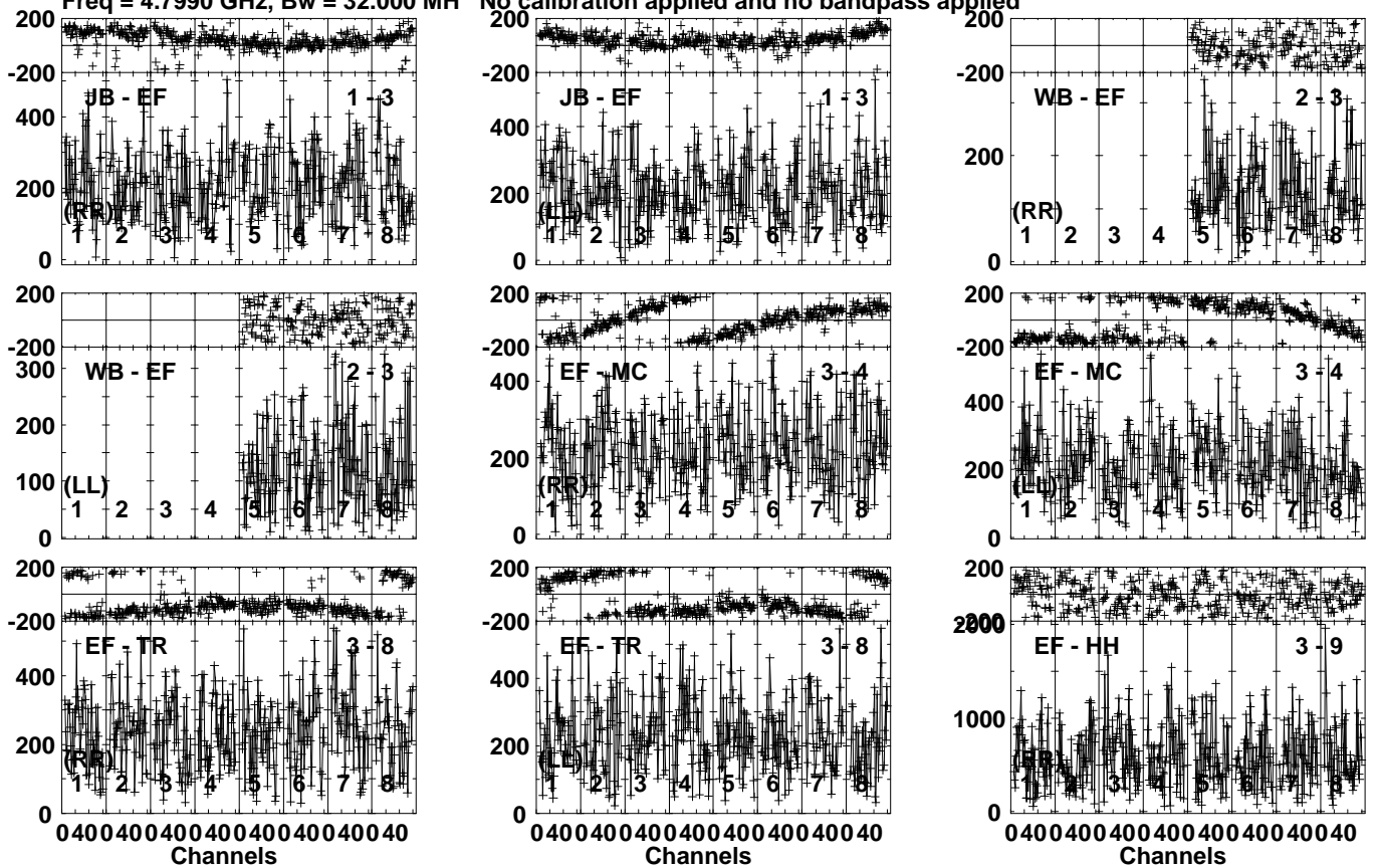
Lower frame: Micro Ampl Jy Top frame: Phas deg Vector averaged cross-power spectrum Several baselines displayed Timerange: 00/21:27:41 to 00/21:28:59
