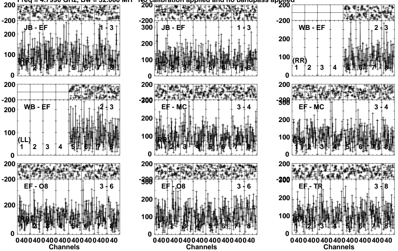
Lower frame: Micro Ampl Jy Top frame: Phas deg Vector averaged cross-power spectrum Several baselines displayed Timerange: 00/12:24:22 to 00/12:26:58
