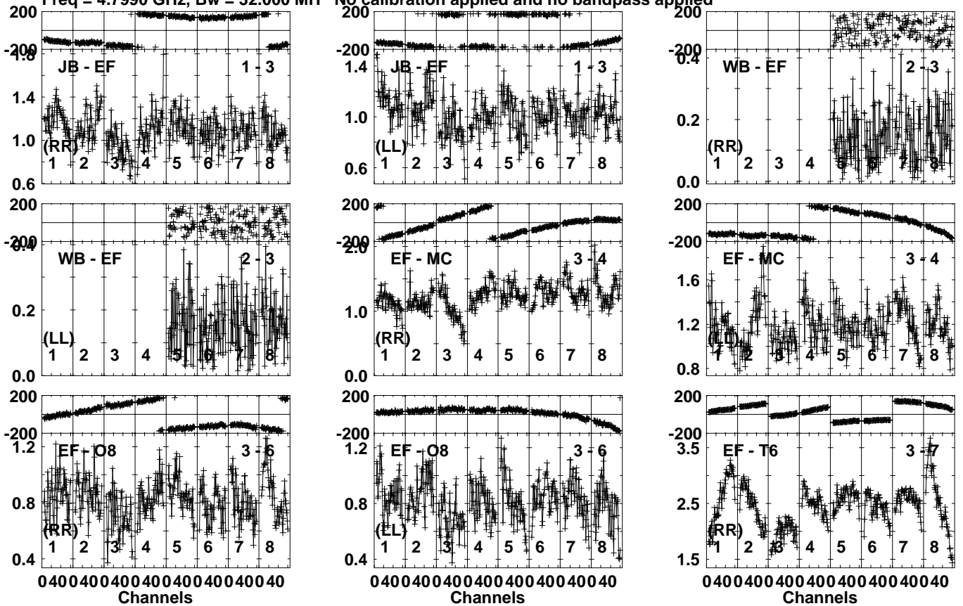
Lower frame: Milli Ampl Jy Top frame: Phas deg Vector averaged cross-power spectrum Several baselines displayed Timerange: 00/16:44:21 to 00/16:45:29
