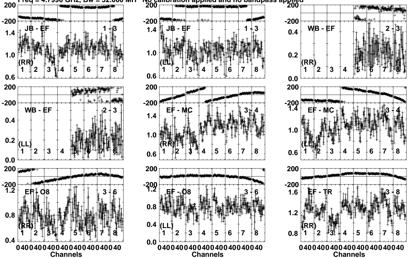
Lower frame: Milli Ampl Jy Top frame: Phas deg Vector averaged cross-power spectrum Several baselines displayed Timerange: 00/12:59:32 to 00/13:00:48
