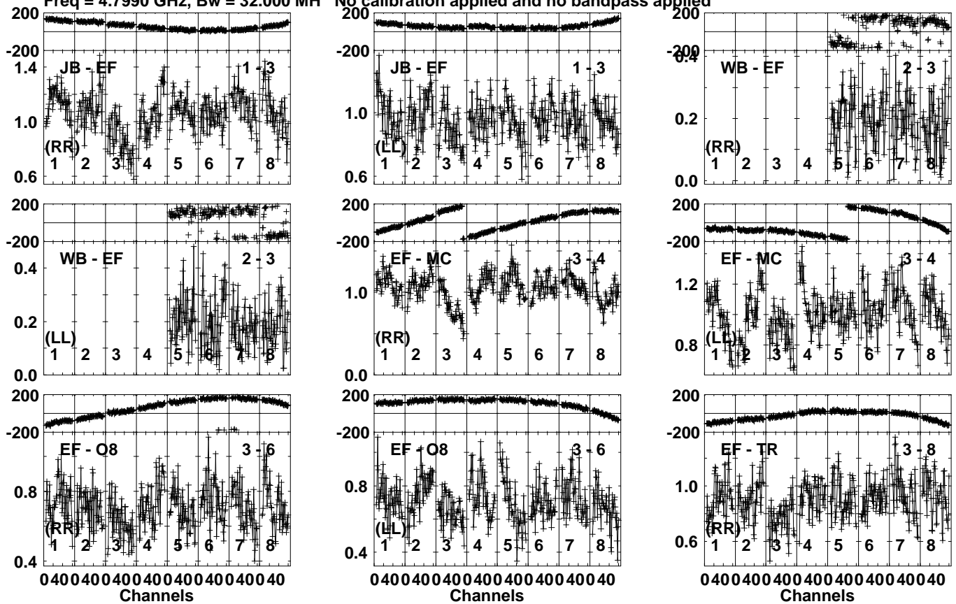
Lower frame: Milli Ampl Jy Top frame: Phas deg Vector averaged cross-power spectrum Several baselines displayed Timerange: 00/14:09:02 to 00/14:10:18
