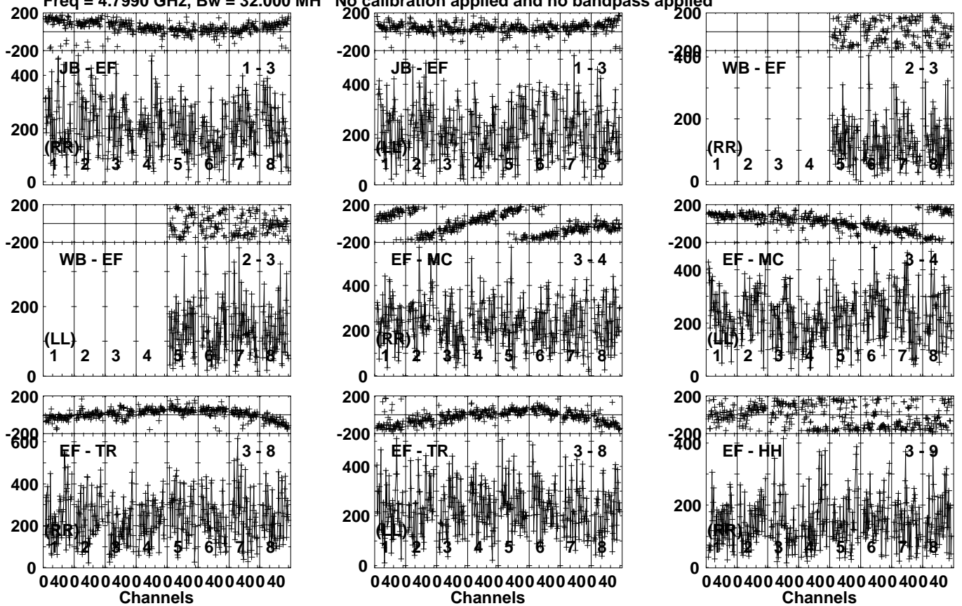
Lower frame: Micro Ampl Jy Top frame: Phas deg Vector averaged cross-power spectrum Several baselines displayed Timerange: 00/21:04:11 to 00/21:05:29
