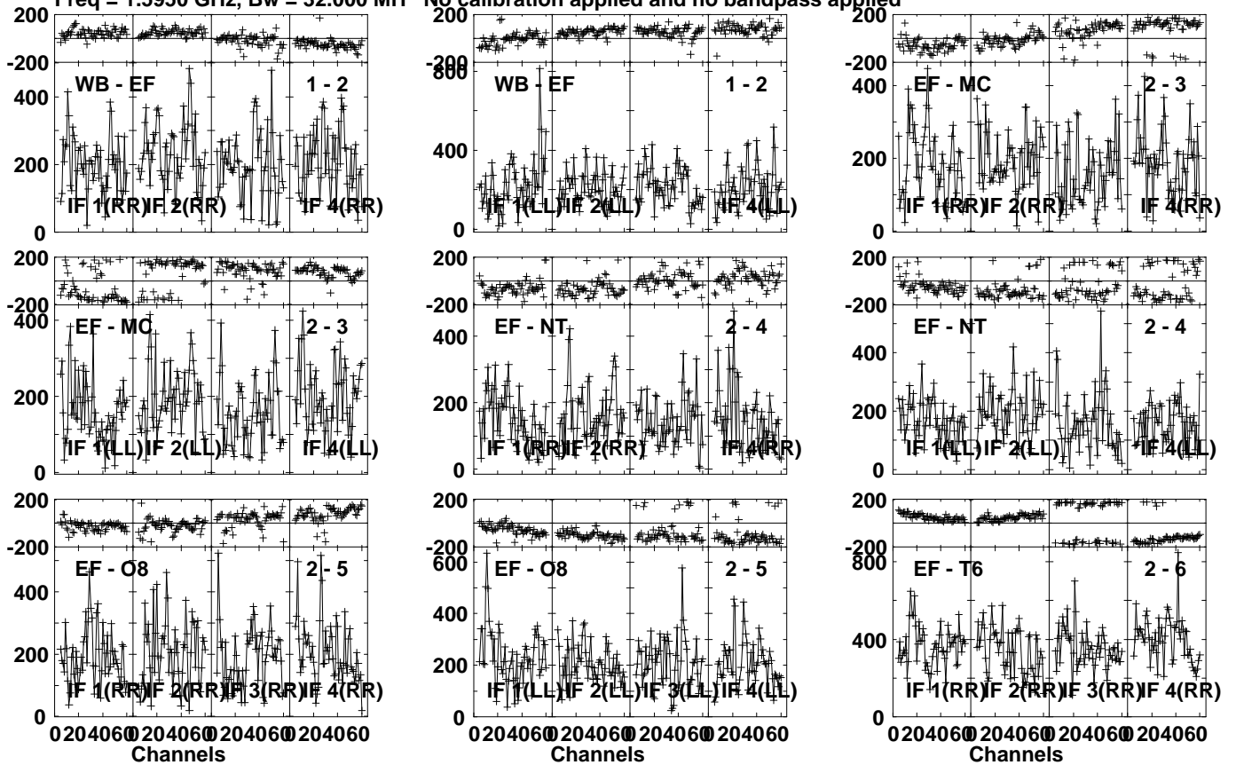
Lower frame: Micro Ampl Jy Top frame: Phas deg Vector averaged cross-power spectrum Several baselines displayed Timerange: 00/14:51:21 to 00/14:52:49
