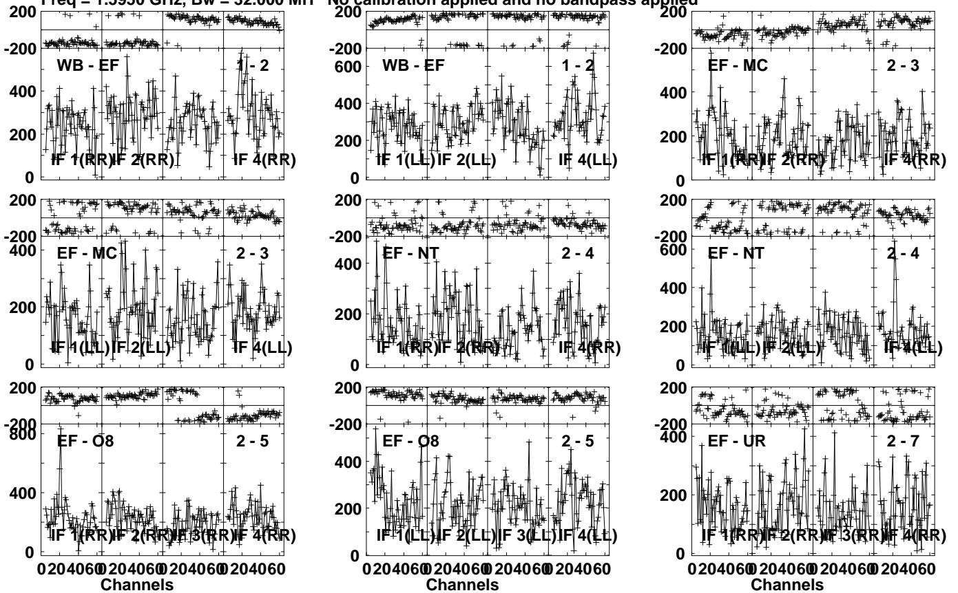
Lower frame: Micro Ampl Jy Top frame: Phas deg Vector averaged cross-power spectrum Several baselines displayed Timerange: 00/18:16:21 to 00/18:17:39
