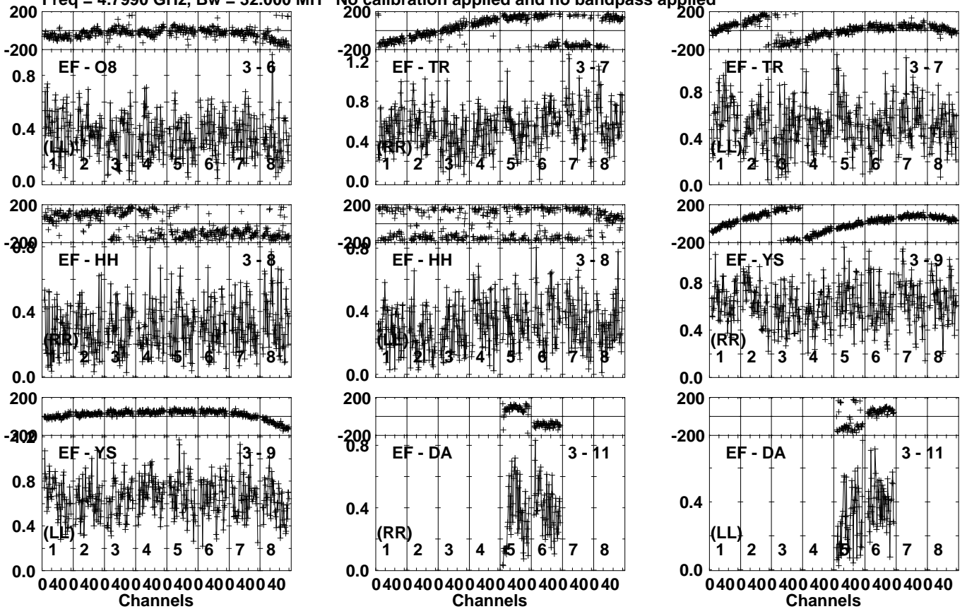
Lower frame: Milli Ampl Jy Top frame: Phas deg Vector averaged cross-power spectrum Several baselines displayed Timerange: 00/13:44:51 to 00/13:45:59
