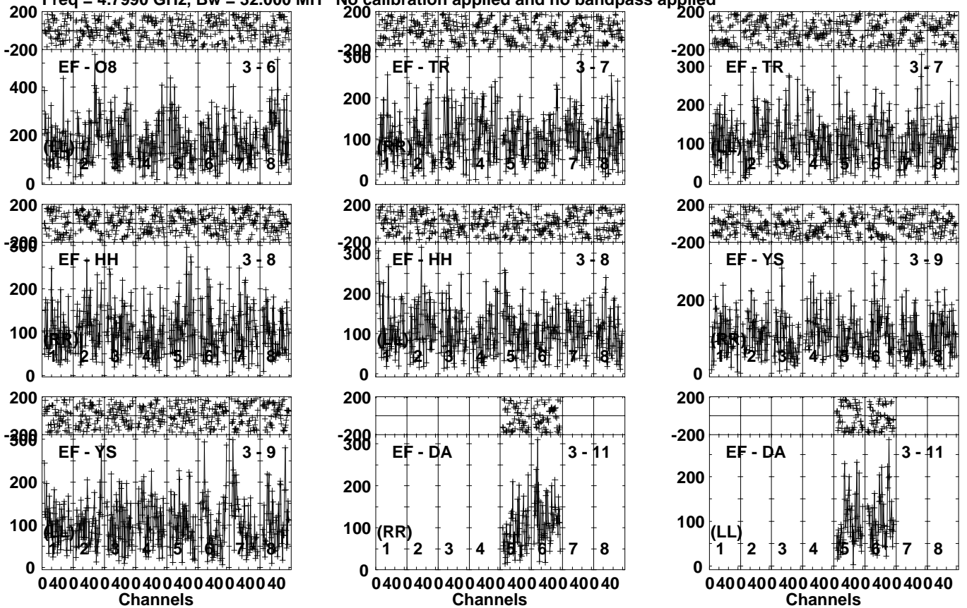
Lower frame: Micro Ampl Jy Top frame: Phas deg Vector averaged cross-power spectrum Several baselines displayed Timerange: 01/11:25:11 to 01/11:27:29
