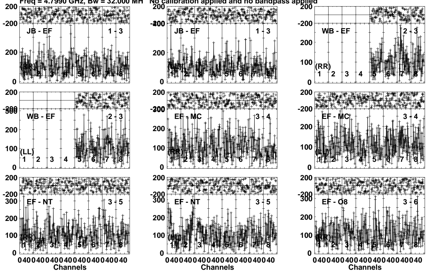
Lower frame: Micro Ampl Jy Top frame: Phas deg Vector averaged cross-power spectrum Several baselines displayed Timerange: 00/14:08:01 to 00/14:10:19
