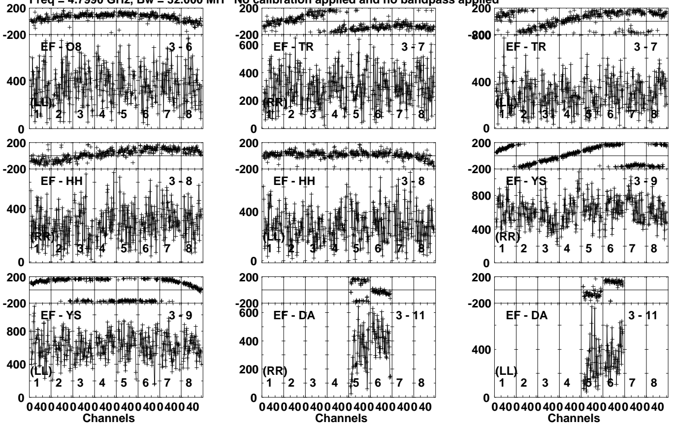
Lower frame: Micro Ampl Jy Top frame: Phas deg Vector averaged cross-power spectrum Several baselines displayed Timerange: 00/13:52:31 to 00/13:53:29
