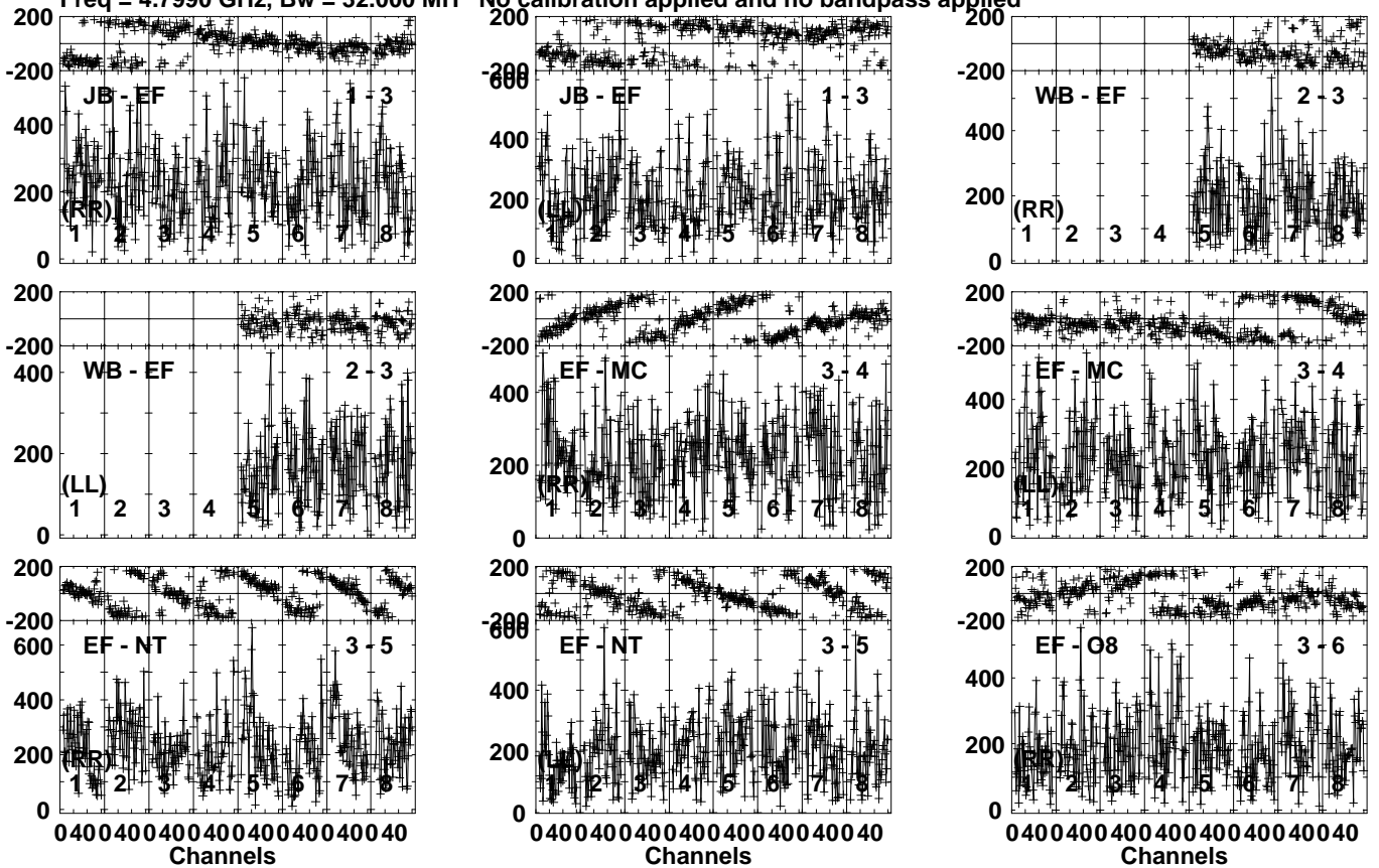
Lower frame: Micro Ampl Jy Top frame: Phas deg Vector averaged cross-power spectrum Several baselines displayed Timerange: 00/15:58:51 to 00/16:00:39
