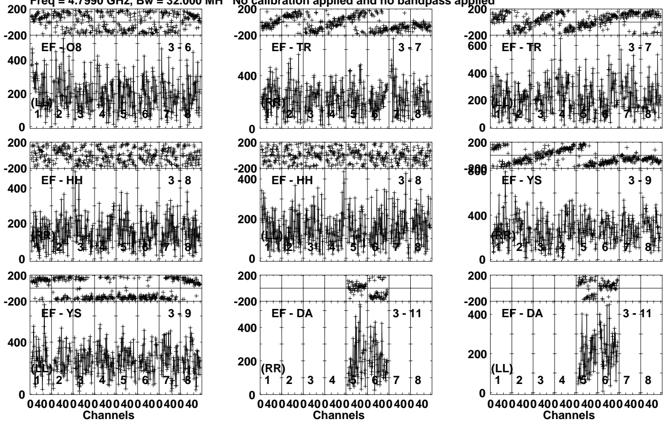
Lower frame: Micro Ampl Jy Top frame: Phas deg Vector averaged cross-power spectrum Several baselines displayed Timerange: 00/16:34:11 to 00/16:35:59
