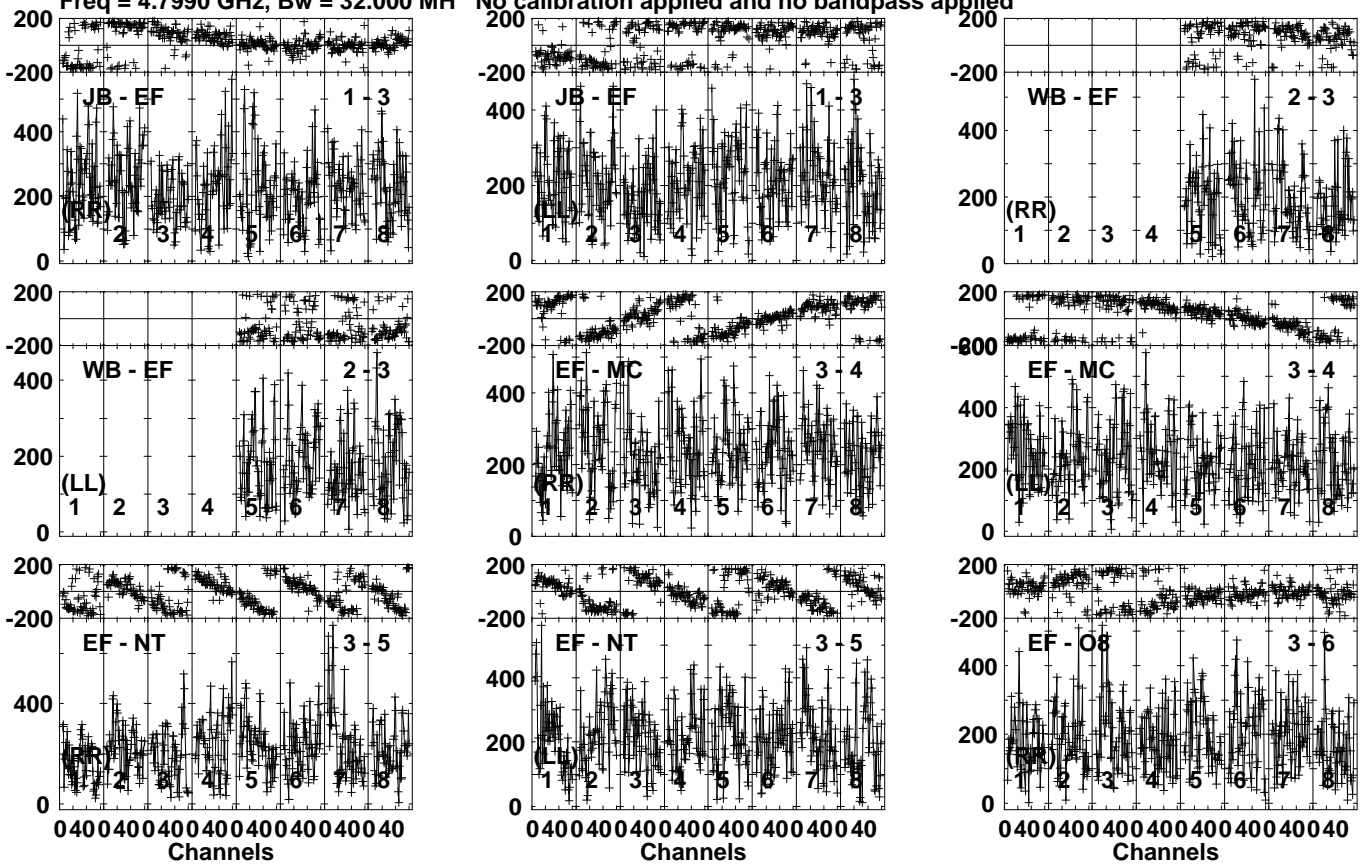
Lower frame: Micro Ampl Jy Top frame: Phas deg Vector averaged cross-power spectrum Several baselines displayed Timerange: 00/13:24:21 to 00/13:25:29
