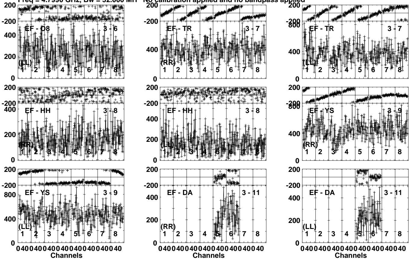
Lower frame: Micro Ampl Jy Top frame: Phas deg Vector averaged cross-power spectrum Several baselines displayed Timerange: 00/18:57:01 to 00/18:58:49
