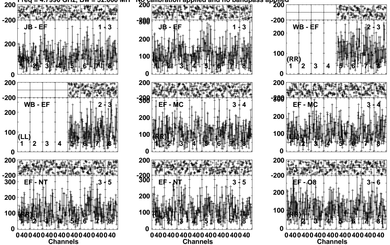
Lower frame: Micro Ampl Jy Top frame: Phas deg Vector averaged cross-power spectrum Several baselines displayed Timerange: 00/19:38:21 to 00/19:40:39
