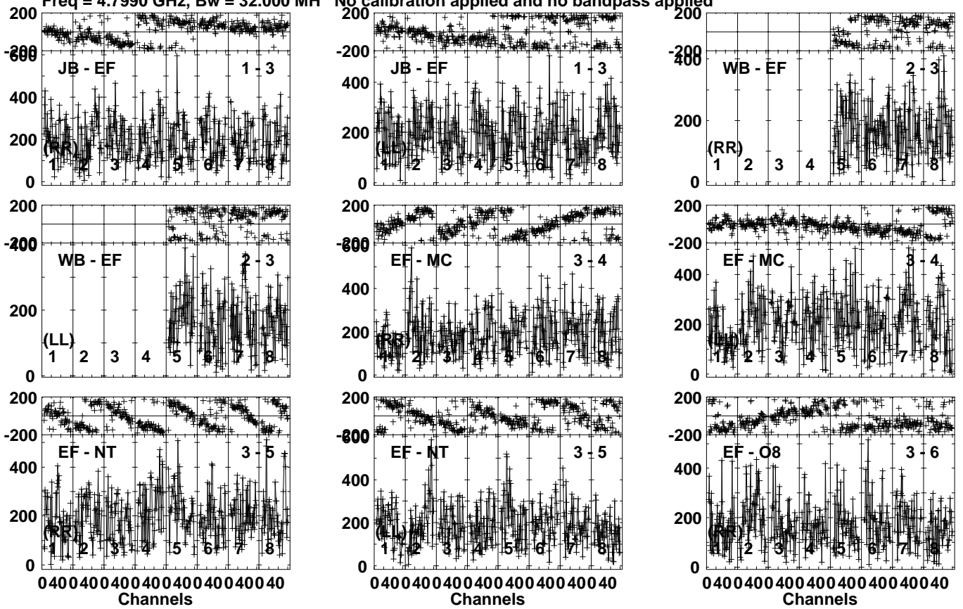
Lower frame: Micro Ampl Jy Top frame: Phas deg Vector averaged cross-power spectrum Several baselines displayed Timerange: 00/19:10:31 to 00/19:12:19
