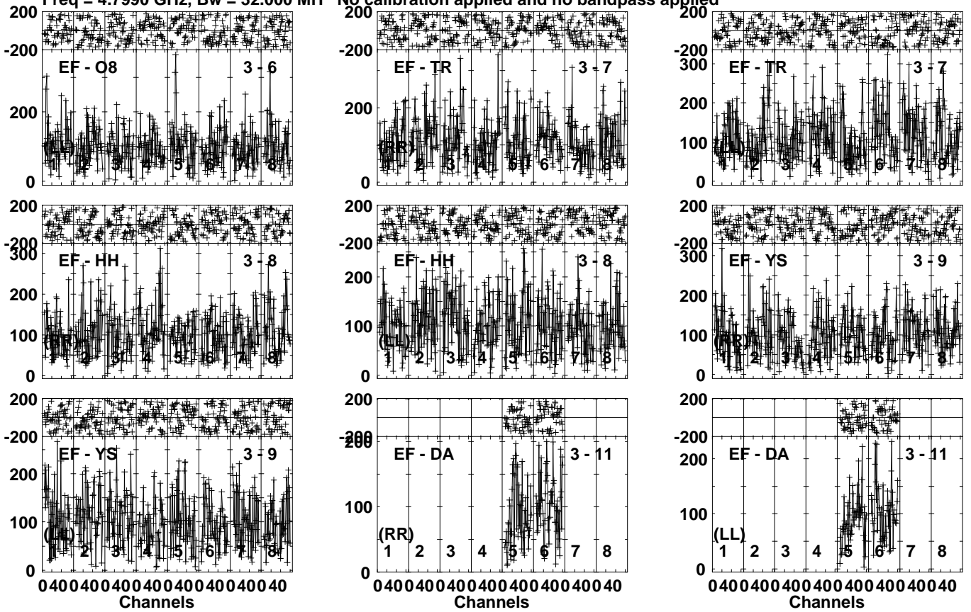
Lower frame: Micro Ampl Jy Top frame: Phas deg Vector averaged cross-power spectrum Several baselines displayed Timerange: 00/18:38:31 to 00/18:40:49
