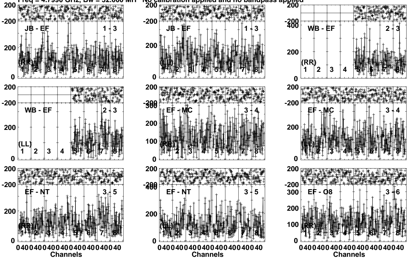
Lower frame: Micro Ampl Jy Top frame: Phas deg Vector averaged cross-power spectrum Several baselines displayed Timerange: 00/14:39:51 to 00/14:42:09
