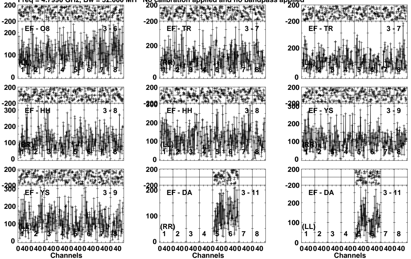
Lower frame: Micro Ampl Jy Top frame: Phas deg Vector averaged cross-power spectrum Several baselines displayed Timerange: 00/13:57:01 to 00/13:59:19
