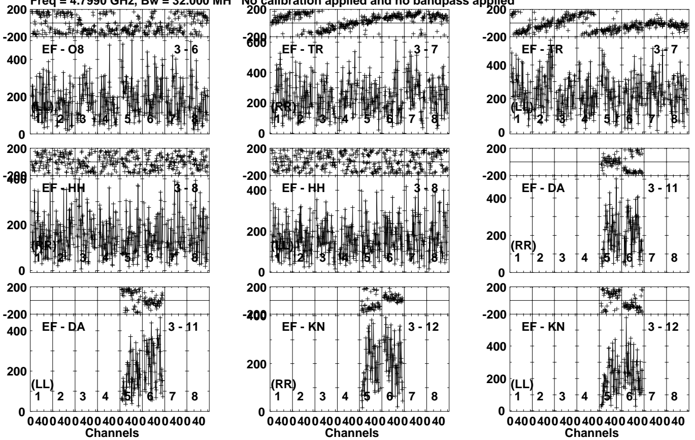
Lower frame: Micro Ampl Jy Top frame: Phas deg Vector averaged cross-power spectrum Several baselines displayed Timerange: 00/14:36:21 to 00/14:38:09
