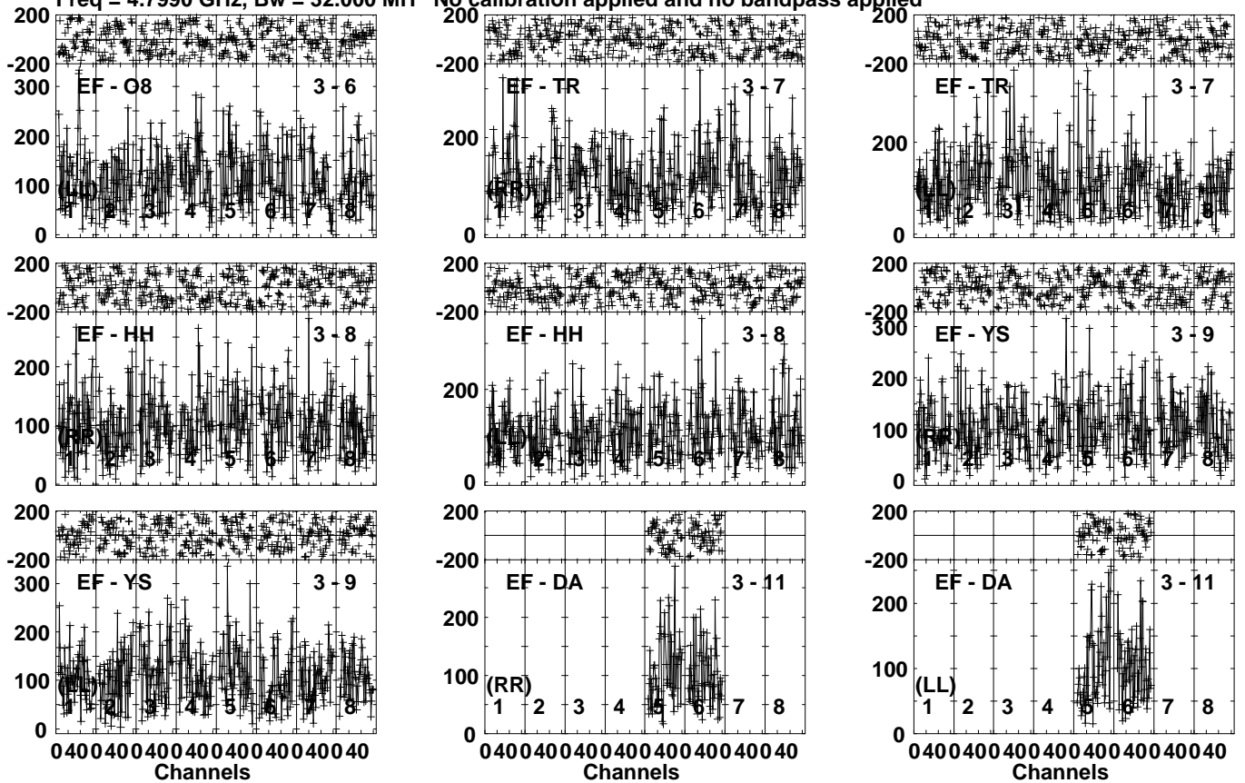
Lower frame: Micro Ampl Jy Top frame: Phas deg Vector averaged cross-power spectrum Several baselines displayed Timerange: 01/12:01:11 to 01/12:03:29
