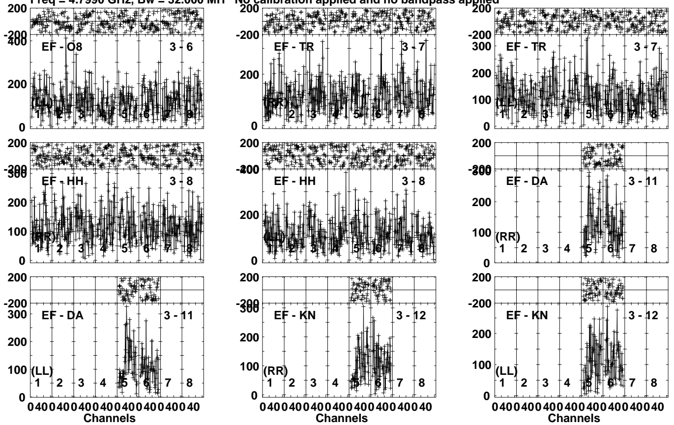
Lower frame: Micro Ampl Jy Top frame: Phas deg Vector averaged cross-power spectrum Several baselines displayed Timerange: 00/14:32:21 to 00/14:34:39
