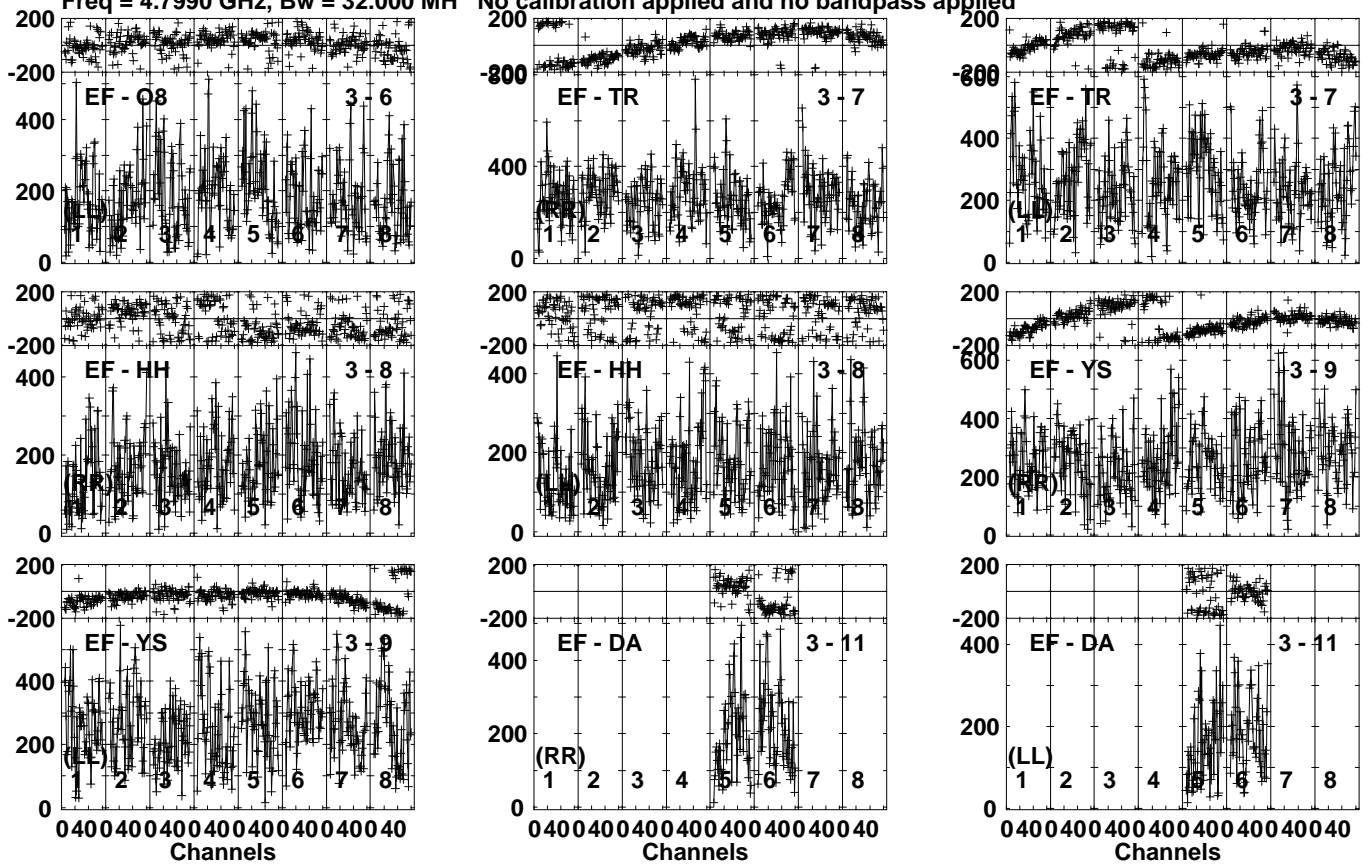
Lower frame: Micro Ampl Jy Top frame: Phas deg Vector averaged cross-power spectrum Several baselines displayed Timerange: 00/13:16:51 to 00/13:17:59
