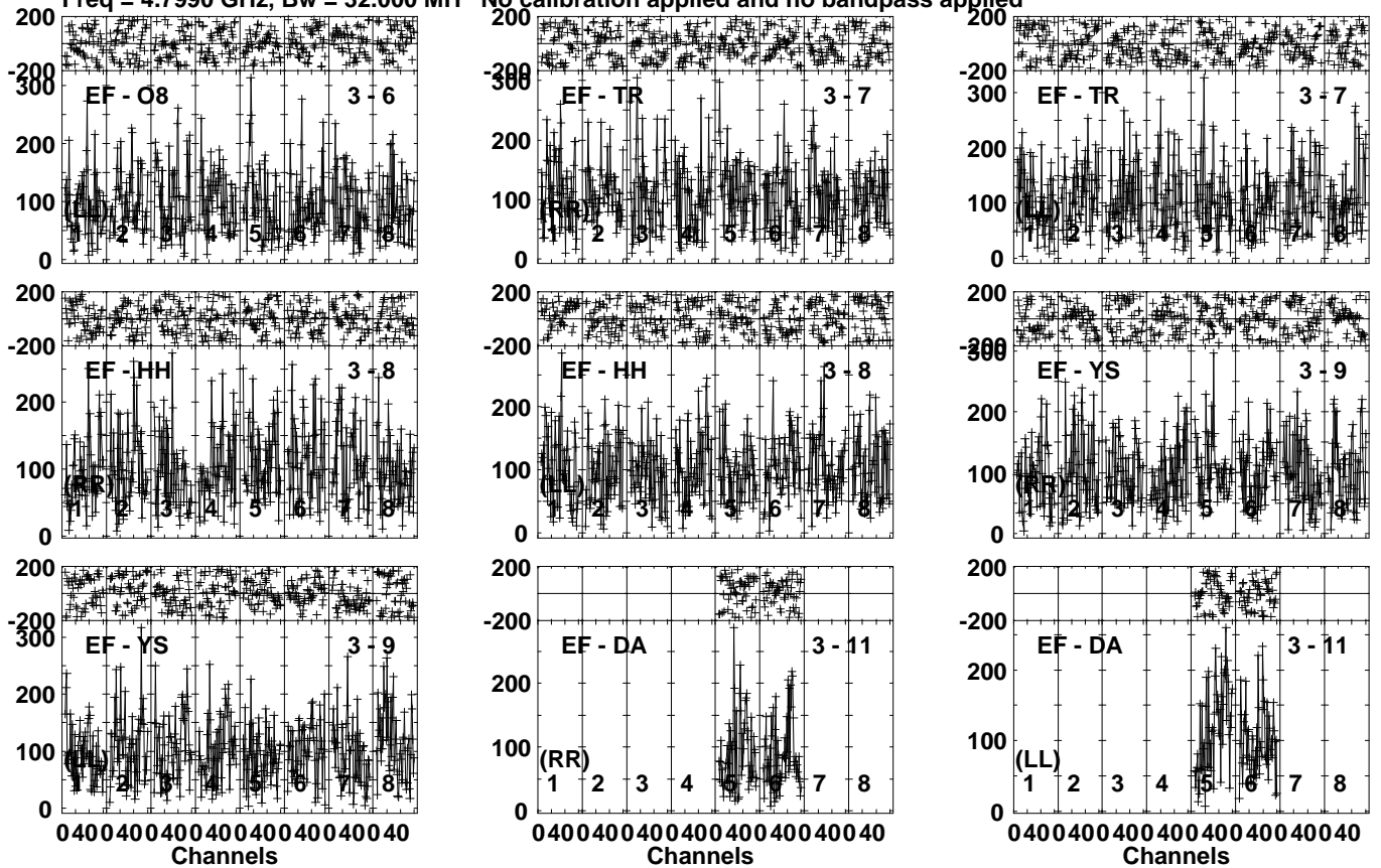
Lower frame: Micro Ampl Jy Top frame: Phas deg Vector averaged cross-power spectrum Several baselines displayed Timerange: 00/16:51:41 to 00/16:53:59
