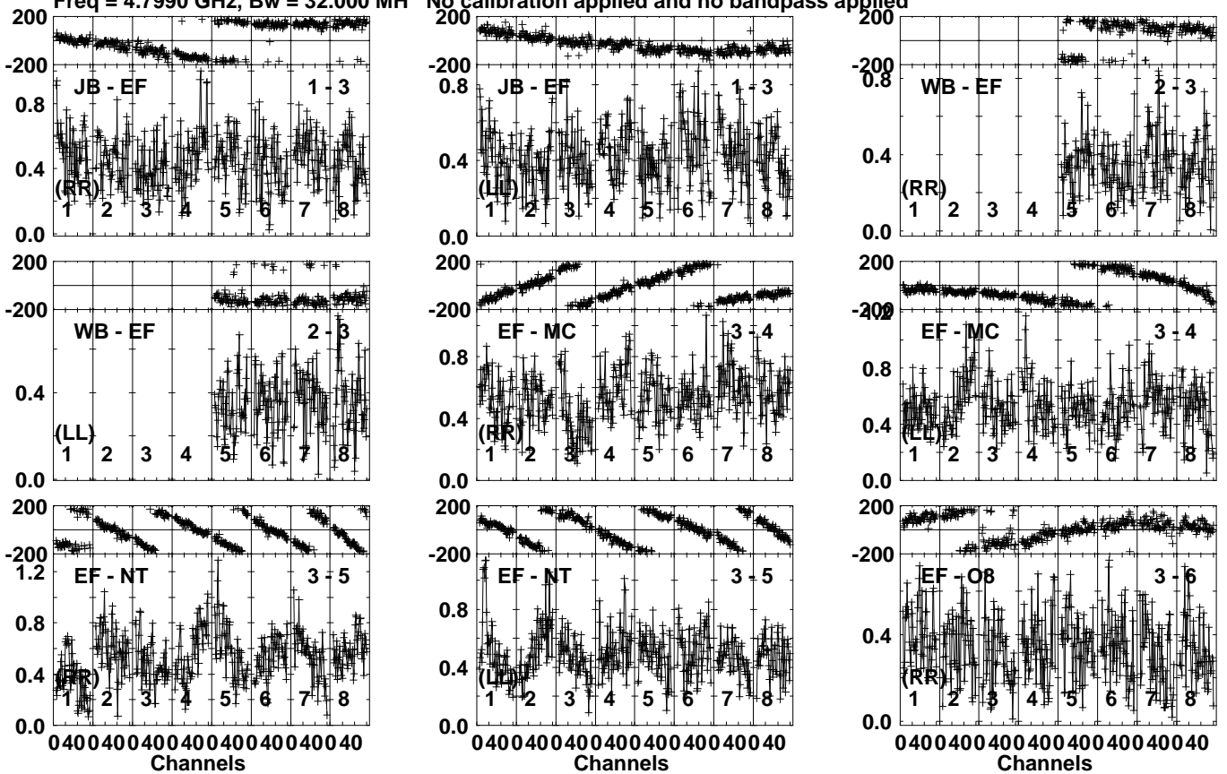
Lower frame: Milli Ampl Jy Top frame: Phas deg Vector averaged cross-power spectrum Several baselines displayed Timerange: 00/13:55:51 to 00/13:56:59
