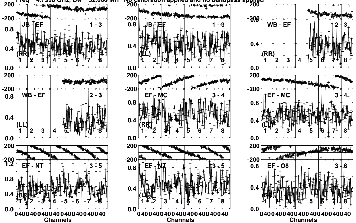
Lower frame: Milli Ampl Jy Top frame: Phas deg Vector averaged cross-power spectrum Several baselines displayed Timerange: 00/14:06:51 to 00/14:07:59
