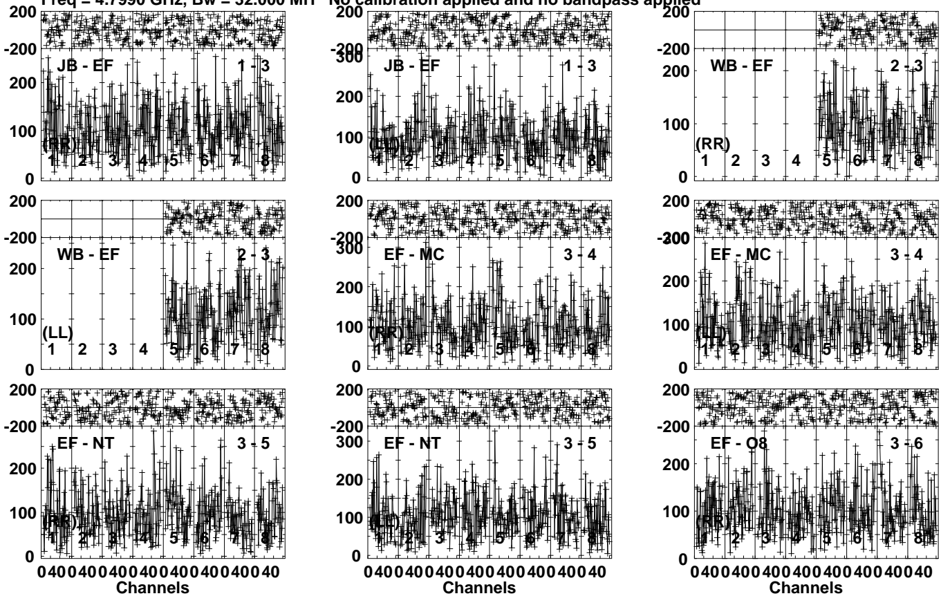
Lower frame: Micro Ampl Jy Top frame: Phas deg Vector averaged cross-power spectrum Several baselines displayed Timerange: 00/15:15:51 to 00/15:18:09
