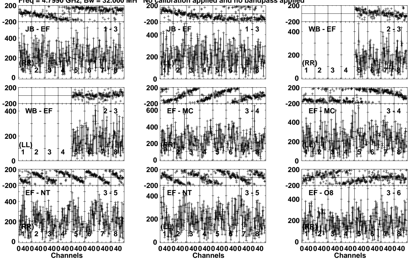
Lower frame: Micro Ampl Jy Top frame: Phas deg Vector averaged cross-power spectrum Several baselines displayed Timerange: 00/17:45:41 to 00/17:47:29
