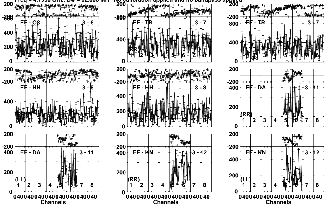
Lower frame: Micro Ampl Jy Top frame: Phas deg Vector averaged cross-power spectrum Several baselines displayed Timerange: 00/14:56:11 to 00/14:57:19
