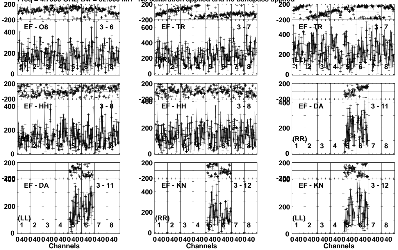
Lower frame: Micro Ampl Jy Top frame: Phas deg Vector averaged cross-power spectrum Several baselines displayed Timerange: 00/14:12:01 to 00/14:13:49
