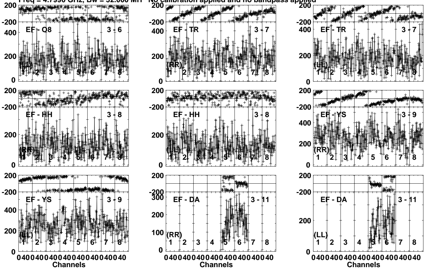
Lower frame: Micro Ampl Jy Top frame: Phas deg Vector averaged cross-power spectrum Several baselines displayed Timerange: 00/18:36:31 to 00/18:38:29
