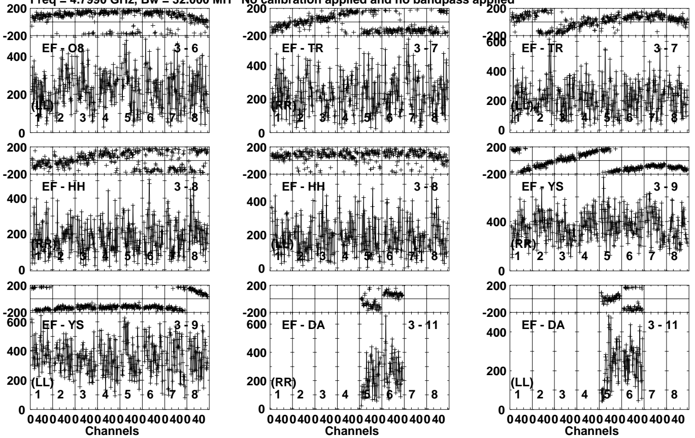
Lower frame: Micro Ampl Jy Top frame: Phas deg Vector averaged cross-power spectrum Several baselines displayed Timerange: 00/13:36:31 to 00/13:38:19
