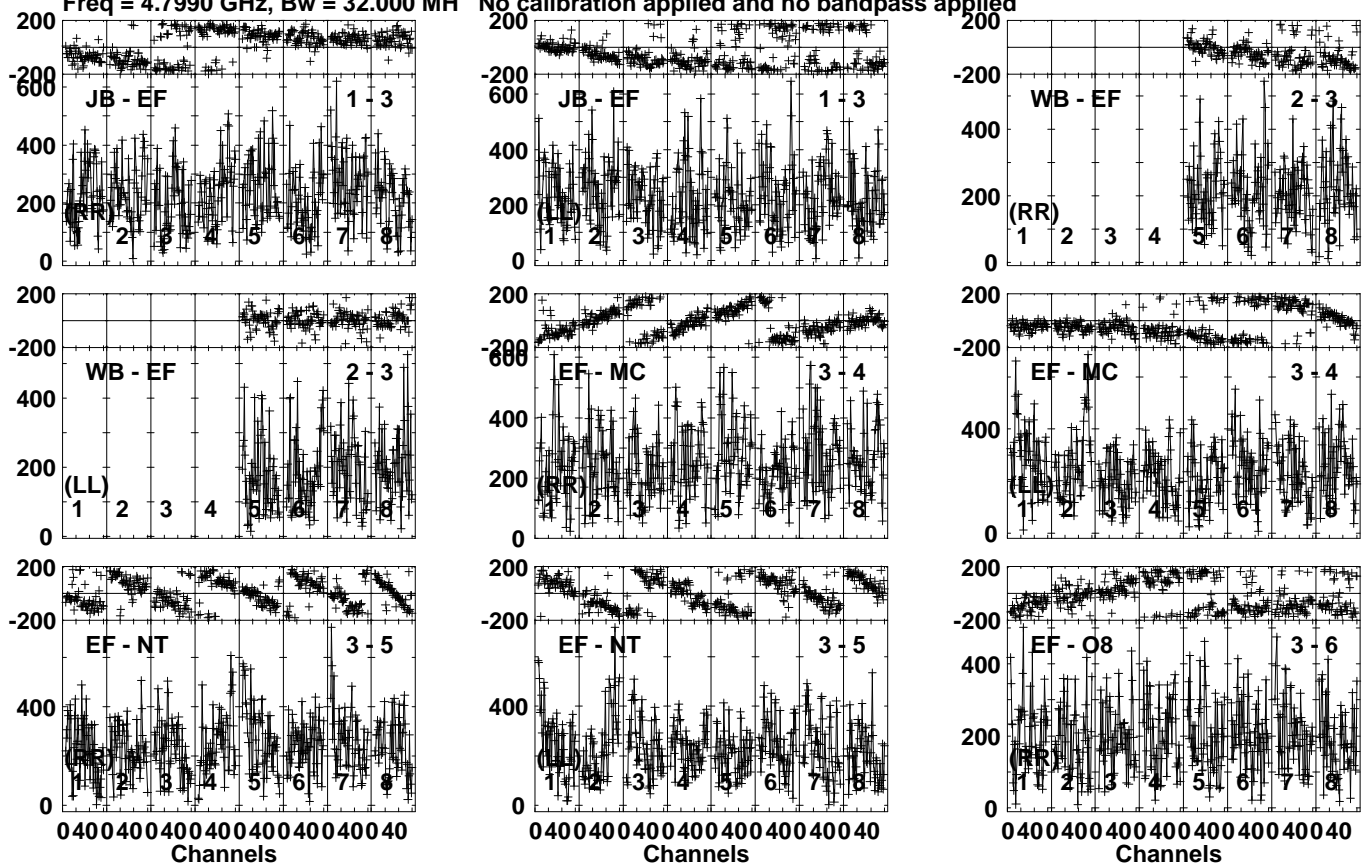
Lower frame: Micro Ampl Jy Top frame: Phas deg Vector averaged cross-power spectrum Several baselines displayed Timerange: 00/15:25:41 to 00/15:26:49
