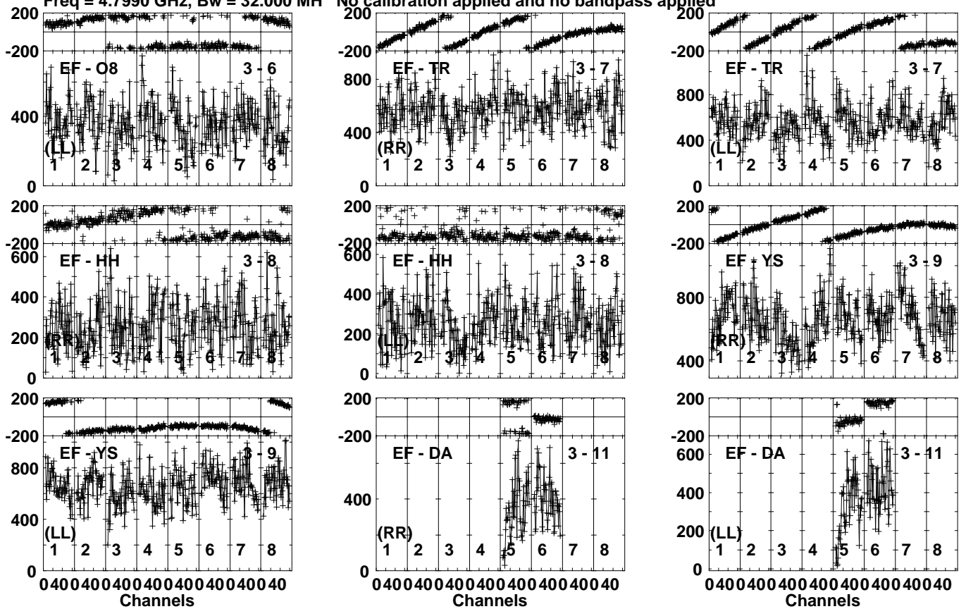
Lower frame: Micro Ampl Jy Top frame: Phas deg Vector averaged cross-power spectrum Several baselines displayed Timerange: 00:17:48:11 to 00:17:49:09
