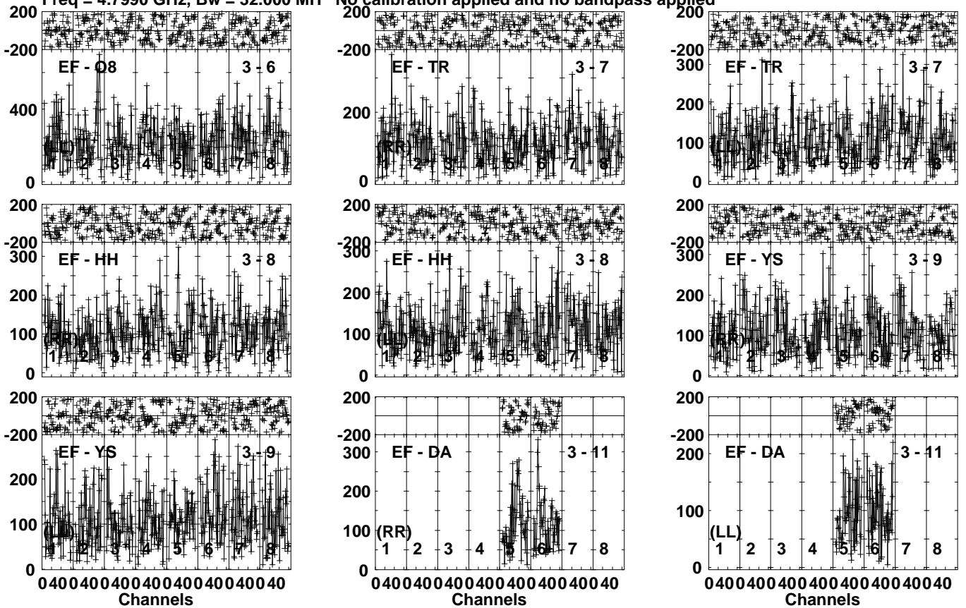
Lower frame: Micro Ampl Jy Top frame: Phas deg Vector averaged cross-power spectrum Several baselines displayed Timerange: 01/11:21:11 to 01/11:23:29
