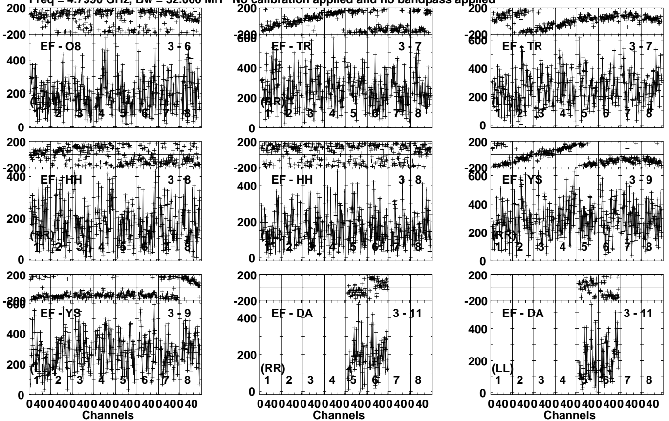
Lower frame: Micro Ampl Jy Top frame: Phas deg Vector averaged cross-power spectrum Several baselines displayed Timerange: 00/13:38:51 to 00/13:39:59
