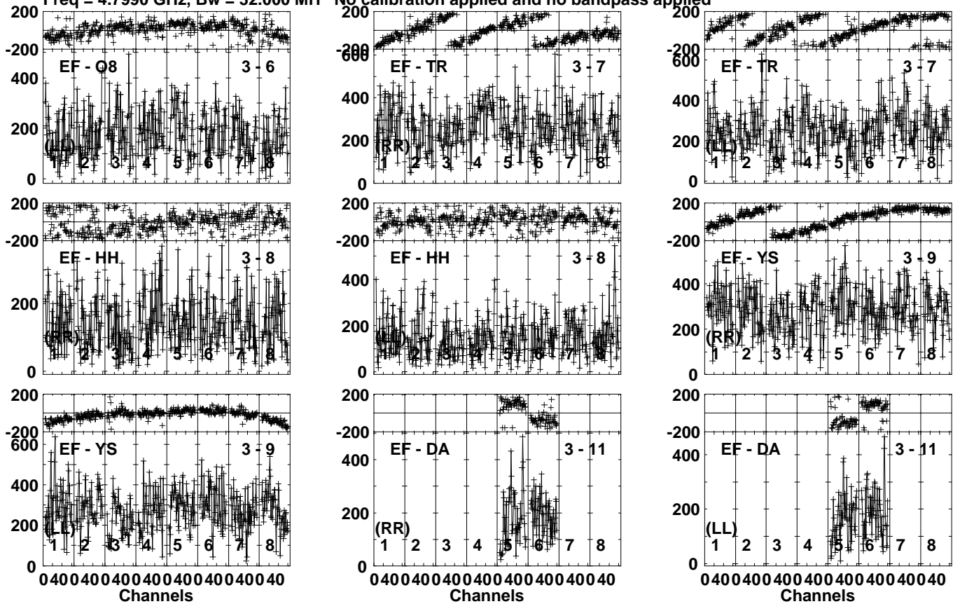
Lower frame: Micro Ampl Jy Top frame: Phas deg Vector averaged cross-power spectrum Several baselines displayed Timerange: 00/17:20:01 to 00/17:21:09
