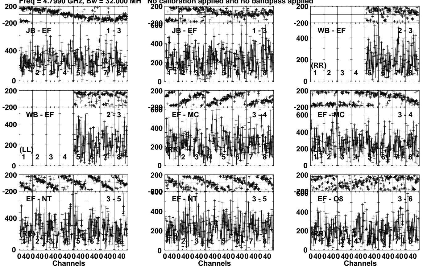
Lower frame: Micro Ampl Jy Top frame: Phas deg Vector averaged cross-power spectrum Several baselines displayed Timerange: 00/17:12:31 to 00/17:13:39
