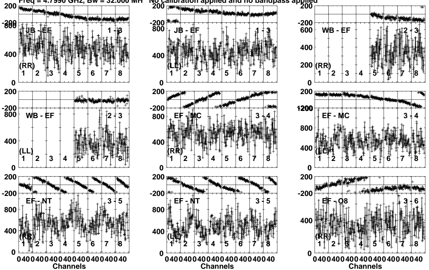
Lower frame: Micro Ampl Jy Top frame: Phas deg Vector averaged cross-power spectrum Several baselines displayed Timerange: 00:15:39:21 to 00:15:40:19
