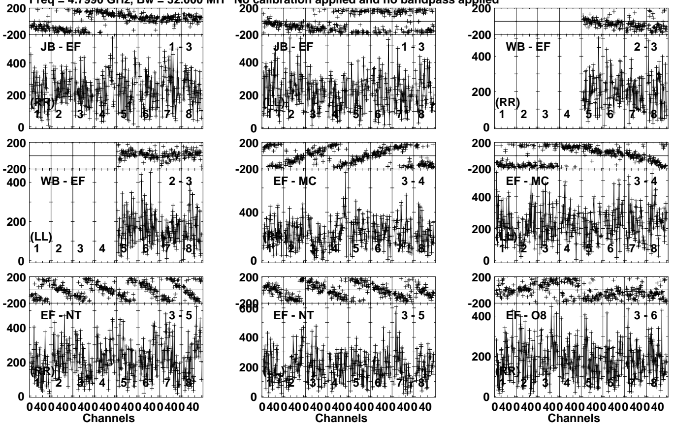
Lower frame: Micro Ampl Jy Top frame: Phas deg Vector averaged cross-power spectrum Several baselines displayed Timerange: 00/14:47:21 to 00/14:49:09
