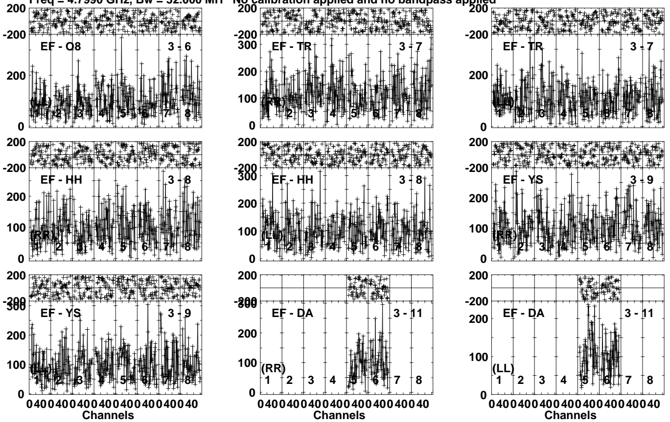
Lower frame: Micro Ampl Jy Top frame: Phas deg Vector averaged cross-power spectrum Several baselines displayed Timerange: 00/13:10:31 to 00/13:12:49
