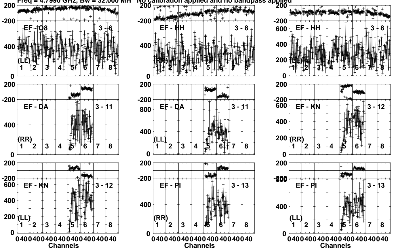
Lower frame: Micro Ampl Jy Top frame: Phas deg Vector averaged cross-power spectrum Several baselines displayed Timerange: 00:16:01:21 to 00:16:02:19
