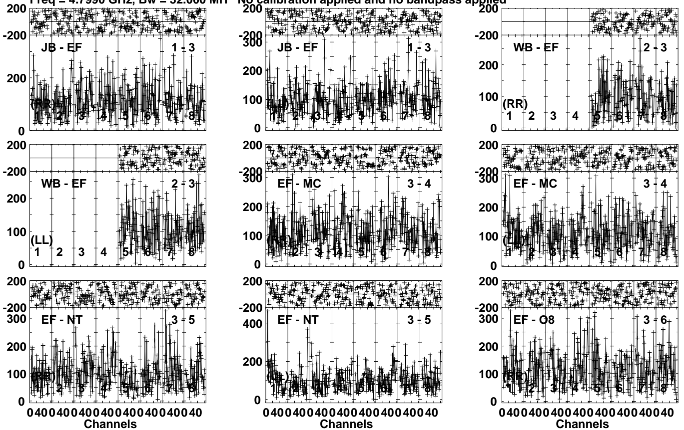
Lower frame: Micro Ampl Jy Top frame: Phas deg Vector averaged cross-power spectrum Several baselines displayed Timerange: 01/12:44:41 to 01/12:46:59
