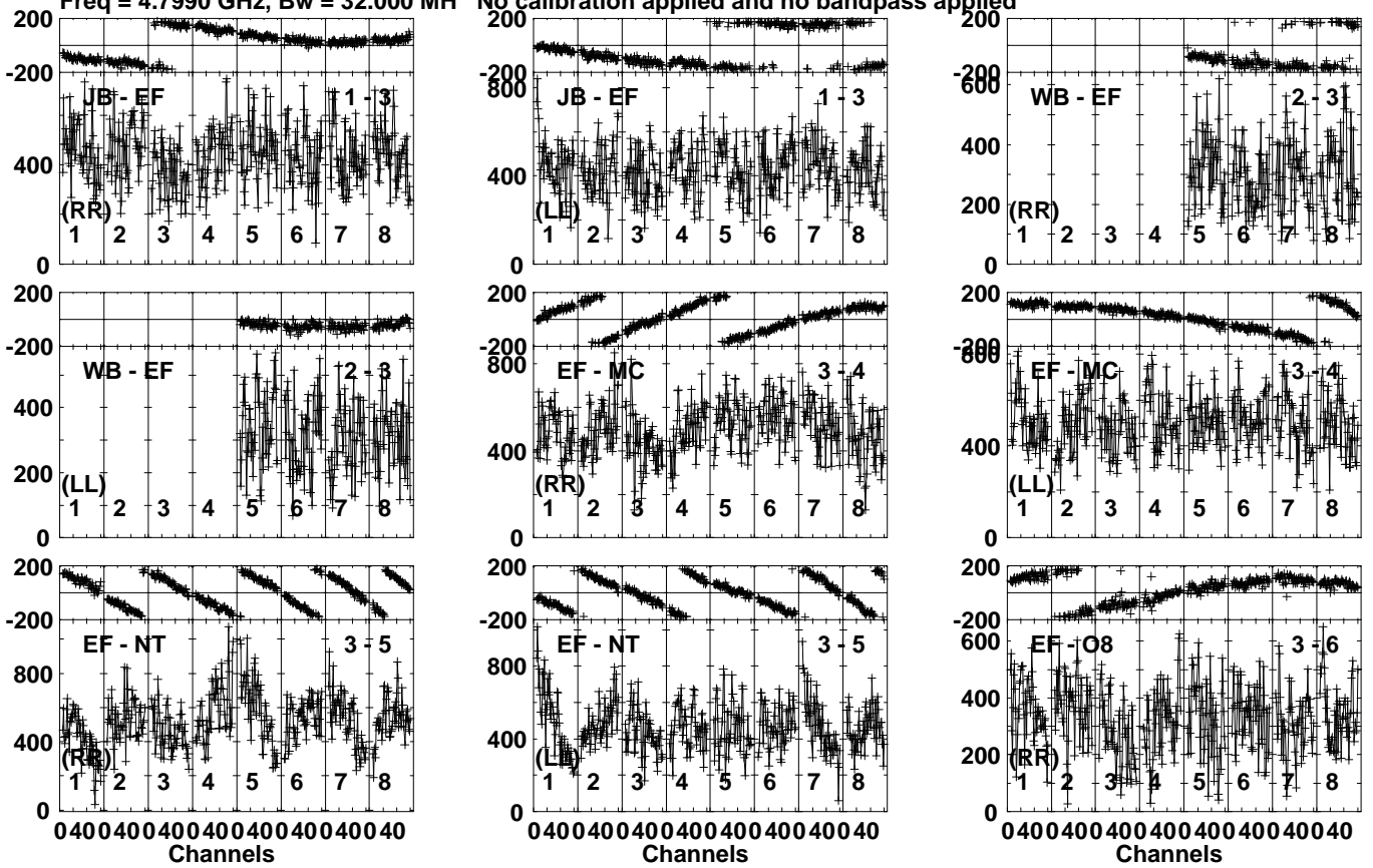
Lower frame: Micro Ampl Jy Top frame: Phas deg Vector averaged cross-power spectrum Several baselines displayed Timerange: 00/14:11:01 to 00/14:11:59
