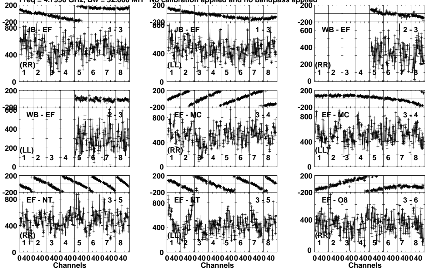
Lower frame: Micro Ampl Jy Top frame: Phas deg Vector averaged cross-power spectrum Several baselines displayed Timerange: 00/18:20:01 to 00/18:20:59
