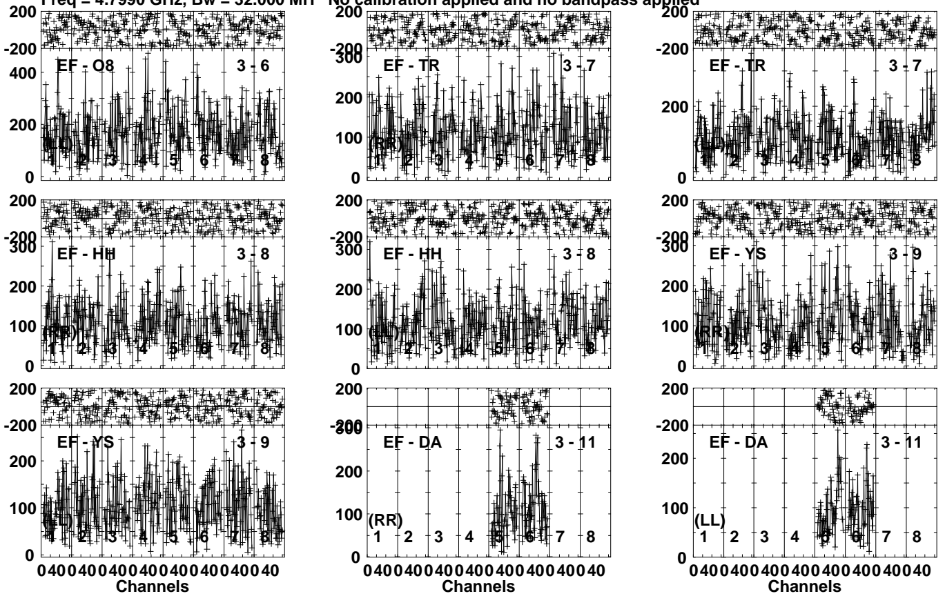
Lower frame: Micro Ampl Jy Top frame: Phas deg Vector averaged cross-power spectrum Several baselines displayed Timerange: 01/11:32:11 to 01/11:34:29
