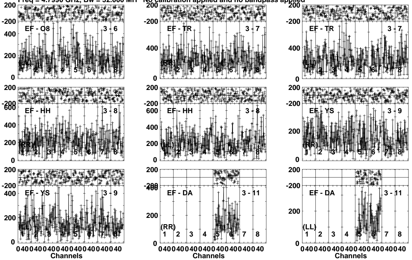
Lower frame: Micro Ampl Jy Top frame: Phas deg Vector averaged cross-power spectrum Several baselines displayed Timerange: 01/11:05:31 to 01/11:06:39
