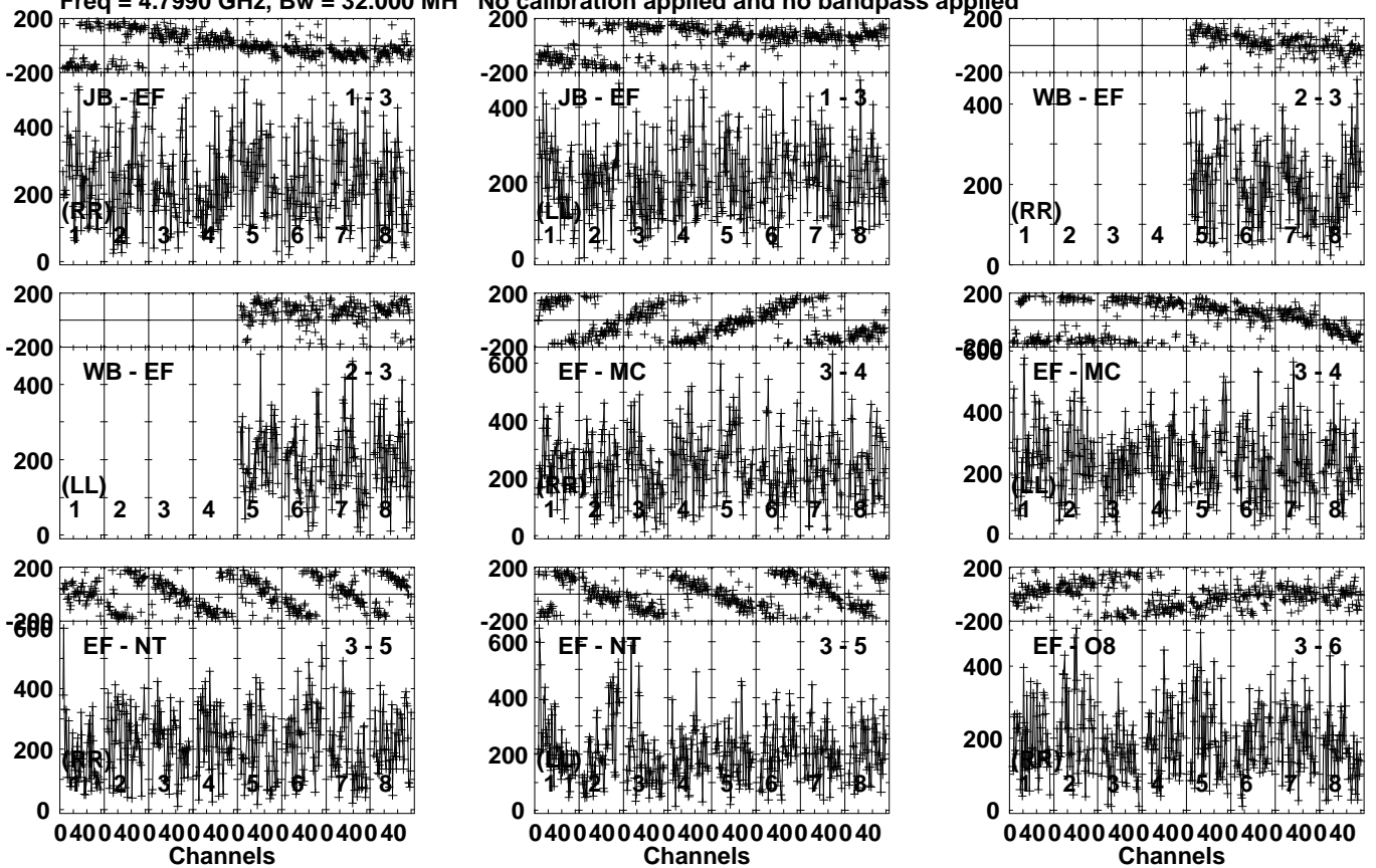
Lower frame: Micro Ampl Jy Top frame: Phas deg Vector averaged cross-power spectrum Several baselines displayed Timerange: 00/16:12:11 to 00/16:13:59
