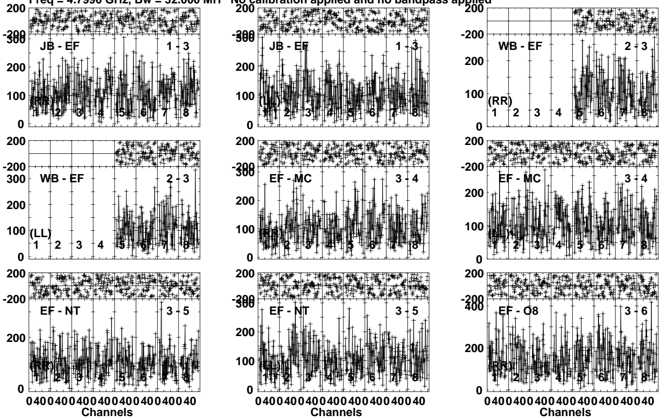
Lower frame: Micro Ampl Jy Top frame: Phas deg Vector averaged cross-power spectrum Several baselines displayed Timerange: 01/12:04:41 to 01/12:06:59
