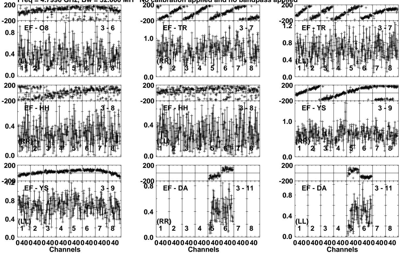
Lower frame: Milli Ampl Jy Top frame: Phas deg Vector averaged cross-power spectrum Several baselines displayed Timerange: 00/19:29:41 to 00/19:30:49
