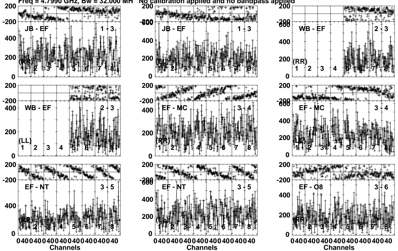
Lower frame: Micro Ampl Jy Top frame: Phas deg Vector averaged cross-power spectrum Several baselines displayed Timerange: 00/15:47:51 to 00/15:49:39
