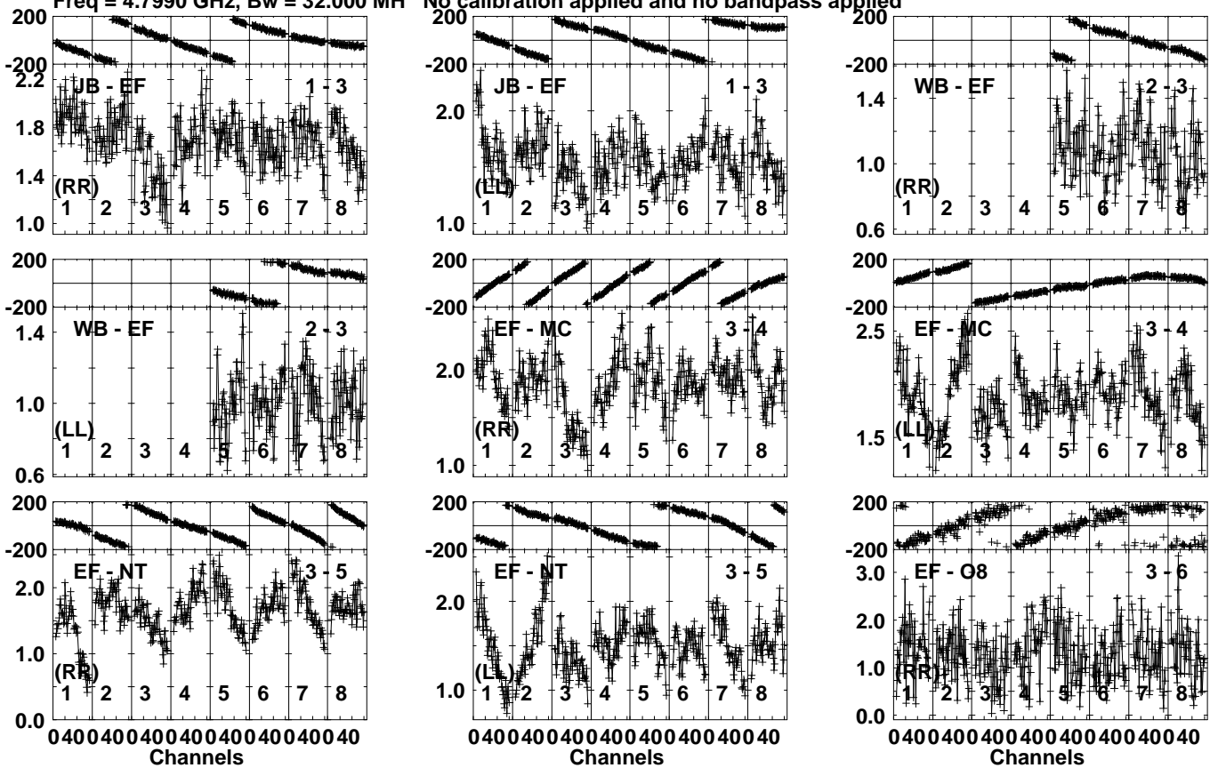
Lower frame: Milli Ampl Jy Top frame: Phas deg Vector averaged cross-power spectrum Several baselines displayed Timerange: 01/12:18:01 to 01/12:19:09
