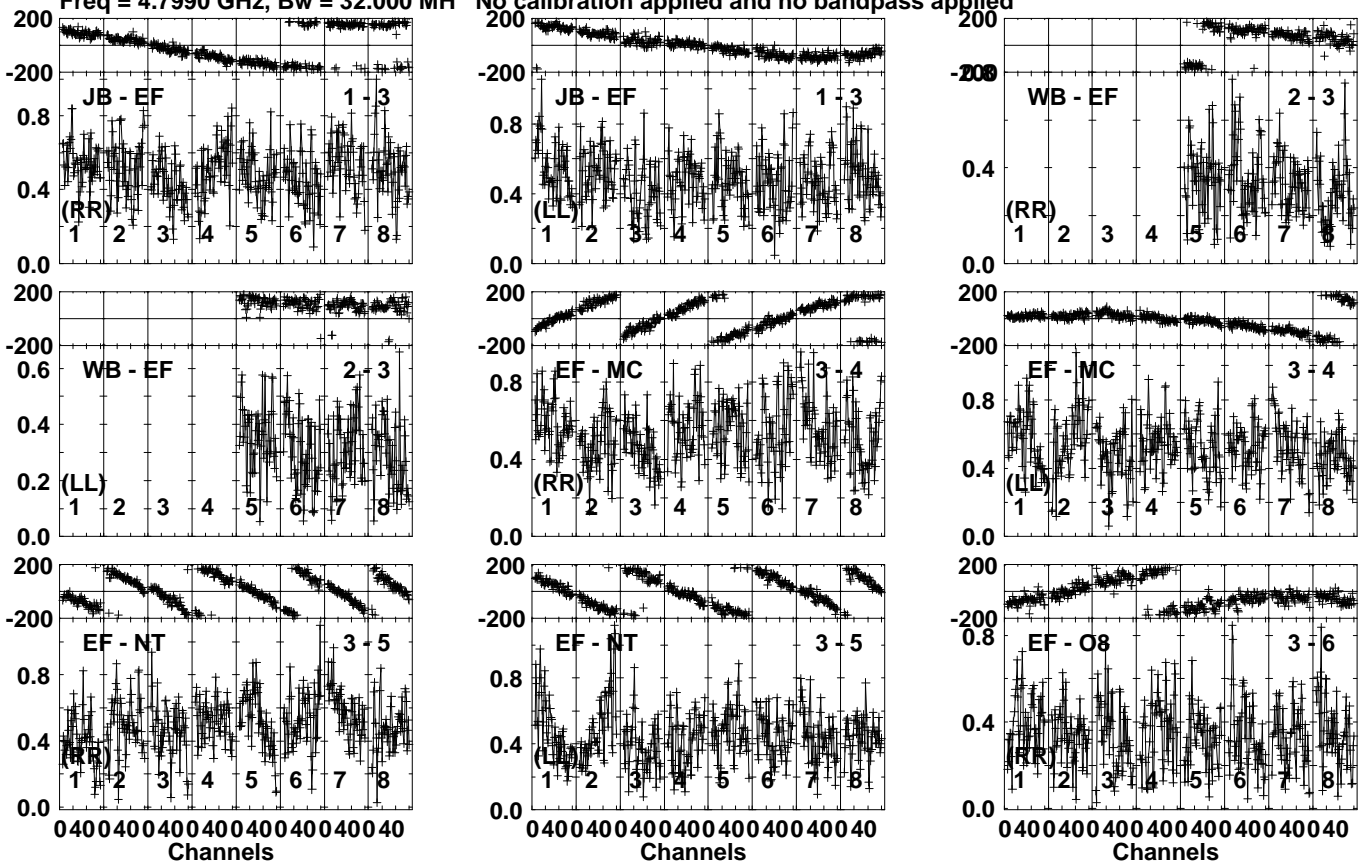
Lower frame: Milli Ampl Jy Top frame: Phas deg Vector averaged cross-power spectrum Several baselines displayed Timerange: 00/18:12:31 to 00/18:13:29
