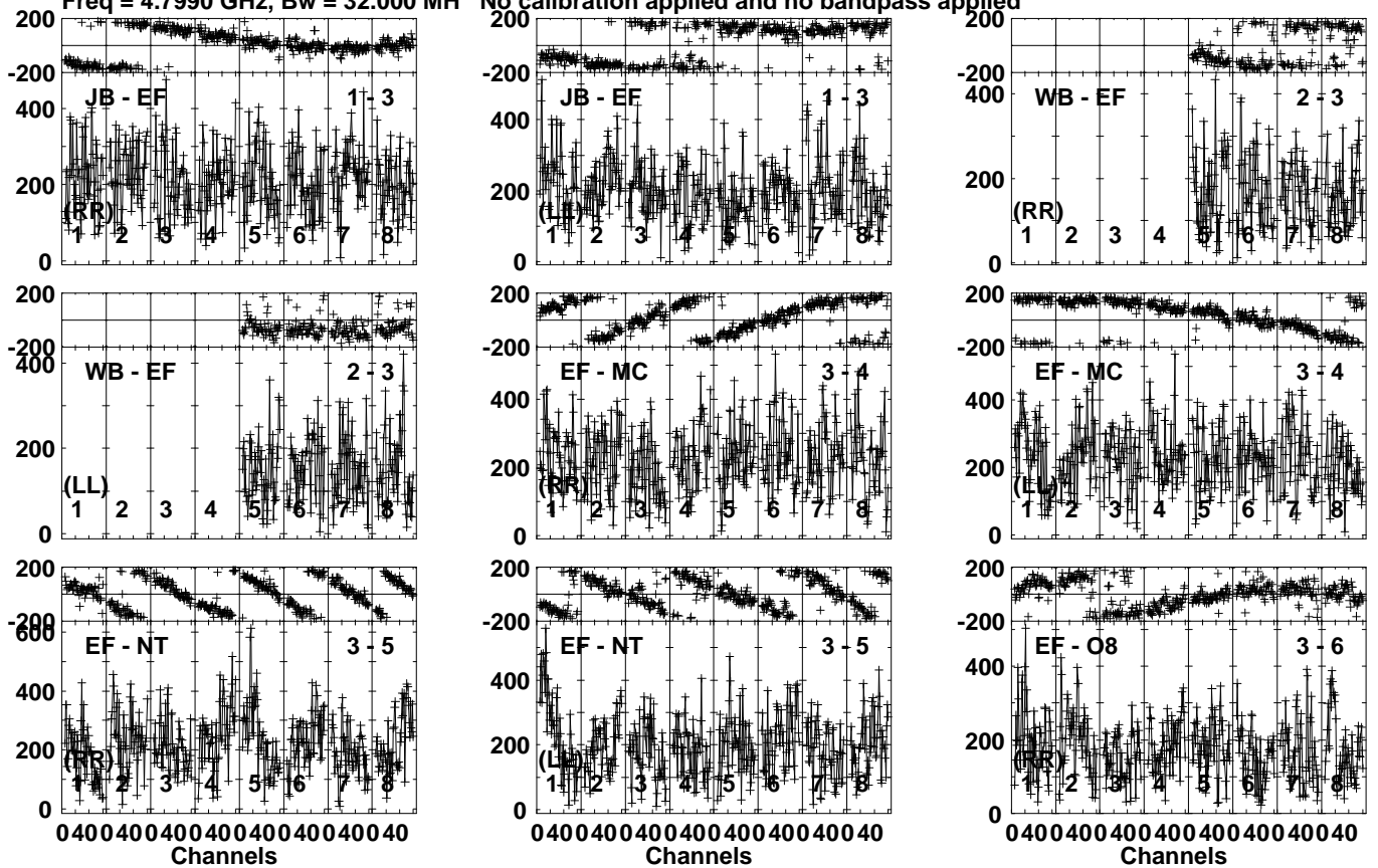
Lower frame: Micro Ampl Jy Top frame: Phas deg Vector averaged cross-power spectrum Several baselines displayed Timerange: 00/14:51:51 to 00/14:53:49
