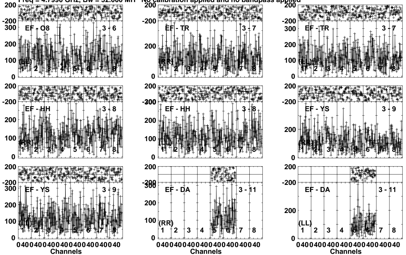
Lower frame: Micro Ampl Jy Top frame: Phas deg Vector averaged cross-power spectrum Several baselines displayed Timerange: 00/18:02:31 to 00/18:04:49
