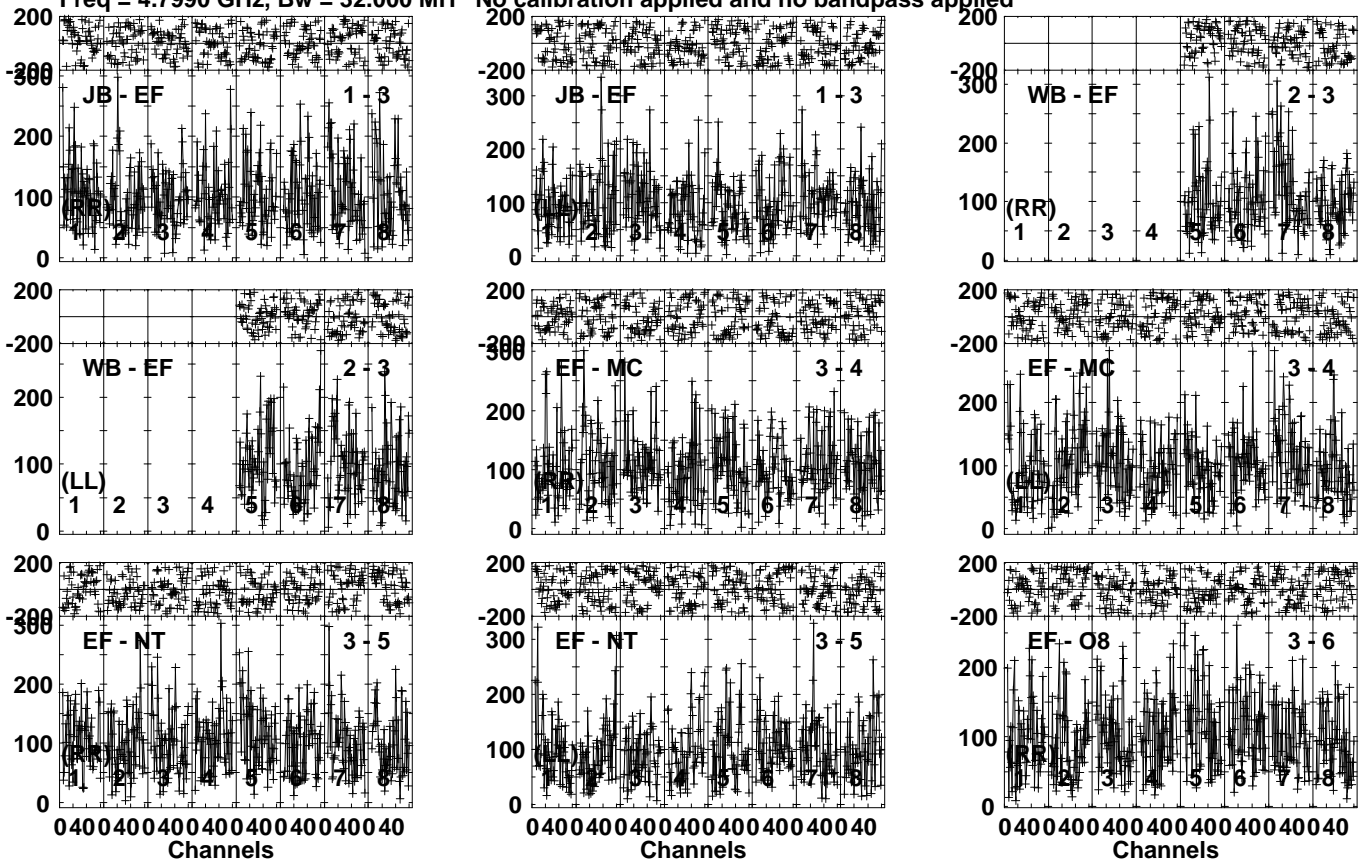
Lower frame: Micro Ampl Jy Top frame: Phas deg Vector averaged cross-power spectrum Several baselines displayed Timerange: 00/13:21:31 to 00/13:23:49
