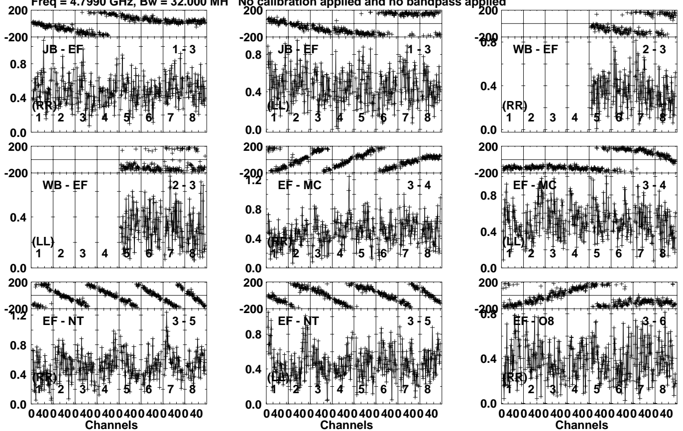
Lower frame: Milli Ampl Jy Top frame: Phas deg Vector averaged cross-power spectrum Several baselines displayed Timerange: 00/19:05:21 to 00/19:06:29
