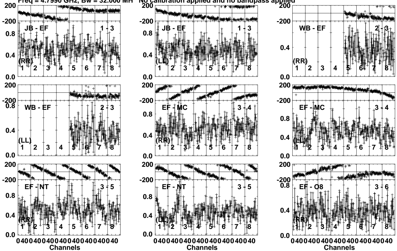
Lower frame: Milli Ampl Jy Top frame: Phas deg Vector averaged cross-power spectrum Several baselines displayed Timerange: 00/18:23:31 to 00/18:24:29
