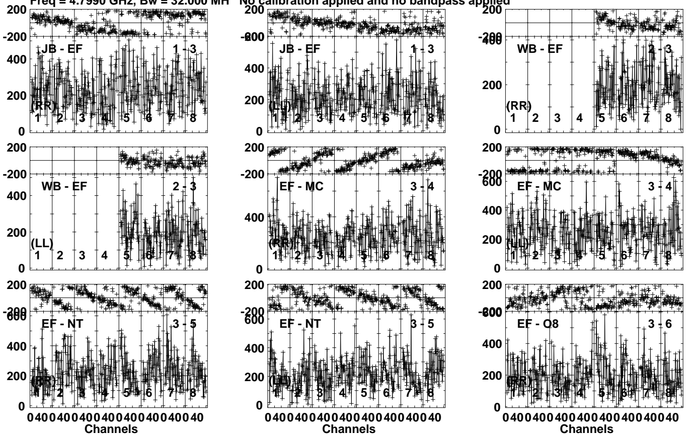
Lower frame: Micro Ampl Jy Top frame: Phas deg Vector averaged cross-power spectrum Several baselines displayed Timerange: 00/18:21:01 to 00/18:22:49
