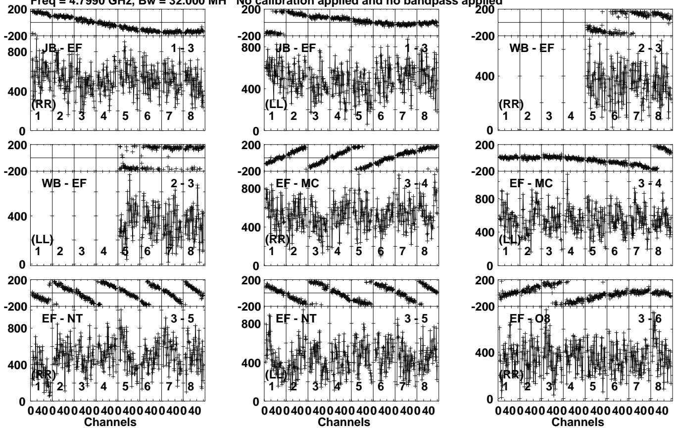
Lower frame: Micro Ampl Jy Top frame: Phas deg Vector averaged cross-power spectrum Several baselines displayed Timerange: 00/18:09:01 to 00/18:09:59
