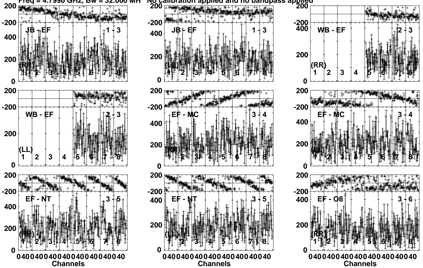
Lower frame: Micro Ampl Jy Top frame: Phas deg Vector averaged cross-power spectrum Several baselines displayed Timerange: 00/13:50:01 to 00/13:51:49
