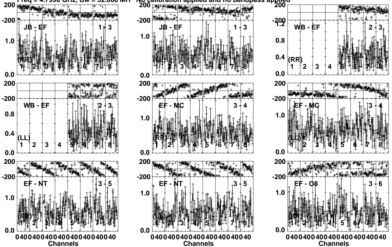
Lower frame: Milli Ampl Jy Top frame: Phas deg Vector averaged cross-power spectrum Several baselines displayed Timerange: 00/14:20:11 to 00/14:21:19
