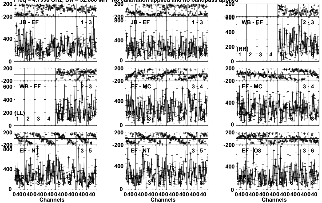
Lower frame: Micro Ampl Jy Top frame: Phas deg Vector averaged cross-power spectrum Several baselines displayed Timerange: 00/13:09:21 to 00/13:10:29
