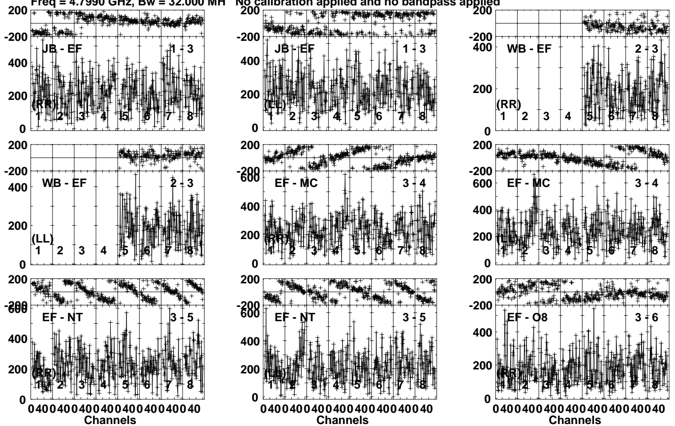
Lower frame: Micro Ampl Jy Top frame: Phas deg Vector averaged cross-power spectrum Several baselines displayed Timerange: 00/13:13:21 to 00/13:14:29
