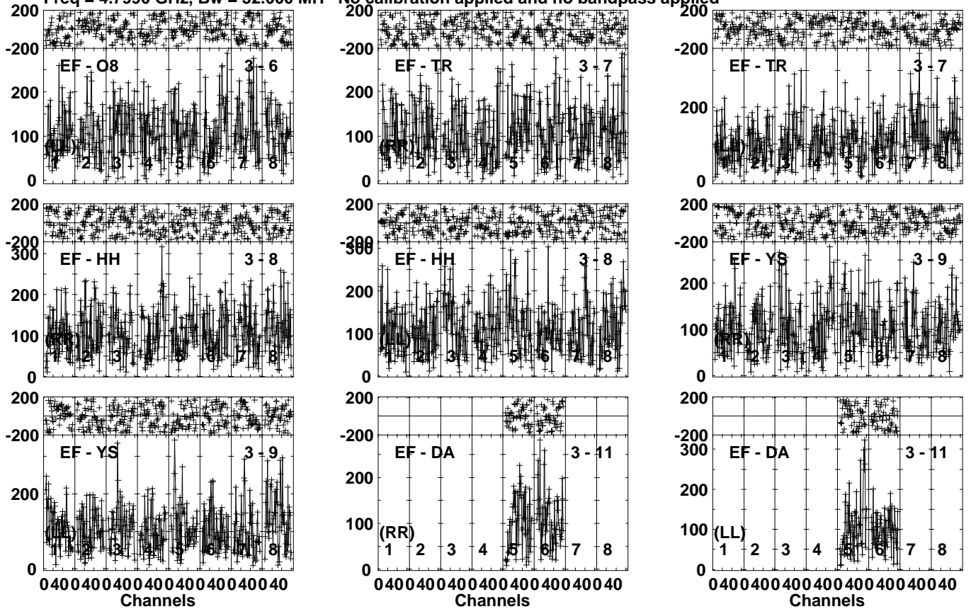
Lower frame: Micro Ampl Jy Top frame: Phas deg Vector averaged cross-power spectrum Several baselines displayed Timerange: 00/13:53:31 to 00/13:55:49
