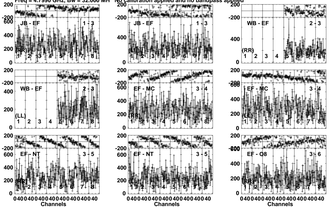
Lower frame: Micro Ampl Jy Top frame: Phas deg Vector averaged cross-power spectrum Several baselines displayed Timerange: 00/17:01:31 to 00/17:02:39
