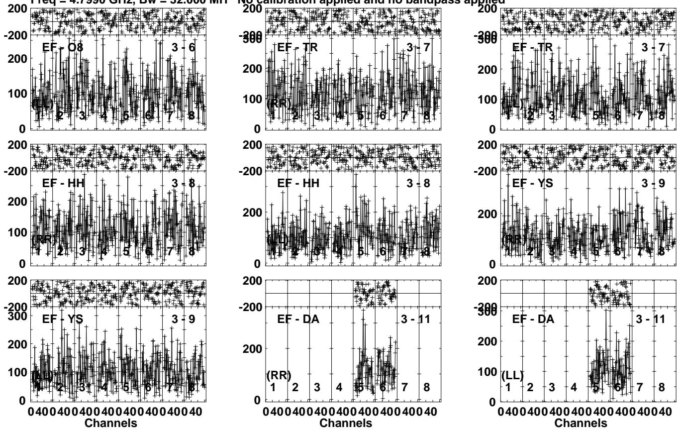
Lower frame: Micro Ampl Jy Top frame: Phas deg Vector averaged cross-power spectrum Several baselines displayed Timerange: 01/12:37:41 to 01/12:39:59
