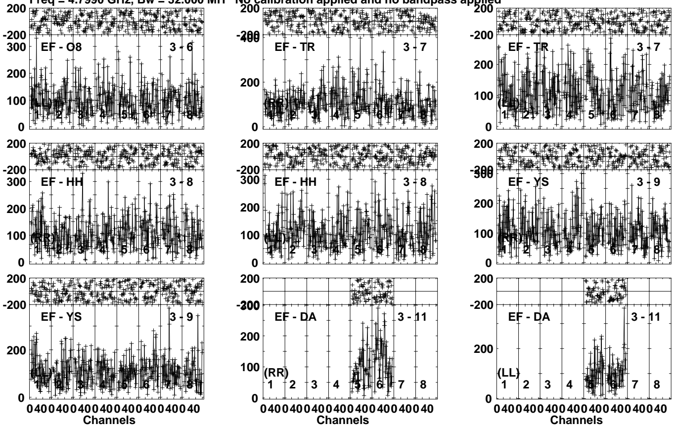
Lower frame: Micro Ampl Jy Top frame: Phas deg Vector averaged cross-power spectrum Several baselines displayed Timerange: 01/12:33:41 to 01/12:35:59
