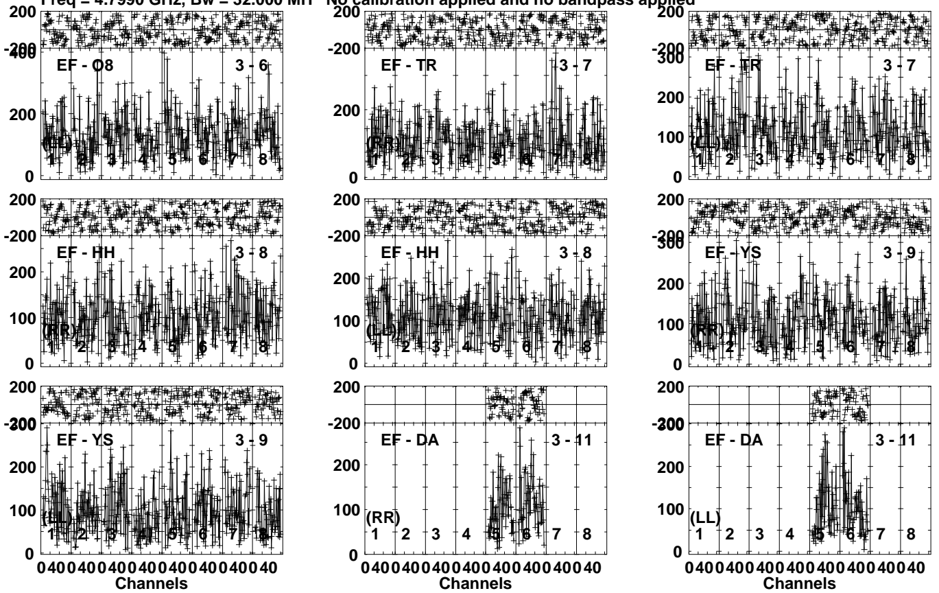
Lower frame: Micro Ampl Jy Top frame: Phas deg Vector averaged cross-power spectrum Several baselines displayed Timerange: 01/11:39:41 to 01/11:41:59
