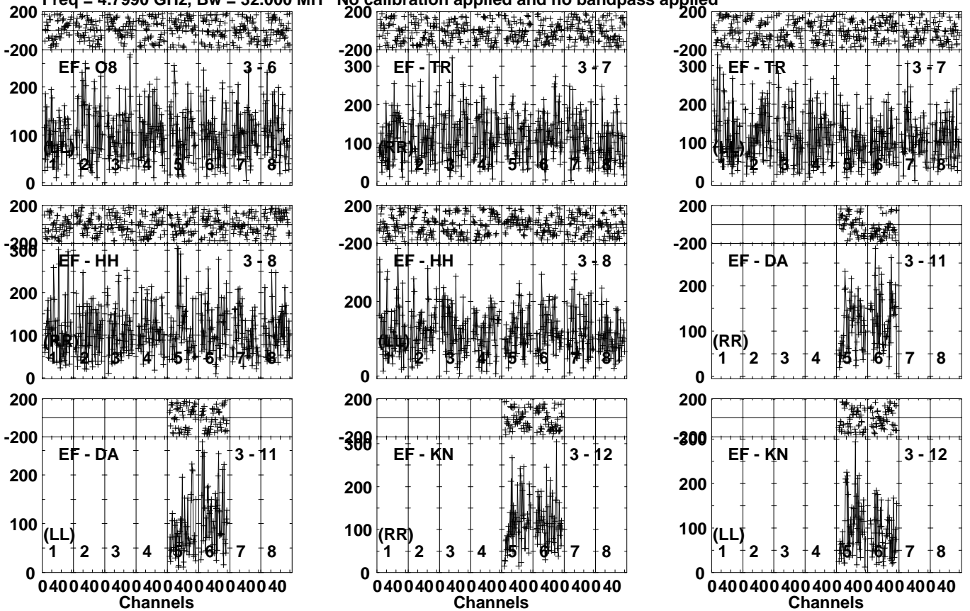
Lower frame: Micro Ampl Jy Top frame: Phas deg Vector averaged cross-power spectrum Several baselines displayed Timerange: 00/16:04:41 to 00/16:06:59
