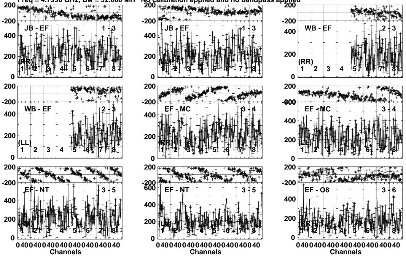
Lower frame: Micro Ampl Jy Top frame: Phas deg Vector averaged cross-power spectrum Several baselines displayed Timerange: 00/14:25:21 to 00/14:27:09
