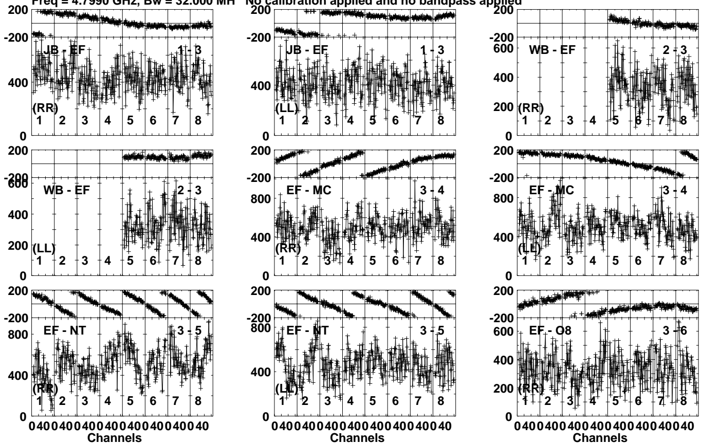
Lower frame: Micro Ampl Jy Top frame: Phas deg Vector averaged cross-power spectrum Several baselines displayed Timerange: 00/13:49:01 to 00/13:49:59
