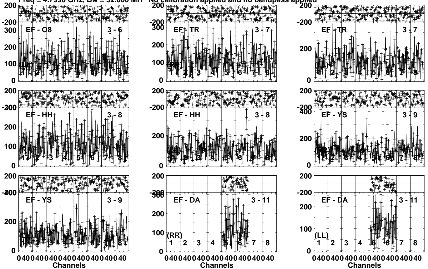
Lower frame: Micro Ampl Jy Top frame: Phas deg Vector averaged cross-power spectrum Several baselines displayed Timerange: 00/19:17:31 to 00/19:19:49
