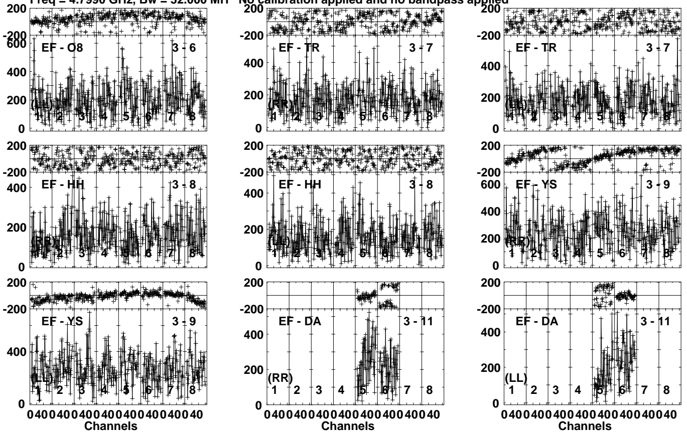
Lower frame: Micro Ampl Jy Top frame: Phas deg Vector averaged cross-power spectrum Several baselines displayed Timerange: 00/18:10:01 to 00/18:11:49
