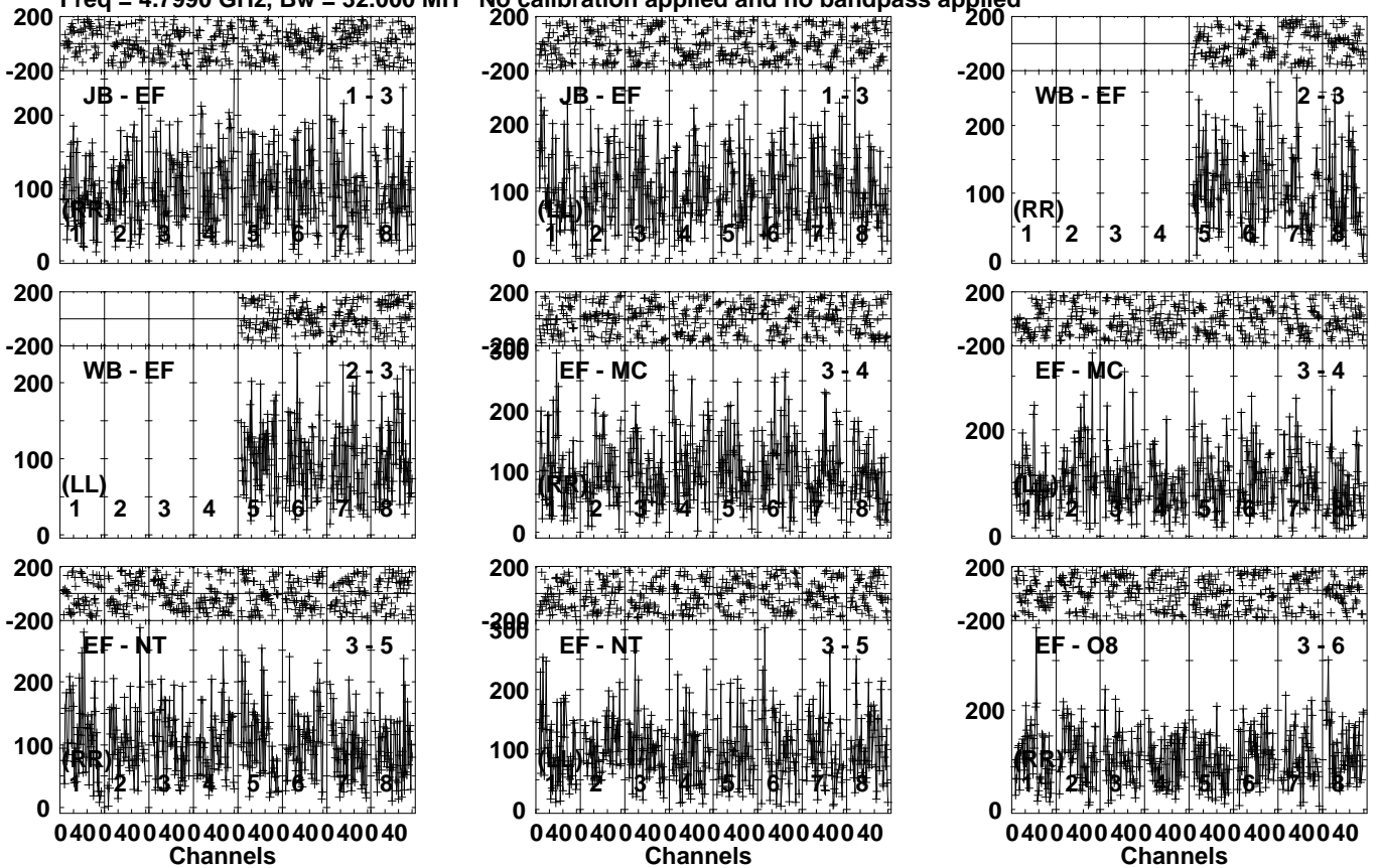
Lower frame: Micro Ampl Jy Top frame: Phas deg Vector averaged cross-power spectrum Several baselines displayed Timerange: 00/17:02:41 to 00/17:04:59
