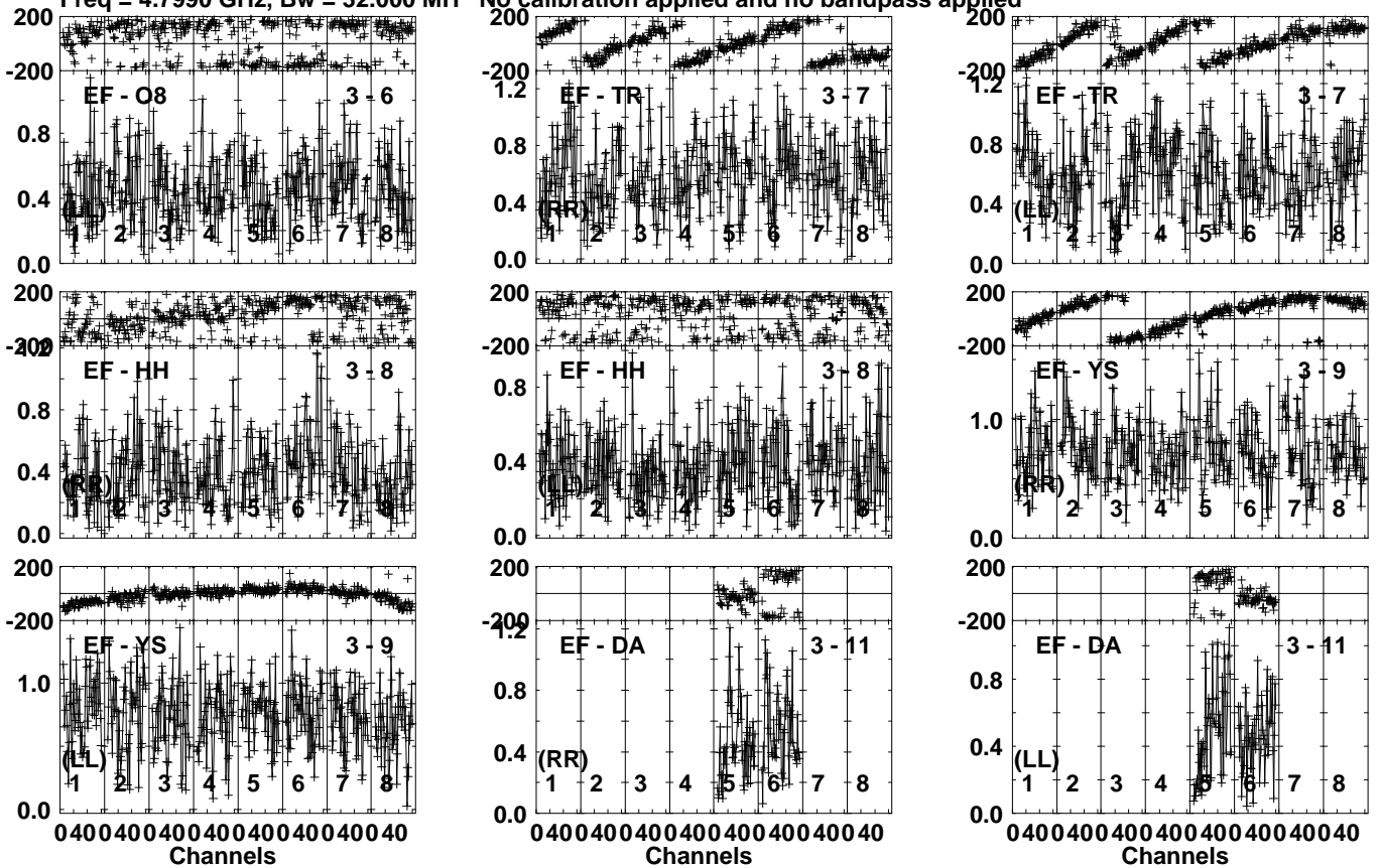
Lower frame: Milli Ampl Jy Top frame: Phas deg Vector averaged cross-power spectrum Several baselines displayed Timerange: 00/18:04:51 to 00/18:05:59
