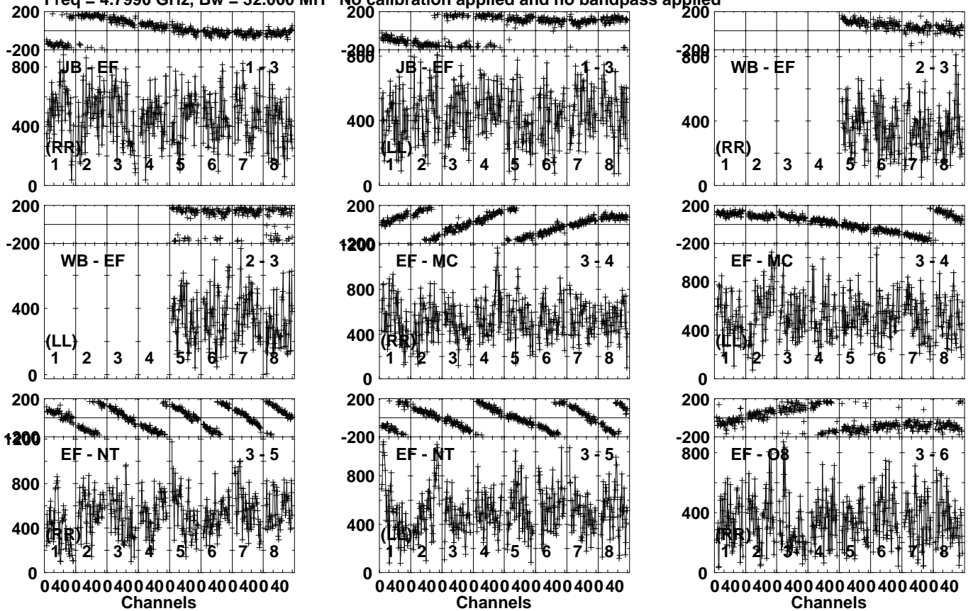
Lower frame: Micro Ampl Jy Top frame: Phas deg Vector averaged cross-power spectrum Several baselines displayed Timerange: 00/13:44:51 to 00/13:45:59
