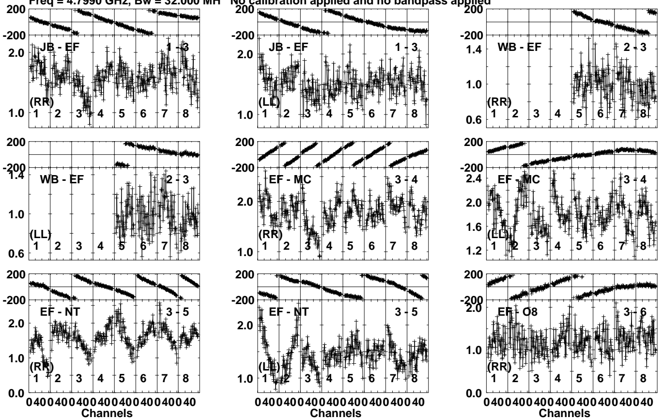
Lower frame: Milli Ampl Jy Top frame: Phas deg Vector averaged cross-power spectrum Several baselines displayed Timerange: 01/11:42:01 to 01/11:43:09
