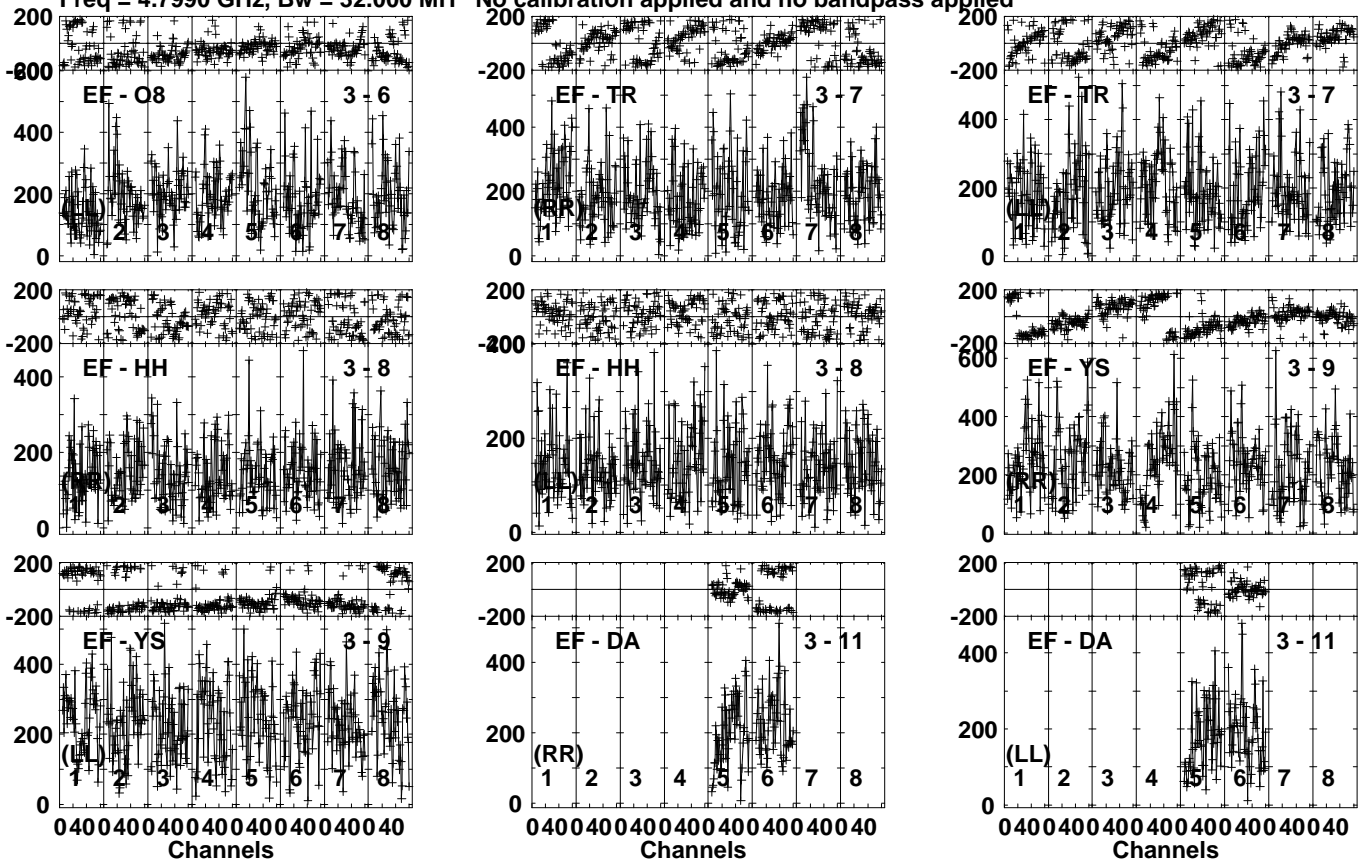
Lower frame: Micro Ampl Jy Top frame: Phas deg Vector averaged cross-power spectrum Several baselines displayed Timerange: 00/19:34:51 to 00/19:36:39
