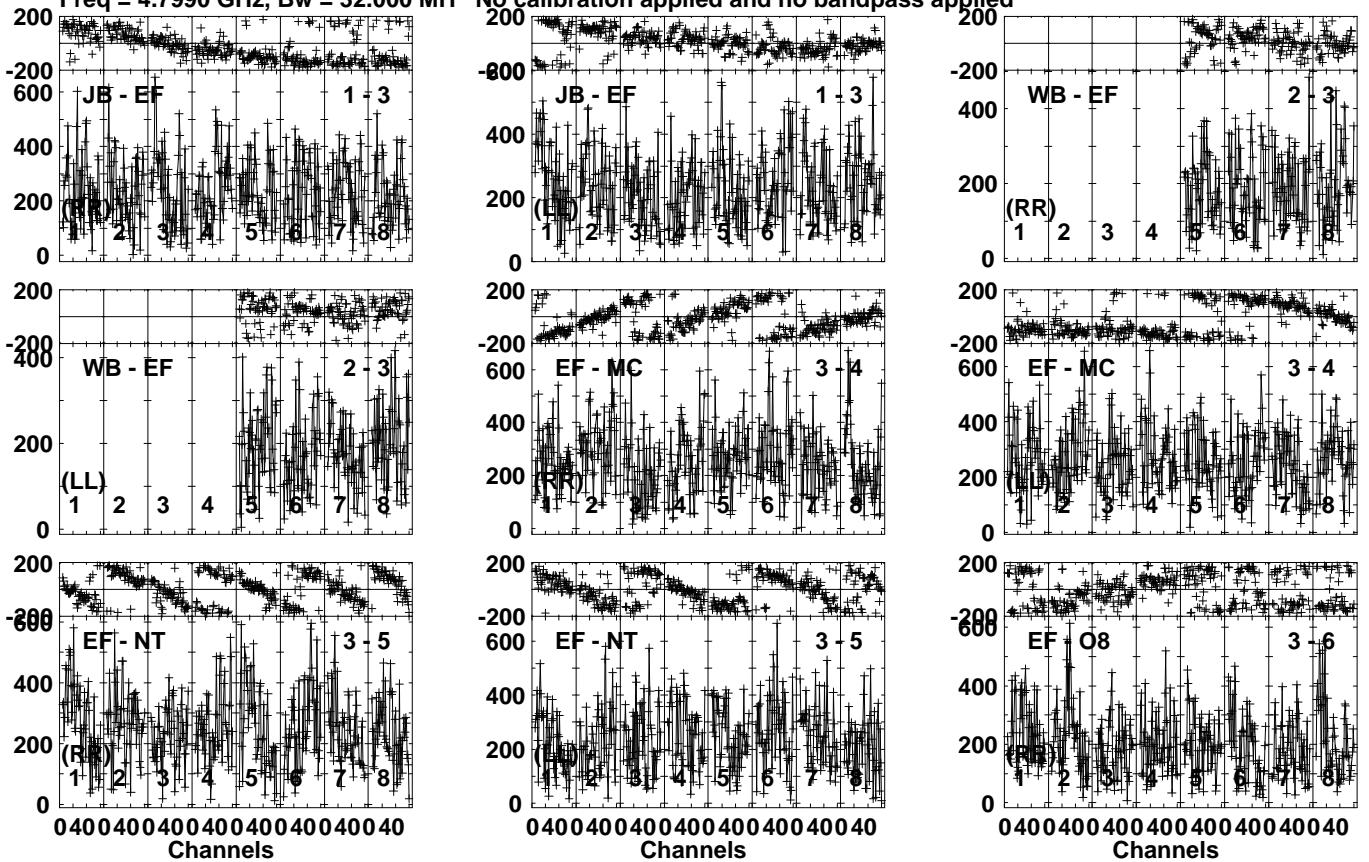
Lower frame: Micro Ampl Jy Top frame: Phas deg Vector averaged cross-power spectrum Several baselines displayed Timerange: 00/17:16:01 to 00/17:17:09
