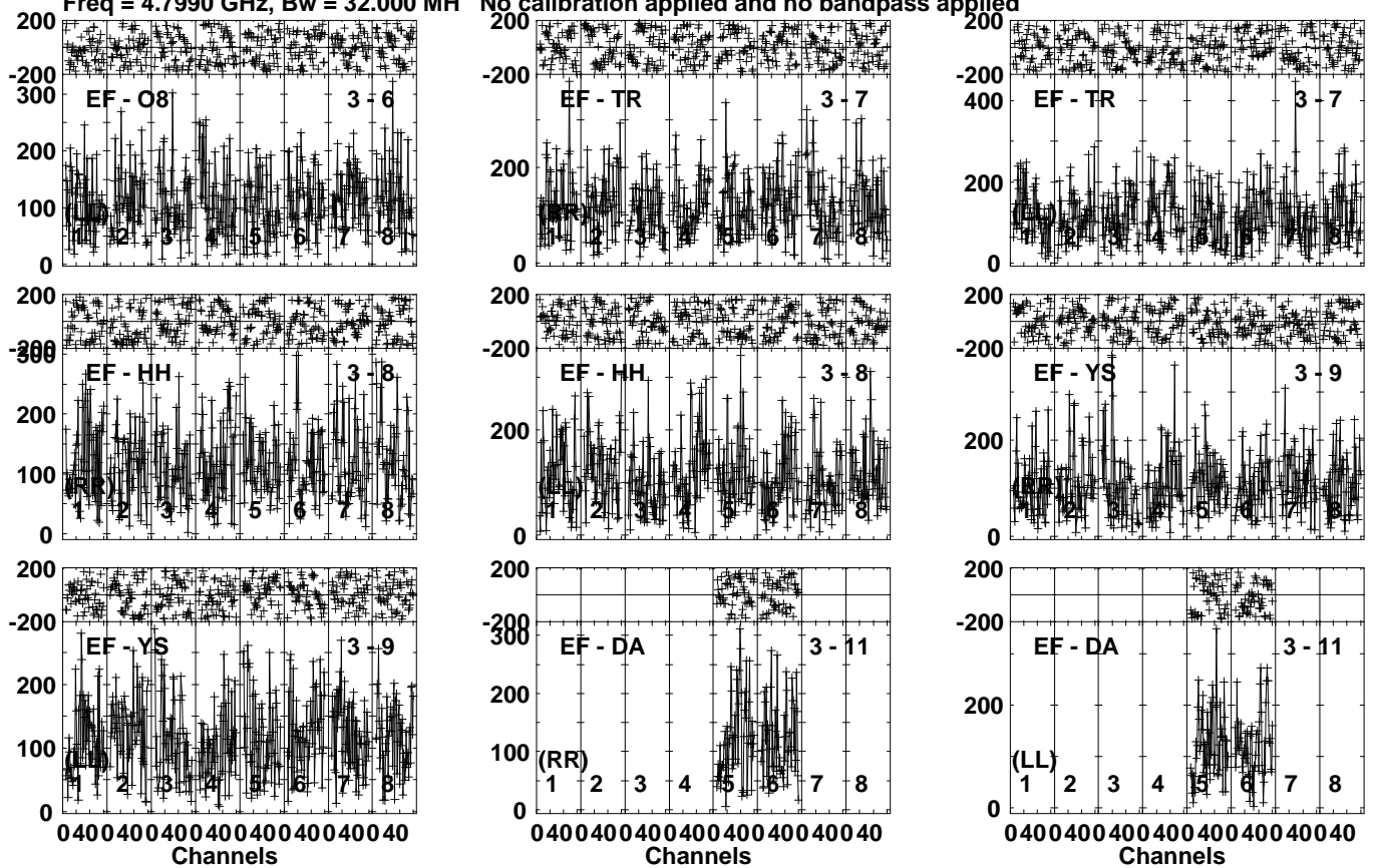
Lower frame: Micro Ampl Jy Top frame: Phas deg Vector averaged cross-power spectrum Several baselines displayed Timerange: 00/17:27:11 to 00/17:29:29
