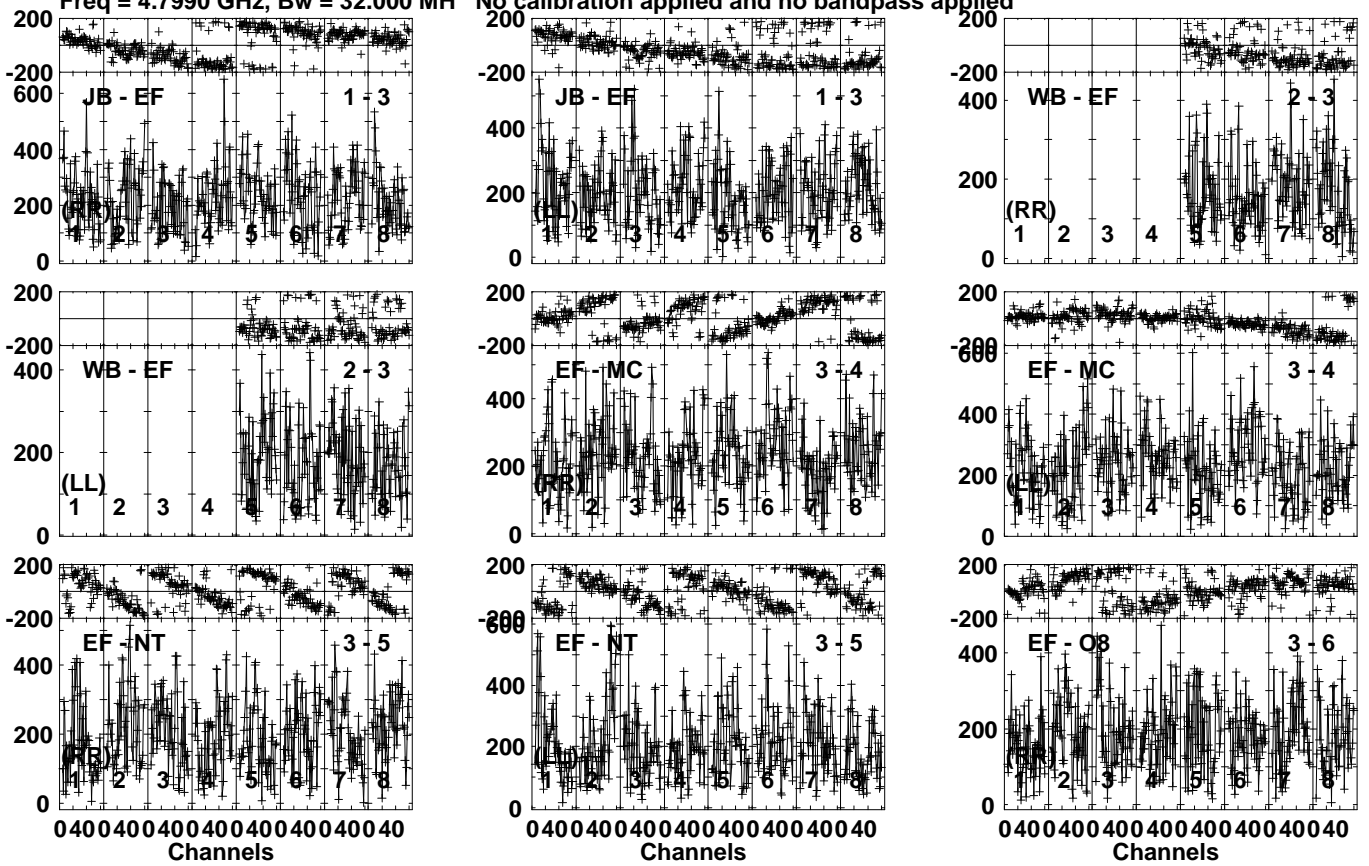
Lower frame: Micro Ampl Jy Top frame: Phas deg Vector averaged cross-power spectrum Several baselines displayed Timerange: 00/19:45:51 to 00/19:47:39
