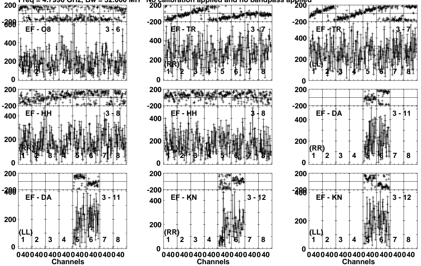
Lower frame: Micro Ampl Jy Top frame: Phas deg Vector averaged cross-power spectrum Several baselines displayed Timerange: 00/15:03:41 to 00/15:04:49
