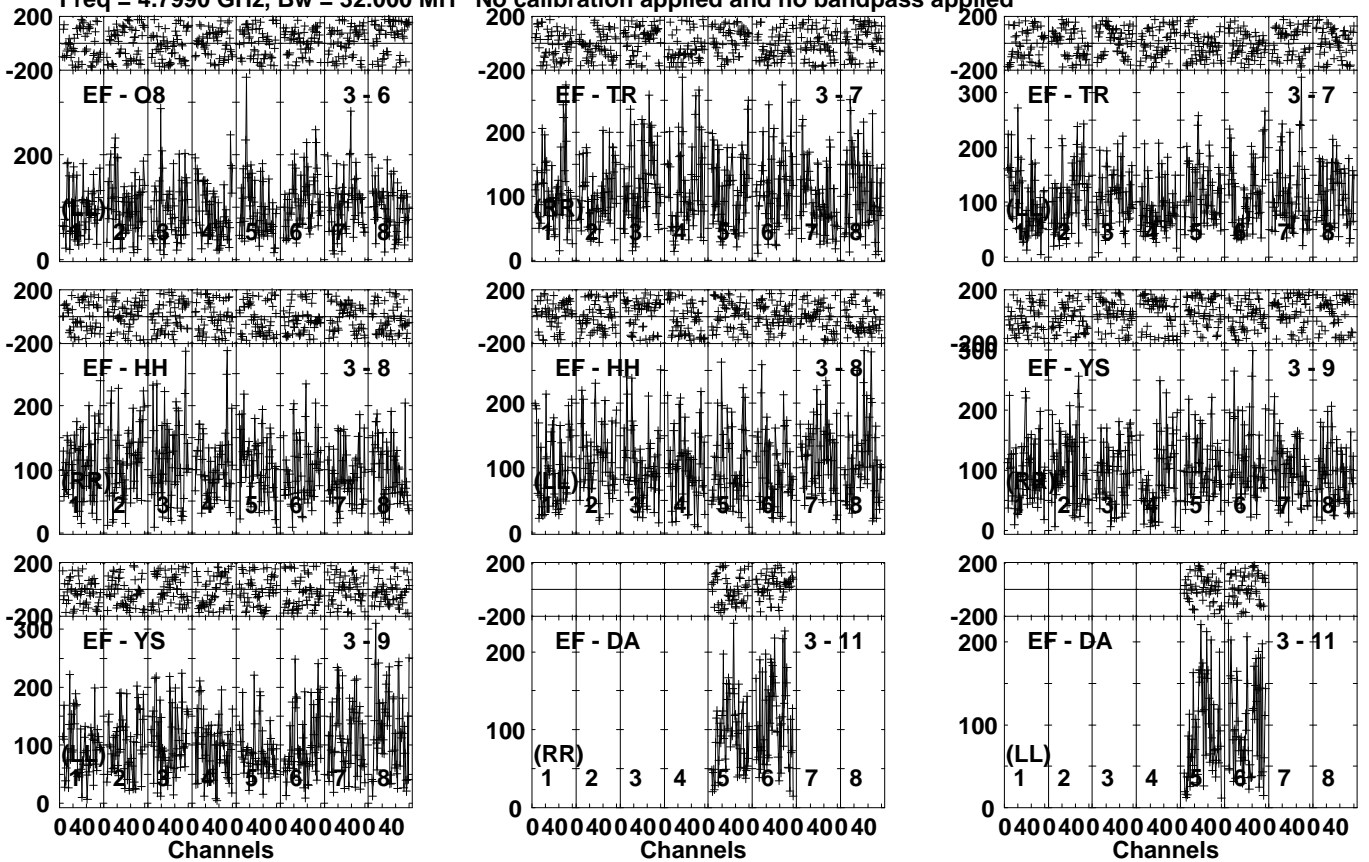
Lower frame: Micro Ampl Jy Top frame: Phas deg Vector averaged cross-power spectrum Several baselines displayed Timerange: 00/18:53:01 to 00/18:55:19
