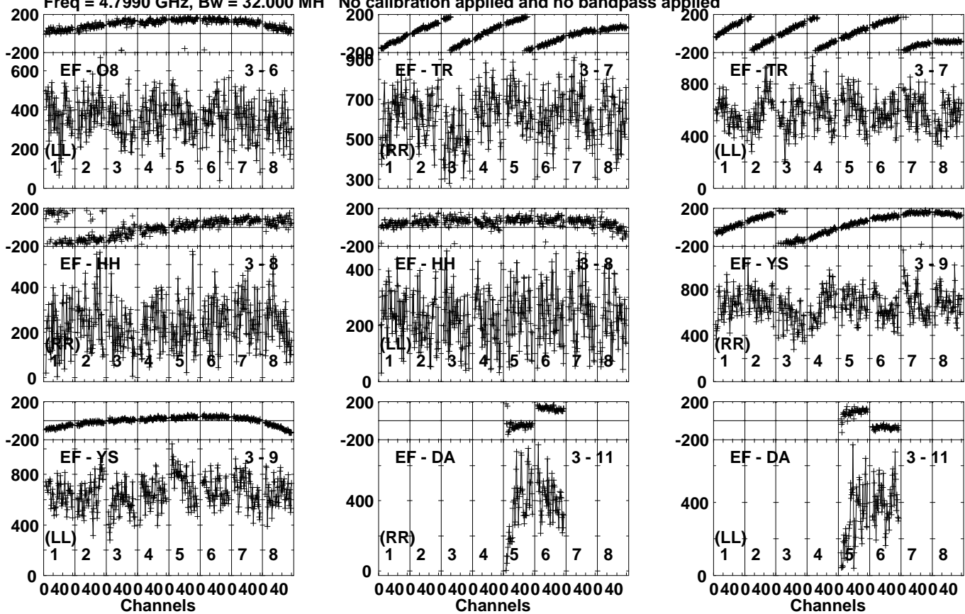
Lower frame: Micro Ampl Jy Top frame: Phas deg Vector averaged cross-power spectrum Several baselines displayed Timerange: 00/18:01:01 to 00/18:02:29
