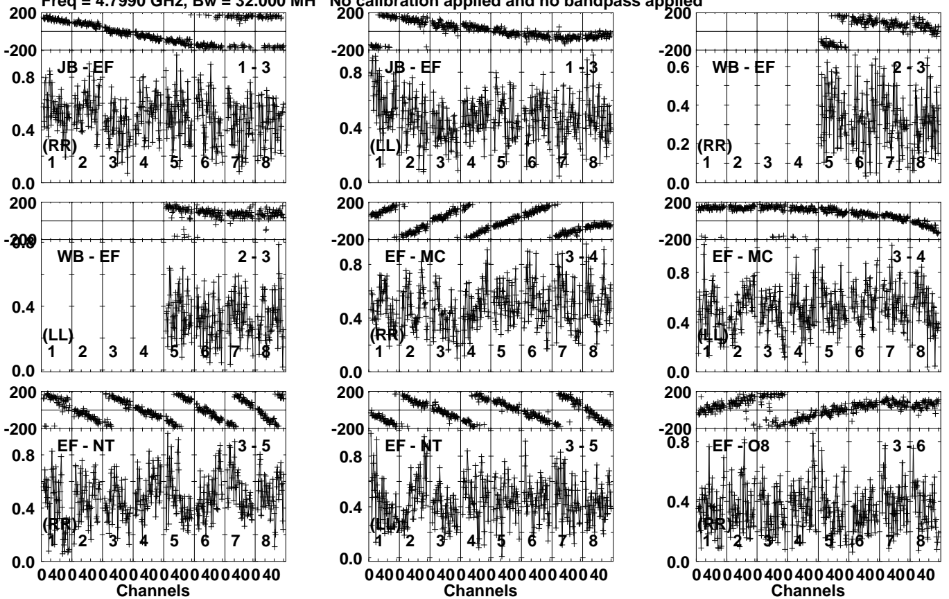
Lower frame: Milli Ampl Jy Top frame: Phas deg Vector averaged cross-power spectrum Several baselines displayed Timerange: 00/19:37:21 to 00/19:38:19
