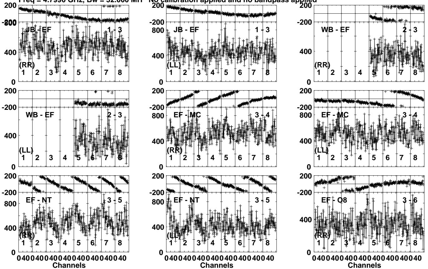
Lower frame: Micro Ampl Jy Top frame: Phas deg Vector averaged cross-power spectrum Several baselines displayed Timerange: 00/16:22:11 to 00/16:23:09
