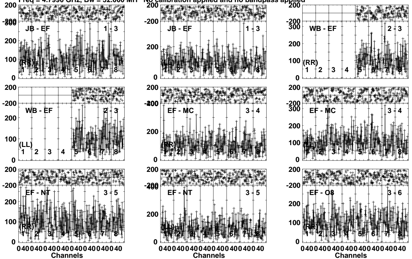
Lower frame: Micro Ampl Jy Top frame: Phas deg Vector averaged cross-power spectrum Several baselines displayed Timerange: 00/17:13:41 to 00/17:15:59
