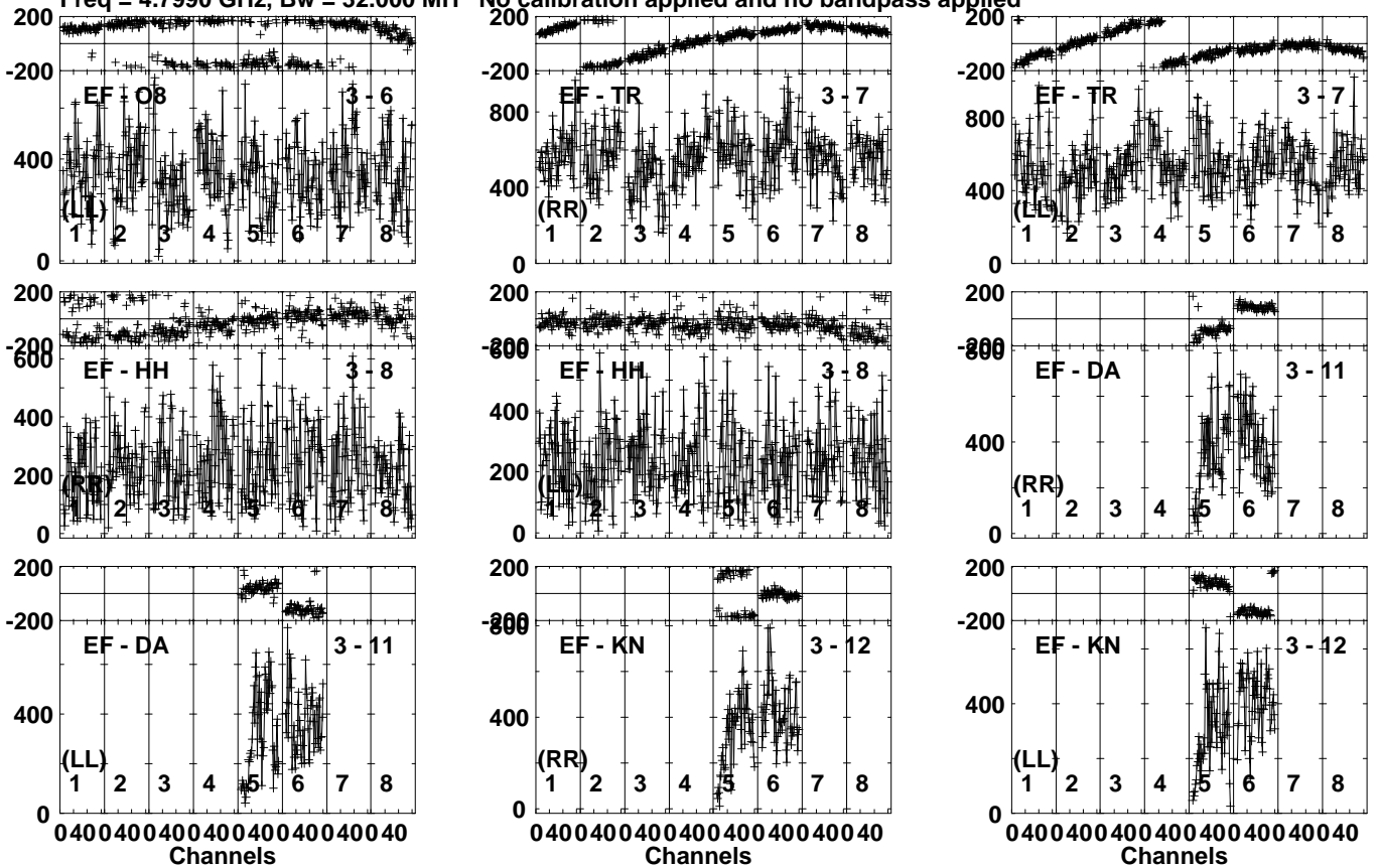
Lower frame: Micro Ampl Jy Top frame: Phas deg Vector averaged cross-power spectrum Several baselines displayed Timerange: 00/14:14:31 to 00/14:15:29
