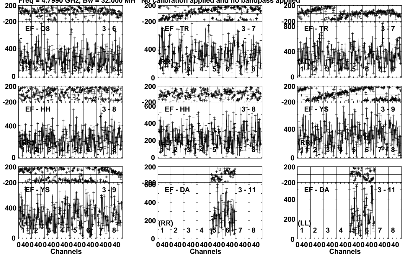
Lower frame: Micro Ampl Jy Top frame: Phas deg Vector averaged cross-power spectrum Several baselines displayed Timerange: 00/13:31:21 to 00/13:32:29
