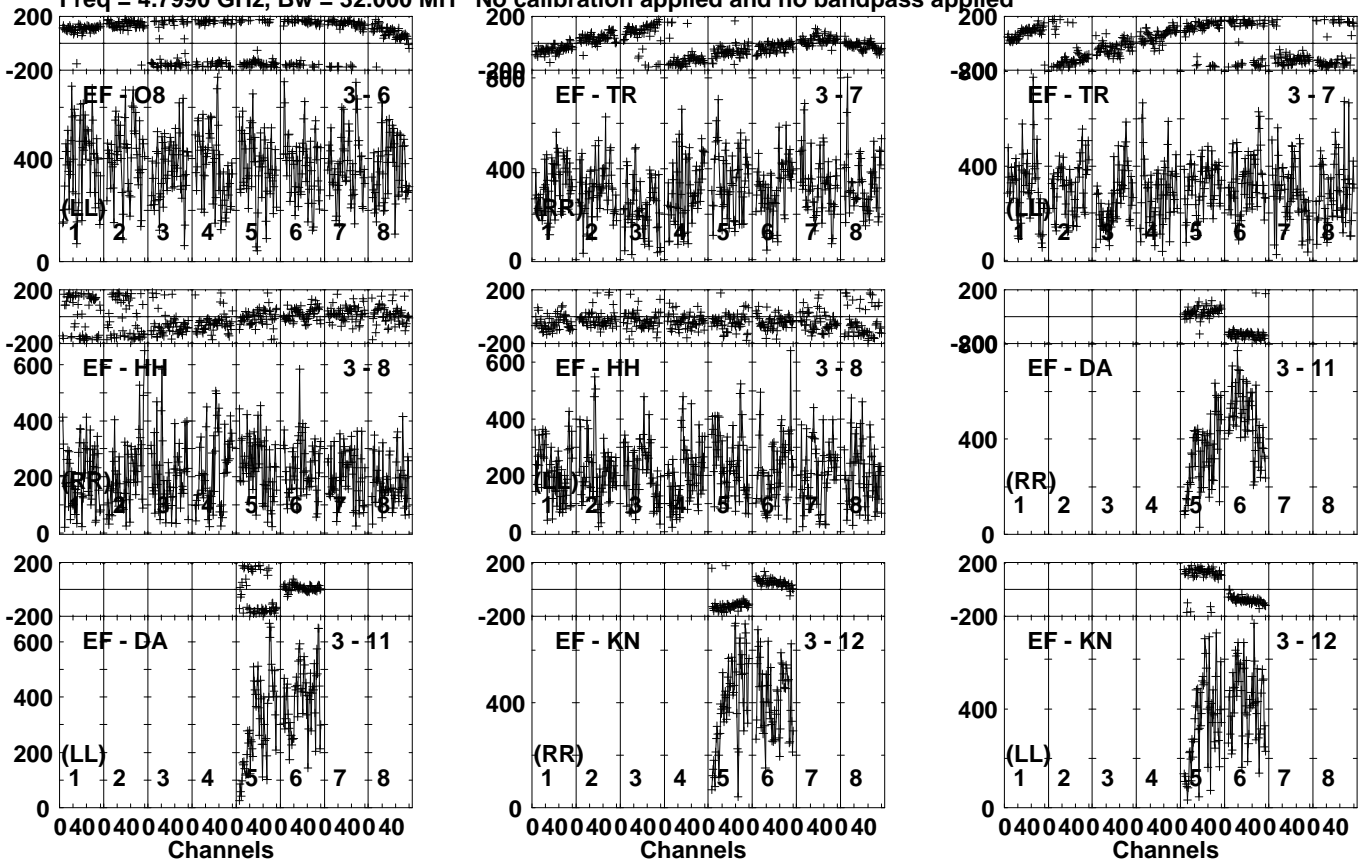
Lower frame: Micro Ampl Jy Top frame: Phas deg Vector averaged cross-power spectrum Several baselines displayed Timerange: 00/14:35:21 to 00/14:36:19
