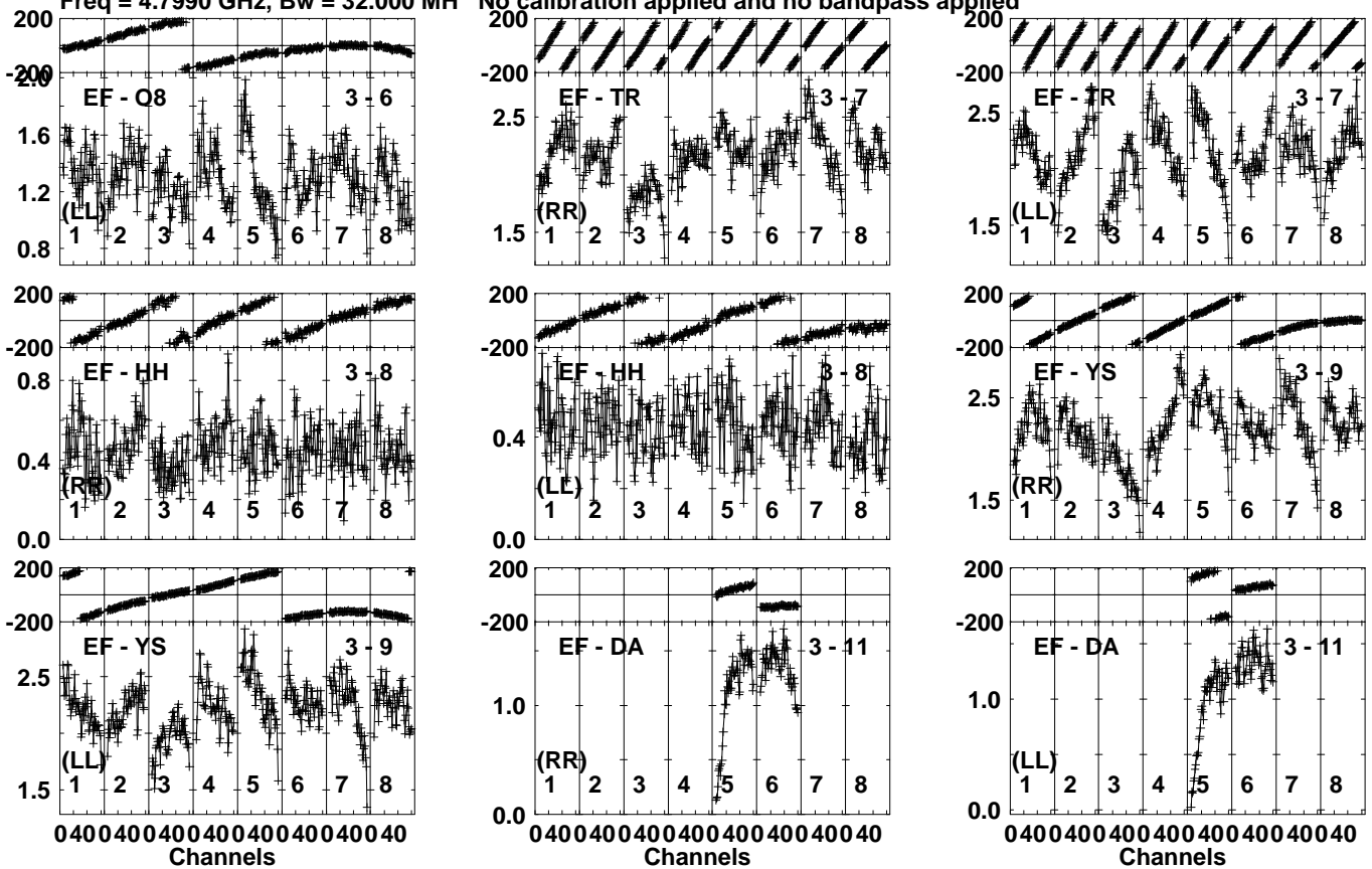
Lower frame: Milli Ampl Jy Top frame: Phas deg Vector averaged cross-power spectrum Several baselines displayed Timerange: 01/12:36:41 to 01/12:37:39
