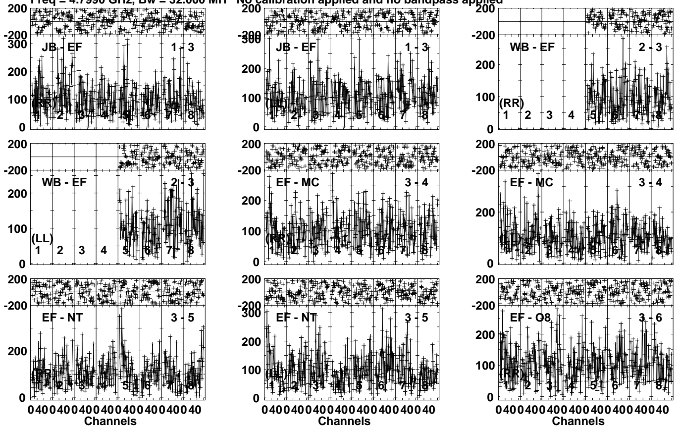
Lower frame: Micro Ampl Jy Top frame: Phas deg Vector averaged cross-power spectrum Several baselines displayed Timerange: 00/16:55:11 to 00/16:57:29
