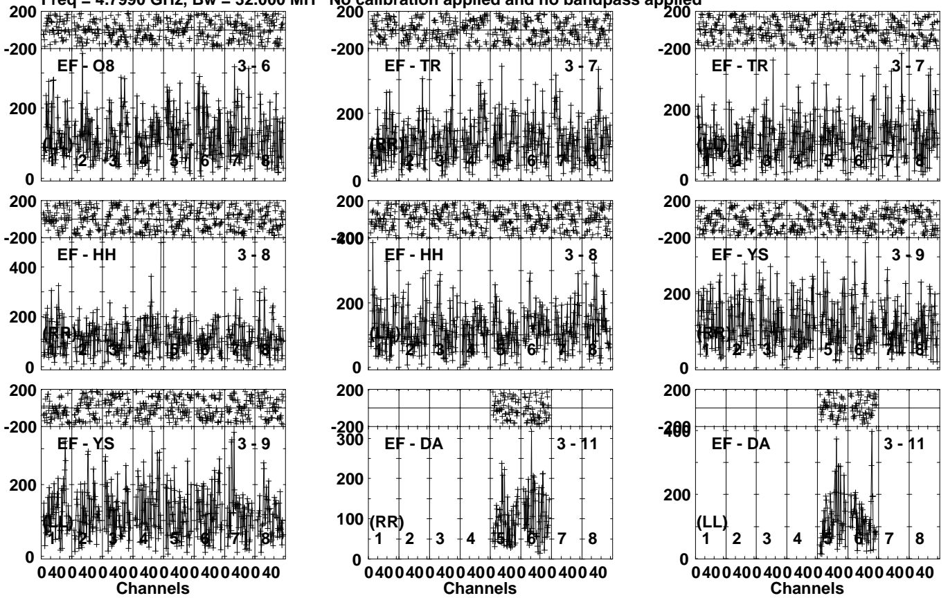
Lower frame: Micro Ampl Jy Top frame: Phas deg Vector averaged cross-power spectrum Several baselines displayed Timerange: 00/18:13:31 to 00/18:15:49
