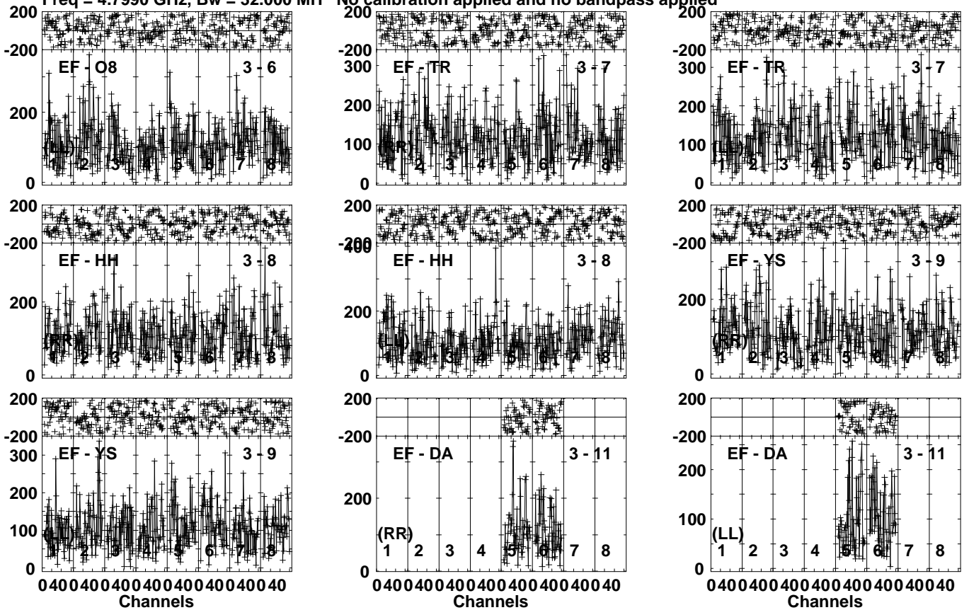
Lower frame: Micro Ampl Jy Top frame: Phas deg Vector averaged cross-power spectrum Several baselines displayed Timerange: 00/19:30:51 to 00/19:33:09
