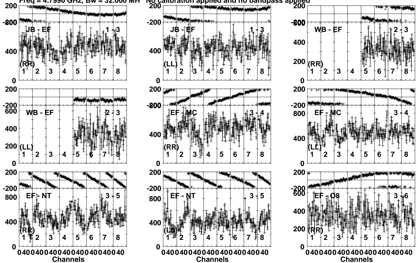
Lower frame: Micro Ampl Jy Top frame: Phas deg Vector averaged cross-power spectrum Several baselines displayed Timerange: 00/14:16:21 to 00/14:17:49
