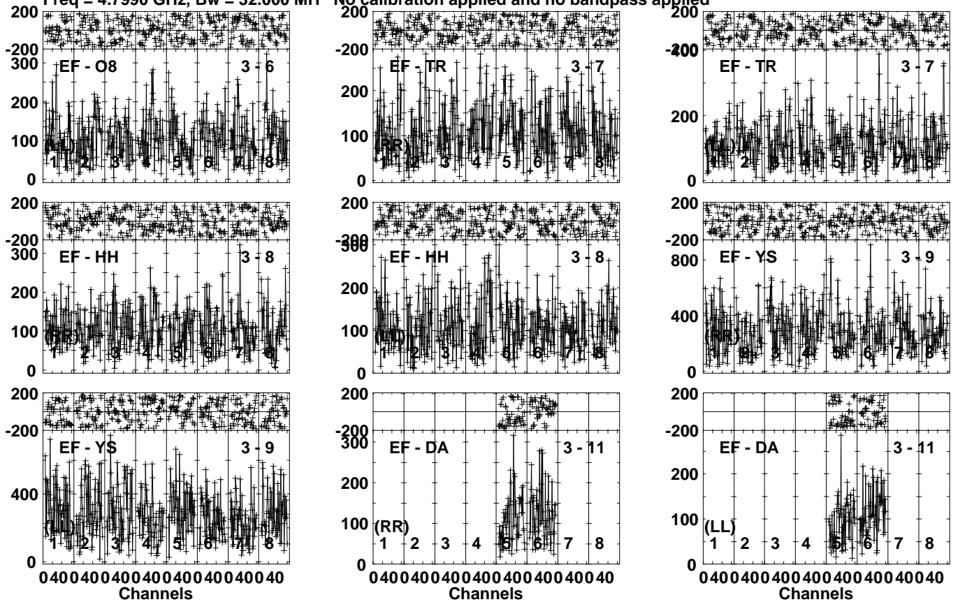
Lower frame: Micro Ampl Jy Top frame: Phas deg Vector averaged cross-power spectrum Several baselines displayed Timerange: 00/16:08:11 to 00/16:10:29
