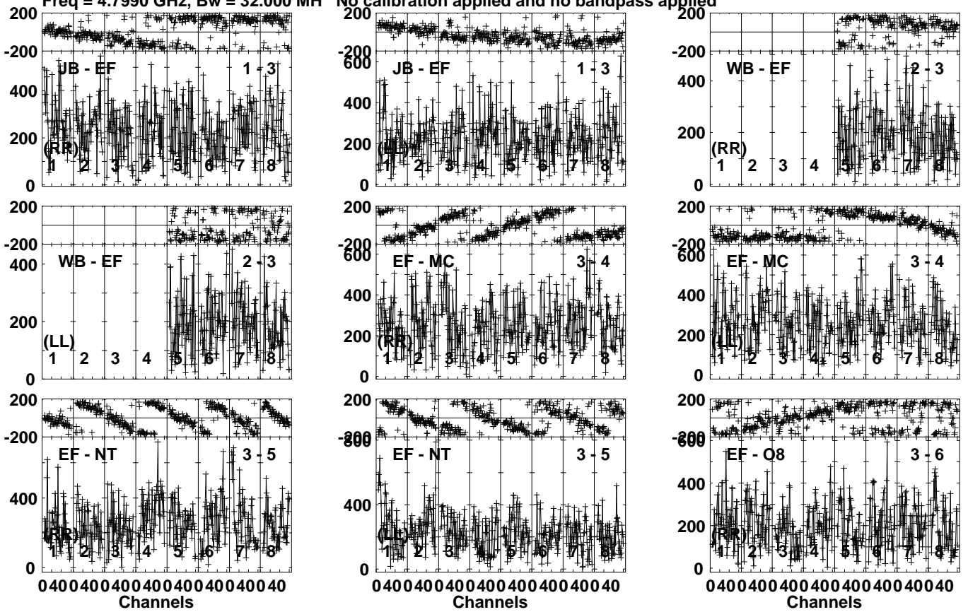
Lower frame: Micro Ampl Jy Top frame: Phas deg Vector averaged cross-power spectrum Several baselines displayed Timerange: 00/15:14:41 to 00/15:15:49
