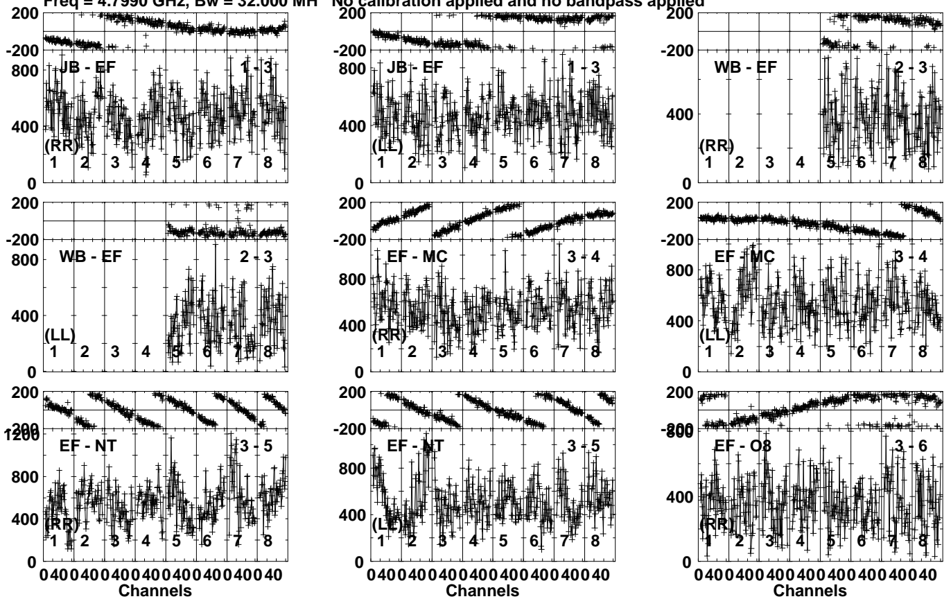
Lower frame: Micro Ampl Jy Top frame: Phas deg Vector averaged cross-power spectrum Several baselines displayed Timerange: 00/15:27:51 to 00/15:29:19
