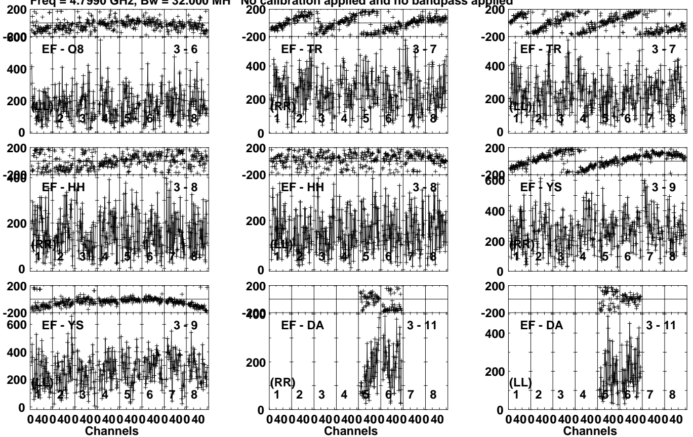
Lower frame: Micro Ampl Jy Top frame: Phas deg Vector averaged cross-power spectrum Several baselines displayed Timerange: 00/17:34:41 to 00/17:36:29
