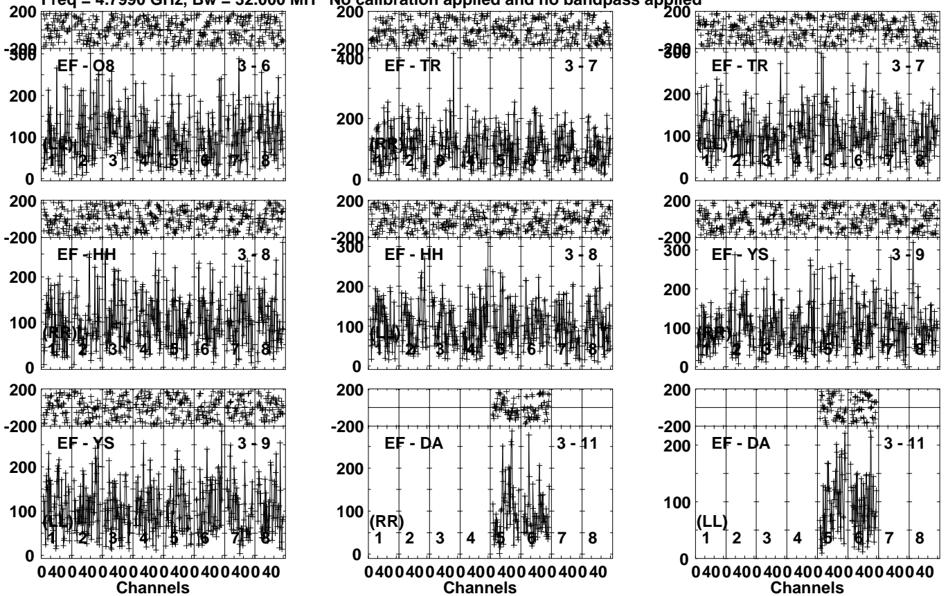
Lower frame: Micro Ampl Jy Top frame: Phas deg Vector averaged cross-power spectrum Several baselines displayed Timerange: 00/13:29:01 to 00/13:31:19
