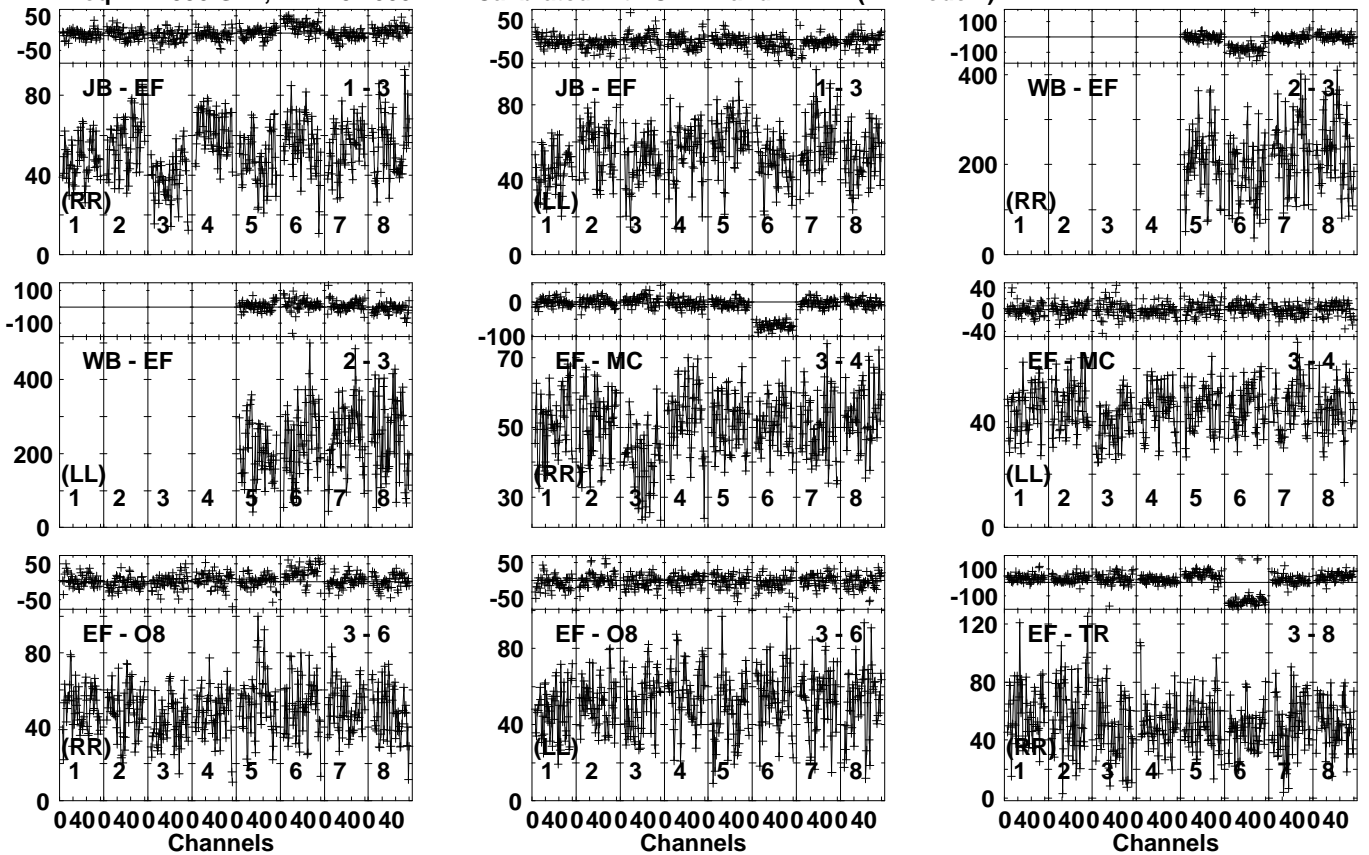
Lower frame: Milli Ampl Jy Top frame: Phas deg Vector averaged cross-power spectrum Several baselines displayed Timerange: 00/10:25:21 to 00/10:26:29
