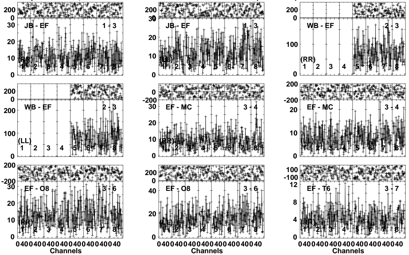
Lower frame: Milli Ampl Jy Top frame: Phas deg Vector averaged cross-power spectrum Several baselines displayed Timerange: 00/09:46:31 to 00/09:48:49
