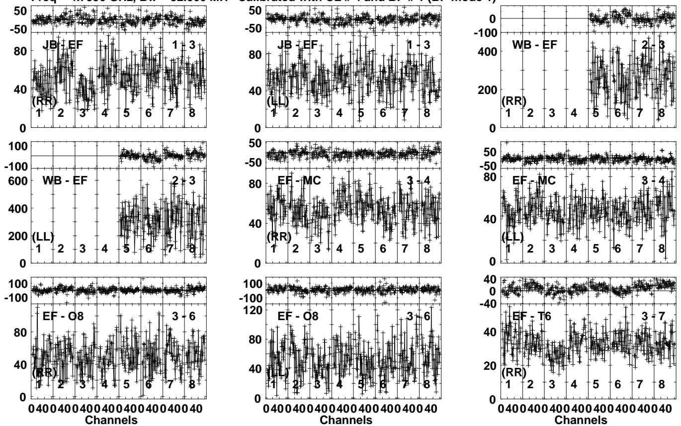
Lower frame: Milli Ampl Jy Top frame: Phas deg Vector averaged cross-power spectrum Several baselines displayed Timerange: 00/09:27:21 to 00/09:28:29
