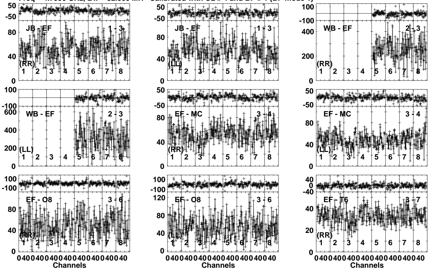
Lower frame: Milli Ampl Jy Top frame: Phas deg Vector averaged cross-power spectrum Several baselines displayed Timerange: 00/09:41:51 to 00/09:42:59
