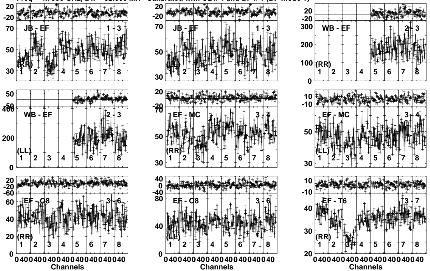
Lower frame: Milli Ampl Jy Top frame: Phas deg Vector averaged cross-power spectrum Several baselines displayed Timerange: 00/09:00:31 to 00/09:02:59
