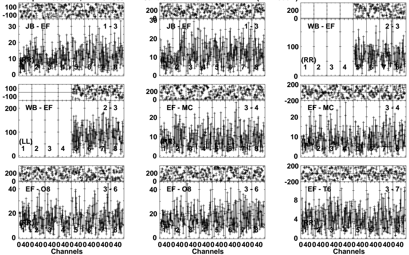
Lower frame: Milli Ampl Jy Top frame: Phas deg Vector averaged cross-power spectrum Several baselines displayed Timerange: 00/09:03:01 to 00/09:05:19
