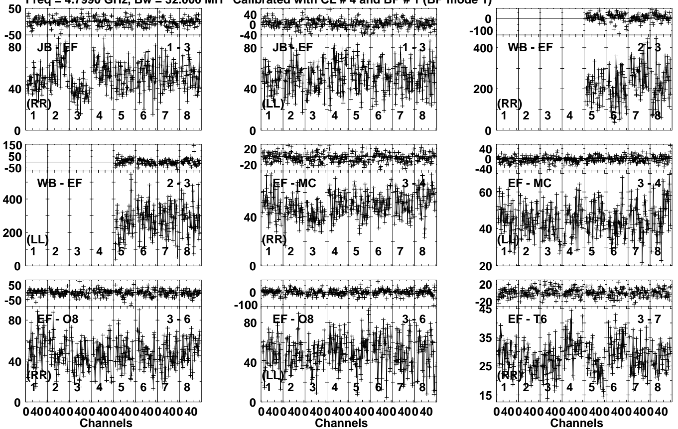
Lower frame: Milli Ampl Jy Top frame: Phas deg Vector averaged cross-power spectrum Several baselines displayed Timerange: 00/10:10:51 to 00/10:11:59
