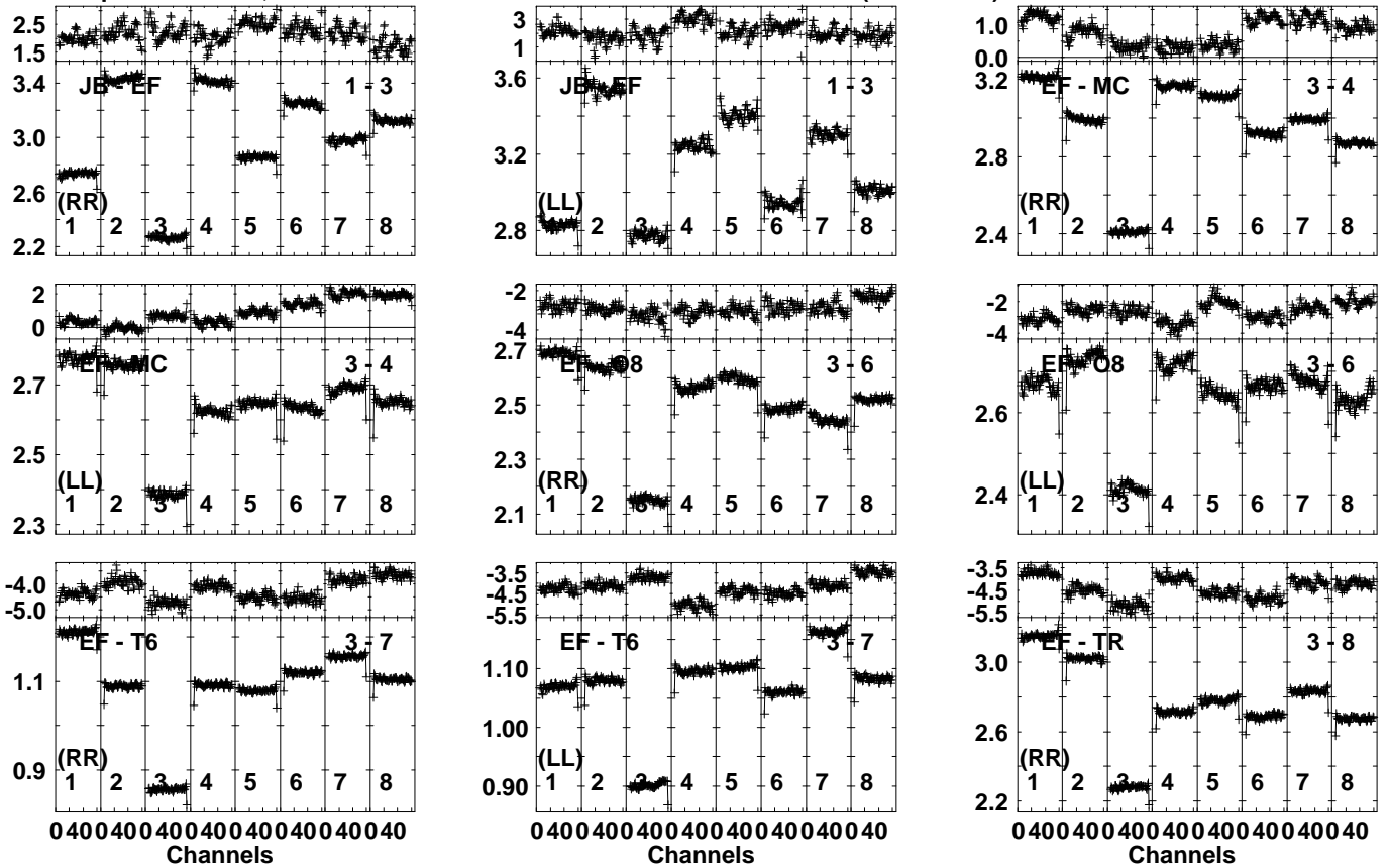
Lower frame: Ampl Jy Top frame: Phas deg Vector averaged cross-power spectrum Several baselines displayed Timerange: 00/08:55:11 to 00/08:58:59
