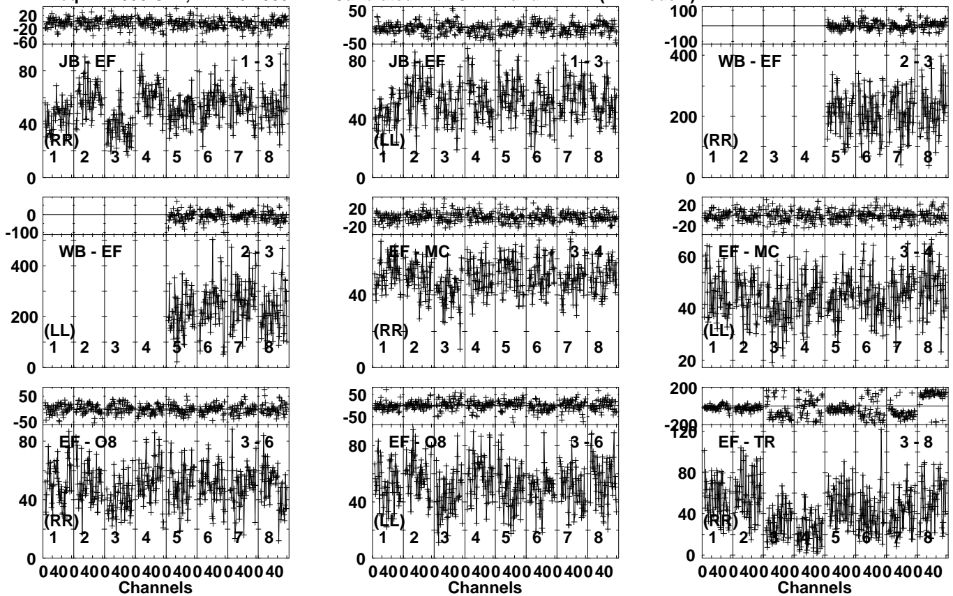
Lower frame: Milli Ampl Jy Top frame: Phas deg Vector averaged cross-power spectrum Several baselines displayed Timerange: 00/10:39:51 to 00/10:40:59
