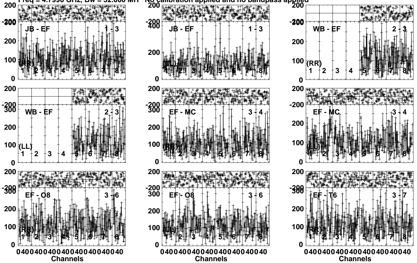
Lower frame: Micro Ampl Jy Top frame: Phas deg Vector averaged cross-power spectrum Several baselines displayed Timerange: 00/09:54:01 to 00/09:56:19
