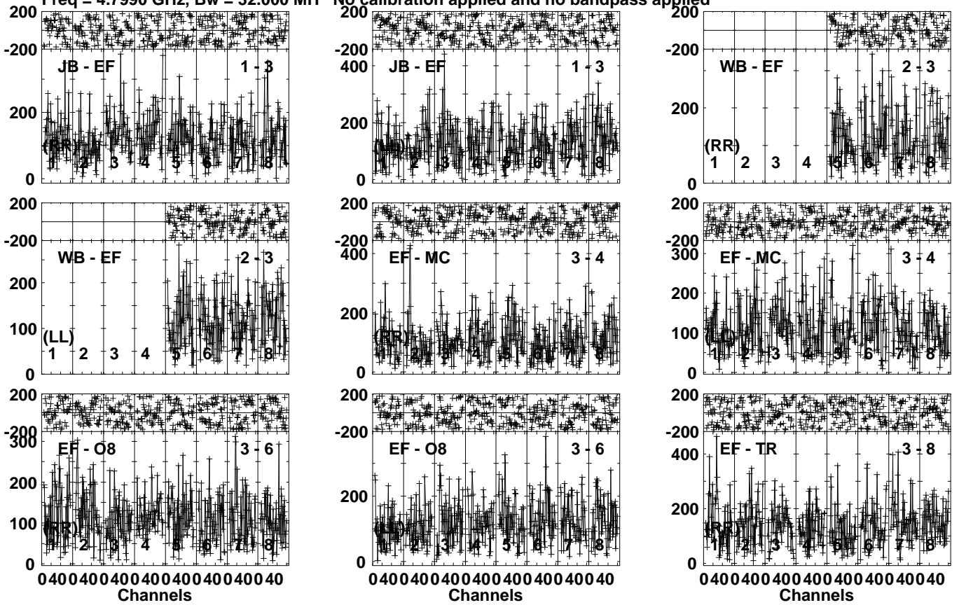
Lower frame: Micro Ampl Jy Top frame: Phas deg Vector averaged cross-power spectrum Several baselines displayed Timerange: 00/10:41:01 to 00/10:42:49
