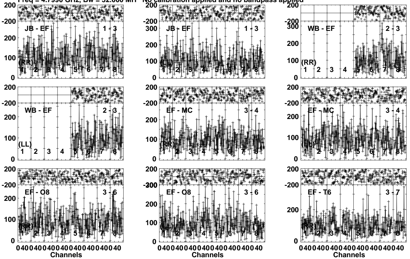
Lower frame: Micro Ampl Jy Top frame: Phas deg Vector averaged cross-power spectrum Several baselines displayed Timerange: 00/10:01:01 to 00/10:03:19
