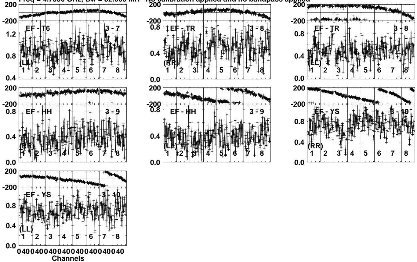
Lower frame: Milli Ampl Jy Top frame: Phas deg Vector averaged cross-power spectrum Several baselines displayed Timerange: 00/09:16:31 to 00/09:17:29
