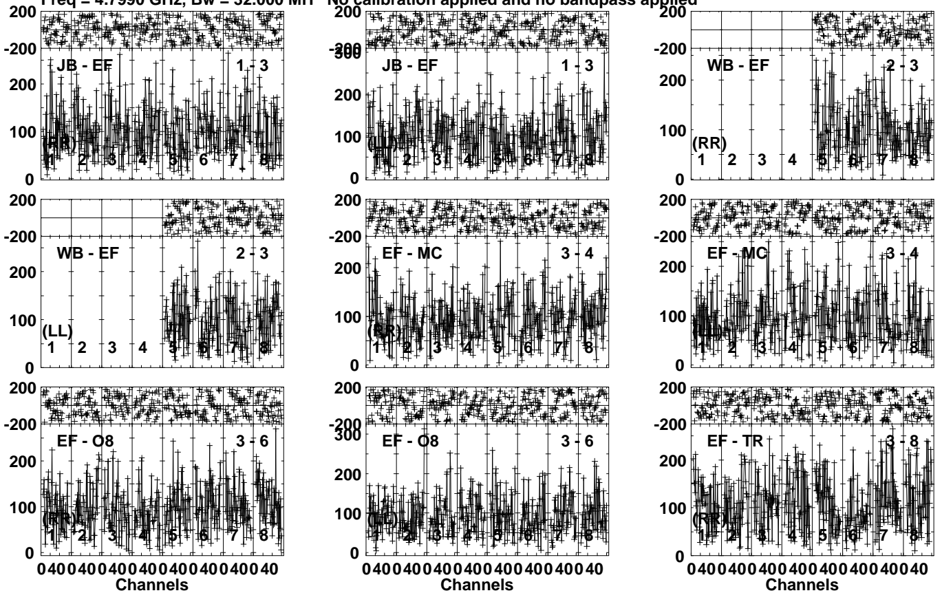
Lower frame: Micro Ampl Jy Top frame: Phas deg Vector averaged cross-power spectrum Several baselines displayed Timerange: 00/10:44:31 to 00/10:46:49
