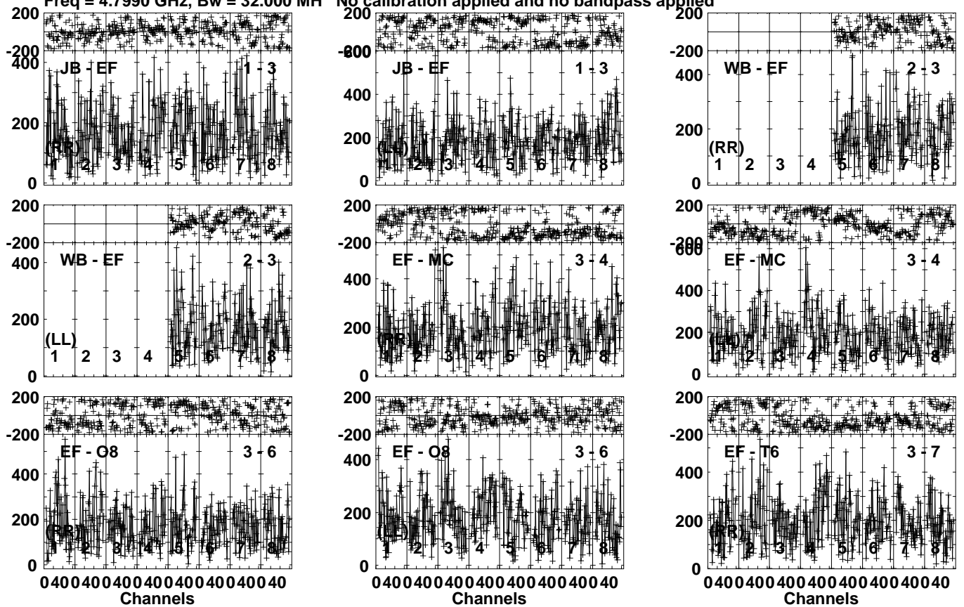
Lower frame: Micro Ampl Jy Top frame: Phas deg Vector averaged cross-power spectrum Several baselines displayed Timerange: 00/09:14:01 to 00/09:15:49
