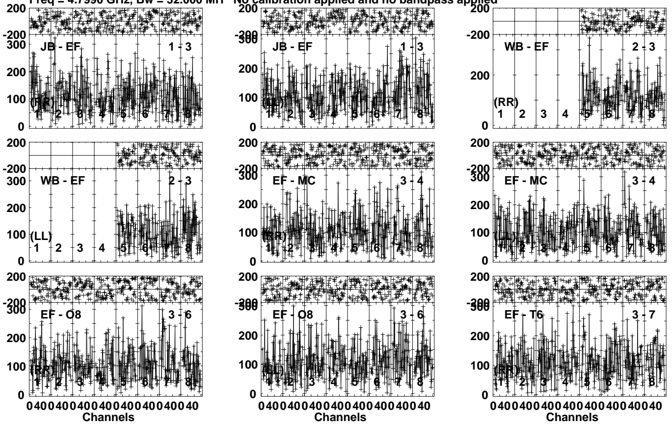
Lower frame: Micro Ampl Jy Top frame: Phas deg Vector averaged cross-power spectrum Several baselines displayed Timerange: 00/09:46:31 to 00/09:48:49
