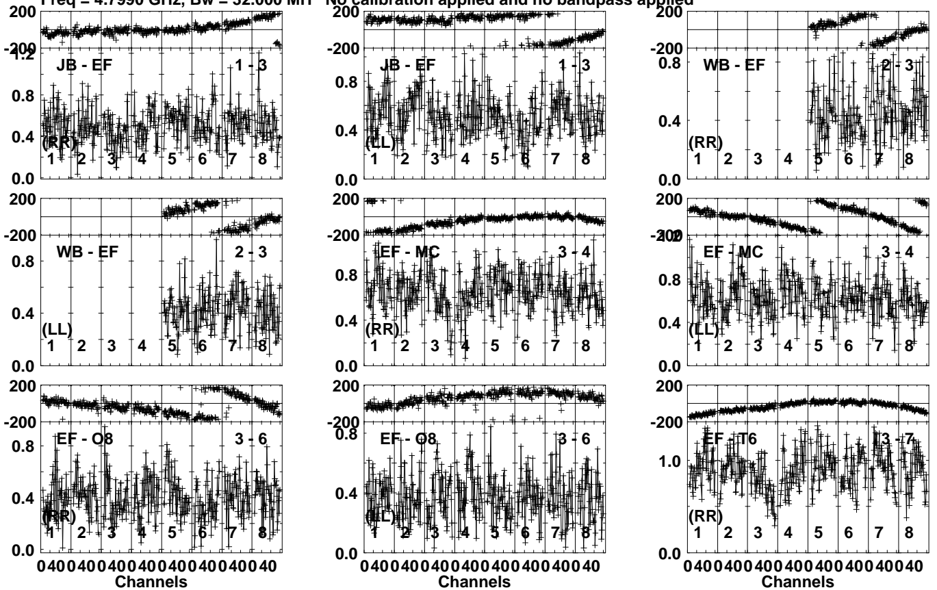
Lower frame: Milli Ampl Jy Top frame: Phas deg Vector averaged cross-power spectrum Several baselines displayed Timerange: 00/09:34:21 to 00/09:35:29
