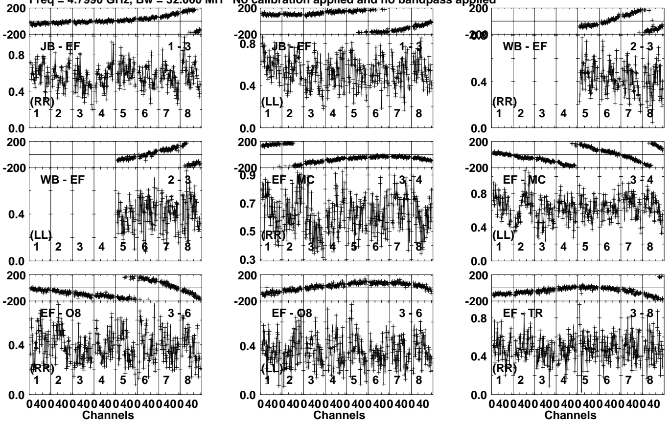
Lower frame: Milli Ampl Jy Top frame: Phas deg Vector averaged cross-power spectrum Several baselines displayed Timerange: 00/10:29:01 to 00/10:29:59
