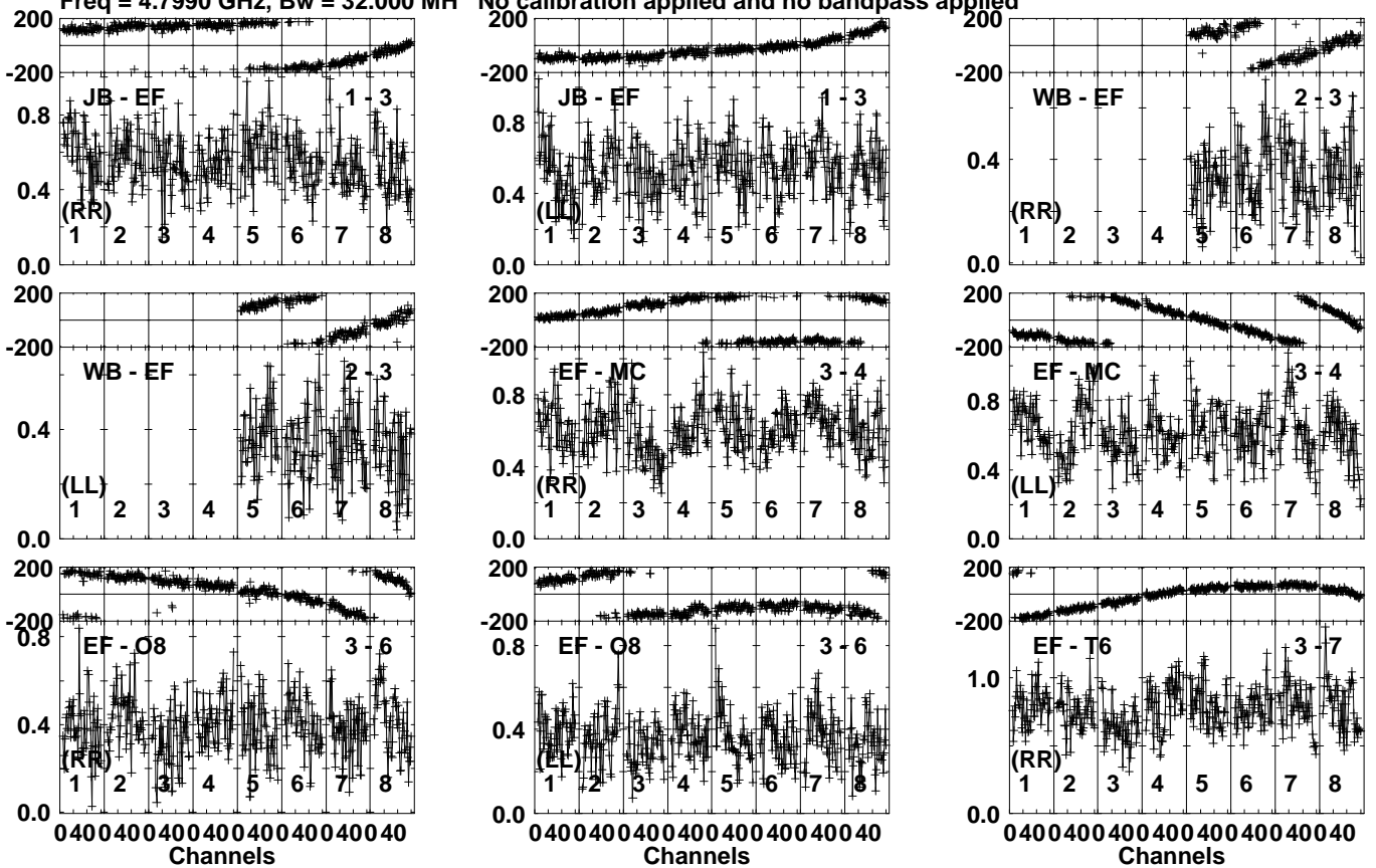
Lower frame: Milli Ampl Jy Top frame: Phas deg Vector averaged cross-power spectrum Several baselines displayed Timerange: 00/10:03:21 to 00/10:04:29
