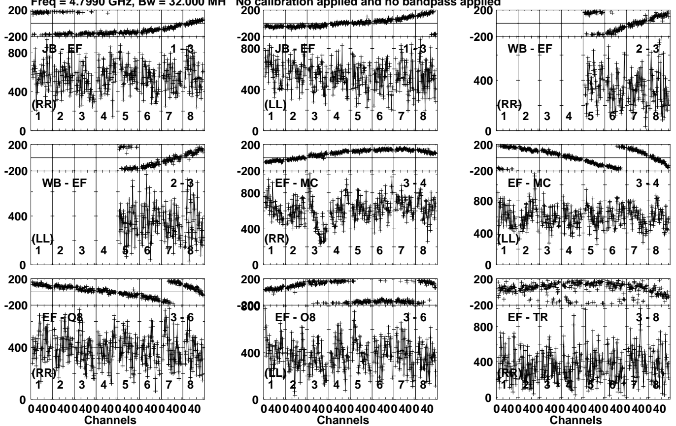
Lower frame: Micro Ampl Jy Top frame: Phas deg Vector averaged cross-power spectrum Several baselines displayed Timerange: 00/10:17:51 to 00/10:18:59
