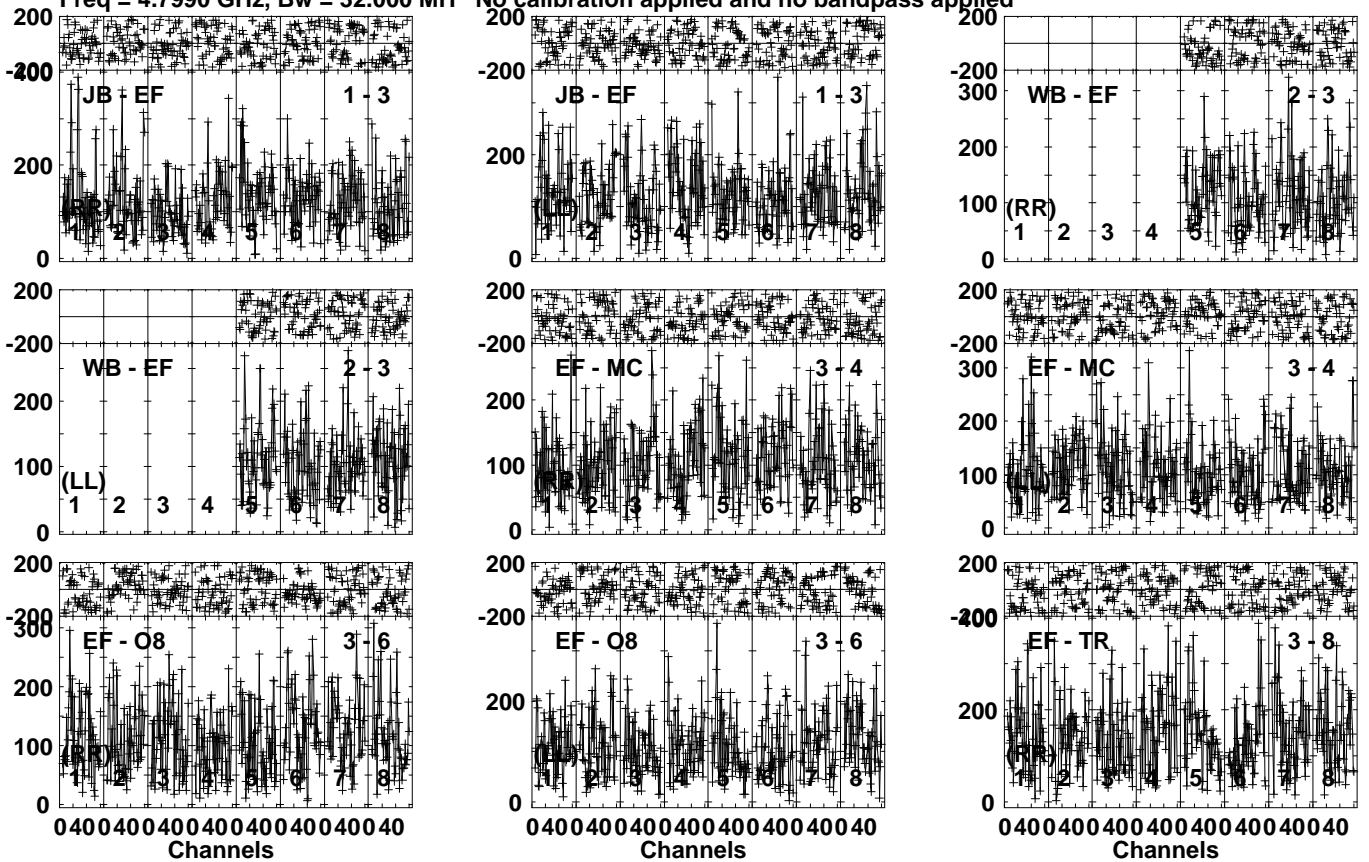
Lower frame: Micro Ampl Jy Top frame: Phas deg Vector averaged cross-power spectrum Several baselines displayed Timerange: 00/10:12:01 to 00/10:13:49
