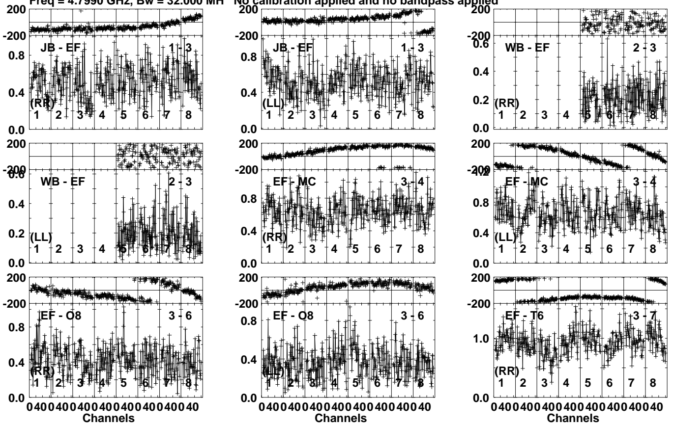
Lower frame: Milli Ampl Jy Top frame: Phas deg Vector averaged cross-power spectrum Several baselines displayed Timerange: 00/09:19:51 to 00/09:20:59
