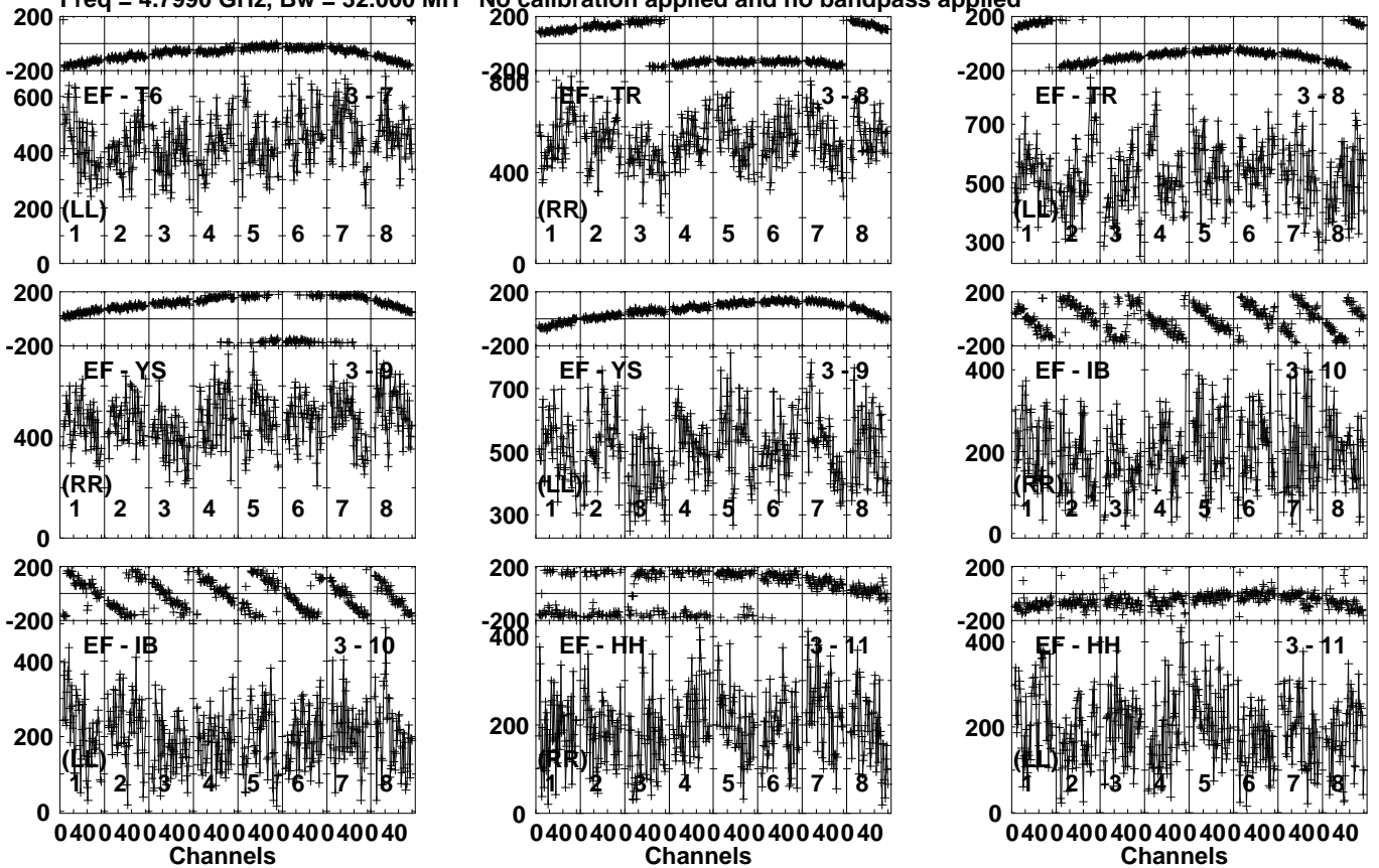
Lower frame: Micro Ampl Jy Top frame: Phas deg Vector averaged cross-power spectrum Several baselines displayed Timerange: 00/18:01:51 to 00/18:03:49
