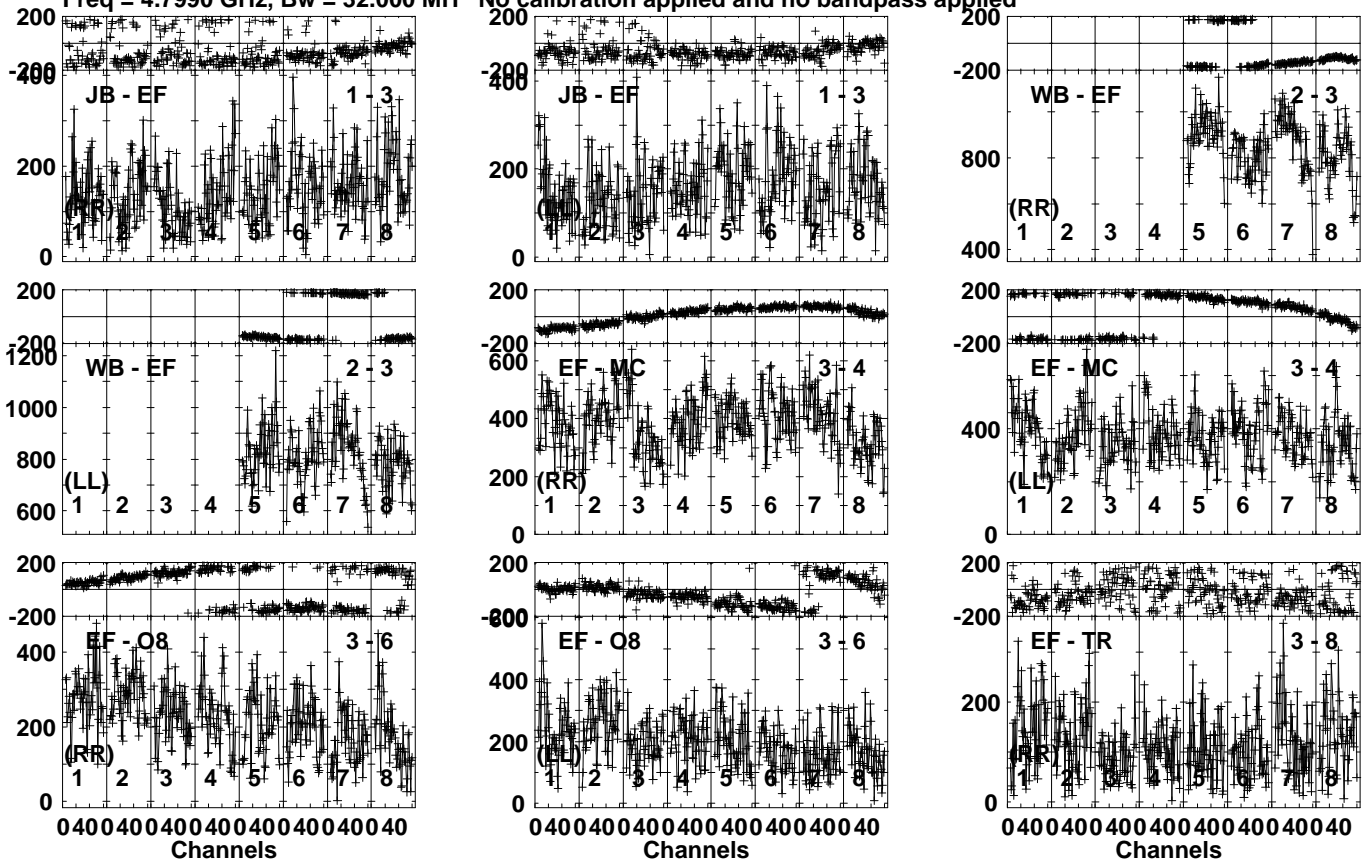
Lower frame: Micro Ampl Jy Top frame: Phas deg Vector averaged cross-power spectrum Several baselines displayed Timerange: 01/09:49:27 to 01/09:51:23
