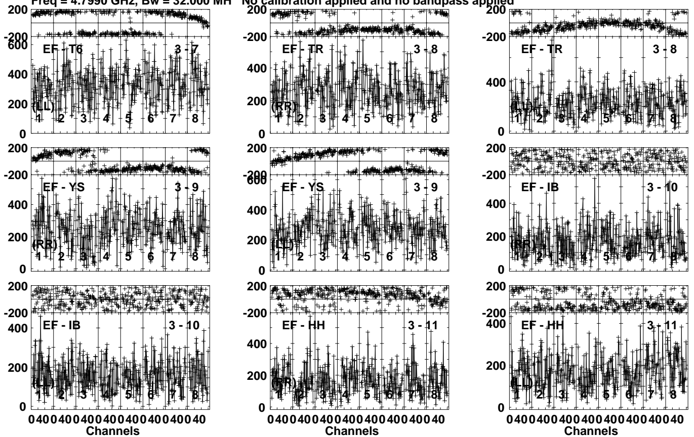
Lower frame: Micro Ampl Jy Top frame: Phas deg Vector averaged cross-power spectrum Several baselines displayed Timerange: 00/16:06:31 to 00/16:07:39
