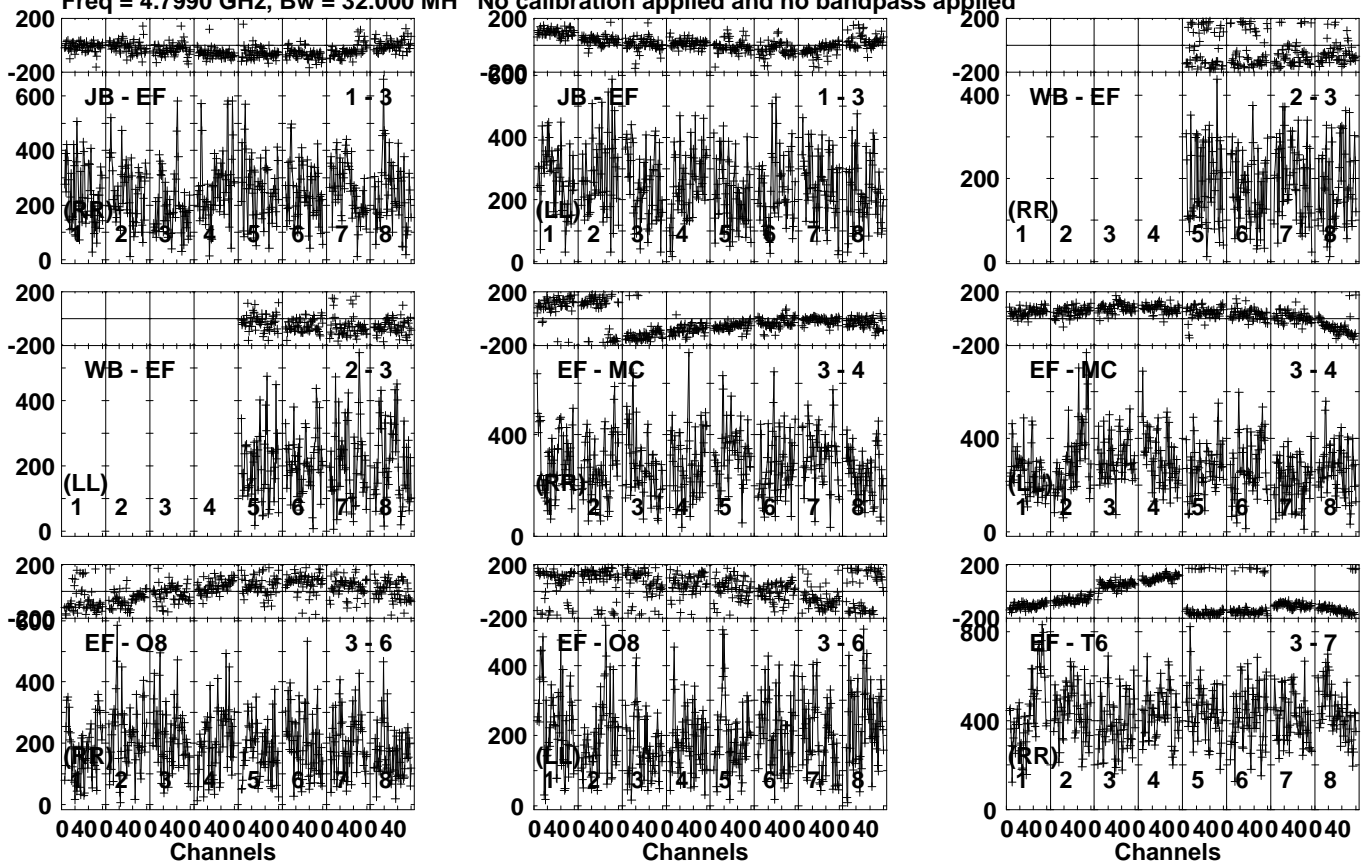
Lower frame: Micro Ampl Jy Top frame: Phas deg Vector averaged cross-power spectrum Several baselines displayed Timerange: 00/17:52:01 to 00/17:53:19
