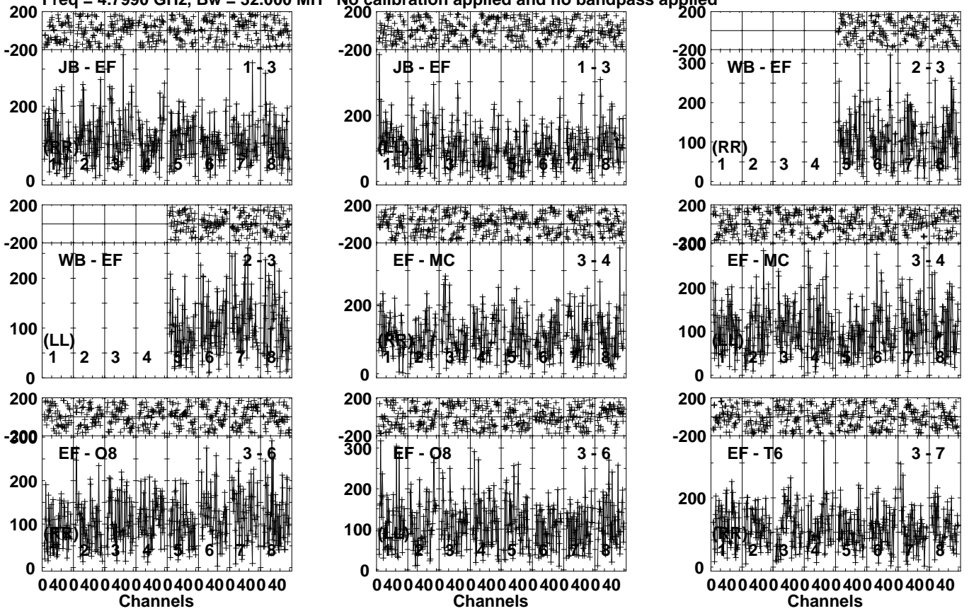
Lower frame: Micro Ampl Jy Top frame: Phas deg Vector averaged cross-power spectrum Several baselines displayed Timerange: 00/15:36:21 to 00/15:38:39
