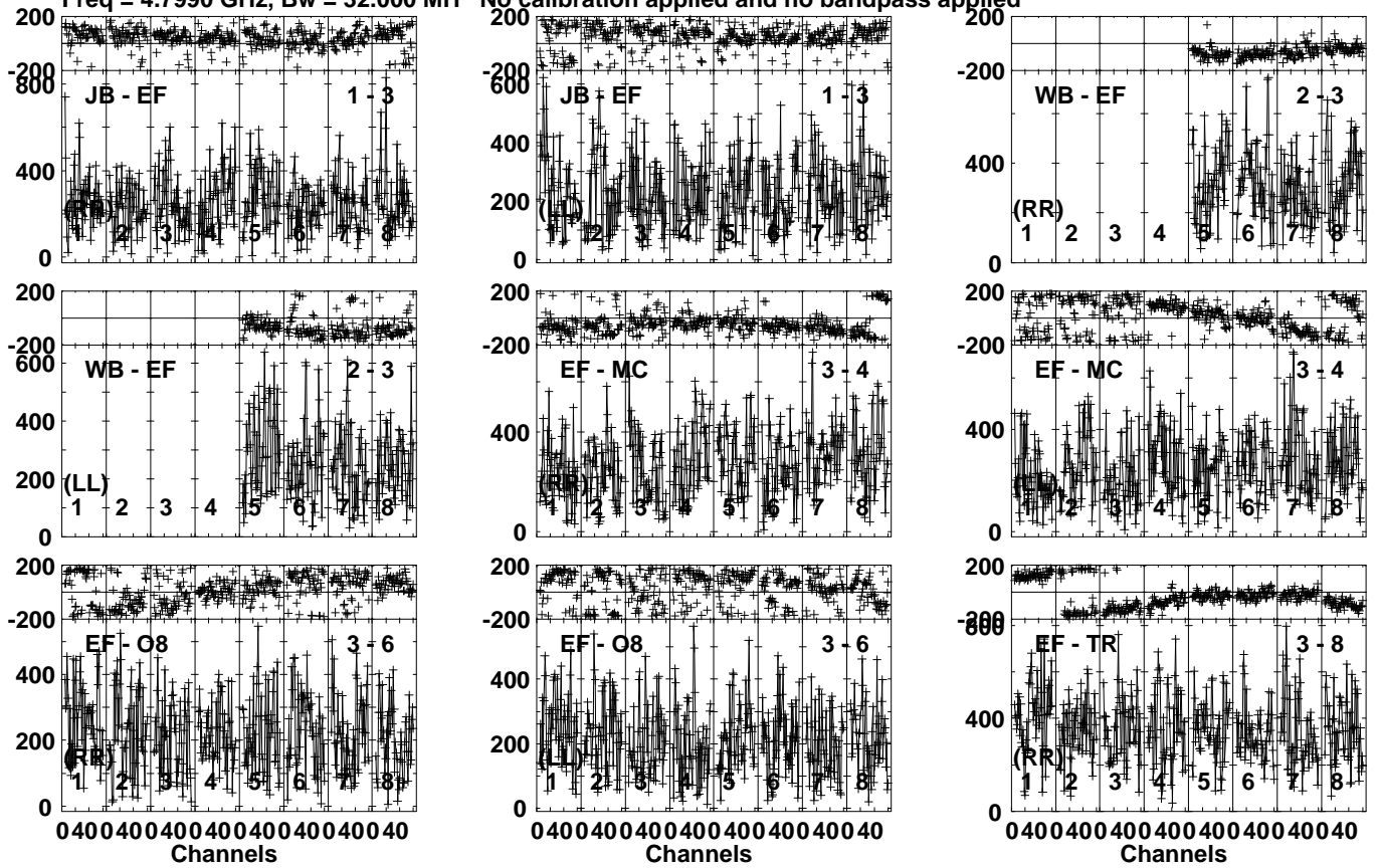
Lower frame: Micro Ampl Jy Top frame: Phas deg Vector averaged cross-power spectrum Several baselines displayed Timerange: 01/10:14:57 to 01/10:16:33
