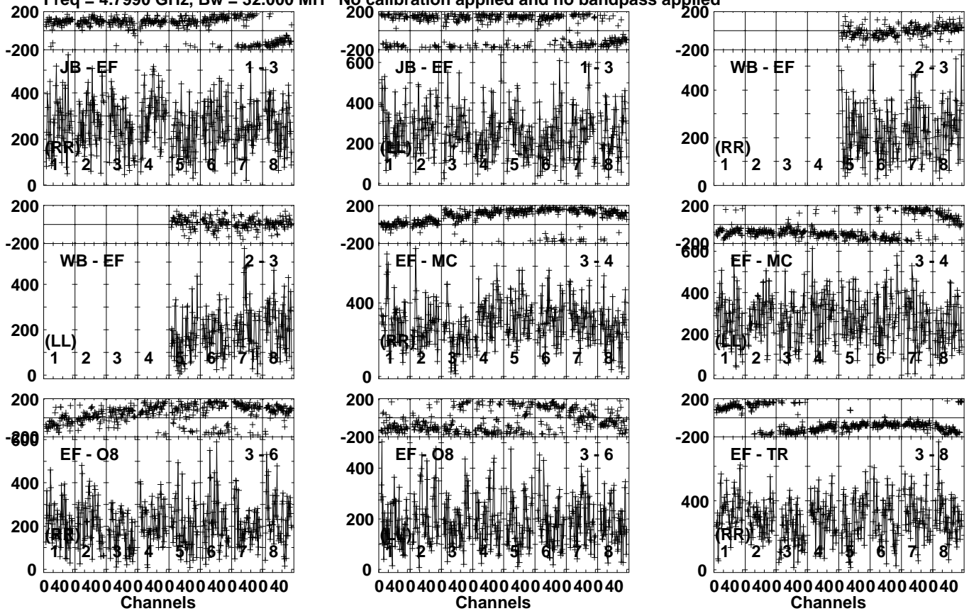
Lower frame: Micro Ampl Jy Top frame: Phas deg Vector averaged cross-power spectrum Several baselines displayed Timerange: 01/08:38:51 to 01/08:40:49
