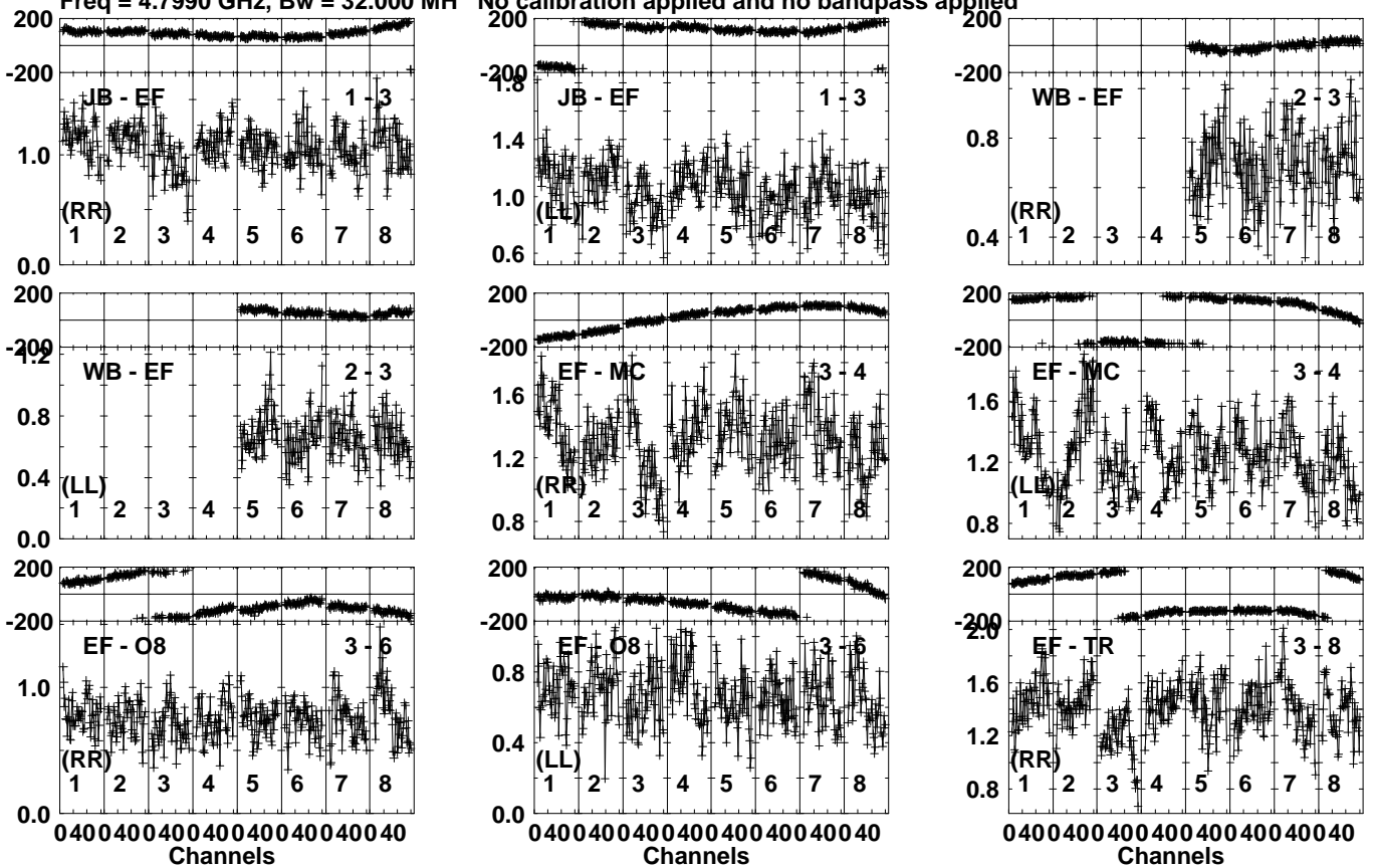
Lower frame: Milli Ampl Jy Top frame: Phas deg Vector averaged cross-power spectrum Several baselines displayed Timerange: 00:18:44:21 to 00:18:46:19
