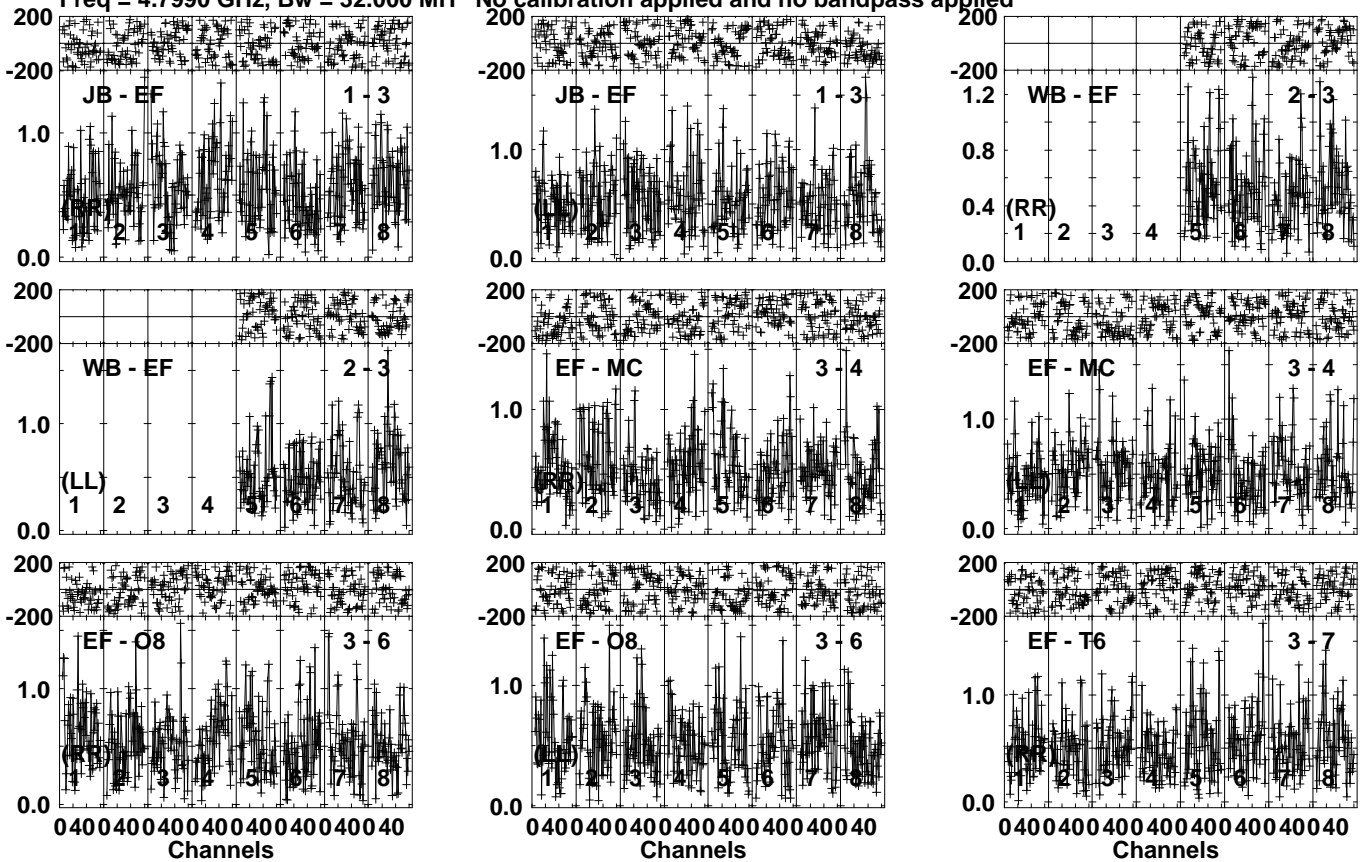
Lower frame: Milli Ampl Jy Top frame: Phas deg Vector averaged cross-power spectrum Several baselines displayed Timerange: 00/14:40:11 to 00/14:42:29
