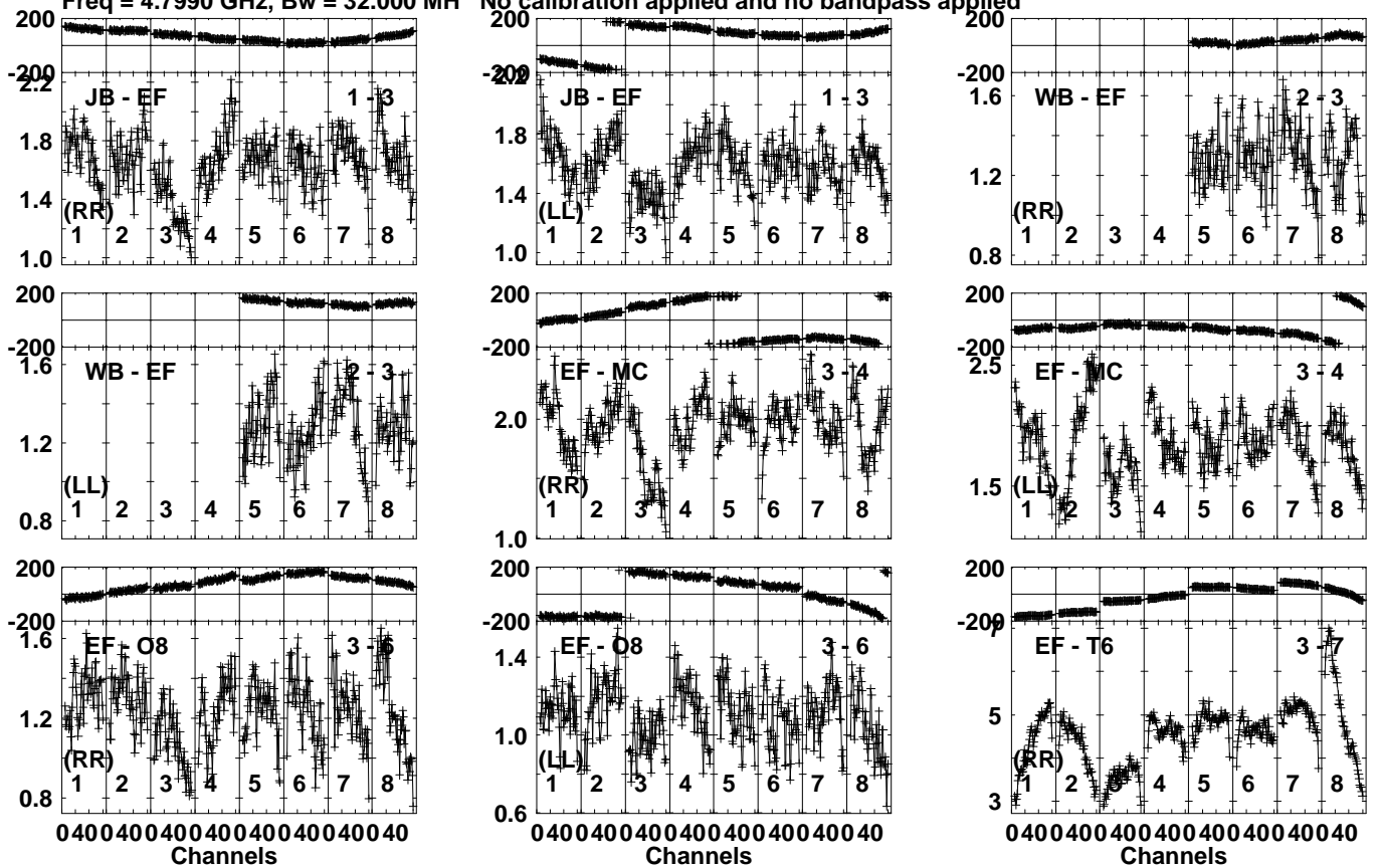
Lower frame: Milli Ampl Jy Top frame: Phas deg Vector averaged cross-power spectrum Several baselines displayed Timerange: 00:15:54:01 to 00:15:55:49
