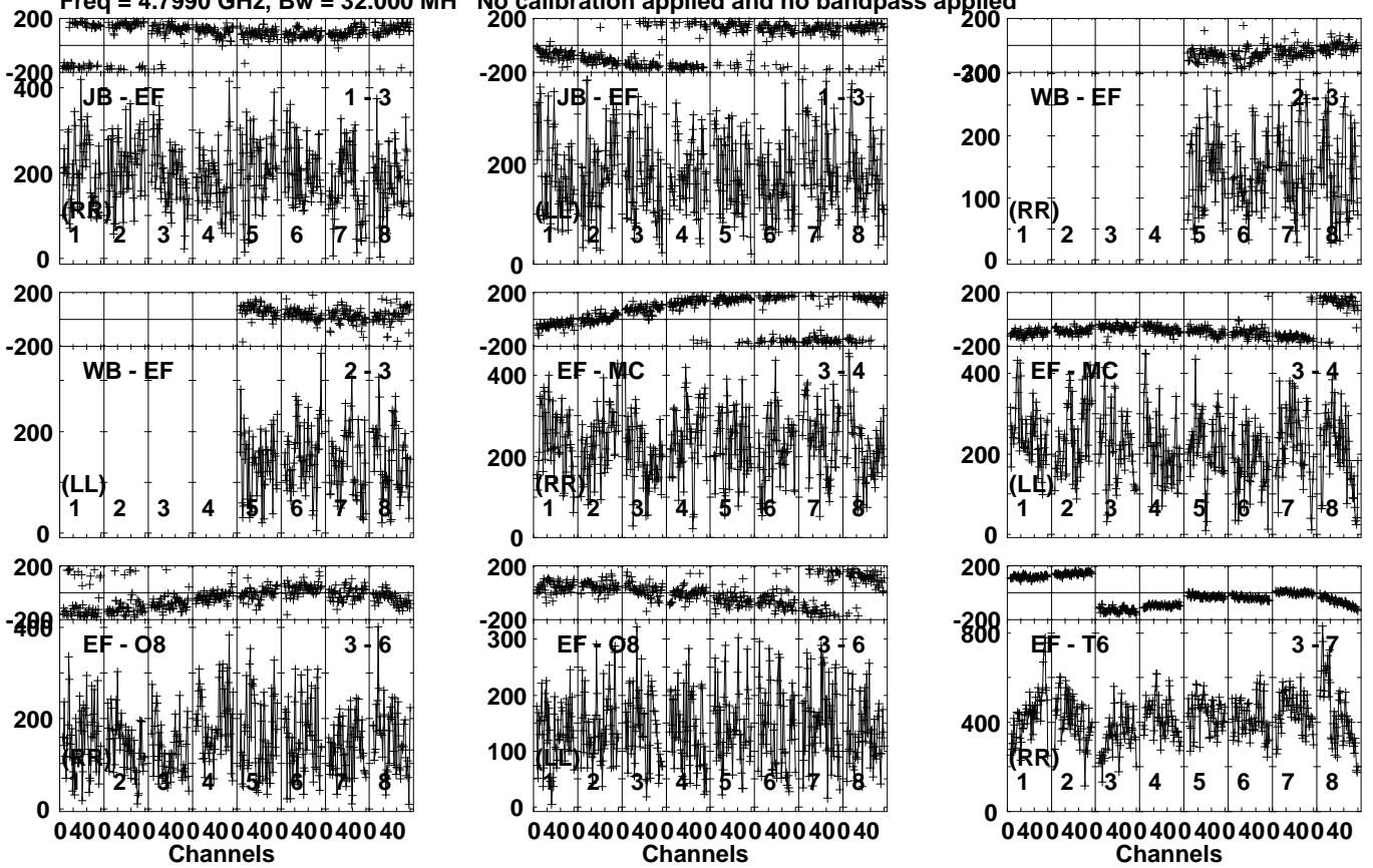
Lower frame: Micro Ampl Jy Top frame: Phas deg Vector averaged cross-power spectrum Several baselines displayed Timerange: 00/15:44:21 to 00/15:46:19
