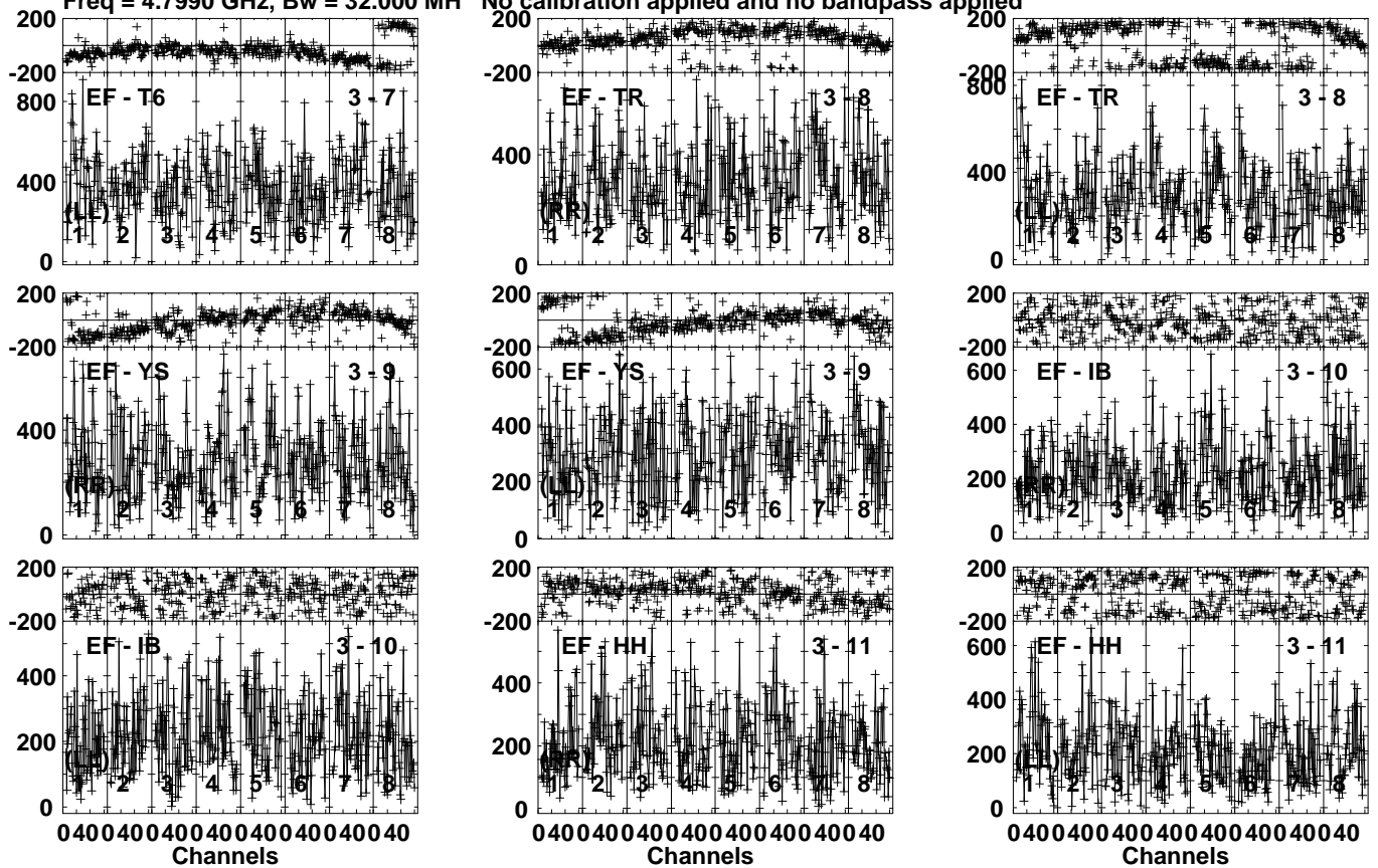
Lower frame: Micro Ampl Jy Top frame: Phas deg Vector averaged cross-power spectrum Several baselines displayed Timerange: 00/15:48:41 to 00/15:49:59
