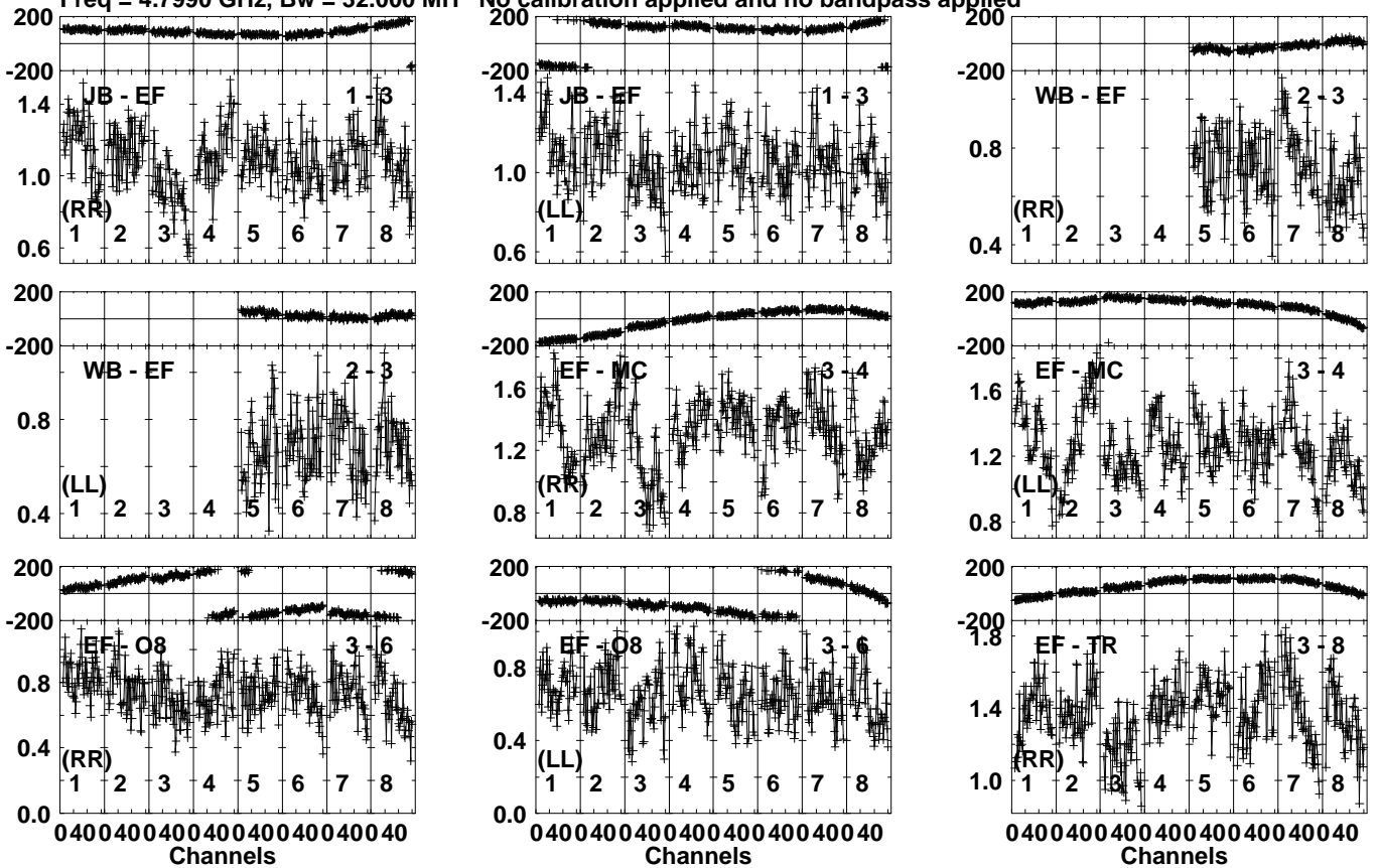
Lower frame: Milli Ampl Jy Top frame: Phas deg Vector averaged cross-power spectrum Several baselines displayed Timerange: 00/19:09:31 to 00/19:11:09
