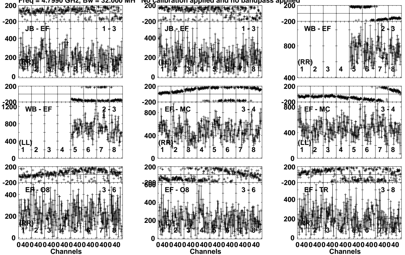
Lower frame: Micro Ampl Jy Top frame: Phas deg Vector averaged cross-power spectrum Several baselines displayed Timerange: 01/09:01:27 to 01/09:02:33
