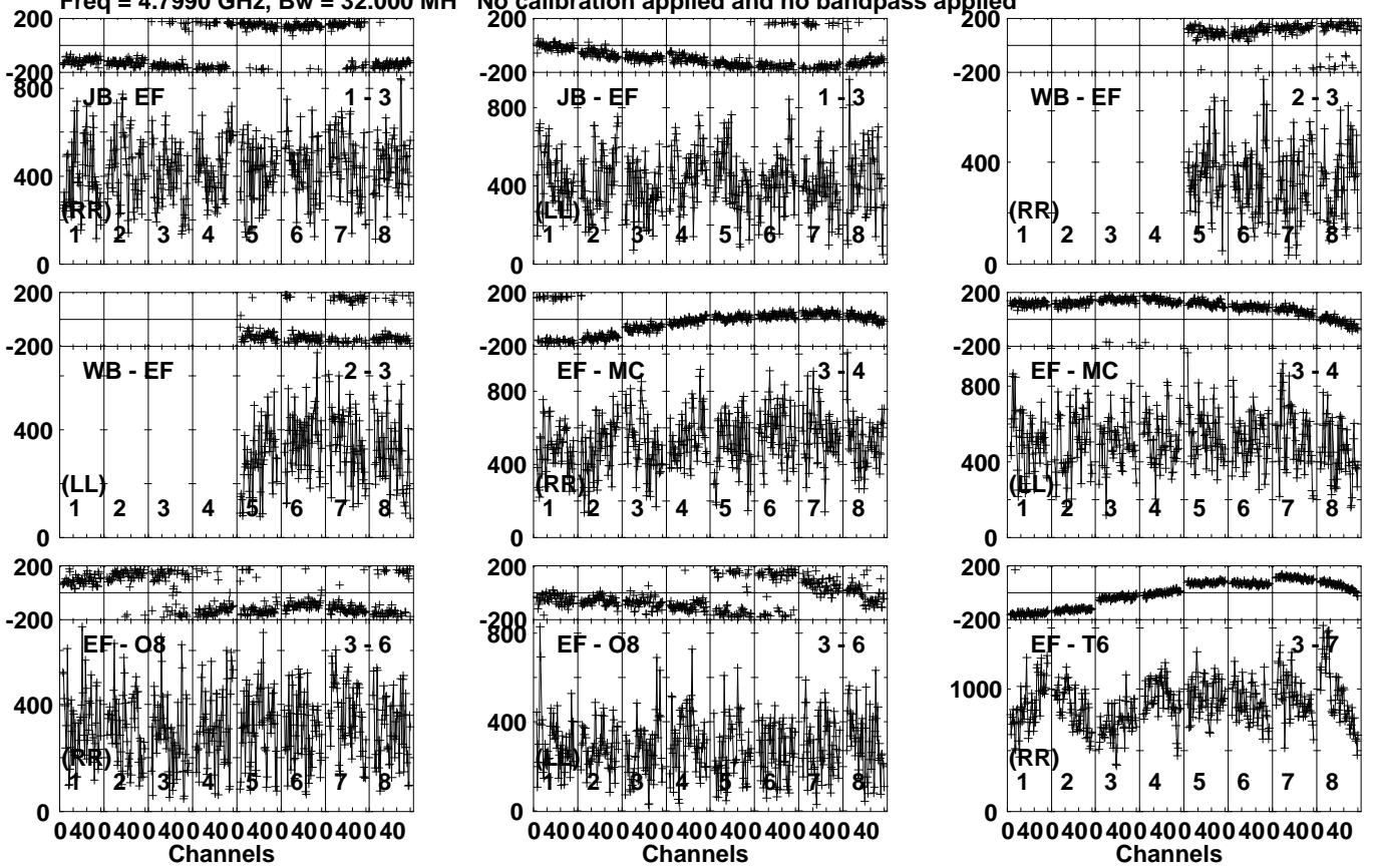
Lower frame: Micro Ampl Jy Top frame: Phas deg Vector averaged cross-power spectrum Several baselines displayed Timerange: 00/16:44:51 to 00/16:46:09
