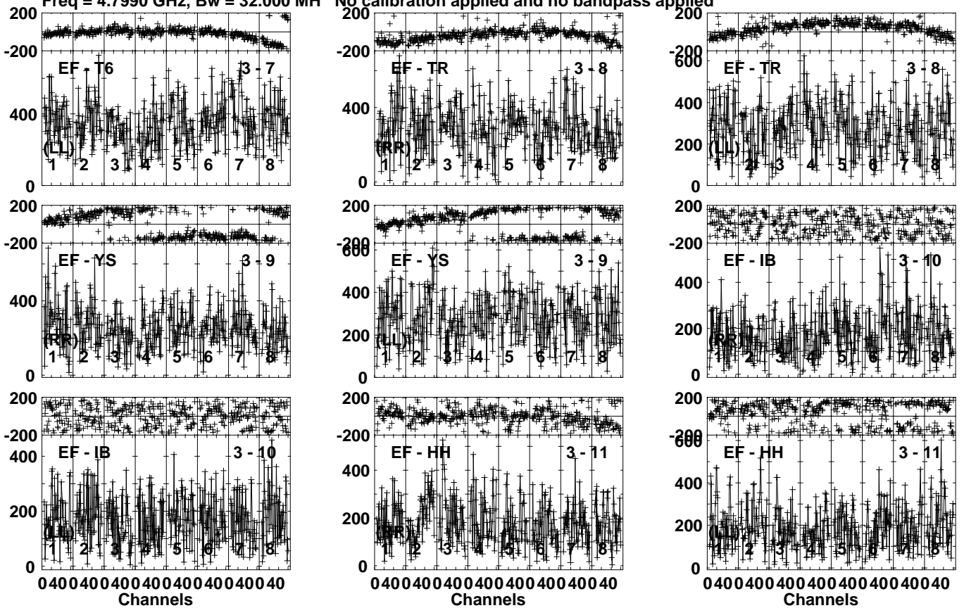
Lower frame: Micro Ampl Jy Top frame: Phas deg Vector averaged cross-power spectrum Several baselines displayed Timerange: 00/15:55:51 to 00/15:57:29
