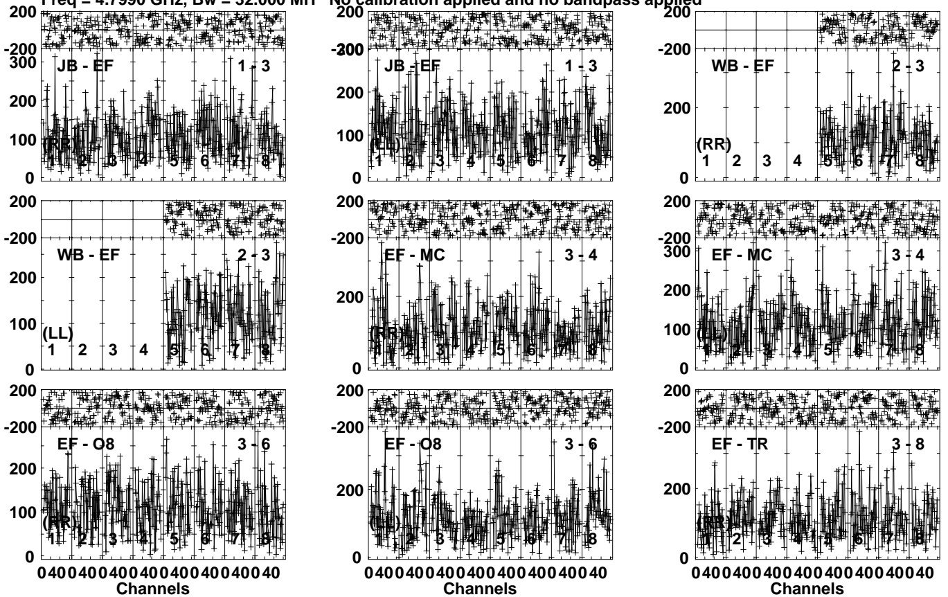
Lower frame: Micro Ampl Jy Top frame: Phas deg Vector averaged cross-power spectrum Several baselines displayed Timerange: 00/19:00:01 to 00/19:02:19
