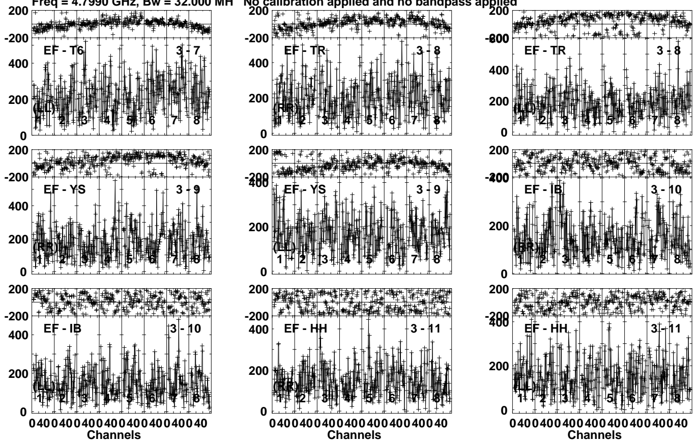
Lower frame: Micro Ampl Jy Top frame: Phas deg Vector averaged cross-power spectrum Several baselines displayed Timerange: 00/17:15:51 to 00/17:17:39
