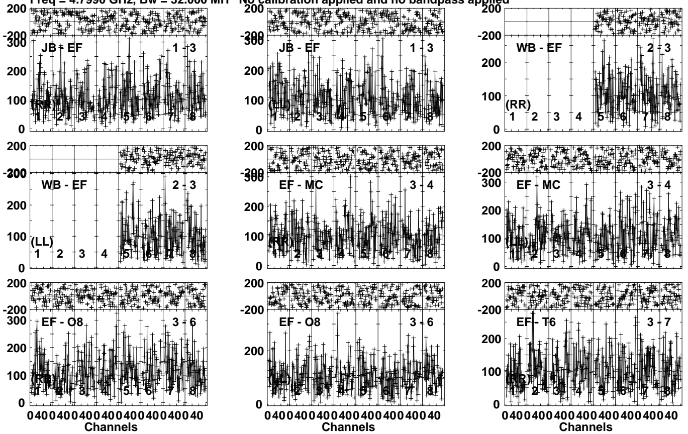
Lower frame: Micro Ampl Jy Top frame: Phas deg Vector averaged cross-power spectrum Several baselines displayed Timerange: 00/16:00:01 to 00/16:02:19
