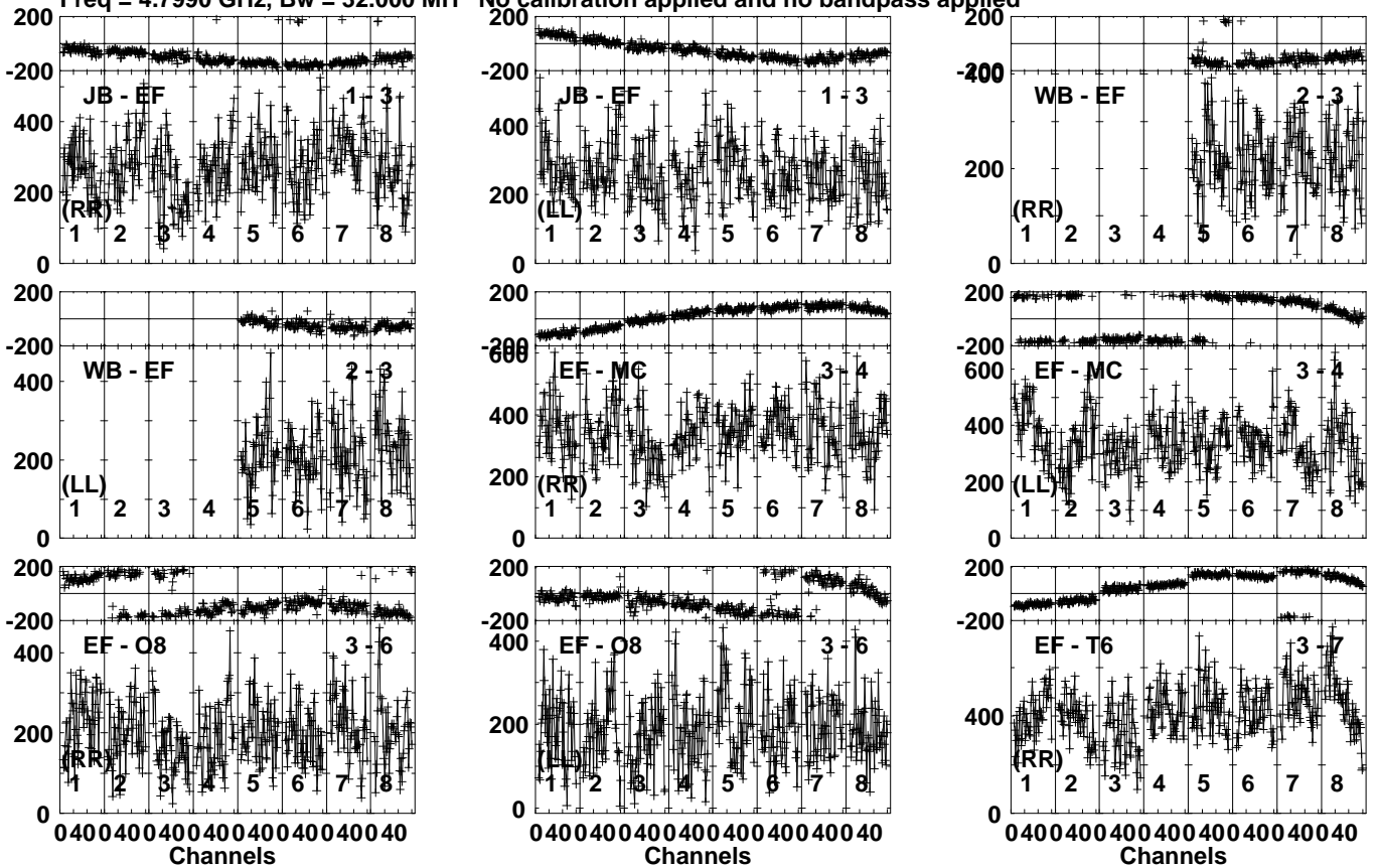
Lower frame: Micro Ampl Jy Top frame: Phas deg Vector averaged cross-power spectrum Several baselines displayed Timerange: 00/16:26:21 to 00/16:28:19
