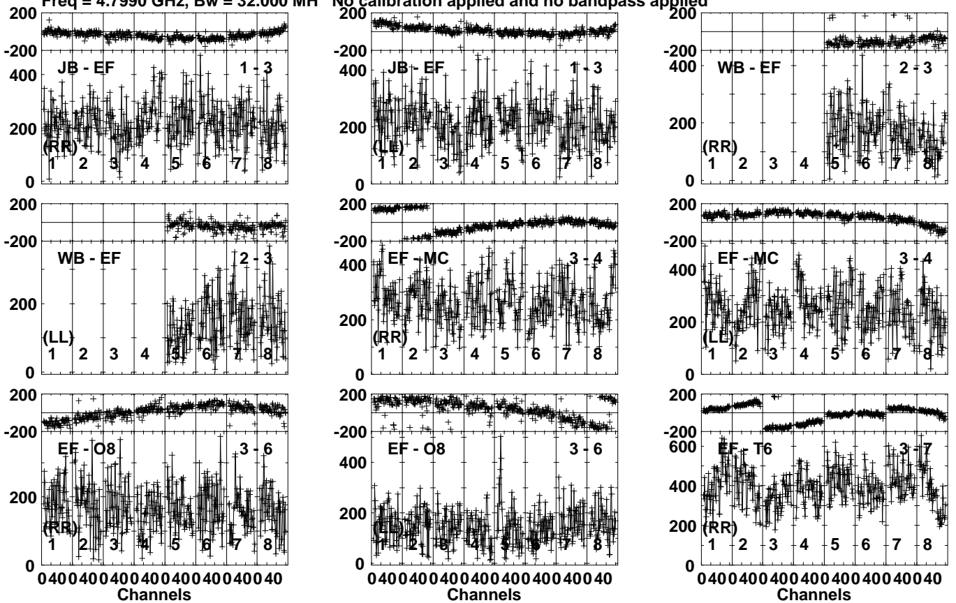
Lower frame: Micro Ampl Jy Top frame: Phas deg Vector averaged cross-power spectrum Several baselines displayed Timerange: 00/17:47:41 to 00/17:49:39
