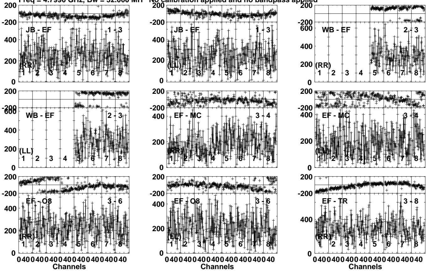
Lower frame: Micro Ampl Jy Top frame: Phas deg Vector averaged cross-power spectrum Several baselines displayed Timerange: 01/09:07:07 to 01/09:09:03
