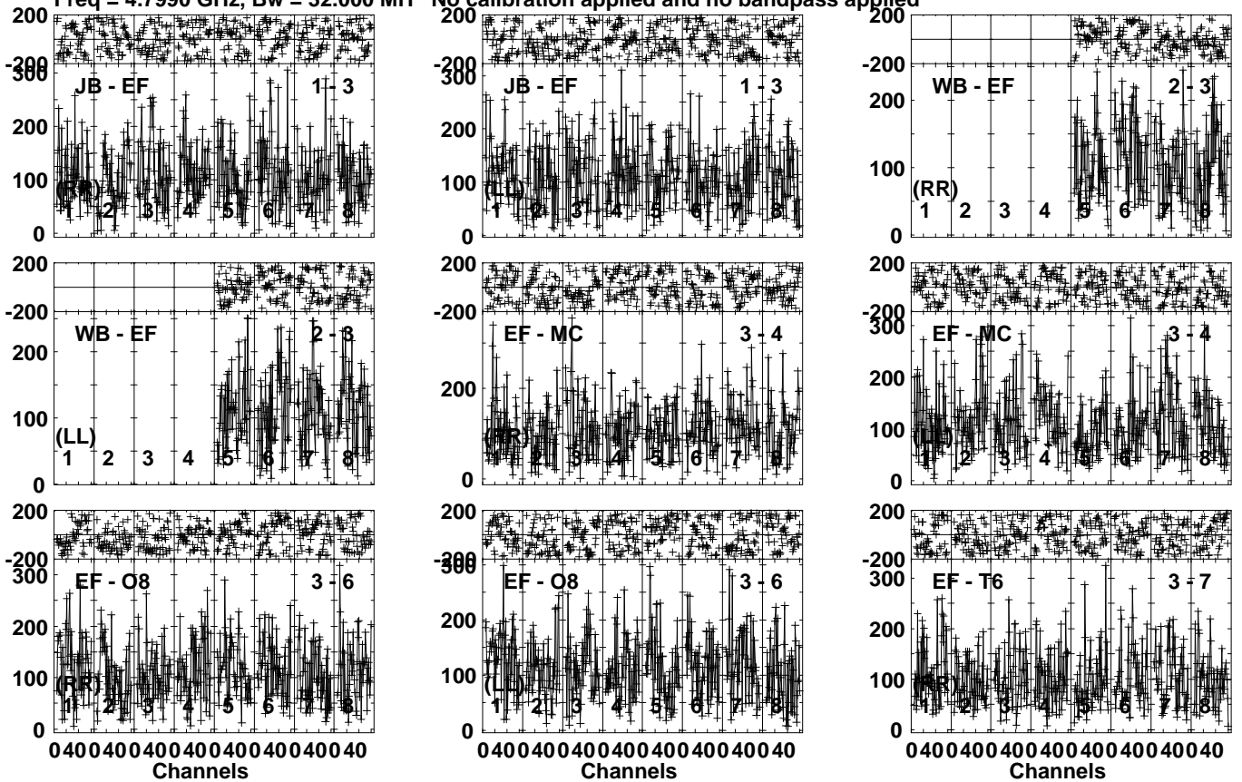
Lower frame: Micro Ampl Jy Top frame: Phas deg Vector averaged cross-power spectrum Several baselines displayed Timerange: 00/17:26:01 to 00/17:28:19
