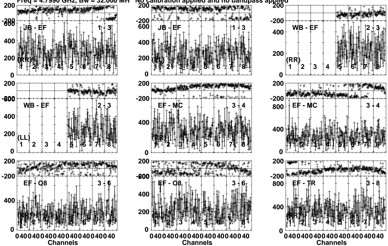
Lower frame: Micro Ampl Jy Top frame: Phas deg Vector averaged cross-power spectrum Several baselines displayed Timerange: 01/08:43:11 to 01/08:44:29
