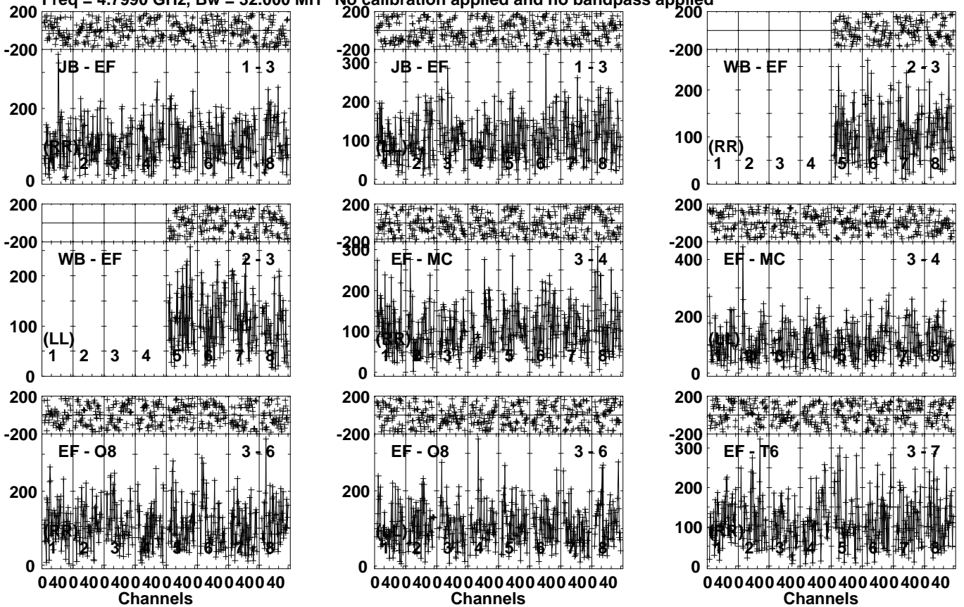
Lower frame: Micro Ampl Jy Top frame: Phas deg Vector averaged cross-power spectrum Several baselines displayed Timerange: 00/16:28:21 to 00/16:30:39
