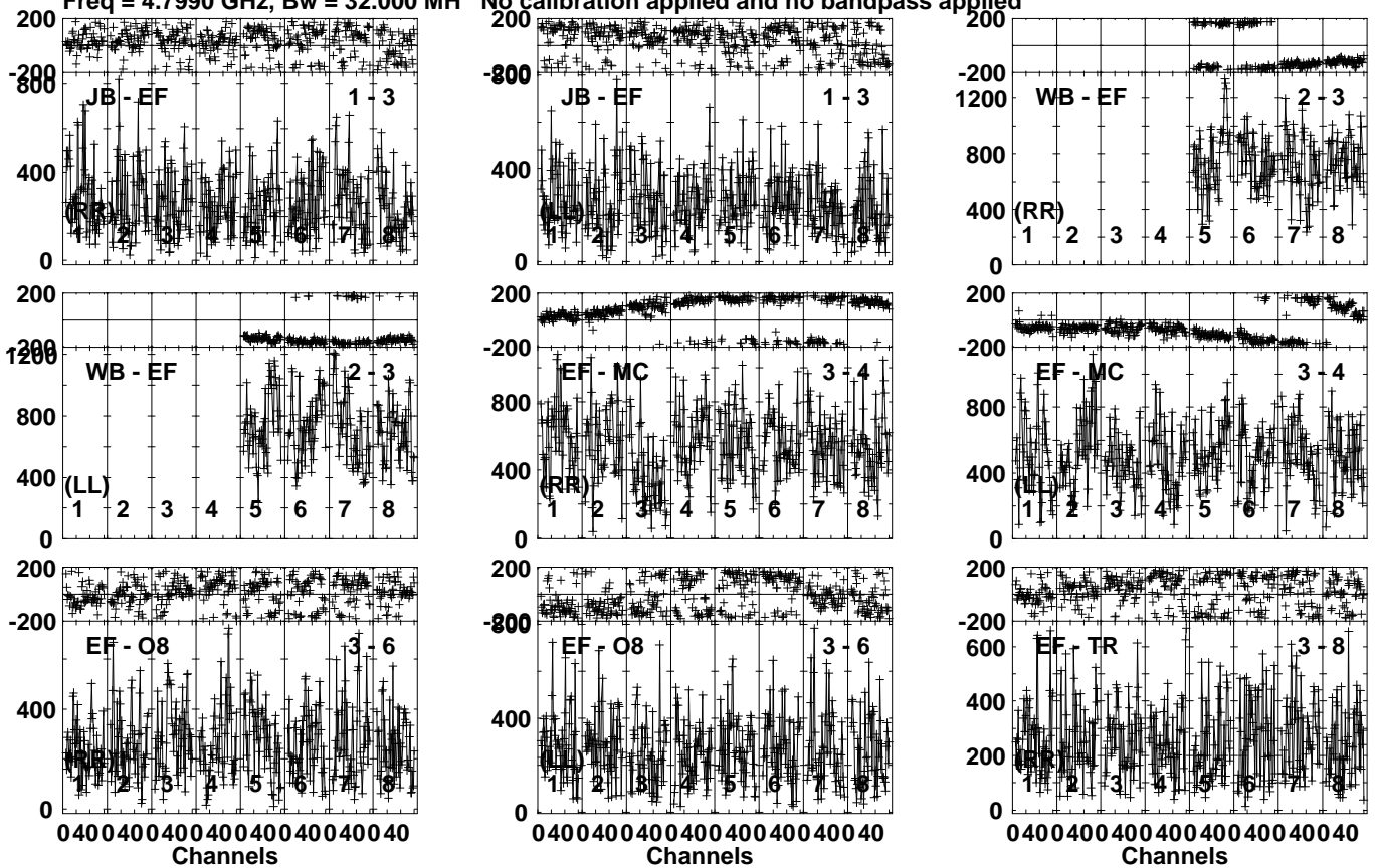
Lower frame: Micro Ampl Jy Top frame: Phas deg Vector averaged cross-power spectrum Several baselines displayed Timerange: 01/08:57:21 to 01/08:58:33
