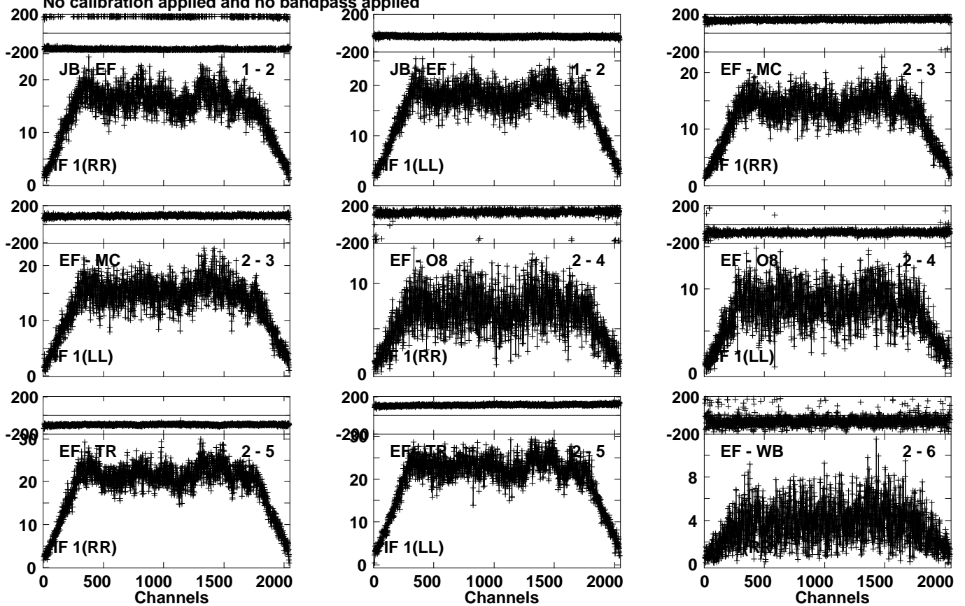
Lower frame: Milli Ampl Jy Top frame: Phas deg Vector averaged cross-power spectrum Several baselines displayed Timerange: 01/00:10:19 to 01/00:12:02
