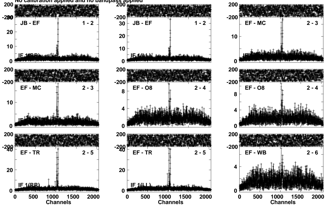
Lower frame: Milli Ampl Jy Top frame: Phas deg Vector averaged cross-power spectrum Several baselines displayed Timerange: 01/05:31:20 to 01/05:34:33
