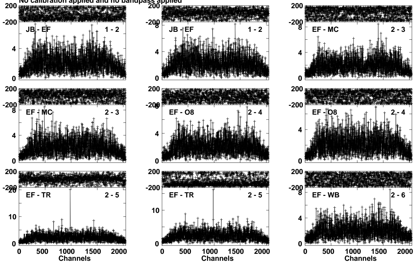
Lower frame: Milli Ampl Jy Top frame: Phas deg Vector averaged cross-power spectrum Several baselines displayed Timerange: 01/01:08:07 to 01/01:09:56
