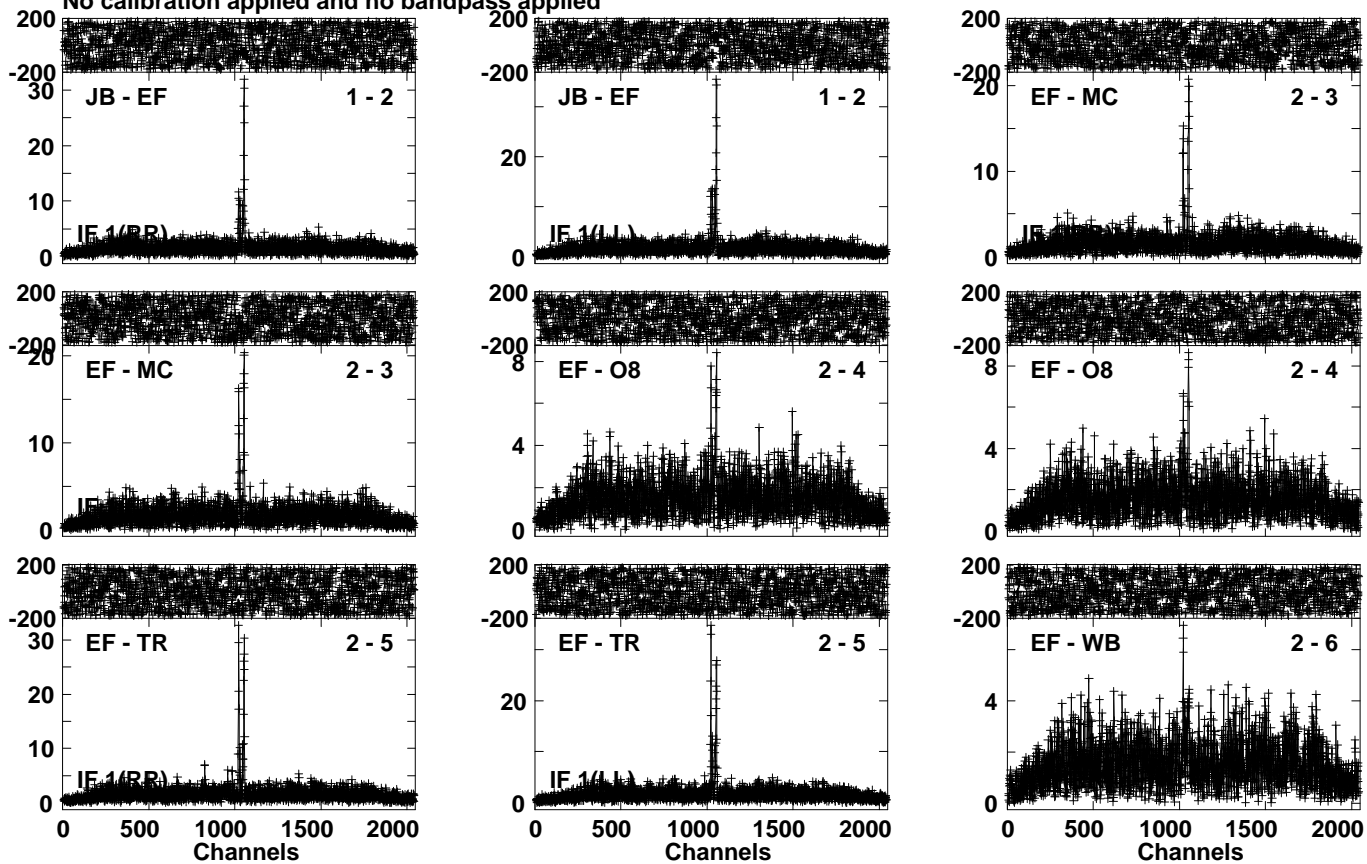
Lower frame: Milli Ampl Jy Top frame: Phas deg Vector averaged cross-power spectrum Several baselines displayed Timerange: 01/07:15:40 to 01/07:18:49
