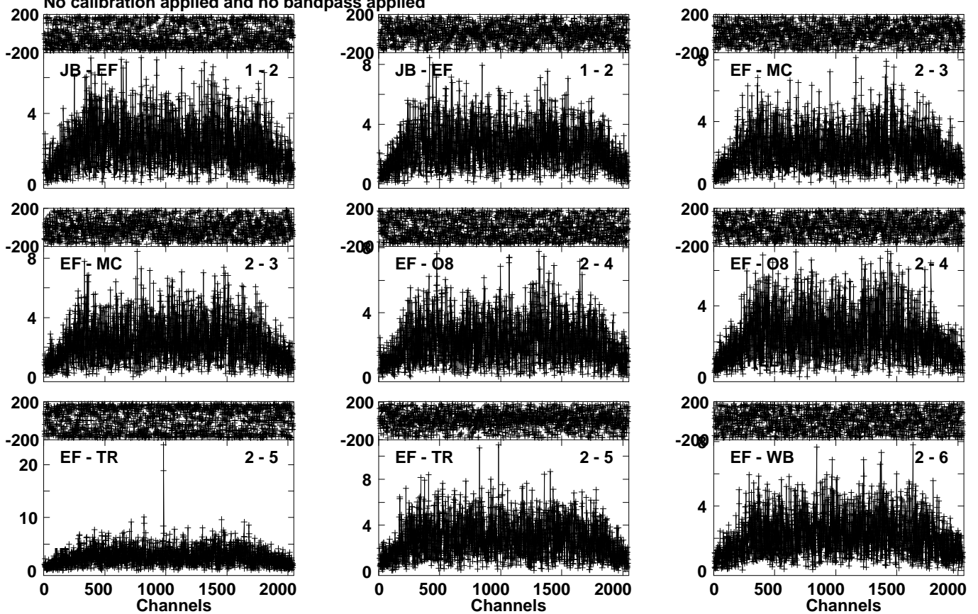
Lower frame: Milli Ampl Jy Top frame: Phas deg Vector averaged cross-power spectrum Several baselines displayed Timerange: 00/23:39:09 to 00/23:40:52
