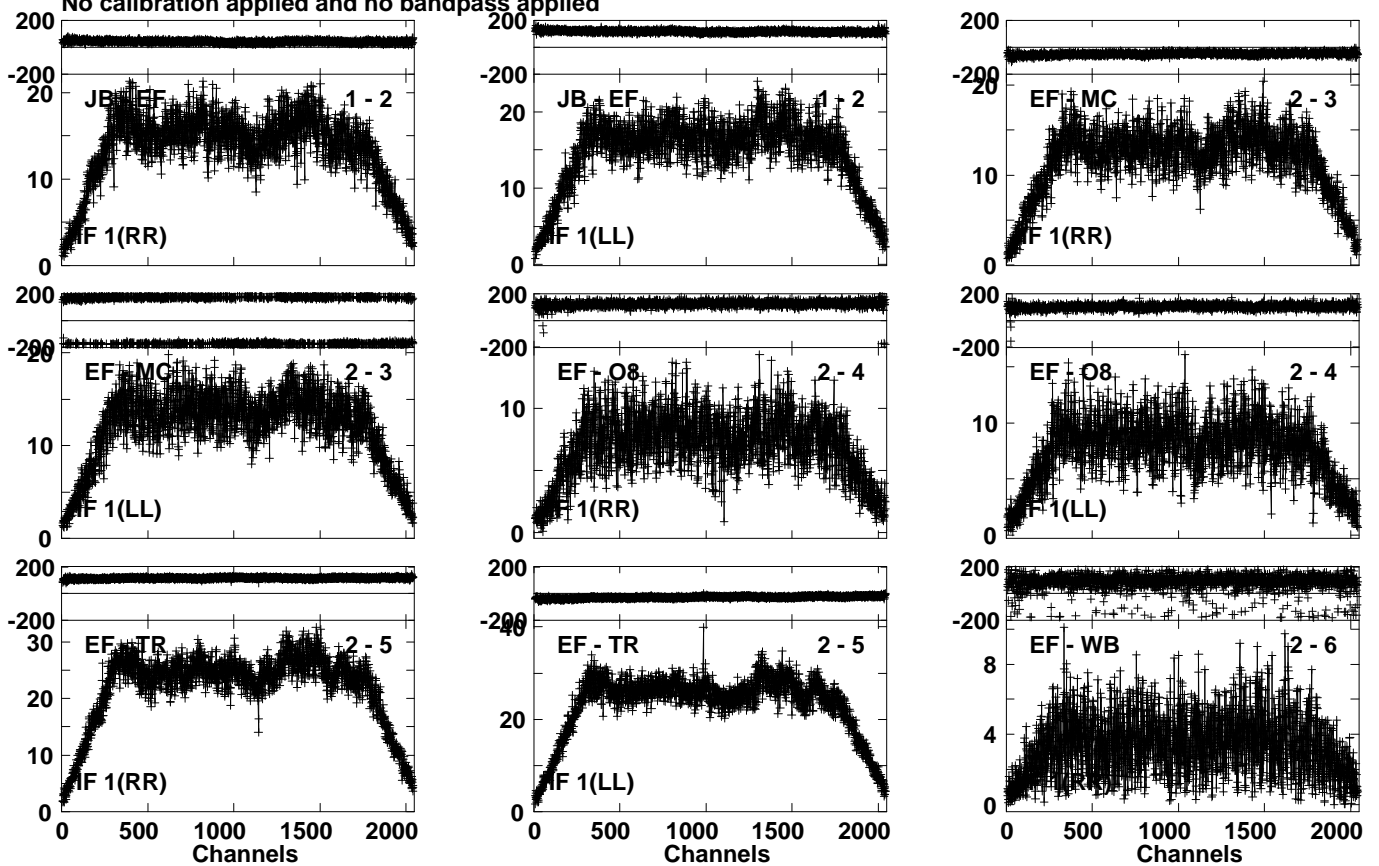
Lower frame: Milli Ampl Jy Top frame: Phas deg Vector averaged cross-power spectrum Several baselines displayed Timerange: 01/03:53:02 to 01/03:54:45
