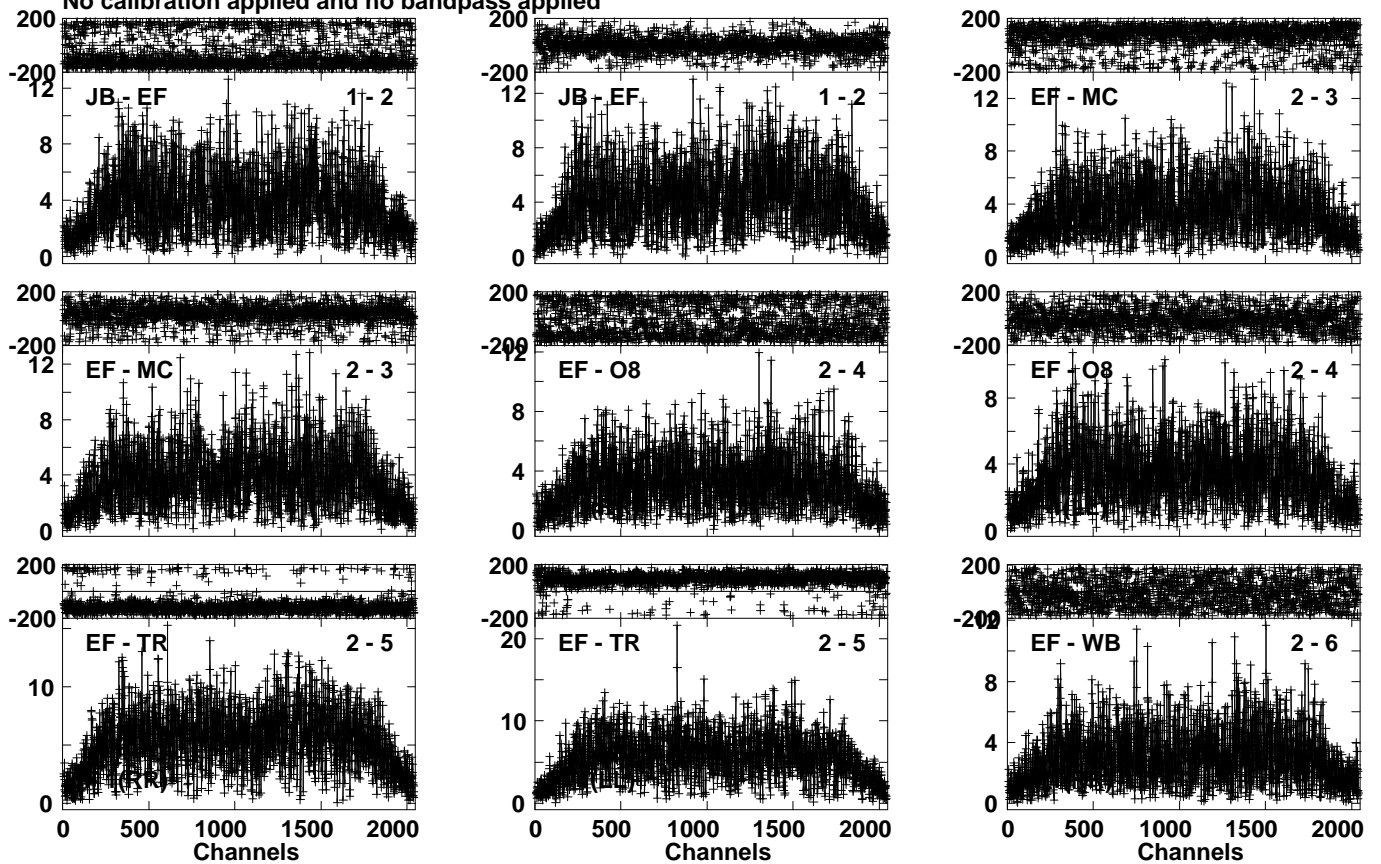
Lower frame: Milli Ampl Jy Top frame: Phas deg Vector averaged cross-power spectrum Several baselines displayed Timerange: 00/23:45:54 to 00/23:47:37
