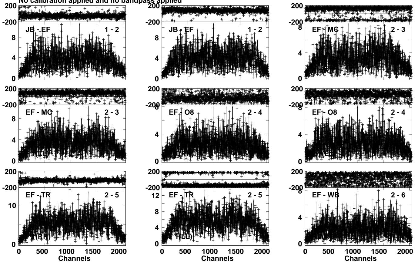
Lower frame: Milli Ampl Jy Top frame: Phas deg Vector averaged cross-power spectrum Several baselines displayed Timerange: 01/01:05:34 to 01/01:07:17
