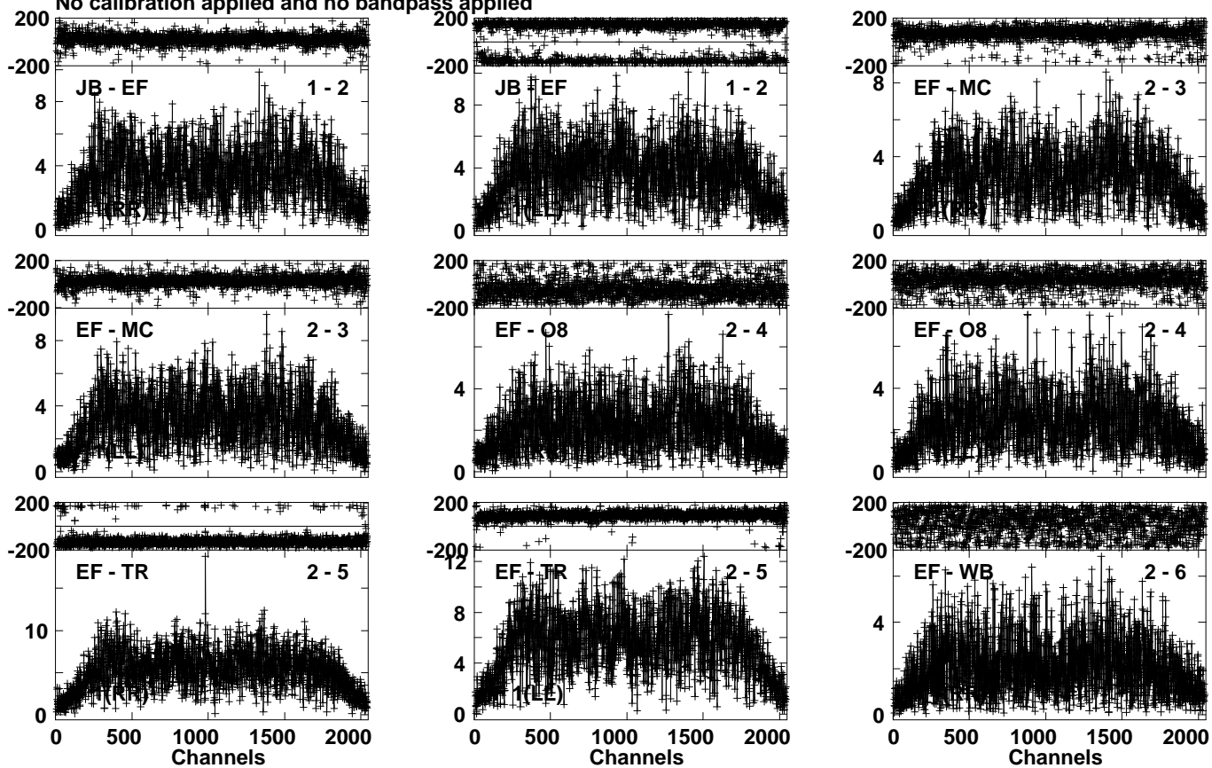
Lower frame: Milli Ampl Jy Top frame: Phas deg Vector averaged cross-power spectrum Several baselines displayed Timerange: 01/00:55:04 to 01/00:56:47
