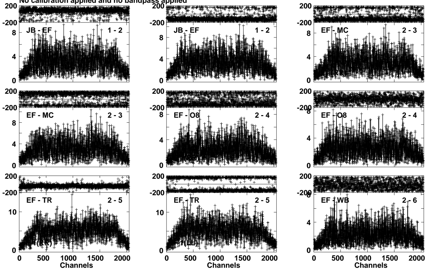
Lower frame: Milli Ampl Jy Top frame: Phas deg Vector averaged cross-power spectrum Several baselines displayed Timerange: 00/22:44:53 to 00/22:46:36
