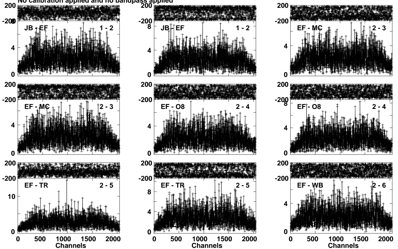
Lower frame: Milli Ampl Jy Top frame: Phas deg Vector averaged cross-power spectrum Several baselines displayed Timerange: 01/06:51:22 to 01/06:53:05
