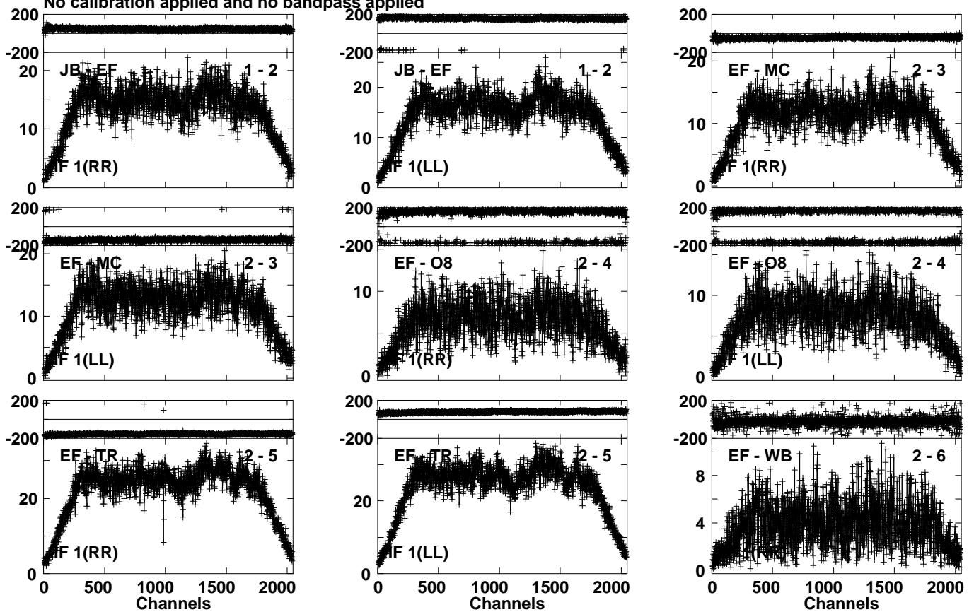
Lower frame: Milli Ampl Jy Top frame: Phas deg Vector averaged cross-power spectrum Several baselines displayed Timerange: 01/05:55:10 to 01/05:56:53
