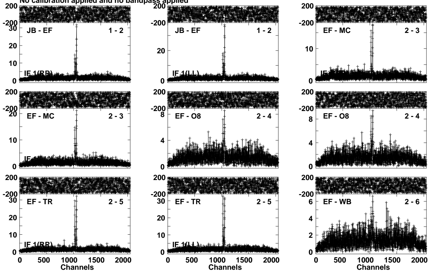
Lower frame: Milli Ampl Jy Top frame: Phas deg Vector averaged cross-power spectrum Several baselines displayed Timerange: 01/07:00:22 to 01/07:03:36
