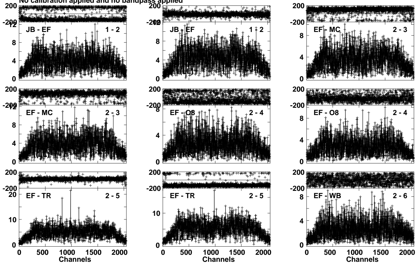
Lower frame: Milli Ampl Jy Top frame: Phas deg Vector averaged cross-power spectrum Several baselines displayed Timerange: 01/02:54:27 to 01/02:56:10
