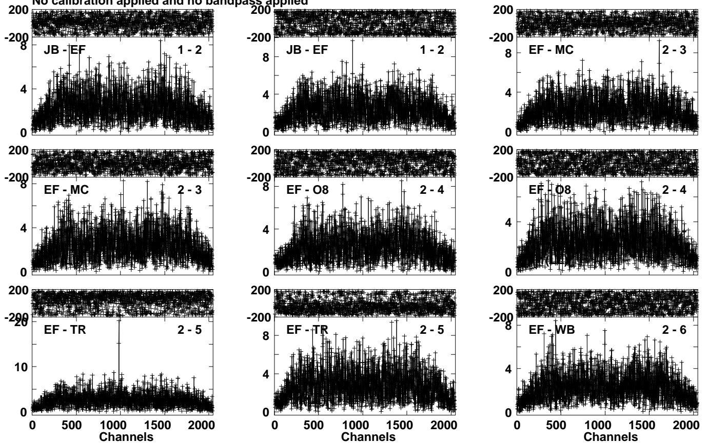
Lower frame: Milli Ampl Jy Top frame: Phas deg Vector averaged cross-power spectrum Several baselines displayed Timerange: 01/02:26:08 to 01/02:27:51
