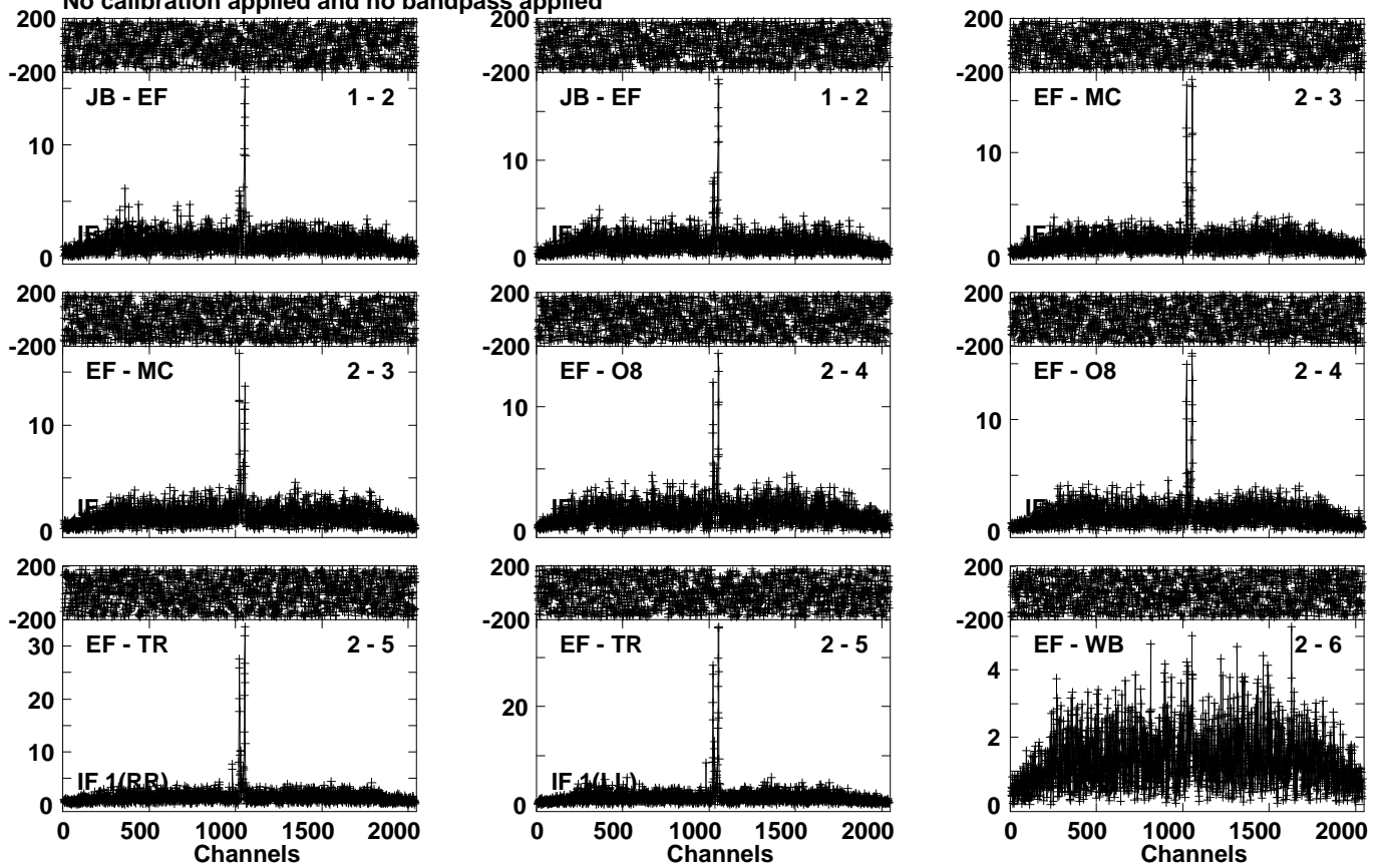
Lower frame: Milli Ampl Jy Top frame: Phas deg Vector averaged cross-power spectrum Several baselines displayed Timerange: 00/23:48:09 to 00/23:51:22
