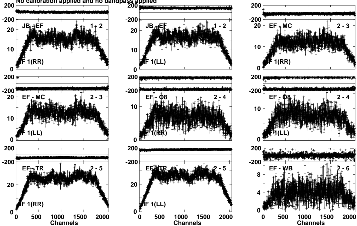
Lower frame: Milli Ampl Jy Top frame: Phas deg Vector averaged cross-power spectrum Several baselines displayed Timerange: 01/06:05:40 to 01/06:07:23
