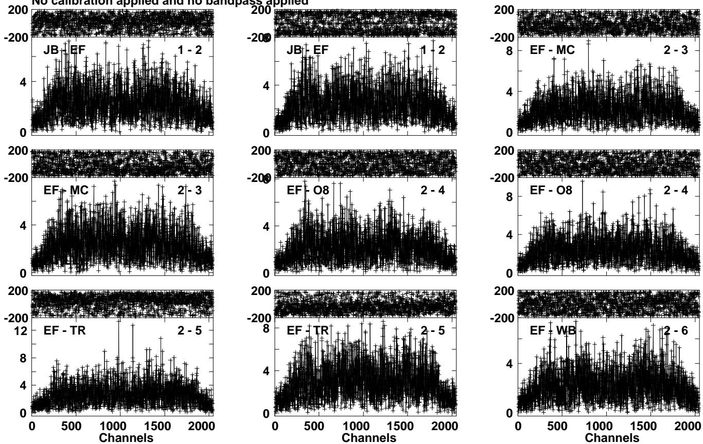
Lower frame: Milli Ampl Jy Top frame: Phas deg Vector averaged cross-power spectrum Several baselines displayed Timerange: 01/01:34:42 to 01/01:36:25
