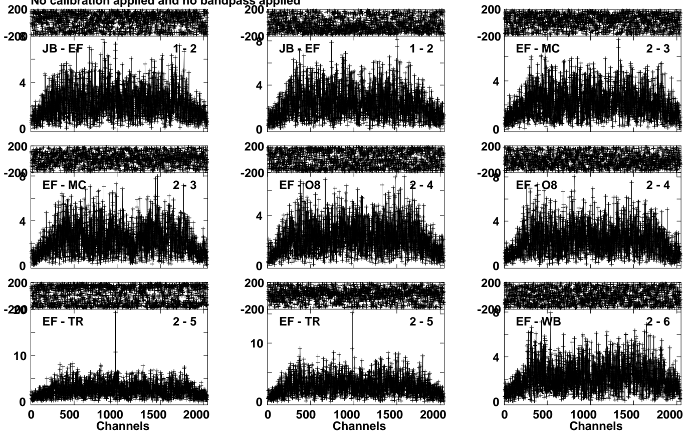
Lower frame: Milli Ampl Jy Top frame: Phas deg Vector averaged cross-power spectrum Several baselines displayed Timerange: 00/22:32:08 to 00/22:33:51
