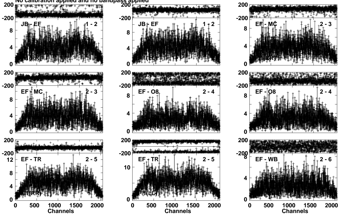
Lower frame: Milli Ampl Jy Top frame: Phas deg Vector averaged cross-power spectrum Several baselines displayed Timerange: 01/02:49:27 to 01/02:51:10
