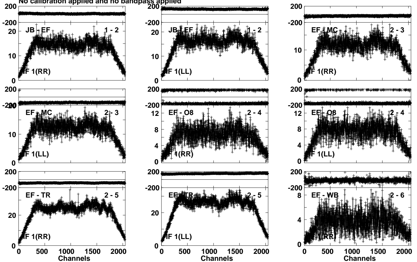
Lower frame: Milli Ampl Jy Top frame: Phas deg Vector averaged cross-power spectrum Several baselines displayed Timerange: 01/06:00:40 to 01/06:02:23
