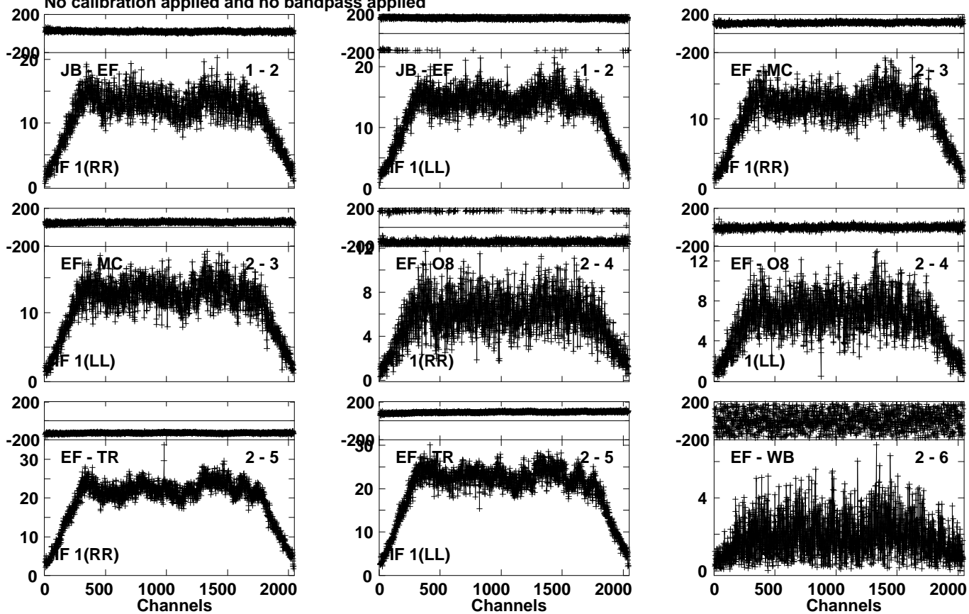
Lower frame: Milli Ampl Jy Top frame: Phas deg Vector averaged cross-power spectrum Several baselines displayed Timerange: 00/21:37:01 to 00/21:38:44
