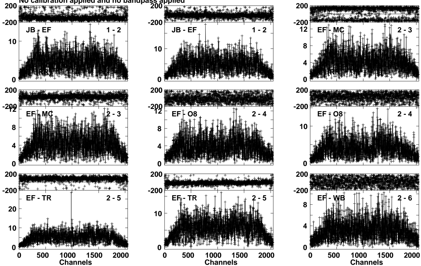
Lower frame: Milli Ampl Jy Top frame: Phas deg Vector averaged cross-power spectrum Several baselines displayed Timerange: 01/05:24:05 to 01/05:25:48
