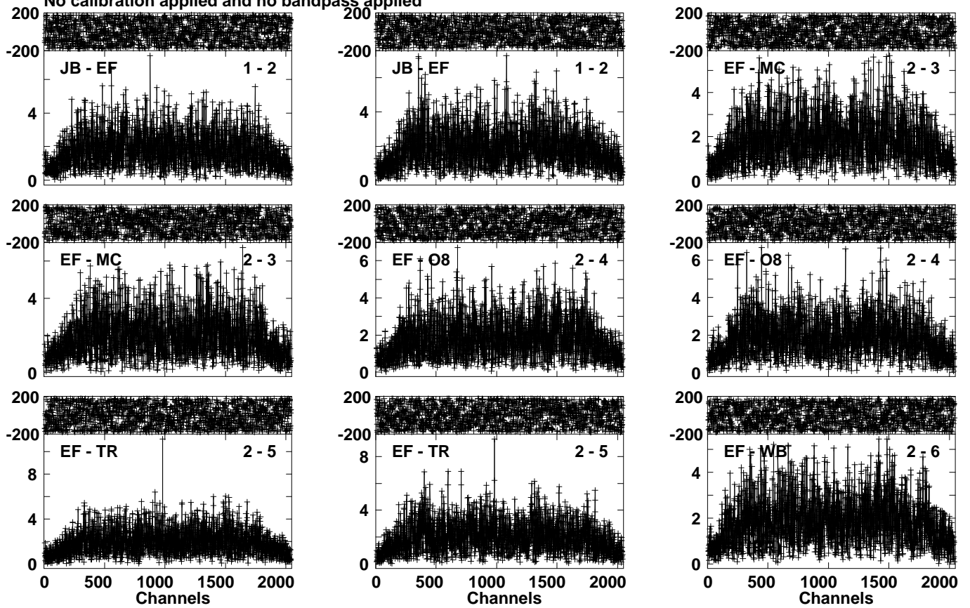
Lower frame: Milli Ampl Jy Top frame: Phas deg Vector averaged cross-power spectrum Several baselines displayed Timerange: 00/23:19:48 to 00/23:21:31
