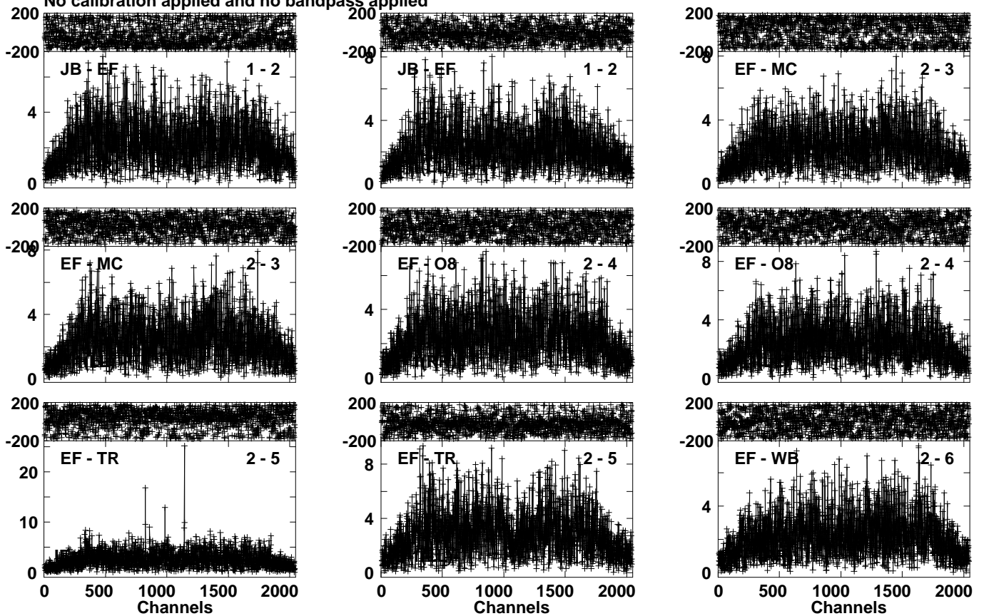
Lower frame: Milli Ampl Jy Top frame: Phas deg Vector averaged cross-power spectrum Several baselines displayed Timerange: 01/05:22:20 to 01/05:24:03
