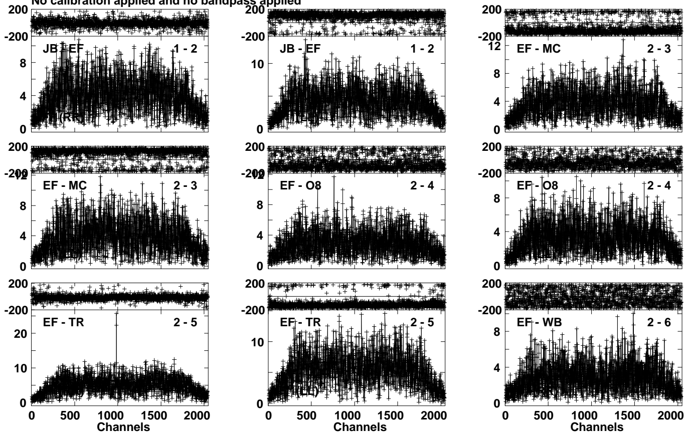
Lower frame: Milli Ampl Jy Top frame: Phas deg Vector averaged cross-power spectrum Several baselines displayed Timerange: 01/06:58:07 to 01/06:59:50
