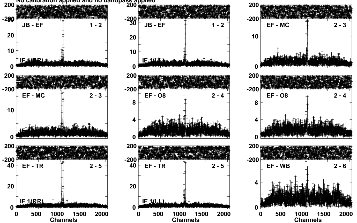
Lower frame: Milli Ampl Jy Top frame: Phas deg Vector averaged cross-power spectrum Several baselines displayed Timerange: 01/05:26:20 to 01/05:29:33
