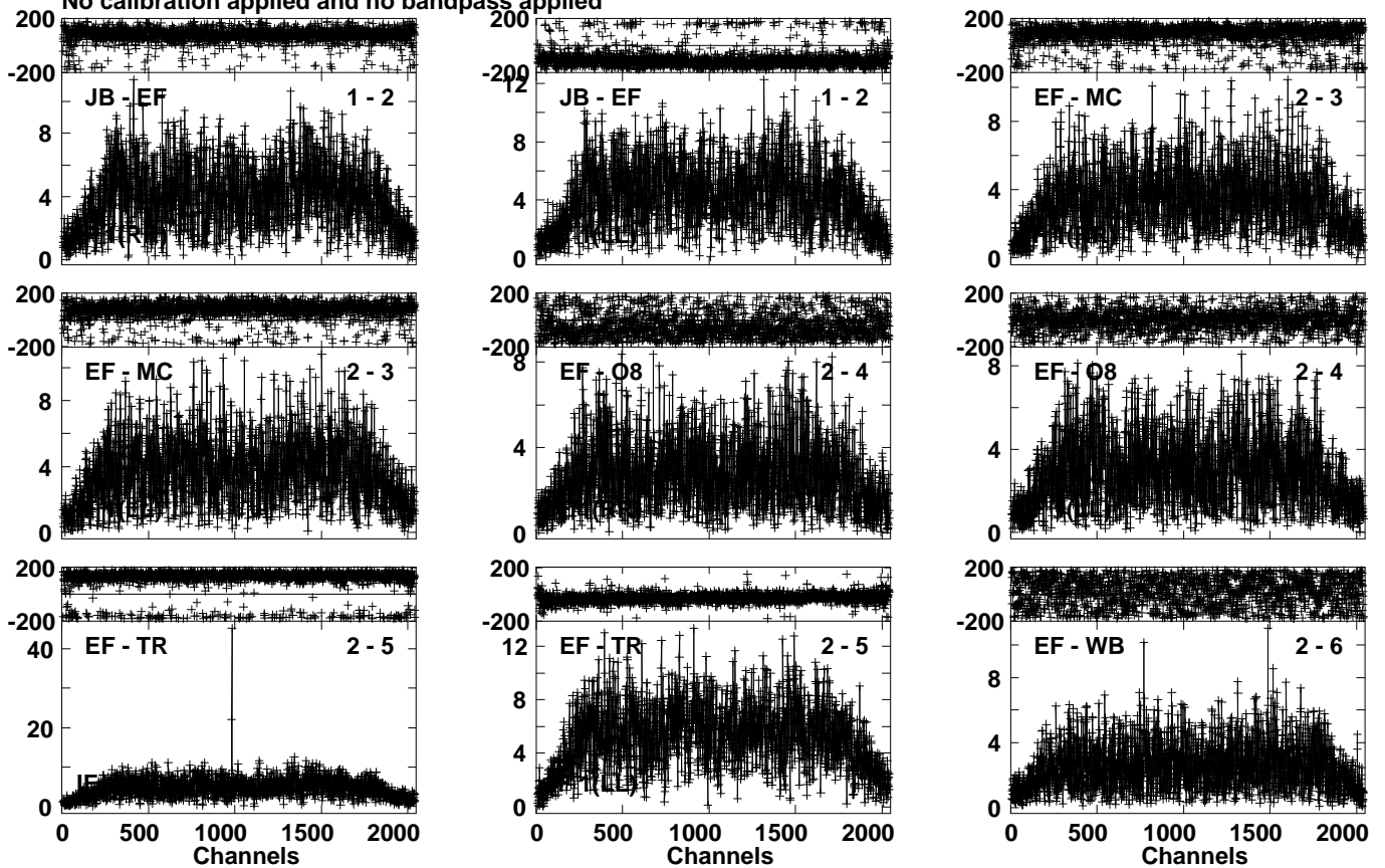
Lower frame: Milli Ampl Jy Top frame: Phas deg Vector averaged cross-power spectrum Several baselines displayed Timerange: 01/03:04:57 to 01/03:06:40
