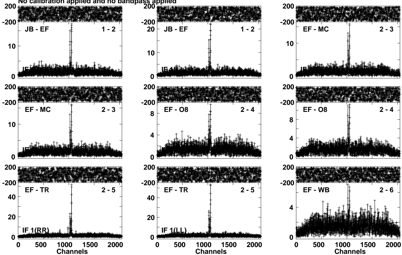
Lower frame: Milli Ampl Jy Top frame: Phas deg Vector averaged cross-power spectrum Several baselines displayed Timerange: 01/02:46:12 to 01/02:49:25
