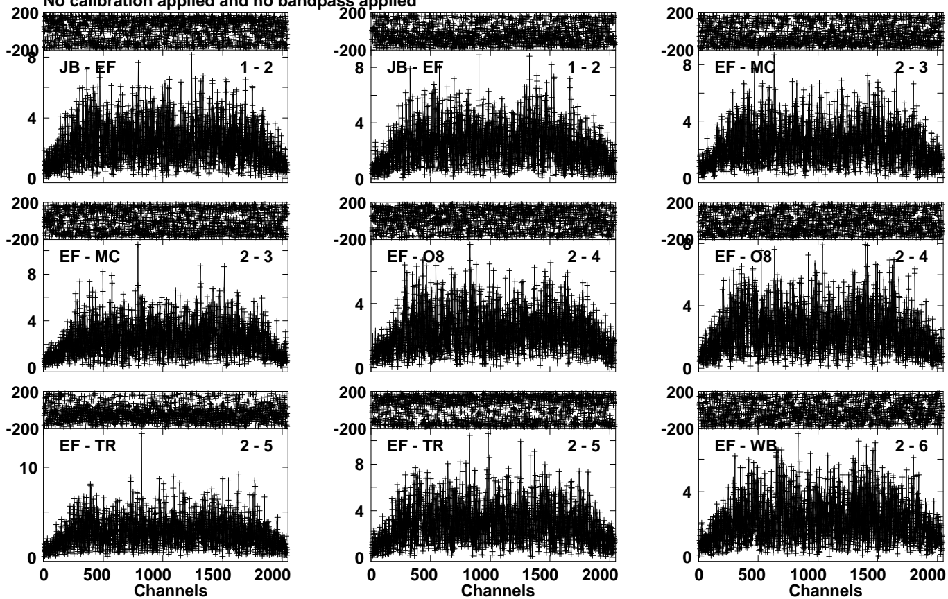
Lower frame: Milli Ampl Jy Top frame: Phas deg Vector averaged cross-power spectrum Several baselines displayed Timerange: 01/01:24:12 to 01/01:25:55
