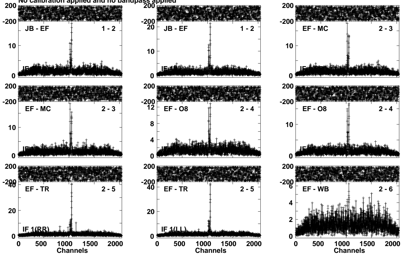
Lower frame: Milli Ampl Jy Top frame: Phas deg Vector averaged cross-power spectrum Several baselines displayed Timerange: 01/00:57:19 to 01/01:00:32
