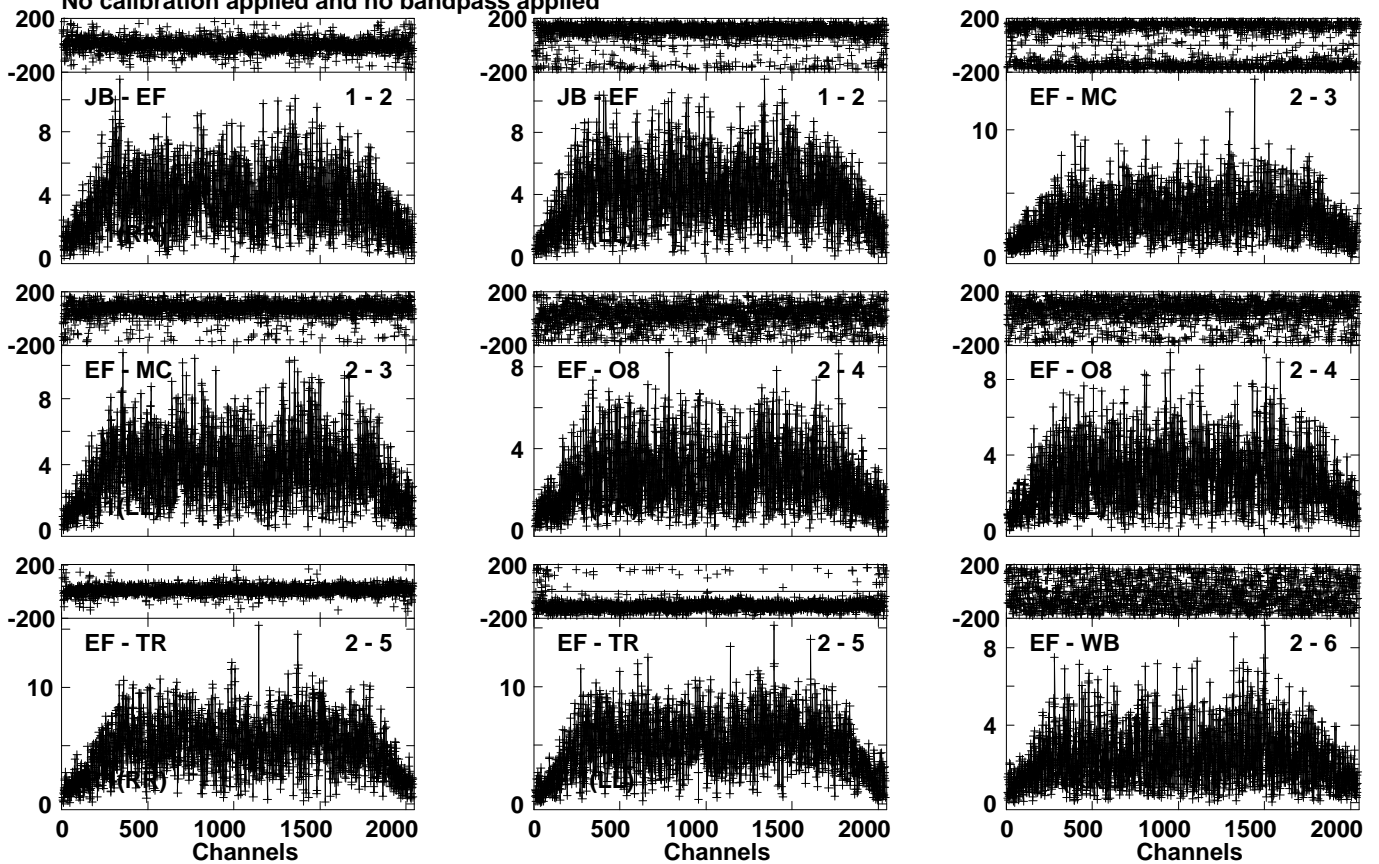
Lower frame: Milli Ampl Jy Top frame: Phas deg Vector averaged cross-power spectrum Several baselines displayed Timerange: 01/07:13:56 to 01/07:15:39
