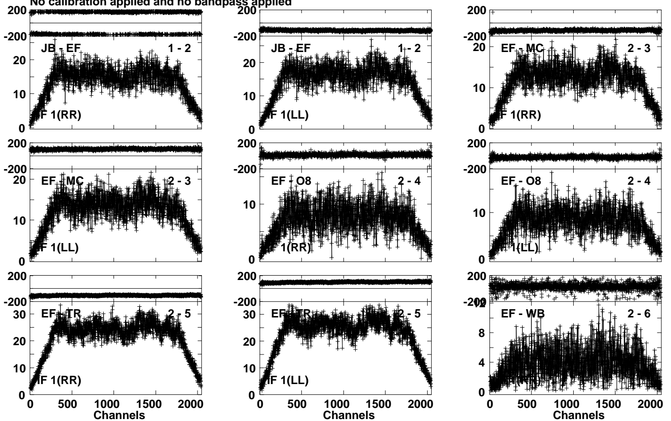
Lower frame: Milli Ampl Jy Top frame: Phas deg Vector averaged cross-power spectrum Several baselines displayed Timerange: 01/03:37:02 to 01/03:38:46
