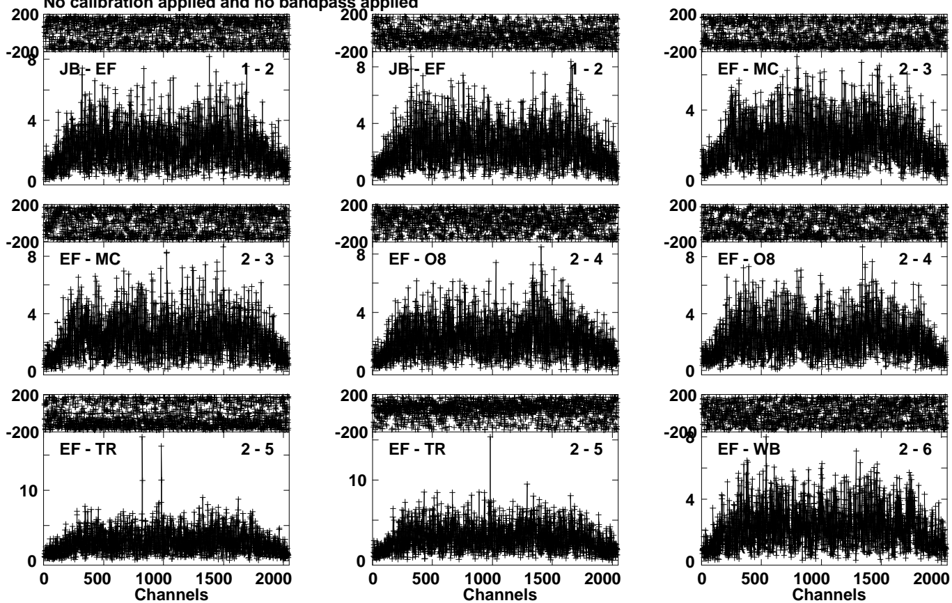
Lower frame: Milli Ampl Jy Top frame: Phas deg Vector averaged cross-power spectrum Several baselines displayed Timerange: 01/01:18:42 to 01/01:20:25
