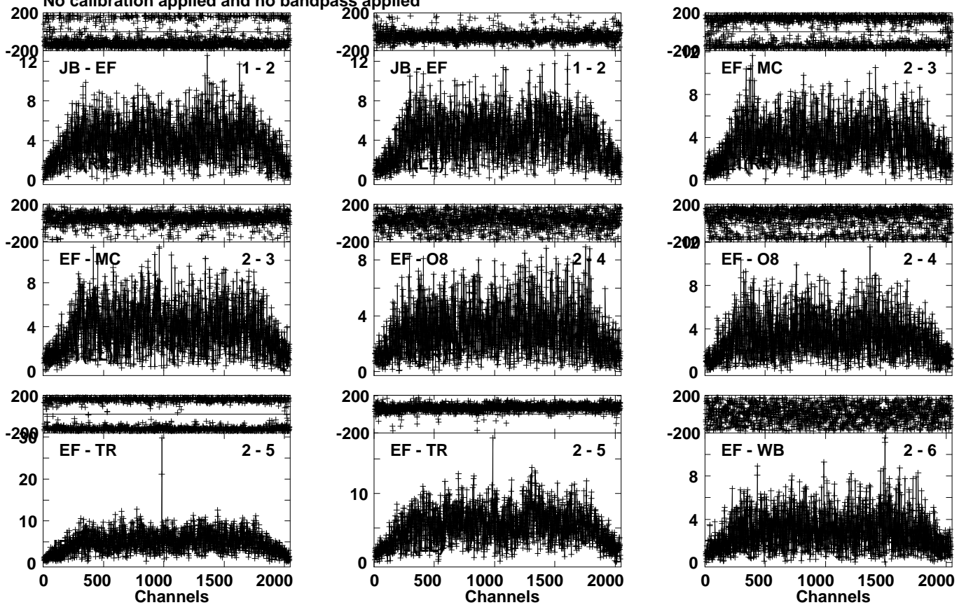
Lower frame: Milli Ampl Jy Top frame: Phas deg Vector averaged cross-power spectrum Several baselines displayed Timerange: 01/05:34:35 to 01/05:36:18
