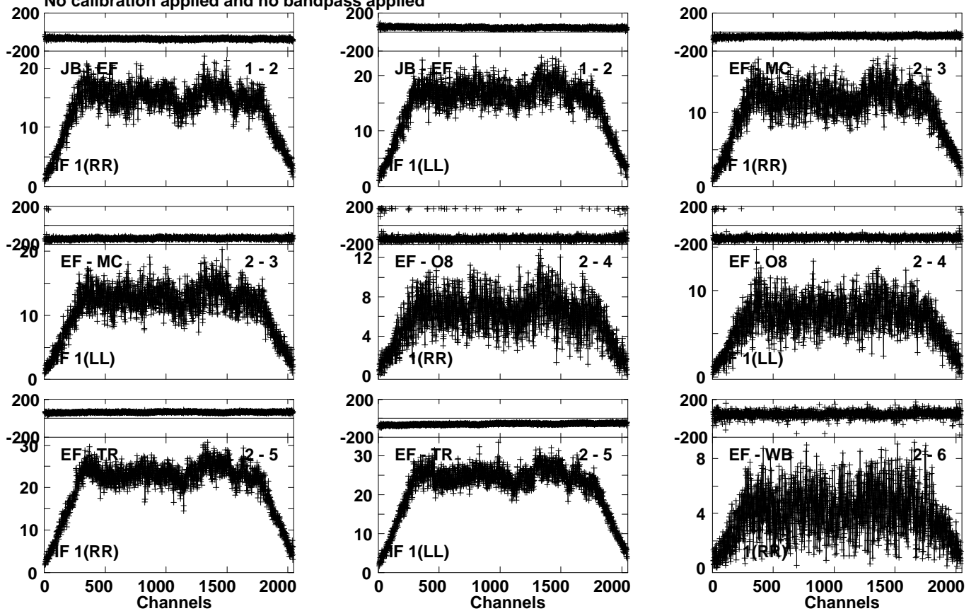
Lower frame: Milli Ampl Jy Top frame: Phas deg Vector averaged cross-power spectrum Several baselines displayed Timerange: 01/06:32:10 to 01/06:33:53
