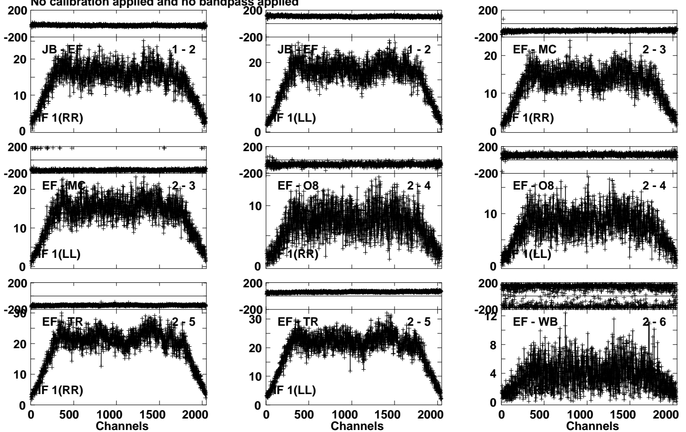
Lower frame: Milli Ampl Jy Top frame: Phas deg Vector averaged cross-power spectrum Several baselines displayed Timerange: 01/00:36:19 to 01/00:38:02
