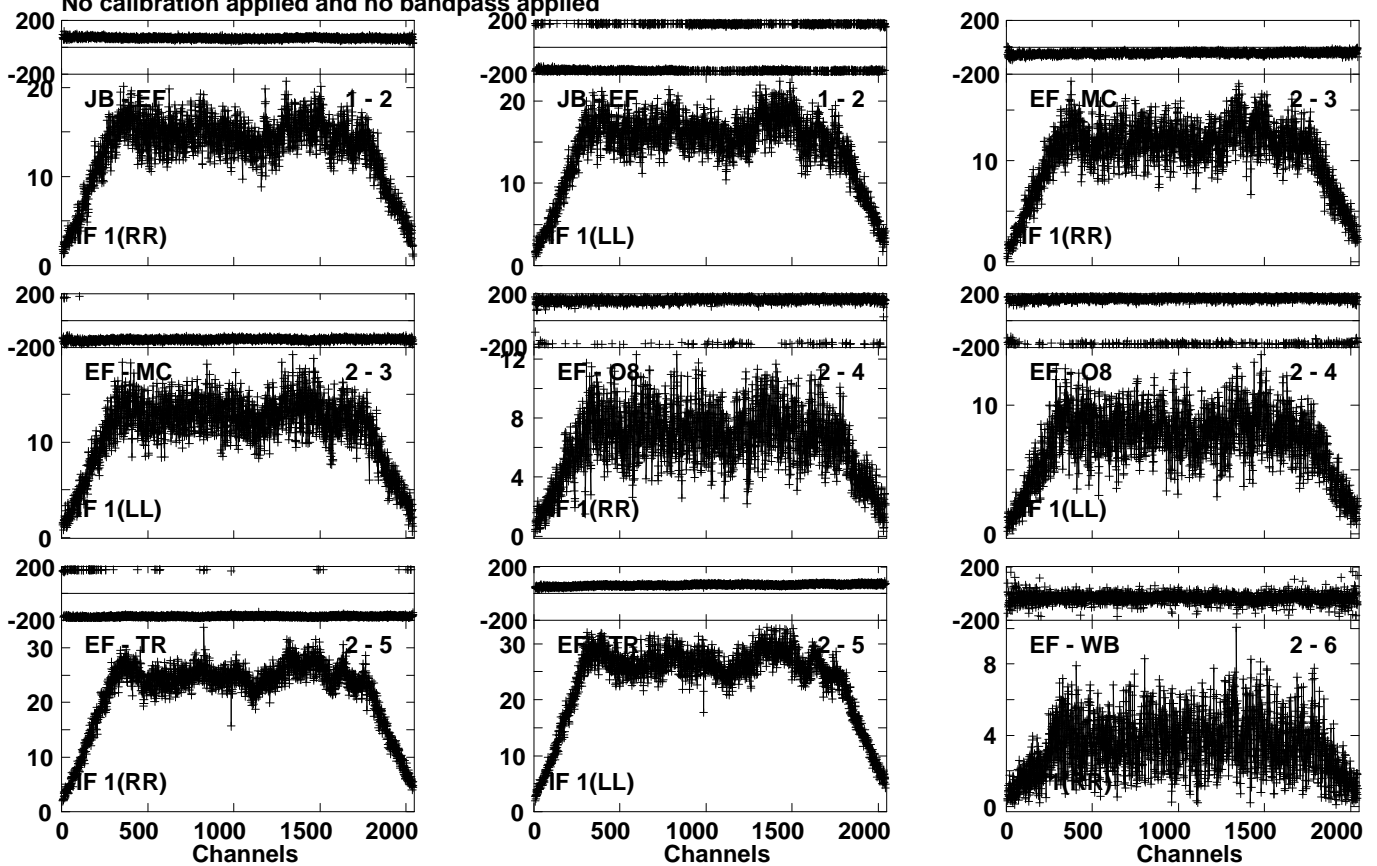
Lower frame: Milli Ampl Jy Top frame: Phas deg Vector averaged cross-power spectrum Several baselines displayed Timerange: 01/05:50:10 to 01/05:51:53
