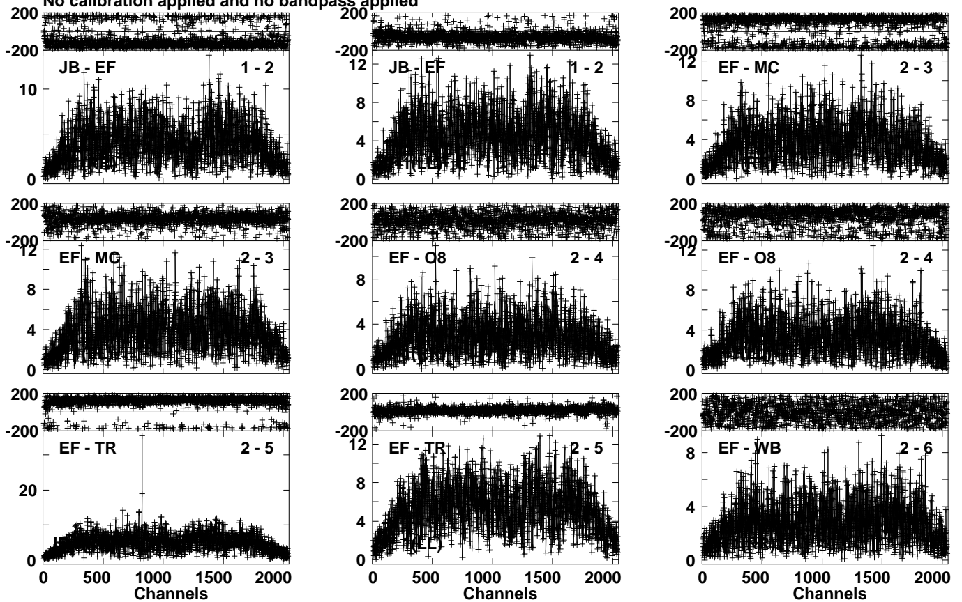
Lower frame: Milli Ampl Jy Top frame: Phas deg Vector averaged cross-power spectrum Several baselines displayed Timerange: 01/05:29:35 to 01/05:31:18
