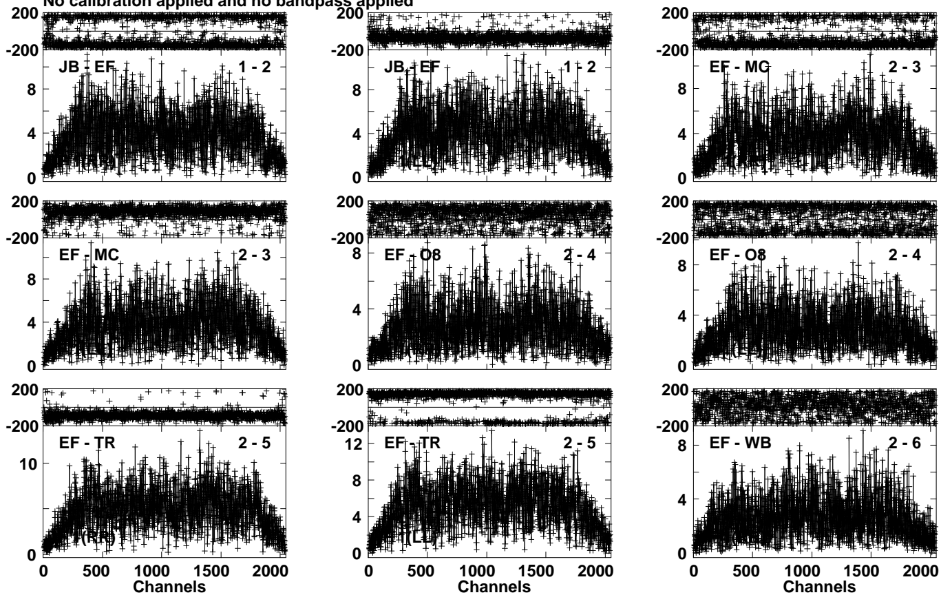
Lower frame: Milli Ampl Jy Top frame: Phas deg Vector averaged cross-power spectrum Several baselines displayed Timerange: 01/05:45:05 to 01/05:46:48
