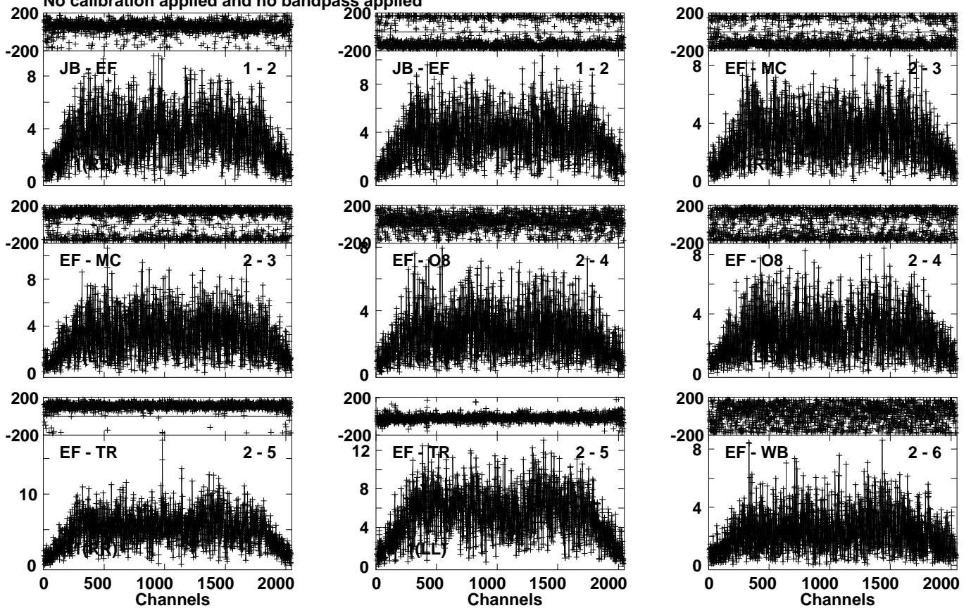
Lower frame: Milli Ampl Jy Top frame: Phas deg Vector averaged cross-power spectrum Several baselines displayed Timerange: 01/00:06:54 to 01/00:08:37
