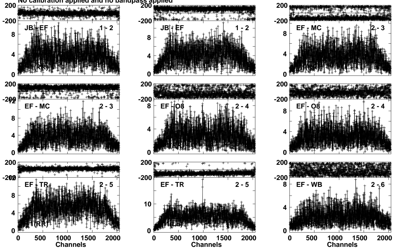
Lower frame: Milli Ampl Jy Top frame: Phas deg Vector averaged cross-power spectrum Several baselines displayed Timerange: 01/07:03:37 to 01/07:05:20
