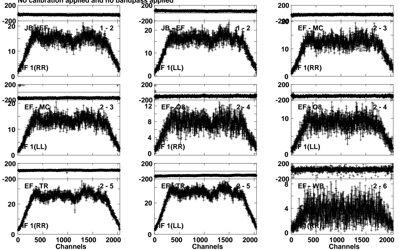
Lower frame: Milli Ampl Jy Top frame: Phas deg Vector averaged cross-power spectrum Several baselines displayed Timerange: 01/04:47:33 to 01/04:49:17
