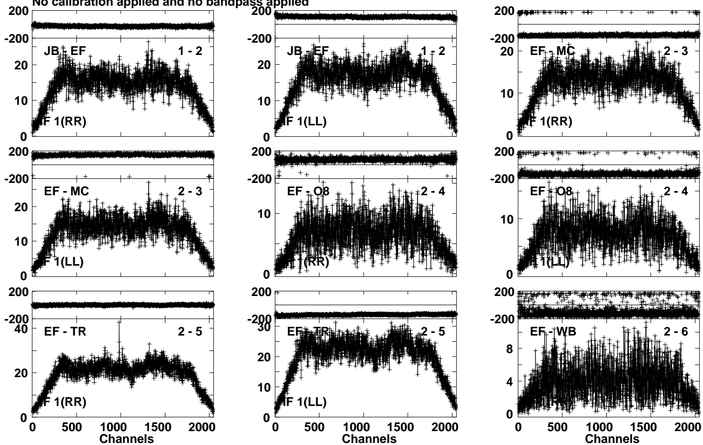
Lower frame: Milli Ampl Jy Top frame: Phas deg Vector averaged cross-power spectrum Several baselines displayed Timerange: 00/23:03:48 to 00/23:05:31
