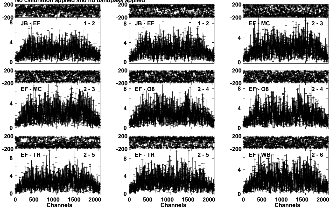
Lower frame: Milli Ampl Jy Top frame: Phas deg Vector averaged cross-power spectrum Several baselines displayed Timerange: 01/06:45:52 to 01/06:47:35
