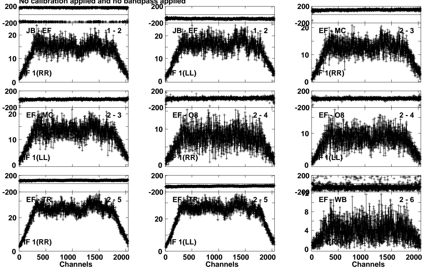
Lower frame: Milli Ampl Jy Top frame: Phas deg Vector averaged cross-power spectrum Several baselines displayed Timerange: 01/04:21:03 to 01/04:22:46
