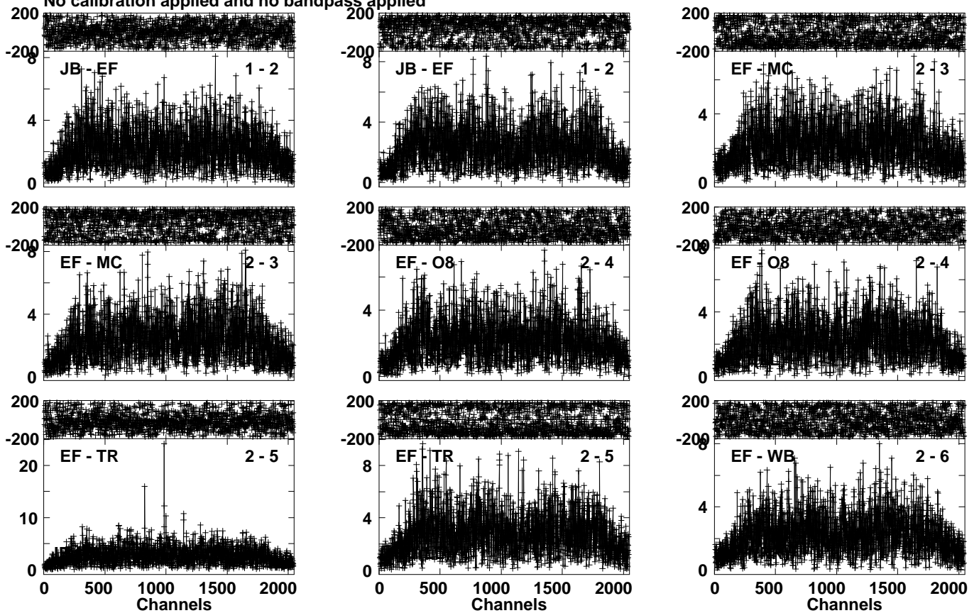
Lower frame: Milli Ampl Jy Top frame: Phas deg Vector averaged cross-power spectrum Several baselines displayed Timerange: 01/06:56:22 to 01/06:58:05
