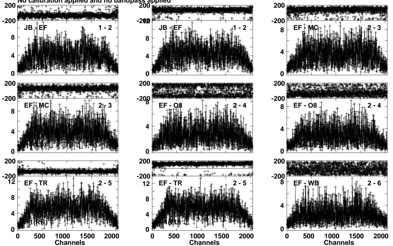
Lower frame: Milli Ampl Jy Top frame: Phas deg Vector averaged cross-power spectrum Several baselines displayed Timerange: 01/02:43:57 to 01/02:45:40
