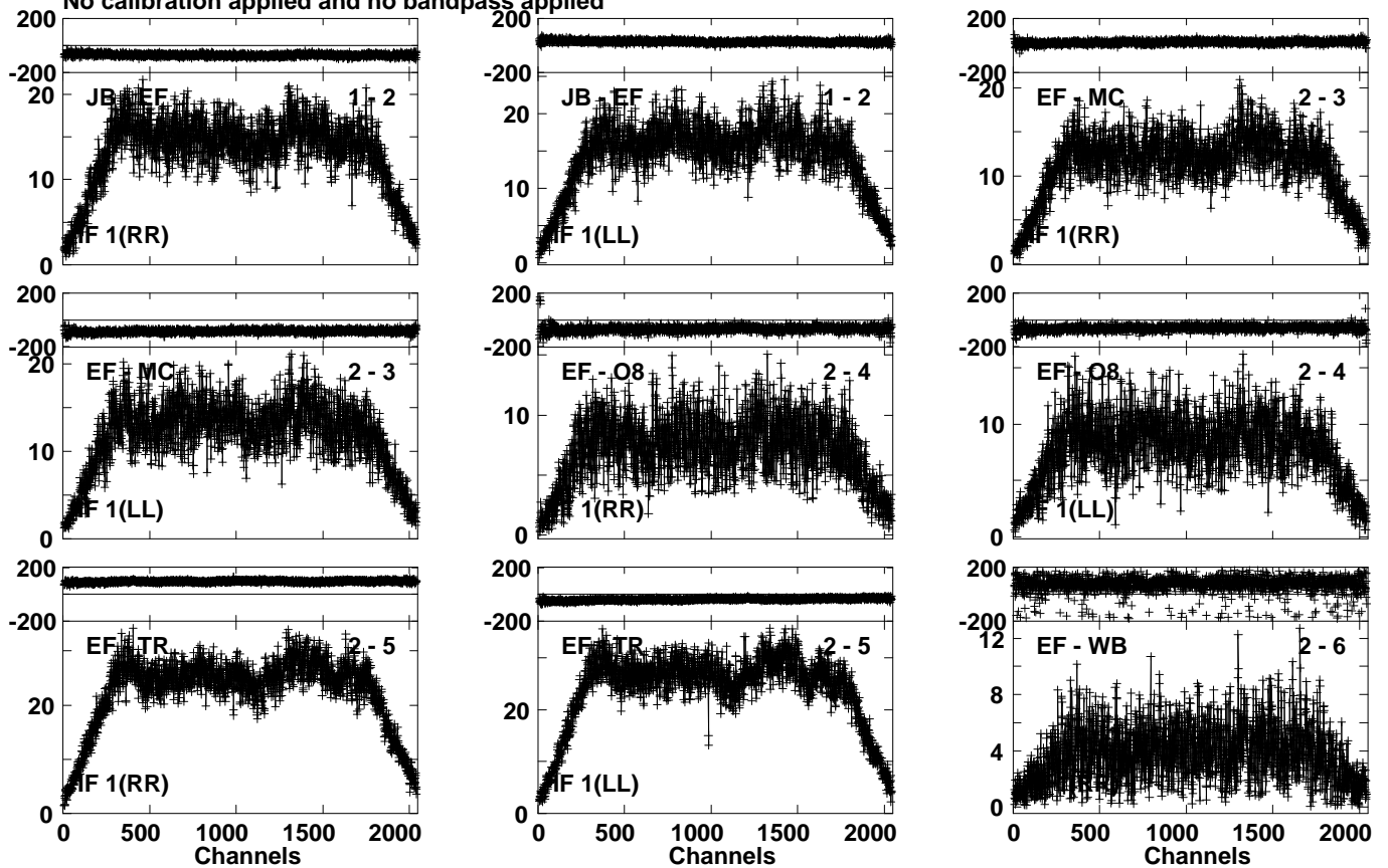
Lower frame: Milli Ampl Jy Top frame: Phas deg Vector averaged cross-power spectrum Several baselines displayed Timerange: 01/04:52:33 to 01/04:54:16
