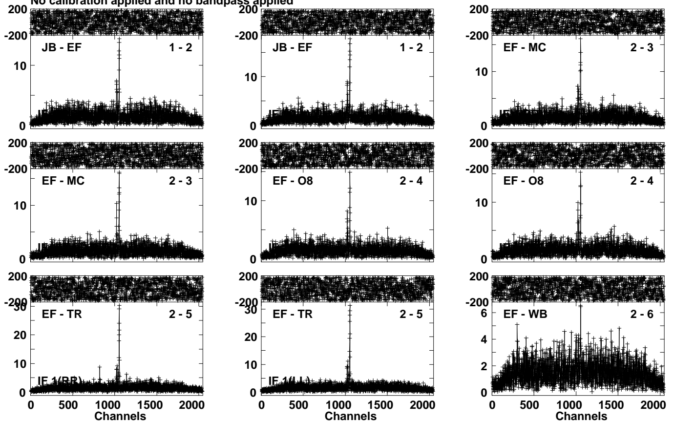
Lower frame: Milli Ampl Jy Top frame: Phas deg Vector averaged cross-power spectrum Several baselines displayed Timerange: 00/22:52:08 to 00/22:55:21
