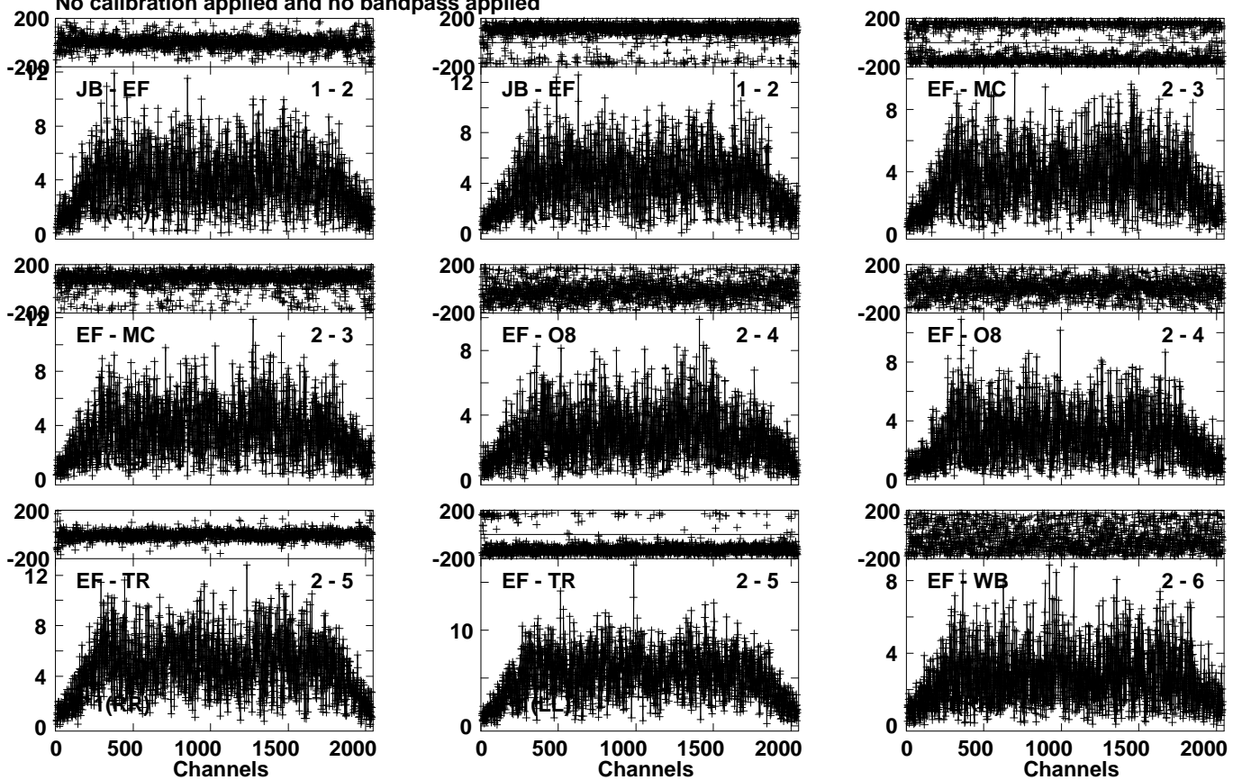
Lower frame: Milli Ampl Jy Top frame: Phas deg Vector averaged cross-power spectrum Several baselines displayed Timerange: 01/07:08:31 to 01/07:10:10
