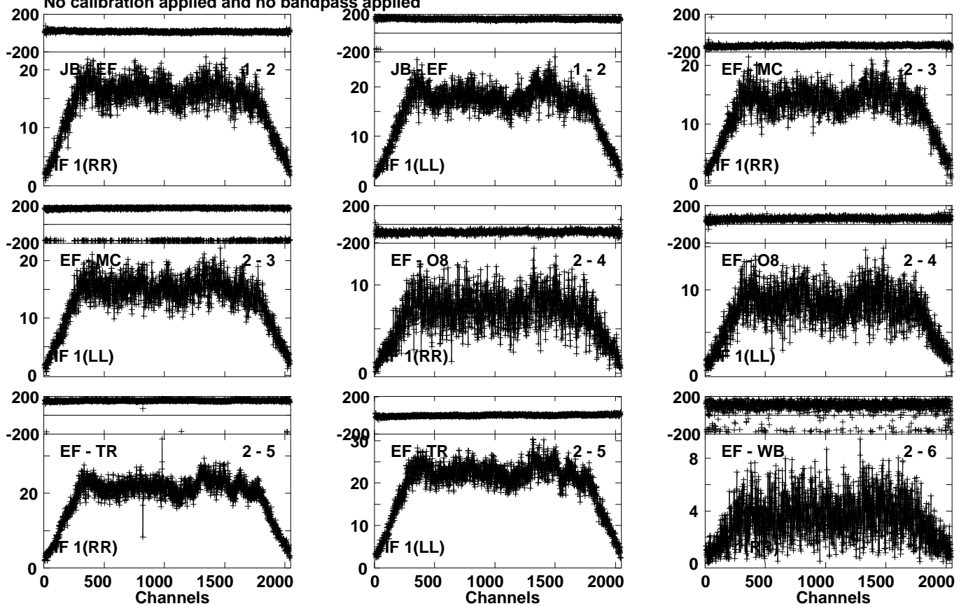
Lower frame: Milli Ampl Jy Top frame: Phas deg Vector averaged cross-power spectrum Several baselines displayed Timerange: 01/00:31:19 to 01/00:33:02
