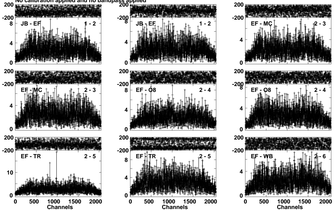
Lower frame: Milli Ampl Jy Top frame: Phas deg Vector averaged cross-power spectrum Several baselines displayed Timerange: 01/05:06:50 to 01/05:08:34
