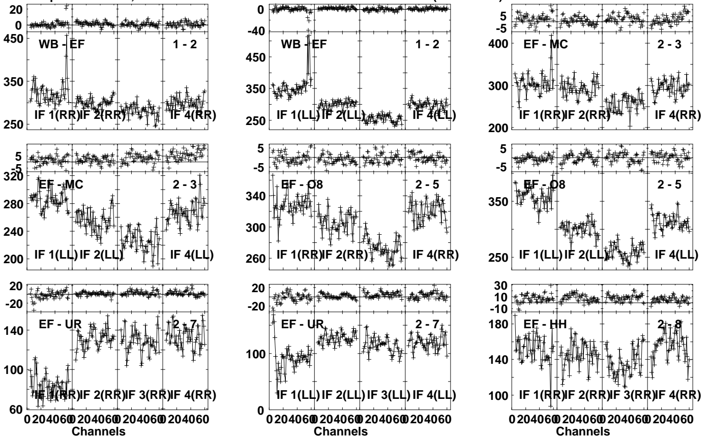
Lower frame: Milli Ampl Jy Top frame: Phas deg Vector averaged cross-power spectrum Several baselines displayed Timerange: 00/22:13:21 to 00/22:14:49
