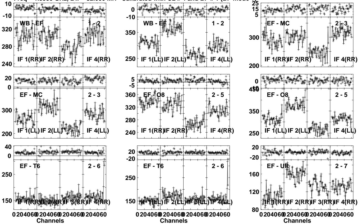
Lower frame: Milli Ampl Jy Top frame: Phas deg Vector averaged cross-power spectrum Several baselines displayed Timerange: 00:19:27:31 to 00:19:28:59
