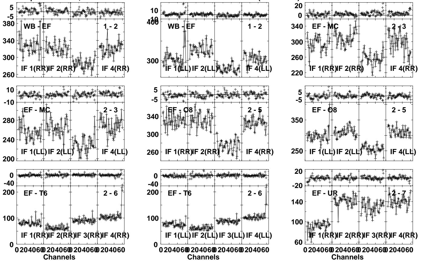
Lower frame: Milli Ampl Jy Top frame: Phas deg Vector averaged cross-power spectrum Several baselines displayed Timerange: 00/21:02:21 to 00/21:03:19
