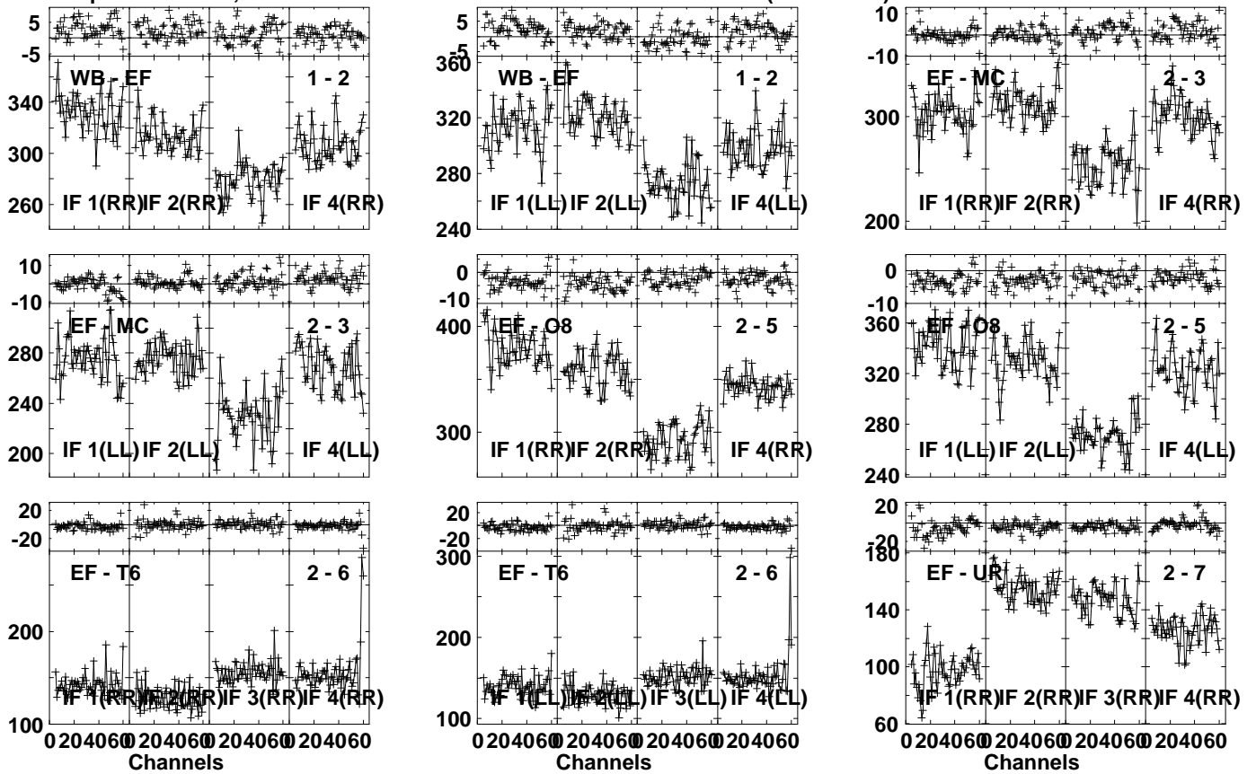
Lower frame: Milli Ampl Jy Top frame: Phas deg Vector averaged cross-power spectrum Several baselines displayed Timerange: 00:19:55:31 to 00:19:56:29
