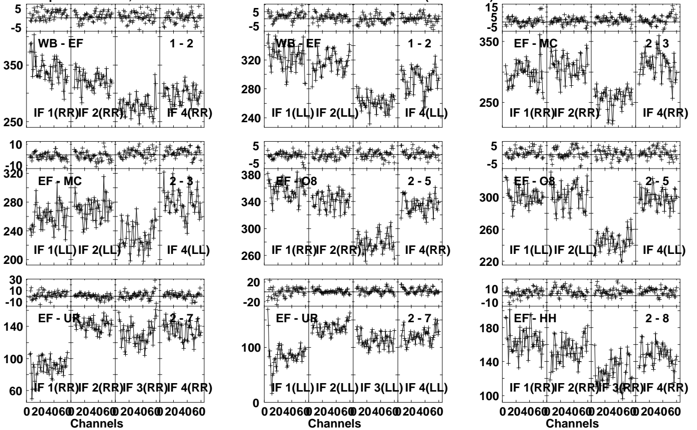
Lower frame: Milli Ampl Jy Top frame: Phas deg Vector averaged cross-power spectrum Several baselines displayed Timerange: 00/21:46:21 to 00/21:47:19
