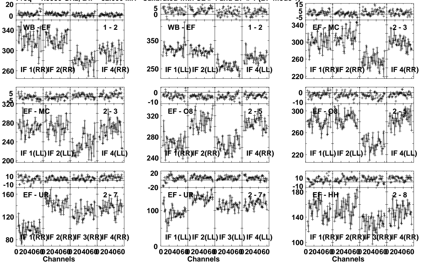
Lower frame: Milli Ampl Jy Top frame: Phas deg Vector averaged cross-power spectrum Several baselines displayed Timerange: 00/21:51:21 to 00/21:52:49
