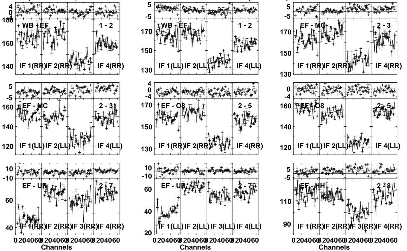
Lower frame: Milli Ampl Jy Top frame: Phas deg Vector averaged cross-power spectrum Several baselines displayed Timerange: 00/22:26:31 to 00/22:29:59
