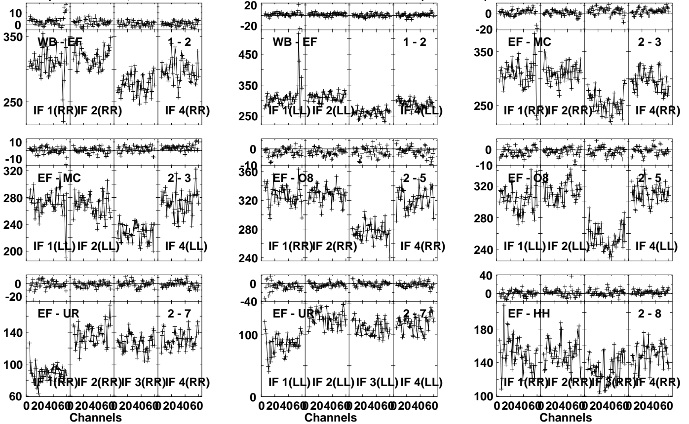
Lower frame: Milli Ampl Jy Top frame: Phas deg Vector averaged cross-power spectrum Several baselines displayed Timerange: 00/22:08:21 to 00/22:09:19
