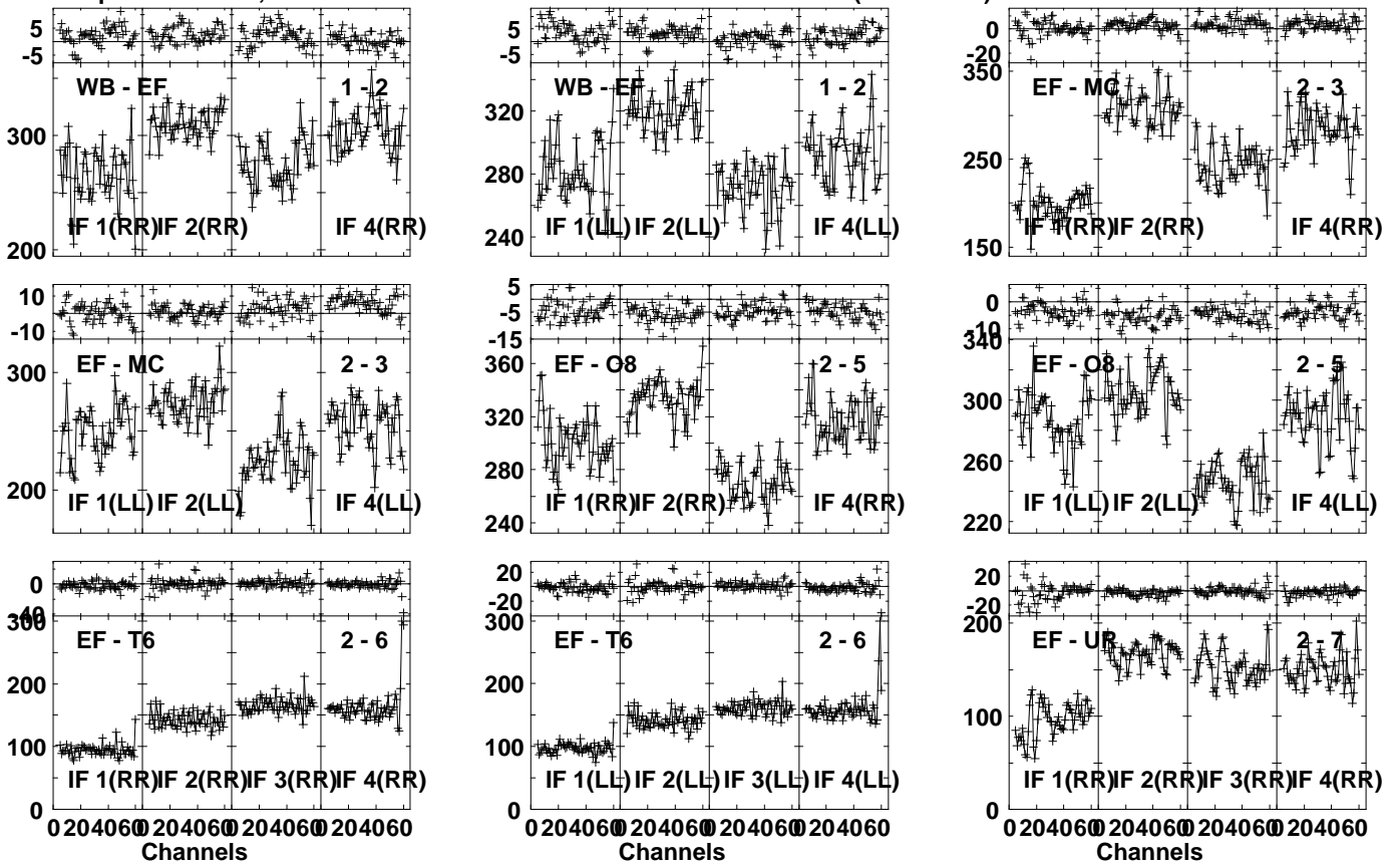
Lower frame: Milli Ampl Jy Top frame: Phas deg Vector averaged cross-power spectrum Several baselines displayed Timerange: 00:19:33:31 to 00:19:34:29
