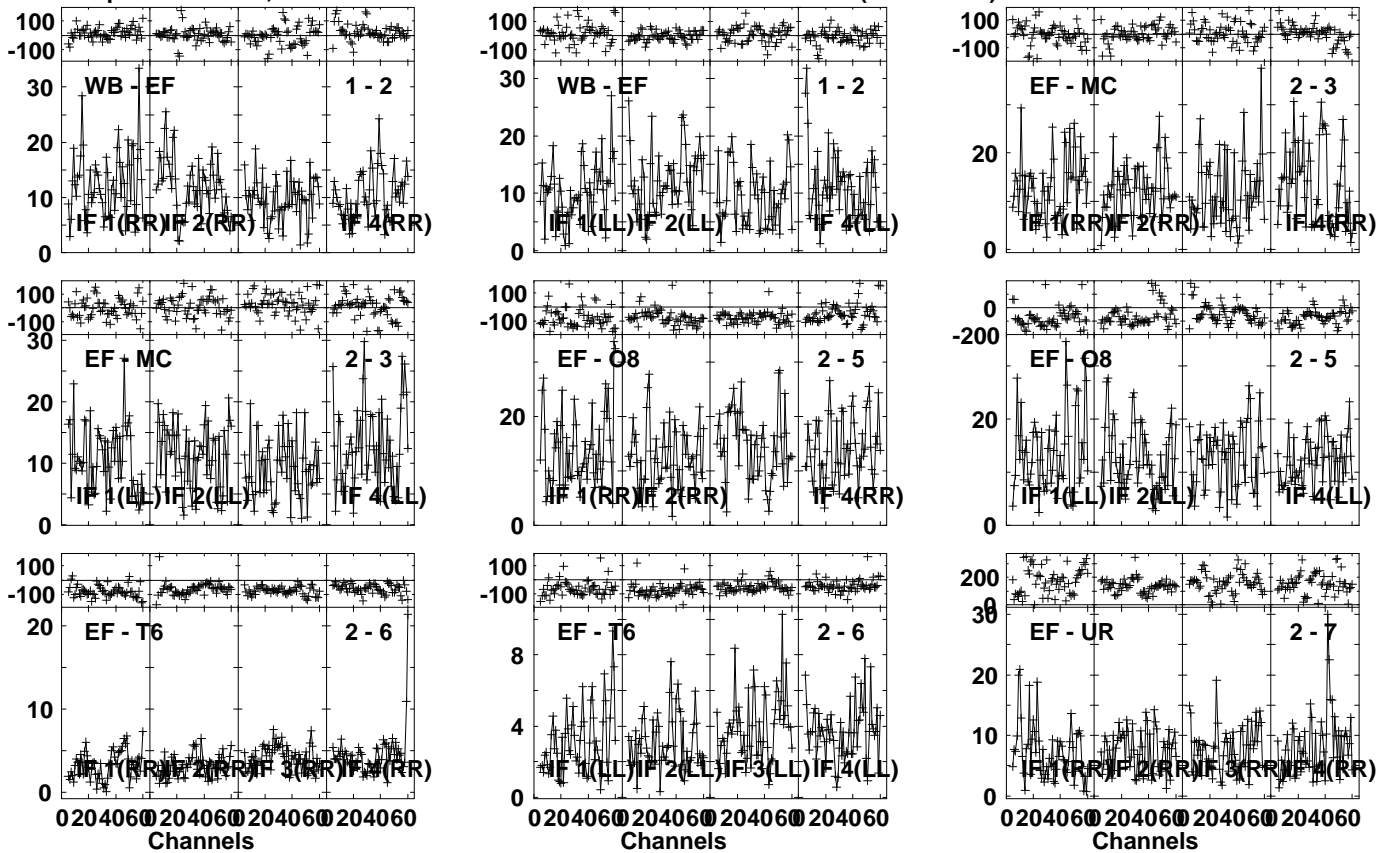
Lower frame: Milli Ampl Jy Top frame: Phas deg Vector averaged cross-power spectrum Several baselines displayed Timerange: 00/19:51:01 to 00/19:54:59
