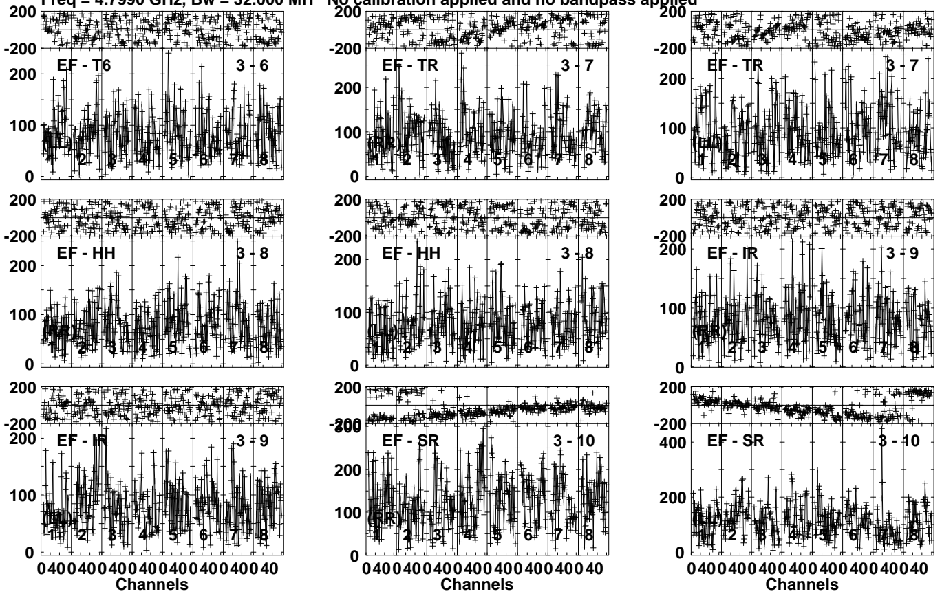
Lower frame: Micro Ampl Jy Top frame: Phas deg Vector averaged cross-power spectrum Several baselines displayed Timerange: 00/07:18:11 to 00/07:22:09
