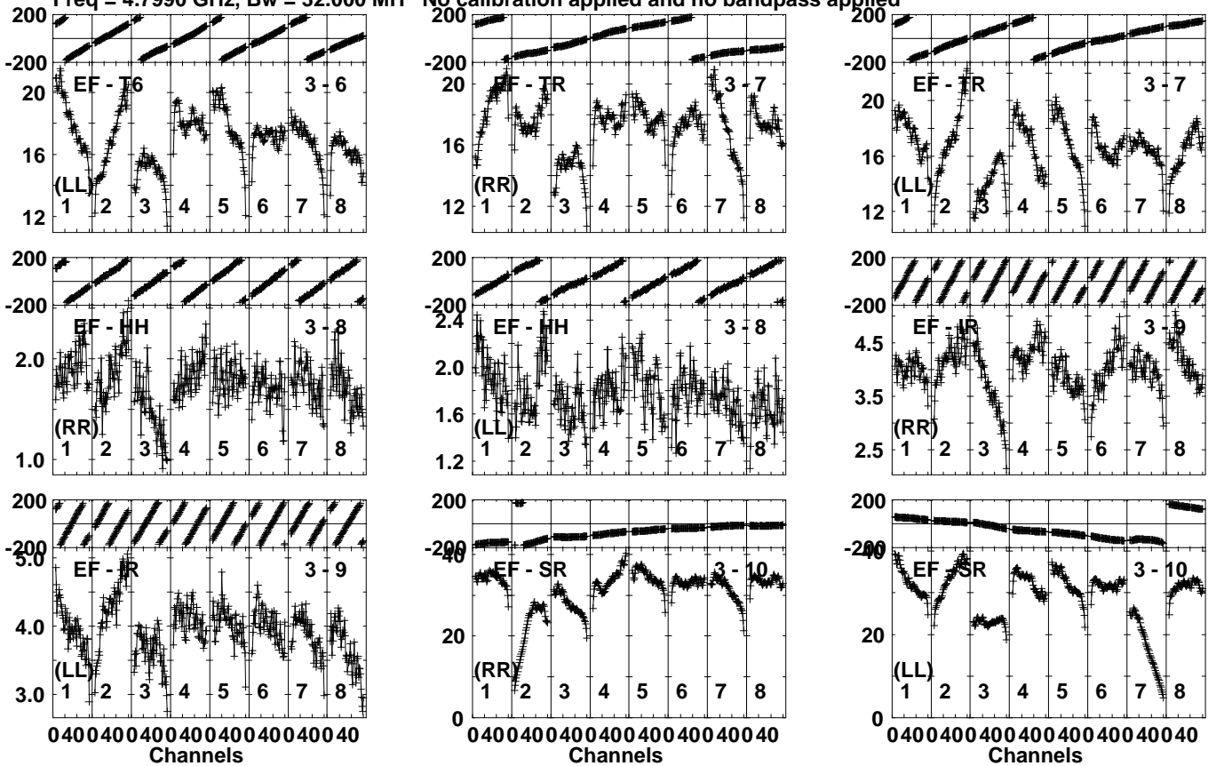
Lower frame: Milli Ampl Jy Top frame: Phas deg Vector averaged cross-power spectrum Several baselines displayed Timerange: 00/07:17:11 to 00/07:18:09
