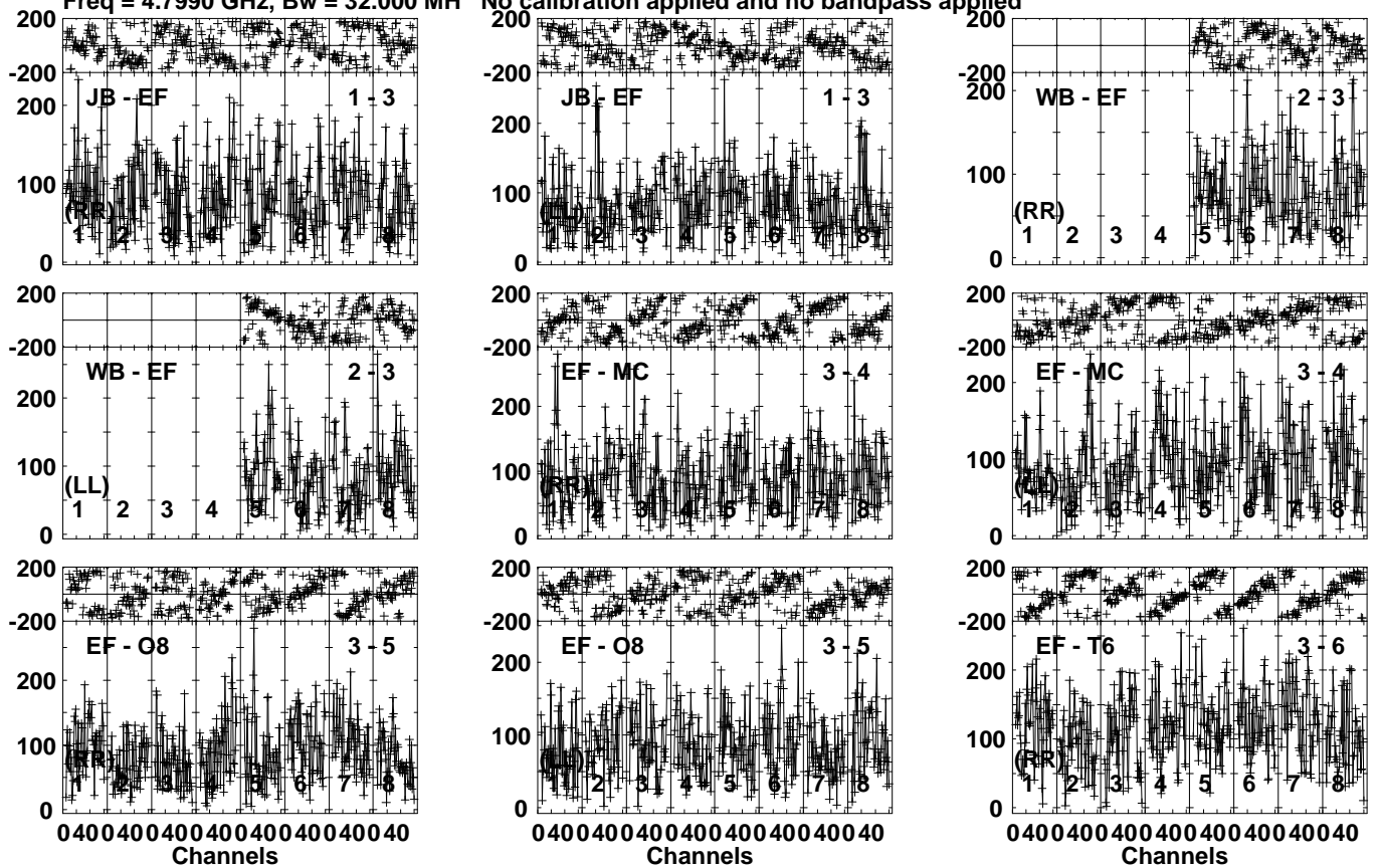
Lower frame: Micro Ampl Jy Top frame: Phas deg Vector averaged cross-power spectrum Several baselines displayed Timerange: 00/08:51:41 to 00/08:55:39
