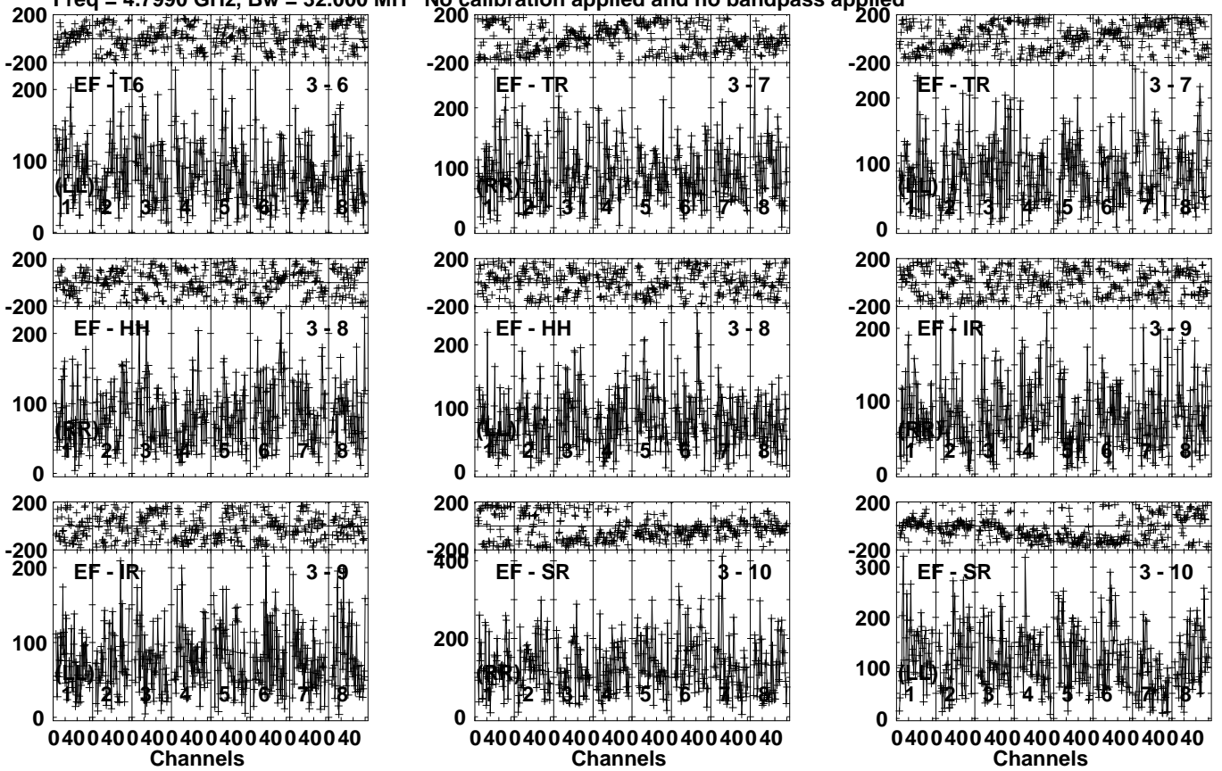
Lower frame: Micro Ampl Jy Top frame: Phas deg Vector averaged cross-power spectrum Several baselines displayed Timerange: 00/06:45:11 to 00/06:49:09
