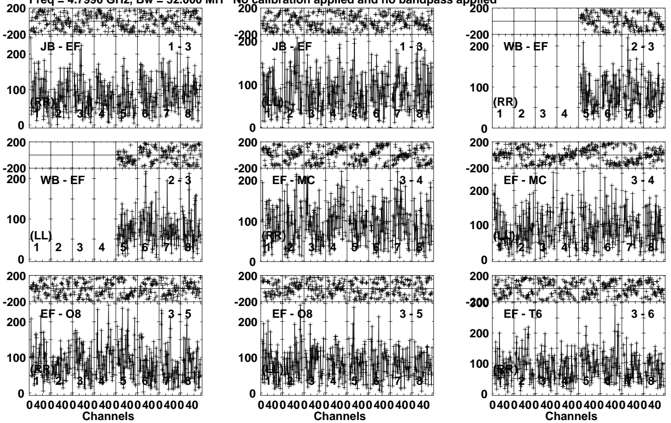
Lower frame: Micro Ampl Jy Top frame: Phas deg Vector averaged cross-power spectrum Several baselines displayed Timerange: 00/05:50:11 to 00/05:54:09
