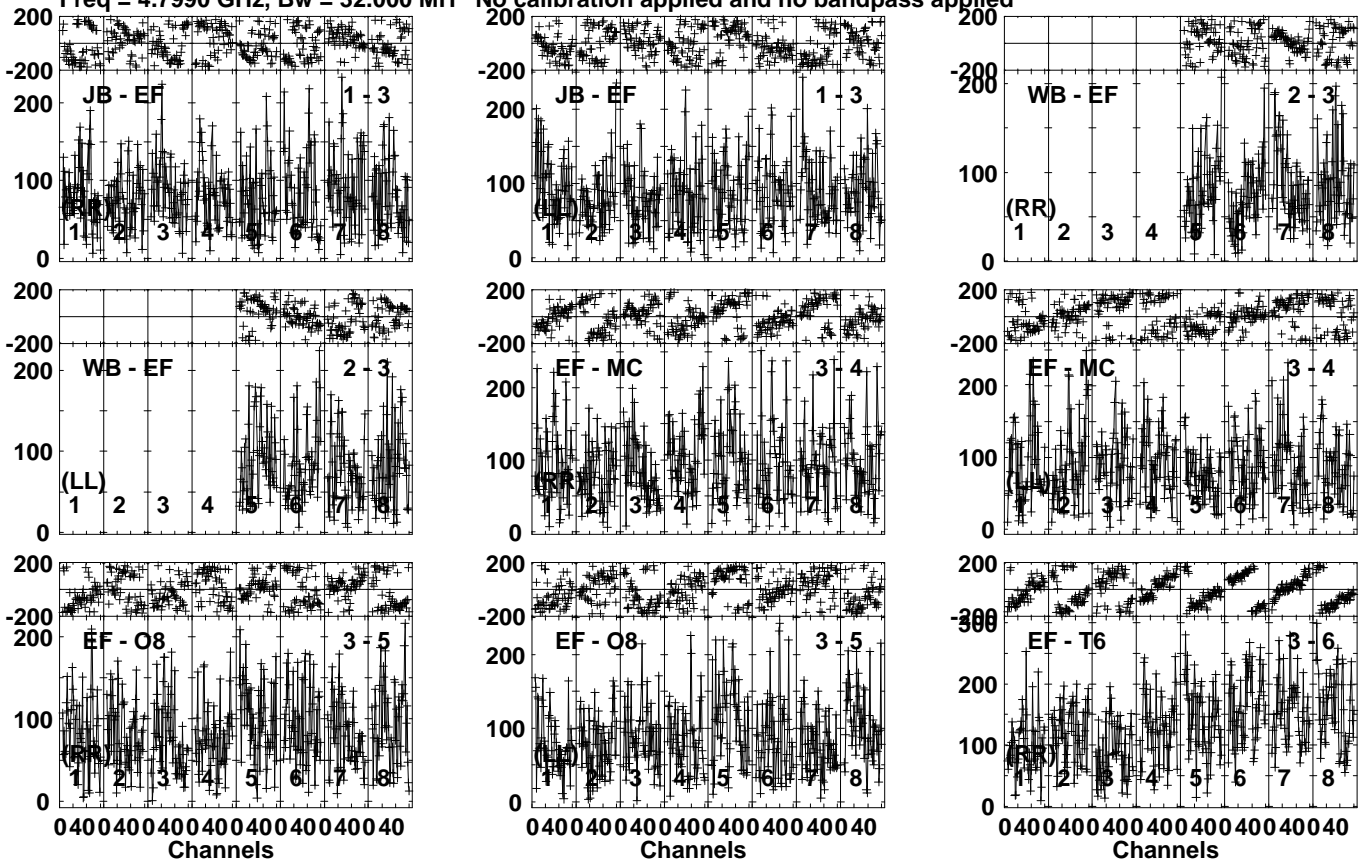
Lower frame: Micro Ampl Jy Top frame: Phas deg Vector averaged cross-power spectrum Several baselines displayed Timerange: 00/08:07:41 to 00/08:11:39
