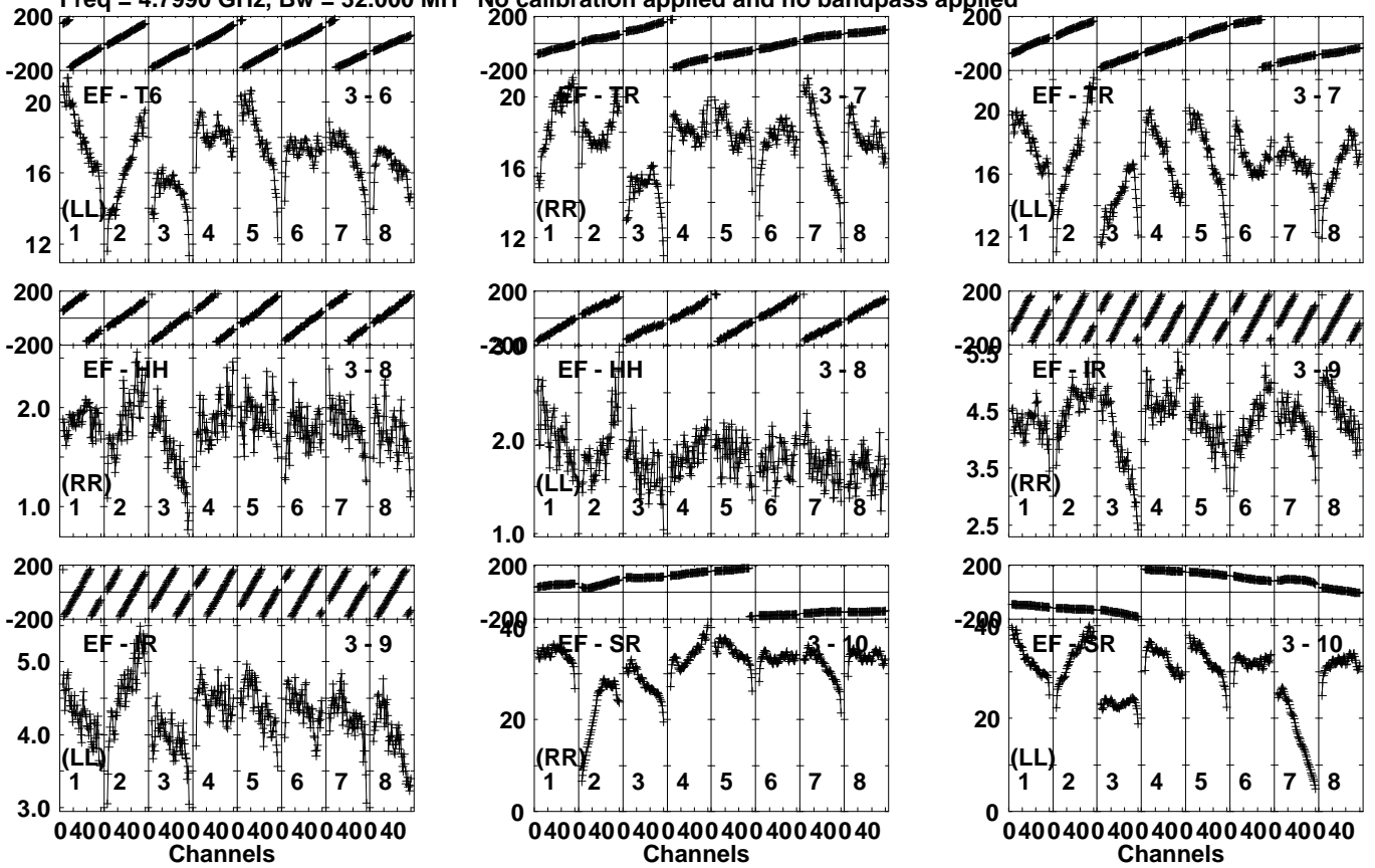
Lower frame: Milli Ampl Jy Top frame: Phas deg Vector averaged cross-power spectrum Several baselines displayed Timerange: 00/07:06:11 to 00/07:07:09
