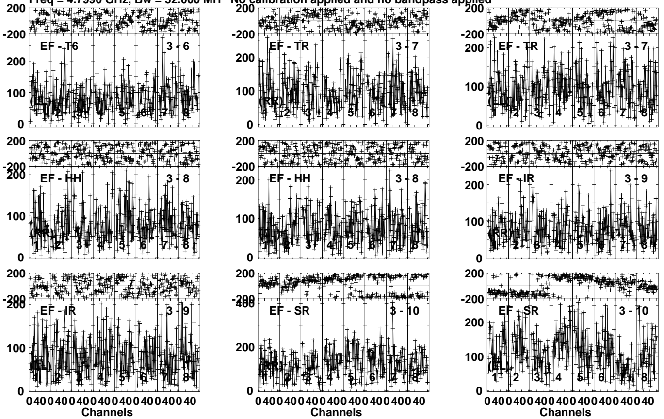
Lower frame: Micro Ampl Jy Top frame: Phas deg Vector averaged cross-power spectrum Several baselines displayed Timerange: 00/07:23:41 to 00/07:27:39
