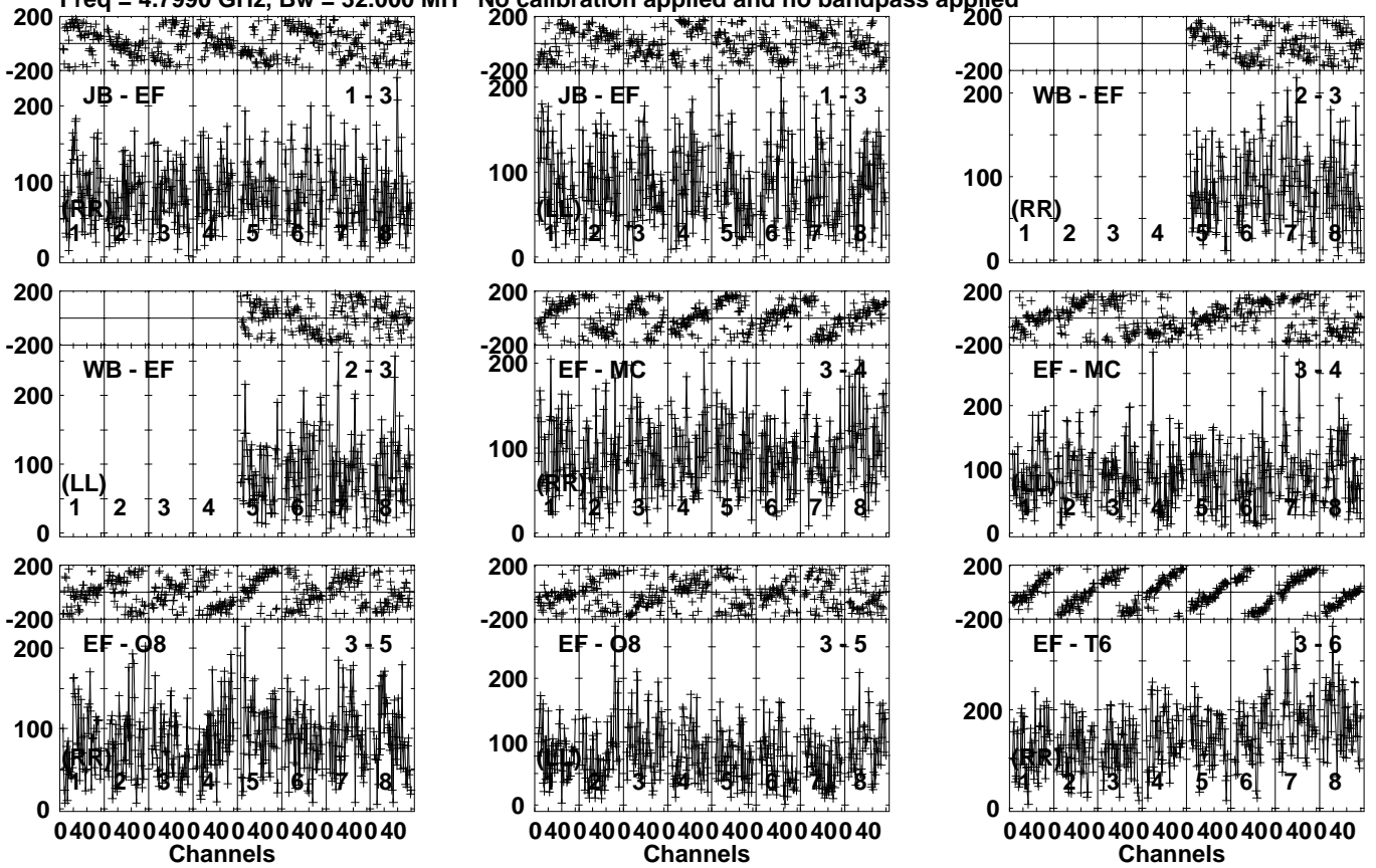
Lower frame: Micro Ampl Jy Top frame: Phas deg Vector averaged cross-power spectrum Several baselines displayed Timerange: 00/08:02:11 to 00/08:06:09
