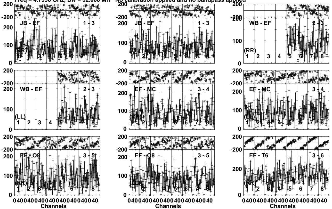
Lower frame: Micro Ampl Jy Top frame: Phas deg Vector averaged cross-power spectrum Several baselines displayed Timerange: 00/07:56:41 to 00/08:00:39
