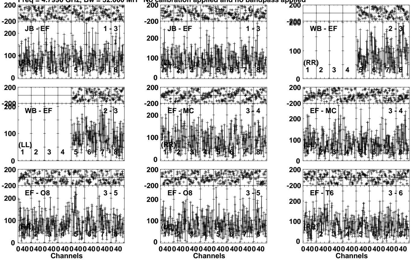
Lower frame: Micro Ampl Jy Top frame: Phas deg Vector averaged cross-power spectrum Several baselines displayed Timerange: 00/05:55:41 to 00/05:59:39
