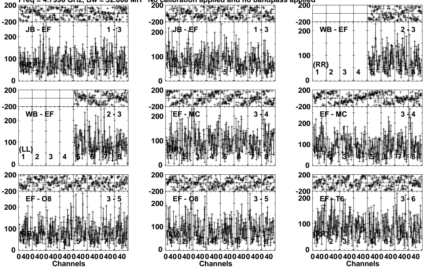
Lower frame: Micro Ampl Jy Top frame: Phas deg Vector averaged cross-power spectrum Several baselines displayed Timerange: 00/06:17:41 to 00/06:21:39
