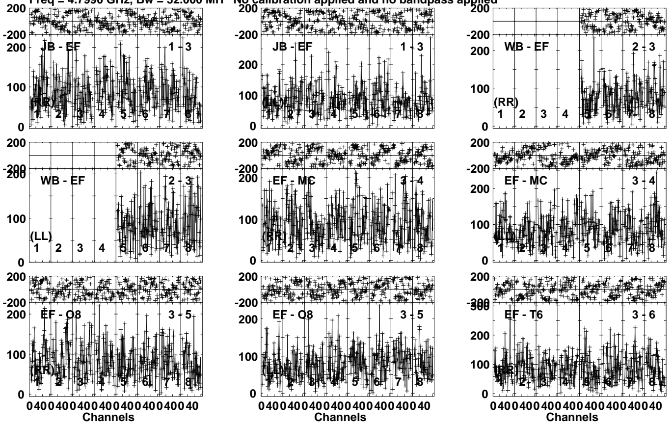
Lower frame: Micro Ampl Jy Top frame: Phas deg Vector averaged cross-power spectrum Several baselines displayed Timerange: 00/05:33:41 to 00/05:37:39
