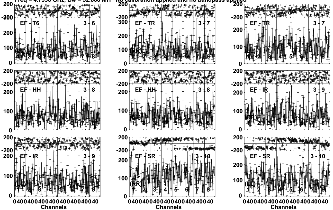
Lower frame: Micro Ampl Jy Top frame: Phas deg Vector averaged cross-power spectrum Several baselines displayed Timerange: 00/07:07:11 to 00/07:11:09
