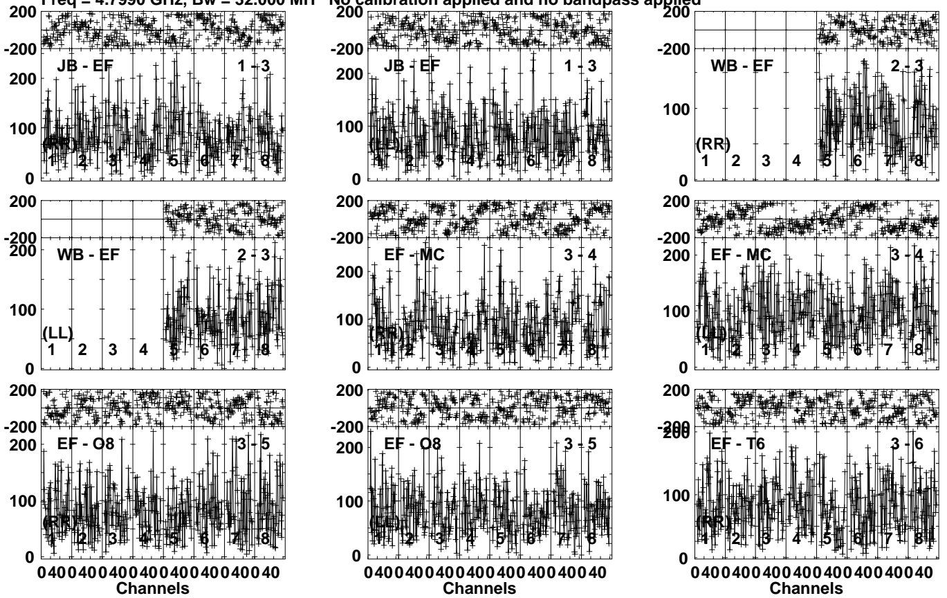
Lower frame: Micro Ampl Jy Top frame: Phas deg Vector averaged cross-power spectrum Several baselines displayed Timerange: 00/06:28:41 to 00/06:32:39
