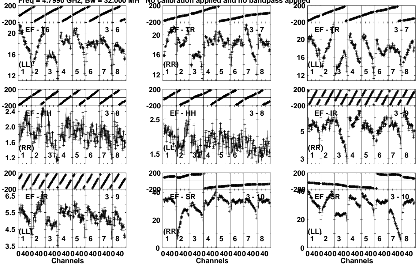
Lower frame: Milli Ampl Jy Top frame: Phas deg Vector averaged cross-power spectrum Several baselines displayed Timerange: 00/06:49:41 to 00/06:50:39
