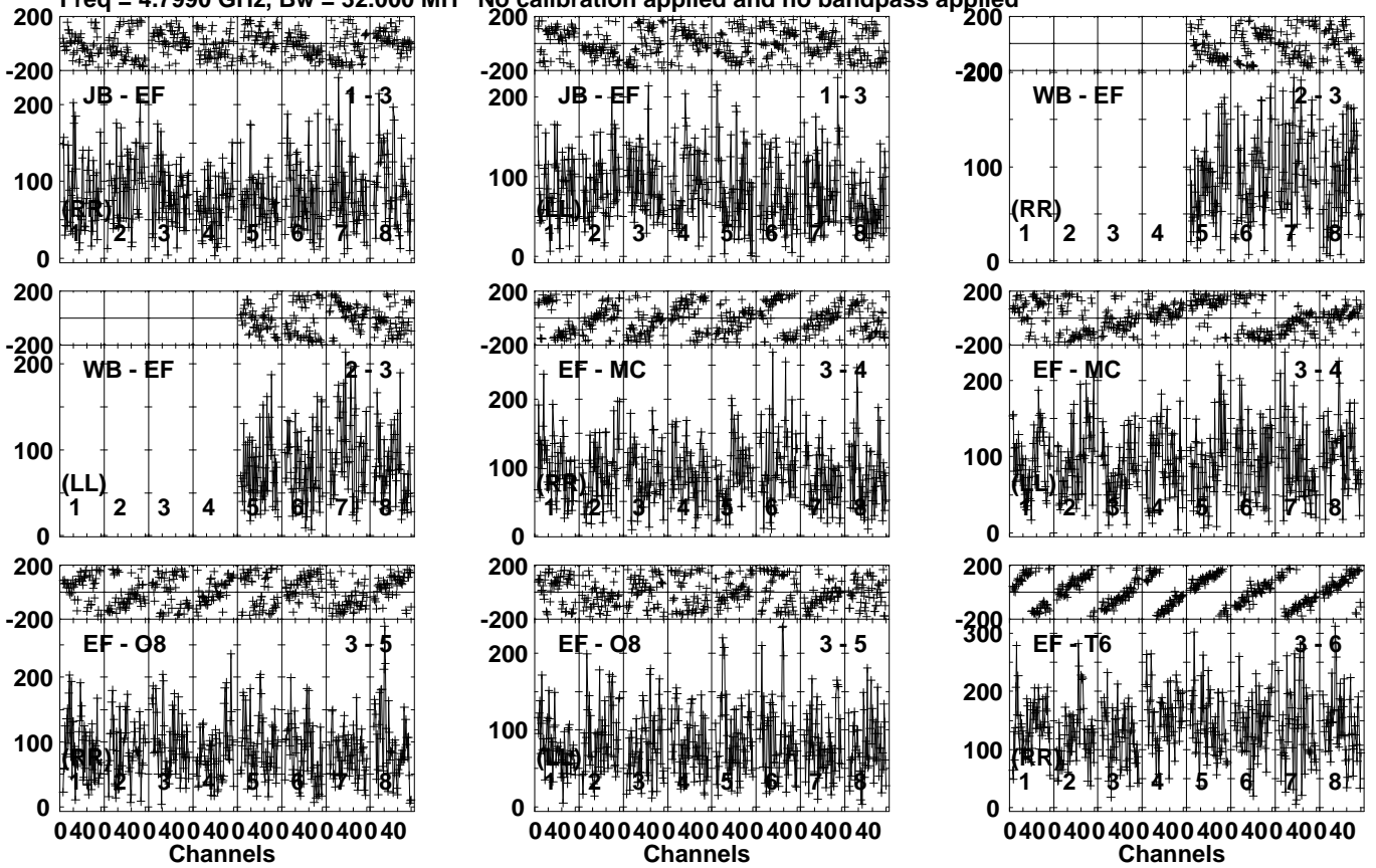
Lower frame: Micro Ampl Jy Top frame: Phas deg Vector averaged cross-power spectrum Several baselines displayed Timerange: 00/07:40:11 to 00/07:44:09
