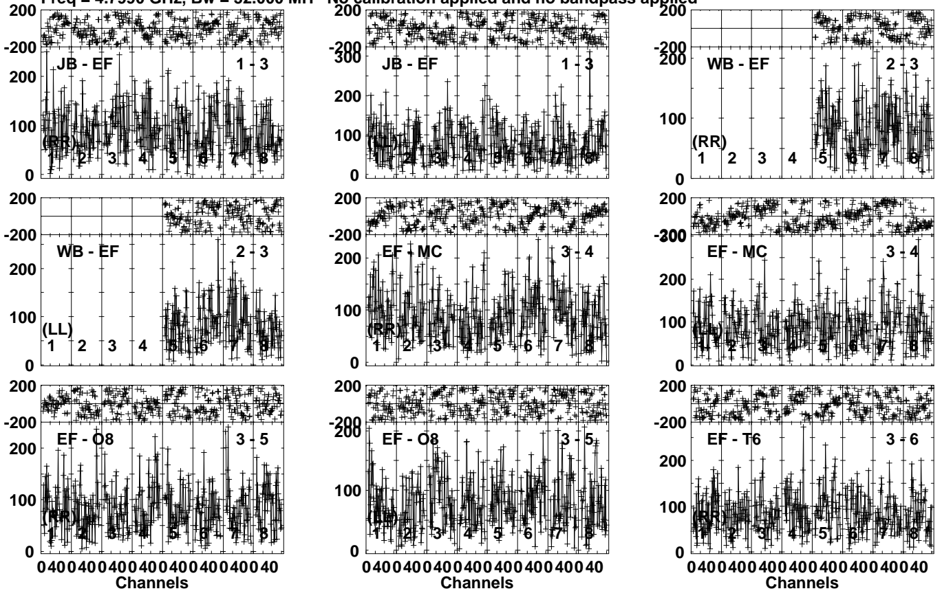
Lower frame: Micro Ampl Jy Top frame: Phas deg Vector averaged cross-power spectrum Several baselines displayed Timerange: 00/06:01:11 to 00/06:05:09
