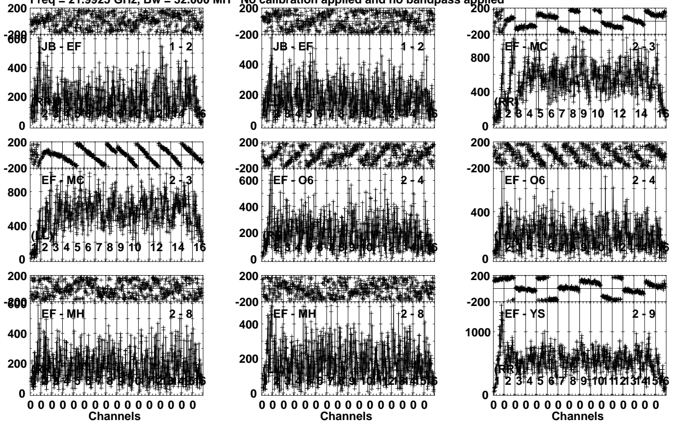
Lower frame: Micro Ampl Jy Top frame: Phas deg Vector averaged cross-power spectrum Several baselines displayed Timerange: 00/23:17:23 to 00/23:18:49
