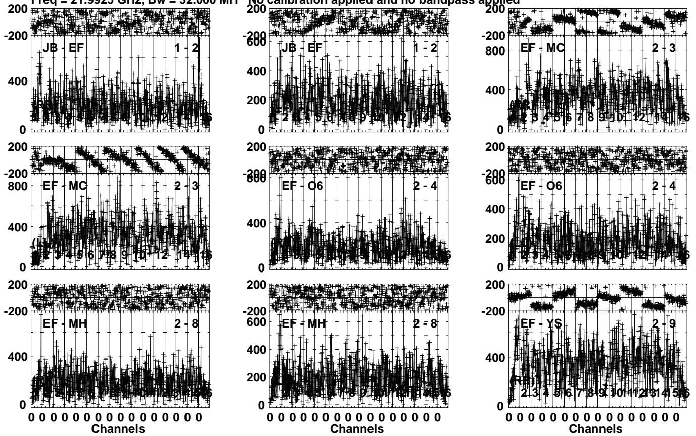
Lower frame: Micro Ampl Jy Top frame: Phas deg Vector averaged cross-power spectrum Several baselines displayed Timerange: 01/02:18:13 to 01/02:19:39
