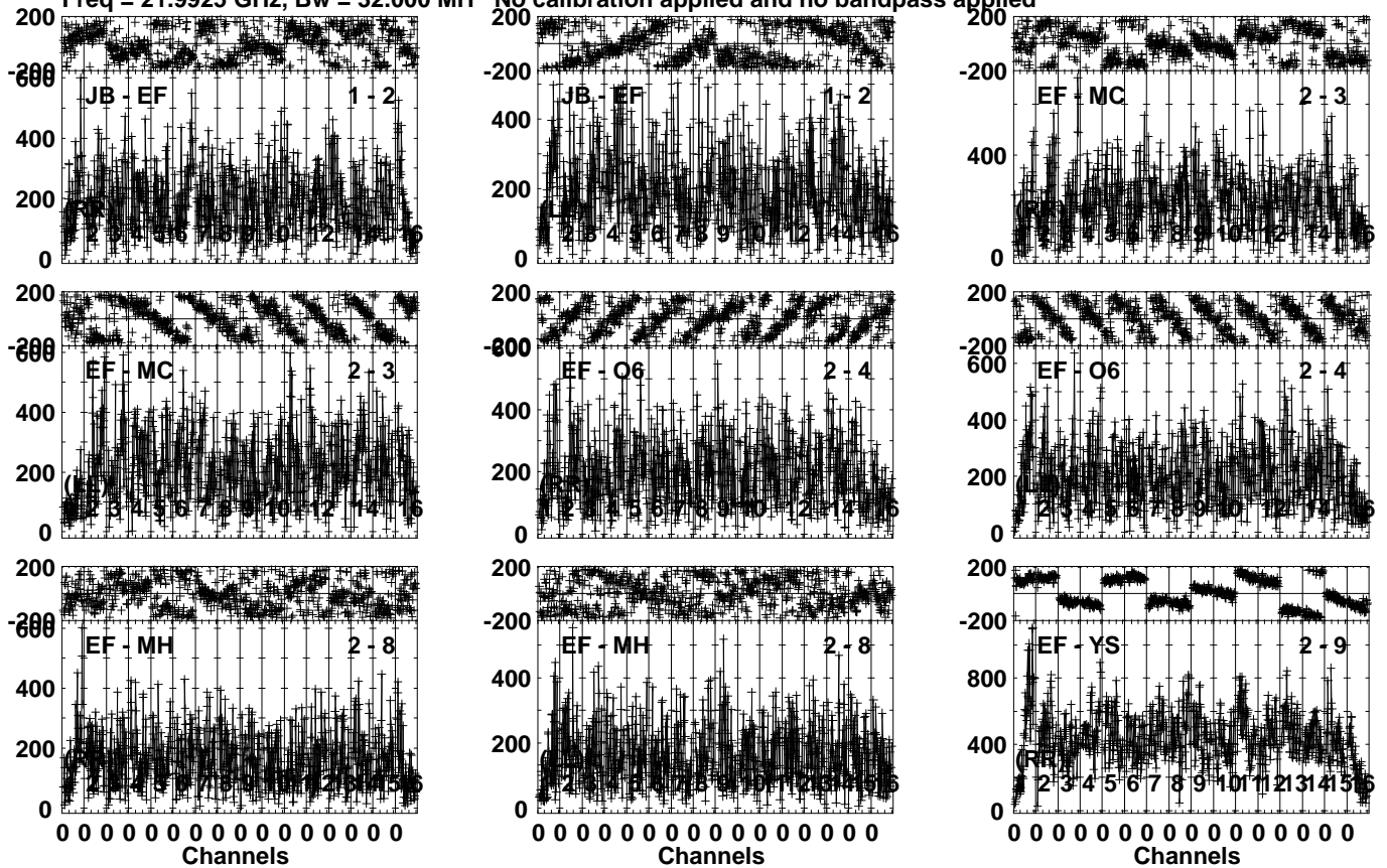
Lower frame: Micro Ampl Jy Top frame: Phas deg Vector averaged cross-power spectrum Several baselines displayed Timerange: 00/20:22:13 to 00/20:23:09
