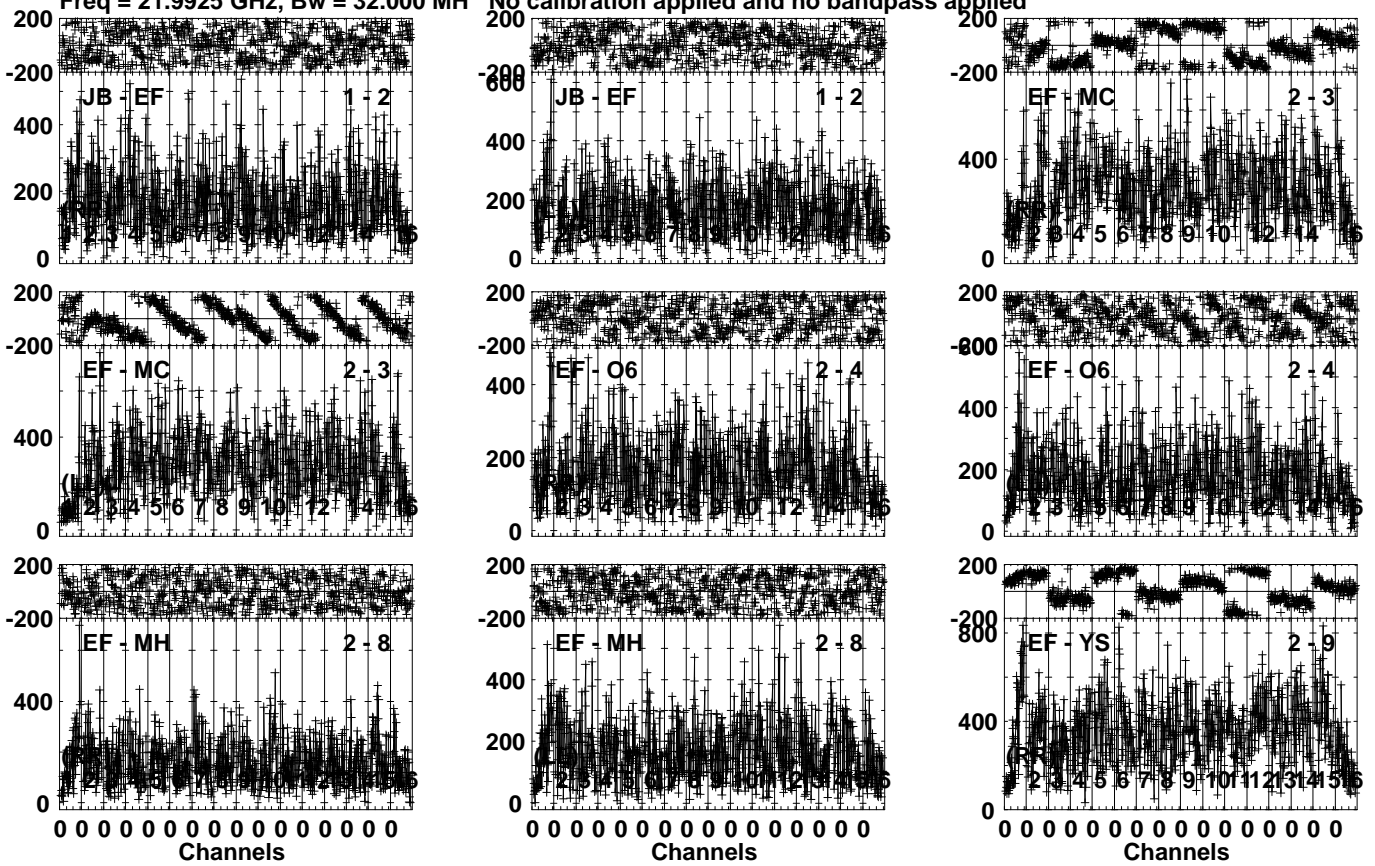
Lower frame: Micro Ampl Jy Top frame: Phas deg Vector averaged cross-power spectrum Several baselines displayed Timerange: 01/00:21:53 to 01/00:23:19
