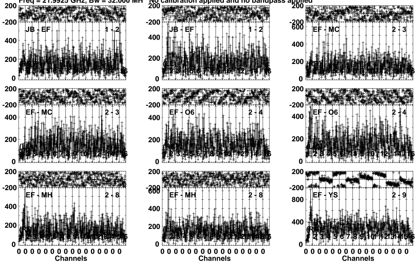
Lower frame: Micro Ampl Jy Top frame: Phas deg Vector averaged cross-power spectrum Several baselines displayed Timerange: 00/19:26:13 to 00/19:27:39
