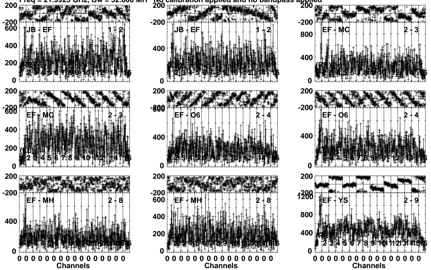
Lower frame: Micro Ampl Jy Top frame: Phas deg Vector averaged cross-power spectrum Several baselines displayed Timerange: 00/20:42:43 to 00/20:44:09
