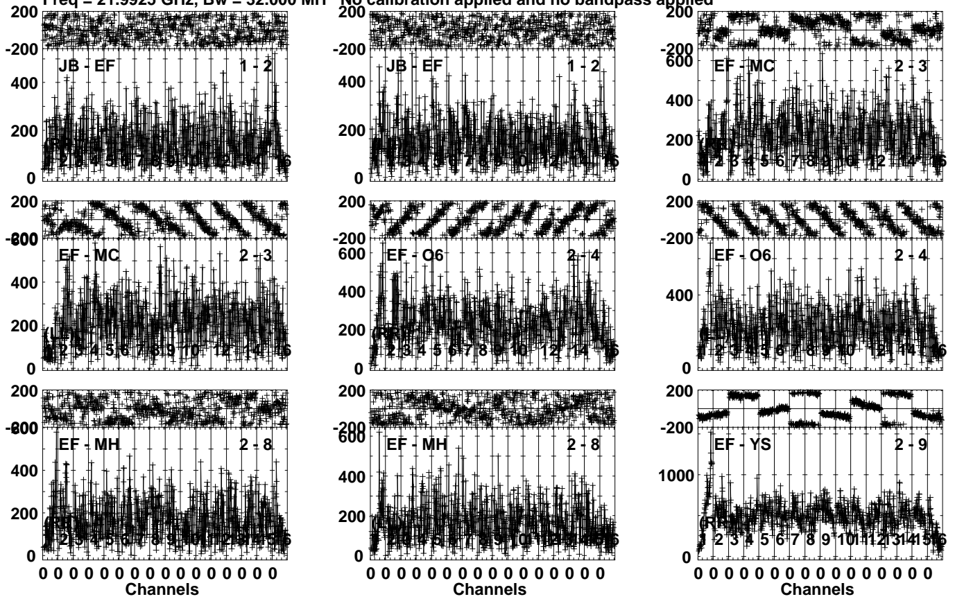
Lower frame: Micro Ampl Jy Top frame: Phas deg Vector averaged cross-power spectrum Several baselines displayed Timerange: 01/04:04:03 to 01/04:05:29
