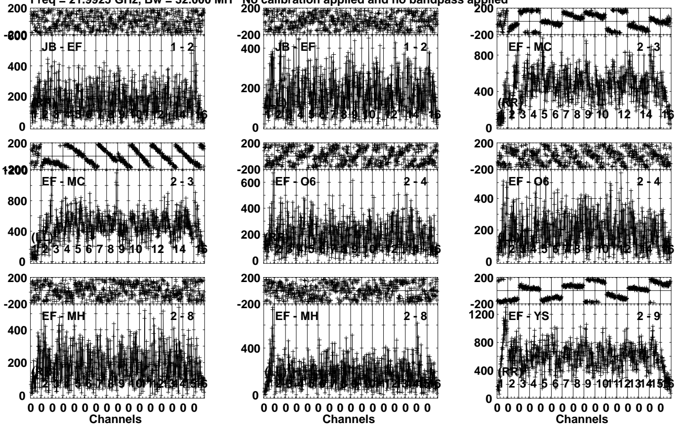
Lower frame: Micro Ampl Jy Top frame: Phas deg Vector averaged cross-power spectrum Several baselines displayed Timerange: 01/00:29:23 to 01/00:30:49
