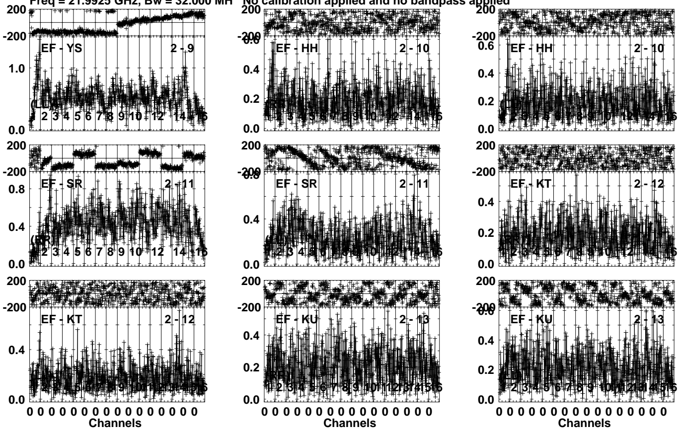
Lower frame: Milli Ampl Jy Top frame: Phas deg Vector averaged cross-power spectrum Several baselines displayed Timerange: 00/21:21:03 to 00/21:22:29
