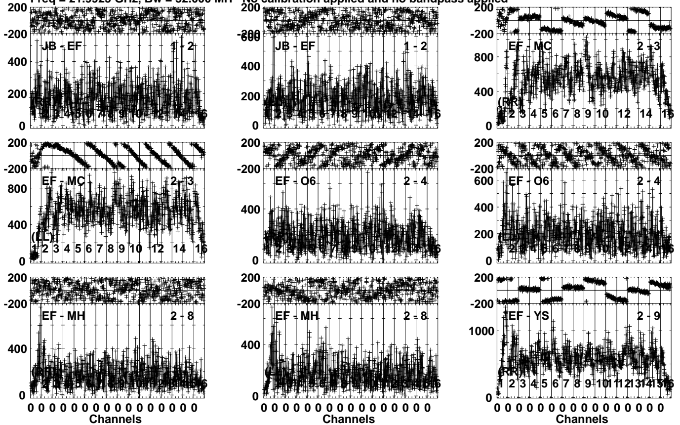
Lower frame: Micro Ampl Jy Top frame: Phas deg Vector averaged cross-power spectrum Several baselines displayed Timerange: 00/23:29:23 to 00/23:30:49
