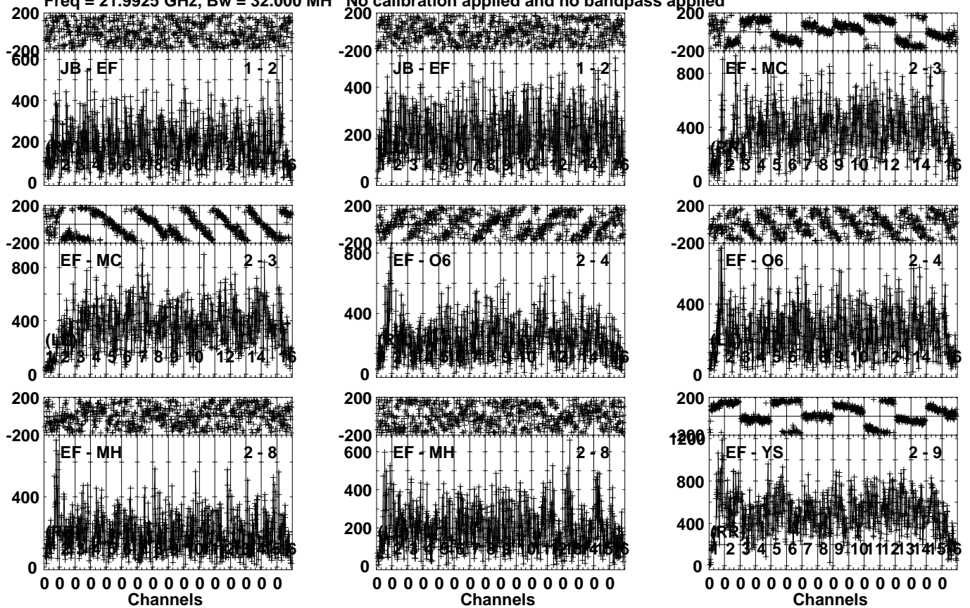
Lower frame: Micro Ampl Jy Top frame: Phas deg Vector averaged cross-power spectrum Several baselines displayed Timerange: 01/01:29:13 to 01/01:30:09
