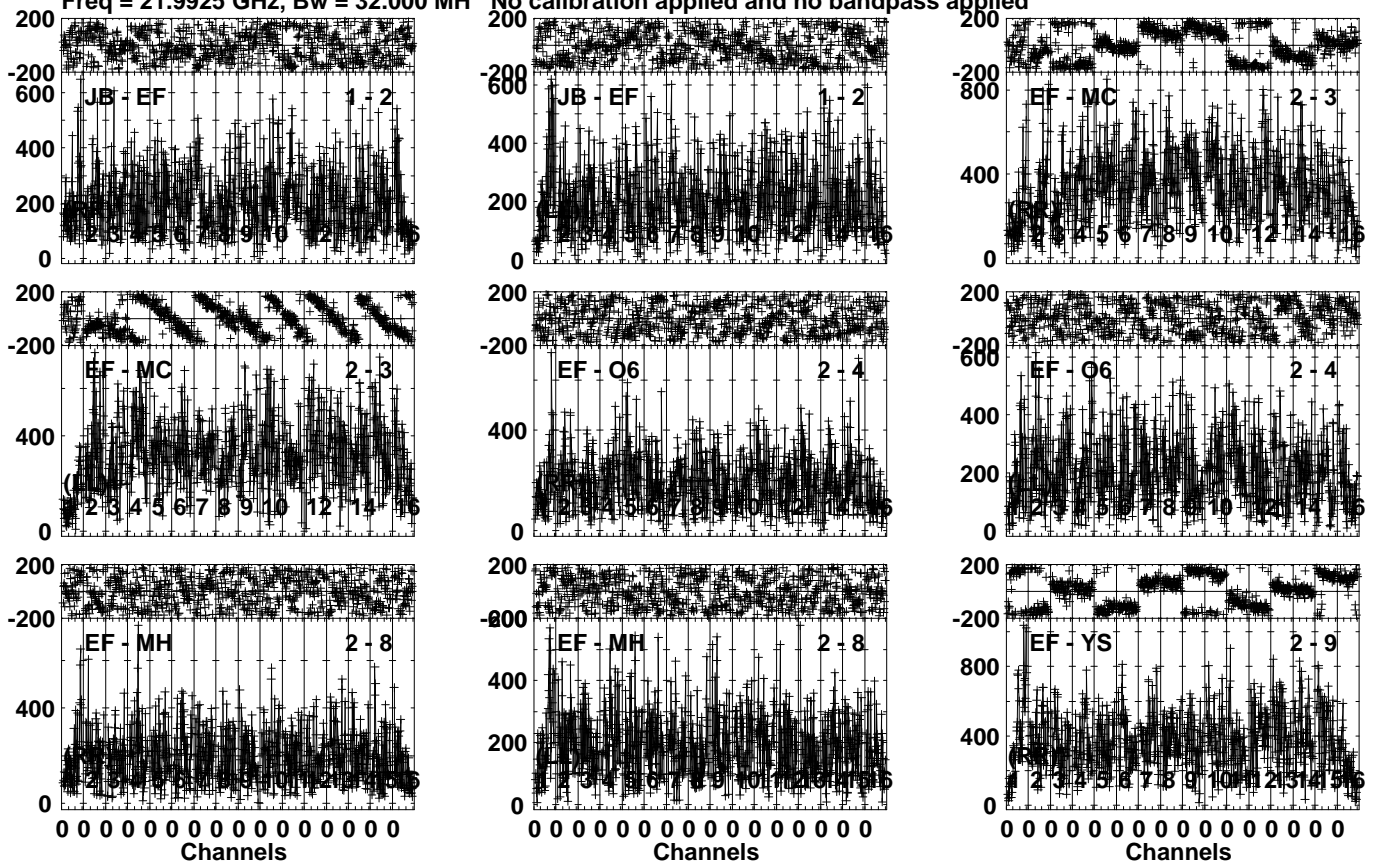
Lower frame: Micro Ampl Jy Top frame: Phas deg Vector averaged cross-power spectrum Several baselines displayed Timerange: 01/01:12:13 to 01/01:13:39
