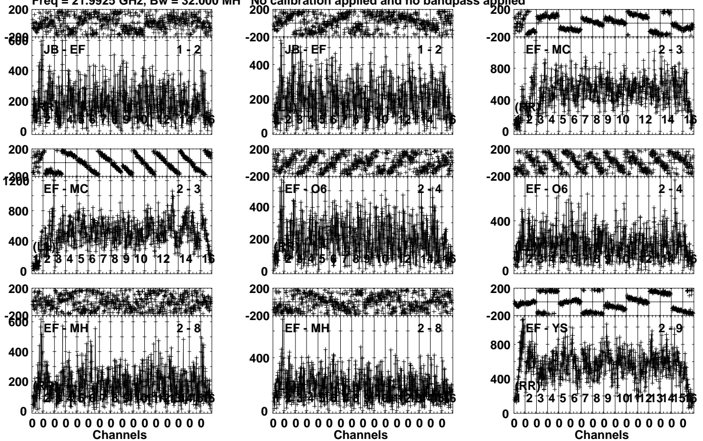
Lower frame: Micro Ampl Jy Top frame: Phas deg Vector averaged cross-power spectrum Several baselines displayed Timerange: 00/22:45:03 to 00/22:46:29
