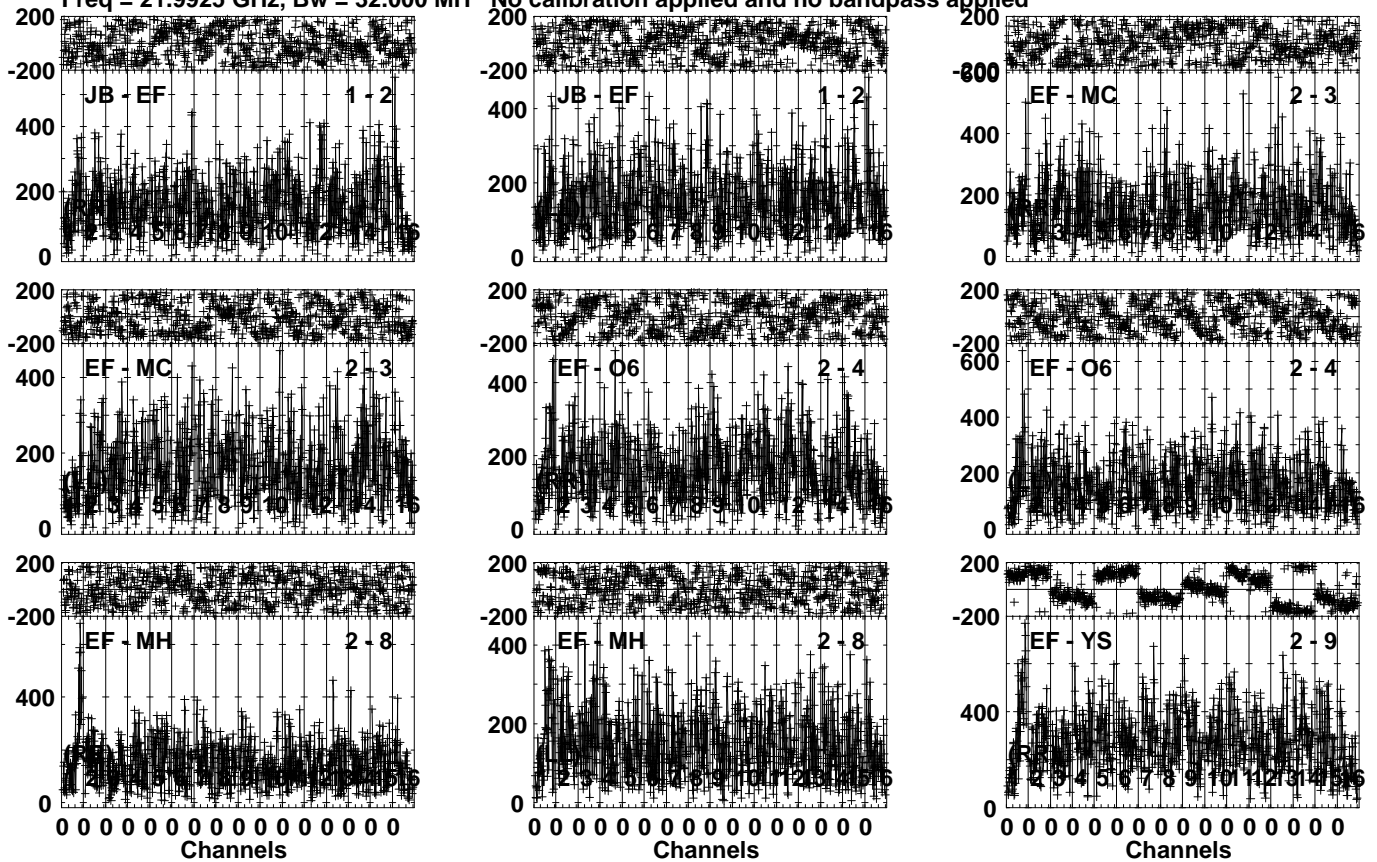
Lower frame: Micro Ampl Jy Top frame: Phas deg Vector averaged cross-power spectrum Several baselines displayed Timerange: 00/19:23:13 to 00/19:24:39
