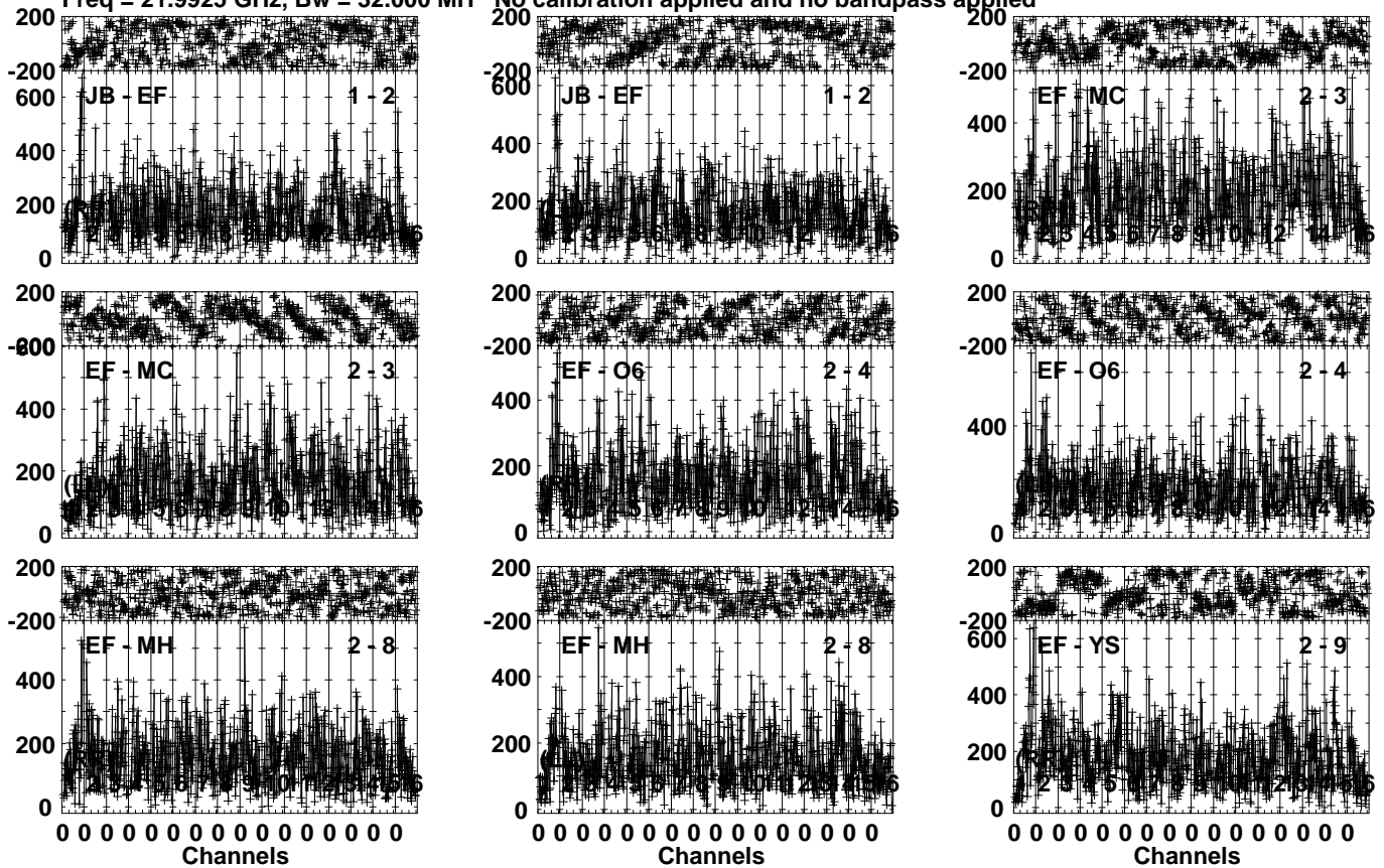
Lower frame: Micro Ampl Jy Top frame: Phas deg Vector averaged cross-power spectrum Several baselines displayed Timerange: 01/04:35:33 to 01/04:36:59
