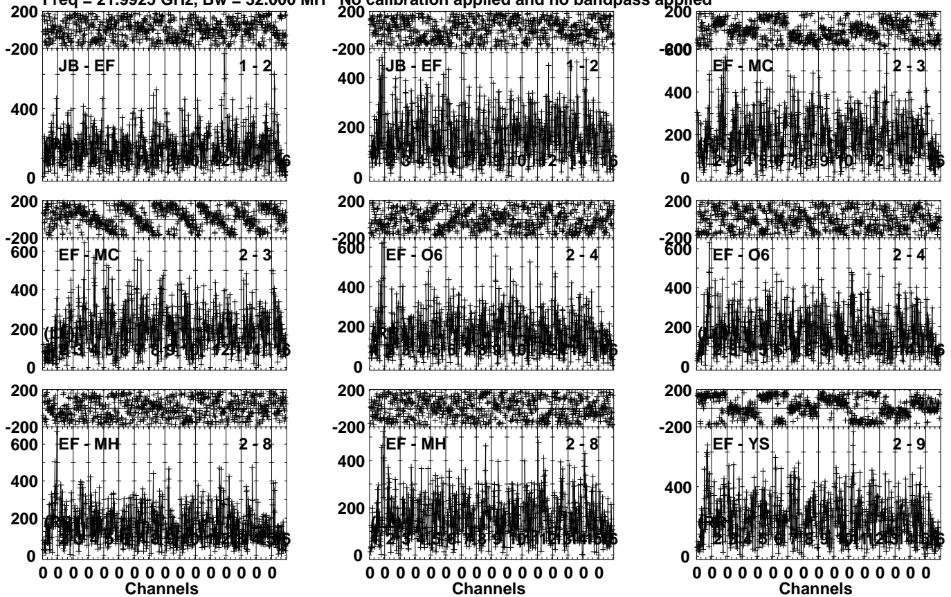
Lower frame: Micro Ampl Jy Top frame: Phas deg Vector averaged cross-power spectrum Several baselines displayed Timerange: 00/22:31:33 to 00/22:32:59
