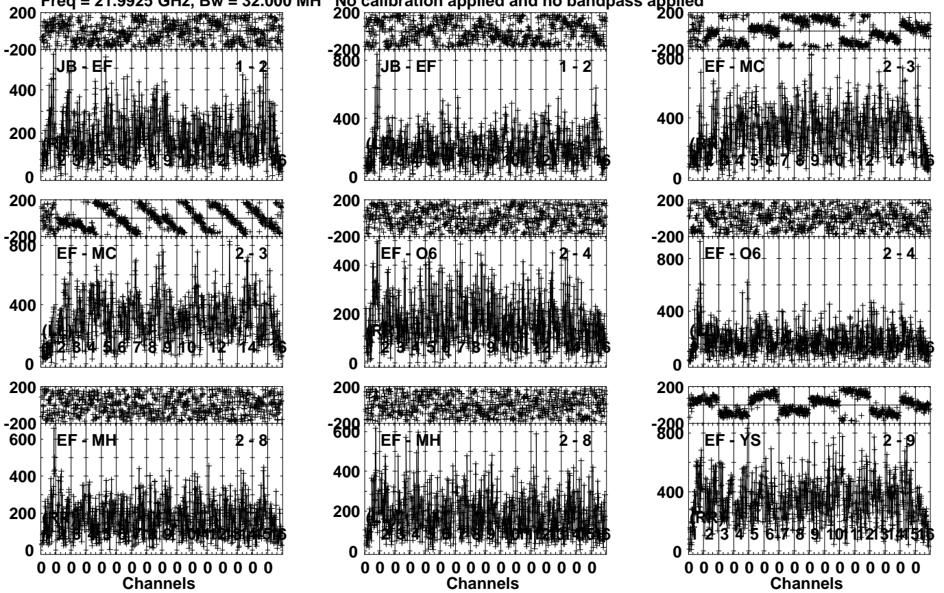
Lower frame: Micro Ampl Jy Top frame: Phas deg Vector averaged cross-power spectrum Several baselines displayed Timerange: 01/02:21:13 to 01/02:22:39
