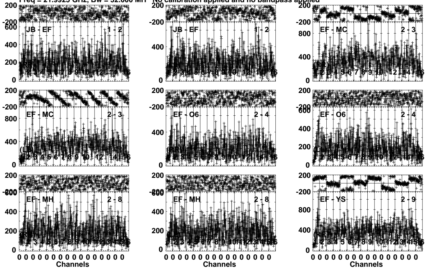
Lower frame: Micro Ampl Jy Top frame: Phas deg Vector averaged cross-power spectrum Several baselines displayed Timerange: 01/02:12:13 to 01/02:13:39
