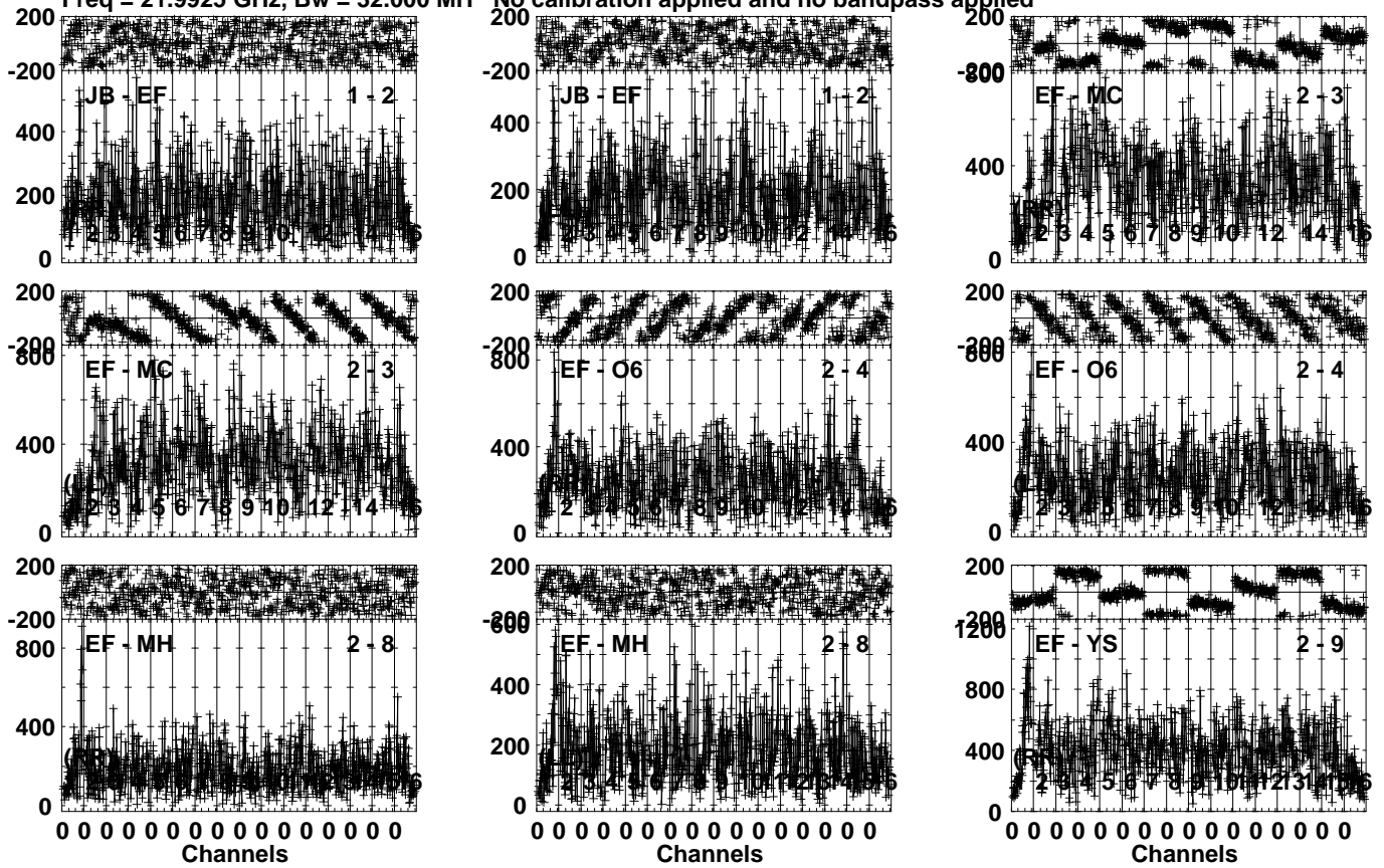
Lower frame: Micro Ampl Jy Top frame: Phas deg Vector averaged cross-power spectrum Several baselines displayed Timerange: 01/02:11:13 to 01/02:12:09
