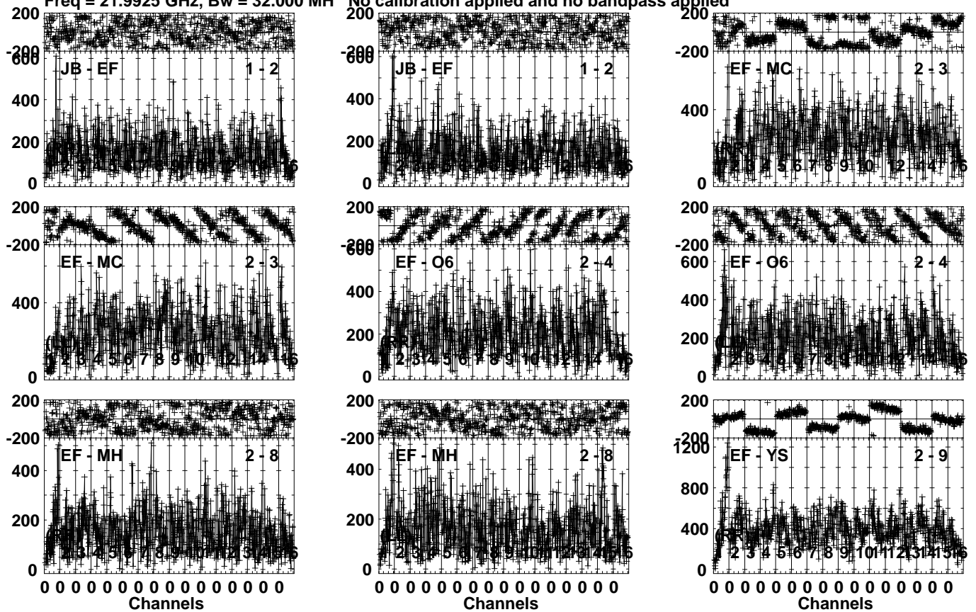
Lower frame: Micro Ampl Jy Top frame: Phas deg Vector averaged cross-power spectrum Several baselines displayed Timerange: 01/03:25:33 to 01/03:26:29
