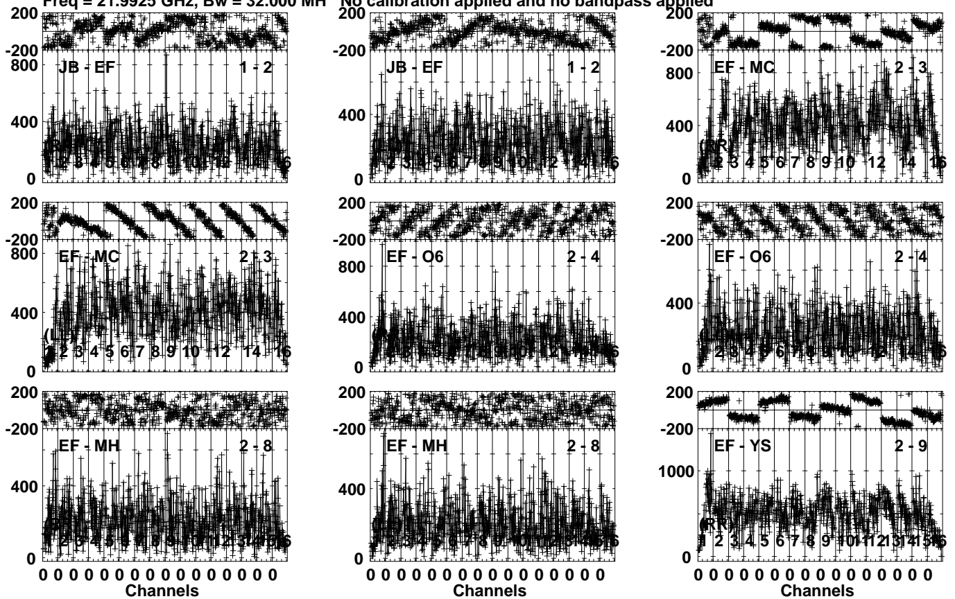
Lower frame: Micro Ampl Jy Top frame: Phas deg Vector averaged cross-power spectrum Several baselines displayed Timerange: 00/21:42:33 to 00/21:43:29
