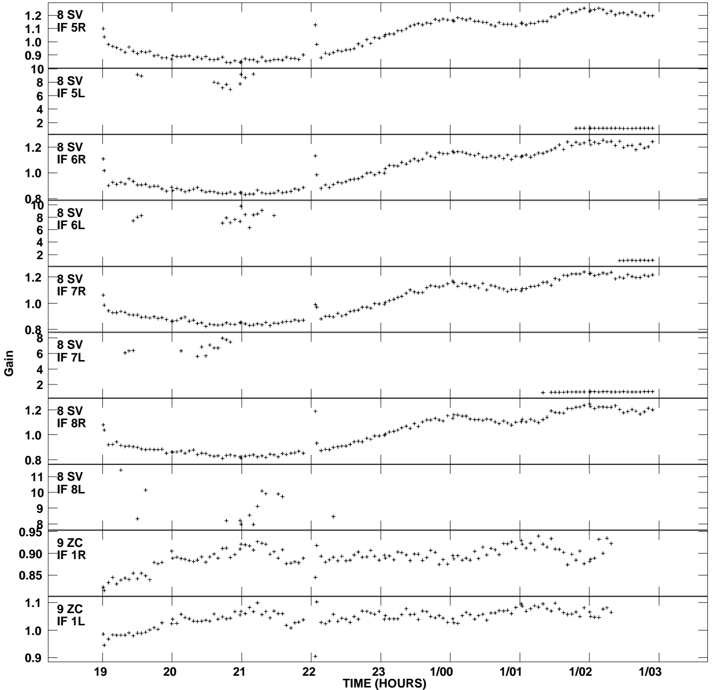
Plot file version 13 created 15-JUN-2012 11:57:36 Gain amp vs UTC time for J1044+0655.MULTI.1 SN 2 Rpol & Lpol IF 1 - 8
