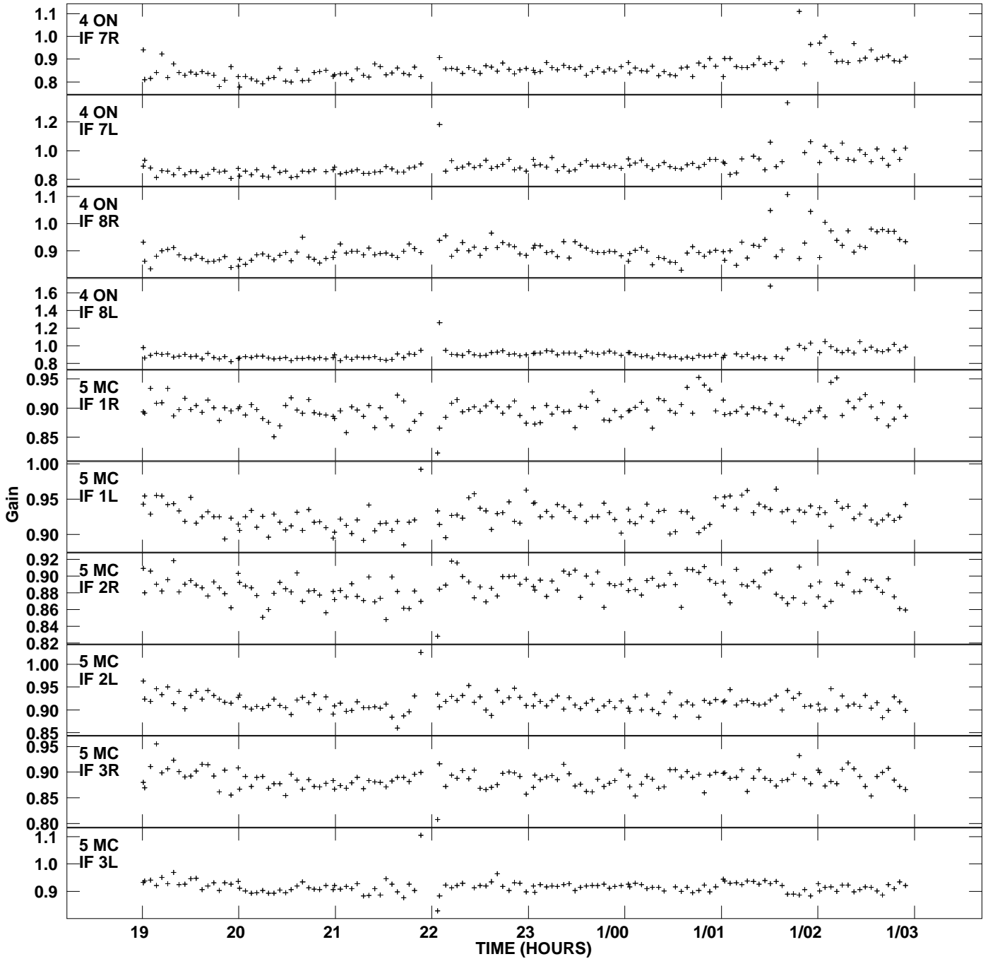
Plot file version 7 created 15-JUN-2012 11:57:36 Gain amp vs UTC time for J1044+0655.MULTI.1 SN 2 Rpol & Lpol IF 1 - 8
