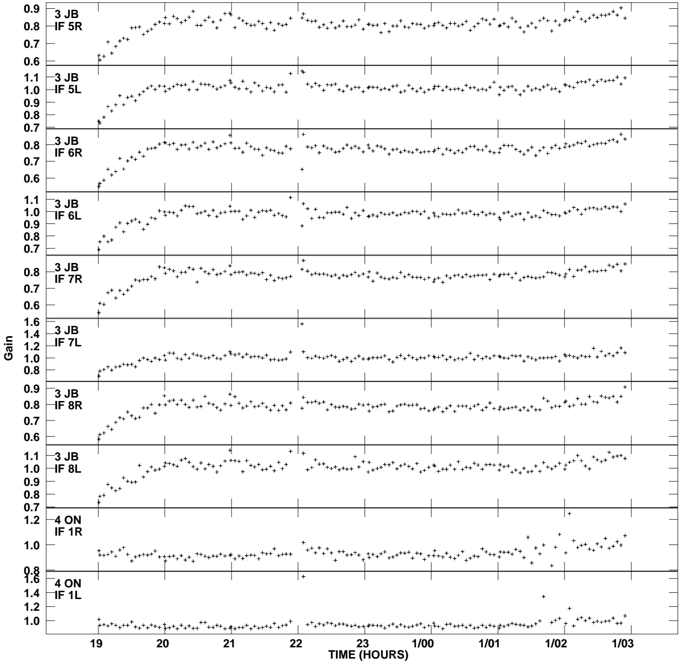
Plot file version 5 created 15-JUN-2012 11:57:36 Gain amp vs UTC time for J1044+0655.MULTI.1 SN 2 Rpol & Lpol IF 1 - 8
