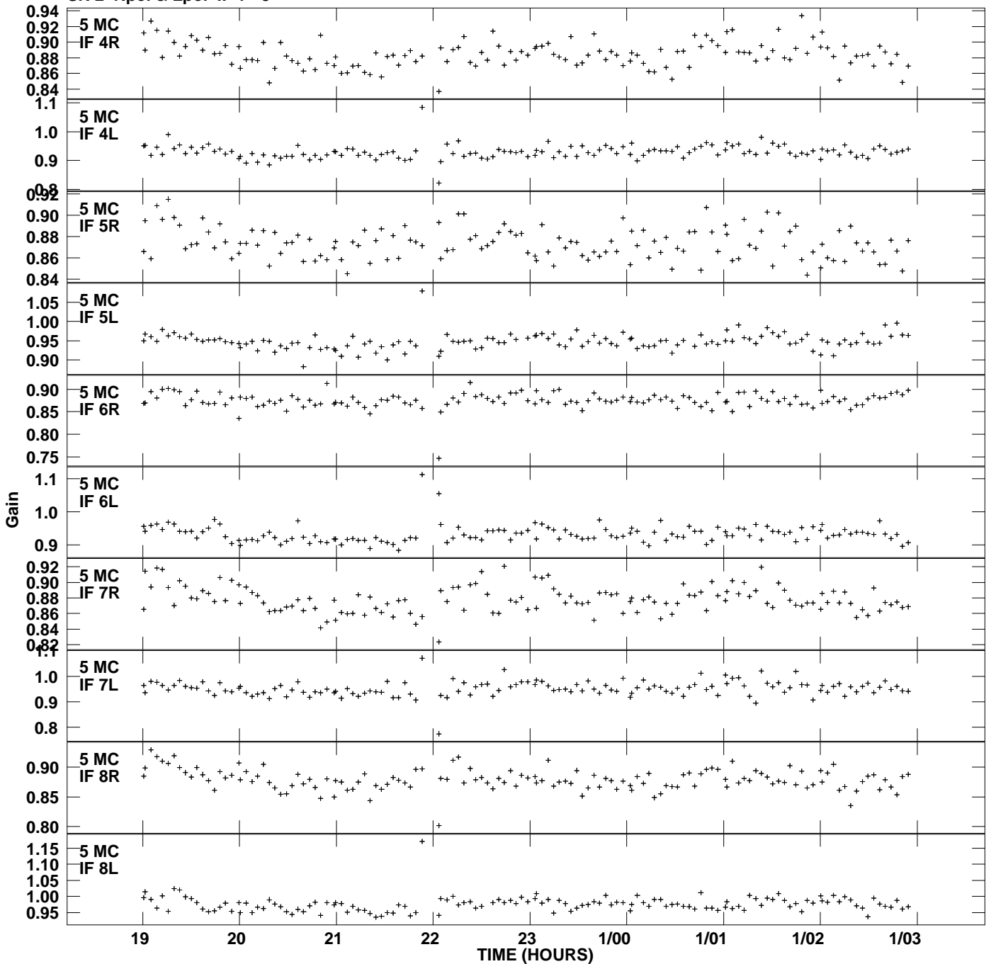
Plot file version 8 created 15-JUN-2012 11:57:36 Gain amp vs UTC time for J1044+0655.MULTI.1 SN 2 Rpol & Lpol IF 1 - 8
