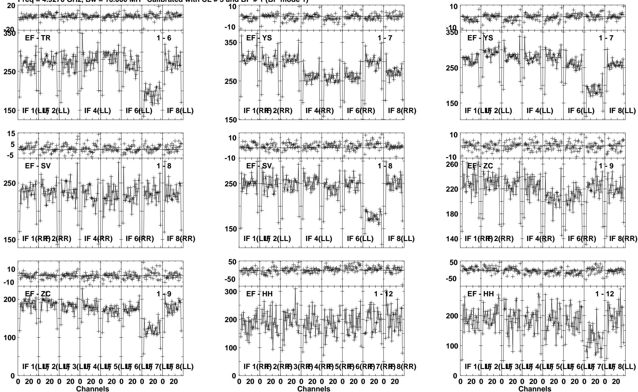
Lower frame: Milli Ampl Jy Top frame: Phas deg Vector averaged cross-power spectrum Several baselines displayed Timerange: 01/01:29:57 to 01/01:31:00
