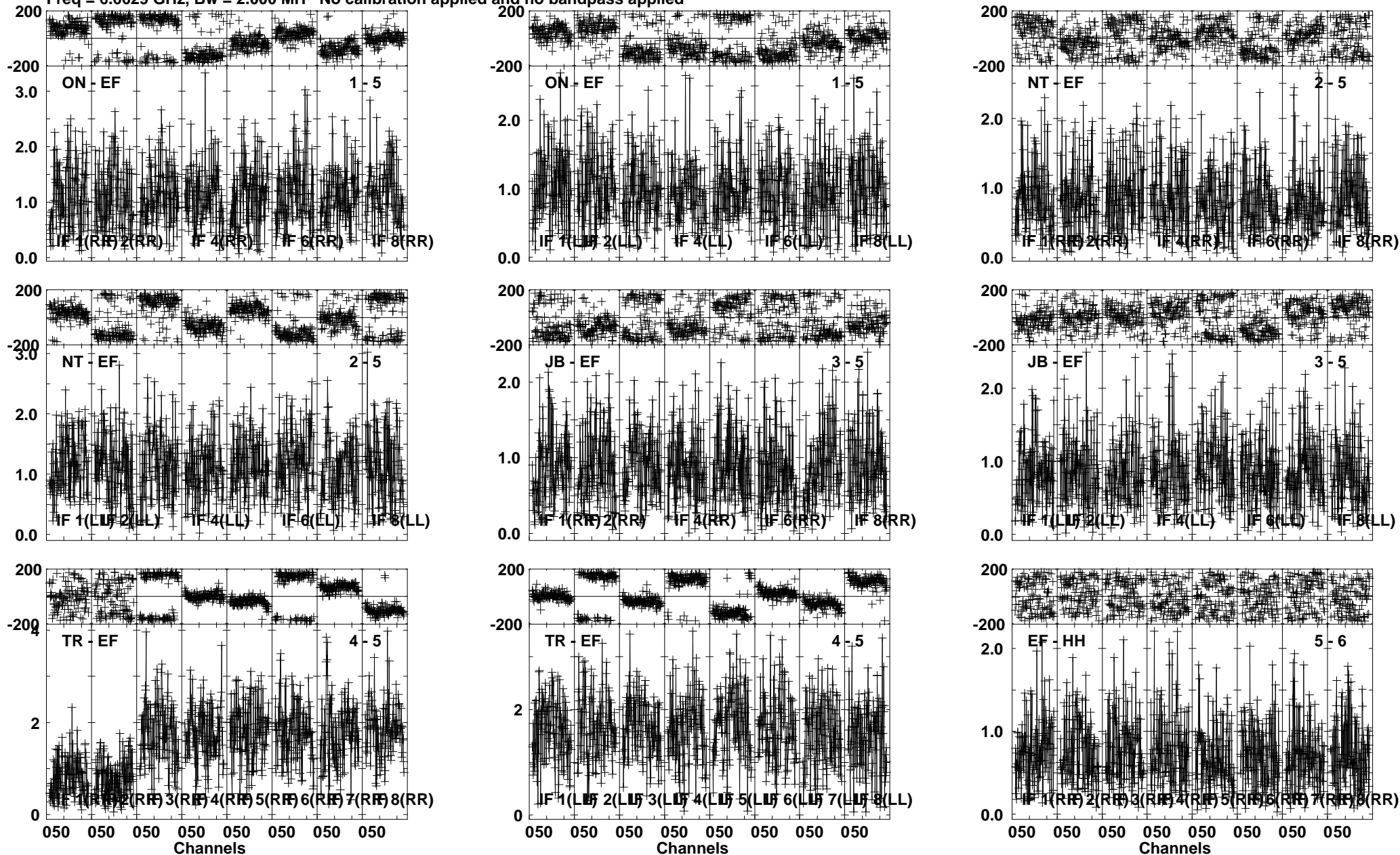
Lower frame: Milli Ampl Jy Top frame: Phas deg Vector averaged cross-power spectrum Several baselines displayed Timerange: 00/05:45:17 to 00/05:46:59
