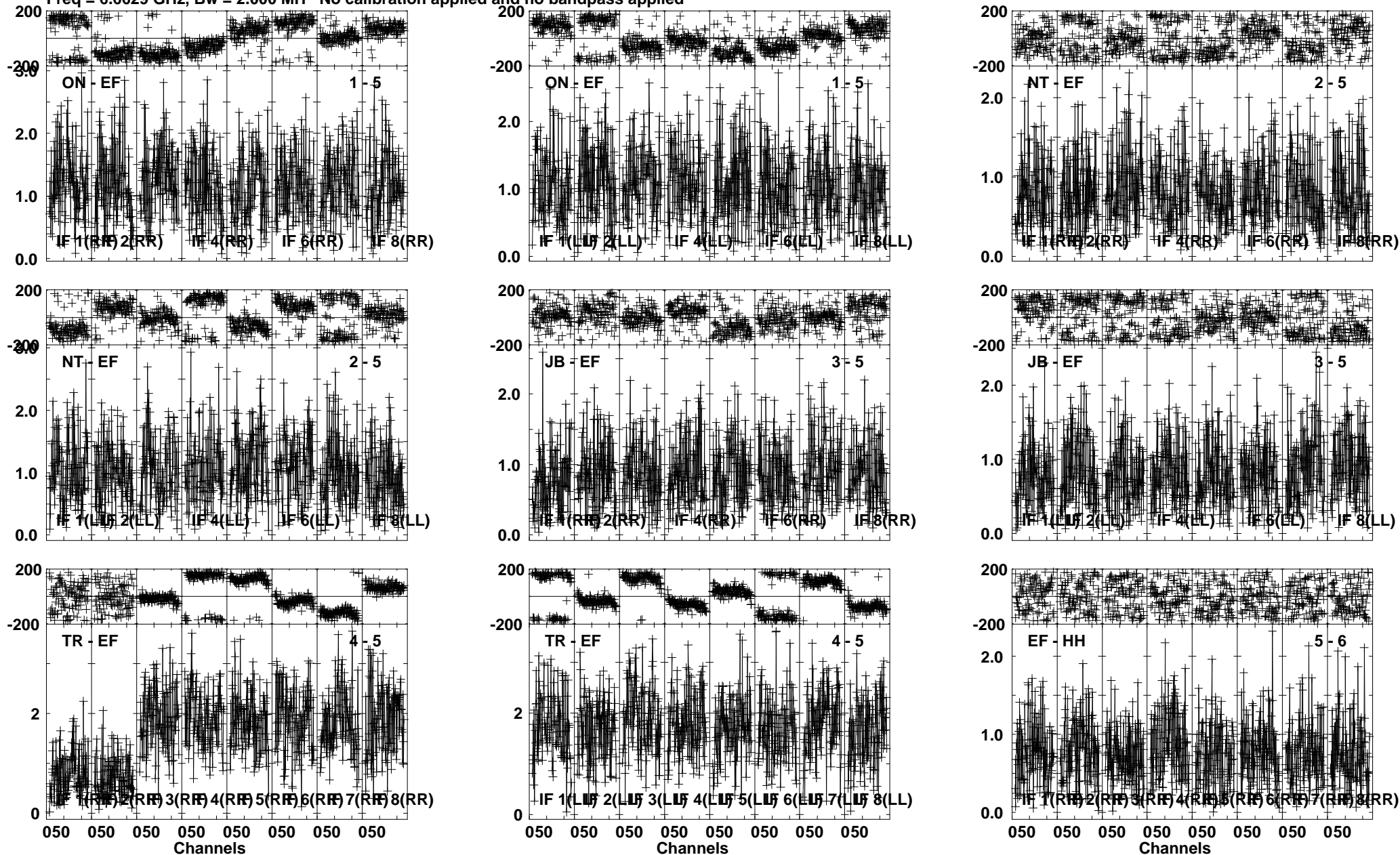
Lower frame: Milli Ampl Jy Top frame: Phas deg Vector averaged cross-power spectrum Several baselines displayed Timerange: 00/06:50:25 to 00/06:52:07
