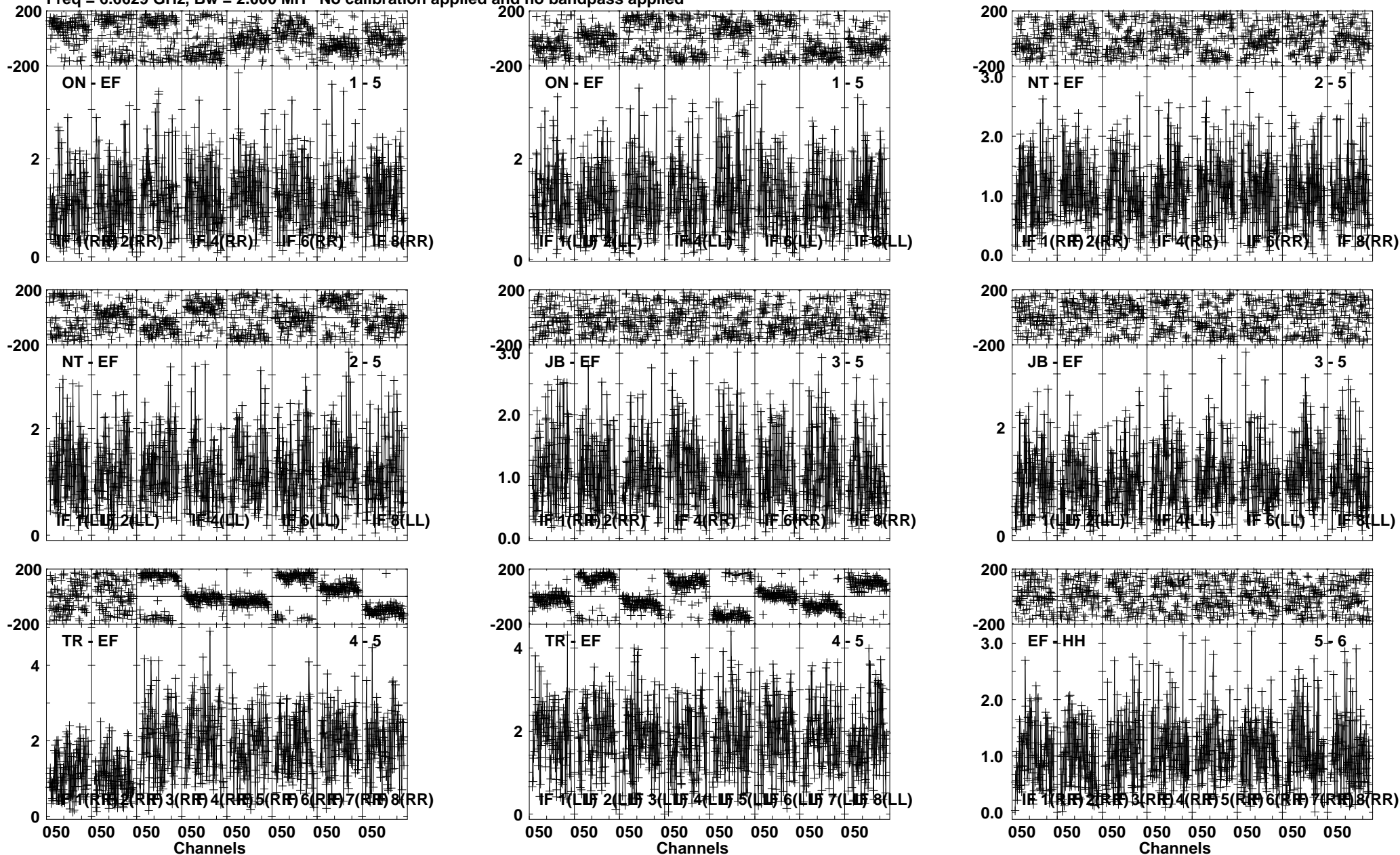
Lower frame: Milli Ampl Jy Top frame: Phas deg Vector averaged cross-power spectrum Several baselines displayed Timerange: 00/10:34:35 to 00/10:36:07
