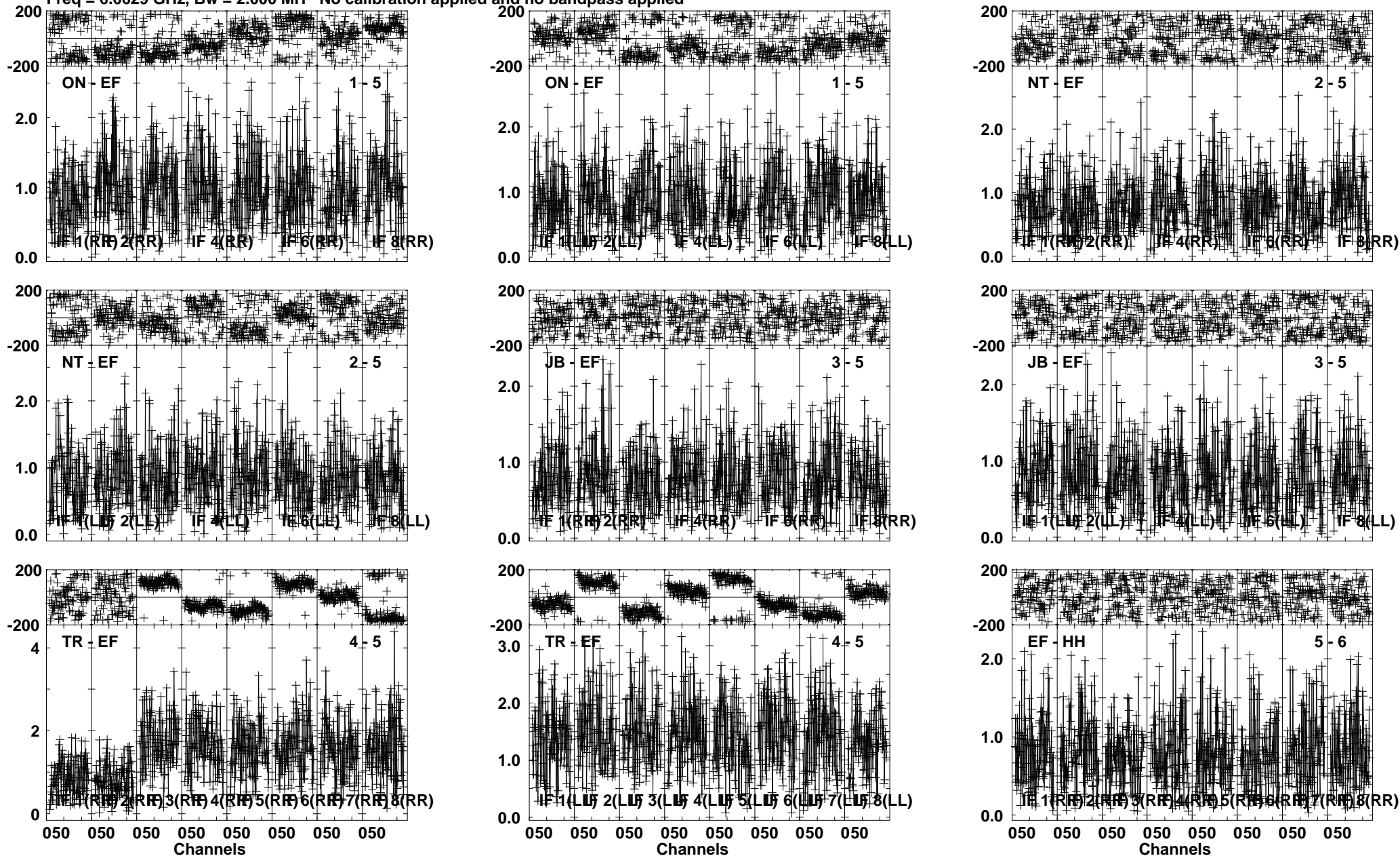
Lower frame: Milli Ampl Jy Top frame: Phas deg Vector averaged cross-power spectrum Several baselines displayed Timerange: 00/11:16:35 to 00/11:18:17
