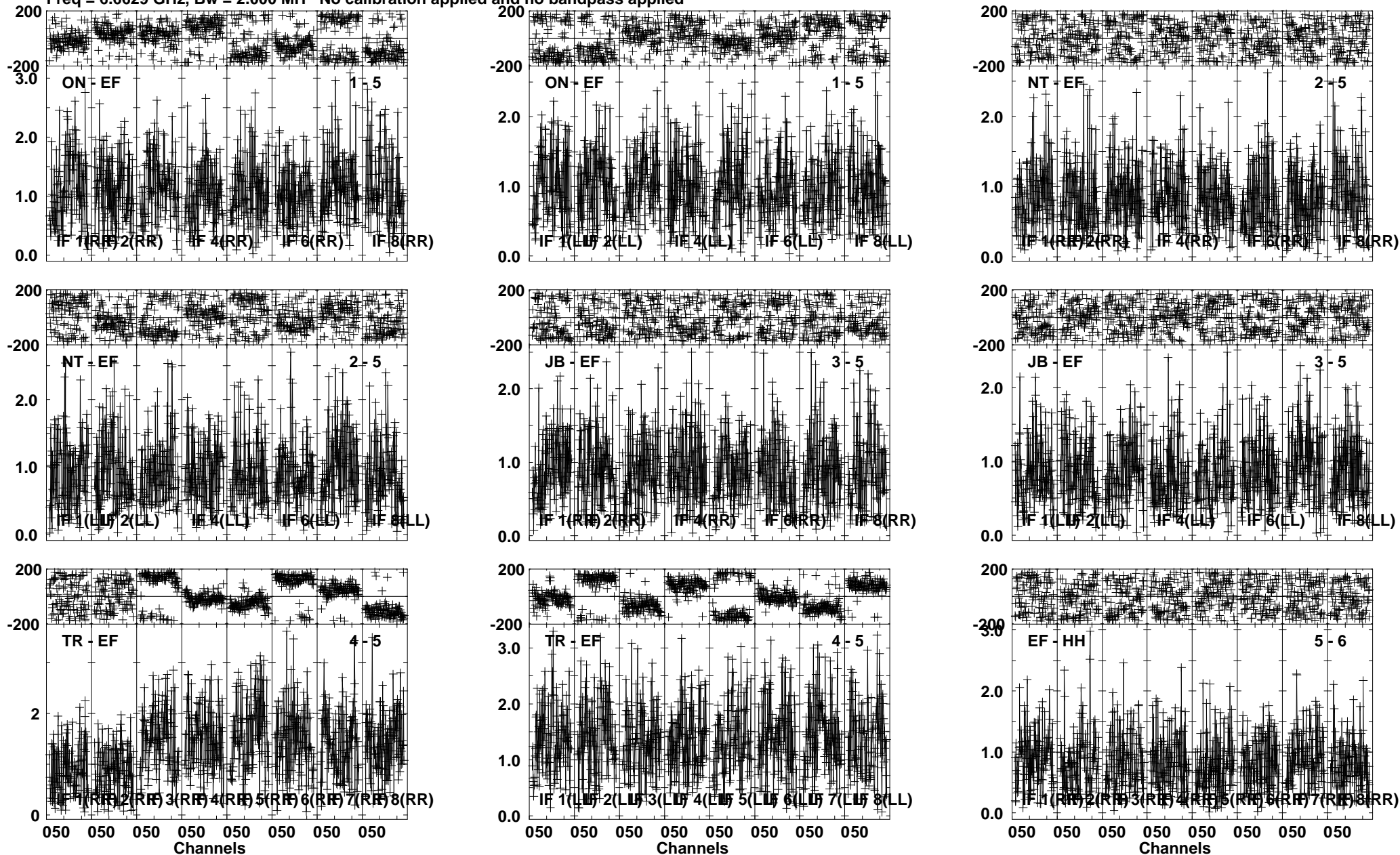
Lower frame: Milli Ampl Jy Top frame: Phas deg Vector averaged cross-power spectrum Several baselines displayed Timerange: 00/11:05:55 to 00/11:07:37
