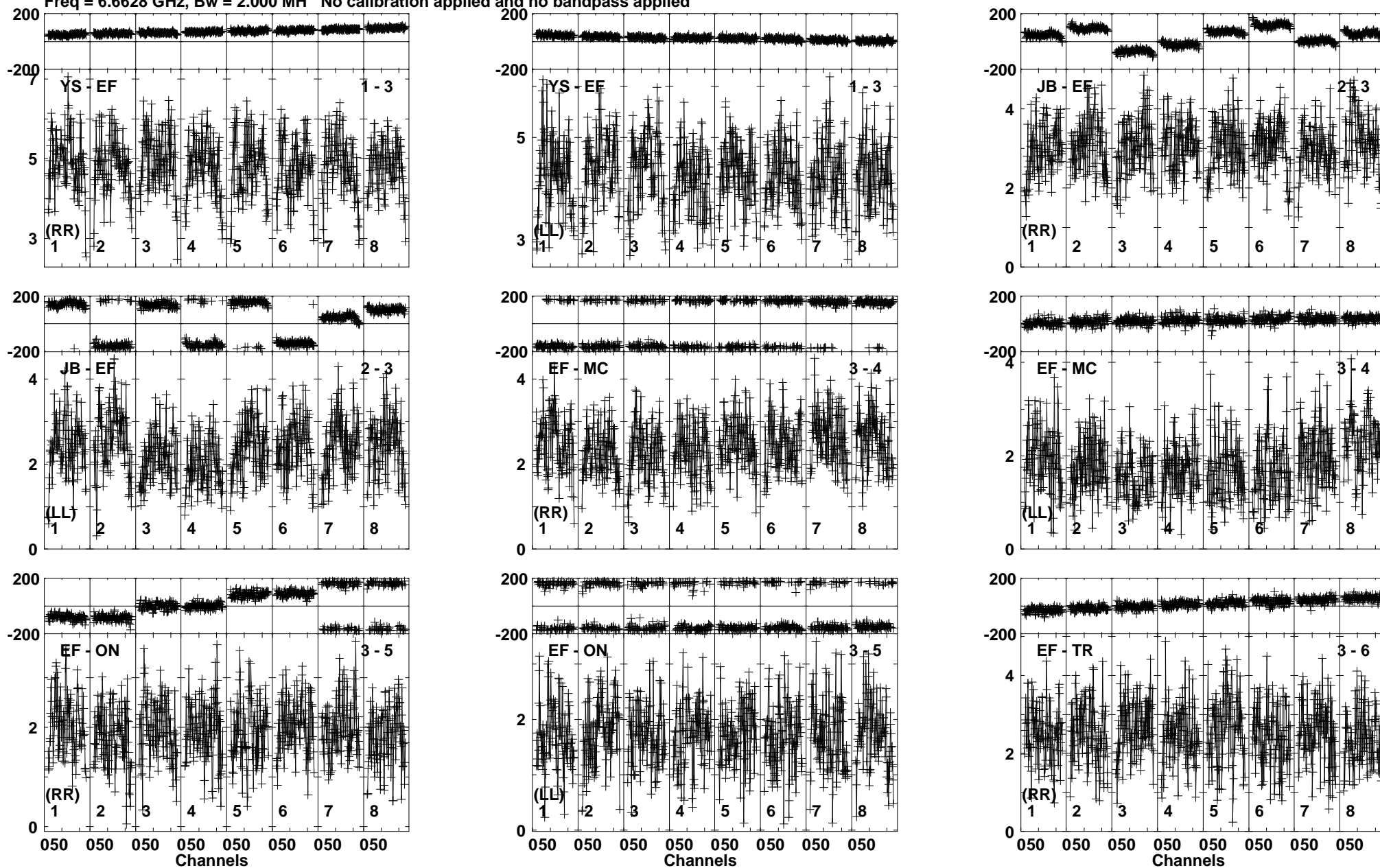
Lower frame: Milli Ampl Jy Top frame: Phas deg Vector averaged cross-power spectrum Baseline: YS (01) - EF (03) Timerange: 00/04:37:36 to 00/04:39:12
