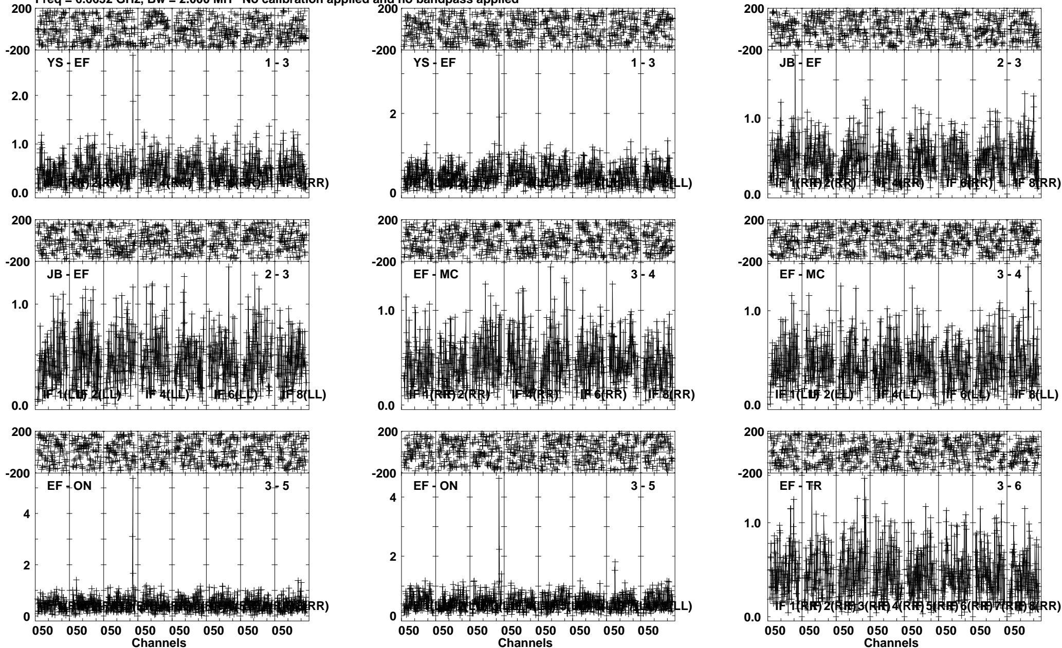
Lower frame: Milli Ampl Jy Top frame: Phas deg Vector averaged cross-power spectrum Several baselines displayed Timerange: 00/09:00:22 to 00/09:03:34
