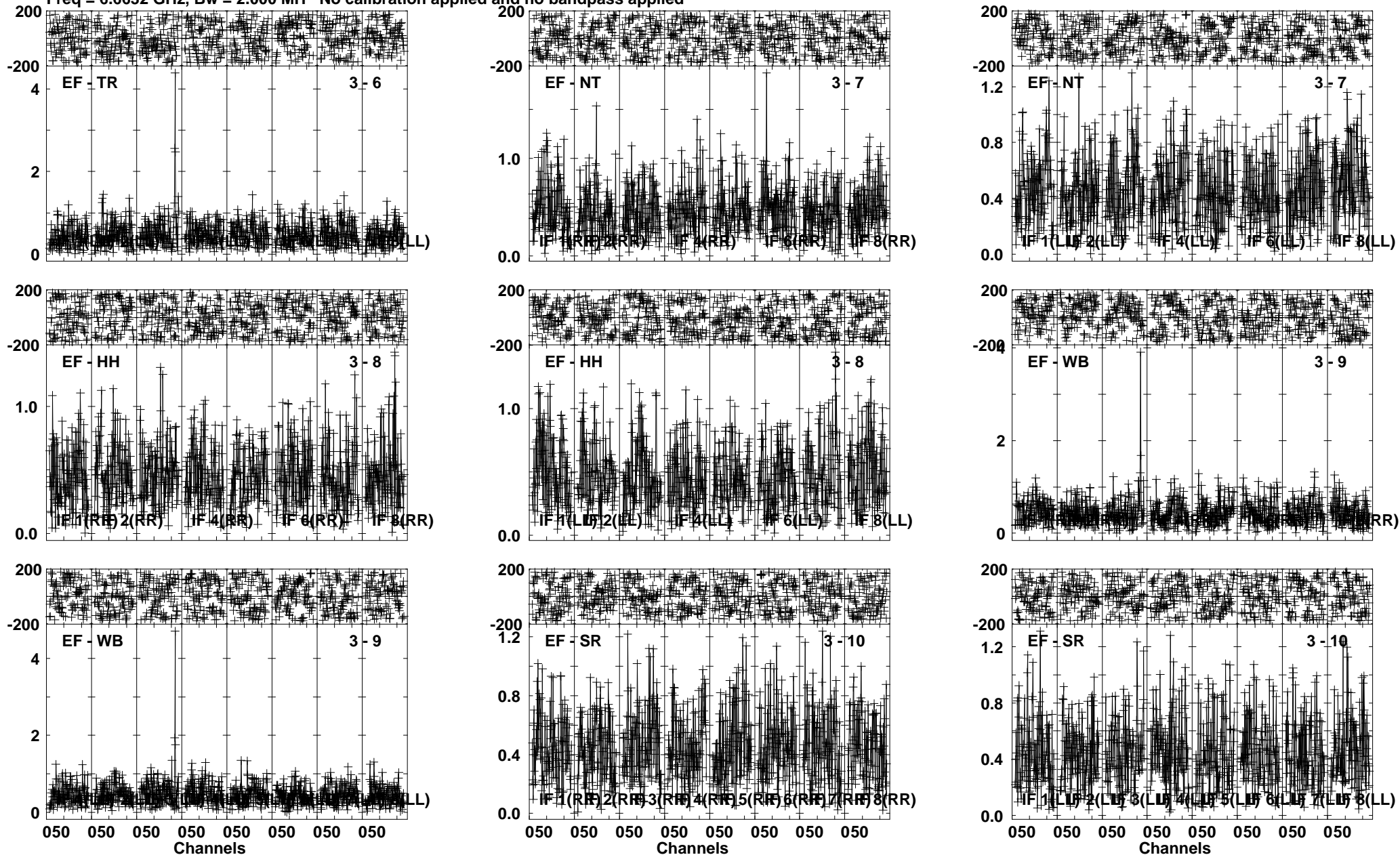
Lower frame: Milli Ampl Jy Top frame: Phas deg Vector averaged cross-power spectrum Several baselines displayed Timerange: 00/09:16:42 to 00/09:19:54
