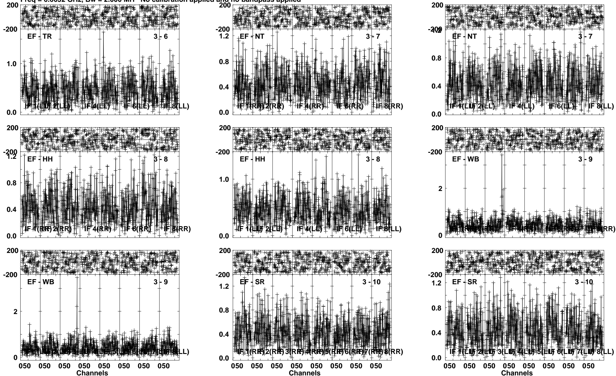
Lower frame: Milli Ampl Jy Top frame: Phas deg Vector averaged cross-power spectrum Several baselines displayed Timerange: 00/03:03:14 to 00/03:06:26
