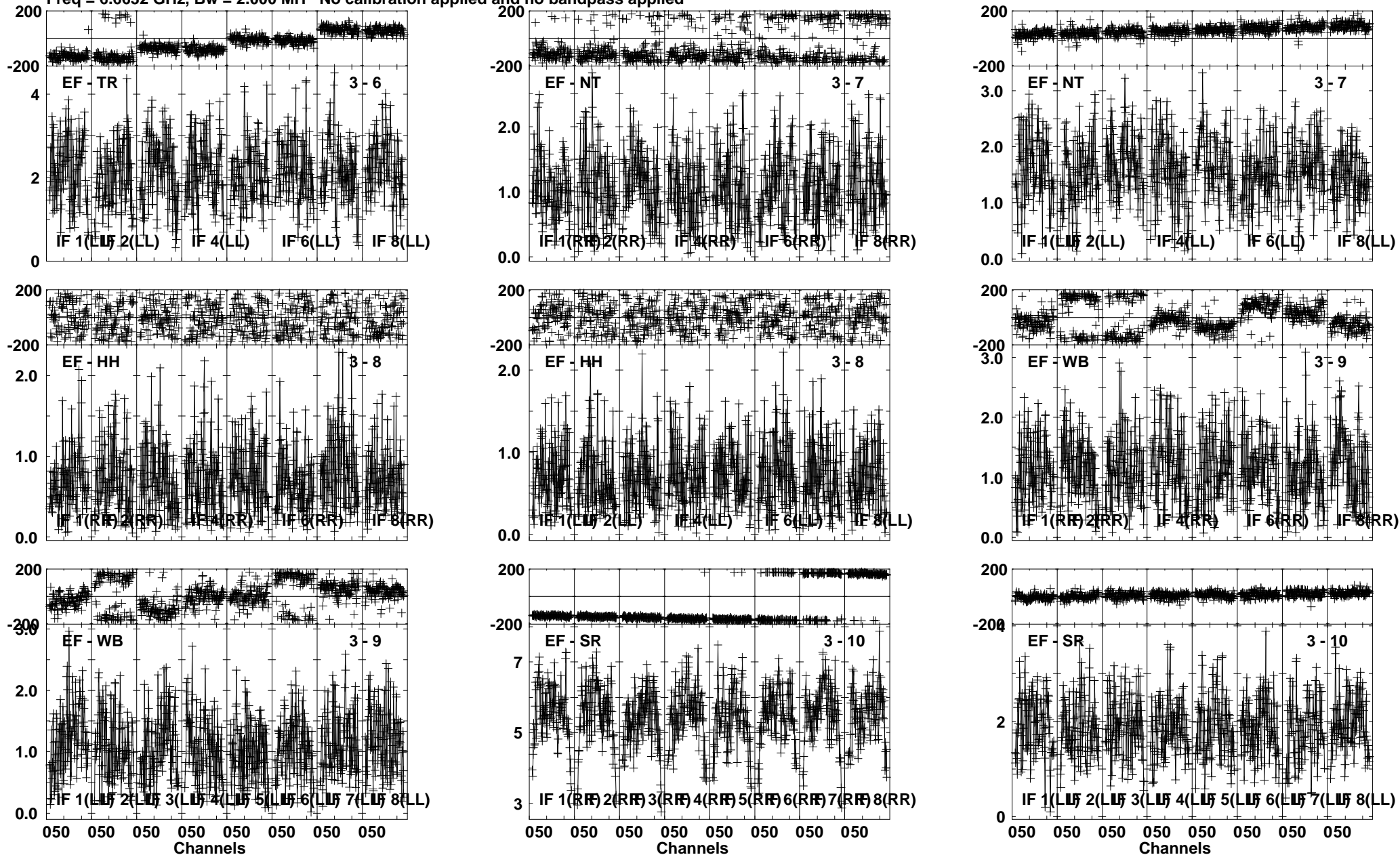
Lower frame: Milli Ampl Jy Top frame: Phas deg Vector averaged cross-power spectrum Several baselines displayed Timerange: 00/02:55:55 to 00/02:57:31
