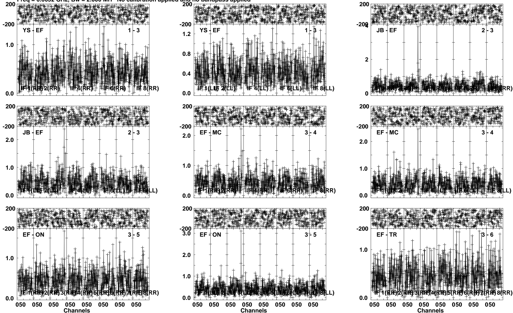
Lower frame: Milli Ampl Jy Top frame: Phas deg Vector averaged cross-power spectrum Several baselines displayed Timerange: 00/05:46:34 to 00/05:49:46
