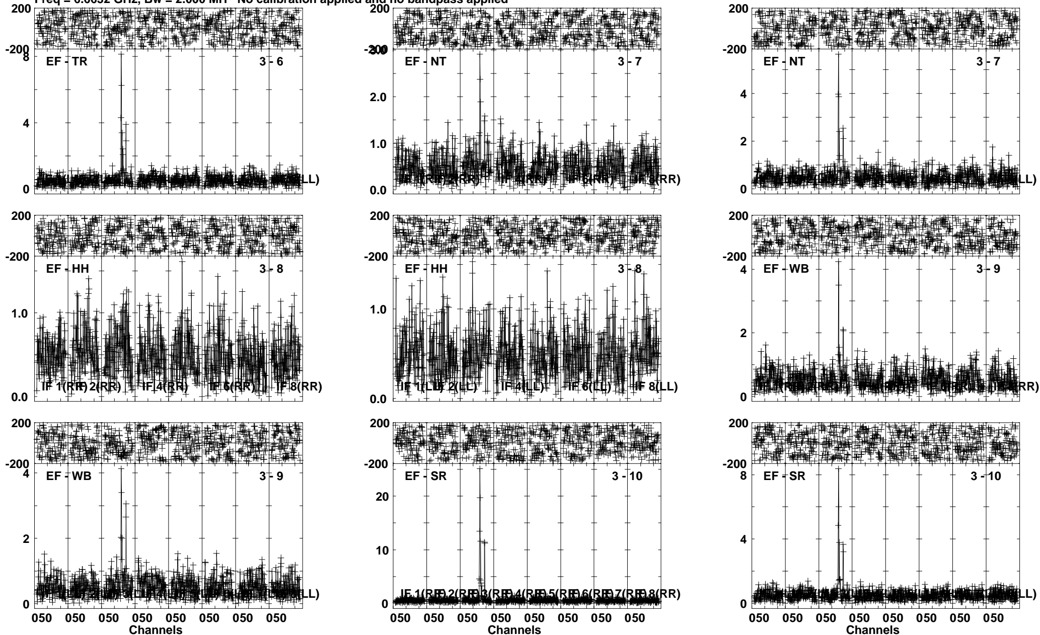
Lower frame: Milli Ampl Jy Top frame: Phas deg Vector averaged cross-power spectrum Several baselines displayed Timerange: 00/07:11:49 to 00/07:14:55
