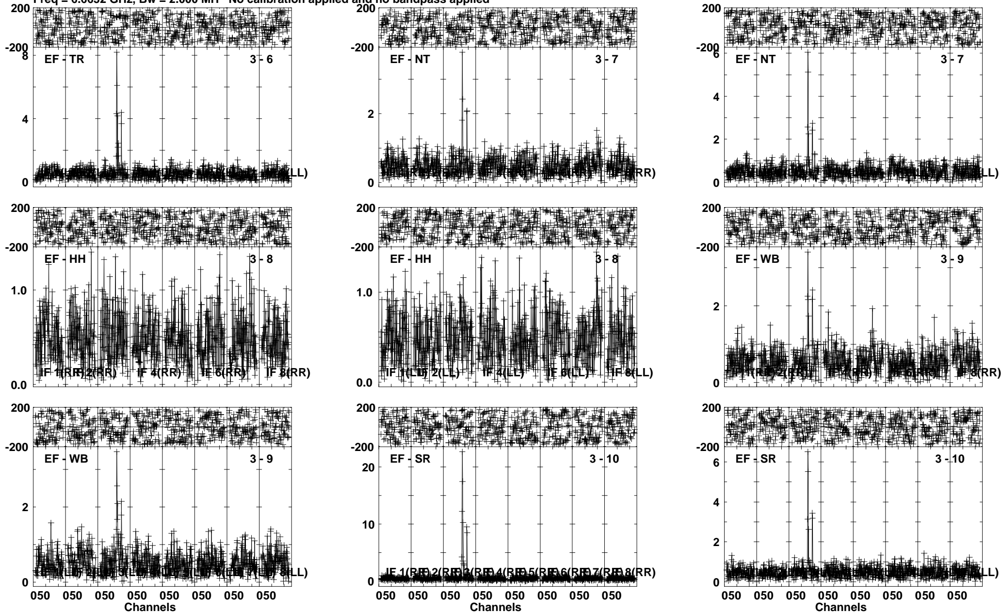
Lower frame: Milli Ampl Jy Top frame: Phas deg Vector averaged cross-power spectrum Several baselines displayed Timerange: 00/07:44:28 to 00/07:47:34
