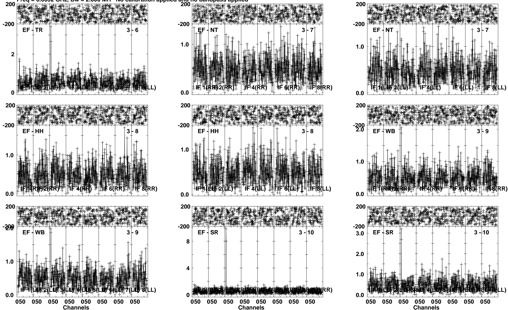
Lower frame: Milli Ampl Jy Top frame: Phas deg Vector averaged cross-power spectrum Several baselines displayed Timerange: 00/08:54:49 to 00/08:57:55
