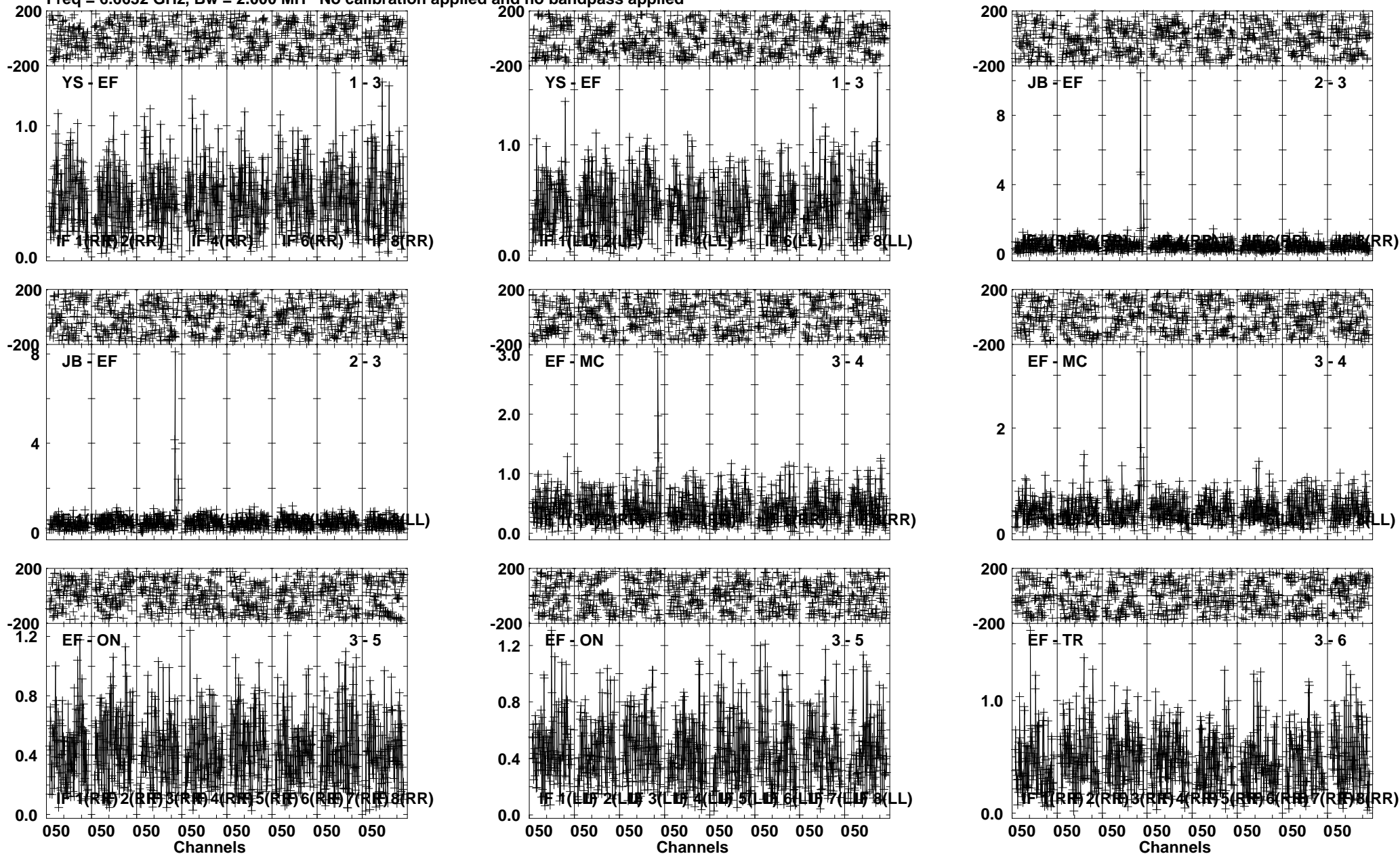
Lower frame: Milli Ampl Jy Top frame: Phas deg Vector averaged cross-power spectrum Several baselines displayed Timerange: 00/03:19:34 to 00/03:22:46
