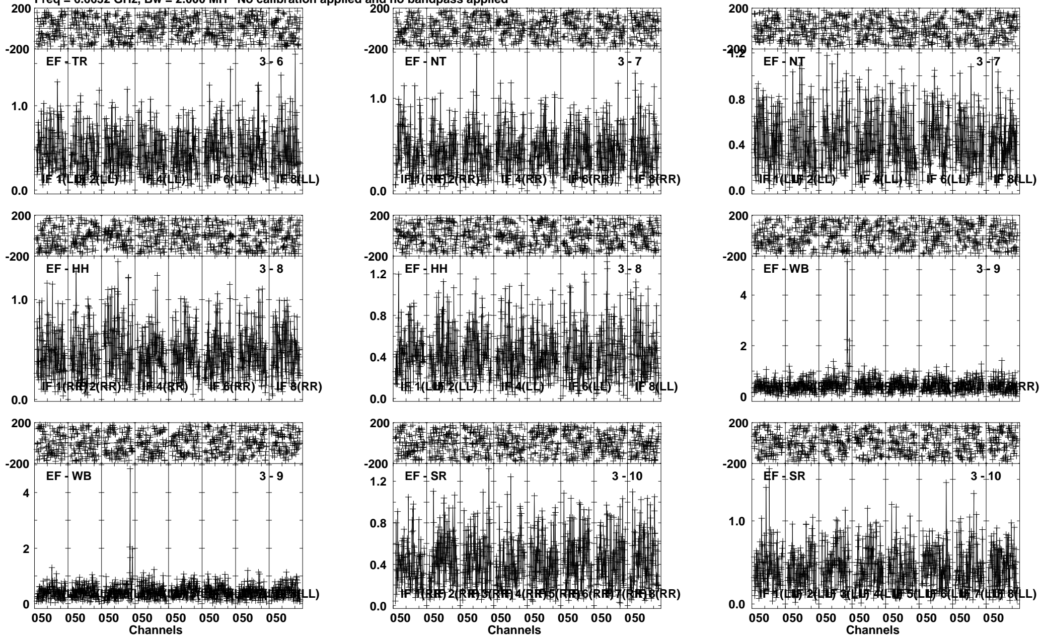
Lower frame: Milli Ampl Jy Top frame: Phas deg Vector averaged cross-power spectrum Several baselines displayed Timerange: 00/04:24:54 to 00/04:28:06
