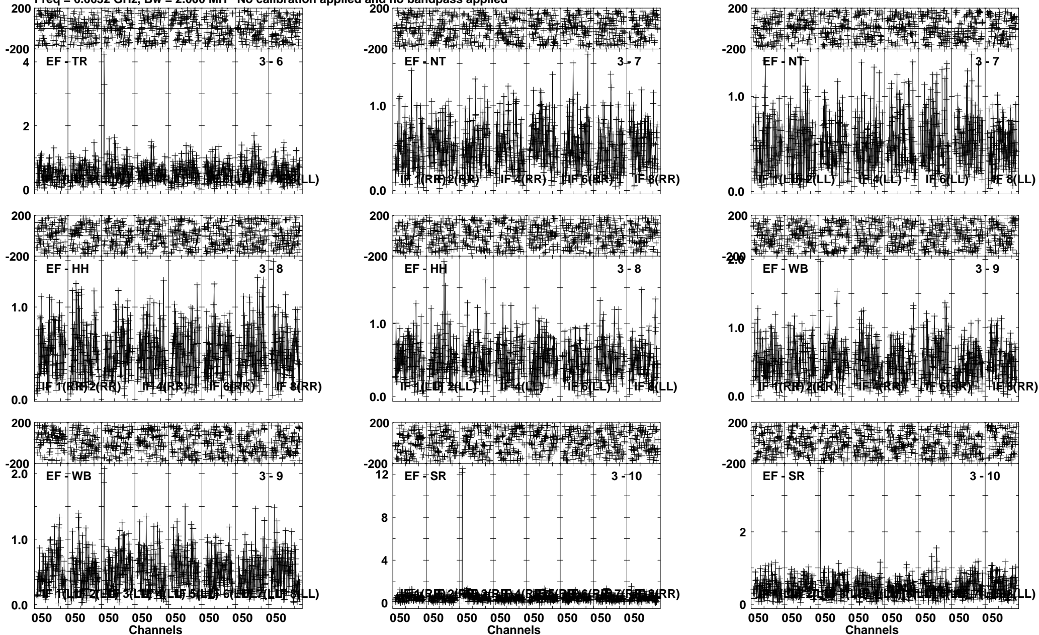
Lower frame: Milli Ampl Jy Top frame: Phas deg Vector averaged cross-power spectrum Several baselines displayed Timerange: 00/07:33:08 to 00/07:36:14
