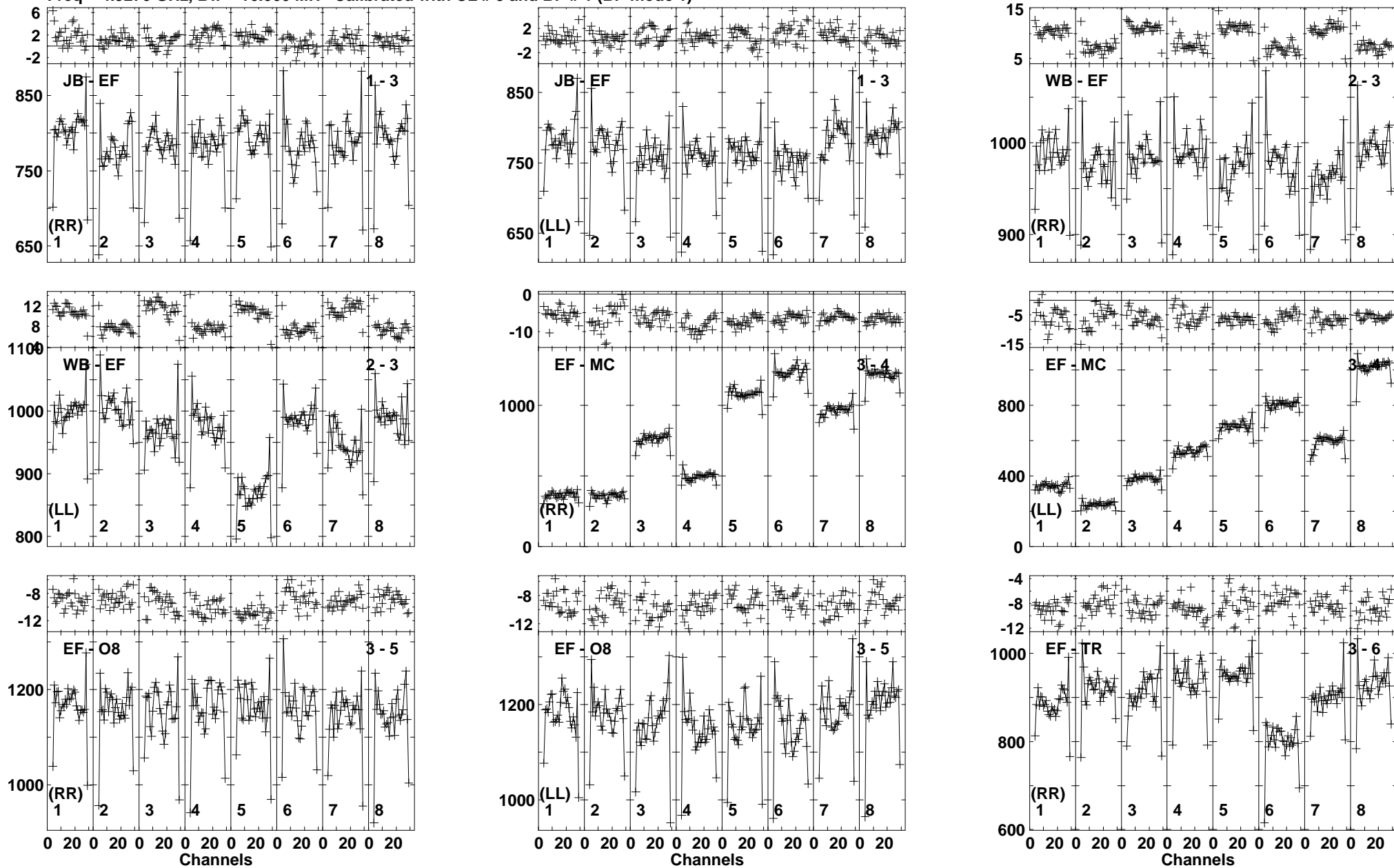
Lower frame: Milli Ampl Jy Top frame: Phas deg Vector averaged cross-power spectrum Baseline: JB (01) - EF (03) Timerange: 00/20/29:03 to 00/20/29:49
