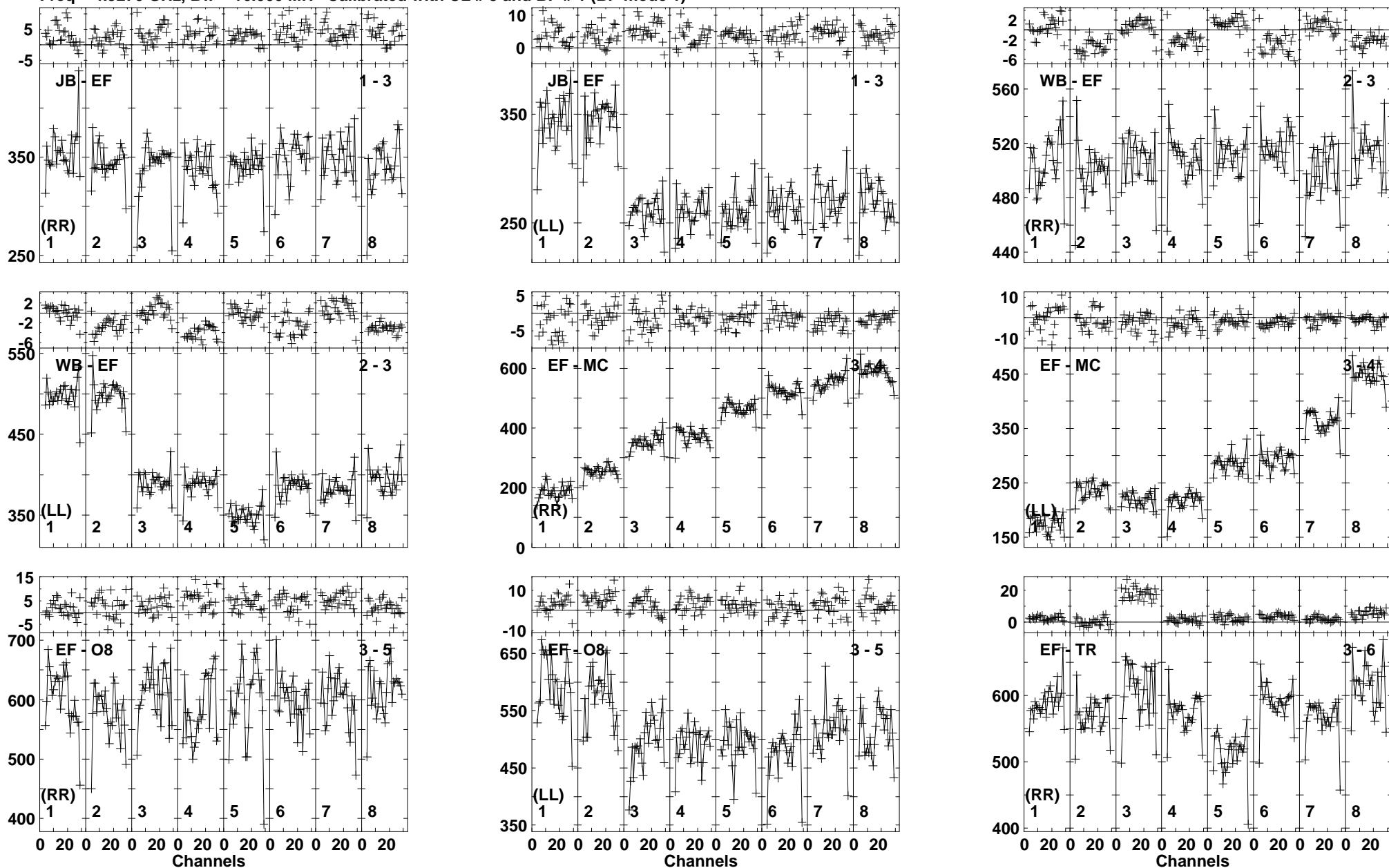
Lower frame: Milli Ampl Jy Top frame: Phas deg Vector averaged cross-power spectrum Baseline: JB (01) - EF (03) Timerange: 00/09:34:53 to 00/09:36:49
