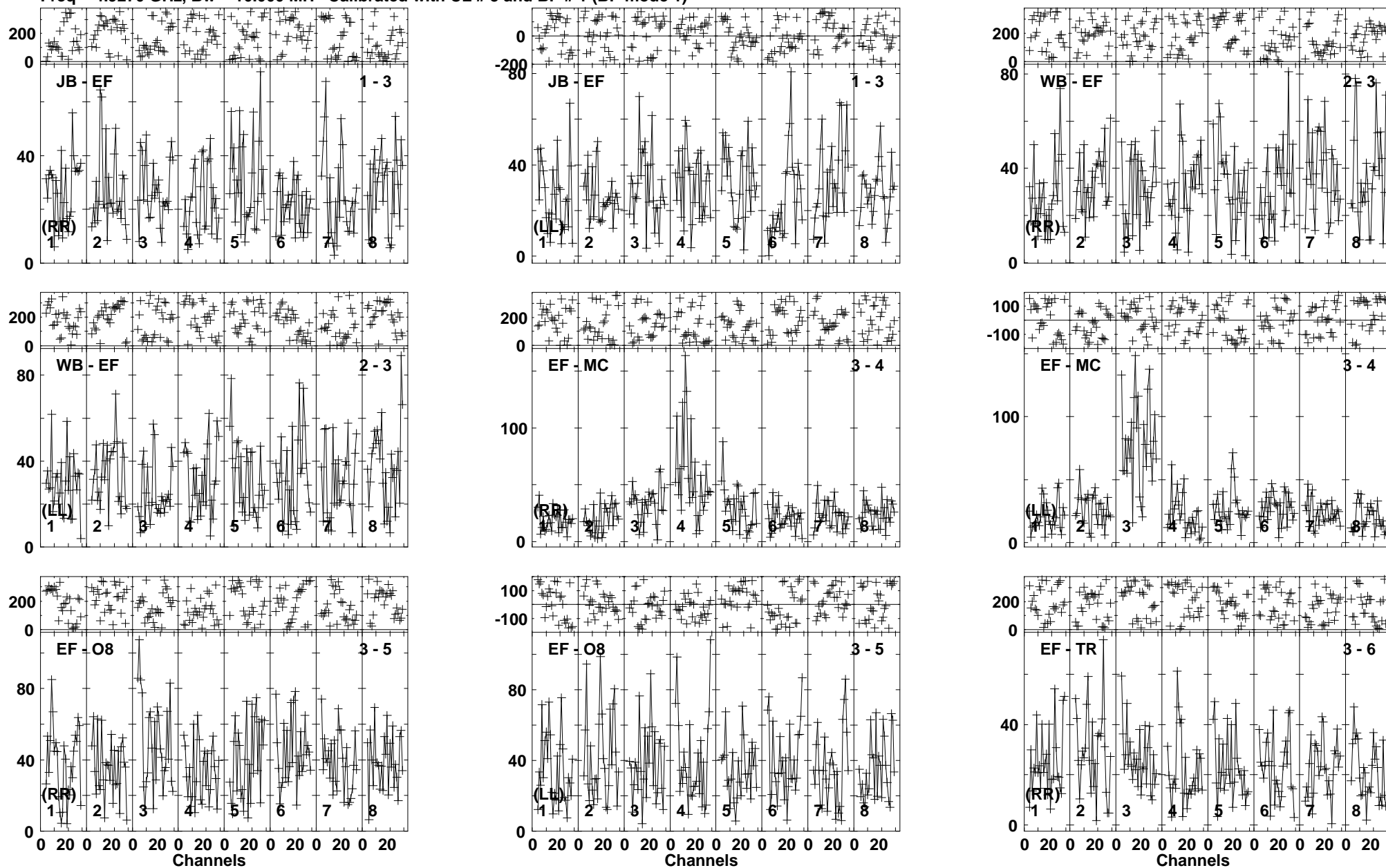
Lower frame: Milli Ampl Jy Top frame: Phas deg Vector averaged cross-power spectrum Baseline: JB (01) - EF (03) Timerange: 00/11:46:45 to 00/11:47:29
