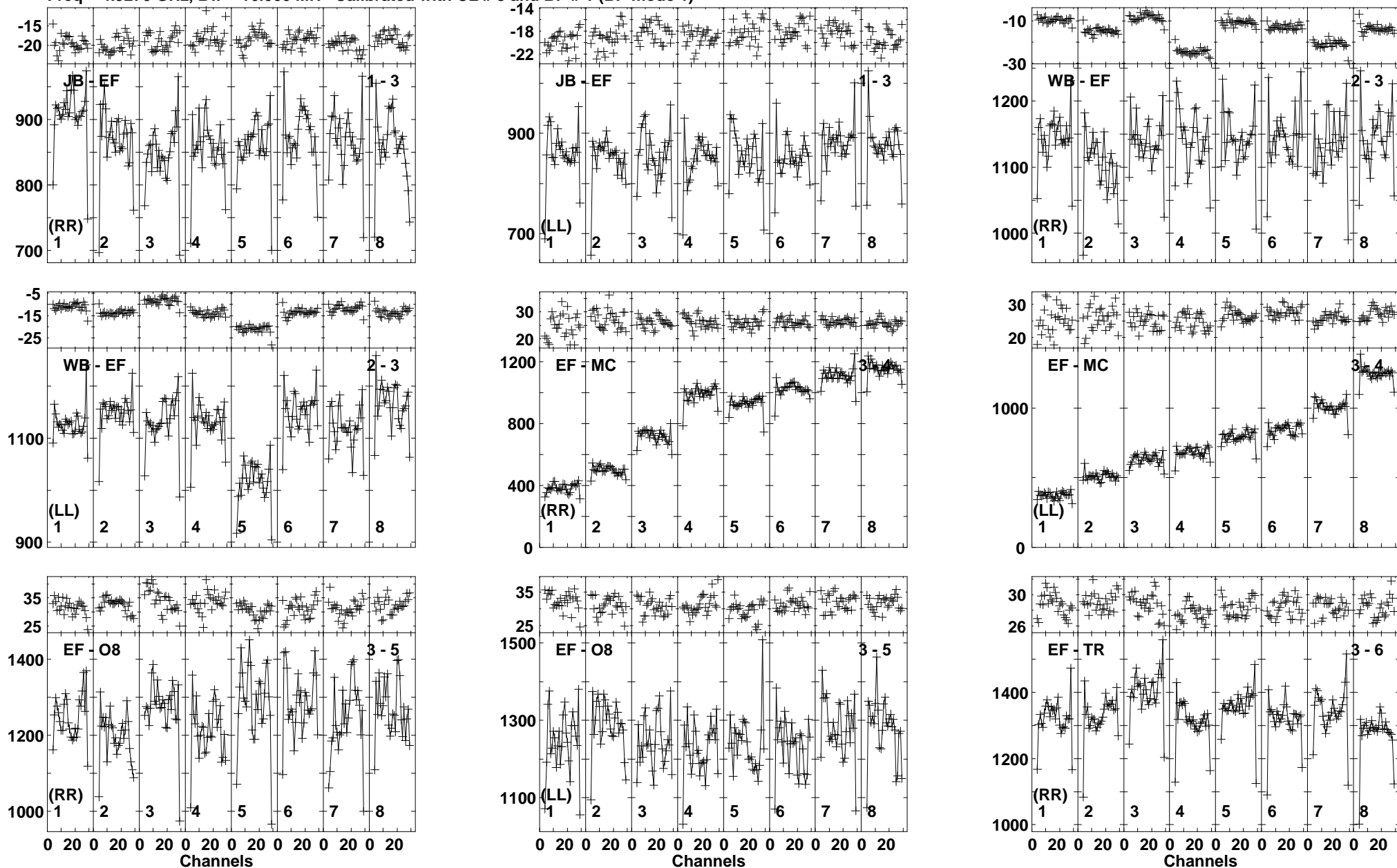
Lower frame: Milli Ampl Jy Top frame: Phas deg Vector averaged cross-power spectrum Baseline: JB (01) - EF (03) Timerange: 00/10:37:55 to 00/10:38:39
