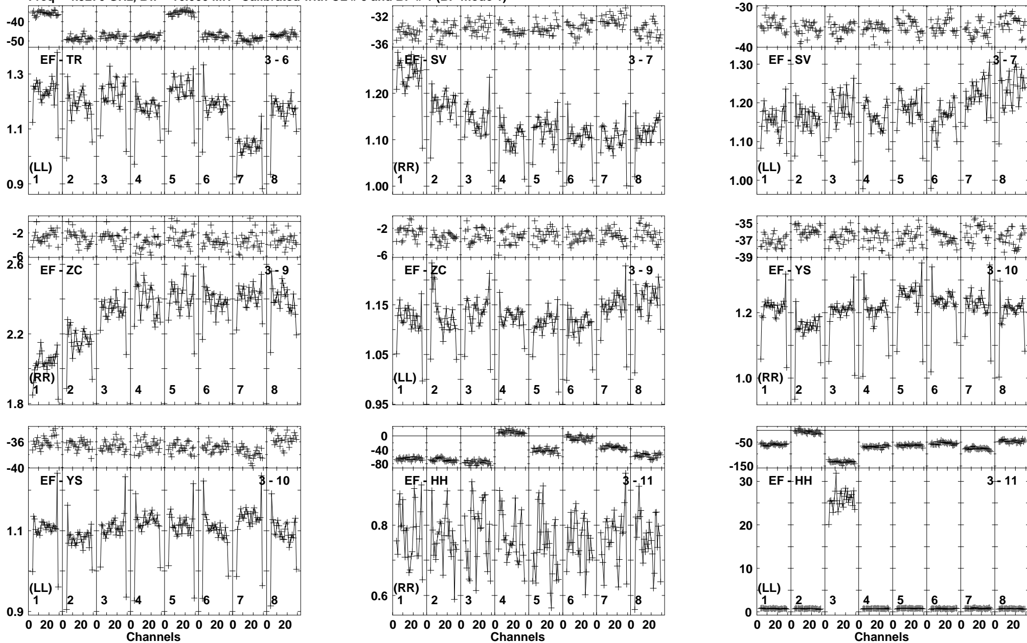
Lower frame: Ampl Jy Top frame: Phas deg Vector averaged cross-power spectrum Baseline: EF (03) - TR (06) Timerange: 00/18:31:33 to 00/18:32:19
