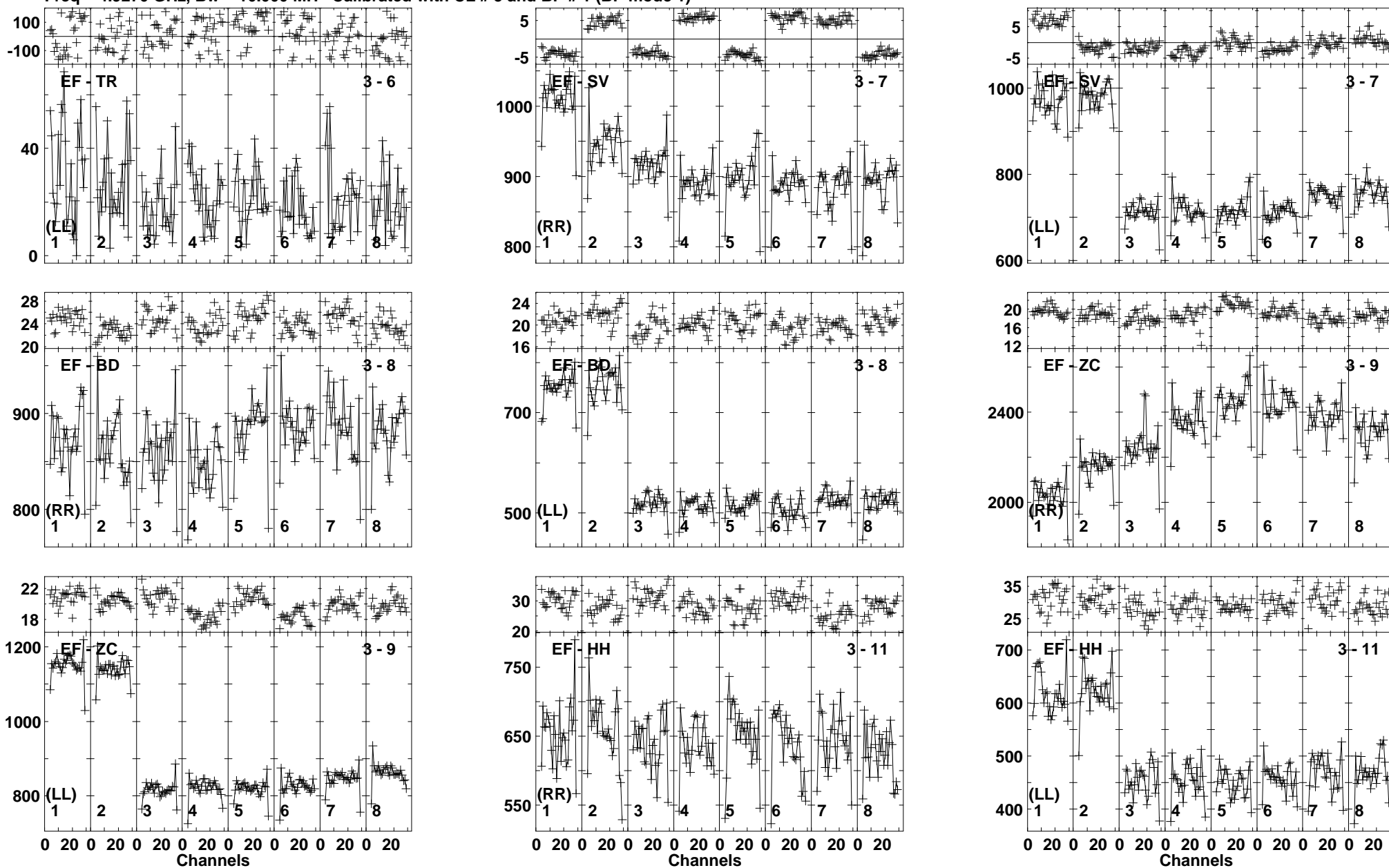
Lower frame: Milli Ampl Jy Top frame: Phas deg Vector averaged cross-power spectrum Baseline: EF (03) - TR (06) Timerange: 00/14:09:26 to 00/14:10:08
