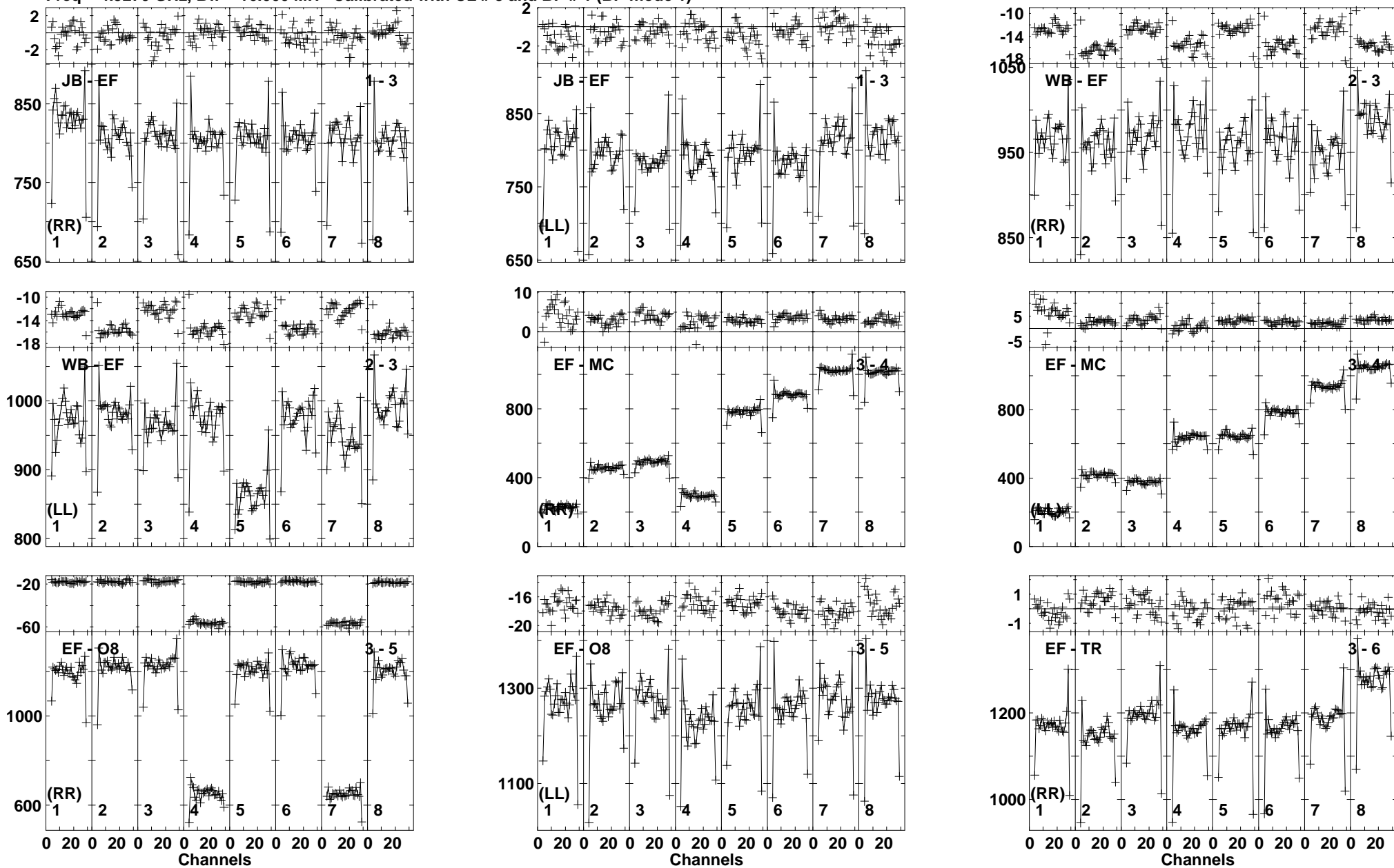
Lower frame: Milli Ampl Jy Top frame: Phas deg Vector averaged cross-power spectrum Baseline: JB (01) - EF (03) Timerange: 00/17:35:13 to 00/17:35:59
