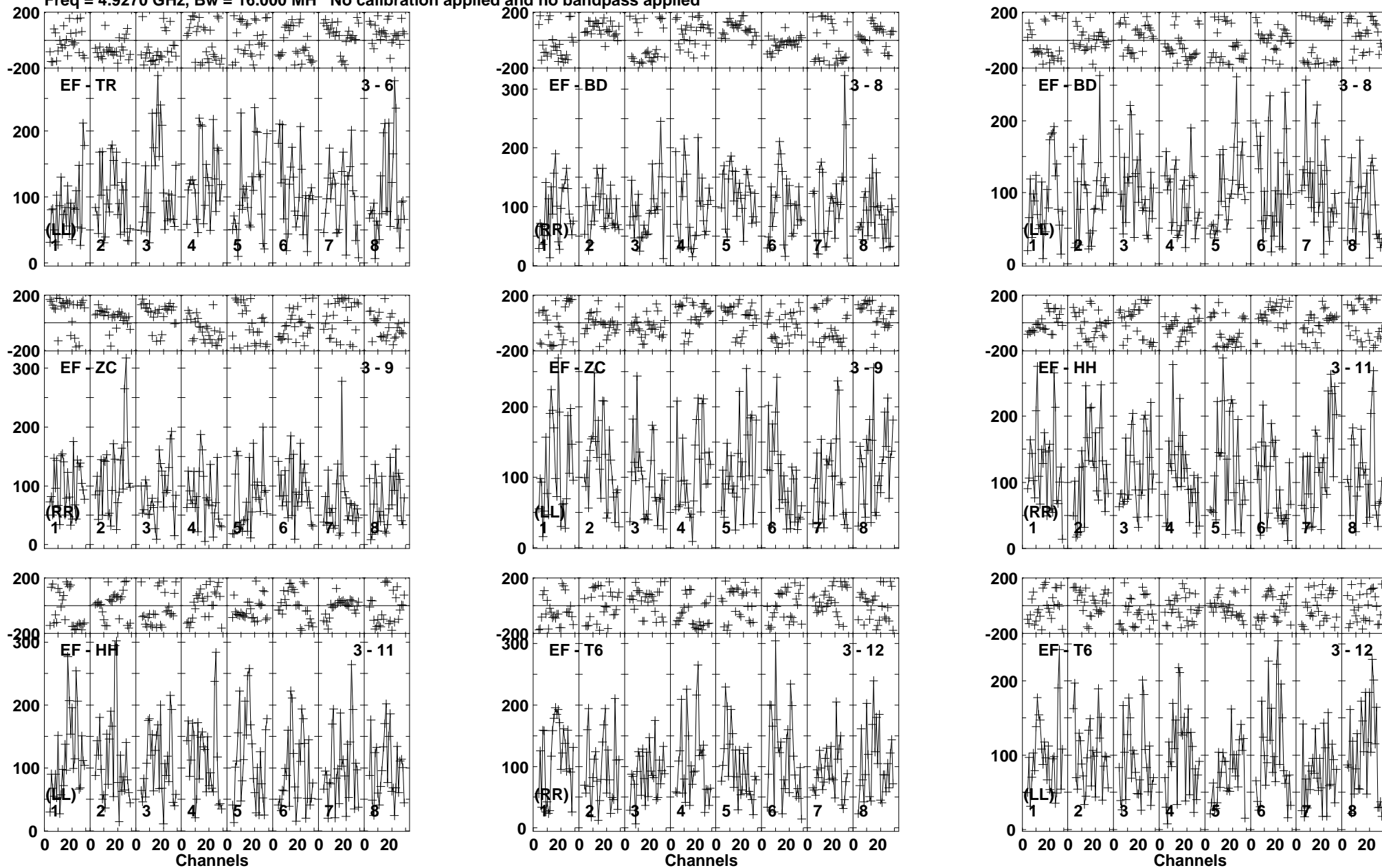
Lower frame: Micro Ampl Jy Top frame: Phas deg Vector averaged cross-power spectrum Baseline: EF (03) - TR (06) Timerange: 00/09:58:55 to 00/10/01:49
