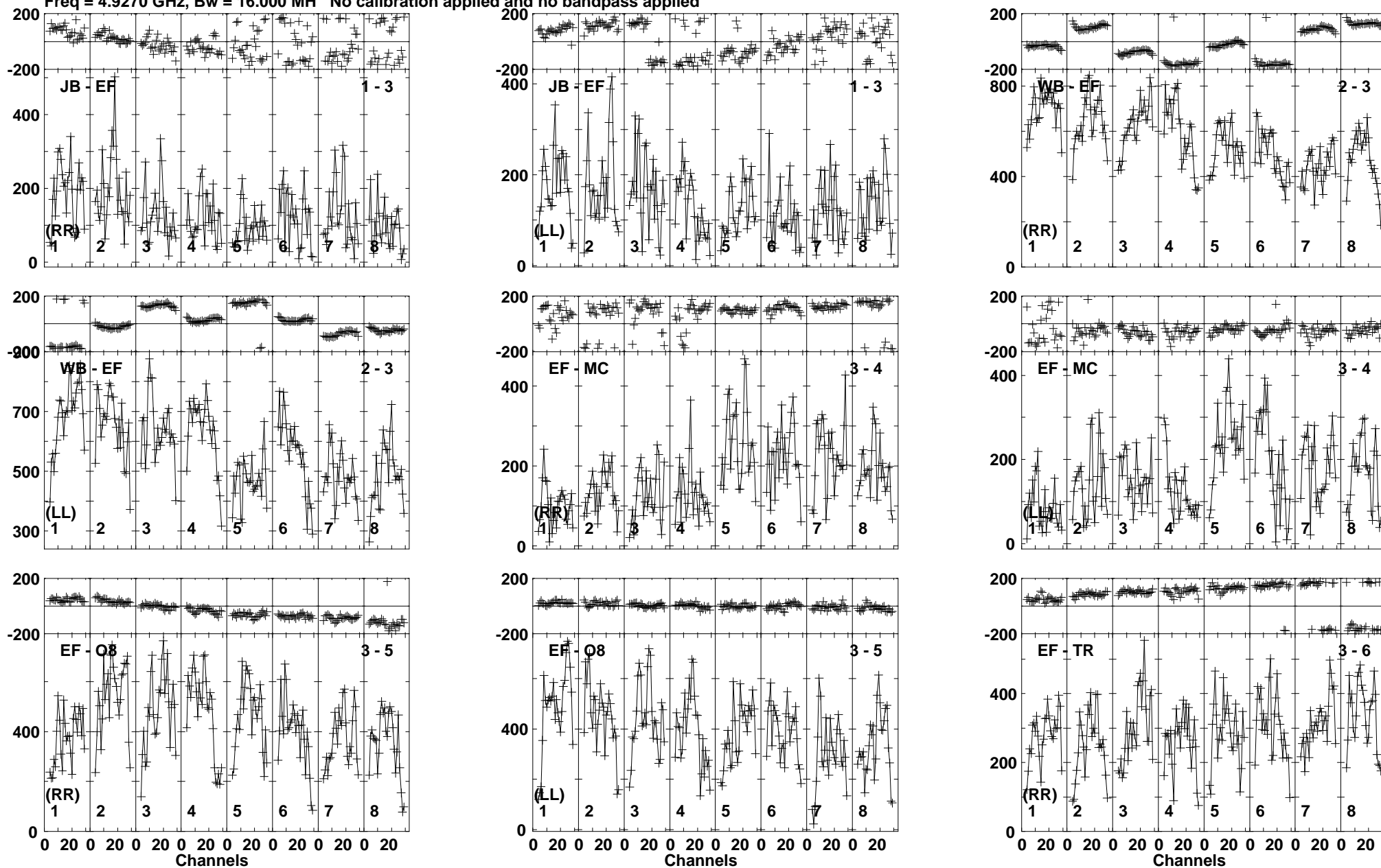
Lower frame: Micro Ampl Jy Top frame: Phas deg Vector averaged cross-power spectrum Baseline: JB (01) - EF (03) Timerange: 00/17:52:26 to 00/17:55:18
