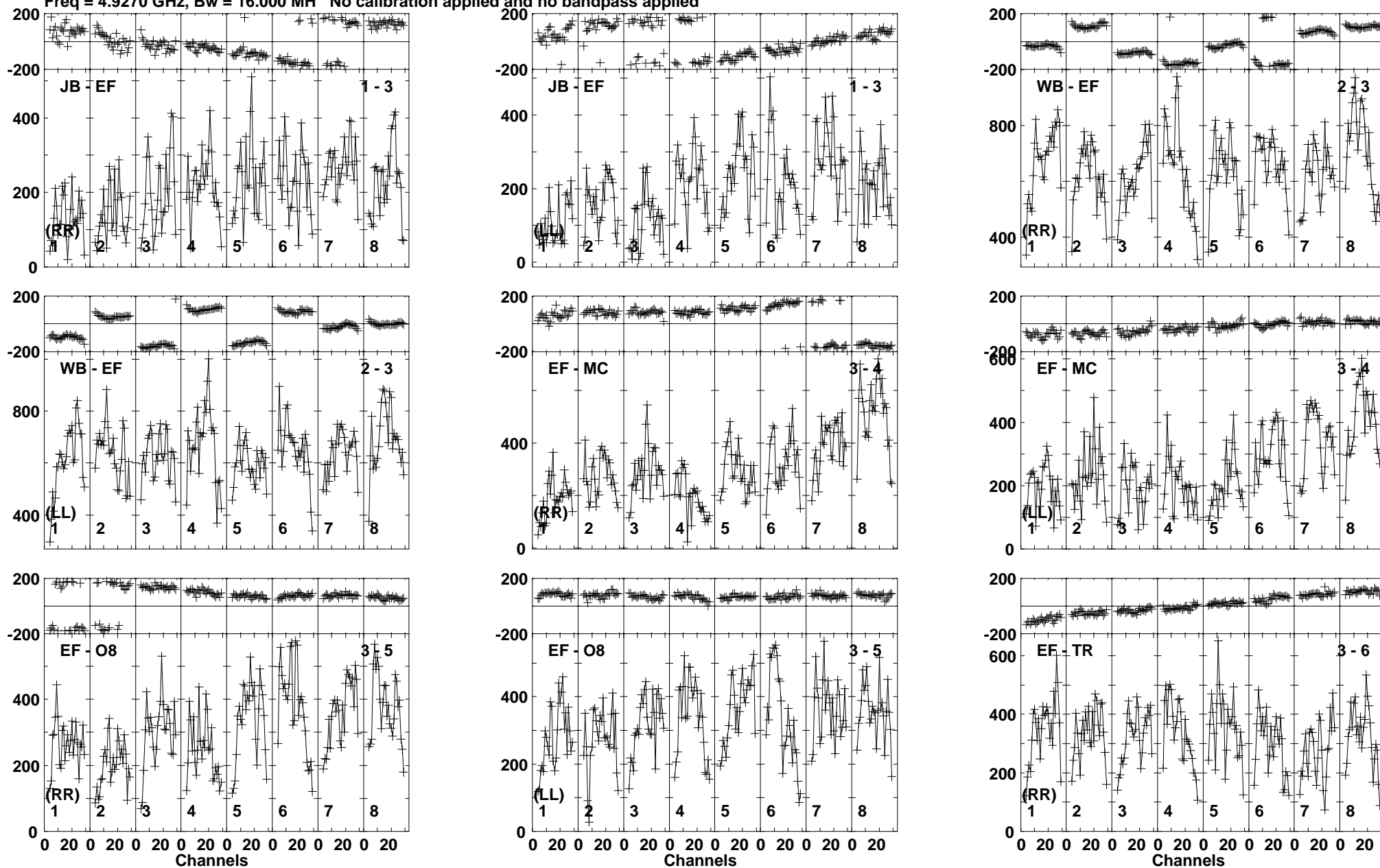
Lower frame: Micro Ampl Jy Top frame: Phas deg Vector averaged cross-power spectrum Baseline: JB (01) - EF (03) Timerange: 00/14:47:16 to 00/14:50:08
