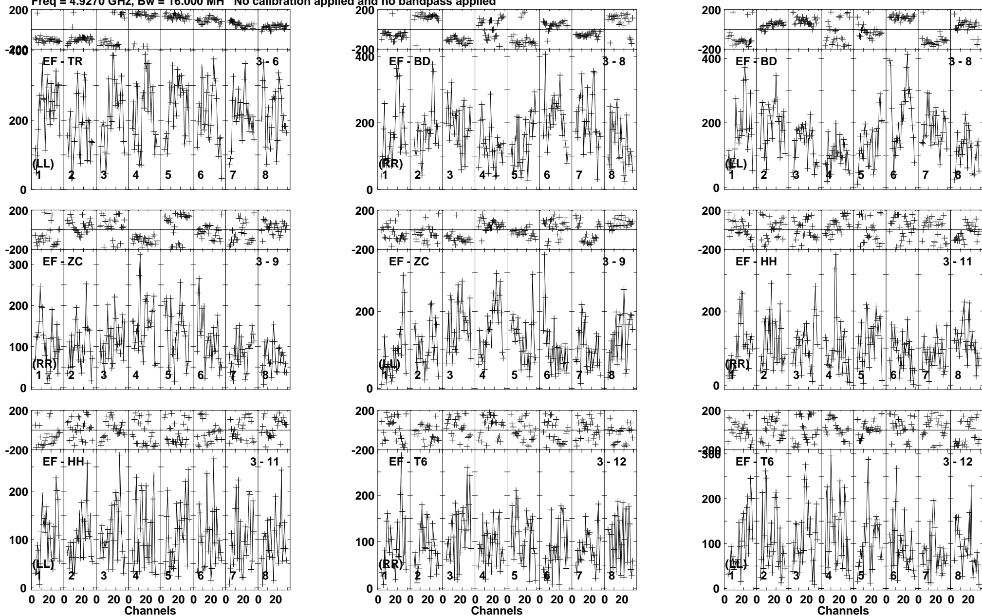
Lower frame: Micro Ampl Jy Top frame: Phas deg Vector average cross-power spectrum Baseline: EF (03) - TR (06) Timerange: 00/11:47:35 to 00/11:50:29
