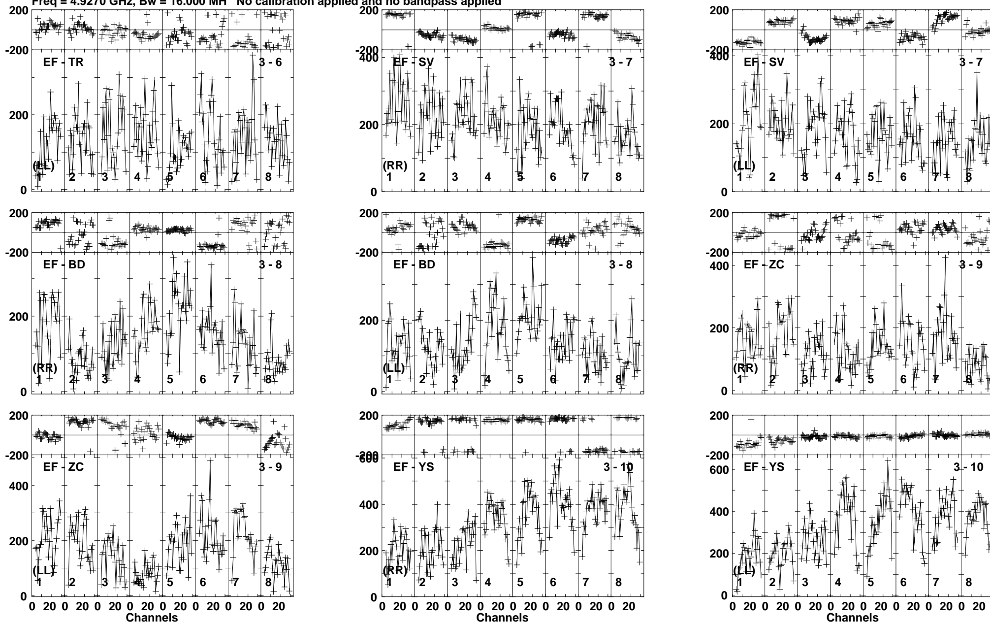
Lower frame: Micro Ampl Jy Top frame: Phas deg Vector averaged cross-power spectrum Baseline: EF (03) - TR (06) Timerange: 00/13:26:26 to 00/13:29:18
