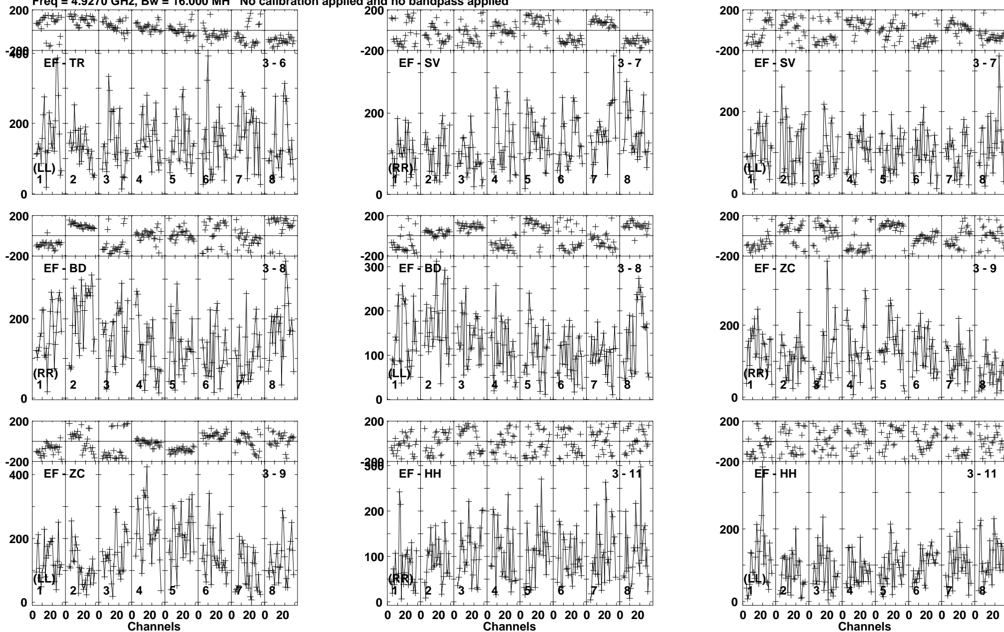
Lower frame: Micro Ampl Jy Top frame: Phas deg Vector averaged cross-power spectrum Baseline: EF (03) - TR (06) Timerange: 00/14:18:56 to 00/14:21:48
