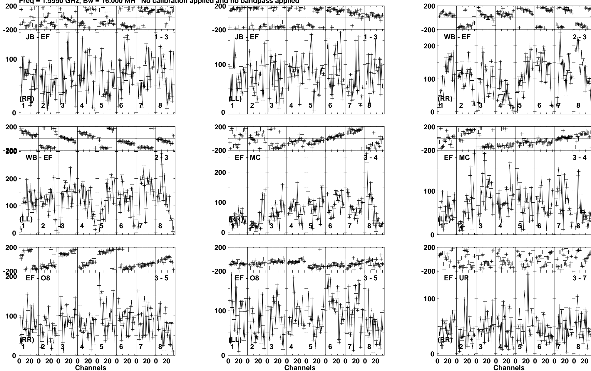
Lower frame: Micro Ampl Jy Top frame: Phas deg Vector averaged cross-power spectrum Baseline: JB (01) - EF (03) Timerange: 01/05:21:01 to 01/05:29:59
