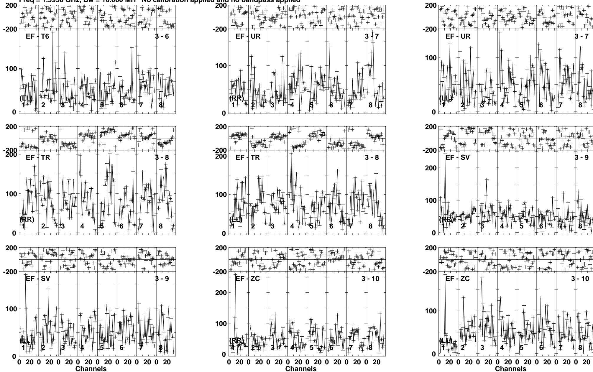
Lower frame: Micro Ampl Jy Top frame: Phas deg Vector averaged cross-power spectrum Baseline: EF (03) - T6 (06) Timerange: 01/02:04:31 to 01/02:14:29
