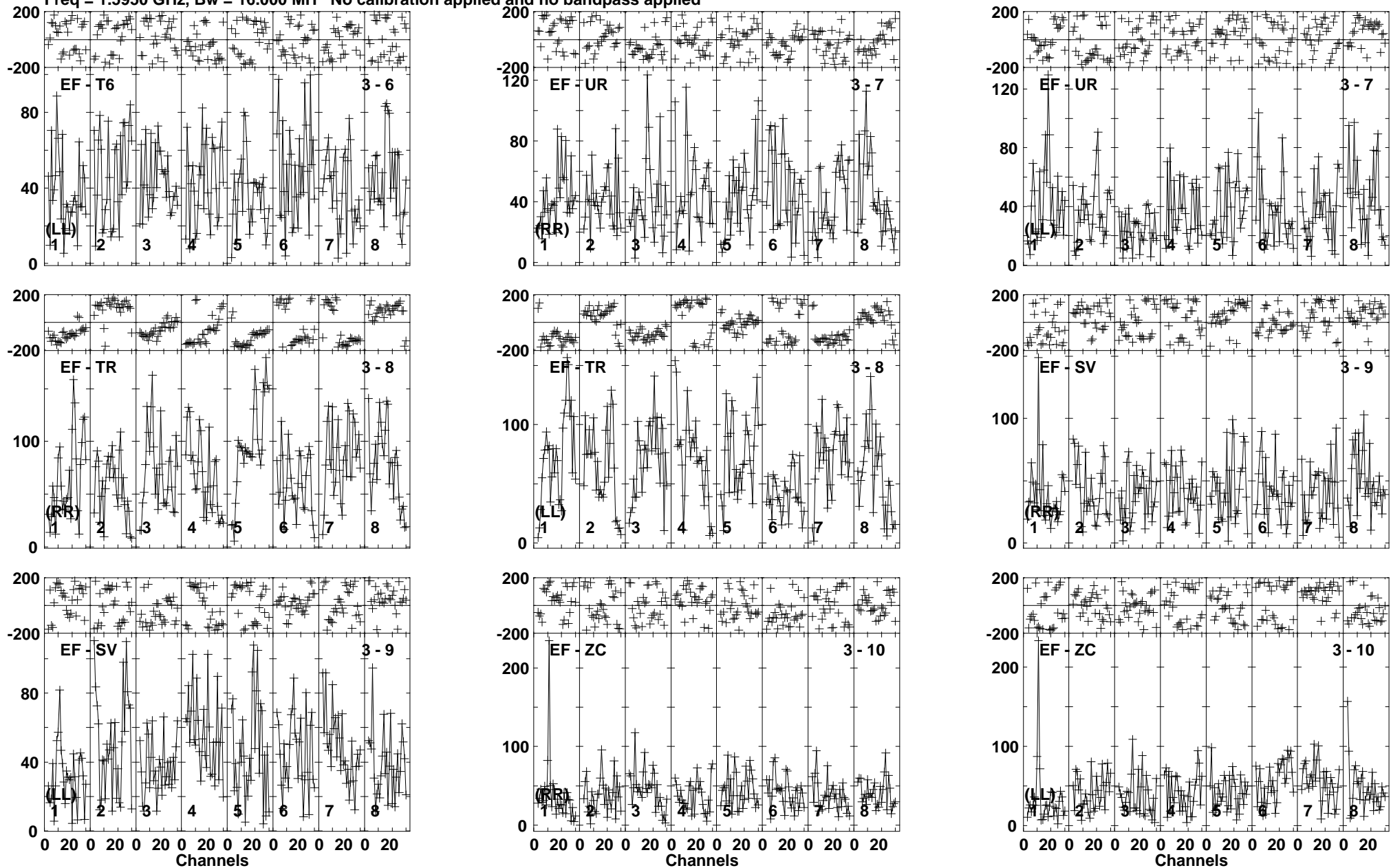
Lower frame: Micro Ampl Jy Top frame: Phas deg Vector averaged cross-power spectrum Baseline: EF (03) - T6 (06) Timerange: 01/02:21:31 to 01/02:31:29
