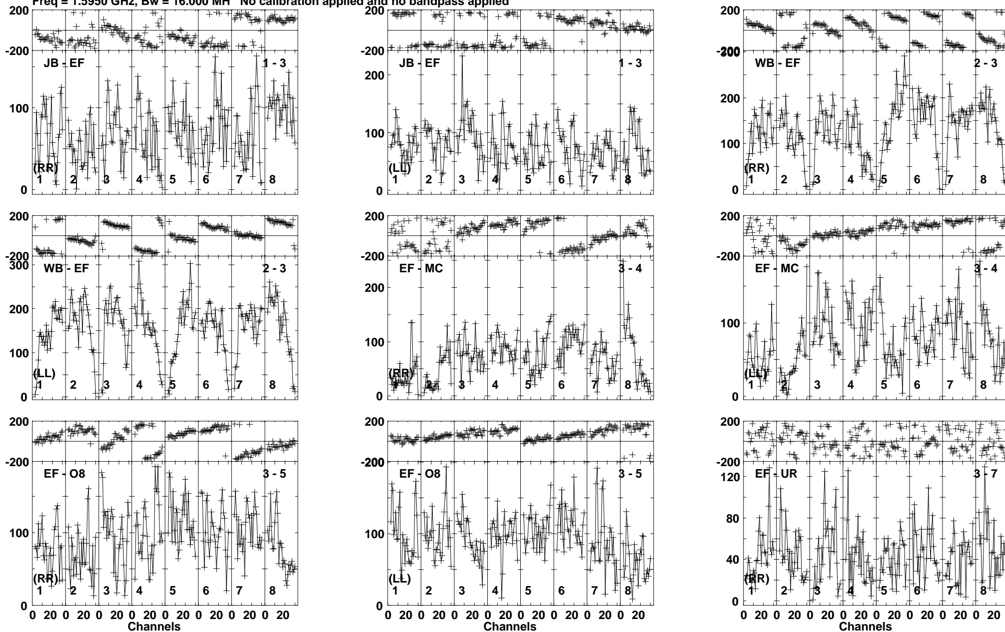
Lower frame: Micro Ampl Jy Top frame: Phas deg Vector averaged cross-power spectrum Baseline: JB (01) - EF (03) Timerange: 01/02:53:01 to 01/03:02:59
