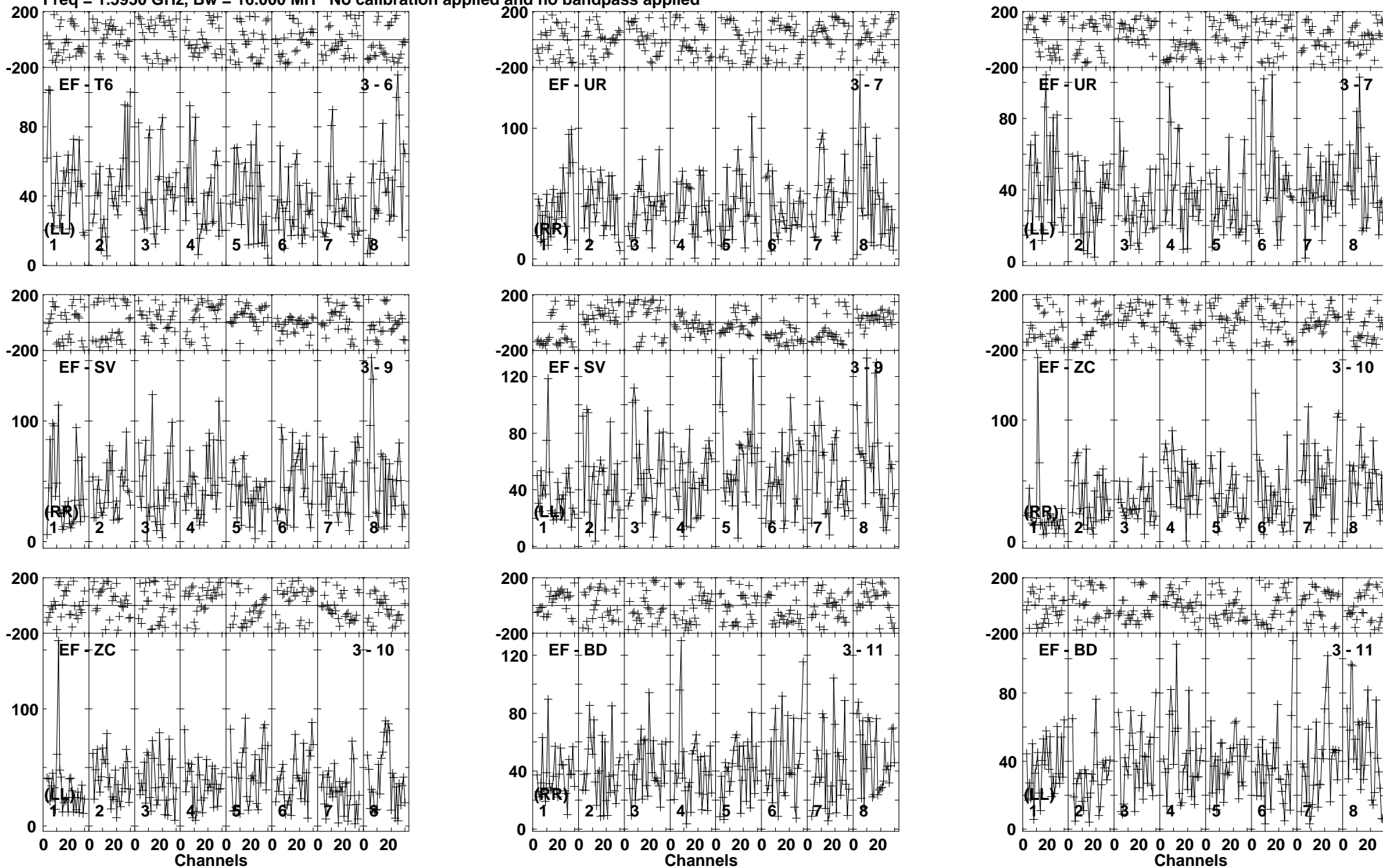
Lower frame: Micro Ampl Jy Top frame: Phas deg Vector averaged cross-power spectrum Baseline: EF (03) - T6 (06) Timerange: 00/22:57:31 to 00/23:07:29
