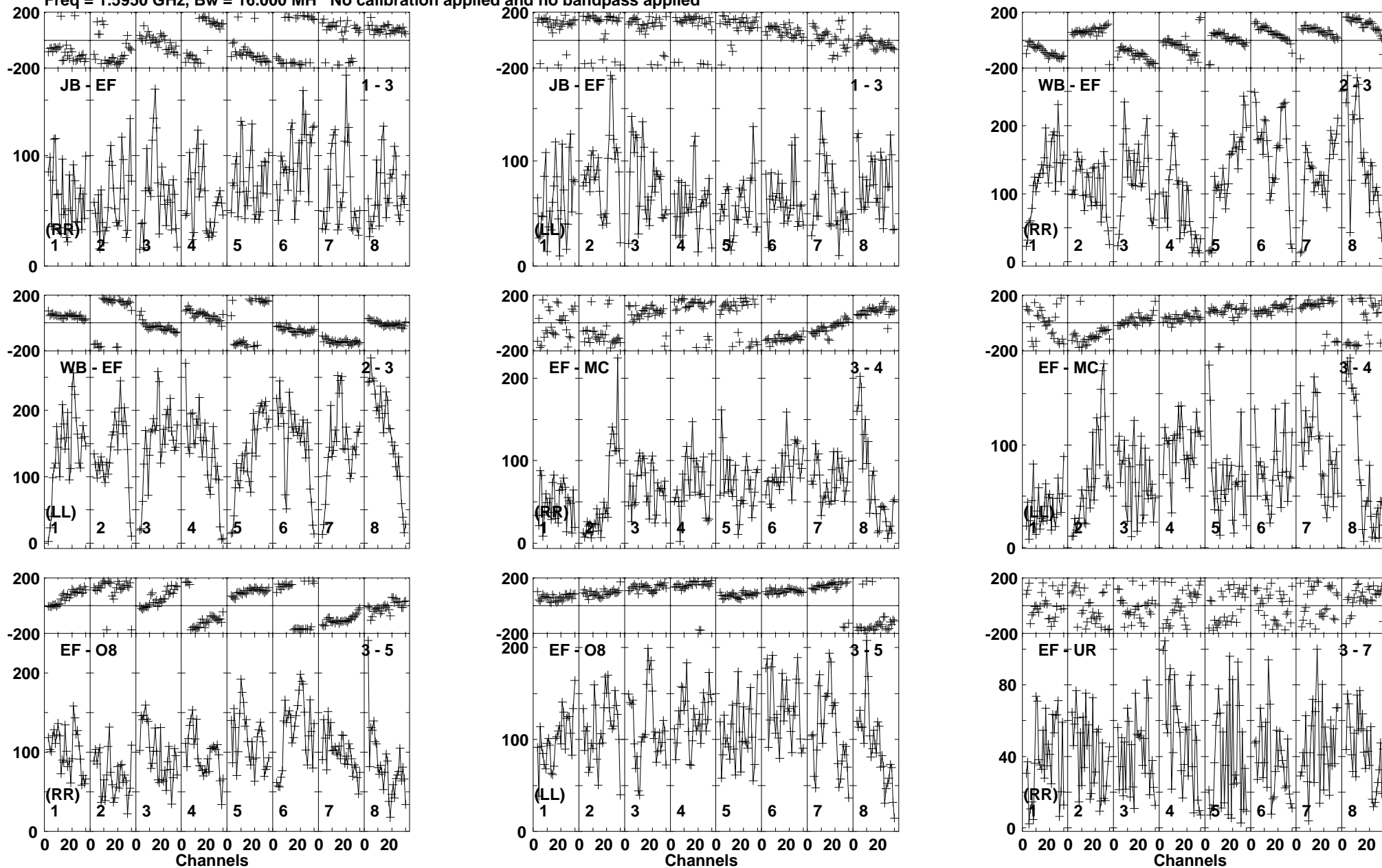
Lower frame: Micro Ampl Jy Top frame: Phas deg Vector averaged cross-power spectrum Baseline: JB (01) - EF (03) Timerange: 01/03:03:31 to 01/03:13:29
