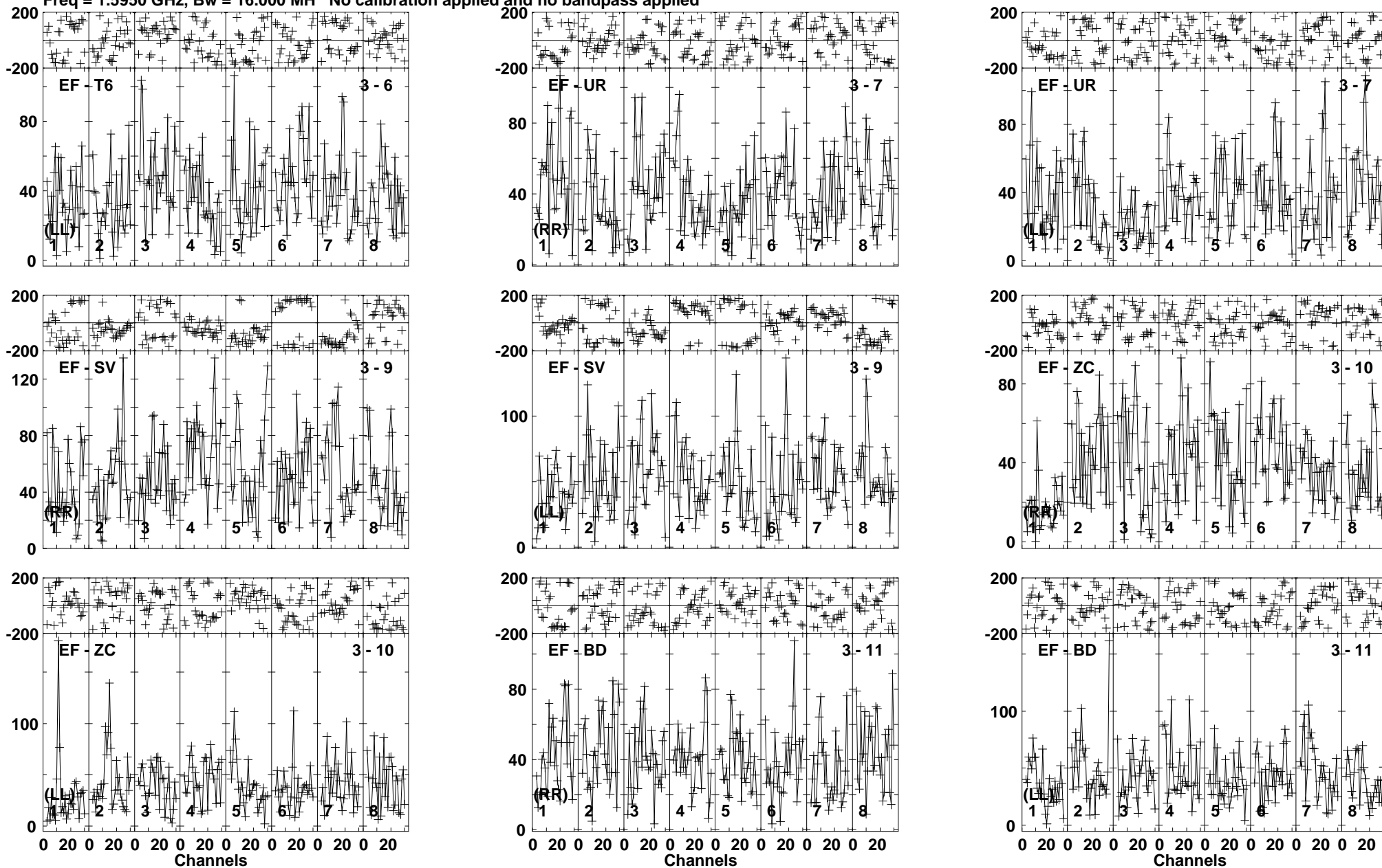
Lower frame: Micro Ampl Jy Top frame: Phas deg Vector averaged cross-power spectrum Baseline: EF (03) - T6 (06) Timerange: 00/22:40:31 to 00/22:50:29
