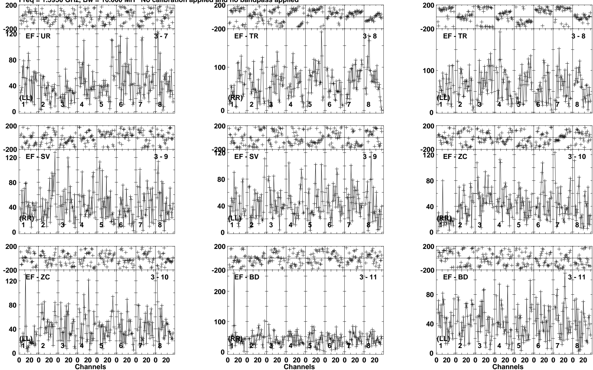
Lower frame: Micro Ampl Jy Top frame: Phas deg Vector averaged cross-power spectrum Baseline: EF (03) - UR (07) Timerange: 01/03:14:01 to 01/03:23:59
