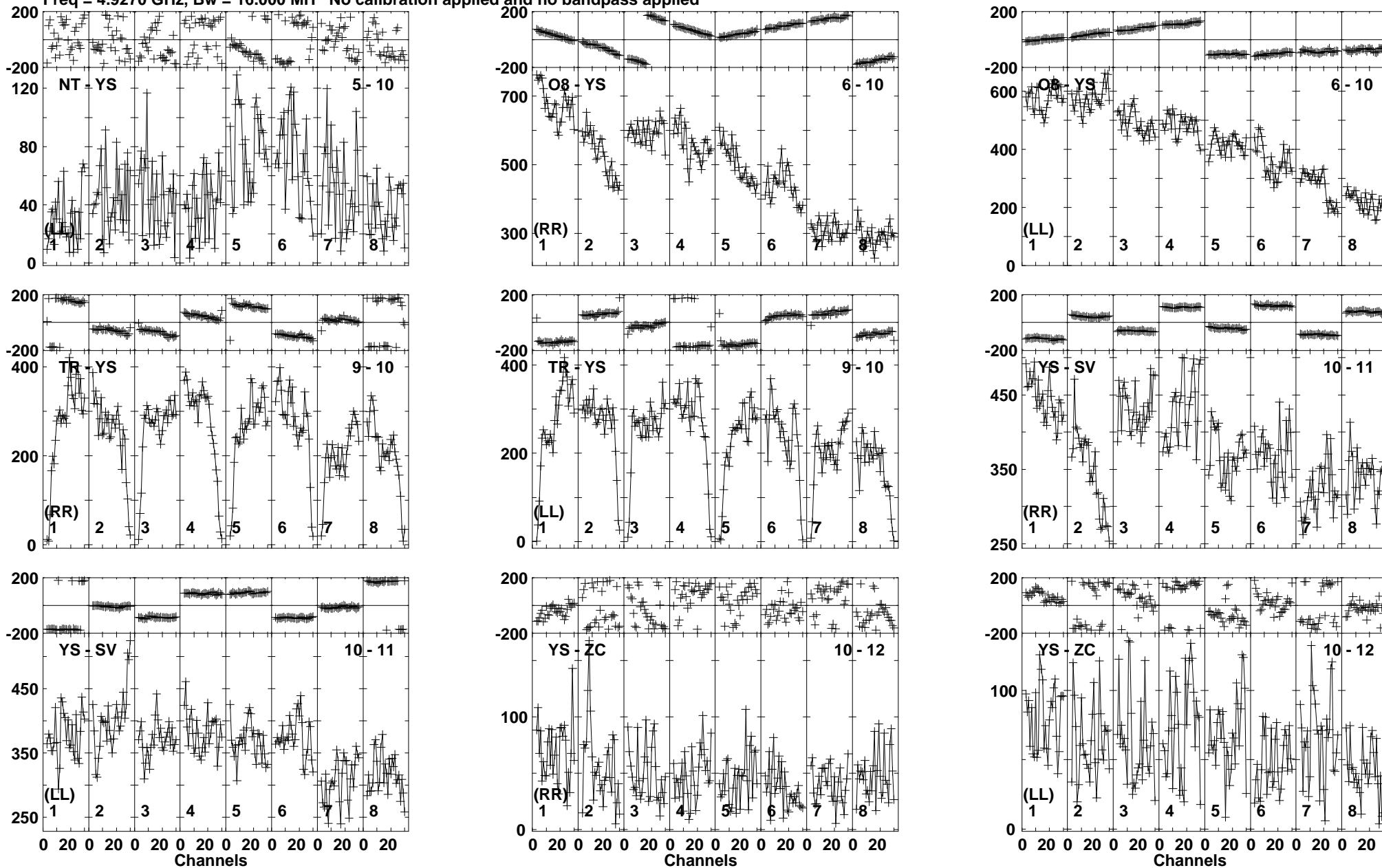
Lower frame: Micro Ampl Jy Top frame: Phas deg Vector average cross-power spectrum Baseline: NT (05) - YS (10) Timerange: 01/02:07:01 to 01/02:16:59
