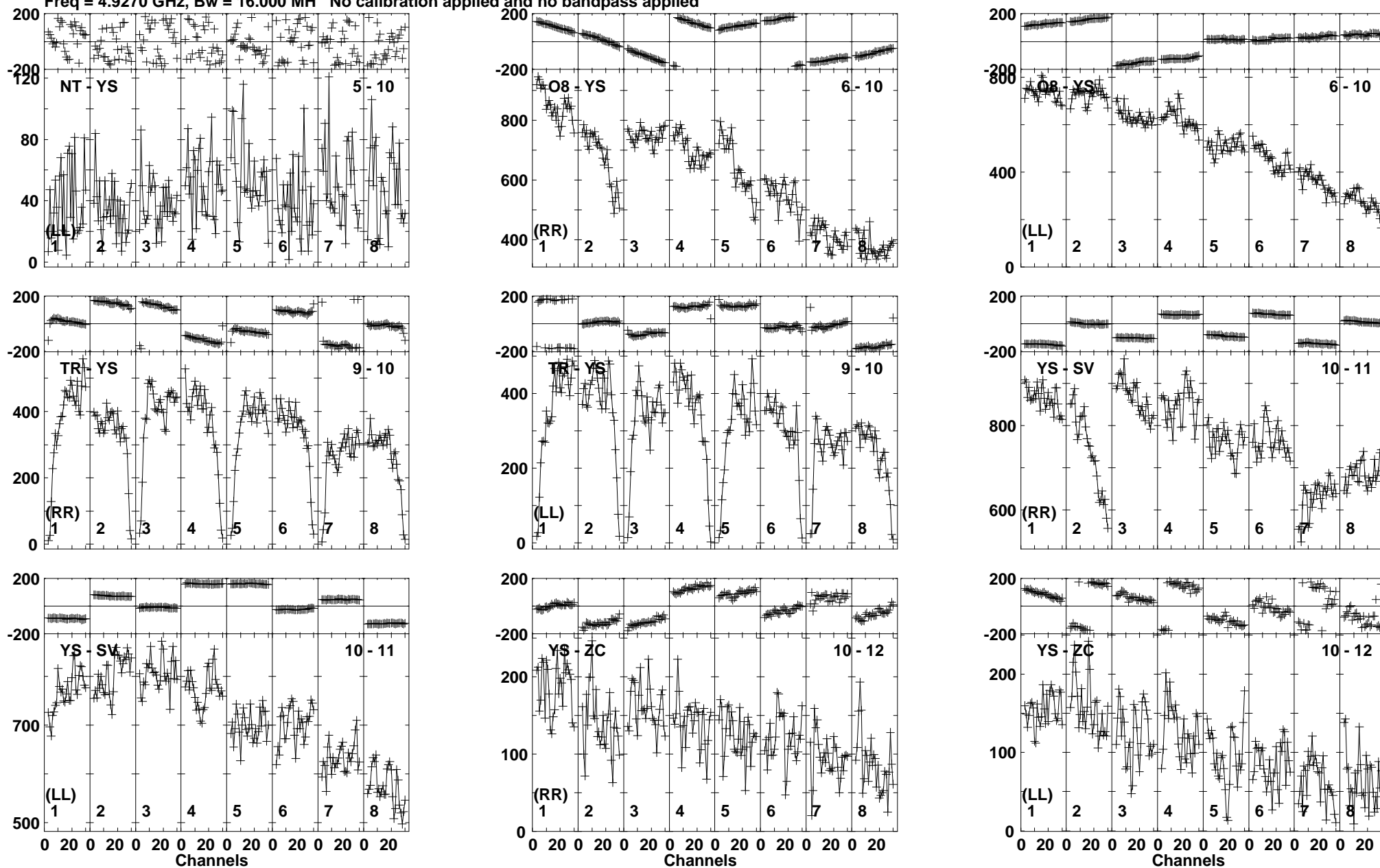
Lower frame: Micro Ampl Jy Top frame: Phas deg Vector averaged cross-power spectrum Baseline: NT (05) - YS (10) Timerange: 01/04:49:20 to 01/04:59:00
