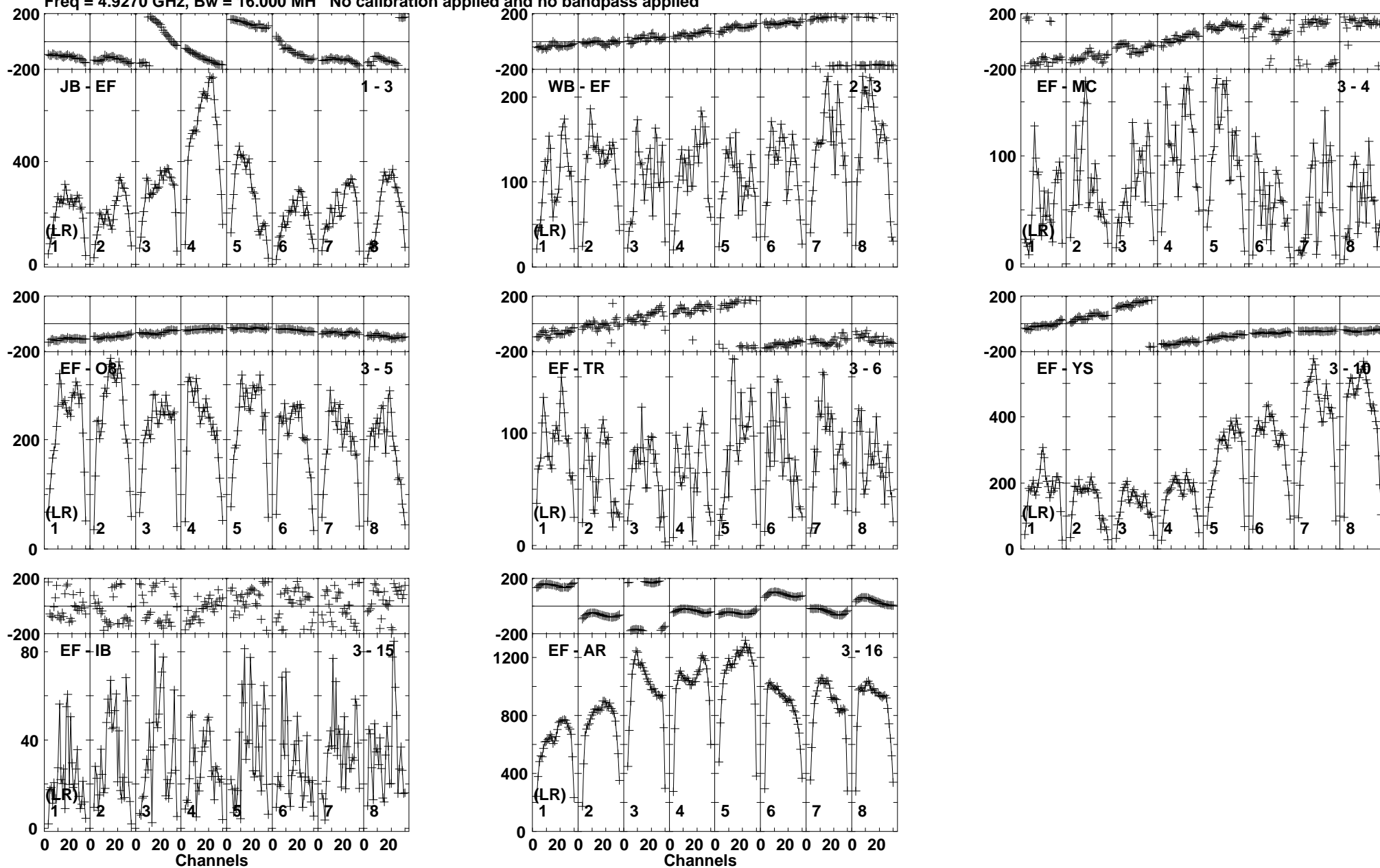
Lower frame: Micro Ampl Jy Top frame: Phas deg Vector averaged cross-power spectrum Baseline: JB (01) - EF (03) Timerange: 00/13:04:01 to 00/13:18:59
