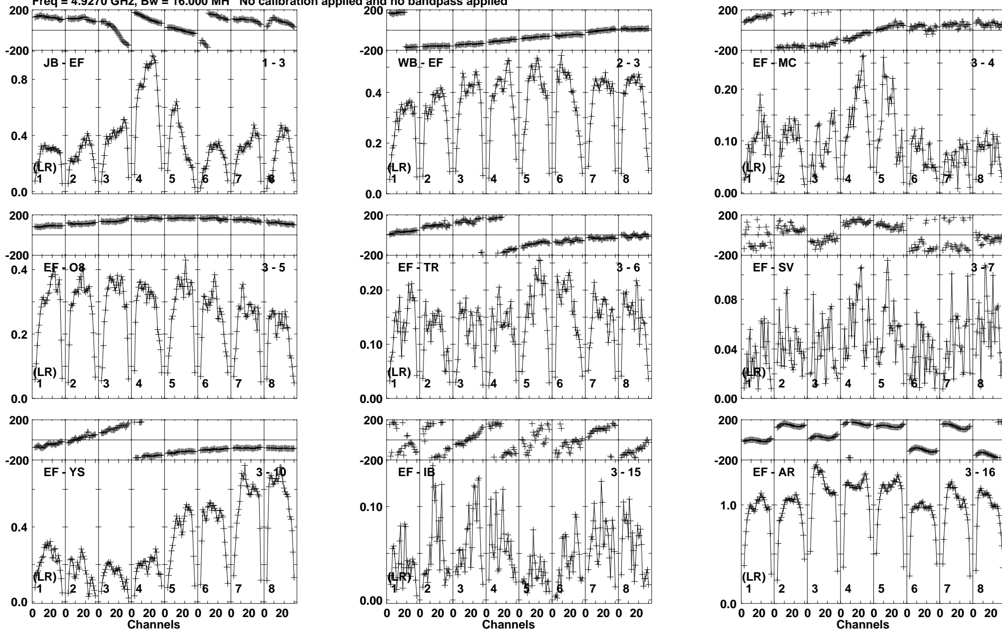
Lower frame: Milli Ampl Jy Top frame: Phas deg Vector averaged cross-power spectrum Baseline: JB (01) - EF (03) Timerange: 00:12:04:01 to 00:12:18:59
