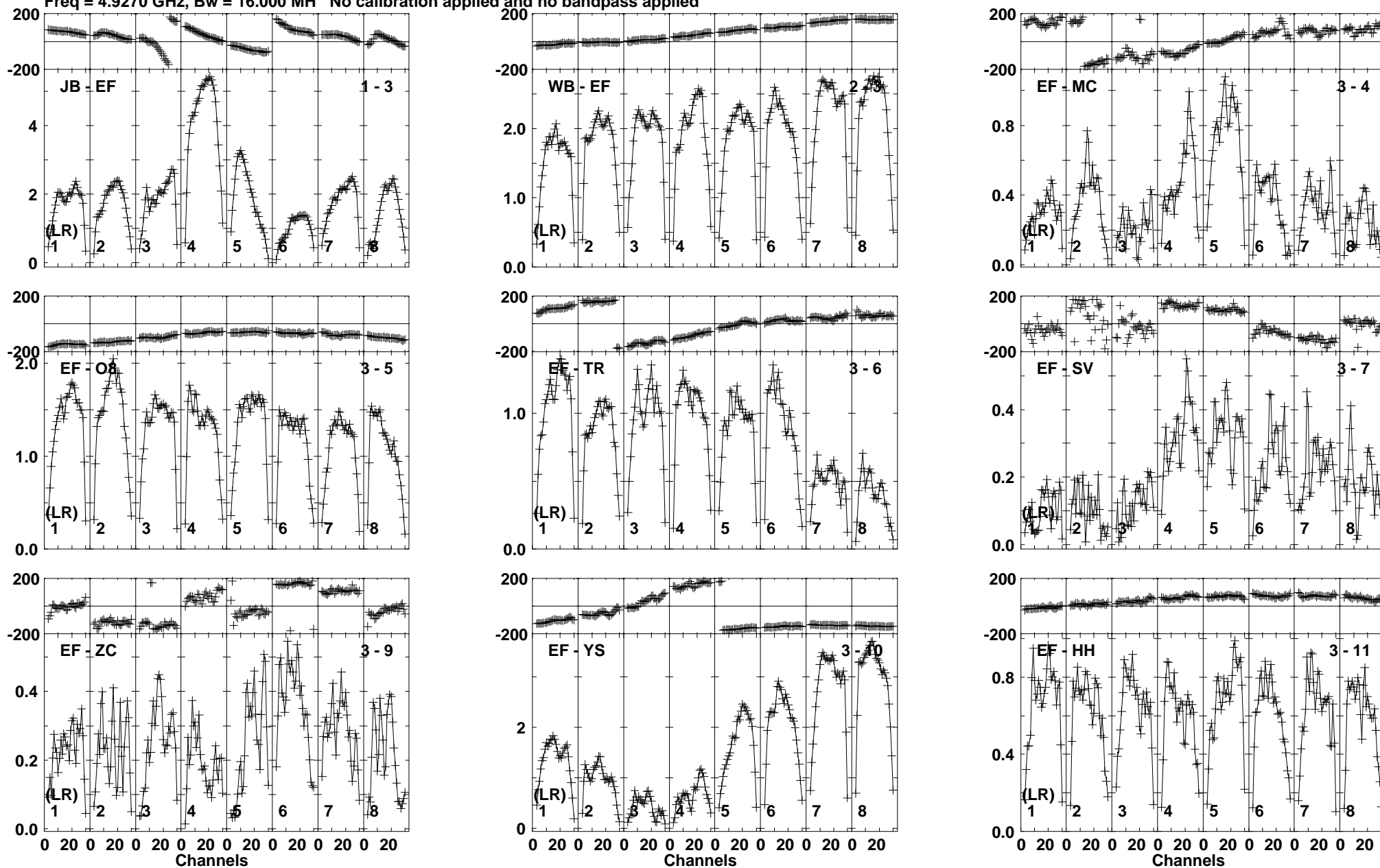
Lower frame: Milli Ampl Jy Top frame: Phas deg Vector averaged cross-power spectrum Baseline: JB (01) - EF (03) Timerange: 00/11:01:01 to 00/11:02:59
