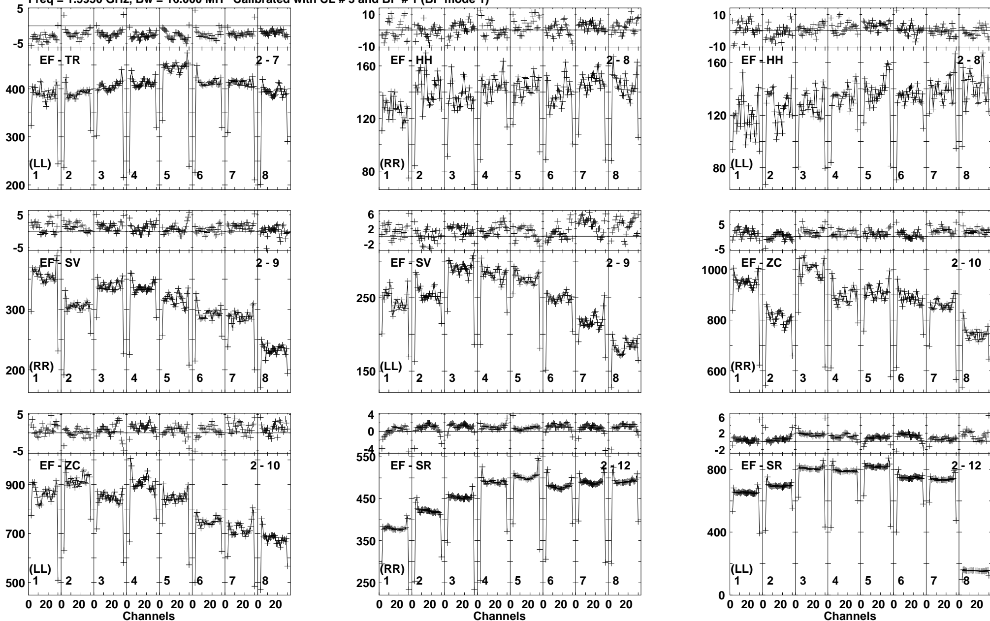
Lower frame: Milli Ampl Jy Top frame: Phas deg Vector averaged cross-power spectrum Baseline: EF (02) - TR (07) Timerange: 00/06:40:01 to 00/06:41:59
