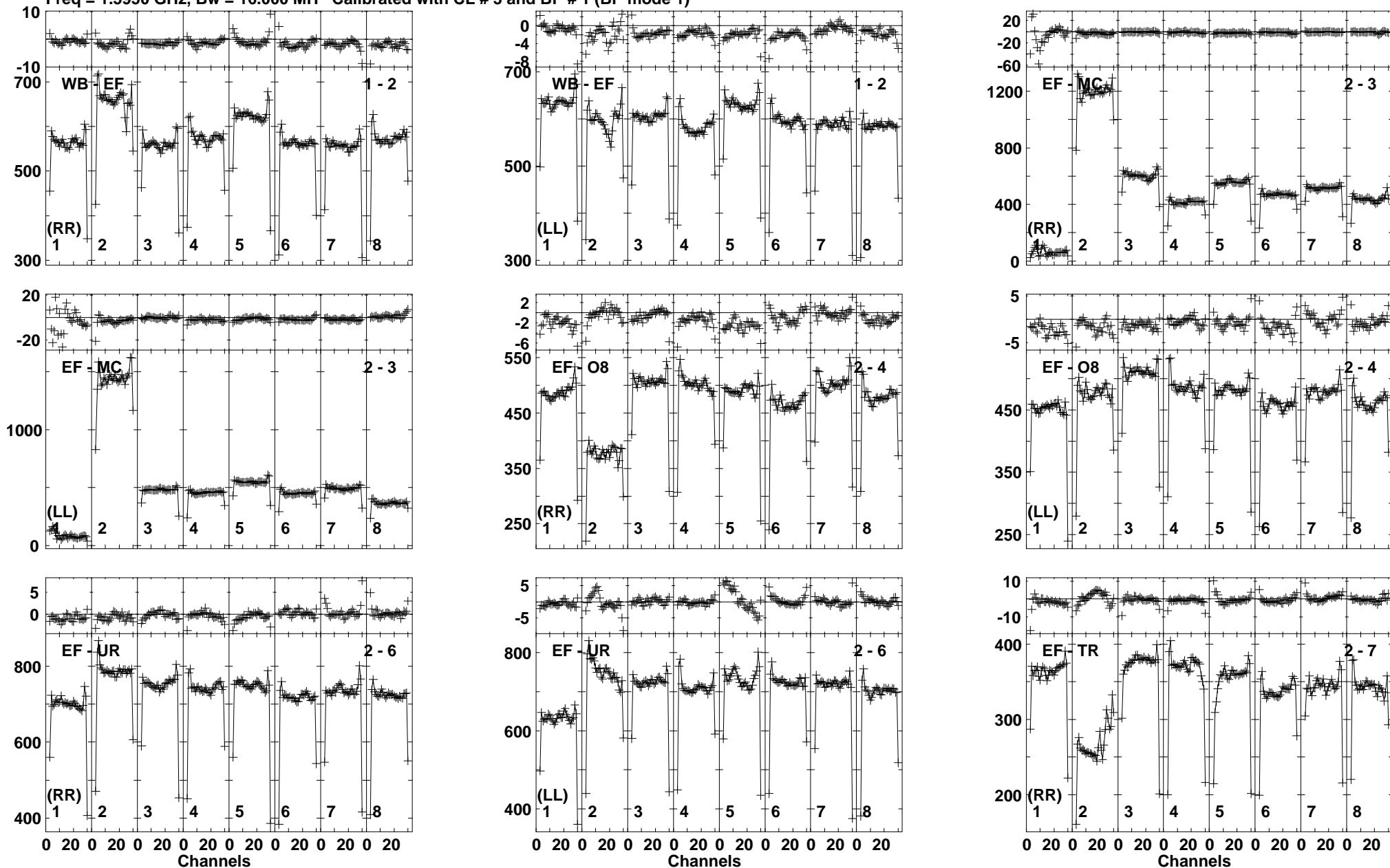
Lower frame: Milli Ampl Jy Top frame: Phas deg Vector averaged cross-power spectrum Baseline: WB (01) - EF (02) Timerange: 00/02:00:01 to 00/02:01:59
