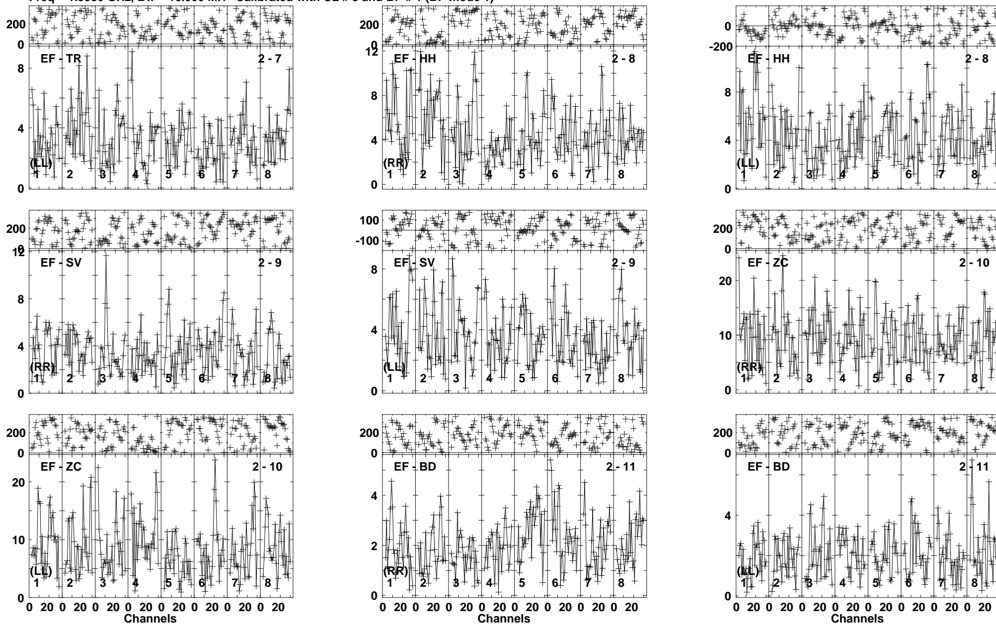
Lower frame: Milli Ampl Jy Top frame: Phas deg Vector averaged cross-power spectrum Baseline: EF (02) - TR (07) Timerange: 00/04:22:01 to 00/04:29:59
