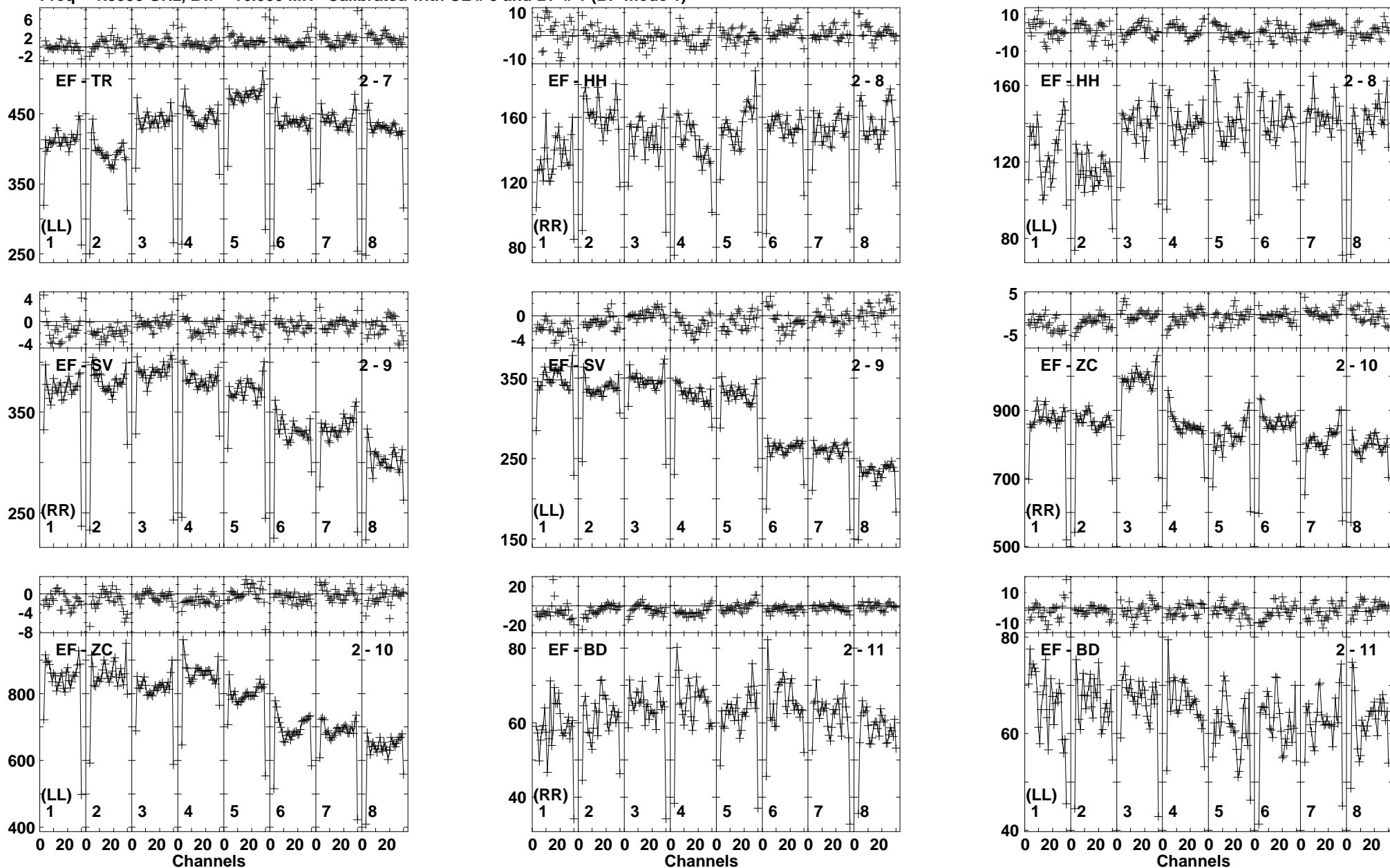
Lower frame: Milli Ampl Jy Top frame: Phas deg Vector averaged cross-power spectrum Baseline: EF (02) - TR (07) Timerange: 00/05:10:41 to 00/05:11:59
