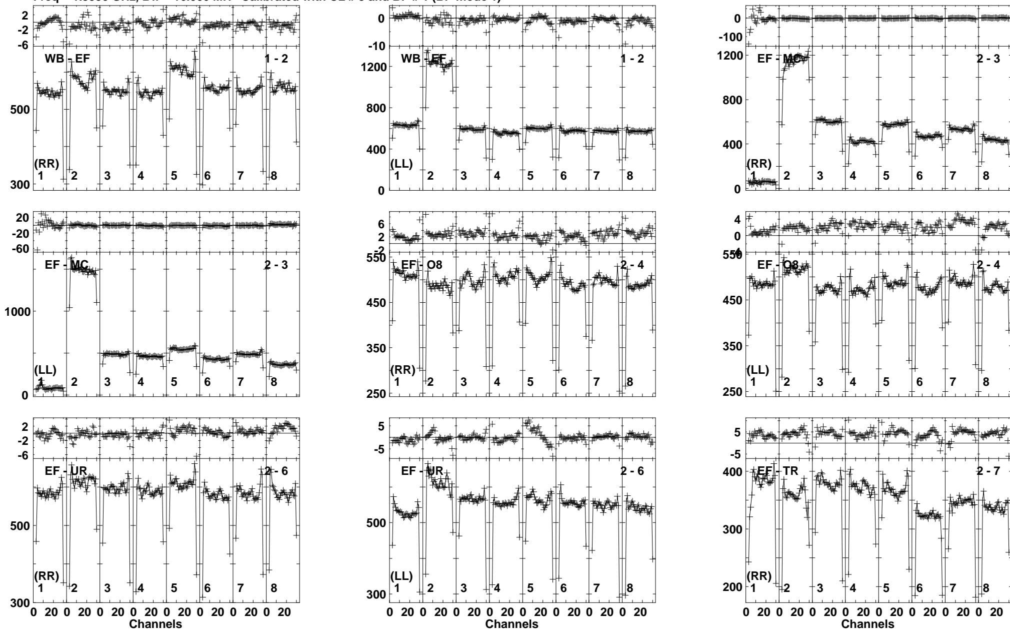
Lower frame: Milli Ampl Jy Top frame: Phas deg Vector averaged cross-power spectrum Baseline: WB (01) - EF (02) Timerange: 00/06:00:01 to 00/06:01:59
