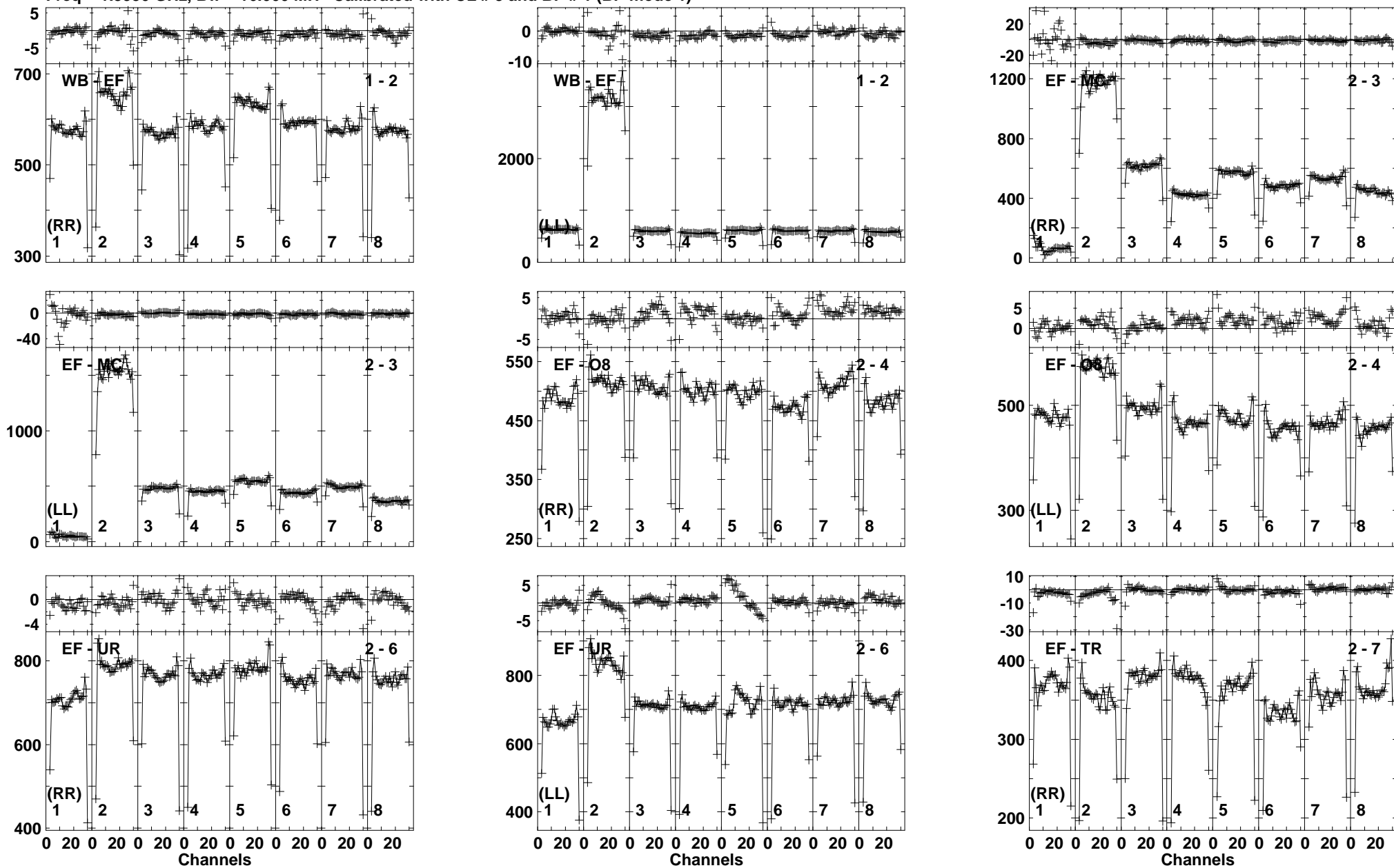
Lower frame: Milli Ampl Jy Top frame: Phas deg Vector averaged cross-power spectrum Baseline: WB (01) - EF (02) Timerange: 00/02:10:41 to 00/02:11:59
