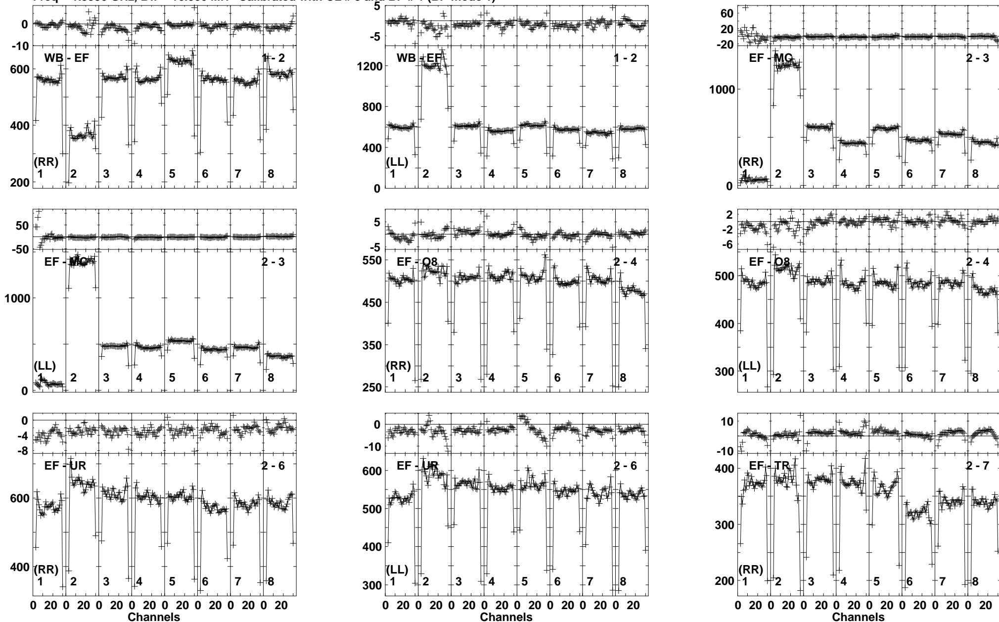
Lower frame: Milli Ampl Jy Top frame: Phas deg Vector averaged cross-power spectrum Baseline: WB (01) - EF (02) Timerange: 00/06:10:41 to 00/06:11:59
