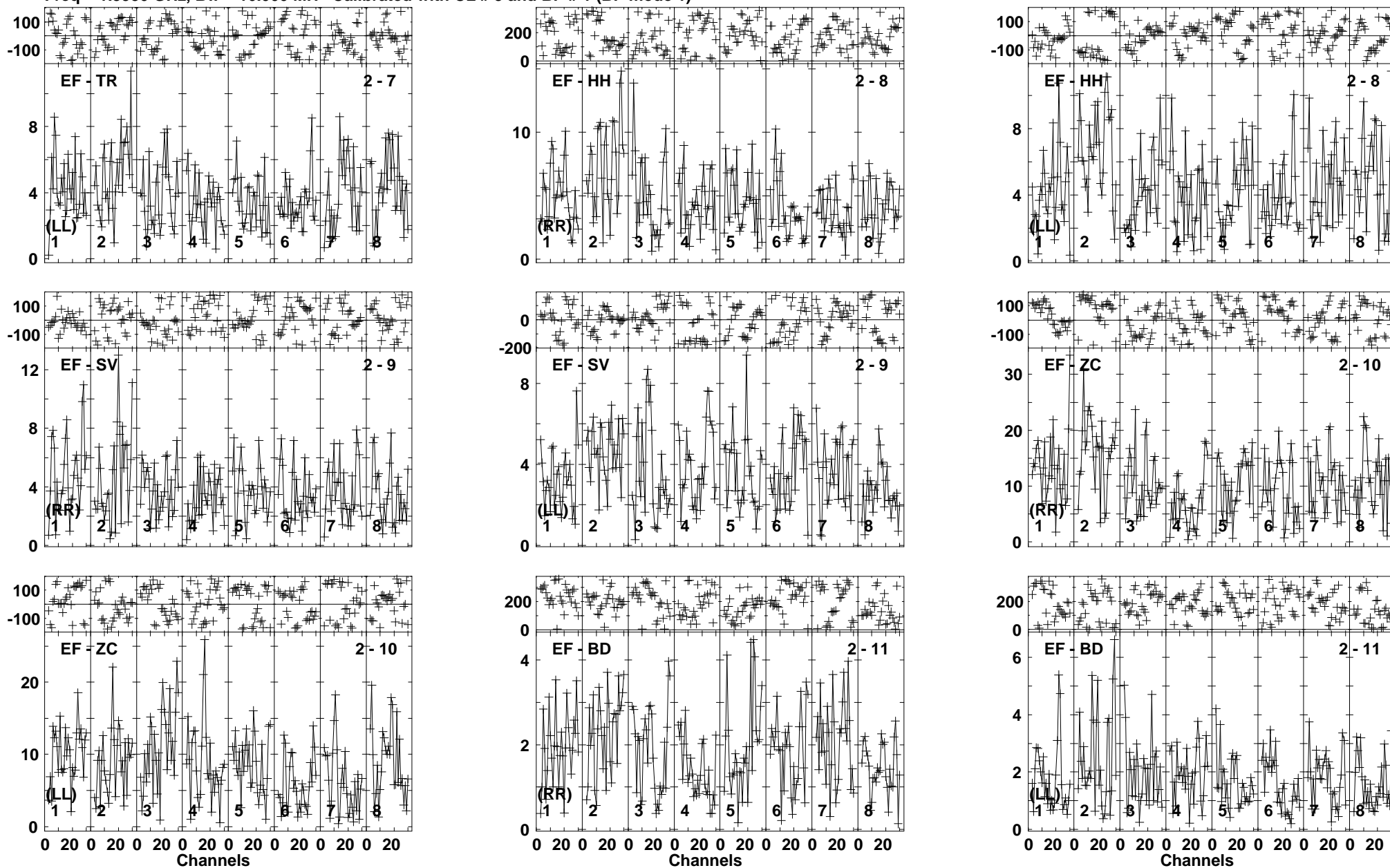
Lower frame: Milli Ampl Jy Top frame: Phas deg Vector averaged cross-power spectrum Baseline: EF (02) - TR (07) Timerange: 00/02:52:01 to 00/02:59:59
