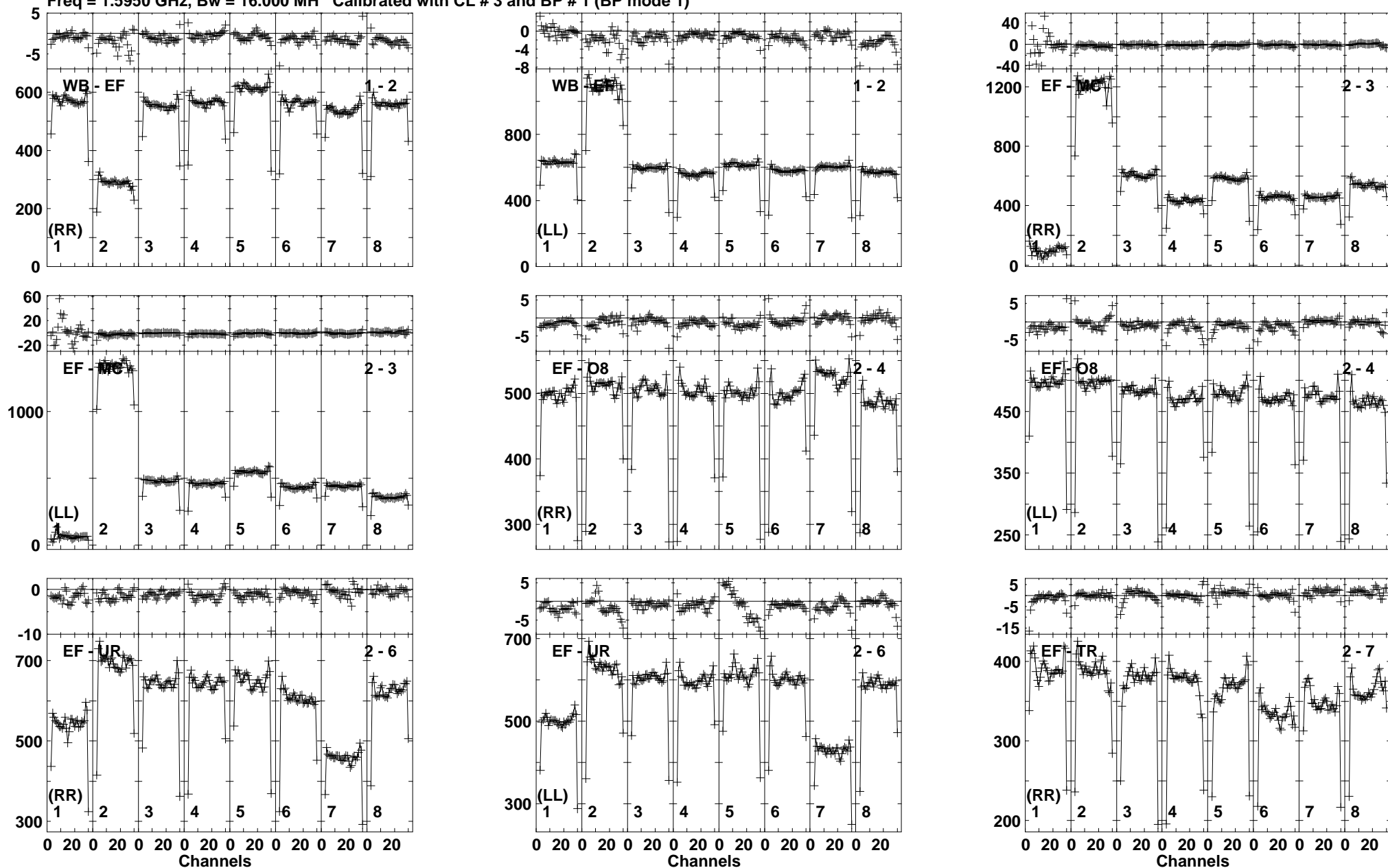
Lower frame: Milli Ampl Jy Top frame: Phas deg Vector averaged cross-power spectrum Baseline: WB (01) - EF (02) Timerange: 00/05:30:41 to 00/05:31:59
