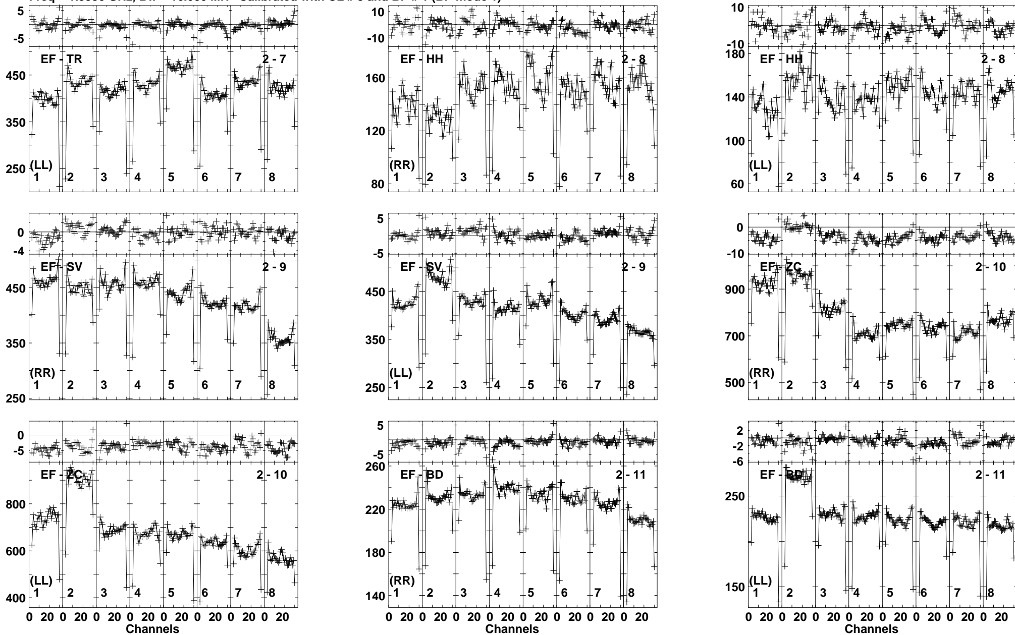
Lower frame: Milli Ampl Jy Top frame: Phas deg Vector averaged cross-power spectrum Baseline: EF (02) - TR (07) Timerange: 00/02:10:41 to 00/02:11:59
