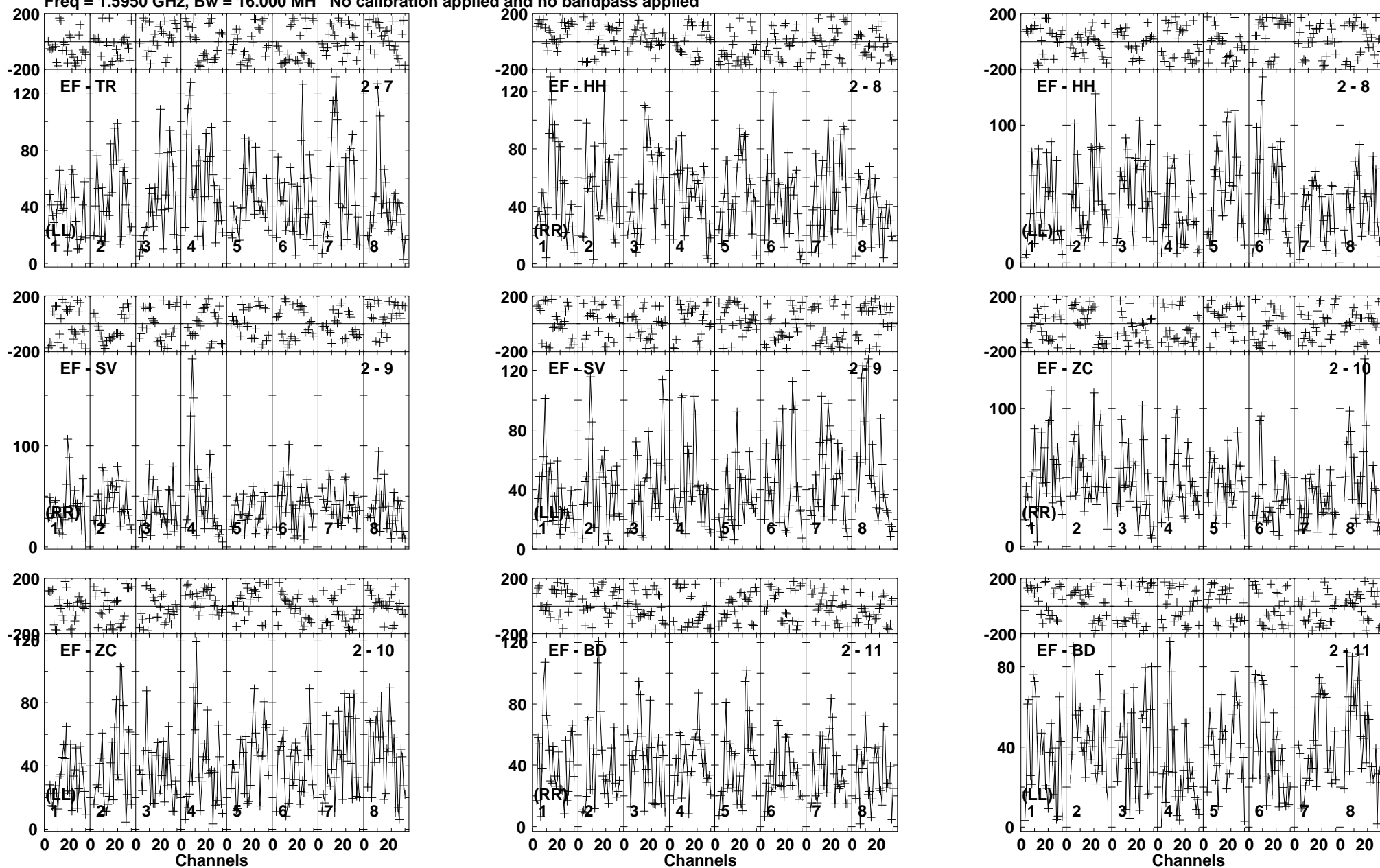
Lower frame: Micro Ampl Jy Top frame: Phas deg Vector averaged cross-power spectrum Baseline: EF (02) - TR (07) Timerange: 00/06:32:01 to 00/06:39:59
