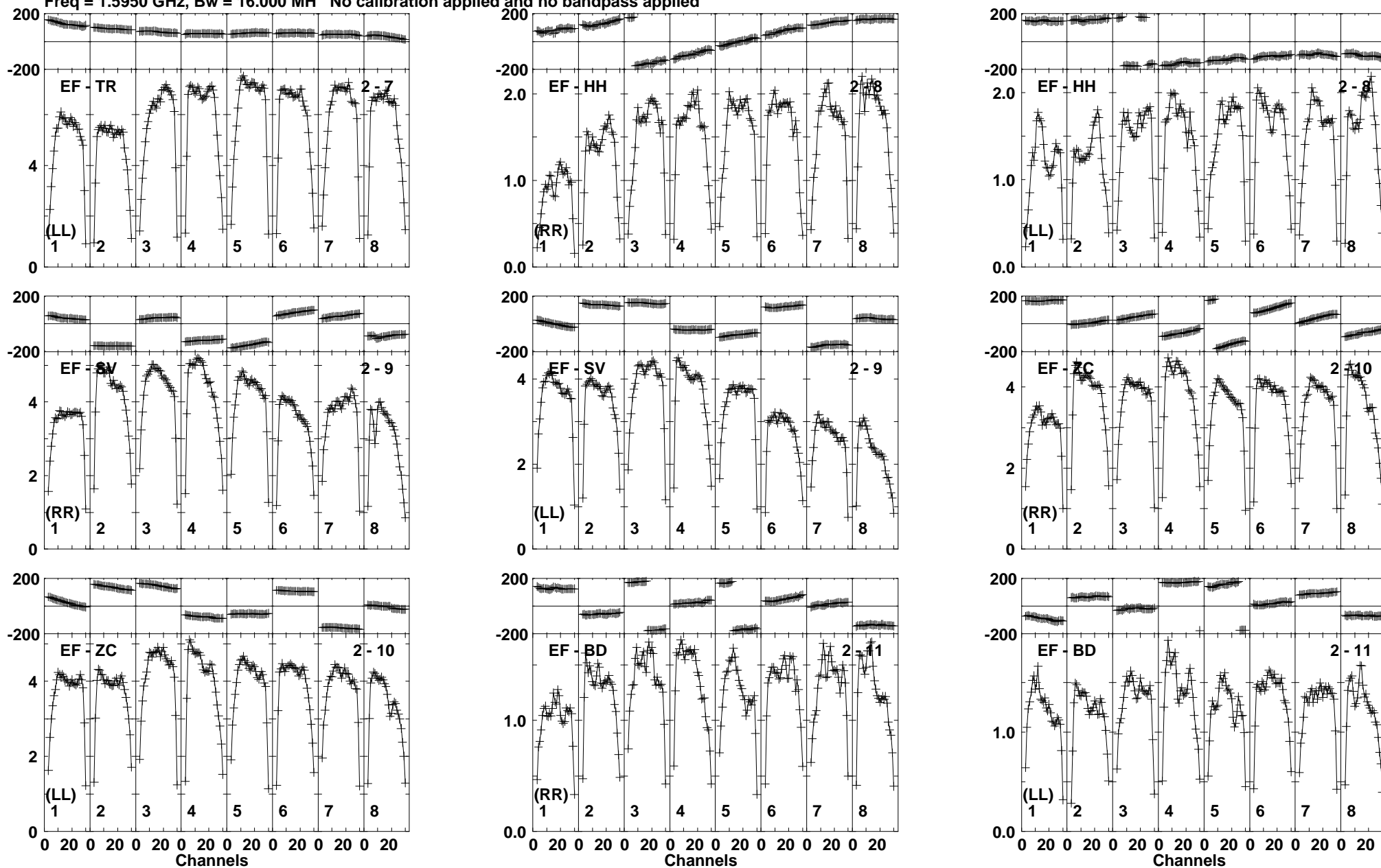
Lower frame: Milli Ampl Jy Top frame: Phas deg Vector averaged cross-power spectrum Baseline: EF (02) - TR (07) Timerange: 00/05:20:01 to 00/05:21:59
