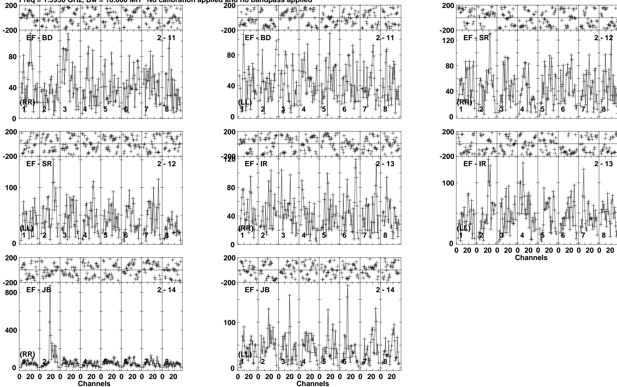
Lower frame: Micro Ampl Jy Top frame: Phas deg Vector averaged cross-power spectrum Baseline: EF (02) - BD (11) Timerange: 00/03:02:01 to 00/03:09:59
