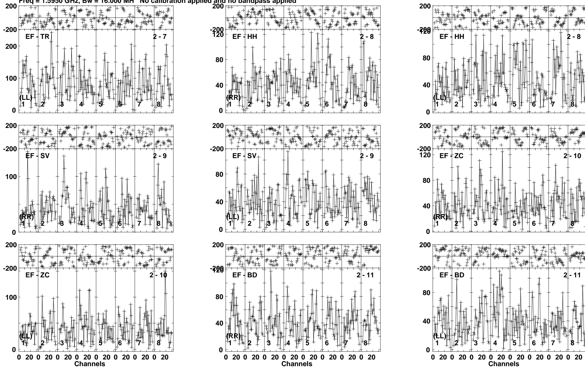
Lower frame: Micro Ampl Jy Top frame: Phas deg Vector averaged cross-power spectrum Baseline: EF (02) - TR (07) Timerange: 00/05:12:01 to 00/05:19:59
