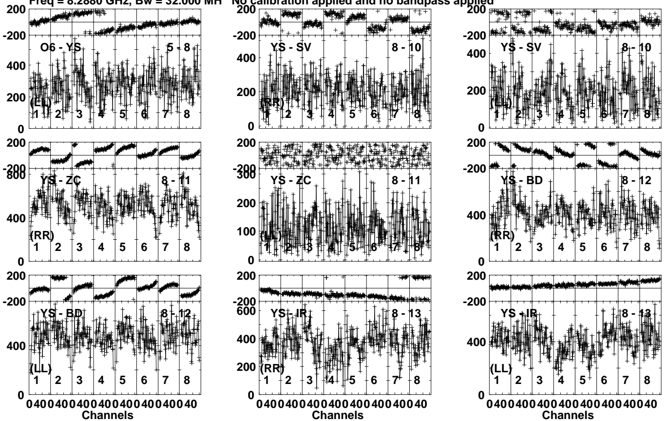
Lower frame: Micro Ampl Jy Top frame: Phas deg Vector averaged cross-power spectrum Several baselines displayed Timerange: 00/08:50:01 to 00/08:51:29
