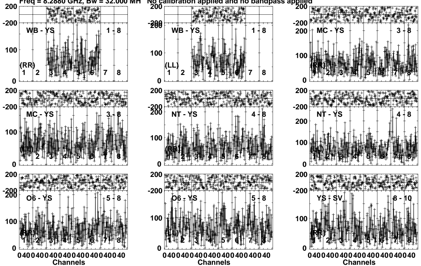
Lower frame: Micro Ampl Jy Top frame: Phas deg Vector averaged cross-power spectrum Several baselines displayed Timerange: 00/11:09:04 to 00/11:13:04
