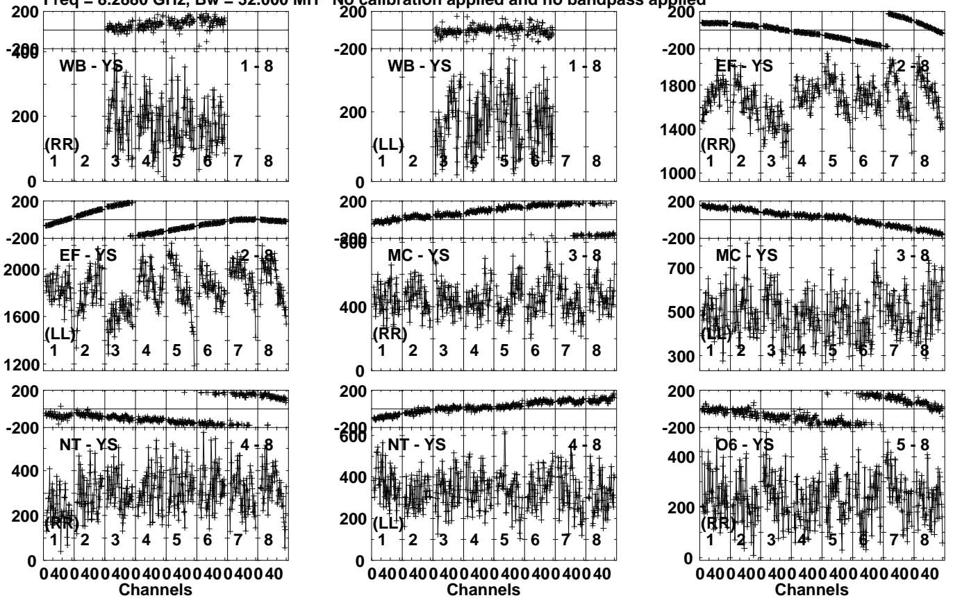
Lower frame: Micro Ampl Jy Top frame: Phas deg Vector averaged cross-power spectrum Several baselines displayed Timerange: 00/12/02:05 to 00/12/03:34
