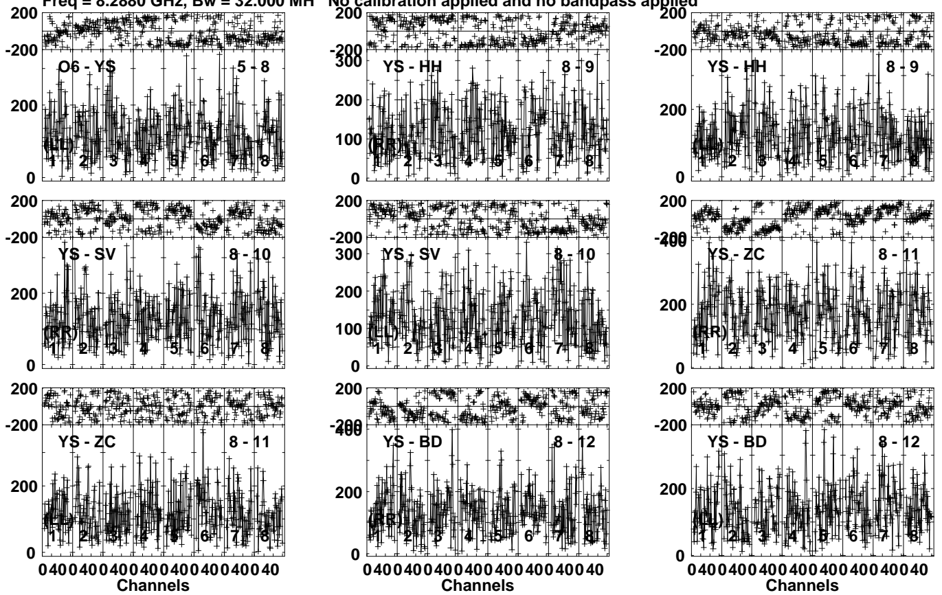
Lower frame: Micro Ampl Jy Top frame: Phas deg Vector averaged cross-power spectrum Several baselines displayed Timerange: 00/12:42:34 to 00/12:44:04
