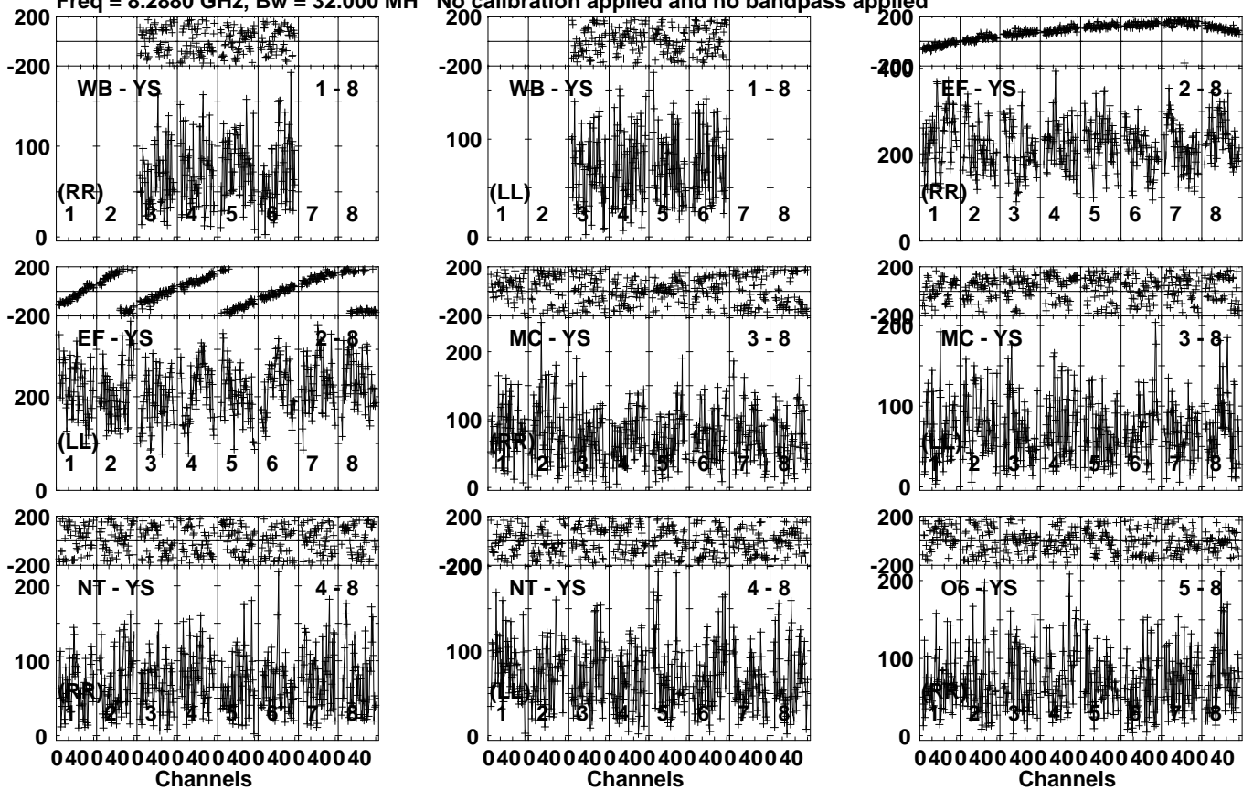
Lower frame: Micro Ampl Jy Top frame: Phas deg Vector averaged cross-power spectrum Several baselines displayed Timerange: 00/10:41:01 to 00/10:44:59
