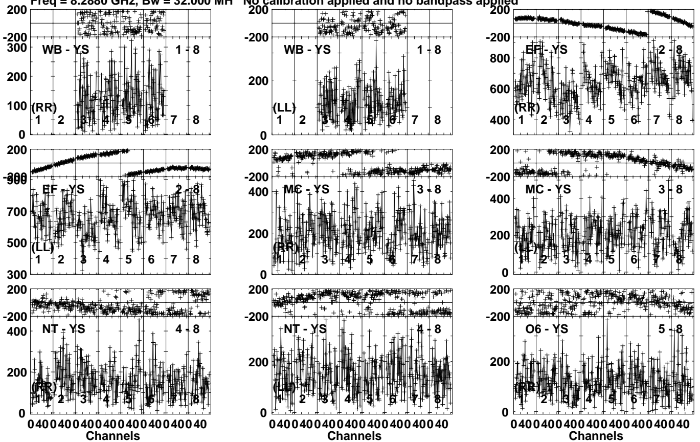
Lower frame: Micro Ampl Jy Top frame: Phas deg Vector averaged cross-power spectrum Several baselines displayed Timerange: 00/13:23:05 to 00/13:24:34
