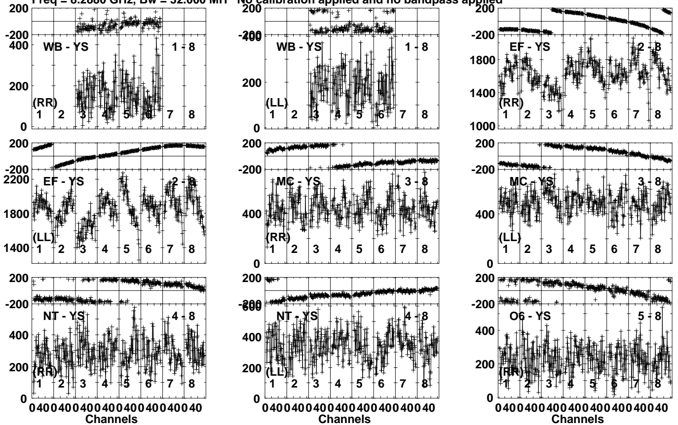
Lower frame: Micro Ampl Jy Top frame: Phas deg Vector averaged cross-power spectrum Several baselines displayed Timerange: 00/12:19:05 to 00/12:20:34
