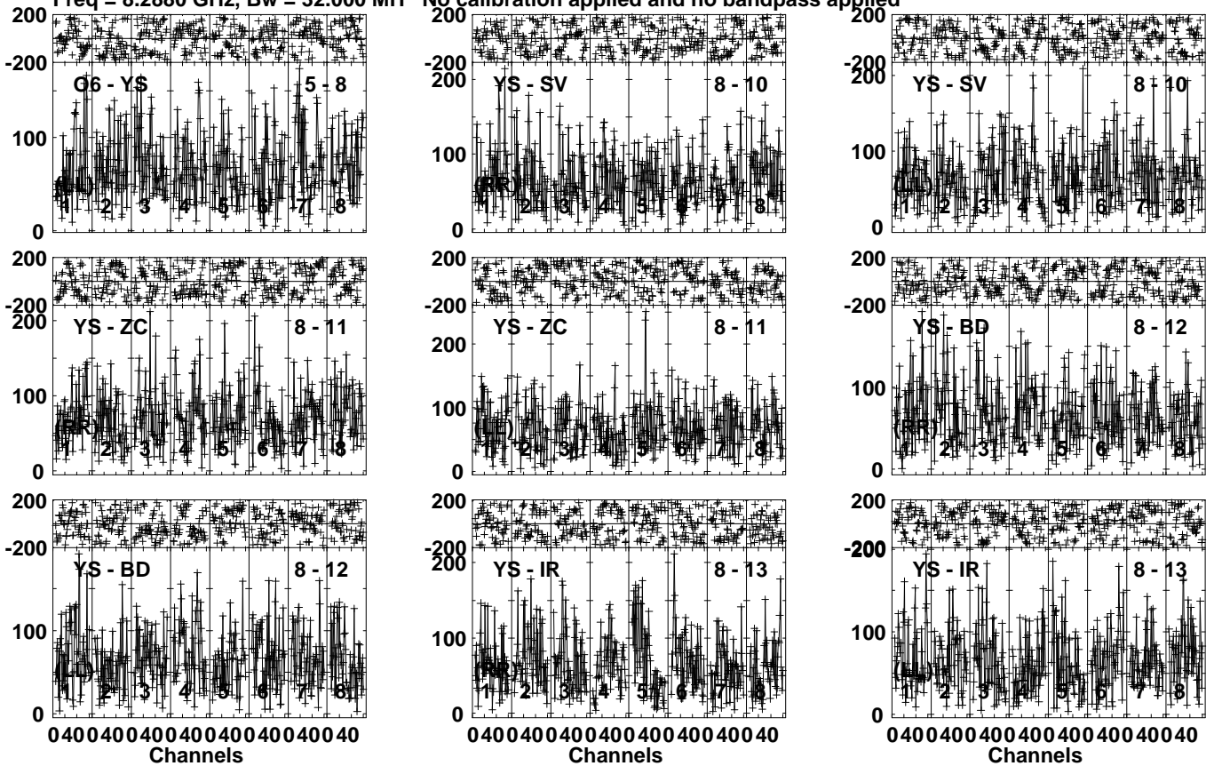
Lower frame: Micro Ampl Jy Top frame: Phas deg Vector averaged cross-power spectrum Several baselines displayed Timerange: 00:07:09:00 to 00:07:13:00
