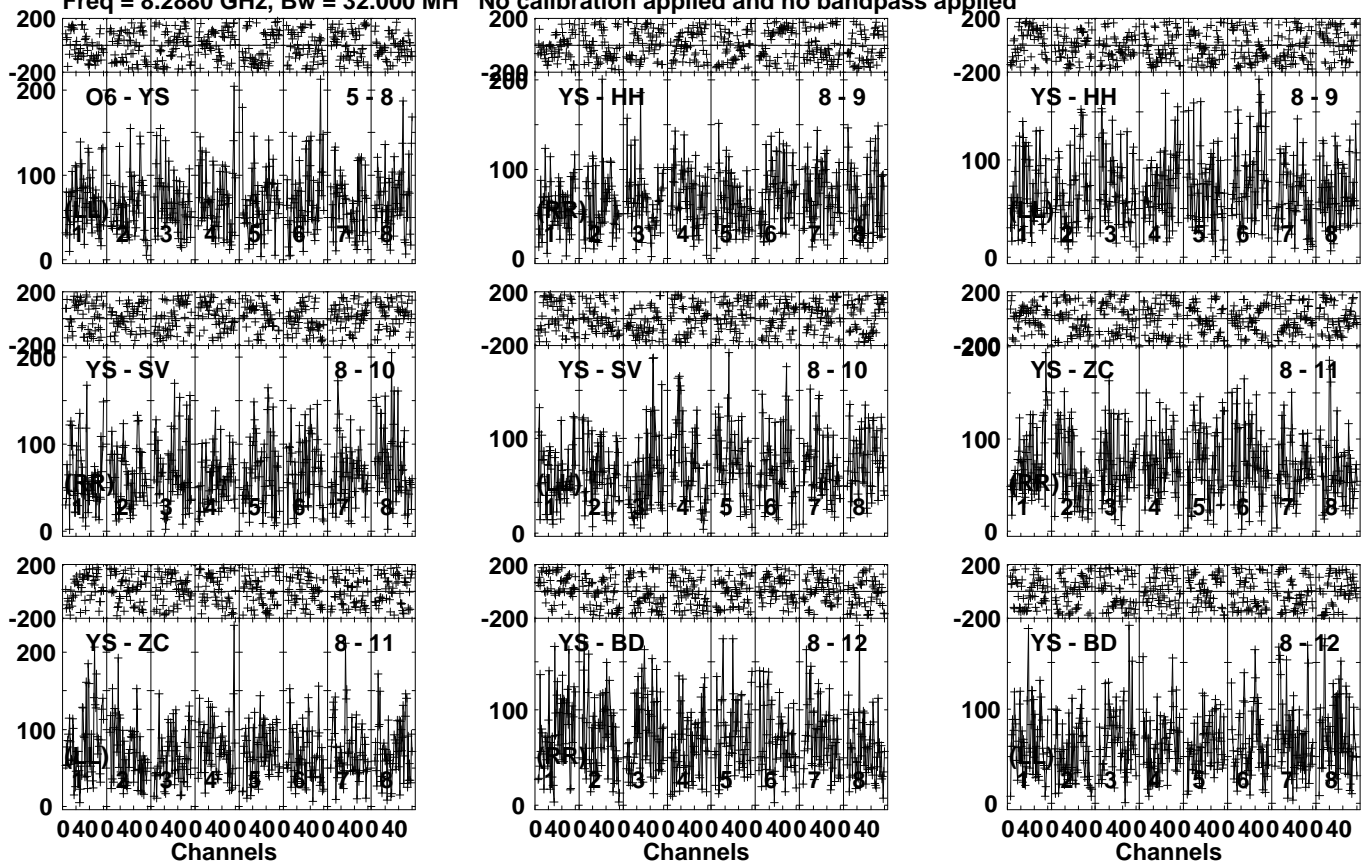
Lower frame: Micro Ampl Jy Top frame: Phas deg Vector averaged cross-power spectrum Several baselines displayed Timerange: 00/09:41:30 to 00/09:45:30
