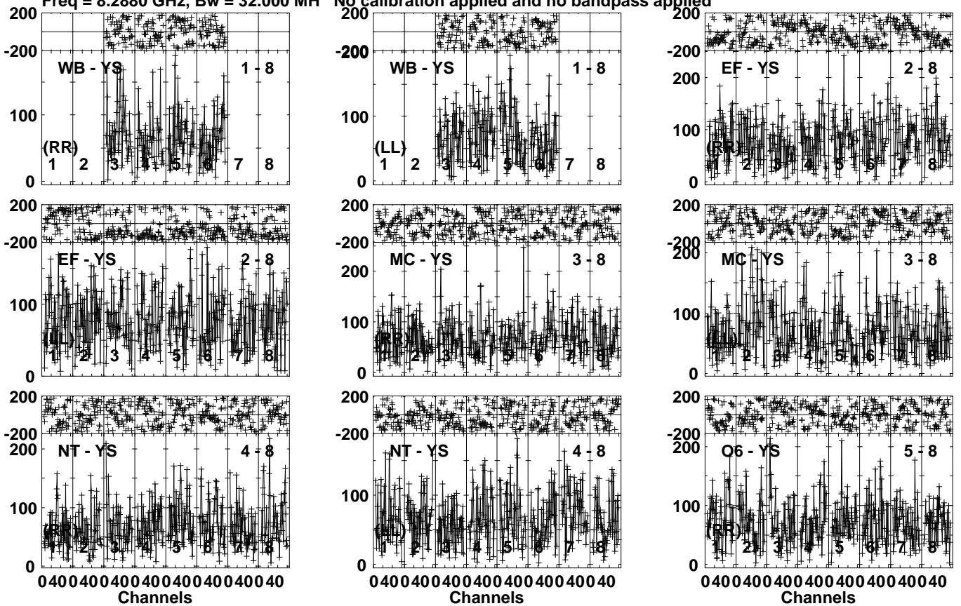
Lower frame: Micro Ampl Jy Top frame: Phas deg Vector averaged cross-power spectrum Several baselines displayed Timerange: 00/06:12:30 to 00/06:16:30
