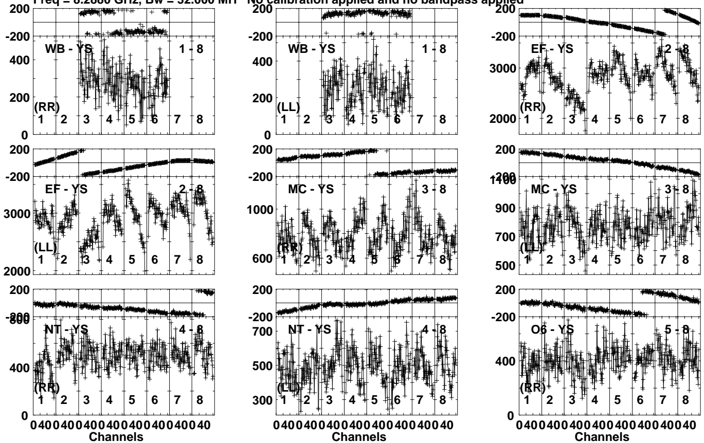
Lower frame: Micro Ampl Jy Top frame: Phas deg Vector averaged cross-power spectrum Several baselines displayed Timerange: 00/13:14:35 to 00/13:16:04
