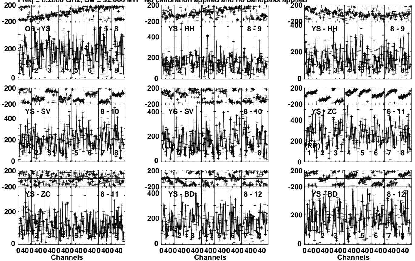
Lower frame: Micro Ampl Jy Top frame: Phas deg Vector averaged cross-power spectrum Several baselines displayed Timerange: 00/10:46:01 to 00/10:47:29
