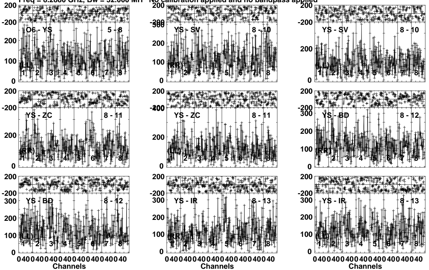
Lower frame: Micro Ampl Jy Top frame: Phas deg Vector averaged cross-power spectrum Several baselines displayed Timerange: 00/06:58:00 to 00/06:59:29
