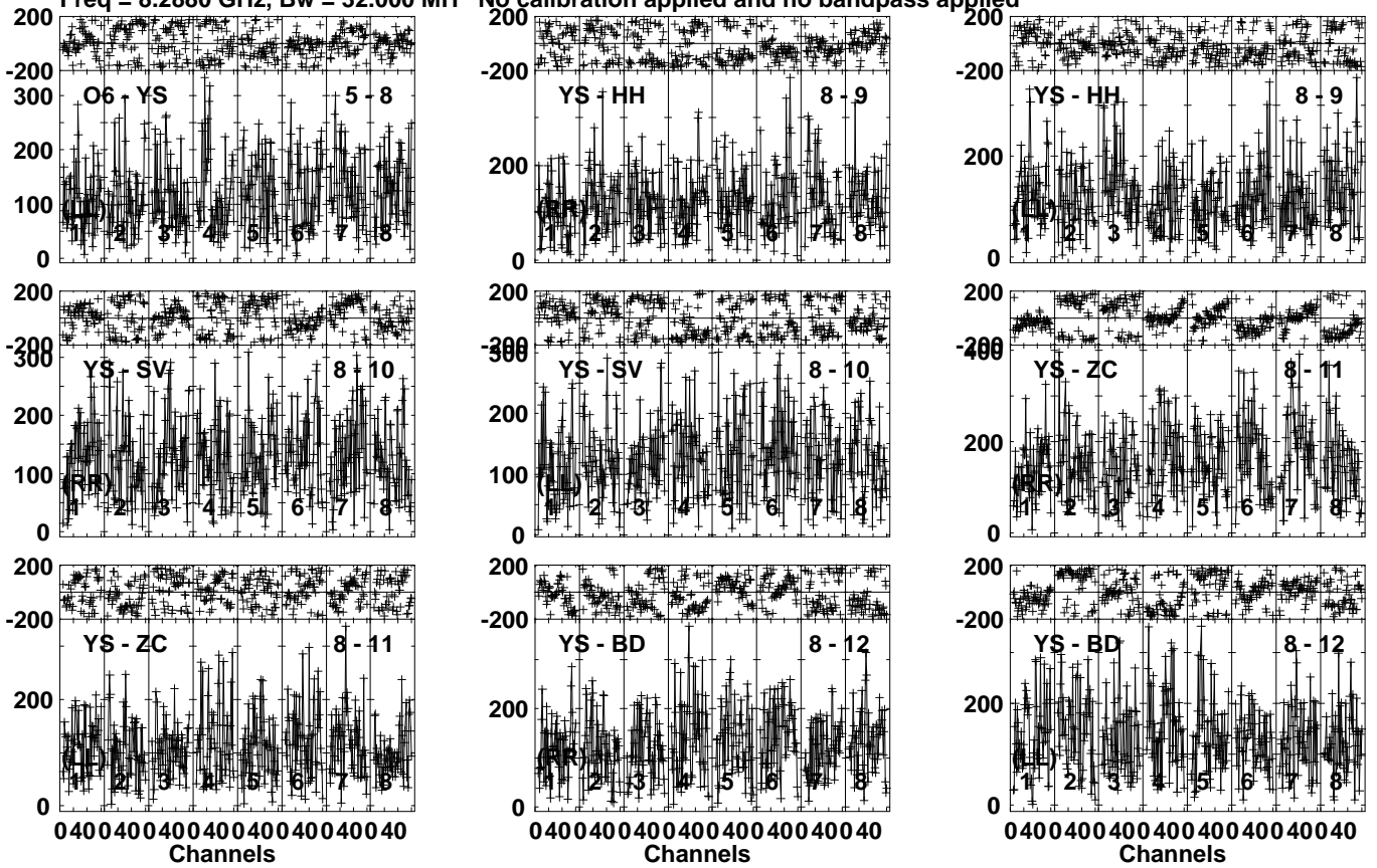
Lower frame: Micro Ampl Jy Top frame: Phas deg Vector averaged cross-power spectrum Several baselines displayed Timerange: 00/12:35:04 to 00/12:36:33
