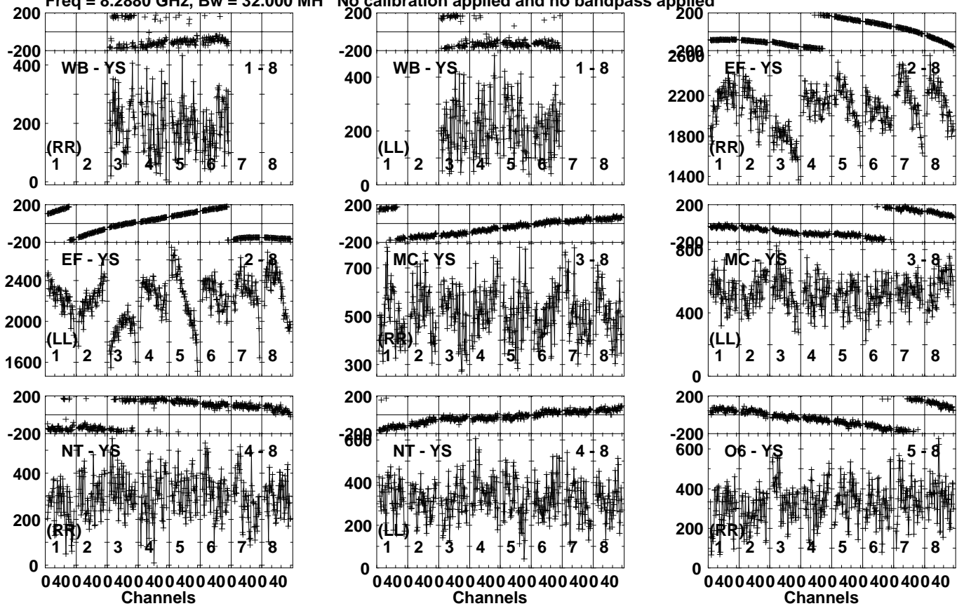
Lower frame: Micro Ampl Jy Top frame: Phas deg Vector averaged cross-power spectrum Several baselines displayed Timerange: 00/07:21:31 to 00/07:23:00
