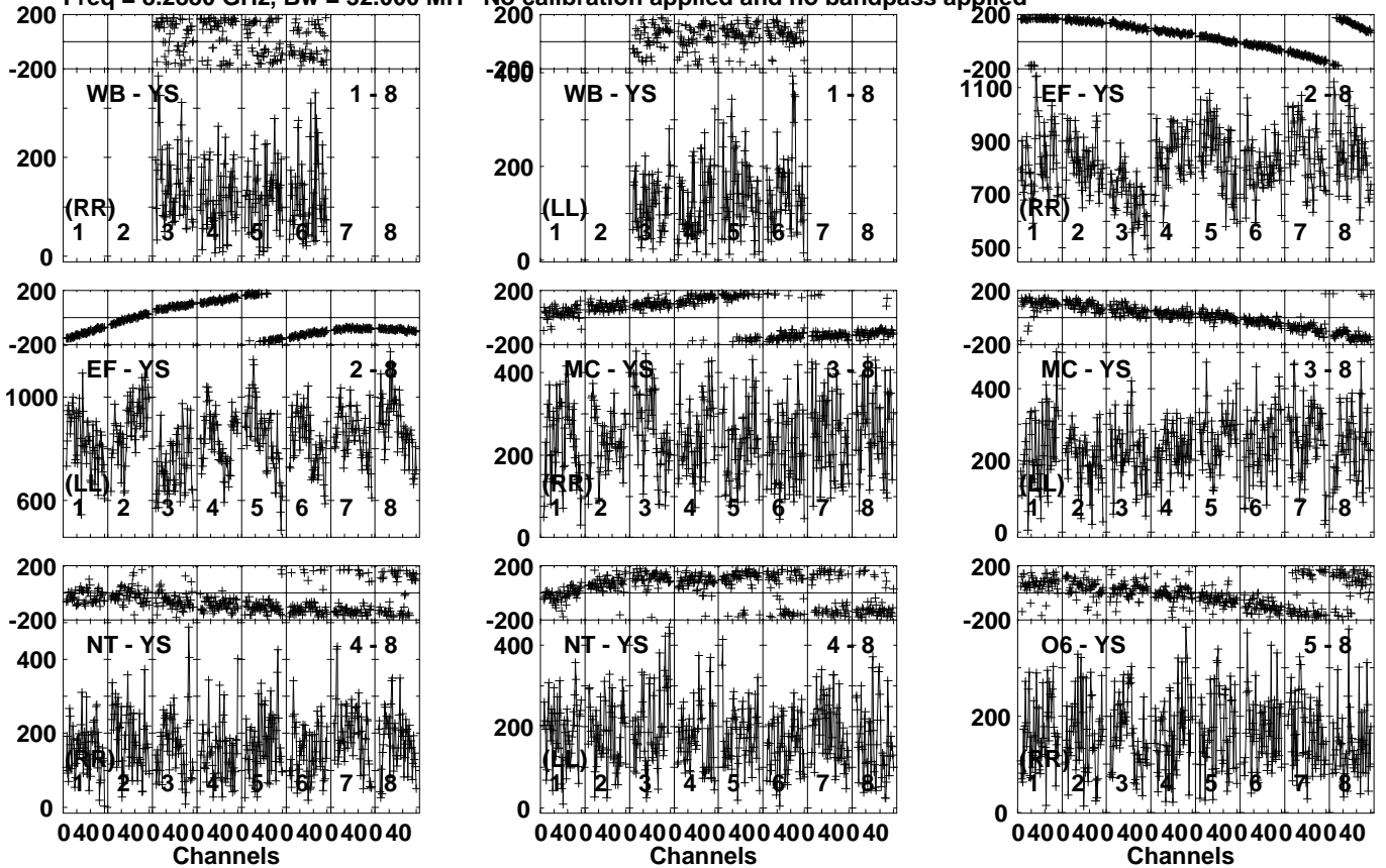
Lower frame: Micro Ampl Jy Top frame: Phas deg Vector averaged cross-power spectrum Several baselines displayed Timerange: 00/10:12:31 to 00/10:13:59
