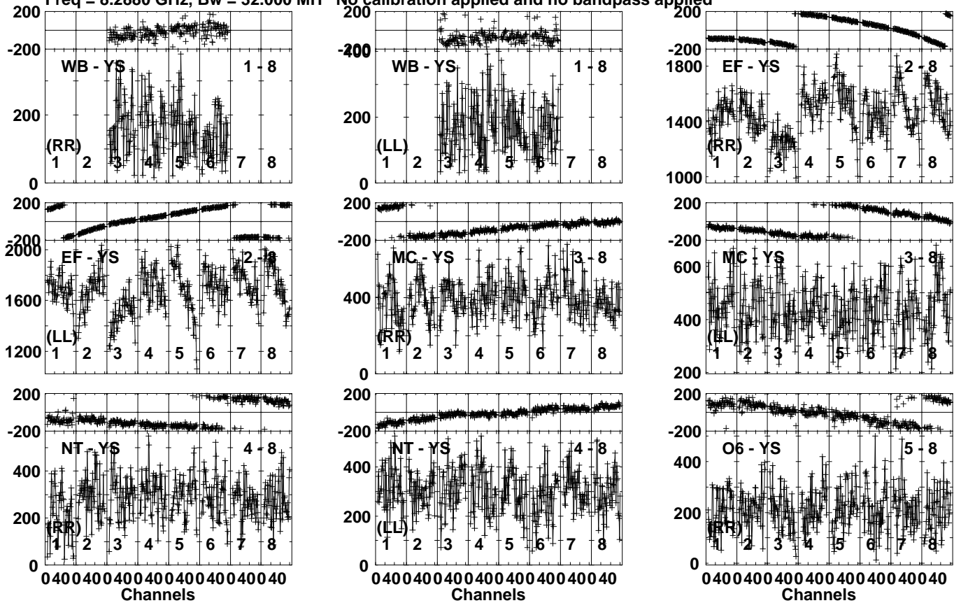
Lower frame: Micro Ampl Jy Top frame: Phas deg Vector averaged cross-power spectrum Several baselines displayed Timerange: 00/12:26:35 to 00/12:28:03
