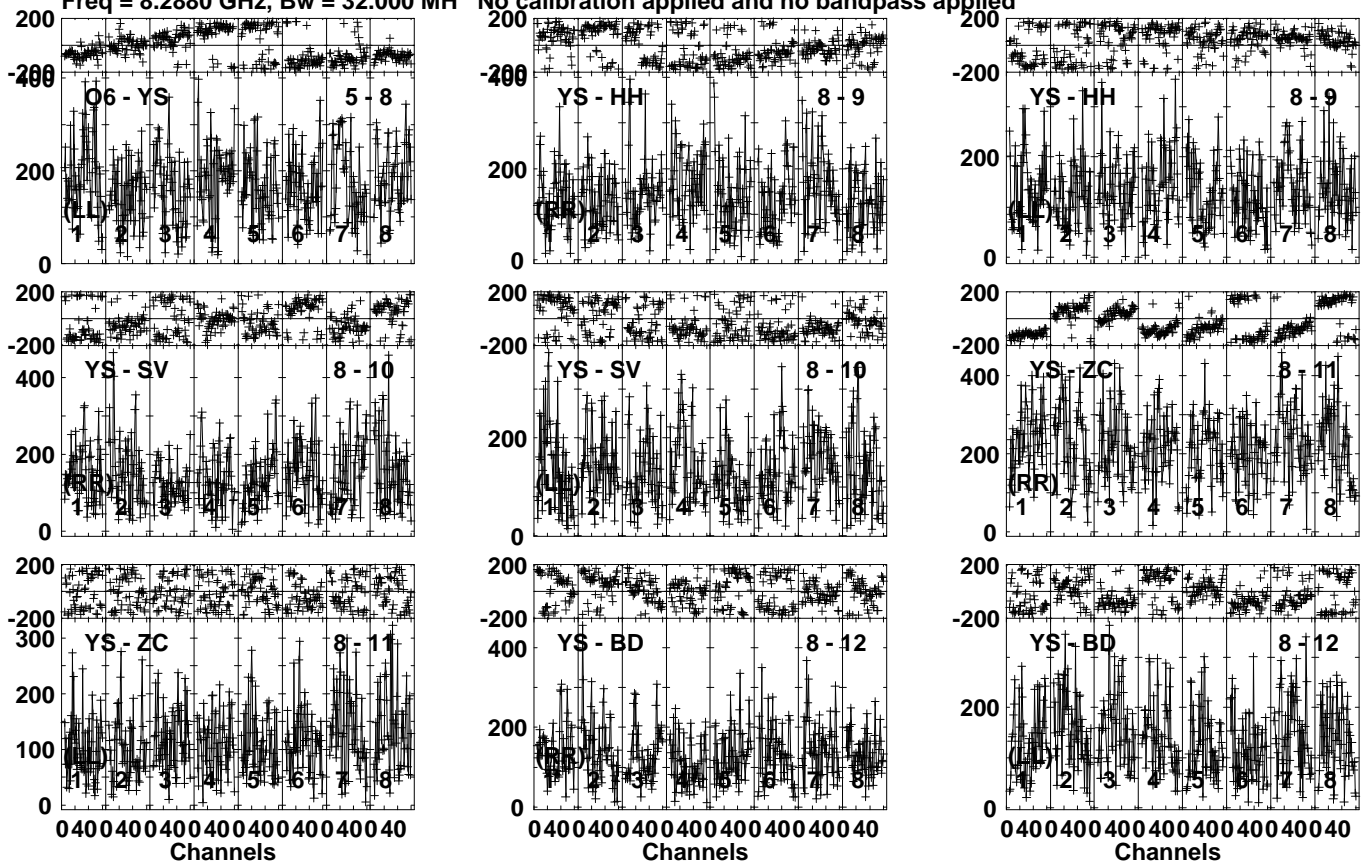
Lower frame: Micro Ampl Jy Top frame: Phas deg Vector averaged cross-power spectrum Several baselines displayed Timerange: 00/09:28:01 to 00/09:29:29
