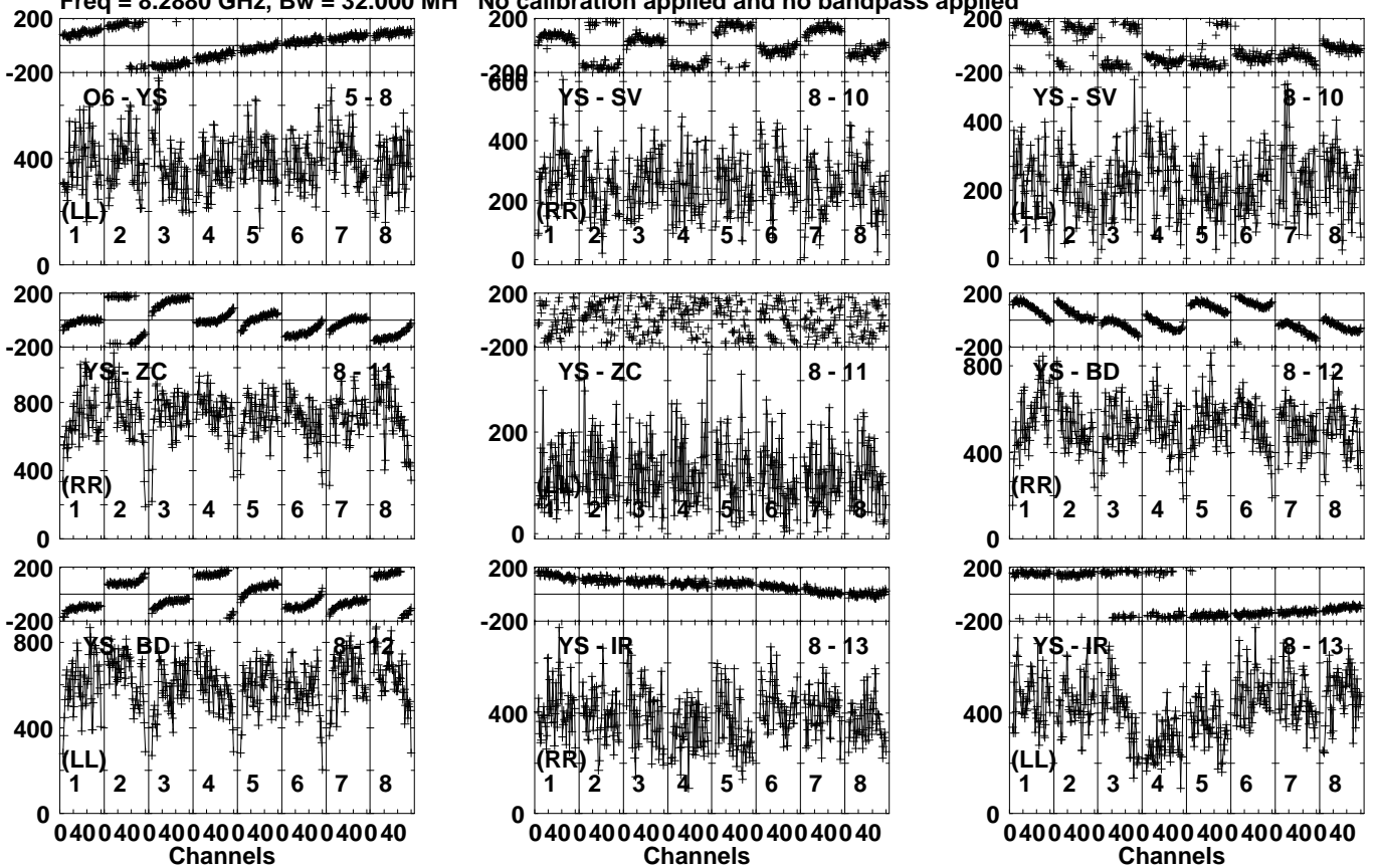
Lower frame: Micro Ampl Jy Top frame: Phas deg Vector averaged cross-power spectrum Several baselines displayed Timerange: 00/06:26:00 to 00/06:27:29
