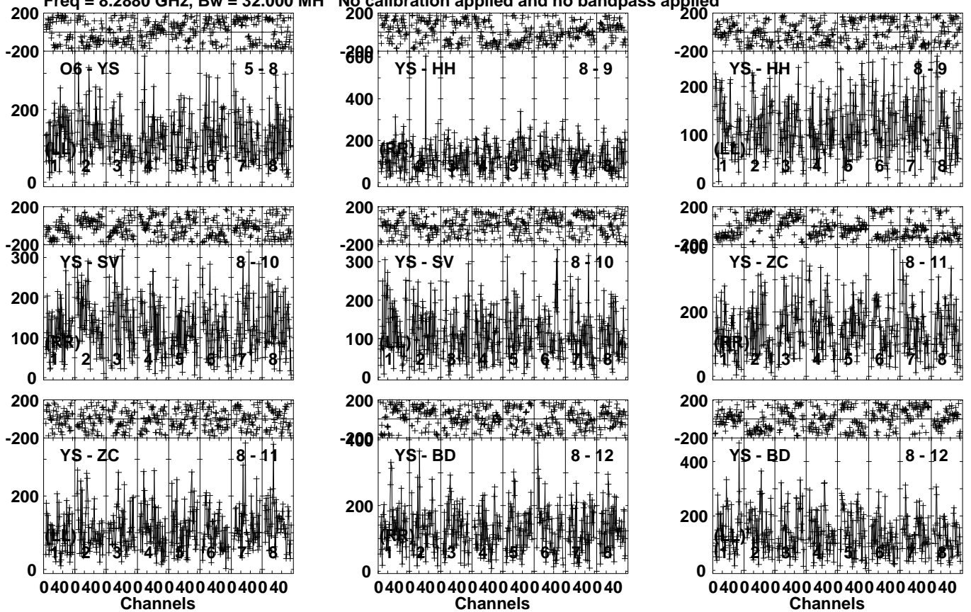
Lower frame: Micro Ampl Jy Top frame: Phas deg Vector averaged cross-power spectrum Several baselines displayed Timerange: 00/11:45:04 to 00/11:46:34
