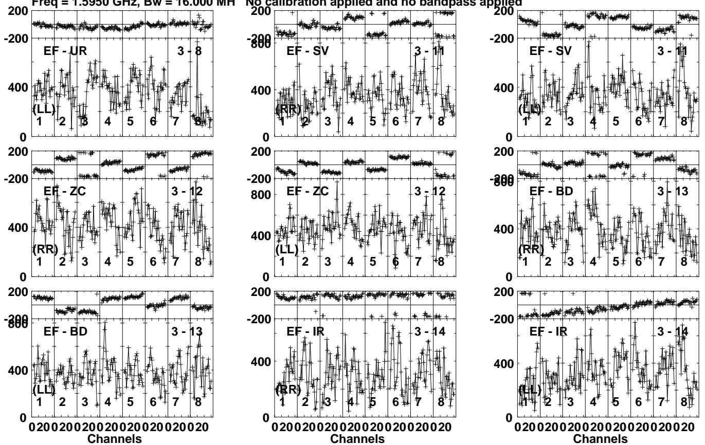
Lower frame: Micro Ampl Jy Top frame: Phas deg Vector averaged cross-power spectrum Several baselines displayed Timerange: 01/09:55:00 to 01/09:58:00
