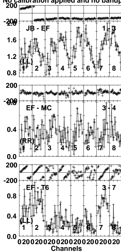
Lower frame: Milli Ampl Jy Top frame: Phas deg Vector averaged cross-power spectrum Several baselines displayed Timerange: 01/12:45:00 to 01/12:48:00
