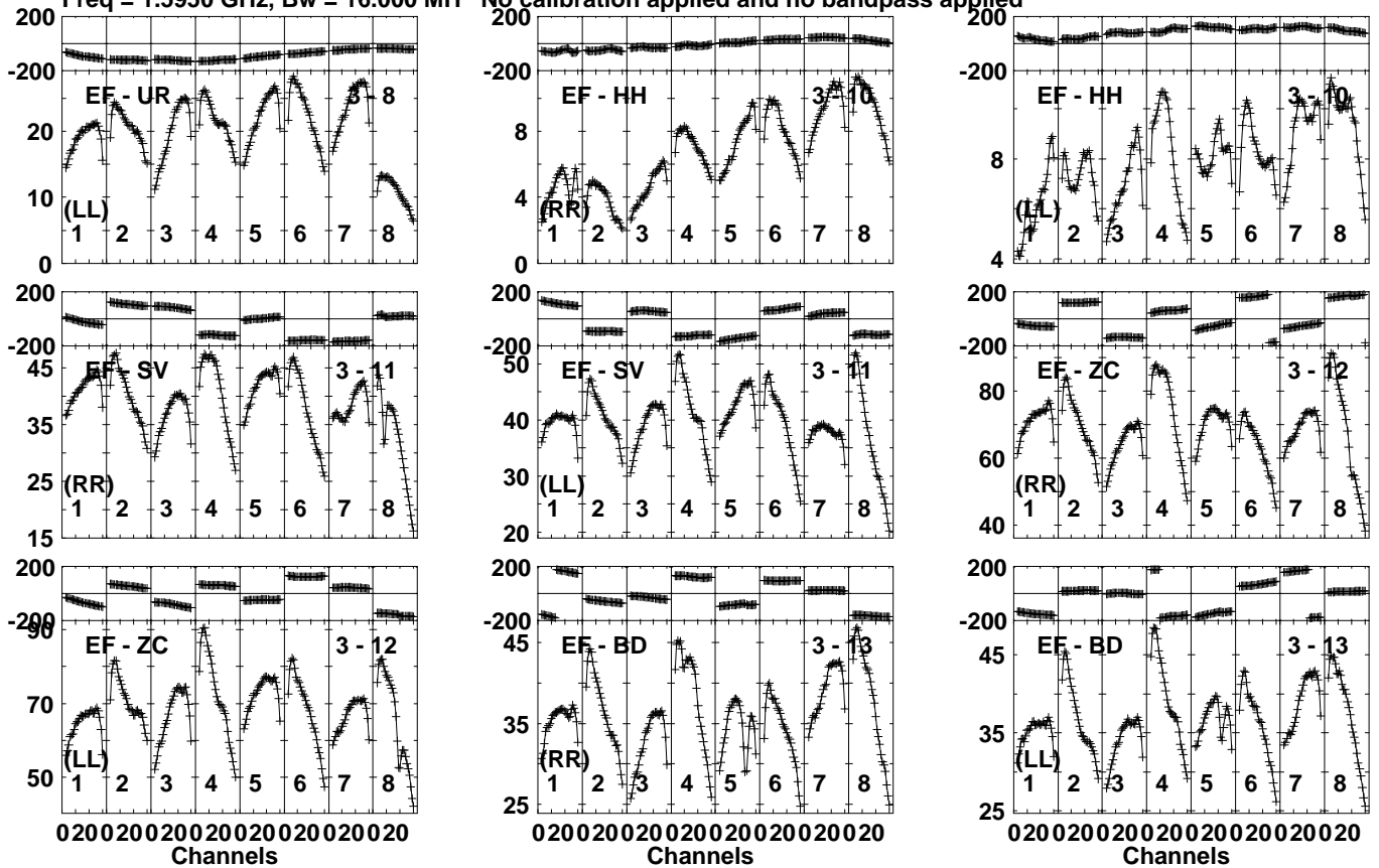
Lower frame: Milli Ampl Jy Top frame: Phas deg Vector averaged cross-power spectrum Several baselines displayed Timerange: 00/23:09:30 to 00/23:10:00
