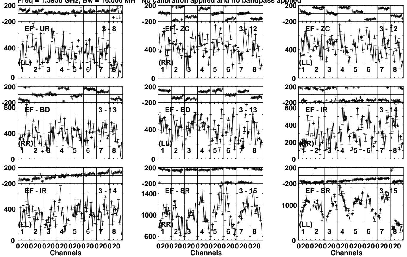
Lower frame: Micro Ampl Jy Top frame: Phas deg Vector averaged cross-power spectrum Several baselines displayed Timerange: 01/10:20:00 to 01/10:23:00
