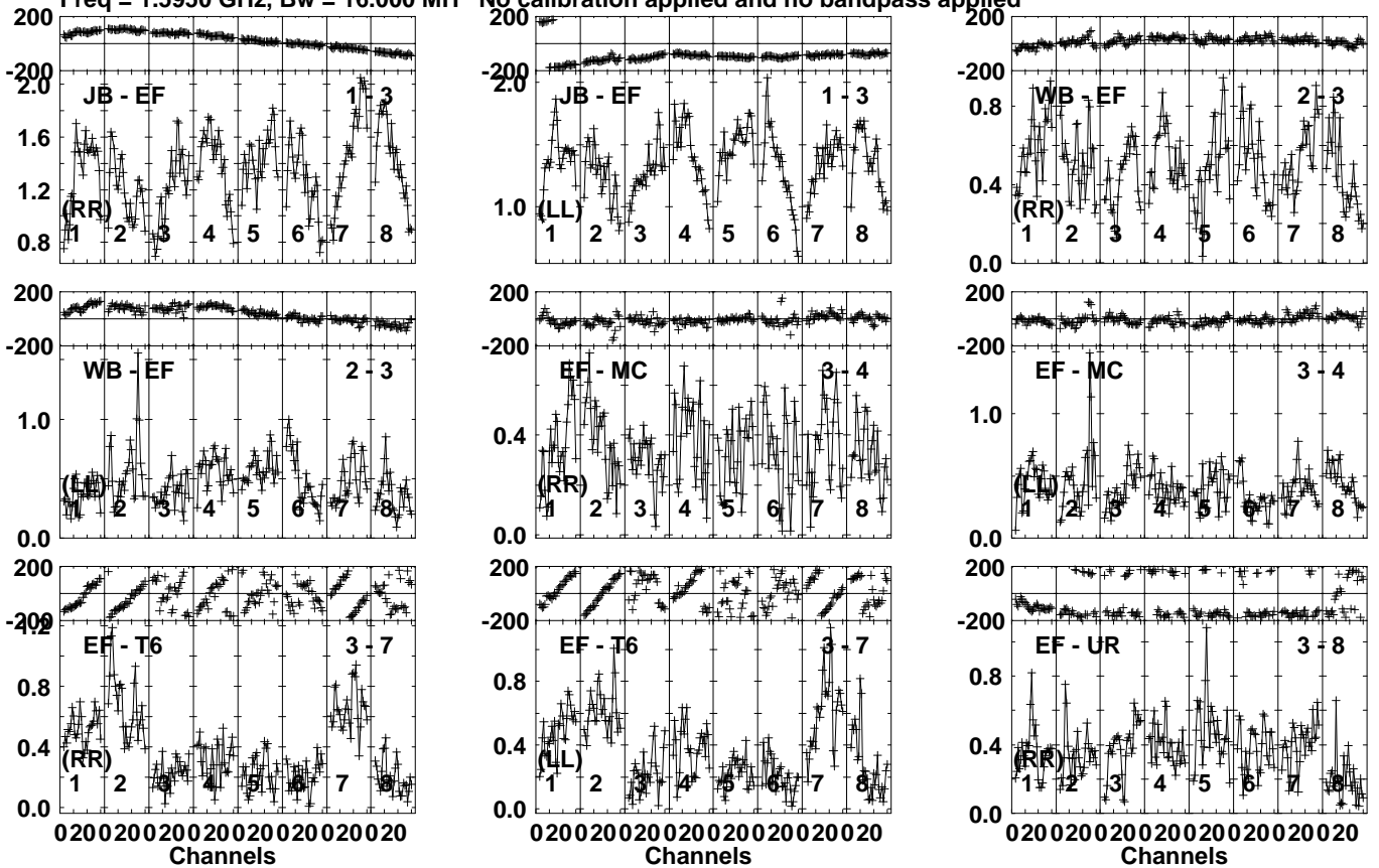
Lower frame: Milli Ampl Jy Top frame: Phas deg Vector averaged cross-power spectrum Several baselines displayed Timerange: 01/12:50:01 to 01/12:53:00
