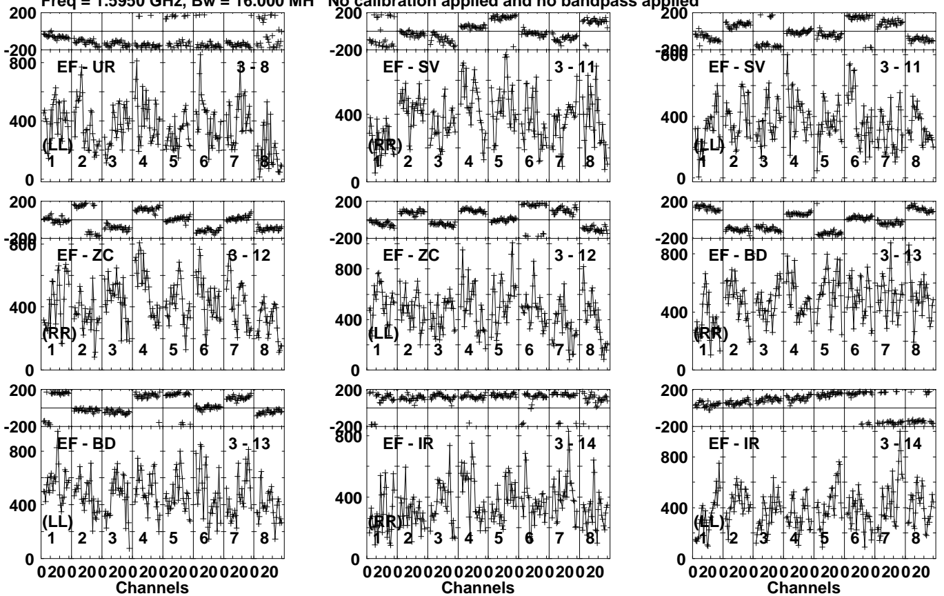
Lower frame: Micro Ampl Jy Top frame: Phas deg Vector averaged cross-power spectrum Several baselines displayed Timerange: 01/13:00:01 to 01/13:03:00
