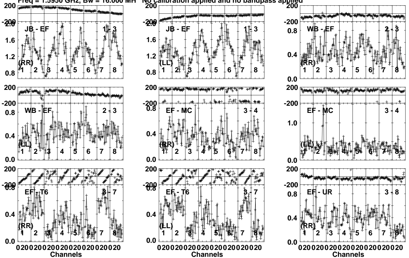
Lower frame: Milli Ampl Jy Top frame: Phas deg Vector averaged cross-power spectrum Several baselines displayed Timerange: 01/13:20:00 to 01/13:23:00
