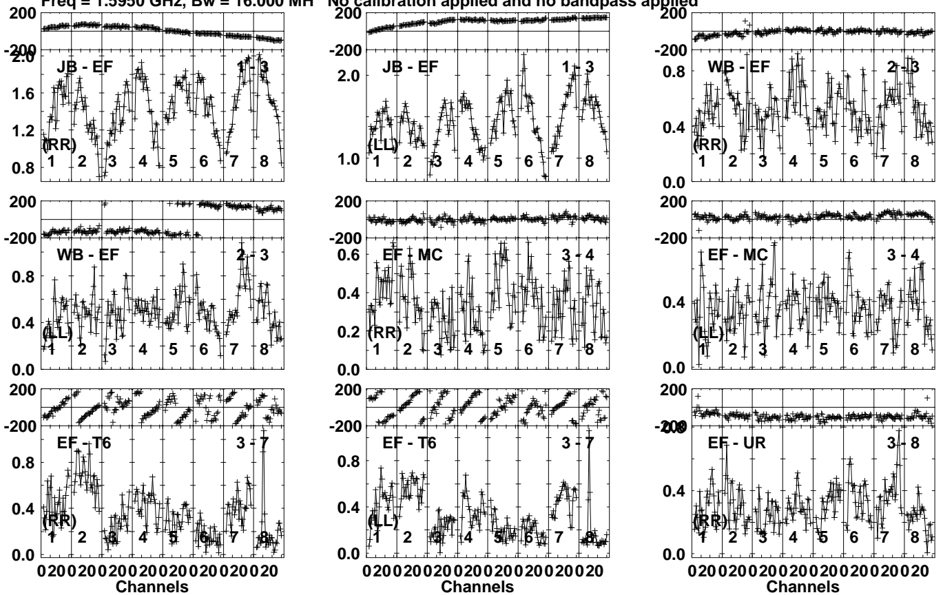
Lower frame: Milli Ampl Jy Top frame: Phas deg Vector averaged cross-power spectrum Several baselines displayed Timerange: 01/11:20:01 to 01/11:23:00
