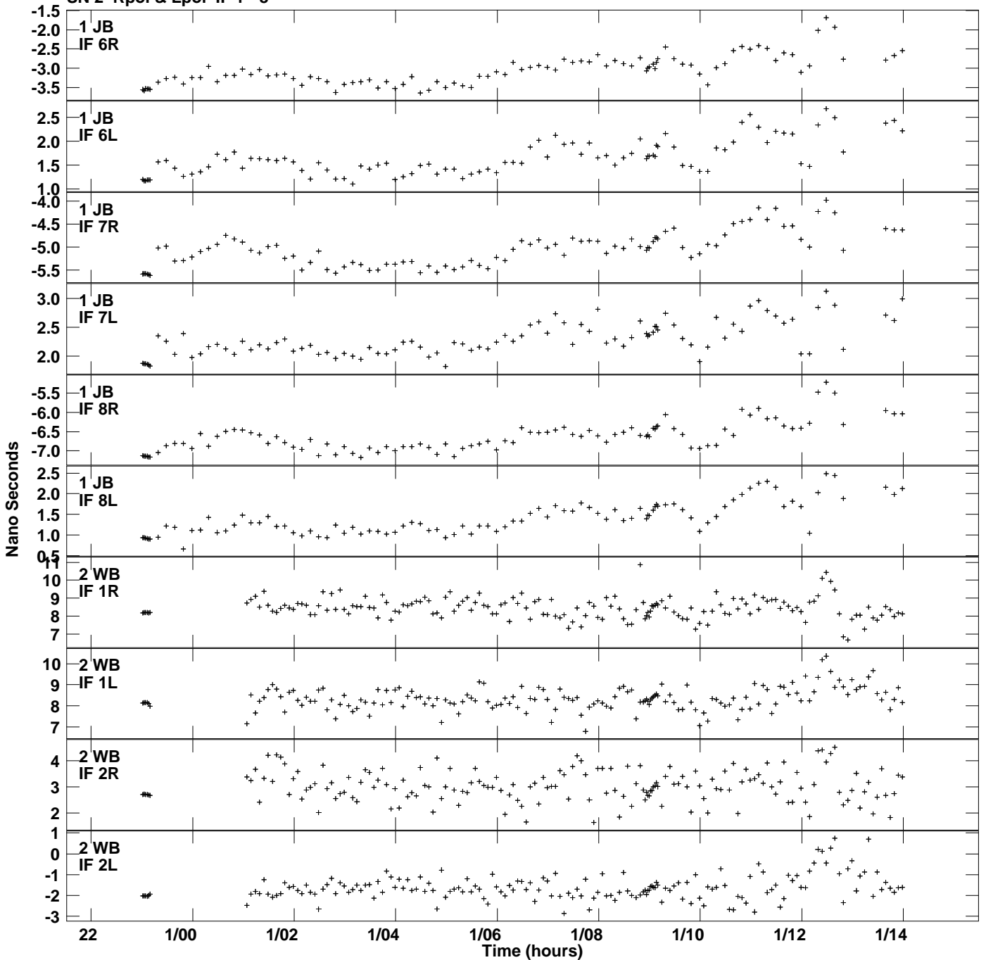
Plot file version 2 created 01-FEB-2021 14:09:28 Delay vs UTC time for EB082.UVDATA.1 SN 2 Rpol & Lpol IF 1 - 8
