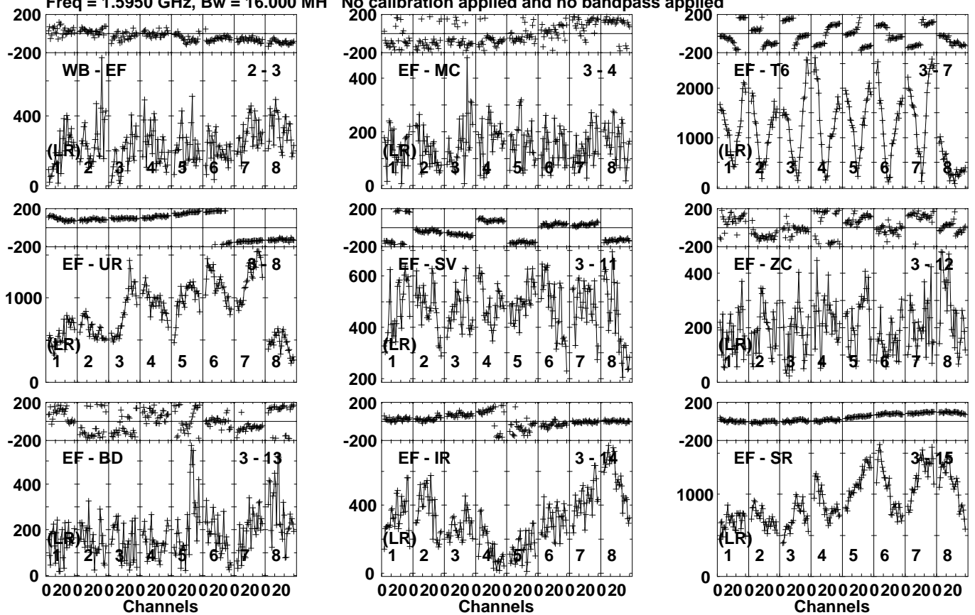
Lower frame: Micro Ampl Jy Top frame: Phas deg Vector averaged cross-power spectrum Several baselines displayed Timerange: 01/02:03:30 to 01/02:04:59
