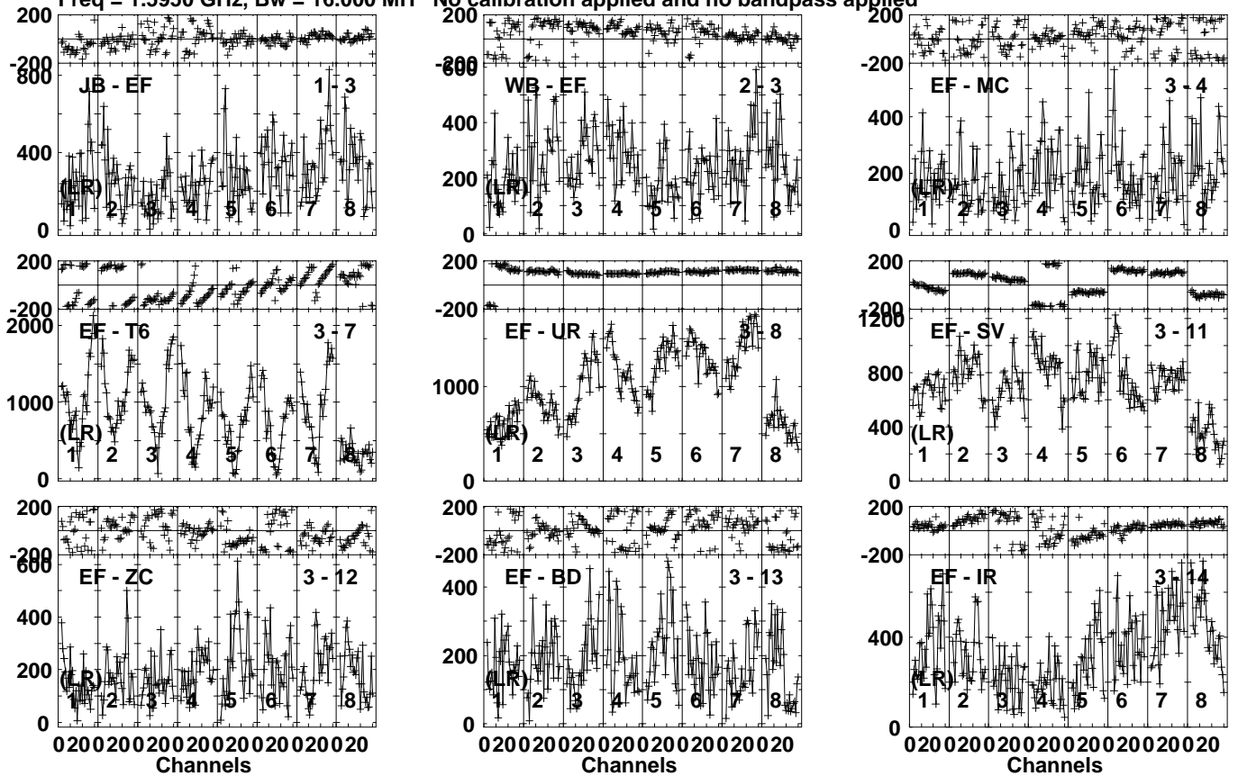
Lower frame: Micro Ampl Jy Top frame: Phas deg Vector averaged cross-power spectrum Several baselines displayed Timerange: 01/12:48:01 to 01/12:49:59
