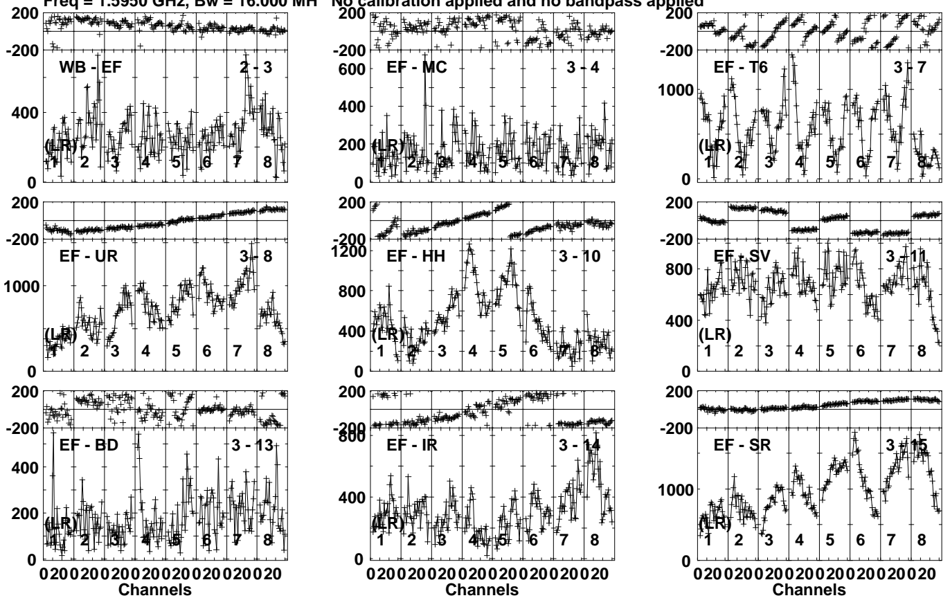
Lower frame: Micro Ampl Jy Top frame: Phas deg Vector averaged cross-power spectrum Several baselines displayed Timerange: 01/06:23:31 to 01/06:24:59
