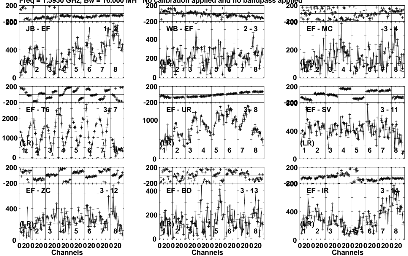
Lower frame: Micro Ampl Jy Top frame: Phas deg Vector averaged cross-power spectrum Several baselines displayed Timerange: 01/01:18:00 to 01/01:19:59
