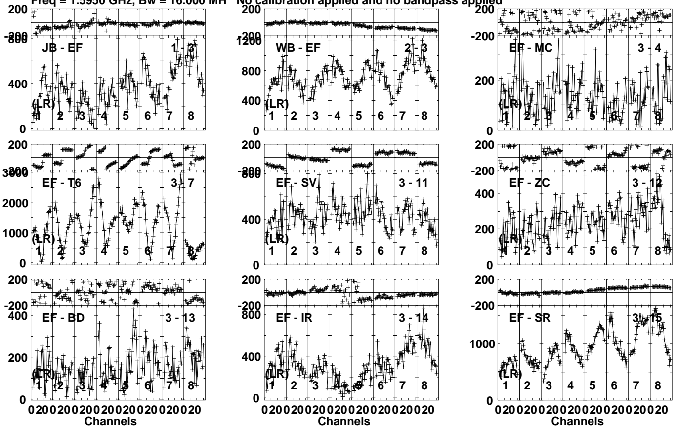
Lower frame: Micro Ampl Jy Top frame: Phas deg Vector averaged cross-power spectrum Several baselines displayed Timerange: 01/01:38:01 to 01/01:40:00
