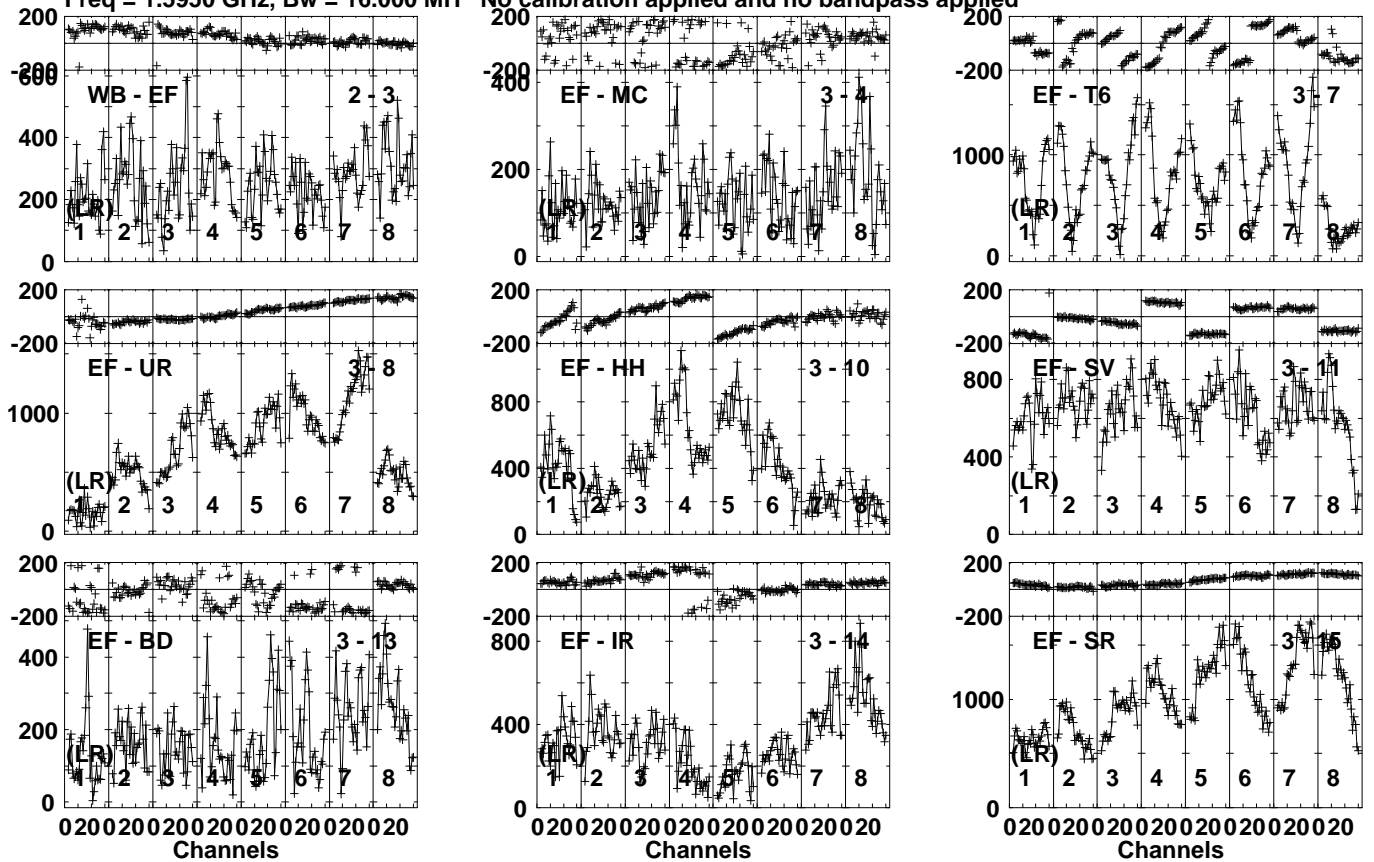
Lower frame: Micro Ampl Jy Top frame: Phas deg Vector averaged cross-power spectrum Several baselines displayed Timerange: 01/04:43:31 to 01/04:44:59
