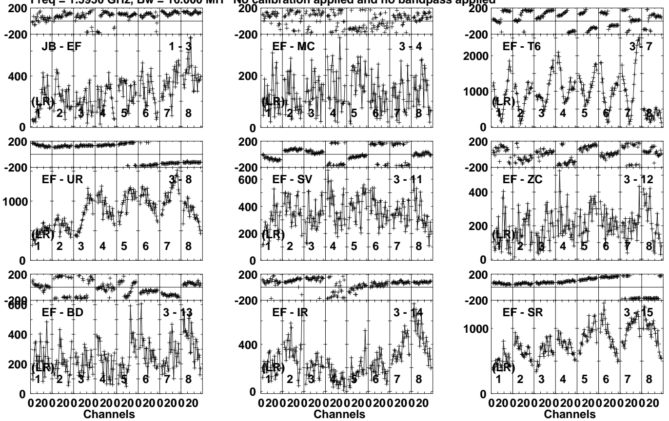
Lower frame: Micro Ampl Jy Top frame: Phas deg Vector averaged cross-power spectrum Several baselines displayed Timerange: 00/23:48:00 to 00/23:50:00
