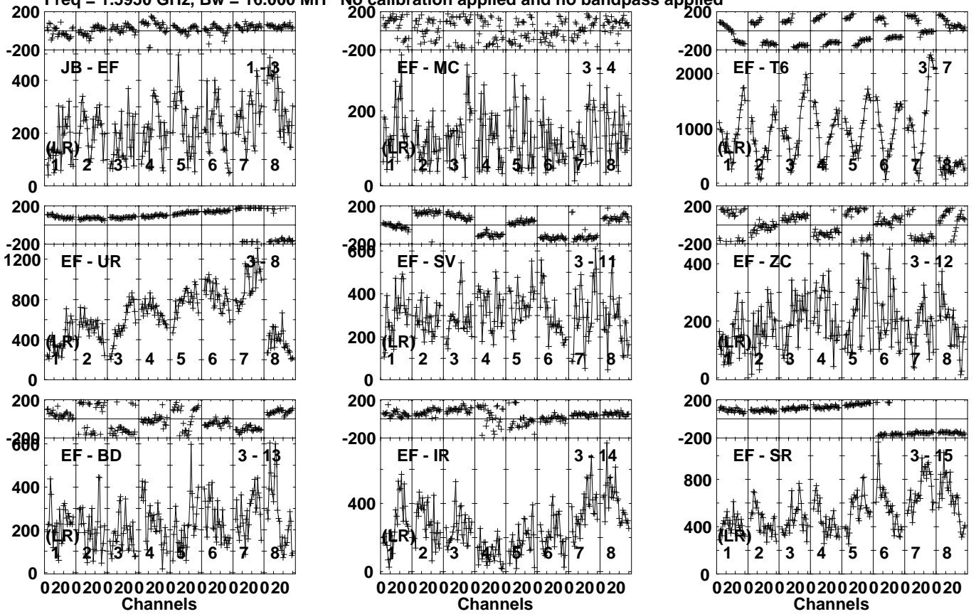
Lower frame: Micro Ampl Jy Top frame: Phas deg Vector averaged cross-power spectrum Several baselines displayed Timerange: 00/23:18:01 to 00/23:20:00
