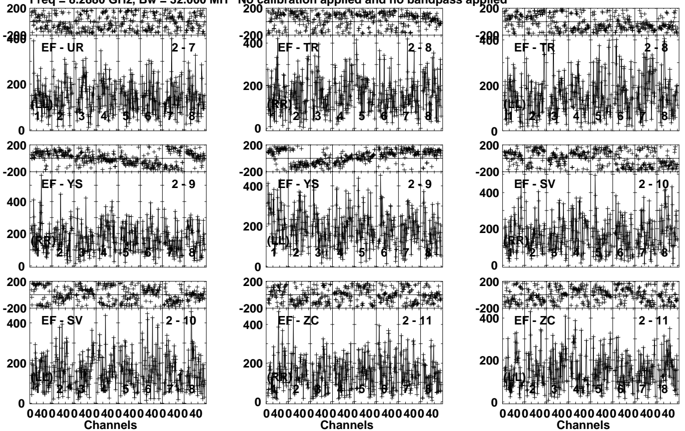
Lower frame: Micro Ampl Jy Top frame: Phas deg Vector averaged cross-power spectrum Several baselines displayed Timerange: 00/13:37:09 to 00/13:39:07
