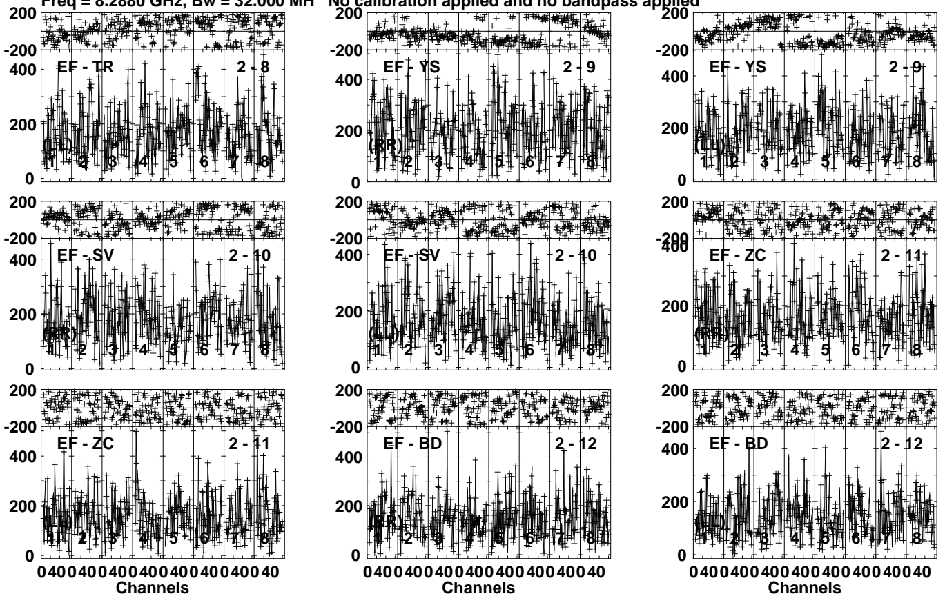
Lower frame: Micro Ampl Jy Top frame: Phas deg Vector averaged cross-power spectrum Several baselines displayed Timerange: 00/19:52:29 to 00/19:54:27
