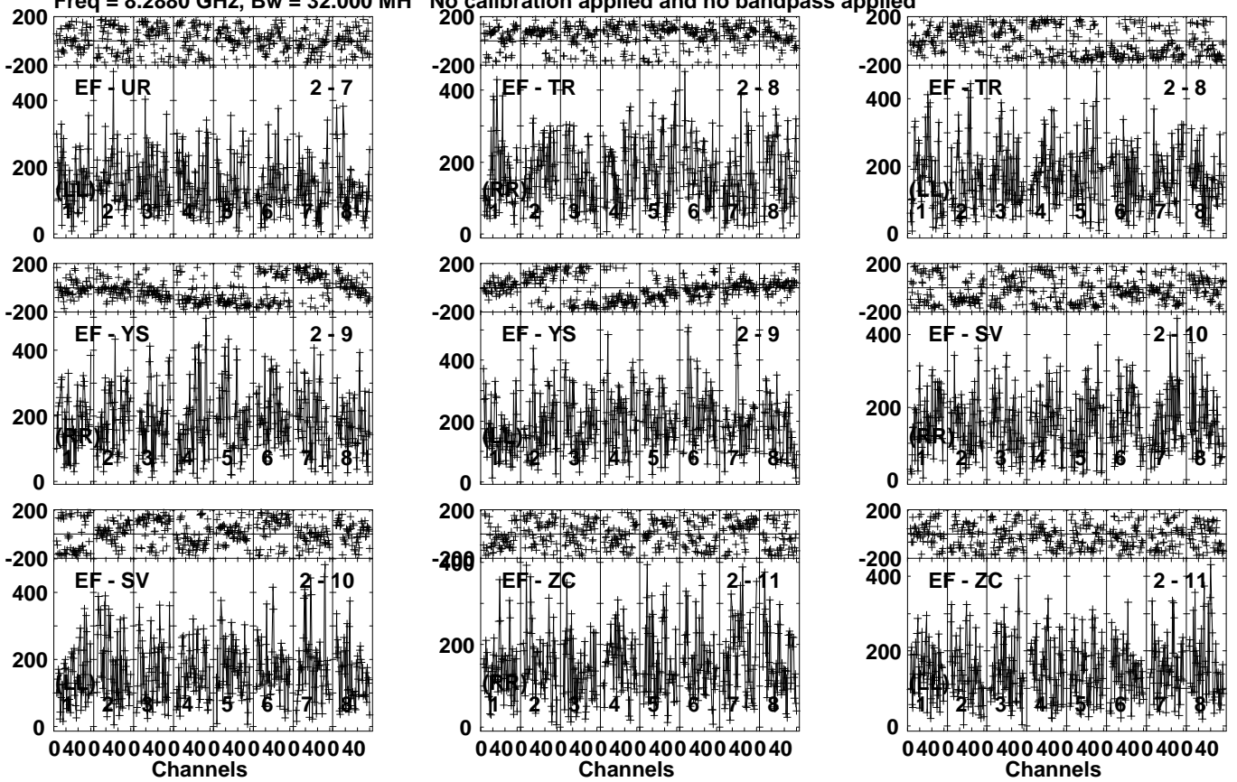
Lower frame: Micro Ampl Jy Top frame: Phas deg Vector averaged cross-power spectrum Several baselines displayed Timerange: 00/16:21:33 to 00/16:23:31
