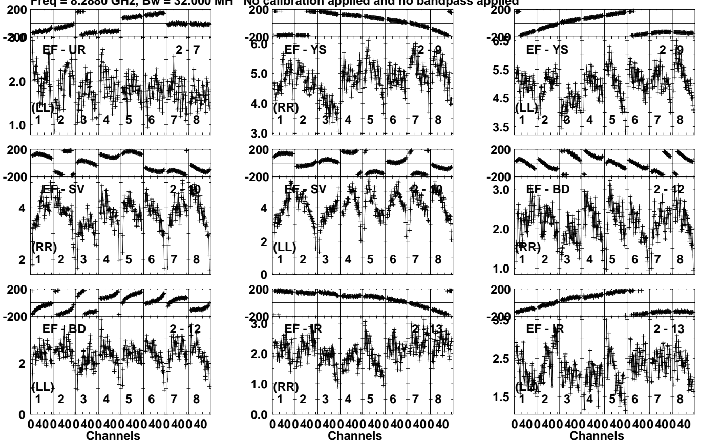
Lower frame: Milli Ampl Jy Top frame: Phas deg Vector averaged cross-power spectrum Several baselines displayed Timerange: 00/16:49:13 to 00/16:50:31
