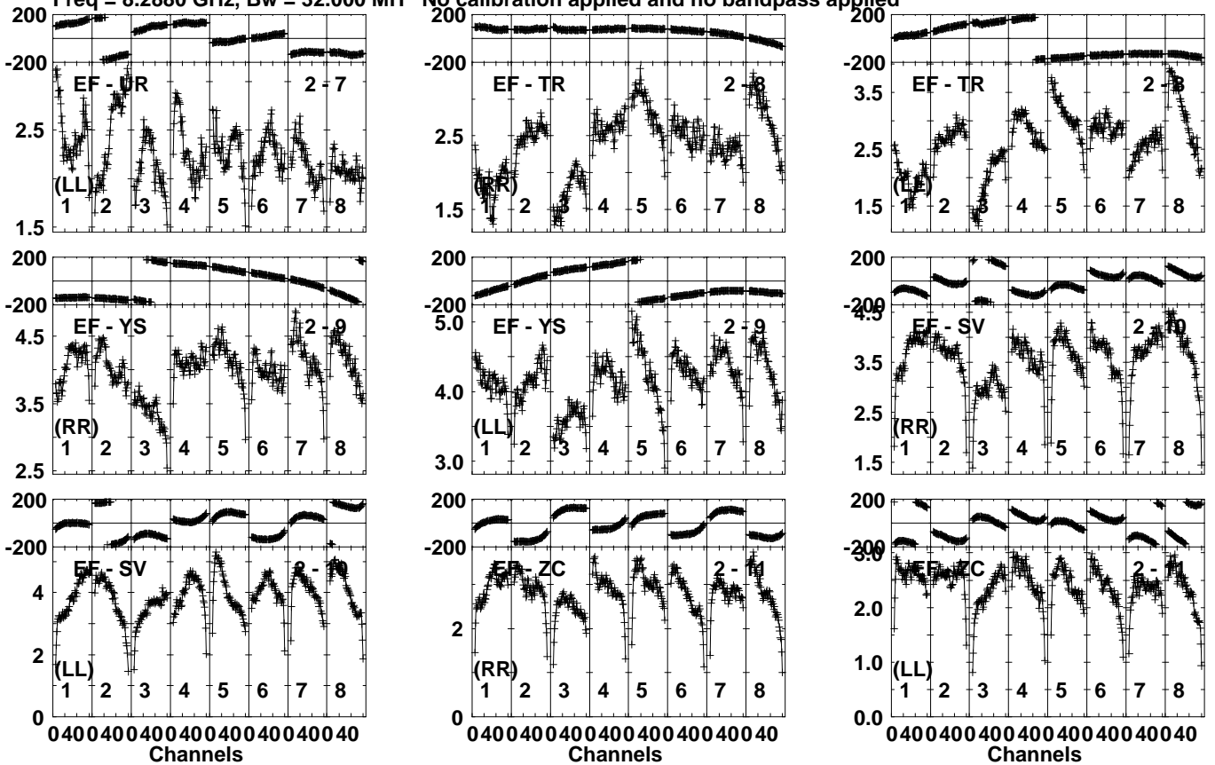
Lower frame: Milli Ampl Jy Top frame: Phas deg Vector averaged cross-power spectrum Several baselines displayed Timerange: 00/13:17:37 to 00/13:19:05
