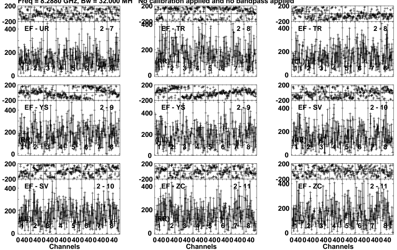
Lower frame: Micro Ampl Jy Top frame: Phas deg Vector averaged cross-power spectrum Several baselines displayed Timerange: 00/14:16:33 to 00/14:18:31
