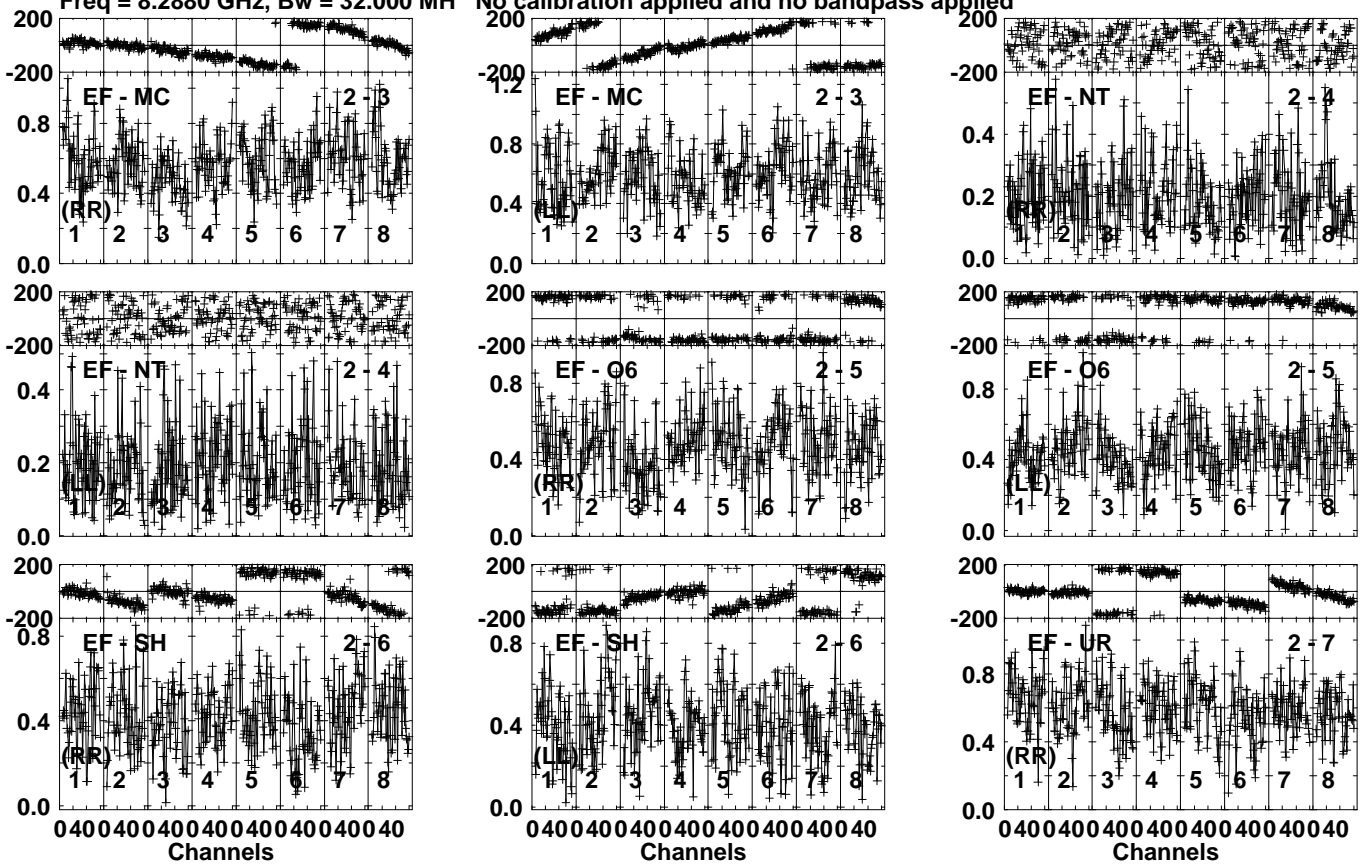
Lower frame: Milli Ampl Jy Top frame: Phas deg Vector averaged cross-power spectrum Several baselines displayed Timerange: 00/11:08:03 to 00/11:09:21
