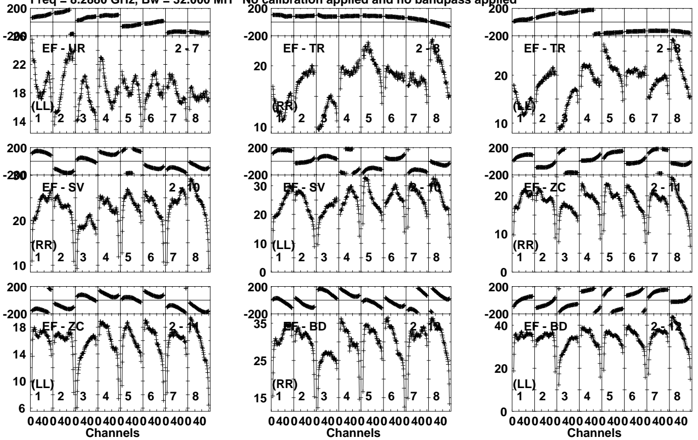
Lower frame: Milli Ampl Jy Top frame: Phas deg Vector averaged cross-power spectrum Several baselines displayed Timerange: 00/09:30:01 to 00/09:33:29
