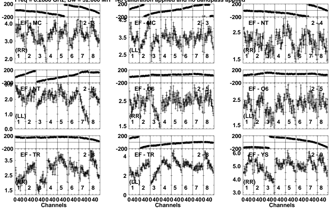
Lower frame: Milli Ampl Jy Top frame: Phas deg Vector averaged cross-power spectrum Several baselines displayed Timerange: 00/22:35:19 to 00/22:36:37
