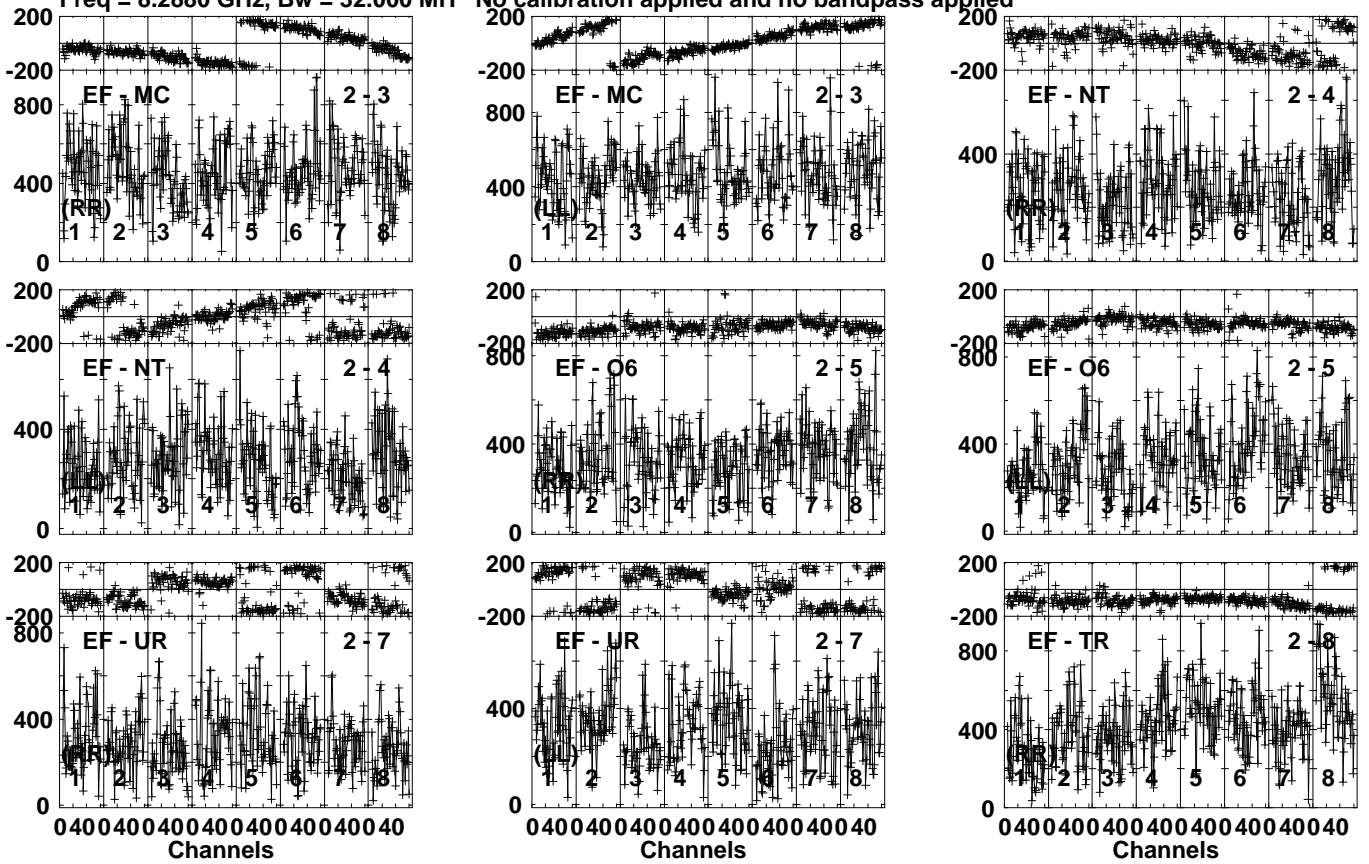
Lower frame: Micro Ampl Jy Top frame: Phas deg Vector averaged cross-power spectrum Several baselines displayed Timerange: 00/21:36:39 to 00/21:38:07
