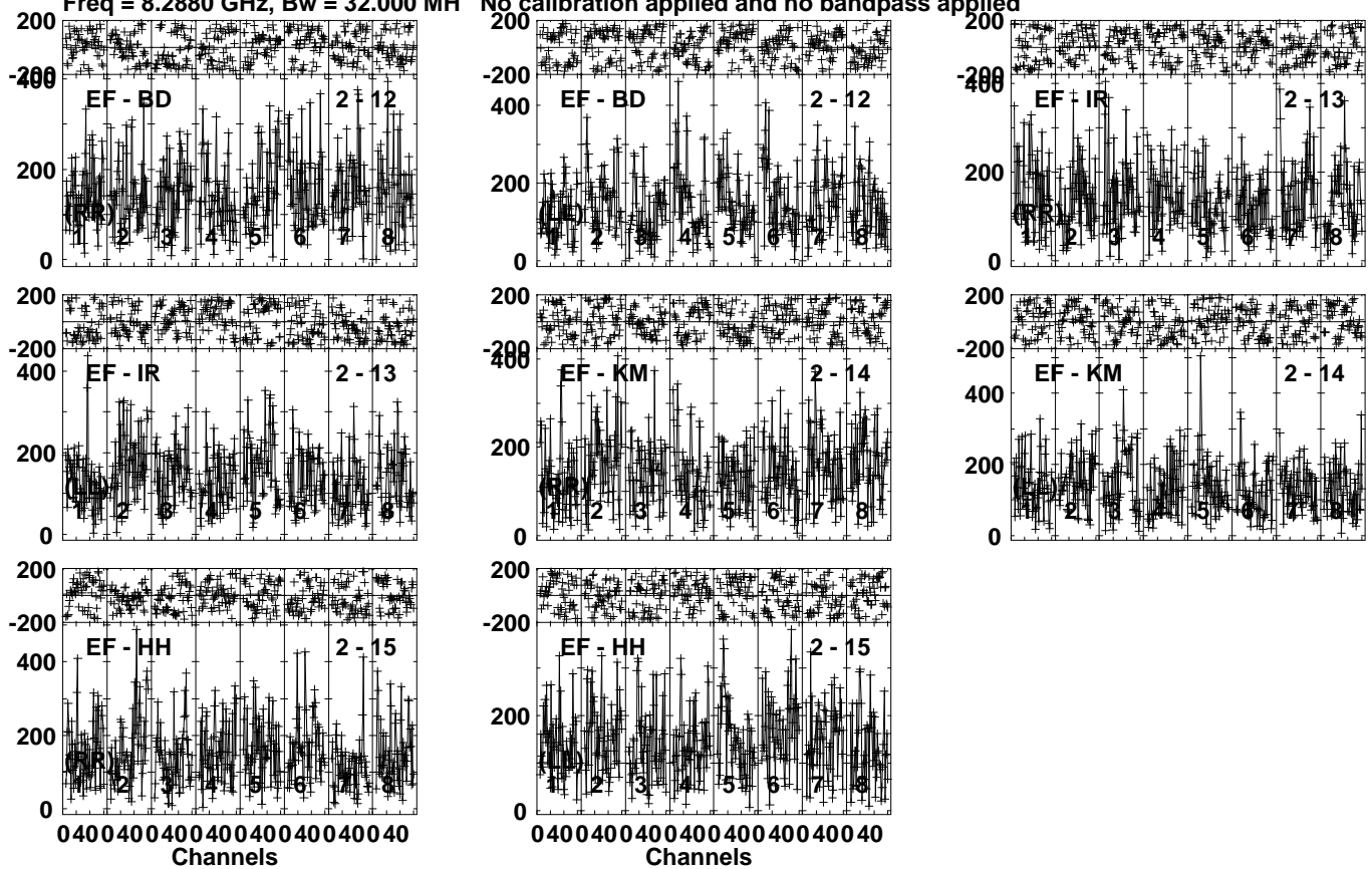
Lower frame: Micro Ampl Jy Top frame: Phas deg Vector averaged cross-power spectrum Several baselines displayed Timerange: 00/15:07:19 to 00/15:09:17
