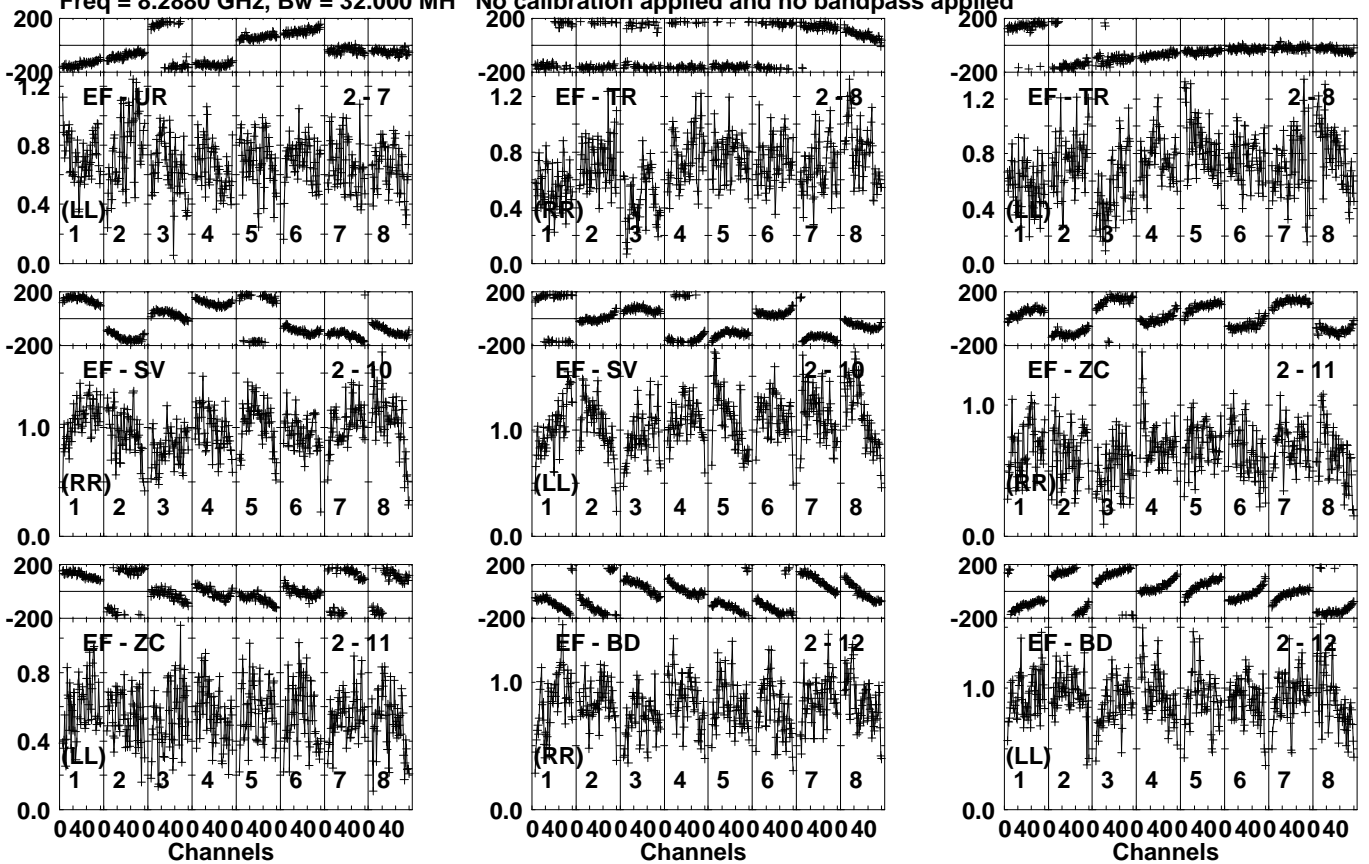
Lower frame: Milli Ampl Jy Top frame: Phas deg Vector averaged cross-power spectrum Several baselines displayed Timerange: 00/11:22:45 to 00/11:24:03
