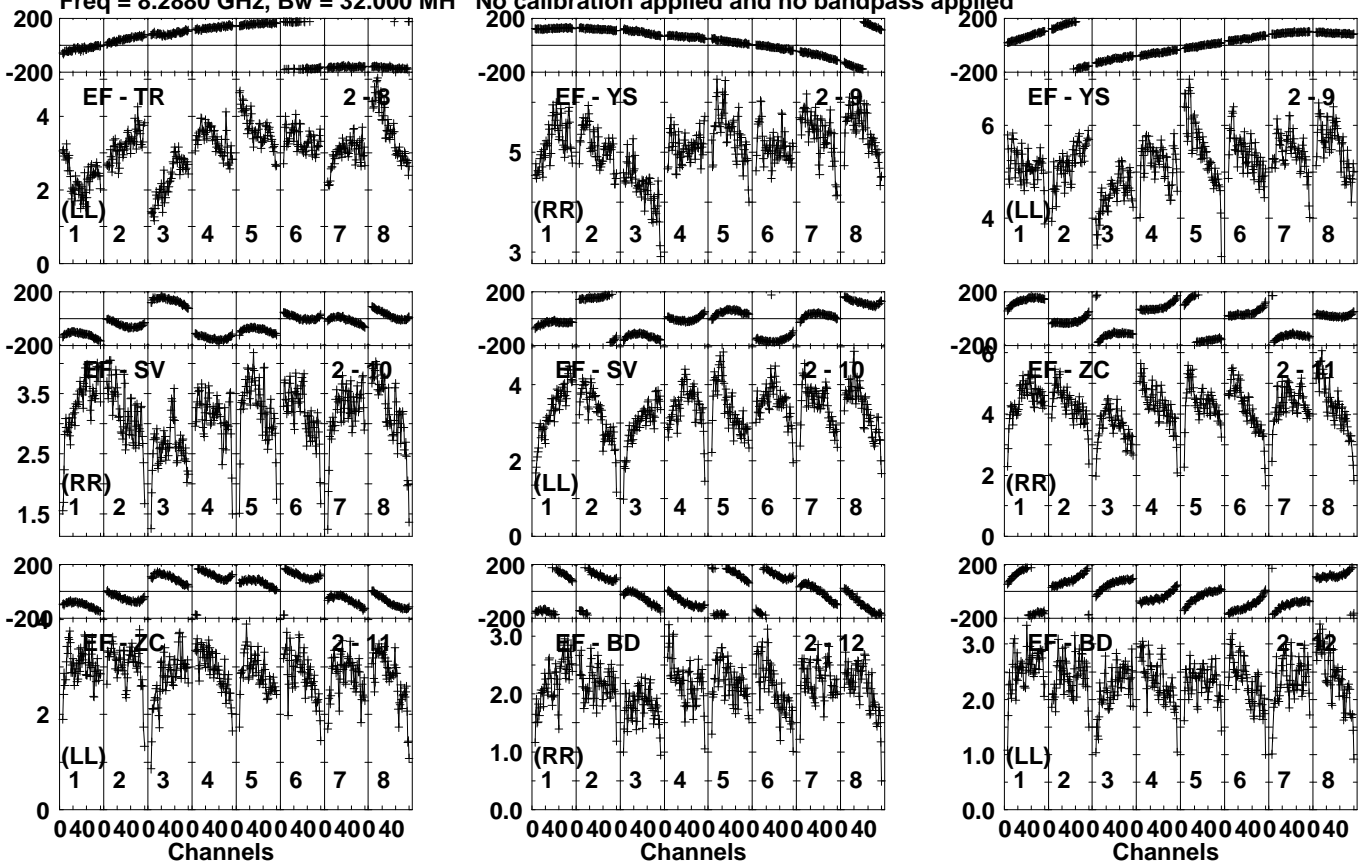
Lower frame: Milli Ampl Jy Top frame: Phas deg Vector averaged cross-power spectrum Several baselines displayed Timerange: 00/20:02:15 to 00/20:03:33
