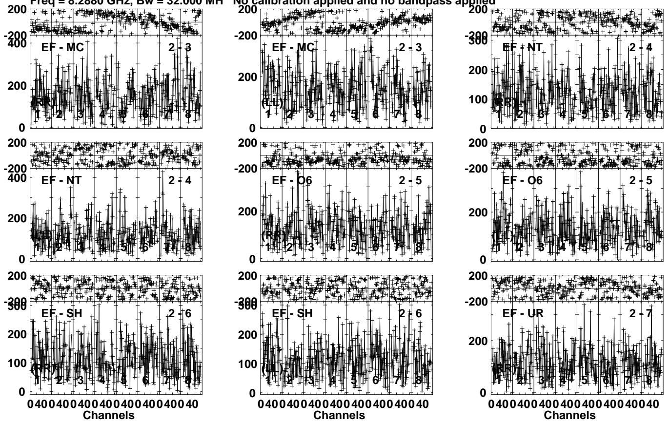
Lower frame: Micro Ampl Jy Top frame: Phas deg Vector averaged cross-power spectrum Several baselines displayed Timerange: 00/14:56:43 to 00/14:58:21
