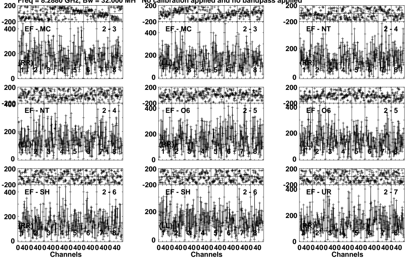
Lower frame: Micro Ampl Jy Top frame: Phas deg Vector averaged cross-power spectrum Several baselines displayed Timerange: 00/13:55:11 to 00/13:57:09
