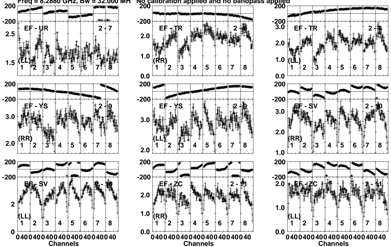
Lower frame: Milli Ampl Jy Top frame: Phas deg Vector averaged cross-power spectrum Several baselines displayed Timerange: 00/12:20:11 to 00/12:21:29
