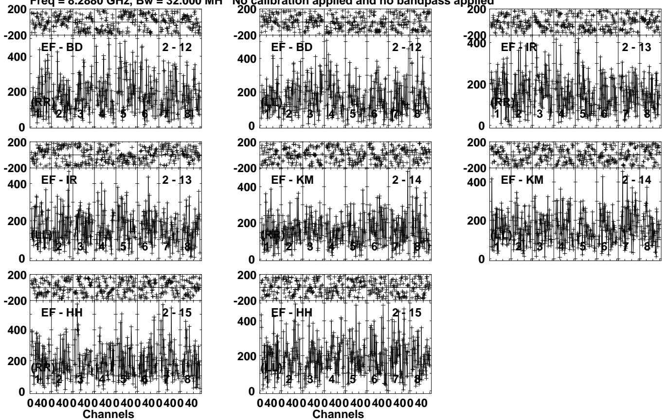
Lower frame: Micro Ampl Jy Top frame: Phas deg Vector averaged cross-power spectrum Several baselines displayed Timerange: 00/17:36:53 to 00/17:38:51
