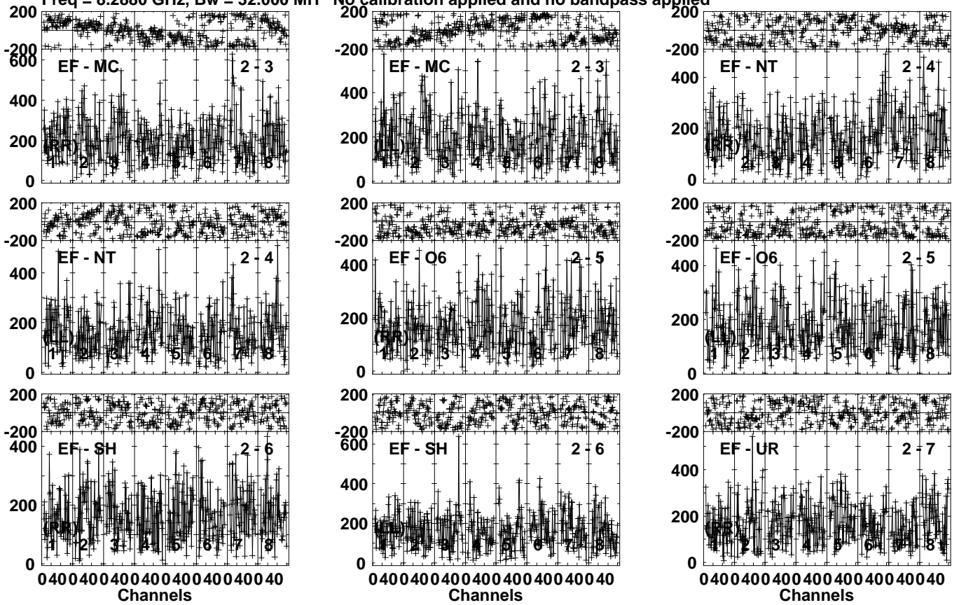
Lower frame: Micro Ampl Jy Top frame: Phas deg Vector averaged cross-power spectrum Several baselines displayed Timerange: 00/17:41:13 to 00/17:43:11
