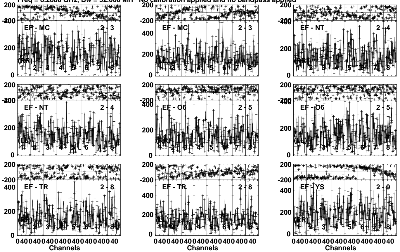
Lower frame: Micro Ampl Jy Top frame: Phas deg Vector averaged cross-power spectrum Several baselines displayed Timerange: 00/23:15:59 to 00/23:17:57
