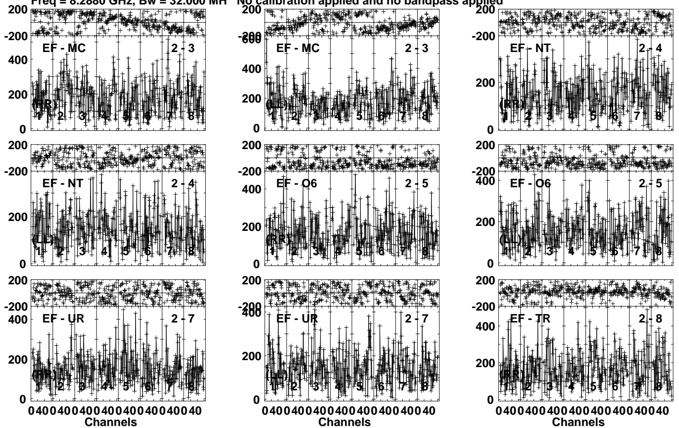
Lower frame: Micro Ampl Jy Top frame: Phas deg Vector averaged cross-power spectrum Several baselines displayed Timerange: 00/20:00:15 to 00/20:02:13
