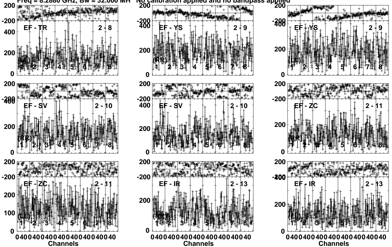
Lower frame: Micro Ampl Jy Top frame: Phas deg Vector averaged cross-power spectrum Several baselines displayed Timerange: 00/20:58:57 to 00/21:00:35
