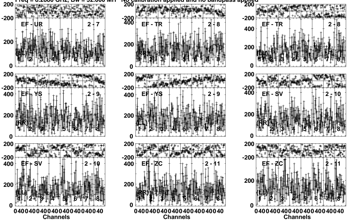
Lower frame: Micro Ampl Jy Top frame: Phas deg Vector averaged cross-power spectrum Several baselines displayed Timerange: 00/13:22:27 to 00/13:24:25
