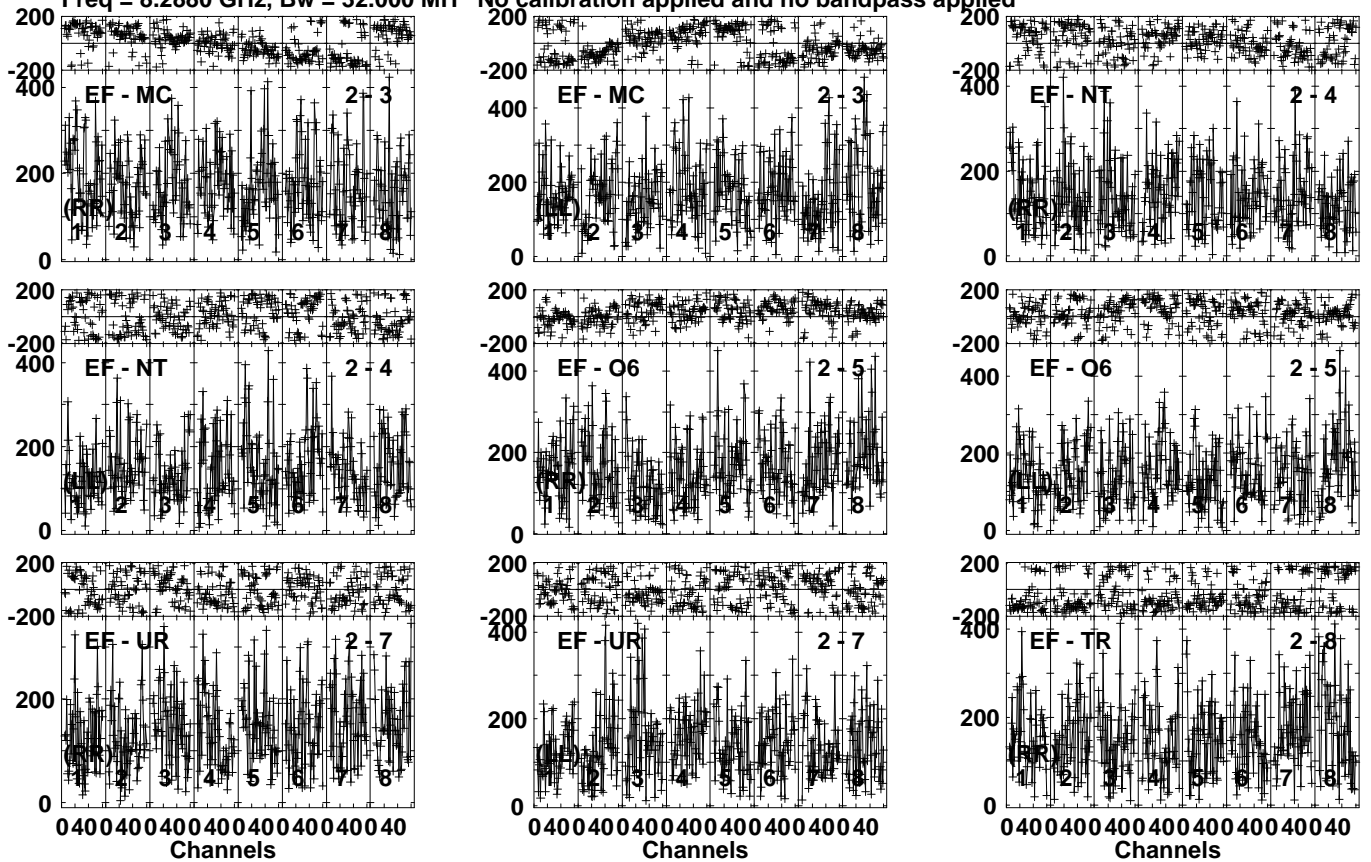
Lower frame: Micro Ampl Jy Top frame: Phas deg Vector averaged cross-power spectrum Several baselines displayed Timerange: 00/20:33:19 to 00/20:35:17
