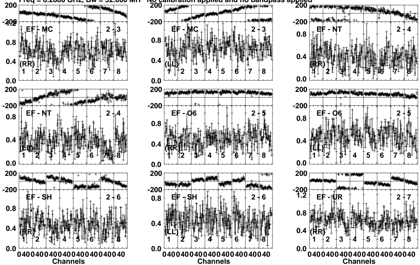
Lower frame: Milli Ampl Jy Top frame: Phas deg Vector averaged cross-power spectrum Several baselines displayed Timerange: 00/11:11:49 to 00/11:13:07
