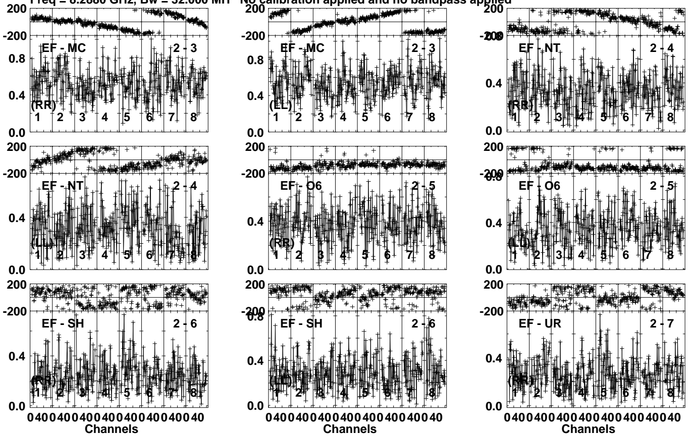
Lower frame: Milli Ampl Jy Top frame: Phas deg Vector averaged cross-power spectrum Several baselines displayed Timerange: 00/15:41:13 to 00/15:42:41
