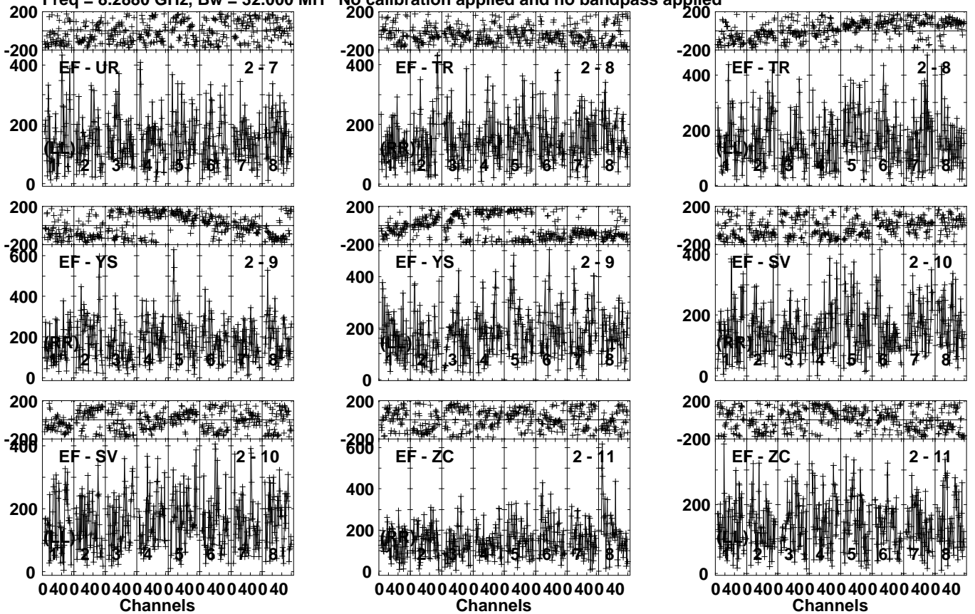
Lower frame: Micro Ampl Jy Top frame: Phas deg Vector averaged cross-power spectrum Several baselines displayed Timerange: 00/14:23:39 to 00/14:25:37
