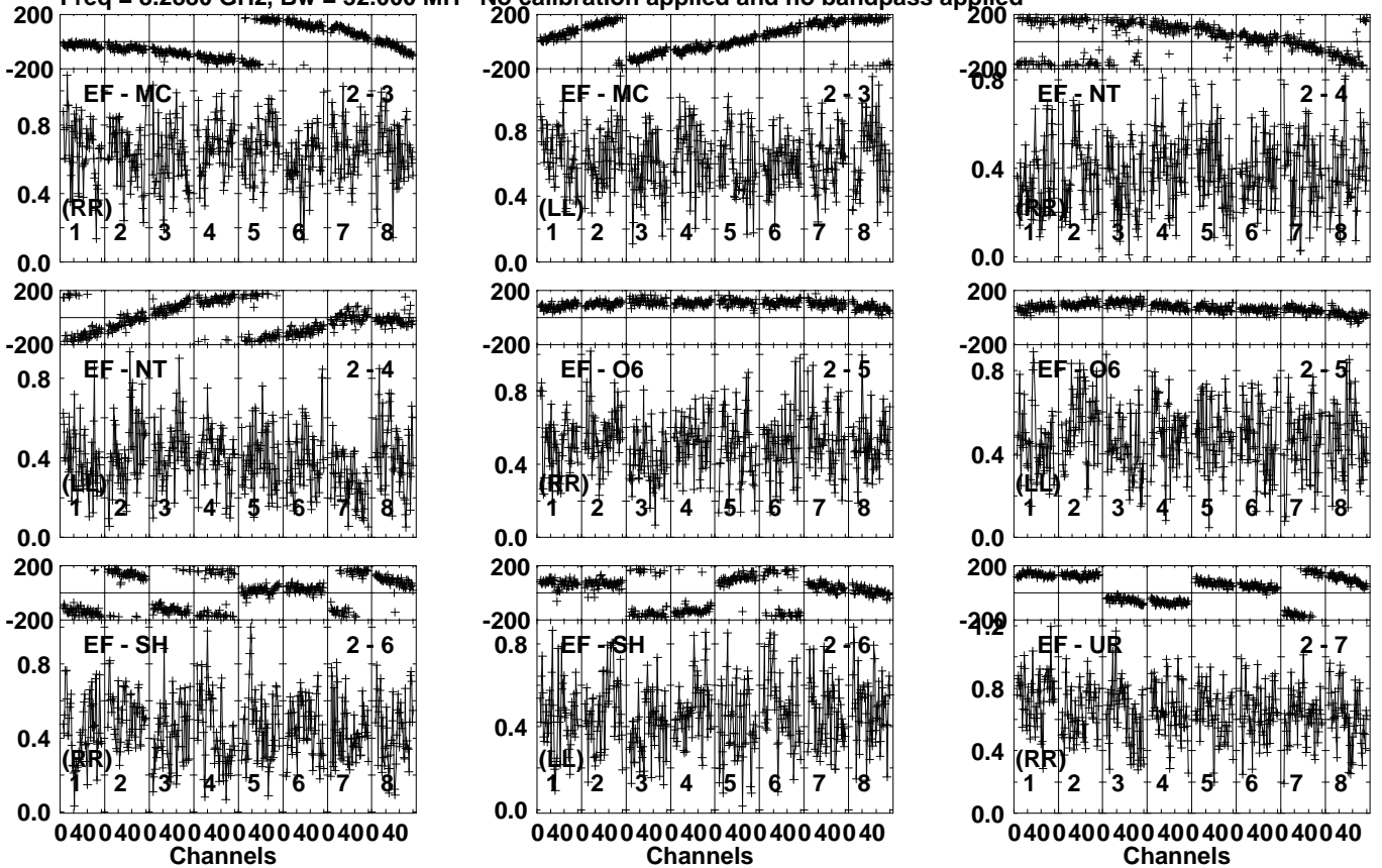
Lower frame: Milli Ampl Jy Top frame: Phas deg Vector averaged cross-power spectrum Several baselines displayed Timerange: 00/11:15:09 to 00/11:16:27
