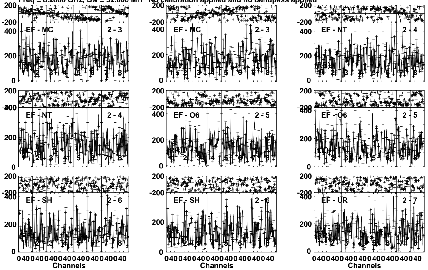
Lower frame: Micro Ampl Jy Top frame: Phas deg Vector averaged cross-power spectrum Several baselines displayed Timerange: 00/17:48:53 to 00/17:50:31
