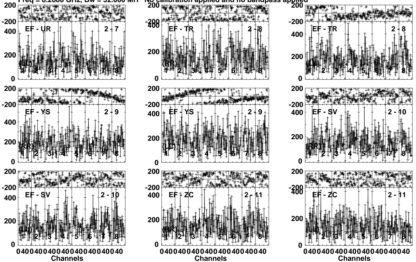
Lower frame: Micro Ampl Jy Top frame: Phas deg Vector averaged cross-power spectrum Several baselines displayed Timerange: 00/15:17:45 to 00/15:19:43
