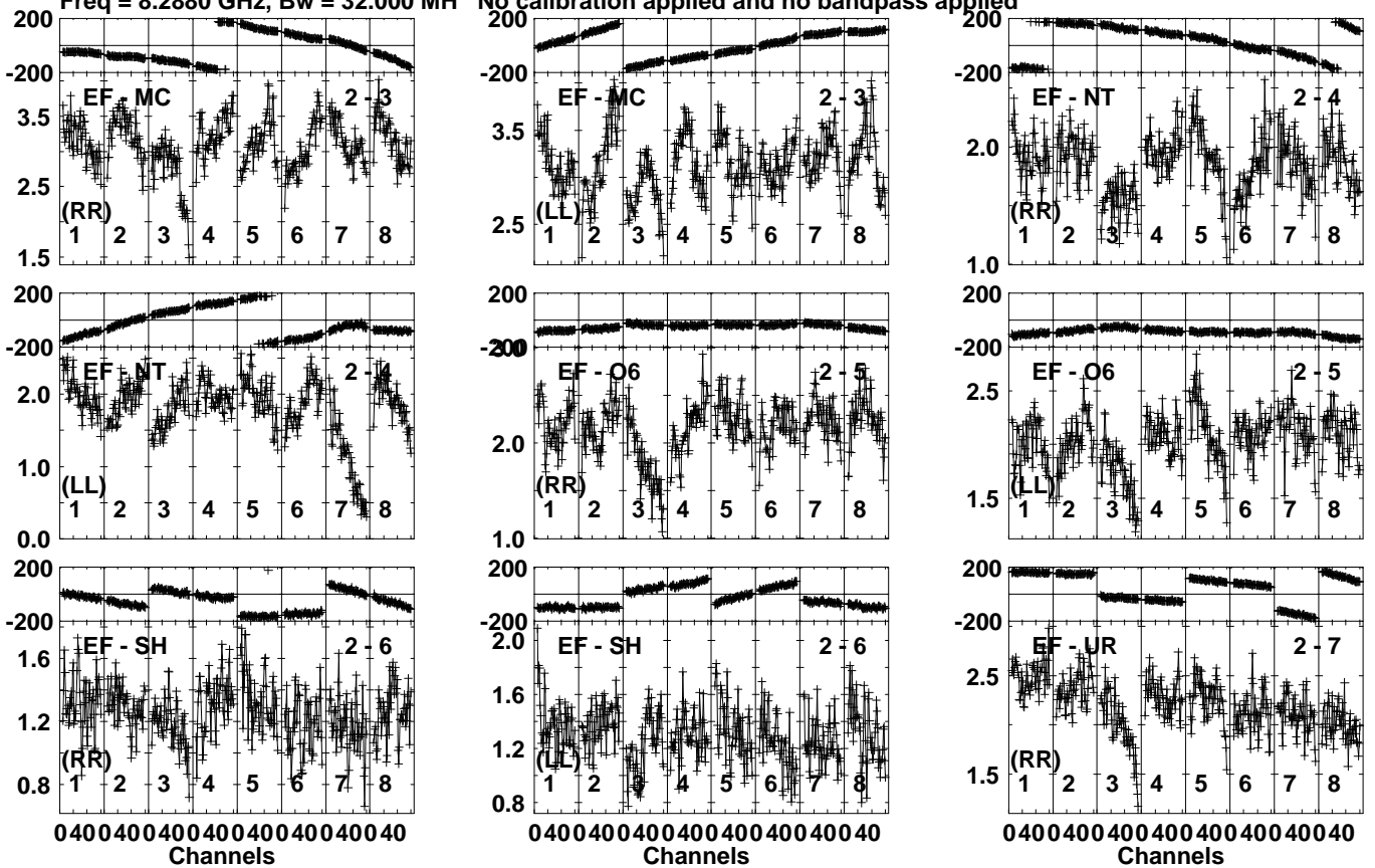
Lower frame: Milli Ampl Jy Top frame: Phas deg Vector averaged cross-power spectrum Several baselines displayed Timerange: 00/13:42:29 to 00/13:43:47
