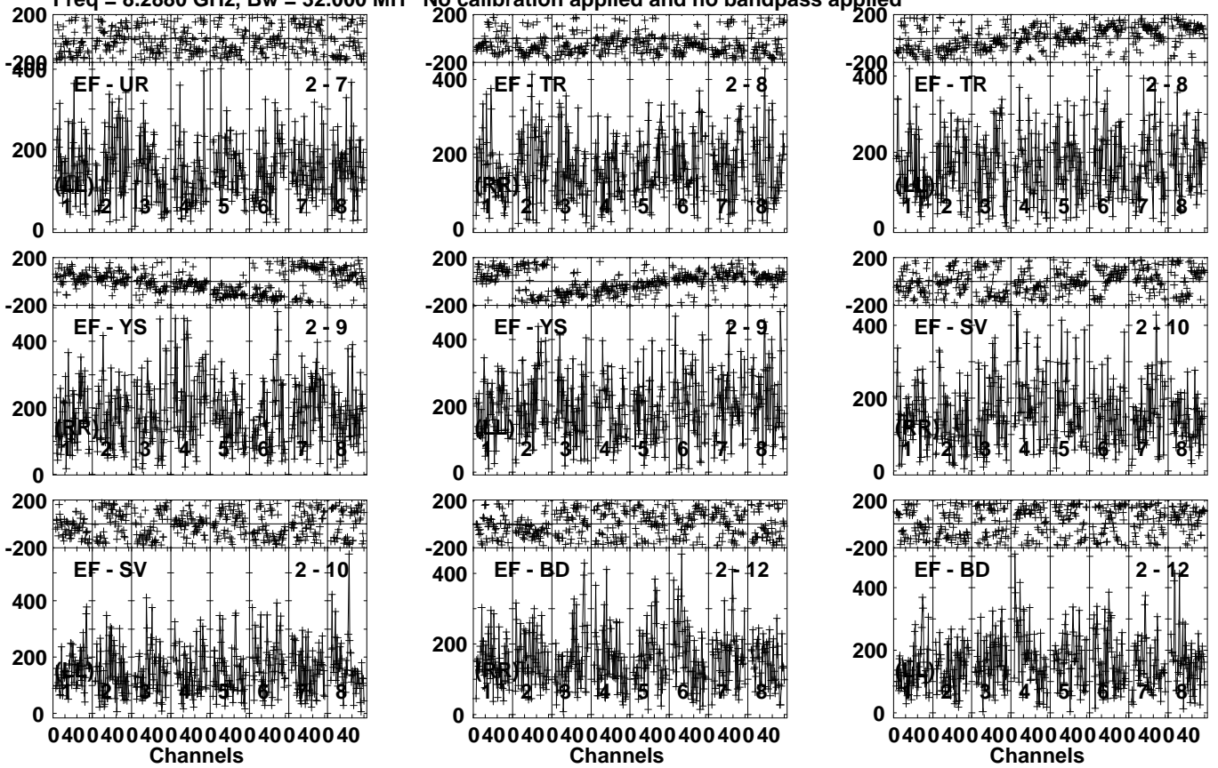
Lower frame: Micro Ampl Jy Top frame: Phas deg Vector averaged cross-power spectrum Several baselines displayed Timerange: 00/16:39:33 to 00/16:41:31
