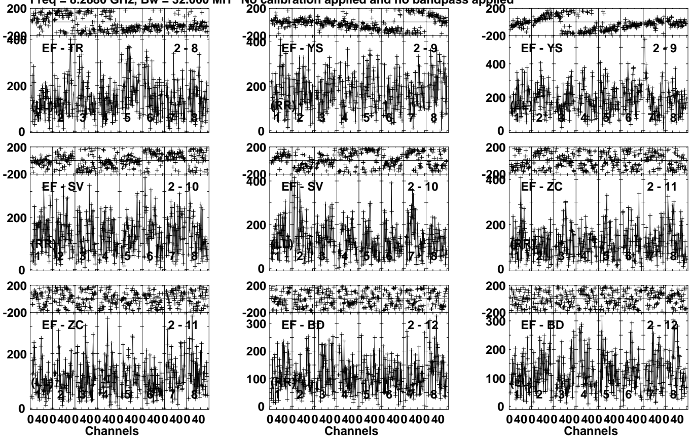
Lower frame: Micro Ampl Jy Top frame: Phas deg Vector averaged cross-power spectrum Several baselines displayed Timerange: 00/20:04:21 to 00/20:05:59
