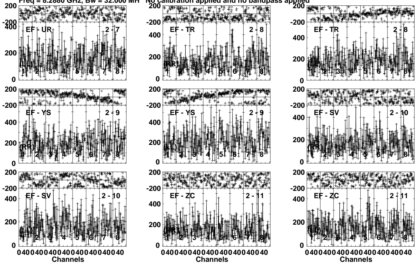
Lower frame: Micro Ampl Jy Top frame: Phas deg Vector averaged cross-power spectrum Several baselines displayed Timerange: 00/17:08:33 to 00/17:10:31
