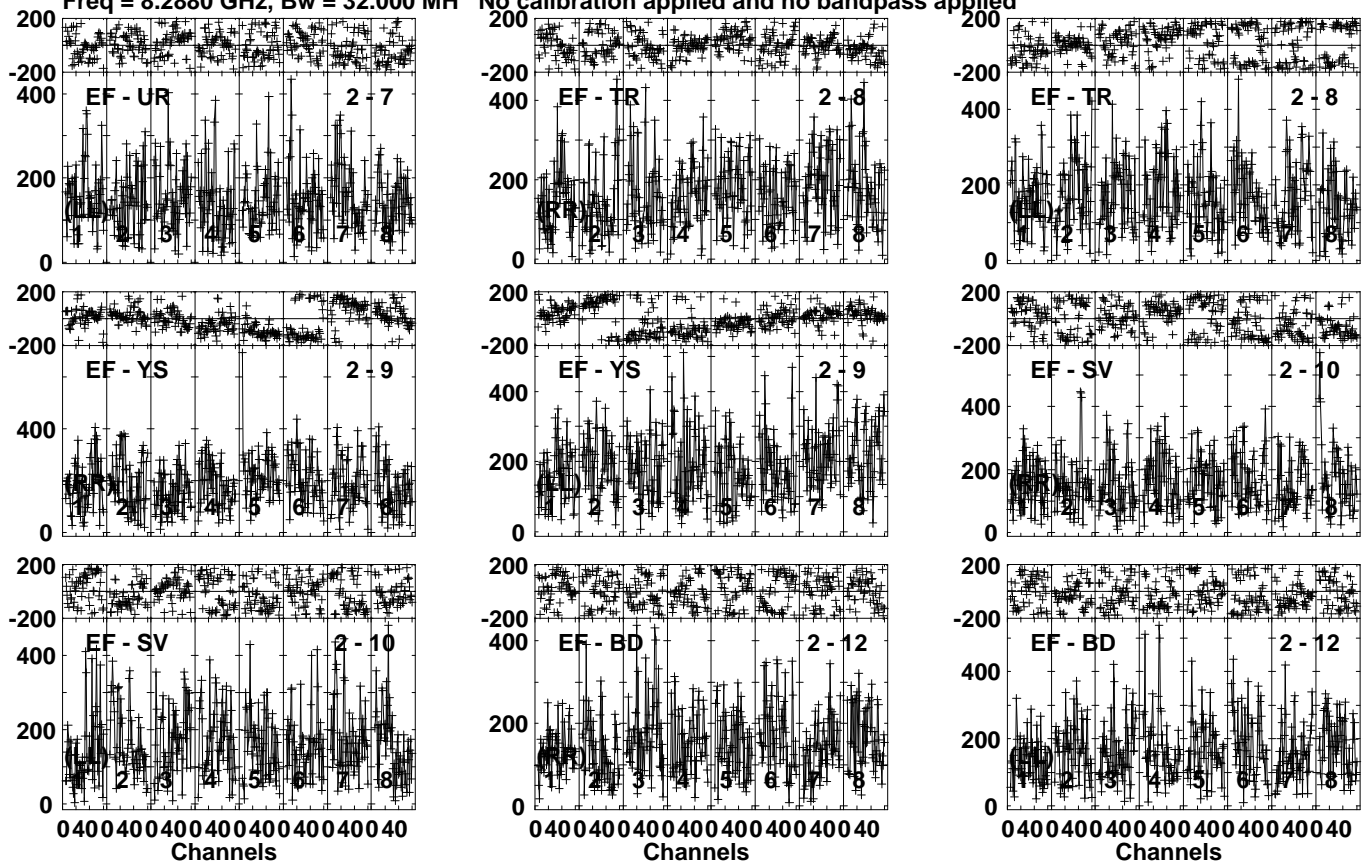
Lower frame: Micro Ampl Jy Top frame: Phas deg Vector averaged cross-power spectrum Several baselines displayed Timerange: 00/16:32:33 to 00/16:34:31
