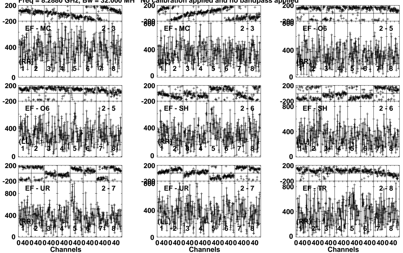
Lower frame: Micro Ampl Jy Top frame: Phas deg Vector averaged cross-power spectrum Several baselines displayed Timerange: 00/10:53:47 to 00/10:55:05
