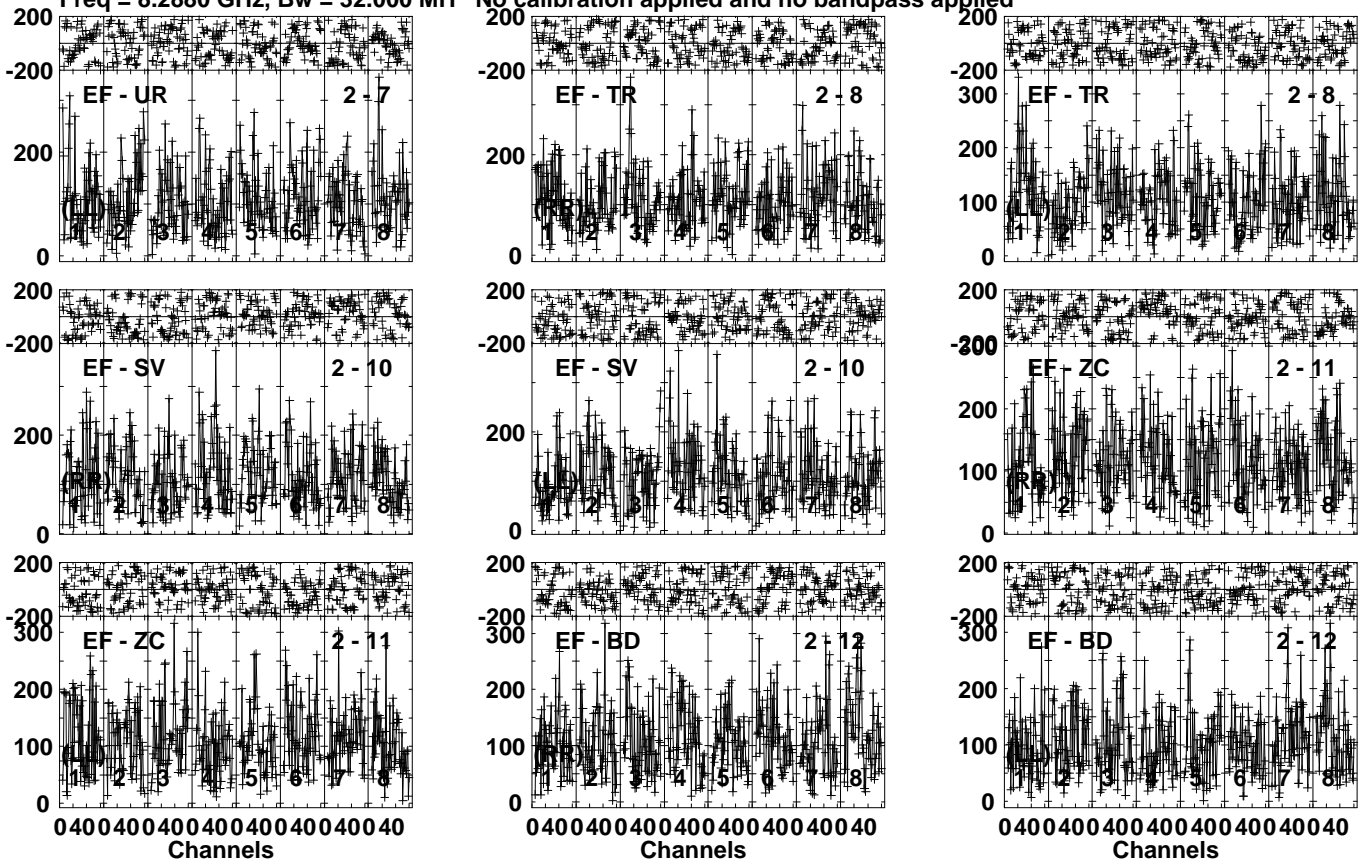
Lower frame: Micro Ampl Jy Top frame: Phas deg Vector averaged cross-power spectrum Several baselines displayed Timerange: 00/11:10:09 to 00/11:11:47
