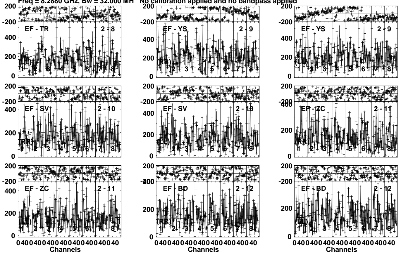
Lower frame: Micro Ampl Jy Top frame: Phas deg Vector averaged cross-power spectrum Several baselines displayed Timerange: 00/19:42:03 to 00/19:44:01
