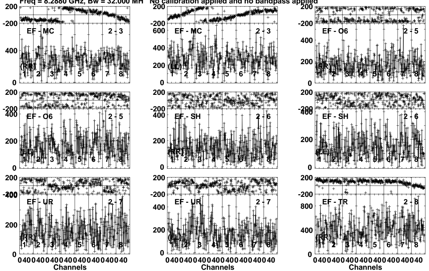
Lower frame: Micro Ampl Jy Top frame: Phas deg Vector averaged cross-power spectrum Several baselines displayed Timerange: 00/10:46:41 to 00/10:47:59
