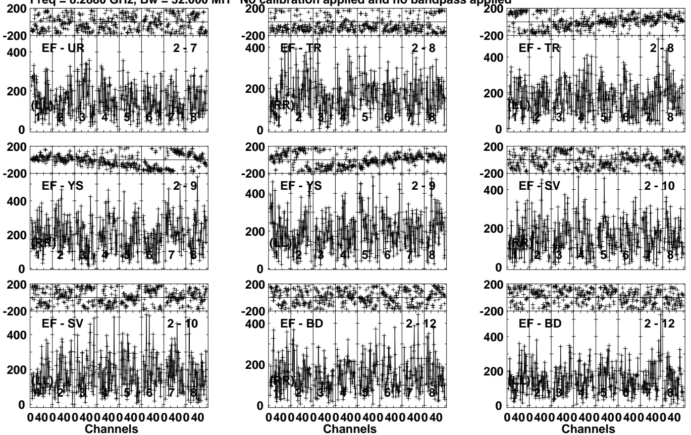
Lower frame: Micro Ampl Jy Top frame: Phas deg Vector averaged cross-power spectrum Several baselines displayed Timerange: 00/16:42:53 to 00/16:44:51
