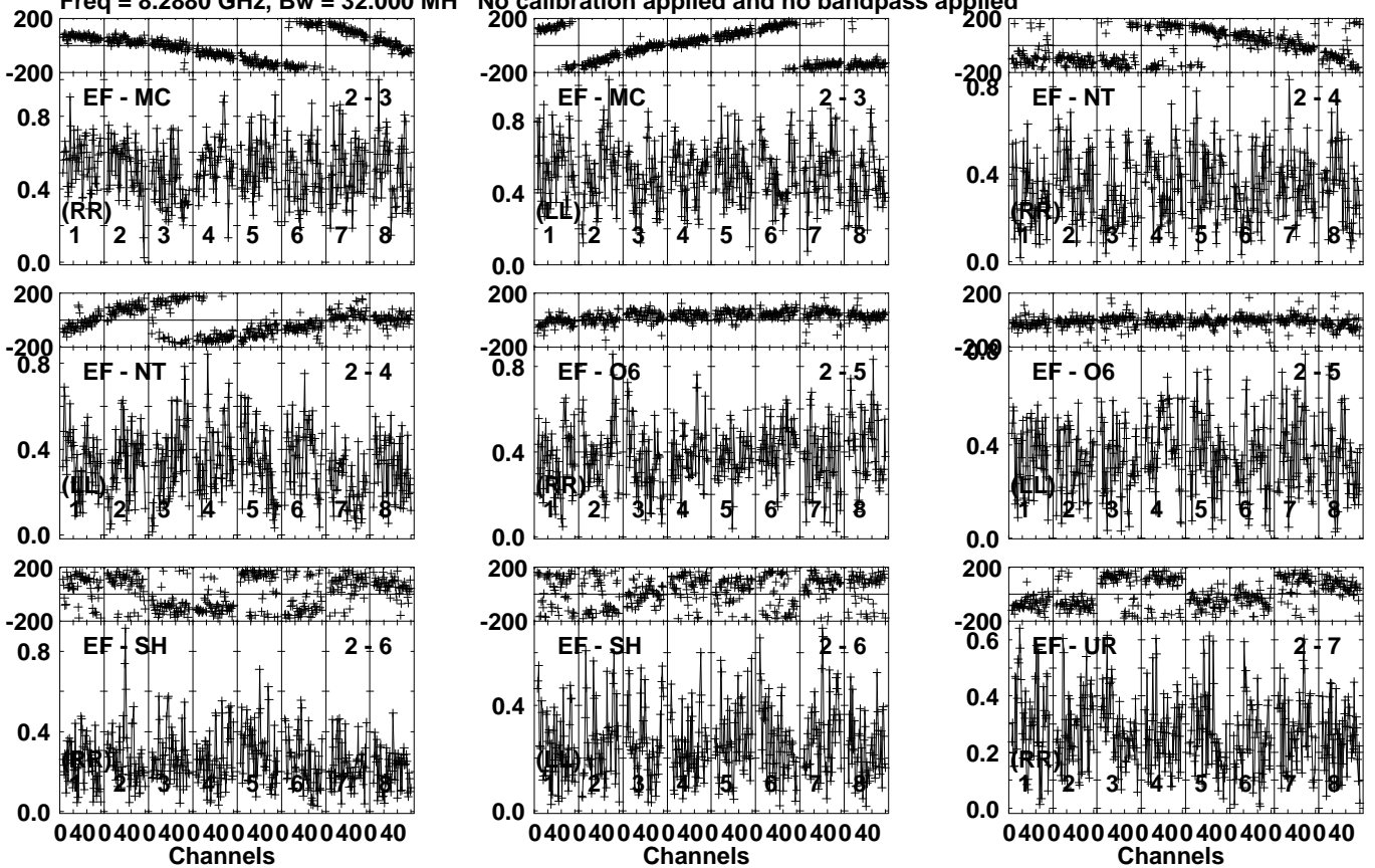
Lower frame: Milli Ampl Jy Top frame: Phas deg Vector averaged cross-power spectrum Several baselines displayed Timerange: 00/15:44:13 to 00/15:45:41
