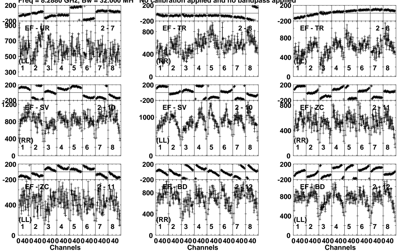
Lower frame: Micro Ampl Jy Top frame: Phas deg Vector averaged cross-power spectrum Several baselines displayed Timerange: 00/11:19:15 to 00/11:20:43
