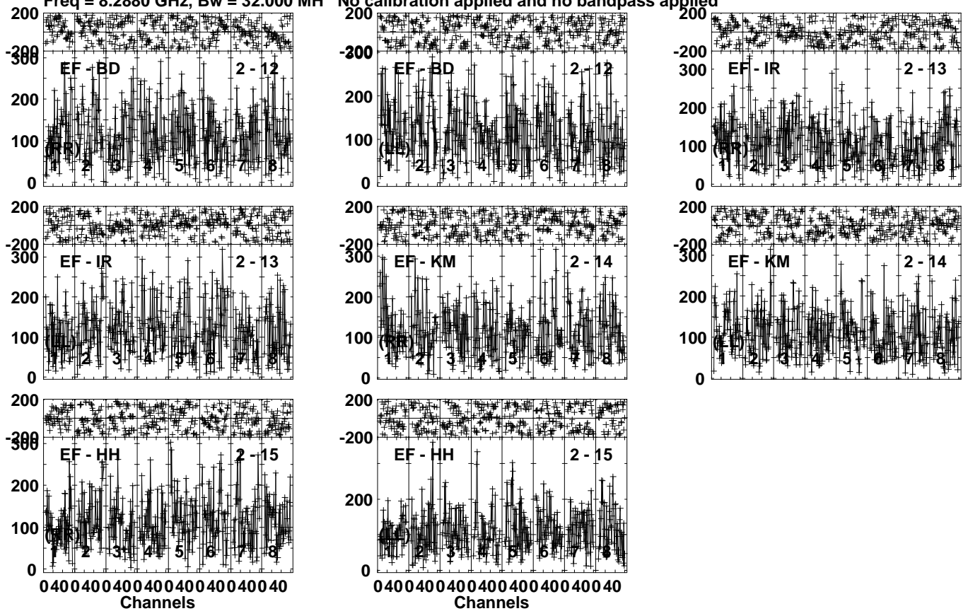
Lower frame: Micro Ampl Jy Top frame: Phas deg Vector averaged cross-power spectrum Several baselines displayed Timerange: 00/13:44:35 to 00/13:46:13
