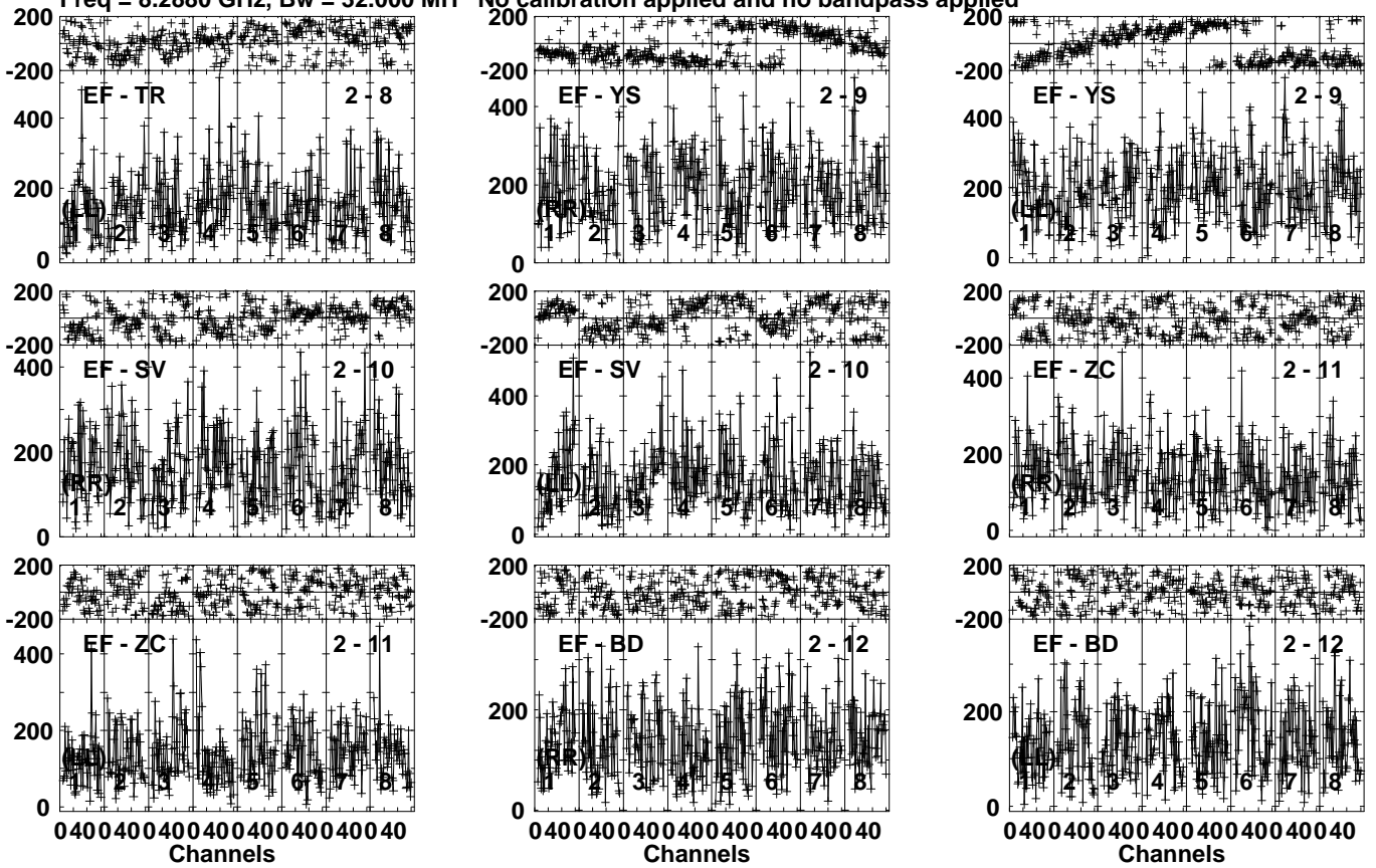
Lower frame: Micro Ampl Jy Top frame: Phas deg Vector averaged cross-power spectrum Several baselines displayed Timerange: 00/20:47:05 to 00/20:49:03
