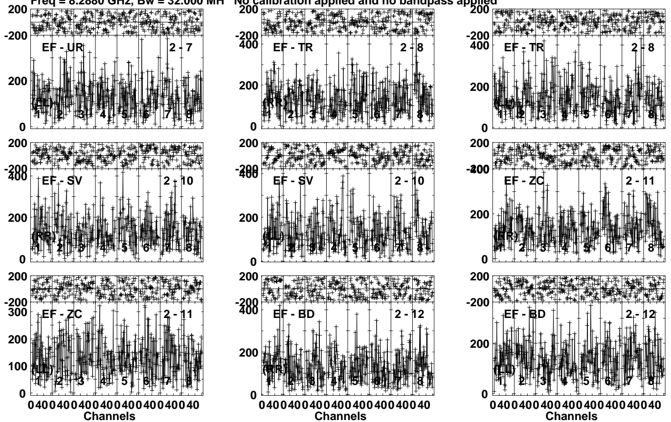
Lower frame: Micro Ampl Jy Top frame: Phas deg Vector averaged cross-power spectrum Several baselines displayed Timerange: 00/11:31:11 to 00/11:33:09
