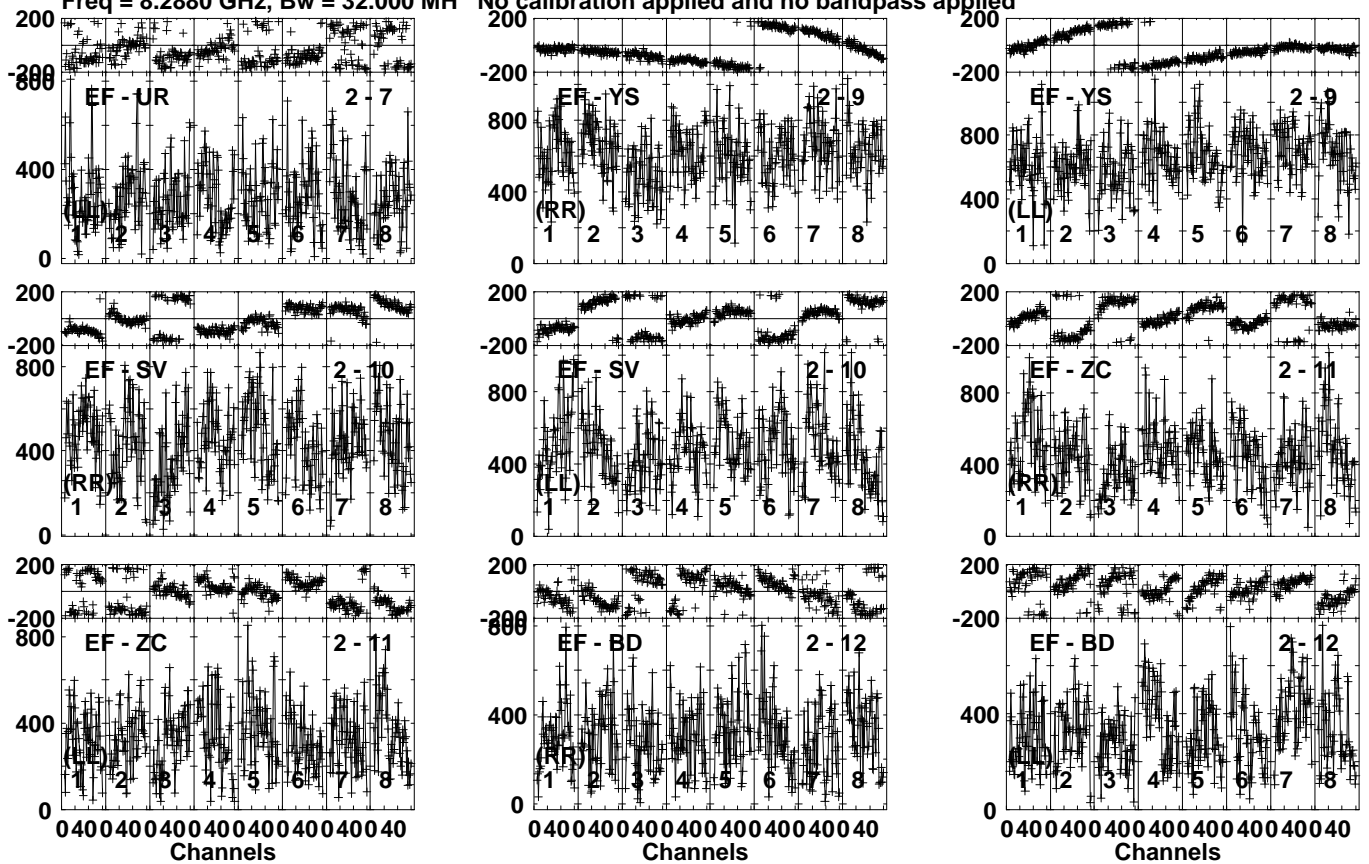
Lower frame: Micro Ampl Jy Top frame: Phas deg Vector averaged cross-power spectrum Several baselines displayed Timerange: 00/15:38:13 to 00/15:39:41
