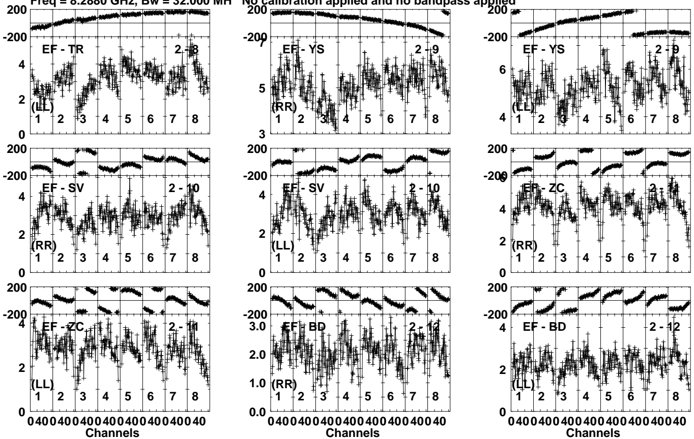
Lower frame: Milli Ampl Jy Top frame: Phas deg Vector averaged cross-power spectrum Several baselines displayed Timerange: 00/19:40:43 to 00/19:42:01
