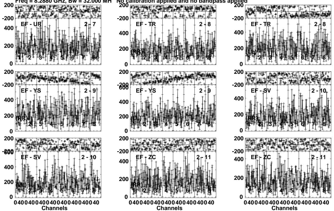
Lower frame: Micro Ampl Jy Top frame: Phas deg Vector averaged cross-power spectrum Several baselines displayed Timerange: 00/18:03:23 to 00/18:05:21
