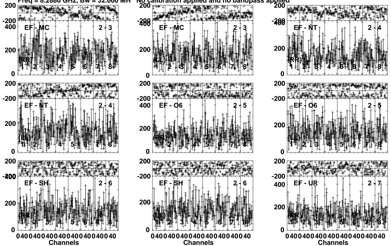
Lower frame: Micro Ampl Jy Top frame: Phas deg Vector averaged cross-power spectrum Several baselines displayed Timerange: 00/14:45:01 to 00/14:46:59
