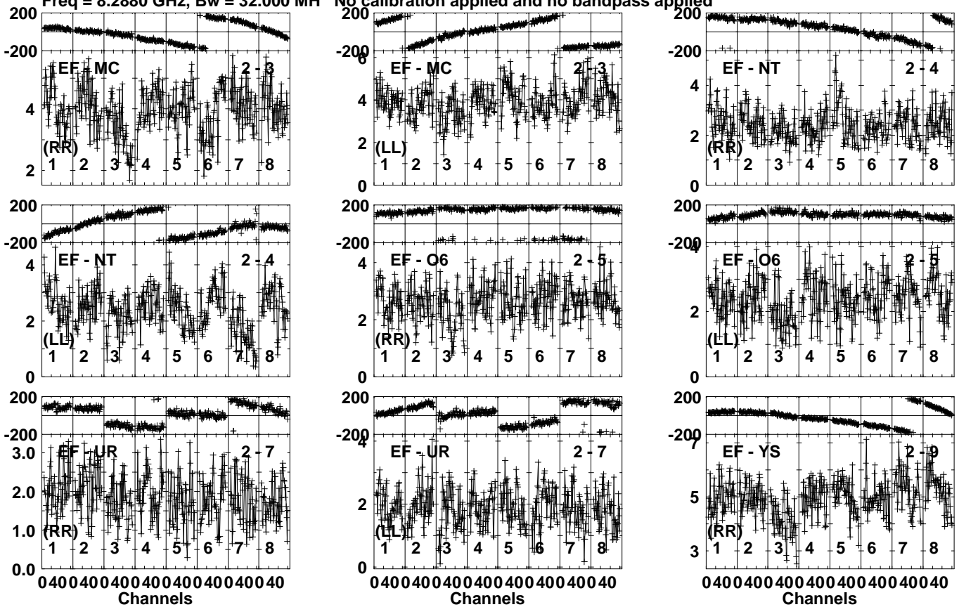
Lower frame: Milli Ampl Jy Top frame: Phas deg Vector averaged cross-power spectrum Several baselines displayed Timerange: 00/17:32:13 to 00/17:33:31
