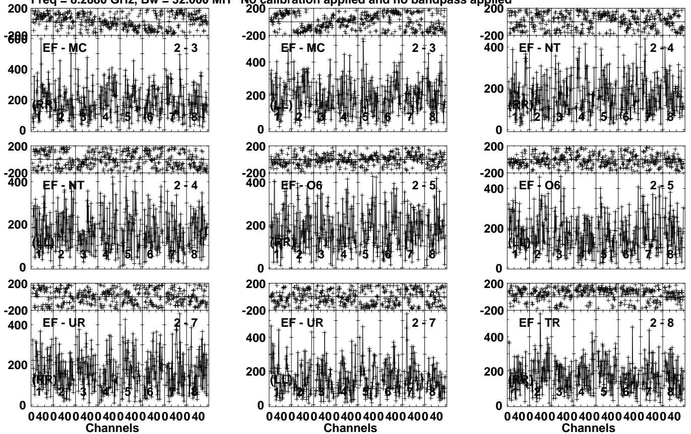
Lower frame: Micro Ampl Jy Top frame: Phas deg Vector averaged cross-power spectrum Several baselines displayed Timerange: 00/19:30:57 to 00/19:32:55
