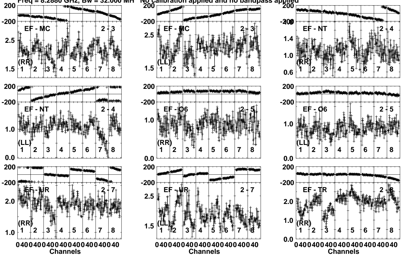
Lower frame: Milli Ampl Jy Top frame: Phas deg Vector averaged cross-power spectrum Several baselines displayed Timerange: 00/12:23:57 to 00/12:25:15
