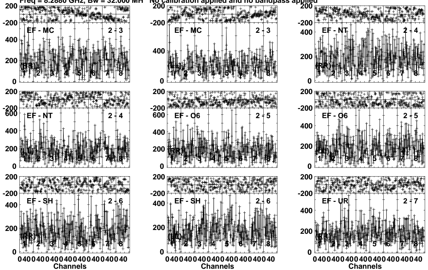
Lower frame: Micro Ampl Jy Top frame: Phas deg Vector averaged cross-power spectrum Several baselines displayed Timerange: 00/17:59:53 to 00/18:01:51
