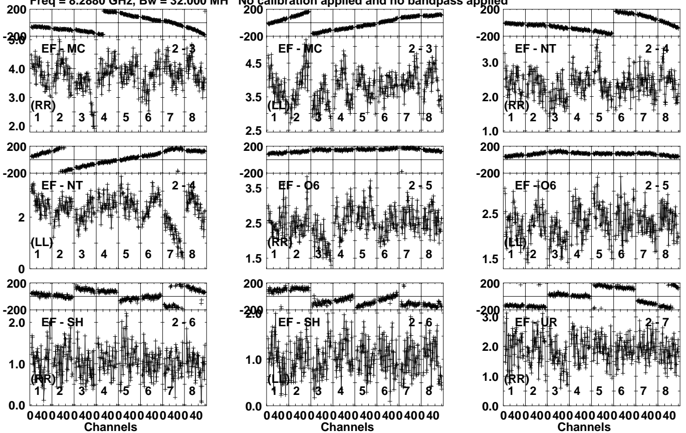
Lower frame: Milli Ampl Jy Top frame: Phas deg Vector averaged cross-power spectrum Several baselines displayed Timerange: 00/16:59:33 to 00/17:00:51
