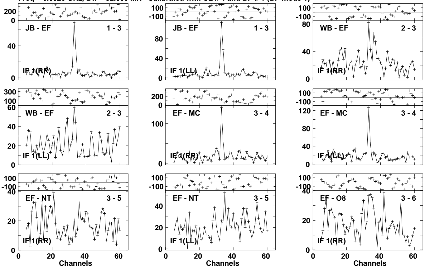
Lower frame: Milli Ampl Jy Top frame: Phas deg Vector averaged cross-power spectrum Several baselines displayed Timerange: 01/01:32:47 to 01/01:35:07
