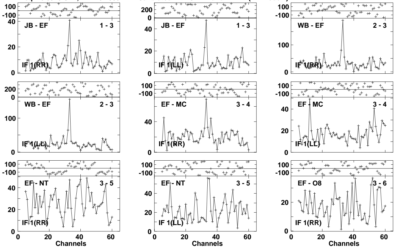
Lower frame: Milli Ampl Jy Top frame: Phas deg Vector averaged cross-power spectrum Several baselines displayed Timerange: 01/00:52:57 to 01/00:55:17
