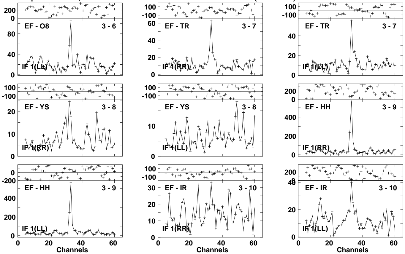
Lower frame: Milli Ampl Jy Top frame: Phas deg Vector averaged cross-power spectrum Several baselines displayed Timerange: 01/04:25:59 to 01/04:28:19
