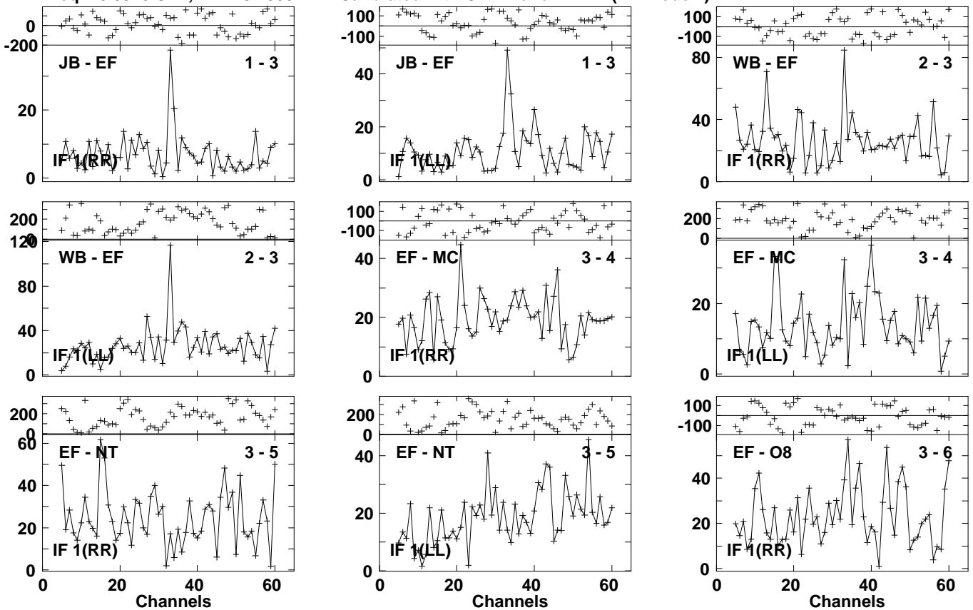
Lower frame: Milli Ampl Jy Top frame: Phas deg Vector averaged cross-power spectrum Several baselines displayed Timerange: 01/05:41:47 to 01/05:44:07
