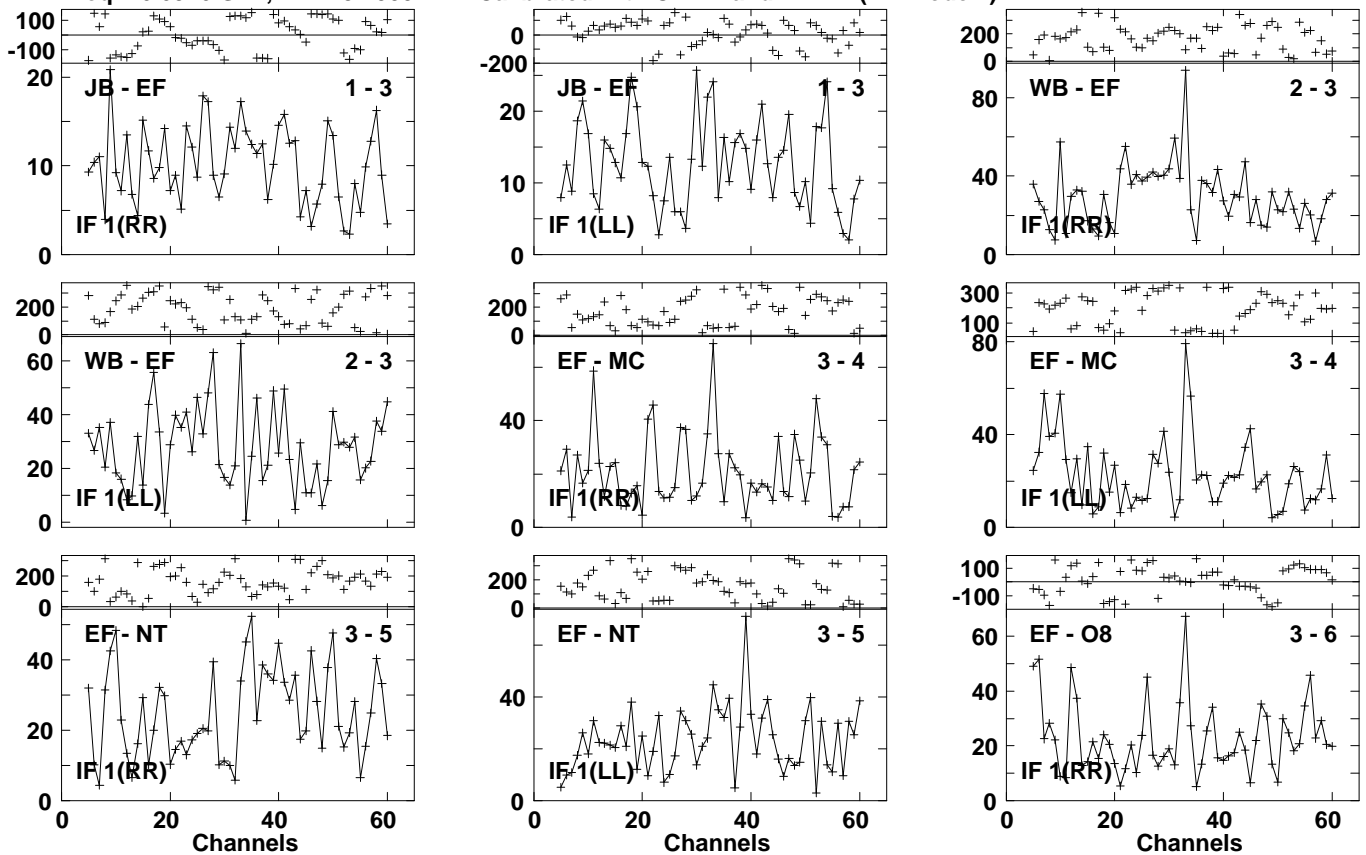
Lower frame: Milli Ampl Jy Top frame: Phas deg Vector averaged cross-power spectrum Several baselines displayed Timerange: 00/23:18:39 to 00/23:20:59
