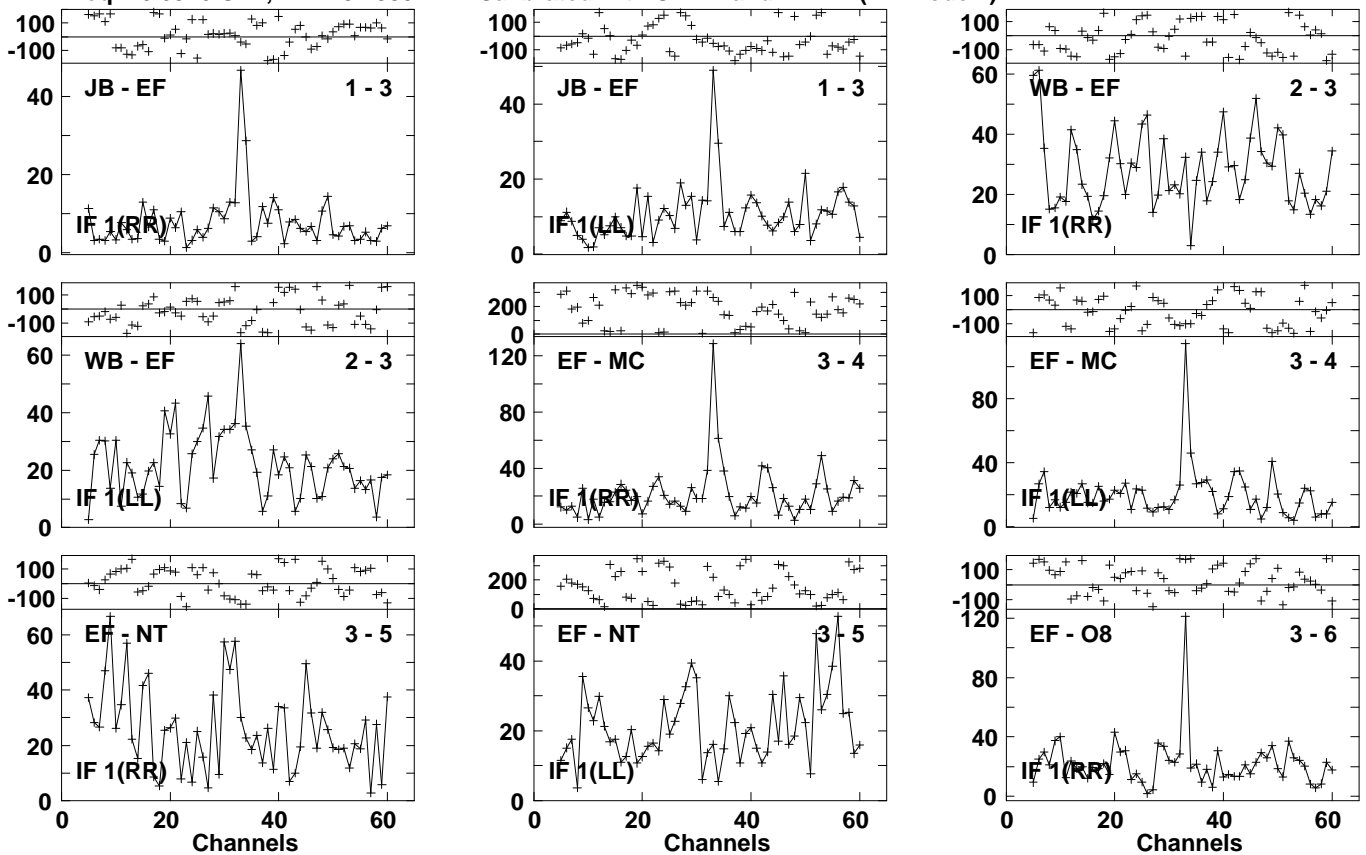
Lower frame: Milli Ampl Jy Top frame: Phas deg Vector averaged cross-power spectrum Several baselines displayed Timerange: 01/06:04:39 to 01/06:06:59
