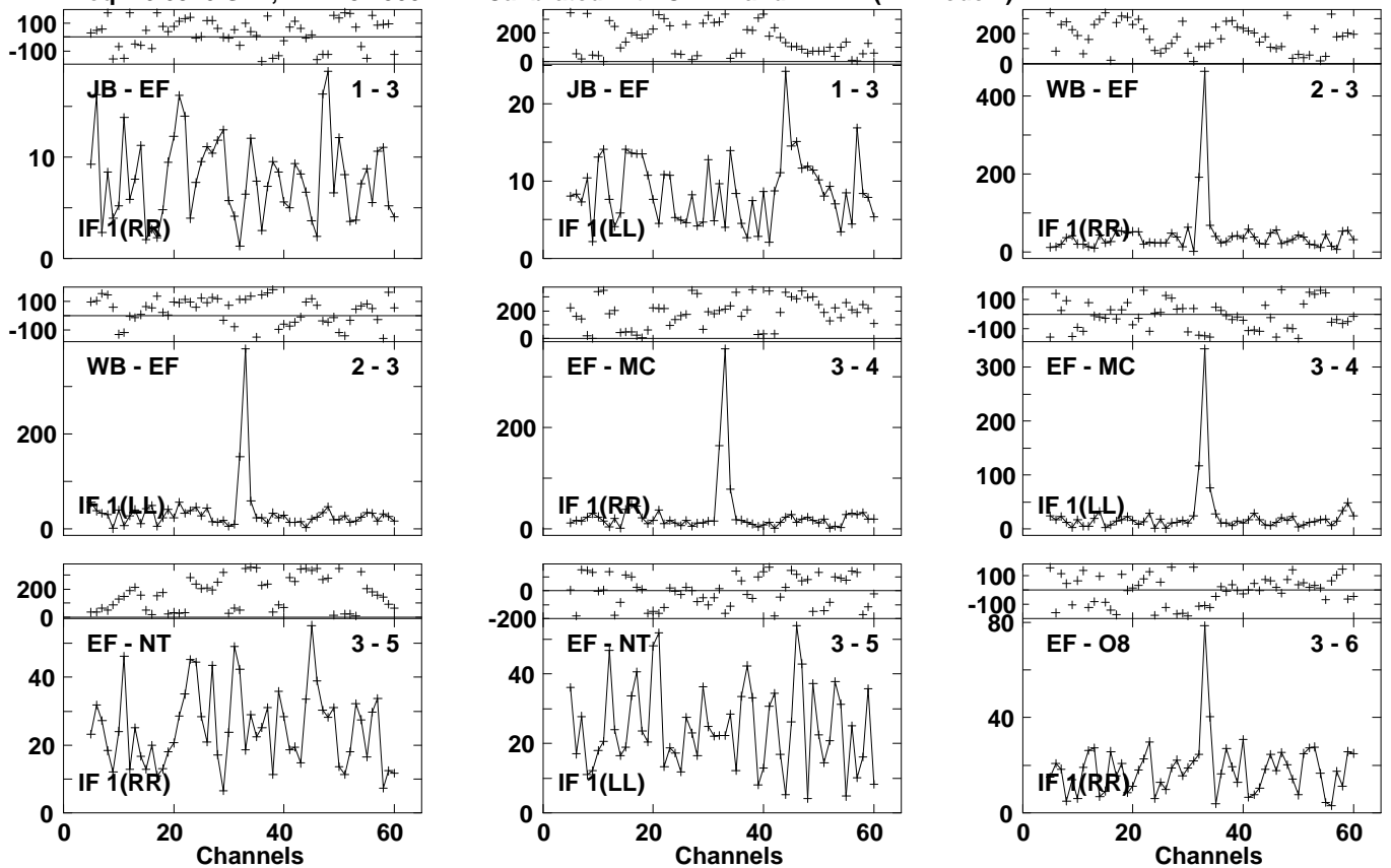
Lower frame: Milli Ampl Jy Top frame: Phas deg Vector averaged cross-power spectrum Several baselines displayed Timerange: 01/04:37:25 to 01/04:39:45
