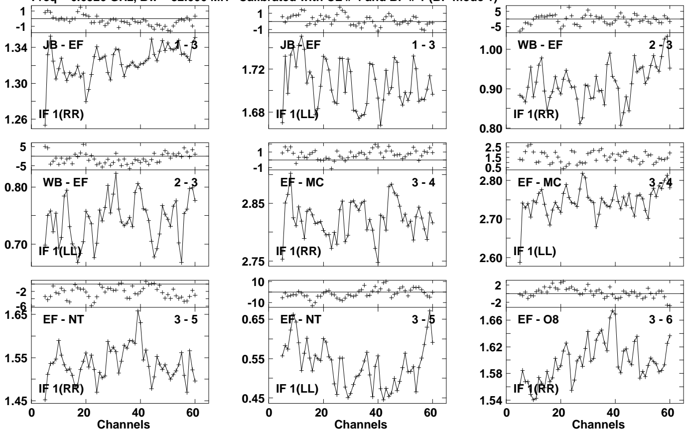
Lower frame: Ampl Jy Top frame: Phas deg Vector averaged cross-power spectrum Several baselines displayed Timerange: 01/05:19:23 to 01/05:19:51
