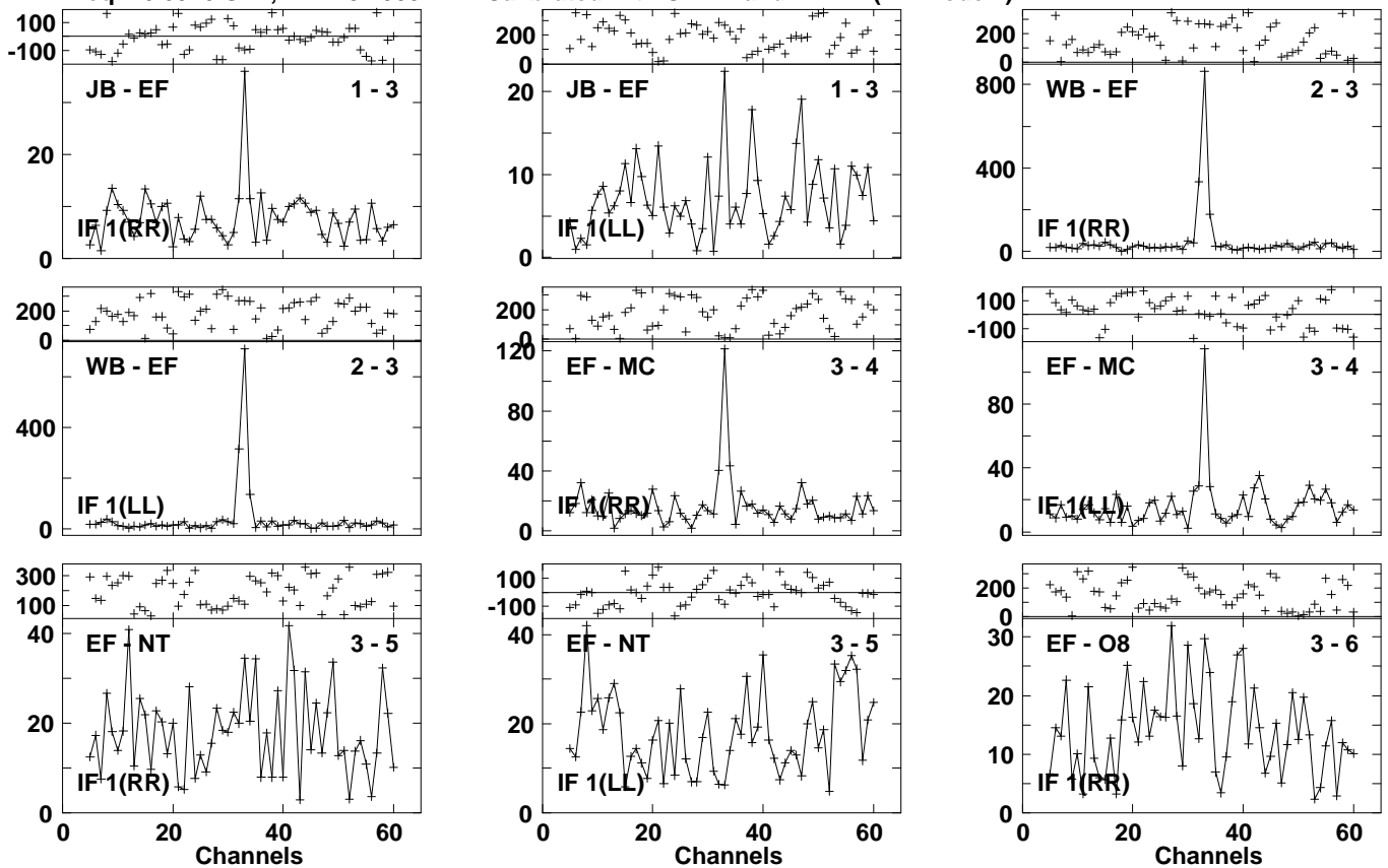
Lower frame: Milli Ampl Jy Top frame: Phas deg Vector averaged cross-power spectrum Several baselines displayed Timerange: 01/04:33:03 to 01/04:35:23
