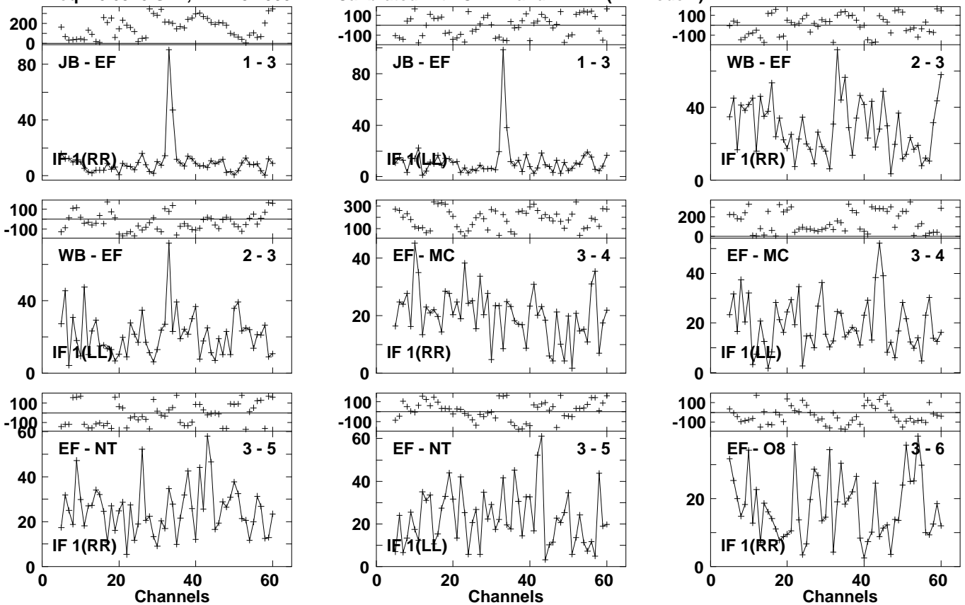
Lower frame: Milli Ampl Jy Top frame: Phas deg Vector averaged cross-power spectrum Several baselines displayed Timerange: 01/03:25:59 to 01/03:28:19
