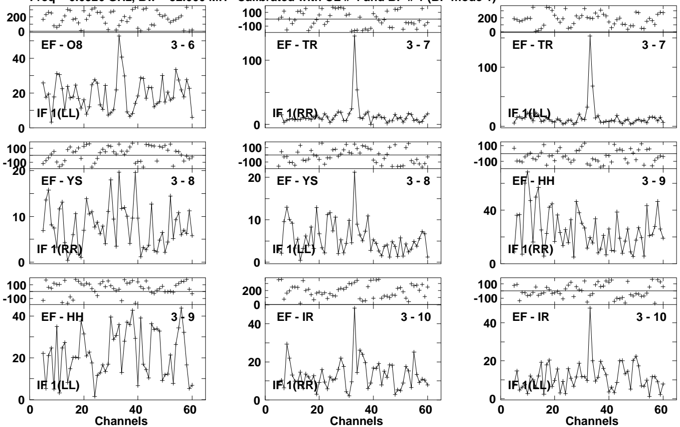
Lower frame: Milli Ampl Jy Top frame: Phas deg Vector averaged cross-power spectrum Several baselines displayed Timerange: 01/01:09:47 to 01/01:12:15
