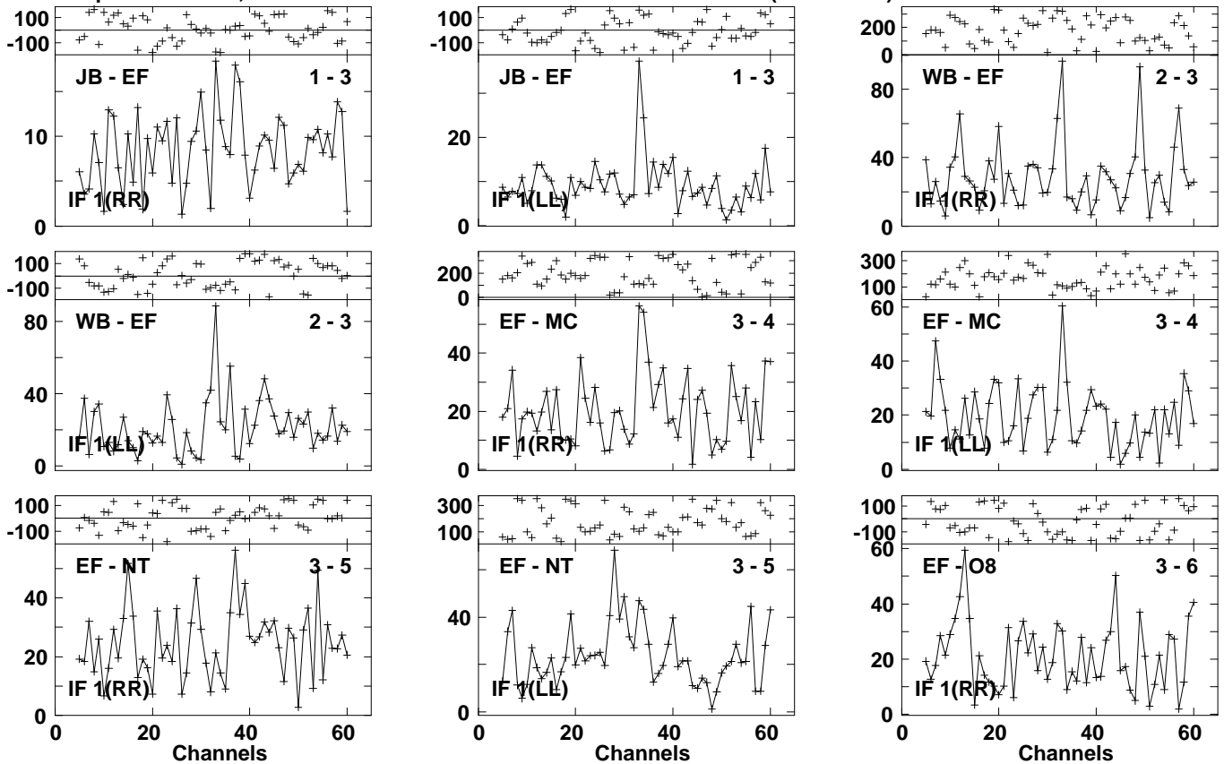
Lower frame: Milli Ampl Jy Top frame: Phas deg Vector averaged cross-power spectrum Several baselines displayed Timerange: 01/06:41:47 to 01/06:44:07
