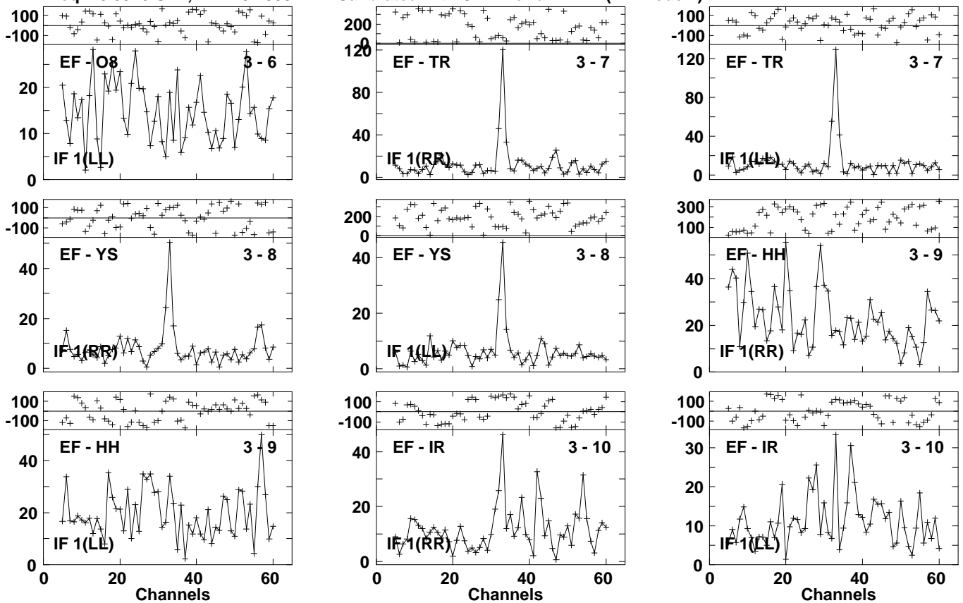
Lower frame: Milli Ampl Jy Top frame: Phas deg Vector averaged cross-power spectrum Several baselines displayed Timerange: 01/00:32:47 to 01/00:35:07
