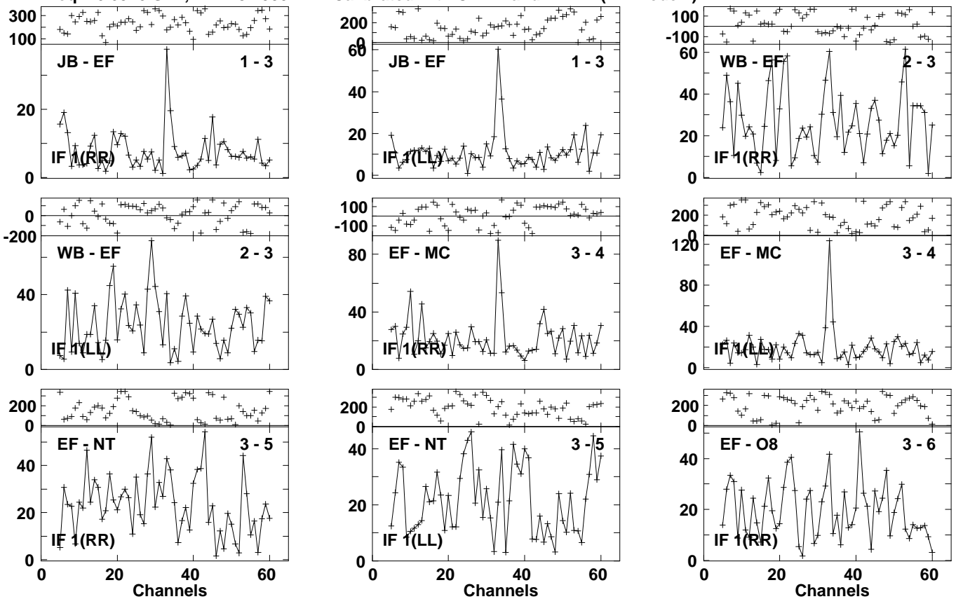
Lower frame: Milli Ampl Jy Top frame: Phas deg Vector averaged cross-power spectrum Several baselines displayed Timerange: 01/03:30:21 to 01/03:32:41
