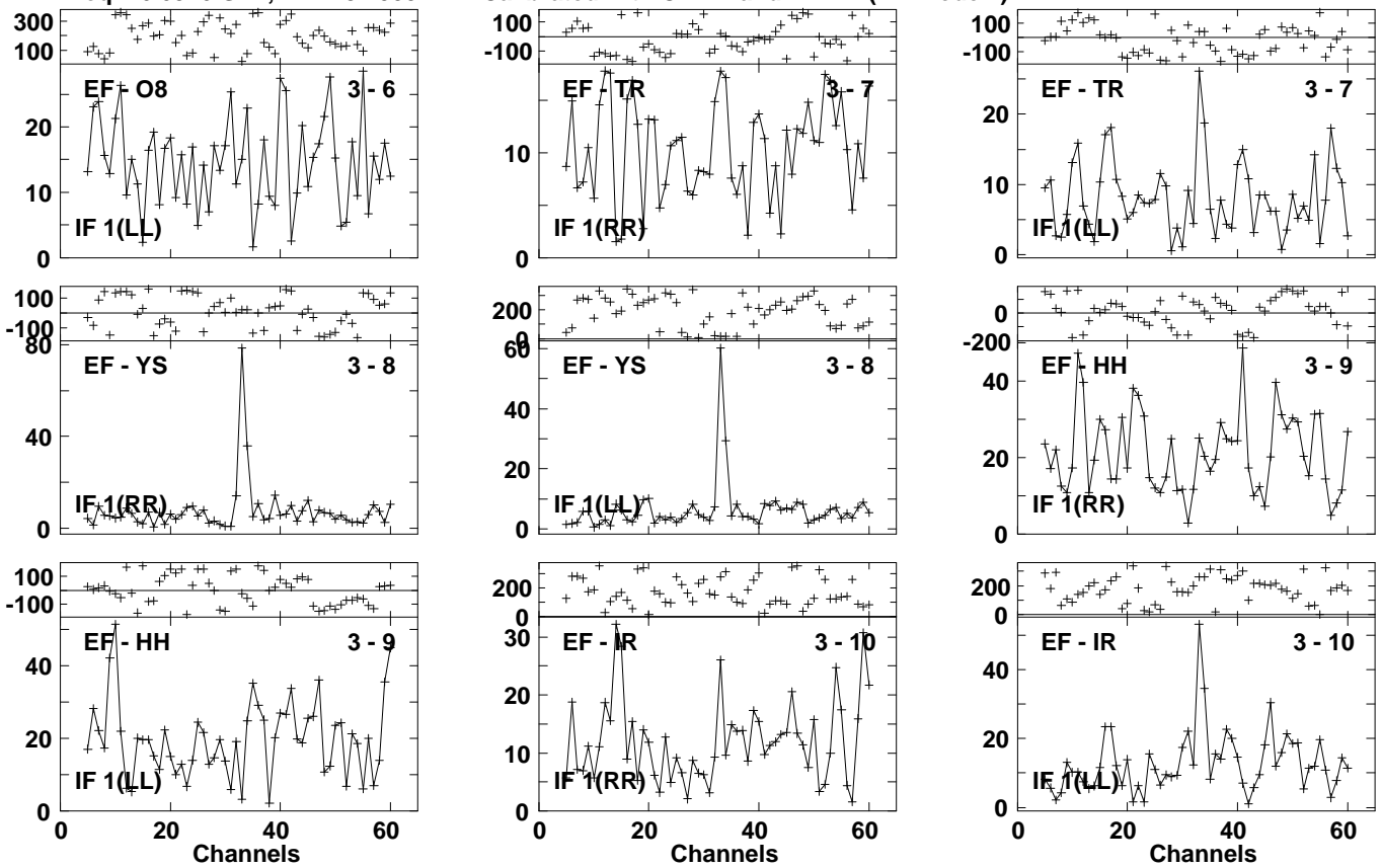
Lower frame: Milli Ampl Jy Top frame: Phas deg Vector averaged cross-power spectrum Several baselines displayed Timerange: 01/01:21:21 to 01/01:23:41
