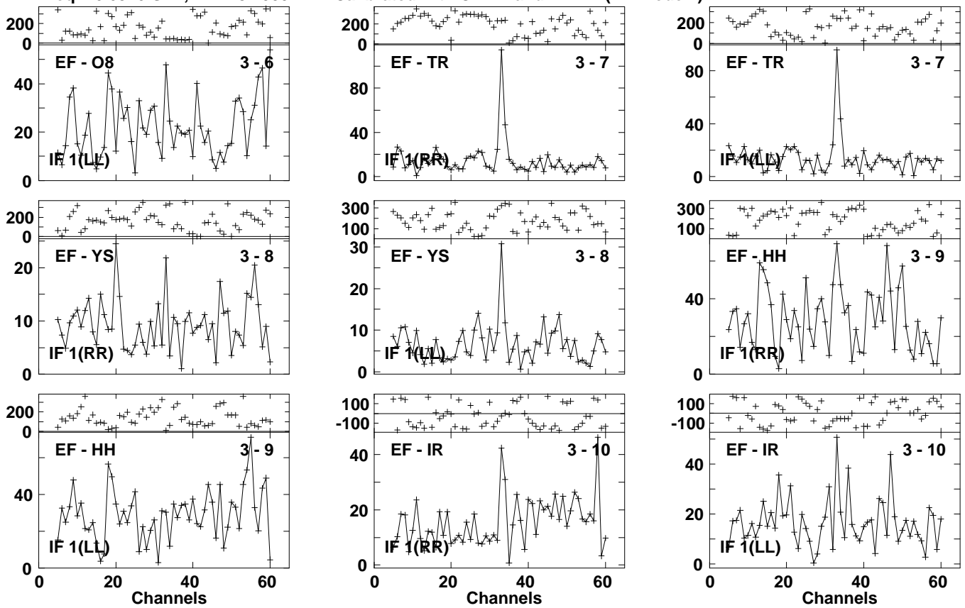
Lower frame: Milli Ampl Jy Top frame: Phas deg Vector averaged cross-power spectrum Several baselines displayed Timerange: 00/23:14:17 to 00/23:16:37
