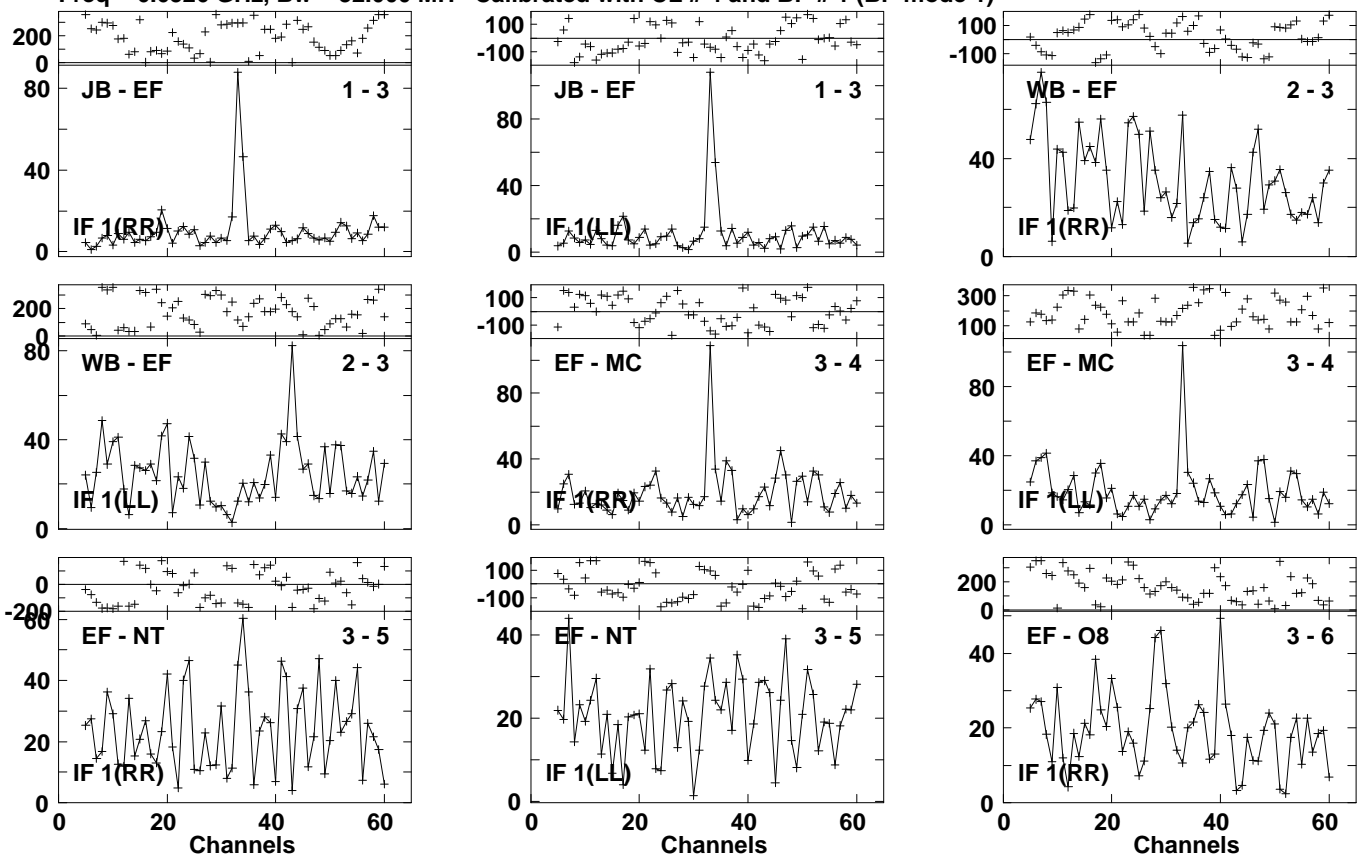
Lower frame: Milli Ampl Jy Top frame: Phas deg Vector averaged cross-power spectrum Several baselines displayed Timerange: 01/01:14:17 to 01/01:16:37
