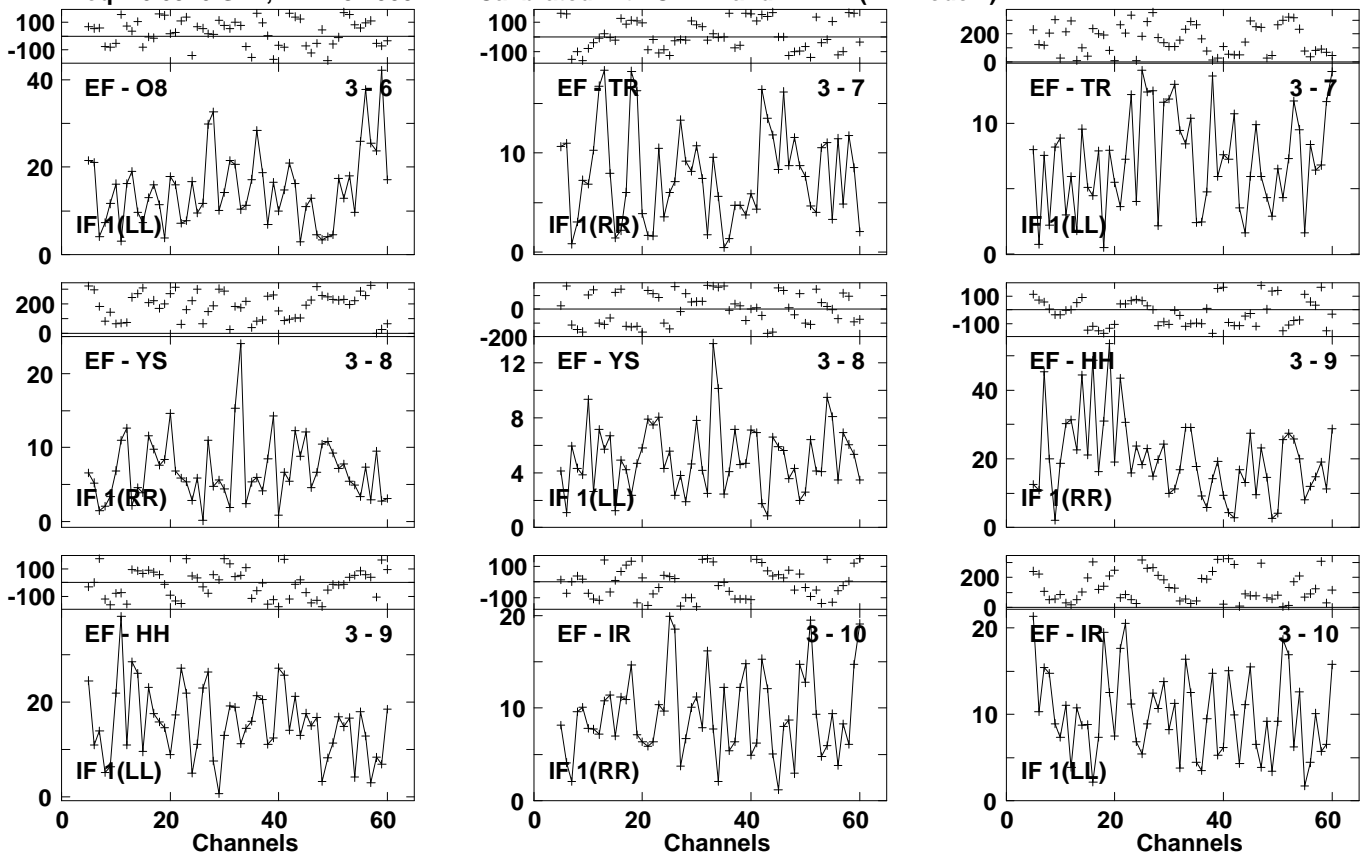
Lower frame: Milli Ampl Jy Top frame: Phas deg Vector averaged cross-power spectrum Several baselines displayed Timerange: 01/02:55:39 to 01/03:00:31
