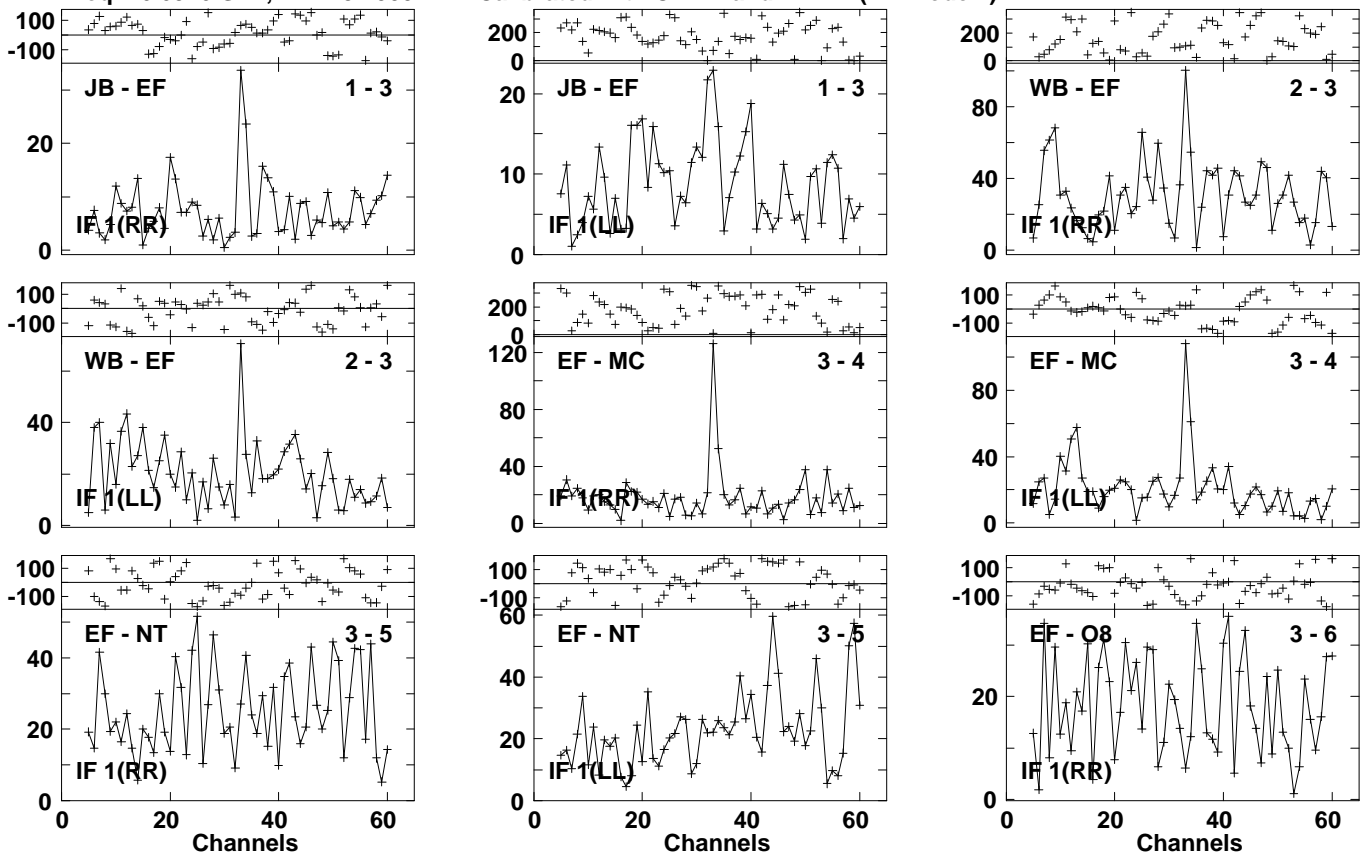
Lower frame: Milli Ampl Jy Top frame: Phas deg Vector averaged cross-power spectrum Several baselines displayed Timerange: 01/01:37:09 to 01/01:39:29
