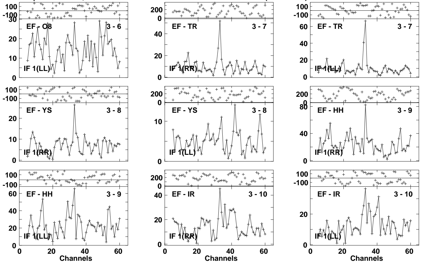
Lower frame: Milli Ampl Jy Top frame: Phas deg Vector averaged cross-power spectrum Several baselines displayed Timerange: 01/04:44:29 to 01/04:46:49
