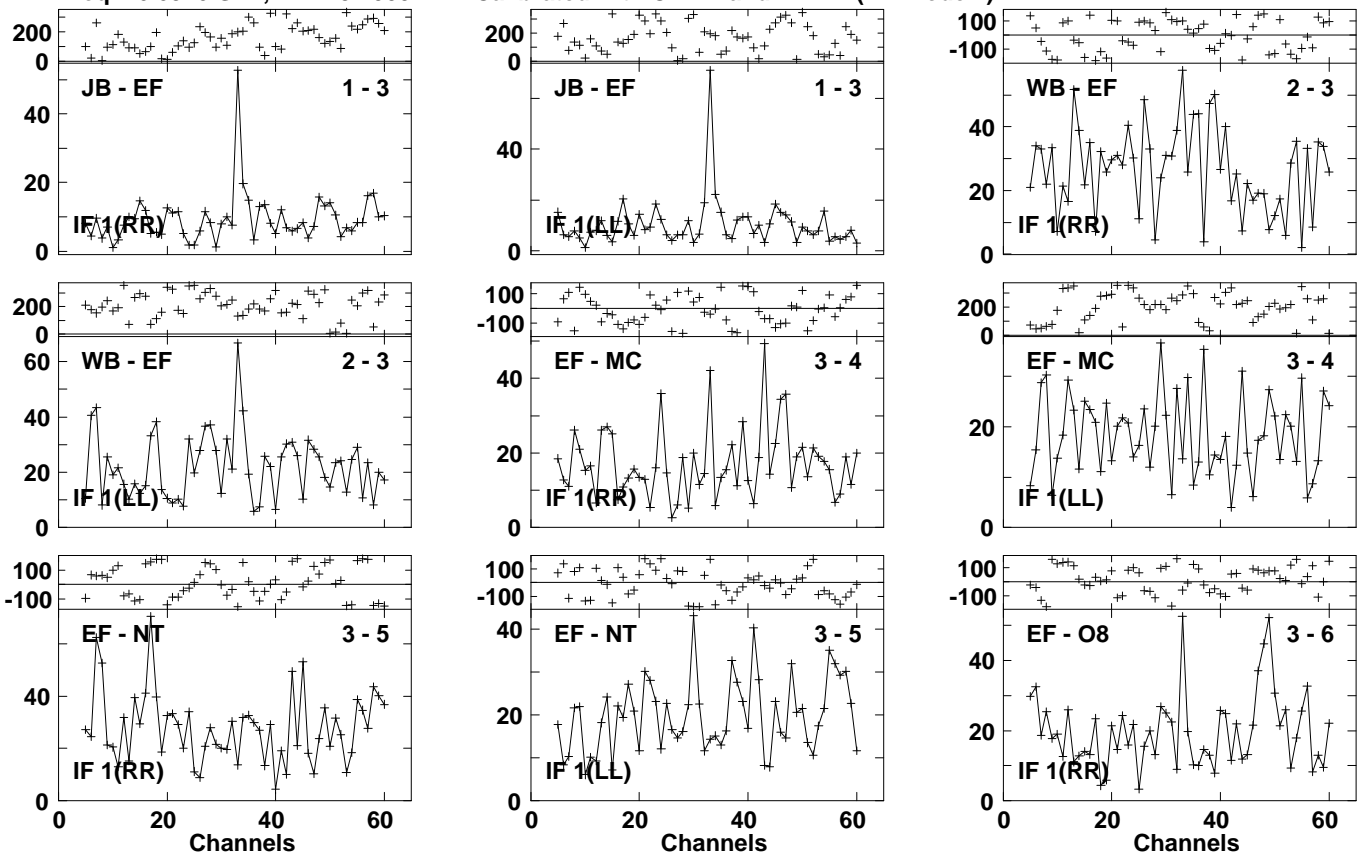
Lower frame: Milli Ampl Jy Top frame: Phas deg Vector averaged cross-power spectrum Several baselines displayed Timerange: 01/01:41:31 to 01/01:43:51
