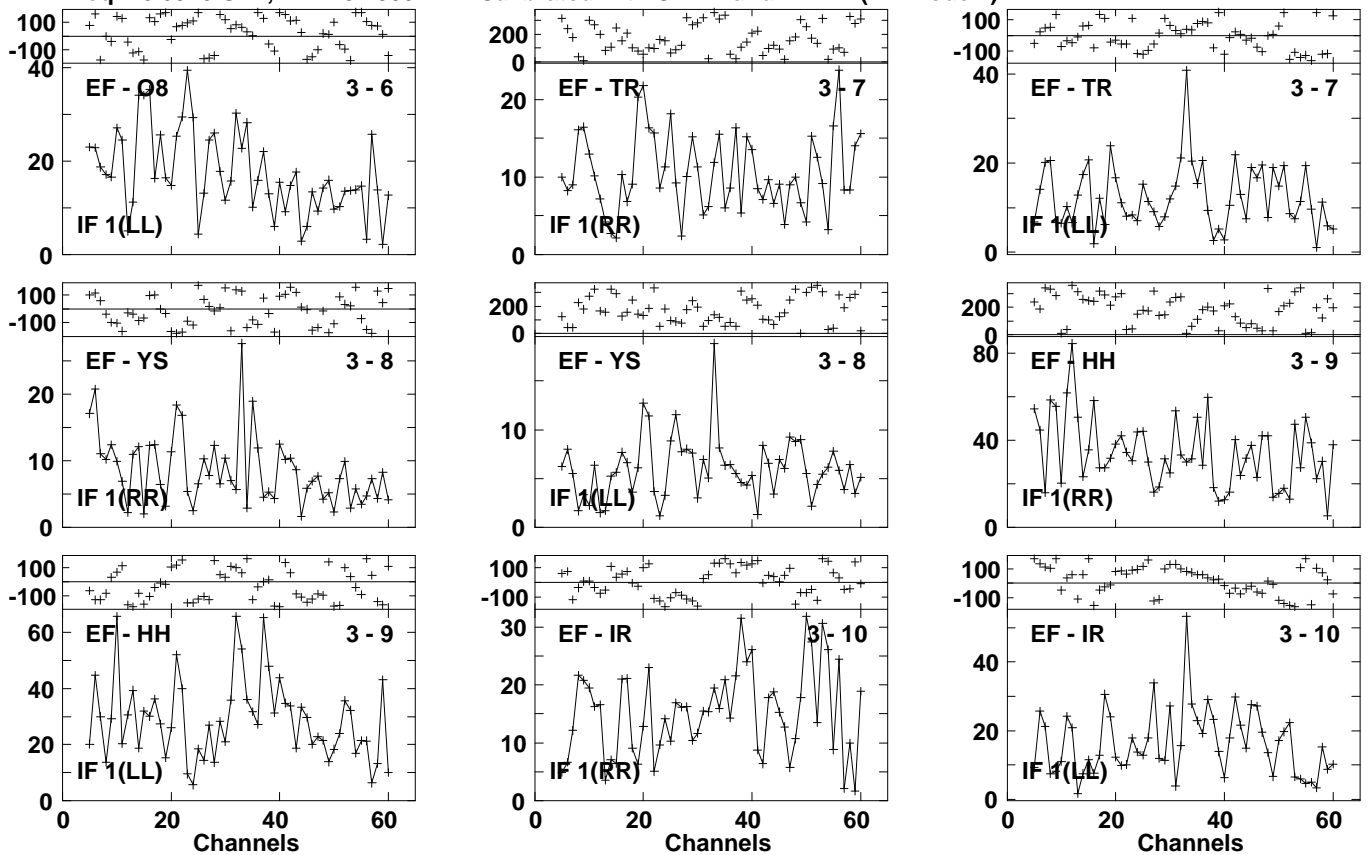
Lower frame: Milli Ampl Jy Top frame: Phas deg Vector averaged cross-power spectrum Several baselines displayed Timerange: 01/05:00:17 to 01/05:02:37
