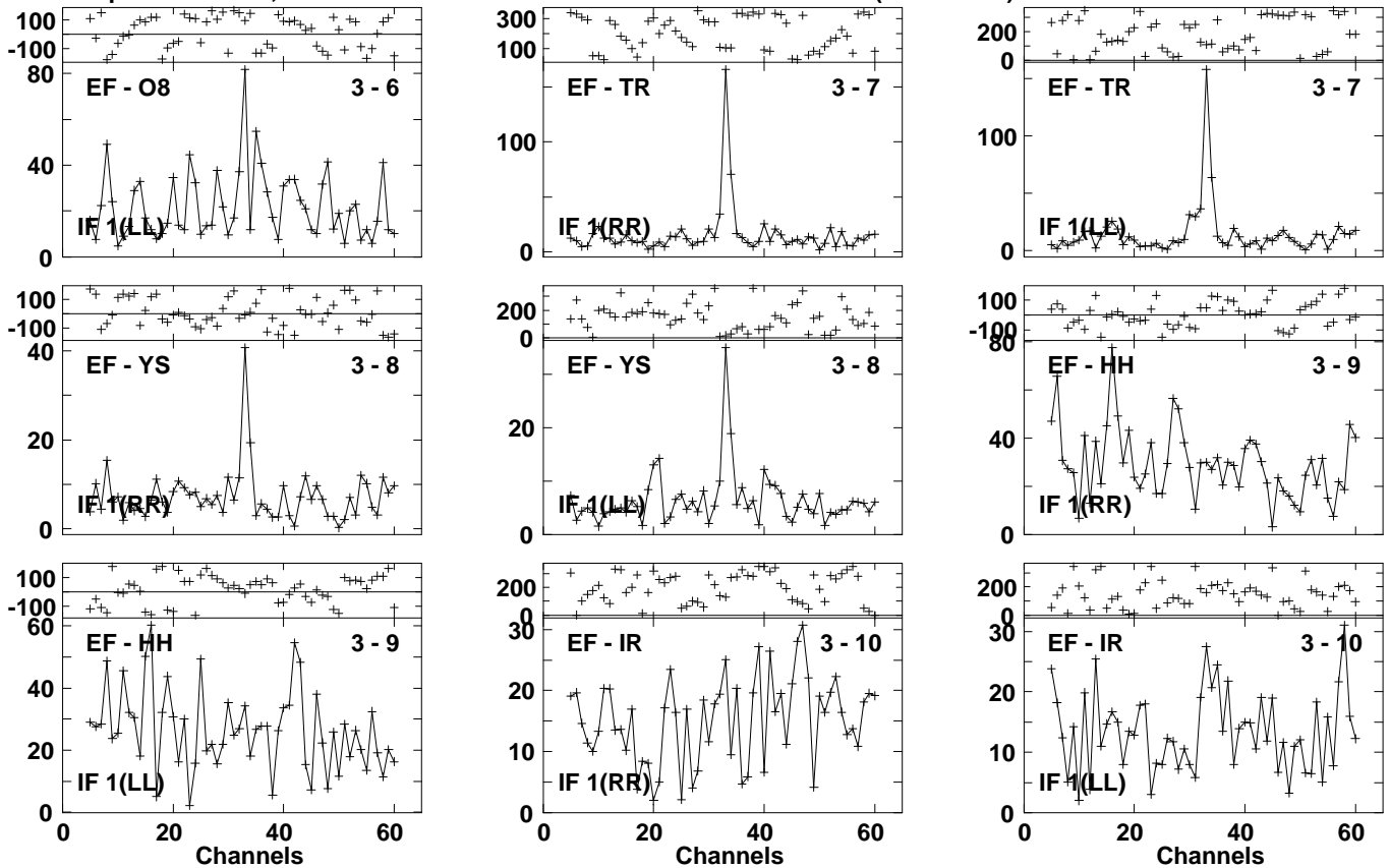
Lower frame: Milli Ampl Jy Top frame: Phas deg Vector averaged cross-power spectrum Several baselines displayed Timerange: 01/05:48:51 to 01/05:51:11
