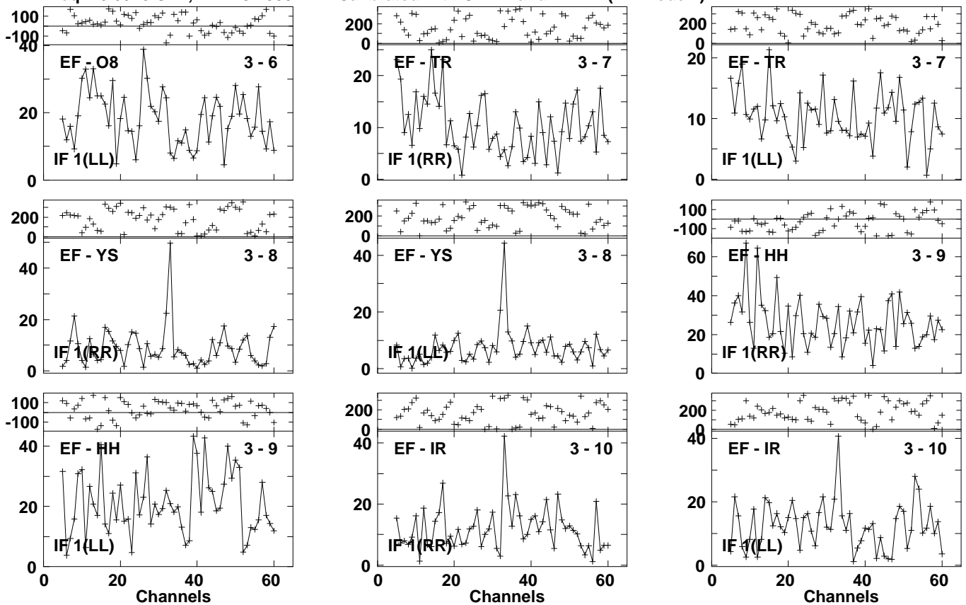
Lower frame: Milli Ampl Jy Top frame: Phas deg Vector averaged cross-power spectrum Several baselines displayed Timerange: 01/02:48:35 to 01/02:50:55
