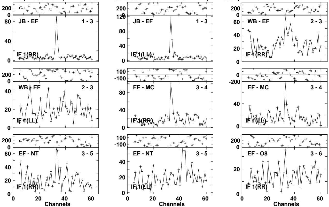
Lower frame: Milli Ampl Jy Top frame: Phas deg Vector averaged cross-power spectrum Several baselines displayed Timerange: 01/03:21:29 to 01/03:23:57
