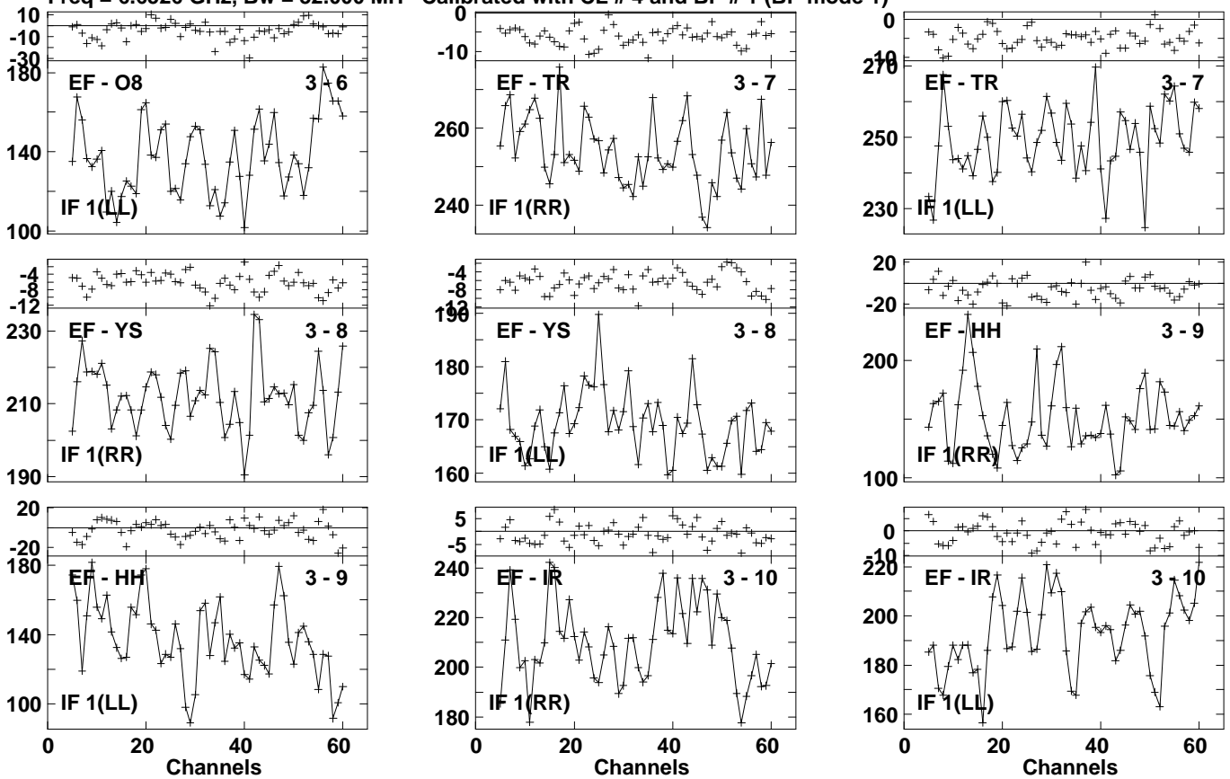
Lower frame: Milli Ampl Jy Top frame: Phas deg Vector averaged cross-power spectrum Several baselines displayed Timerange: 01/01:46:45 to 01/01:48:23
