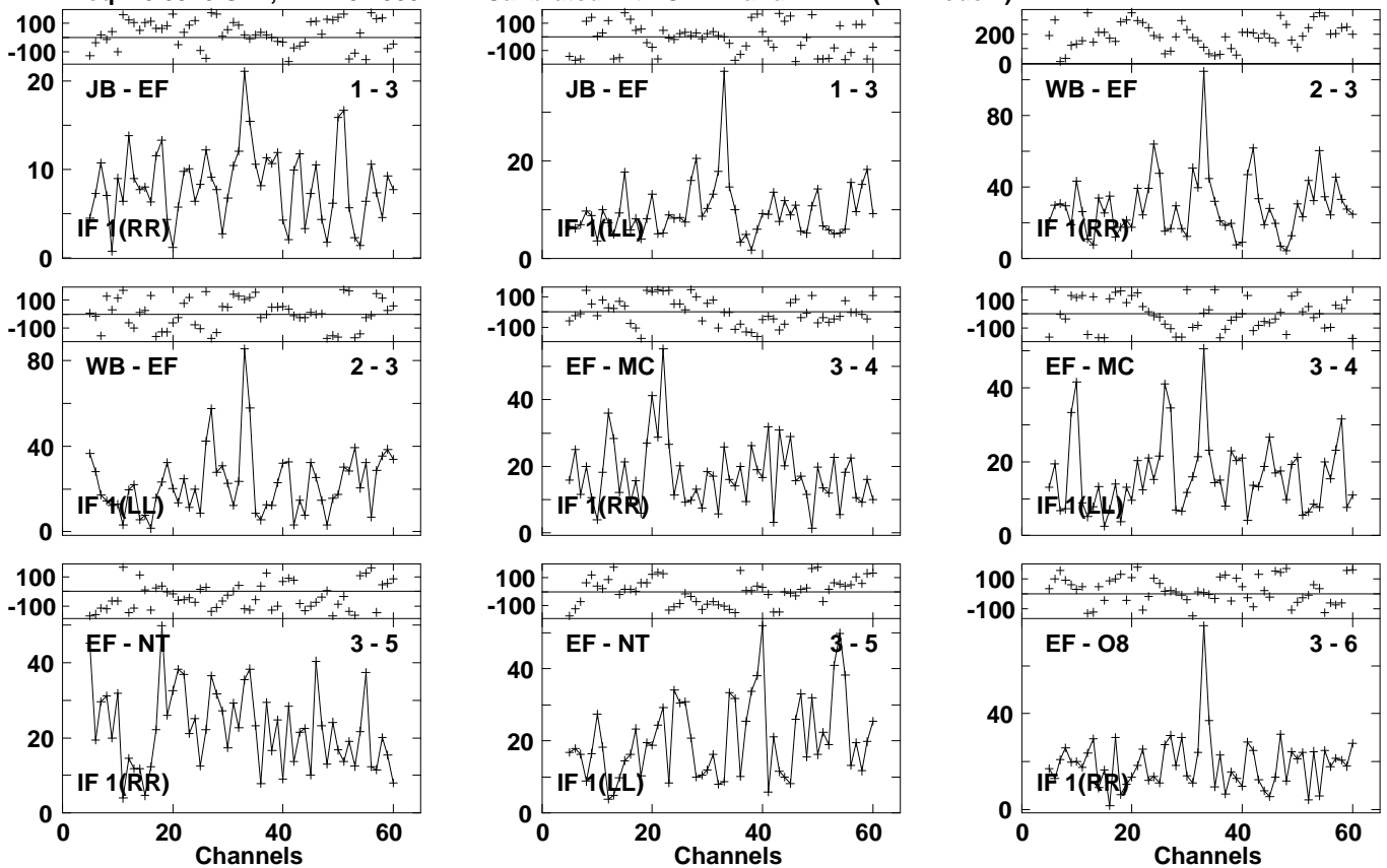
Lower frame: Milli Ampl Jy Top frame: Phas deg Vector averaged cross-power spectrum Several baselines displayed Timerange: 00/23:21:21 to 00/23:23:41
