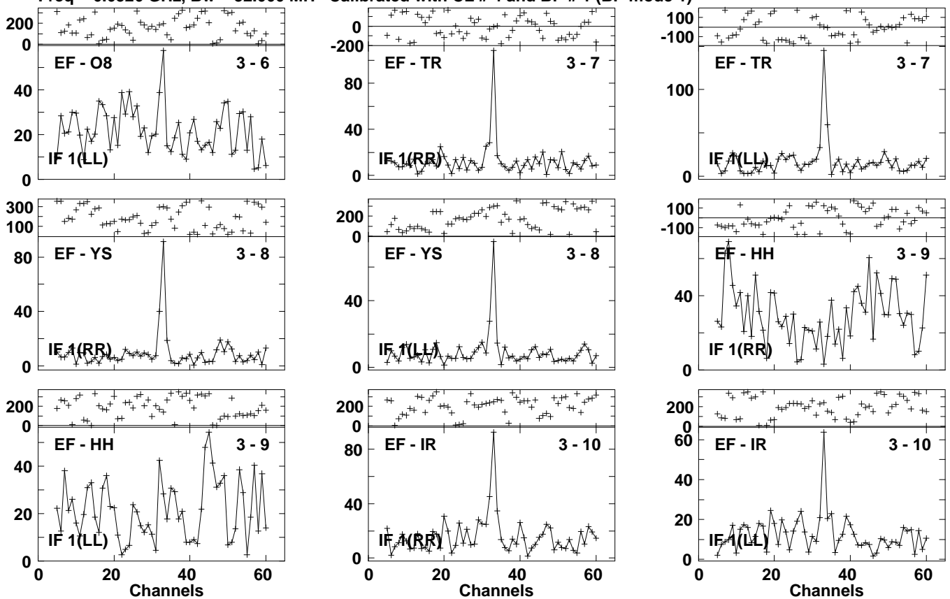
Lower frame: Milli Ampl Jy Top frame: Phas deg Vector averaged cross-power spectrum Several baselines displayed Timerange: 01/00:37:09 to 01/00:39:29
