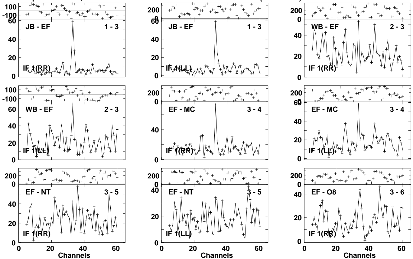
Lower frame: Milli Ampl Jy Top frame: Phas deg Vector averaged cross-power spectrum Several baselines displayed Timerange: 01/06:44:29 to 01/06:46:49
