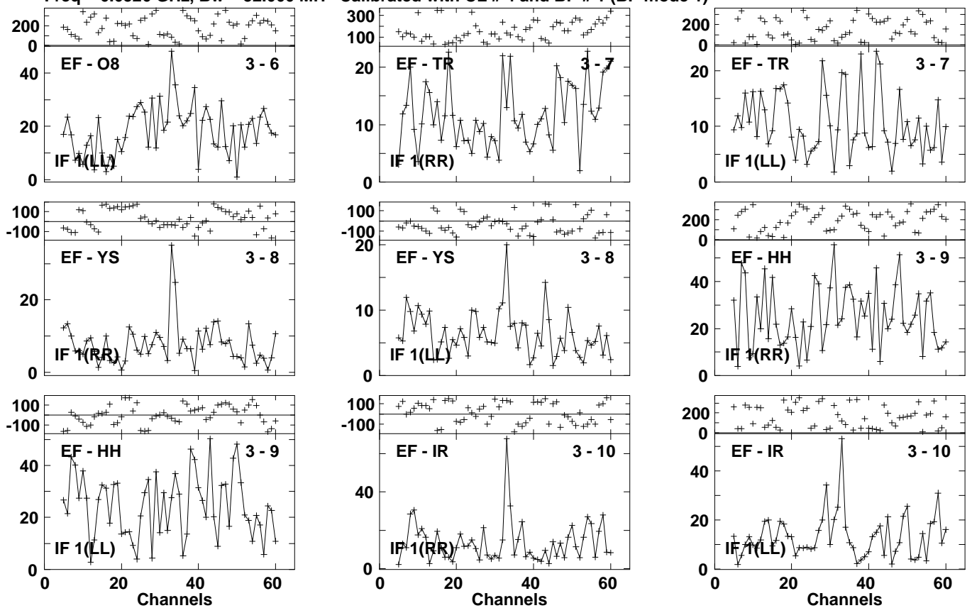
Lower frame: Milli Ampl Jy Top frame: Phas deg Vector averaged cross-power spectrum Several baselines displayed Timerange: 01/01:30:05 to 01/01:32:25
