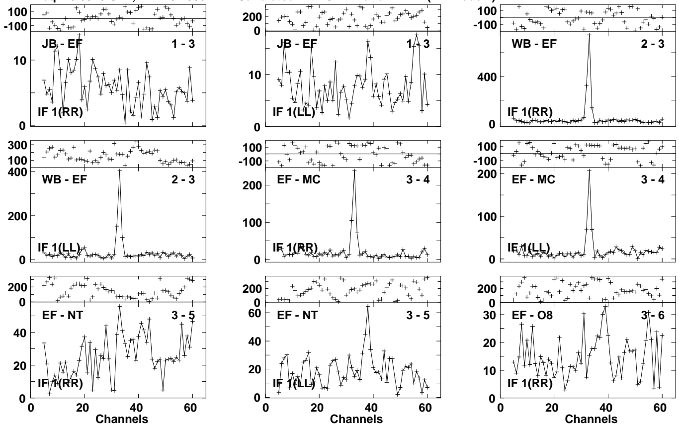
Lower frame: Milli Ampl Jy Top frame: Phas deg Vector averaged cross-power spectrum Several baselines displayed Timerange: 01/04:55:55 to 01/04:58:15
