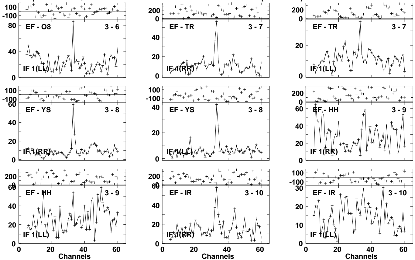
Lower frame: Milli Ampl Jy Top frame: Phas deg Vector averaged cross-power spectrum Several baselines displayed Timerange: 01/06:00:17 to 01/06:02:37
