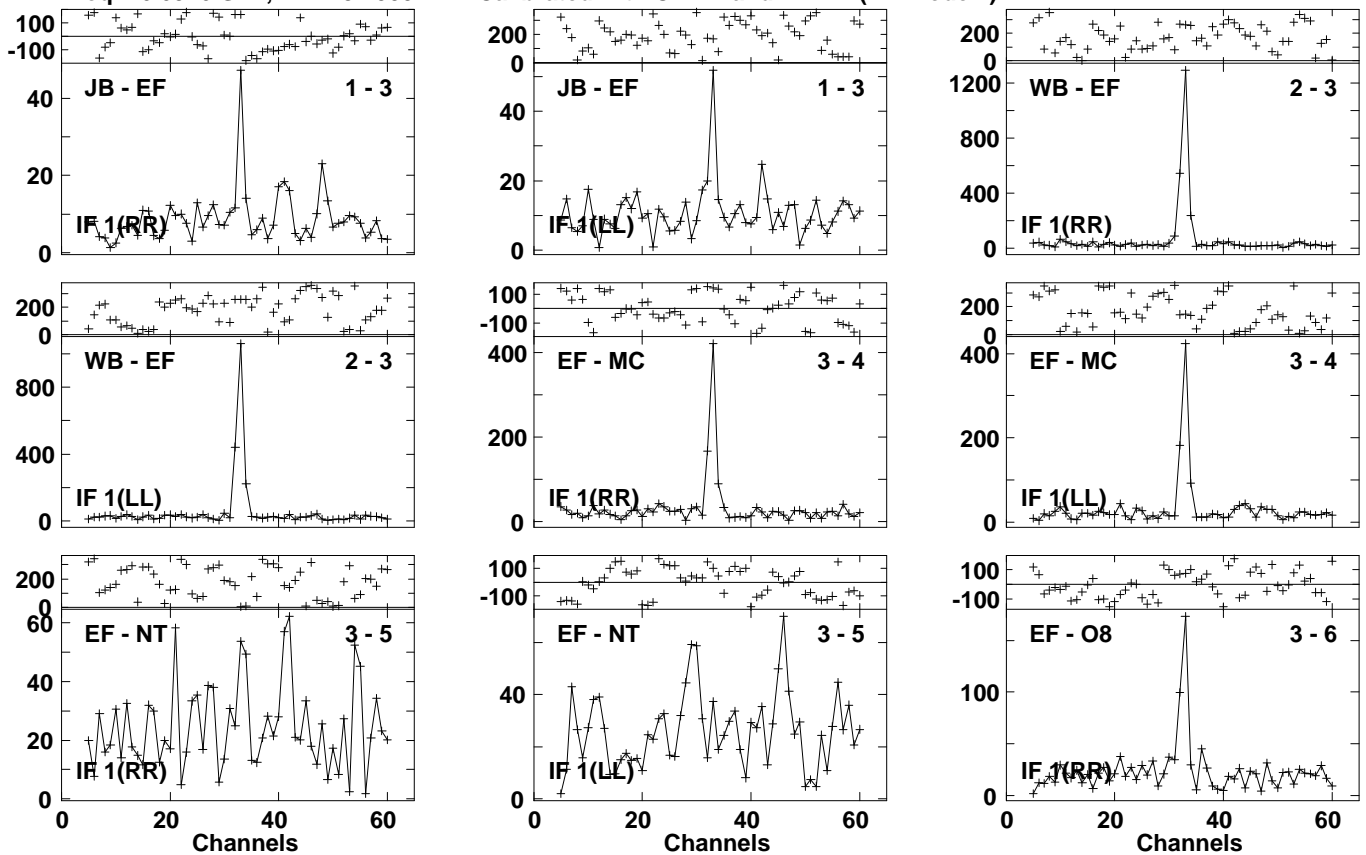
Lower frame: Milli Ampl Jy Top frame: Phas deg Vector averaged cross-power spectrum Several baselines displayed Timerange: 01/04:30:21 to 01/04:32:41
