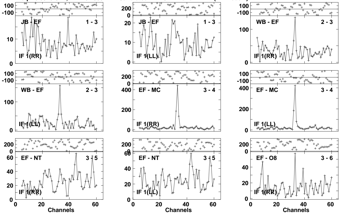
Lower frame: Milli Ampl Jy Top frame: Phas deg Vector averaged cross-power spectrum Several baselines displayed Timerange: 01/02:14:17 to 01/02:16:37
