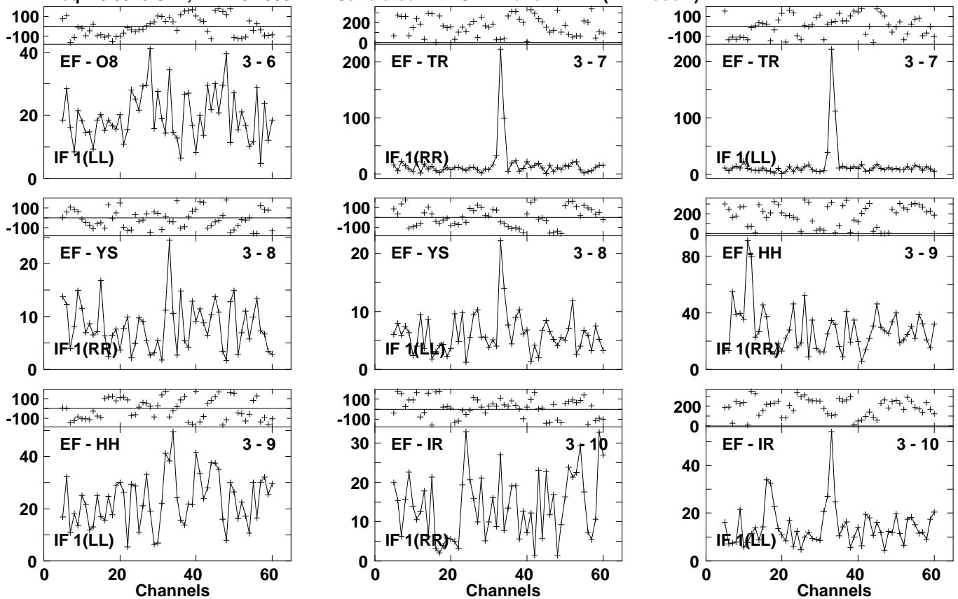
Lower frame: Milli Ampl Jy Top frame: Phas deg Vector averaged cross-power spectrum Several baselines displayed Timerange: 01/03:48:51 to 01/03:51:11
