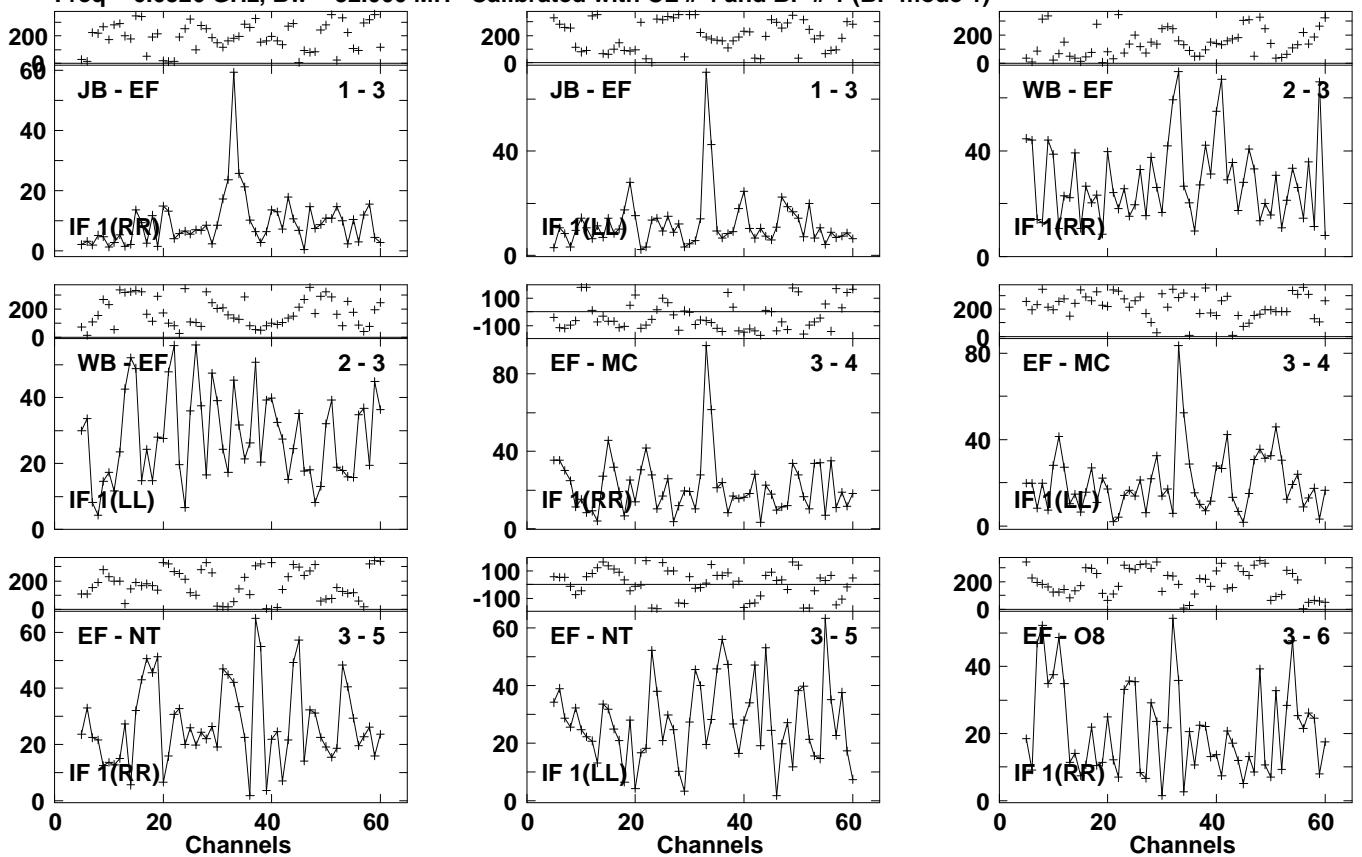
Lower frame: Milli Ampl Jy Top frame: Phas deg Vector averaged cross-power spectrum Several baselines displayed Timerange: 00/23:37:09 to 00/23:39:29
