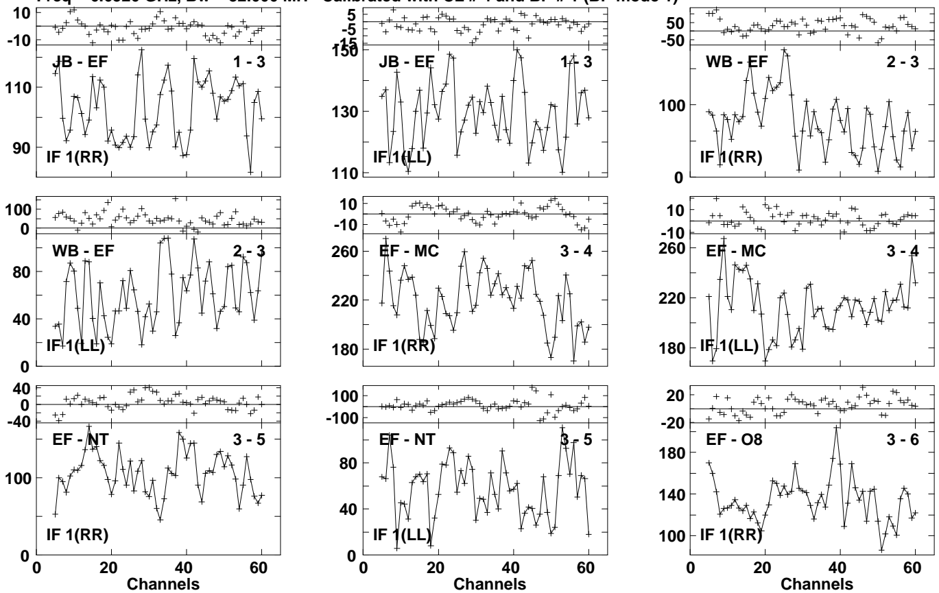
Lower frame: Milli Ampl Jy Top frame: Phas deg Vector averaged cross-power spectrum Several baselines displayed Timerange: 00/23:35:19 to 00/23:36:57
