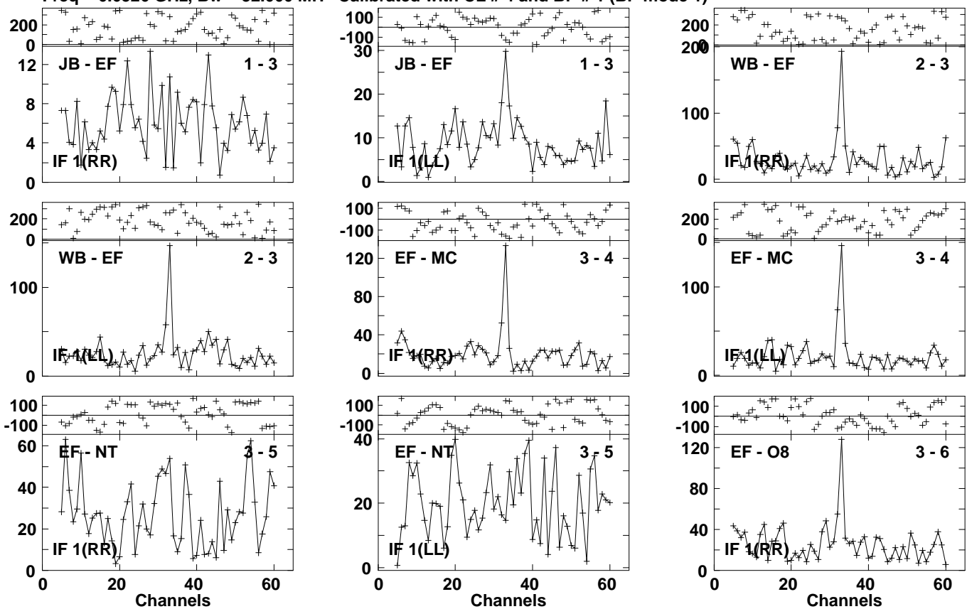
Lower frame: Milli Ampl Jy Top frame: Phas deg Vector averaged cross-power spectrum Several baselines displayed Timerange: 01/06:21:29 to 01/06:23:57
