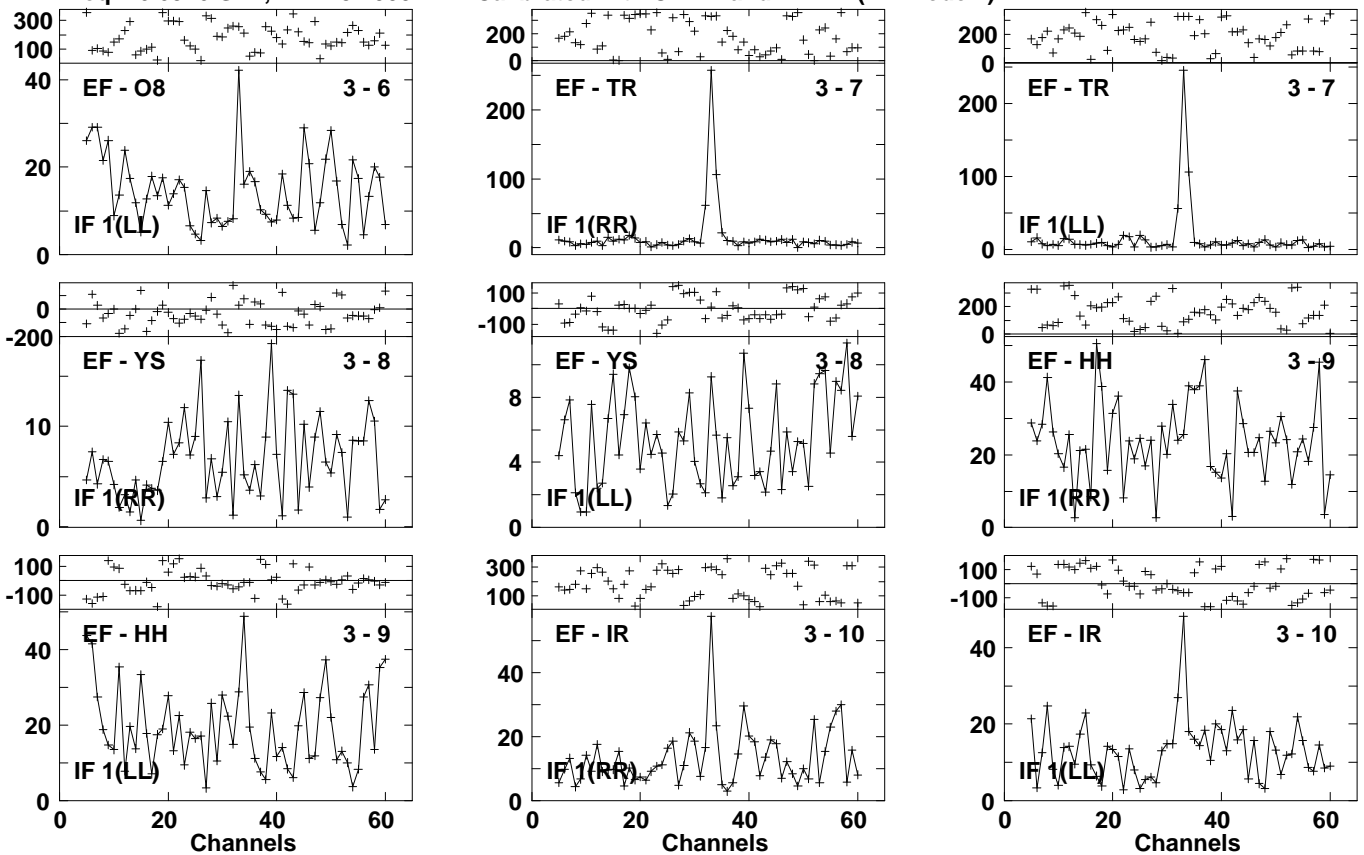
Lower frame: Milli Ampl Jy Top frame: Phas deg Vector averaged cross-power spectrum Several baselines displayed Timerange: 01/03:33:03 to 01/03:35:23
