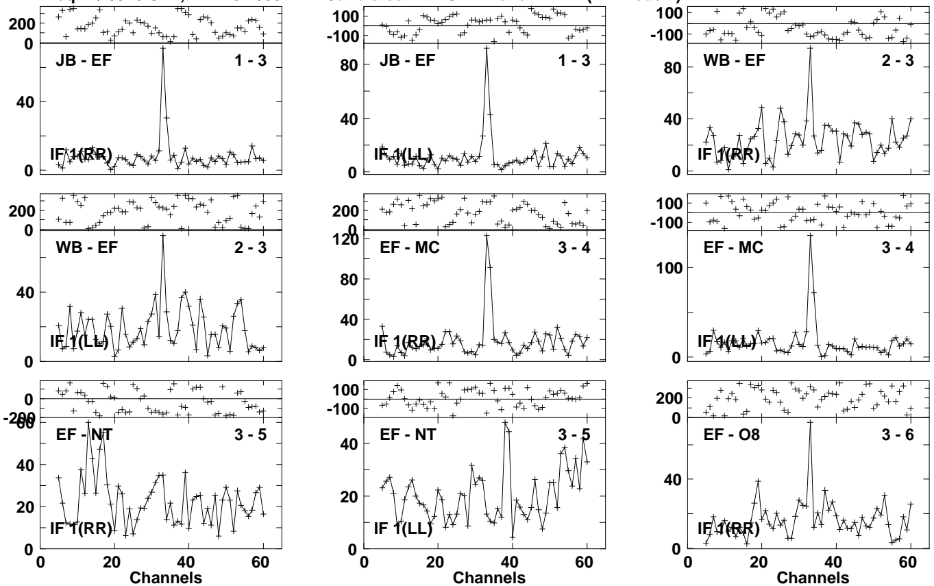
Lower frame: Milli Ampl Jy Top frame: Phas deg Vector averaged cross-power spectrum Several baselines displayed Timerange: 01/05:33:03 to 01/05:35:23
