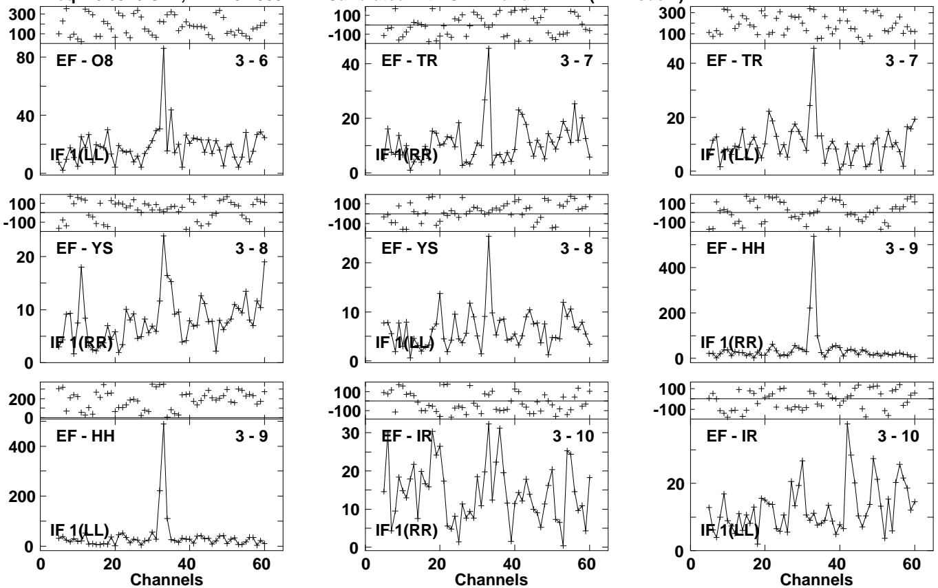
Lower frame: Milli Ampl Jy Top frame: Phas deg Vector averaged cross-power spectrum Several baselines displayed Timerange: 01/04:21:29 to 01/04:23:57
