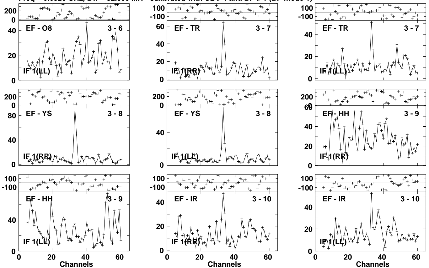
Lower frame: Milli Ampl Jy Top frame: Phas deg Vector averaged cross-power spectrum Several baselines displayed Timerange: 01/01:18:39 to 01/01:20:59
