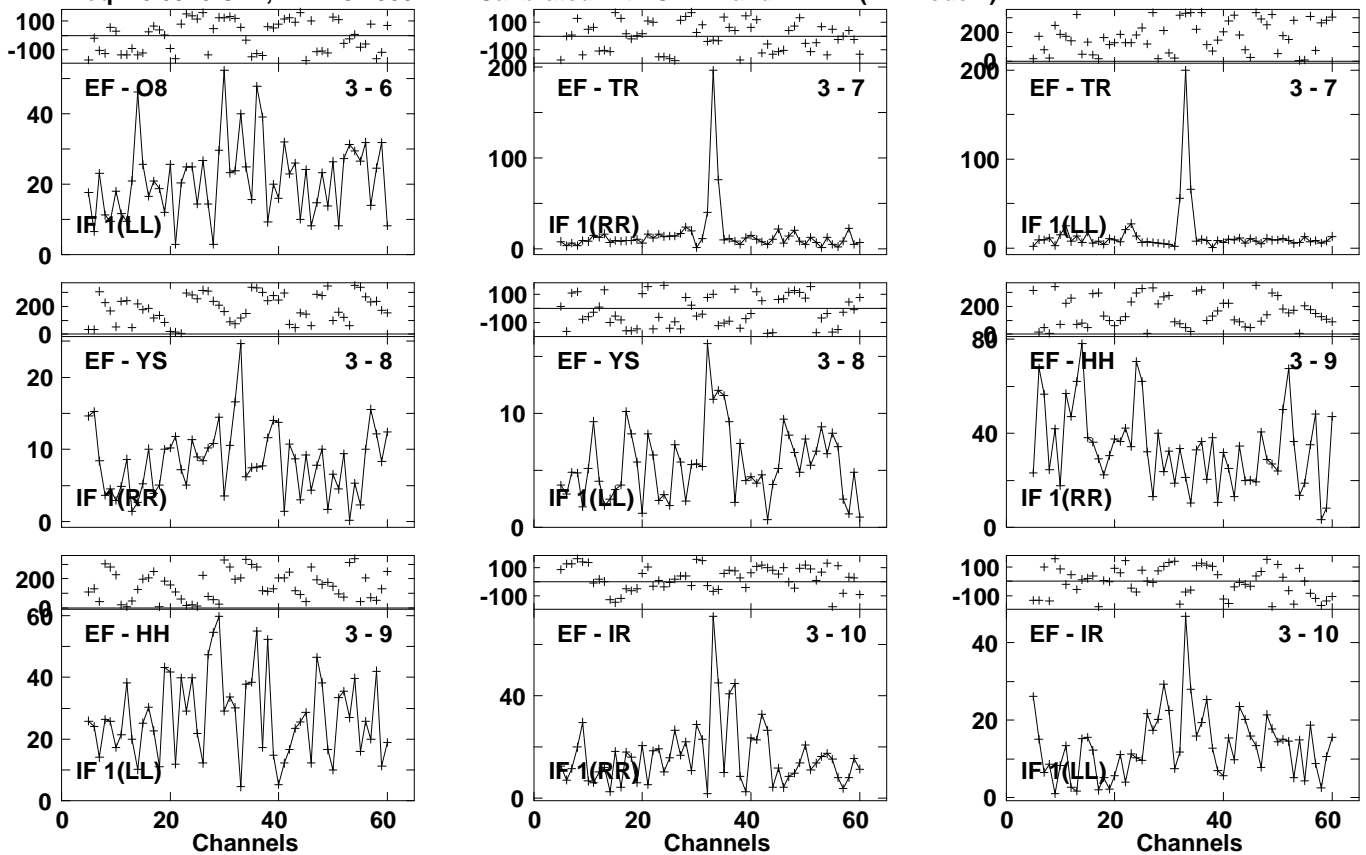
Lower frame: Milli Ampl Jy Top frame: Phas deg Vector averaged cross-power spectrum Several baselines displayed Timerange: 01/05:37:25 to 01/05:39:45
