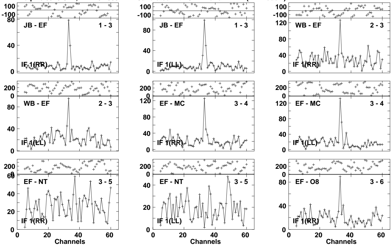
Lower frame: Milli Ampl Jy Top frame: Phas deg Vector averaged cross-power spectrum Several baselines displayed Timerange: 01/05:30:21 to 01/05:32:41
