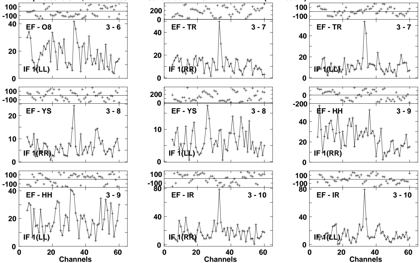
Lower frame: Milli Ampl Jy Top frame: Phas deg Vector averaged cross-power spectrum Several baselines displayed Timerange: 01/03:37:25 to 01/03:39:45
