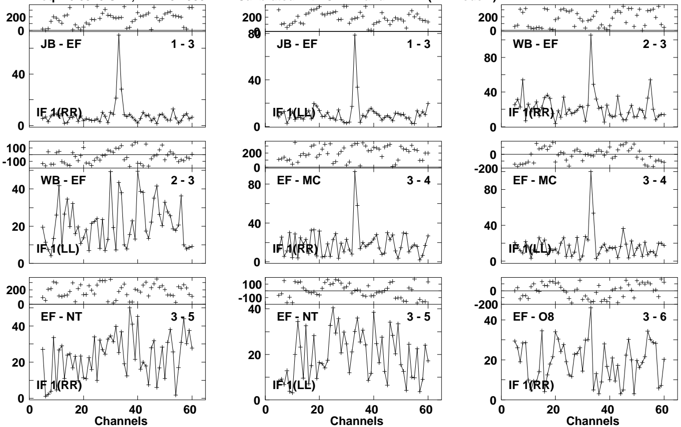
Lower frame: Milli Ampl Jy Top frame: Phas deg Vector averaged cross-power spectrum Several baselines displayed Timerange: 01/05:55:55 to 01/05:58:15
