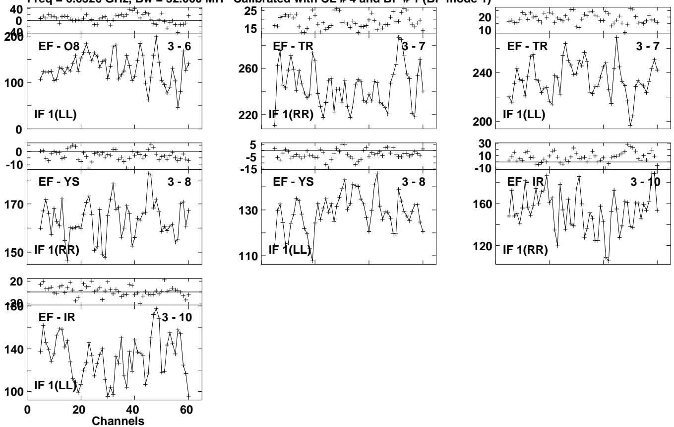
Lower frame: Milli Ampl Jy Top frame: Phas deg Vector averaged cross-power spectrum Several baselines displayed Timerange: 01/06:35:35 to 01/06:37:13
