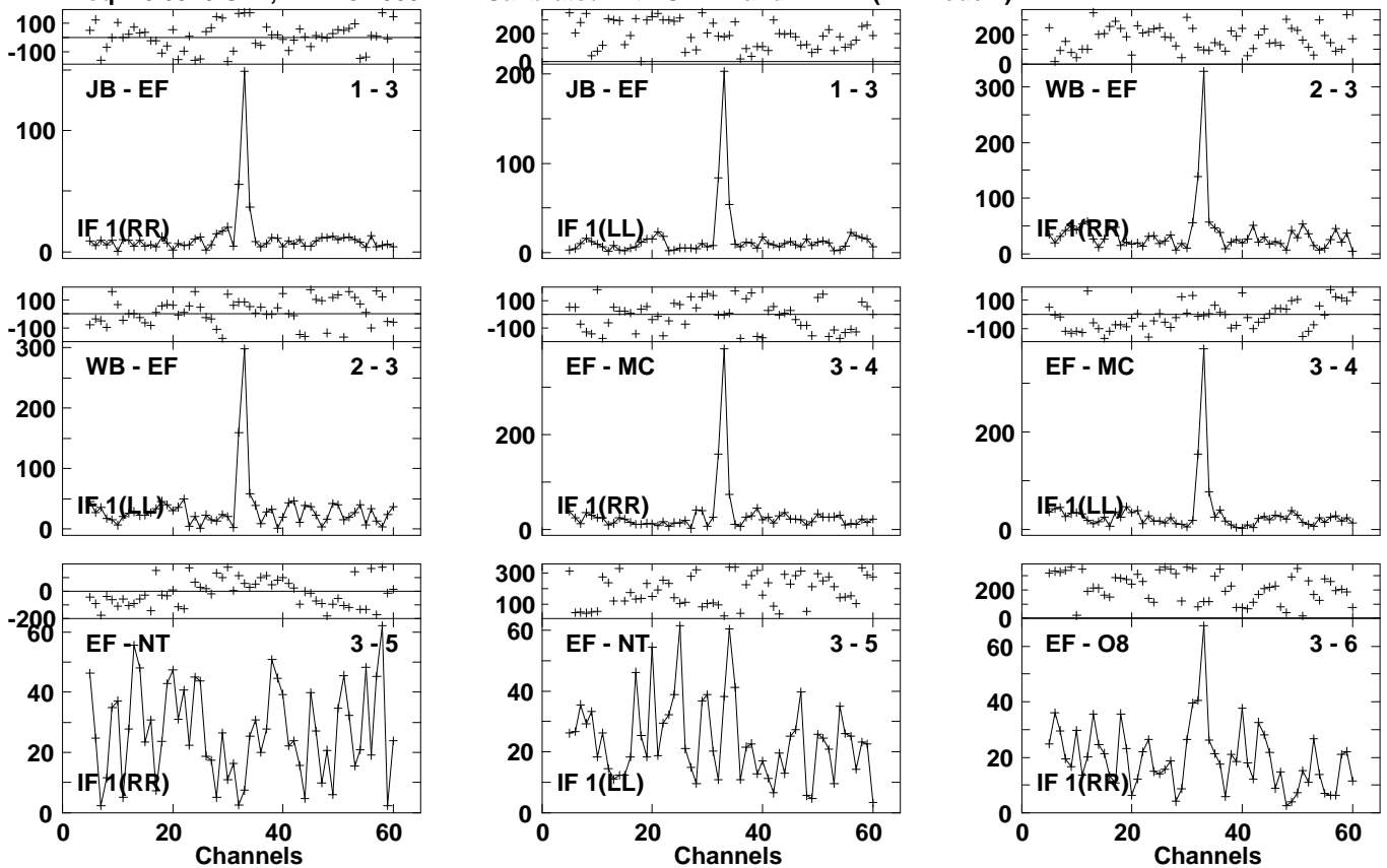
Lower frame: Milli Ampl Jy Top frame: Phas deg Vector averaged cross-power spectrum Several baselines displayed Timerange: 01/02:30:05 to 01/02:32:25
