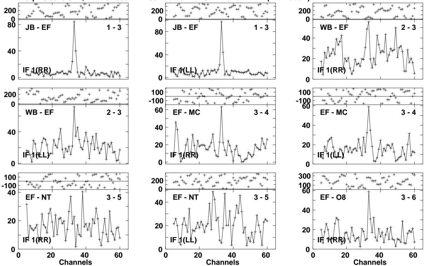
Lower frame: Milli Ampl Jy Top frame: Phas deg Vector averaged cross-power spectrum Several baselines displayed Timerange: 01/01:44:13 to 01/01:46:33
