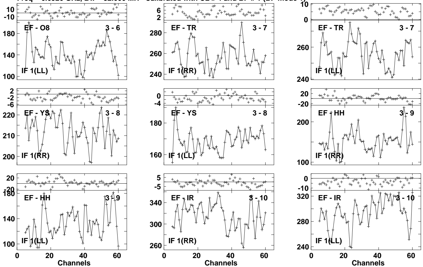
Lower frame: Milli Ampl Jy Top frame: Phas deg Vector averaged cross-power spectrum Several baselines displayed Timerange: 01/01:35:19 to 01/01:36:57
