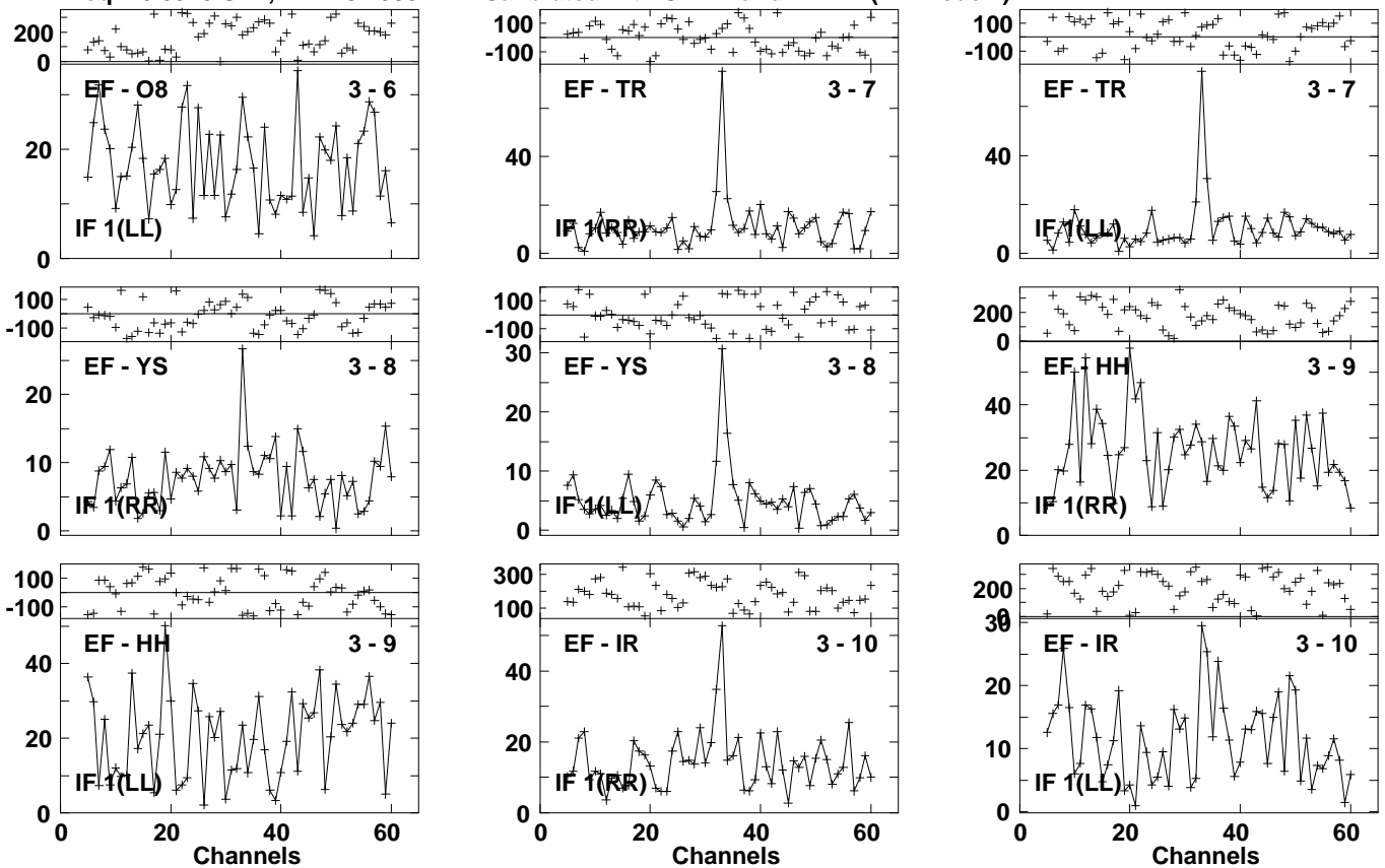
Lower frame: Milli Ampl Jy Top frame: Phas deg Vector averaged cross-power spectrum Several baselines displayed Timerange: 00/23:32:47 to 00/23:35:07
