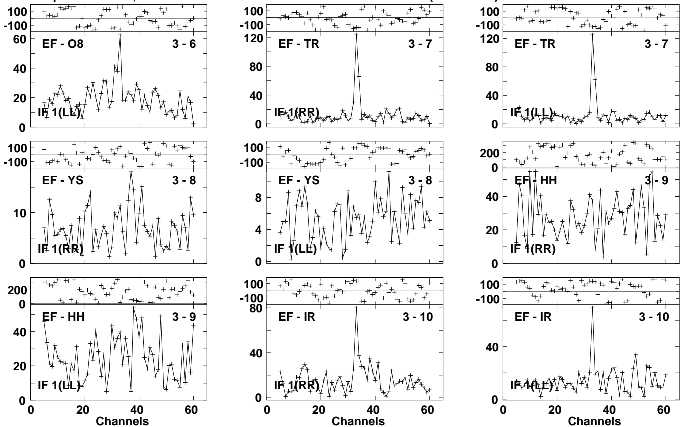
Lower frame: Milli Ampl Jy Top frame: Phas deg Vector averaged cross-power spectrum Several baselines displayed Timerange: 01/06:07:21 to 01/06:09:41
