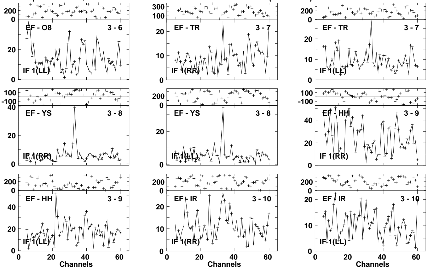
Lower frame: Milli Ampl Jy Top frame: Phas deg Vector averaged cross-power spectrum Several baselines displayed Timerange: 01/02:44:13 to 01/02:46:33
