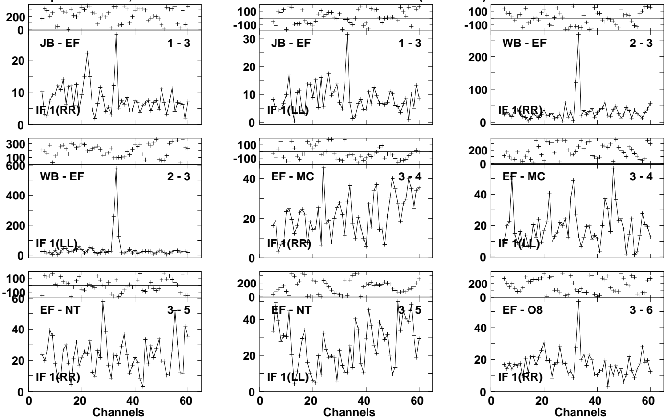
Lower frame: Milli Ampl Jy Top frame: Phas deg Vector averaged cross-power spectrum Several baselines displayed Timerange: 01/04:53:13 to 01/04:55:33
