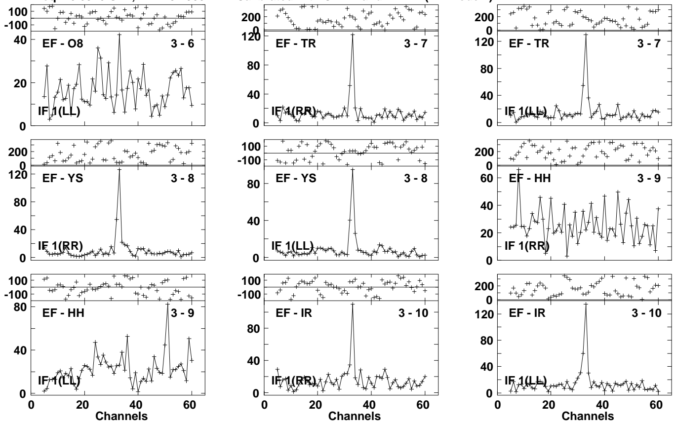
Lower frame: Milli Ampl Jy Top frame: Phas deg Vector averaged cross-power spectrum Several baselines displayed Timerange: 01/00:14:17 to 01/00:16:37
