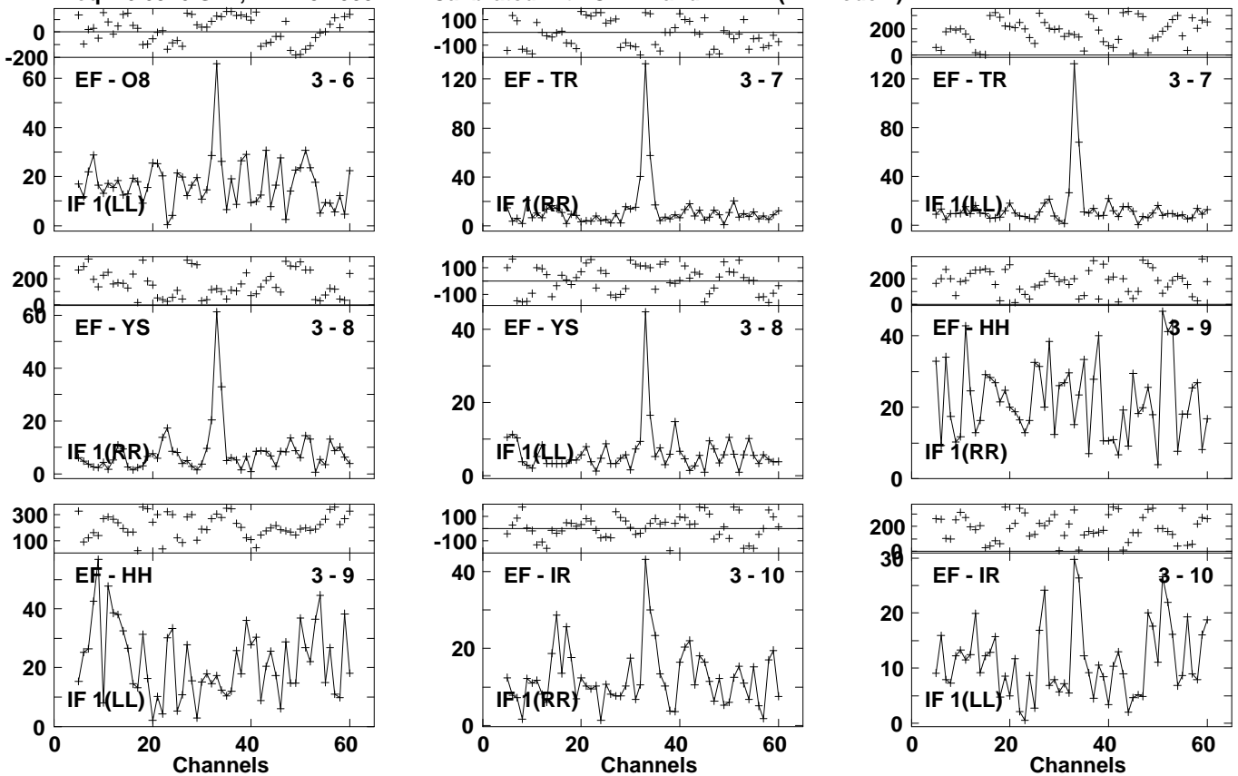
Lower frame: Milli Ampl Jy Top frame: Phas deg Vector averaged cross-power spectrum Several baselines displayed Timerange: 00/23:44:13 to 00/23:46:33
