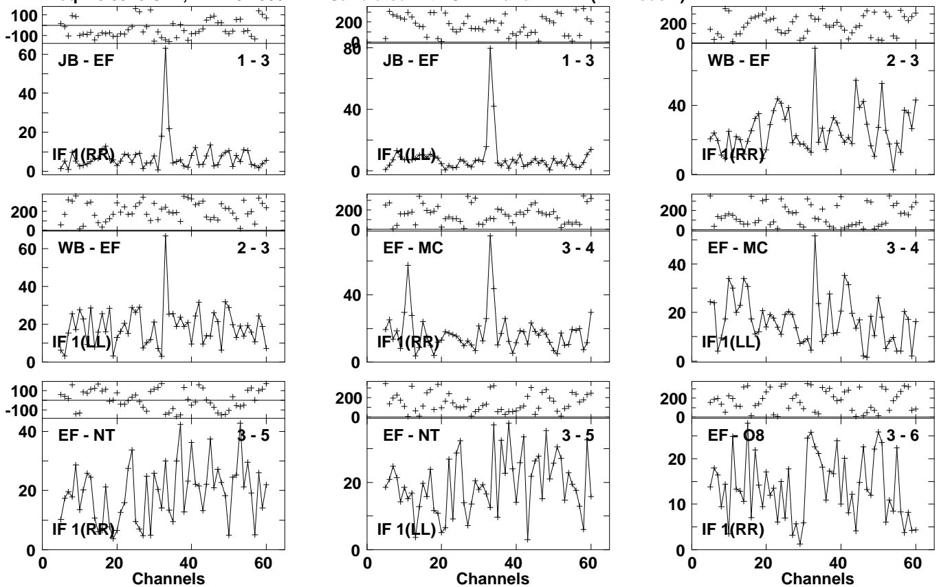
Lower frame: Milli Ampl Jy Top frame: Phas deg Vector averaged cross-power spectrum Several baselines displayed Timerange: 01/03:44:29 to 01/03:46:49
