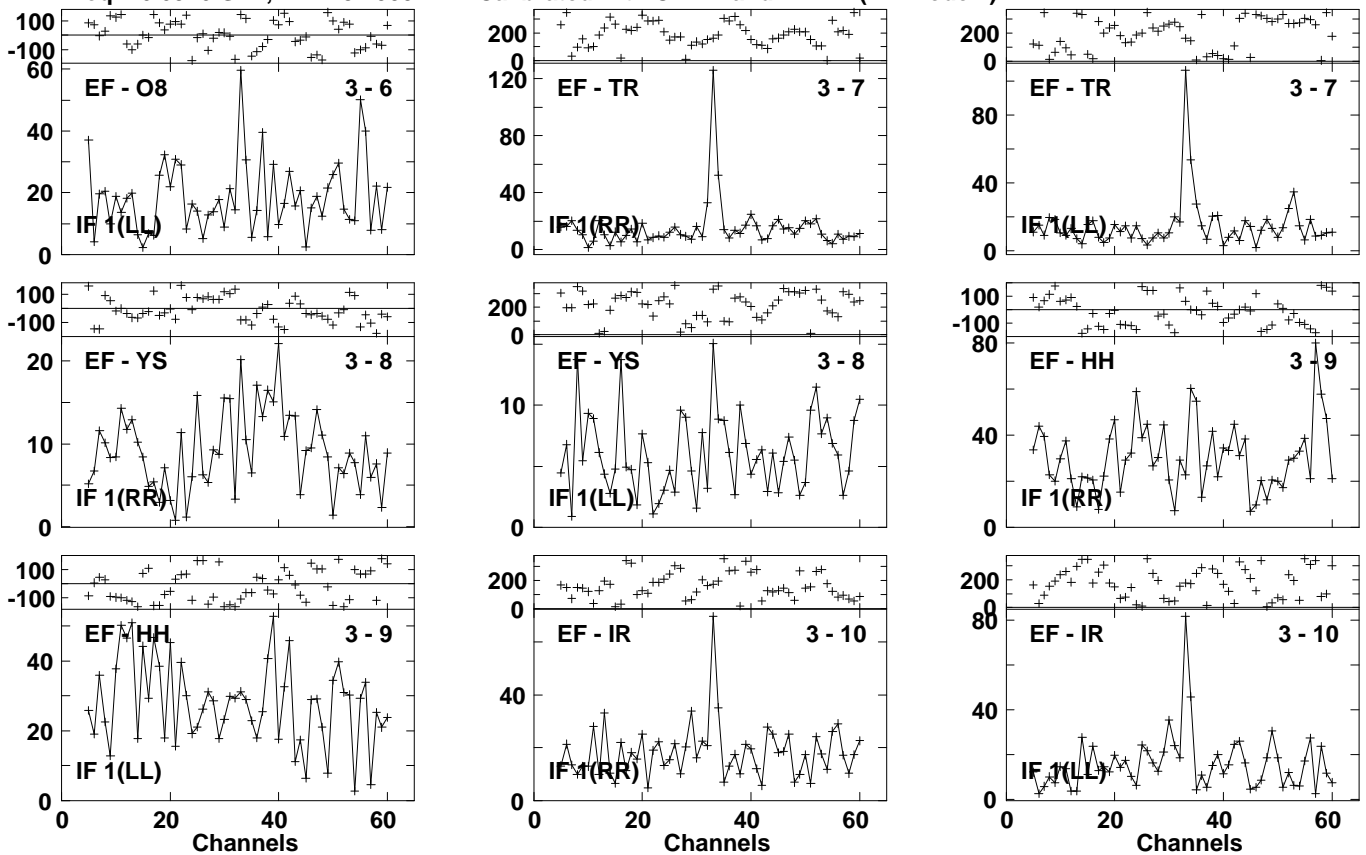
Lower frame: Milli Ampl Jy Top frame: Phas deg Vector averaged cross-power spectrum Several baselines displayed Timerange: 01/05:53:13 to 01/05:55:33
