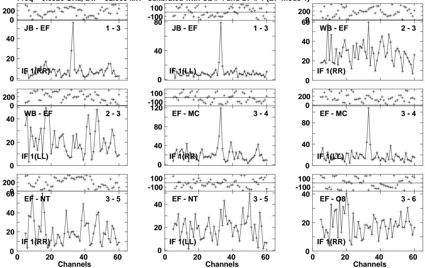
Lower frame: Milli Ampl Jy Top frame: Phas deg Vector averaged cross-power spectrum Several baselines displayed Timerange: 01/00:09:47 to 01/00:12:15
