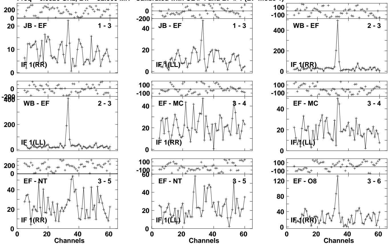
Lower frame: Milli Ampl Jy Top frame: Phas deg Vector averaged cross-power spectrum Several baselines displayed Timerange: 01/06:30:21 to 01/06:32:41
