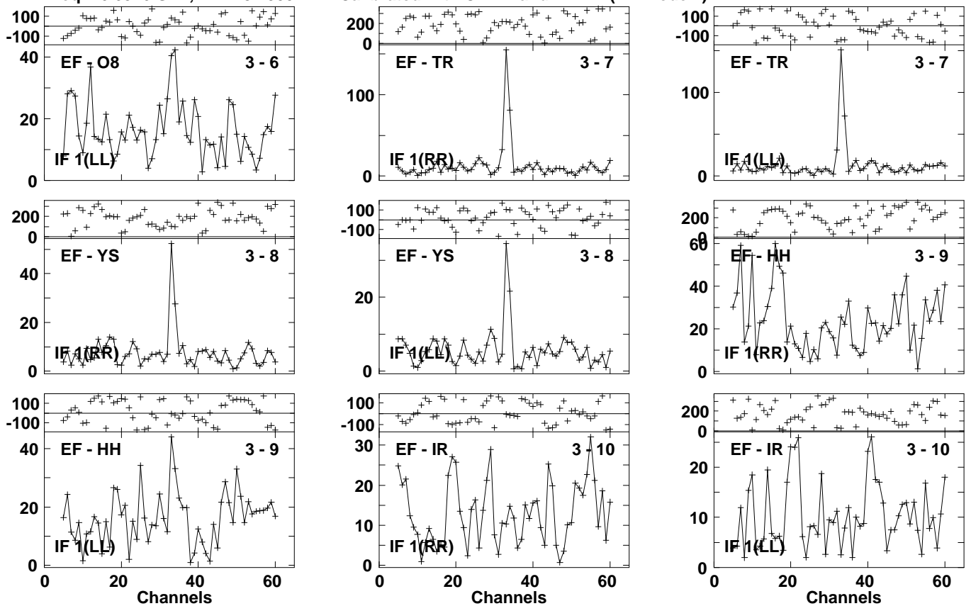
Lower frame: Milli Ampl Jy Top frame: Phas deg Vector averaged cross-power spectrum Several baselines displayed Timerange: 00/23:55:39 to 00/23:57:59
