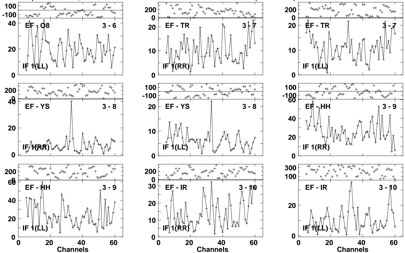
Lower frame: Milli Ampl Jy Top frame: Phas deg Vector averaged cross-power spectrum Several baselines displayed Timerange: 01/05:07:21 to 01/05:09:41
