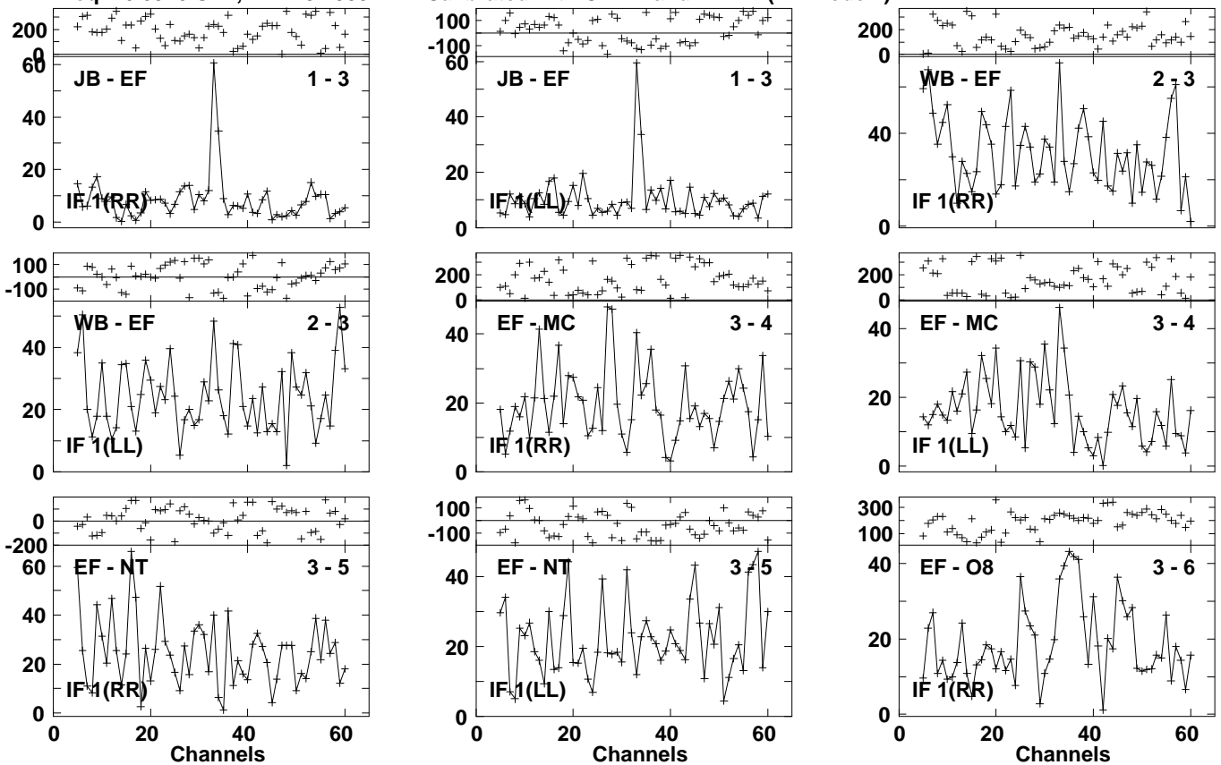
Lower frame: Milli Ampl Jy Top frame: Phas deg Vector averaged cross-power spectrum Several baselines displayed Timerange: 01/03:41:47 to 01/03:44:07
