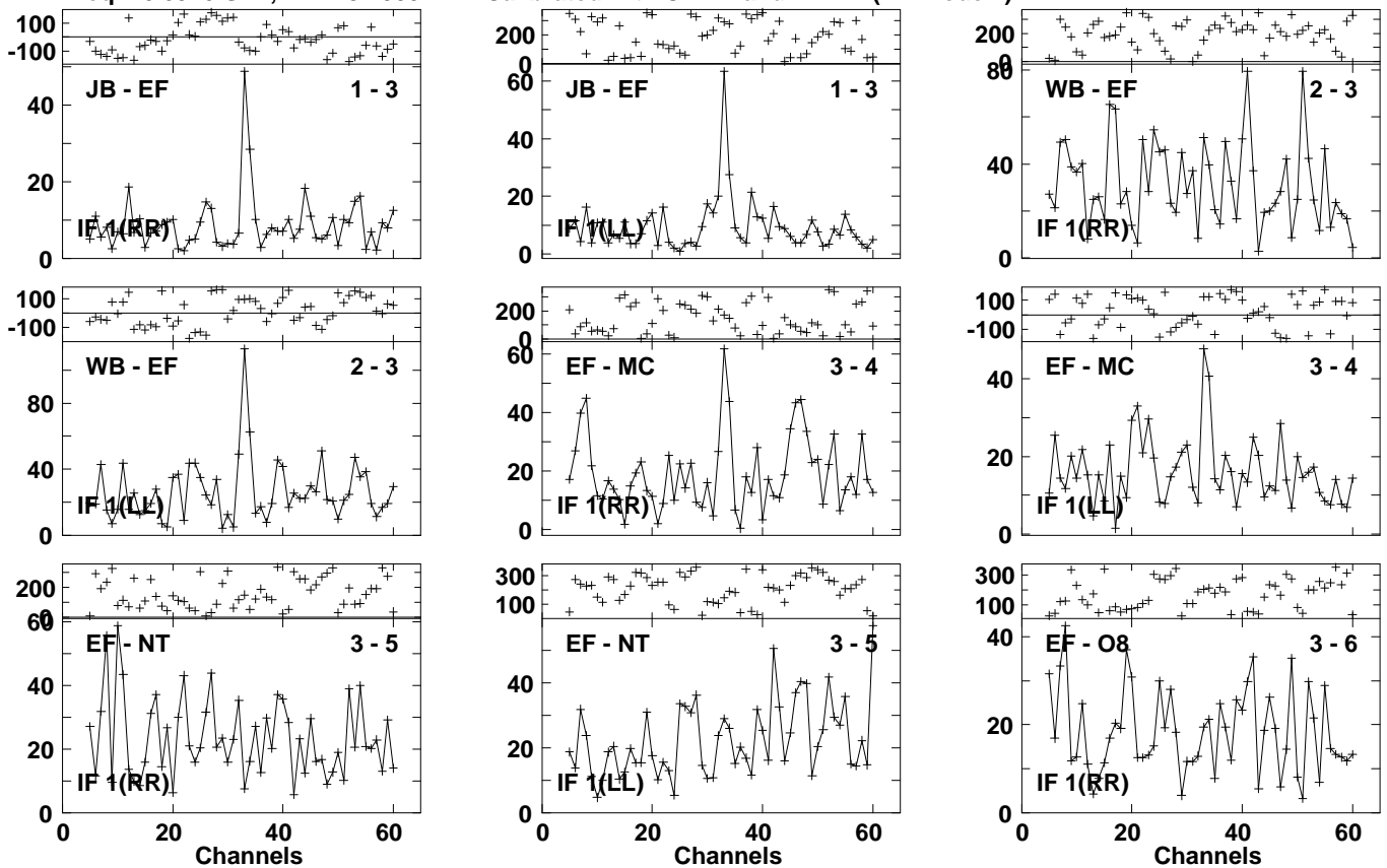
Lower frame: Milli Ampl Jy Top frame: Phas deg Vector averaged cross-power spectrum Several baselines displayed Timerange: 01/01:25:43 to 01/01:28:03
