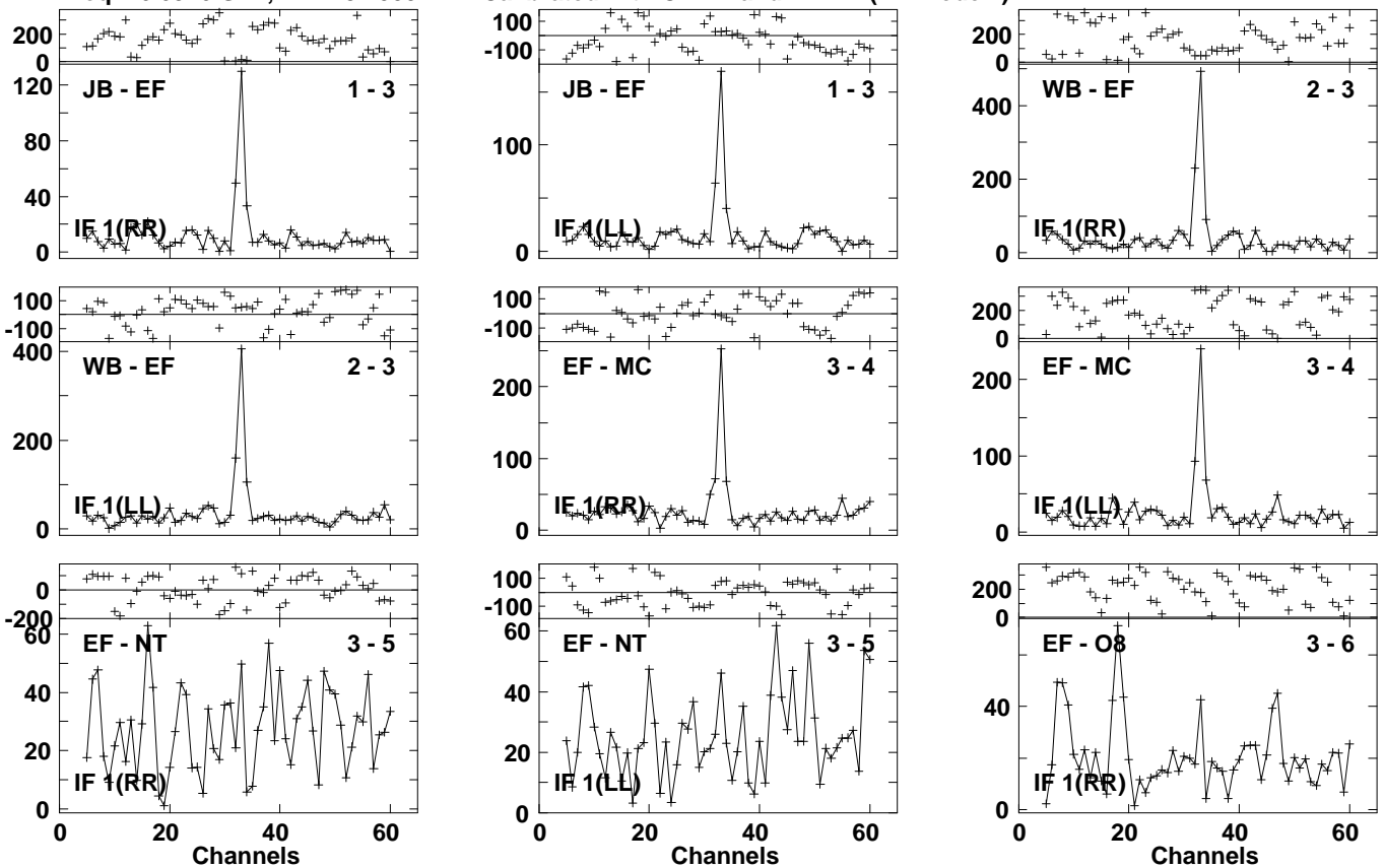
Lower frame: Milli Ampl Jy Top frame: Phas deg Vector averaged cross-power spectrum Several baselines displayed Timerange: 01/02:25:43 to 01/02:28:03
