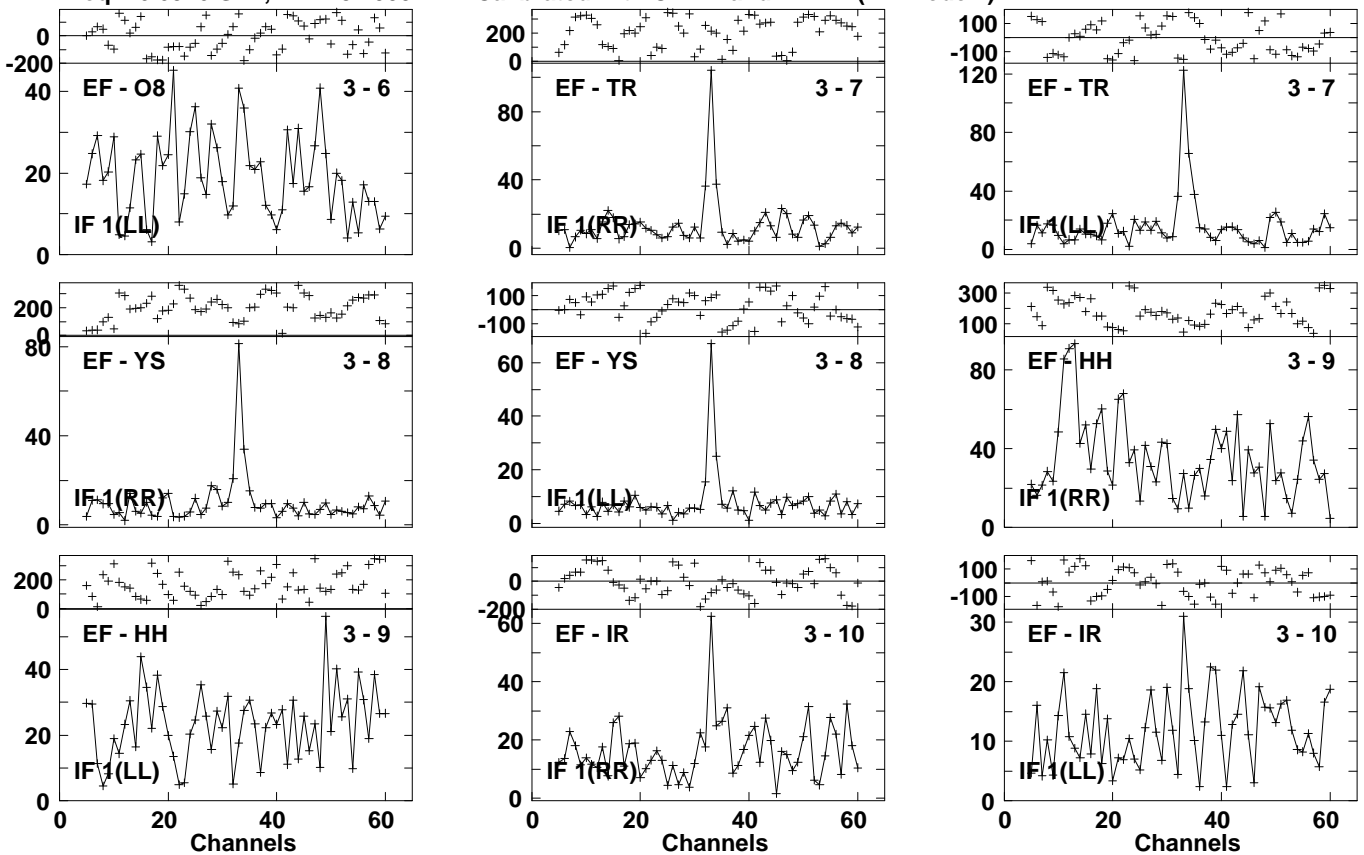
Lower frame: Milli Ampl Jy Top frame: Phas deg Vector averaged cross-power spectrum Several baselines displayed Timerange: 00/23:41:31 to 00/23:43:51
