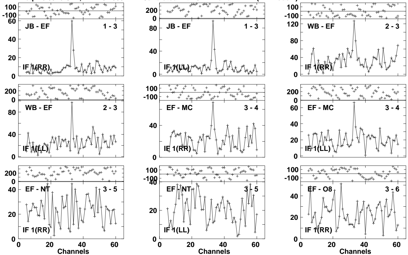
Lower frame: Milli Ampl Jy Top frame: Phas deg Vector averaged cross-power spectrum Several baselines displayed Timerange: 00/23:30:05 to 00/23:32:25
