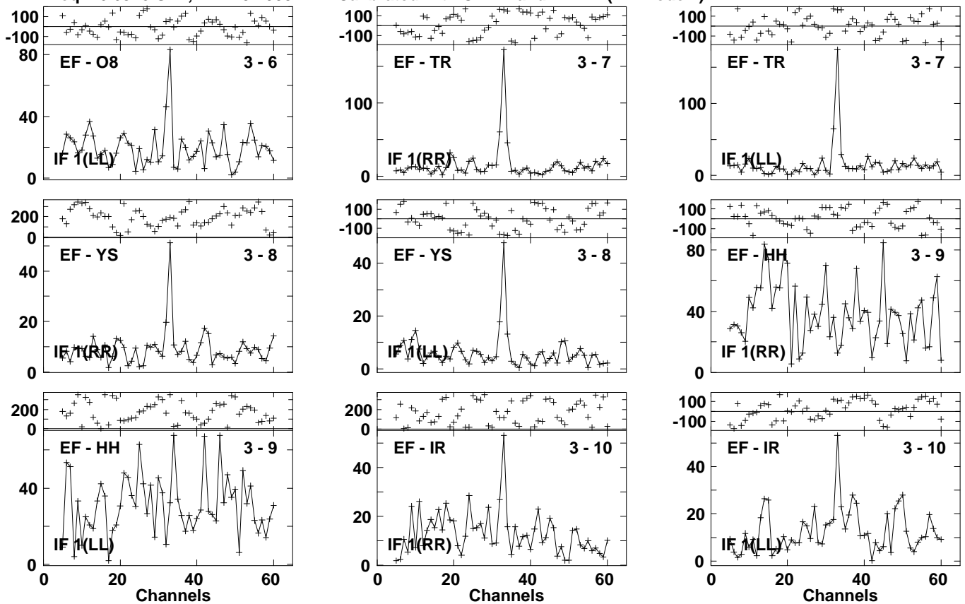
Lower frame: Milli Ampl Jy Top frame: Phas deg Vector averaged cross-power spectrum Several baselines displayed Timerange: 01/00:30:05 to 01/00:32:25
