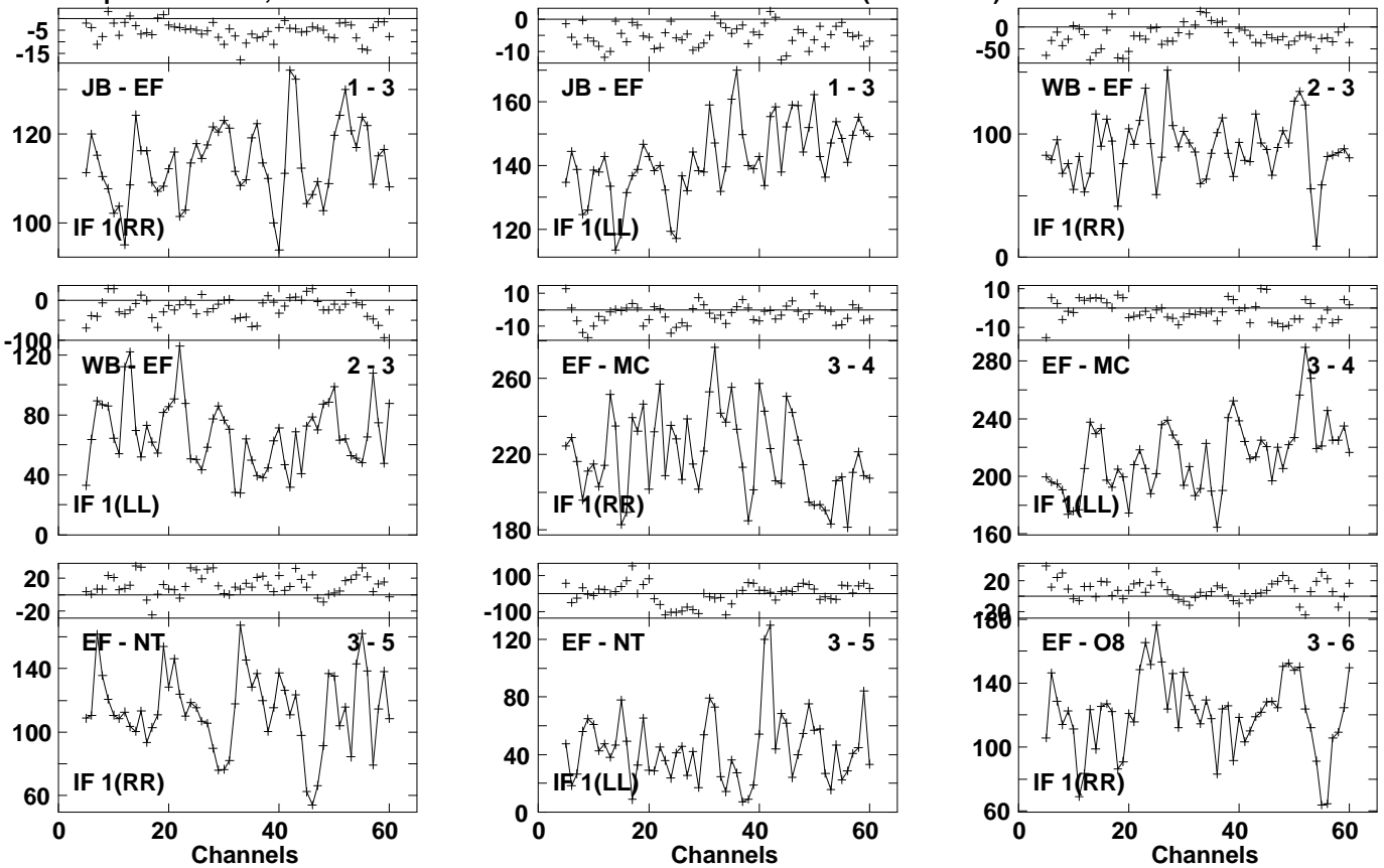
Lower frame: Milli Ampl Jy Top frame: Phas deg Vector averaged cross-power spectrum Several baselines displayed Timerange: 01/05:28:31 to 01/05:30:09
