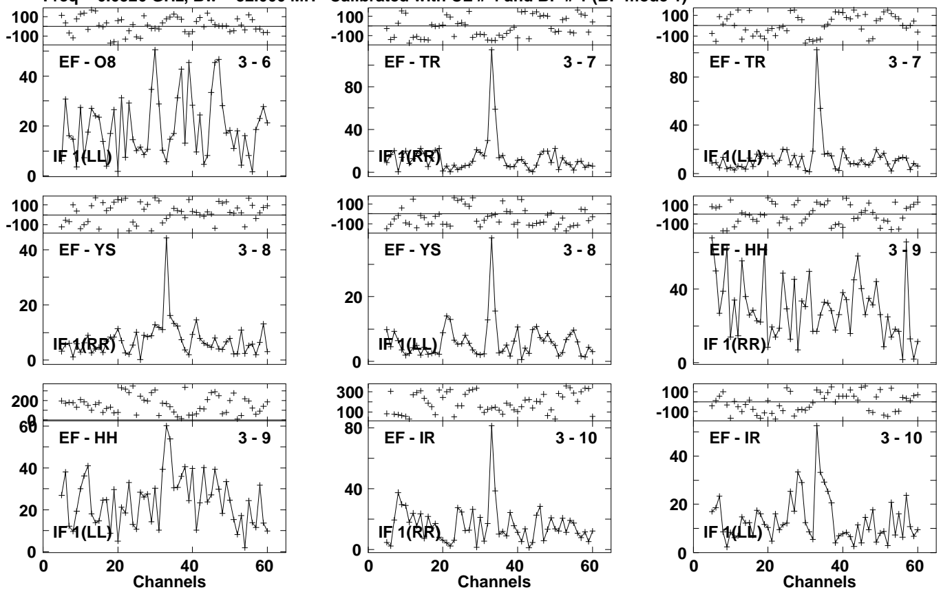
Lower frame: Milli Ampl Jy Top frame: Phas deg Vector averaged cross-power spectrum Several baselines displayed Timerange: 01/05:21:29 to 01/05:23:57
