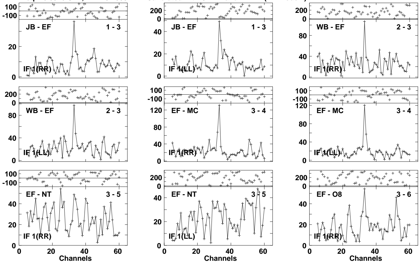
Lower frame: Milli Ampl Jy Top frame: Phas deg Vector averaged cross-power spectrum Several baselines displayed Timerange: 00/23:09:47 to 00/23:12:15
