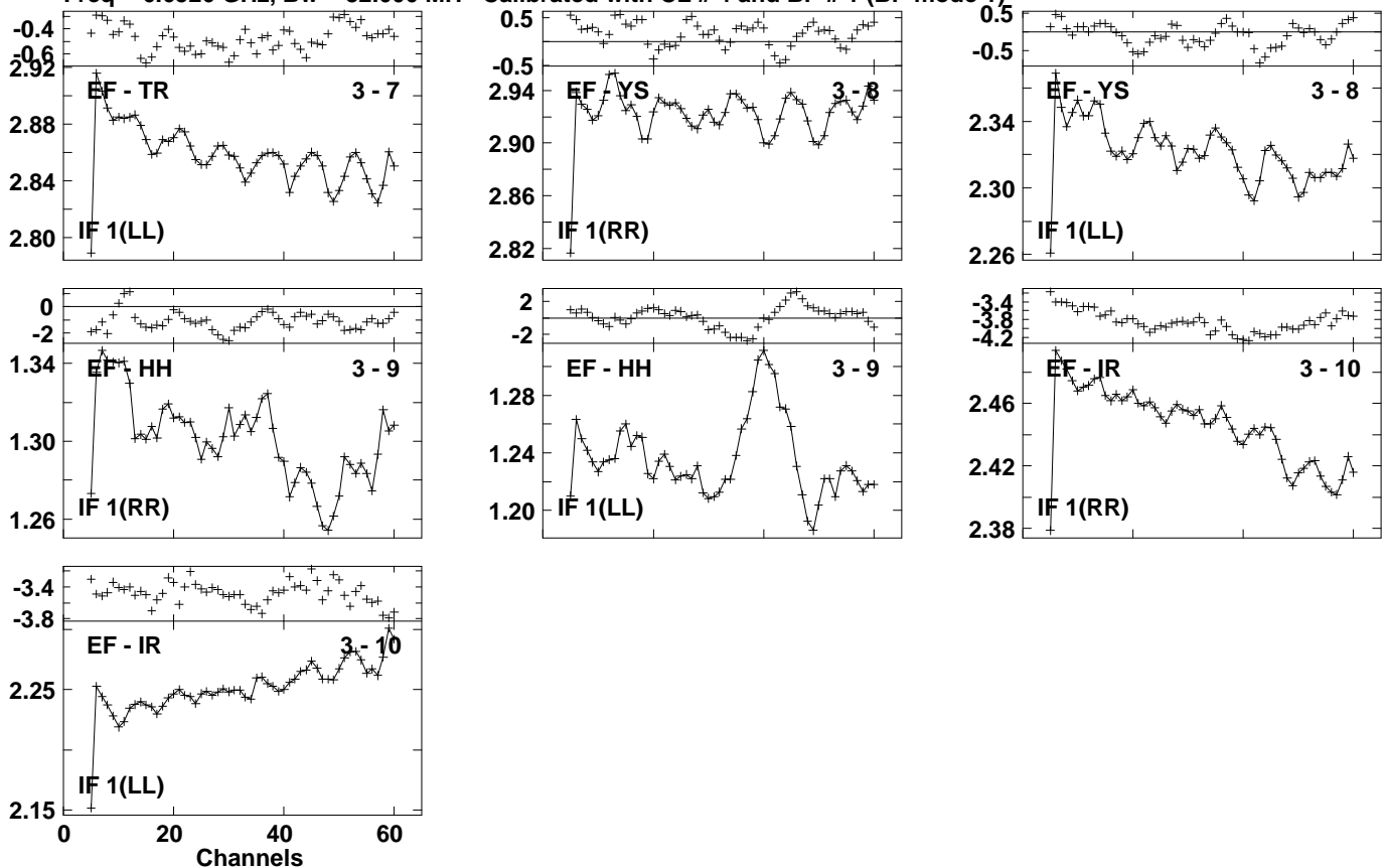
Lower frame: Ampl Jy Top frame: Phas deg Vector averaged cross-power spectrum Several baselines displayed Timerange: 01/02:00:01 to 01/02:07:09
