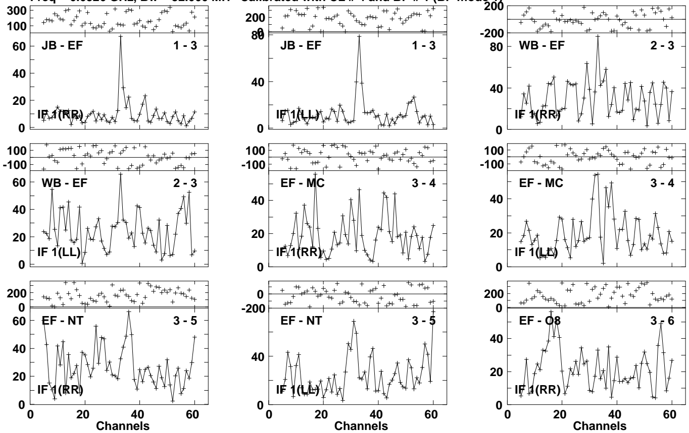
Lower frame: Milli Ampl Jy Top frame: Phas deg Vector averaged cross-power spectrum Several baselines displayed Timerange: 00/23:52:57 to 00/23:55:17
