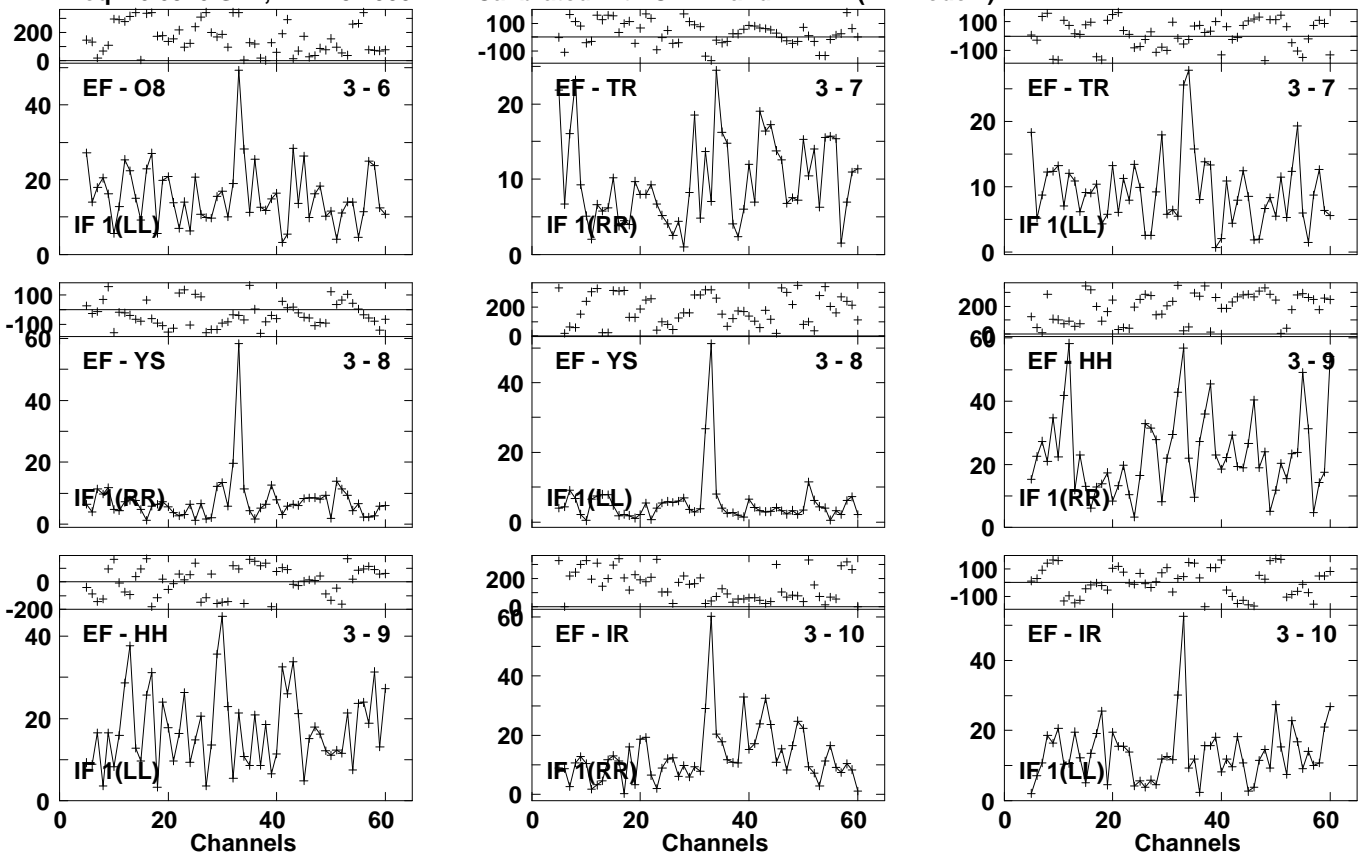
Lower frame: Milli Ampl Jy Top frame: Phas deg Vector averaged cross-power spectrum Several baselines displayed Timerange: 01/00:21:21 to 01/00:23:41
