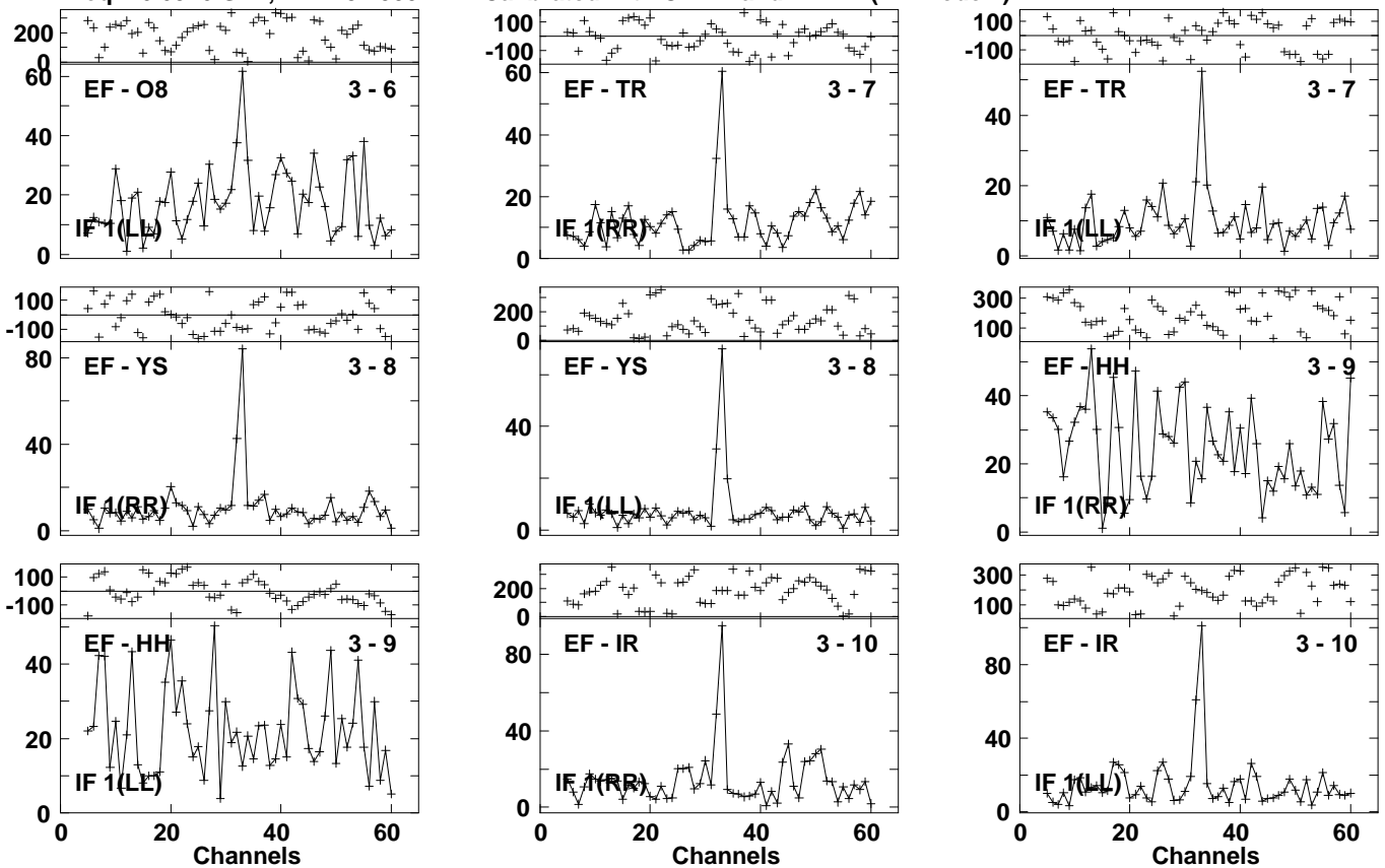
Lower frame: Milli Ampl Jy Top frame: Phas deg Vector averaged cross-power spectrum Several baselines displayed Timerange: 01/00:18:39 to 01/00:20:59
