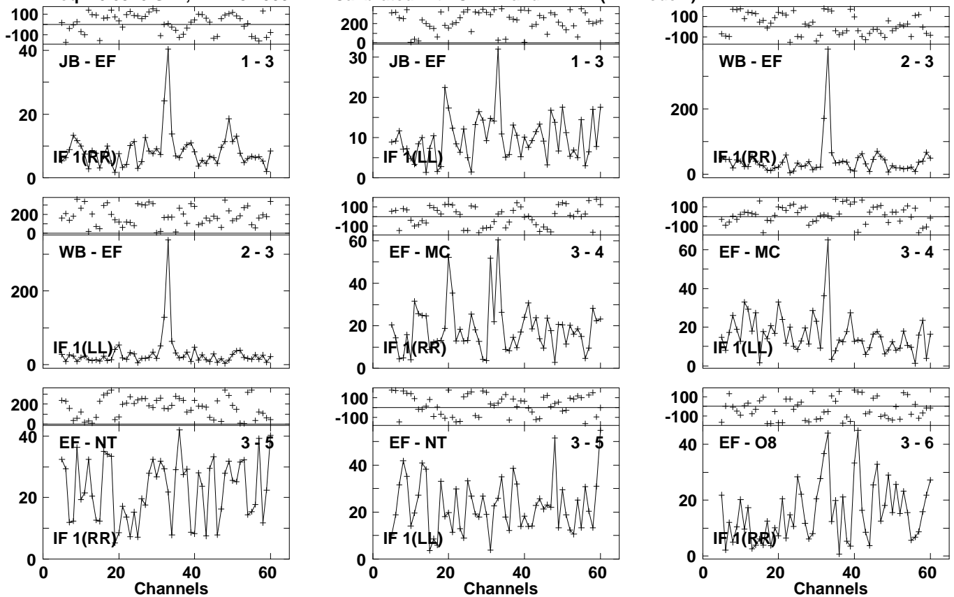
Lower frame: Milli Ampl Jy Top frame: Phas deg Vector averaged cross-power spectrum Several baselines displayed Timerange: 01/00:48:35 to 01/00:50:55
