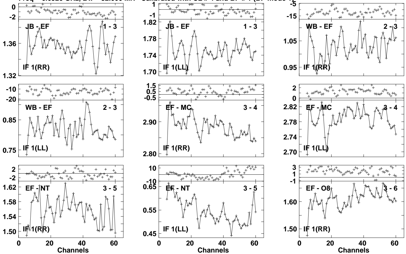
Lower frame: Ampl Jy Top frame: Phas deg Vector averaged cross-power spectrum Several baselines displayed Timerange: 01/04:19:23 to 01/04:19:51
