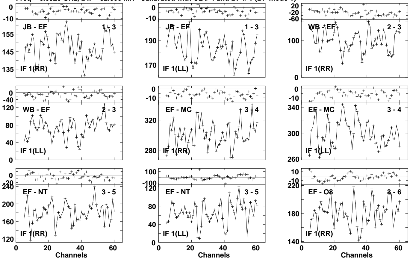
Lower frame: Milli Ampl Jy Top frame: Phas deg Vector averaged cross-power spectrum Several baselines displayed Timerange: 01/00:35:19 to 01/00:36:57
