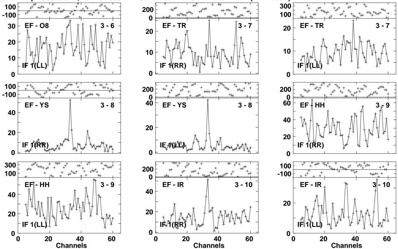
Lower frame: Milli Ampl Jy Top frame: Phas deg Vector averaged cross-power spectrum Several baselines displayed Timerange: 01/05:44:29 to 01/05:46:49
