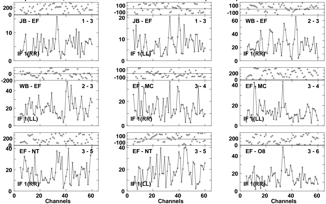
Lower frame: Milli Ampl Jy Top frame: Phas deg Vector averaged cross-power spectrum Several baselines displayed Timerange: 01/03:55:55 to 01/03:58:15
