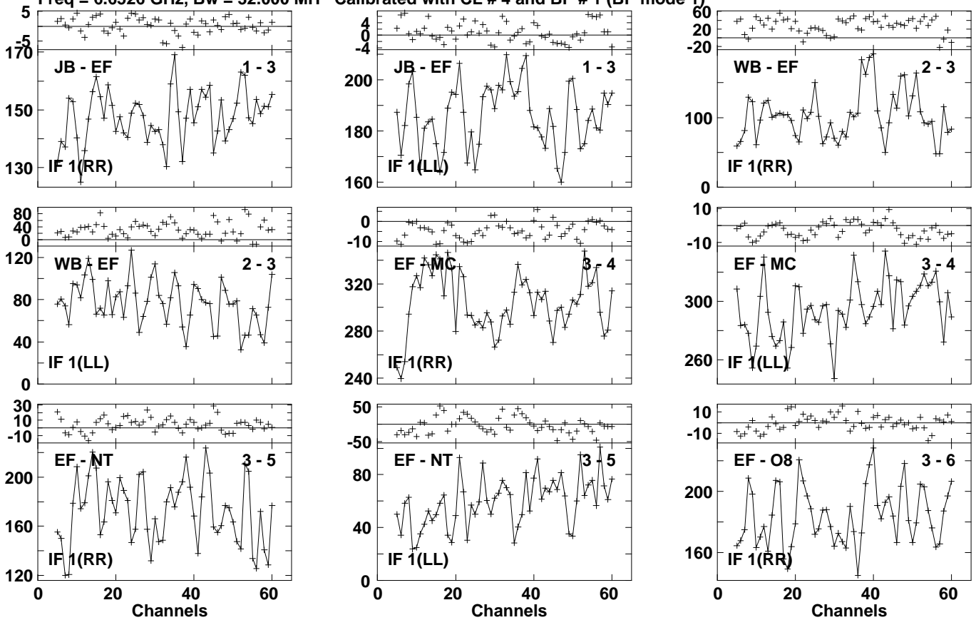
Lower frame: Milli Ampl Jy Top frame: Phas deg Vector averaged cross-power spectrum Several baselines displayed Timerange: 01/00:46:45 to 01/00:48:23
