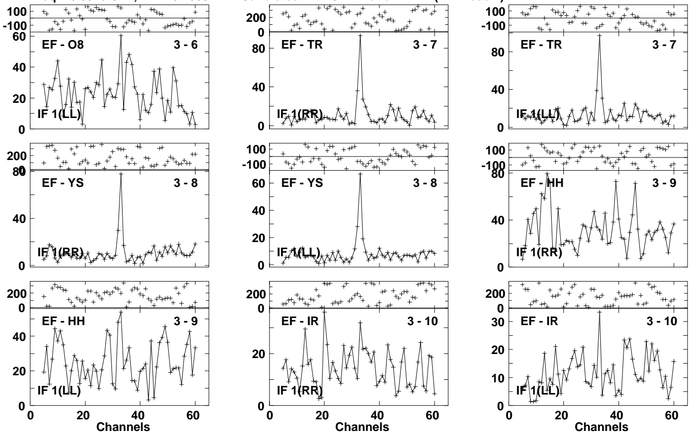
Lower frame: Milli Ampl Jy Top frame: Phas deg Vector averaged cross-power spectrum Several baselines displayed Timerange: 01/00:41:31 to 01/00:43:51
