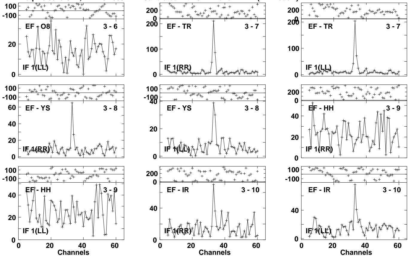
Lower frame: Milli Ampl Jy Top frame: Phas deg Vector averaged cross-power spectrum Several baselines displayed Timerange: 01/04:04:39 to 01/04:06:59
