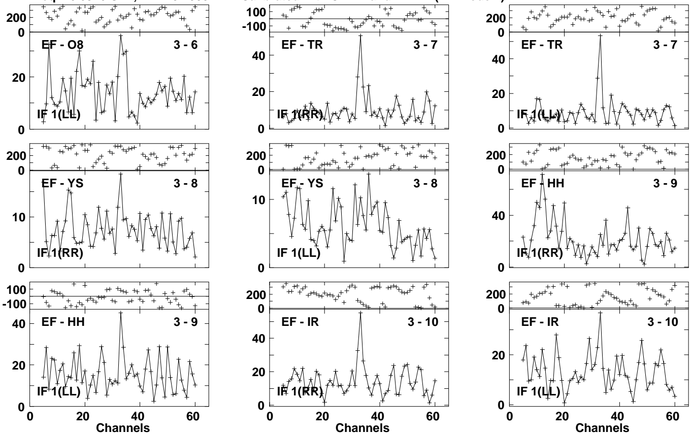
Lower frame: Milli Ampl Jy Top frame: Phas deg Vector averaged cross-power spectrum Several baselines displayed Timerange: 01/02:21:21 to 01/02:23:41
