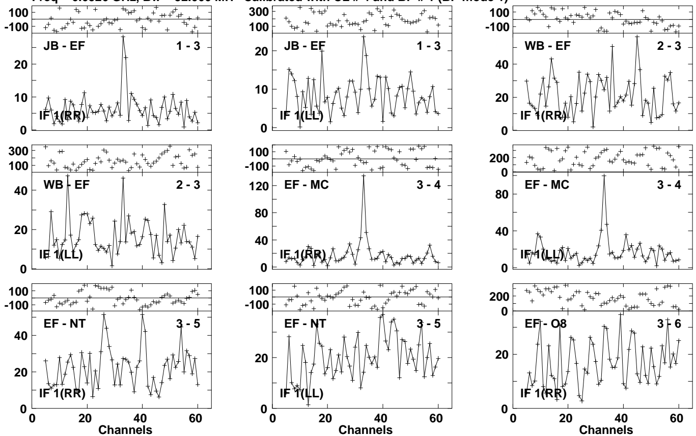
Lower frame: Milli Ampl Jy Top frame: Phas deg Vector averaged cross-power spectrum Several baselines displayed Timerange: 01/01:55:39 to 01/01:57:59
