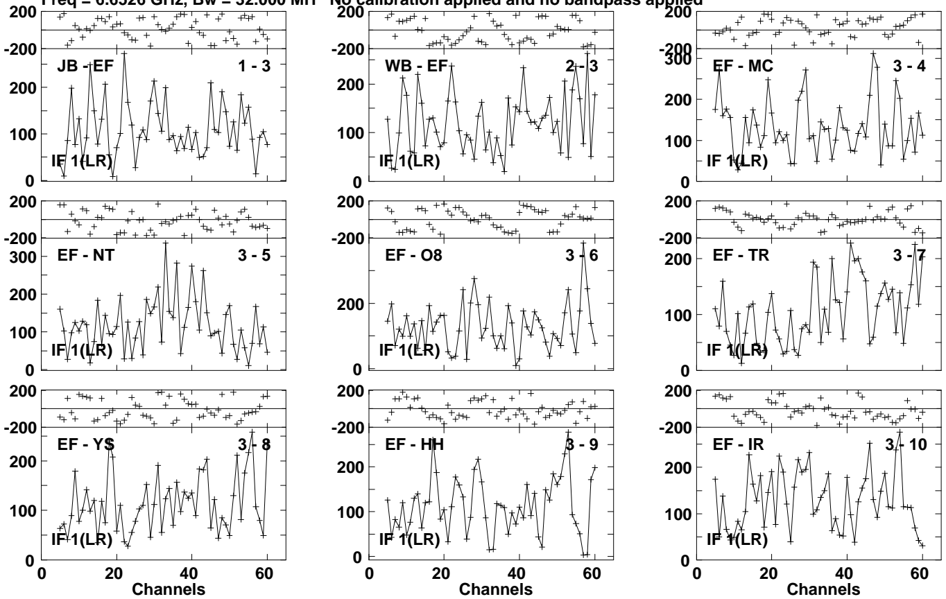
Lower frame: Micro Ampl Jy Top frame: Phas deg Vector averaged cross-power spectrum Several baselines displayed Timerange: 01/01:55:39 to 01/01:57:59
