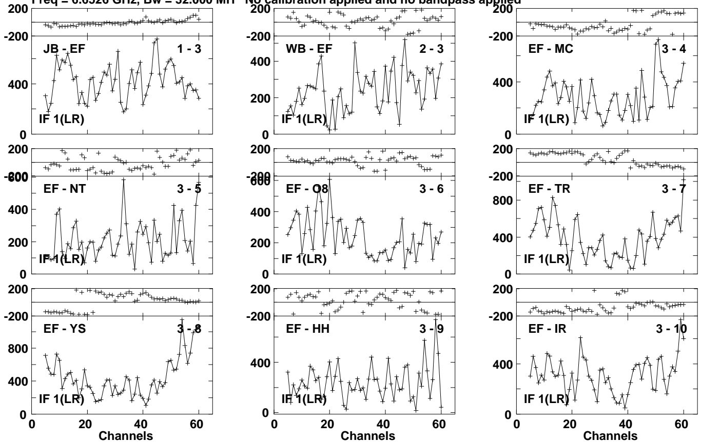
Lower frame: Micro Ampl Jy Top frame: Phas deg Vector averaged cross-power spectrum Several baselines displayed Timerange: 01/04:02:49 to 01/04:04:27
