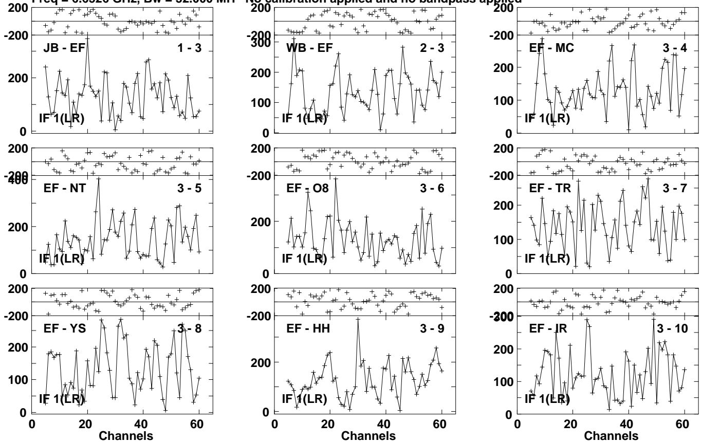
Lower frame: Micro Ampl Jy Top frame: Phas deg Vector averaged cross-power spectrum Several baselines displayed Timerange: 01/06:04:39 to 01/06:06:59
