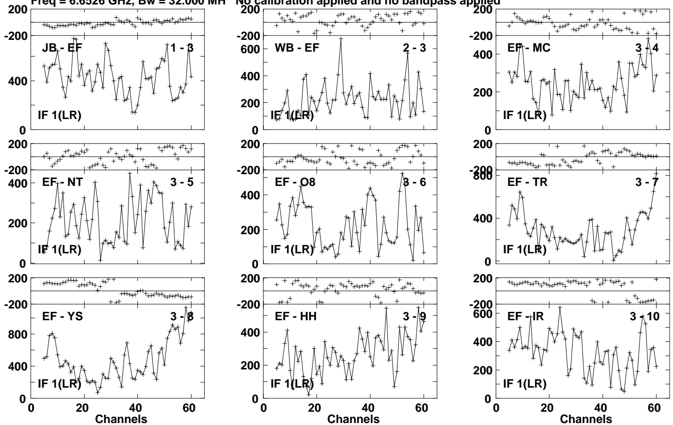
Lower frame: Micro Ampl Jy Top frame: Phas deg Vector averaged cross-power spectrum Several baselines displayed Timerange: 00/23:23:53 to 00/23:25:31
