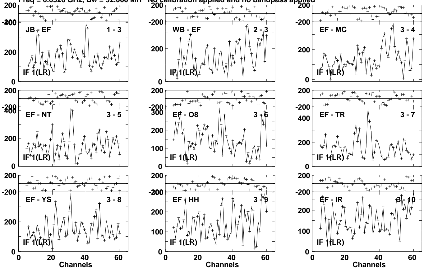
Lower frame: Micro Ampl Jy Top frame: Phas deg Vector averaged cross-power spectrum Several baselines displayed Timerange: 00/23:14:17 to 00/23:16:37
