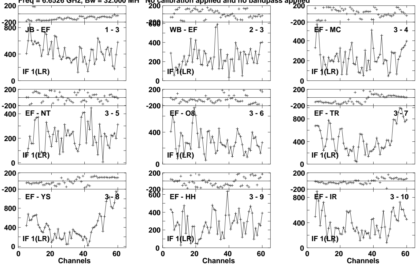
Lower frame: Micro Ampl Jy Top frame: Phas deg Vector averaged cross-power spectrum Several baselines displayed Timerange: 00/23:39:41 to 00/23:41:19
