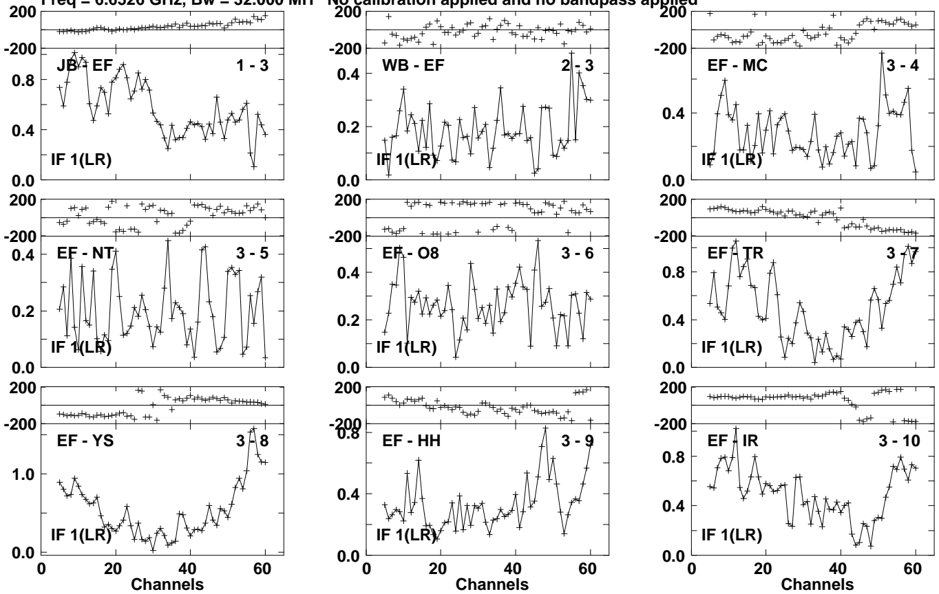
Lower frame: Milli Ampl Jy Top frame: Phas deg Vector averaged cross-power spectrum Several baselines displayed Timerange: 01/00:39:41 to 01/00:41:19
