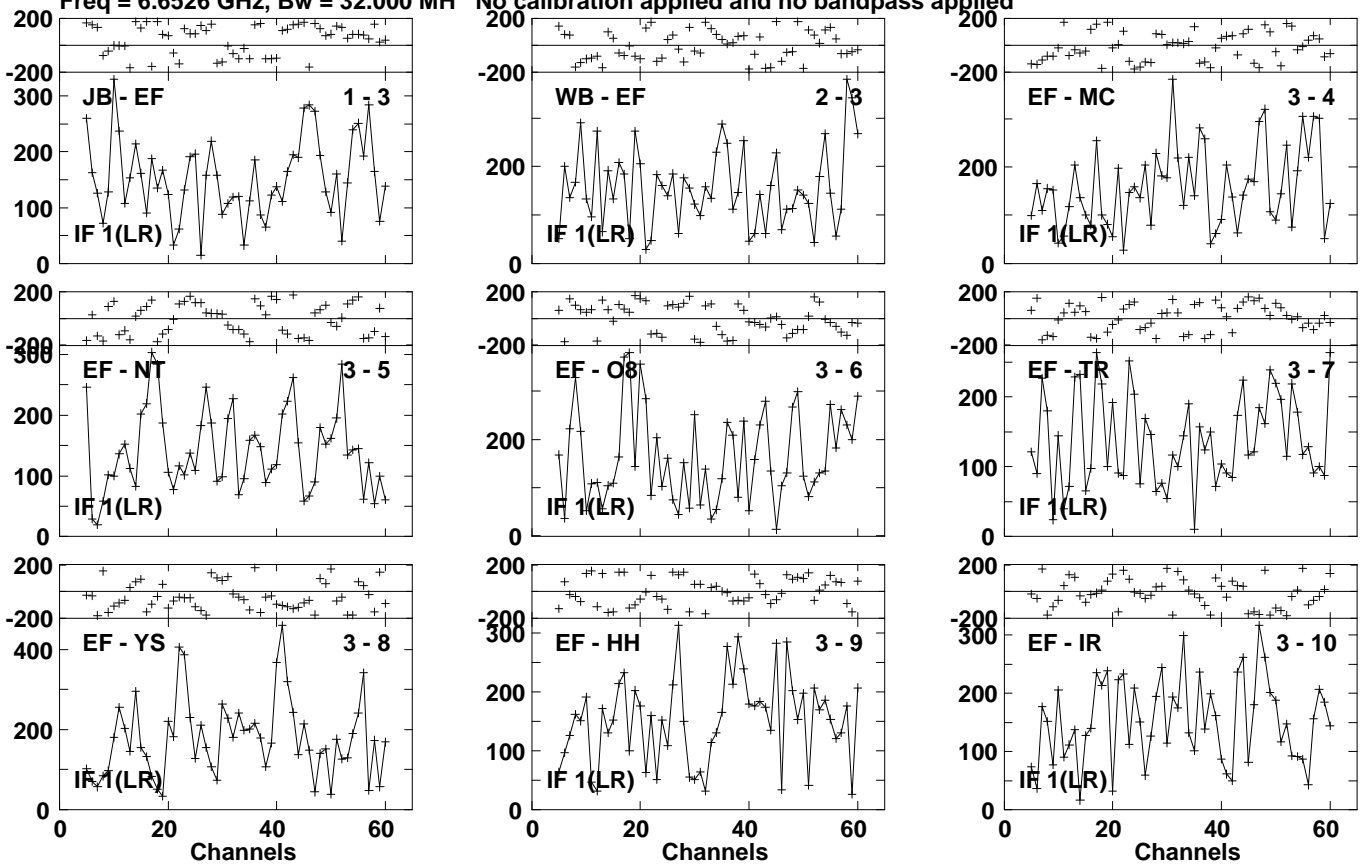
Lower frame: Micro Ampl Jy Top frame: Phas deg Vector averaged cross-power spectrum Several baselines displayed Timerange: 00/23:25:43 to 00/23:28:03
