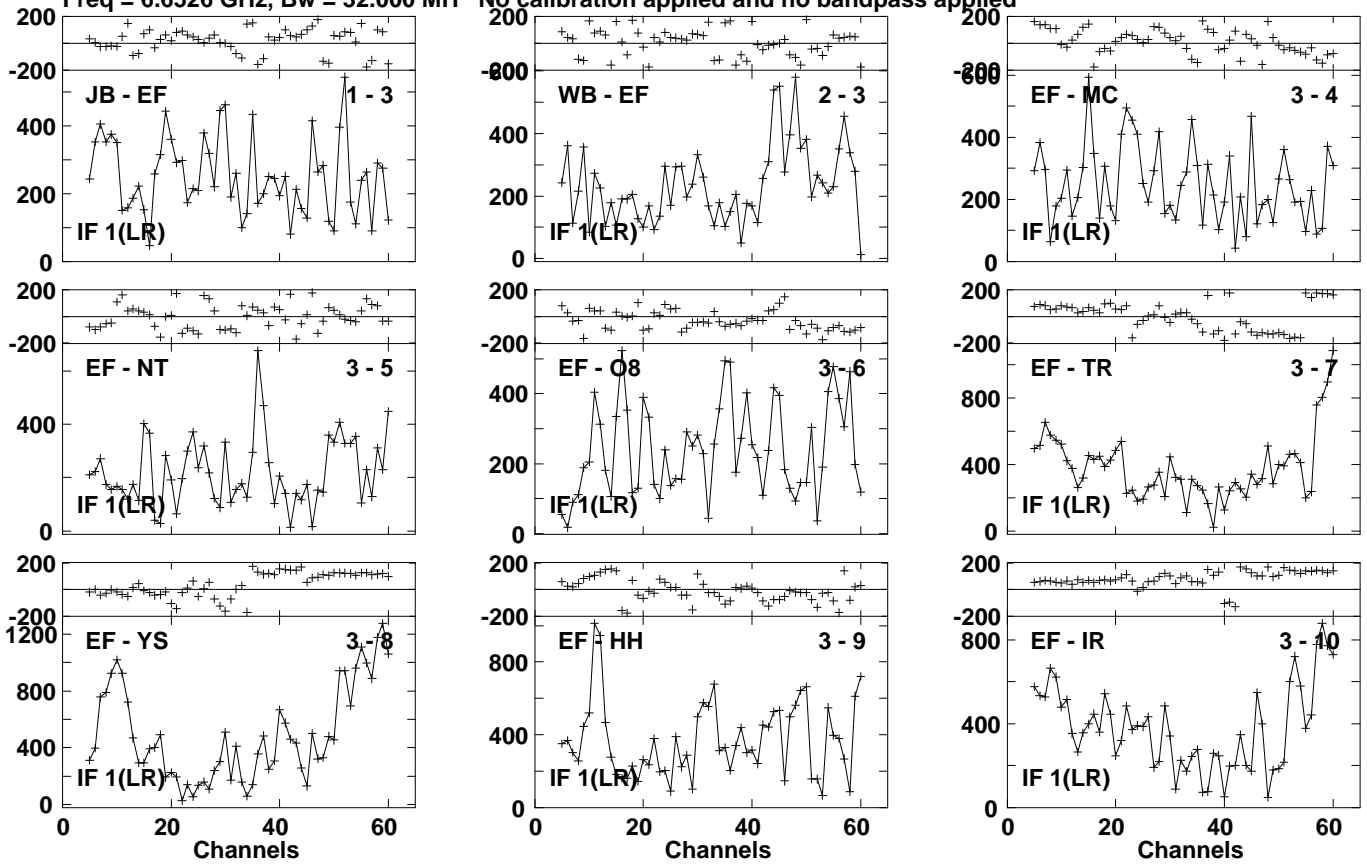
Lower frame: Micro Ampl Jy Top frame: Phas deg Vector averaged cross-power spectrum Several baselines displayed Timerange: 00/23:46:45 to 00/23:48:23
