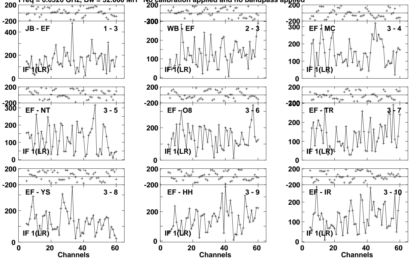
Lower frame: Micro Ampl Jy Top frame: Phas deg Vector averaged cross-power spectrum Several baselines displayed Timerange: 01/04:21:29 to 01/04:23:57
