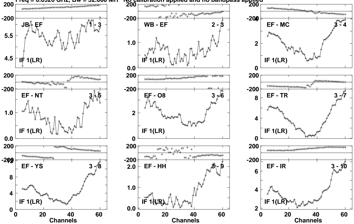
Lower frame: Milli Ampl Jy Top frame: Phas deg Vector averaged cross-power spectrum Several baselines displayed Timerange: 01/04:19:23 to 01/04:19:51
