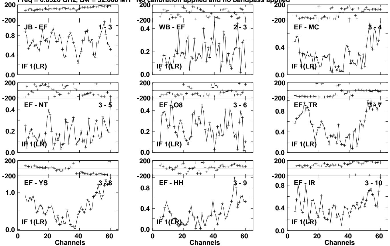
Lower frame: Milli Ampl Jy Top frame: Phas deg Vector averaged cross-power spectrum Several baselines displayed Timerange: 01/04:58:27 to 01/05:00:05
