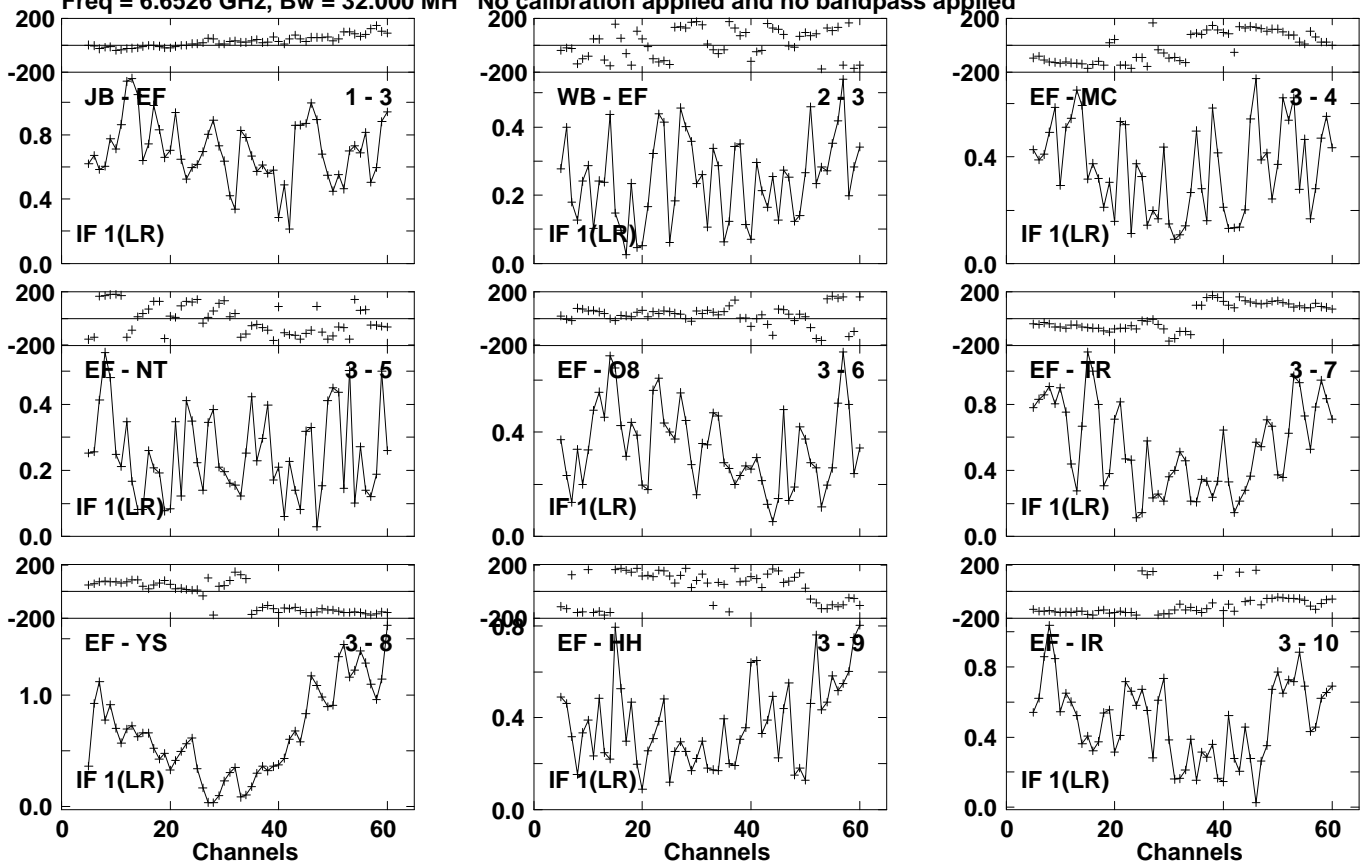
Lower frame: Milli Ampl Jy Top frame: Phas deg Vector averaged cross-power spectrum Several baselines displayed Timerange: 01/02:39:41 to 01/02:41:19
