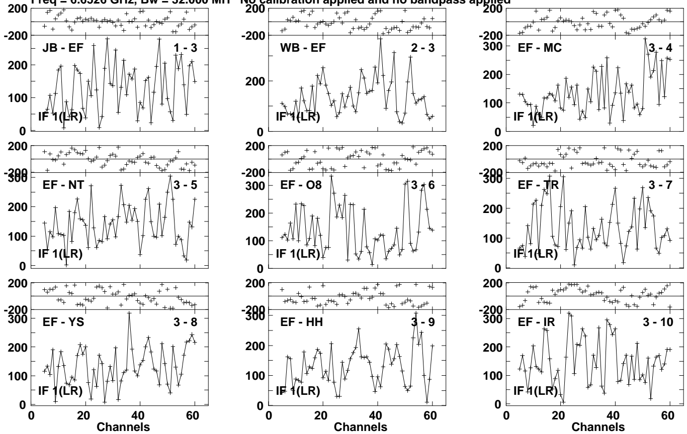
Lower frame: Micro Ampl Jy Top frame: Phas deg Vector averaged cross-power spectrum Several baselines displayed Timerange: 01/05:21:29 to 01/05:23:57
