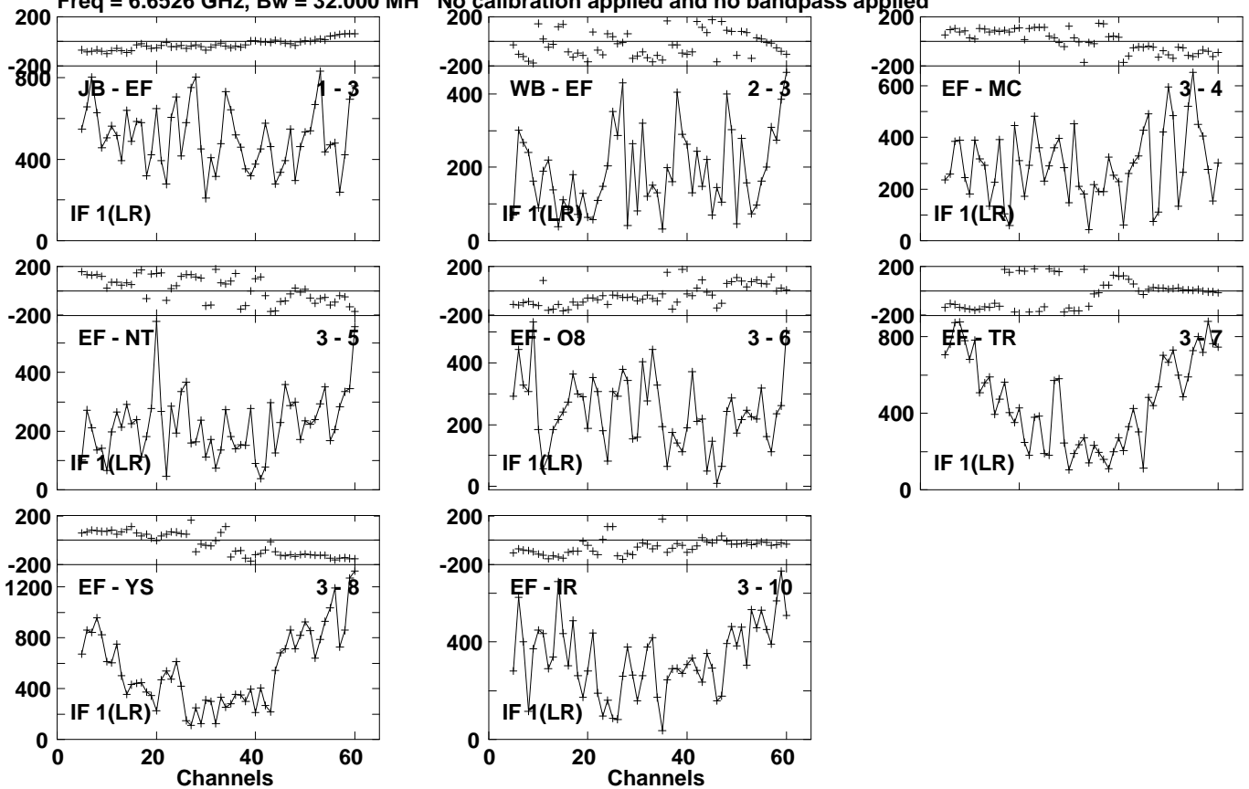
Lower frame: Micro Ampl Jy Top frame: Phas deg Vector averaged cross-power spectrum Several baselines displayed Timerange: 01/06:28:31 to 01/06:30:09
