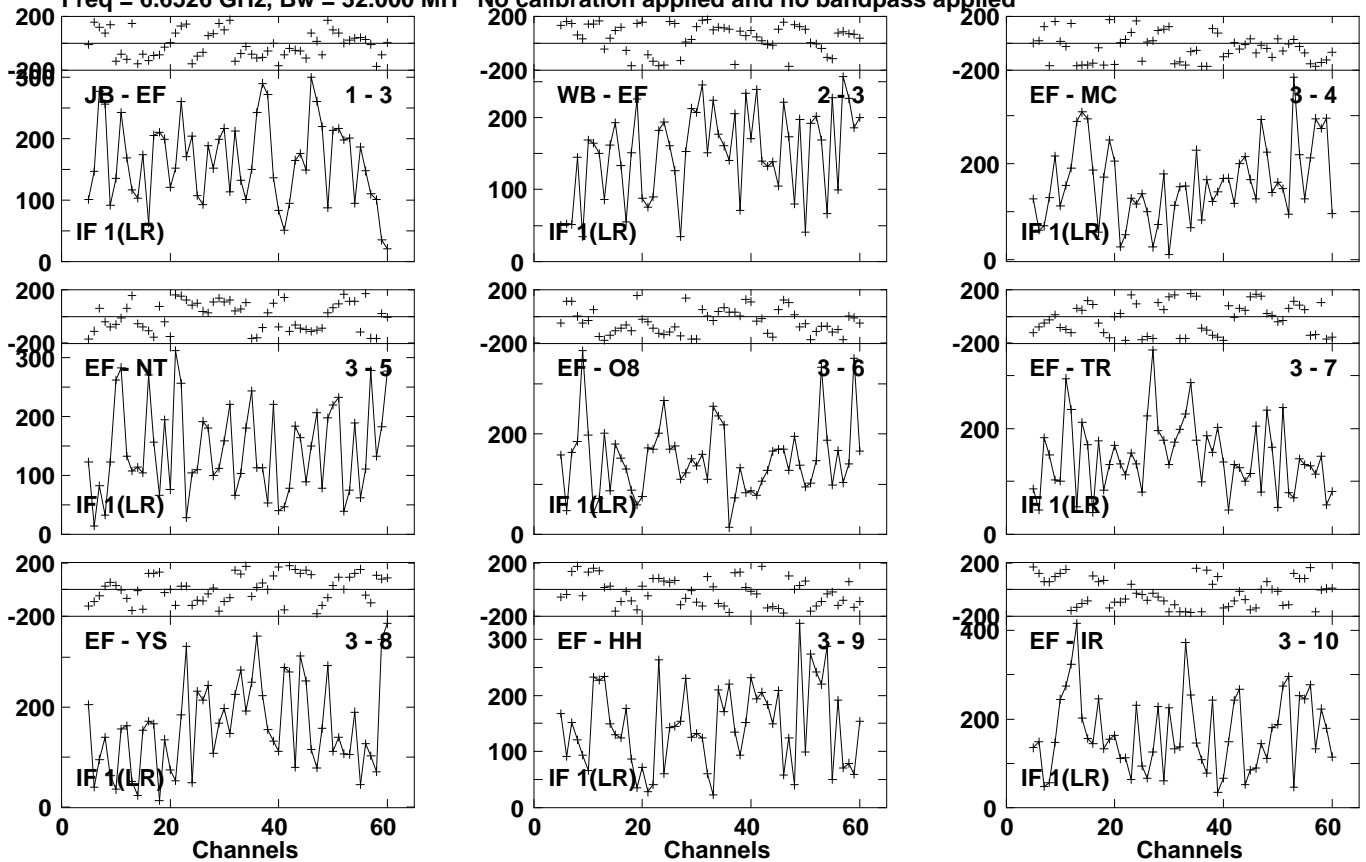
Lower frame: Micro Ampl Jy Top frame: Phas deg Vector averaged cross-power spectrum Several baselines displayed Timerange: 01/02:14:17 to 01/02:16:37
