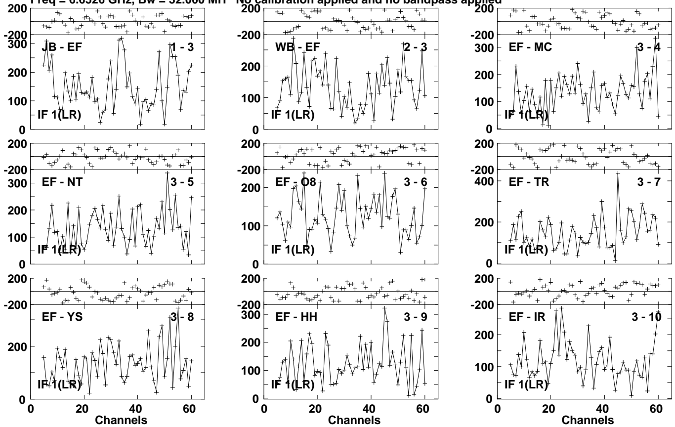
Lower frame: Micro Ampl Jy Top frame: Phas deg Vector averaged cross-power spectrum Several baselines displayed Timerange: 01/05:41:47 to 01/05:44:07
