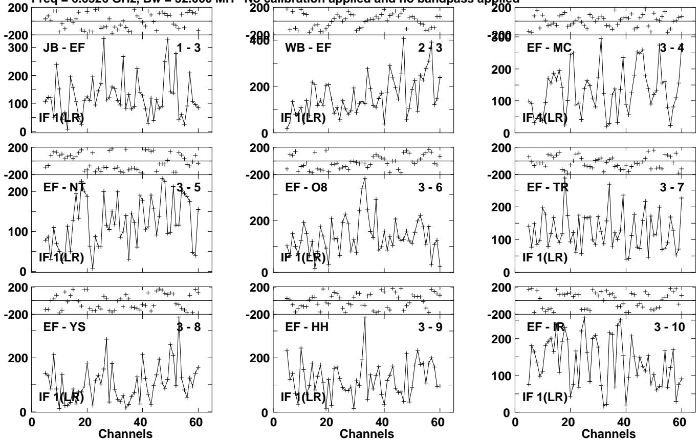
Lower frame: Micro Ampl Jy Top frame: Phas deg Vector averaged cross-power spectrum Several baselines displayed Timerange: 01/00:09:47 to 01/00:12:15
