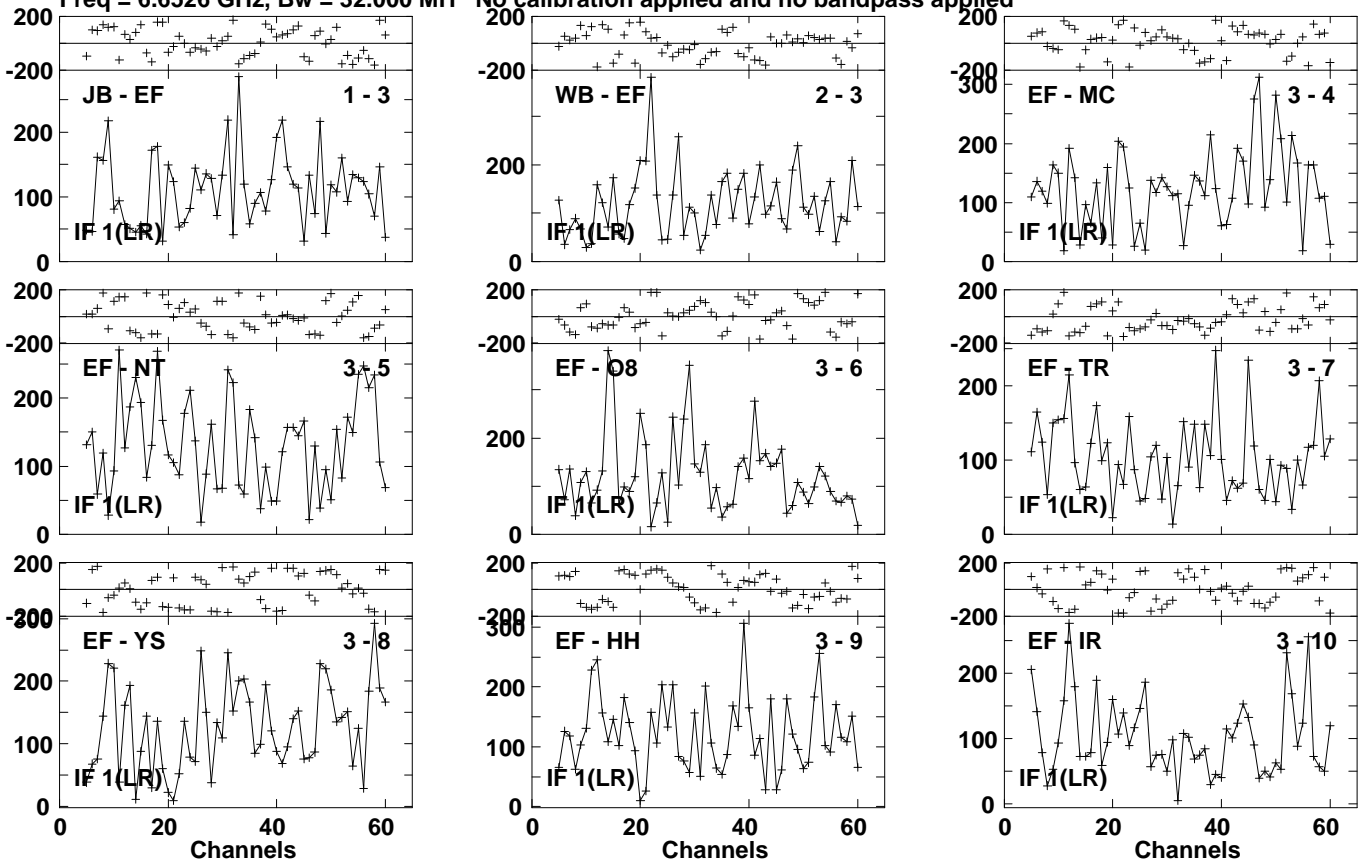
Lower frame: Micro Ampl Jy Top frame: Phas deg Vector averaged cross-power spectrum Several baselines displayed Timerange: 01/04:07:21 to 01/04:09:41
