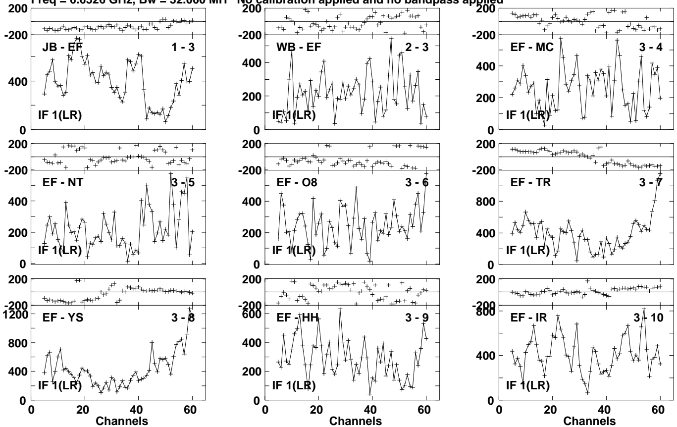
Lower frame: Micro Ampl Jy Top frame: Phas deg Vector averaged cross-power spectrum Several baselines displayed Timerange: 00/23:35:19 to 00/23:36:57
