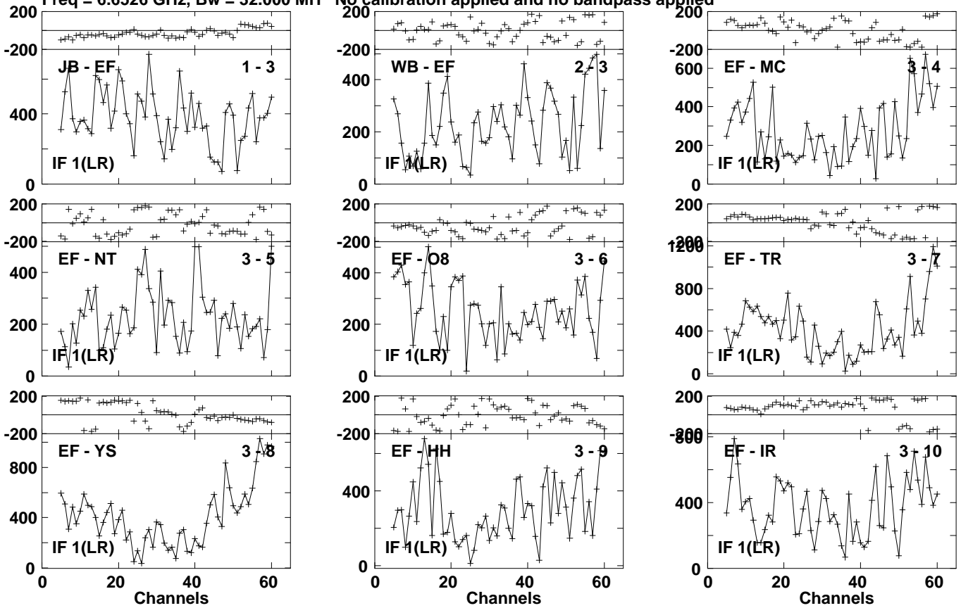
Lower frame: Micro Ampl Jy Top frame: Phas deg Vector averaged cross-power spectrum Several baselines displayed Timerange: 00/23:28:15 to 00/23:29:53
