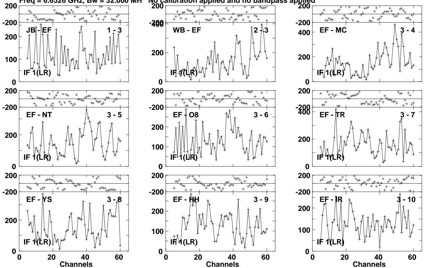
Lower frame: Micro Ampl Jy Top frame: Phas deg Vector averaged cross-power spectrum Several baselines displayed Timerange: 01/04:00:17 to 01/04:02:37
