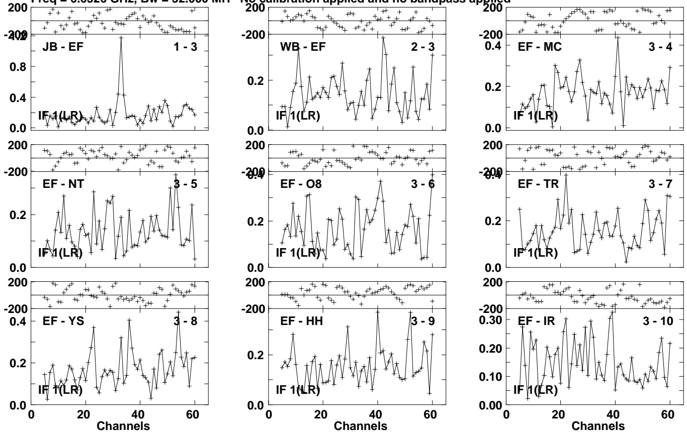
Lower frame: Milli Ampl Jy Top frame: Phas deg Vector averaged cross-power spectrum Several baselines displayed Timerange: 01/02:37:09 to 01/02:39:29
