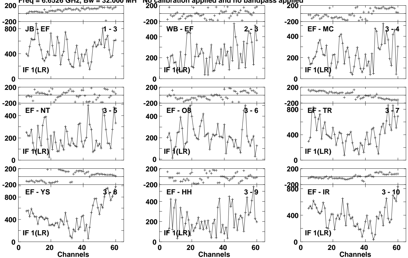
Lower frame: Micro Ampl Jy Top frame: Phas deg Vector averaged cross-power spectrum Several baselines displayed Timerange: 01/03:35:35 to 01/03:37:13
