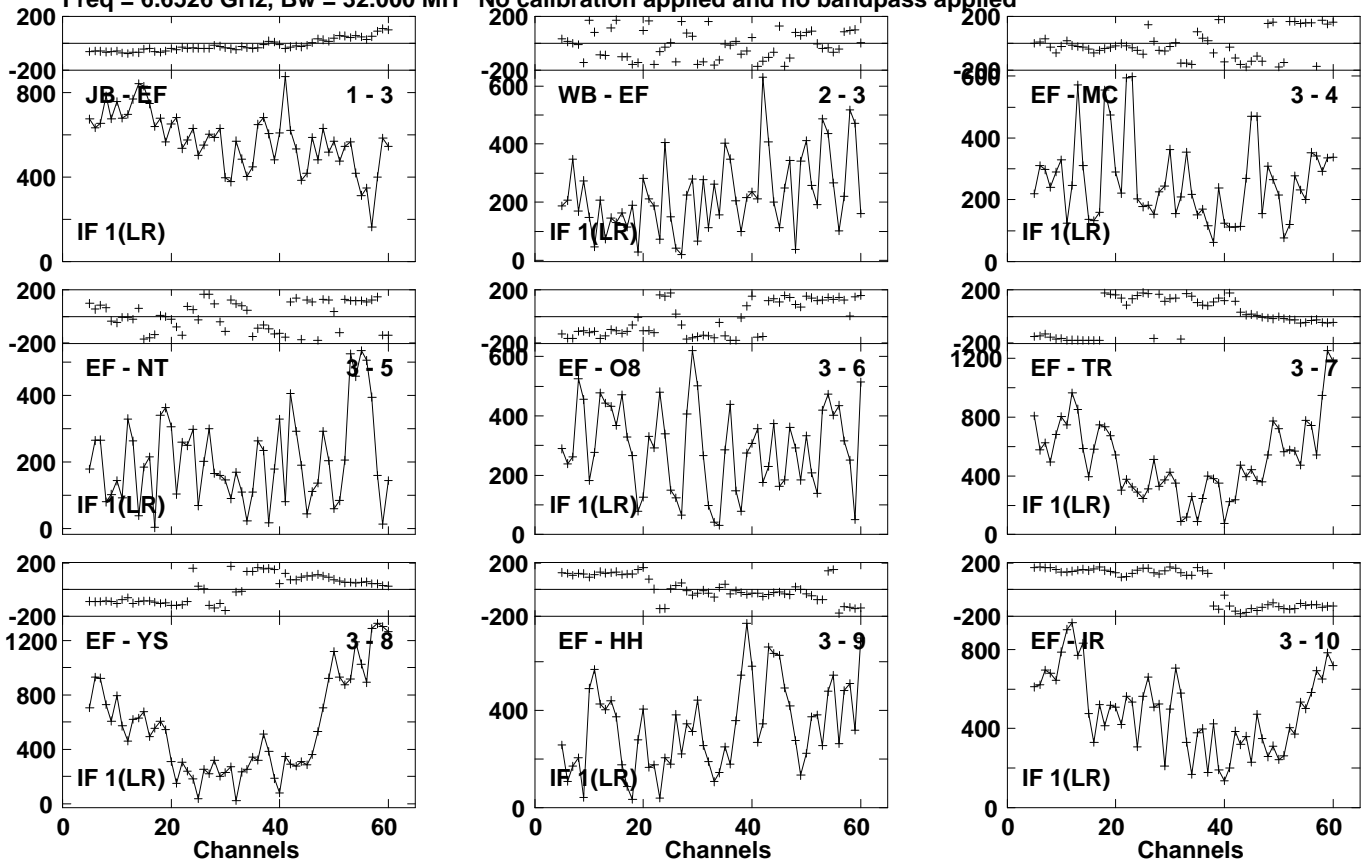
Lower frame: Micro Ampl Jy Top frame: Phas deg Vector averaged cross-power spectrum Several baselines displayed Timerange: 01/00:46:45 to 01/00:48:23
