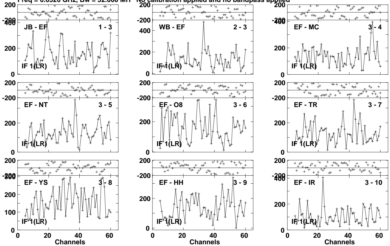
Lower frame: Micro Ampl Jy Top frame: Phas deg Vector averaged cross-power spectrum Several baselines displayed Timerange: 01/00:18:39 to 01/00:20:59
