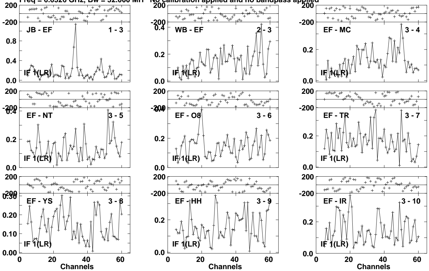
Lower frame: Milli Ampl Jy Top frame: Phas deg Vector averaged cross-power spectrum Several baselines displayed Timerange: 01/02:52:57 to 01/02:55:17
