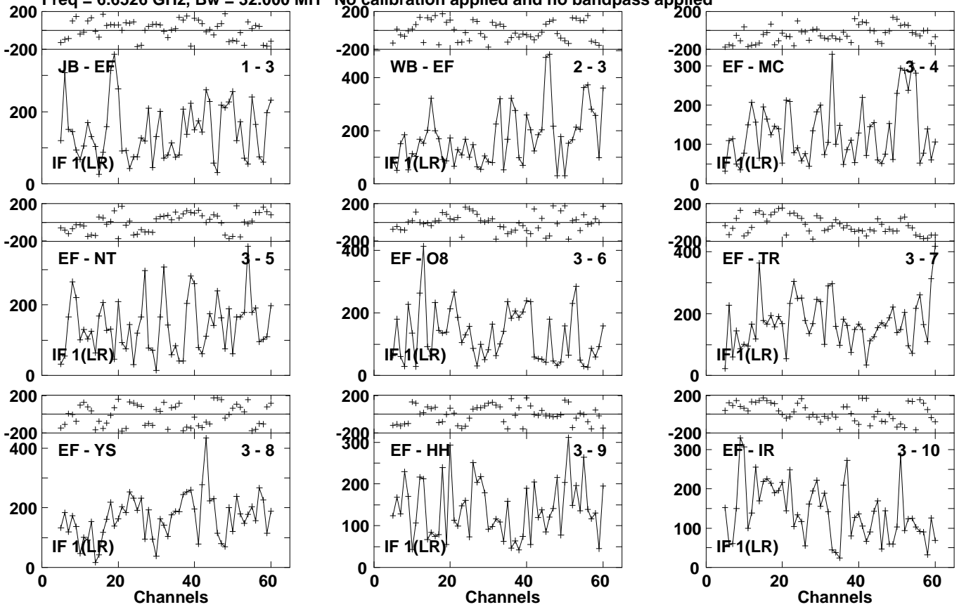
Lower frame: Micro Ampl Jy Top frame: Phas deg Vector averaged cross-power spectrum Several baselines displayed Timerange: 01/04:37:25 to 01/04:39:45
