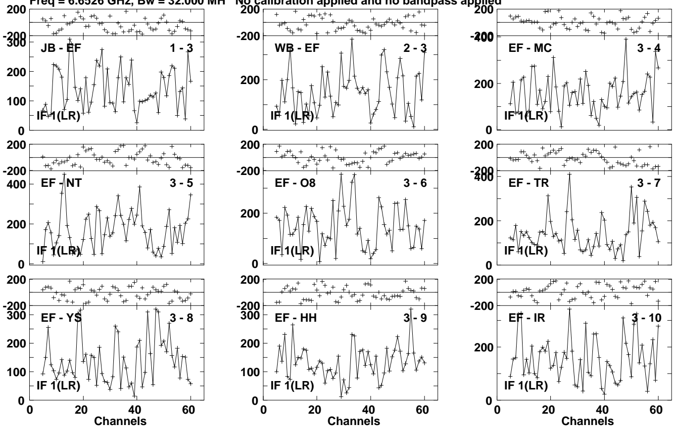
Lower frame: Micro Ampl Jy Top frame: Phas deg Vector averaged cross-power spectrum Several baselines displayed Timerange: 01/04:30:21 to 01/04:32:41
