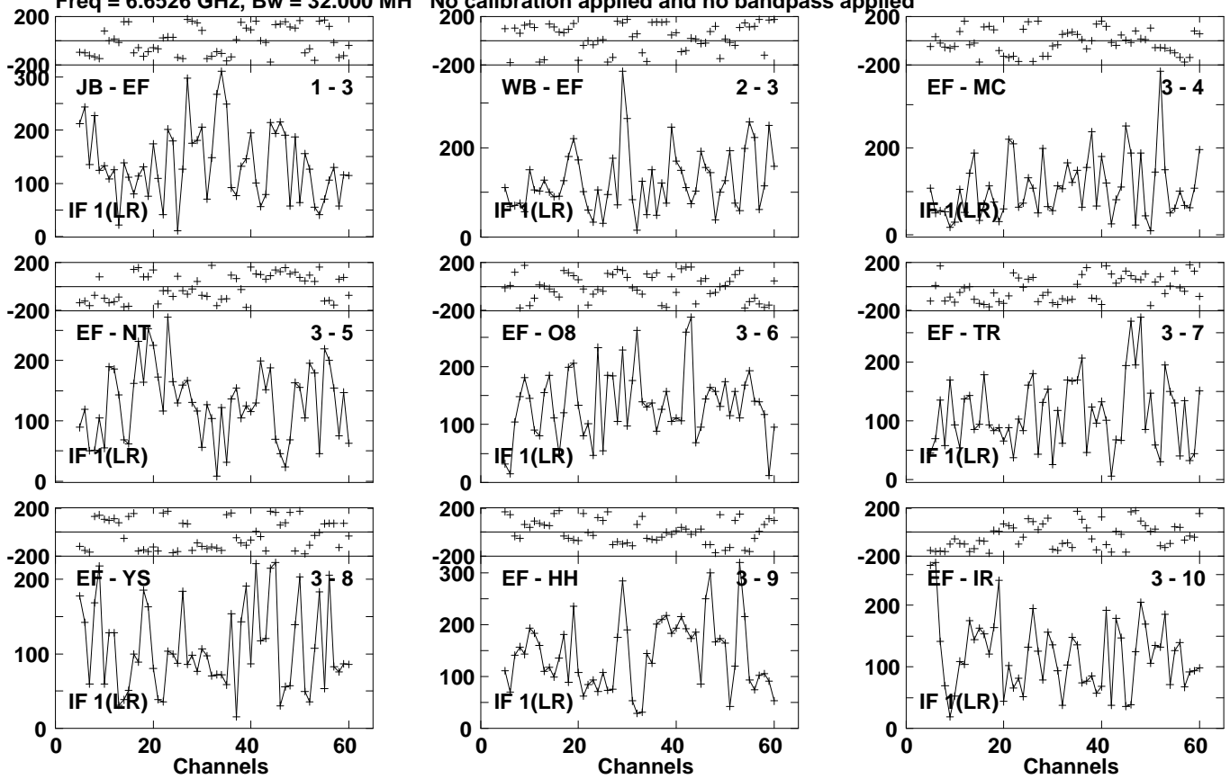
Lower frame: Micro Ampl Jy Top frame: Phas deg Vector averaged cross-power spectrum Several baselines displayed Timerange: 01/01:21:21 to 01/01:23:41
