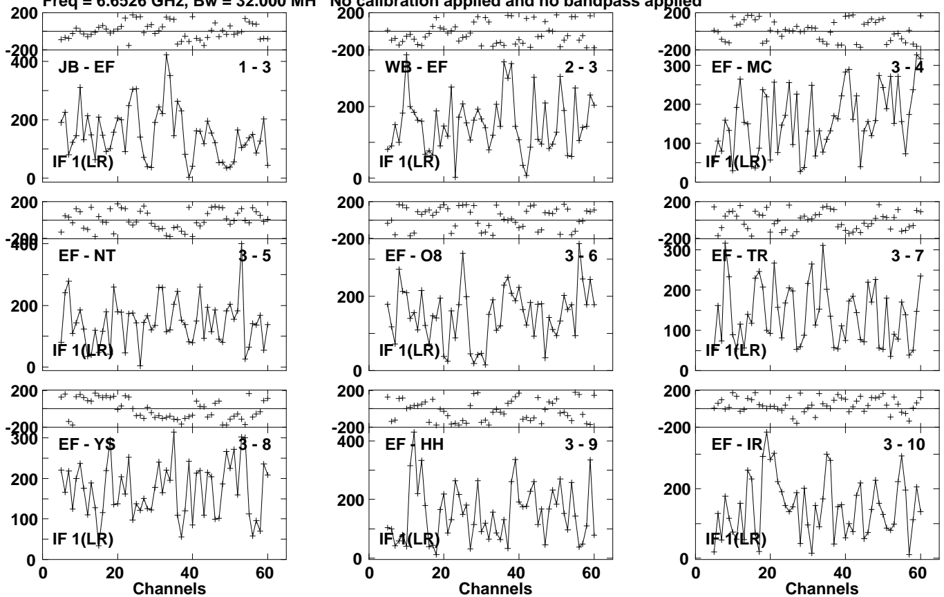
Lower frame: Micro Ampl Jy Top frame: Phas deg Vector averaged cross-power spectrum Several baselines displayed Timerange: 01/01:14:17 to 01/01:16:37
