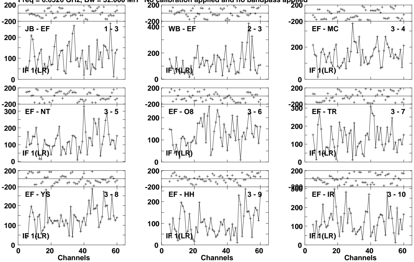
Lower frame: Micro Ampl Jy Top frame: Phas deg Vector averaged cross-power spectrum Several baselines displayed Timerange: 00/23:21:21 to 00/23:23:41
