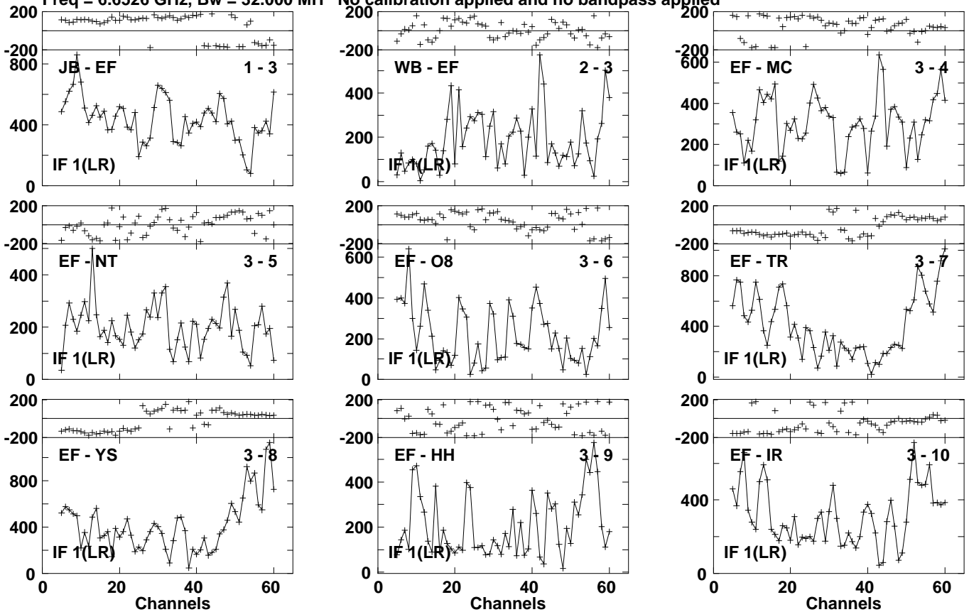
Lower frame: Micro Ampl Jy Top frame: Phas deg Vector averaged cross-power spectrum Several baselines displayed Timerange: 01/05:39:57 to 01/05:41:35
