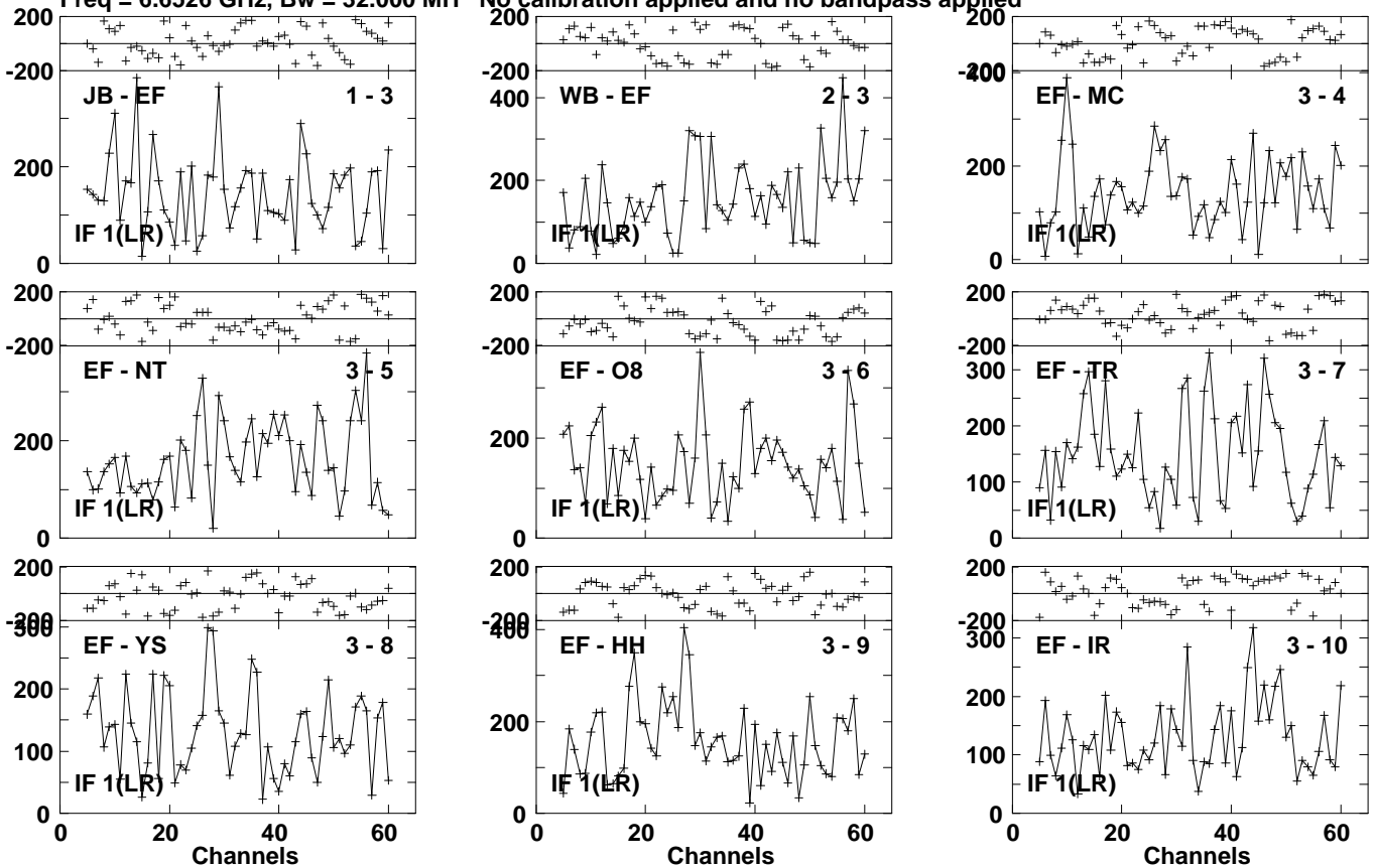
Lower frame: Micro Ampl Jy Top frame: Phas deg Vector averaged cross-power spectrum Several baselines displayed Timerange: 01/03:48:51 to 01/03:51:11
