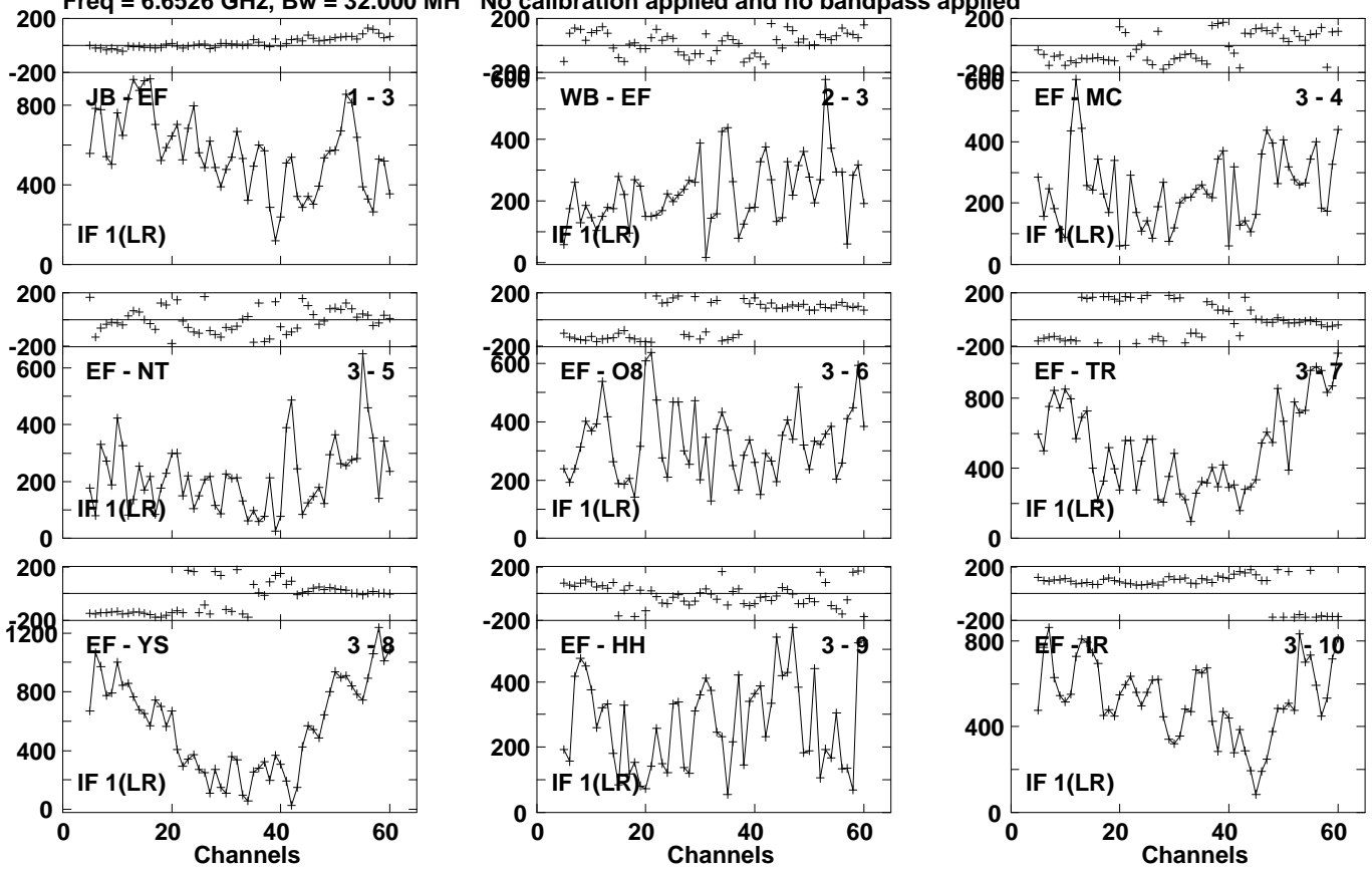
Lower frame: Micro Ampl Jy Top frame: Phas deg Vector averaged cross-power spectrum Several baselines displayed Timerange: 01/00:35:19 to 01/00:36:57
