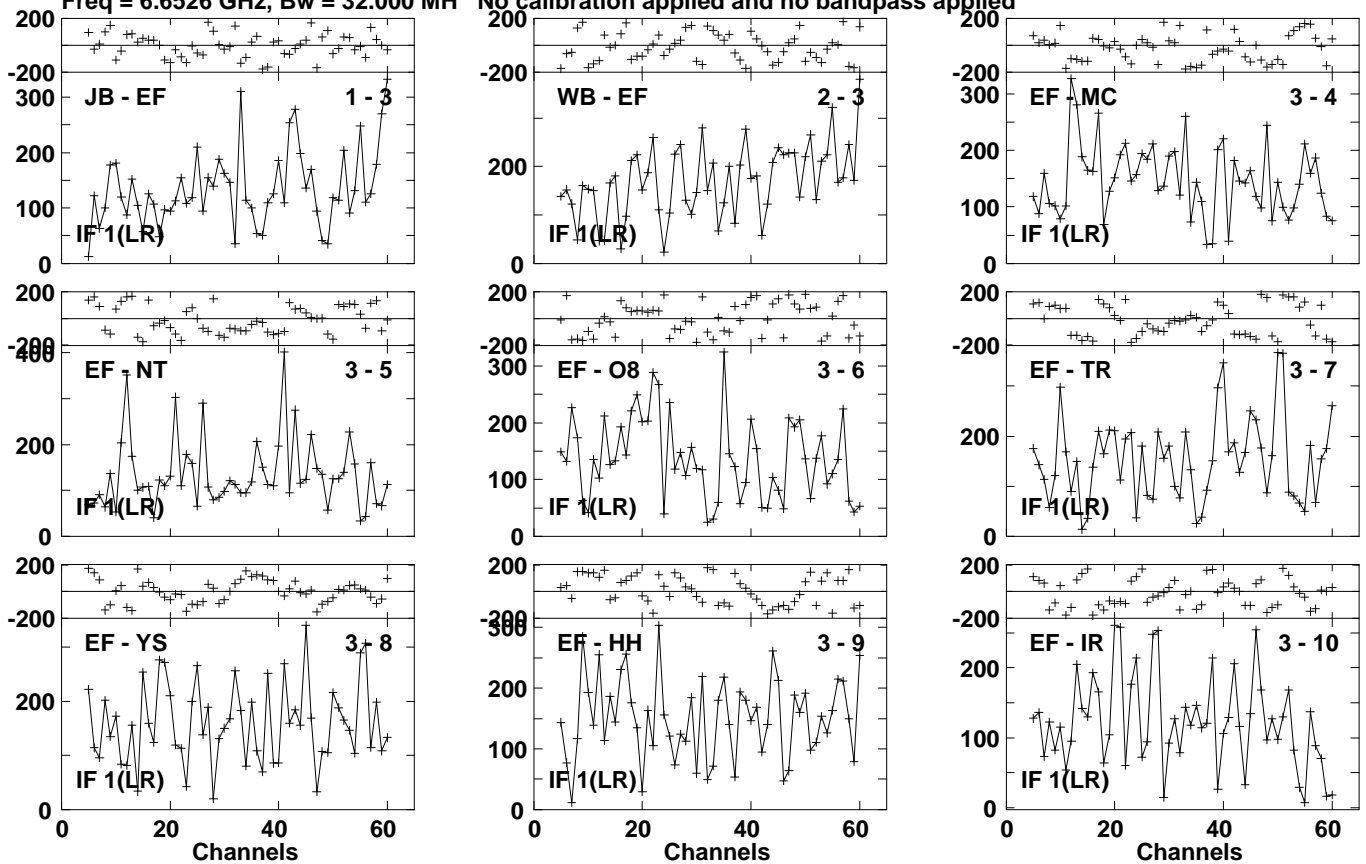
Lower frame: Micro Ampl Jy Top frame: Phas deg Vector averaged cross-power spectrum Several baselines displayed Timerange: 01/04:04:39 to 01/04:06:59
