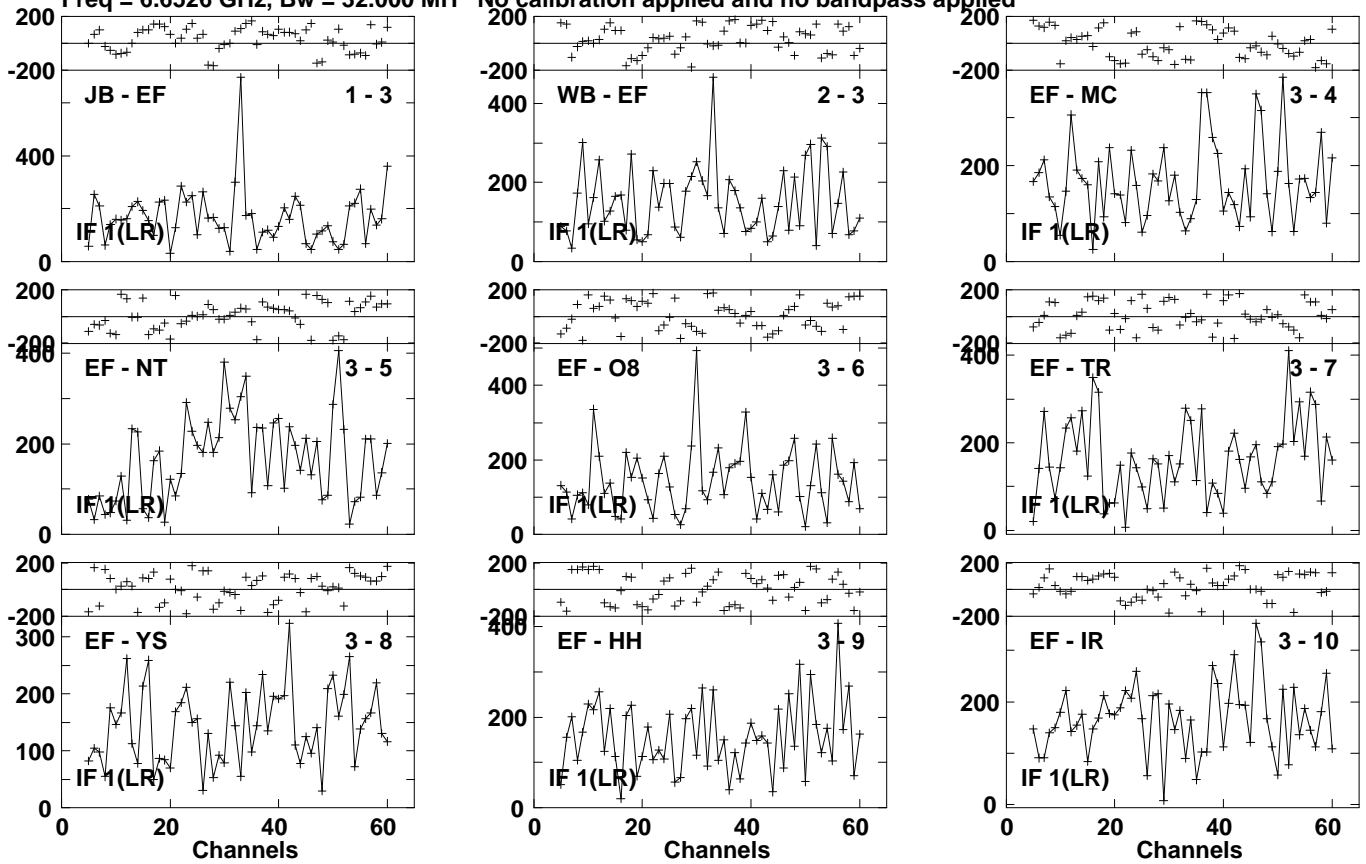
Lower frame: Micro Ampl Jy Top frame: Phas deg Vector averaged cross-power spectrum Several baselines displayed Timerange: 01/02:25:43 to 01/02:28:03
