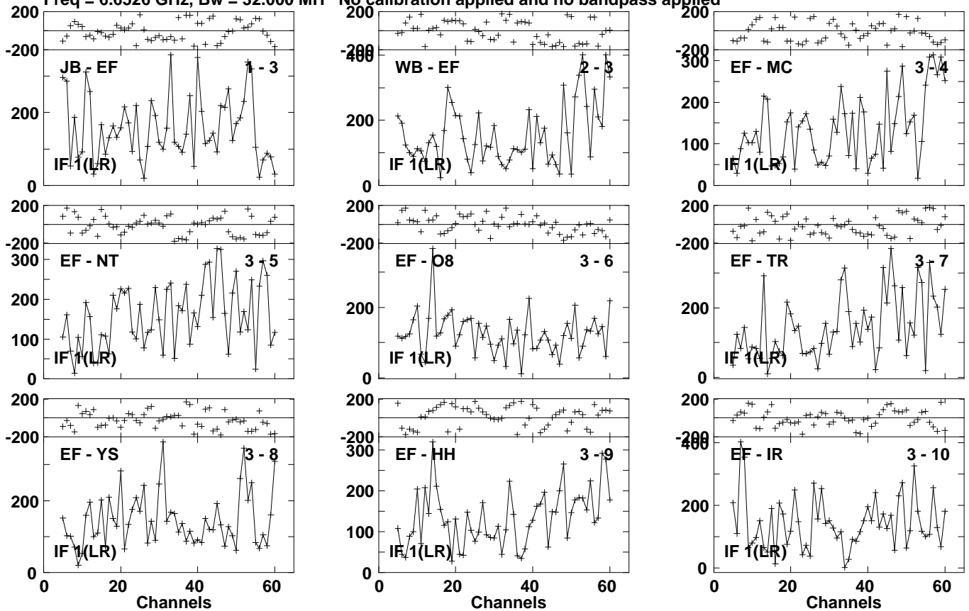
Lower frame: Micro Ampl Jy Top frame: Phas deg Vector averaged cross-power spectrum Several baselines displayed Timerange: 01/03:25:59 to 01/03:28:19
