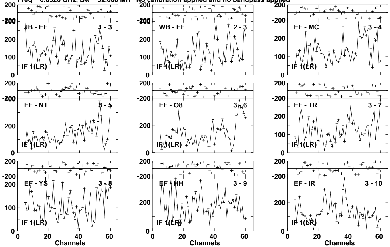
Lower frame: Micro Ampl Jy Top frame: Phas deg Vector averaged cross-power spectrum Several baselines displayed Timerange: 00/23:09:47 to 00/23:12:15
