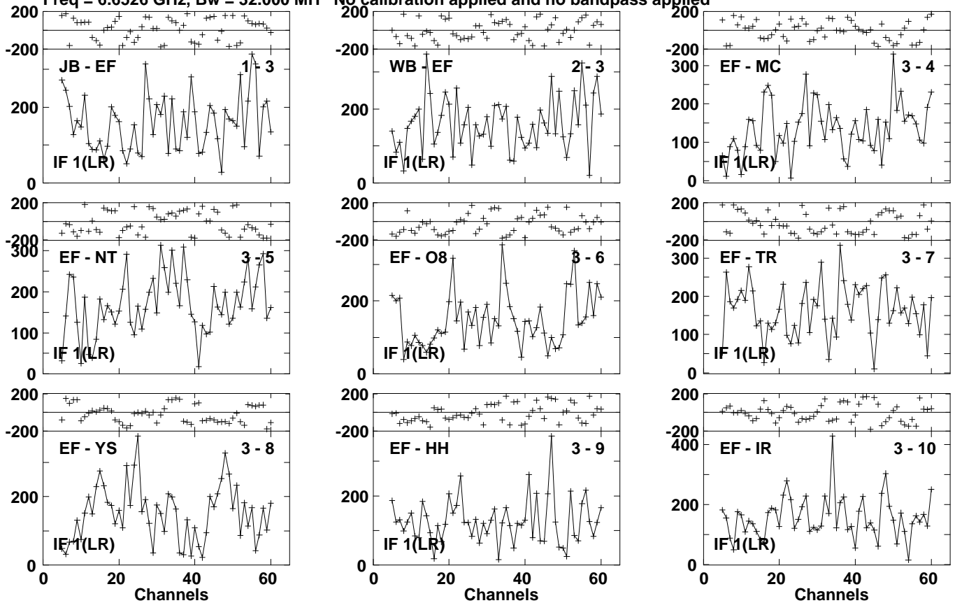
Lower frame: Micro Ampl Jy Top frame: Phas deg Vector averaged cross-power spectrum Several baselines displayed Timerange: 00/23:52:57 to 00/23:55:17
