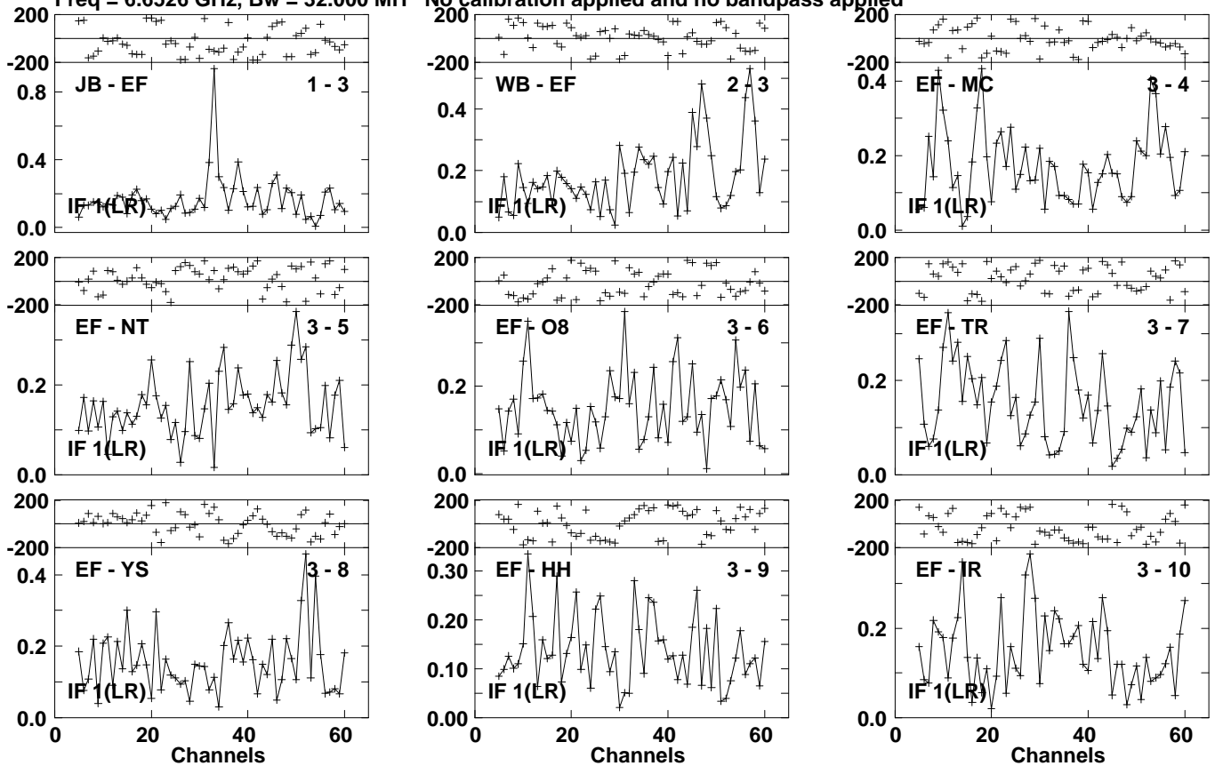
Lower frame: Milli Ampl Jy Top frame: Phas deg Vector averaged cross-power spectrum Several baselines displayed Timerange: 01/02:41:31 to 01/02:43:51
