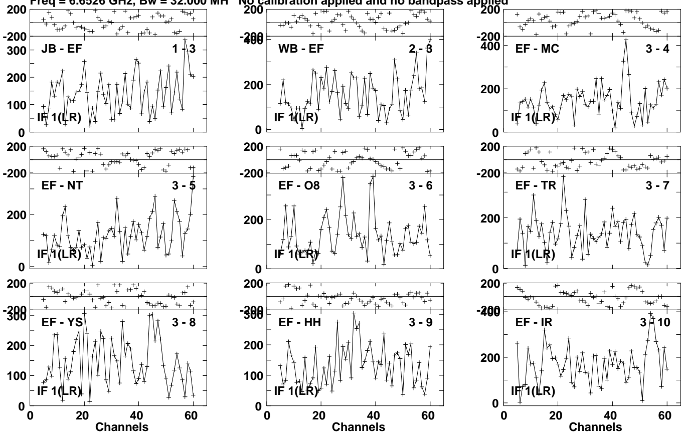
Lower frame: Micro Ampl Jy Top frame: Phas deg Vector averaged cross-power spectrum Several baselines displayed Timerange: 01/01:25:43 to 01/01:28:03
