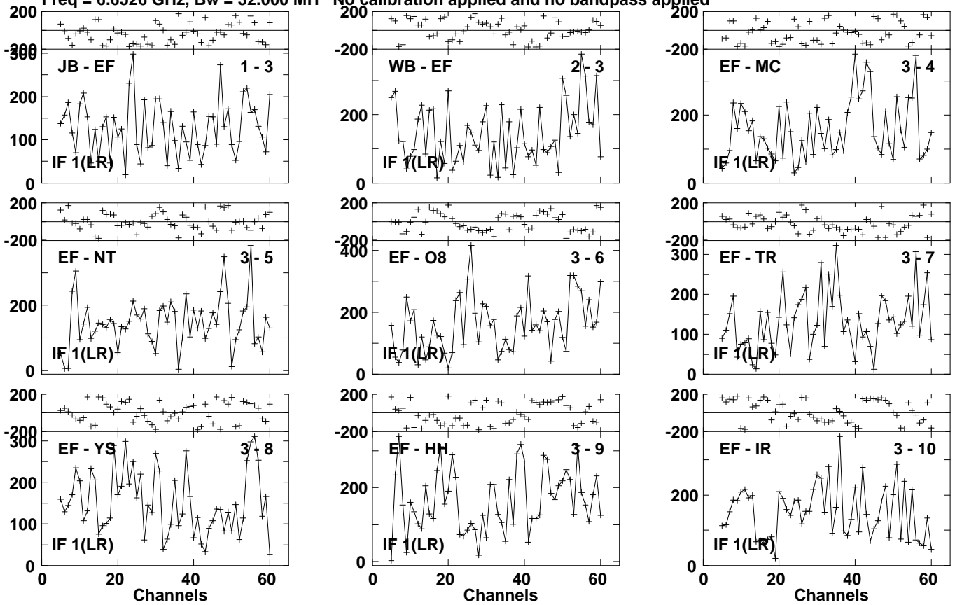
Lower frame: Micro Ampl Jy Top frame: Phas deg Vector averaged cross-power spectrum Several baselines displayed Timerange: 01/05:04:39 to 01/05:06:59
