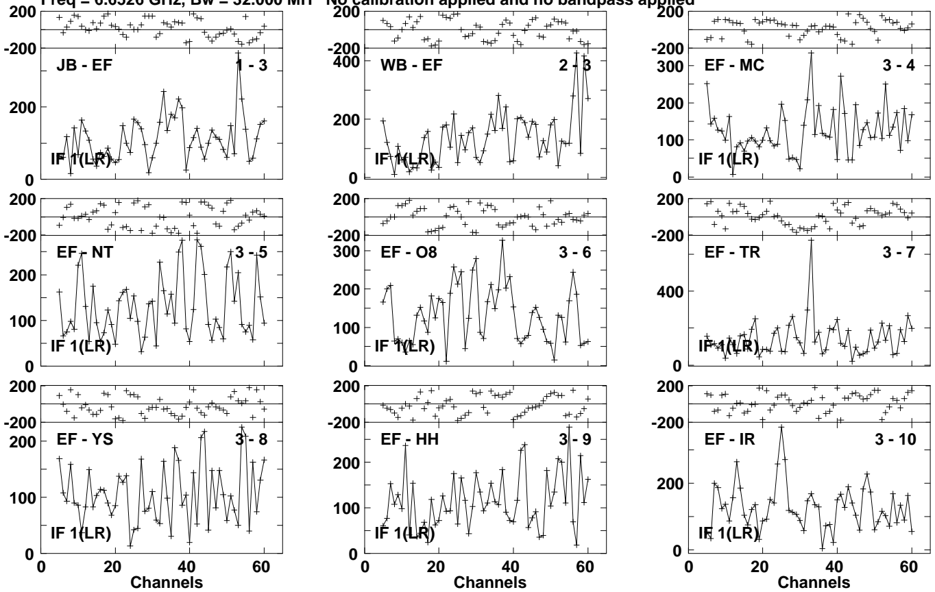
Lower frame: Micro Ampl Jy Top frame: Phas deg Vector averaged cross-power spectrum Several baselines displayed Timerange: 01/00:55:39 to 01/00:57:59
