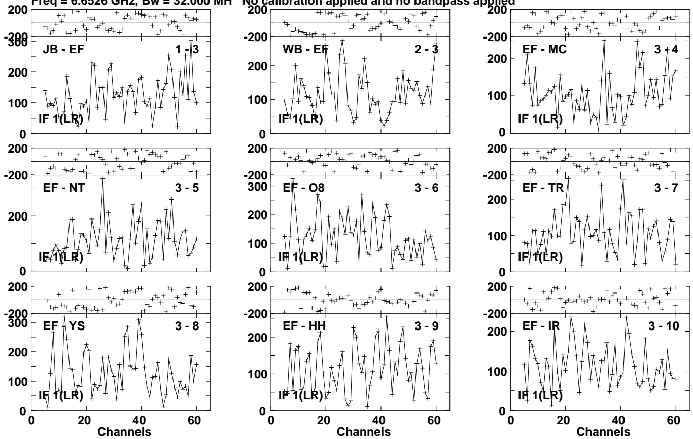
Lower frame: Micro Ampl Jy Top frame: Phas deg Vector averaged cross-power spectrum Several baselines displayed Timerange: 01/03:55:55 to 01/03:58:15
