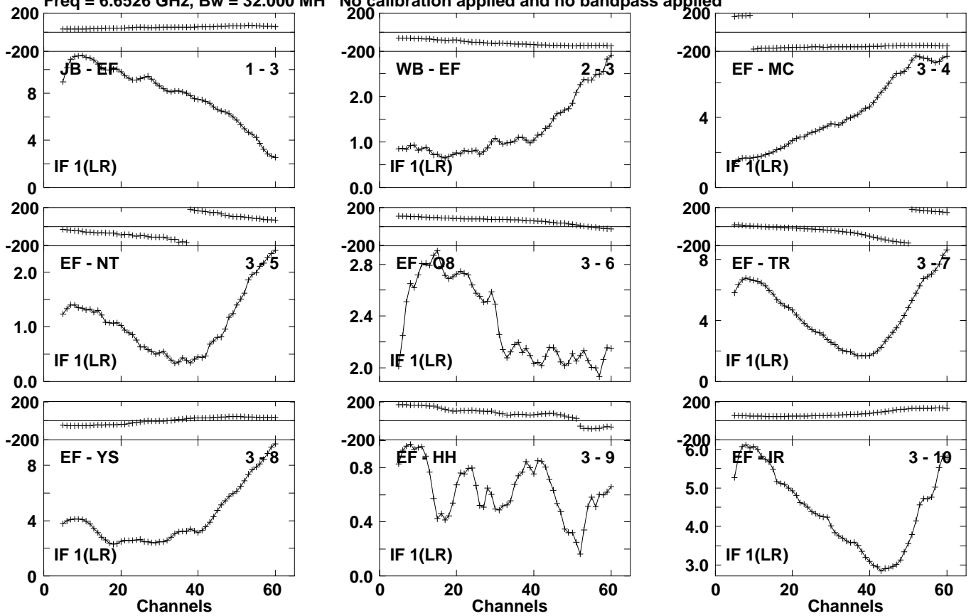
Lower frame: Milli Ampl Jy Top frame: Phas deg Vector averaged cross-power spectrum Several baselines displayed Timerange: 01/06:52:51 to 01/06:59:59
