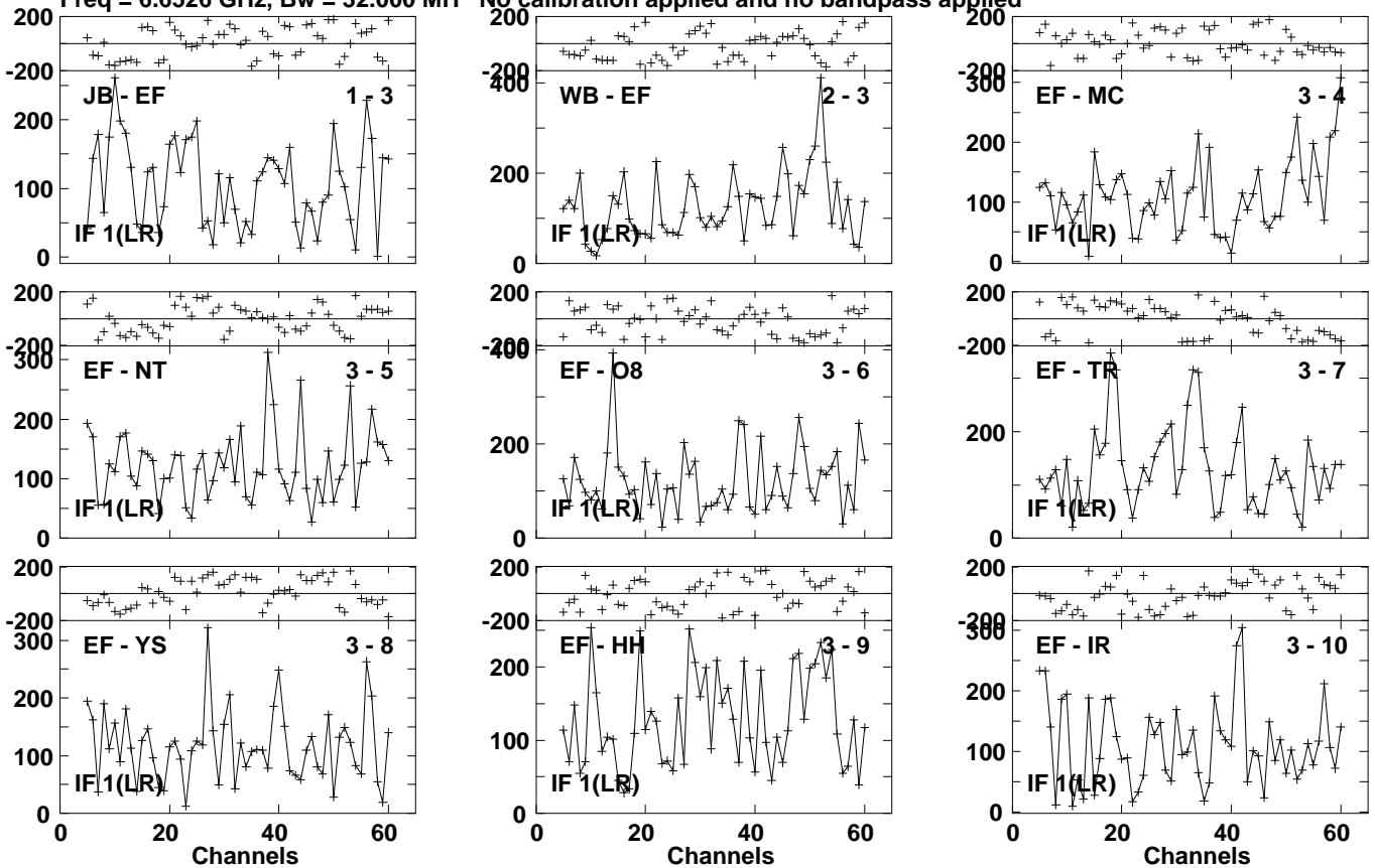
Lower frame: Micro Ampl Jy Top frame: Phas deg Vector averaged cross-power spectrum Several baselines displayed Timerange: 01/04:55:55 to 01/04:58:15
