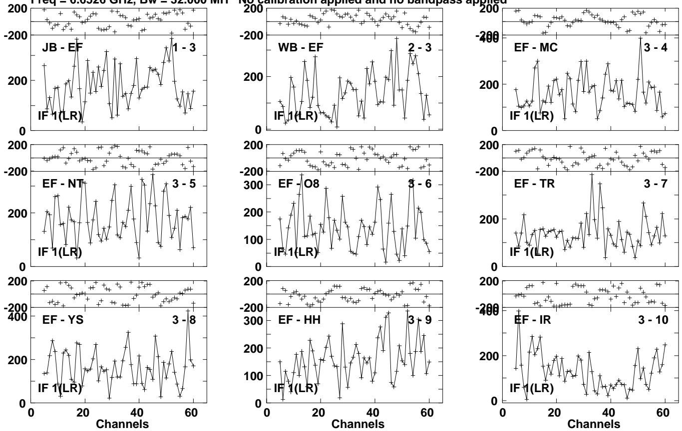
Lower frame: Micro Ampl Jy Top frame: Phas deg Vector averaged cross-power spectrum Several baselines displayed Timerange: 01/04:25:59 to 01/04:28:19
