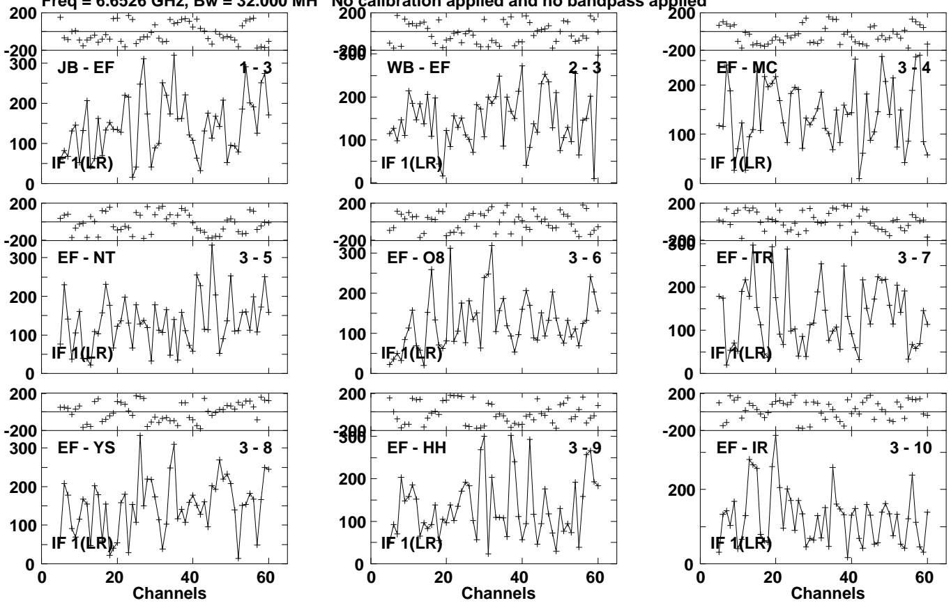
Lower frame: Micro Ampl Jy Top frame: Phas deg Vector averaged cross-power spectrum Several baselines displayed Timerange: 01/05:53:13 to 01/05:55:33
