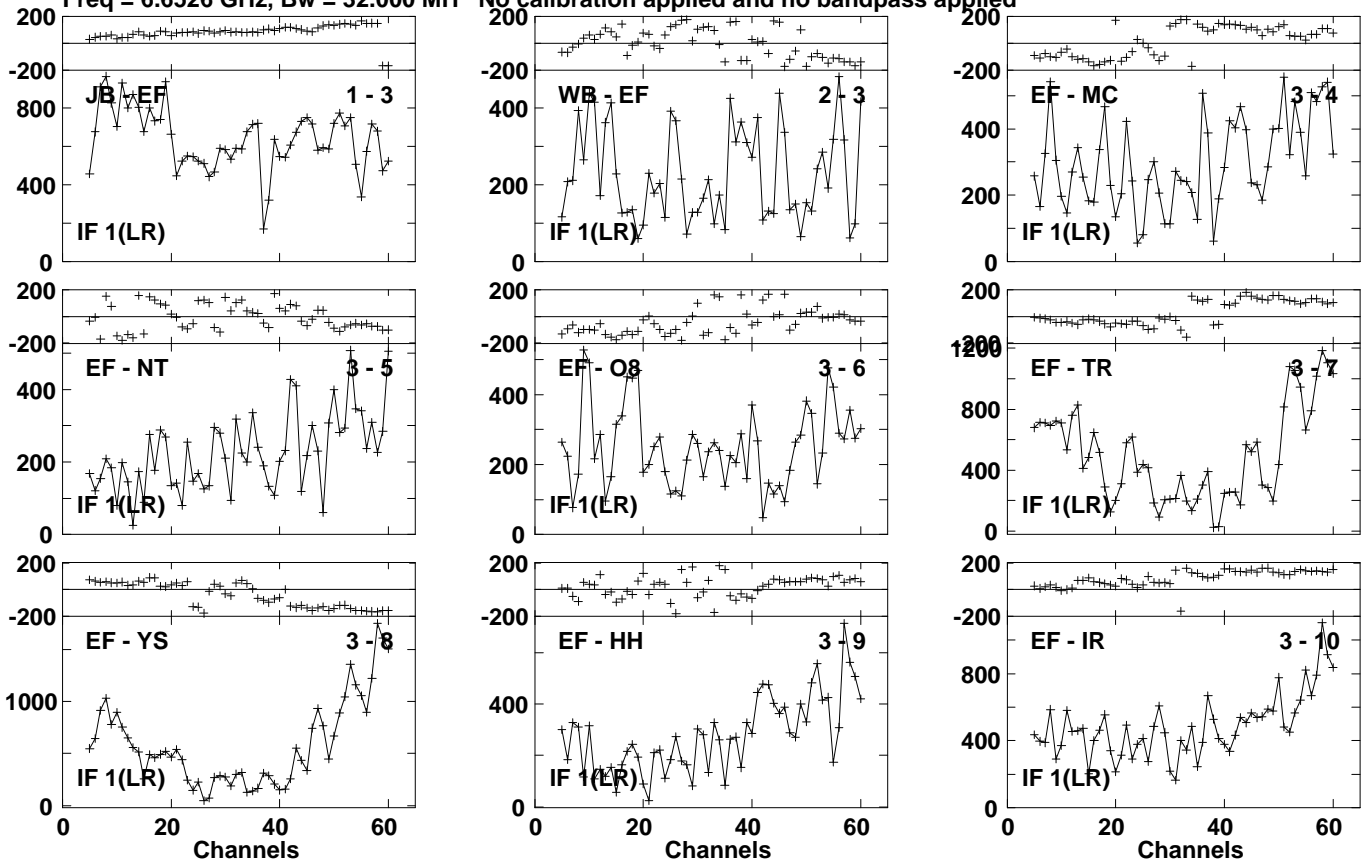
Lower frame: Micro Ampl Jy Top frame: Phas deg Vector averaged cross-power spectrum Several baselines displayed Timerange: 01/05:02:49 to 01/05:04:27
