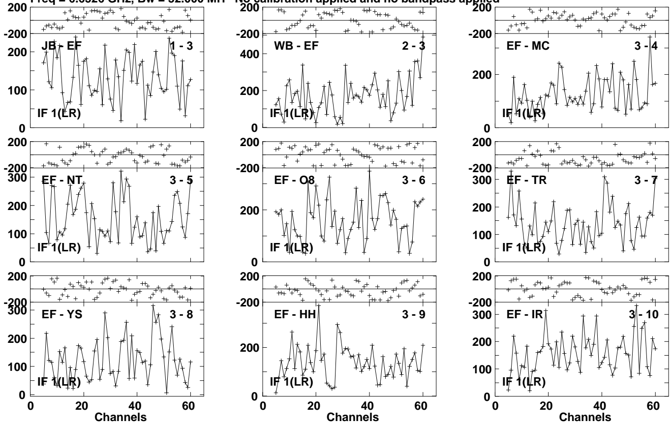
Lower frame: Micro Ampl Jy Top frame: Phas deg Vector averaged cross-power spectrum Several baselines displayed Timerange: 01/04:53:13 to 01/04:55:33
