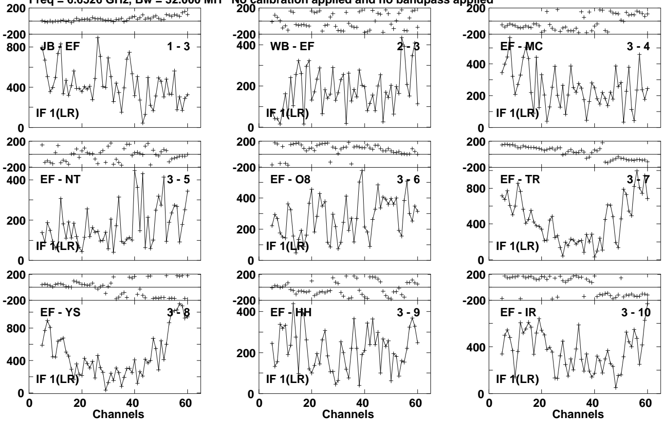
Lower frame: Micro Ampl Jy Top frame: Phas deg Vector averaged cross-power spectrum Several baselines displayed Timerange: 01/01:39:41 to 01/01:41:19
