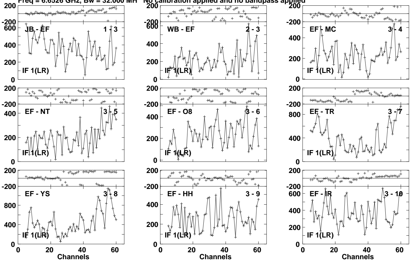
Lower frame: Micro Ampl Jy Top frame: Phas deg Vector averaged cross-power spectrum Several baselines displayed Timerange: 00/23:16:49 to 00/23:18:27
