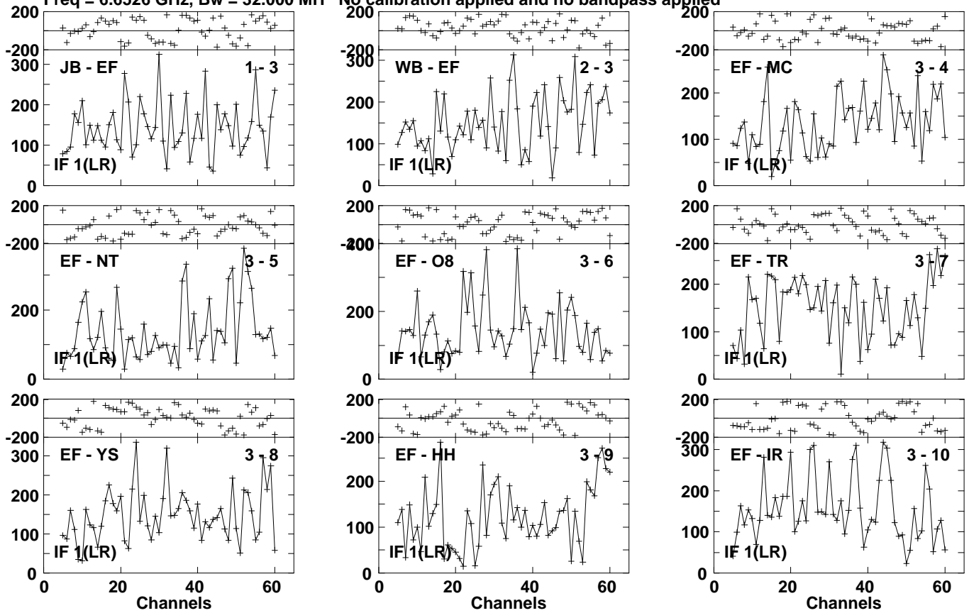
Lower frame: Micro Ampl Jy Top frame: Phas deg Vector averaged cross-power spectrum Several baselines displayed Timerange: 01/05:30:21 to 01/05:32:41
