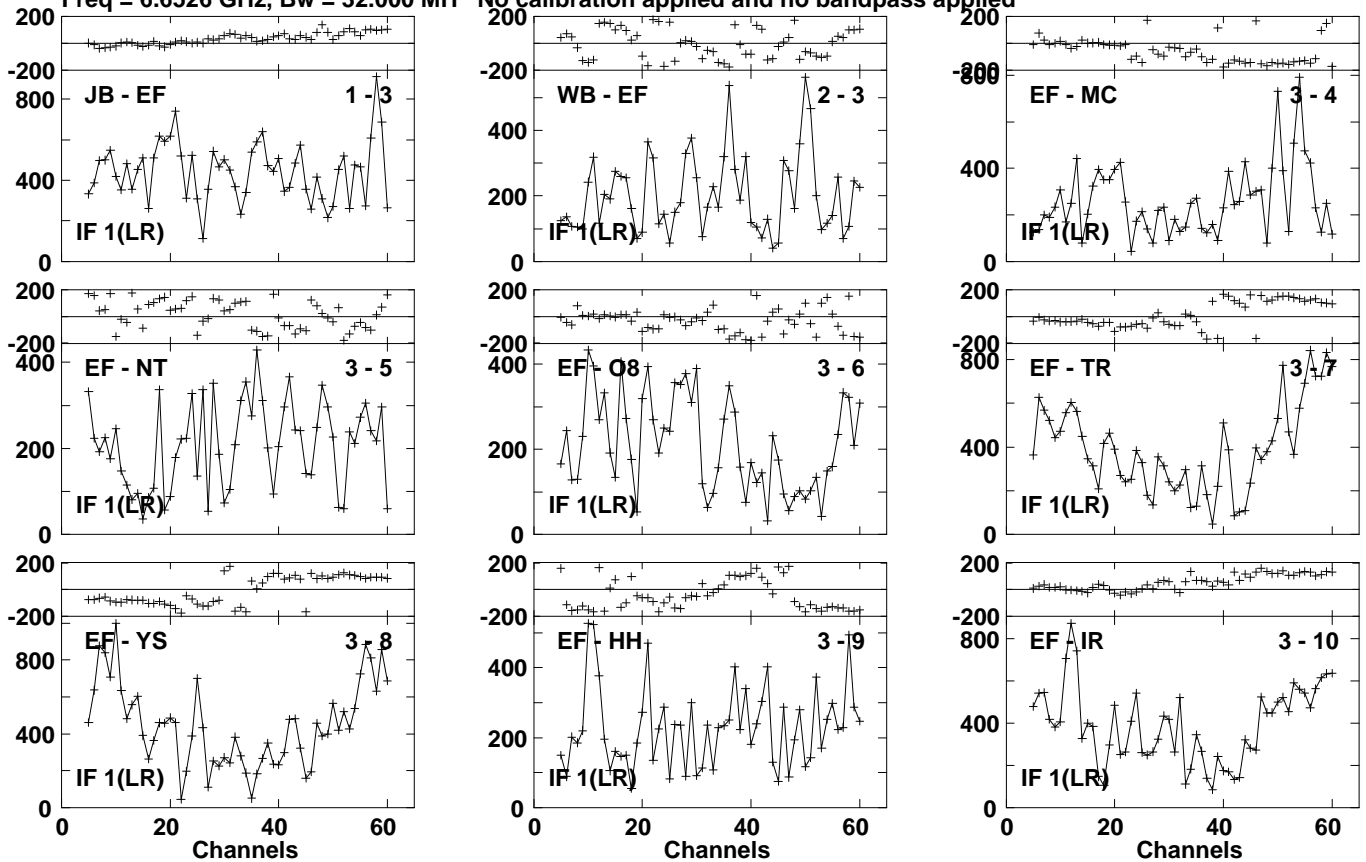
Lower frame: Micro Ampl Jy Top frame: Phas deg Vector averaged cross-power spectrum Several baselines displayed Timerange: 01/03:51:23 to 01/03:53:01
