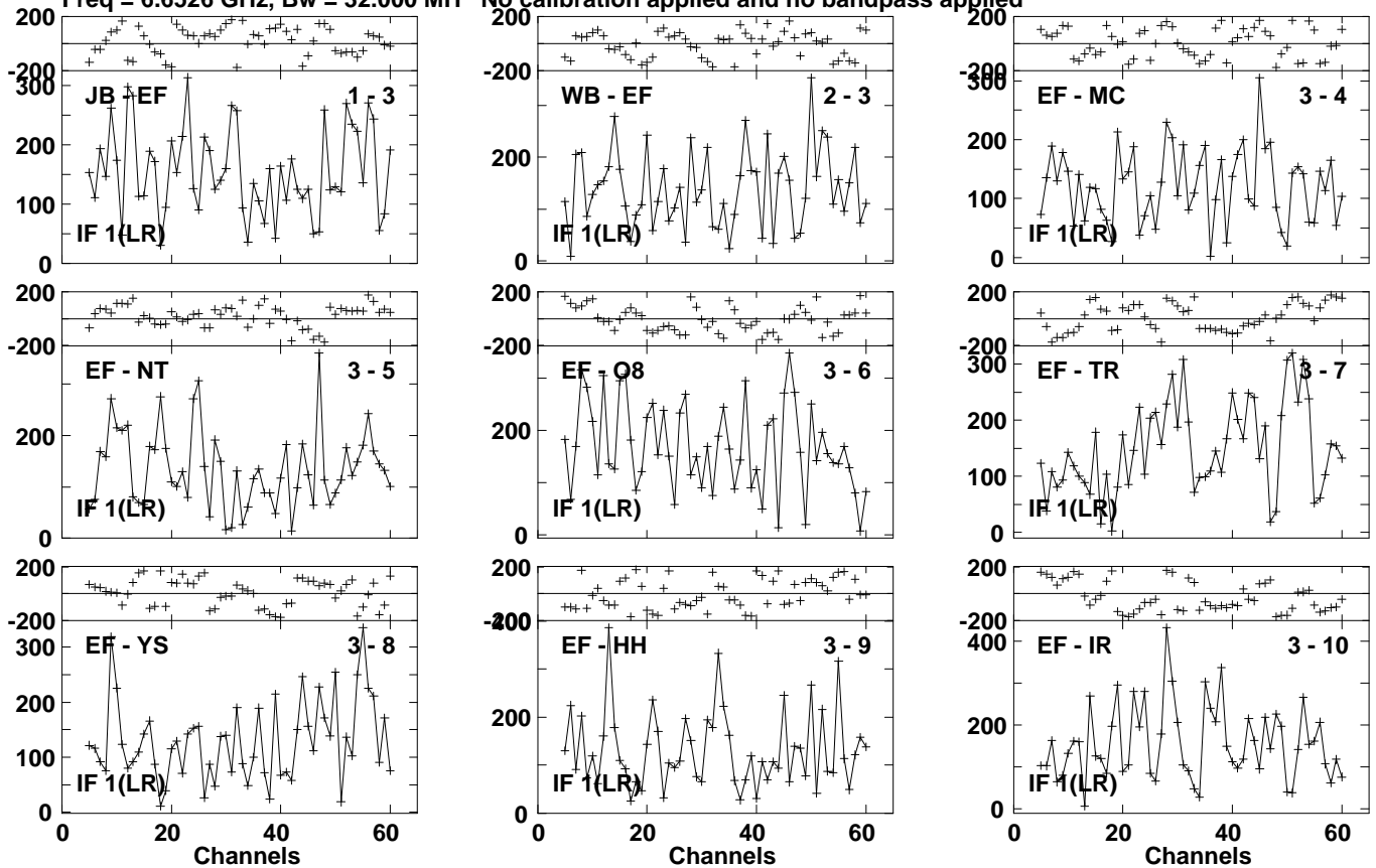
Lower frame: Micro Ampl Jy Top frame: Phas deg Vector averaged cross-power spectrum Several baselines displayed Timerange: 01/04:41:47 to 01/04:44:07
