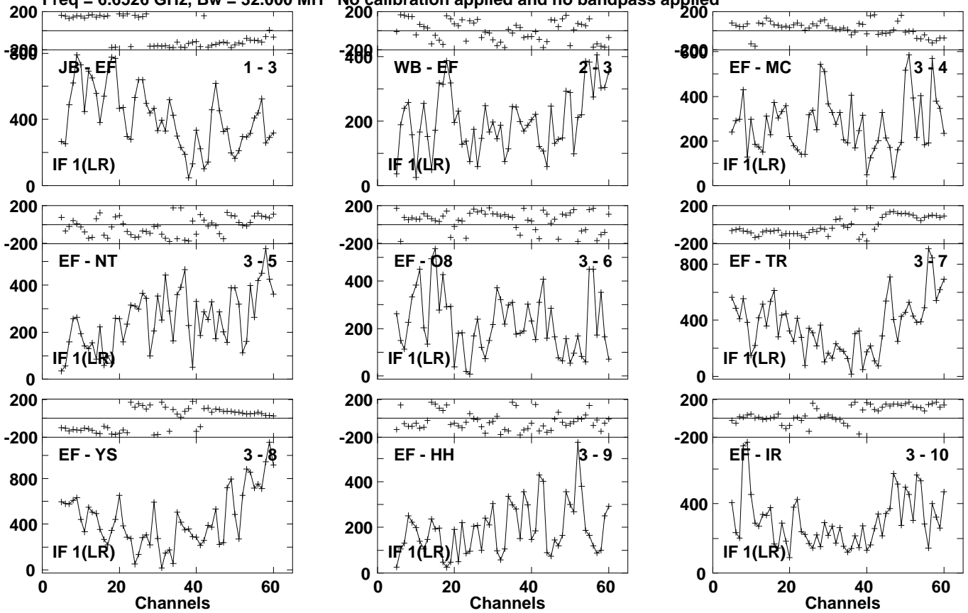
Lower frame: Micro Ampl Jy Top frame: Phas deg Vector averaged cross-power spectrum Several baselines displayed Timerange: 01/05:28:31 to 01/05:30:09
