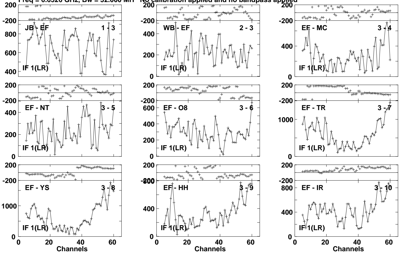
Lower frame: Micro Ampl Jy Top frame: Phas deg Vector averaged cross-power spectrum Several baselines displayed Timerange: 01/04:28:31 to 01/04:30:09
