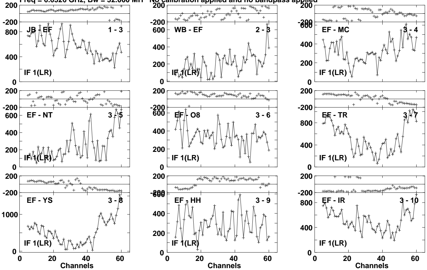
Lower frame: Micro Ampl Jy Top frame: Phas deg Vector averaged cross-power spectrum Several baselines displayed Timerange: 01/00:16:49 to 01/00:18:27
