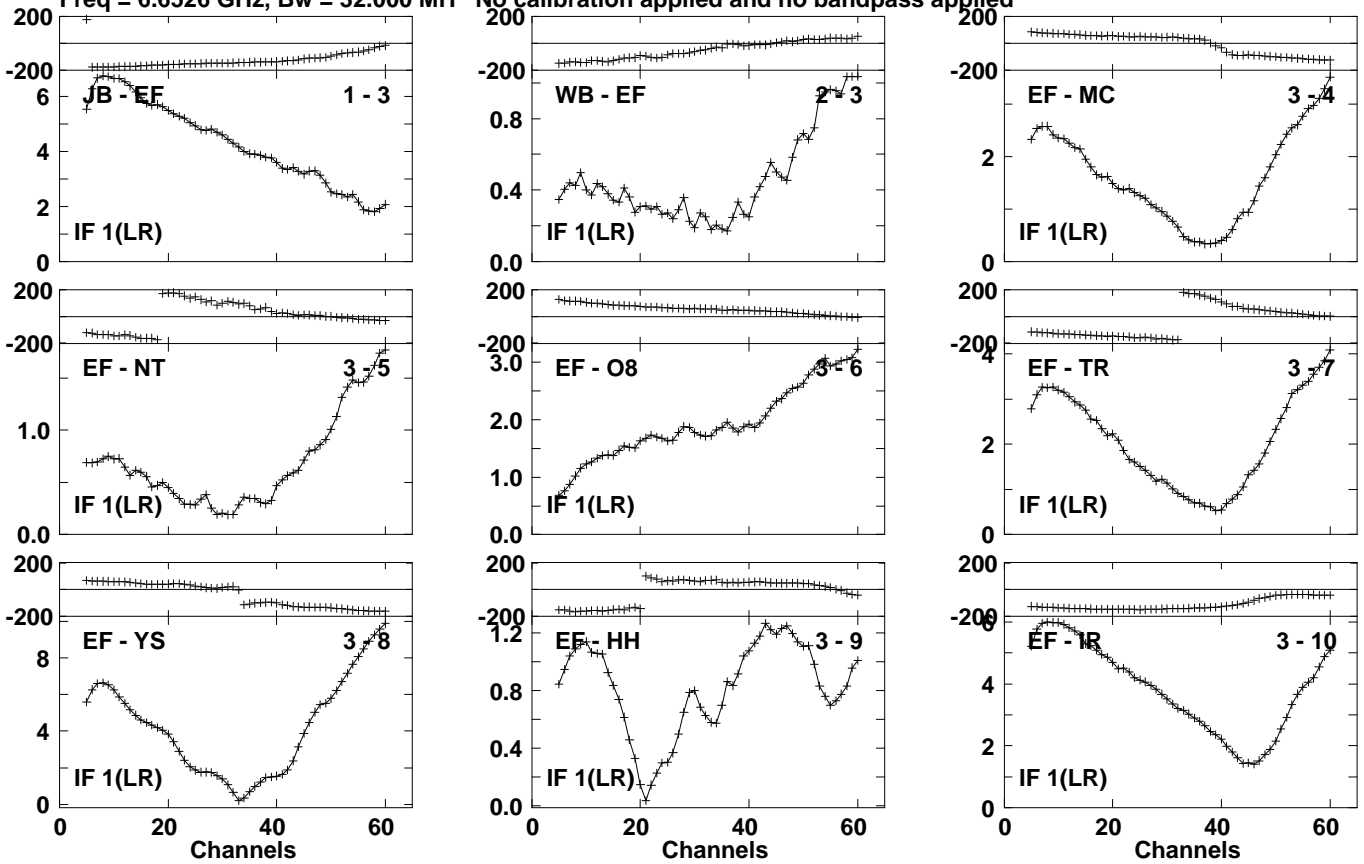
Lower frame: Milli Ampl Jy Top frame: Phas deg Vector averaged cross-power spectrum Several baselines displayed Timerange: 01/00:00:01 to 01/00:07:09
