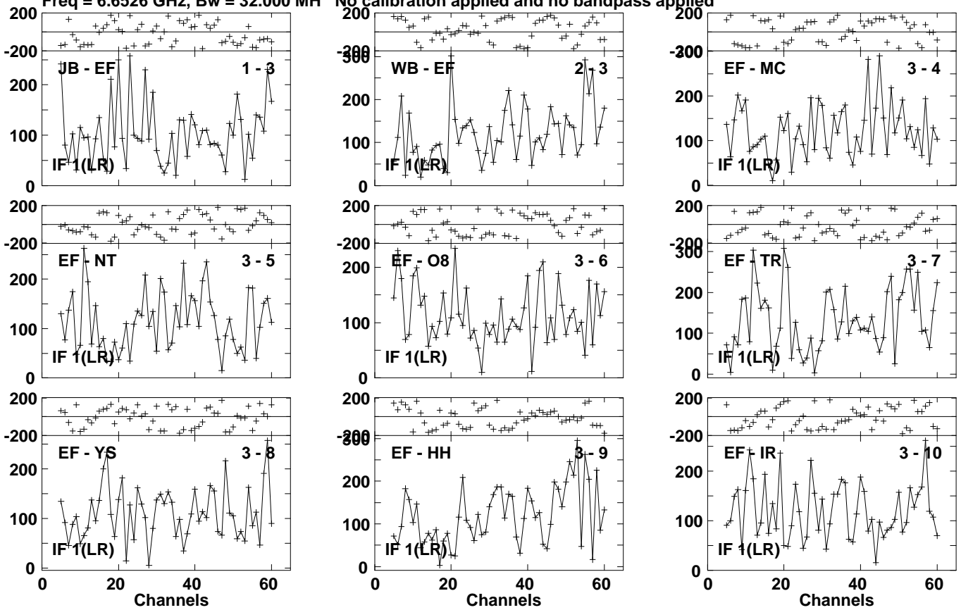
Lower frame: Micro Ampl Jy Top frame: Phas deg Vector averaged cross-power spectrum Several baselines displayed Timerange: 01/05:44:29 to 01/05:46:49
