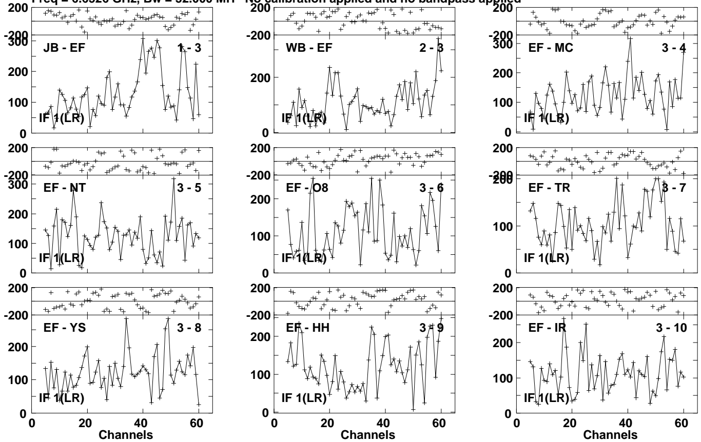
Lower frame: Micro Ampl Jy Top frame: Phas deg Vector averaged cross-power spectrum Several baselines displayed Timerange: 01/02:21:21 to 01/02:23:41
