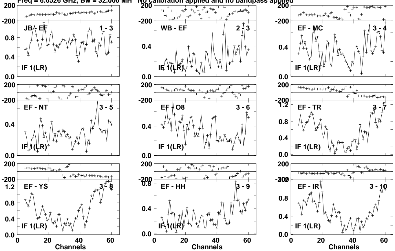
Lower frame: Milli Ampl Jy Top frame: Phas deg Vector averaged cross-power spectrum Several baselines displayed Timerange: 01/02:46:45 to 01/02:48:23
