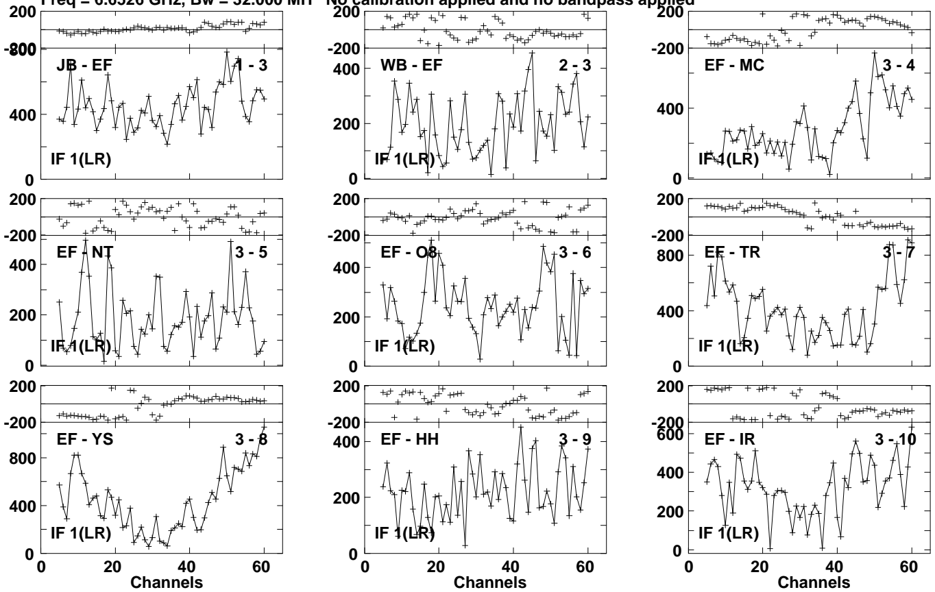
Lower frame: Micro Ampl Jy Top frame: Phas deg Vector averaged cross-power spectrum Several baselines displayed Timerange: 01/03:58:27 to 01/04:00:05
