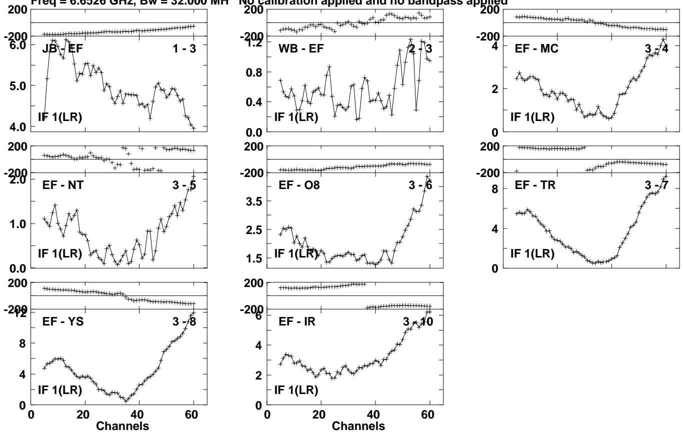
Lower frame: Milli Ampl Jy Top frame: Phas deg Vector averaged cross-power spectrum Several baselines displayed Timerange: 01/05:19:23 to 01/05:19:51
