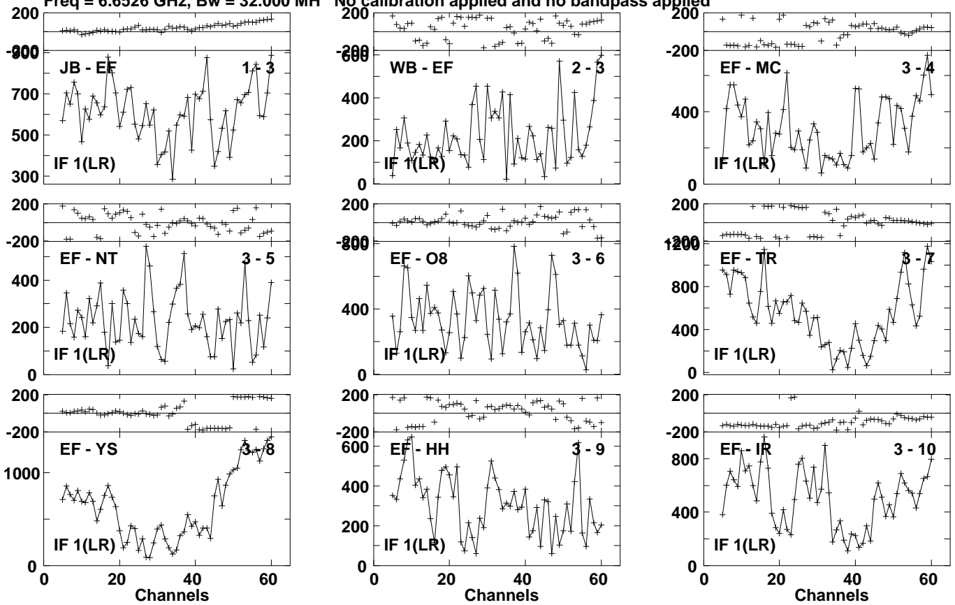
Lower frame: Micro Ampl Jy Top frame: Phas deg Vector averaged cross-power spectrum Several baselines displayed Timerange: 01/02:35:19 to 01/02:36:57
