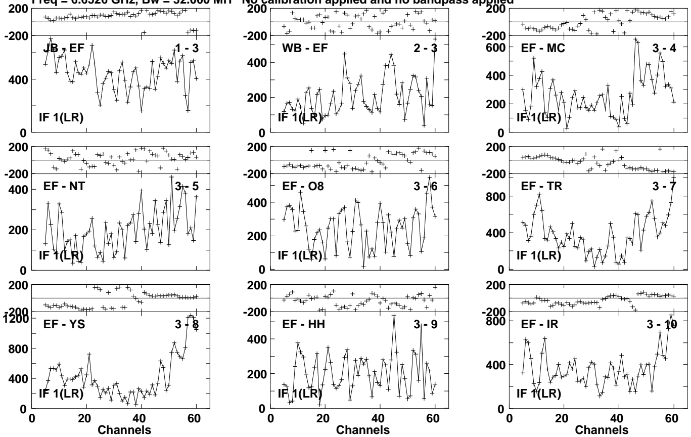
Lower frame: Micro Ampl Jy Top frame: Phas deg Vector averaged cross-power spectrum Several baselines displayed Timerange: 01/03:28:31 to 01/03:30:09
