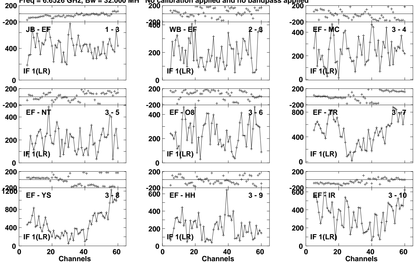
Lower frame: Micro Ampl Jy Top frame: Phas deg Vector averaged cross-power spectrum Several baselines displayed Timerange: 01/01:46:45 to 01/01:48:23
