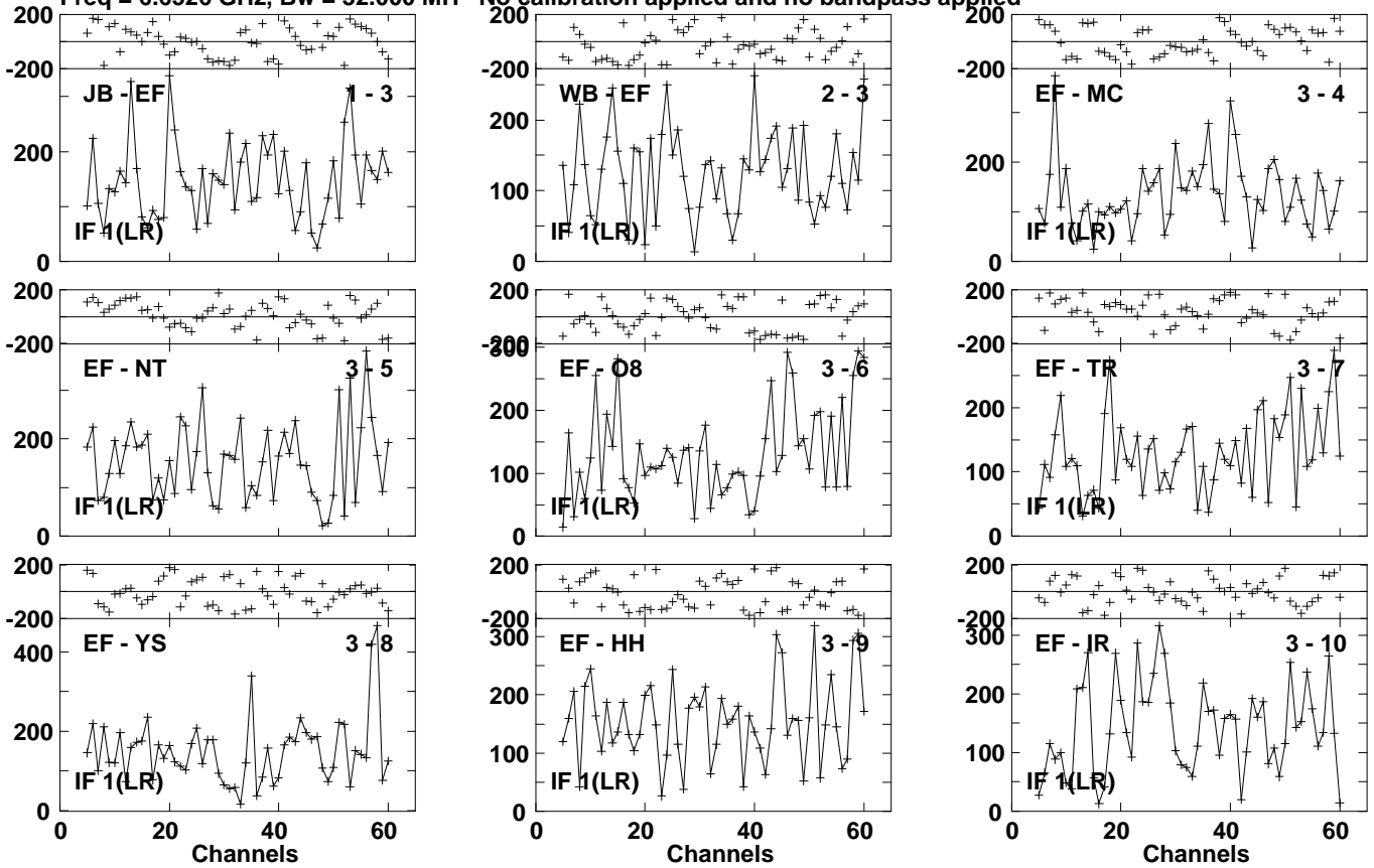
Lower frame: Micro Ampl Jy Top frame: Phas deg Vector averaged cross-power spectrum Several baselines displayed Timerange: 01/01:48:35 to 01/01:50:55
