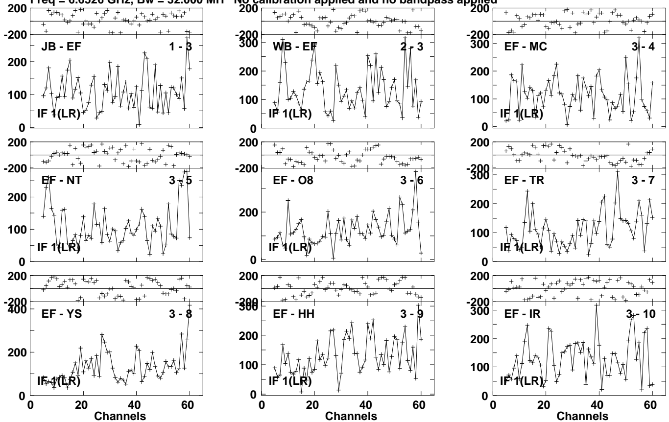
Lower frame: Micro Ampl Jy Top frame: Phas deg Vector averaged cross-power spectrum Several baselines displayed Timerange: 01/05:07:21 to 01/05:09:41
