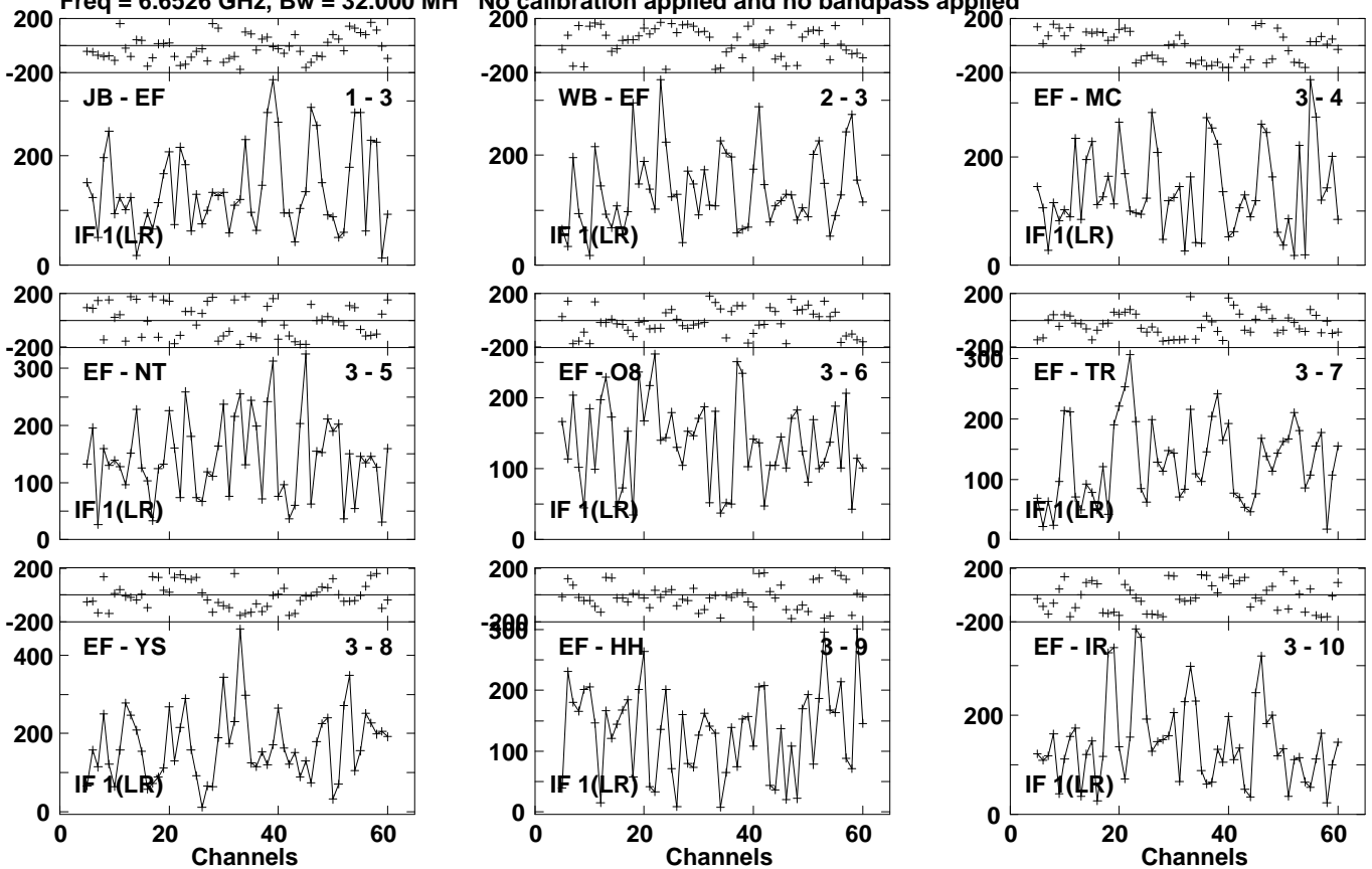
Lower frame: Micro Ampl Jy Top frame: Phas deg Vector averaged cross-power spectrum Several baselines displayed Timerange: 01/03:53:13 to 01/03:55:33
