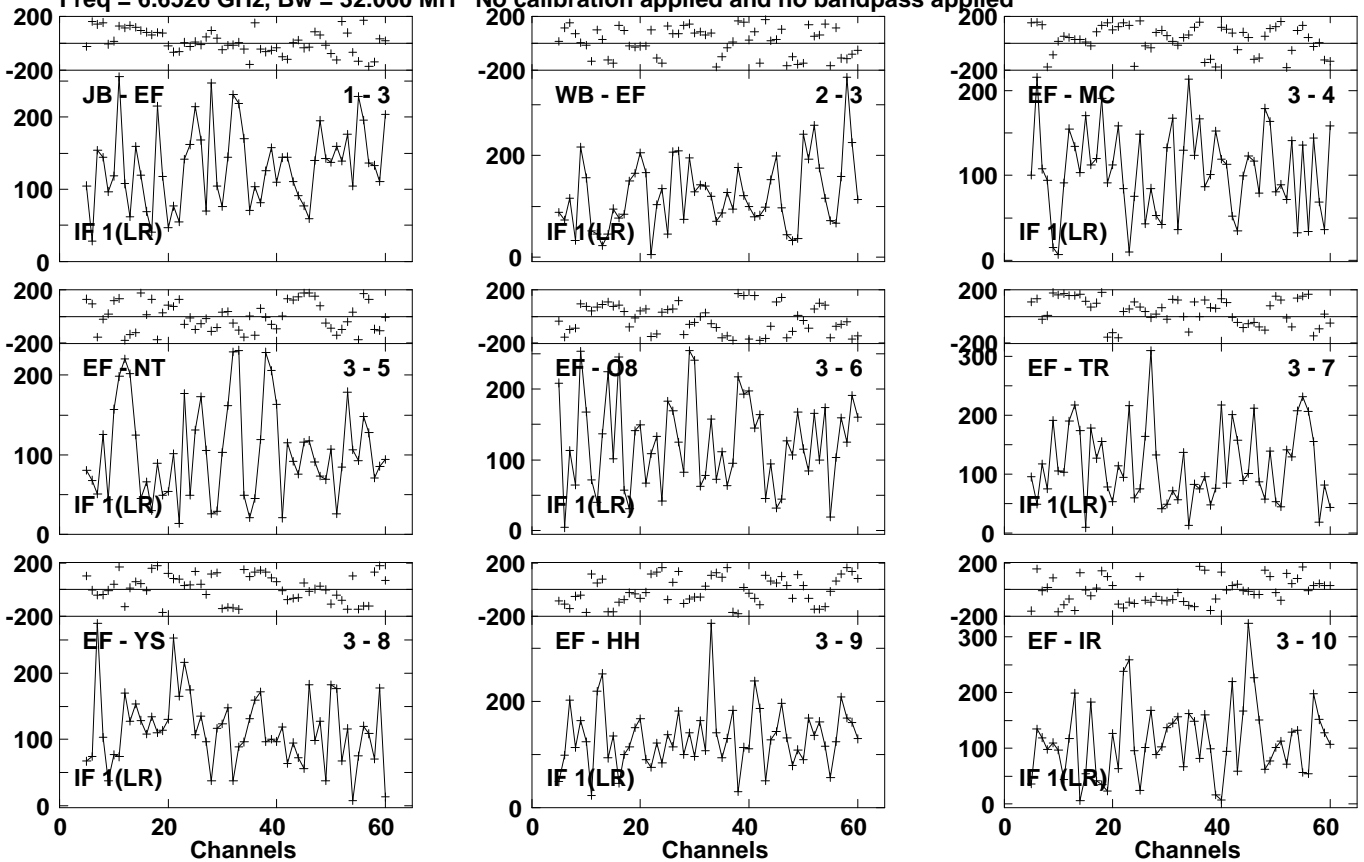
Lower frame: Micro Ampl Jy Top frame: Phas deg Vector averaged cross-power spectrum Several baselines displayed Timerange: 01/04:33:03 to 01/04:35:23
