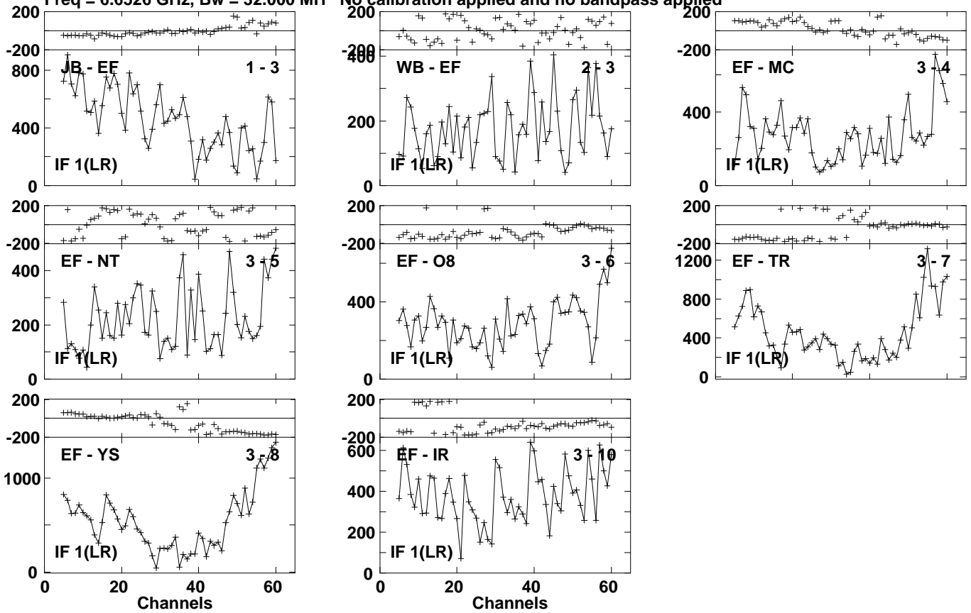
Lower frame: Micro Ampl Jy Top frame: Phas deg Vector averaged cross-power spectrum Several baselines displayed Timerange: 01/06:24:09 to 01/06:25:47
