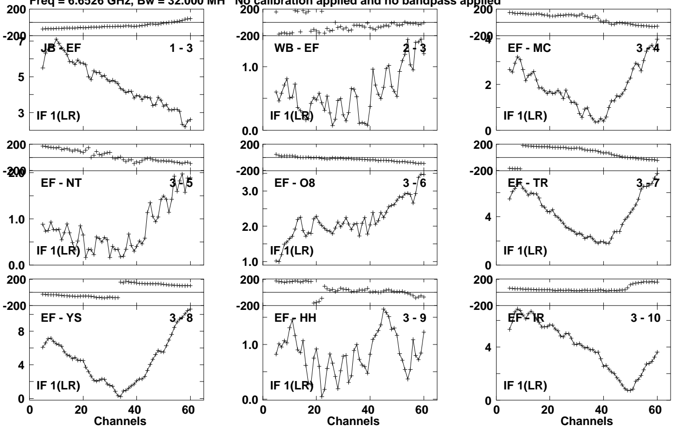
Lower frame: Milli Ampl Jy Top frame: Phas deg Vector averaged cross-power spectrum Several baselines displayed Timerange: 01/01:07:41 to 01/01:08:09
