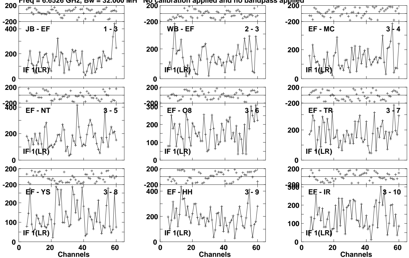
Lower frame: Micro Ampl Jy Top frame: Phas deg Vector averaged cross-power spectrum Several baselines displayed Timerange: 01/00:30:05 to 01/00:32:25
