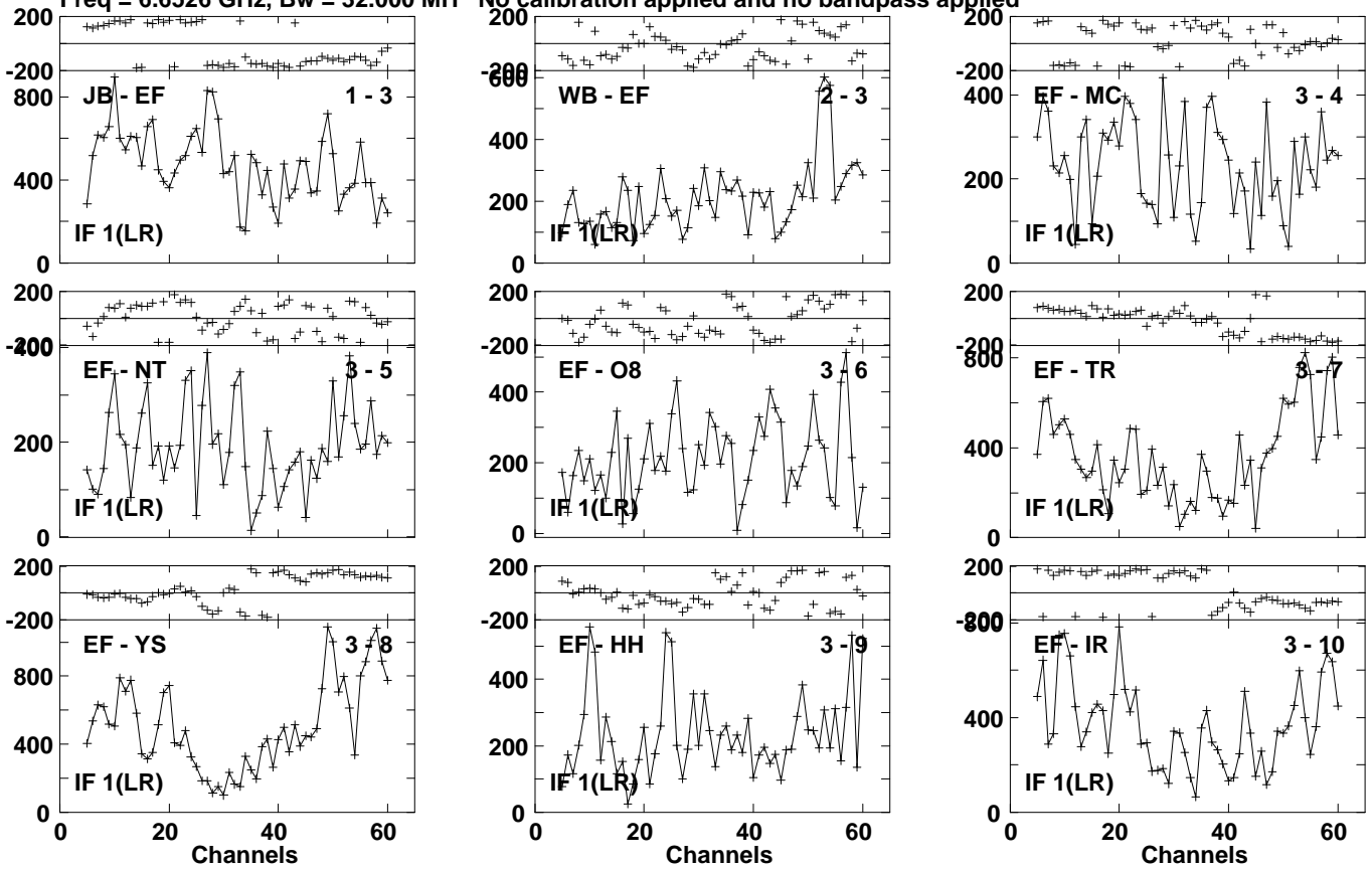
Lower frame: Micro Ampl Jy Top frame: Phas deg Vector averaged cross-power spectrum Several baselines displayed Timerange: 01/01:12:27 to 01/01:14:05
