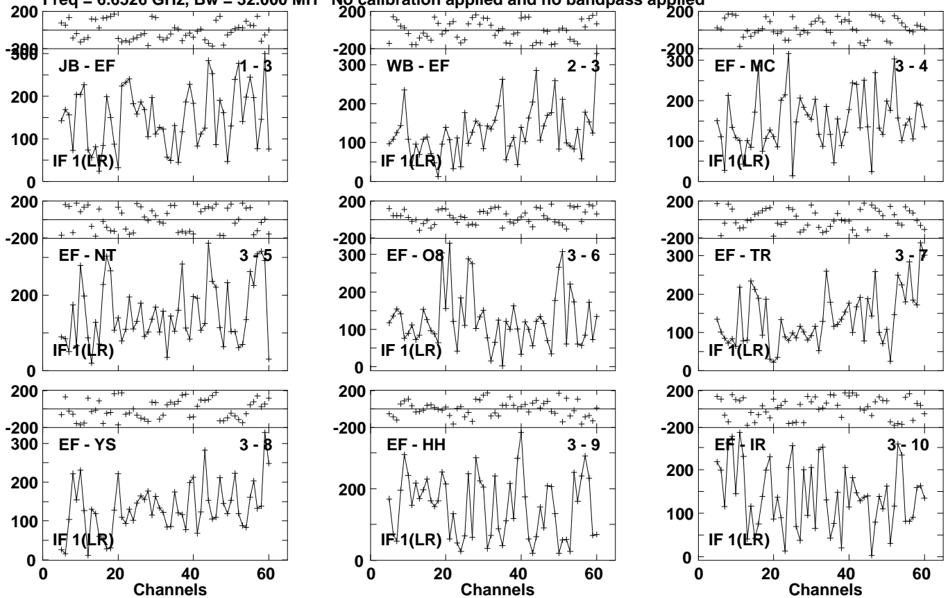
Lower frame: Micro Ampl Jy Top frame: Phas deg Vector averaged cross-power spectrum Several baselines displayed Timerange: 01/01:37:09 to 01/01:39:29
