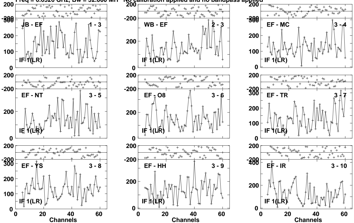
Lower frame: Micro Ampl Jy Top frame: Phas deg Vector averaged cross-power spectrum Several baselines displayed Timerange: 01/05:37:25 to 01/05:39:45
