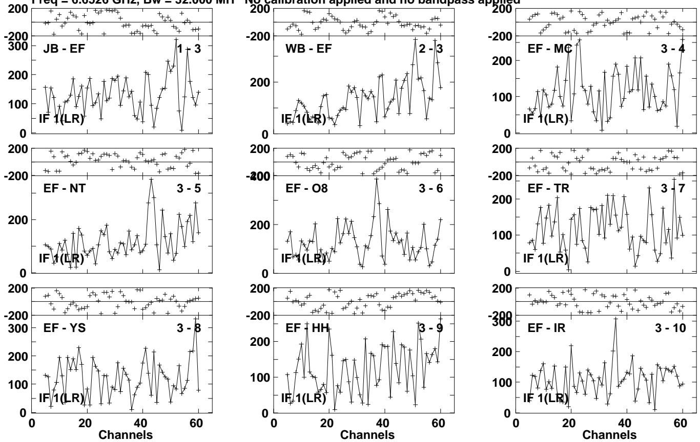
Lower frame: Micro Ampl Jy Top frame: Phas deg Vector averaged cross-power spectrum Several baselines displayed Timerange: 01/05:55:55 to 01/05:58:15
