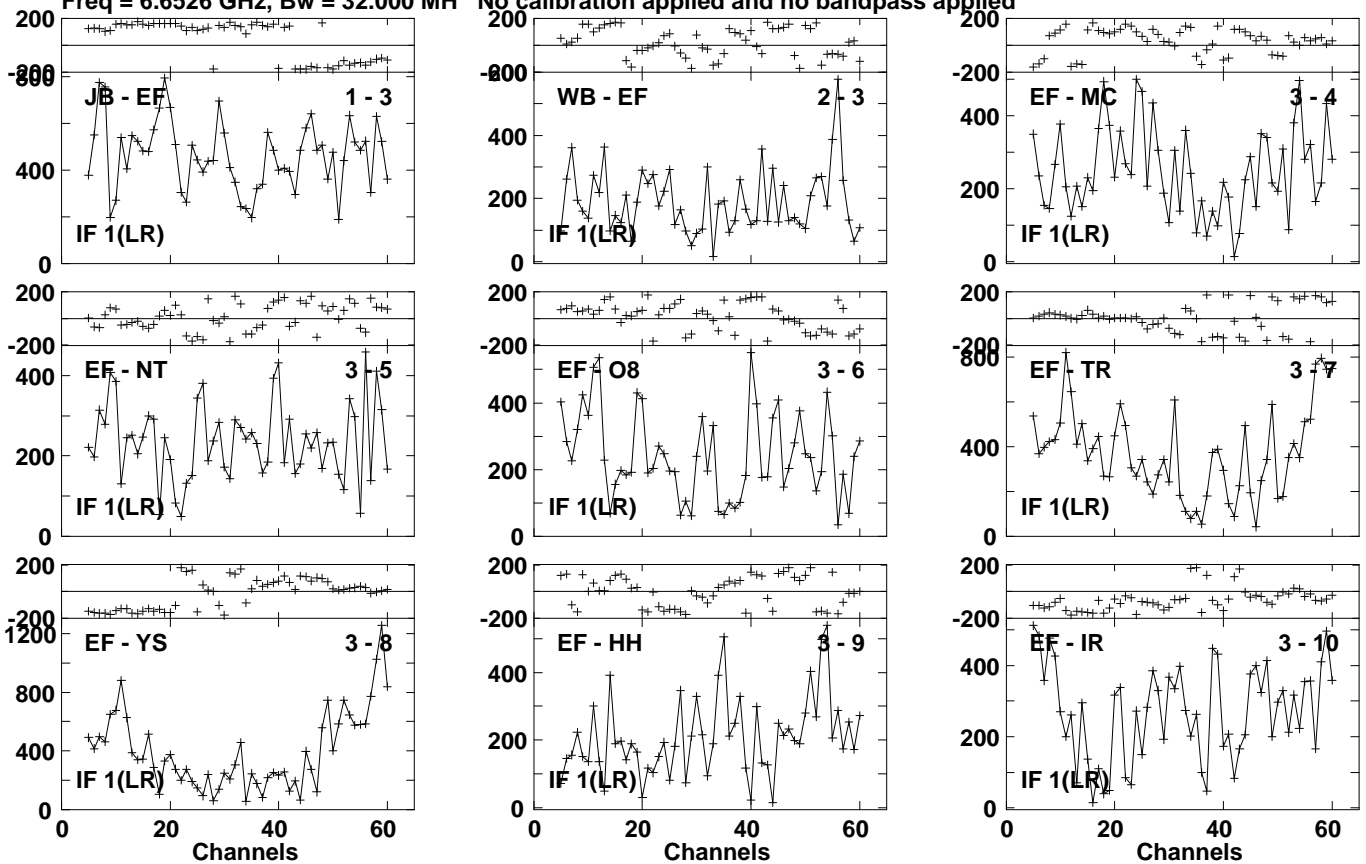
Lower frame: Micro Ampl Jy Top frame: Phas deg Vector averaged cross-power spectrum Several baselines displayed Timerange: 01/05:35:35 to 01/05:37:13
