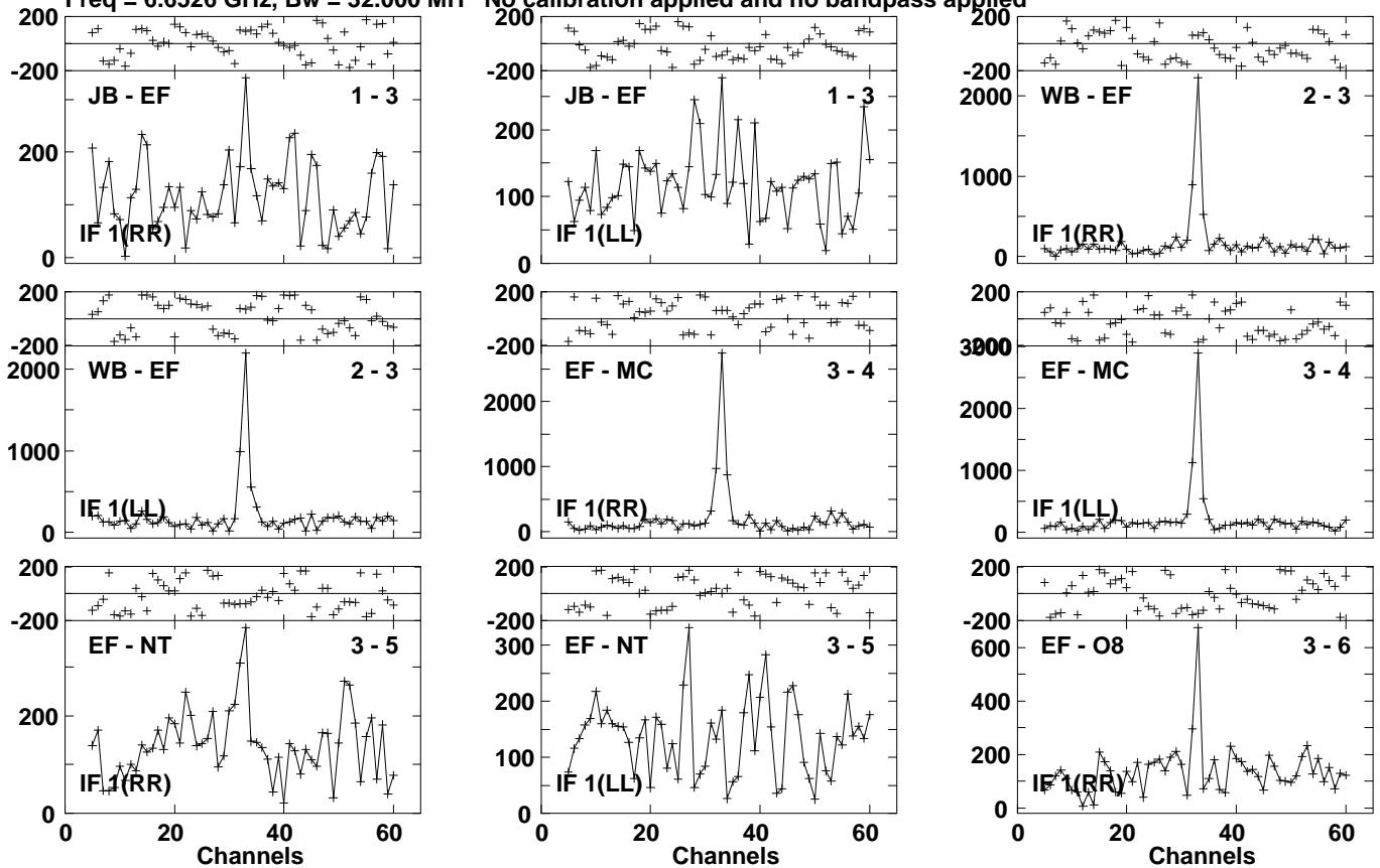
Lower frame: Micro Ampl Jy Top frame: Phas deg Vector averaged cross-power spectrum Several baselines displayed Timerange: 01/06:33:03 to 01/06:35:23
