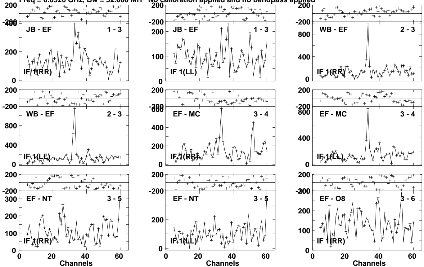
Lower frame: Micro Ampl Jy Top frame: Phas deg Vector averaged cross-power spectrum Several baselines displayed Timerange: 01/00:32:47 to 01/00:35:07
