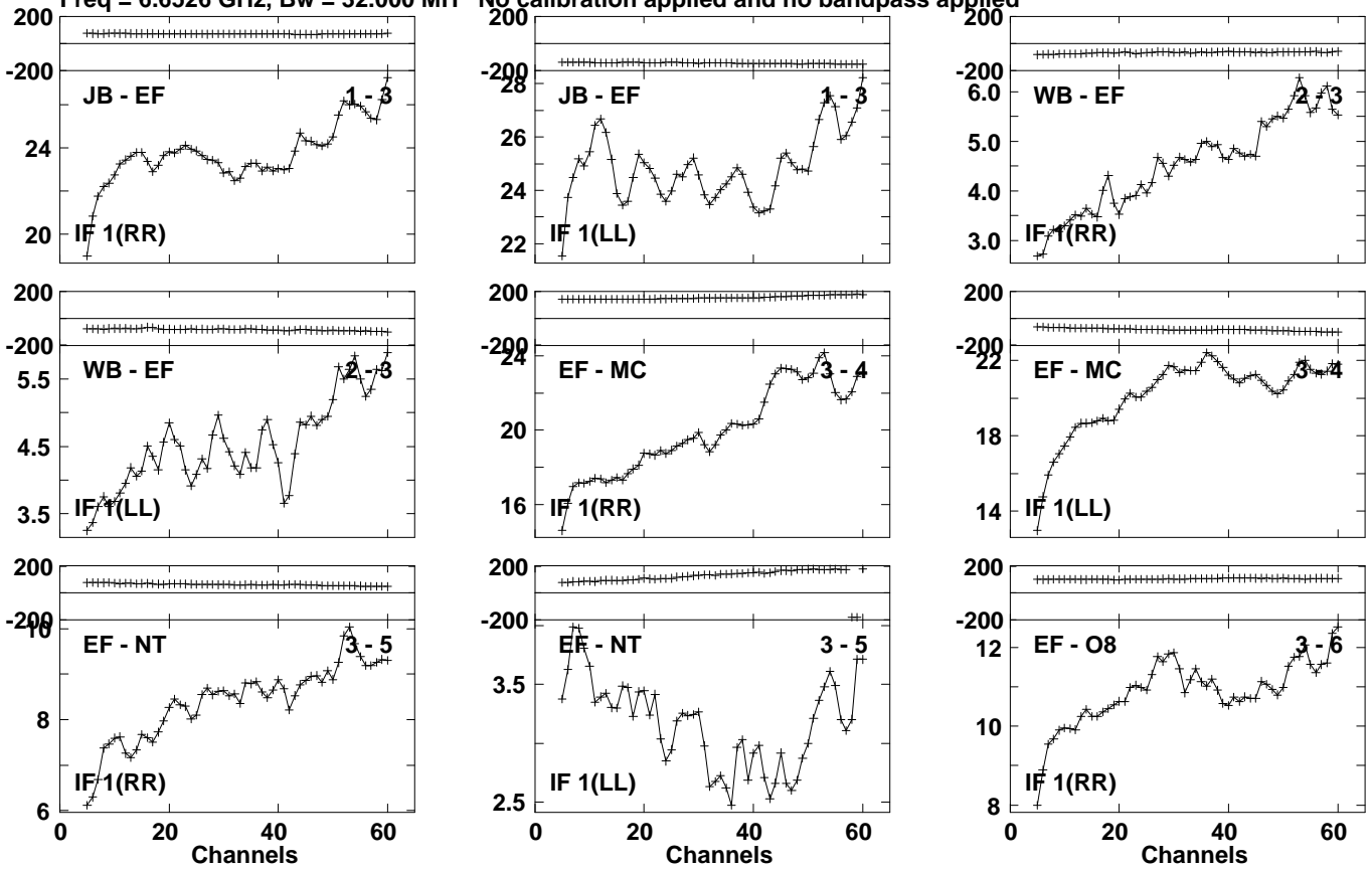
Lower frame: Milli Ampl Jy Top frame: Phas deg Vector averaged cross-power spectrum Several baselines displayed Timerange: 01/06:19:23 to 01/06:19:51
