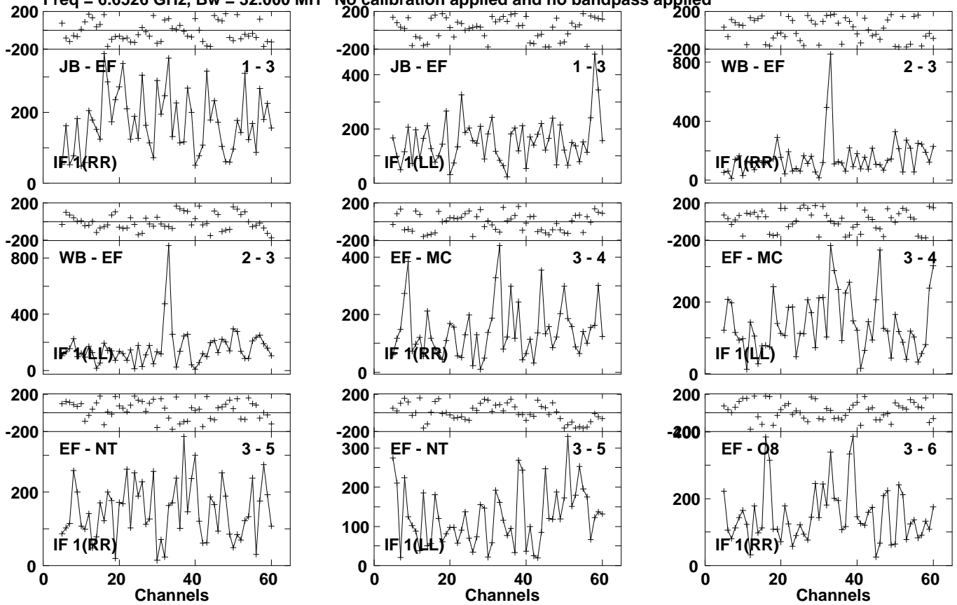
Lower frame: Micro Ampl Jy Top frame: Phas deg Vector averaged cross-power spectrum Several baselines displayed Timerange: 01/00:41:31 to 01/00:43:51
