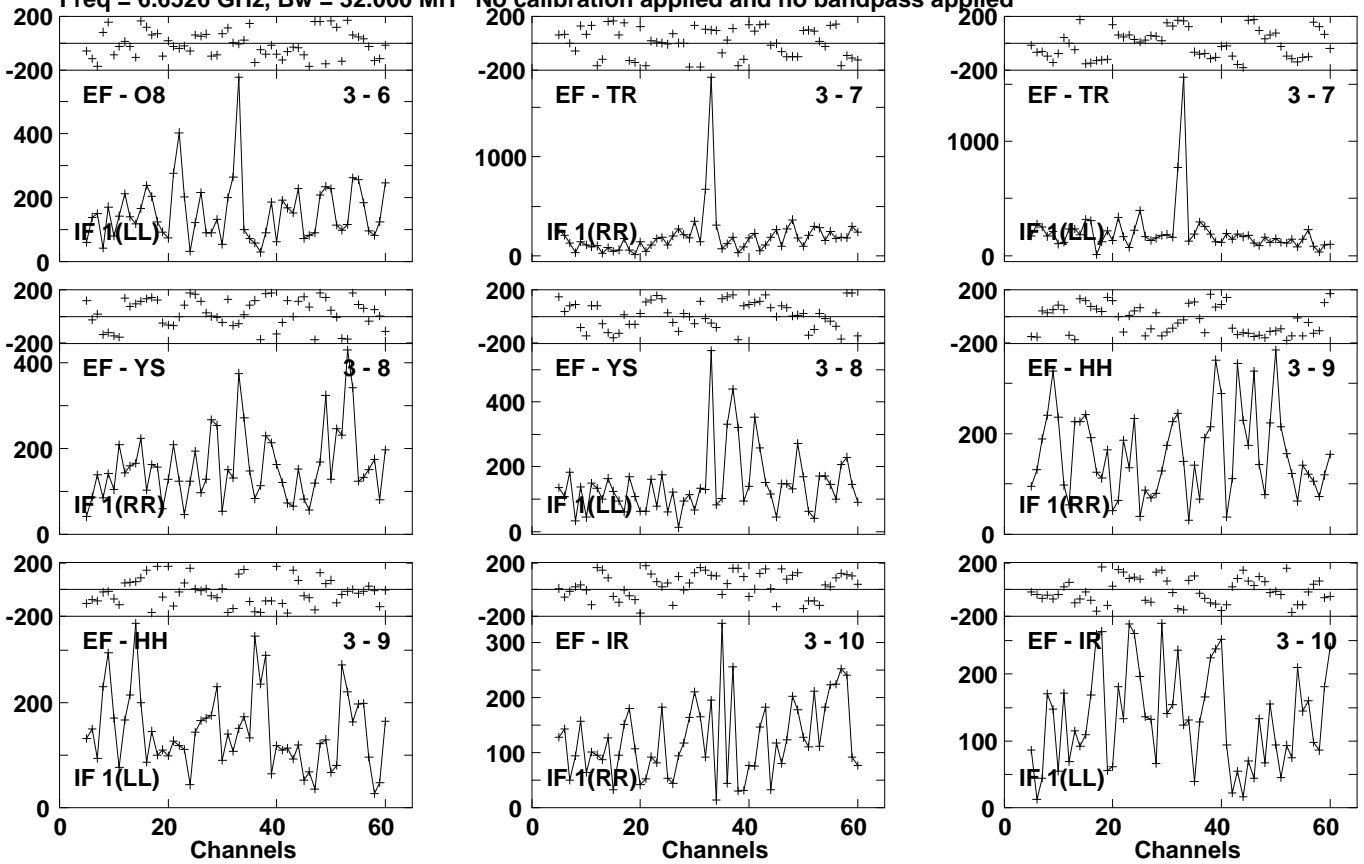
Lower frame: Micro Ampl Jy Top frame: Phas deg Vector averaged cross-power spectrum Several baselines displayed Timerange: 01/00:25:43 to 01/00:28:03
