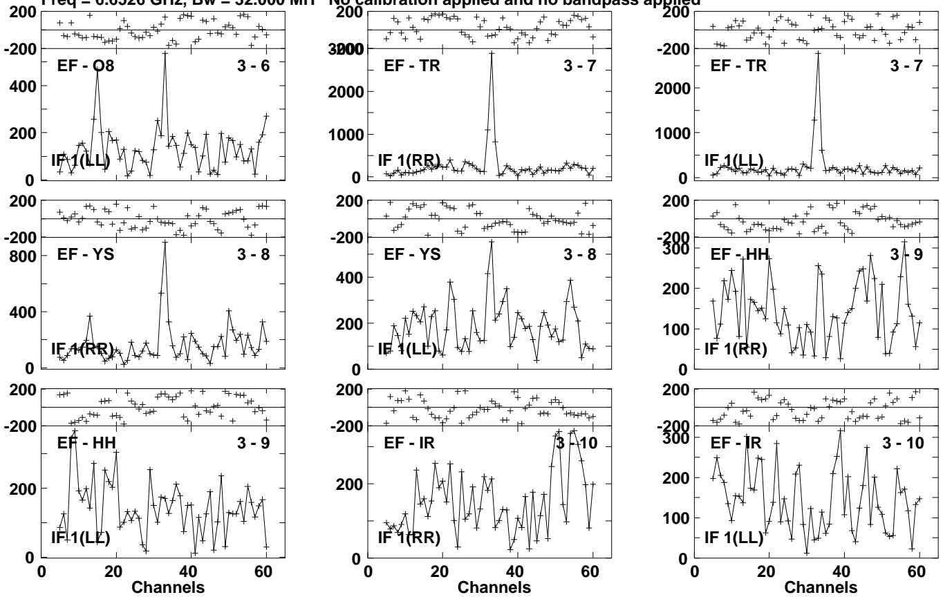
Lower frame: Micro Ampl Jy Top frame: Phas deg Vector averaged cross-power spectrum Several baselines displayed Timerange: 01/00:48:35 to 01/00:50:55
