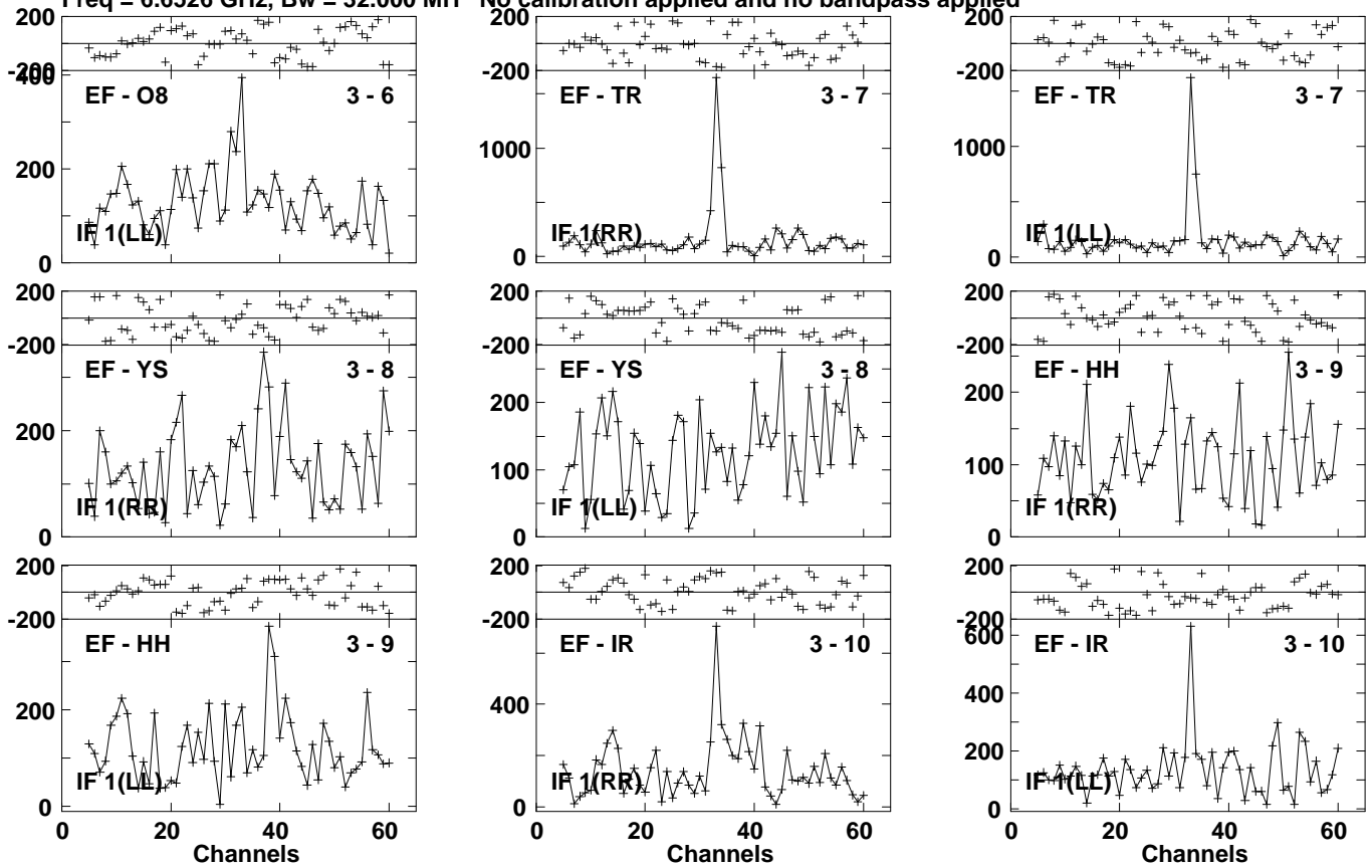
Lower frame: Micro Ampl Jy Top frame: Phas deg Vector averaged cross-power spectrum Several baselines displayed Timerange: 01/06:07:21 to 01/06:09:41
