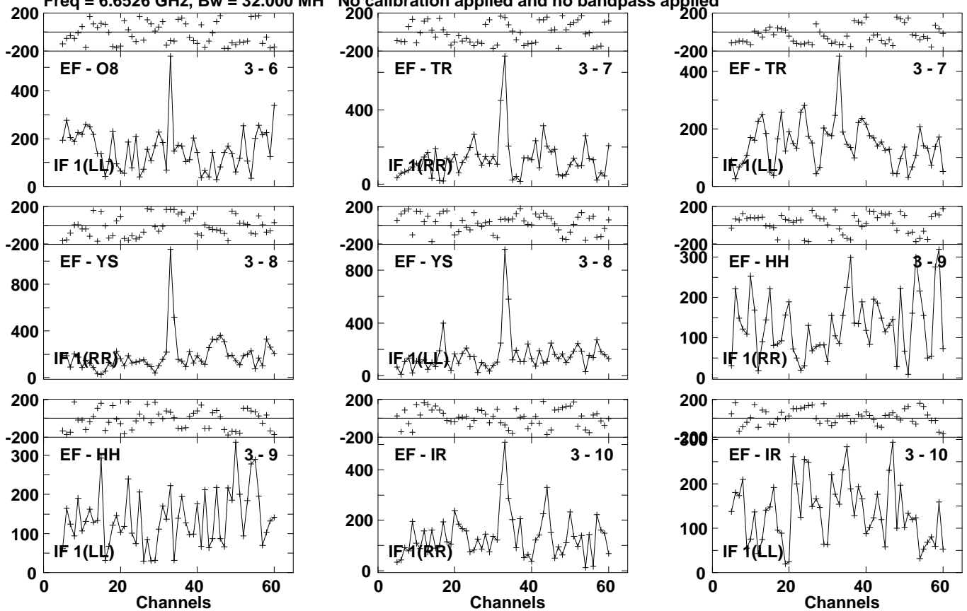
Lower frame: Micro Ampl Jy Top frame: Phas deg Vector averaged cross-power spectrum Several baselines displayed Timerange: 01/06:00:17 to 01/06:02:37
