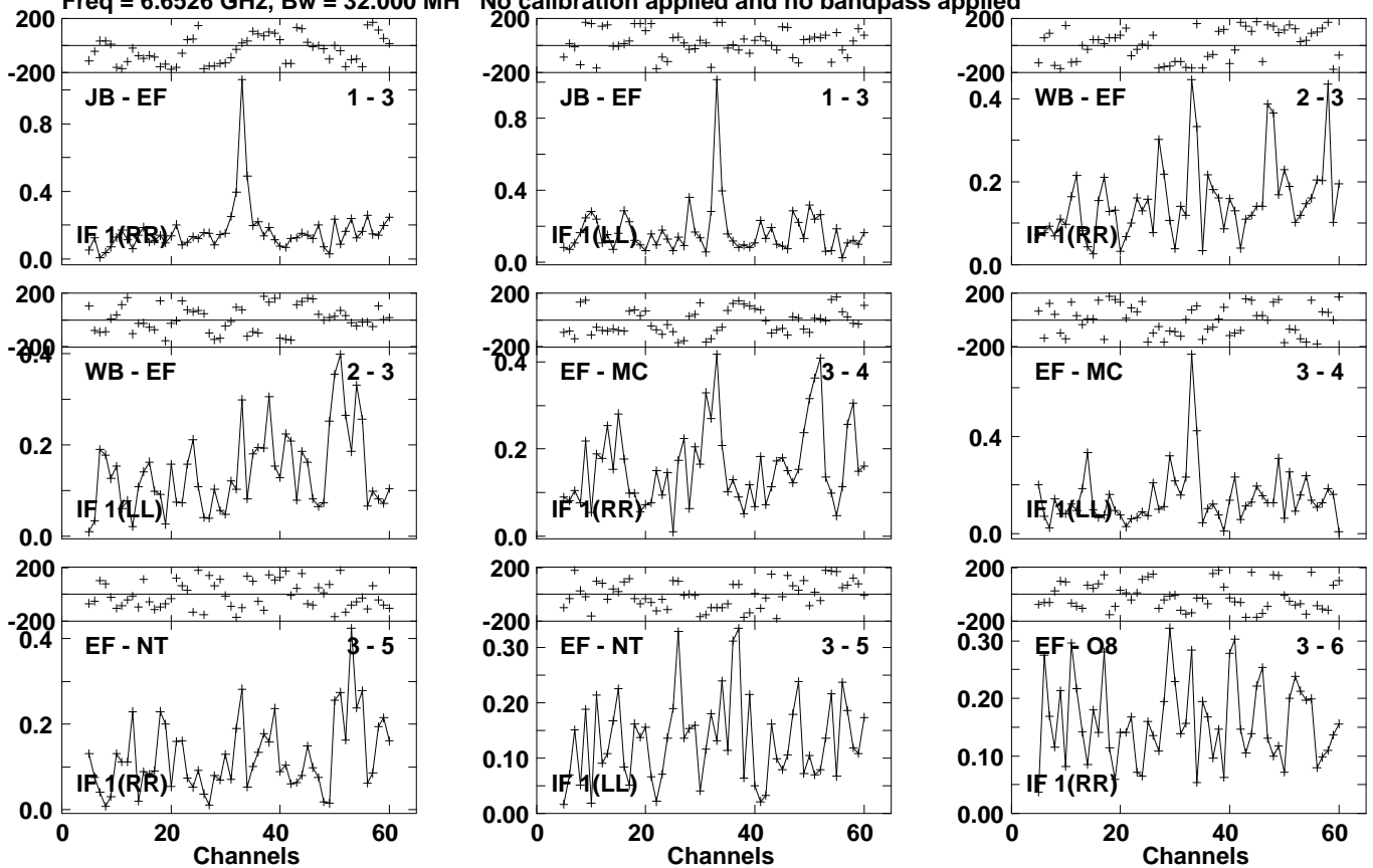
Lower frame: Milli Ampl Jy Top frame: Phas deg Vector averaged cross-power spectrum Several baselines displayed Timerange: 00/23:25:43 to 00/23:28:03
