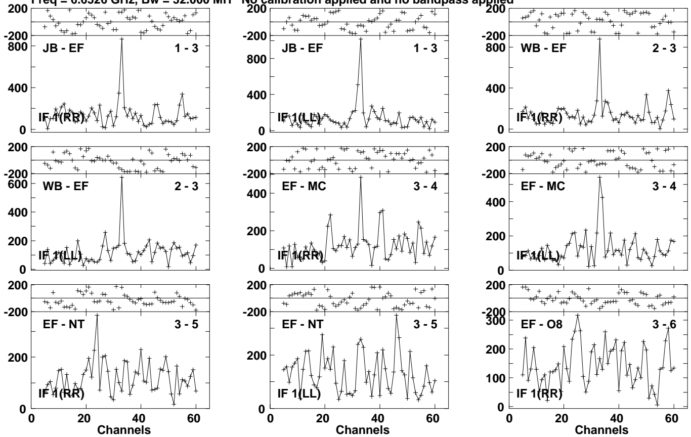
Lower frame: Micro Ampl Jy Top frame: Phas deg Vector averaged cross-power spectrum Several baselines displayed Timerange: 01/00:21:21 to 01/00:23:41
