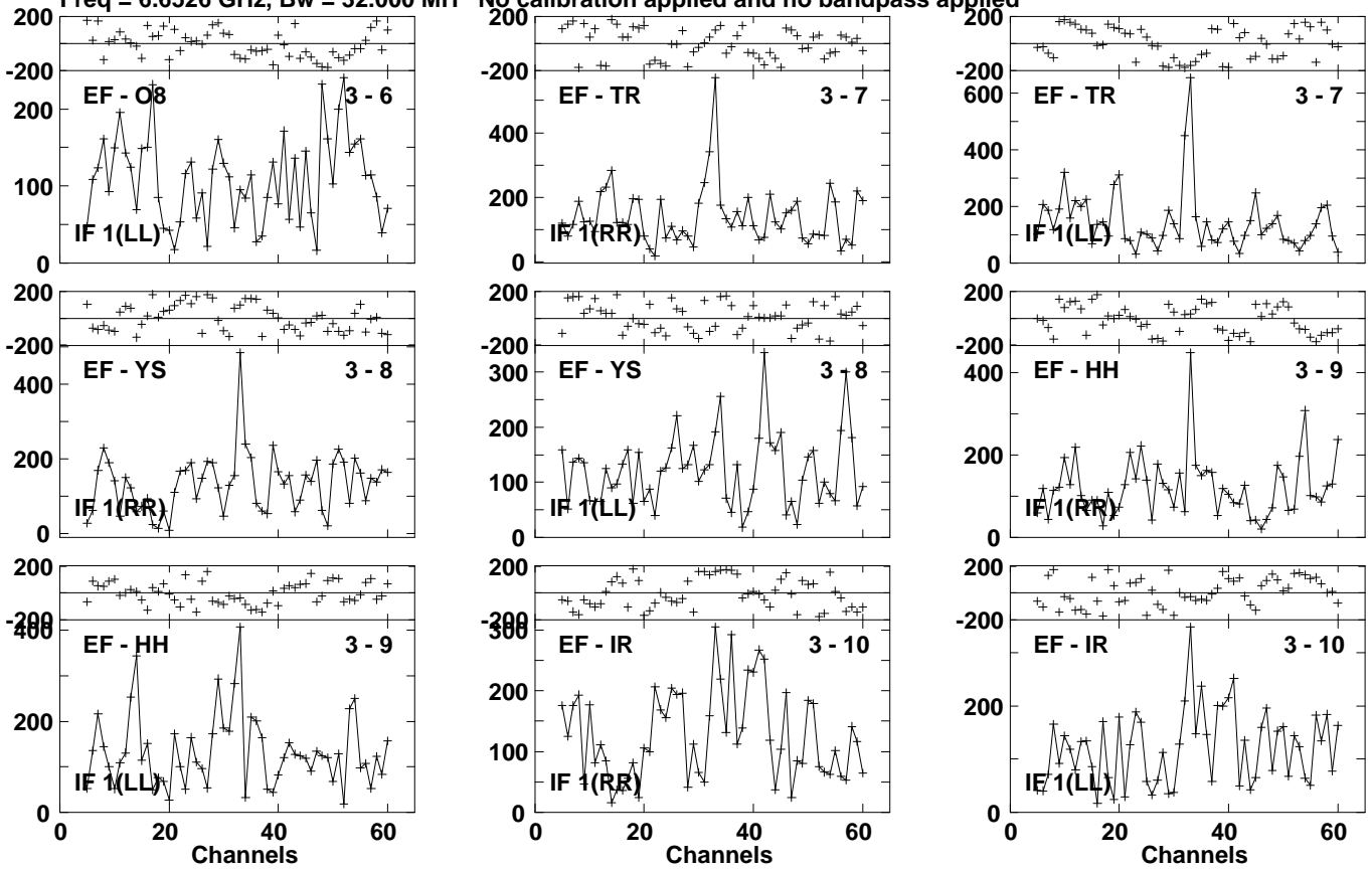
Lower frame: Micro Ampl Jy Top frame: Phas deg Vector averaged cross-power spectrum Several baselines displayed Timerange: 01/04:44:29 to 01/04:46:49
