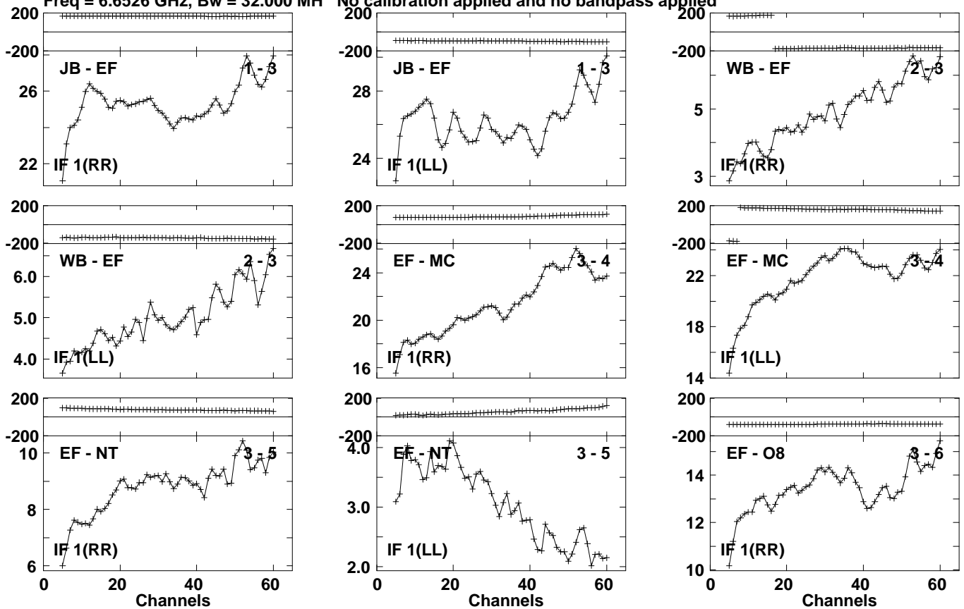
Lower frame: Milli Ampl Jy Top frame: Phas deg Vector averaged cross-power spectrum Several baselines displayed Timerange: 01/03:19:23 to 01/03:19:51
