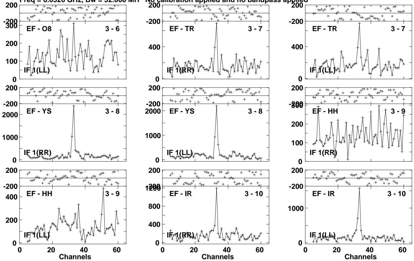
Lower frame: Micro Ampl Jy Top frame: Phas deg Vector averaged cross-power spectrum Several baselines displayed Timerange: 01/00:14:17 to 01/00:16:37
