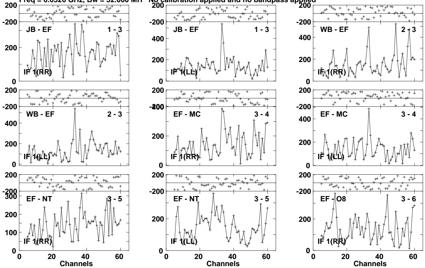
Lower frame: Micro Ampl Jy Top frame: Phas deg Vector averaged cross-power spectrum Several baselines displayed Timerange: 01/06:41:47 to 01/06:44:07
