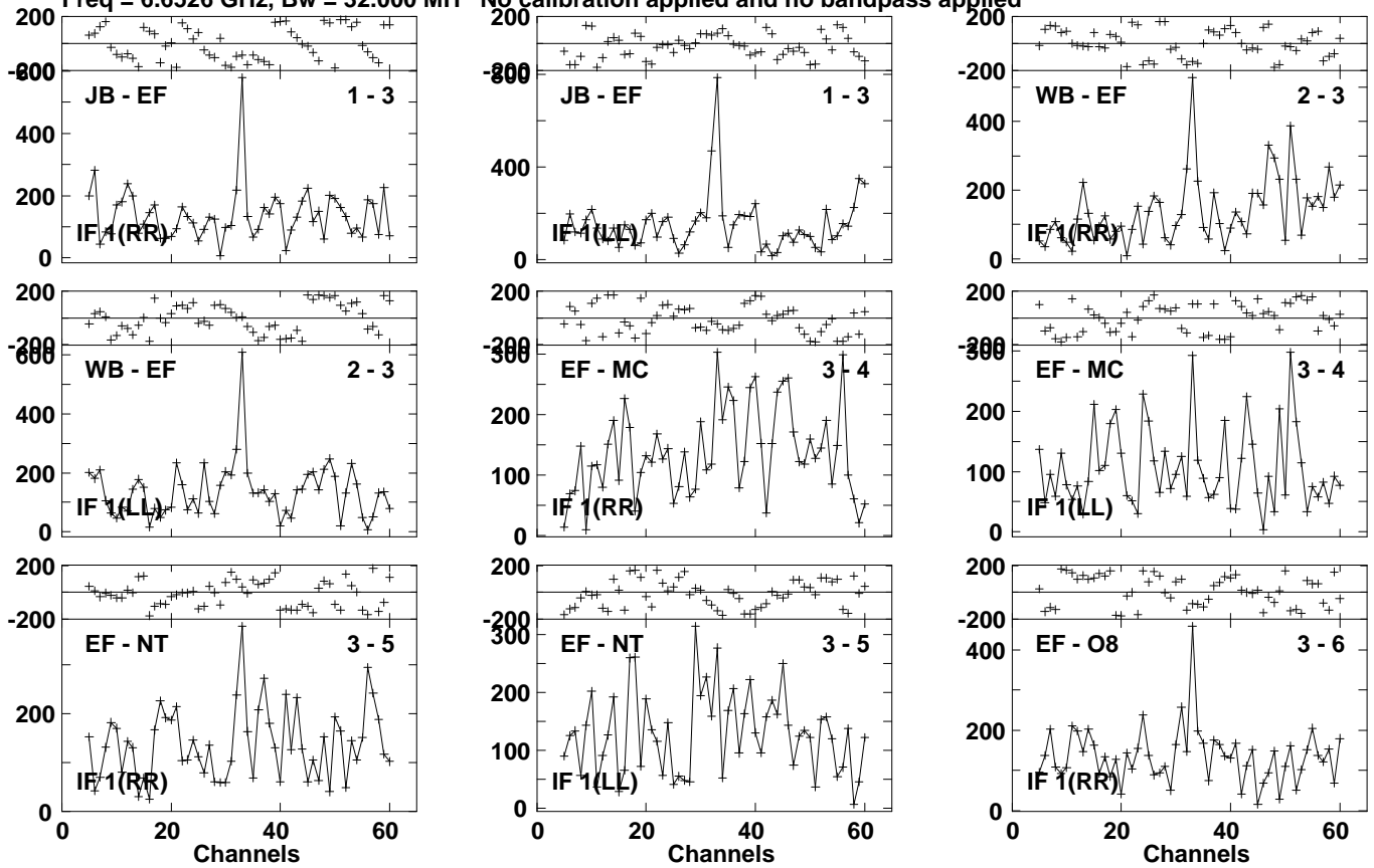
Lower frame: Micro Ampl Jy Top frame: Phas deg Vector averaged cross-power spectrum Several baselines displayed Timerange: 01/00:44:13 to 01/00:46:33
