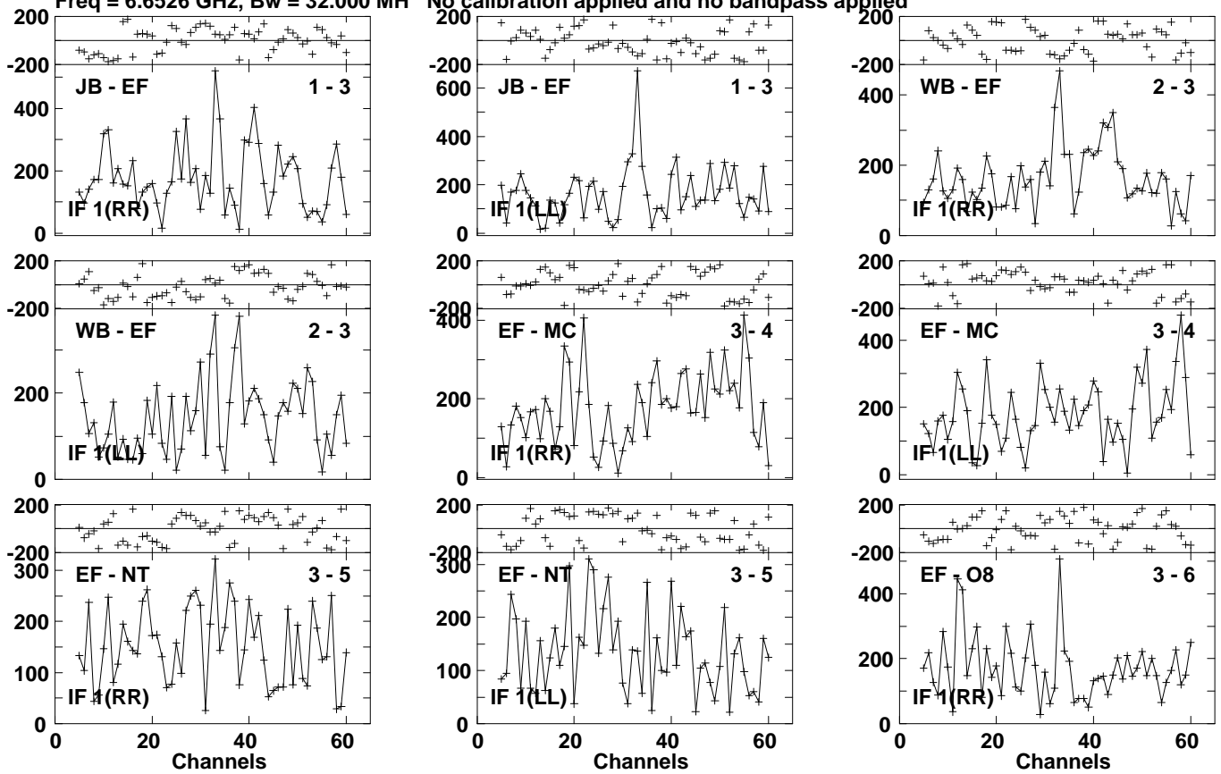
Lower frame: Micro Ampl Jy Top frame: Phas deg Vector averaged cross-power spectrum Several baselines displayed Timerange: 00/23:48:35 to 00/23:50:55
