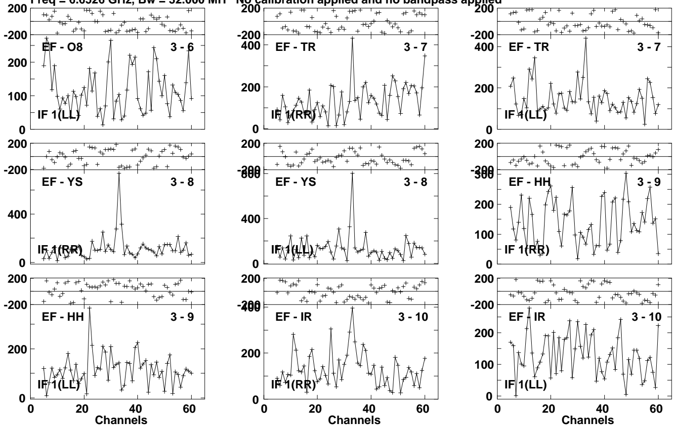
Lower frame: Micro Ampl Jy Top frame: Phas deg Vector averaged cross-power spectrum Several baselines displayed Timerange: 01/02:44:13 to 01/02:46:33
