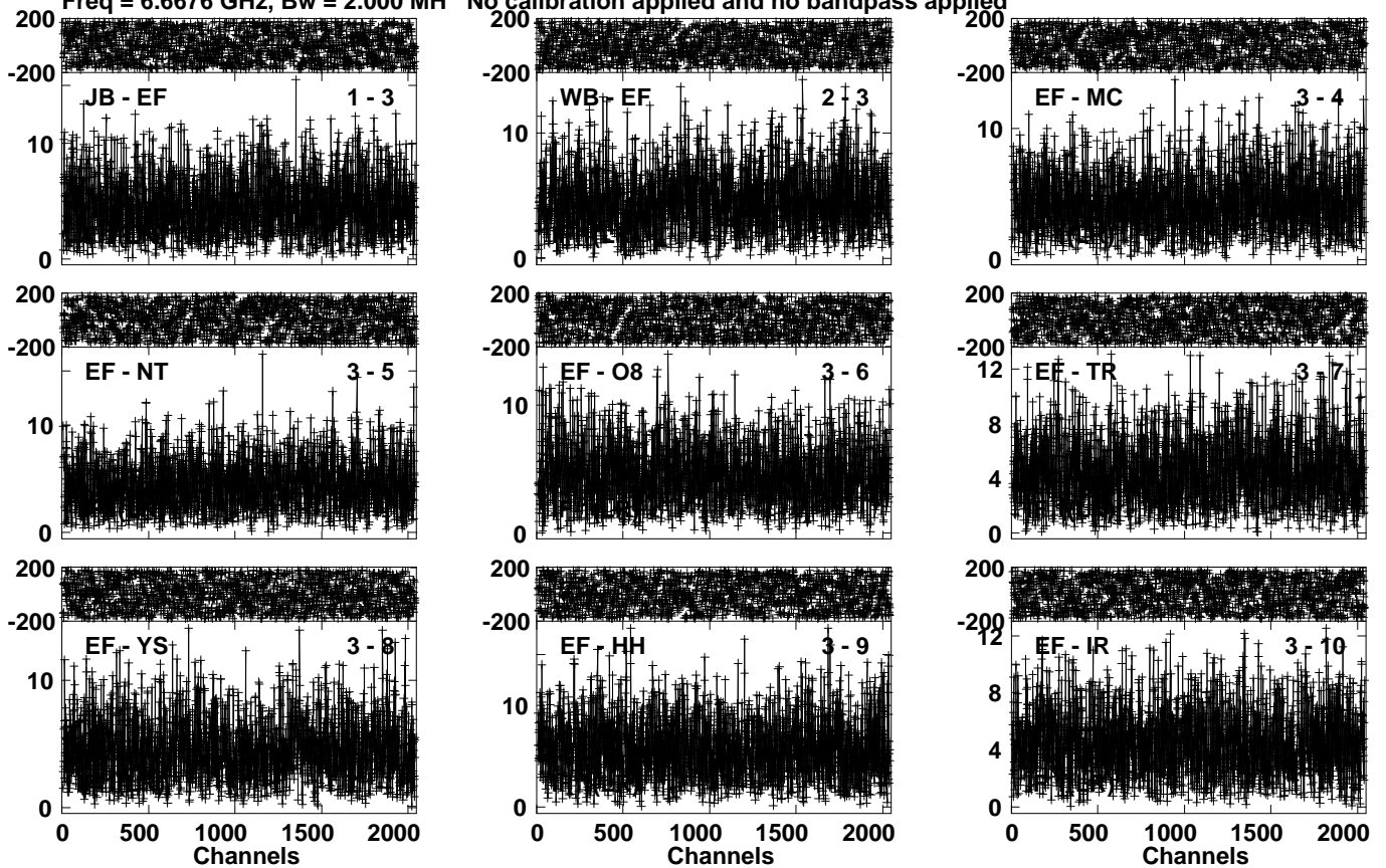
Lower frame: Milli Ampl Jy Top frame: Phas deg Vector averaged cross-power spectrum Several baselines displayed Timerange: 00/23:28:15 to 00/23:29:53
