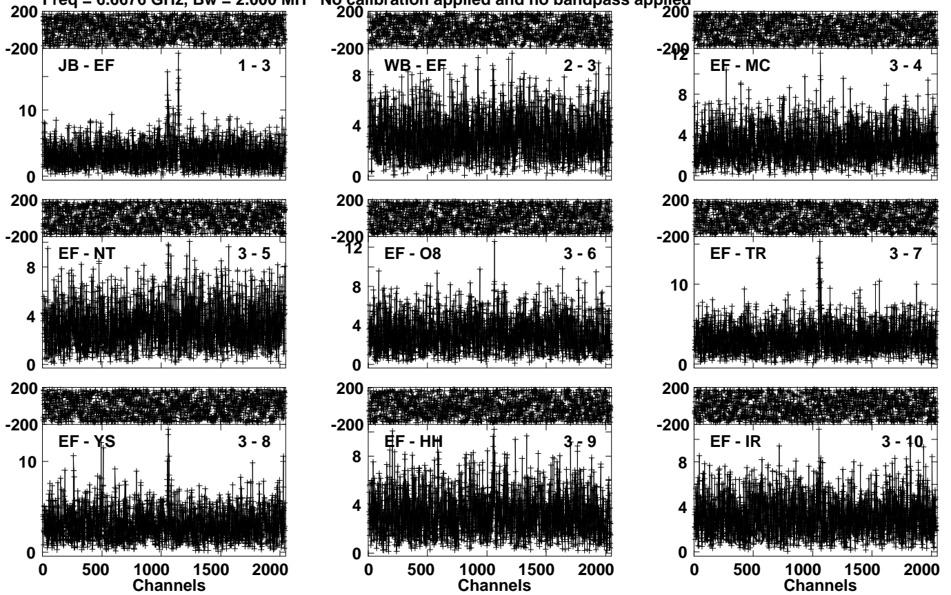
Lower frame: Milli Ampl Jy Top frame: Phas deg Vector averaged cross-power spectrum Several baselines displayed Timerange: 01/01:52:57 to 01/01:55:17
