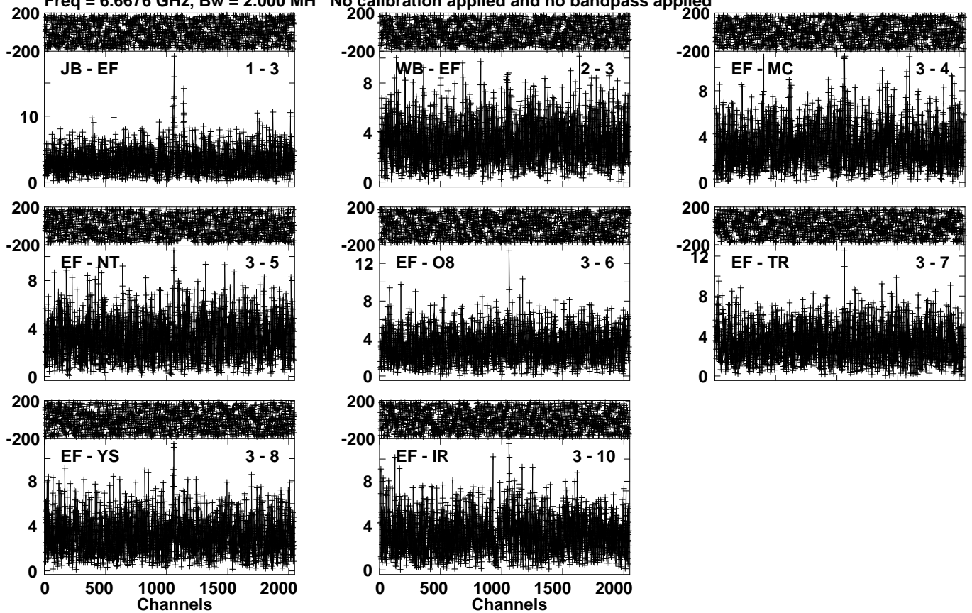
Lower frame: Milli Ampl Jy Top frame: Phas deg Vector averaged cross-power spectrum Several baselines displayed Timerange: 01/06:37:25 to 01/06:39:45
