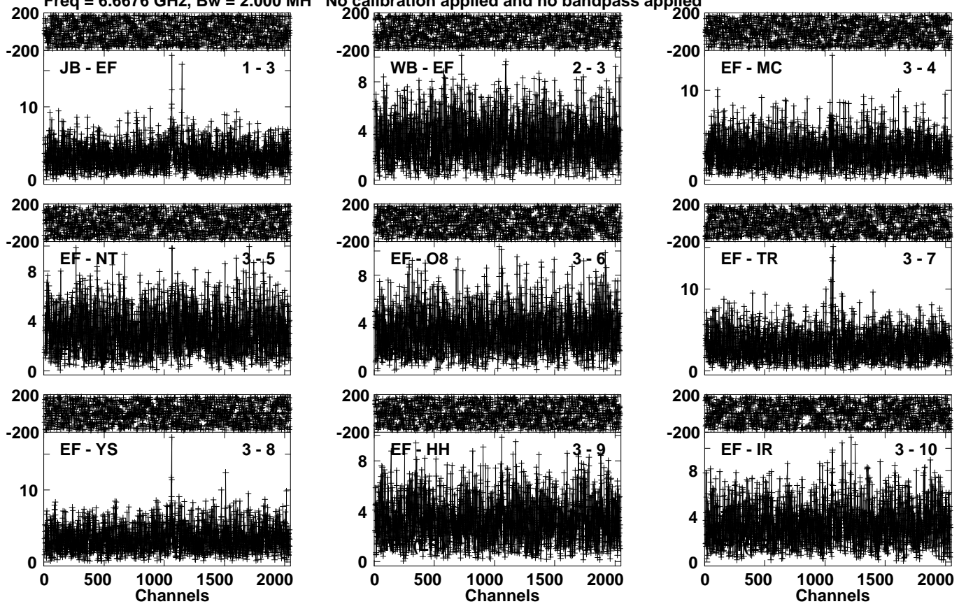
Lower frame: Milli Amp Jy Top frame: Phas deg Vector averaged cross-power spectrum Several baselines displayed Timerange: 00/23:25:43 to 00/23:28:03
