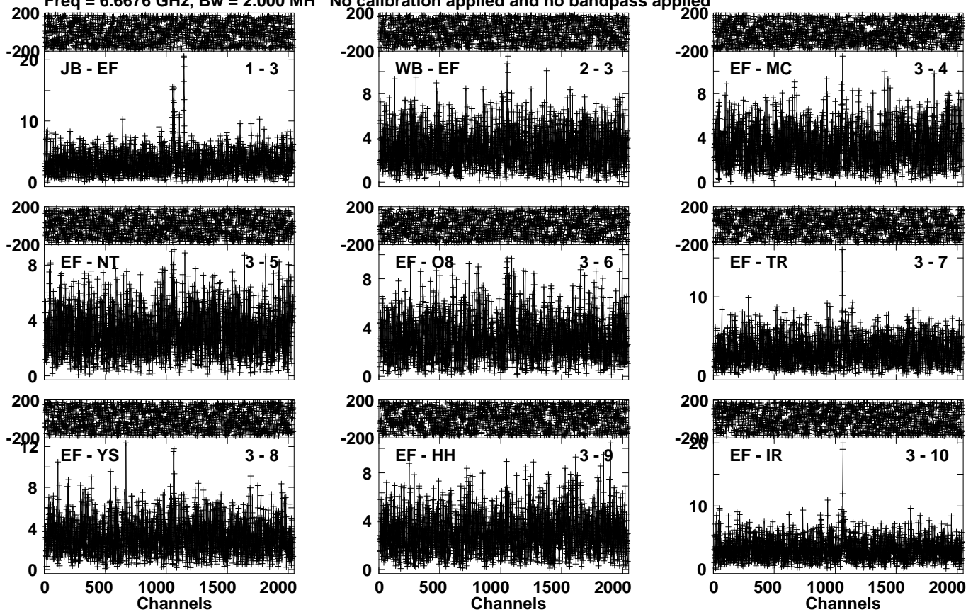
Lower frame: Milli Ampl Jy Top frame: Phas deg Vector averaged cross-power spectrum Several baselines displayed Timerange: 01/01:48:35 to 01/01:50:55
