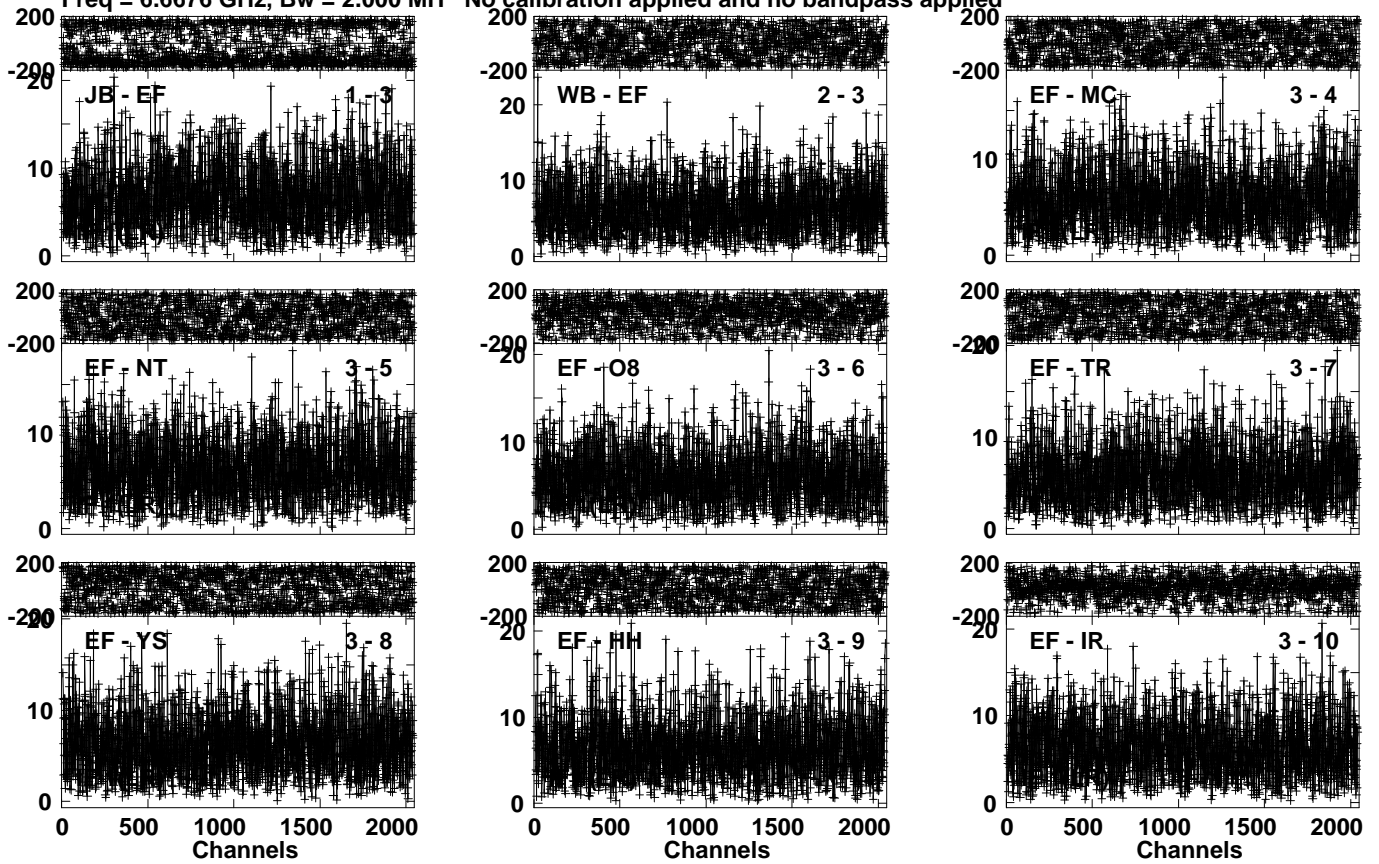
Lower frame: Milli Ampl Jy Top frame: Phas deg Vector averaged cross-power spectrum Several baselines displayed Timerange: 01/00:07:41 to 01/00:08:09
