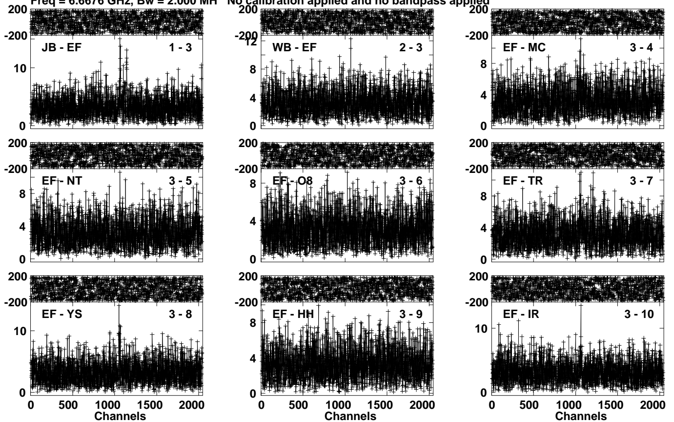
Lower frame: Milli Amp Jy Top frame: Phas deg Vector averaged cross-power spectrum Several baselines displayed Timerange: 00/23:41:31 to 00/23:43:51
