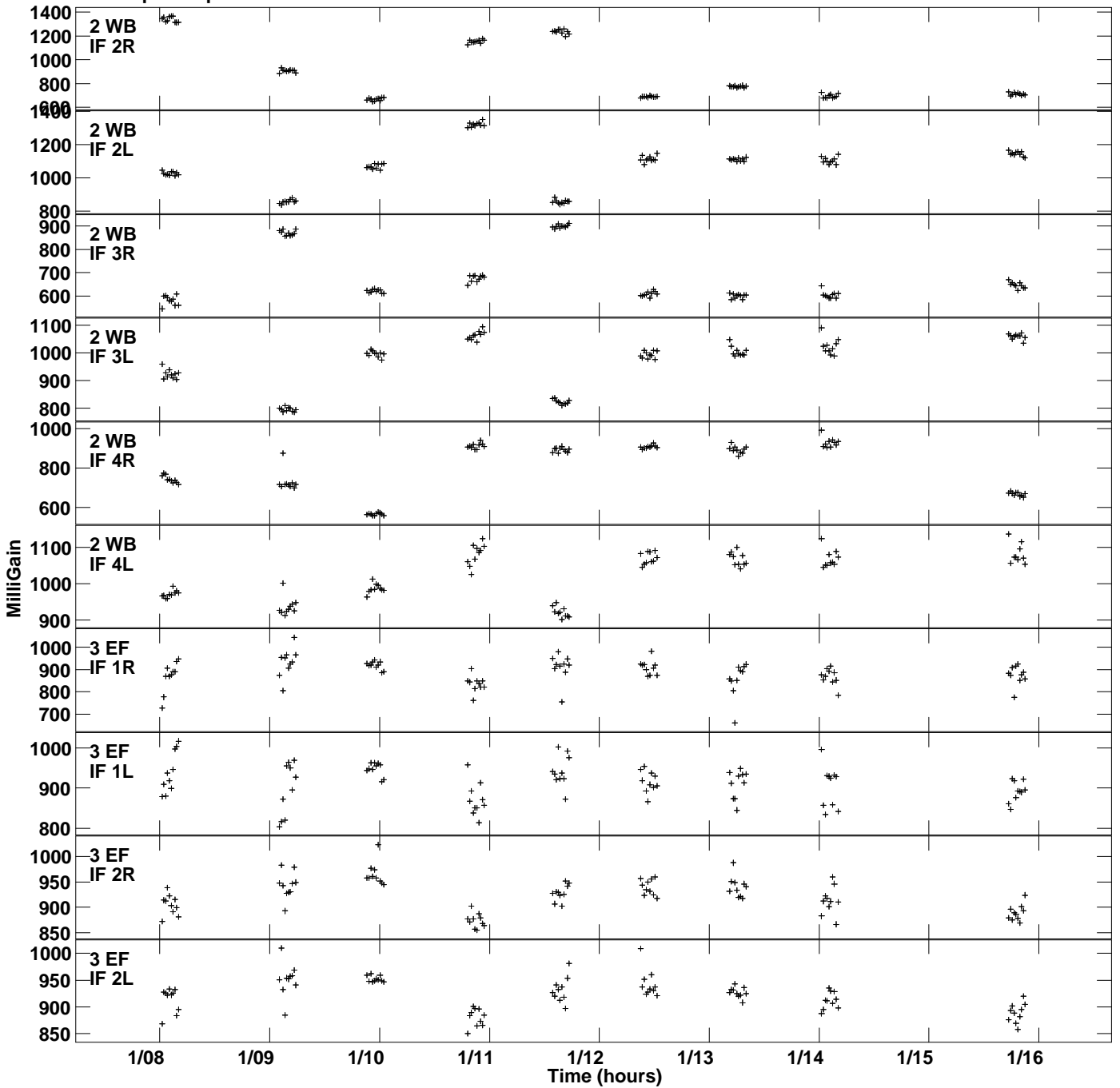
Plot file version 2 created 15-MAR-2022 21:15:05 Gain amp vs UTC time for 3C338.MULTI.1 SN 2 Rpol & Lpol IF 1 - 4
