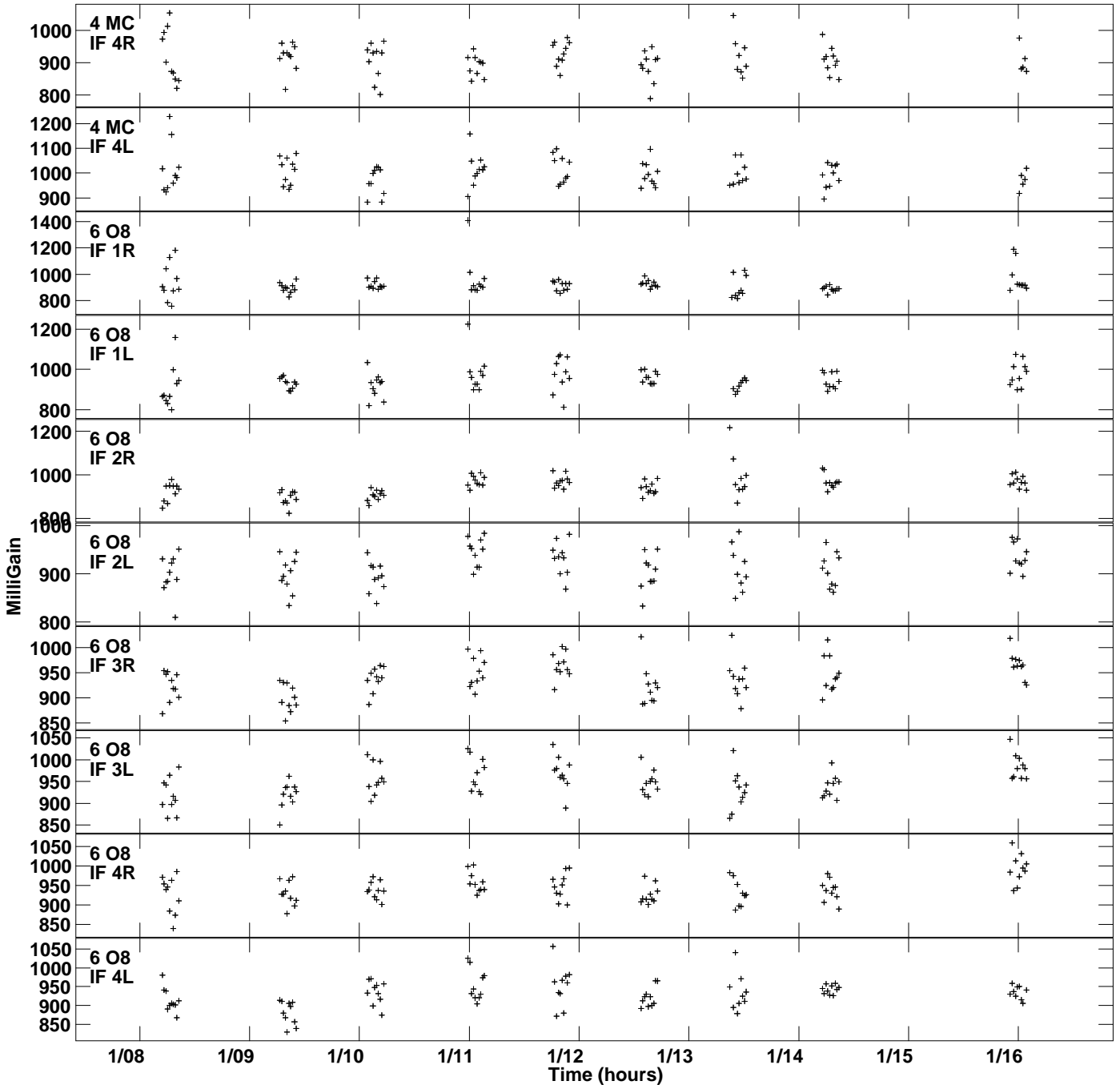
Plot file version 4 created 15-MAR-2022 21:13:46 Gain amp vs UTC time for 4C30.31.MULTI.1 SN 2 Rpol & Lpol IF 1 - 4
