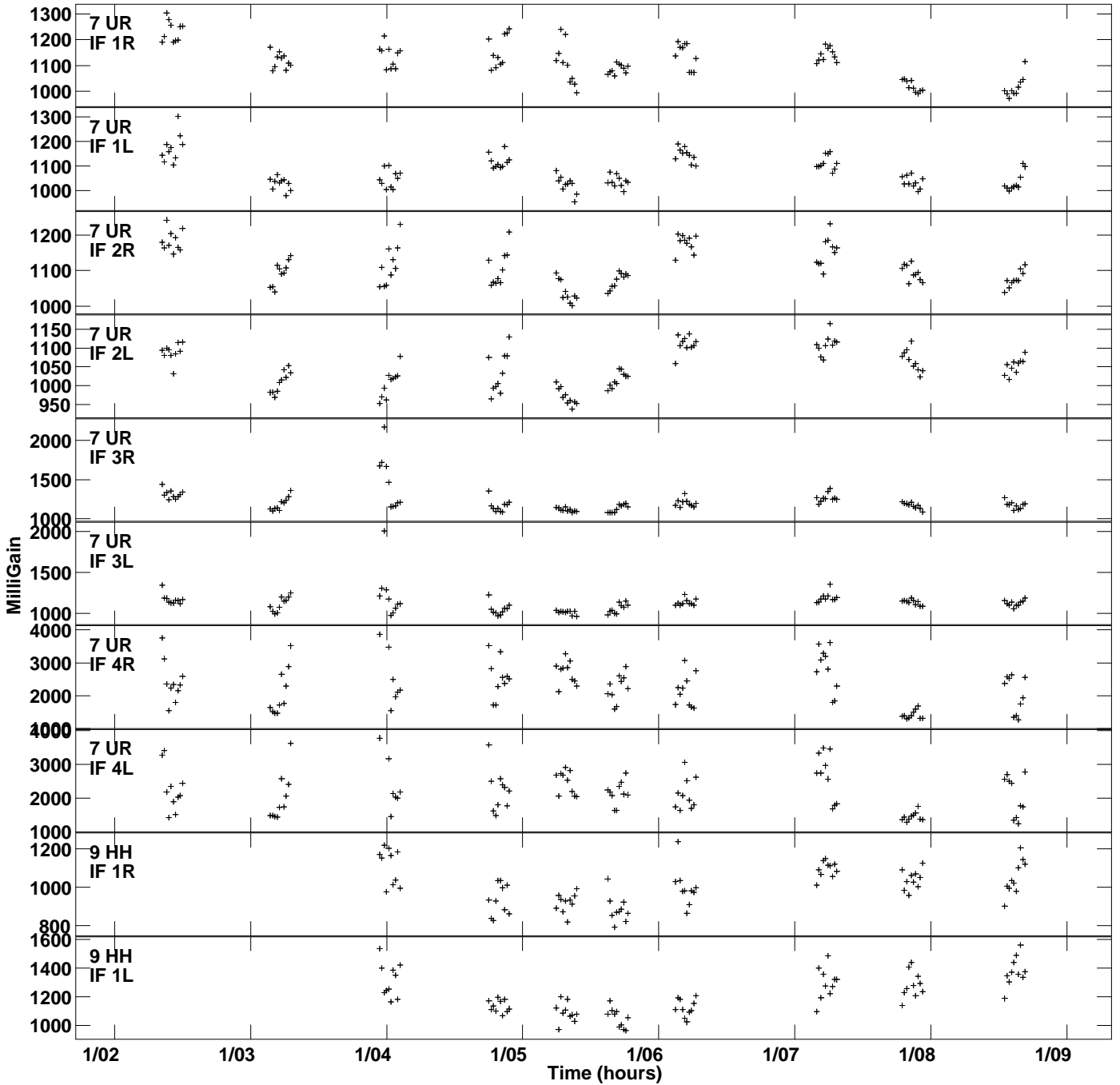
Plot file version 5 created 15-MAR-2022 21:16:06 Gain amp vs UTC time for NGC4278.MULTI.1 SN 2 Rpol & Lpol IF 1 - 4
