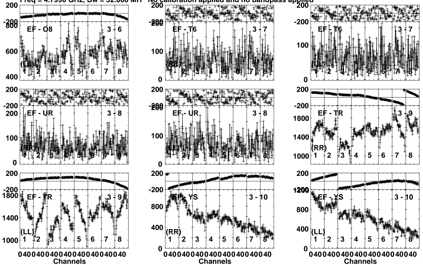
Lower frame: Micro Ampl Jy Top frame: Phas deg Vector averaged cross-power spectrum Several baselines displayed Timerange: 00/21:15:38 to 00/21:20:36
