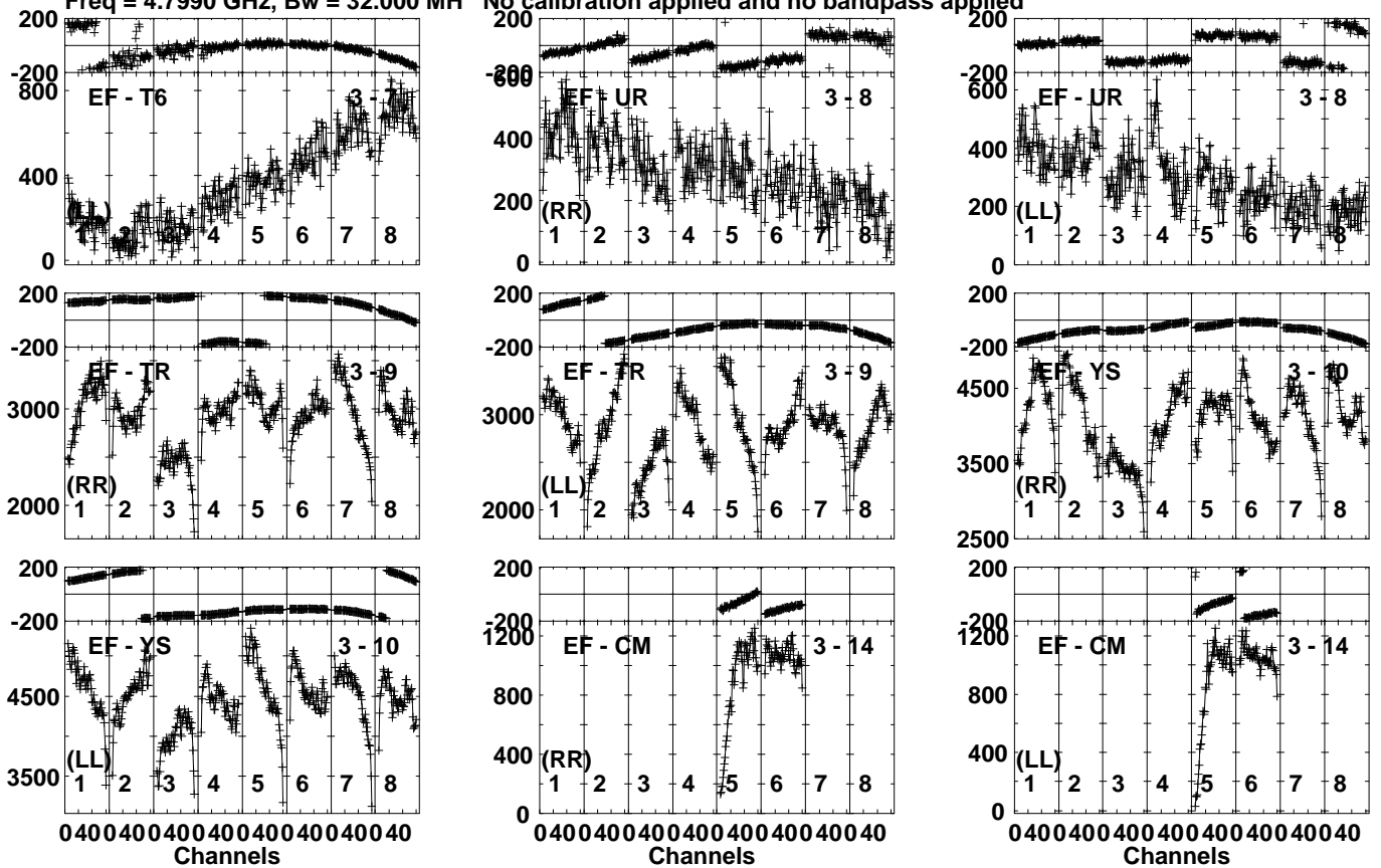
Lower frame: Micro Ampl Jy Top frame: Phas deg Vector averaged cross-power spectrum Several baselines displayed Timerange: 00/18:54:57 to 00/18:57:55
