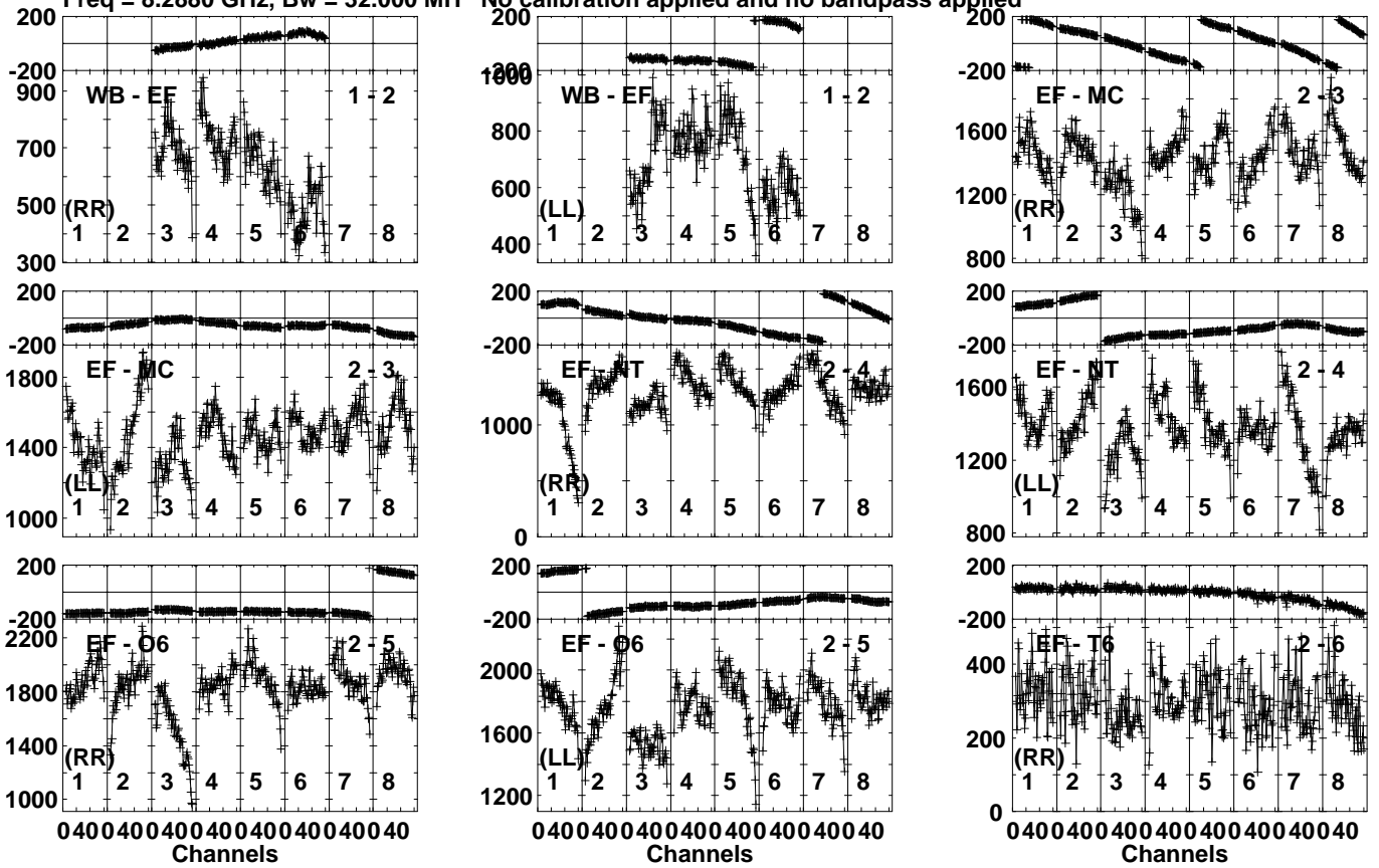
Lower frame: Micro Ampl Jy Top frame: Phas deg Vector averaged cross-power spectrum Several baselines displayed Timerange: 00/06:45:25 to 00/06:48:23
