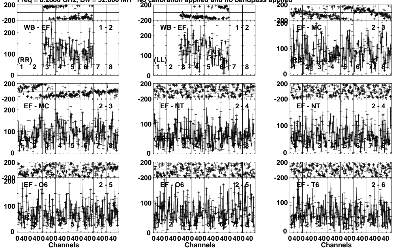
Lower frame: Micro Ampl Jy Top frame: Phas deg Vector averaged cross-power spectrum Several baselines displayed Timerange: 00/09:01:07 to 00/09:06:05
