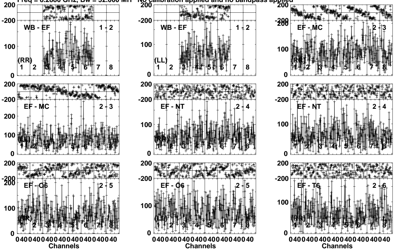
Lower frame: Micro Ampl Jy Top frame: Phas deg Vector averaged cross-power spectrum Several baselines displayed Timerange: 00/05:12:02 to 00/05:17:00
