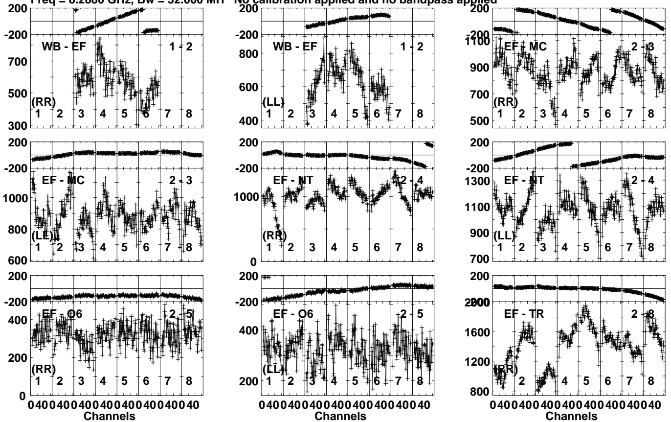
Lower frame: Micro Ampl Jy Top frame: Phas deg Vector averaged cross-power spectrum Several baselines displayed Timerange: 00/10:52:35 to 00/10:57:33
