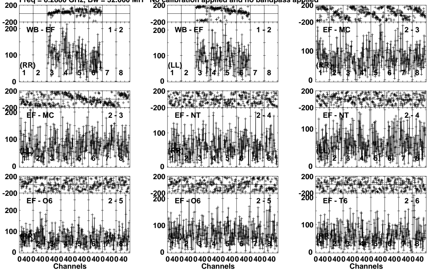
Lower frame: Micro Ampl Jy Top frame: Phas deg Vector averaged cross-power spectrum Several baselines displayed Timerange: 00/05:01:02 to 00/05:06:00
