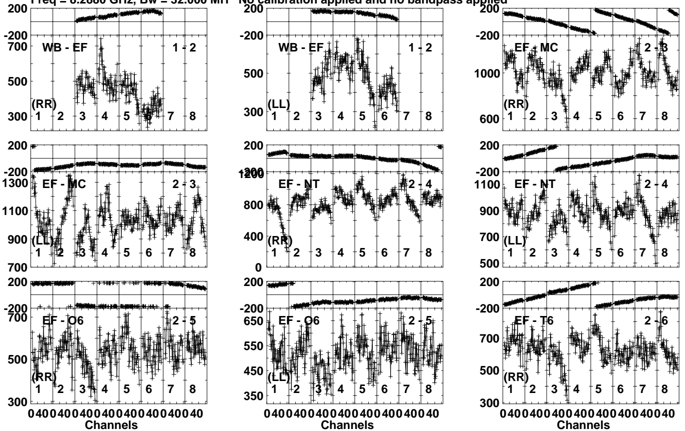
Lower frame: Micro Ampl Jy Top frame: Phas deg Vector averaged cross-power spectrum Several baselines displayed Timerange: 00/08:28:01 to 00/08:32:59
