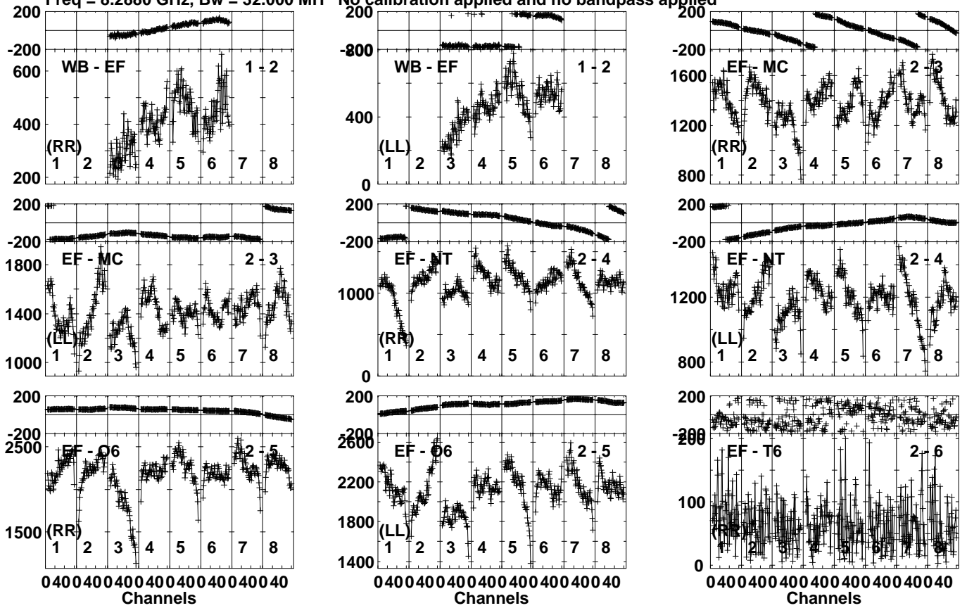
Lower frame: Micro Ampl Jy Top frame: Phas deg Vector averaged cross-power spectrum Several baselines displayed Timerange: 00/05:43:31 to 00/05:48:29
