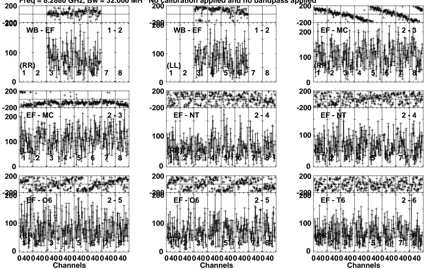
Lower frame: Micro Ampl Jy Top frame: Phas deg Vector averaged cross-power spectrum Several baselines displayed Timerange: 00/07:50:52 to 00/07:55:50
