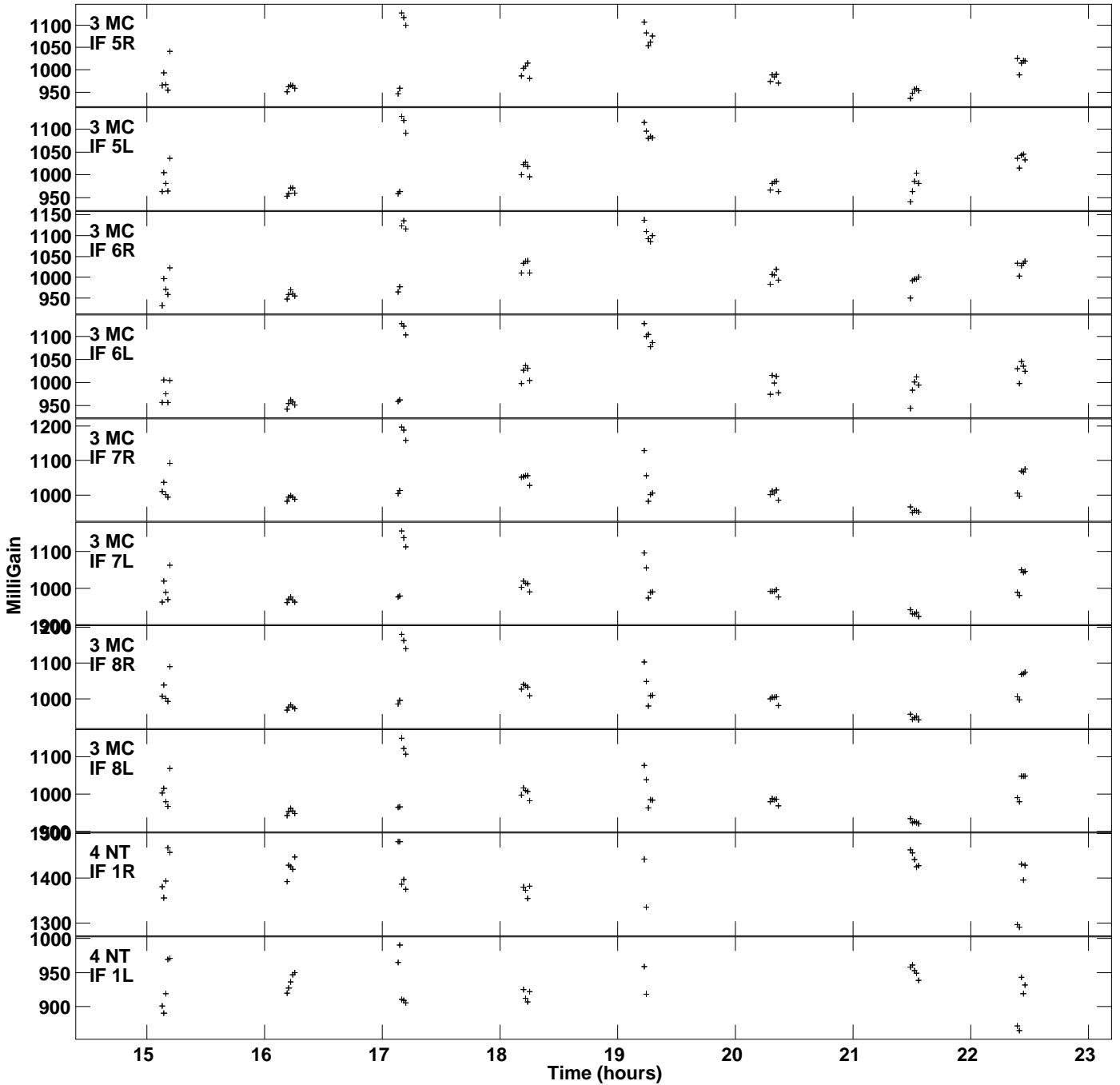
Plot file version 5 created 21-FEB-2023 17:56:15 Gain amp vs UTC time for BLLAC.MULTI.1 SN 2 Rpol & Lpol IF 1 - 8
