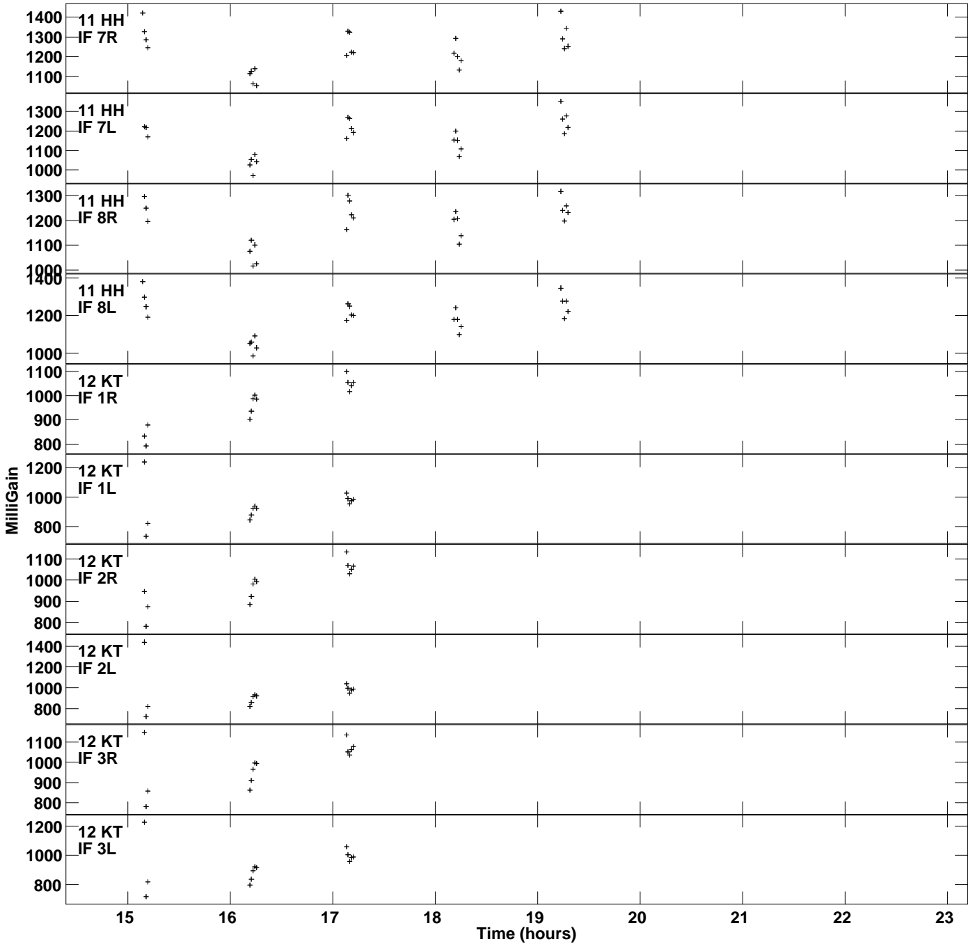
Plot file version 15 created 21-FEB-2023 17:56:15 Gain amp vs UTC time for BLLAC.MULTI.1 SN 2 Rpol & Lpol IF 1 - 8
