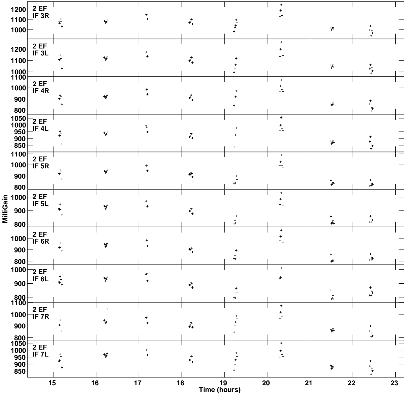
Plot file version 3 created 21-FEB-2023 17:56:15 Gain amp vs UTC time for BLLAC.MULTI.1 SN 2 Rpol & Lpol IF 1 - 8
