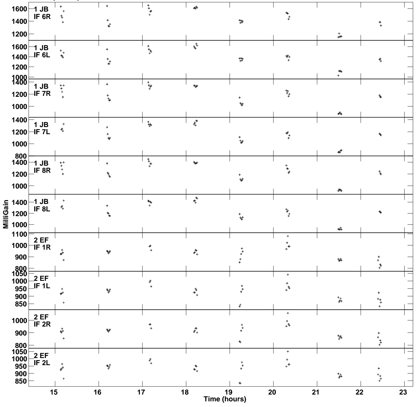
Plot file version 2 created 21-FEB-2023 17:56:15 Gain amp vs UTC time for BLLAC.MULTI.1 SN 2 Rpol & Lpol IF 1 - 8
