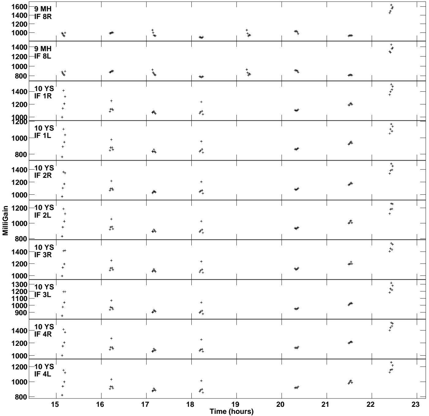
Plot file version 12 created 21-FEB-2023 17:56:15 Gain amp vs UTC time for BLLAC.MULTI.1 SN 2 Rpol & Lpol IF 1 - 8
