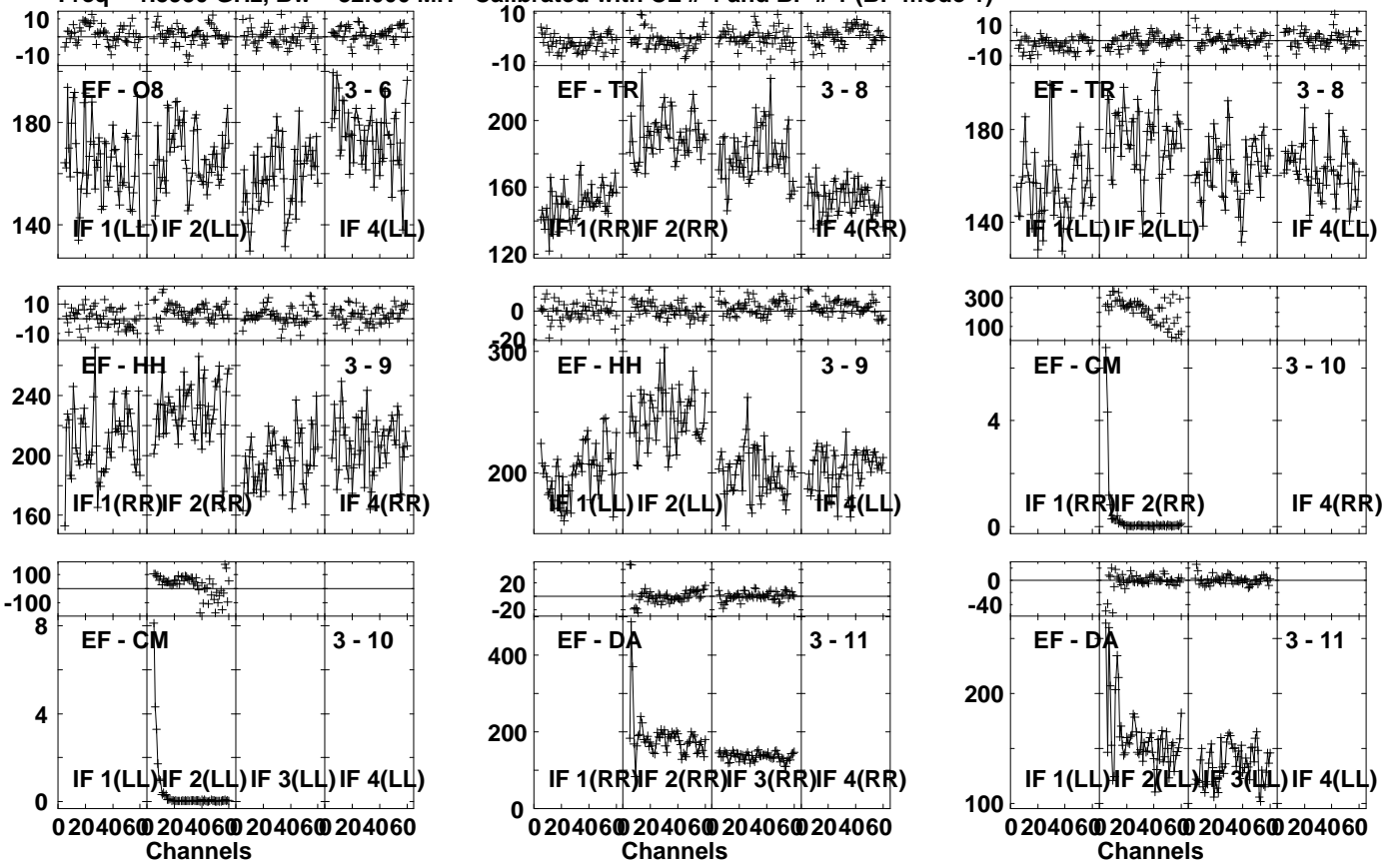
Lower frame: Milli Ampl Jy Top frame: Phas deg Vector averaged cross-power spectrum Several baselines displayed Timerange: 00/02:31:41 to 00/02:32:29
