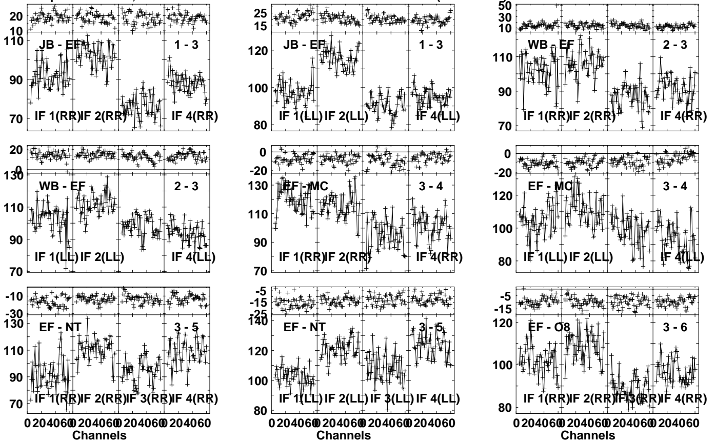
Lower frame: Milli Ampl Jy Top frame: Phas deg Vector averaged cross-power spectrum Several baselines displayed Timerange: 00/02:32:31 to 00/02:35:59
