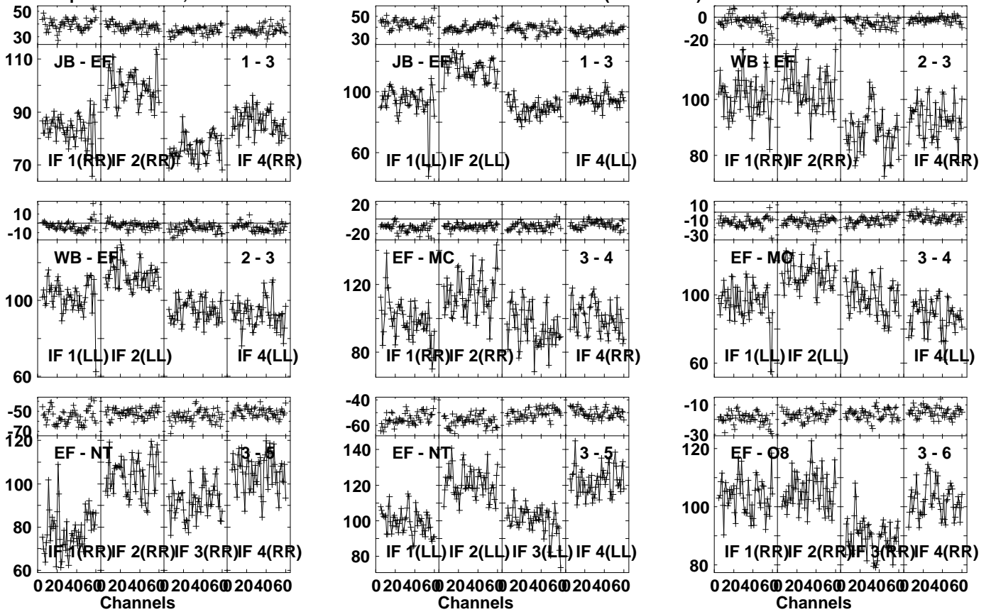
Lower frame: Milli Ampl Jy Top frame: Phas deg Vector averaged cross-power spectrum Several baselines displayed Timerange: 00/03:13:31 to 00/03:16:59
