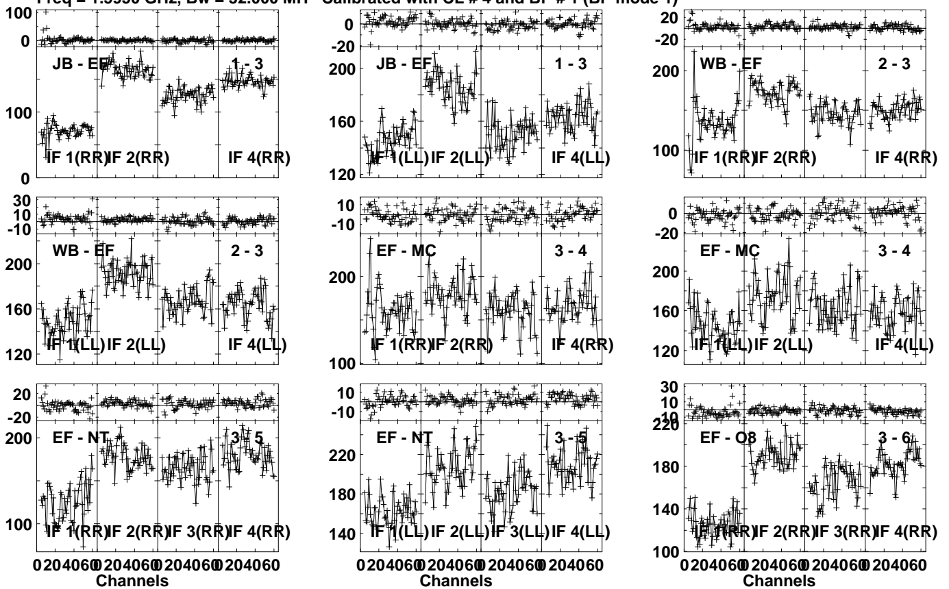
Lower frame: Milli Ampl Jy Top frame: Phas deg Vector averaged cross-power spectrum Several baselines displayed Timerange: 00/01:34:11 to 00/01:34:59
