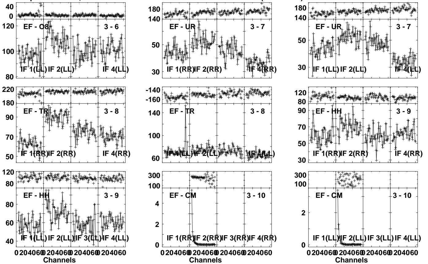
Lower frame: Milli Ampl Jy Top frame: Phas deg Vector averaged cross-power spectrum Several baselines displayed Timerange: 00/01:39:31 to 00/01:42:59
