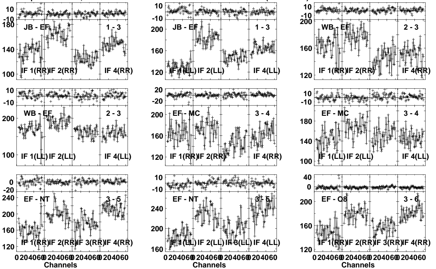
Lower frame: Milli Ampl Jy Top frame: Phas deg Vector averaged cross-power spectrum Several baselines displayed Timerange: 00/00:46:01 to 00/00:46:59
