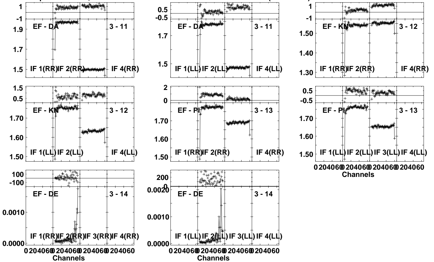
Lower frame: Ampl Jy Top frame: Phas deg Vector averaged cross-power spectrum Several baselines displayed Timerange: 00/03:56:31 to 00/03:59:59
