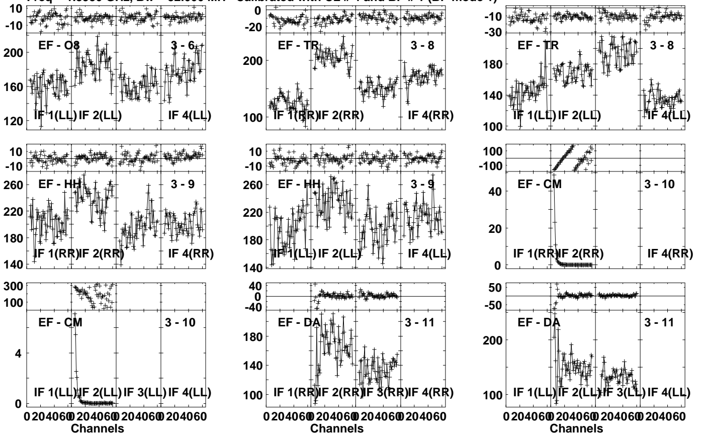
Lower frame: Milli Ampl Jy Top frame: Phas deg Vector averaged cross-power spectrum Several baselines displayed Timerange: 00/02:36:31 to 00/02:37:29
