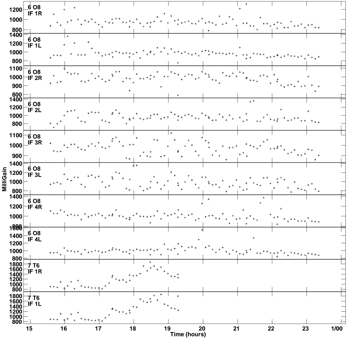
Plot file version 5 created 08-MAY-2023 17:06:14 Gain amp vs UTC time for J1411+2134.MULTI.1 SN 2 Rpol & Lpol IF 1 - 4
