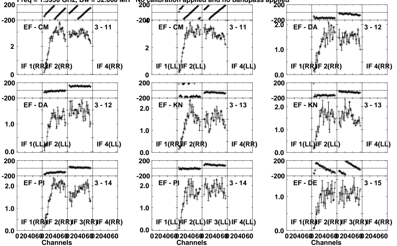
Lower frame: Milli Ampl Jy Top frame: Phas deg Vector averaged cross-power spectrum Several baselines displayed Timerange: 00/16:16:01 to 00/16:17:29
