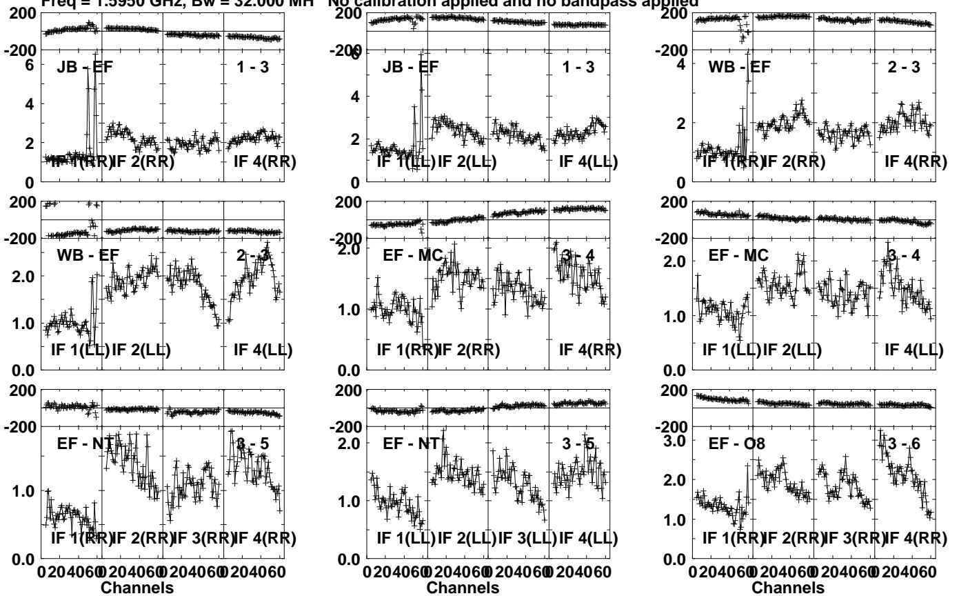
Lower frame: Milli Ampl Jy Top frame: Phas deg Vector averaged cross-power spectrum Several baselines displayed Timerange: 00/15:58:41 to 00/15:59:29
