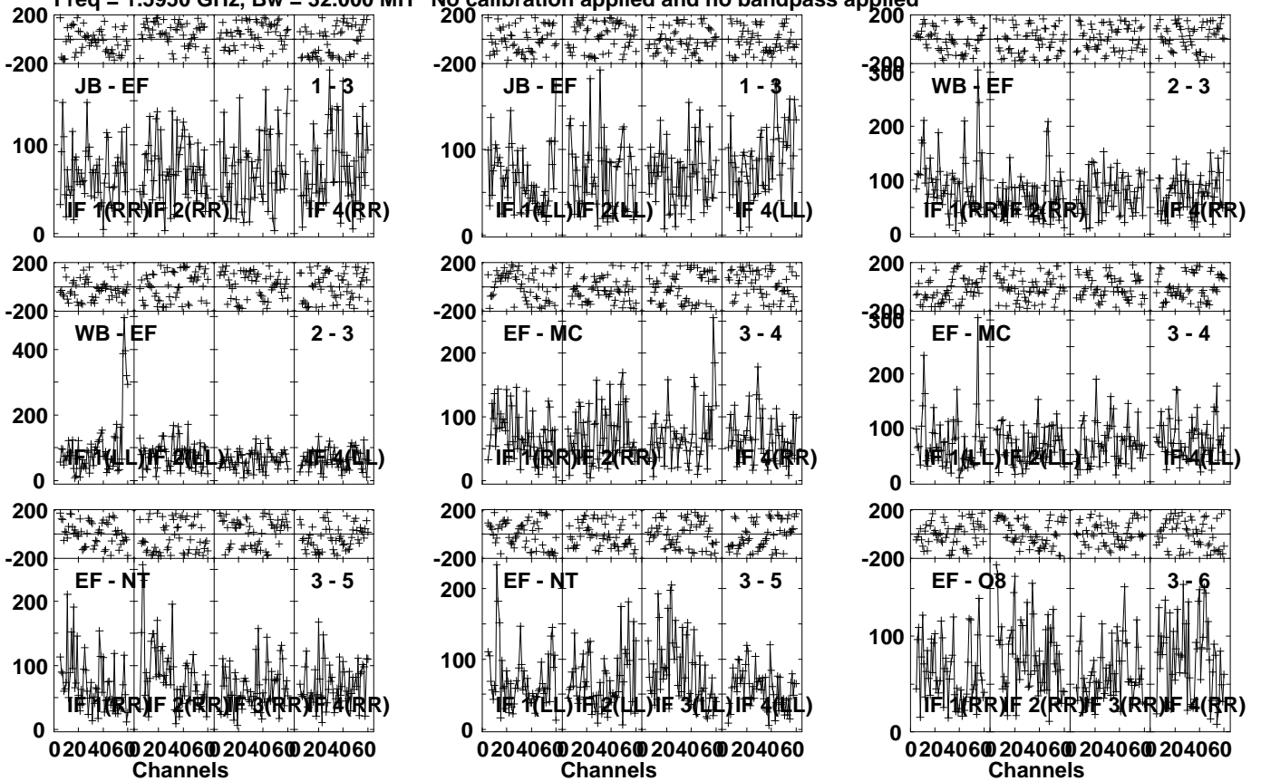
Lower frame: Micro Ampl Jy Top frame: Phas deg Vector averaged cross-power spectrum Several baselines displayed Timerange: 00/17:35:31 to 00/17:39:59
